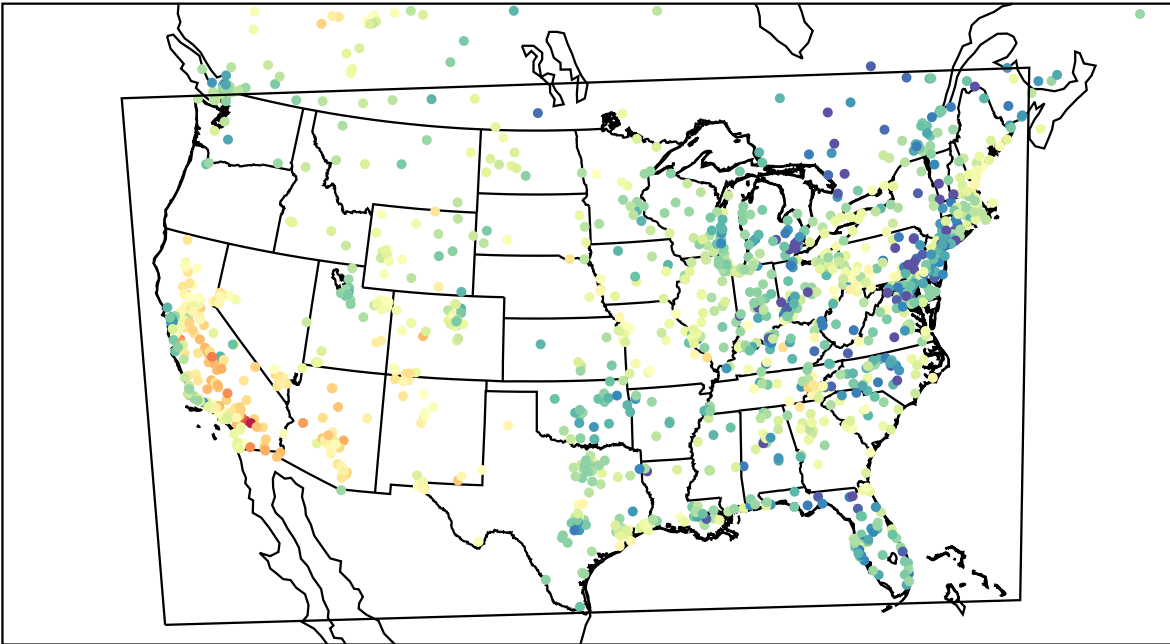
AirNOW (2023-04-26_01:00:00)
