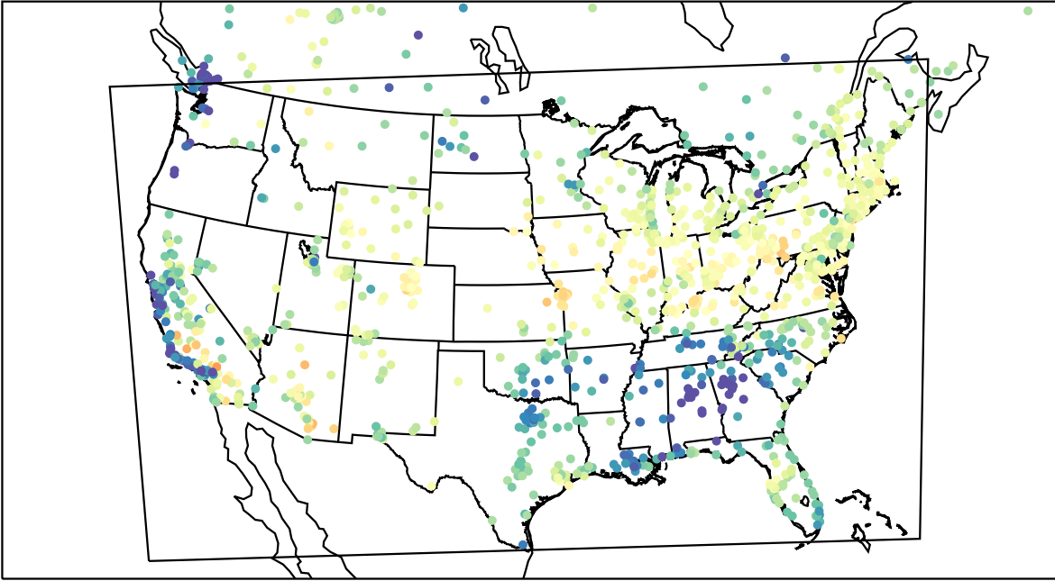
AirNOW (2023-04-27_16:00:00)
