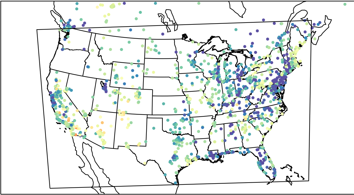
AirNOW (2023-04-26_04:00:00)
