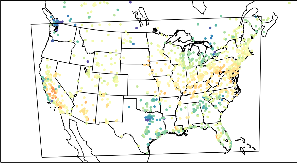
AirNOW (2023-04-26_19:00:00)
