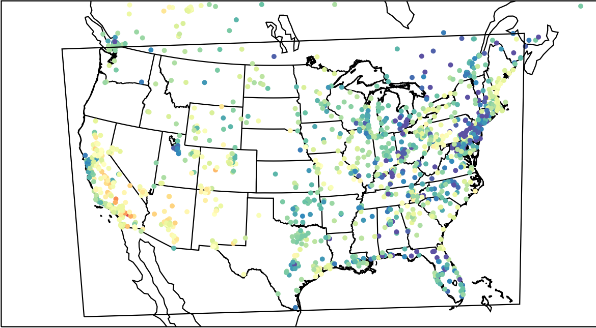
AirNOW (2023-04-26_02:00:00)
