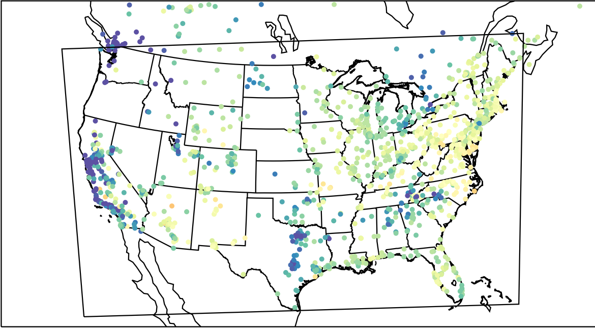
AirNOW (2023-04-26_15:00:00)
