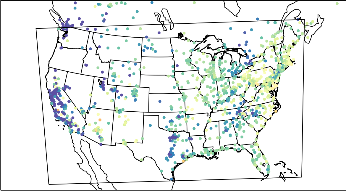
AirNOW (2023-04-26_14:00:00)
