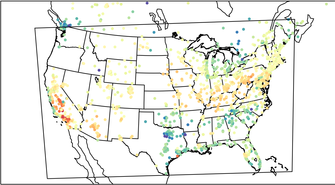
AirNOW (2023-04-26_21:00:00)
