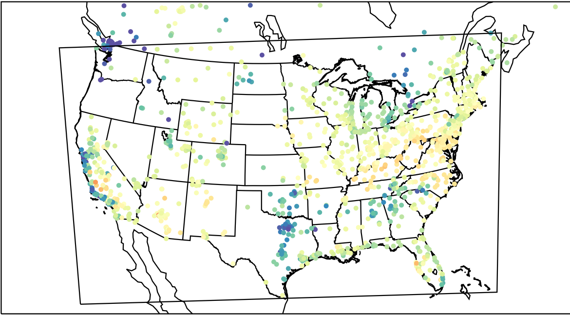
AirNOW (2023-04-26_17:00:00)
