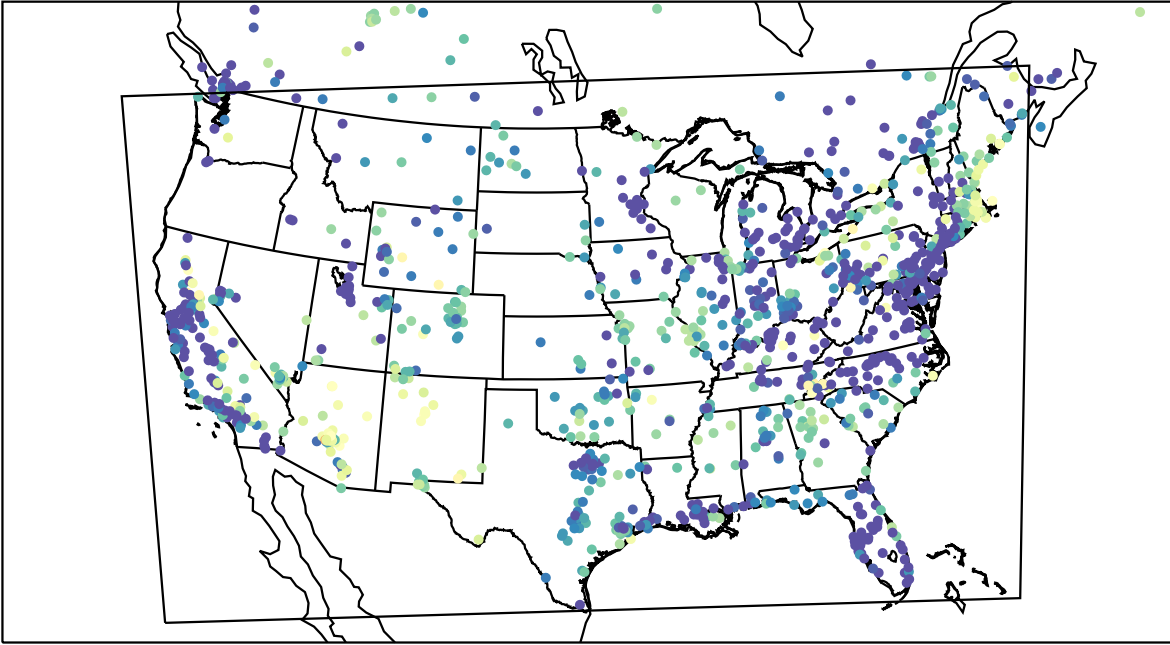
AirNOW (2023-04-26_10:00:00)
