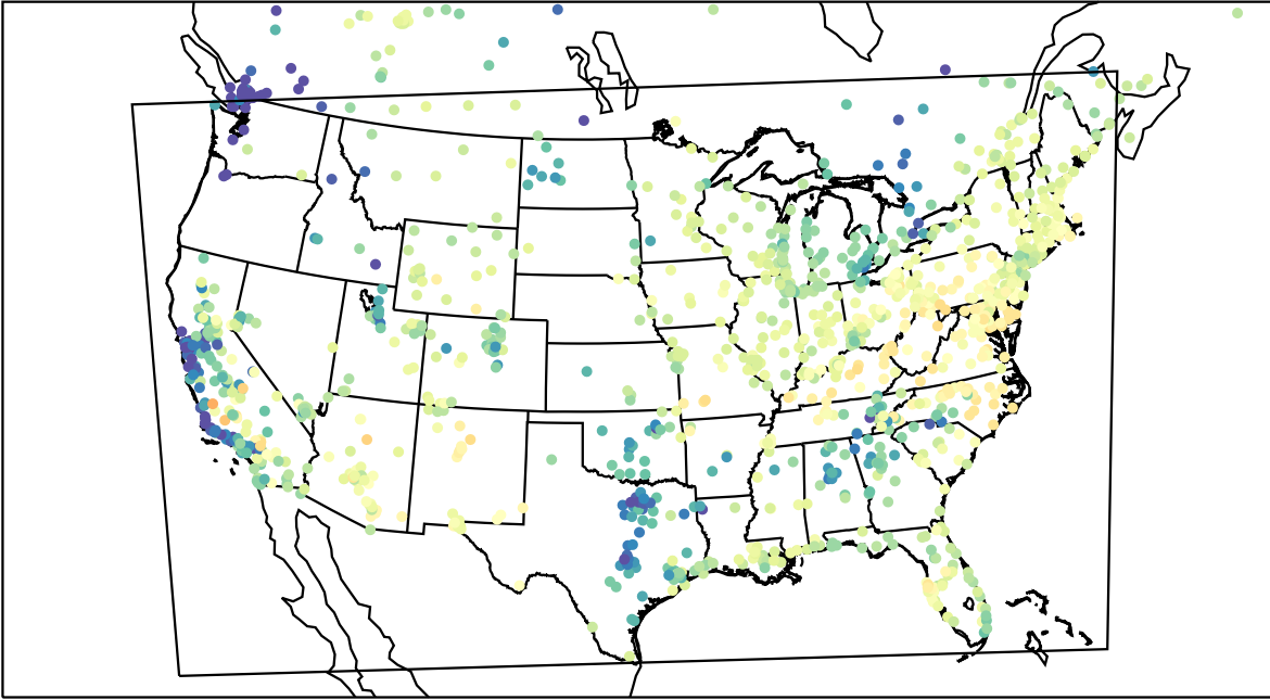
AirNOW (2023-04-26_16:00:00)
