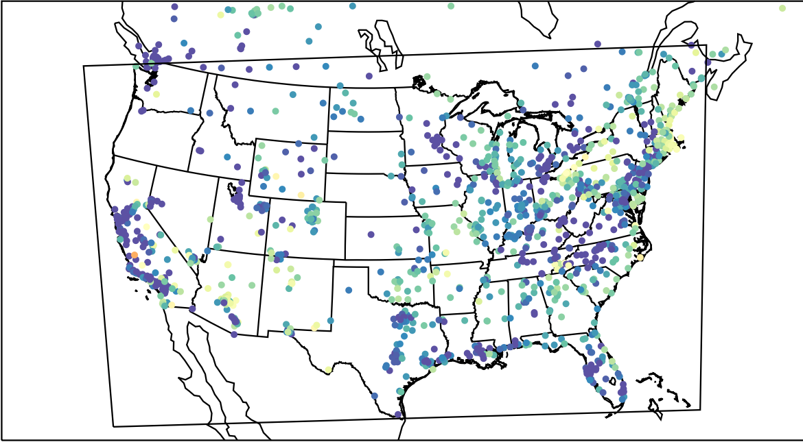
AirNOW (2023-04-26_12:00:00)
