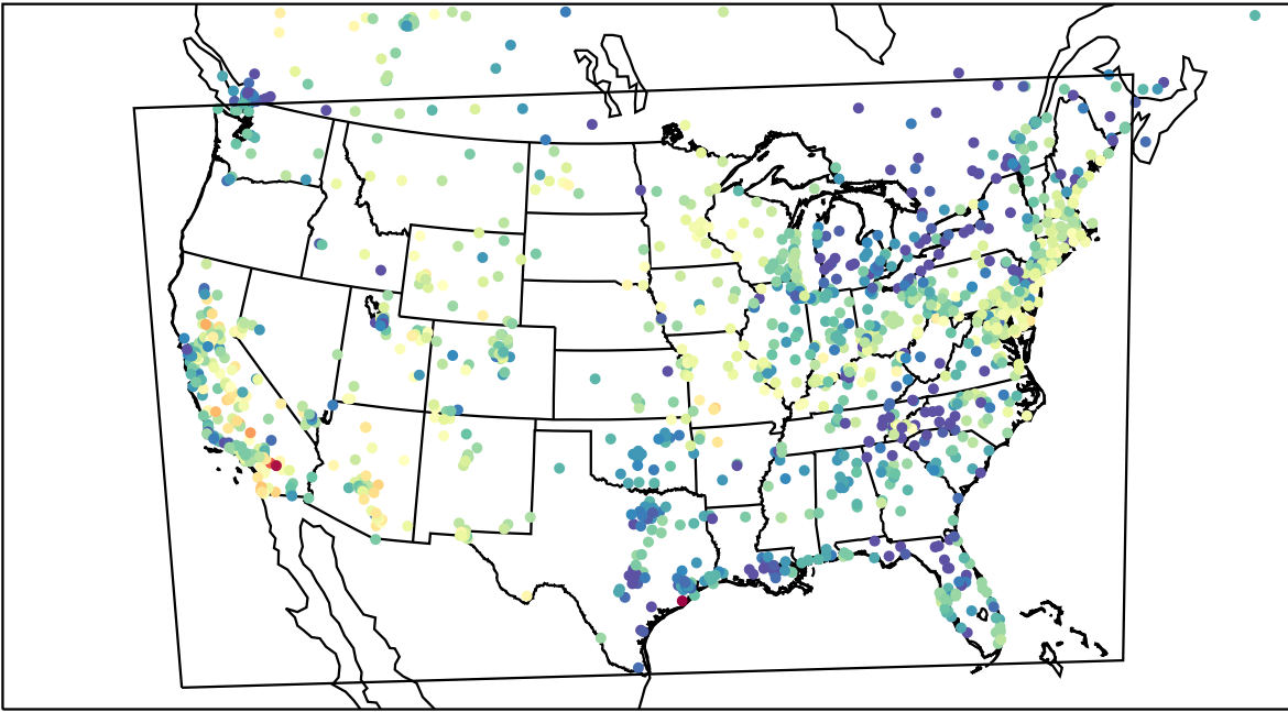
AirNOW (2023-04-27_03:00:00)
