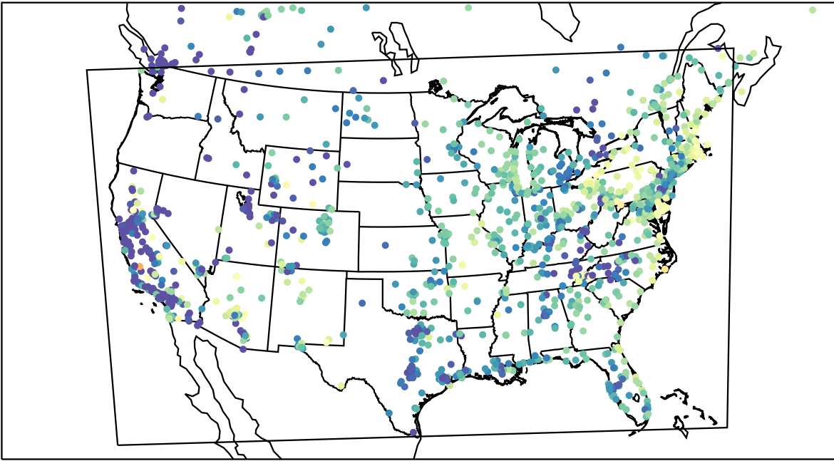
AirNOW (2023-04-26_13:00:00)
