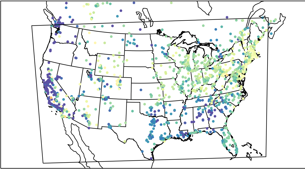
AirNOW (2023-04-27_14:00:00)
