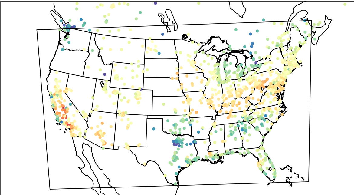
AirNOW (2023-04-26_20:00:00)
