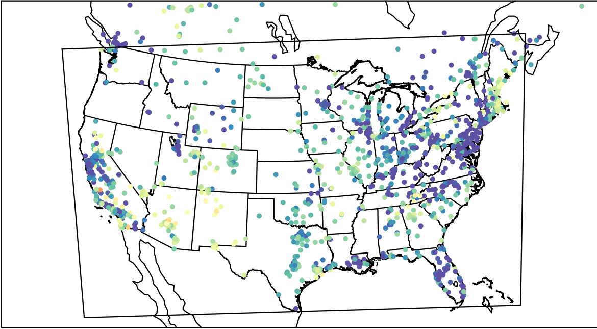
AirNOW (2023-04-26_07:00:00)
