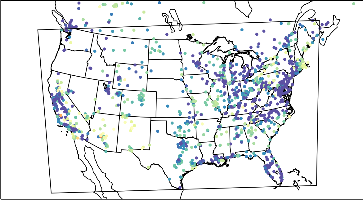
AirNOW (2023-04-26_09:00:00)
