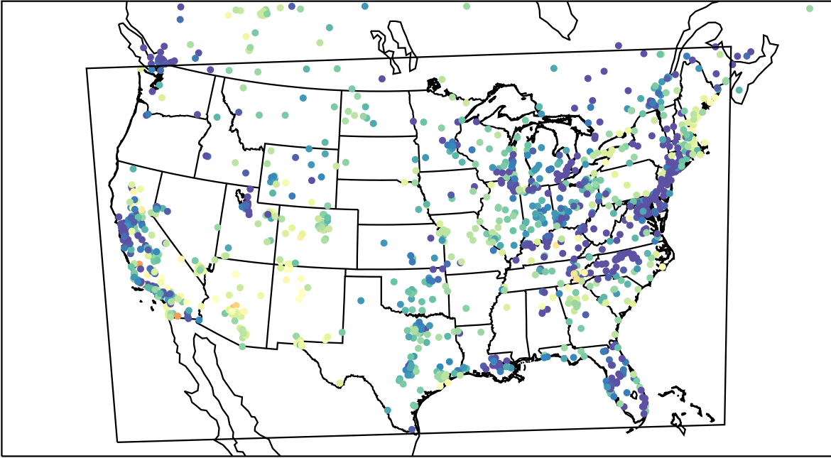
AirNOW (2023-04-26_06:00:00)
