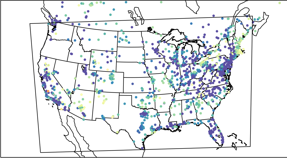
AirNOW (2023-04-26_11:00:00)
