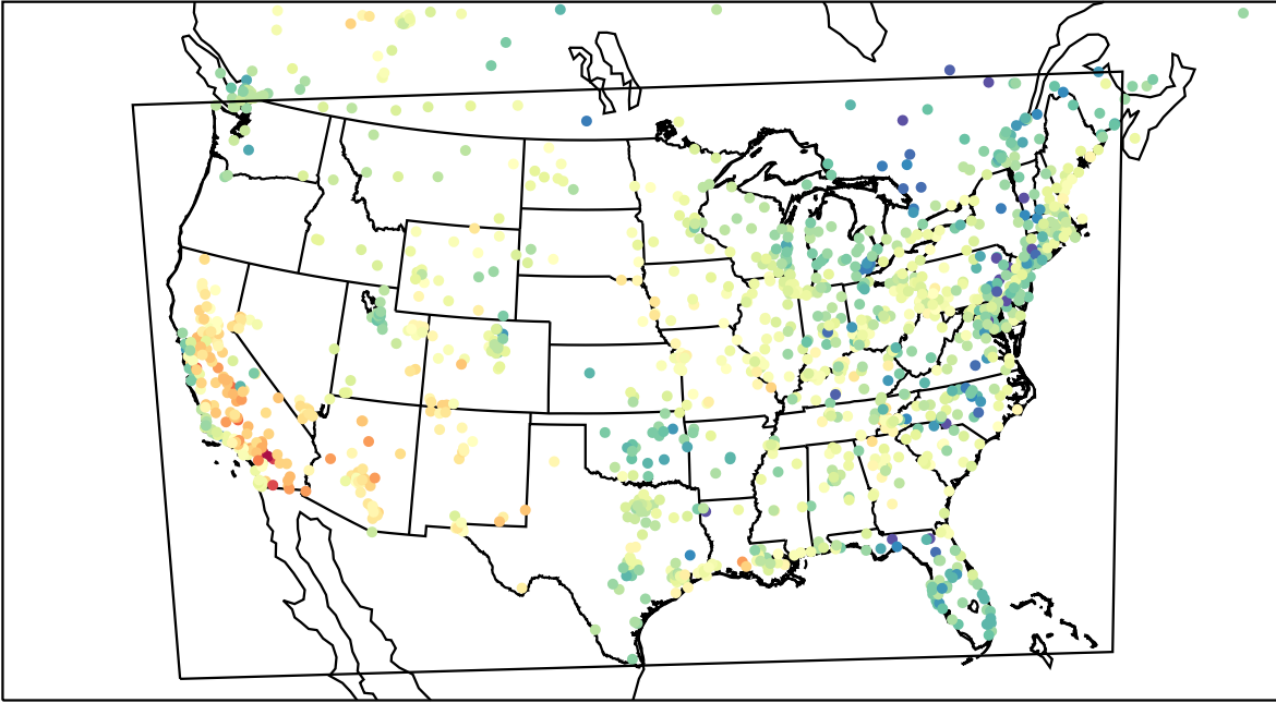
AirNOW (2023-04-26_00:00:00)
