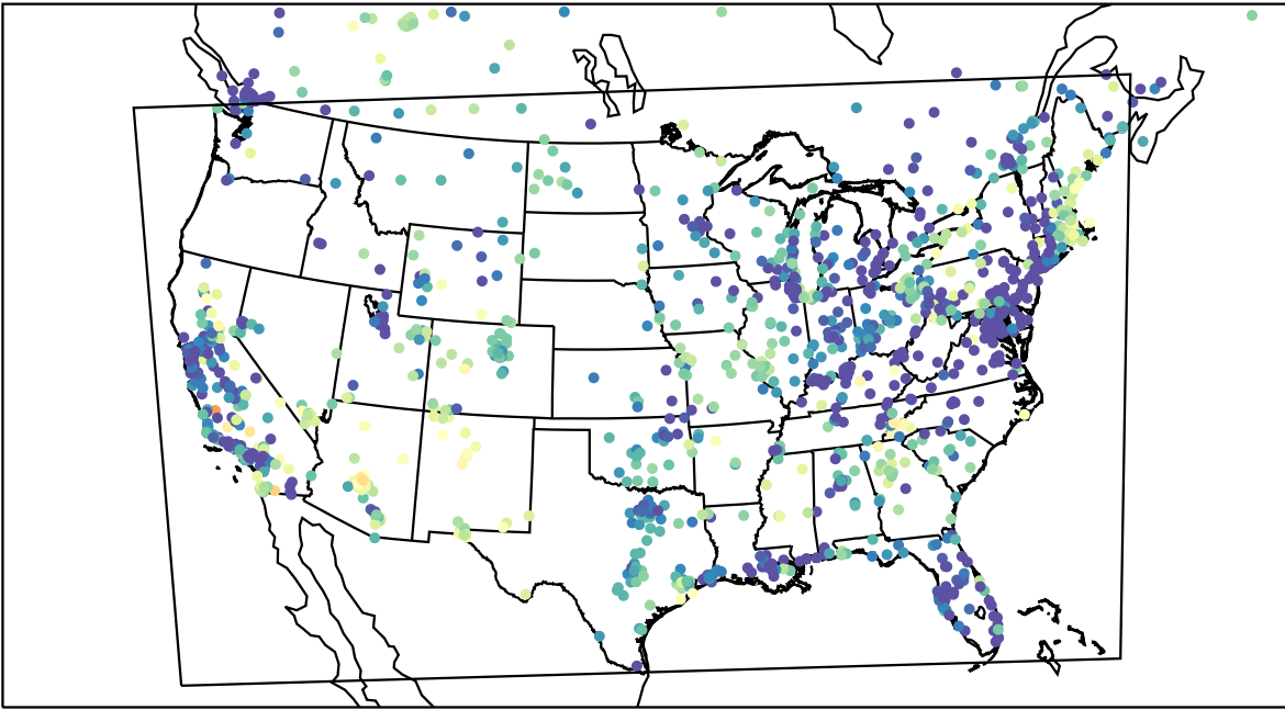
AirNOW (2023-04-26_08:00:00)
