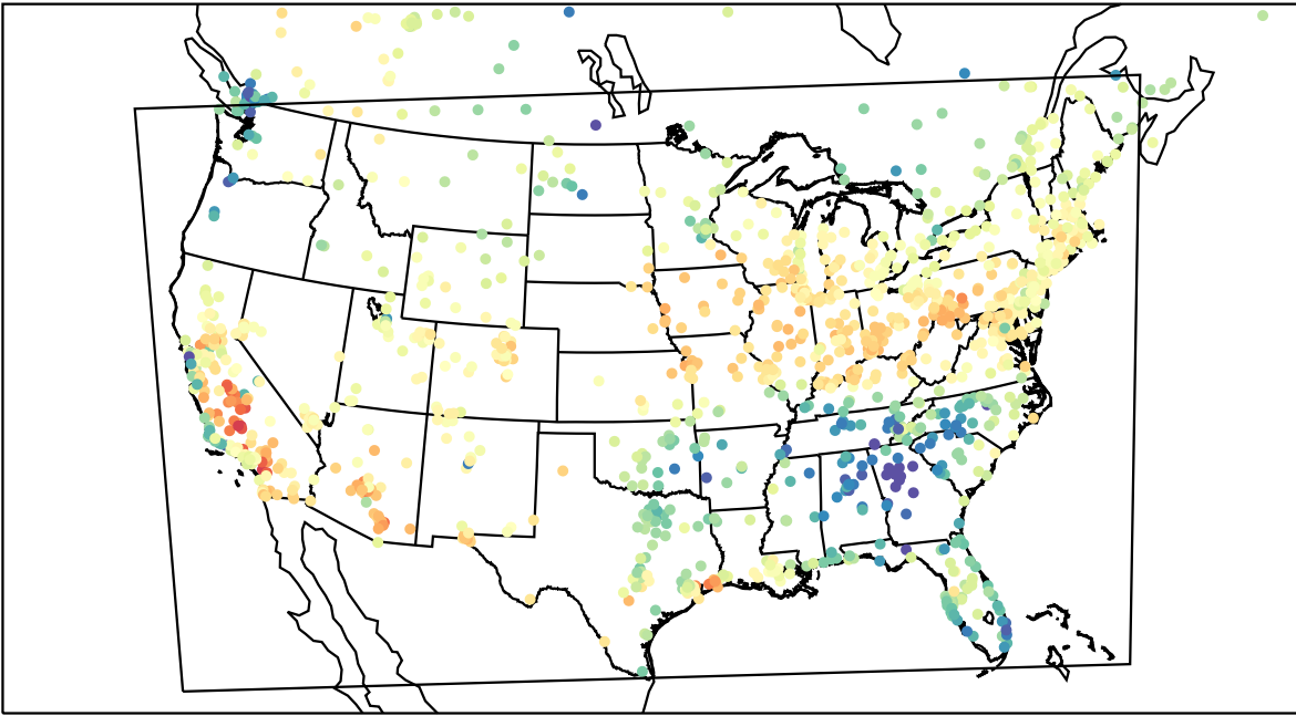
AirNOW (2023-04-27_19:00:00)
