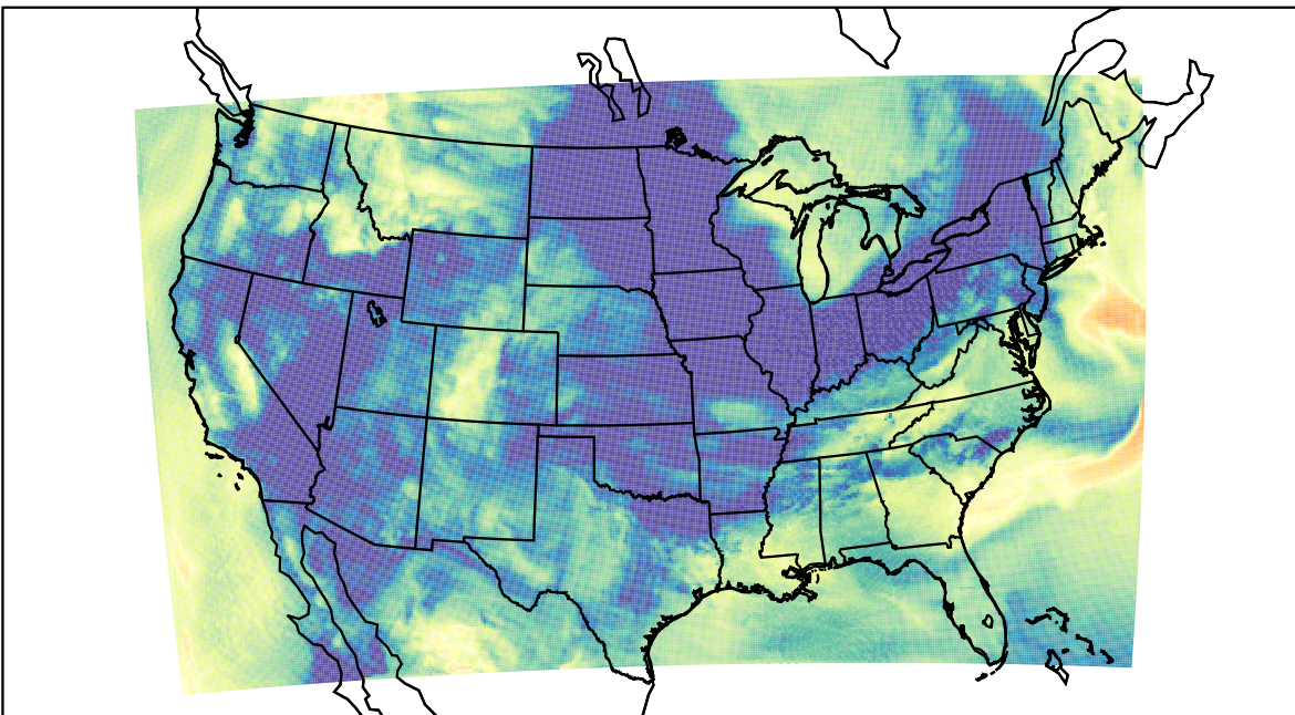
WRF (2023-04-26_15:00:00)
