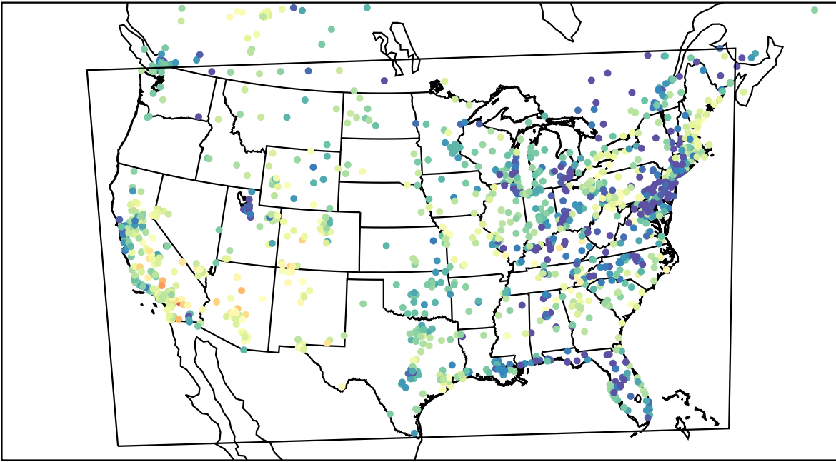
AirNOW (2023-04-26_03:00:00)
