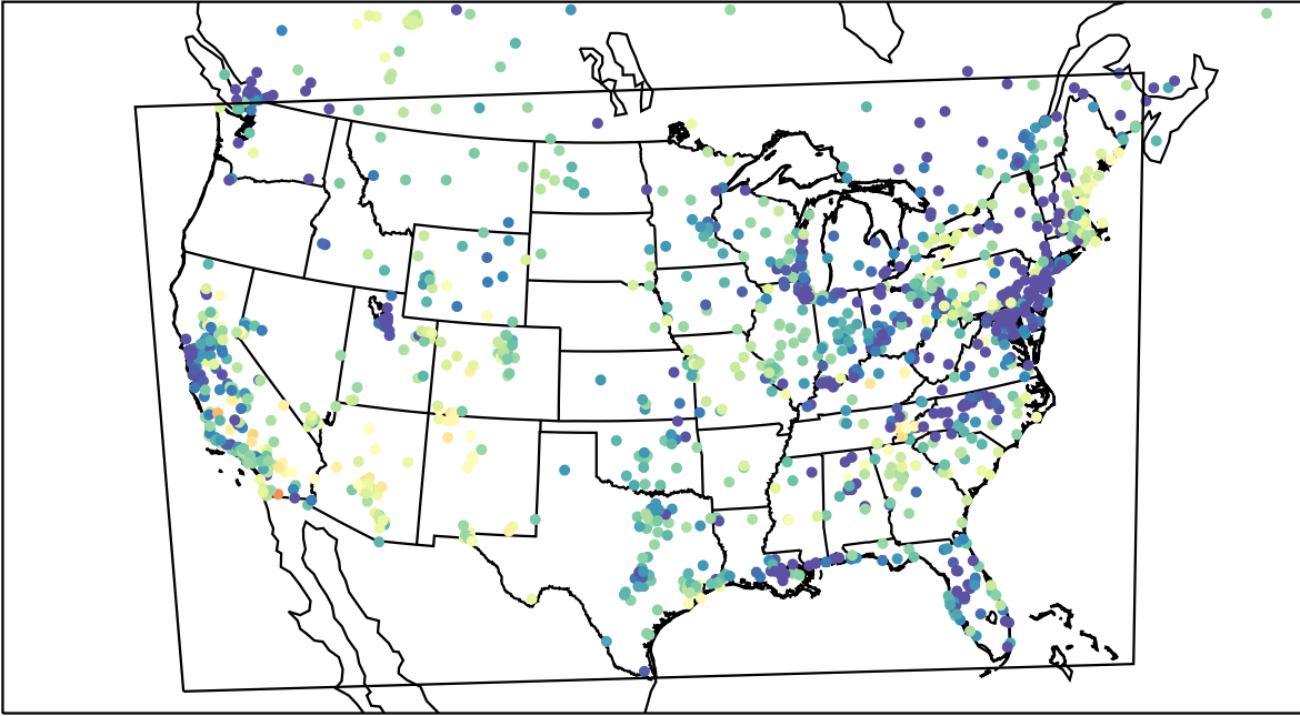
AirNOW (2023-04-26_05:00:00)
