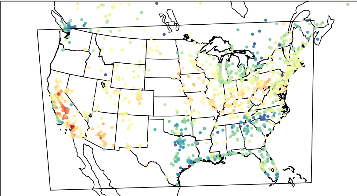
AirNOW (2023-04-26_23:00:00)
