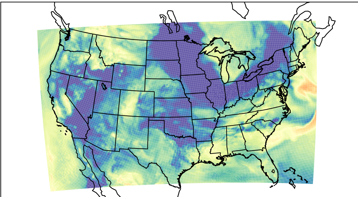
WRF (2023-04-26_16:00:00)
