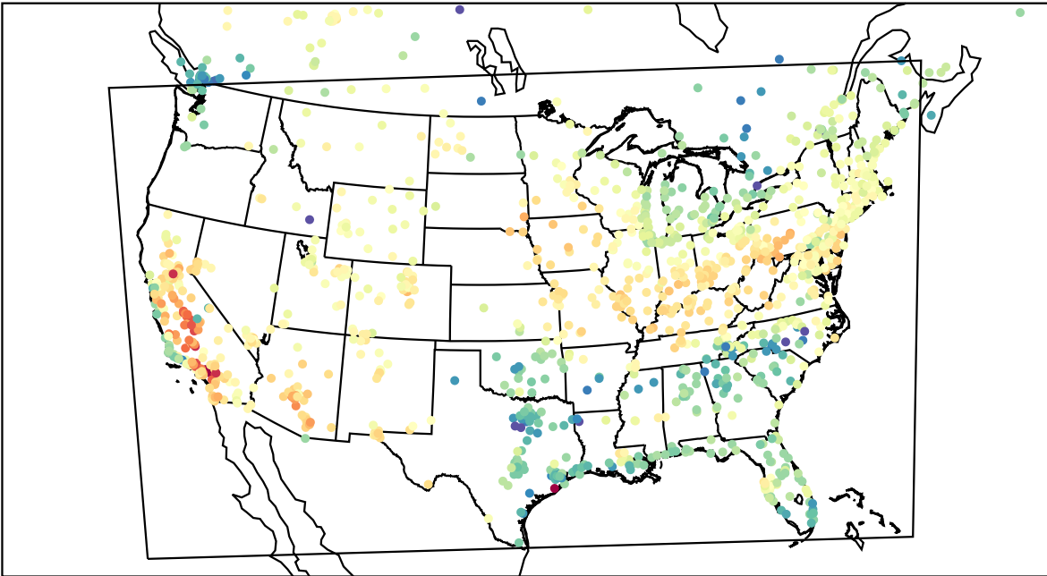
AirNOW (2023-04-26_22:00:00)
