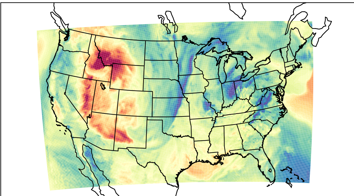
WRF (2023-04-28_17:00:00)
