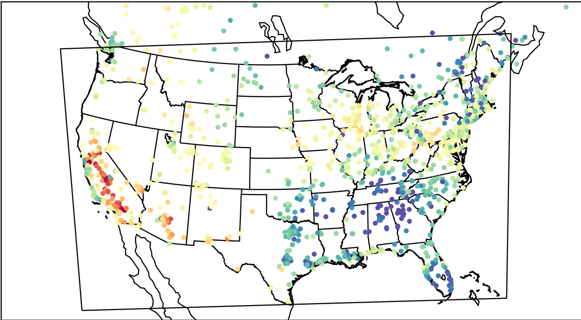
AirNOW (2023-04-28_01:00:00)
