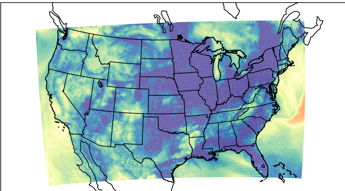
WRF (2023-04-27_10:00:00)
