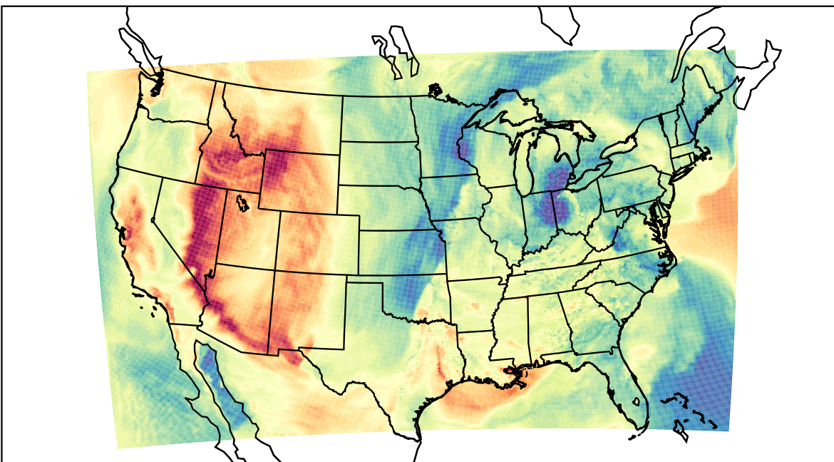
WRF (2023-04-28_23:00:00)
