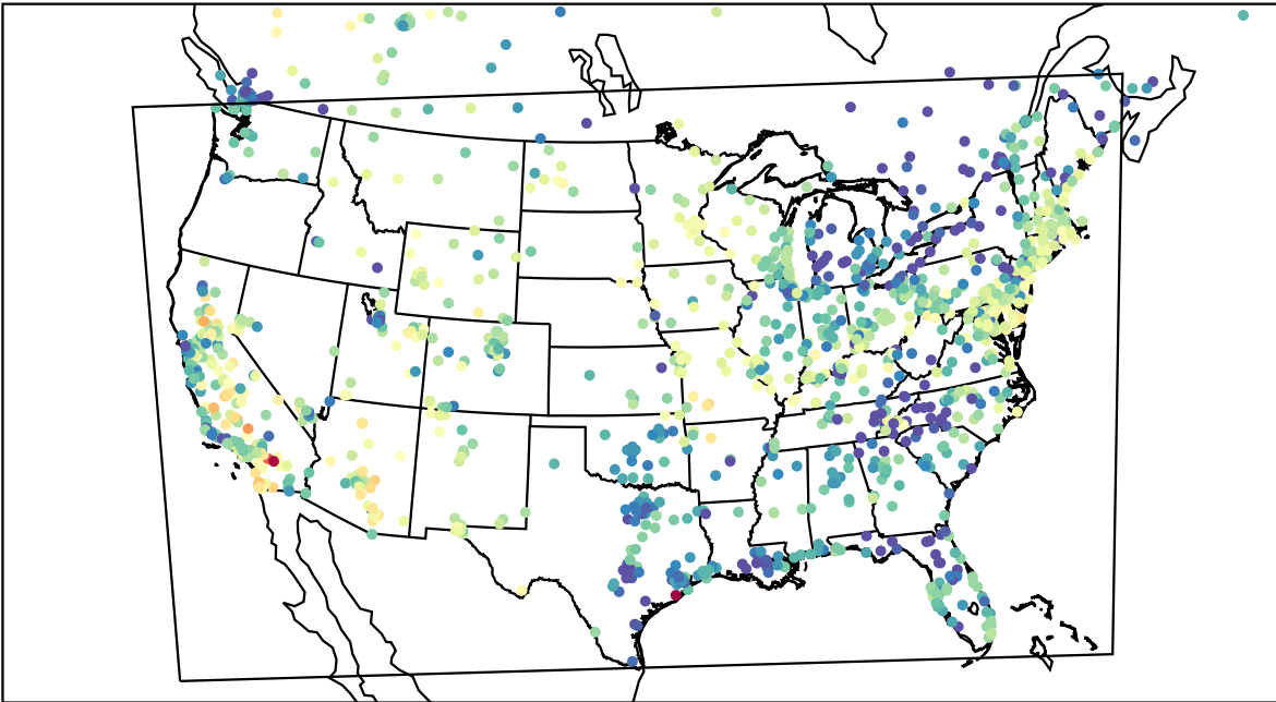
AirNOW (2023-04-27_03:00:00)
