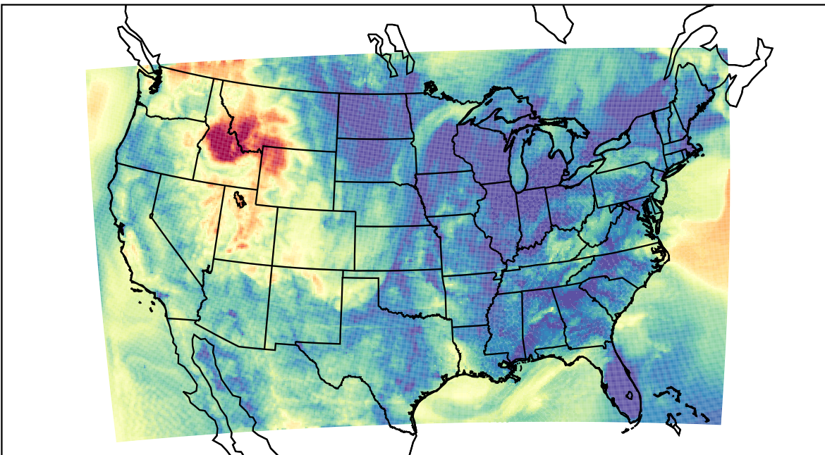
WRF (2023-04-28_12:00:00)
