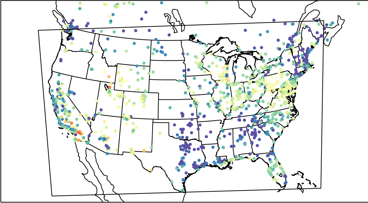
AirNOW (2023-04-28_05:00:00)
