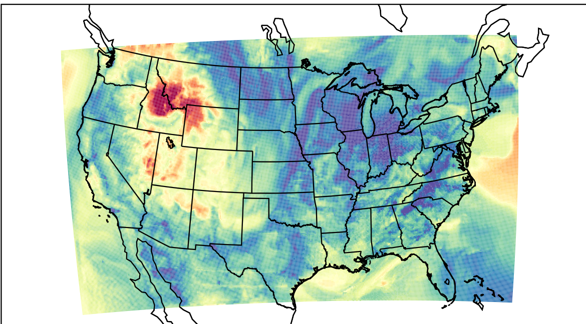
WRF (2023-04-28_14:00:00)
