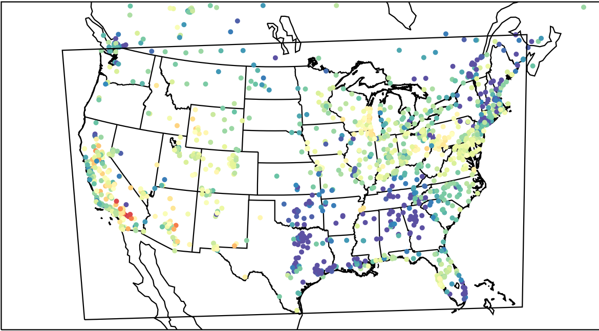
AirNOW (2023-04-28_03:00:00)
