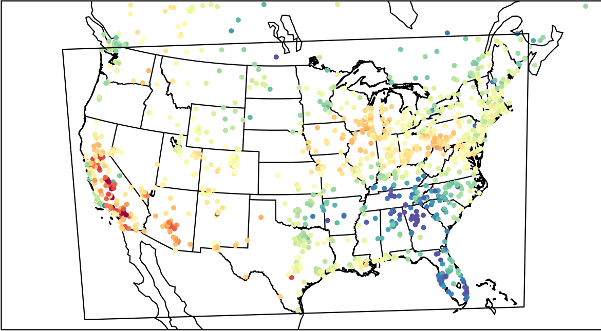
AirNOW (2023-04-27_23:00:00)
