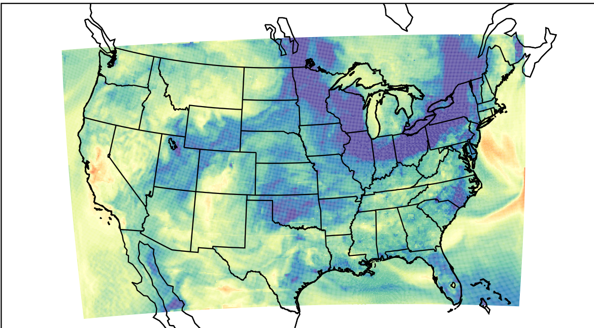
WRF (2023-04-27_01:00:00)
