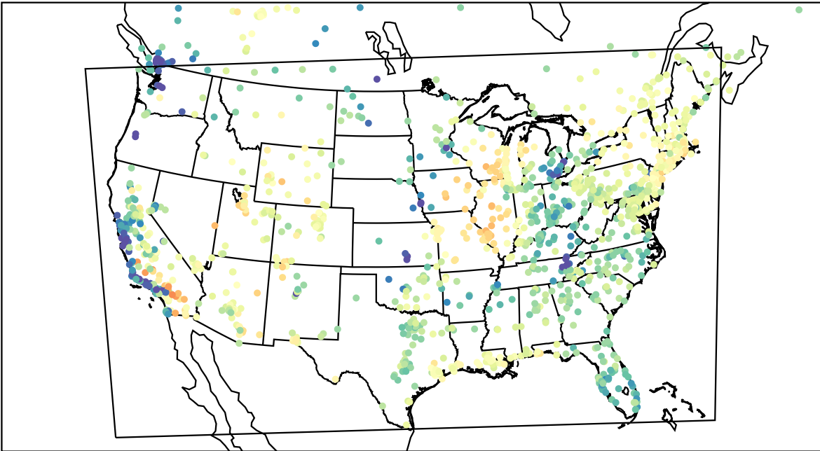
AirNOW (2023-04-28_16:00:00)
