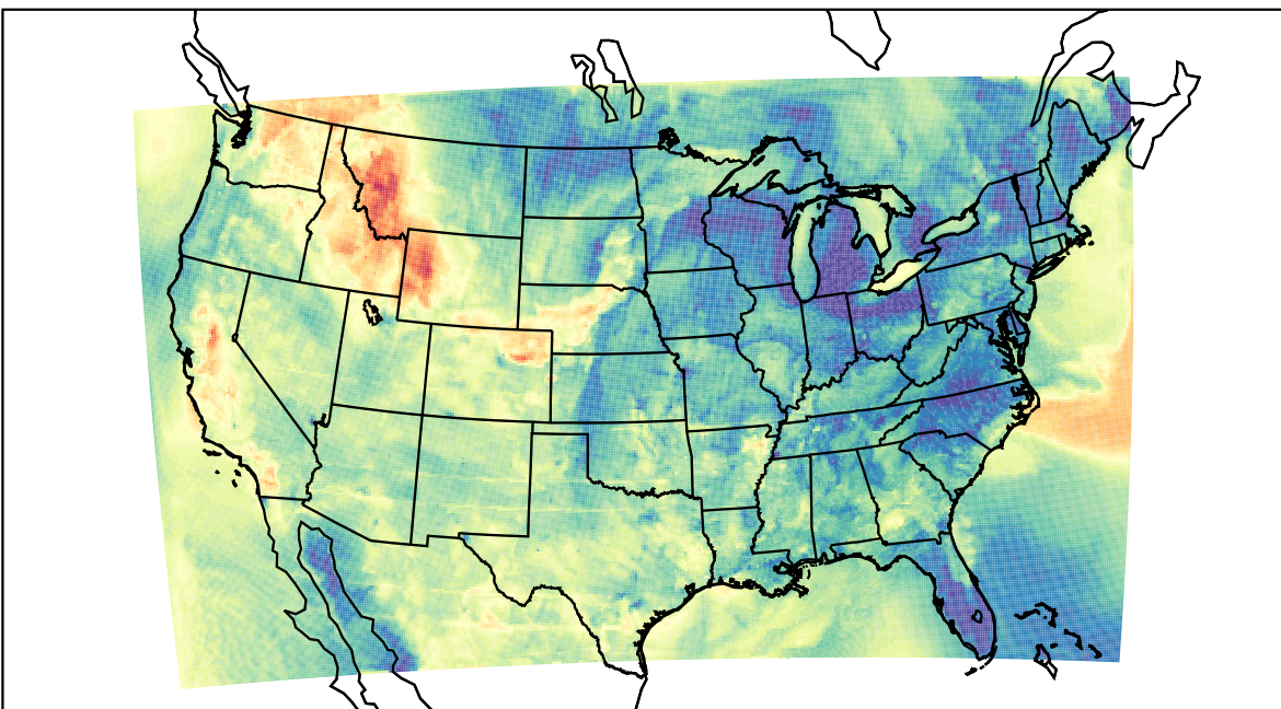
WRF (2023-04-28_02:00:00)
