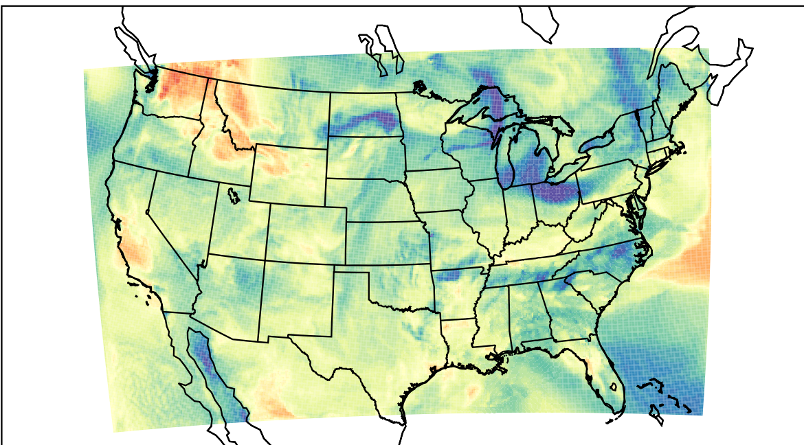
WRF (2023-04-27_19:00:00)
