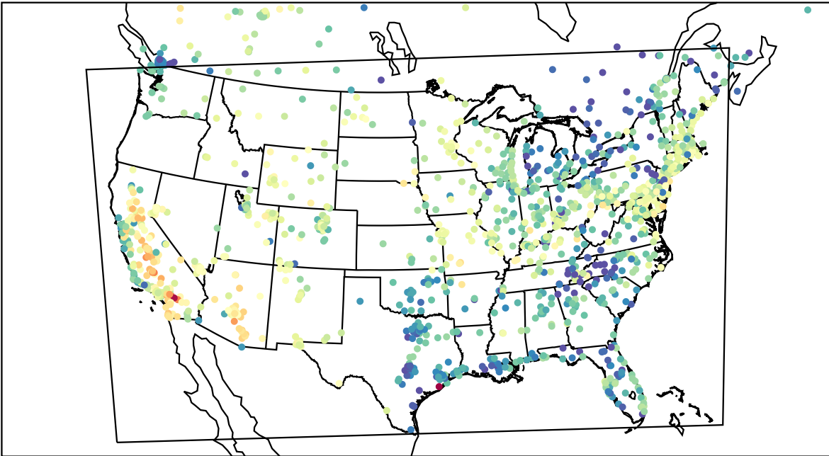
AirNOW (2023-04-27_02:00:00)
