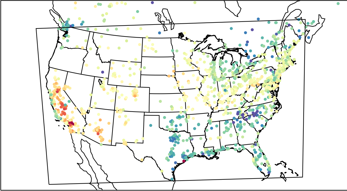
AirNOW (2023-04-27_00:00:00)
