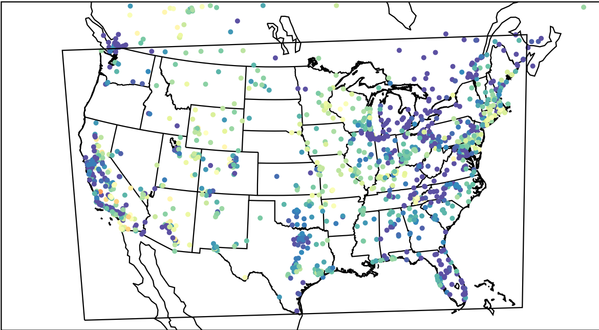
AirNOW (2023-04-27_07:00:00)
