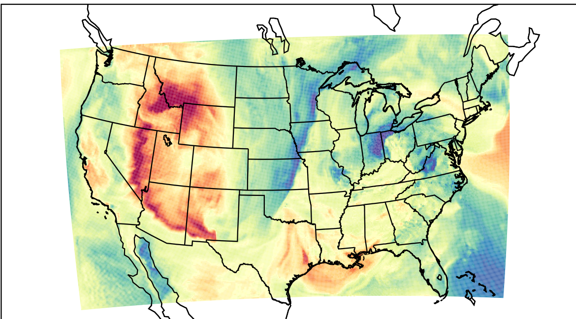
WRF (2023-04-28_19:00:00)
