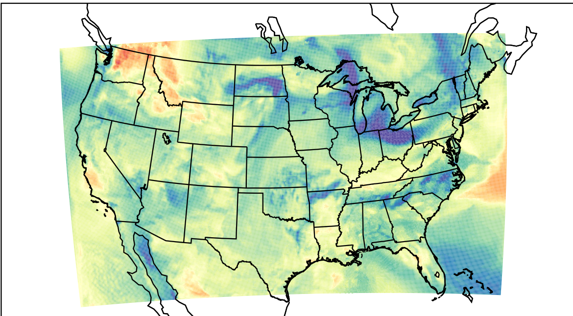
WRF (2023-04-27_18:00:00)
