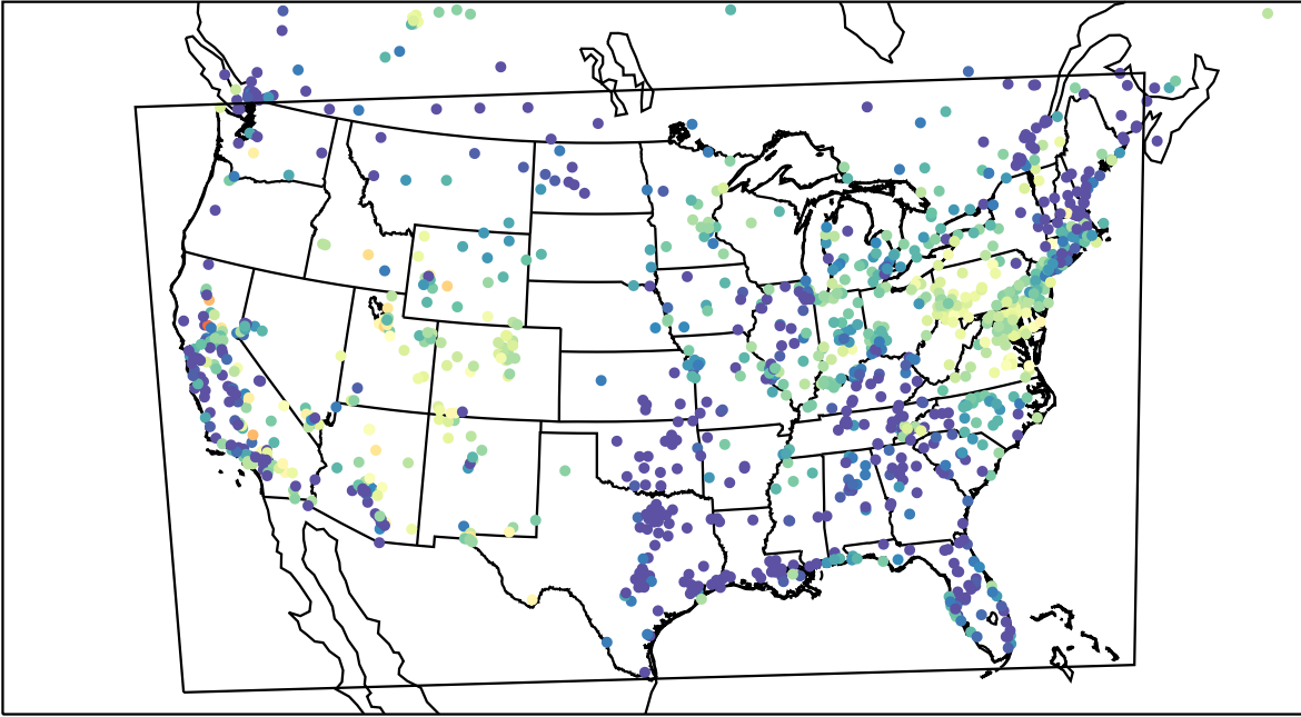
AirNOW (2023-04-28_10:00:00)
