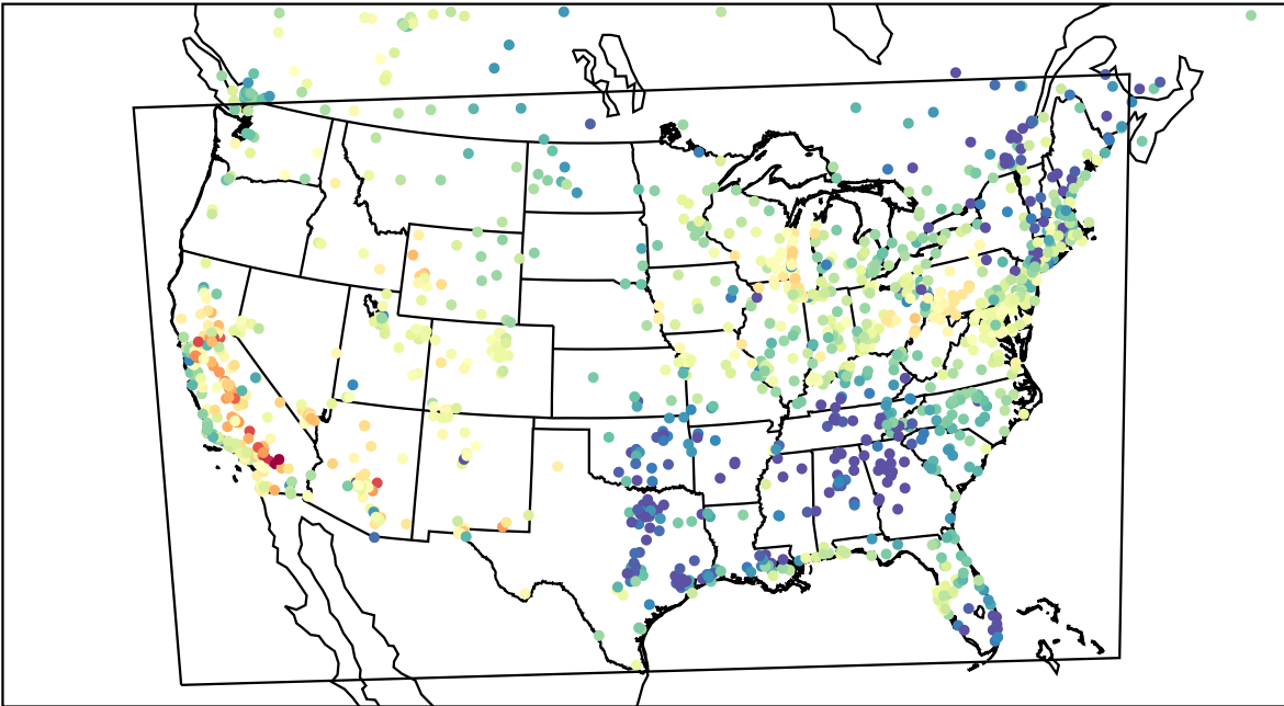
AirNOW (2023-04-28_02:00:00)
