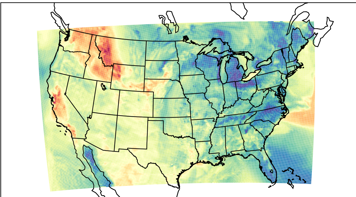
WRF (2023-04-28_00:00:00)
