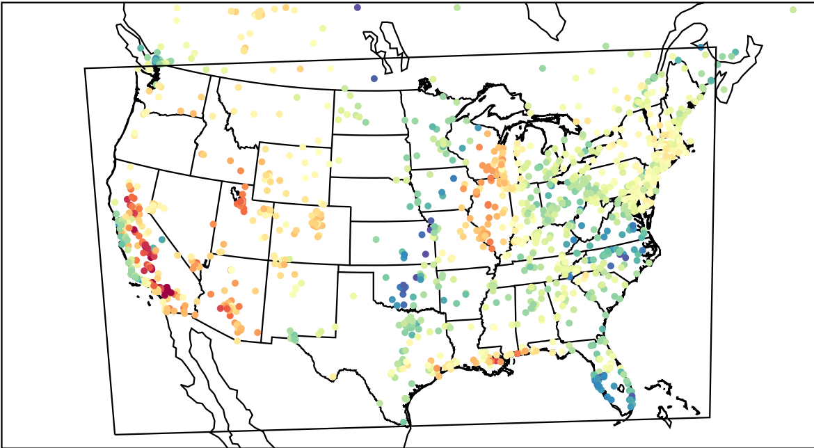
AirNOW (2023-04-28_23:00:00)
