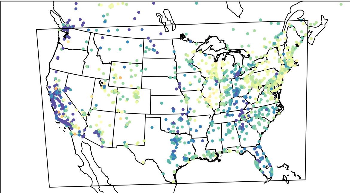
AirNOW (2023-04-28_14:00:00)
