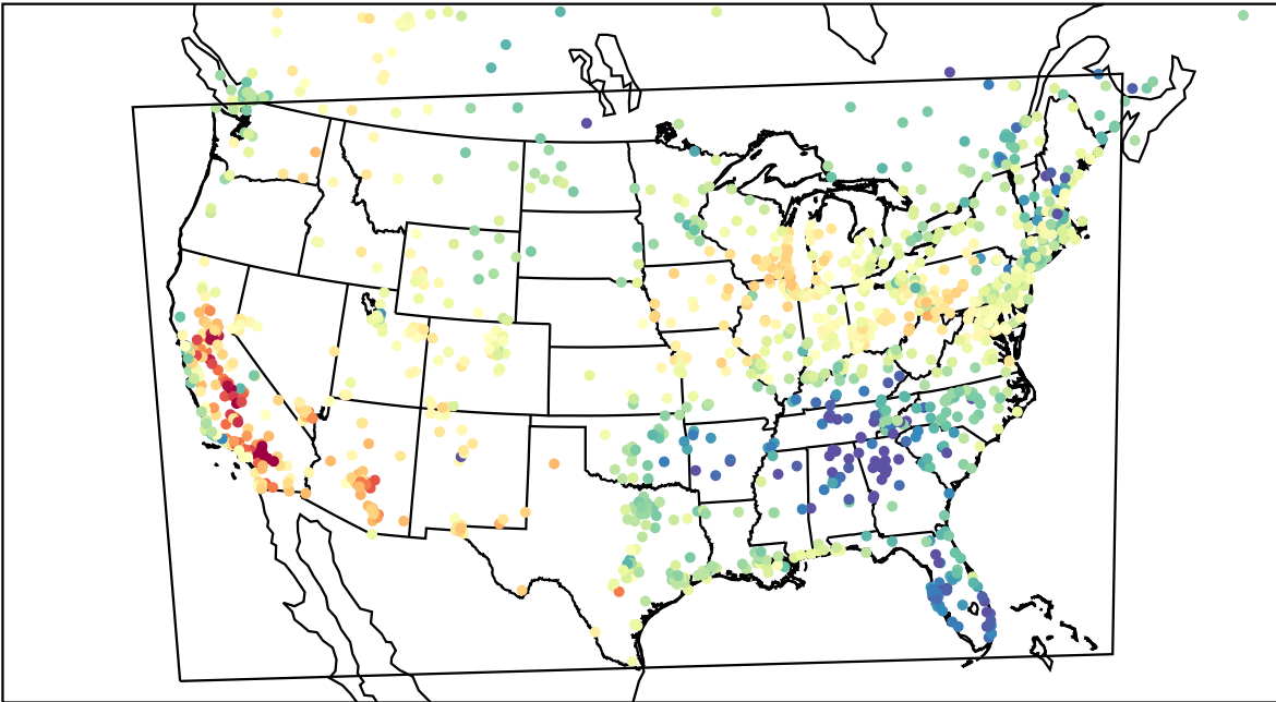
AirNOW (2023-04-28_00:00:00)
