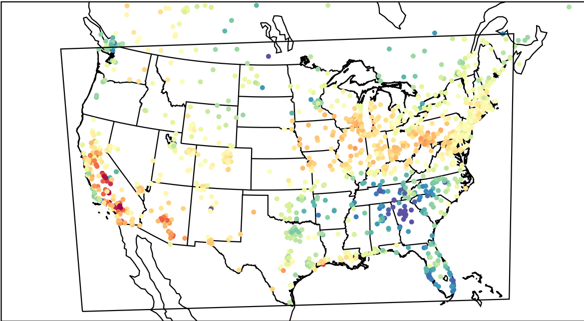
AirNOW (2023-04-27_21:00:00)
