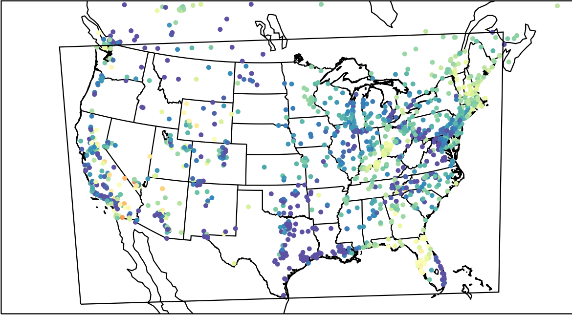
AirNOW (2023-04-30_11:00:00)
