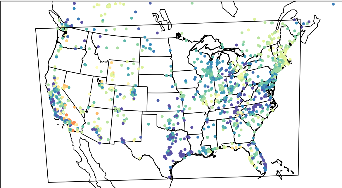
AirNOW (2023-04-30_06:00:00)
