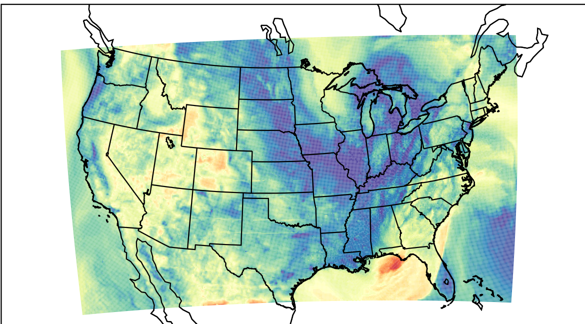
WRF (2023-04-30_11:00:00)
