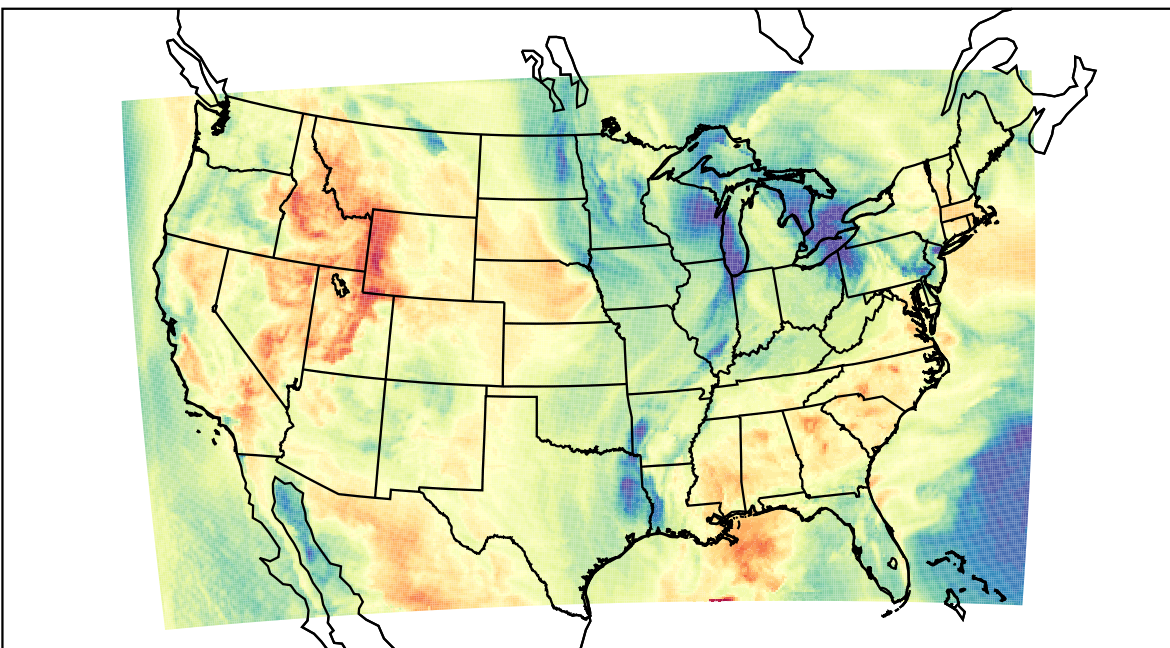
WRF (2023-04-29_18:00:00)
