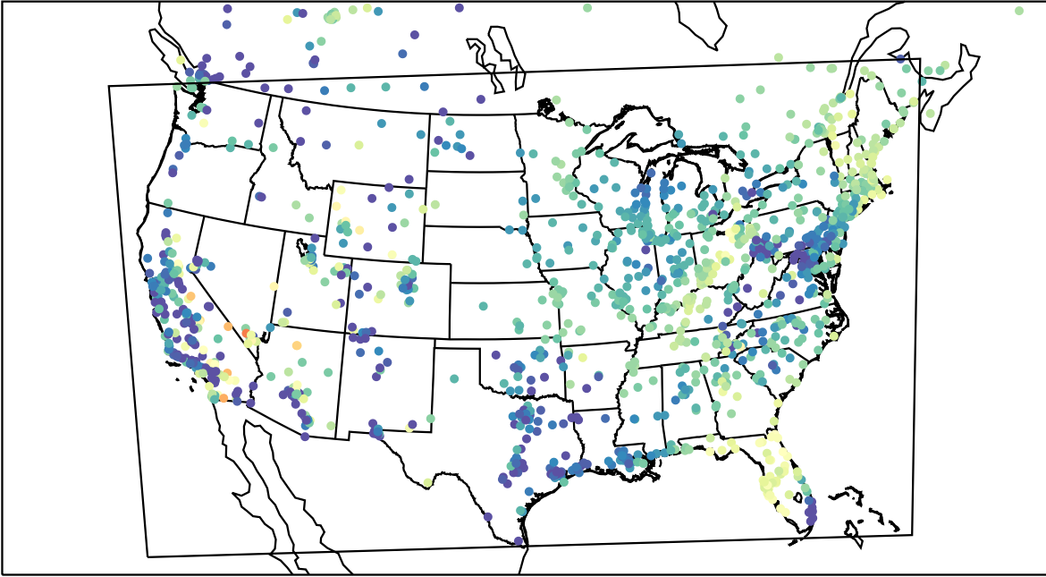
AirNOW (2023-04-30_13:00:00)
