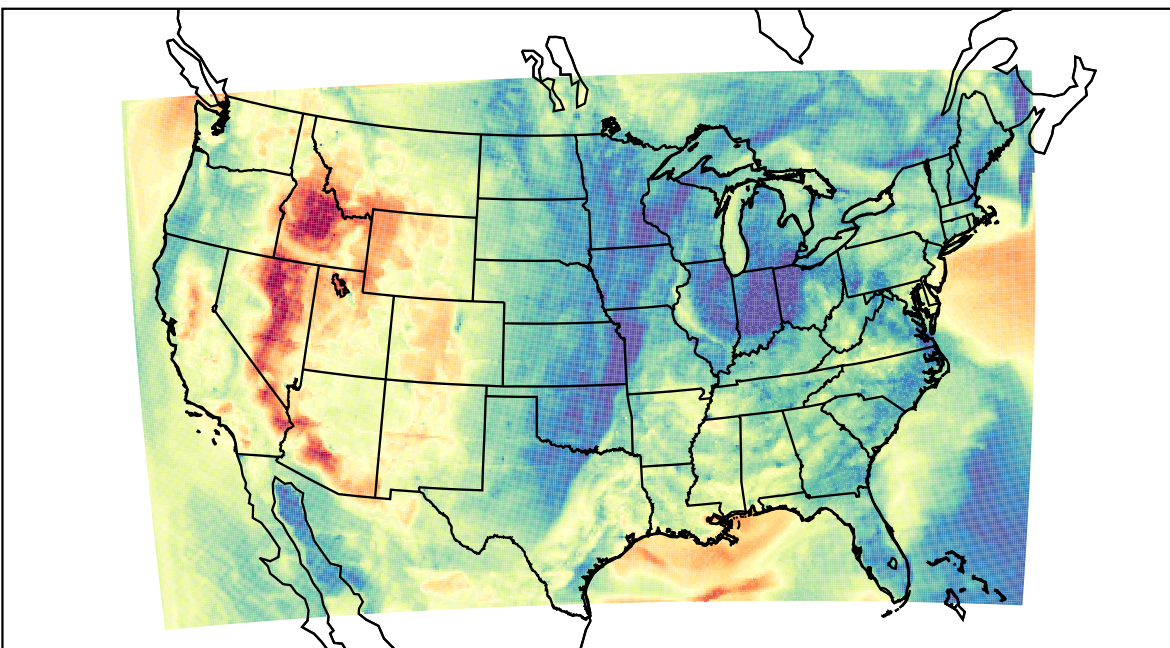
WRF (2023-04-29_02:00:00)
