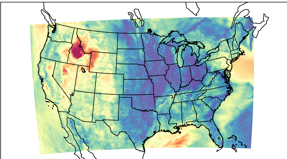
WRF (2023-04-29_09:00:00)
