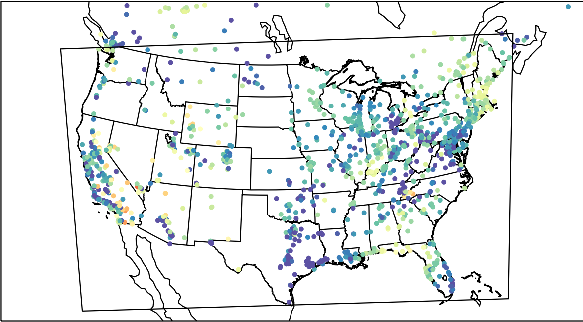
AirNOW (2023-04-30_08:00:00)
