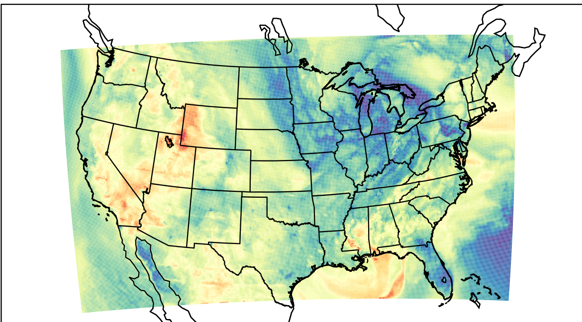
WRF (2023-04-30_02:00:00)
