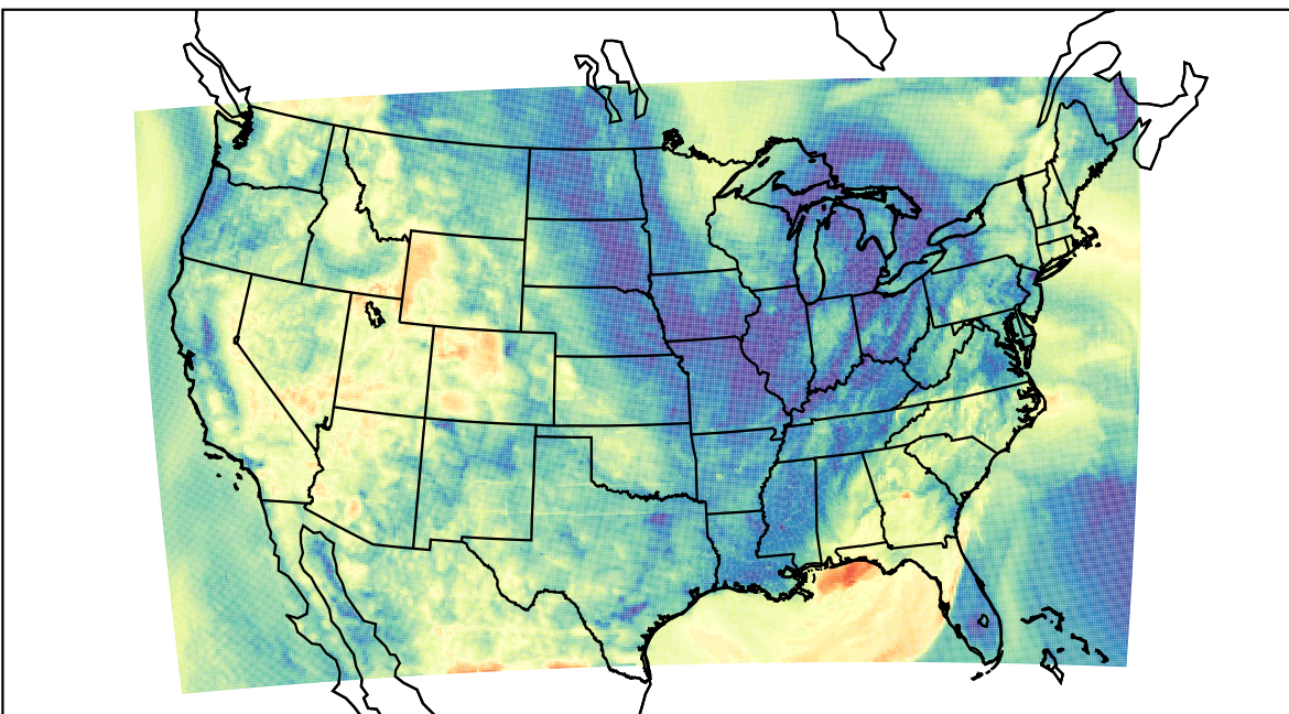
WRF (2023-04-30_09:00:00)
