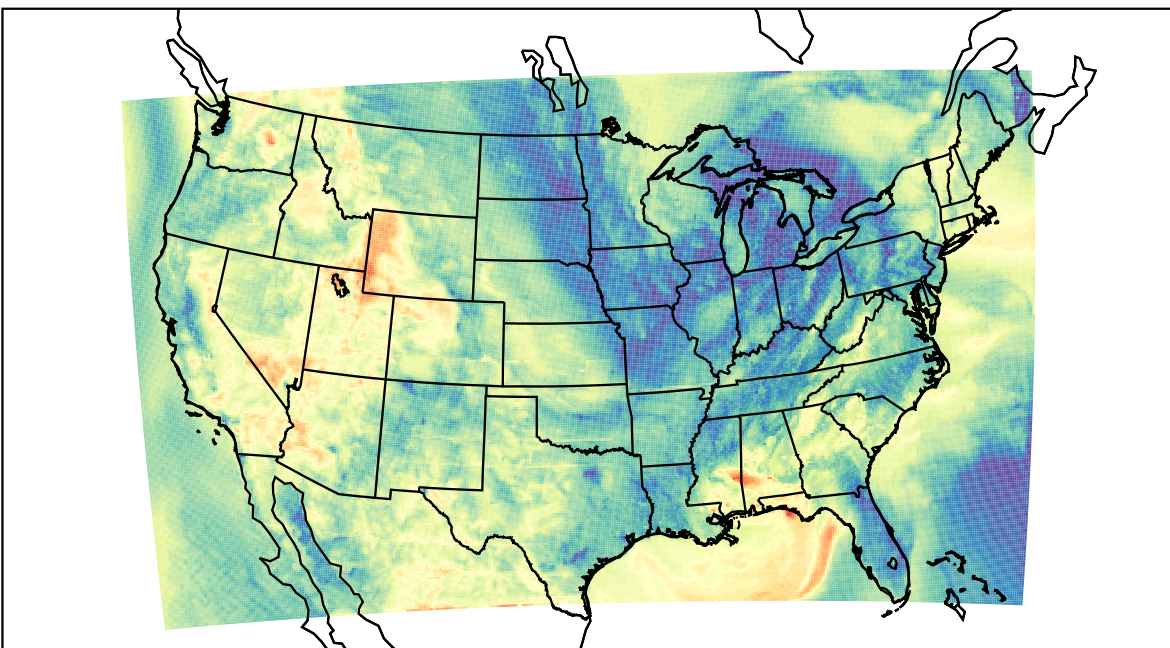
WRF (2023-04-30_05:00:00)
