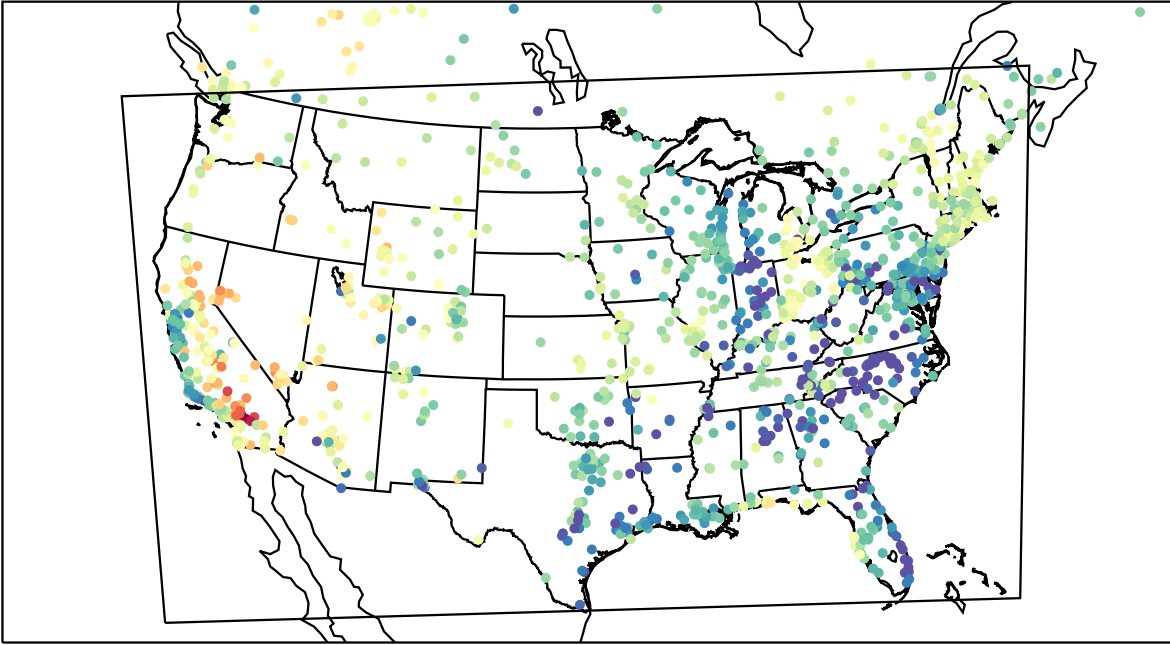
AirNOW (2023-04-30_02:00:00)
