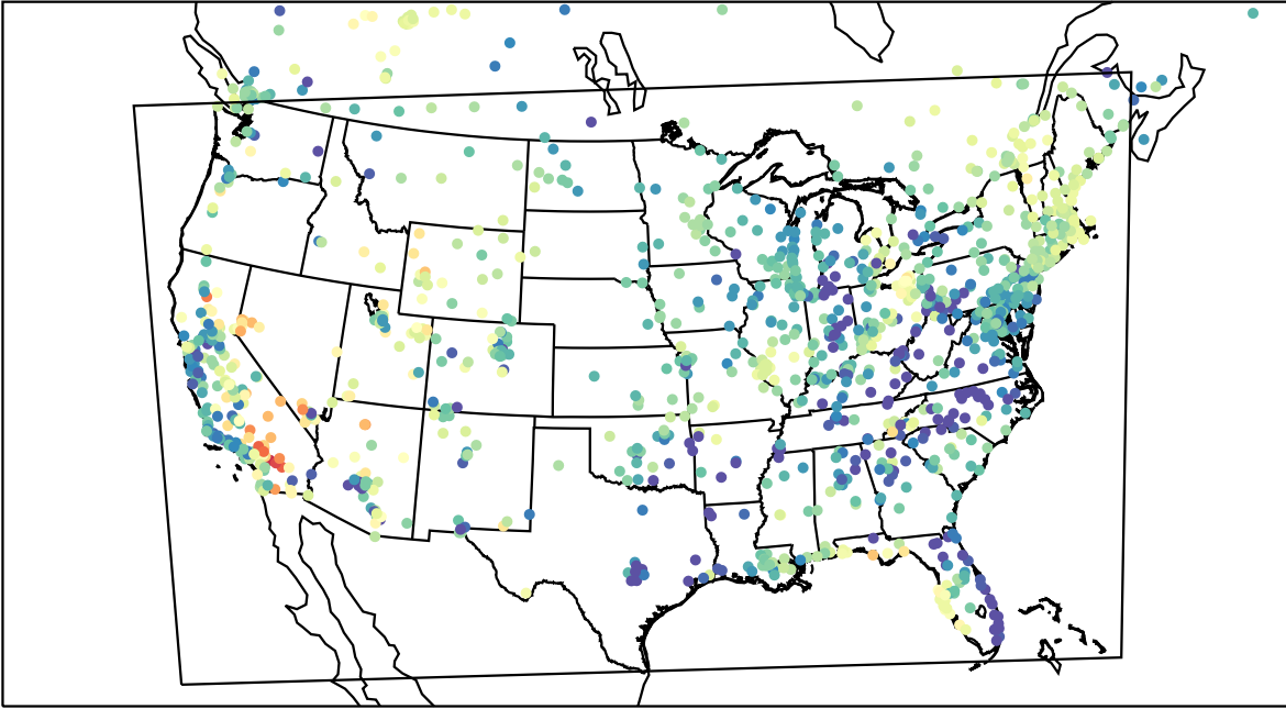
AirNOW (2023-04-30_04:00:00)
