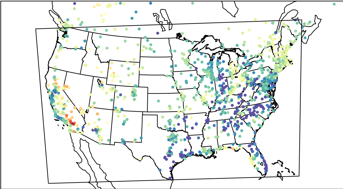
AirNOW (2023-04-30_03:00:00)
