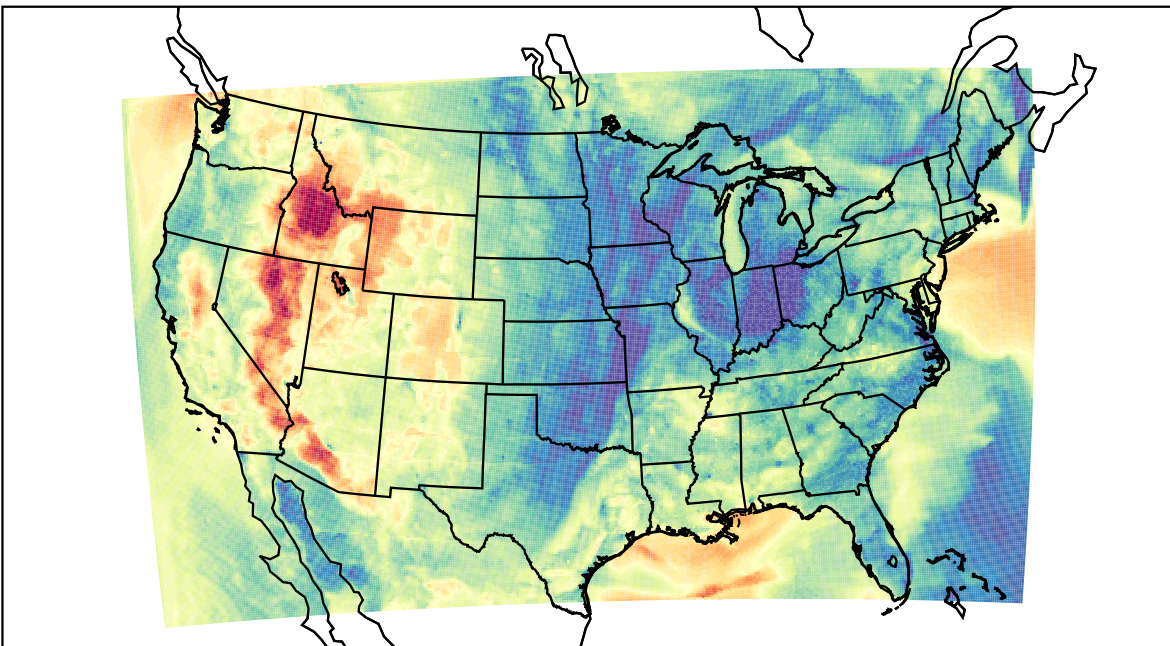
WRF (2023-04-29_03:00:00)
