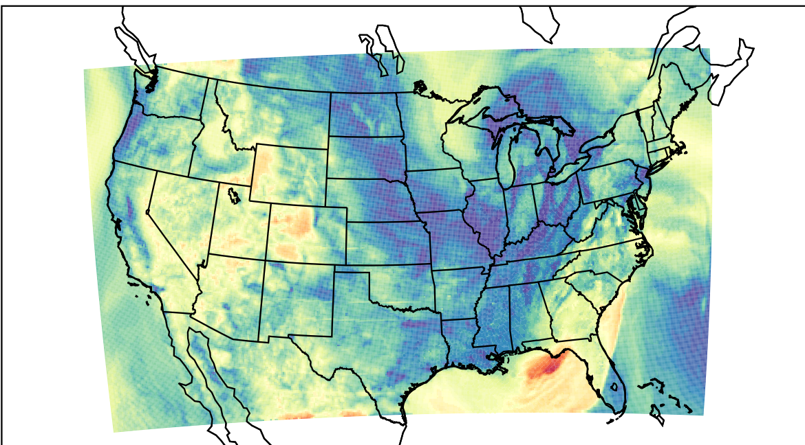
WRF (2023-04-30_12:00:00)
