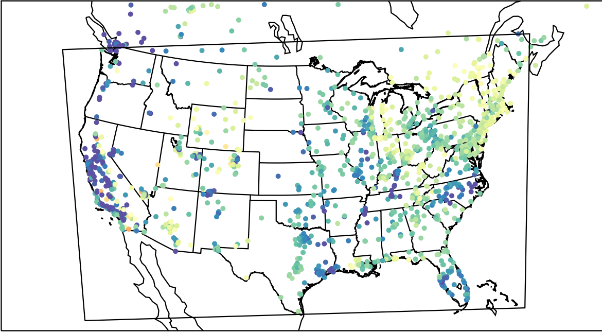
AirNOW (2023-04-29_14:00:00)
