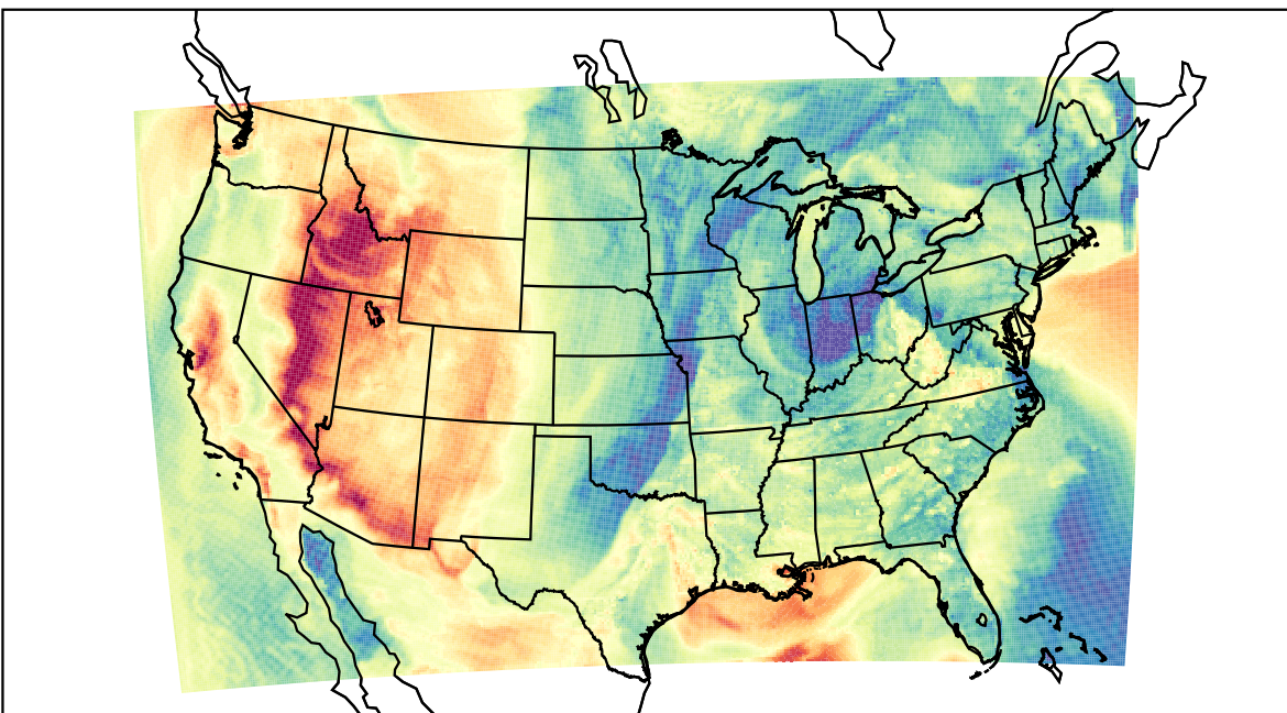
WRF (2023-04-29_00:00:00)
