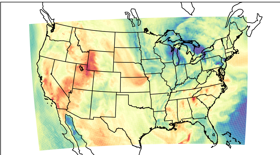
WRF (2023-04-29_22:00:00)
