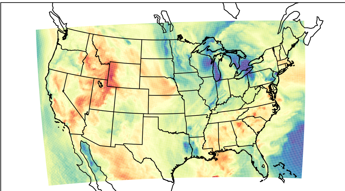
WRF (2023-04-29_19:00:00)
