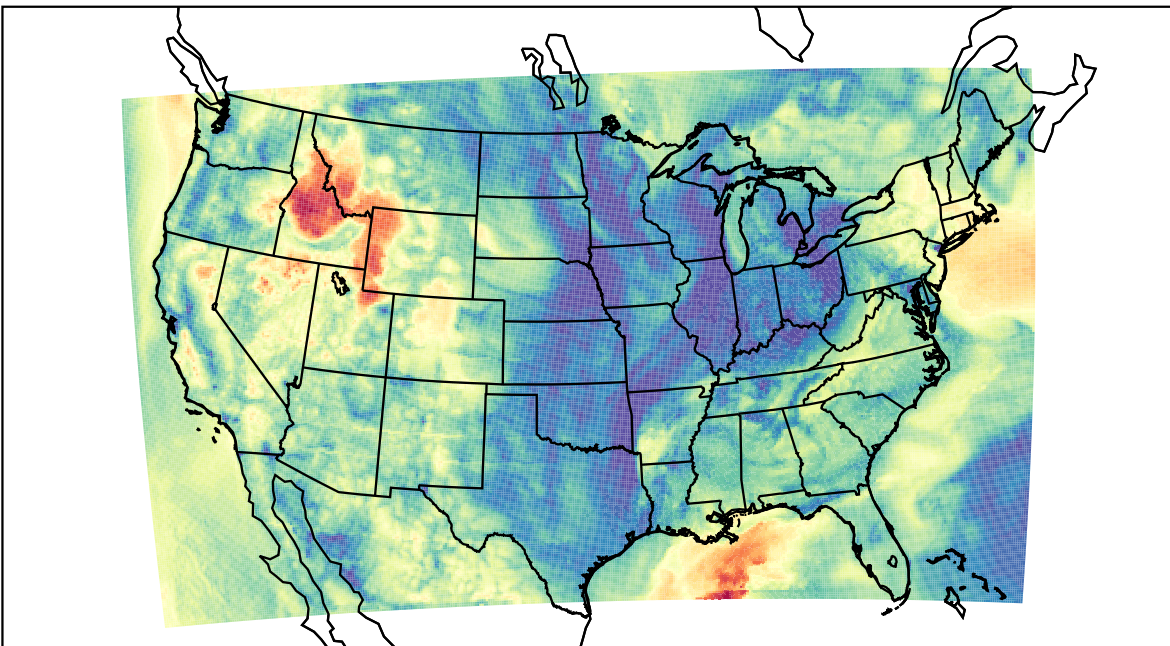
WRF (2023-04-29_14:00:00)
