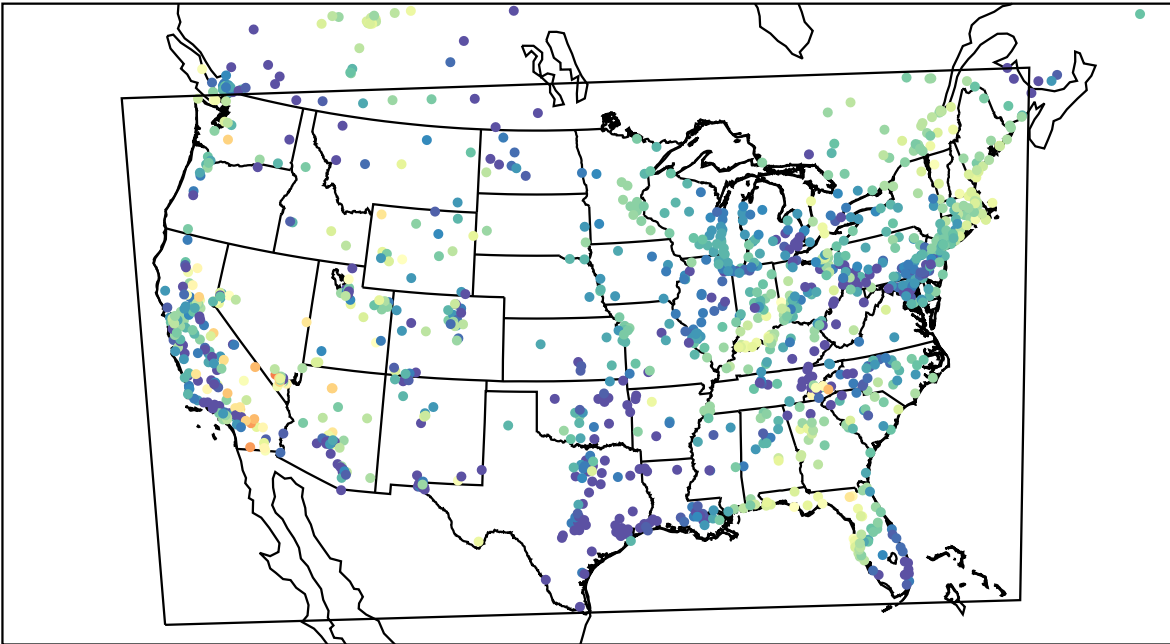
AirNOW (2023-04-30_09:00:00)
