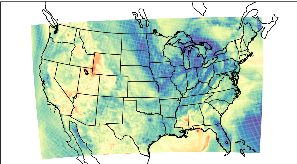
WRF (2023-04-30_04:00:00)
