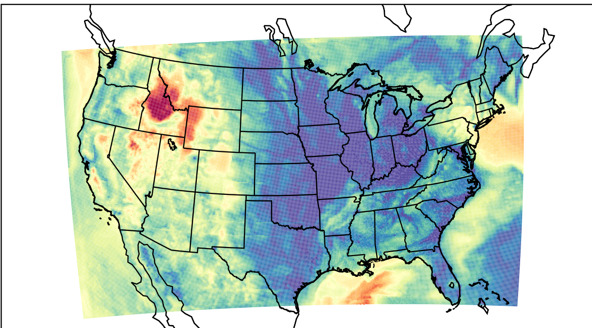
WRF (2023-04-29_11:00:00)
