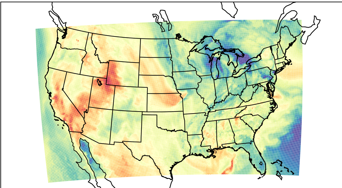
WRF (2023-04-29_23:00:00)
