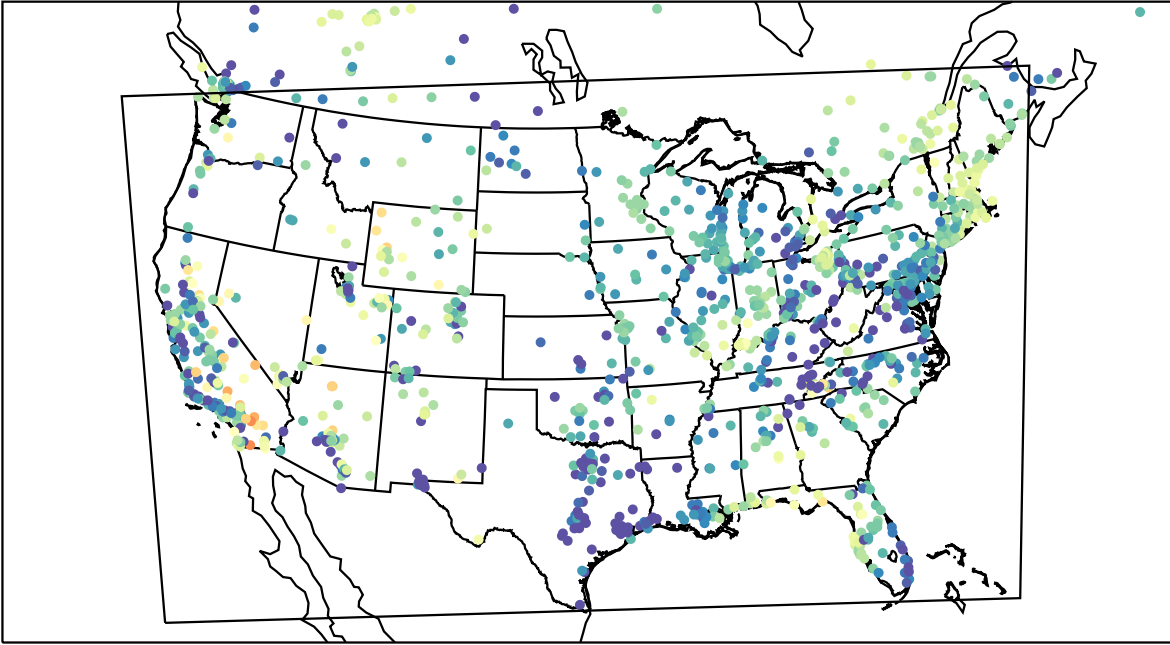
AirNOW (2023-04-30_07:00:00)
