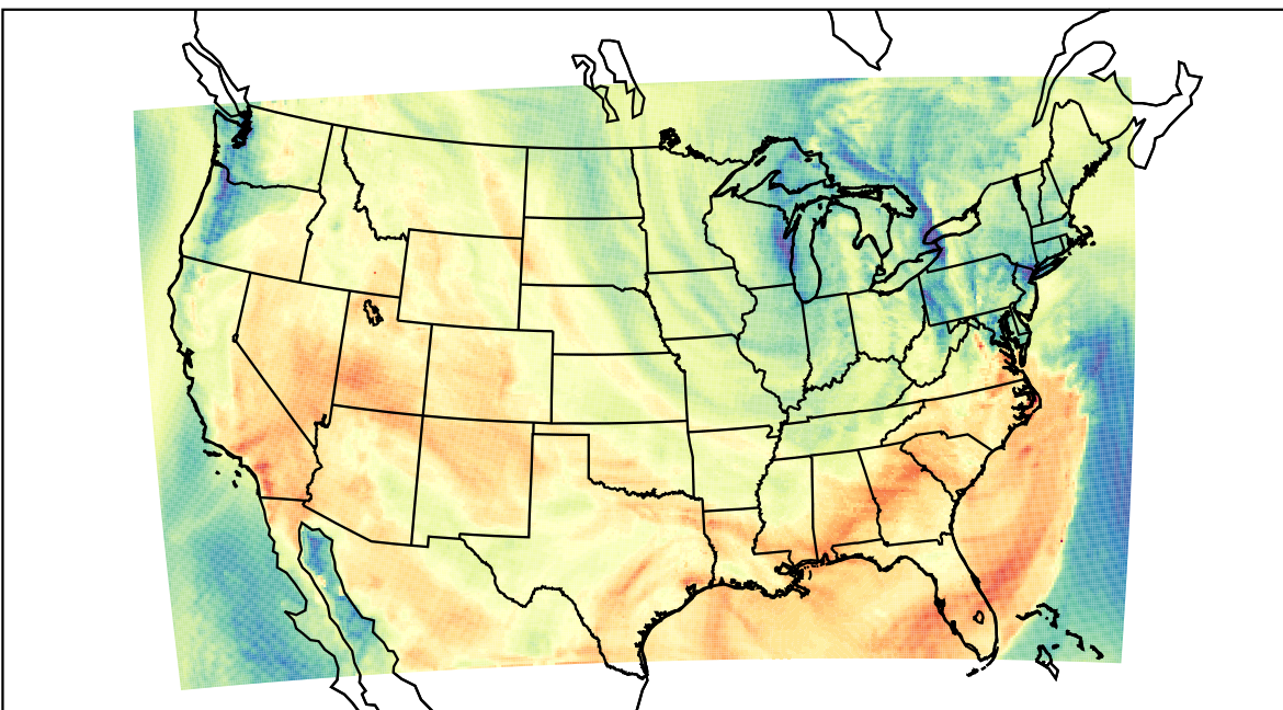
WRF (2023-04-30_21:00:00)
