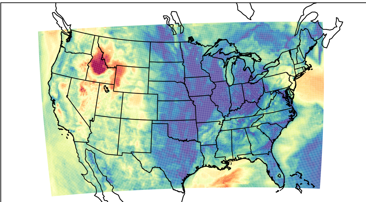
WRF (2023-04-29_10:00:00)
