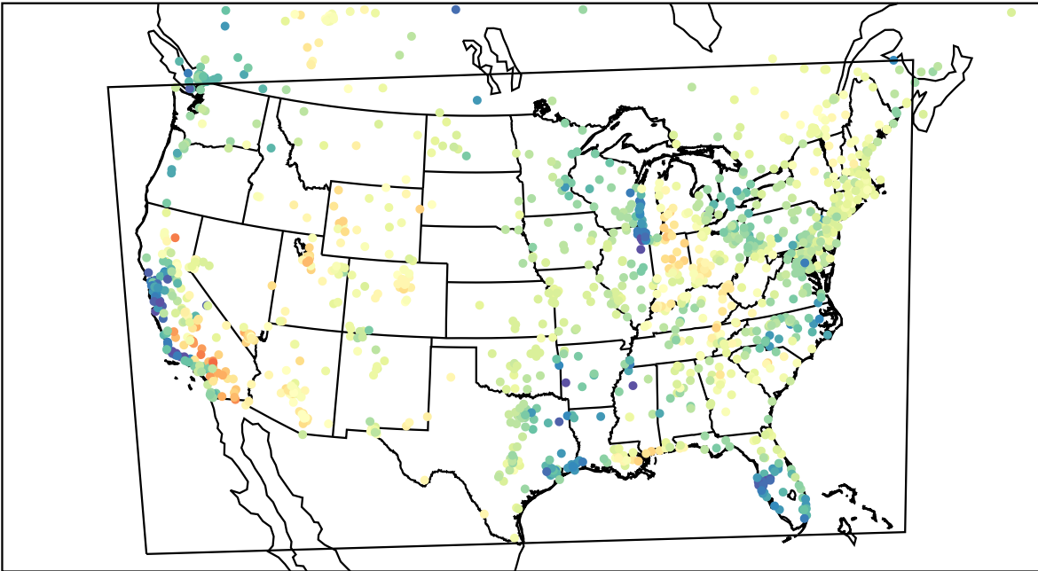
AirNOW (2023-04-29_17:00:00)
