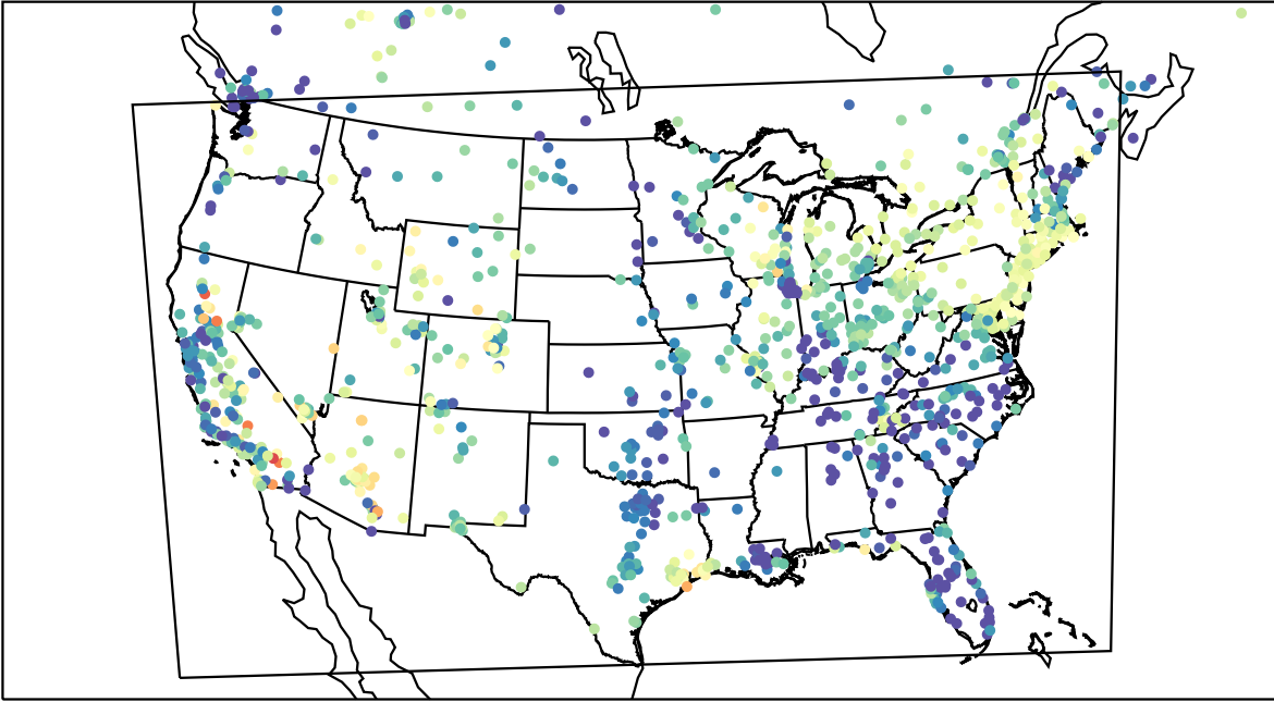
AirNOW (2023-04-29_06:00:00)
