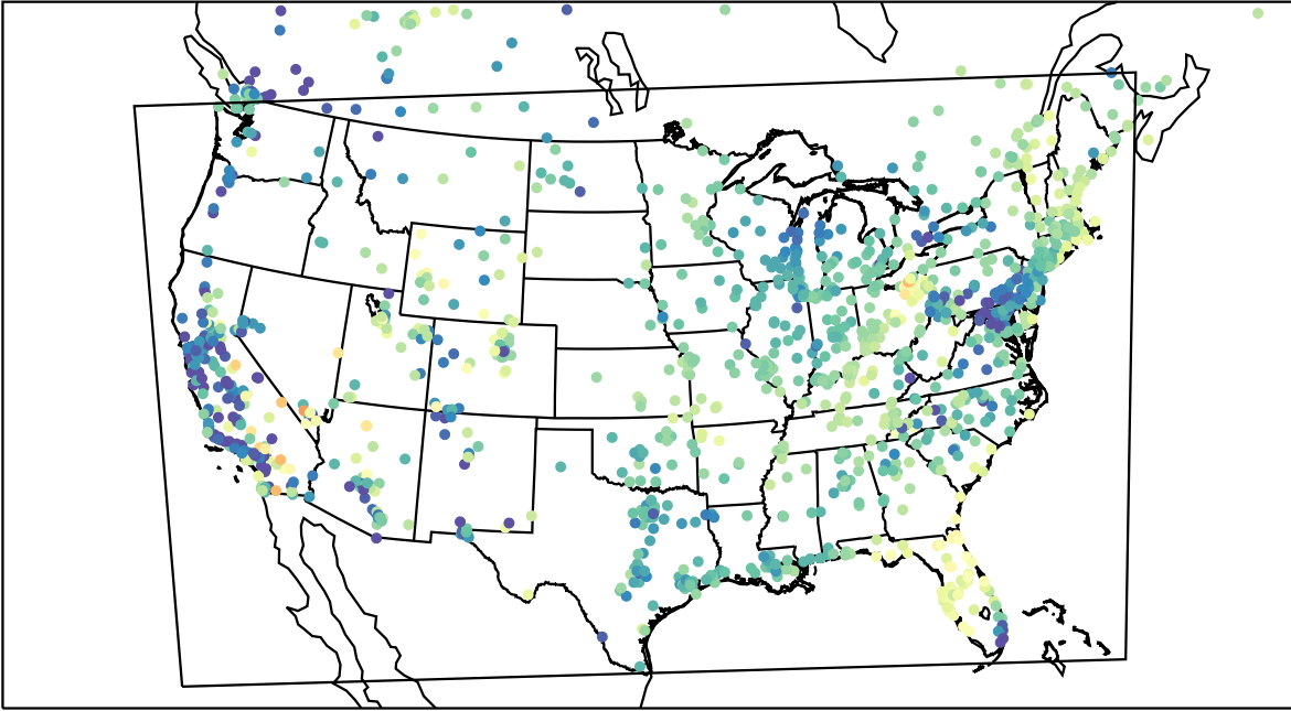
AirNOW (2023-04-30_14:00:00)
