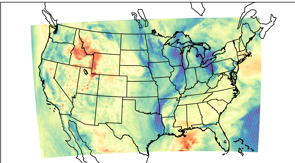
WRF (2023-04-29_16:00:00)
