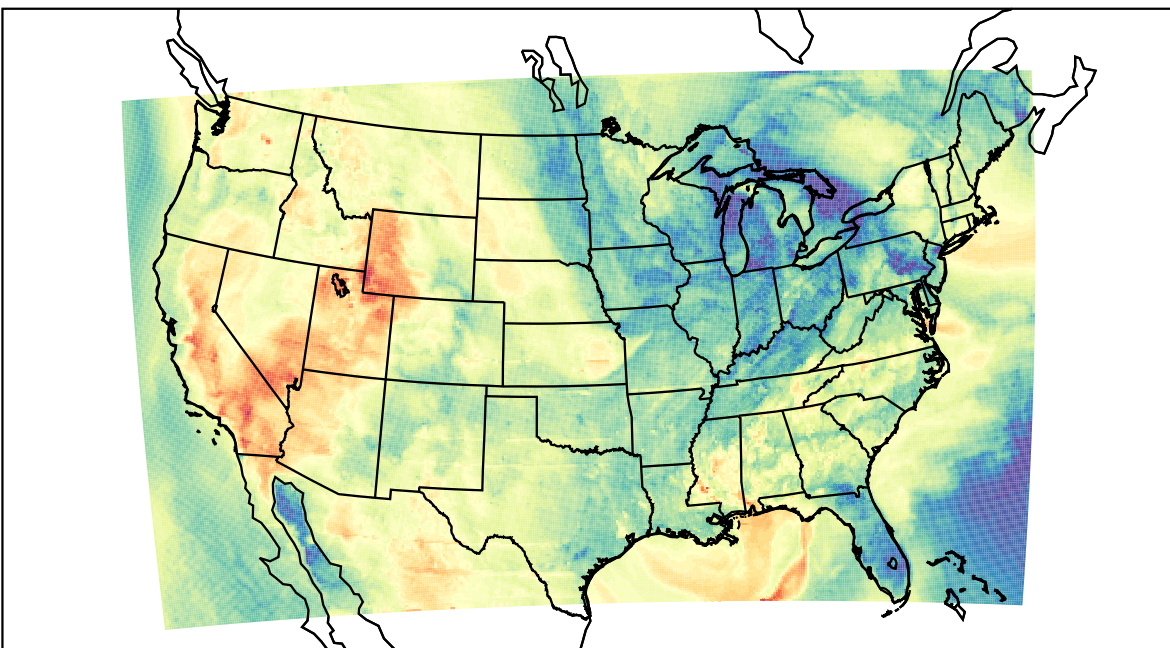
WRF (2023-04-30_01:00:00)
