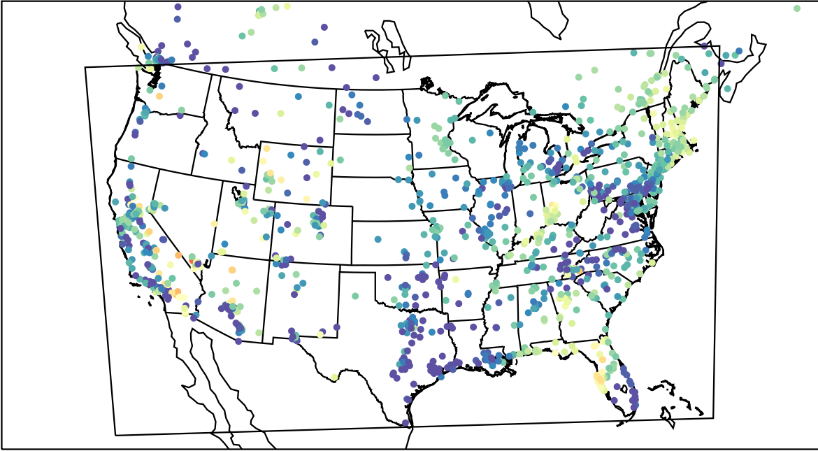
AirNOW (2023-04-30_10:00:00)
