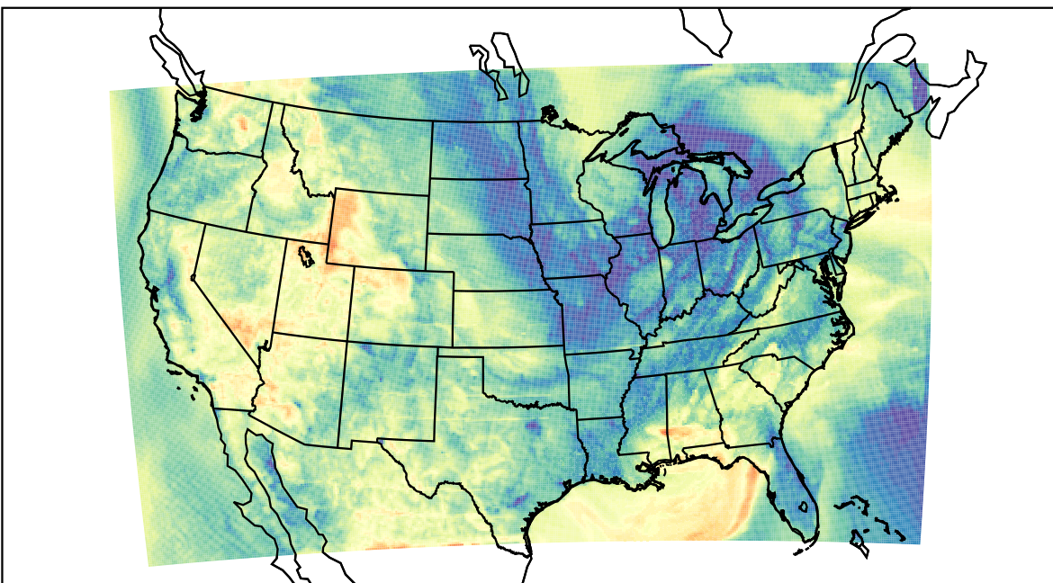
WRF (2023-04-30_06:00:00)
