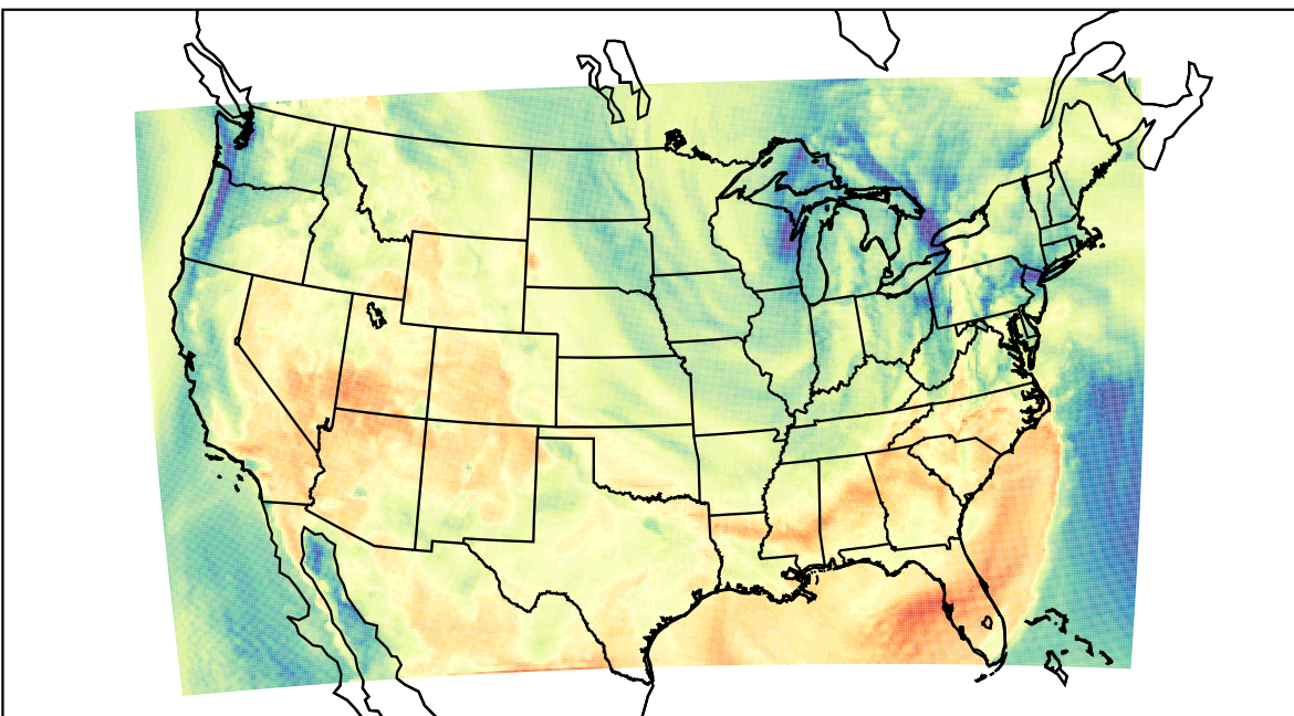
WRF (2023-04-30_18:00:00)
