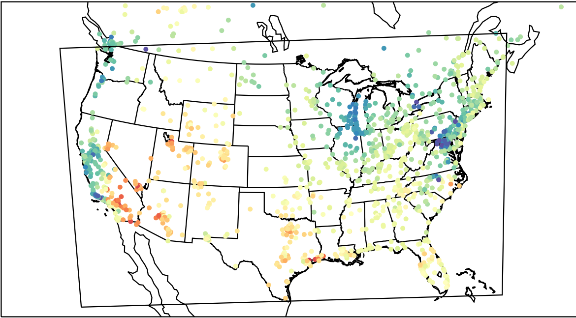
AirNOW (2023-04-30_19:00:00)
