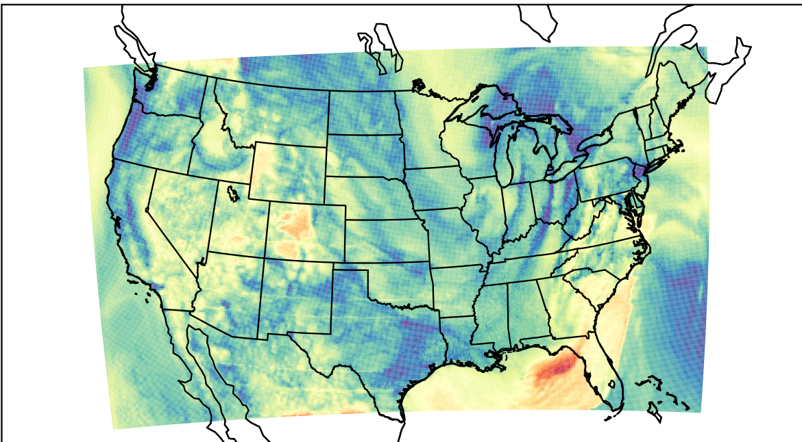
WRF (2023-04-30_14:00:00)
