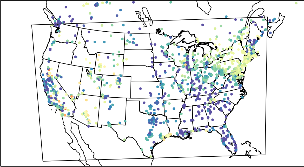
AirNOW (2023-04-29_08:00:00)
