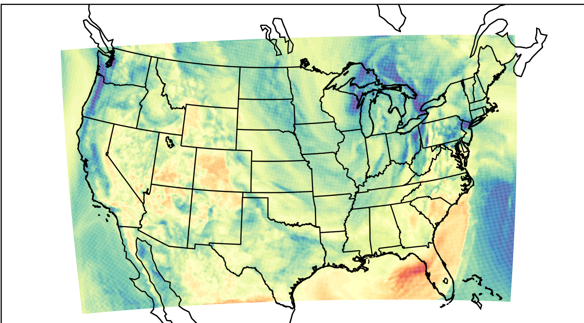
WRF (2023-04-30_16:00:00)
