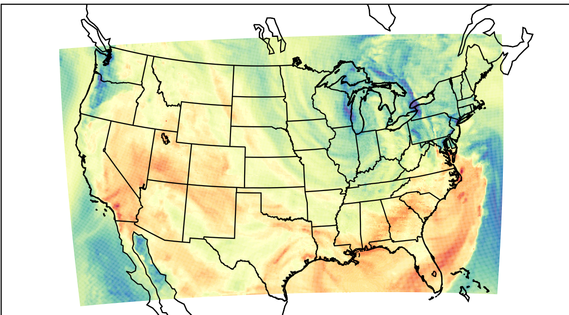
WRF (2023-04-30_22:00:00)
