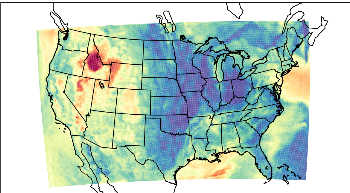
WRF (2023-04-29_07:00:00)
