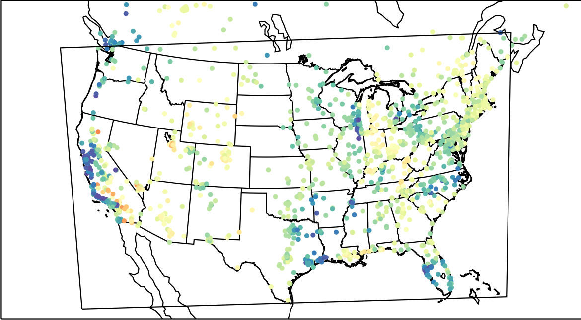
AirNOW (2023-04-29_16:00:00)
