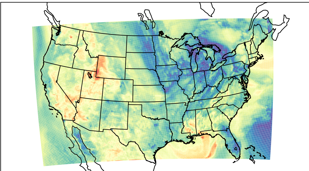
WRF (2023-04-30_03:00:00)
