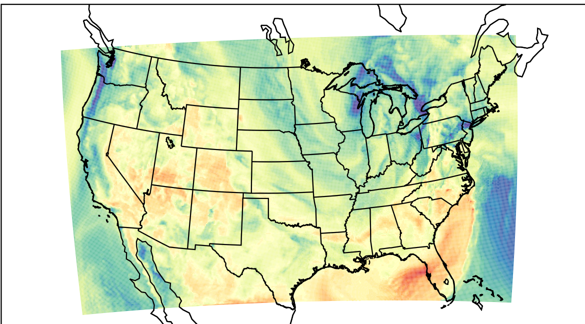
WRF (2023-04-30_17:00:00)
