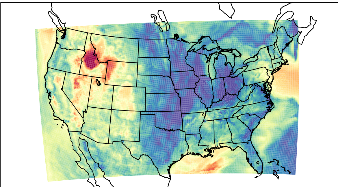
WRF (2023-04-29_08:00:00)
