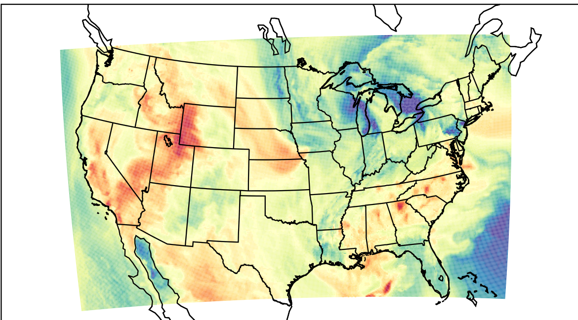
WRF (2023-04-29_21:00:00)
