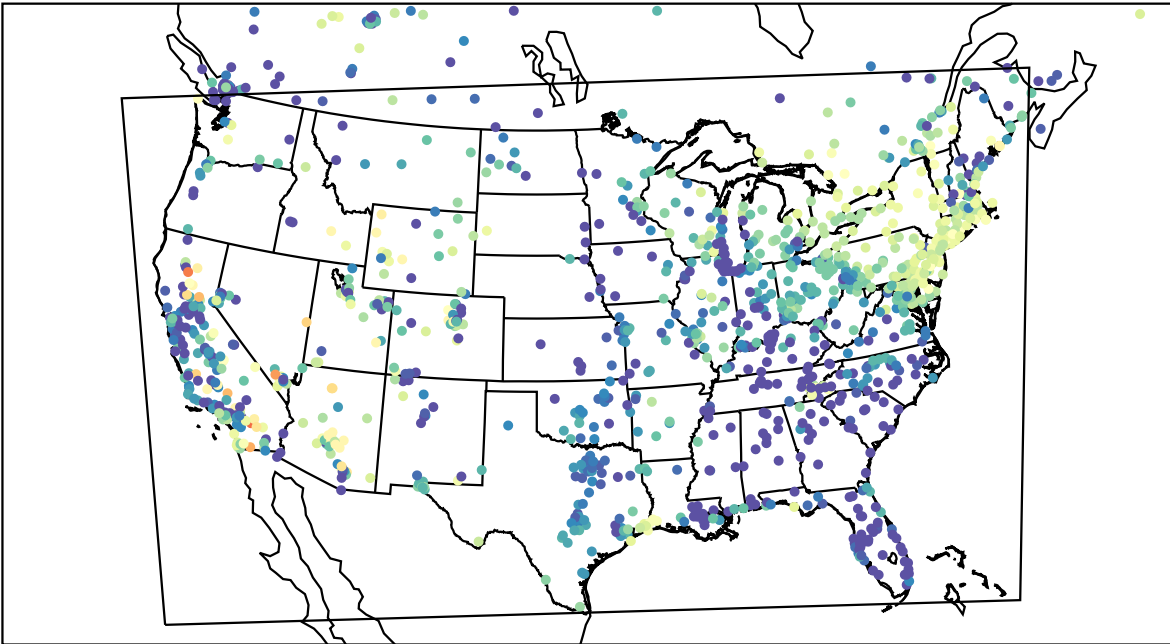
AirNOW (2023-04-29_09:00:00)
