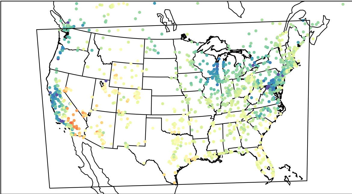
AirNOW (2023-04-30_17:00:00)
