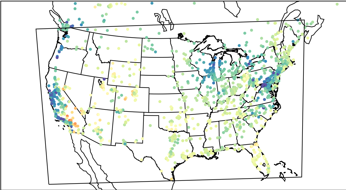
AirNOW (2023-04-30_16:00:00)
