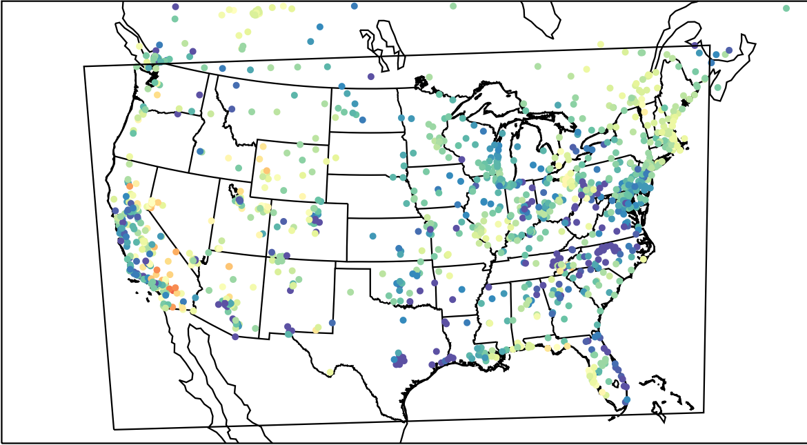
AirNOW (2023-04-30_05:00:00)
