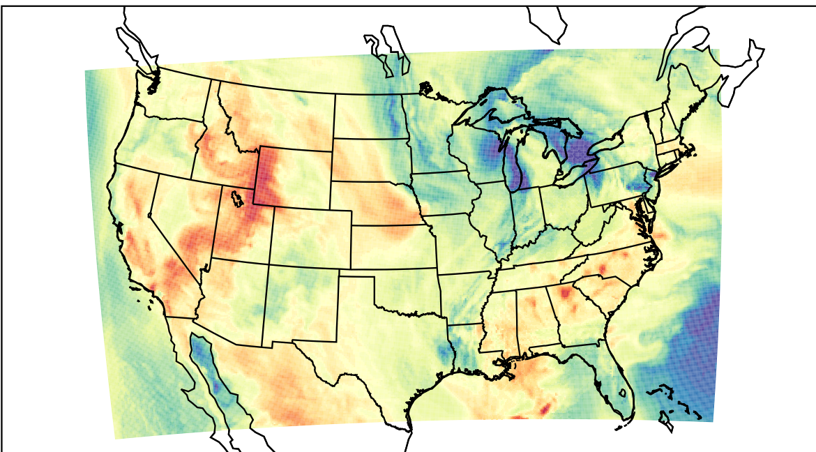
WRF (2023-04-29_20:00:00)
