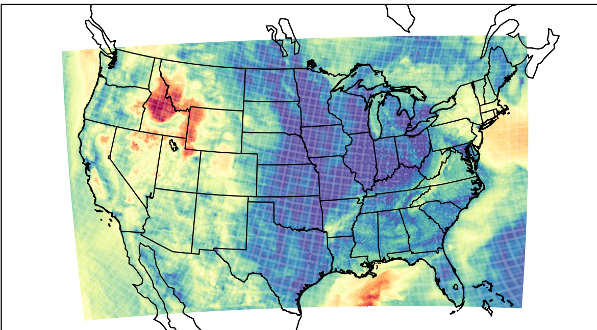
WRF (2023-04-29_13:00:00)
