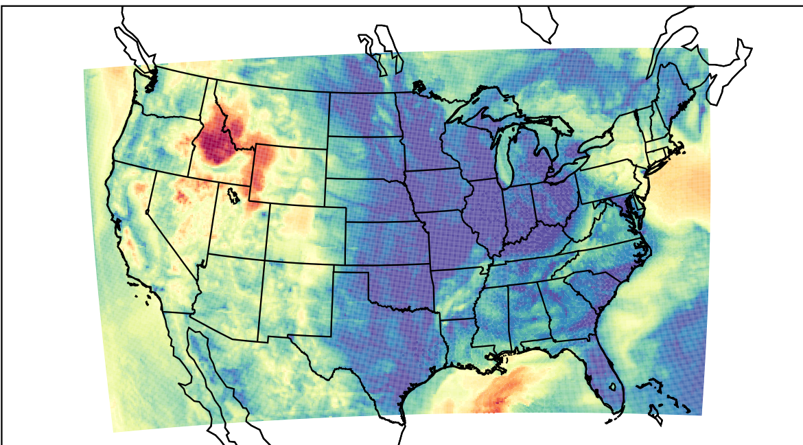
WRF (2023-04-29_12:00:00)
