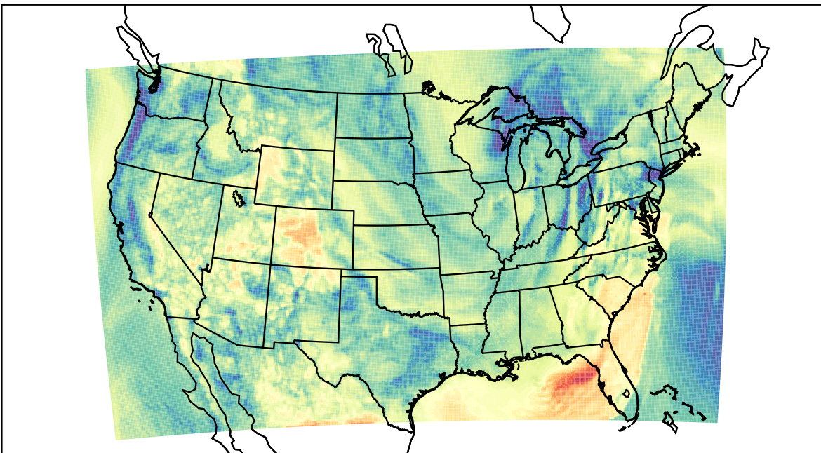
WRF (2023-04-30_15:00:00)
