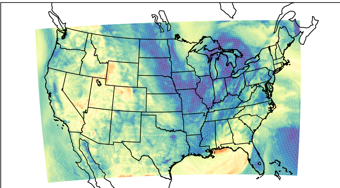
WRF (2023-04-30_08:00:00)
