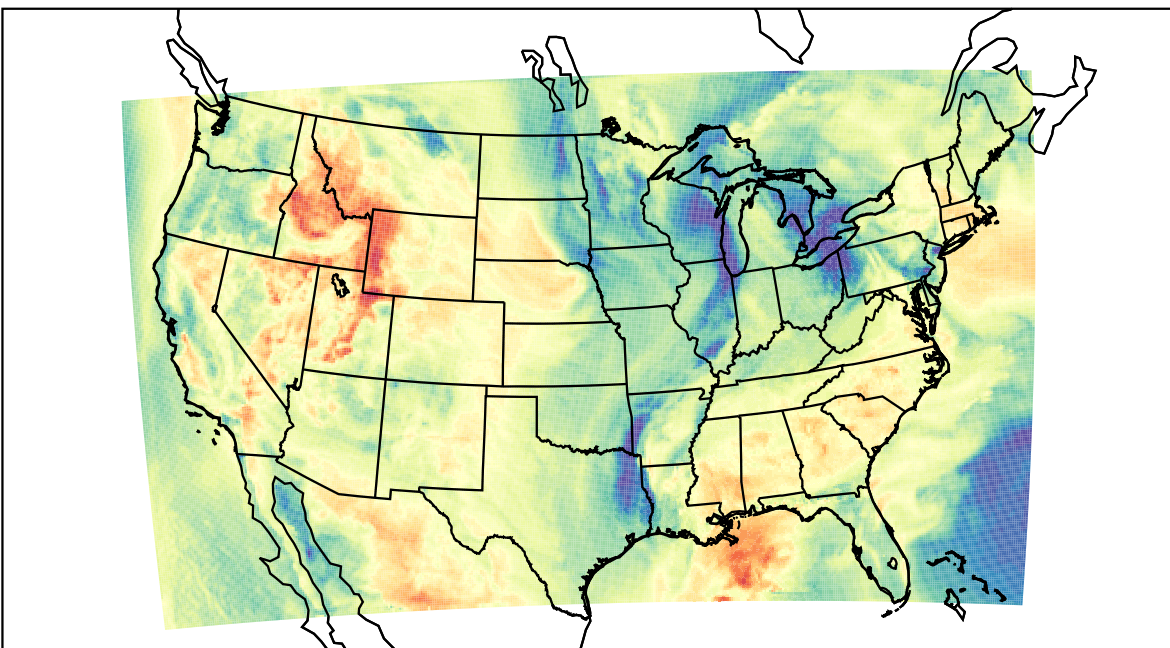
WRF (2023-04-29_17:00:00)
