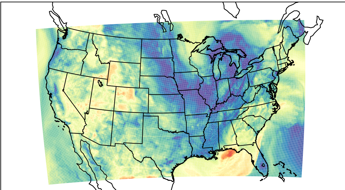
WRF (2023-04-30_10:00:00)
