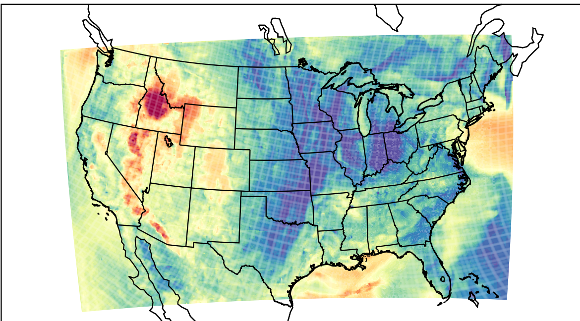
WRF (2023-04-29_05:00:00)
