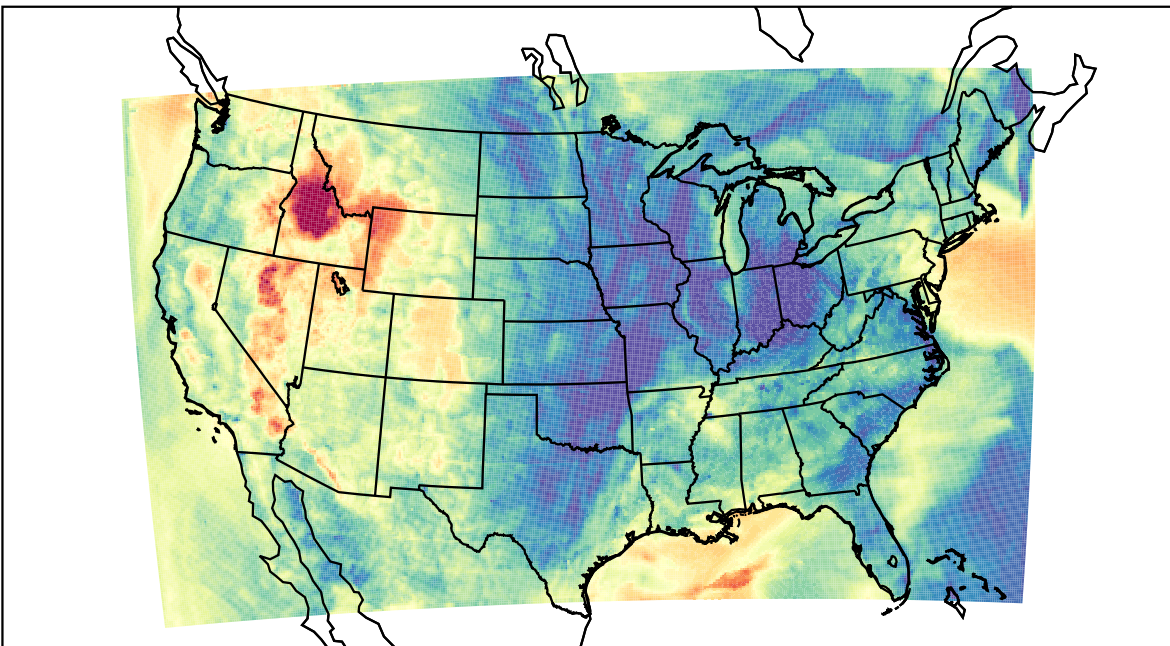
WRF (2023-04-29_06:00:00)
