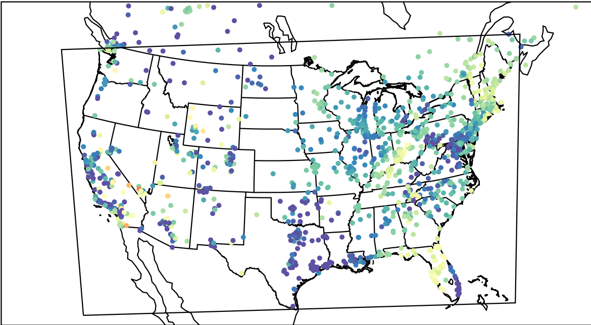
AirNOW (2023-04-30_12:00:00)
