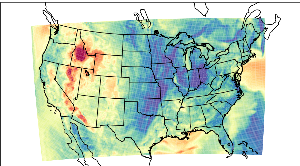
WRF (2023-04-29_04:00:00)
