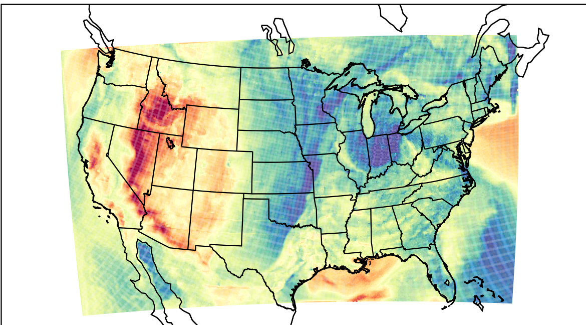
WRF (2023-04-29_01:00:00)
