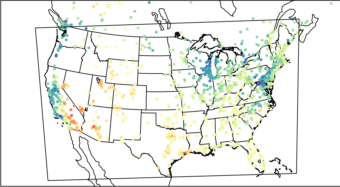
AirNOW (2023-04-30_18:00:00)
