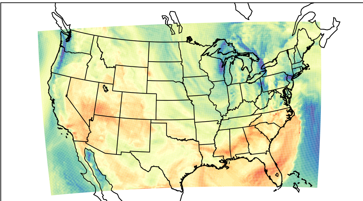
WRF (2023-04-30_19:00:00)
