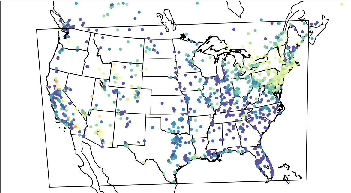
AirNOW (2023-04-29_10:00:00)
