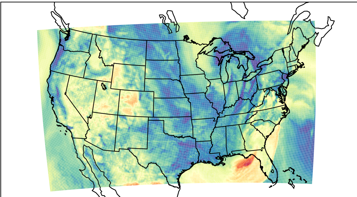
WRF (2023-04-30_13:00:00)
