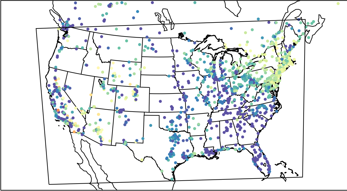
AirNOW (2023-04-29_11:00:00)
