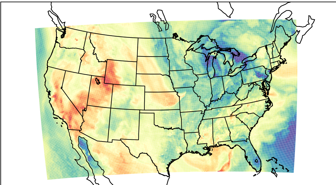
WRF (2023-04-30_00:00:00)
