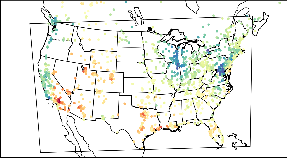
AirNOW (2023-04-30_21:00:00)
