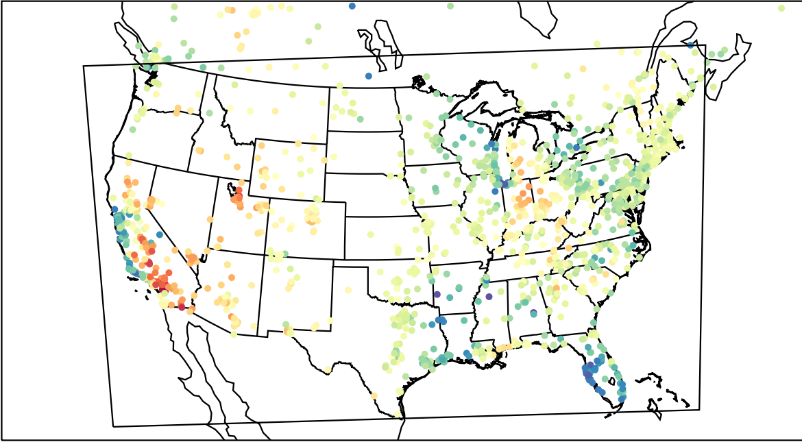
AirNOW (2023-04-29_19:00:00)
