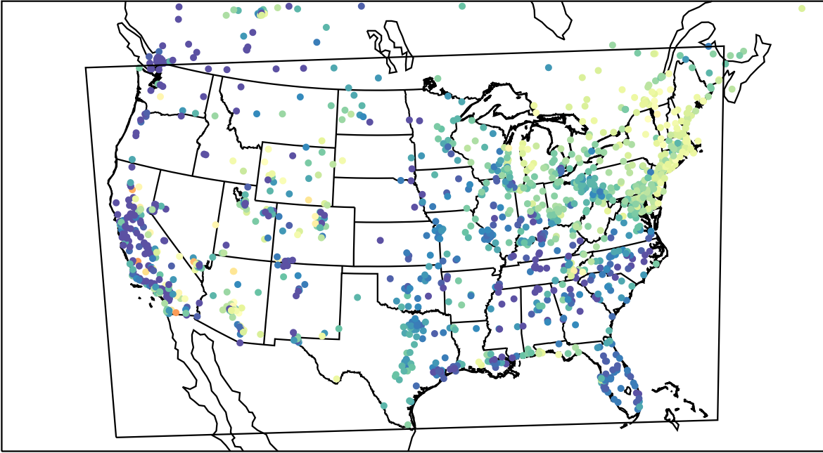
AirNOW (2023-04-29_13:00:00)
