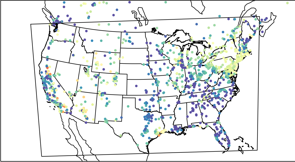
AirNOW (2023-04-29_07:00:00)
