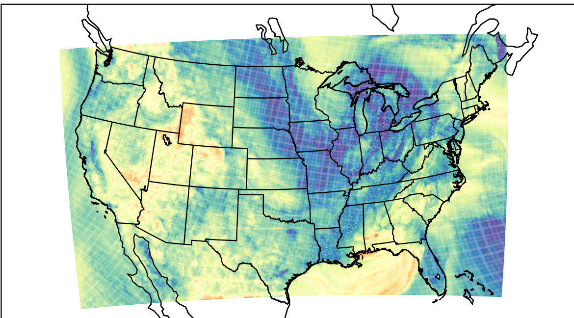
WRF (2023-04-30_07:00:00)
