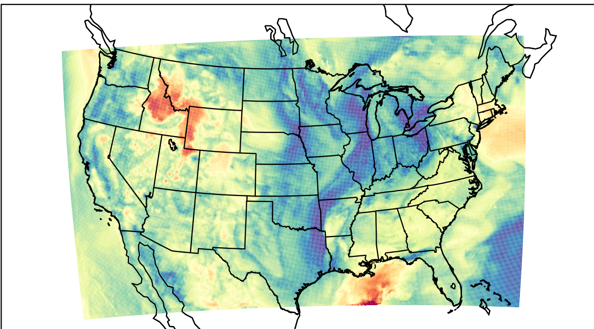
WRF (2023-04-29_15:00:00)
