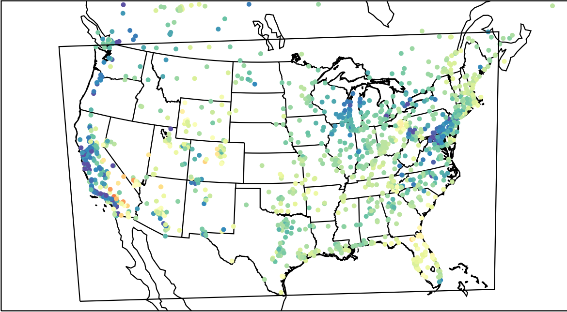
AirNOW (2023-04-30_15:00:00)
