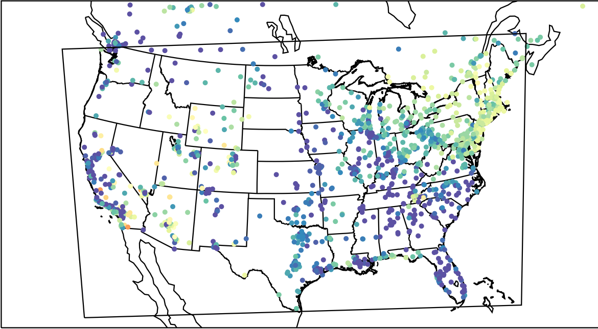
AirNOW (2023-04-29_12:00:00)
