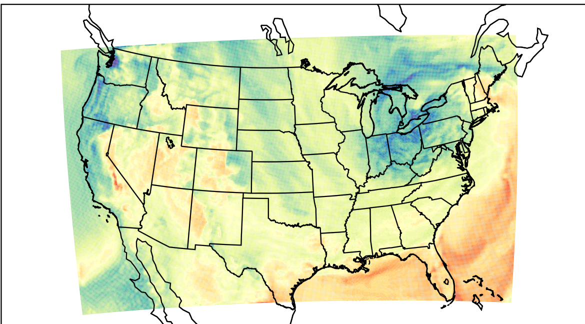
WRF (2023-05-01_17:00:00)
