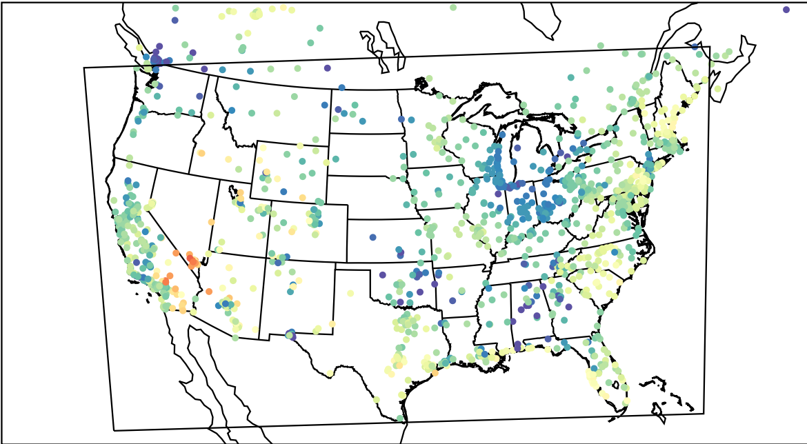
AirNOW (2023-05-01_05:00:00)
