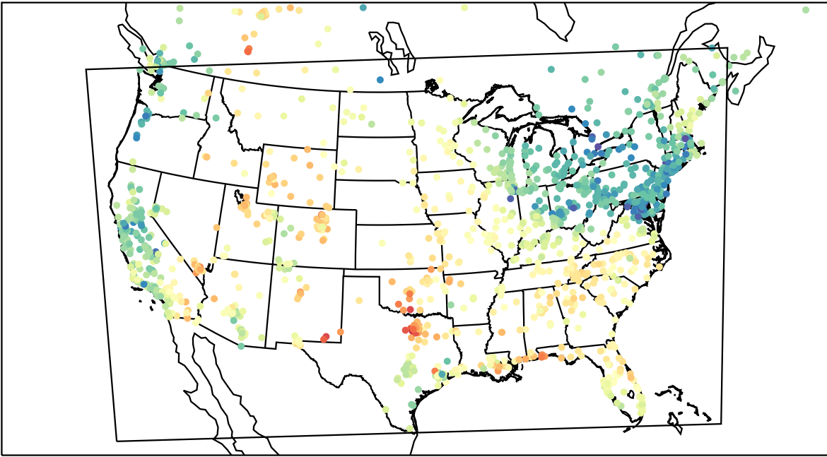
AirNOW (2023-05-02_23:00:00)
