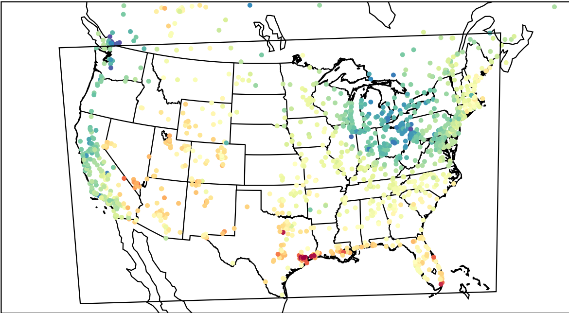
AirNOW (2023-05-01_19:00:00)
