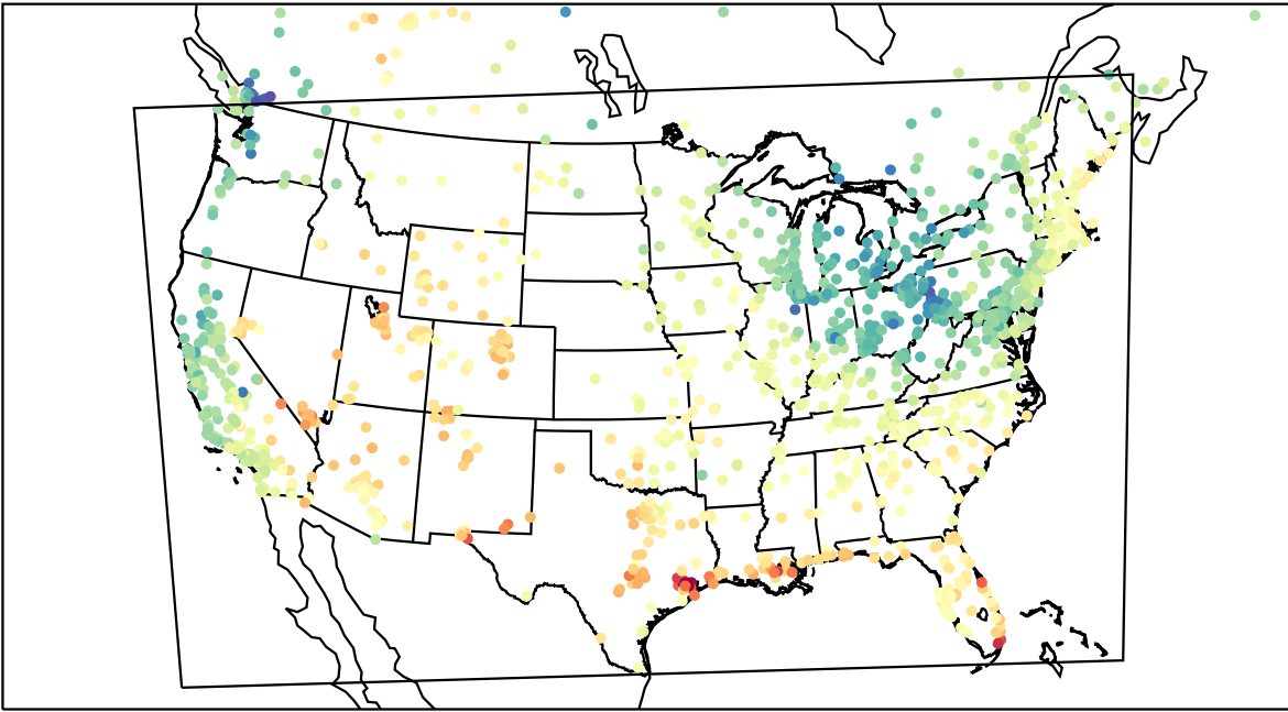
AirNOW (2023-05-01_20:00:00)
