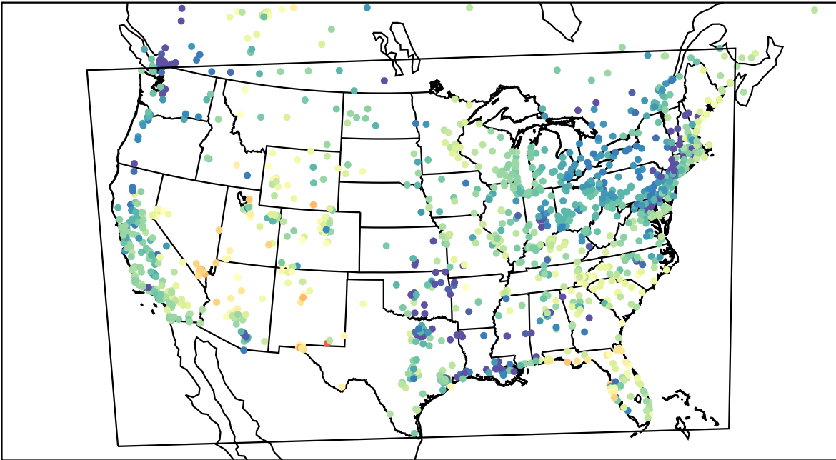
AirNOW (2023-05-02_04:00:00)
