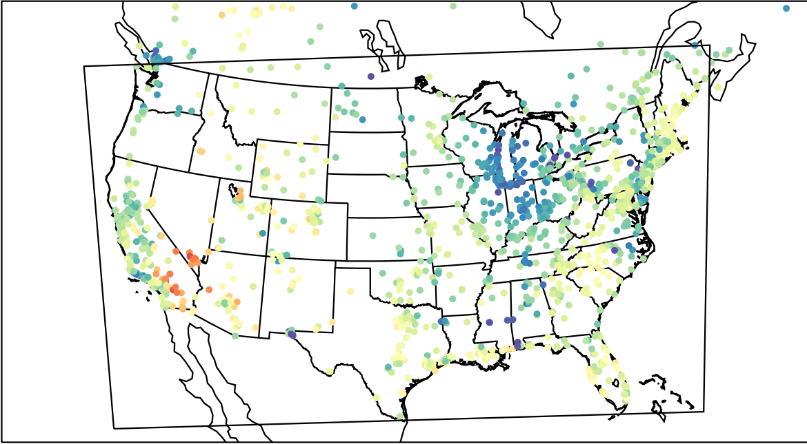
AirNOW (2023-05-01_02:00:00)
