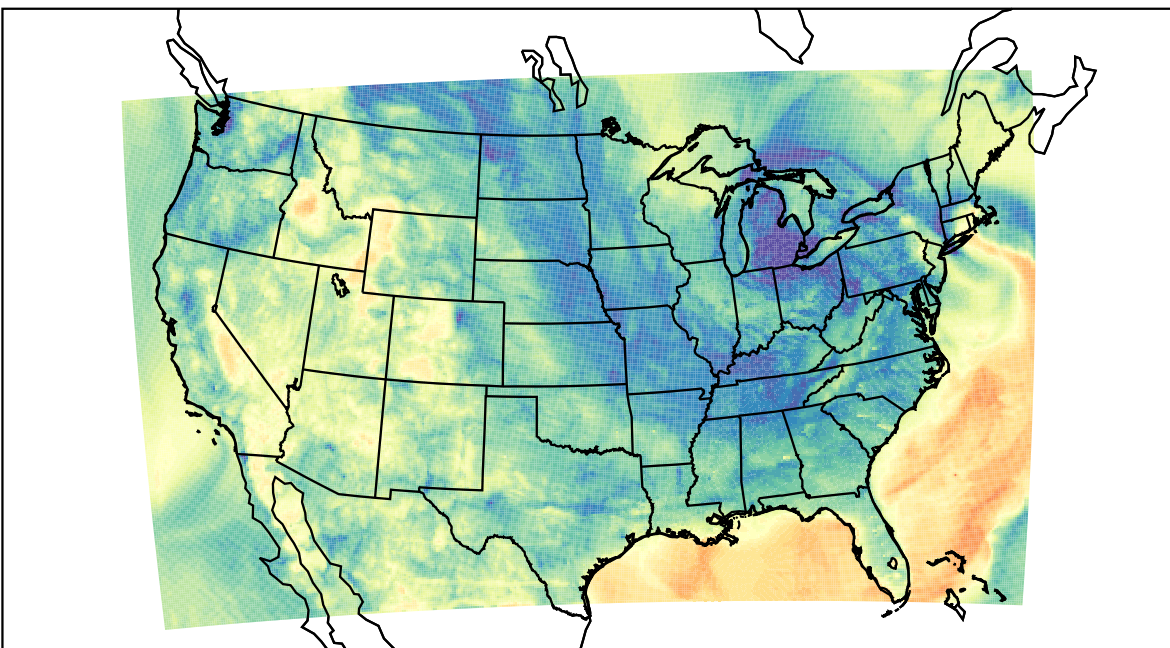
WRF (2023-05-01_07:00:00)
