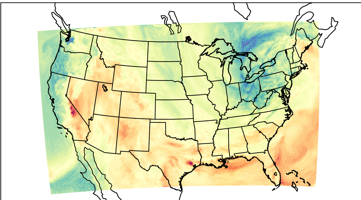
WRF (2023-05-01_21:00:00)
