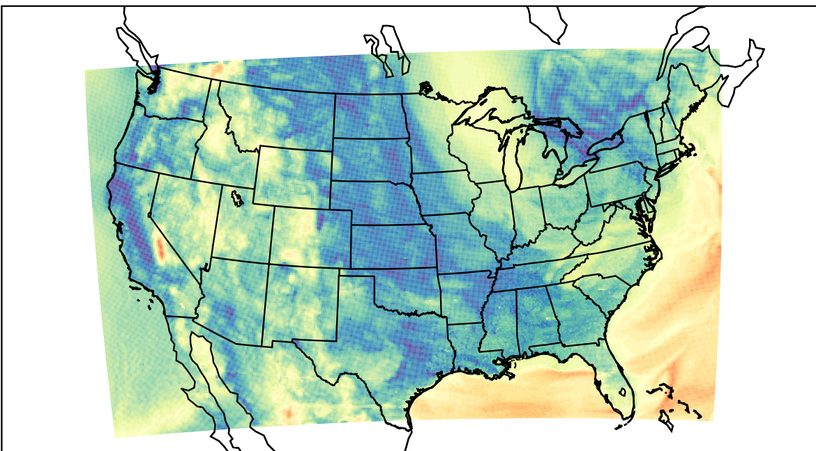
WRF (2023-05-02_13:00:00)
