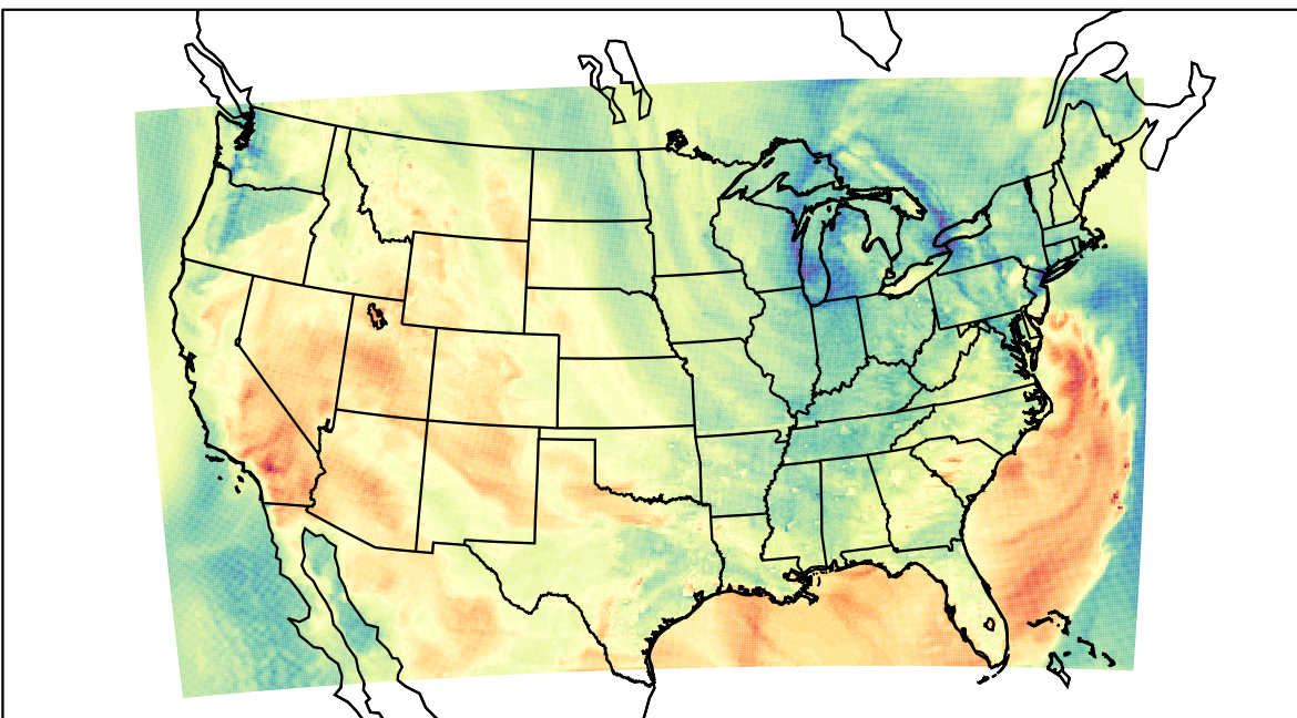
WRF (2023-05-01_00:00:00)
