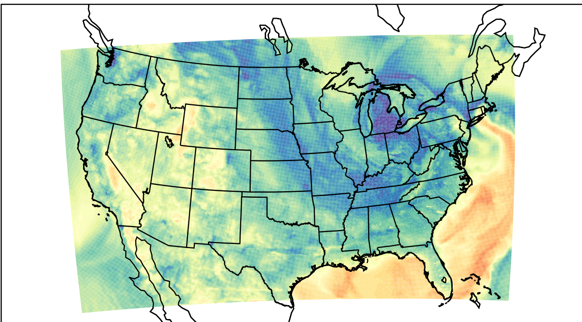
WRF (2023-05-01_06:00:00)
