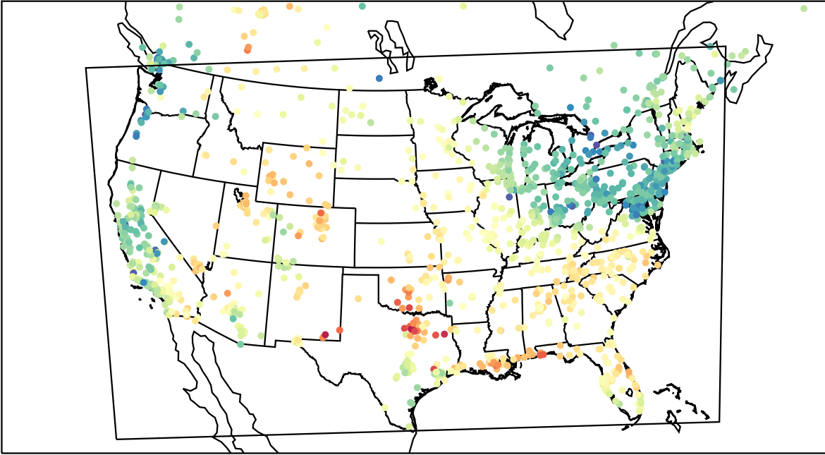
AirNOW (2023-05-02_22:00:00)
