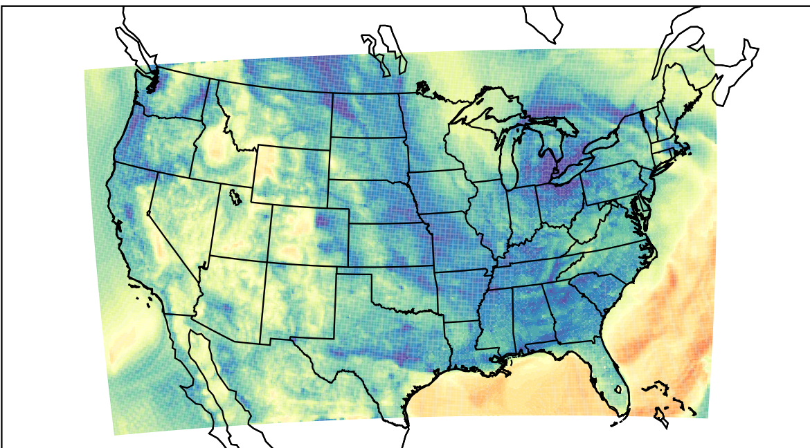
WRF (2023-05-01_12:00:00)
