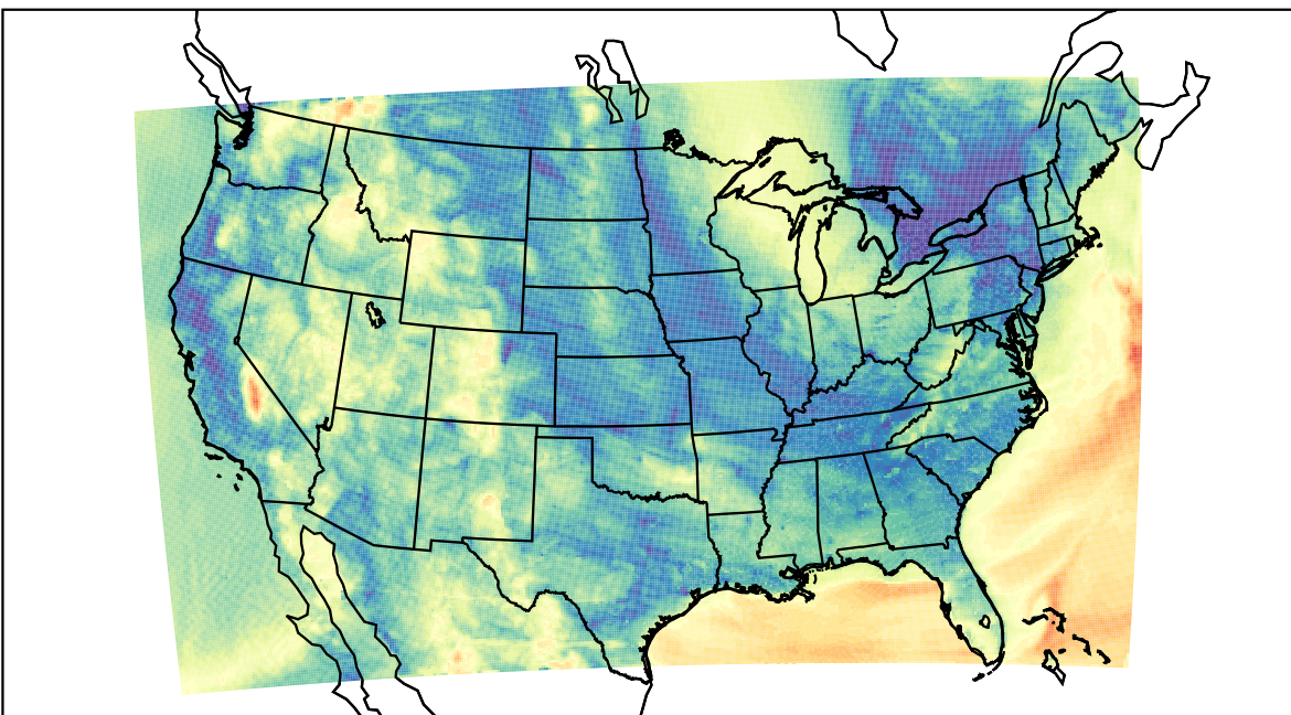
WRF (2023-05-02_11:00:00)
