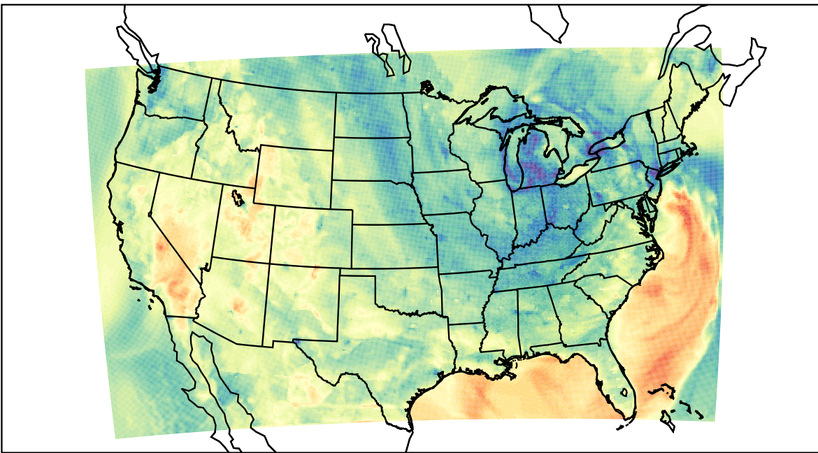
WRF (2023-05-01_02:00:00)
