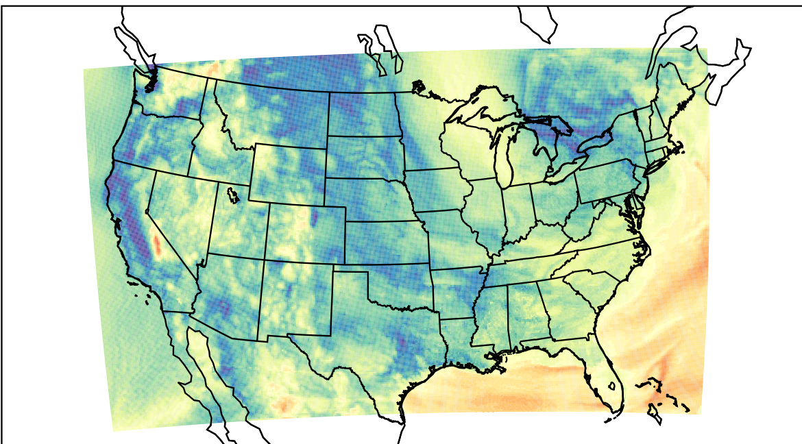
WRF (2023-05-02_14:00:00)
