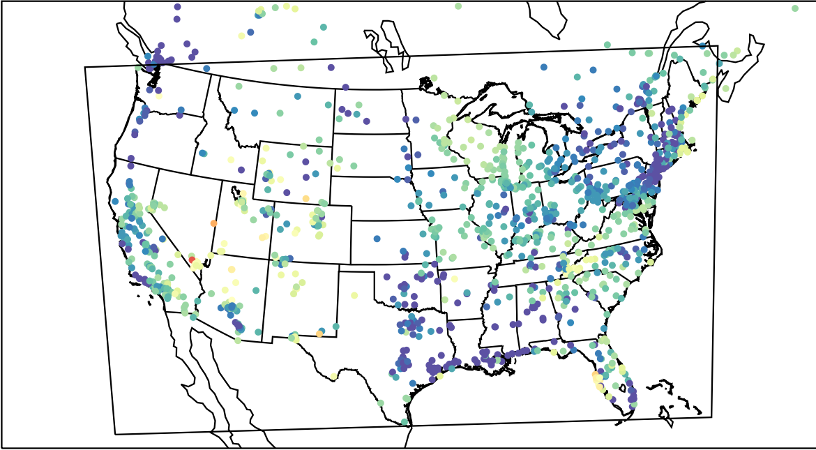
AirNOW (2023-05-02_10:00:00)
