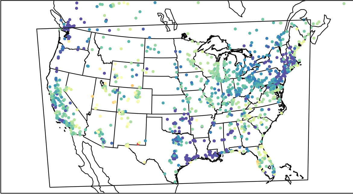
AirNOW (2023-05-02_08:00:00)
