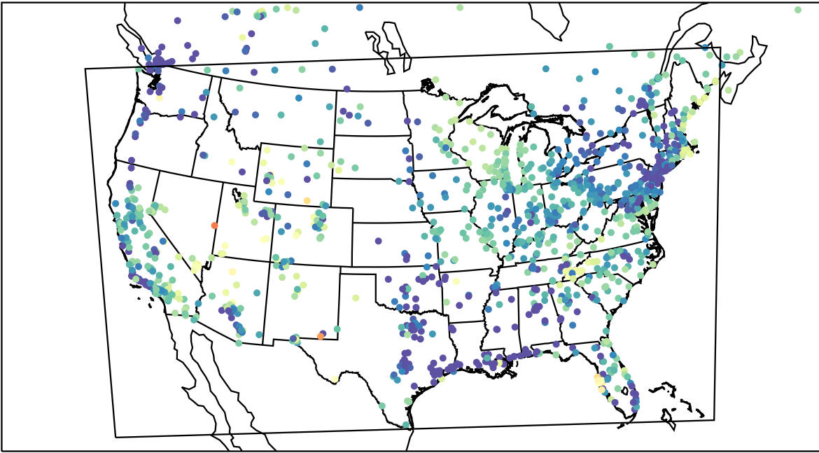
AirNOW (2023-05-02_11:00:00)
