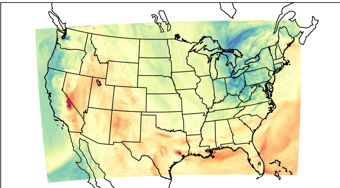
WRF (2023-05-01_22:00:00)
