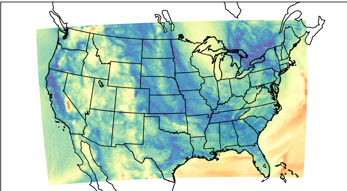
WRF (2023-05-02_12:00:00)
