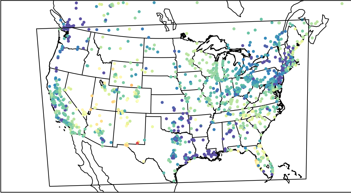
AirNOW (2023-05-02_07:00:00)
