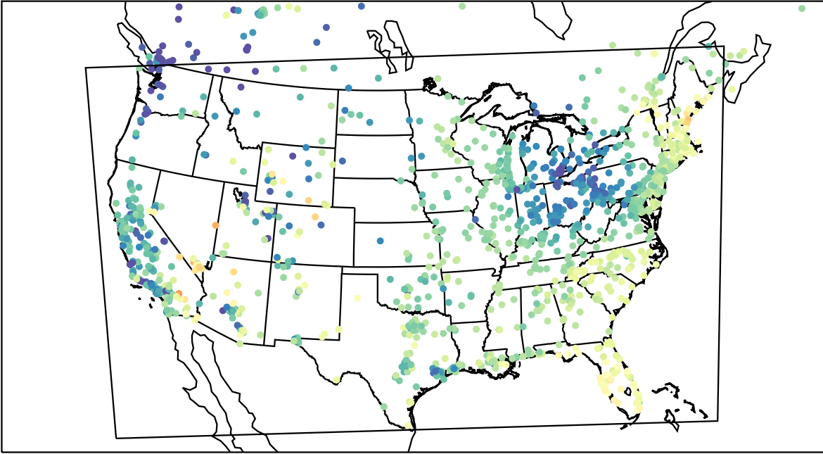
AirNOW (2023-05-01_14:00:00)
