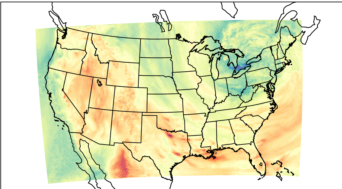
WRF (2023-05-02_22:00:00)
