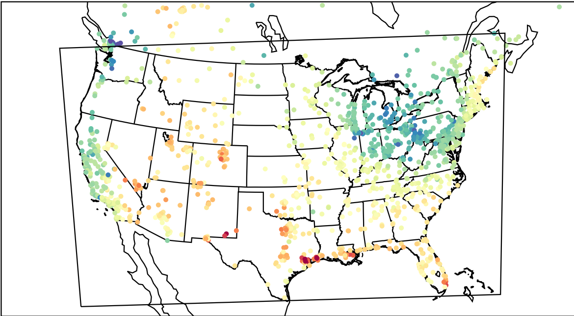
AirNOW (2023-05-01_22:00:00)
