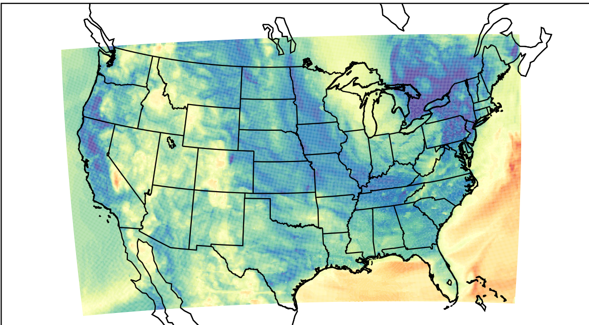
WRF (2023-05-02_09:00:00)
