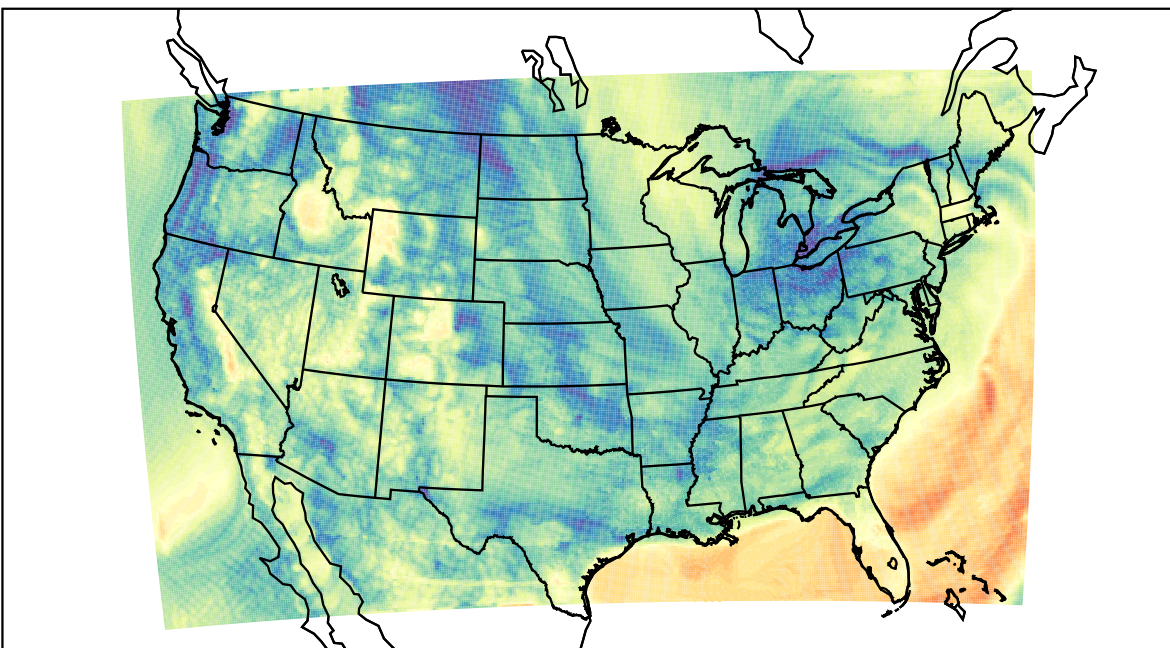
WRF (2023-05-01_14:00:00)
