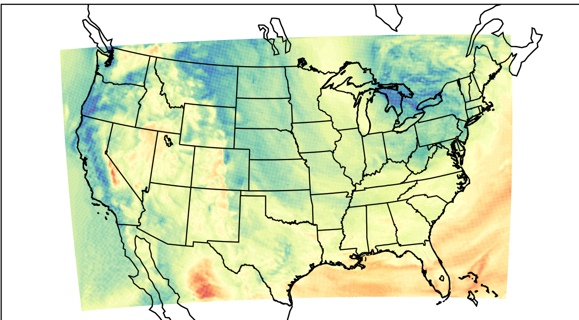
WRF (2023-05-02_16:00:00)
