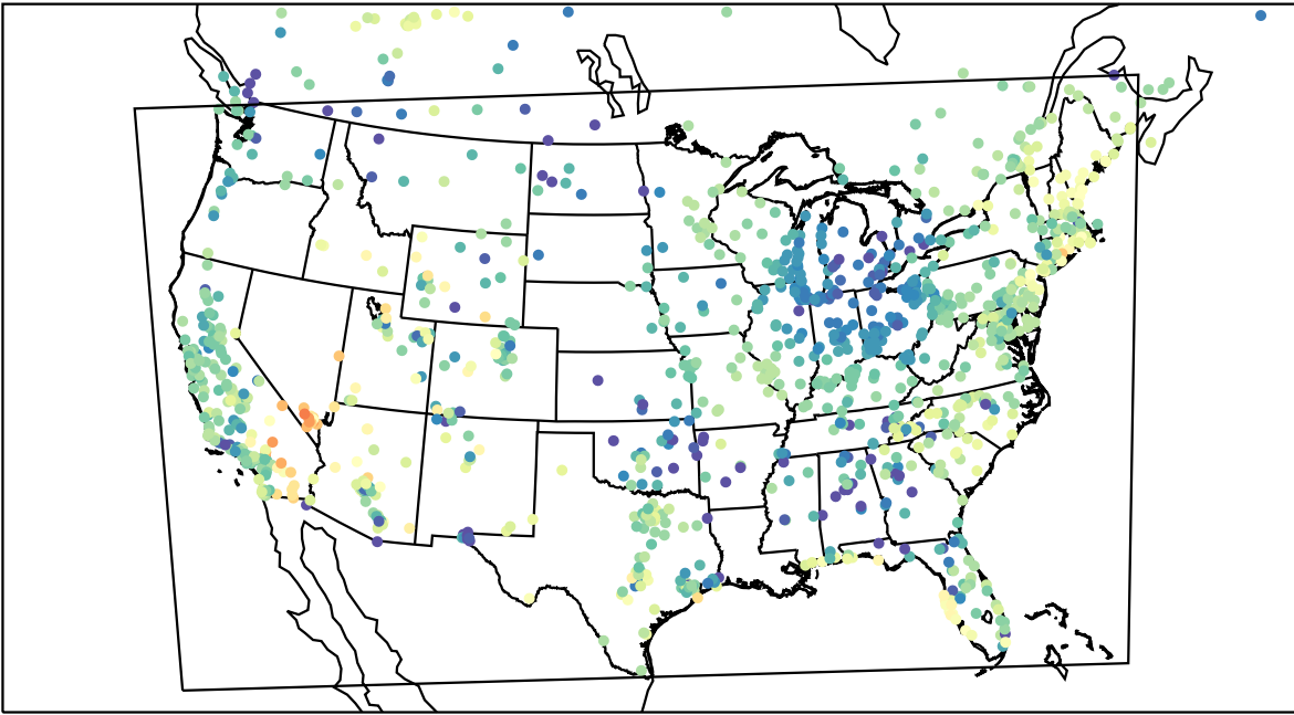
AirNOW (2023-05-01_07:00:00)
