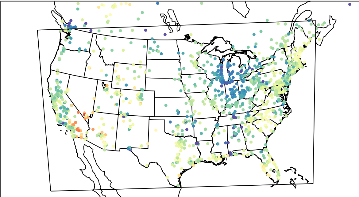
AirNOW (2023-05-01_03:00:00)
