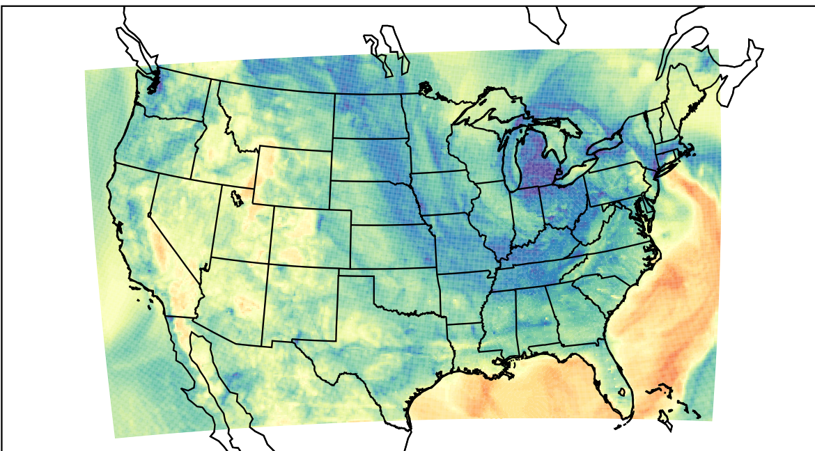
WRF (2023-05-01_05:00:00)
