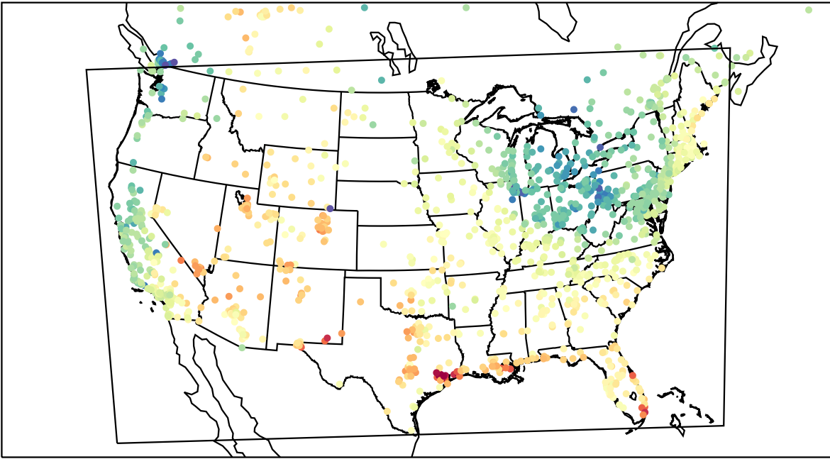
AirNOW (2023-05-01_21:00:00)
