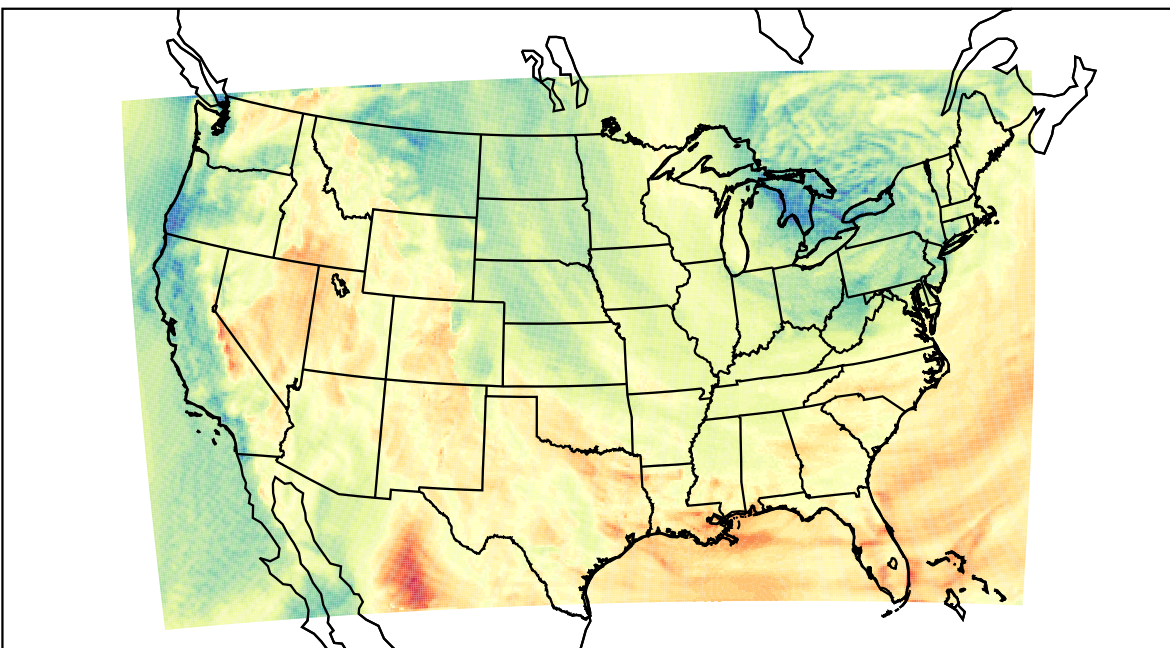
WRF (2023-05-02_18:00:00)
