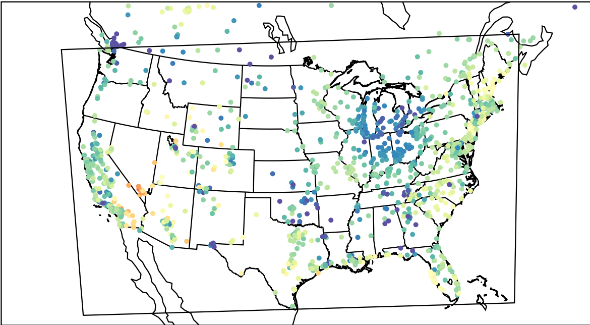
AirNOW (2023-05-01_06:00:00)
