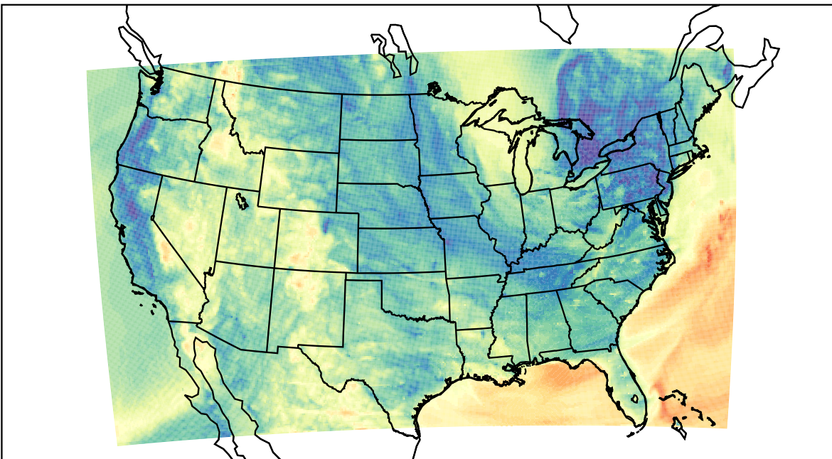
WRF (2023-05-02_06:00:00)
