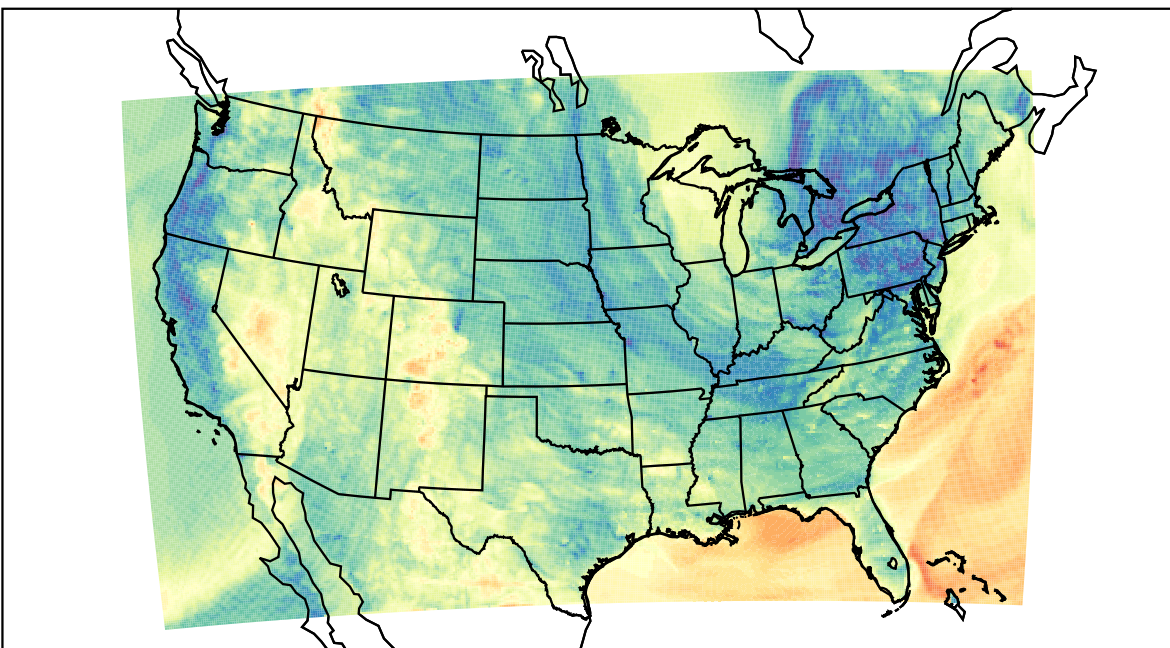
WRF (2023-05-02_04:00:00)
