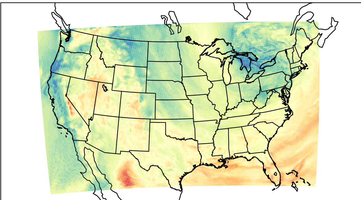
WRF (2023-05-02_17:00:00)
