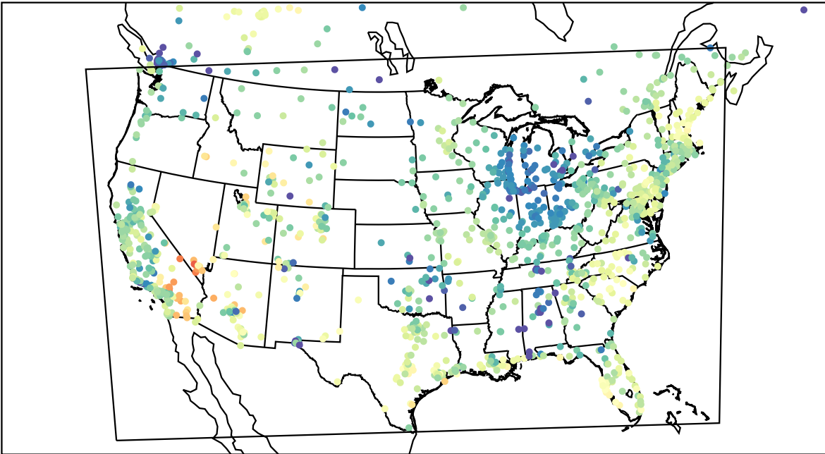
AirNOW (2023-05-01_04:00:00)
