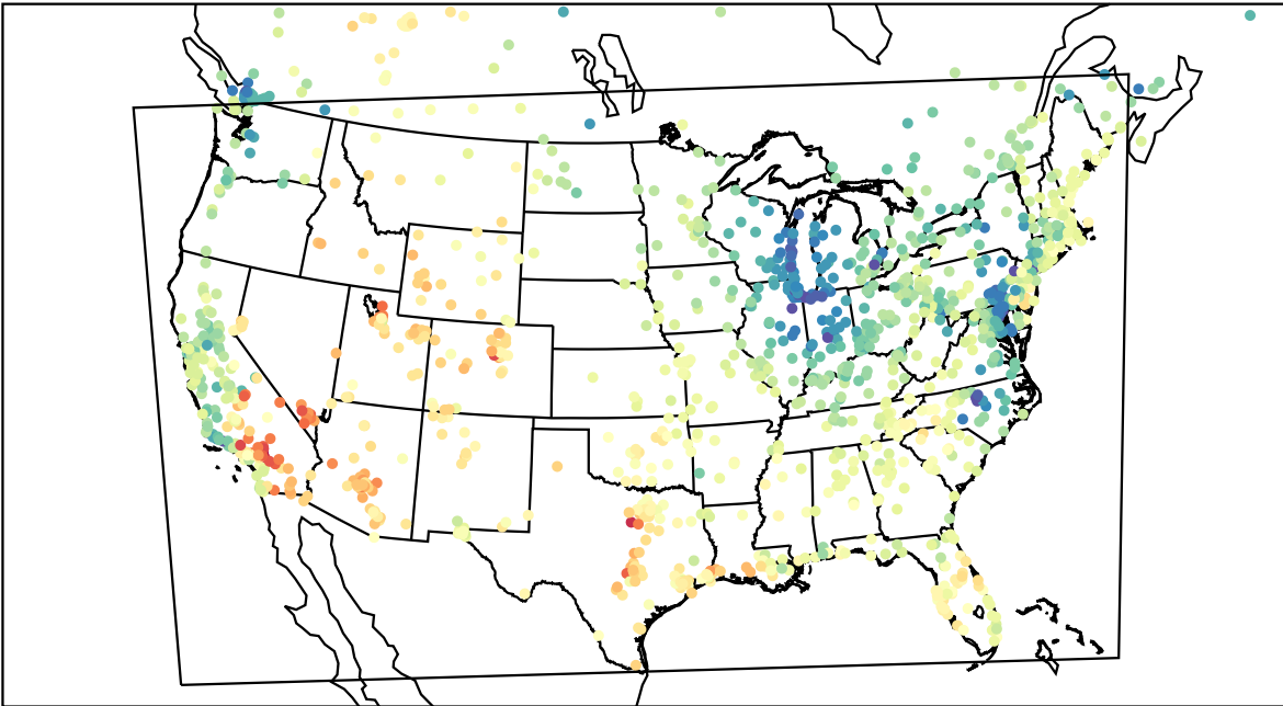
AirNOW (2023-05-01_00:00:00)
