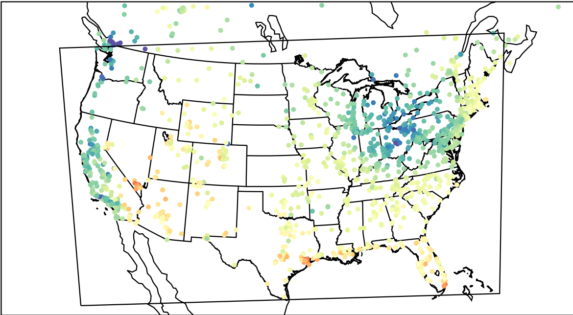
AirNOW (2023-05-01_17:00:00)
