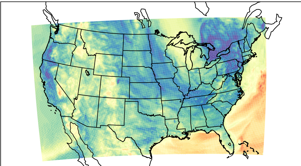
WRF (2023-05-02_08:00:00)
