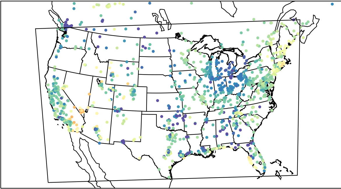
AirNOW (2023-05-01_08:00:00)
