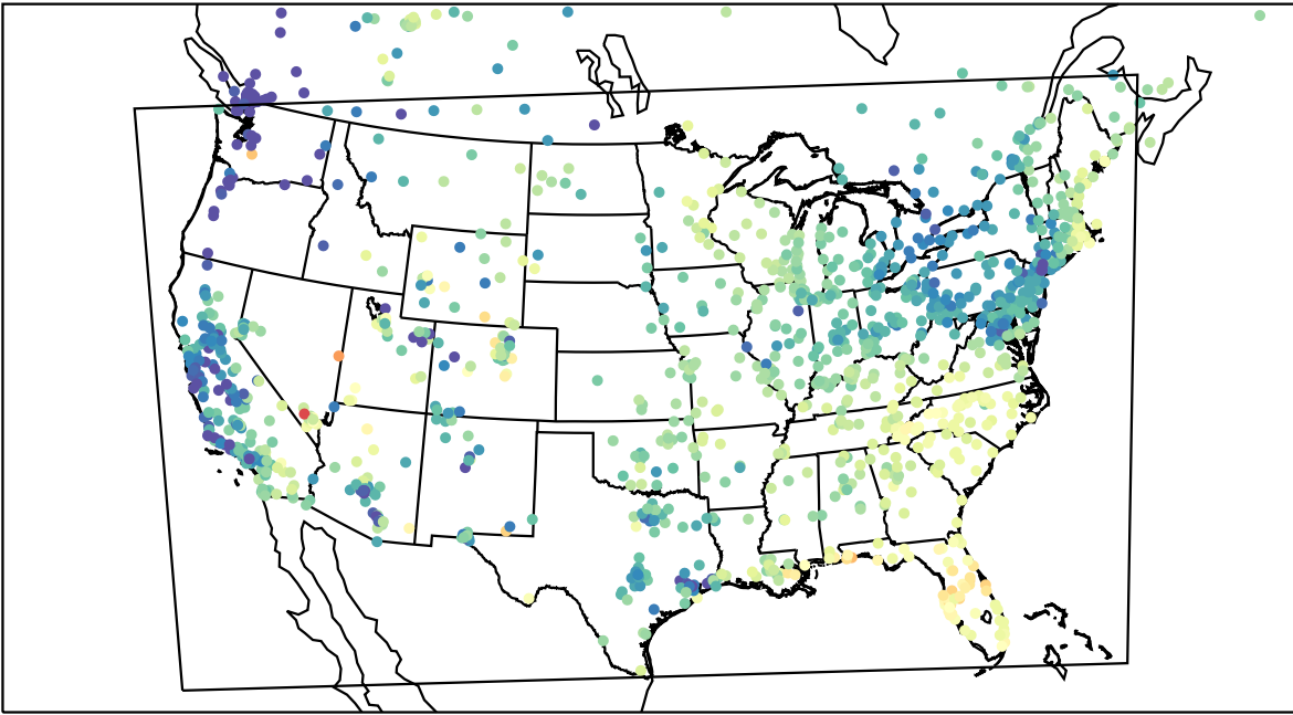
AirNOW (2023-05-02_14:00:00)
