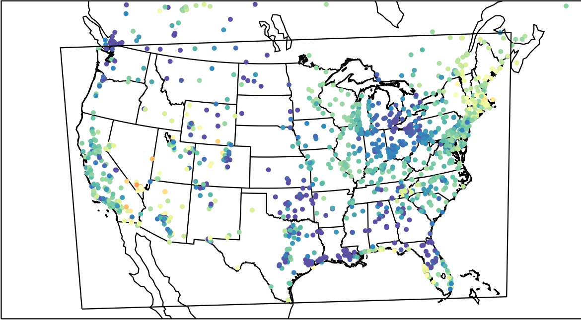
AirNOW (2023-05-01_11:00:00)
