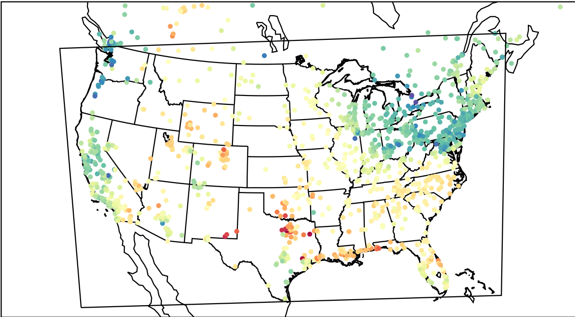
AirNOW (2023-05-02_21:00:00)
