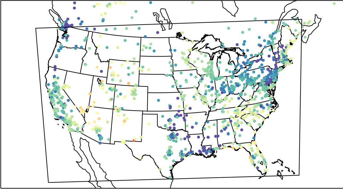
AirNOW (2023-05-02_05:00:00)
