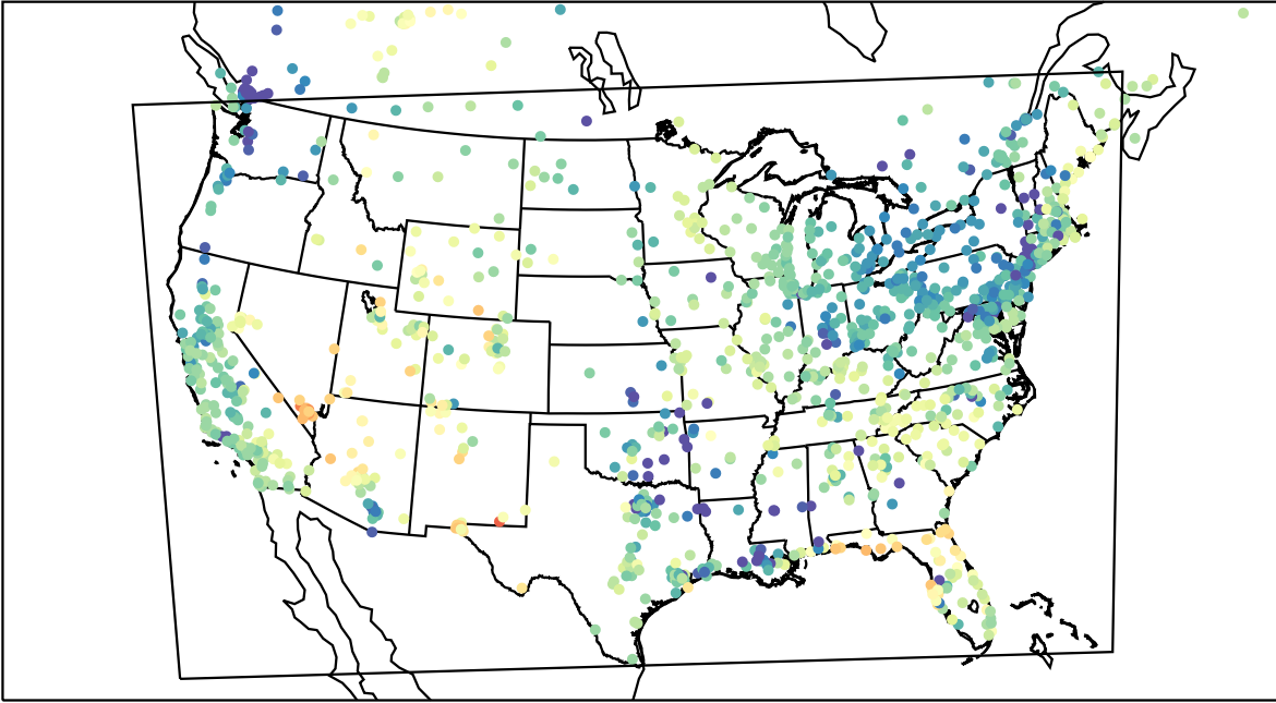
AirNOW (2023-05-02_03:00:00)
