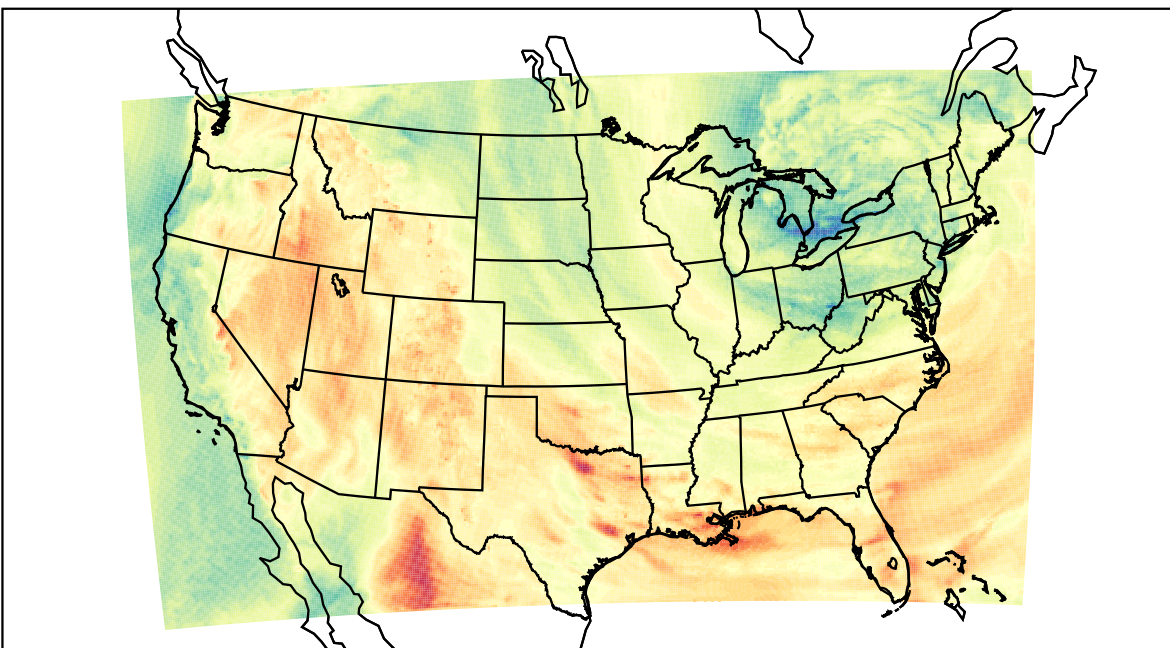
WRF (2023-05-02_21:00:00)
