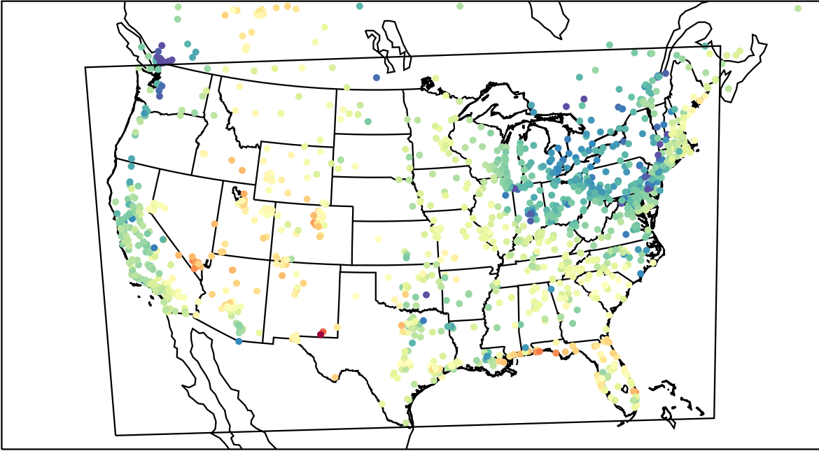
AirNOW (2023-05-02_01:00:00)
