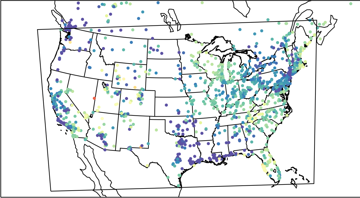
AirNOW (2023-05-02_12:00:00)
