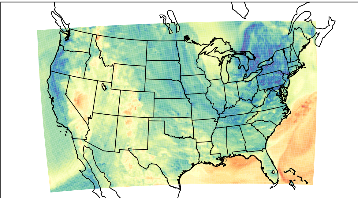
WRF (2023-05-02_03:00:00)
