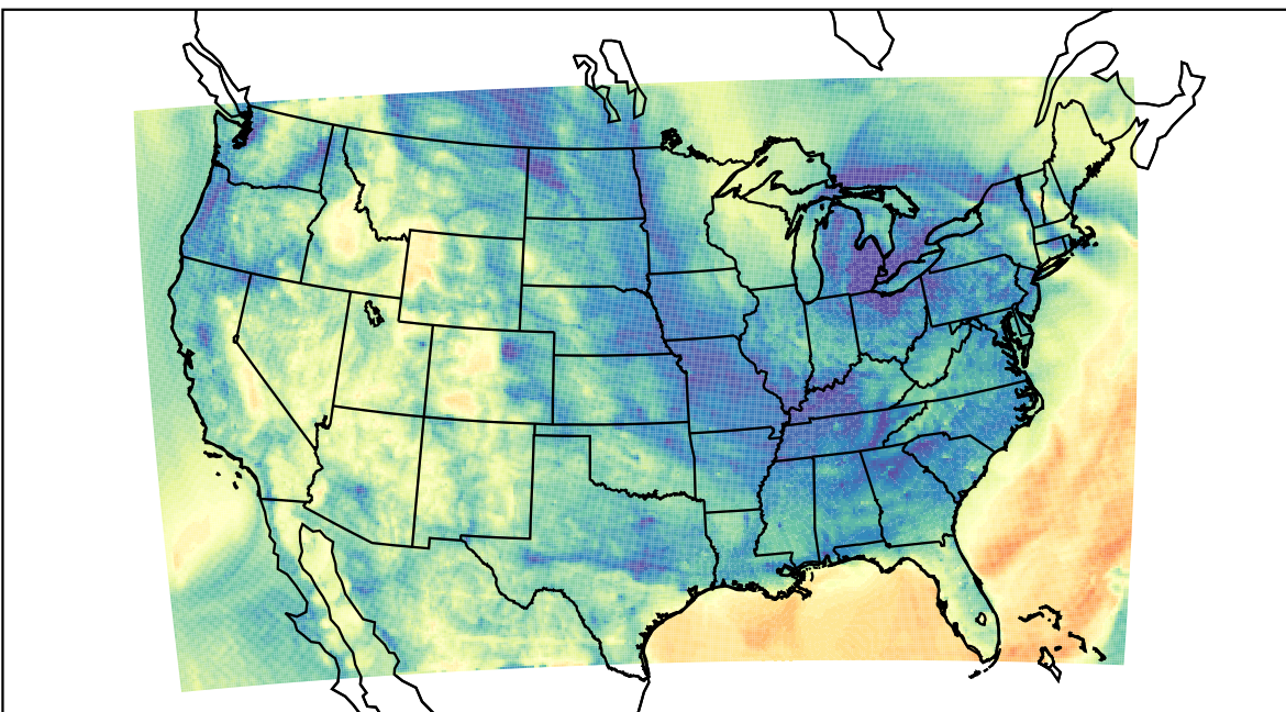
WRF (2023-05-01_11:00:00)
