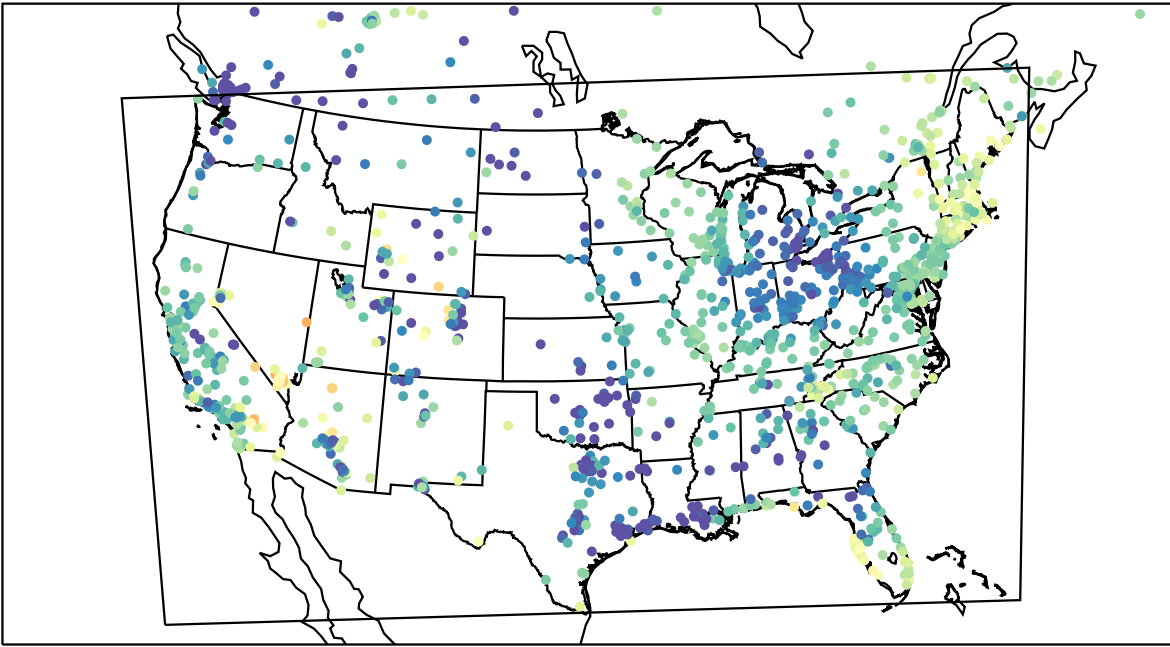
AirNOW (2023-05-01_12:00:00)
