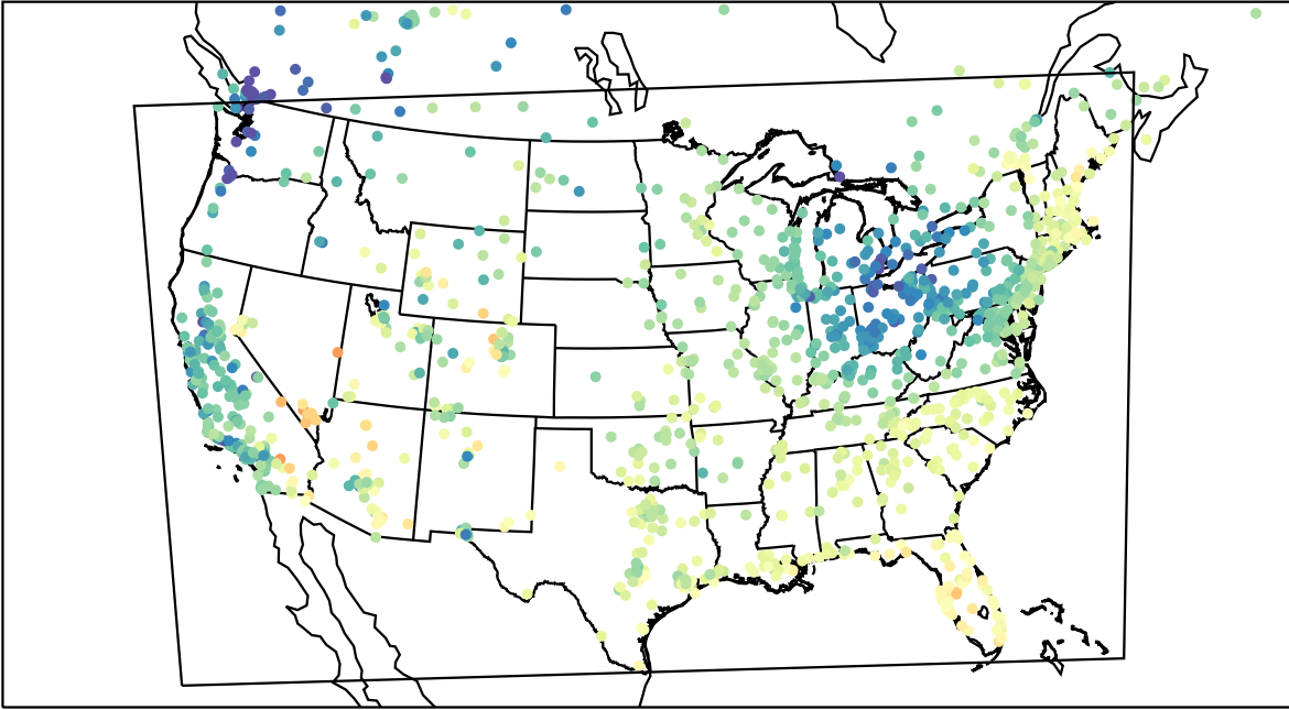
AirNOW (2023-05-01_15:00:00)
