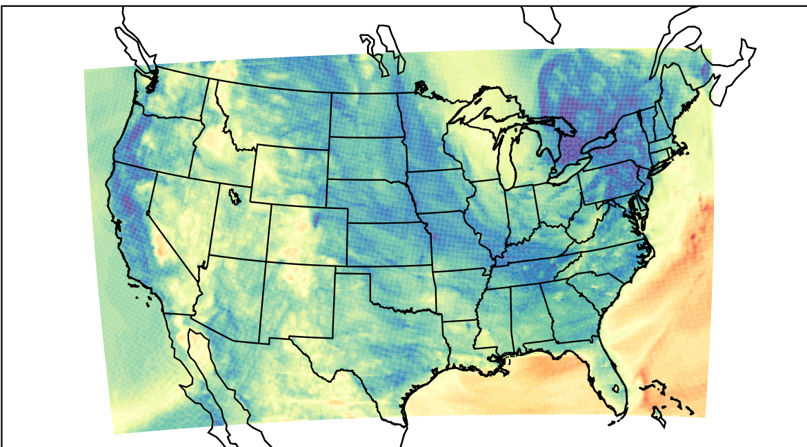
WRF (2023-05-02_07:00:00)
