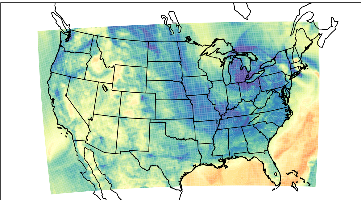
WRF (2023-05-01_09:00:00)
