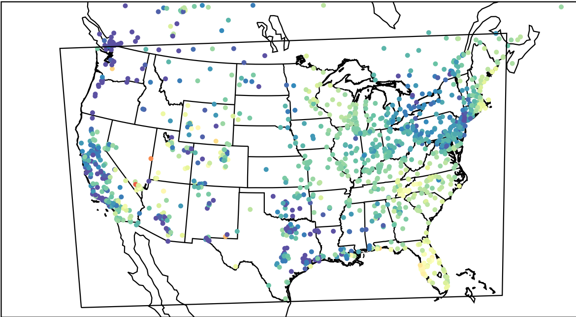
AirNOW (2023-05-02_13:00:00)
