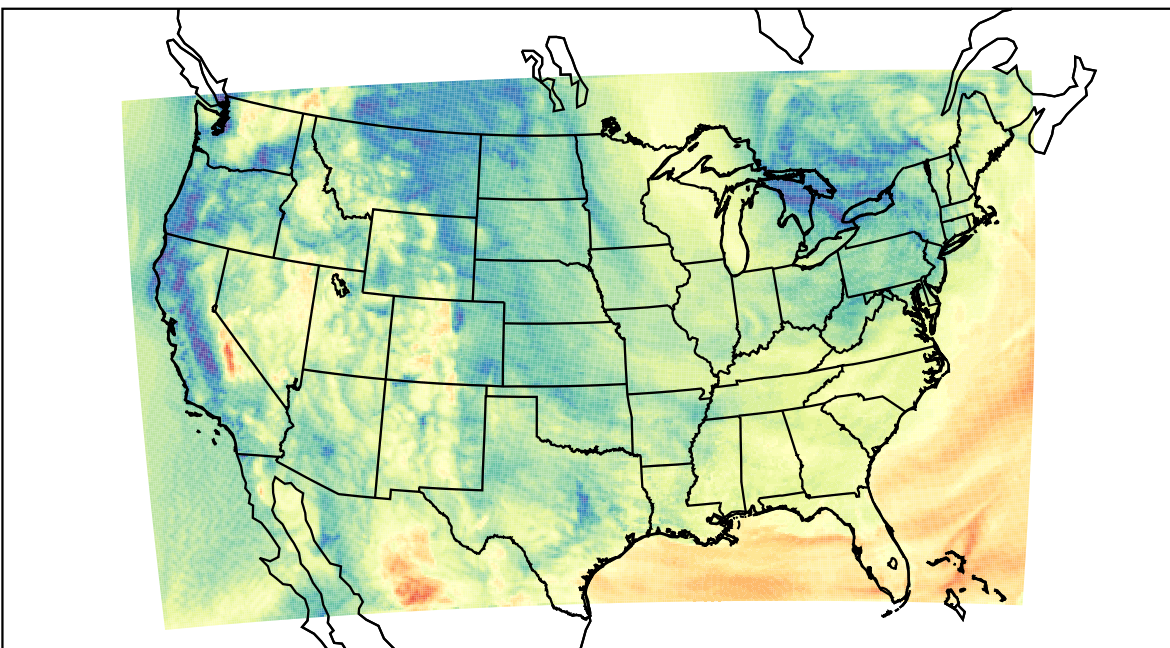
WRF (2023-05-02_15:00:00)
