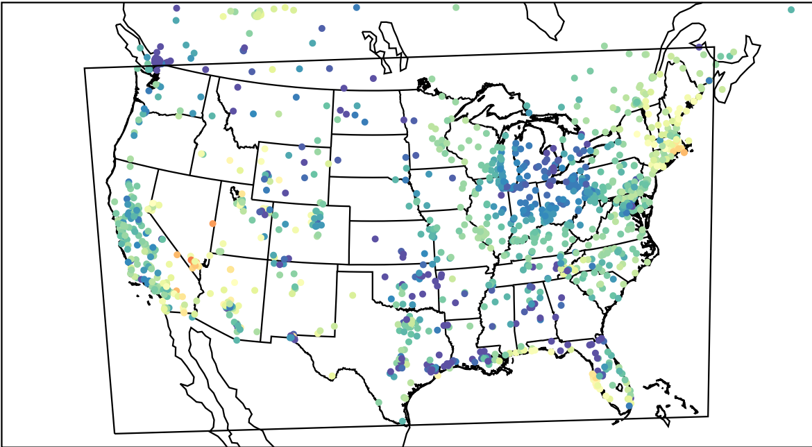
AirNOW (2023-05-01_09:00:00)
