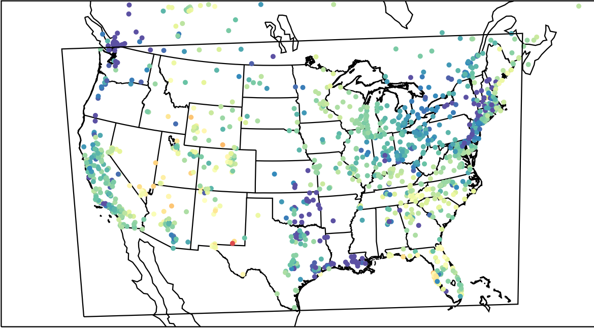
AirNOW (2023-05-02_06:00:00)
