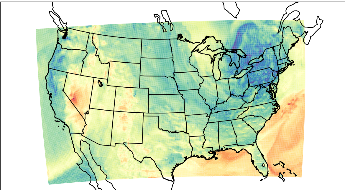
WRF (2023-05-02_02:00:00)
