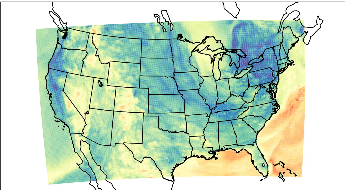
WRF (2023-05-02_05:00:00)
