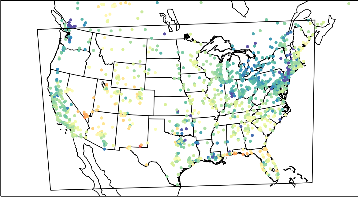
AirNOW (2023-05-02_02:00:00)
