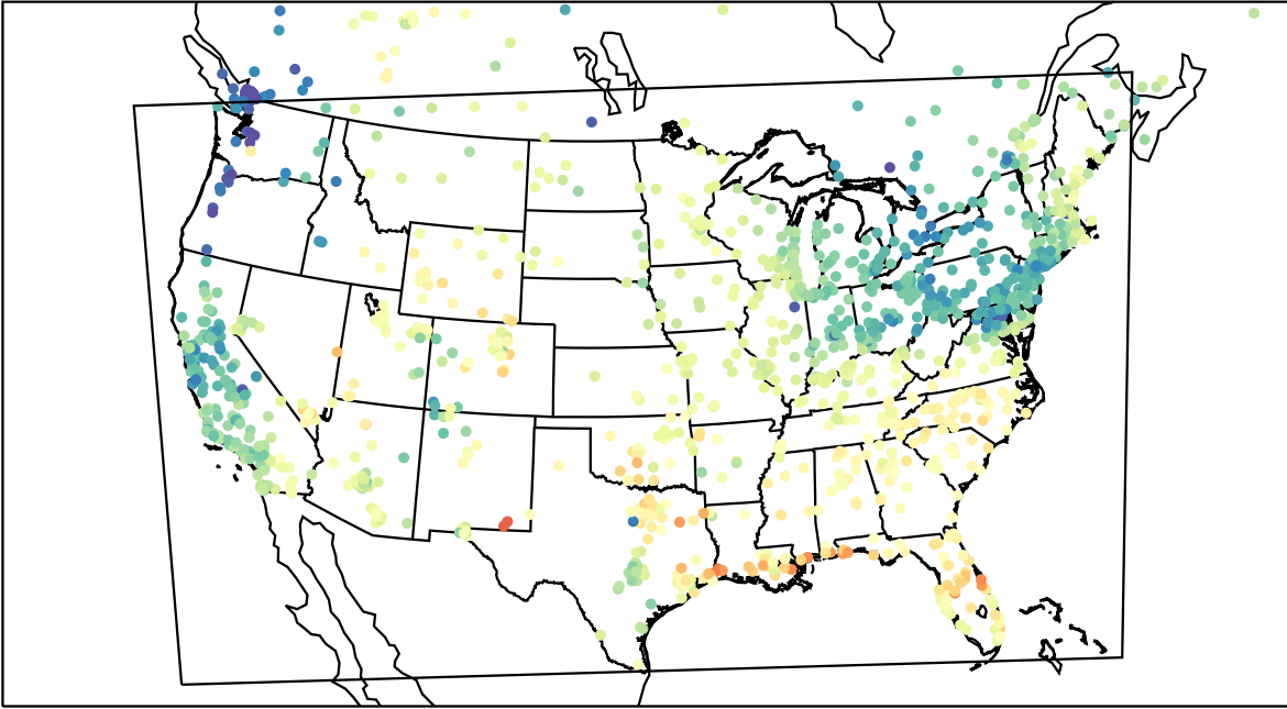
AirNOW (2023-05-02_17:00:00)
