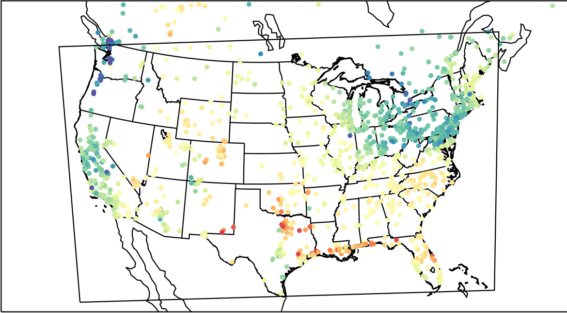
AirNOW (2023-05-02_19:00:00)
