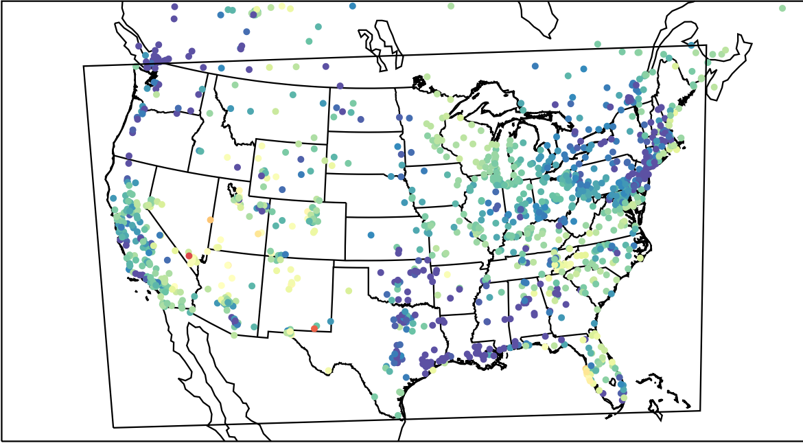
AirNOW (2023-05-02_09:00:00)
