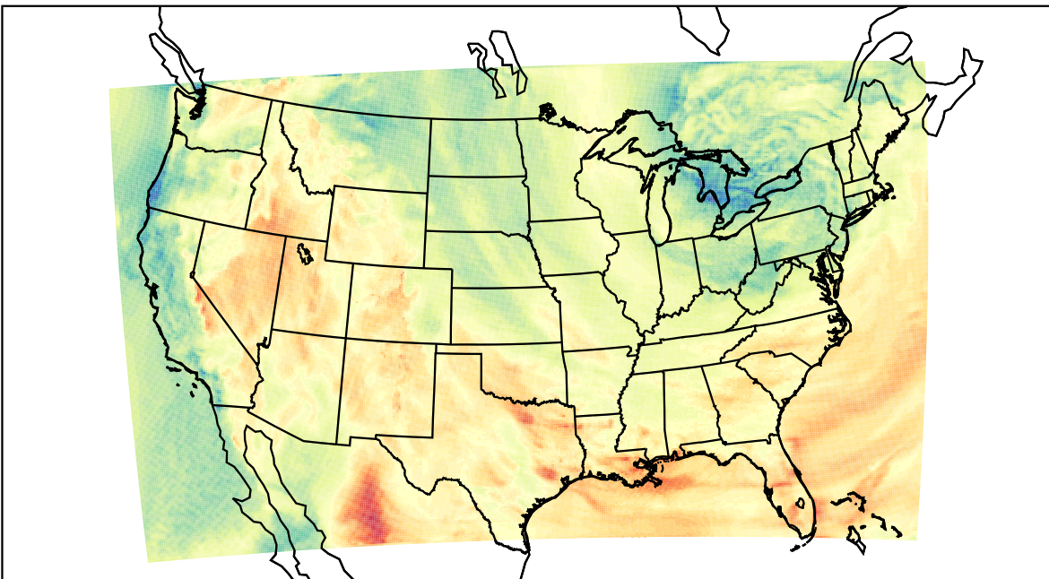
WRF (2023-05-02_19:00:00)
