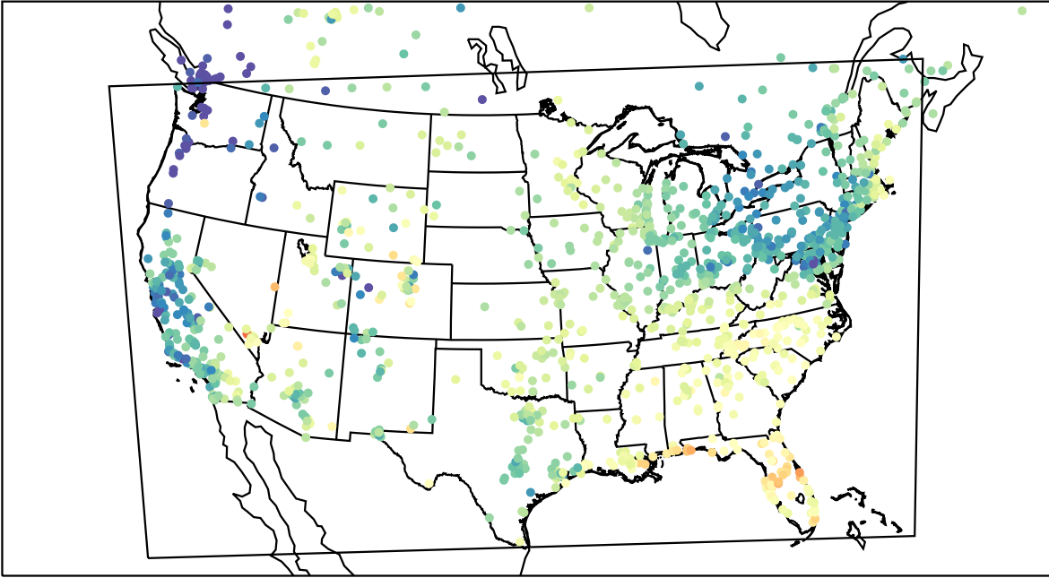
AirNOW (2023-05-02_15:00:00)
