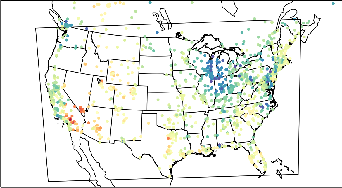
AirNOW (2023-05-01_01:00:00)
