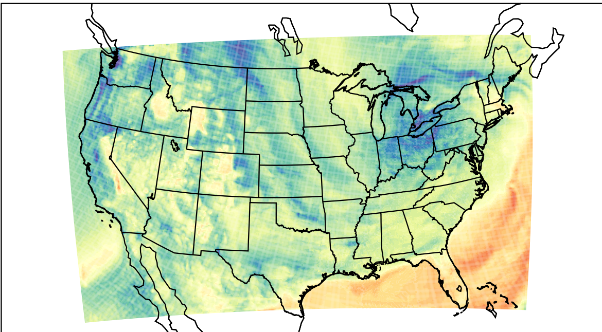
WRF (2023-05-01_15:00:00)
