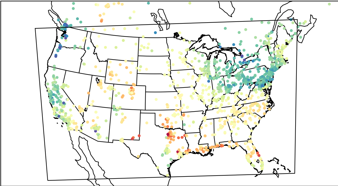
AirNOW (2023-05-02_20:00:00)
