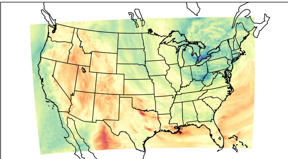
WRF (2023-05-02_23:00:00)
