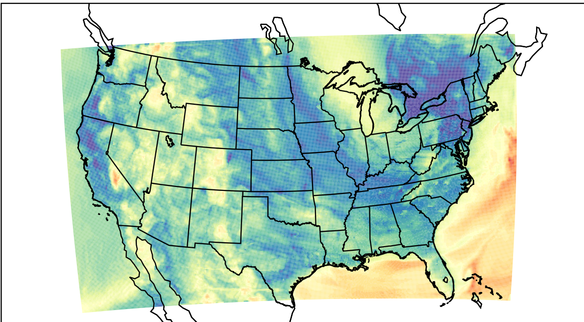
WRF (2023-05-02_10:00:00)
