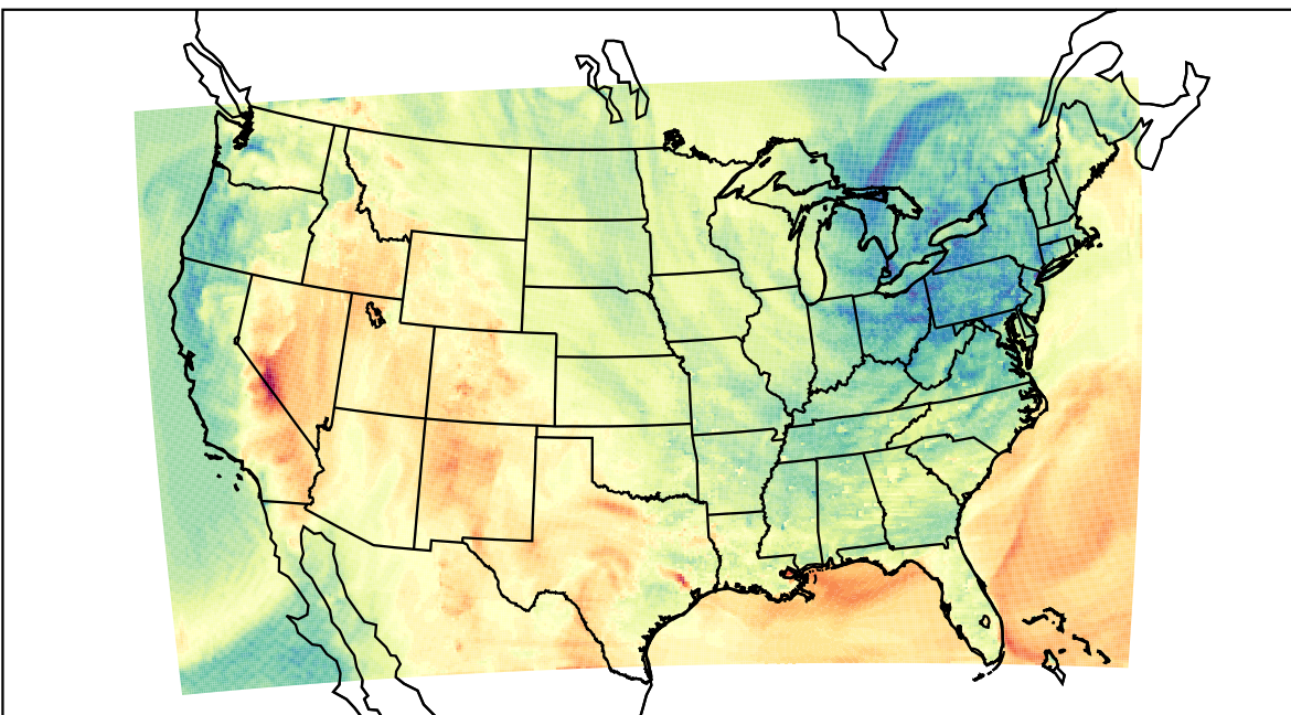
WRF (2023-05-02_00:00:00)
