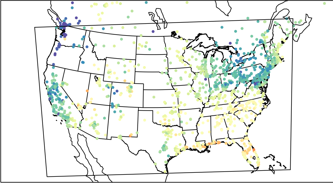
AirNOW (2023-05-02_16:00:00)
