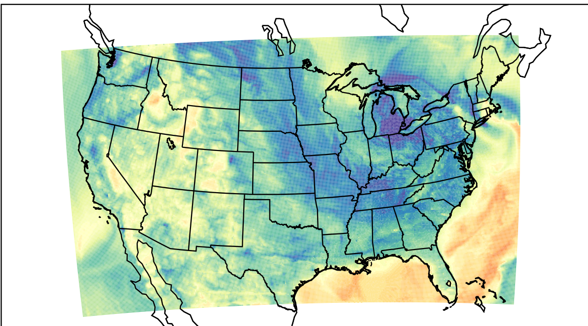
WRF (2023-05-01_08:00:00)
