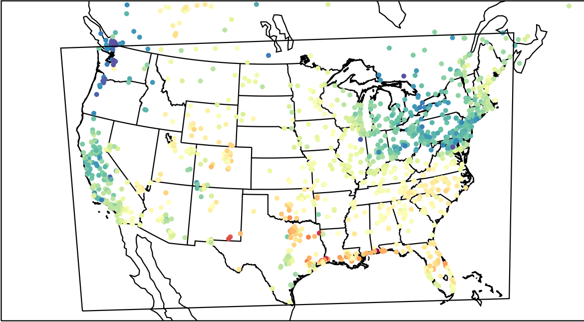
AirNOW (2023-05-02_18:00:00)
