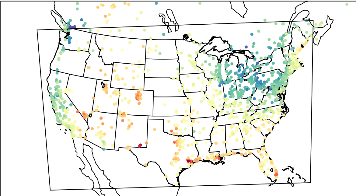
AirNOW (2023-05-01_23:00:00)
