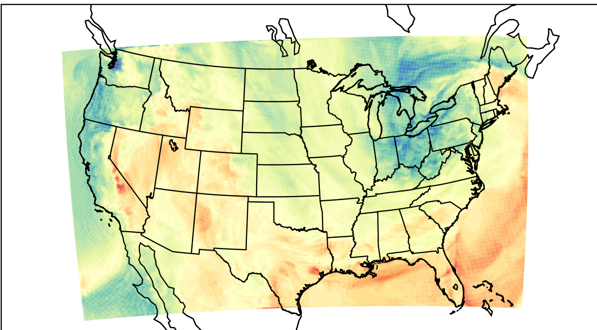
WRF (2023-05-01_19:00:00)
