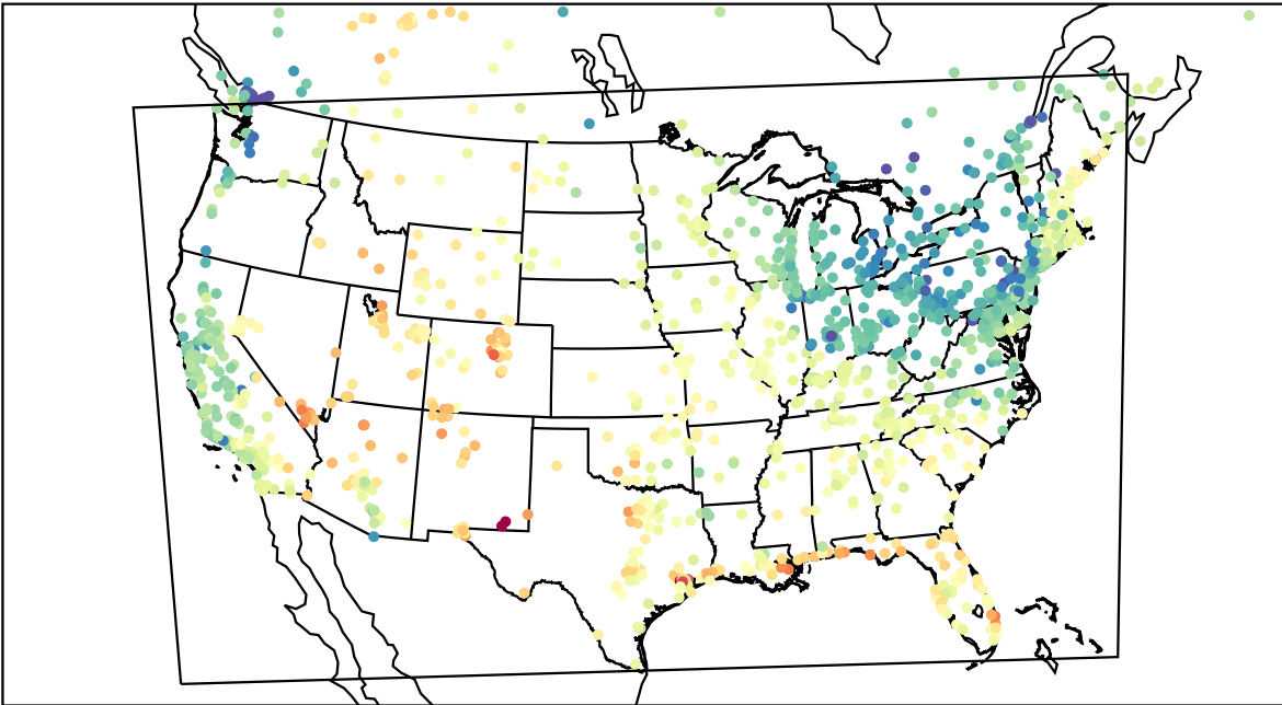
AirNOW (2023-05-02_00:00:00)
