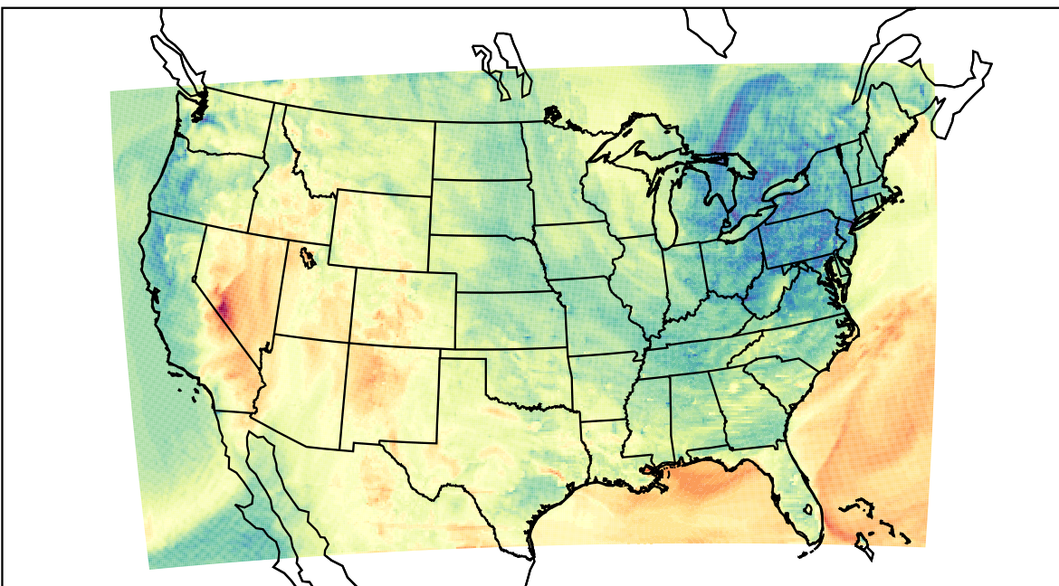
WRF (2023-05-02_01:00:00)
