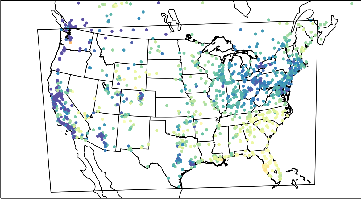
AirNOW (2023-05-03_14:00:00)
