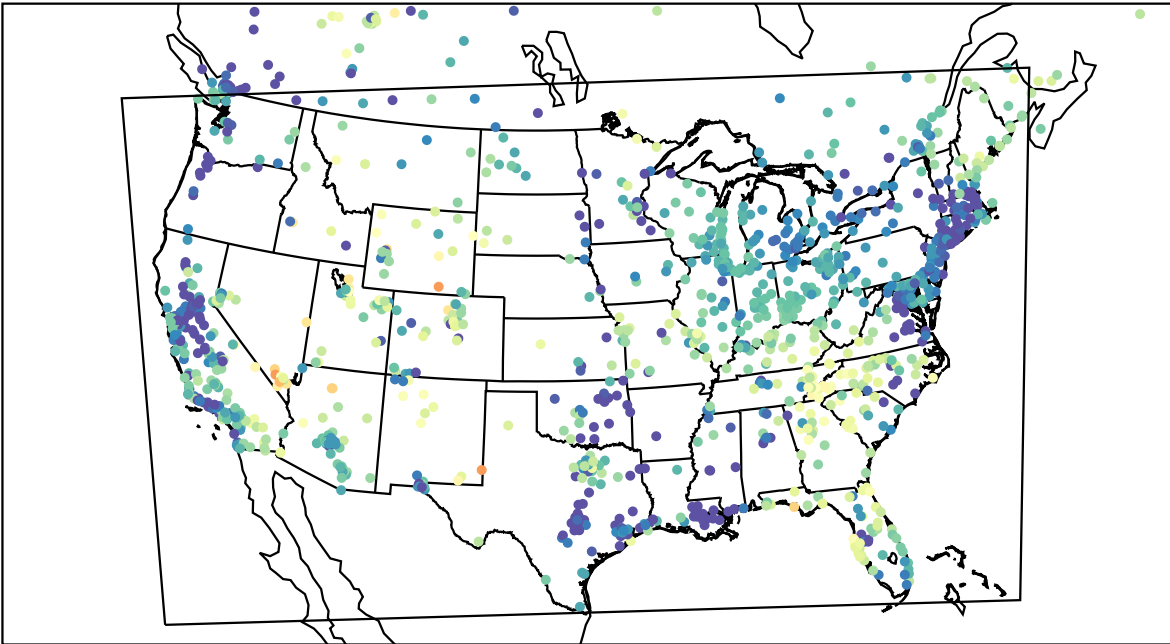
AirNOW (2023-05-03_06:00:00)
