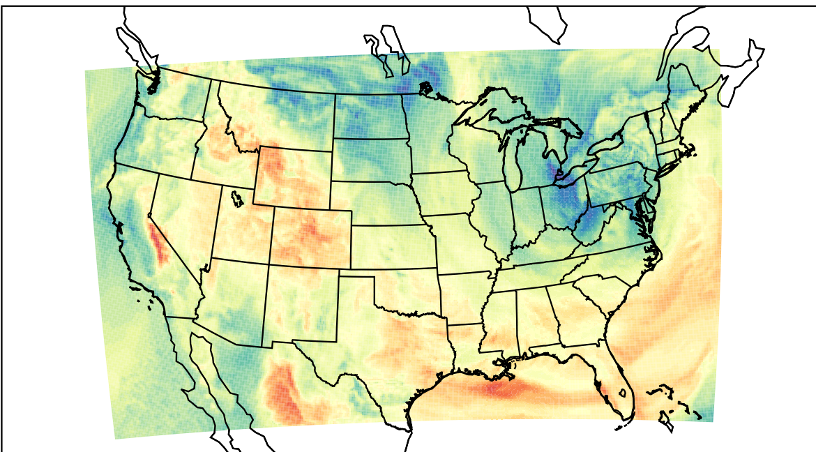
WRF (2023-05-03_17:00:00)
