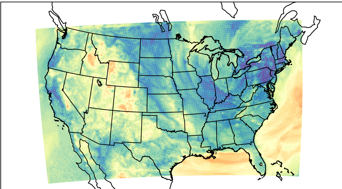
WRF (2023-05-03_08:00:00)
