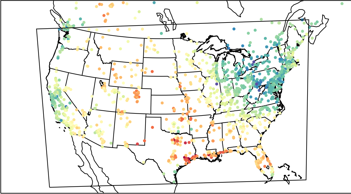
AirNOW (2023-05-03_21:00:00)
