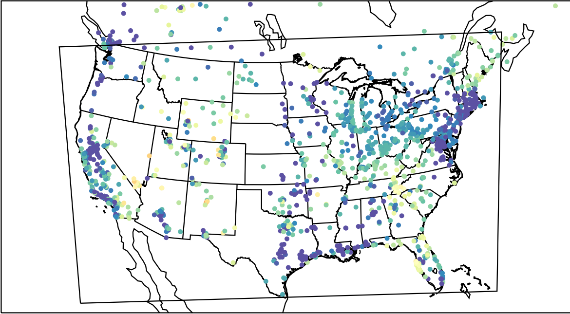
AirNOW (2023-05-03_08:00:00)
