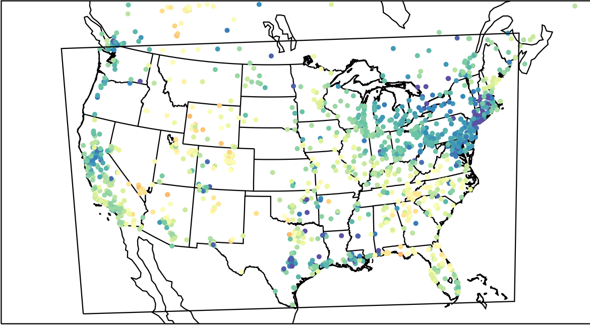
AirNOW (2023-05-03_02:00:00)
