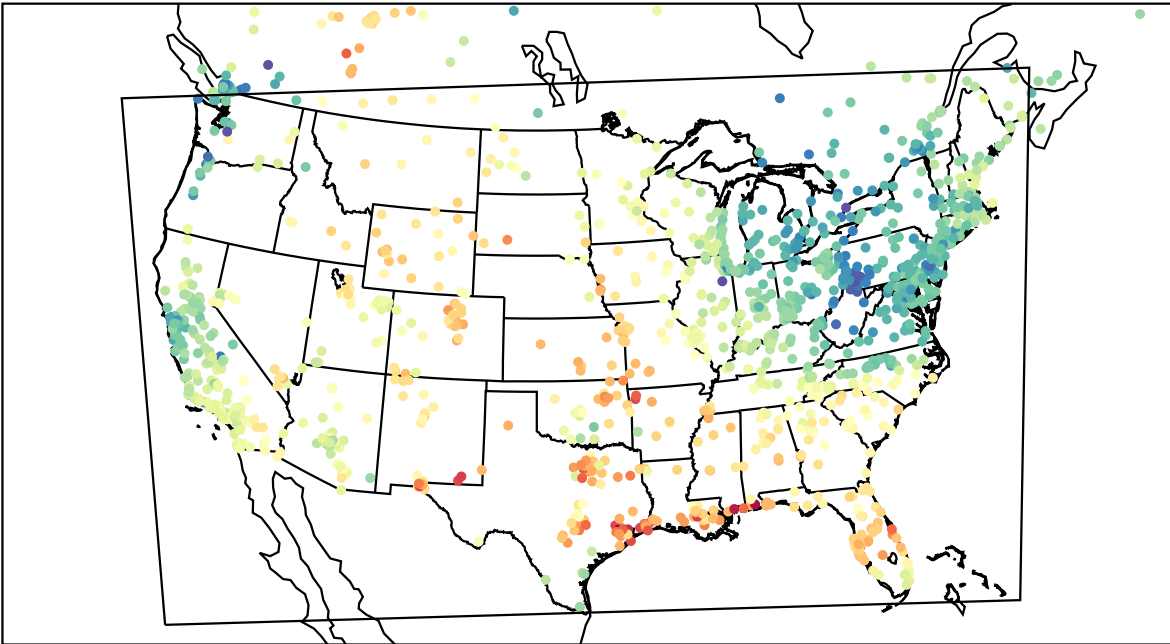
AirNOW (2023-05-03_19:00:00)
