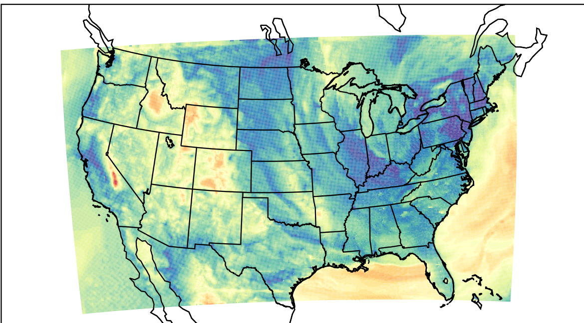
WRF (2023-05-03_10:00:00)
