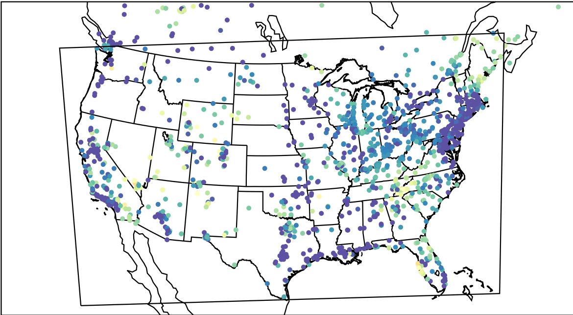
AirNOW (2023-05-03_11:00:00)
