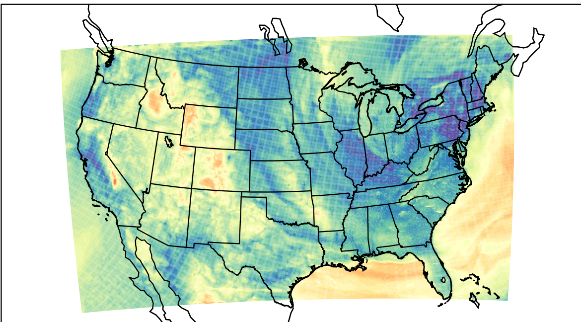
WRF (2023-05-03_09:00:00)
