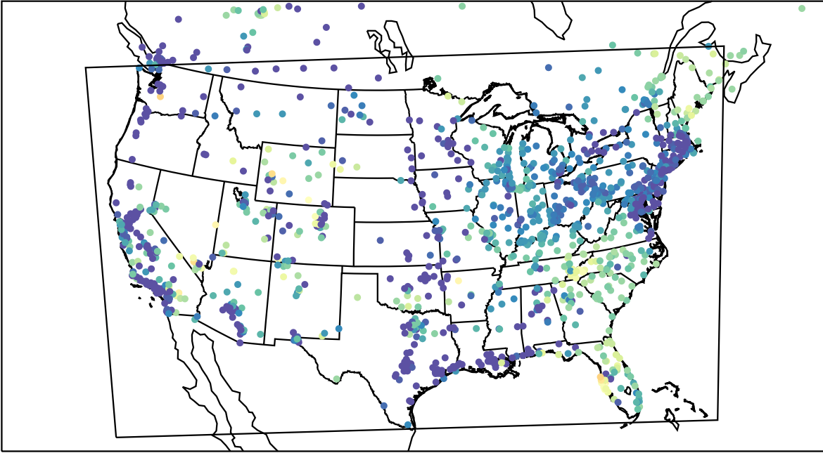
AirNOW (2023-05-03_12:00:00)
