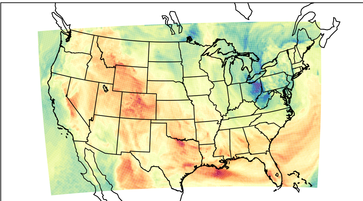
WRF (2023-05-03_20:00:00)
