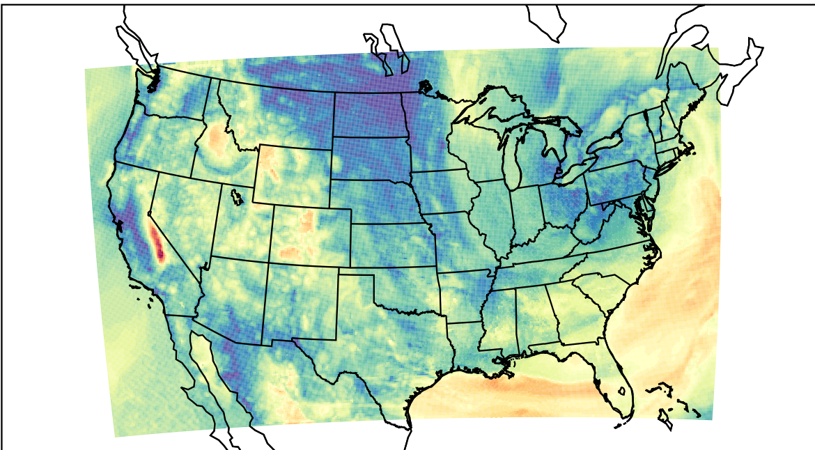
WRF (2023-05-03_14:00:00)
