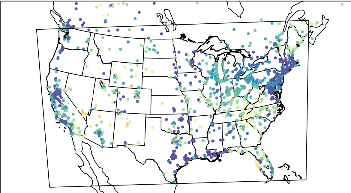
AirNOW (2023-05-03_07:00:00)
