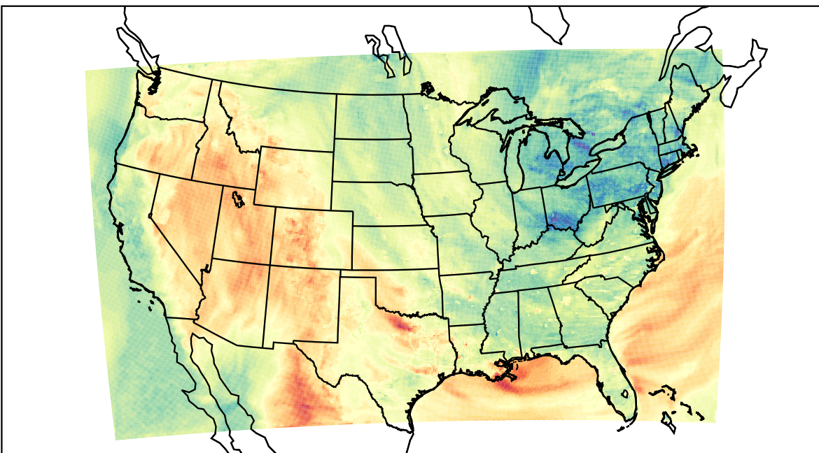
WRF (2023-05-03_00:00:00)
