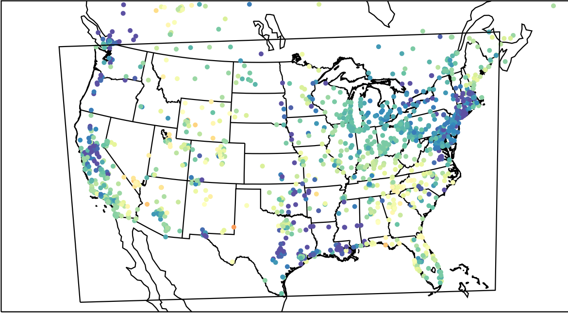
AirNOW (2023-05-03_04:00:00)
