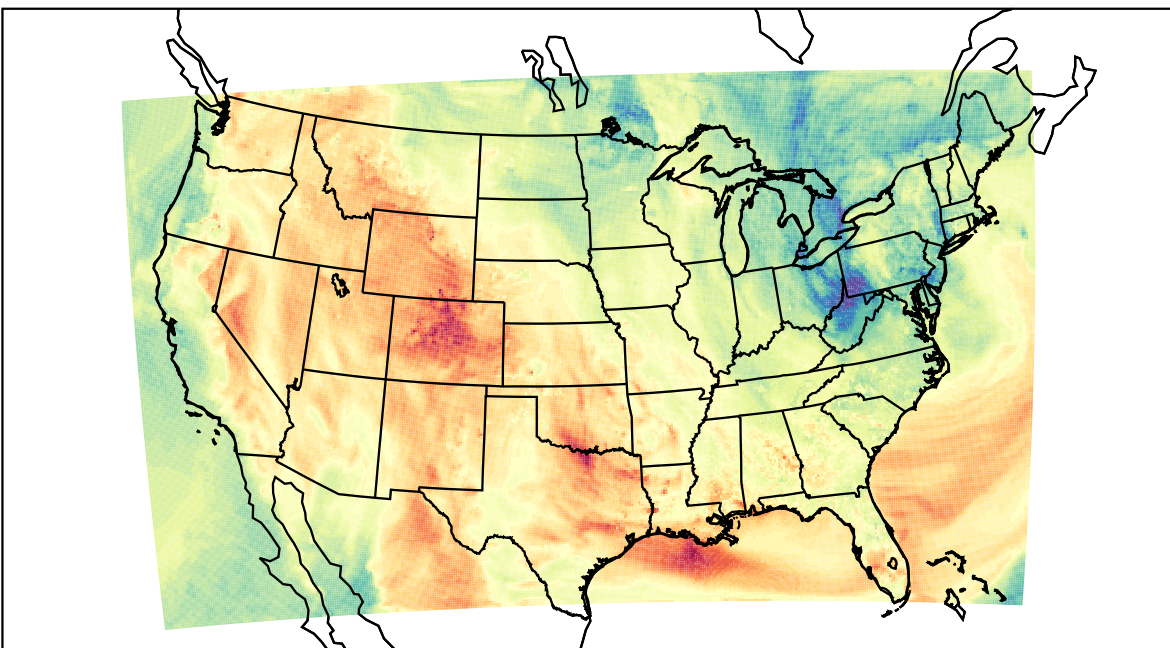
WRF (2023-05-03_23:00:00)
