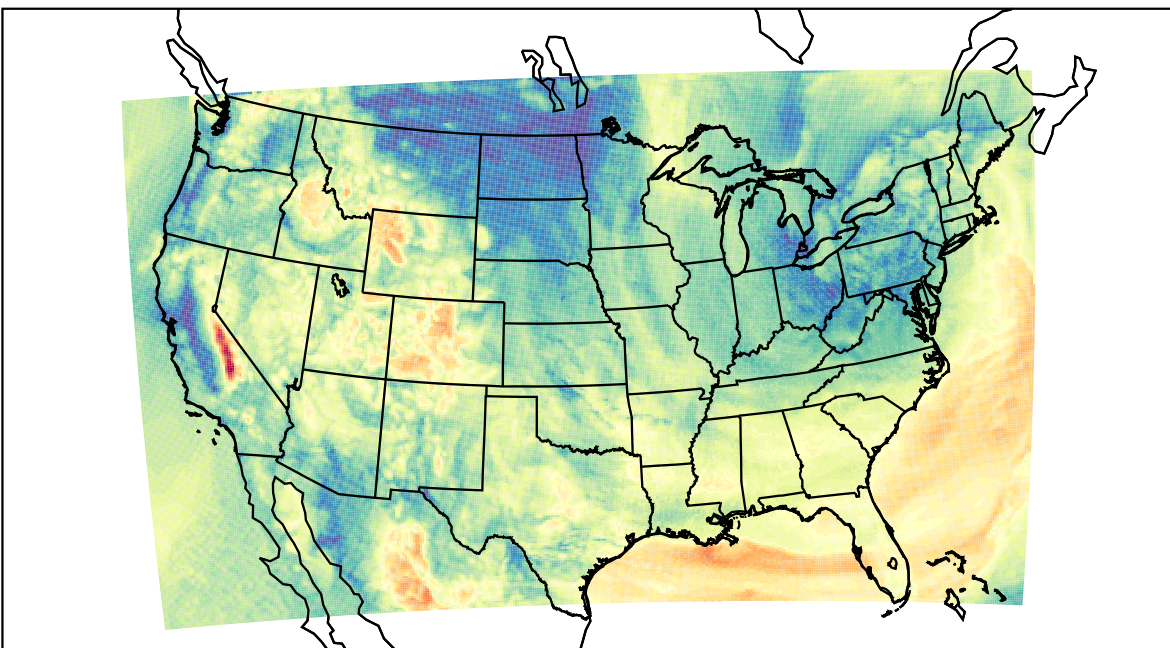
WRF (2023-05-03_15:00:00)
