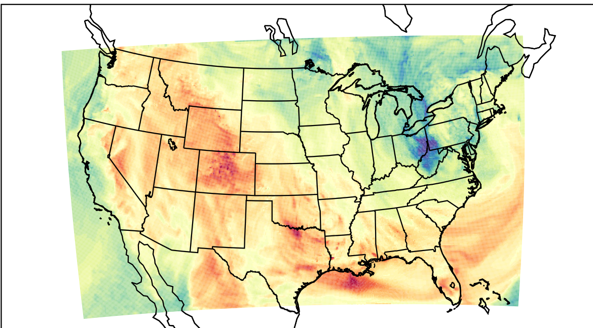
WRF (2023-05-03_22:00:00)
