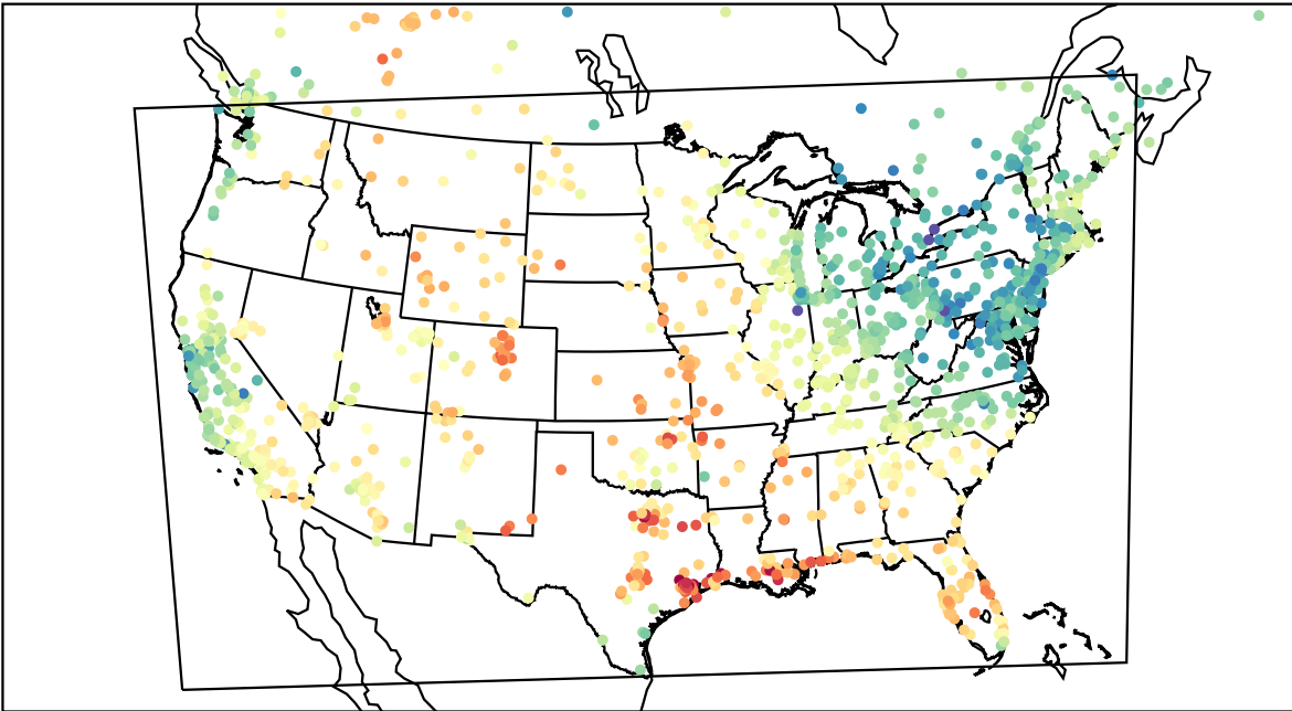
AirNOW (2023-05-03_22:00:00)
