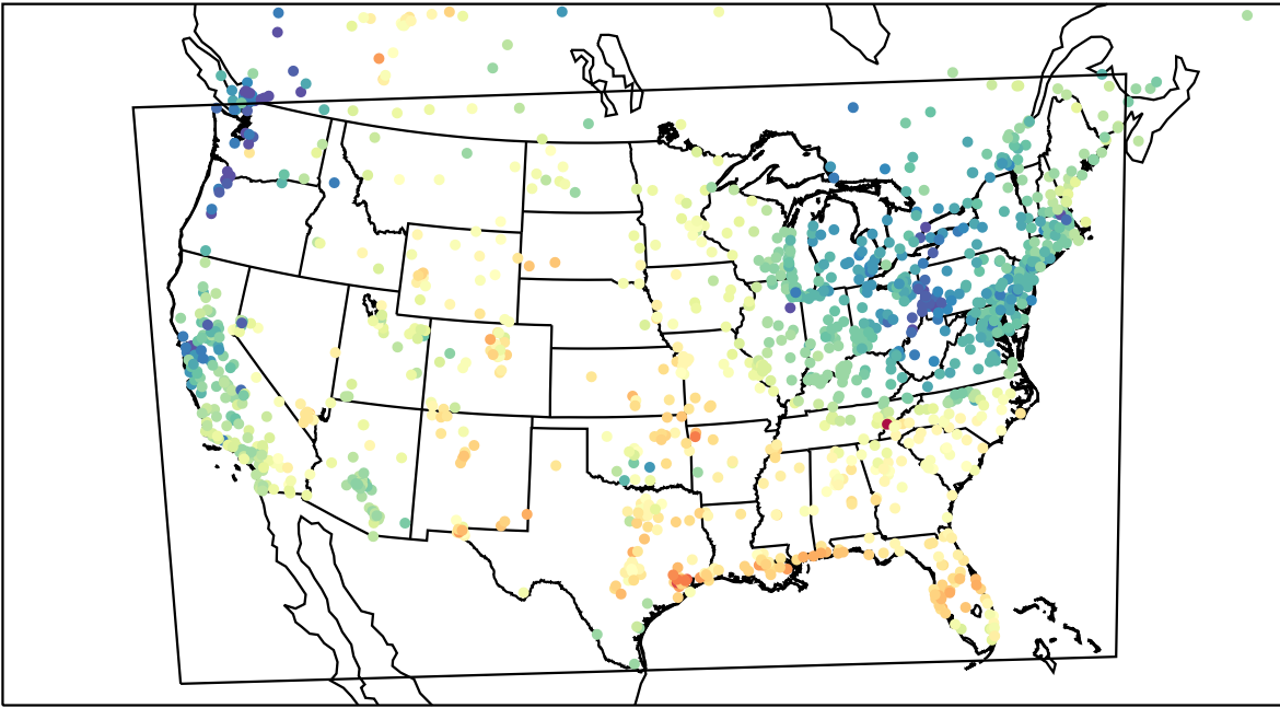
AirNOW (2023-05-03_17:00:00)
