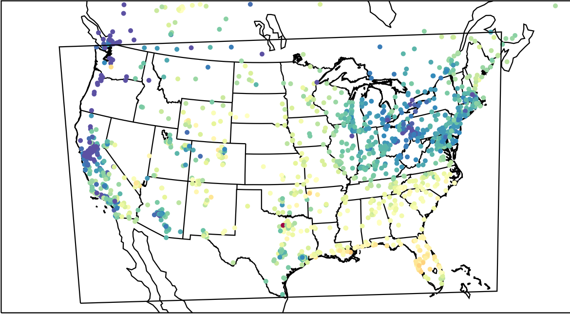
AirNOW (2023-05-03_15:00:00)
