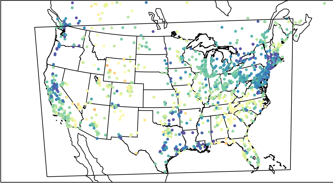
AirNOW (2023-05-03_03:00:00)
