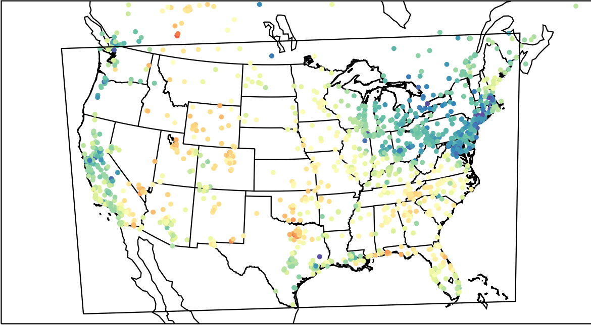
AirNOW (2023-05-03_00:00:00)
