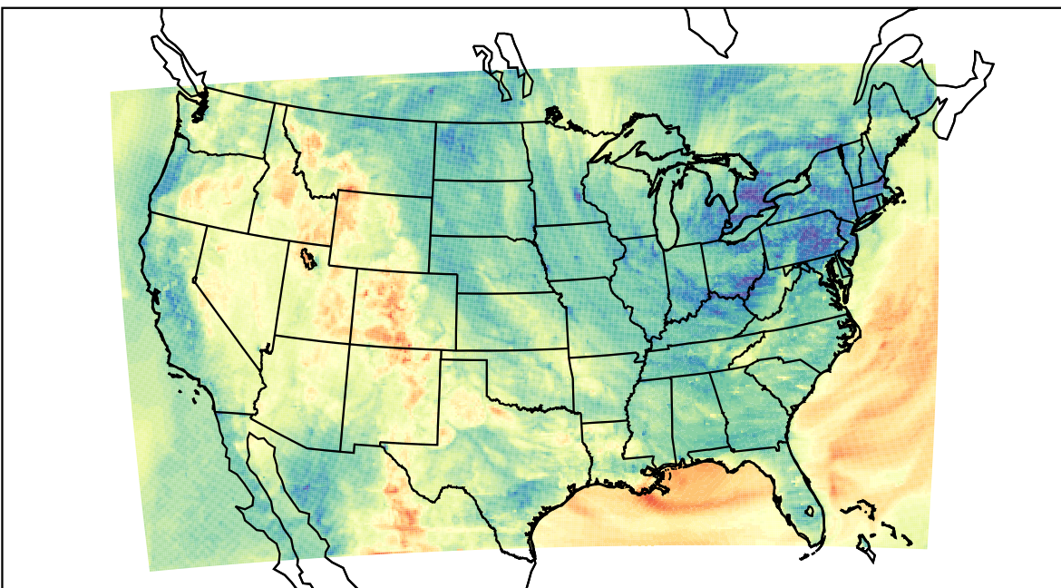
WRF (2023-05-03_03:00:00)
