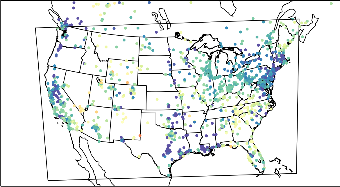
AirNOW (2023-05-03_05:00:00)
