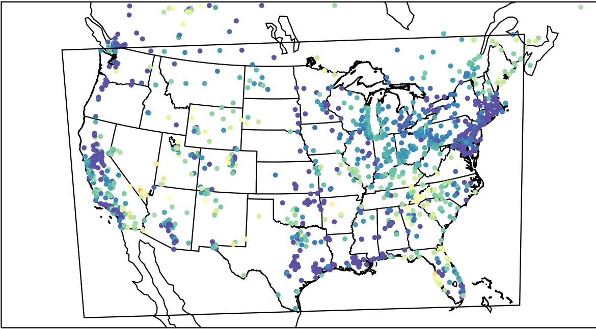
AirNOW (2023-05-03_09:00:00)
