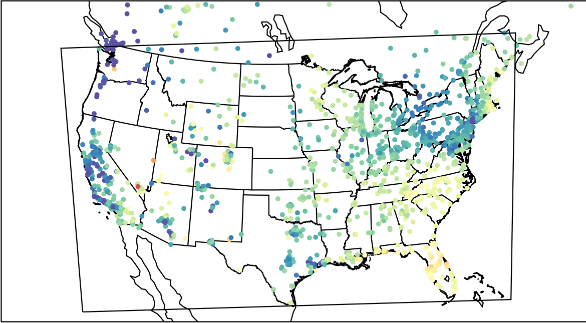
AirNOW (2023-05-02_14:00:00)
