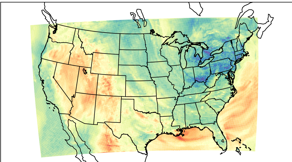
WRF (2023-05-03_01:00:00)
