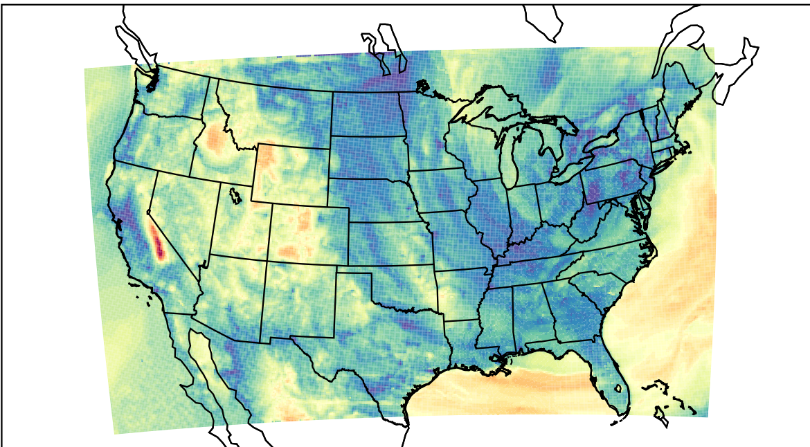
WRF (2023-05-03_12:00:00)
