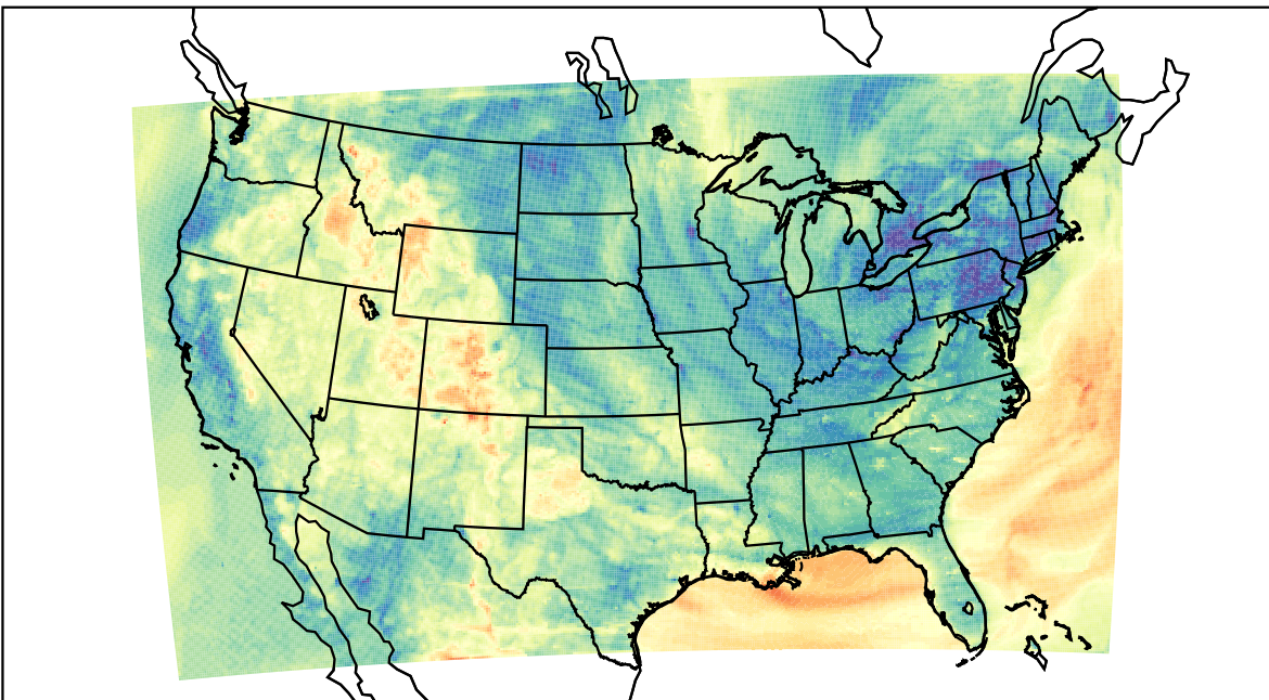
WRF (2023-05-03_05:00:00)
