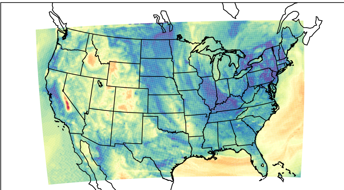
WRF (2023-05-03_11:00:00)
