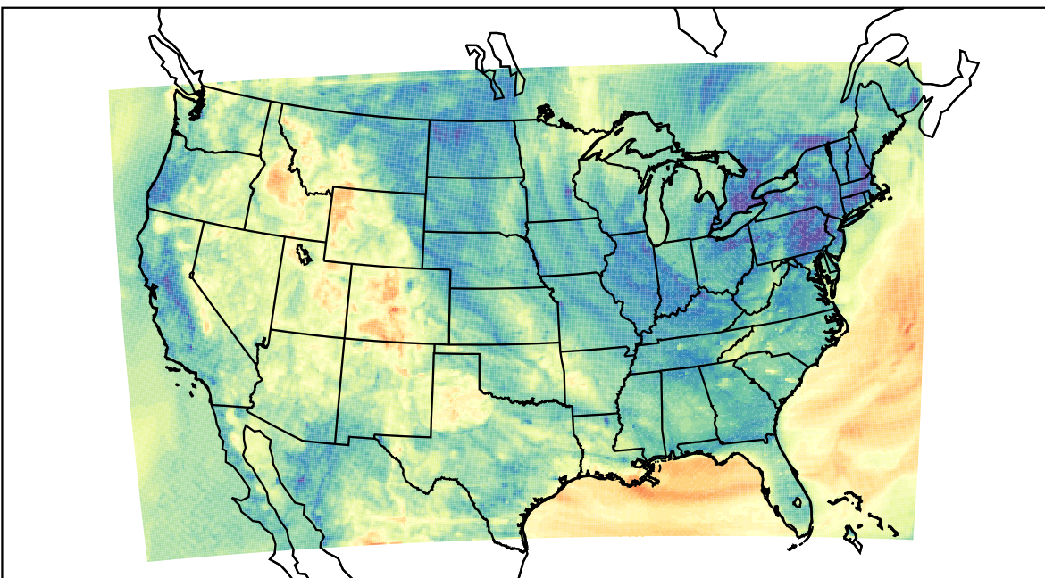
WRF (2023-05-03_06:00:00)
