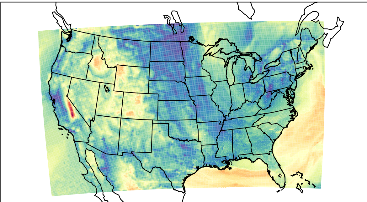
WRF (2023-05-03_13:00:00)
