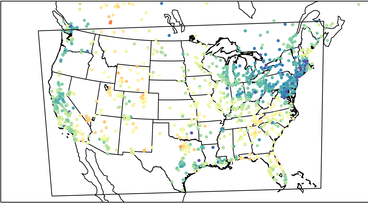
AirNOW (2023-05-03_01:00:00)
