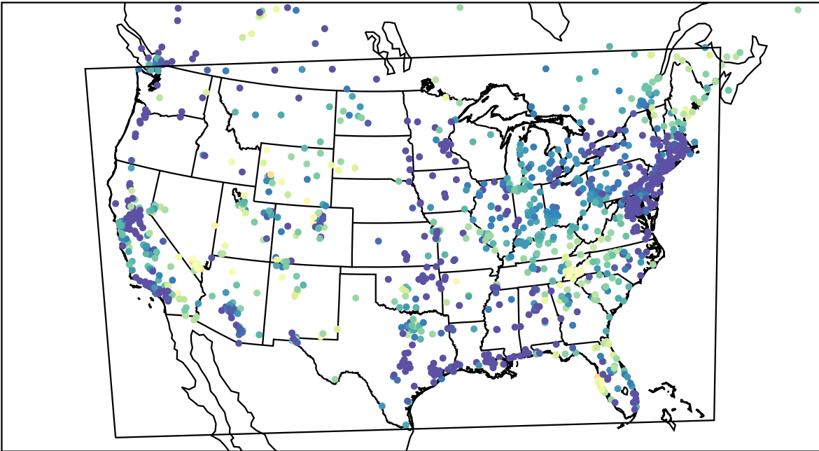
AirNOW (2023-05-03_10:00:00)
