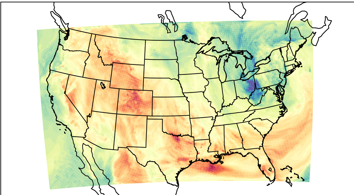
WRF (2023-05-03_21:00:00)
