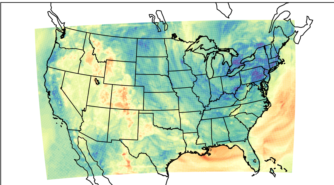
WRF (2023-05-03_04:00:00)
