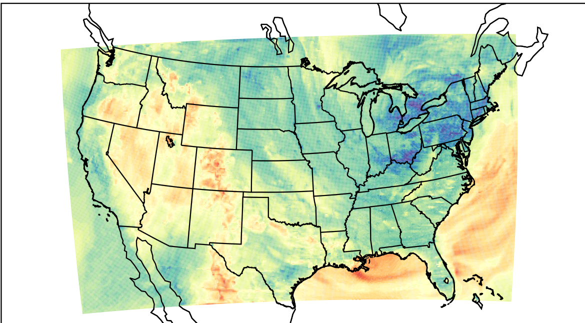
WRF (2023-05-03_02:00:00)
