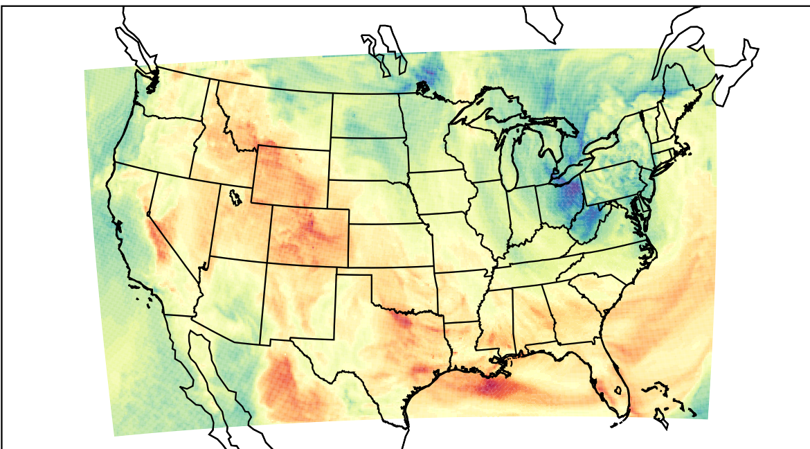
WRF (2023-05-03_19:00:00)
