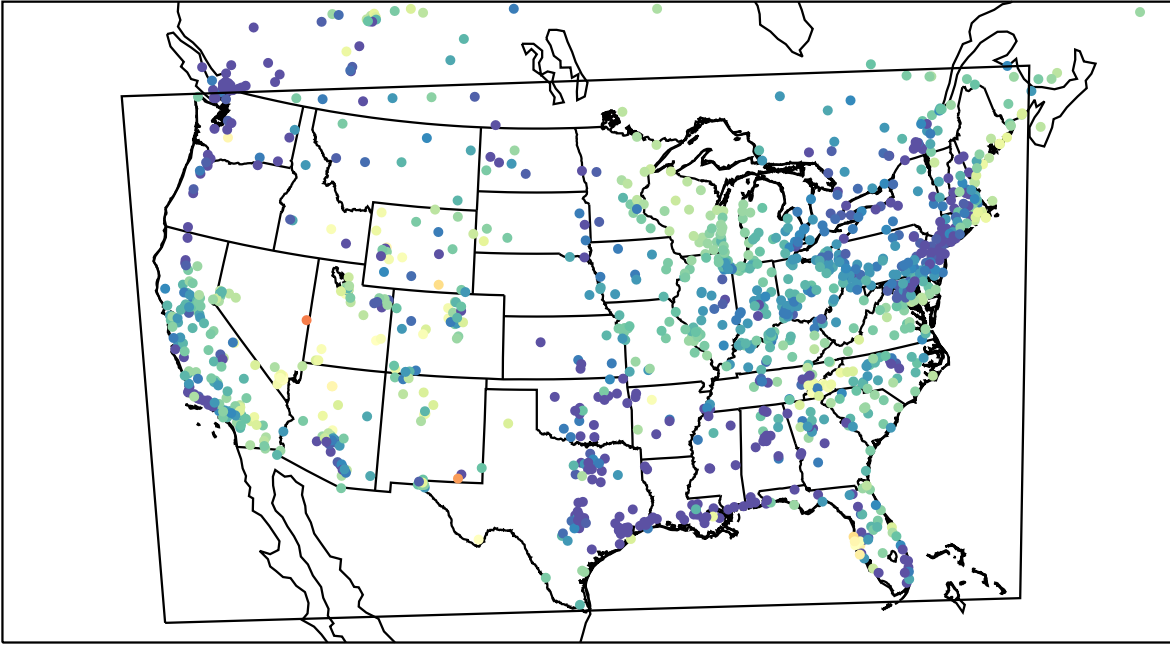
AirNOW (2023-05-02_11:00:00)
