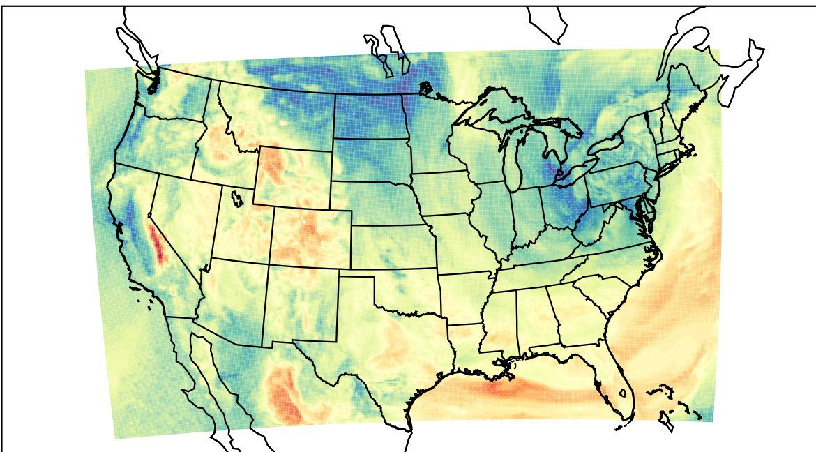
WRF (2023-05-03_16:00:00)
