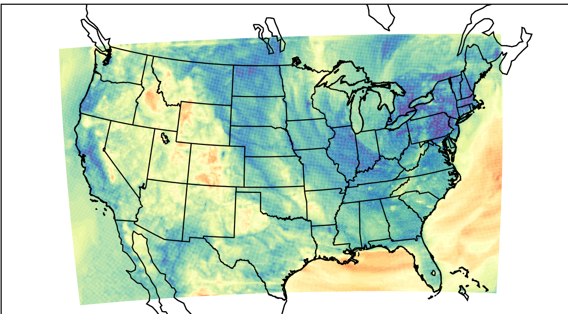
WRF (2023-05-03_07:00:00)
