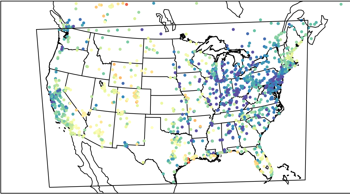
AirNOW (2023-05-04_03:00:00)
