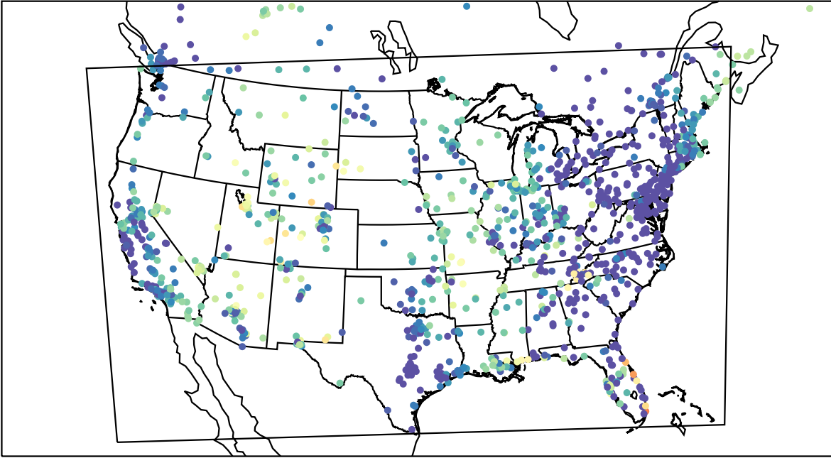
AirNOW (2023-05-05_10:00:00)
