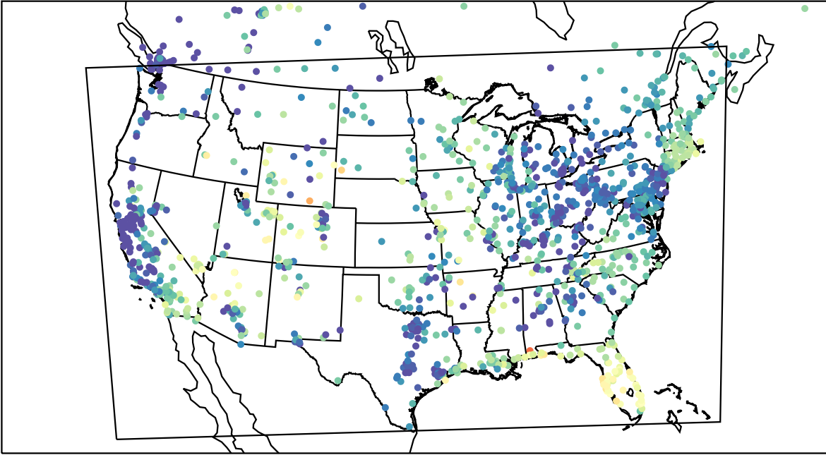
AirNOW (2023-05-04_13:00:00)
