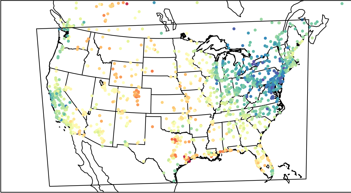
AirNOW (2023-05-04_00:00:00)
