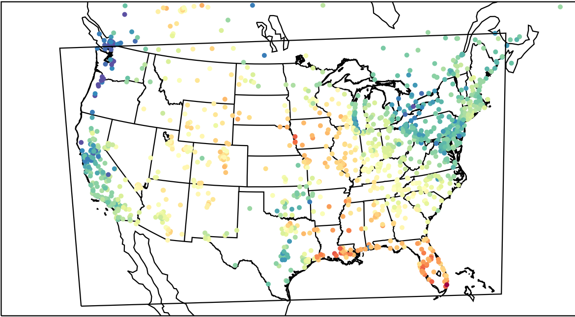
AirNOW (2023-05-04_17:00:00)
