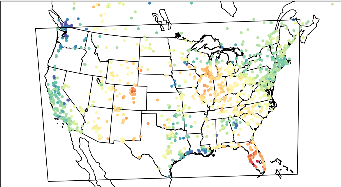
AirNOW (2023-05-05_18:00:00)
