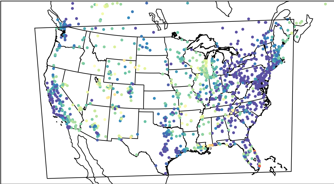
AirNOW (2023-05-05_09:00:00)
