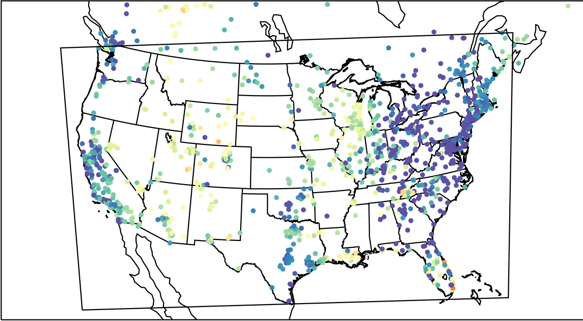
AirNOW (2023-05-05_06:00:00)
