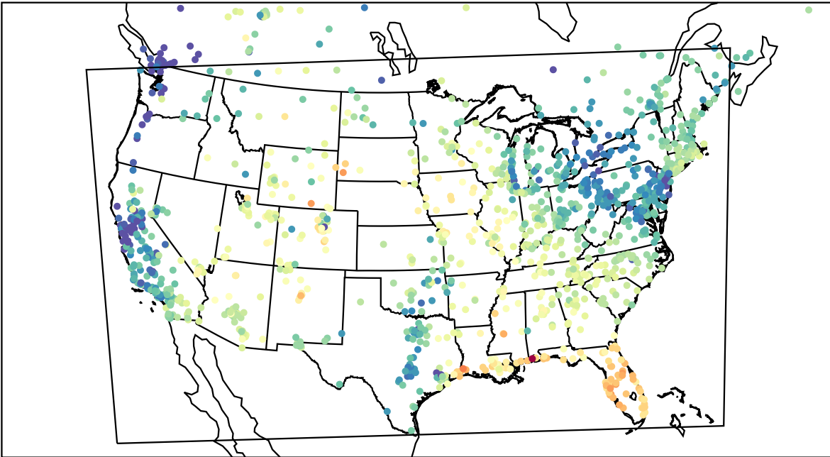
AirNOW (2023-05-04_15:00:00)
