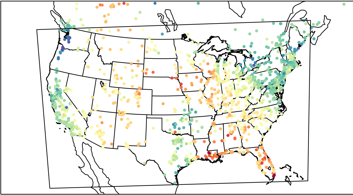
AirNOW (2023-05-04_22:00:00)
