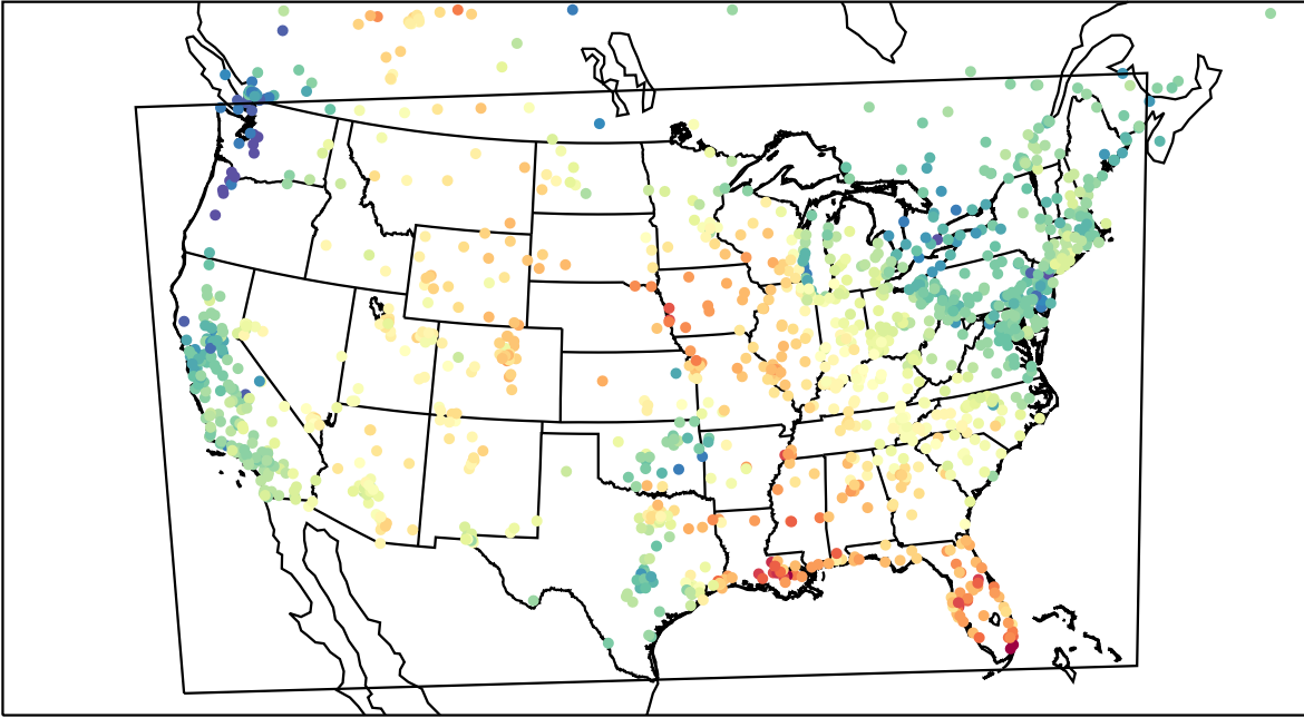
AirNOW (2023-05-04_18:00:00)
