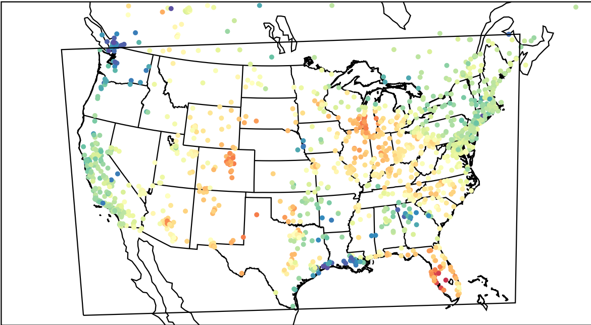
AirNOW (2023-05-05_21:00:00)
