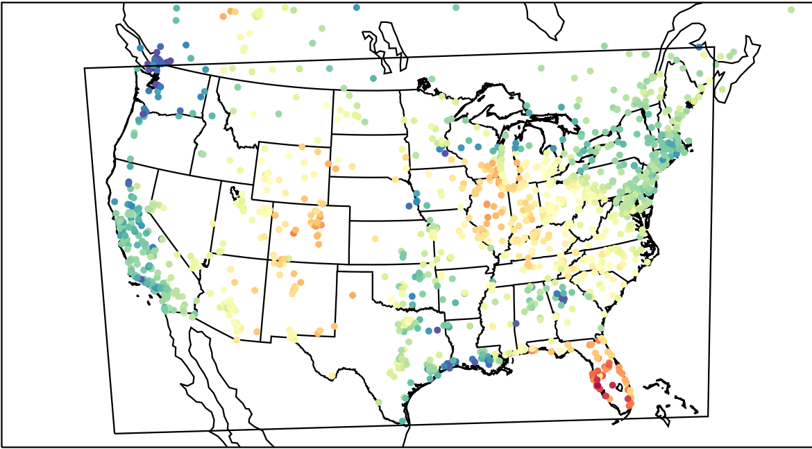
AirNOW (2023-05-05_17:00:00)
