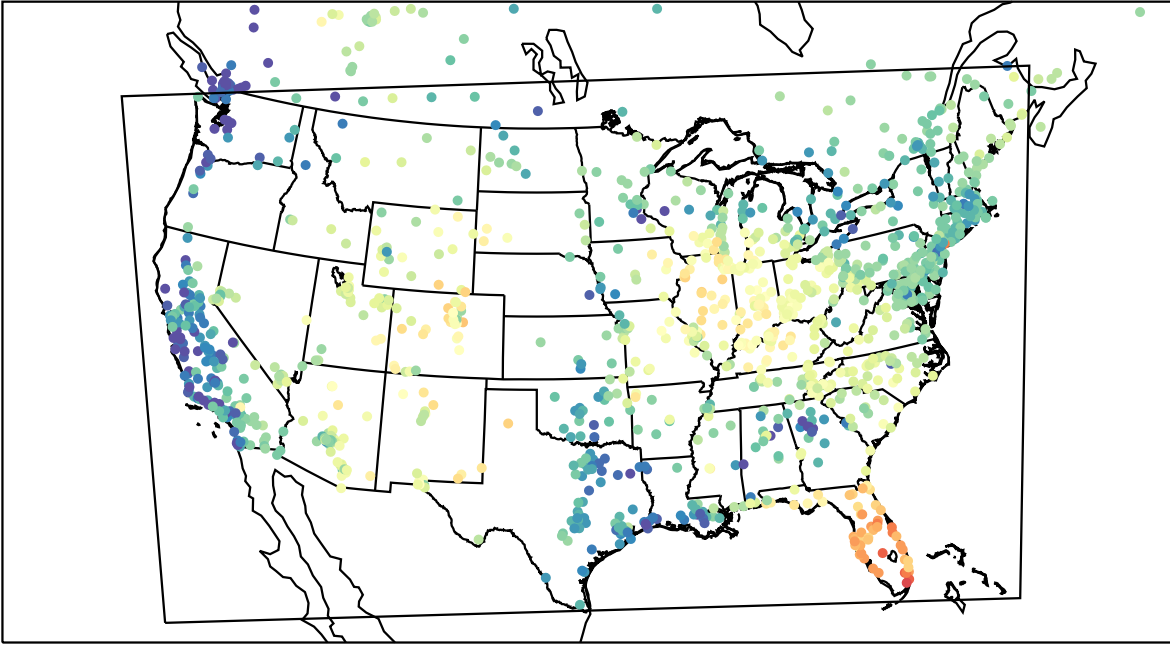
AirNOW (2023-05-05_15:00:00)
