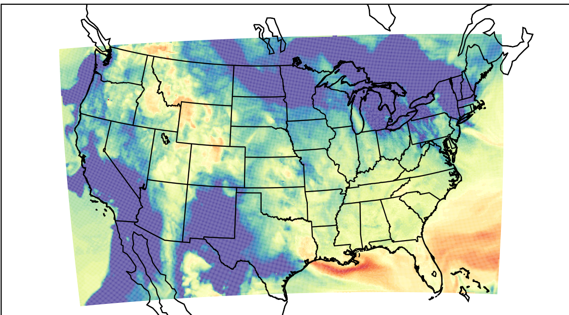
WRF (2023-05-04_15:00:00)
