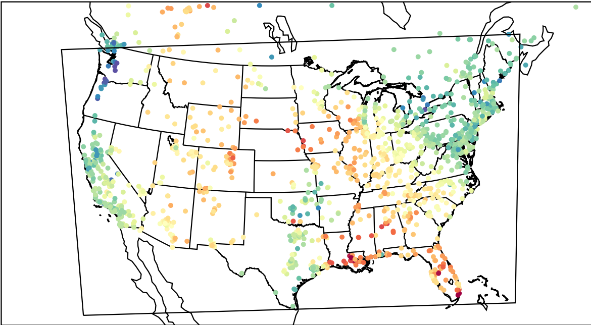
AirNOW (2023-05-04_21:00:00)
