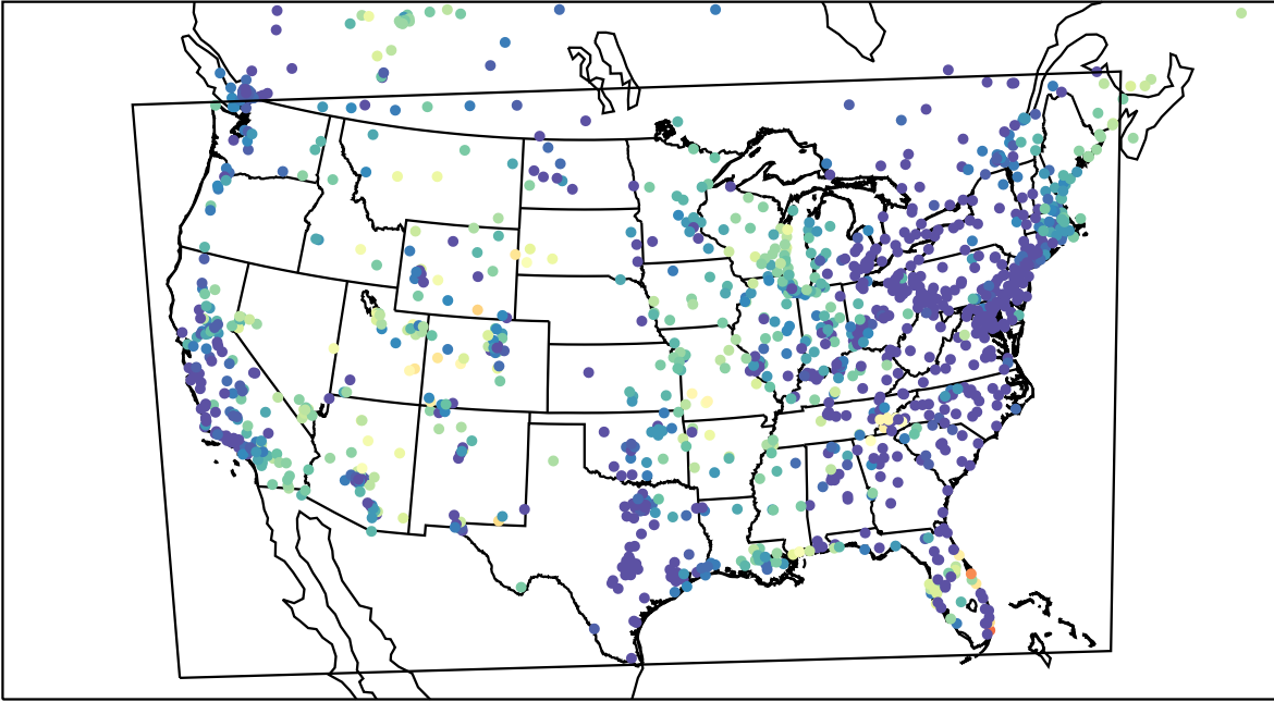
AirNOW (2023-05-05_11:00:00)
