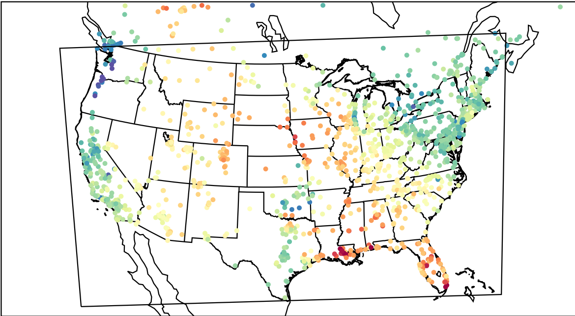
AirNOW (2023-05-04_19:00:00)
