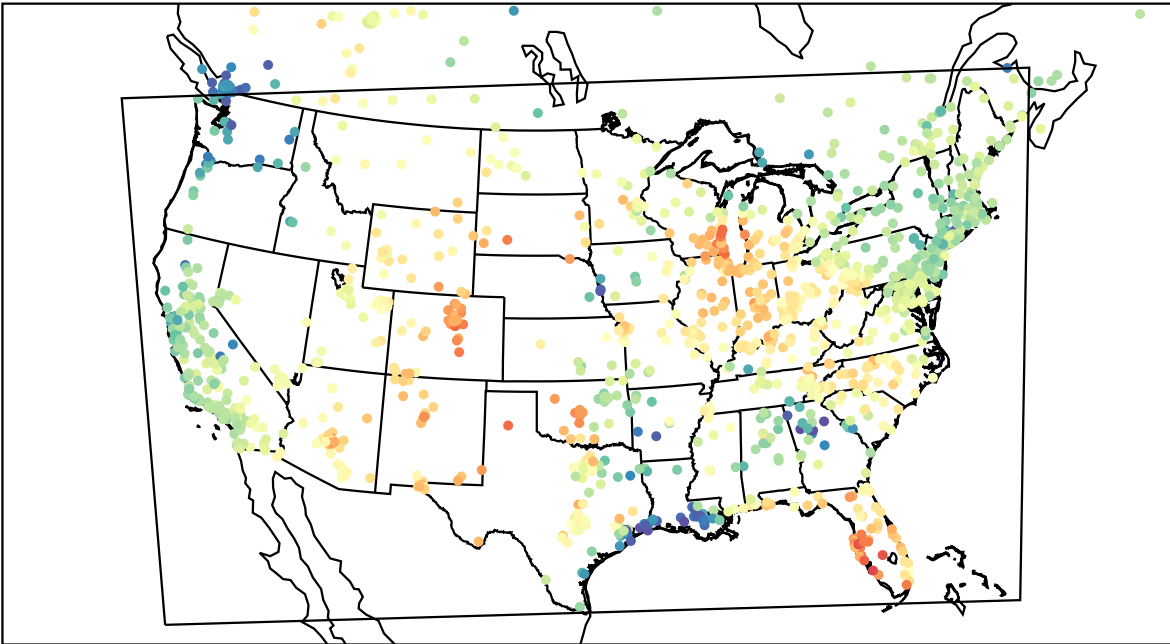
AirNOW (2023-05-05_22:00:00)
