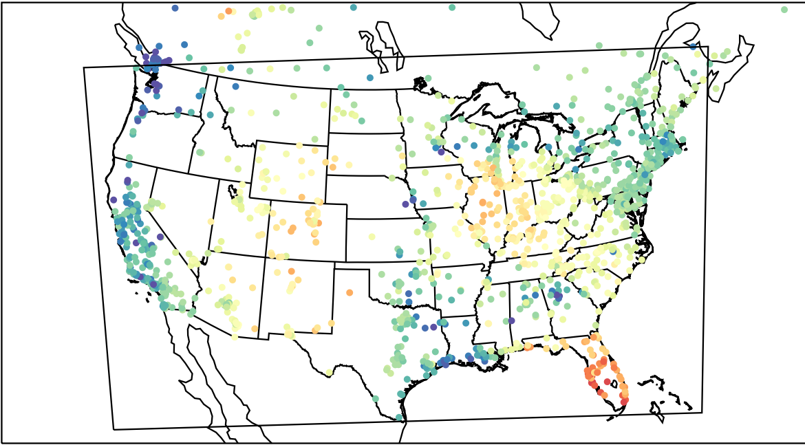
AirNOW (2023-05-05_16:00:00)
