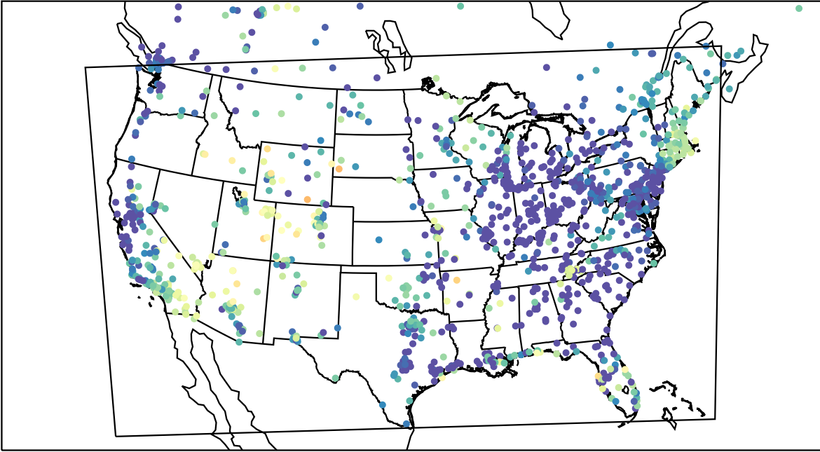
AirNOW (2023-05-04_11:00:00)
