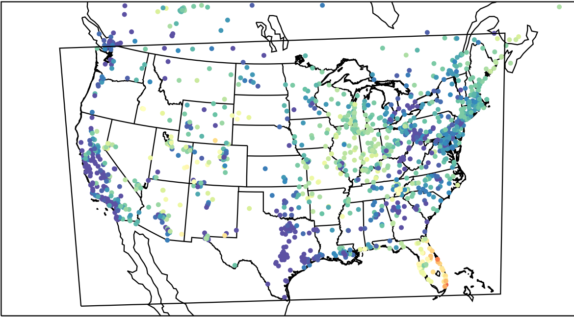
AirNOW (2023-05-05_13:00:00)
