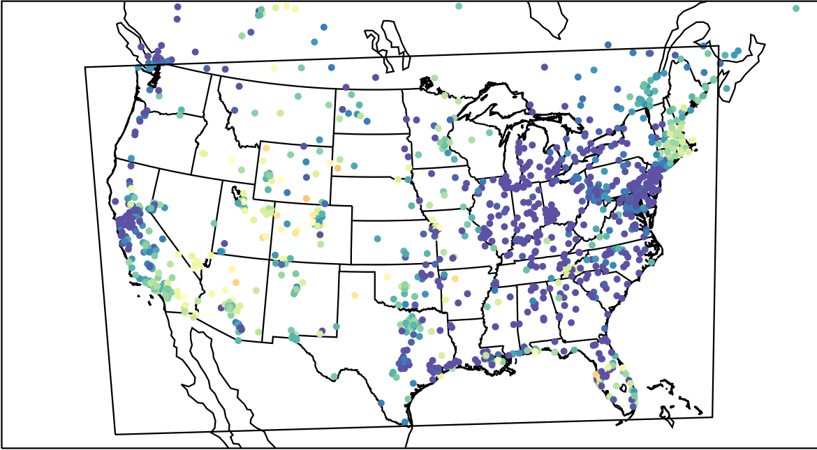
AirNOW (2023-05-04_10:00:00)
