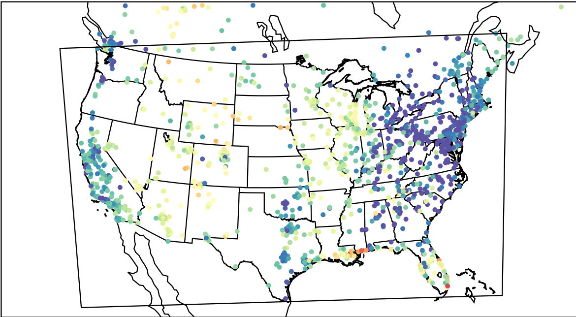
AirNOW (2023-05-05_04:00:00)
