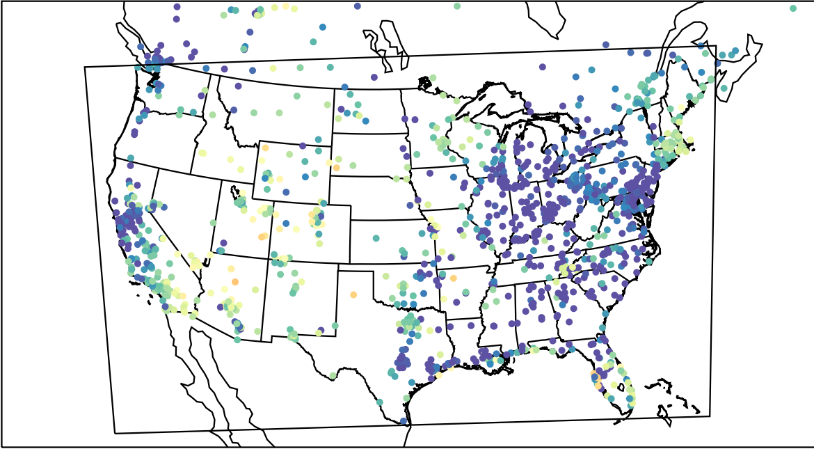
AirNOW (2023-05-04_09:00:00)
