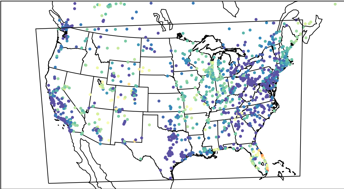
AirNOW (2023-05-05_12:00:00)
