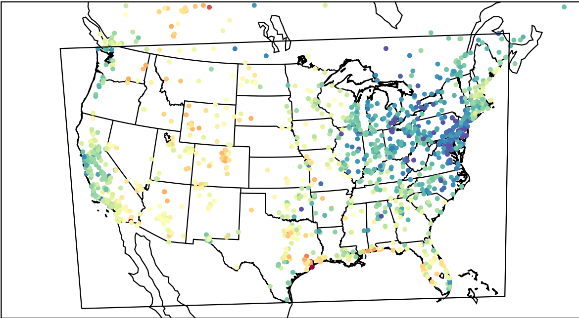
AirNOW (2023-05-04_01:00:00)
