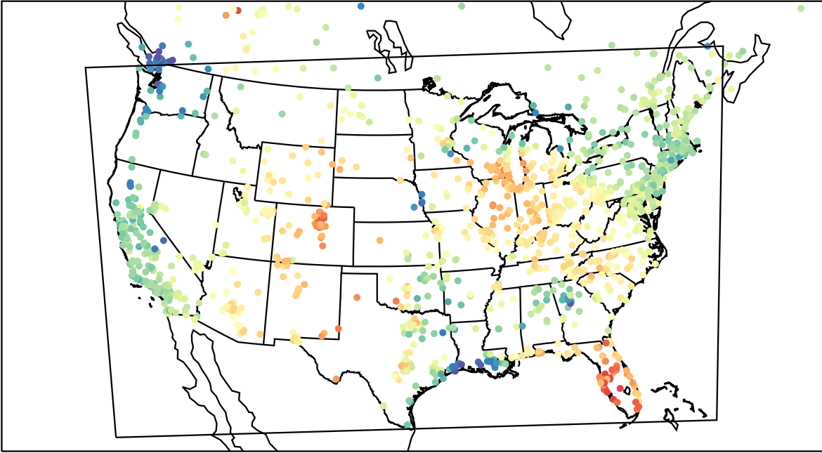
AirNOW (2023-05-05_19:00:00)
