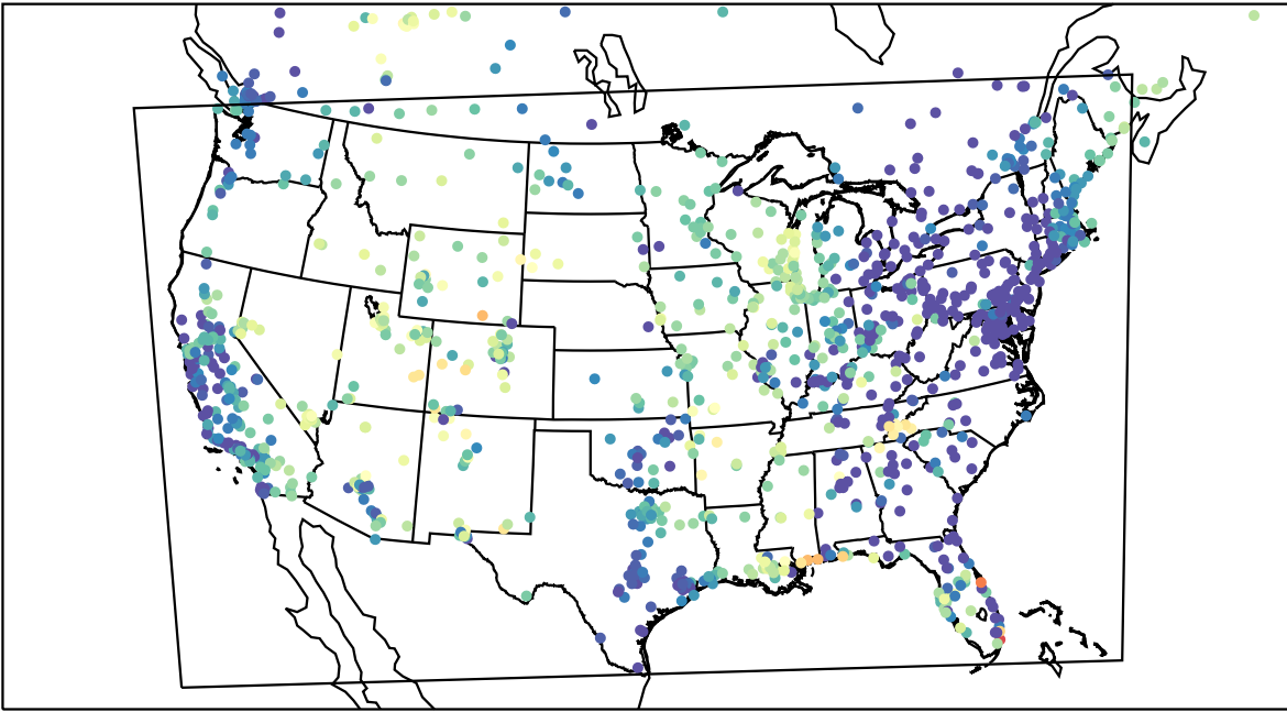
AirNOW (2023-05-05_08:00:00)
