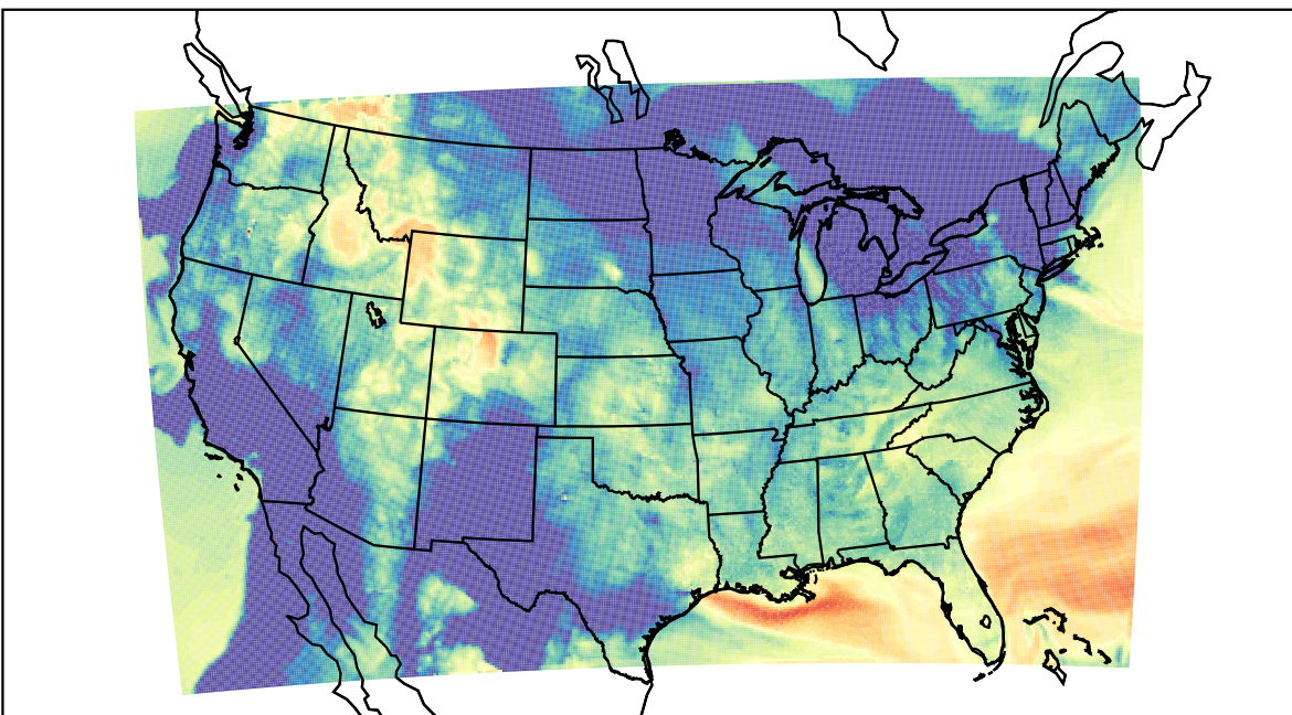
WRF (2023-05-04_14:00:00)
