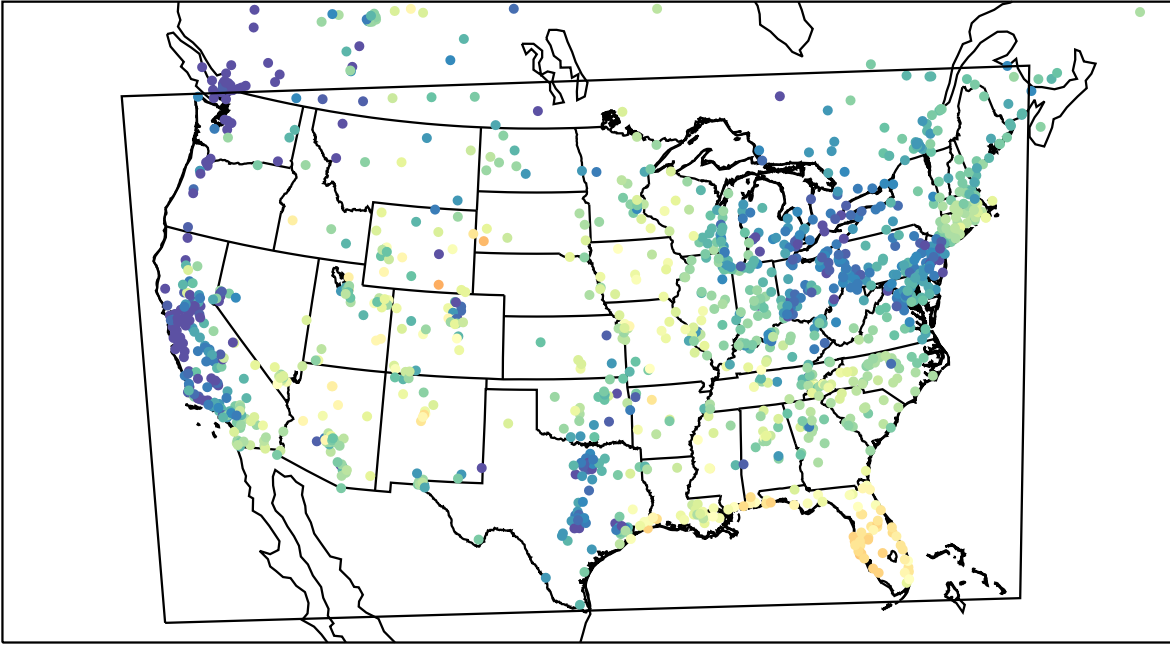
AirNOW (2023-05-04_14:00:00)
