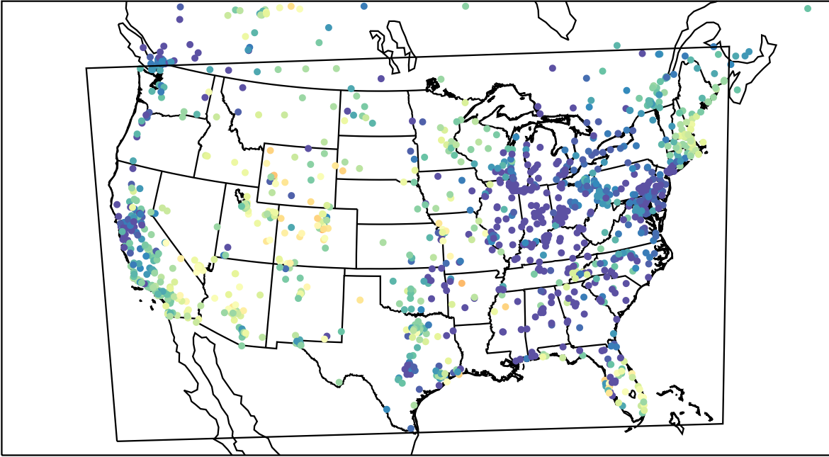
AirNOW (2023-05-04_07:00:00)
