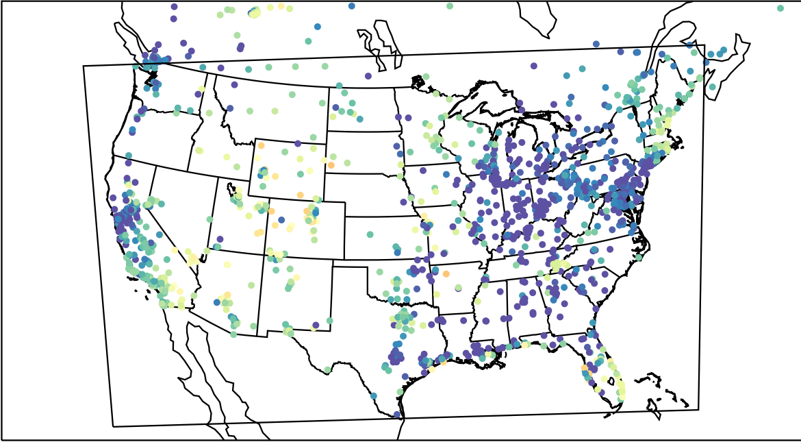
AirNOW (2023-05-04_08:00:00)
