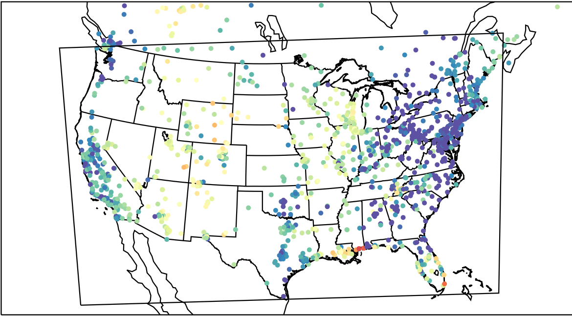
AirNOW (2023-05-05_05:00:00)
