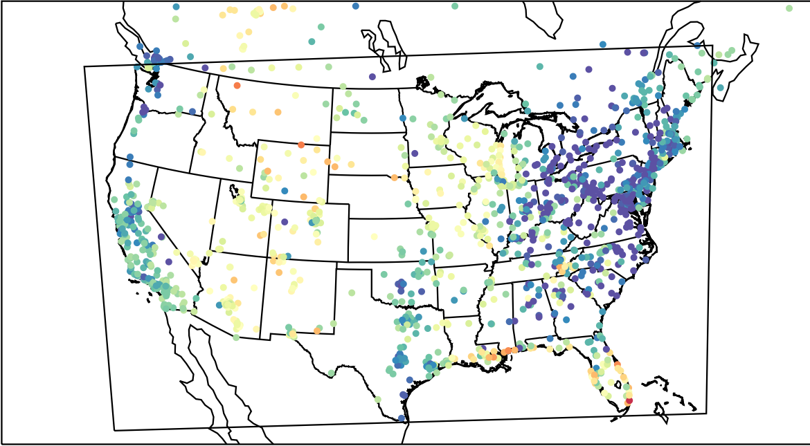
AirNOW (2023-05-05_03:00:00)
