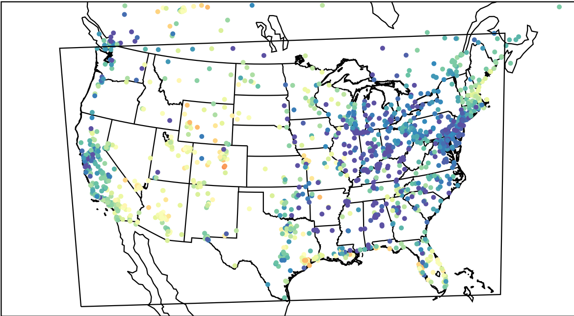
AirNOW (2023-05-04_04:00:00)
