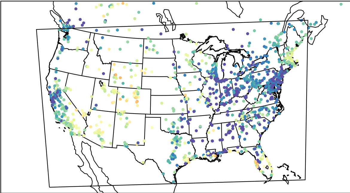
AirNOW (2023-05-04_05:00:00)
