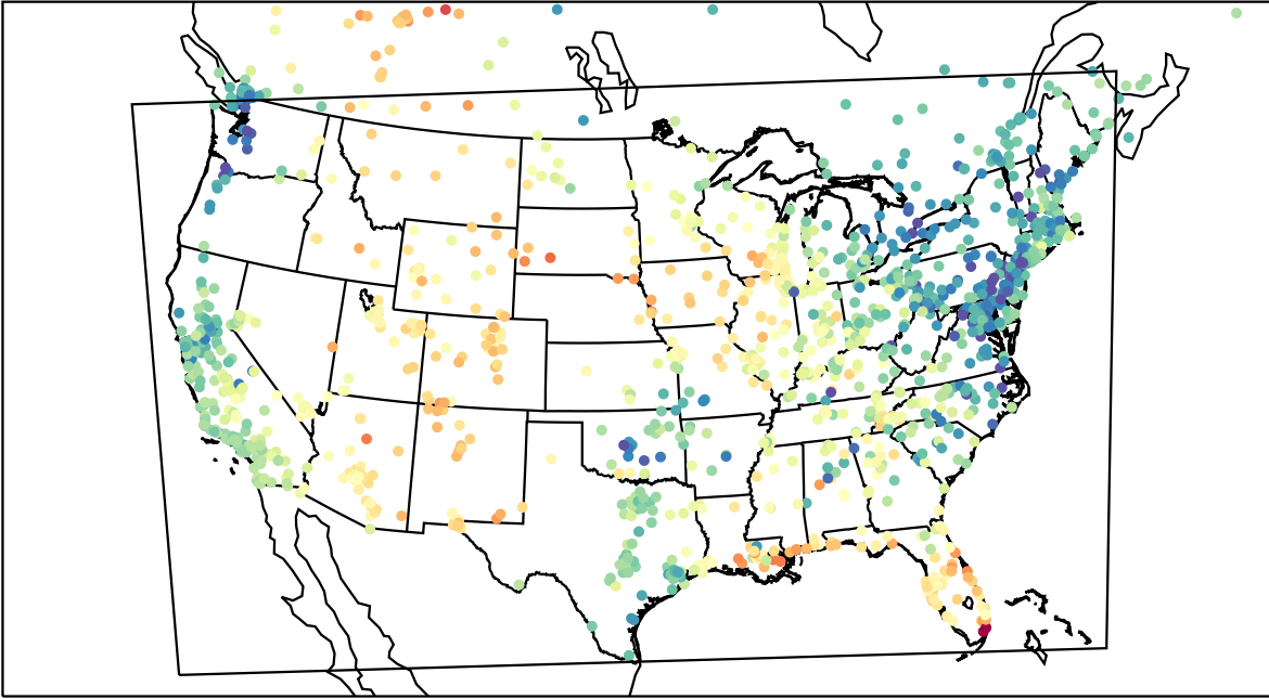
AirNOW (2023-05-05_00:00:00)
