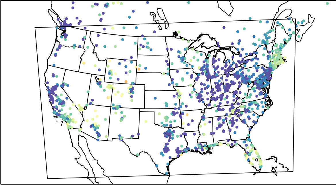
AirNOW (2023-05-04_12:00:00)
