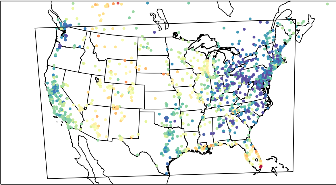
AirNOW (2023-05-05_02:00:00)
