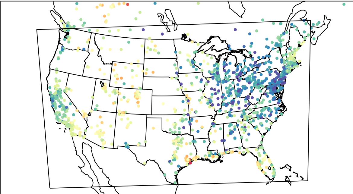
AirNOW (2023-05-04_02:00:00)
