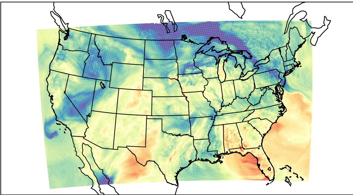
WRF (2023-05-05_23:00:00)
