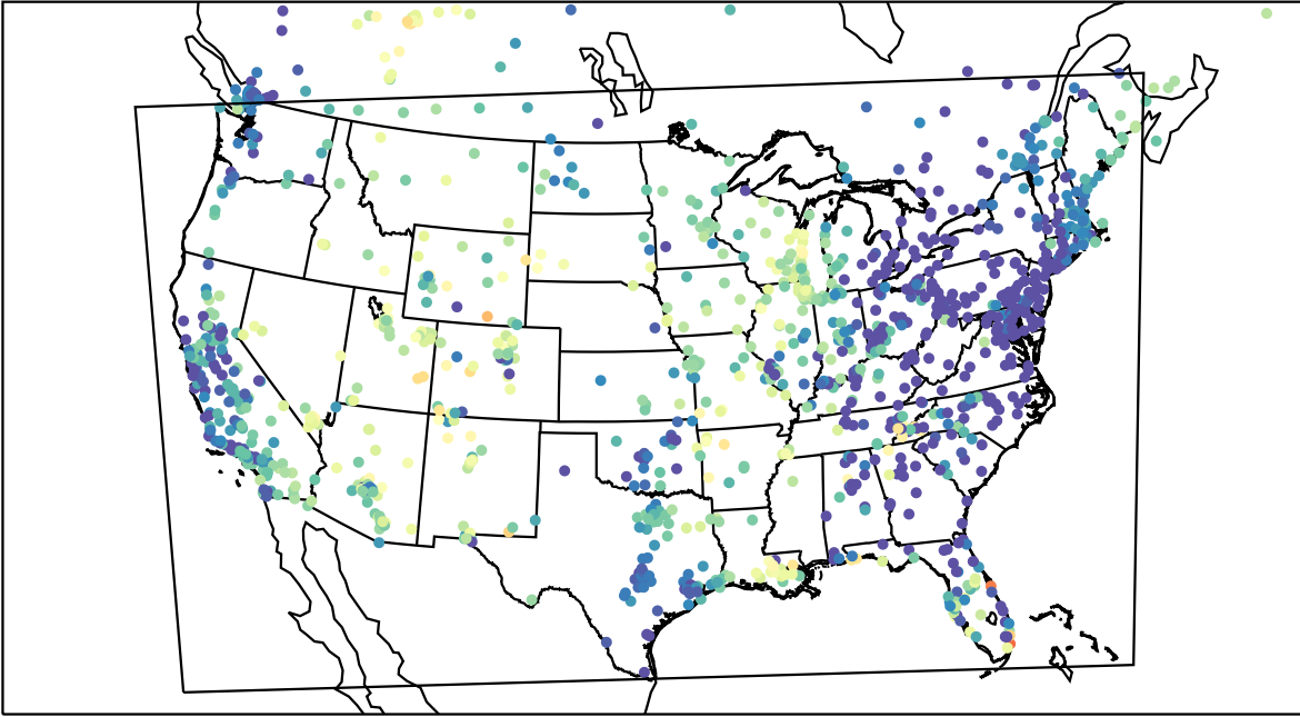
AirNOW (2023-05-05_07:00:00)
