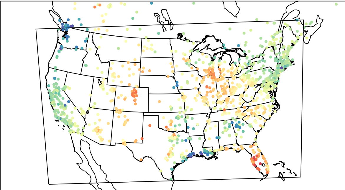
AirNOW (2023-05-05_20:00:00)
