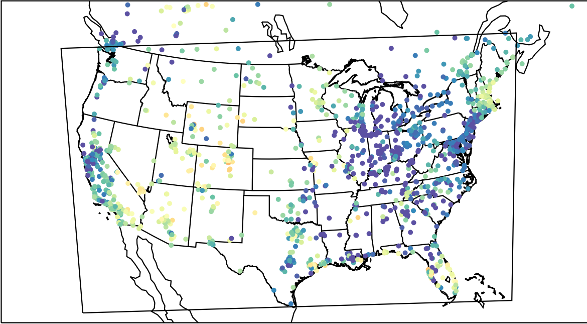
AirNOW (2023-05-04_06:00:00)
