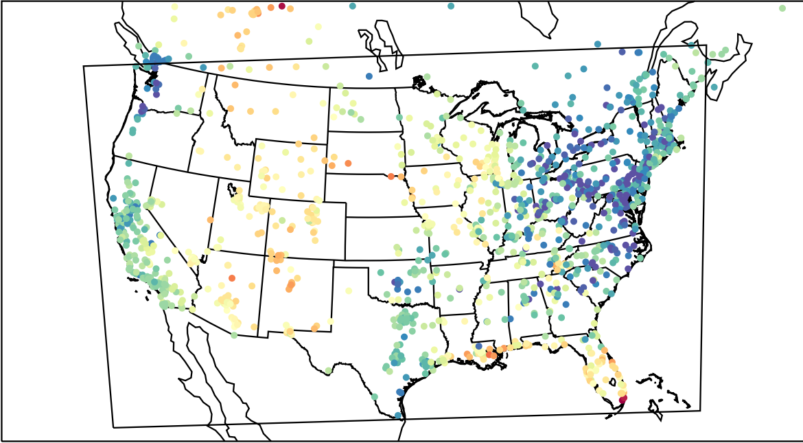
AirNOW (2023-05-05_01:00:00)
