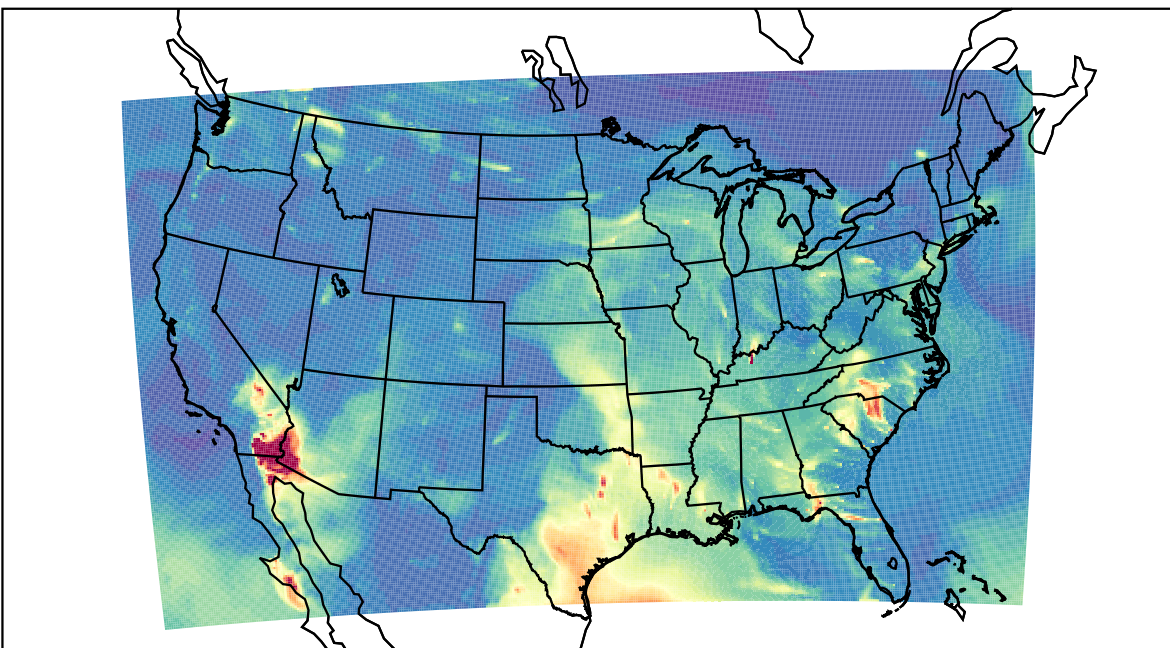
WRF 2023-05-06_06:00:00
