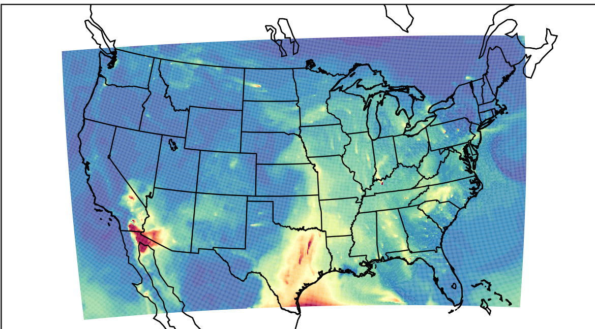
WRF 2023-05-06_13:00:00
