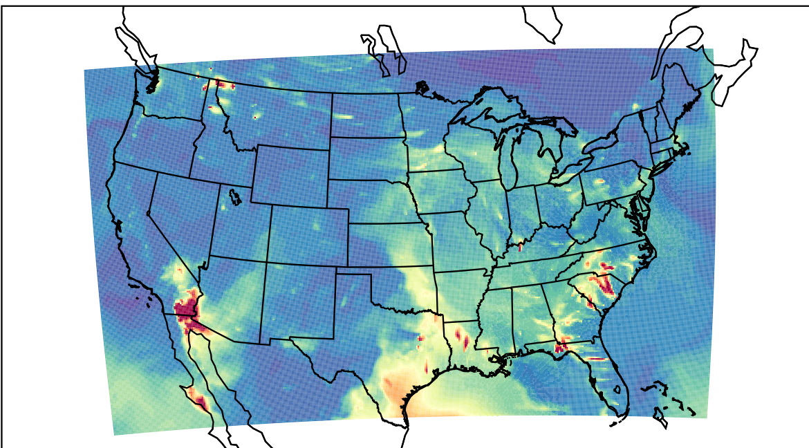
WRF 2023-05-06_04:00:00
