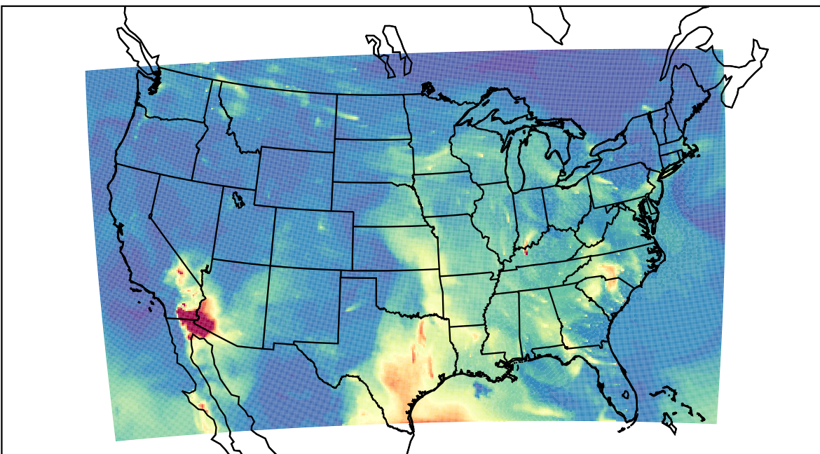
WRF 2023-05-06_08:00:00
