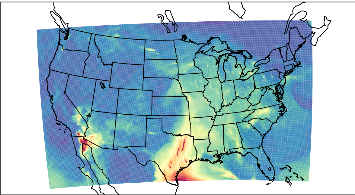
WRF 2023-05-06_15:00:00
