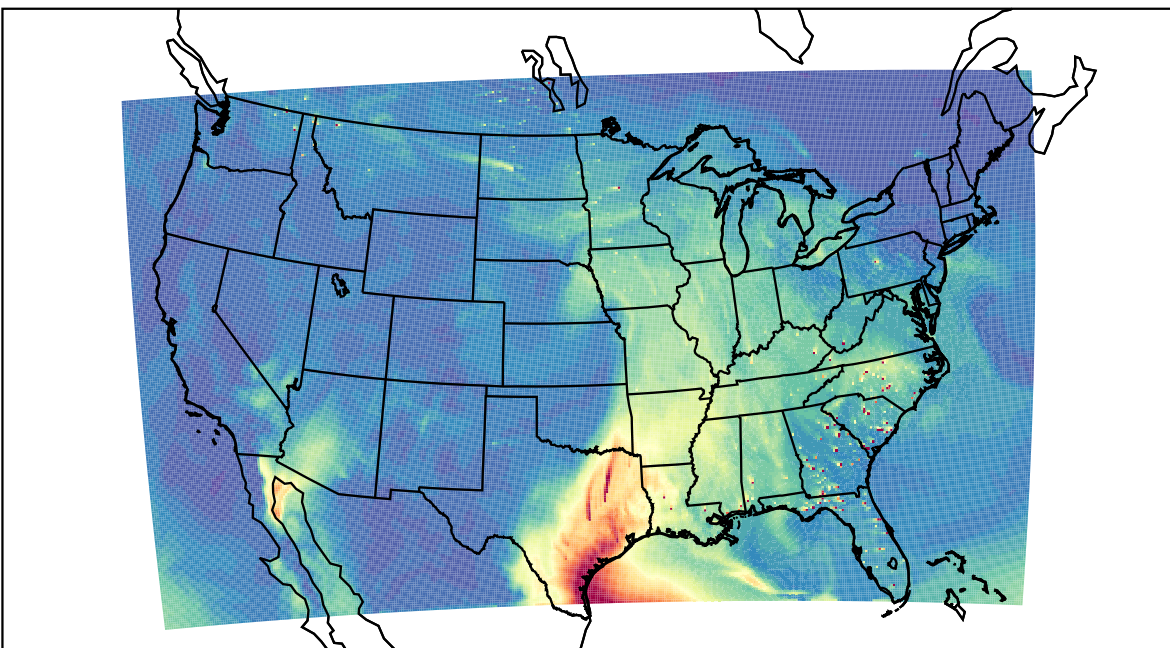
WRF 2023-05-06_19:00:00
