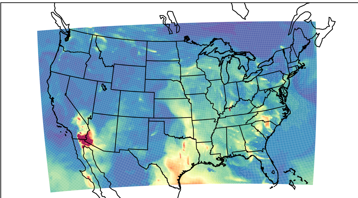
WRF 2023-05-06_07:00:00
