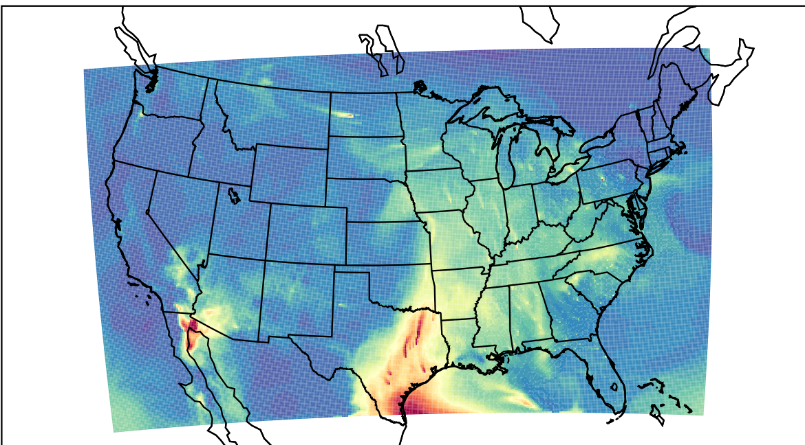
WRF 2023-05-06_16:00:00
