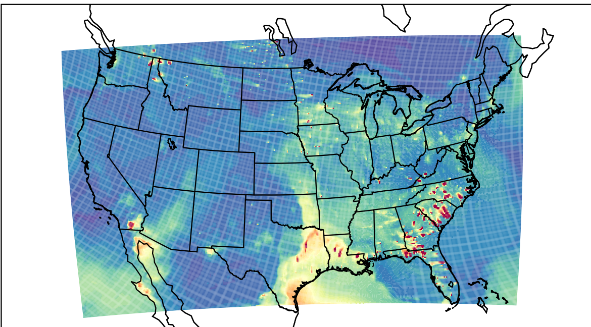
WRF 2023-05-06_01:00:00
