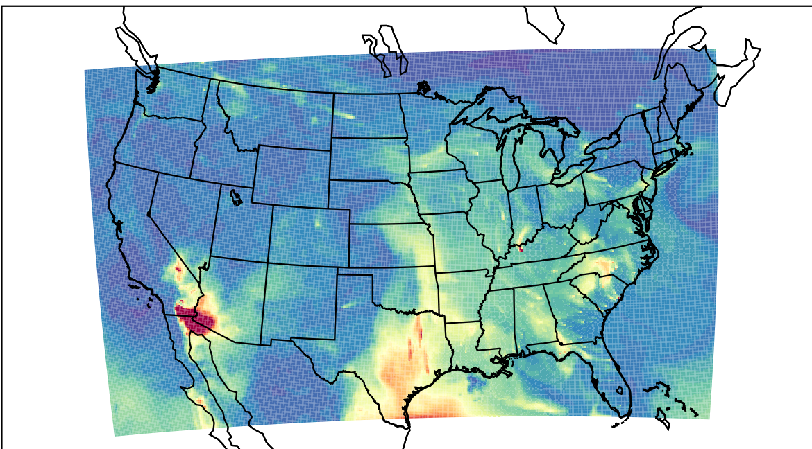
WRF 2023-05-06_09:00:00
