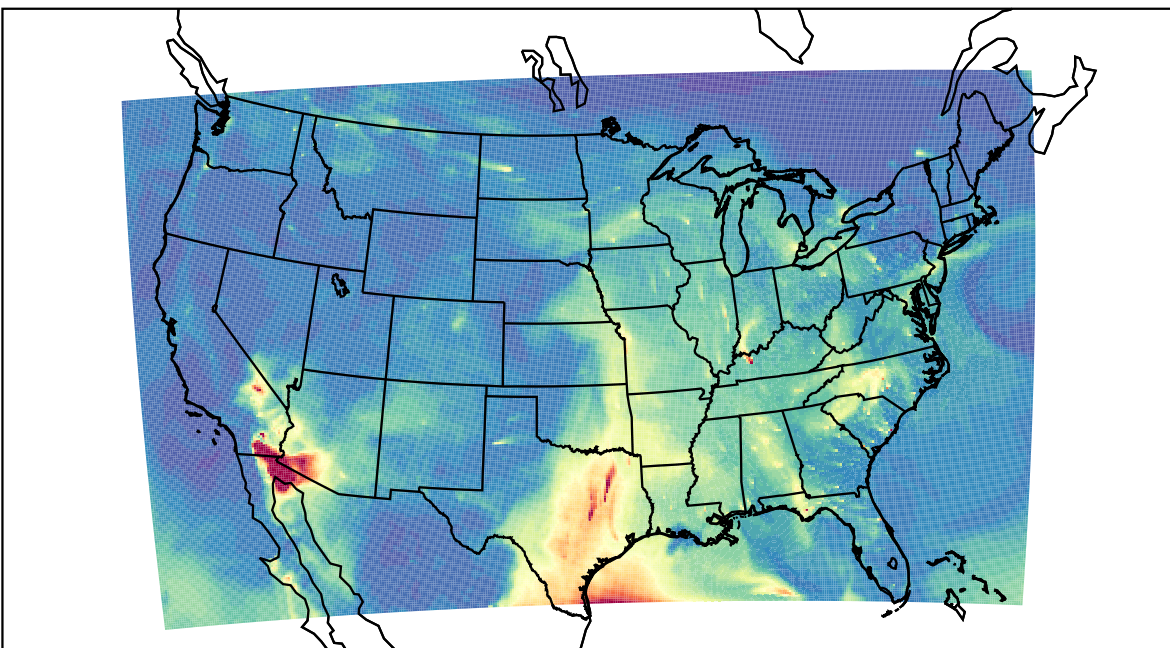
WRF 2023-05-06_12:00:00
