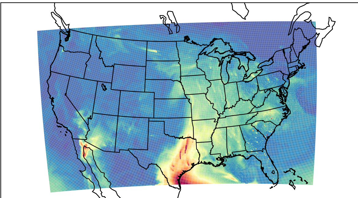
WRF 2023-05-06_17:00:00
