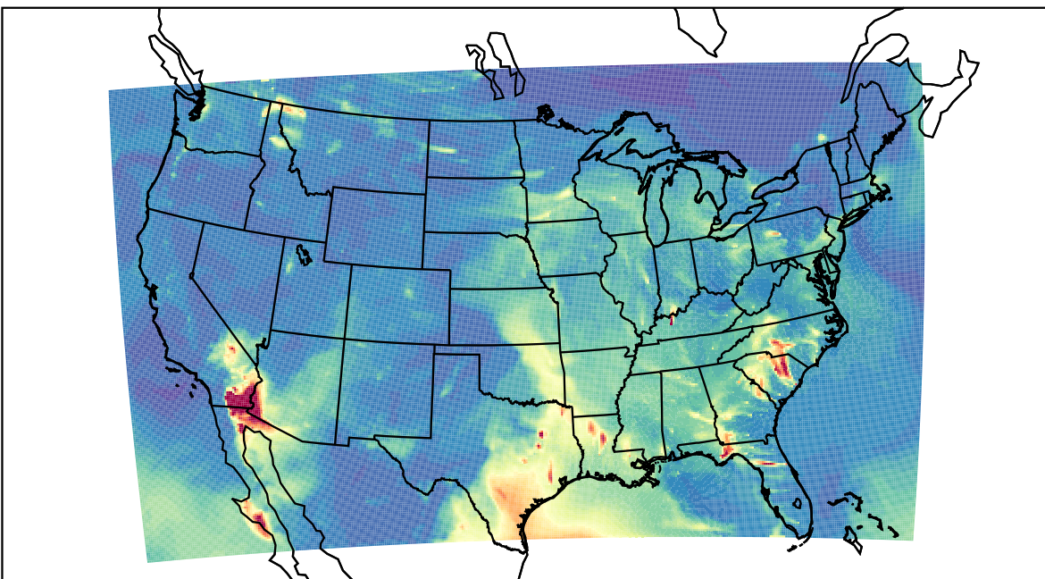
WRF 2023-05-06_05:00:00
