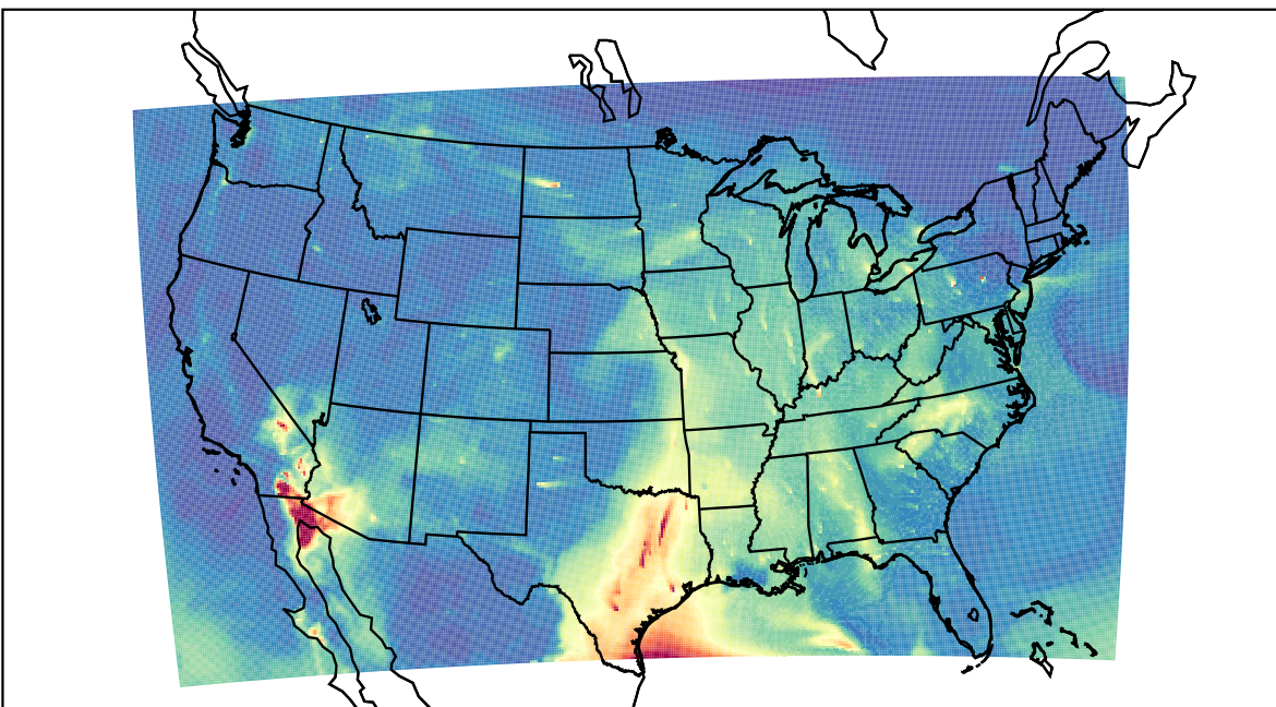
WRF 2023-05-06_14:00:00
