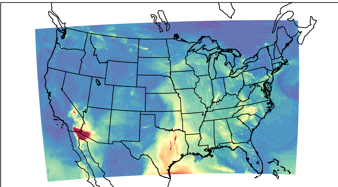
WRF 2023-05-06_10:00:00
