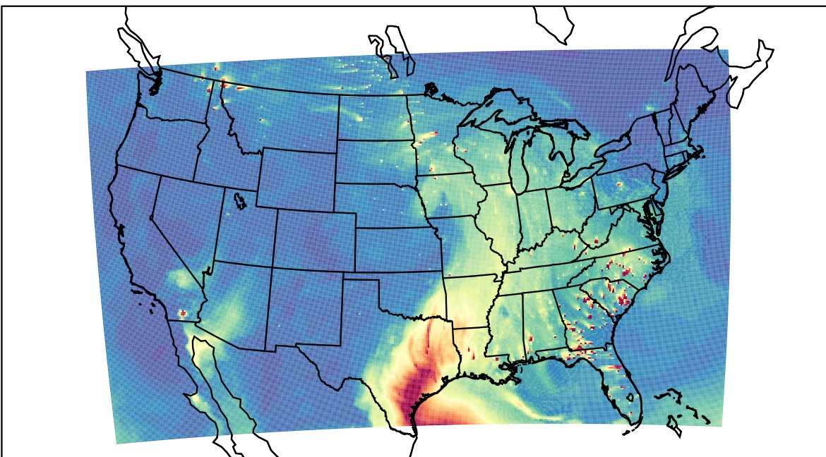
WRF 2023-05-06_23:00:00
