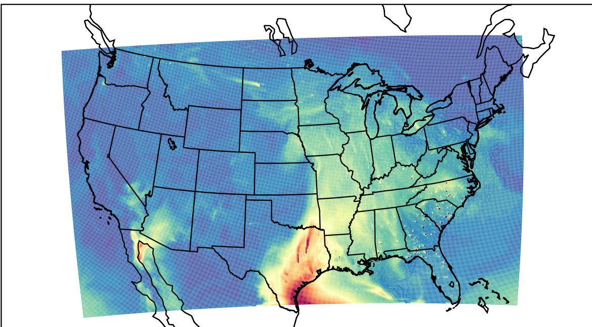
WRF 2023-05-06_18:00:00
