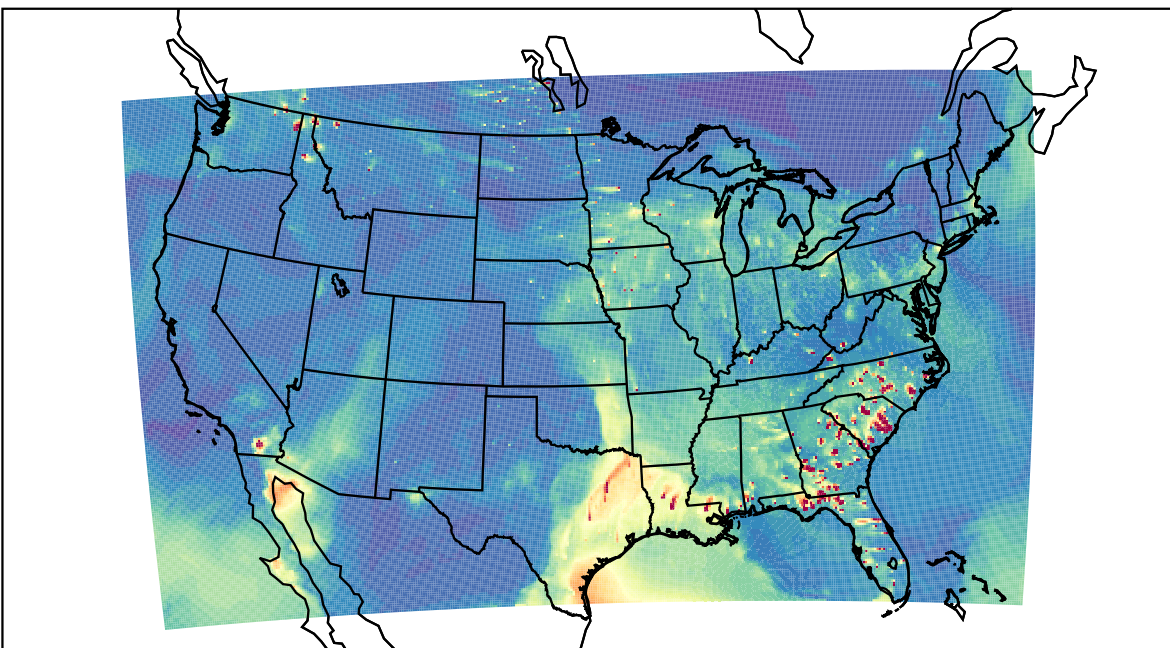
WRF 2023-05-06_00:00:00
