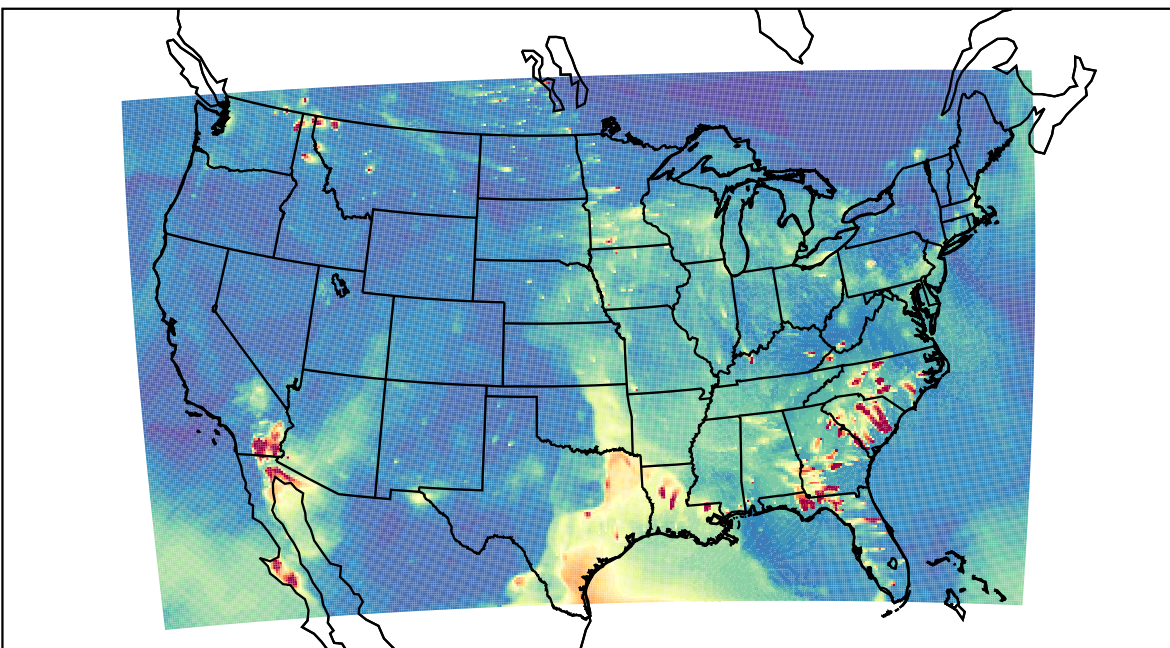
WRF 2023-05-06_02:00:00
