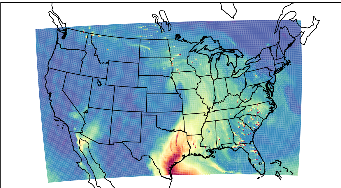
WRF 2023-05-06_21:00:00
