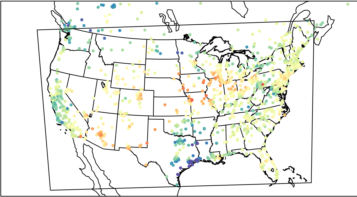
AirNOW (2023-05-07_20:00:00)
