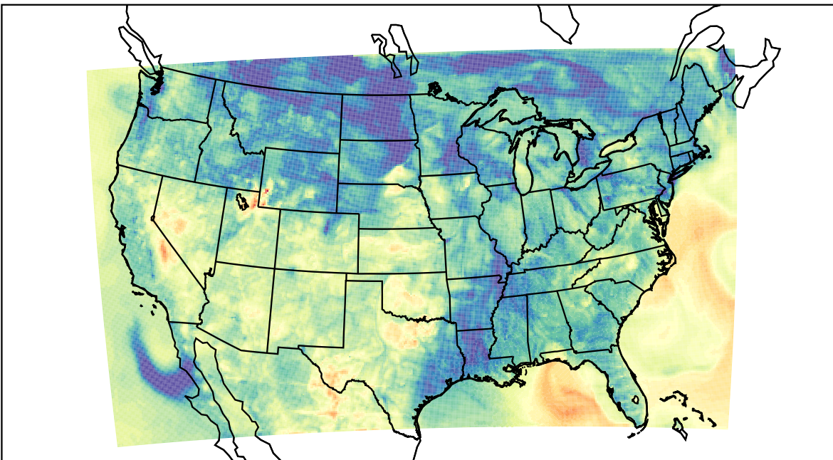
WRF (2023-05-07_04:00:00)
