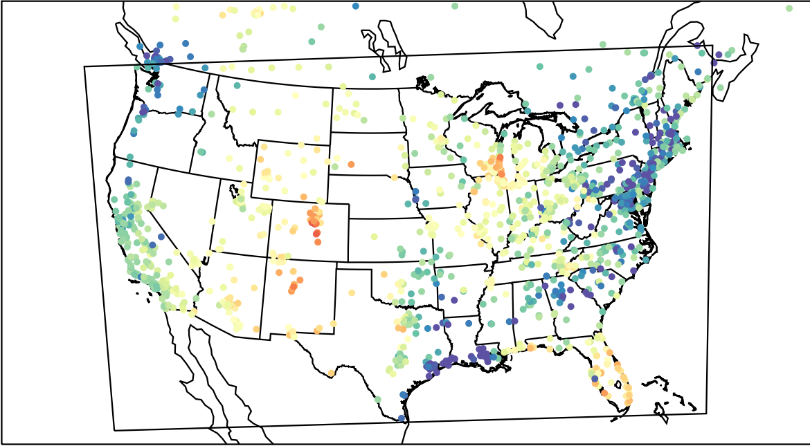
AirNOW (2023-05-06_01:00:00)
