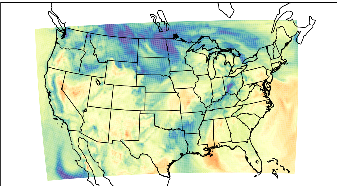
WRF (2023-05-07_16:00:00)
