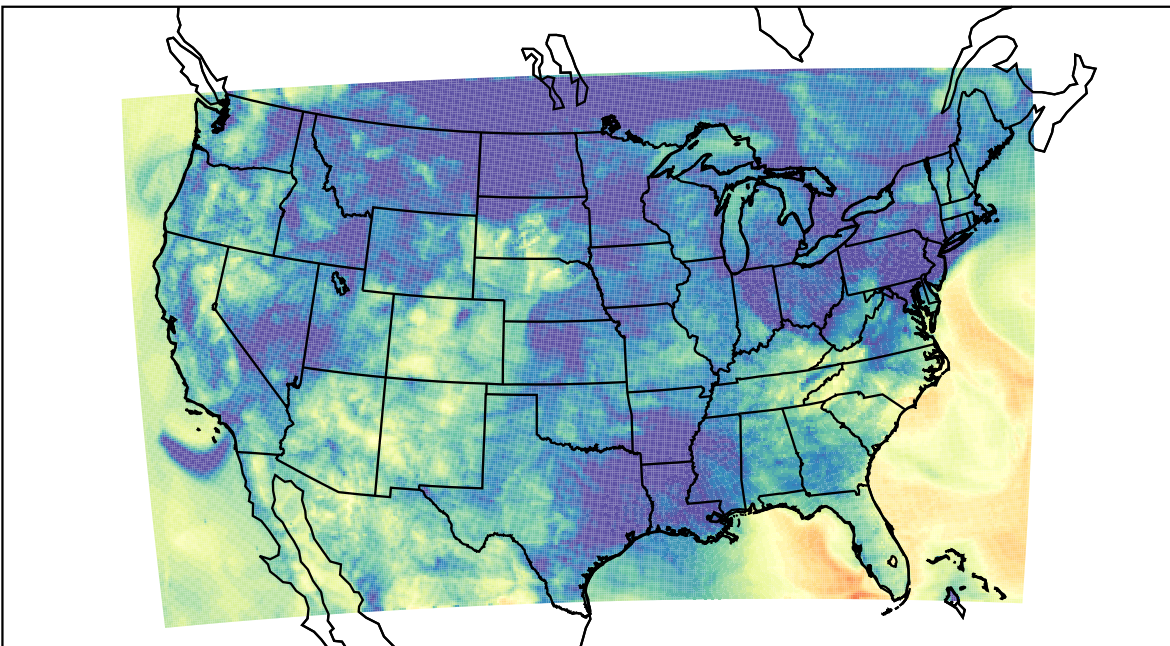
WRF (2023-05-06_11:00:00)
