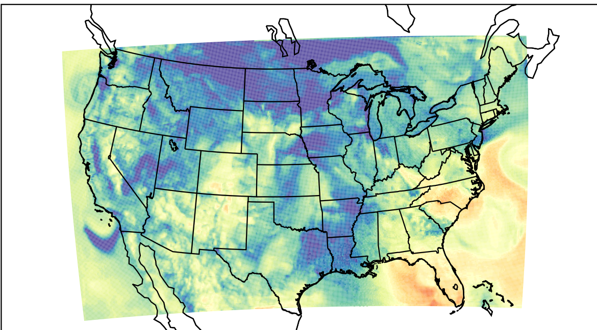
WRF (2023-05-06_15:00:00)
