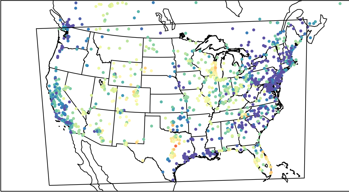
AirNOW (2023-05-06_05:00:00)
