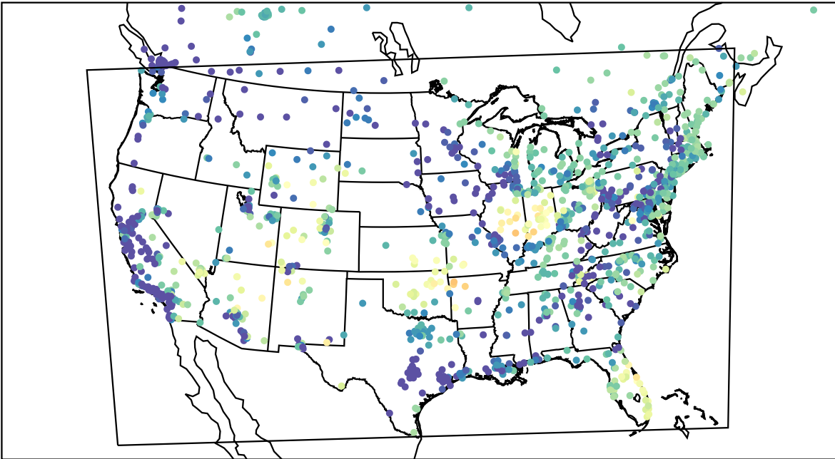
AirNOW (2023-05-07_12:00:00)
