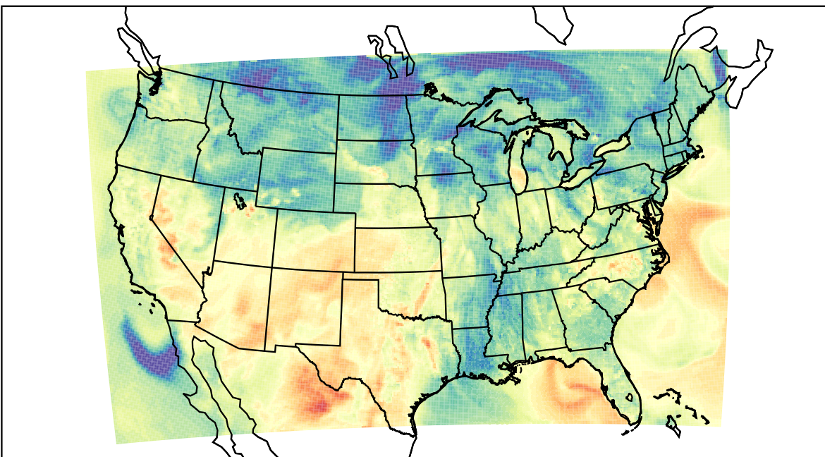
WRF (2023-05-07_00:00:00)
