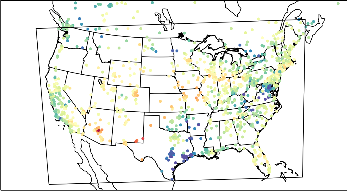
AirNOW (2023-05-07_23:00:00)
