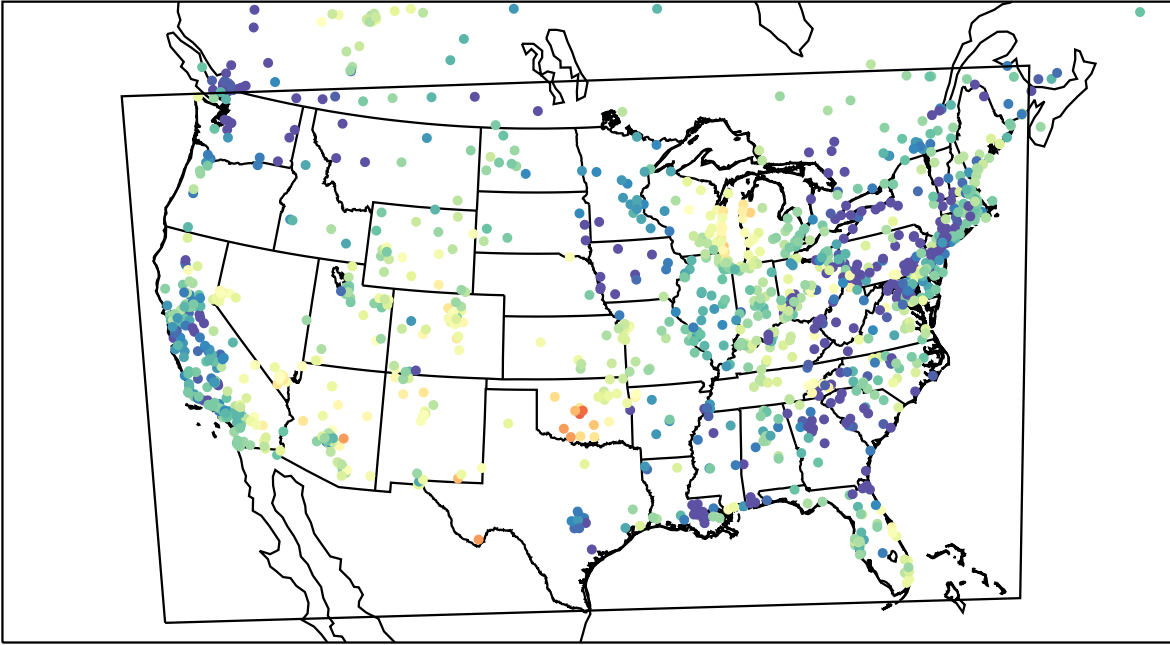
AirNOW (2023-05-07_04:00:00)
