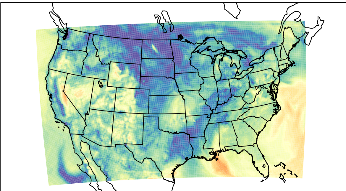
WRF (2023-05-07_14:00:00)
