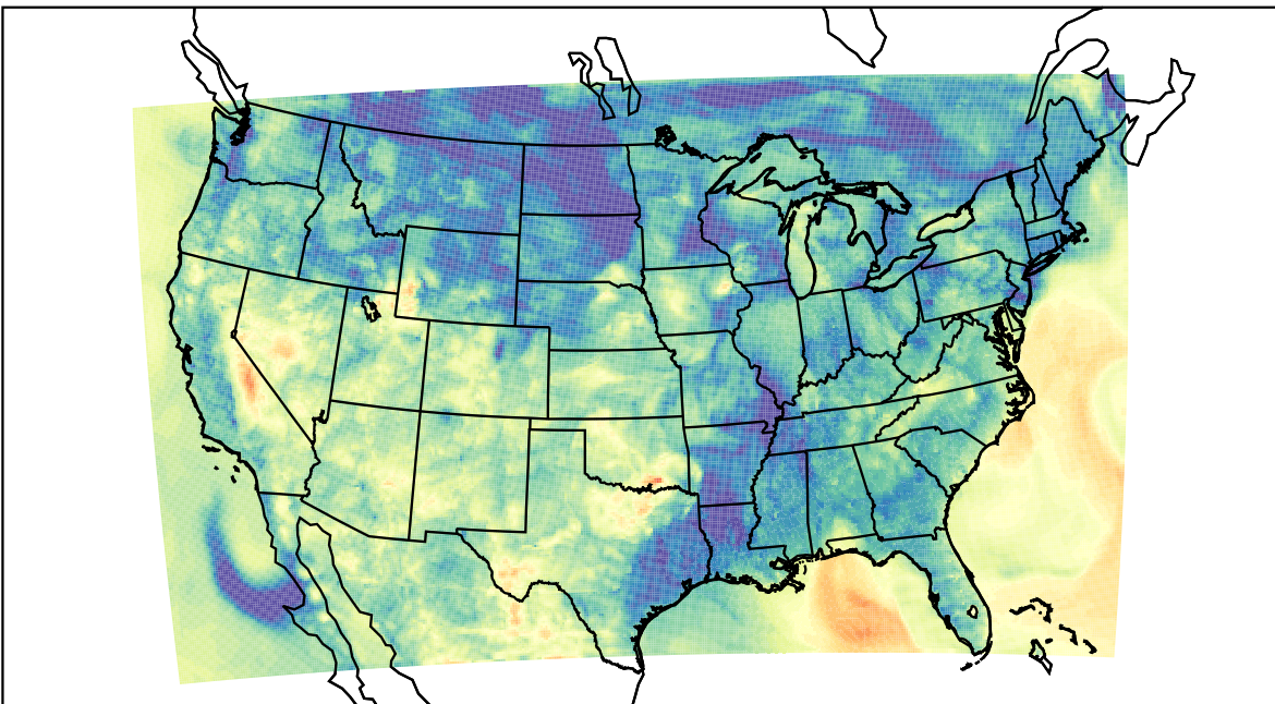
WRF (2023-05-07_06:00:00)
