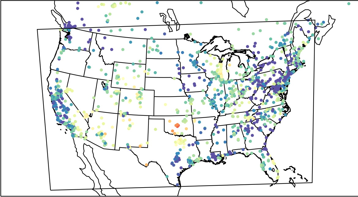
AirNOW (2023-05-07_05:00:00)
