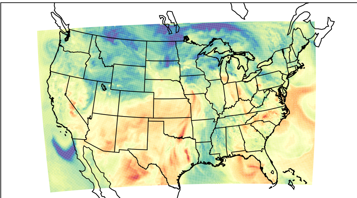
WRF (2023-05-06_22:00:00)
