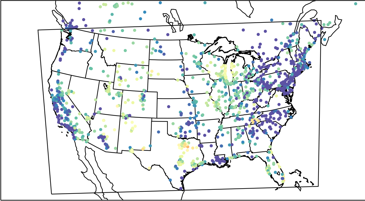
AirNOW (2023-05-06_09:00:00)
