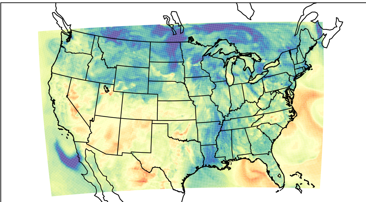
WRF (2023-05-07_01:00:00)
