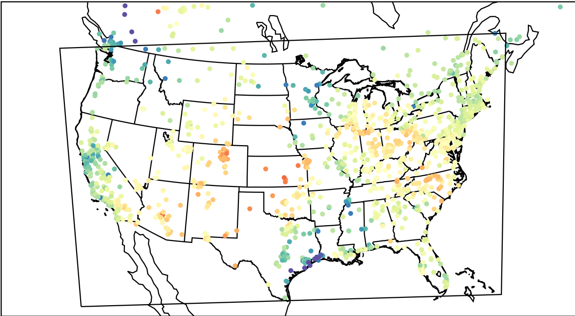
AirNOW (2023-05-06_22:00:00)
