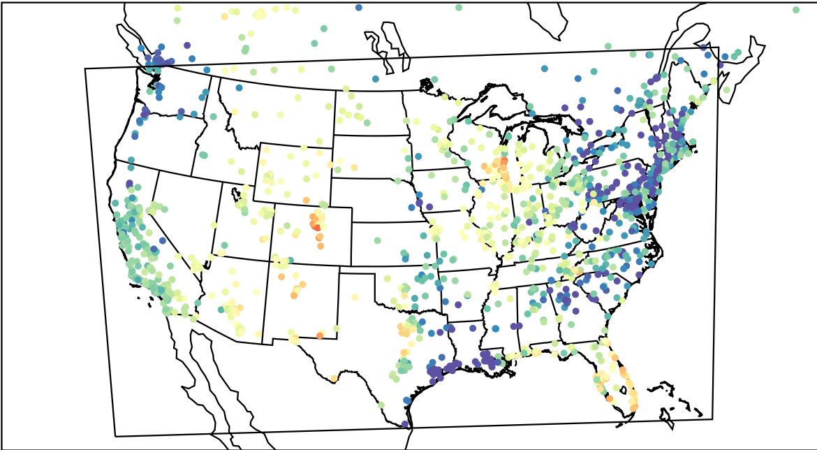
AirNOW (2023-05-06_02:00:00)
