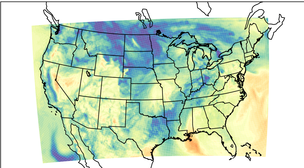
WRF (2023-05-07_15:00:00)
