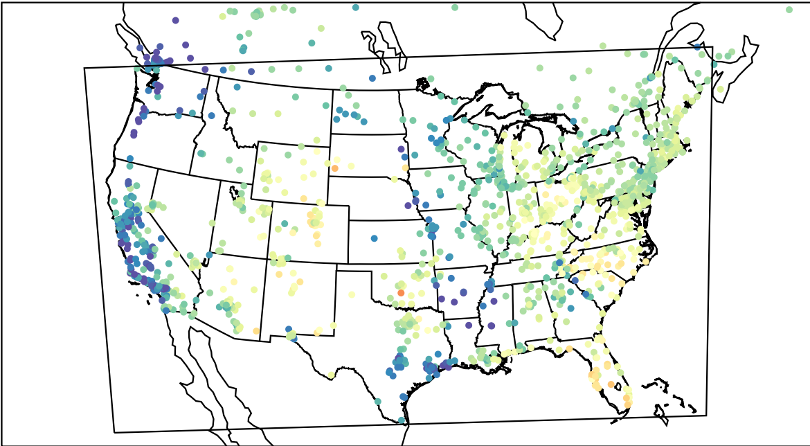
AirNOW (2023-05-06_15:00:00)
