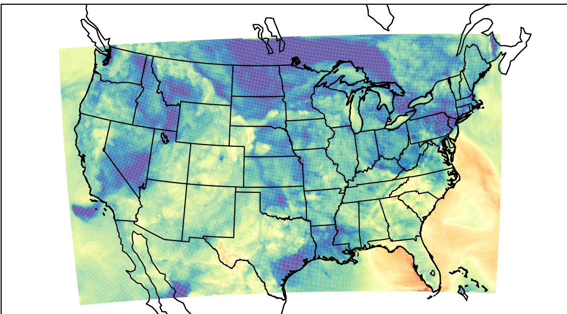
WRF (2023-05-06_03:00:00)
