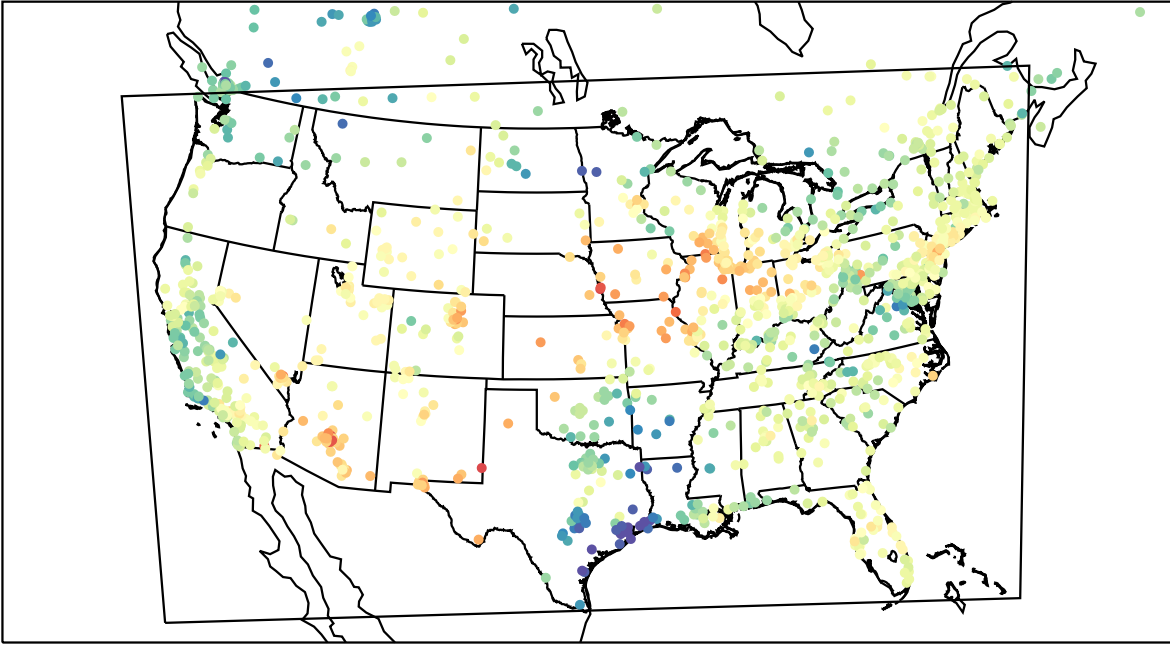
AirNOW (2023-05-07_21:00:00)
