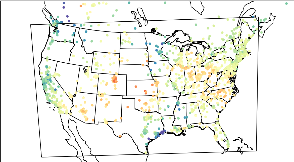
AirNOW (2023-05-06_21:00:00)
