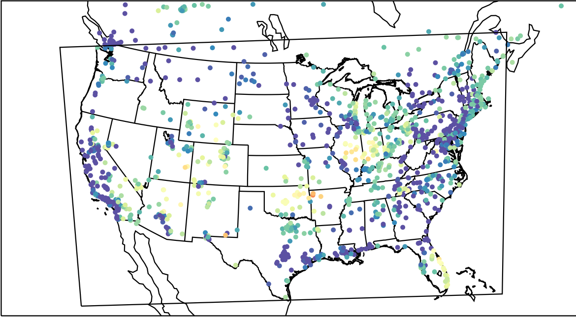
AirNOW (2023-05-07_11:00:00)
