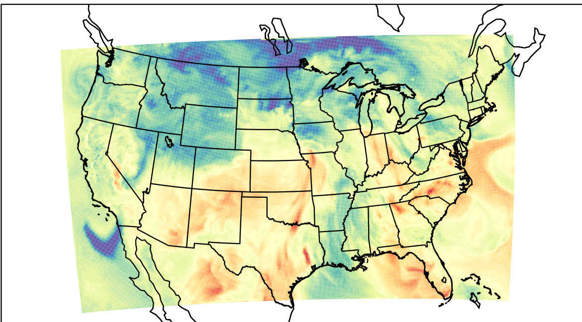
WRF (2023-05-06_20:00:00)
