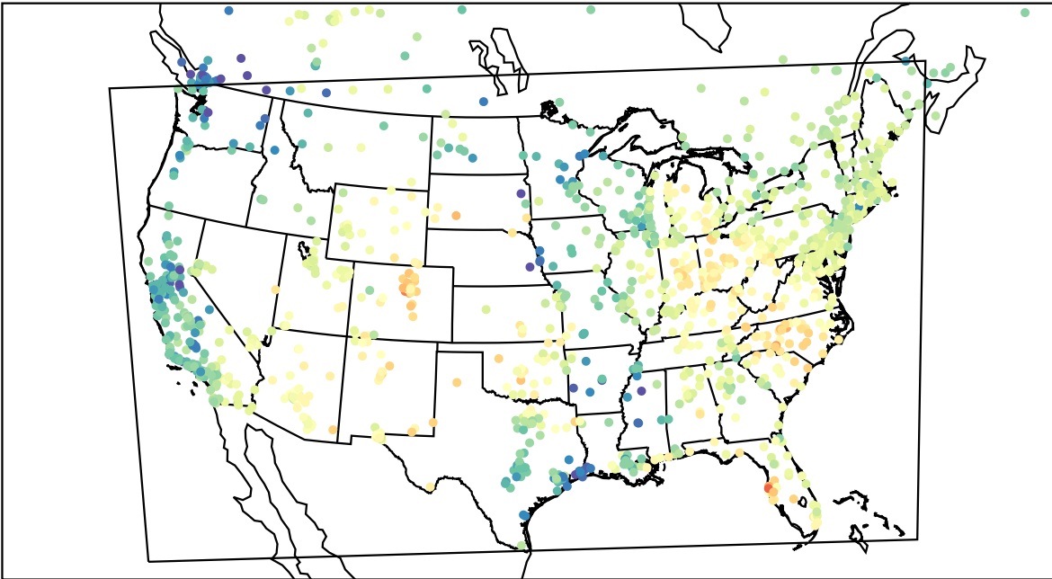
AirNOW (2023-05-06_17:00:00)
