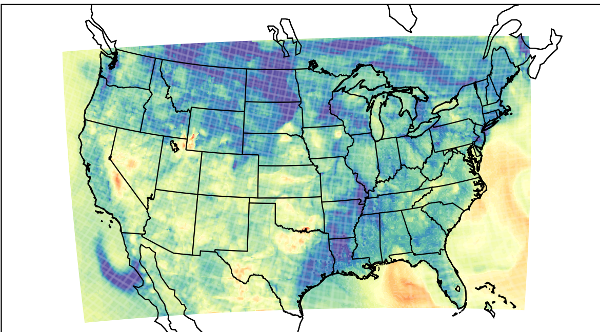
WRF (2023-05-07_05:00:00)
