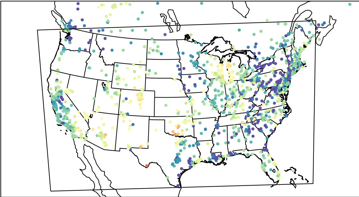
AirNOW (2023-05-07_03:00:00)
