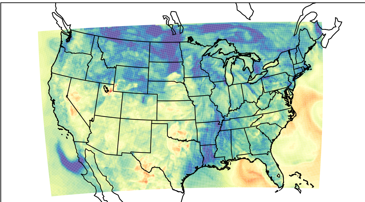
WRF (2023-05-07_03:00:00)
