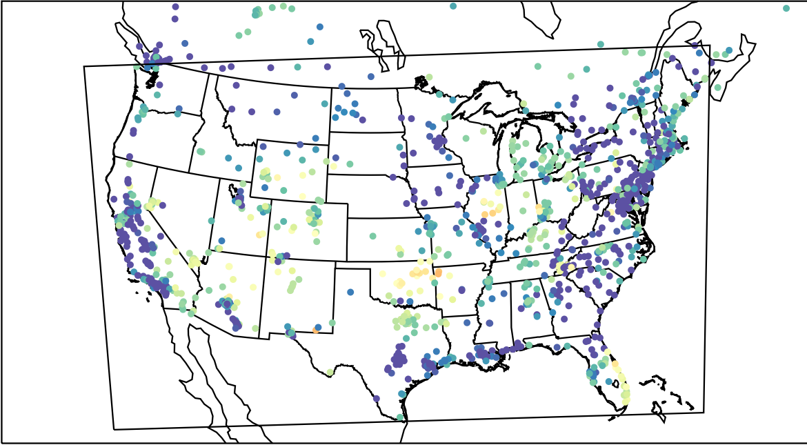
AirNOW (2023-05-07_10:00:00)
