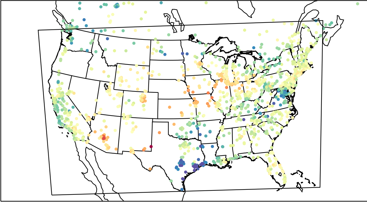
AirNOW (2023-05-07_22:00:00)
