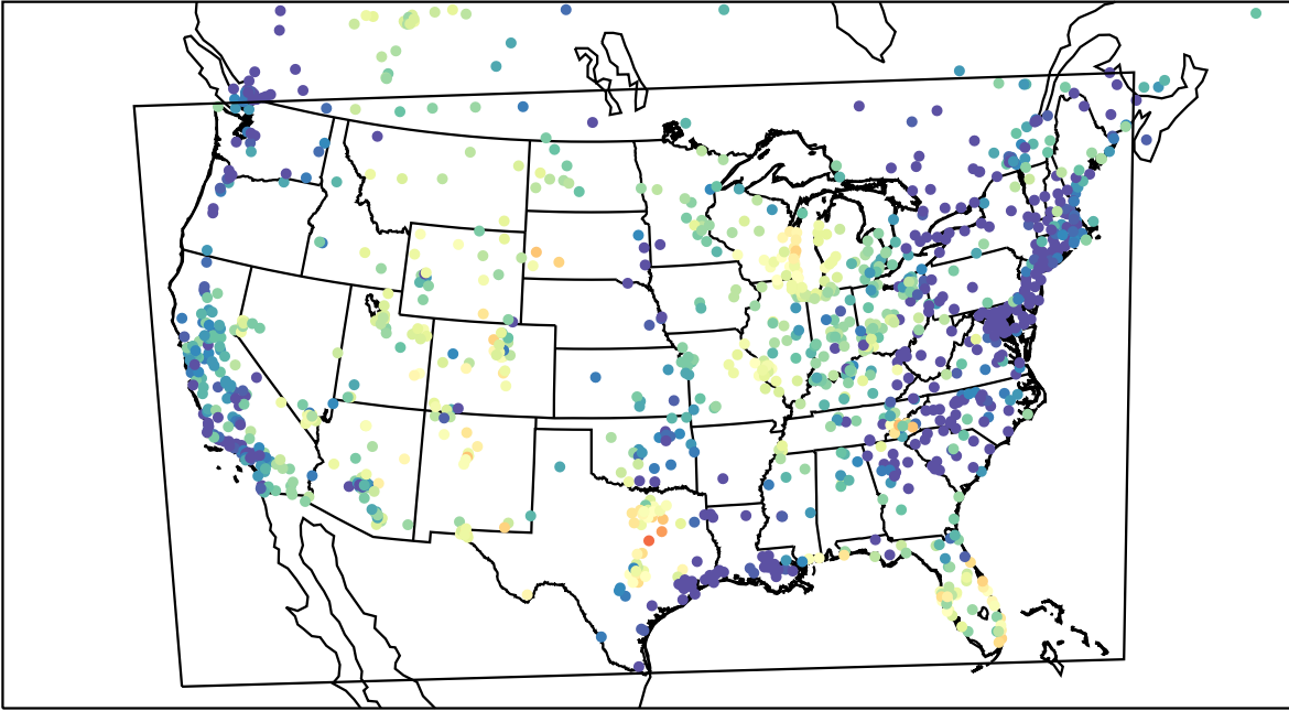
AirNOW (2023-05-06_06:00:00)
