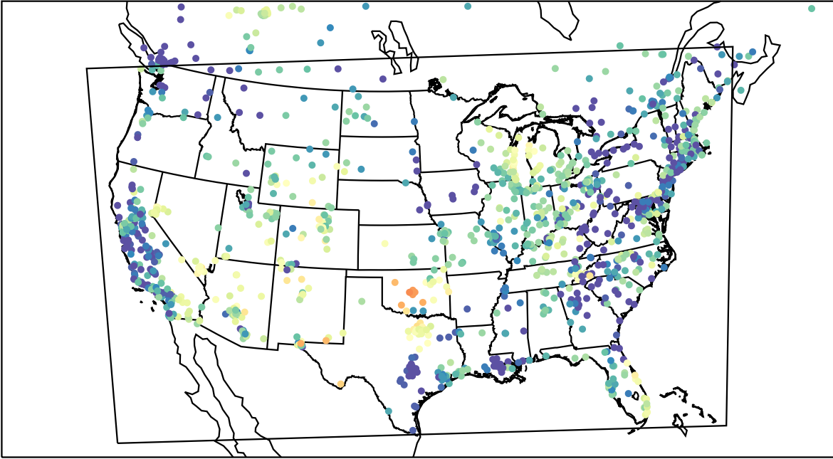
AirNOW (2023-05-07_06:00:00)
