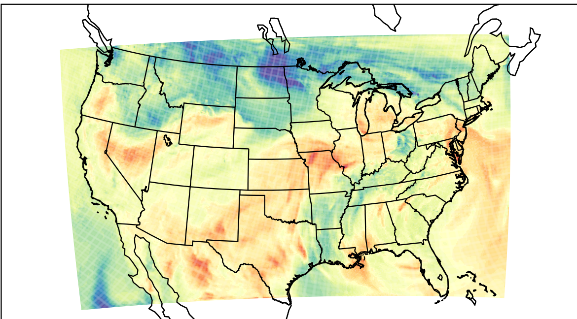
WRF (2023-05-07_19:00:00)
