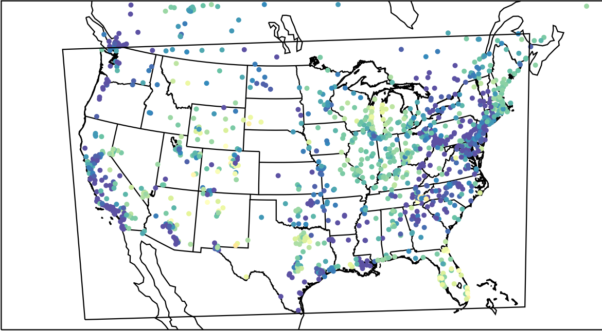
AirNOW (2023-05-06_12:00:00)
