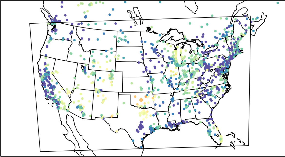
AirNOW (2023-05-07_07:00:00)
