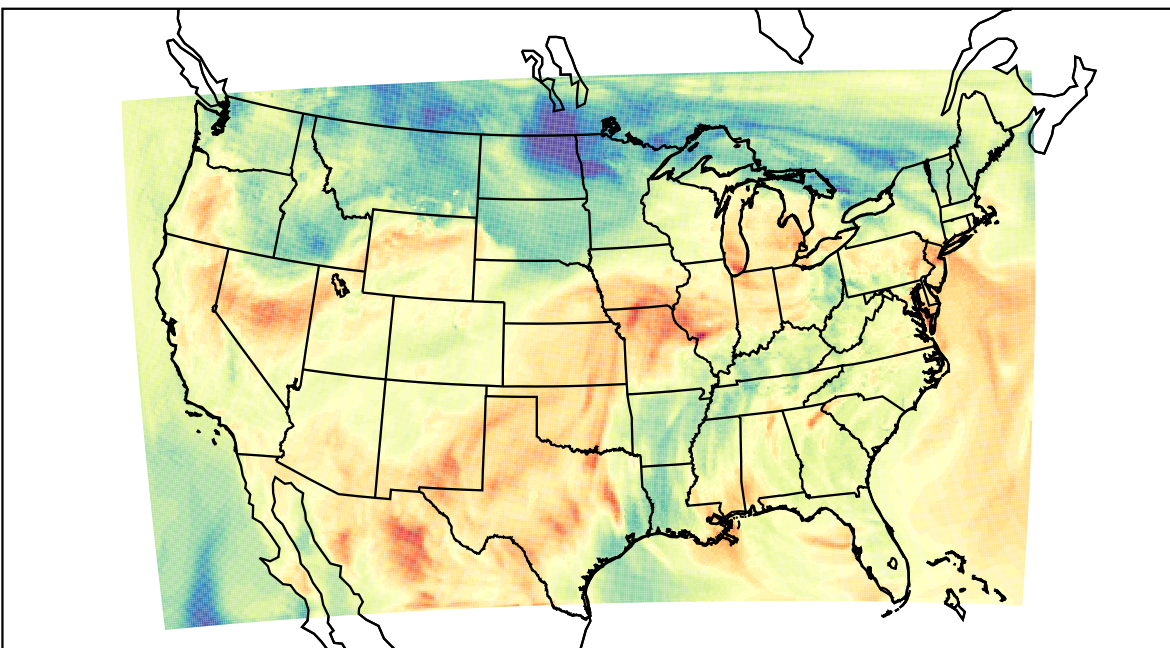
WRF (2023-05-07_20:00:00)
