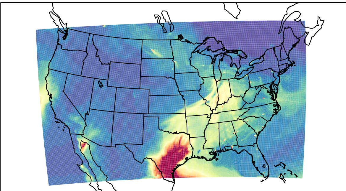
WRF 2023-05-08_21:00:00
