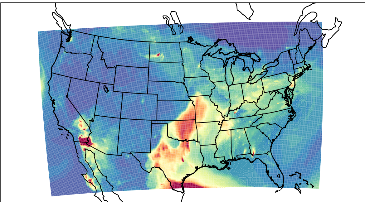
WRF 2023-05-08_06:00:00
