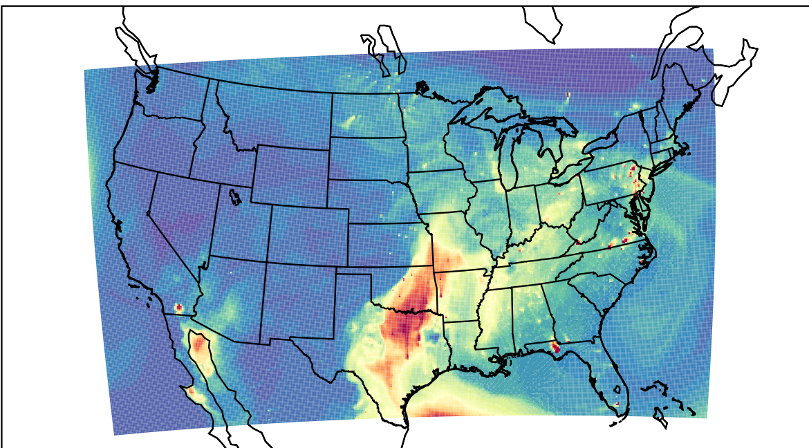
WRF 2023-05-08_00:00:00
