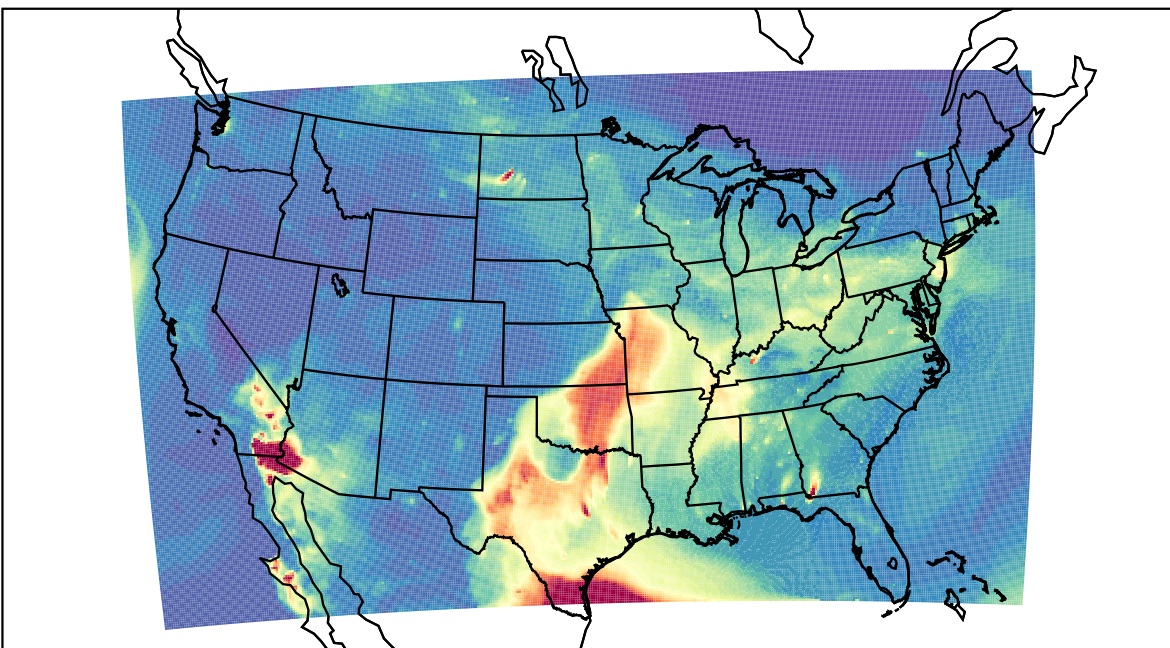
WRF 2023-05-08_07:00:00
