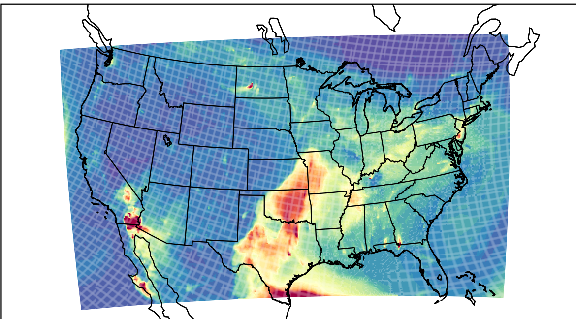
WRF 2023-05-08_05:00:00
