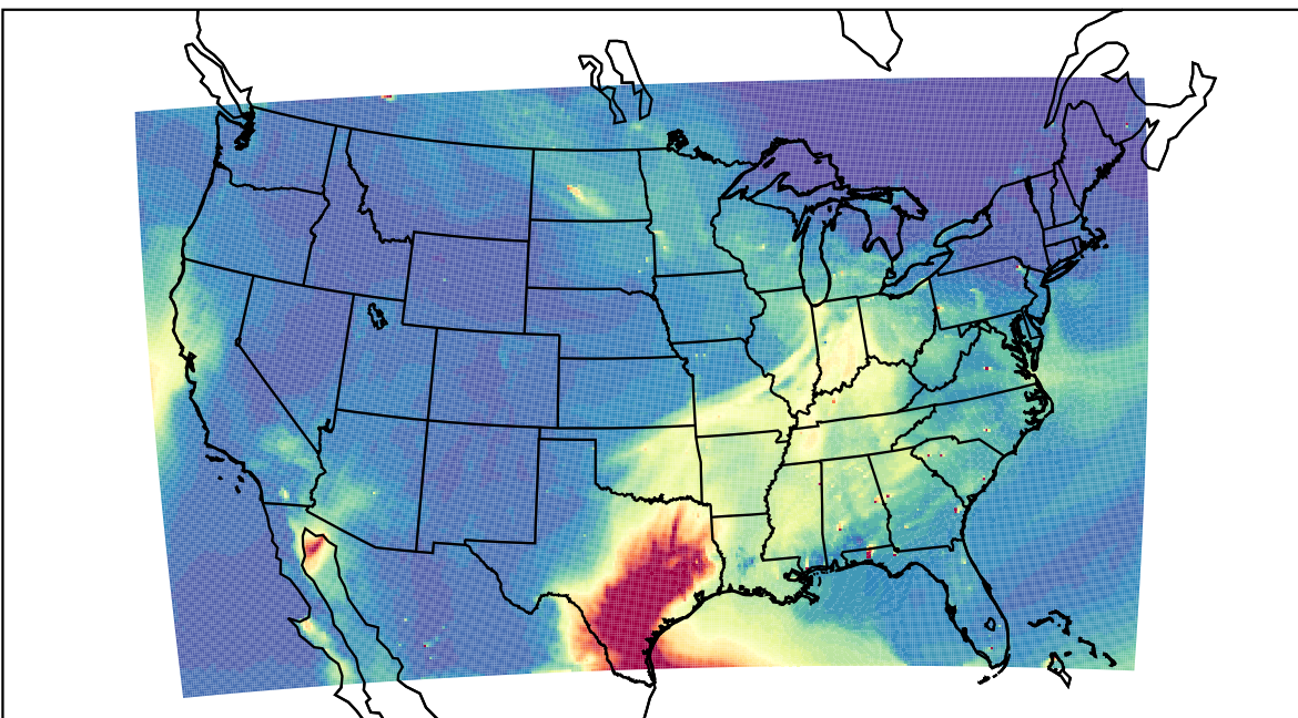
WRF 2023-05-08_22:00:00
