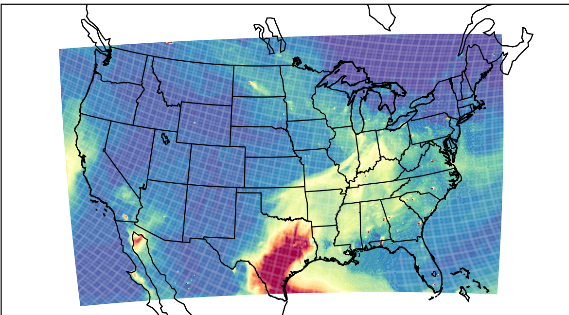
WRF 2023-05-08_23:00:00
