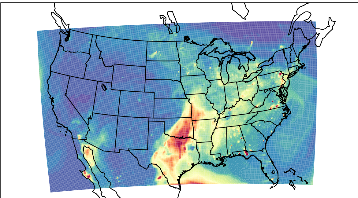
WRF 2023-05-08_01:00:00
