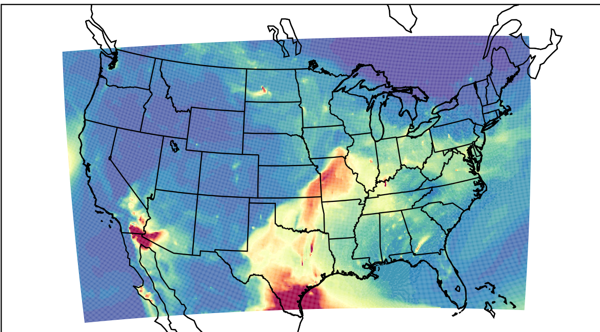
WRF 2023-05-08_12:00:00
