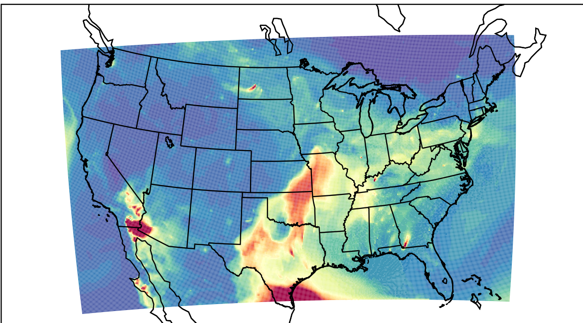
WRF 2023-05-08_08:00:00
