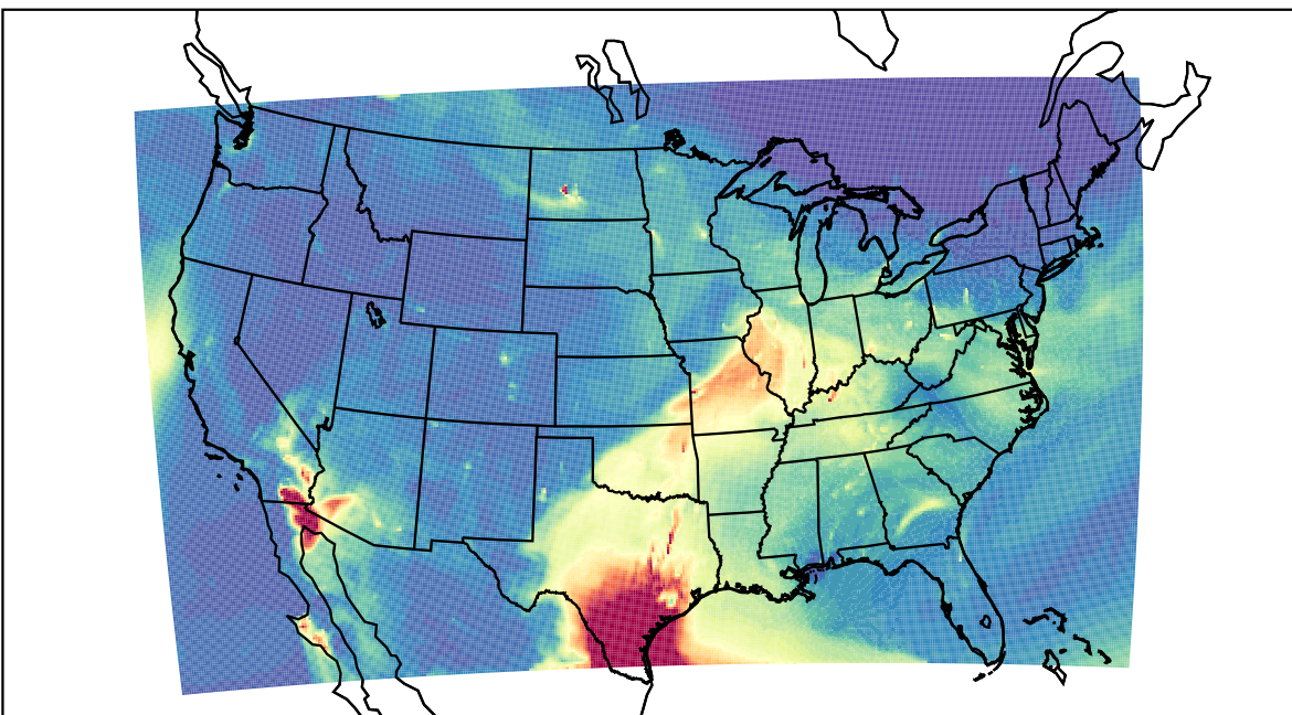
WRF 2023-05-08_15:00:00
