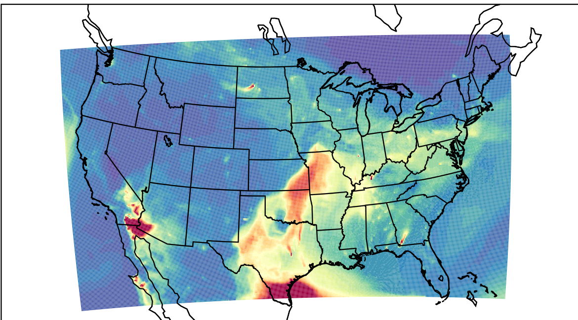
WRF 2023-05-08_09:00:00
