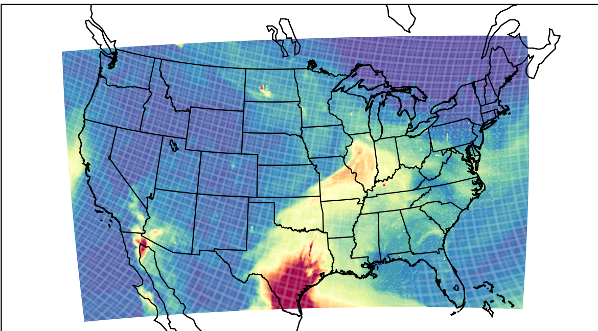
WRF 2023-05-08_17:00:00
