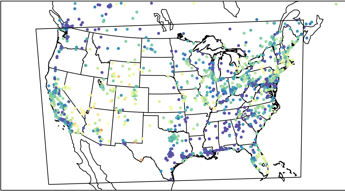
AirNOW (2023-05-09_05:00:00)
