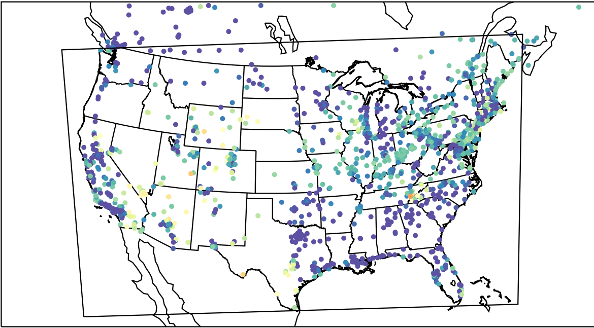
AirNOW (2023-05-09_11:00:00)
