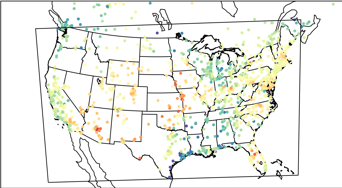
AirNOW (2023-05-08_22:00:00)
