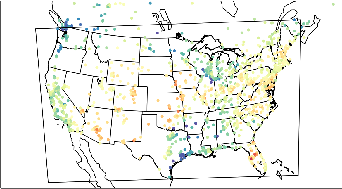
AirNOW (2023-05-08_19:00:00)
