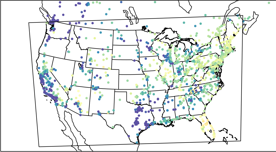
AirNOW (2023-05-08_14:00:00)
