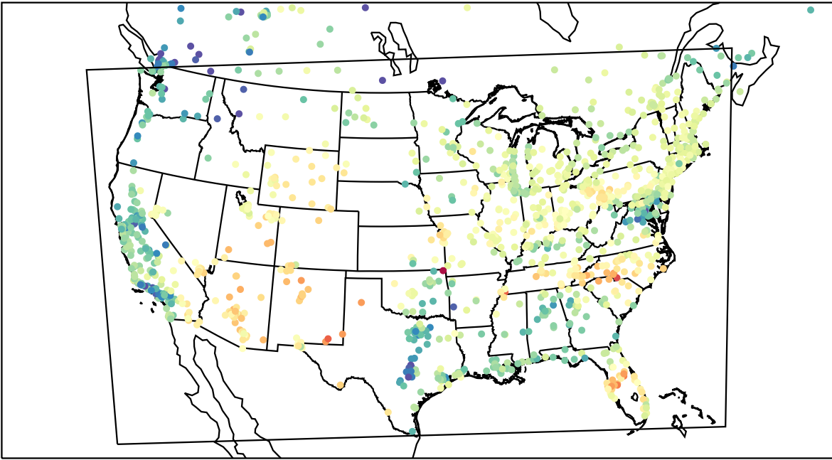
AirNOW (2023-05-09_17:00:00)
