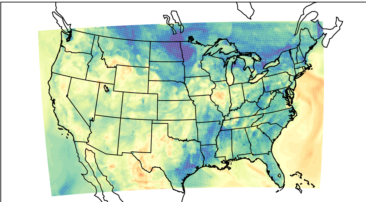
WRF (2023-05-08_02:00:00)
