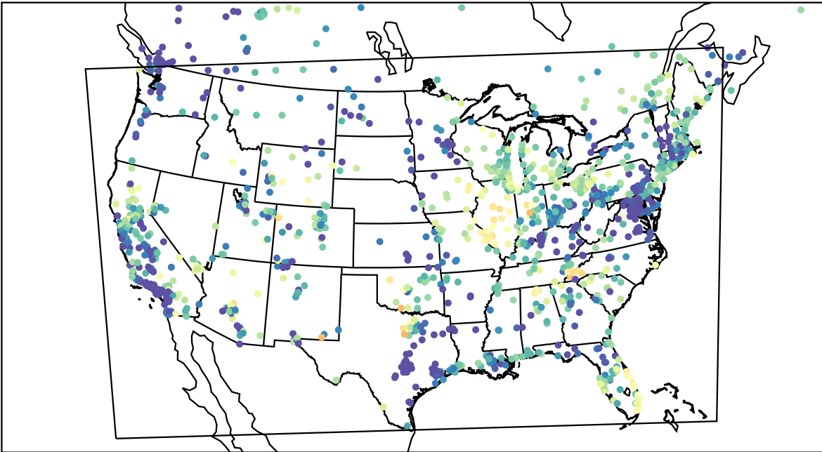
AirNOW (2023-05-08_08:00:00)
