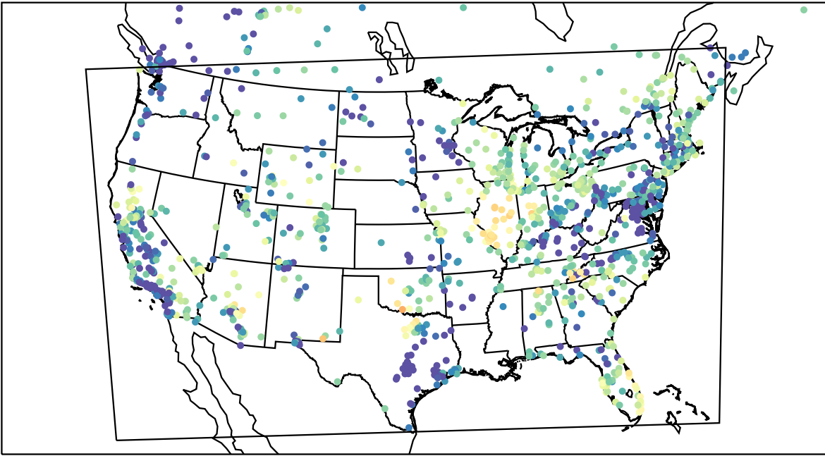
AirNOW (2023-05-08_07:00:00)
