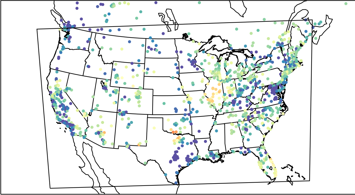
AirNOW (2023-05-08_06:00:00)
