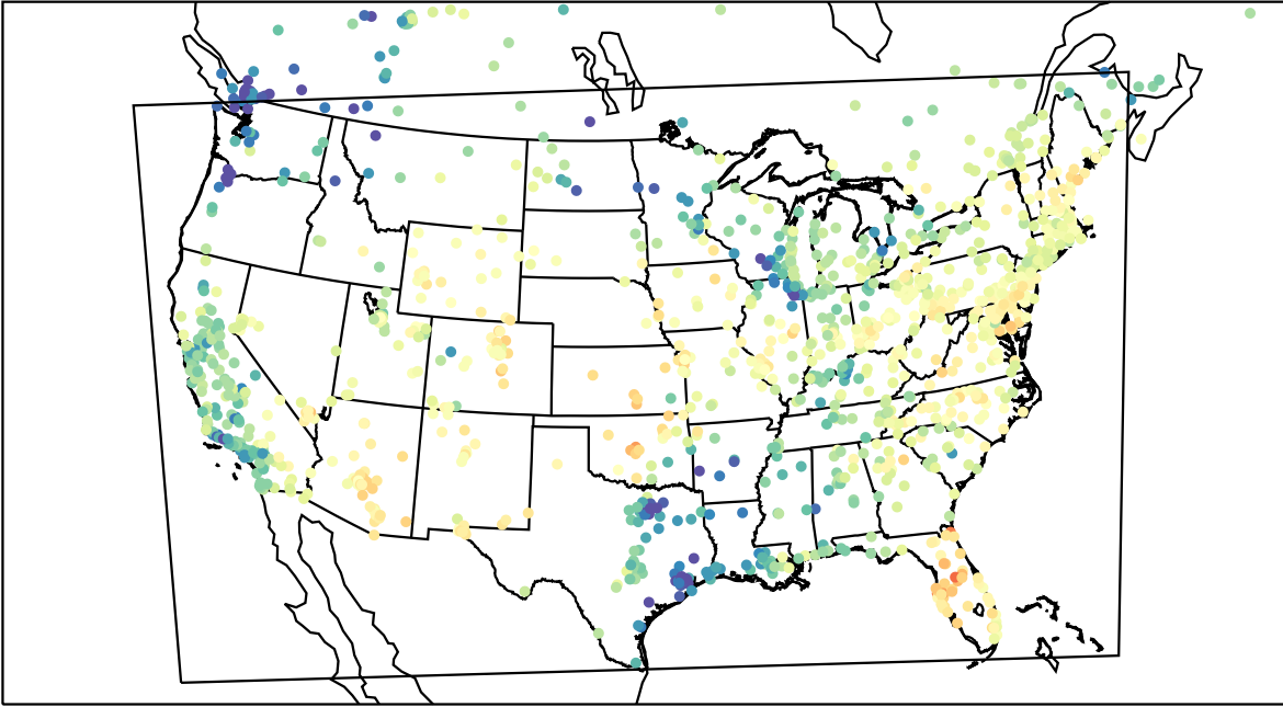
AirNOW (2023-05-08_17:00:00)
