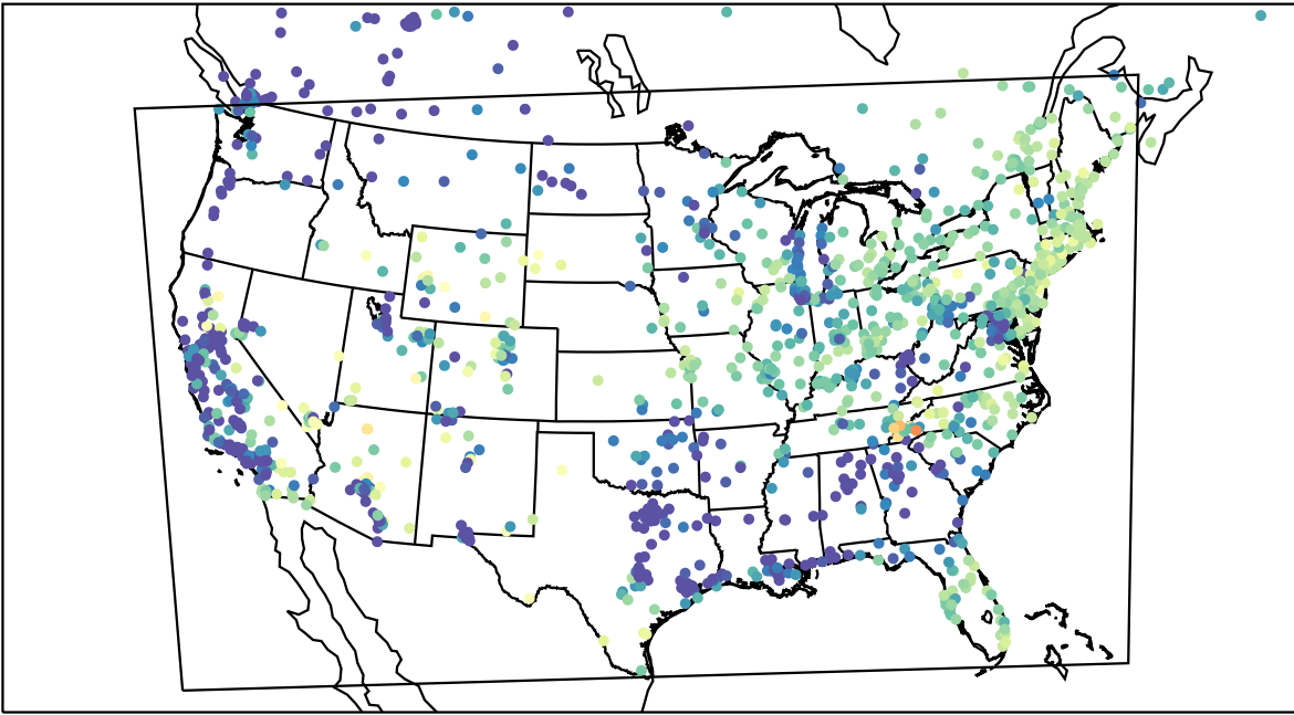
AirNOW (2023-05-09_13:00:00)
