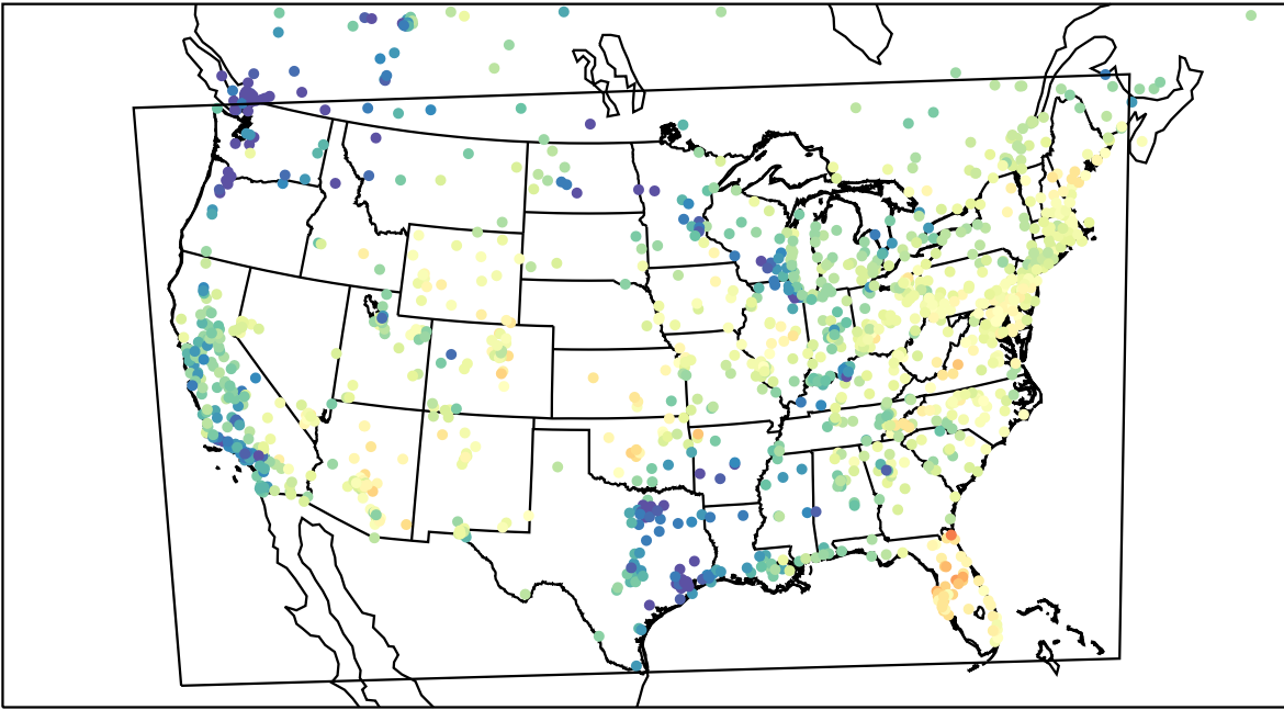
AirNOW (2023-05-08_16:00:00)
