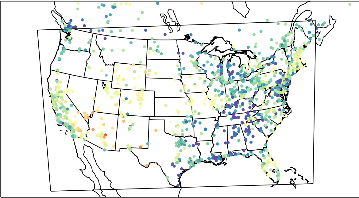
AirNOW (2023-05-09_02:00:00)
