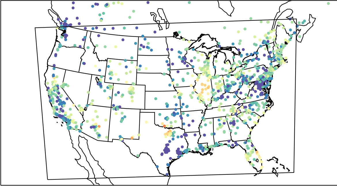
AirNOW (2023-05-08_05:00:00)
