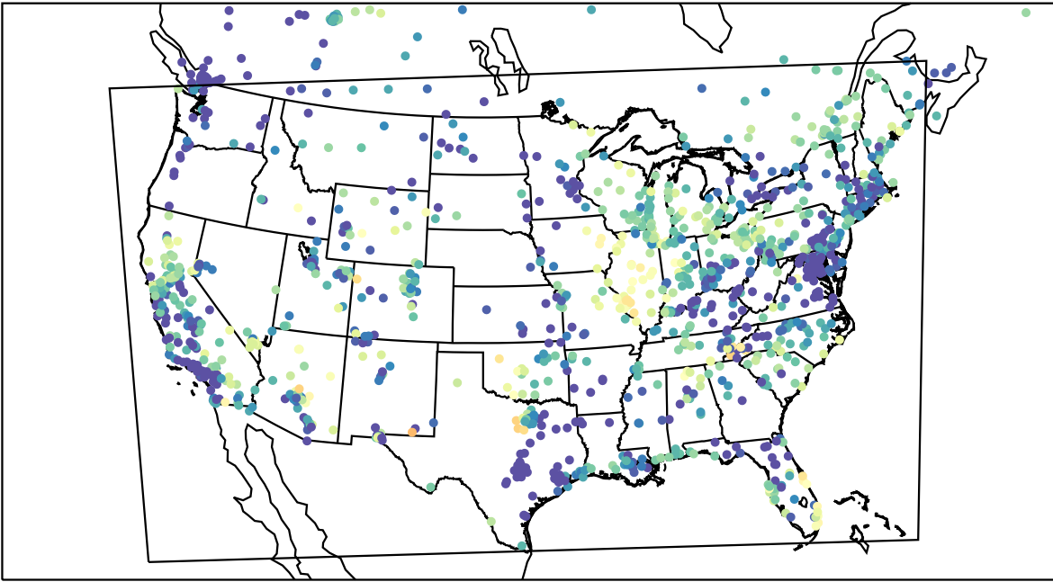
AirNOW (2023-05-08_09:00:00)
