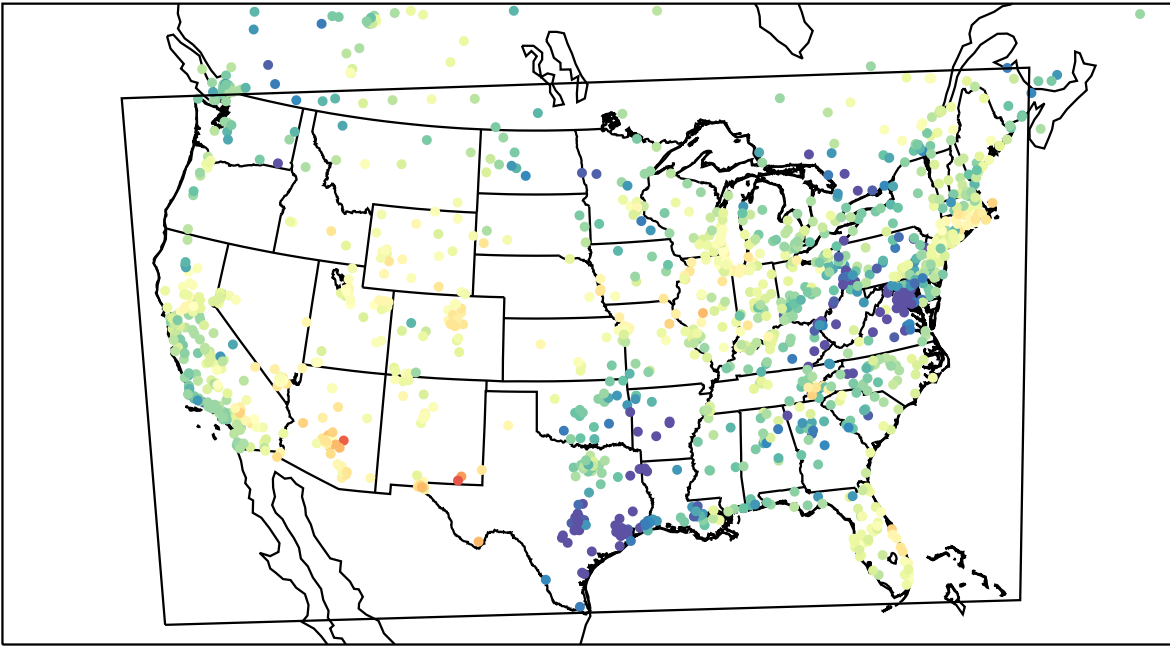
AirNOW (2023-05-08_01:00:00)
