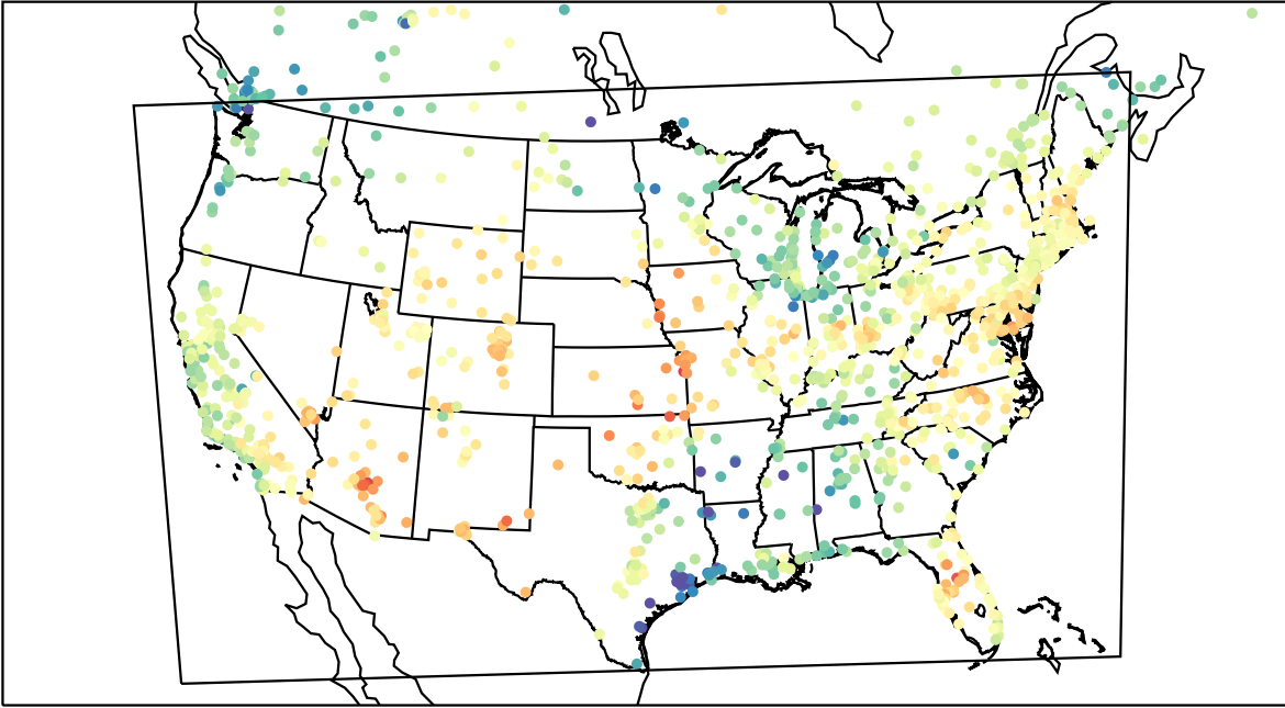
AirNOW (2023-05-08_21:00:00)
