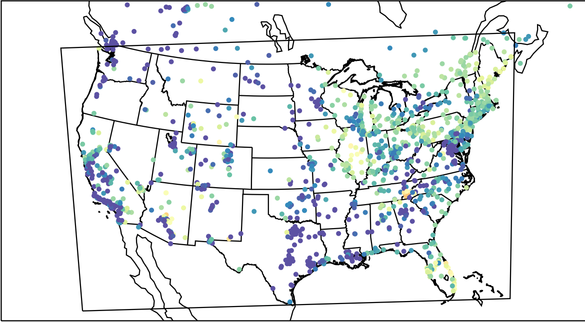
AirNOW (2023-05-08_12:00:00)
