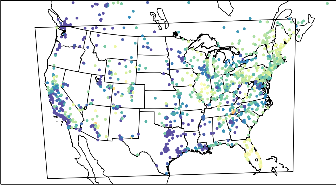
AirNOW (2023-05-08_13:00:00)
