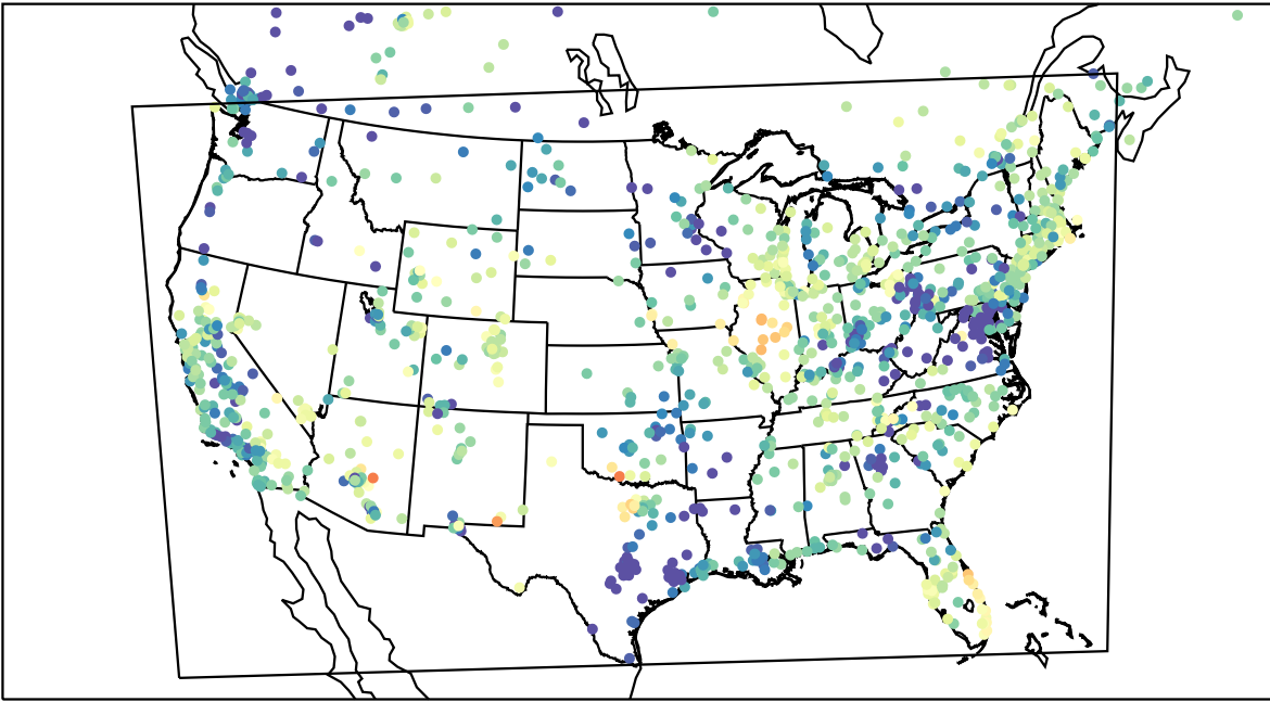
AirNOW (2023-05-08_04:00:00)
