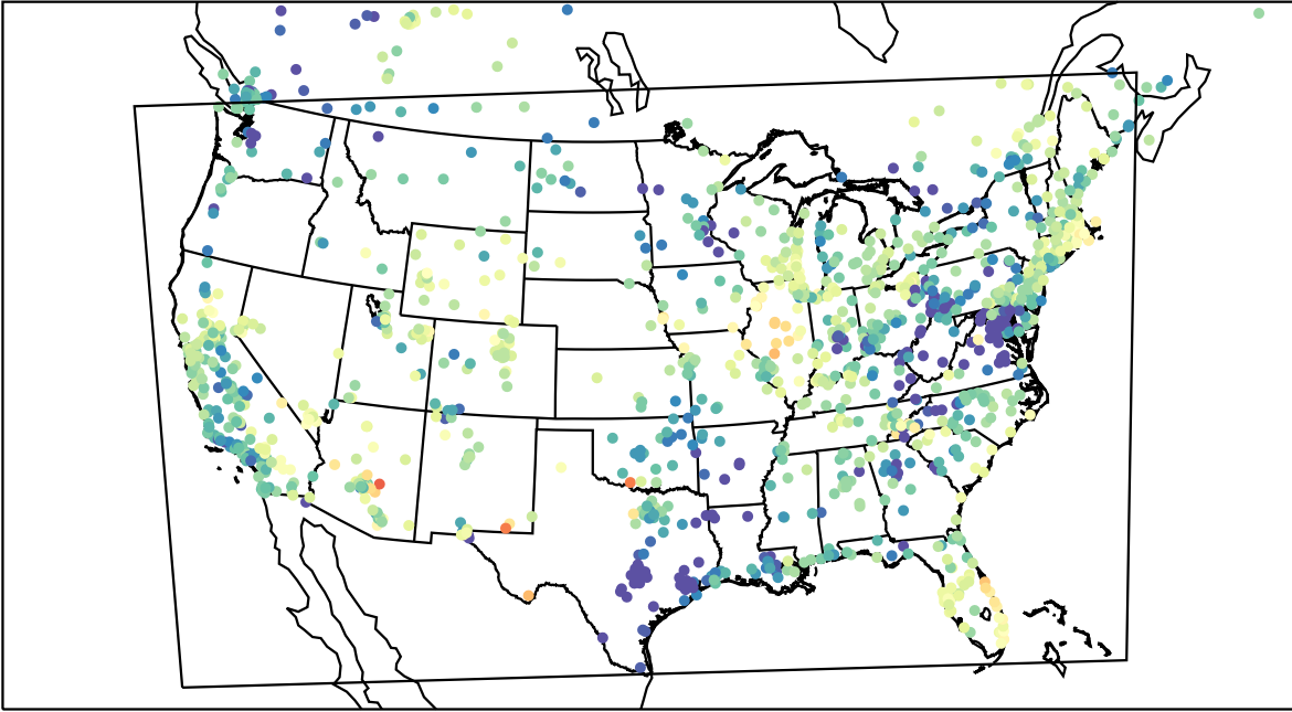
AirNOW (2023-05-08_03:00:00)
