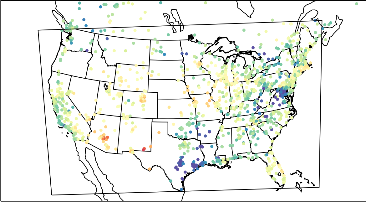
AirNOW (2023-05-08_00:00:00)
