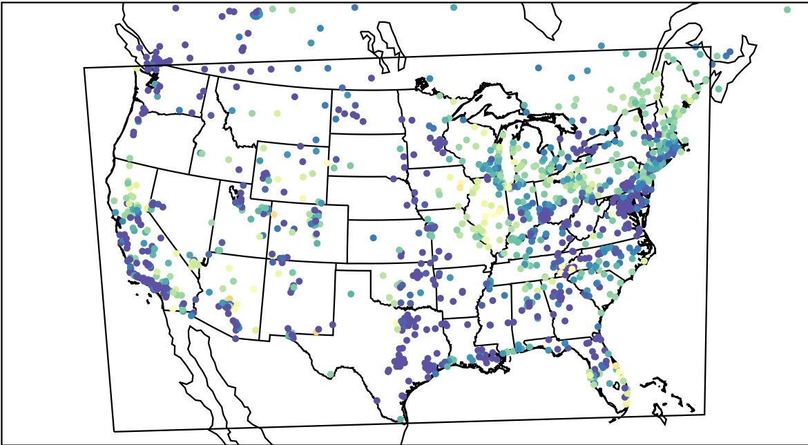
AirNOW (2023-05-08_11:00:00)
