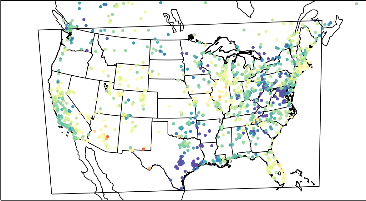
AirNOW (2023-05-08_02:00:00)
