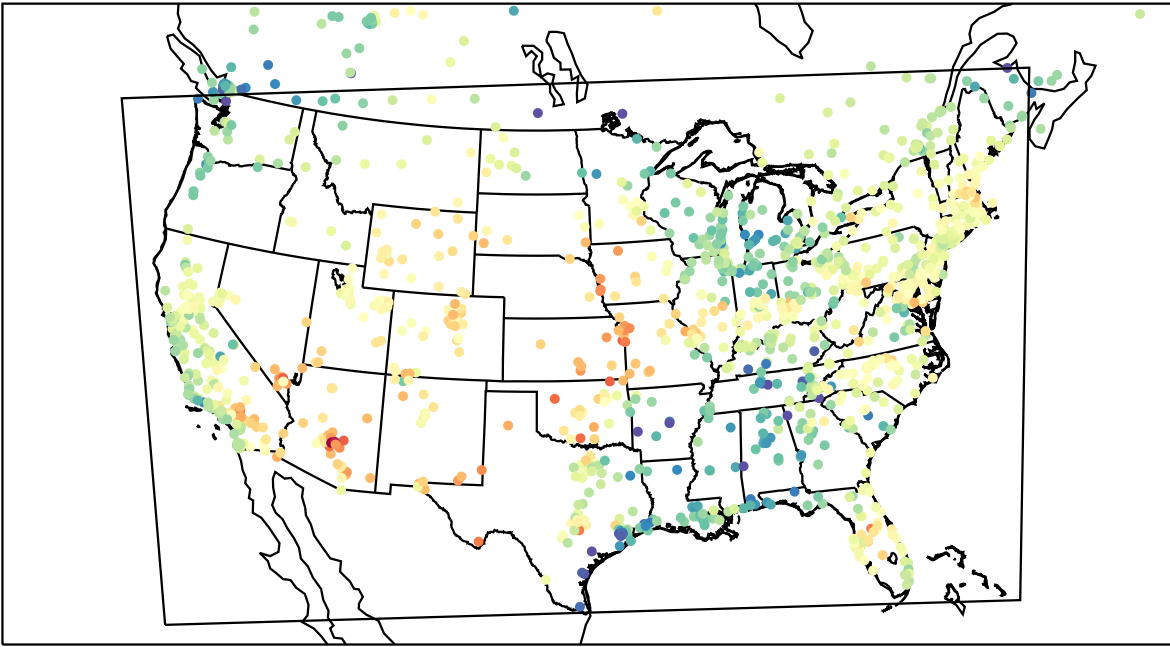
AirNOW (2023-05-08_23:00:00)
