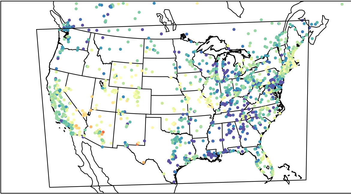
AirNOW (2023-05-09_03:00:00)
