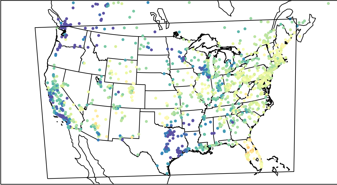
AirNOW (2023-05-08_15:00:00)
