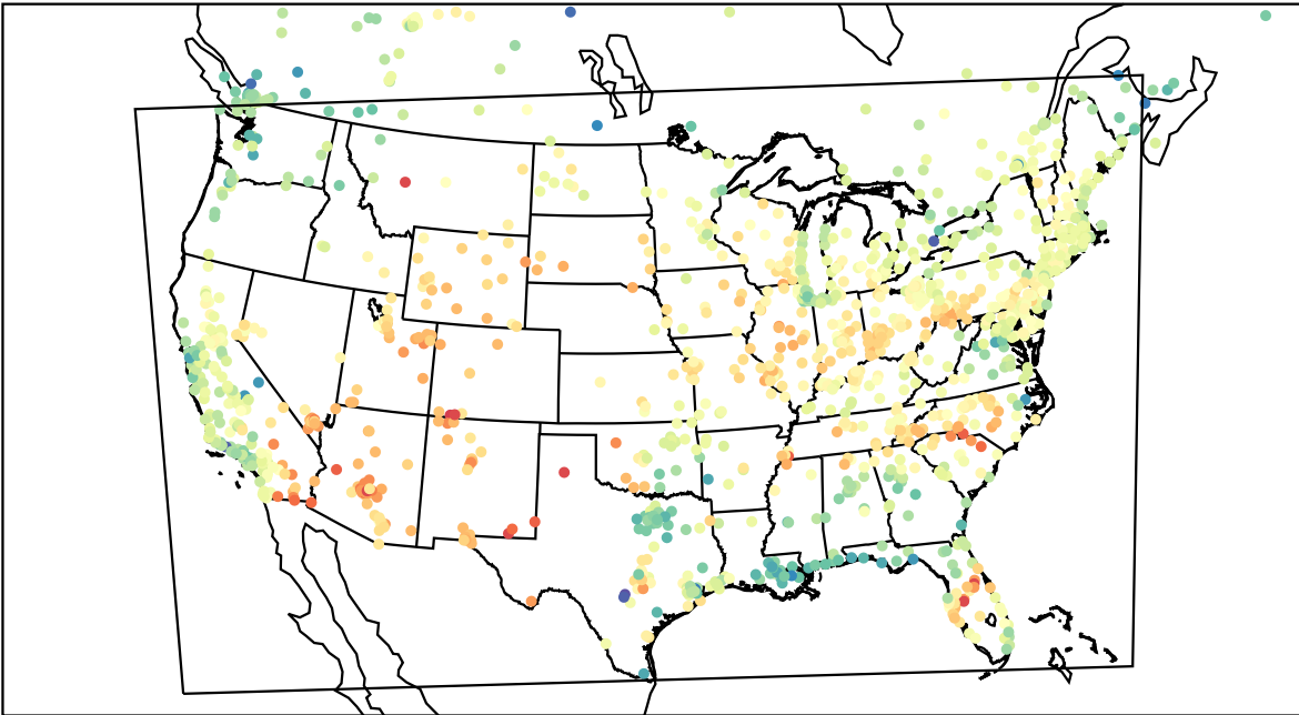
AirNOW (2023-05-09_21:00:00)
