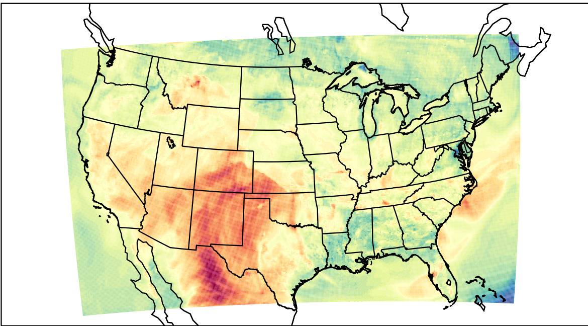
WRF (2023-05-09_23:00:00)
