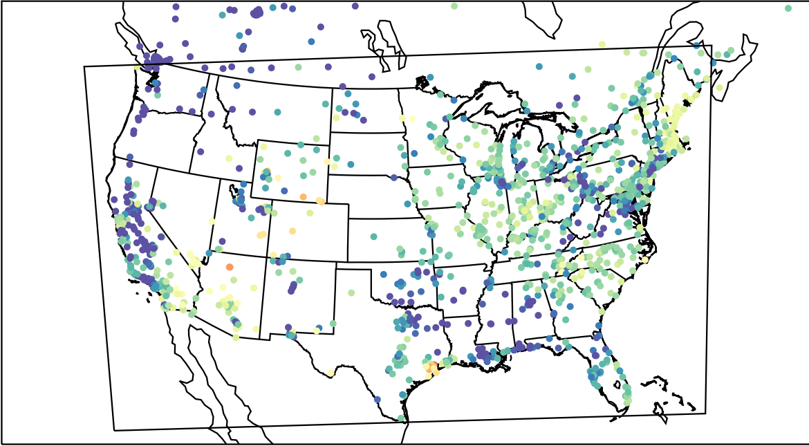
AirNOW (2023-05-10_13:00:00)
