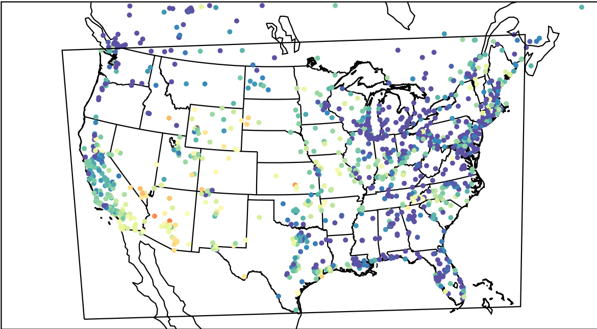
AirNOW (2023-05-10_07:00:00)
