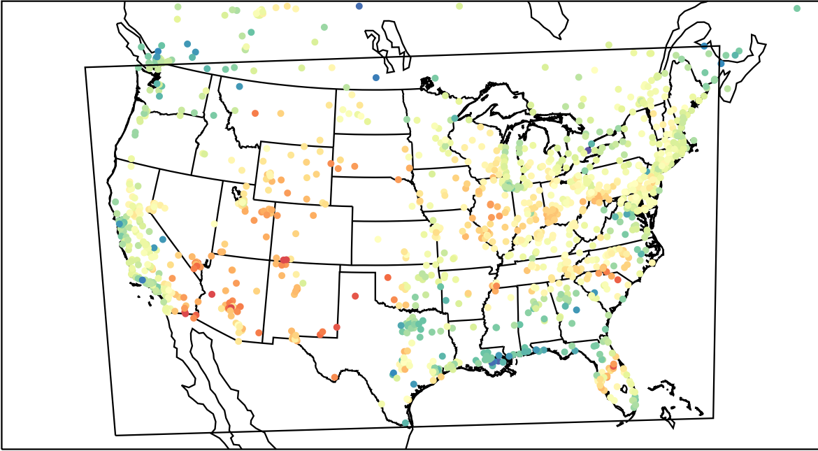
AirNOW (2023-05-09_22:00:00)
