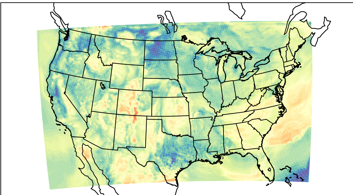
WRF (2023-05-10_15:00:00)
