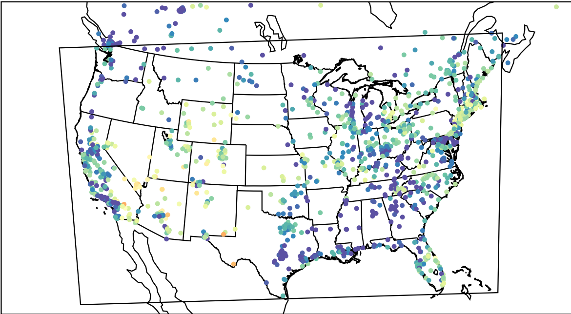
AirNOW (2023-05-09_06:00:00)
