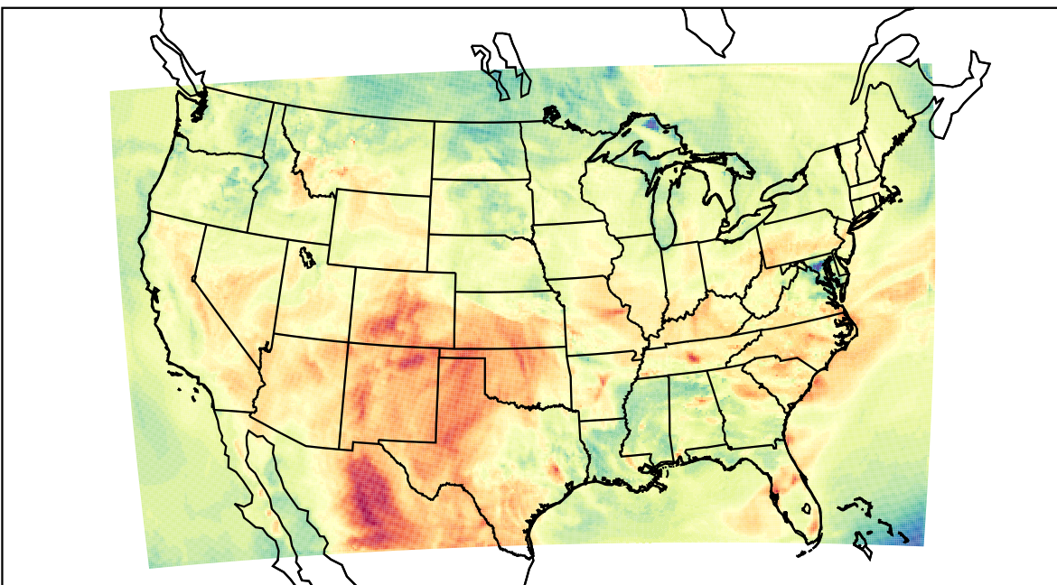
WRF (2023-05-09_19:00:00)
