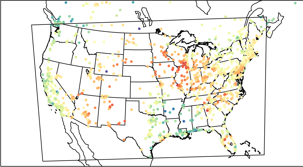
AirNOW (2023-05-10_21:00:00)
