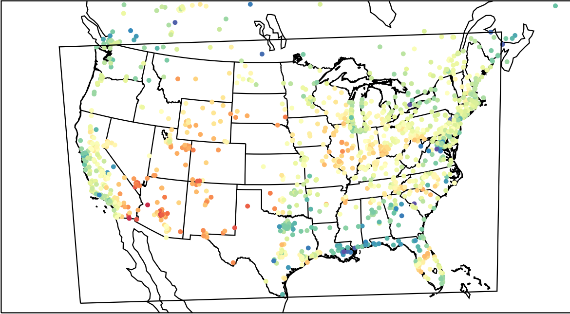
AirNOW (2023-05-09_23:00:00)
