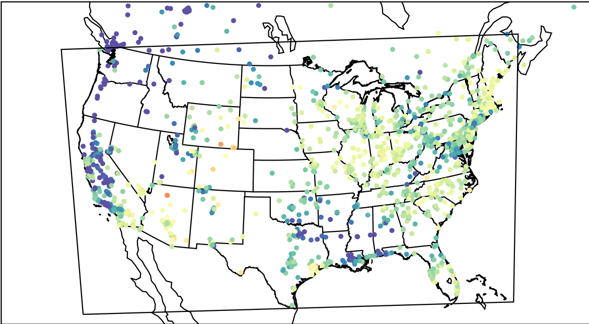
AirNOW (2023-05-10_14:00:00)
