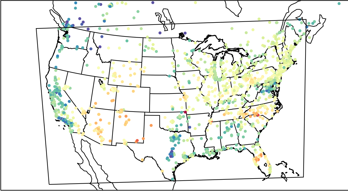
AirNOW (2023-05-09_17:00:00)
