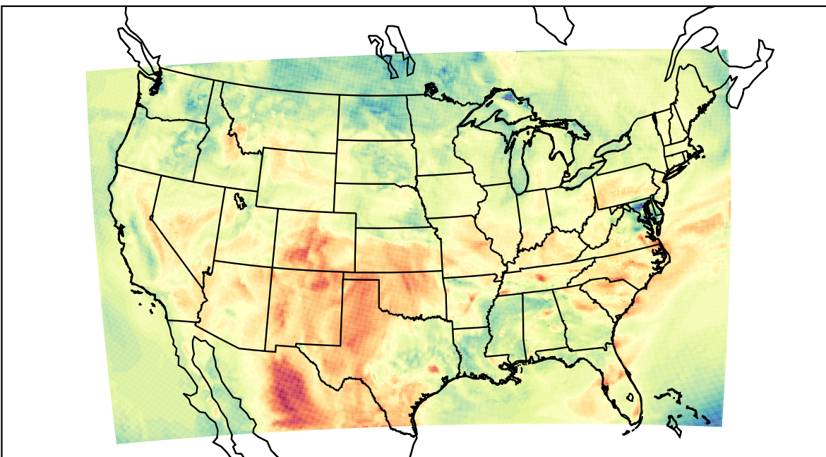
WRF (2023-05-09_18:00:00)
