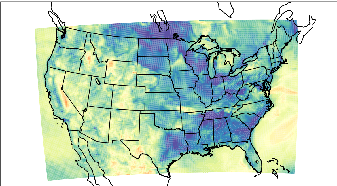
WRF (2023-05-09_09:00:00)
