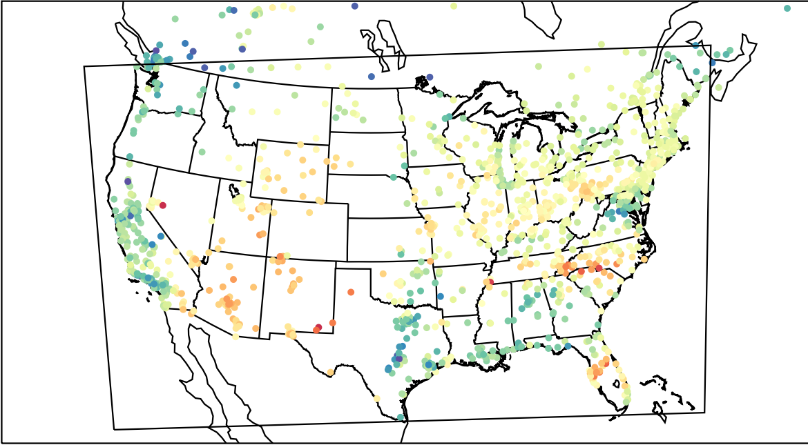
AirNOW (2023-05-09_18:00:00)
