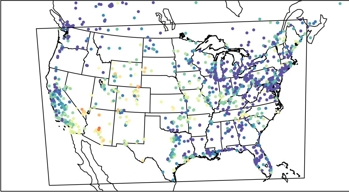
AirNOW (2023-05-10_08:00:00)
