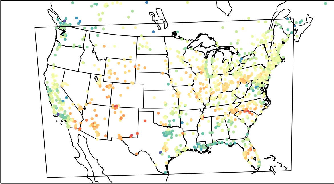
AirNOW (2023-05-09_20:00:00)
