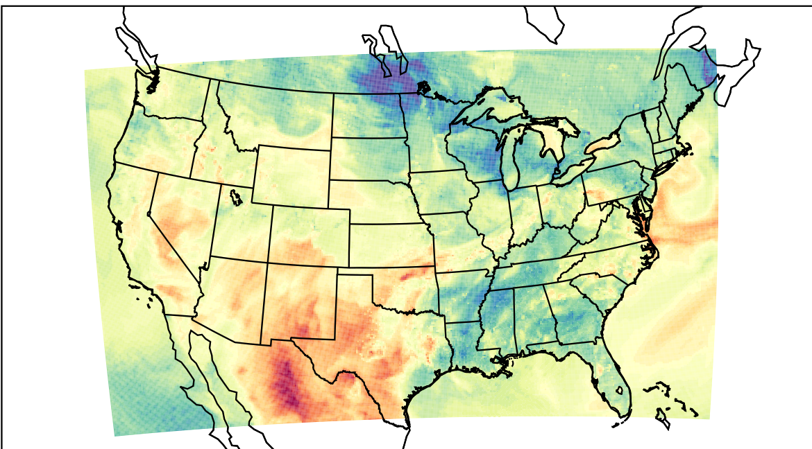
WRF (2023-05-09_00:00:00)
