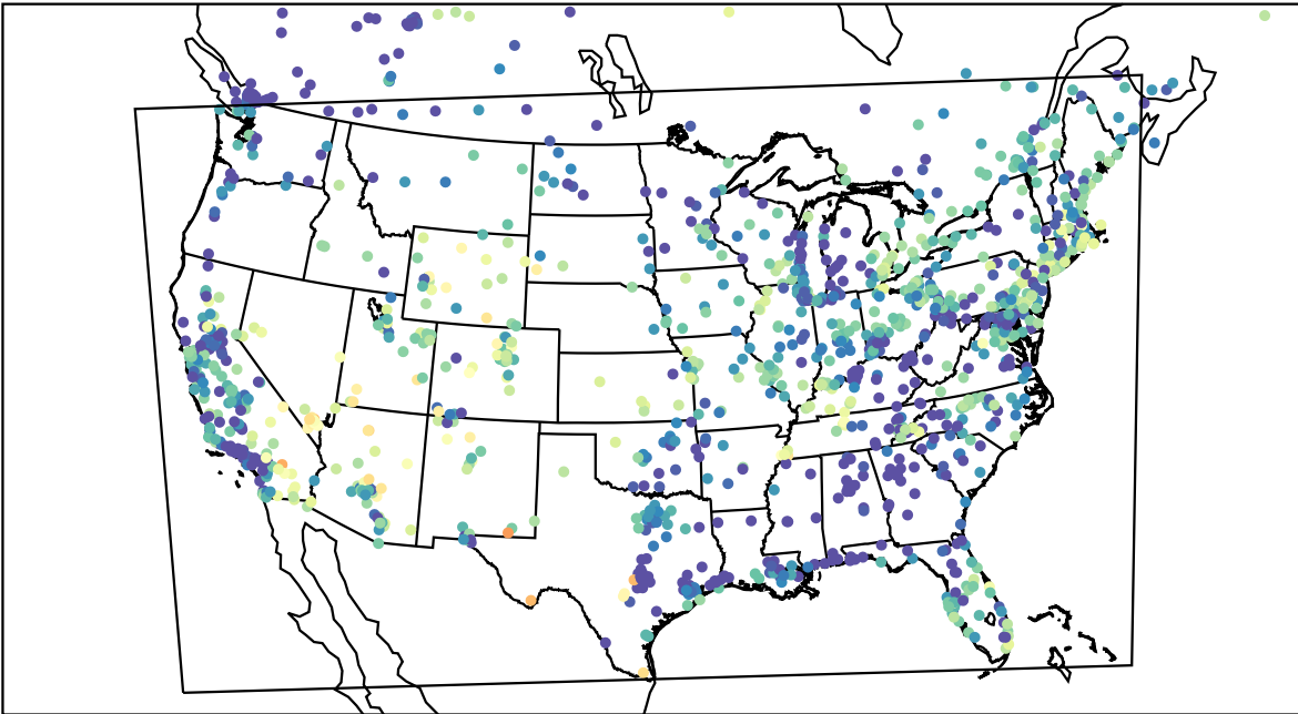
AirNOW (2023-05-09_07:00:00)
