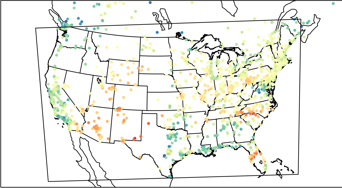
AirNOW (2023-05-09_19:00:00)
