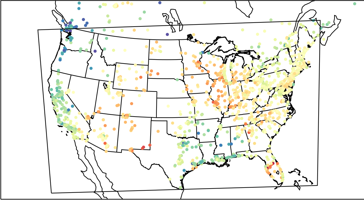
AirNOW (2023-05-10_18:00:00)
