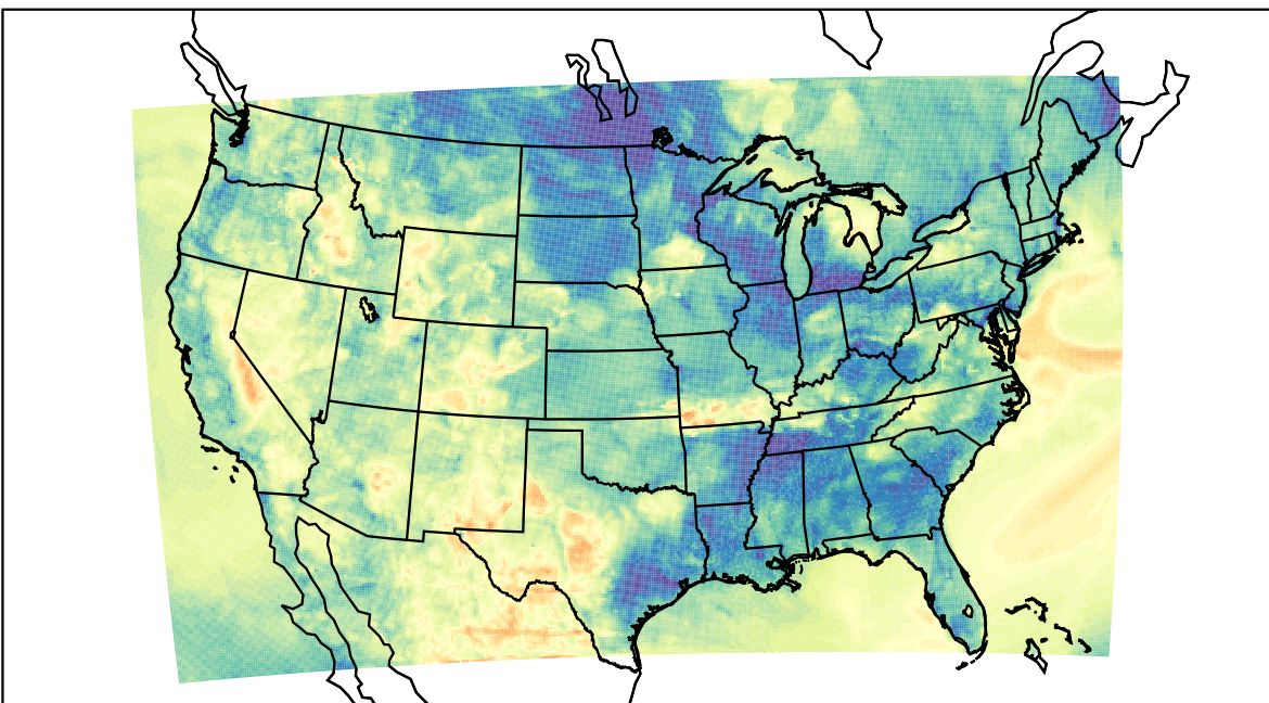
WRF (2023-05-09_05:00:00)
