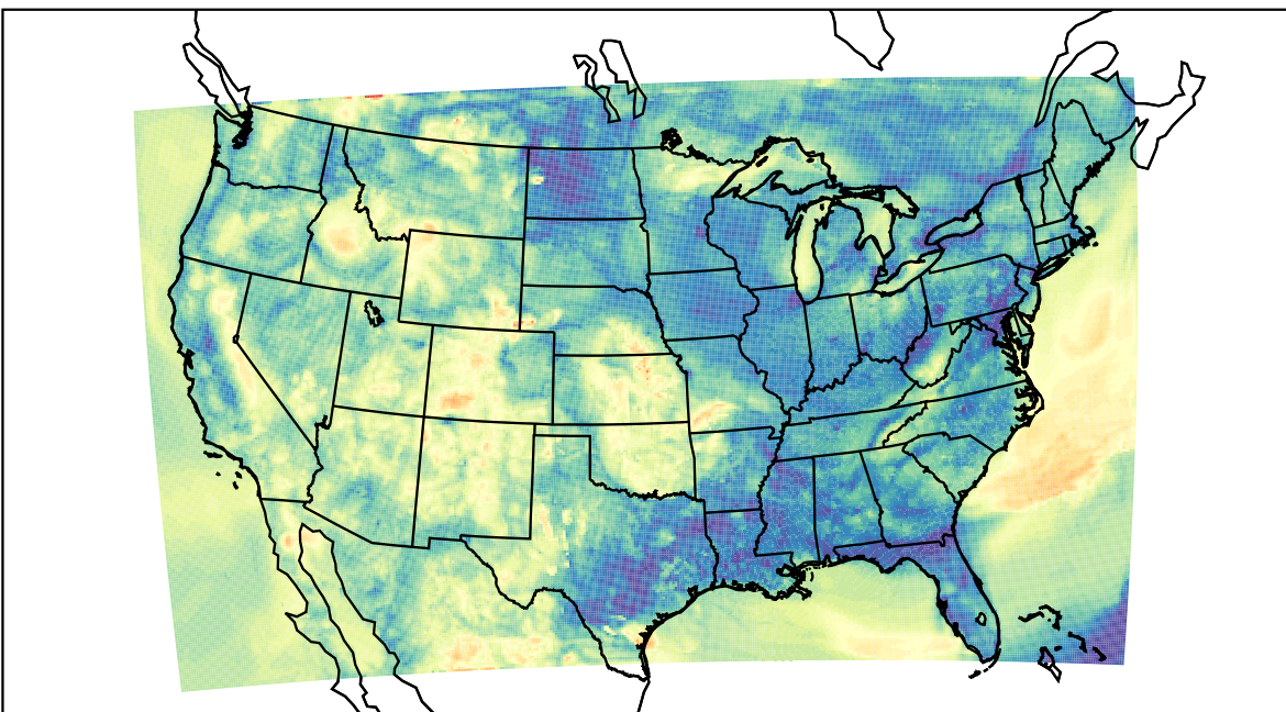
WRF (2023-05-10_11:00:00)
