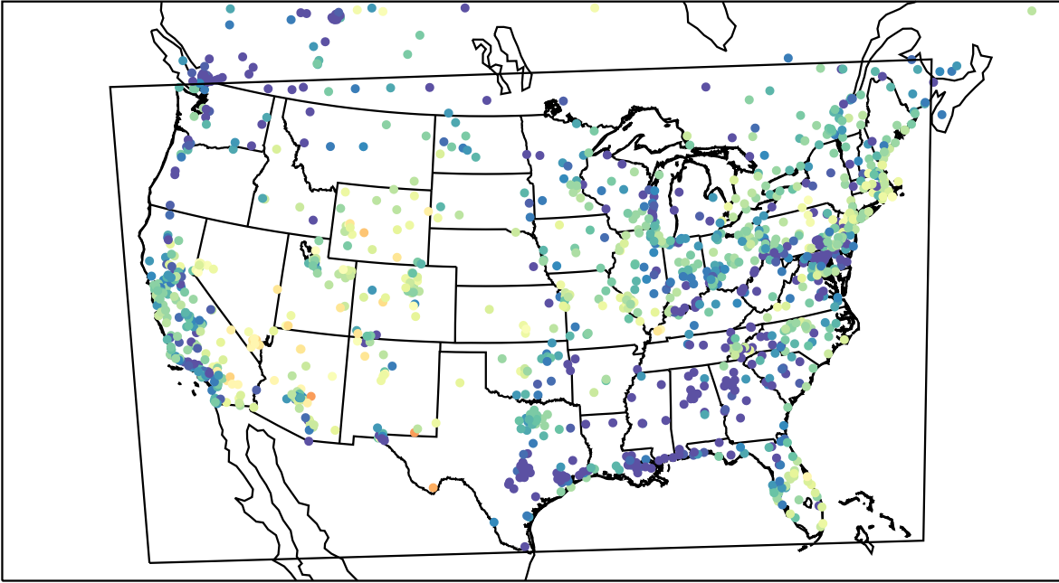
AirNOW (2023-05-09_05:00:00)
