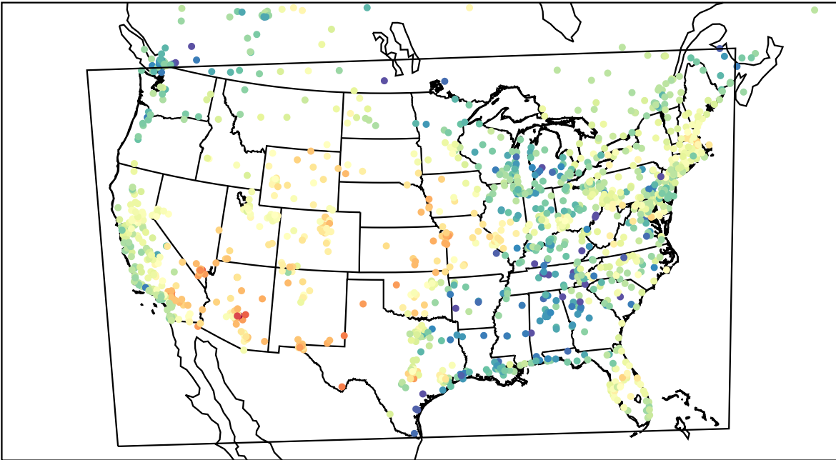
AirNOW (2023-05-09_00:00:00)
