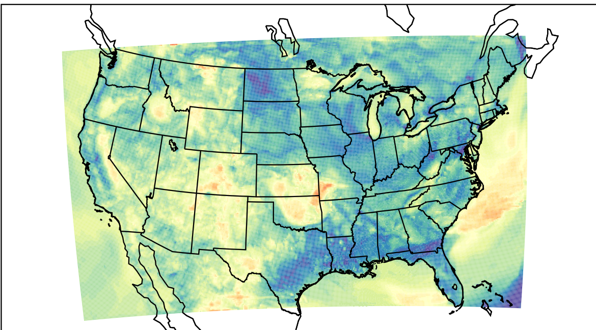
WRF (2023-05-10_08:00:00)
