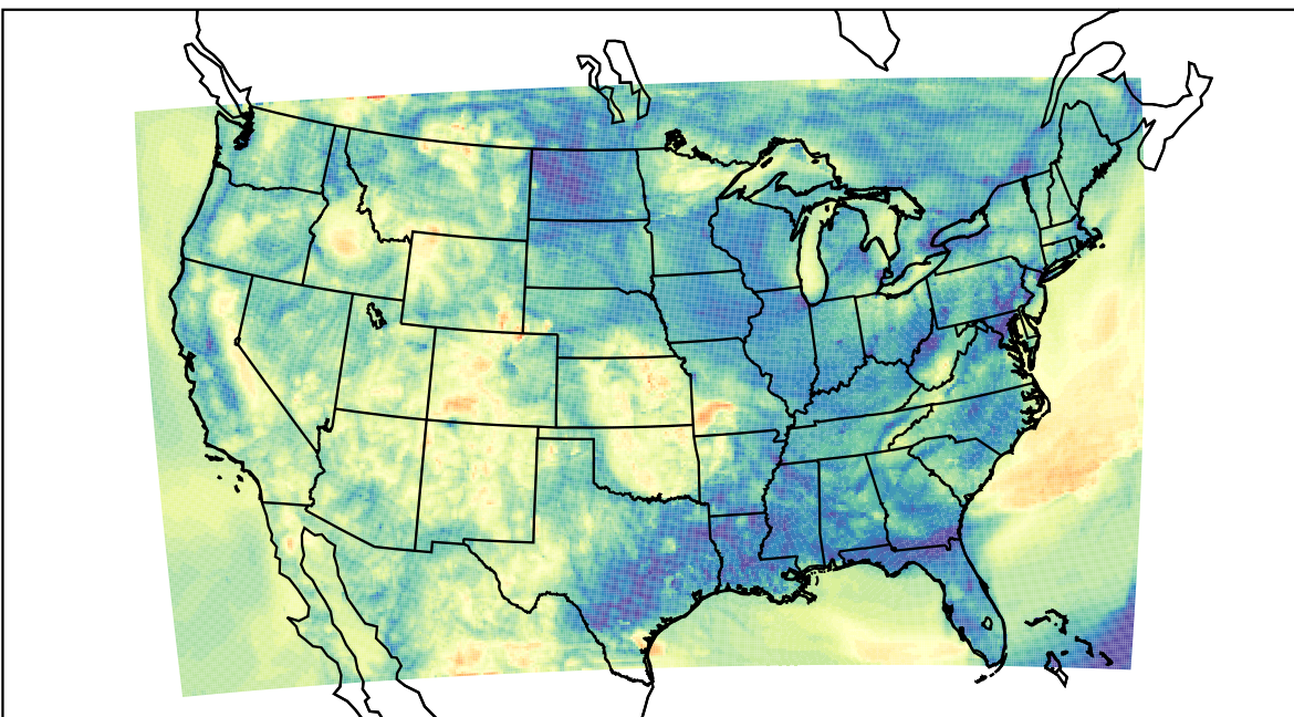
WRF (2023-05-10_10:00:00)
