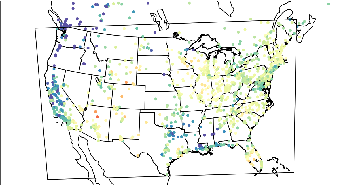
AirNOW (2023-05-10_15:00:00)
