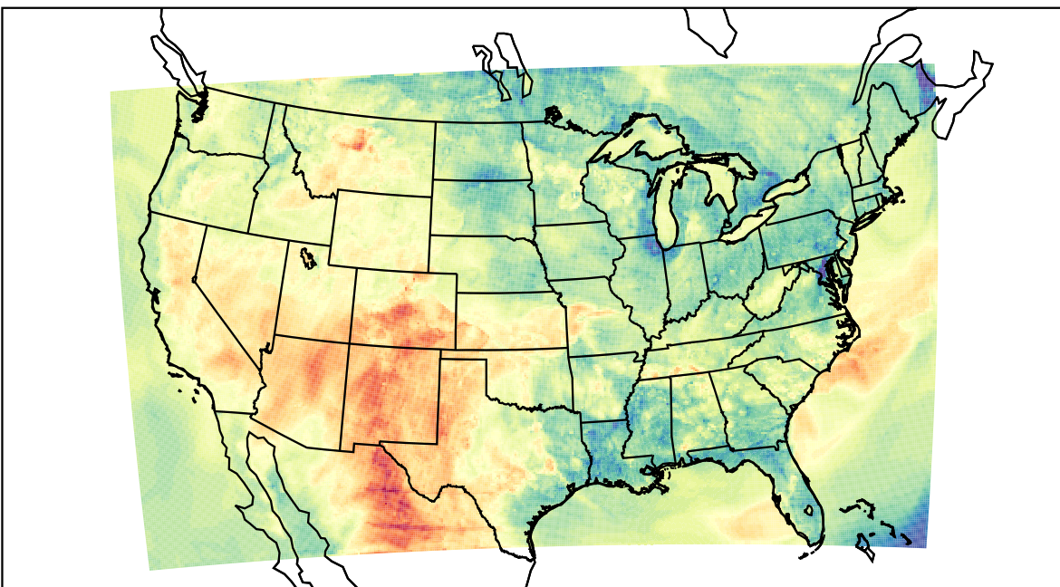
WRF (2023-05-10_01:00:00)
