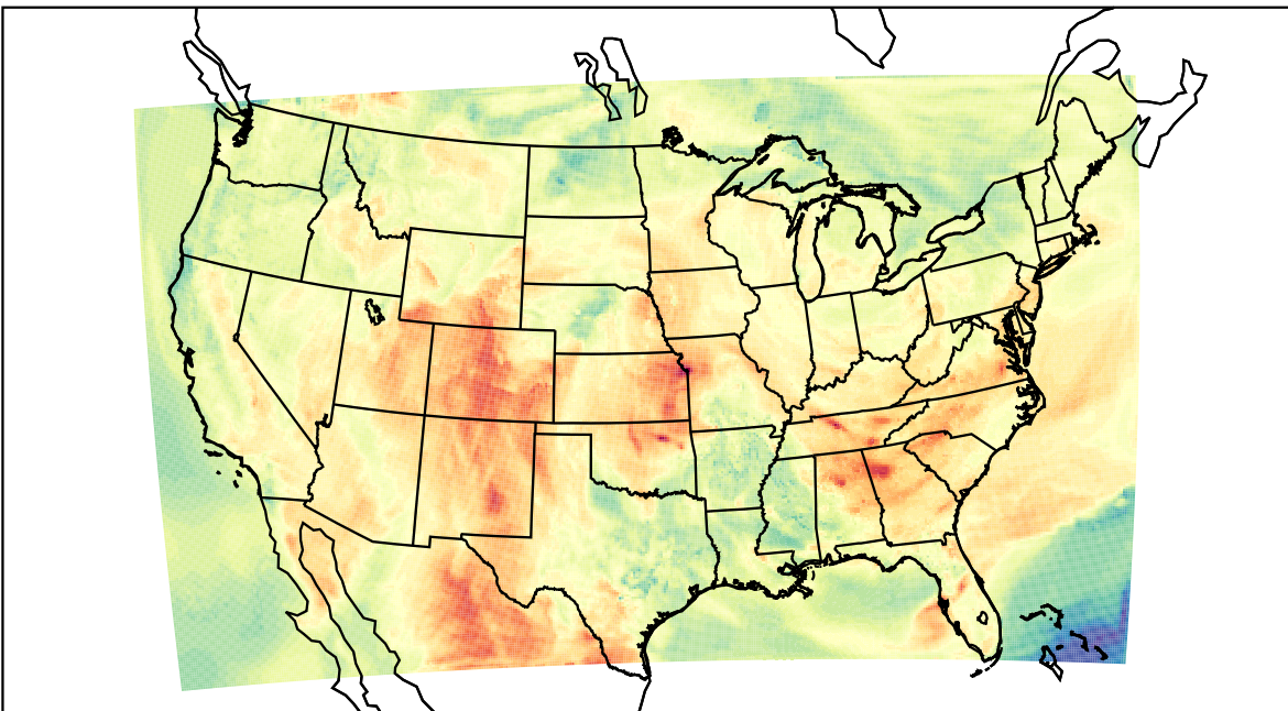
WRF (2023-05-10_19:00:00)
