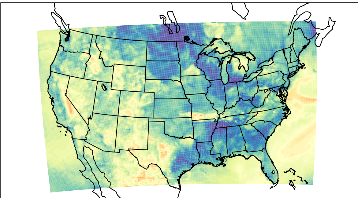
WRF (2023-05-09_06:00:00)
