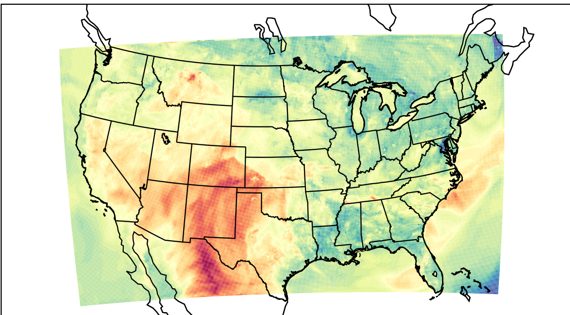
WRF (2023-05-10_00:00:00)
