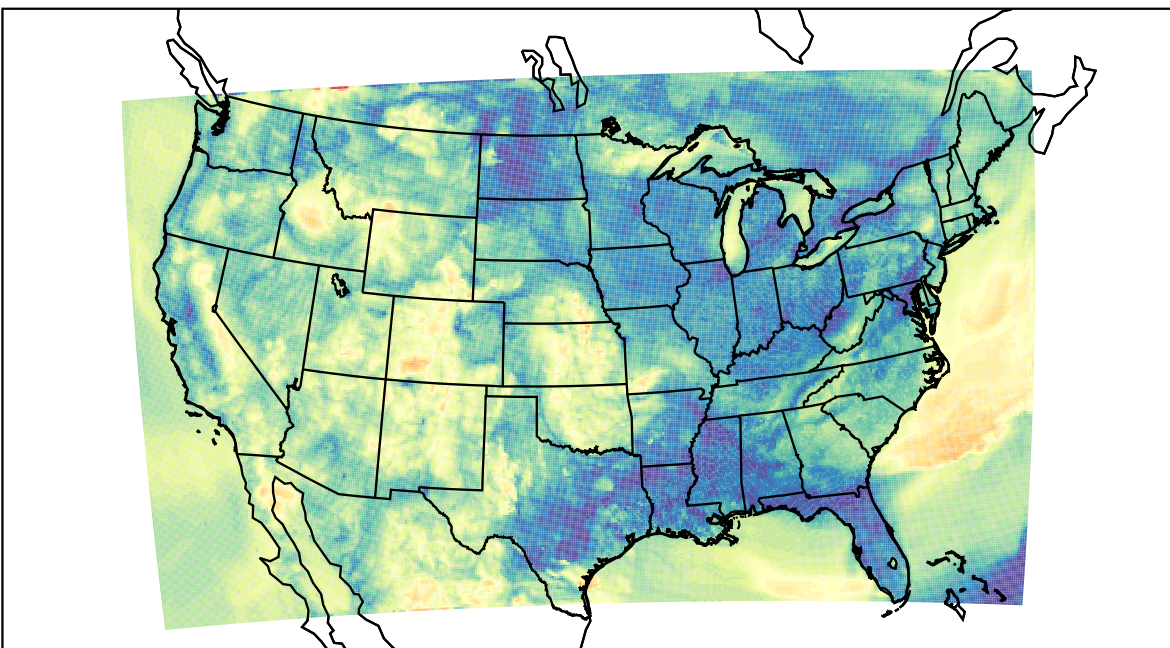
WRF (2023-05-10_12:00:00)
