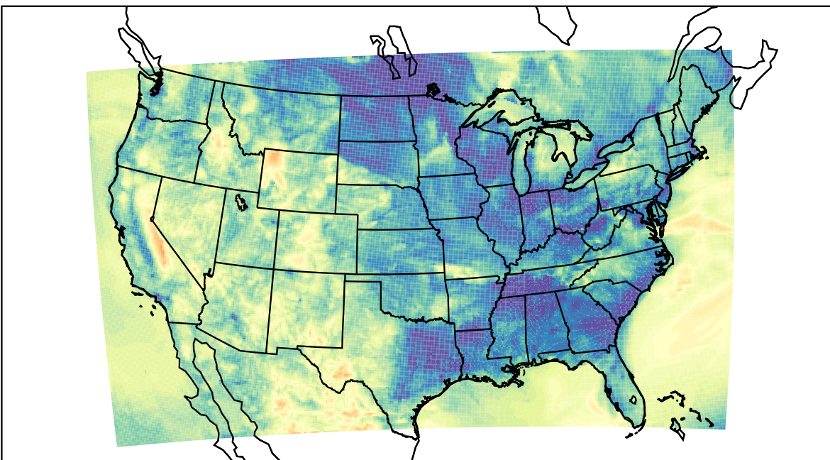
WRF (2023-05-09_10:00:00)
