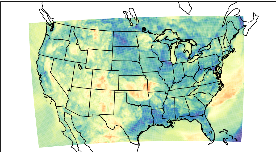
WRF (2023-05-10_06:00:00)
