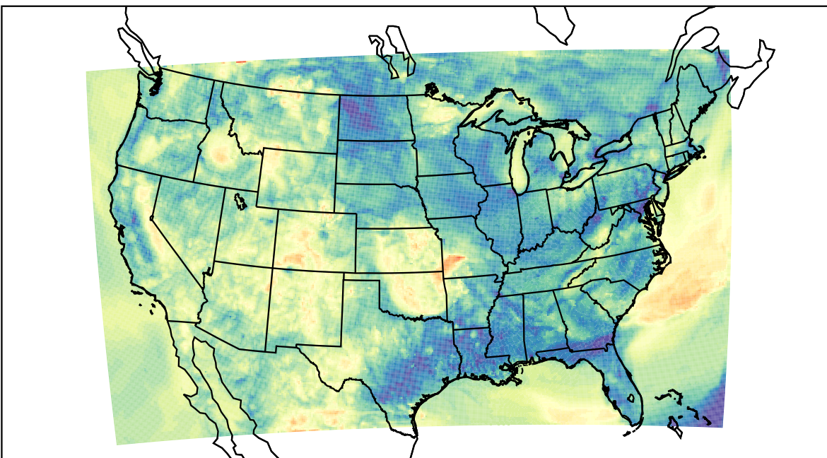
WRF (2023-05-10_09:00:00)
