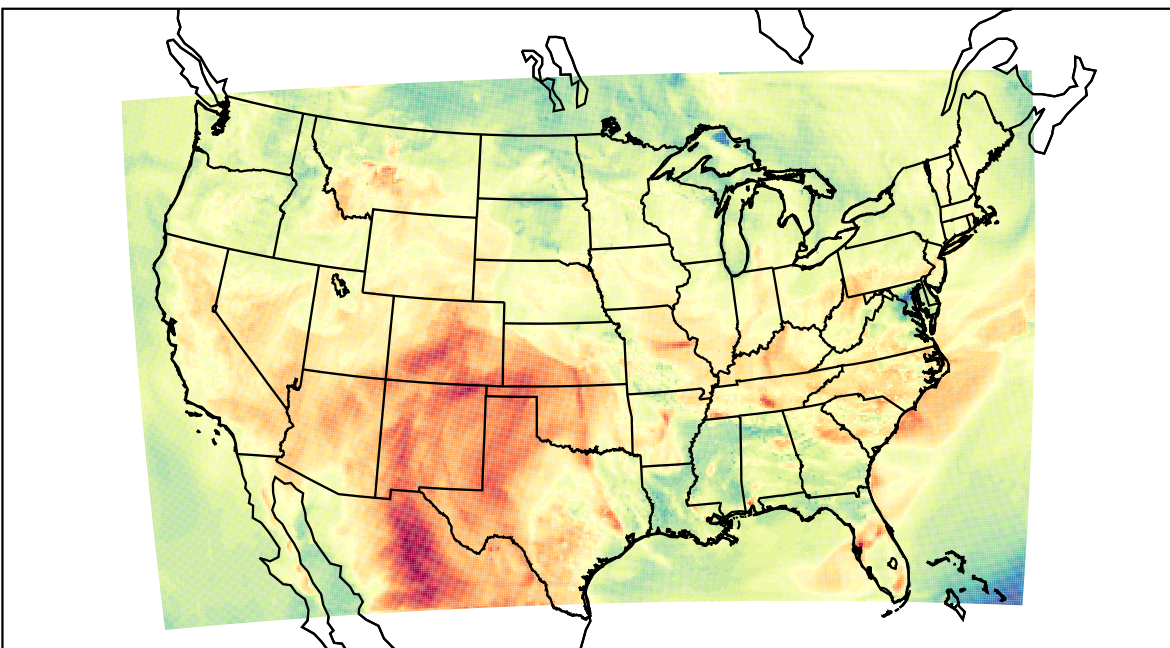
WRF (2023-05-09_21:00:00)
