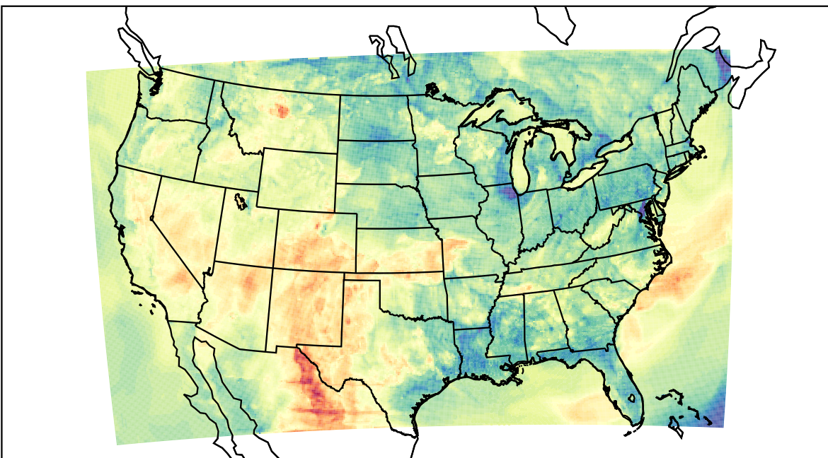
WRF (2023-05-10_02:00:00)
