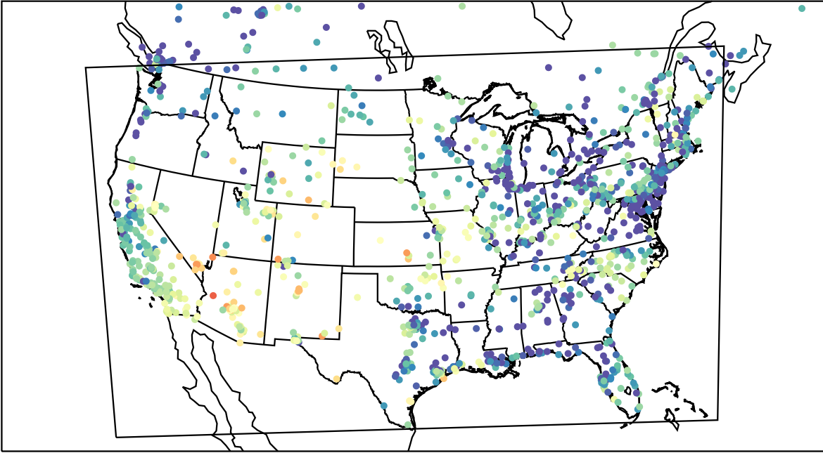
AirNOW (2023-05-10_05:00:00)
