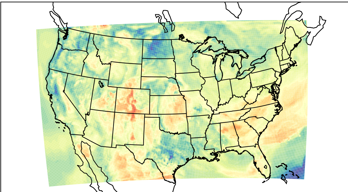
WRF (2023-05-10_16:00:00)
