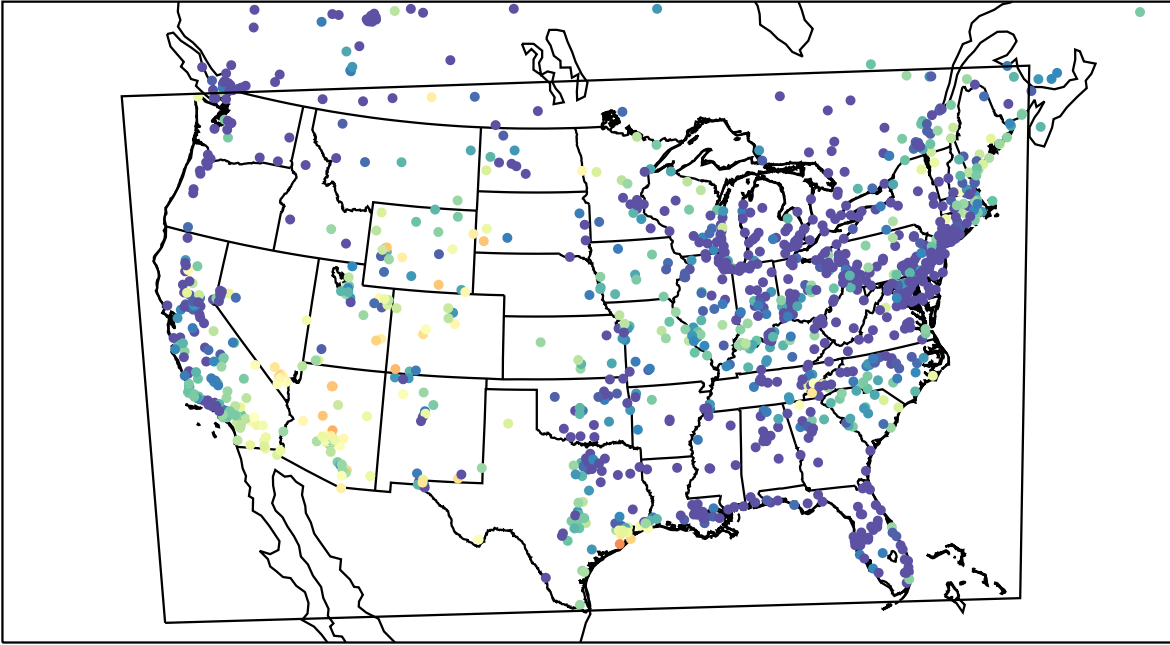
AirNOW (2023-05-10_11:00:00)
