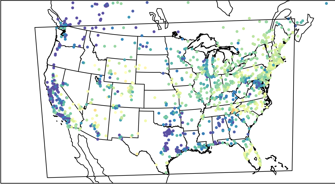
AirNOW (2023-05-09_14:00:00)
