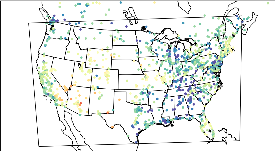
AirNOW (2023-05-09_02:00:00)
