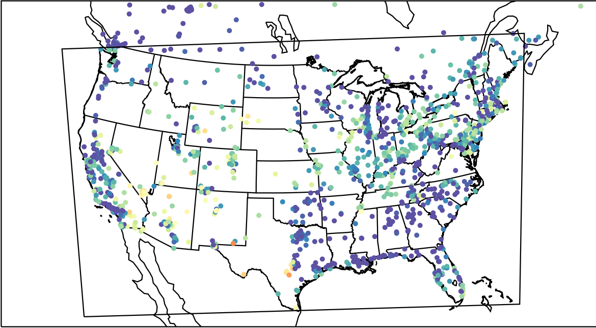
AirNOW (2023-05-09_09:00:00)
