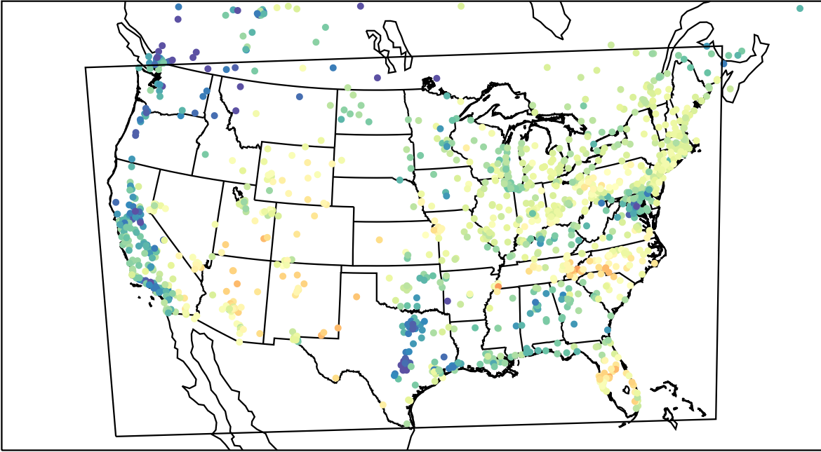
AirNOW (2023-05-09_16:00:00)
