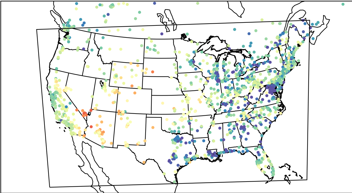
AirNOW (2023-05-10_02:00:00)
