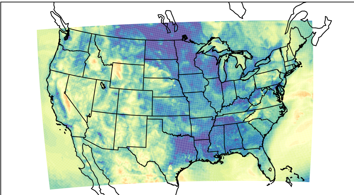
WRF (2023-05-09_13:00:00)
