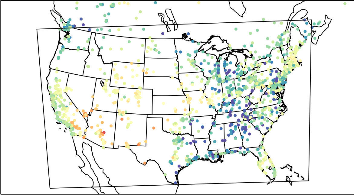
AirNOW (2023-05-09_01:00:00)
