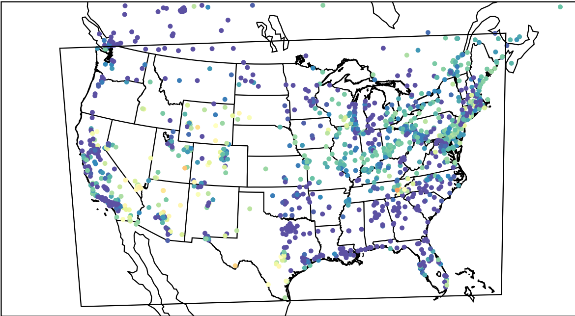
AirNOW (2023-05-09_11:00:00)
