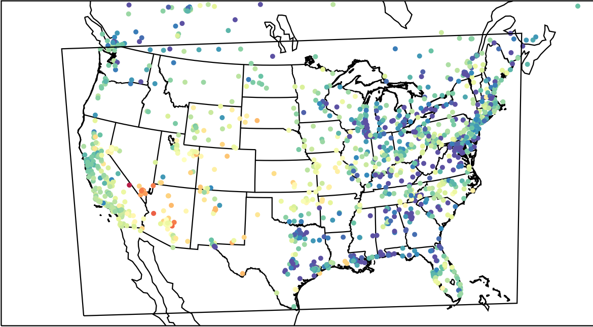
AirNOW (2023-05-10_03:00:00)
