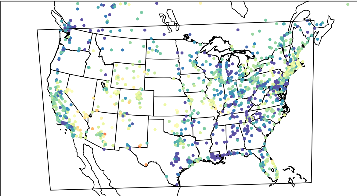
AirNOW (2023-05-09_04:00:00)
