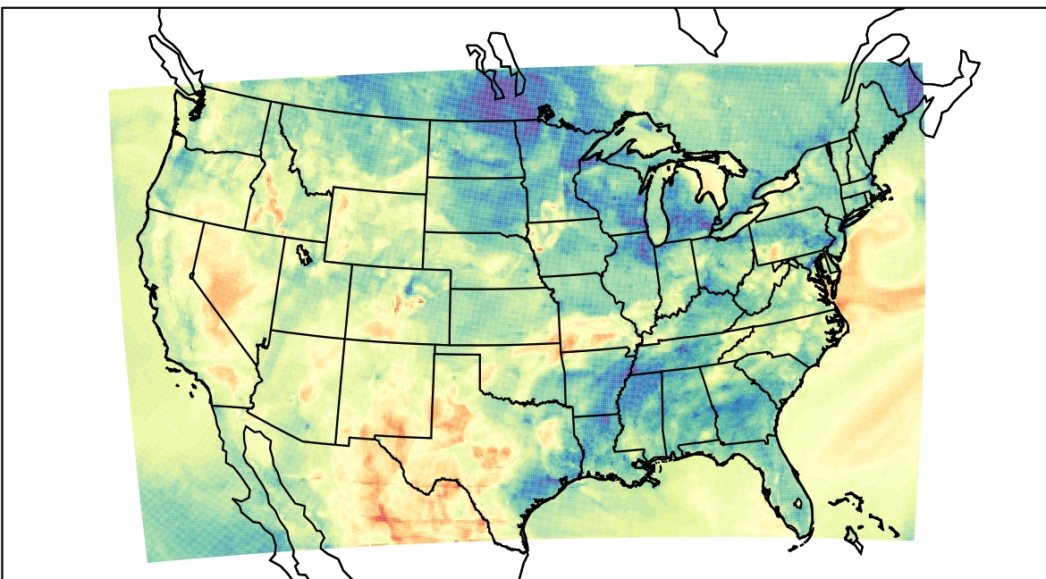
WRF (2023-05-09_02:00:00)
