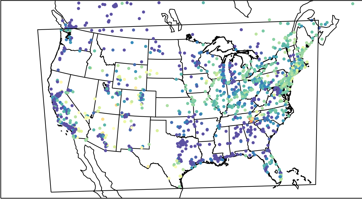
AirNOW (2023-05-09_12:00:00)
