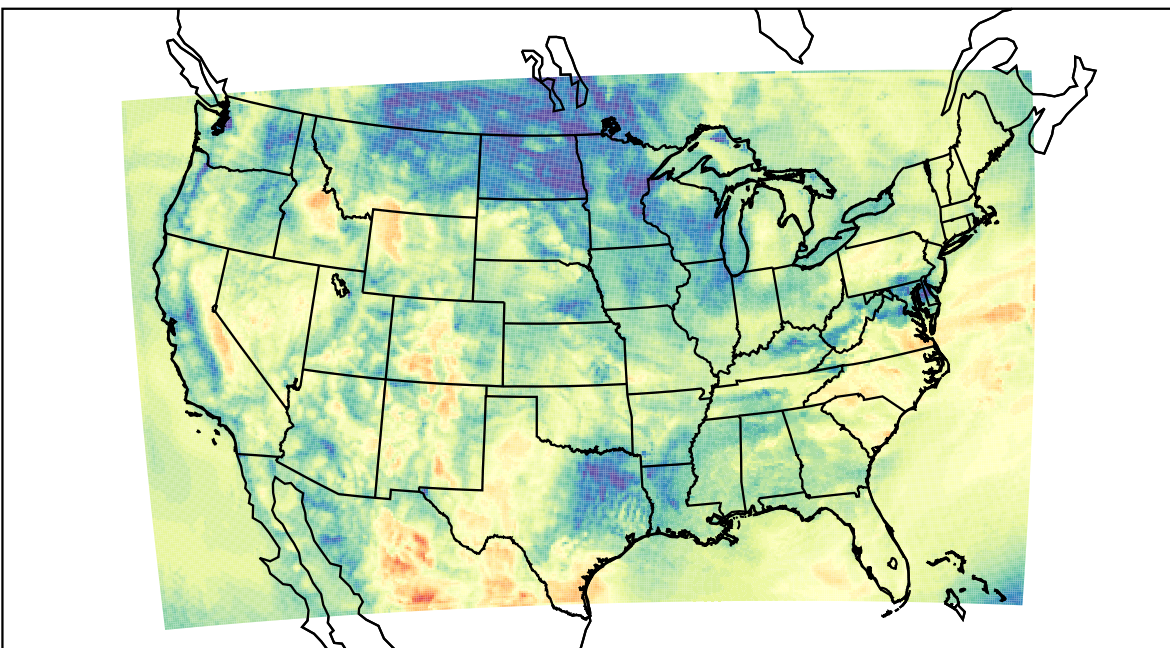
WRF (2023-05-09_15:00:00)
