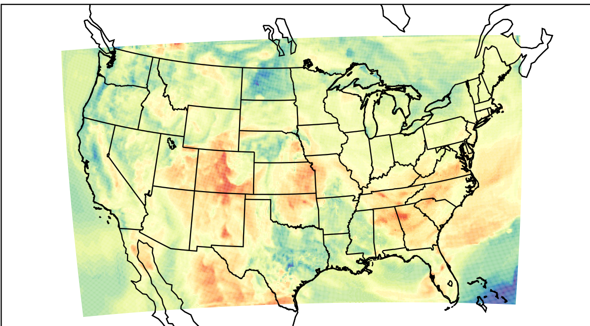
WRF (2023-05-10_17:00:00)
