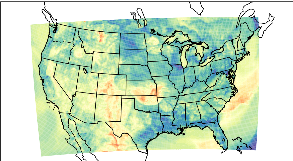
WRF (2023-05-10_05:00:00)
