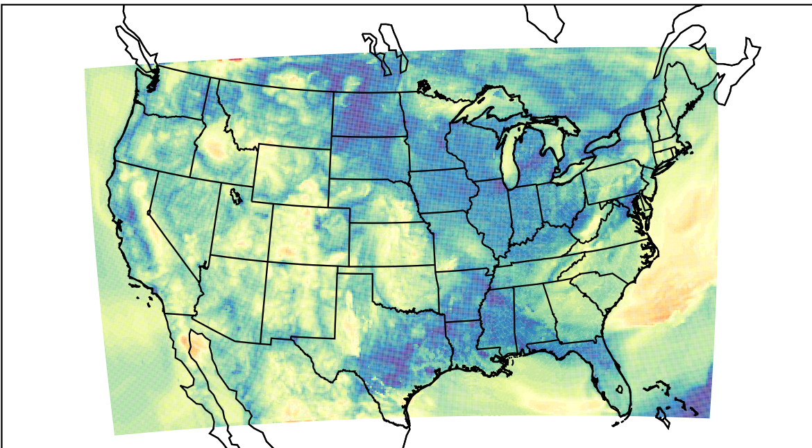
WRF (2023-05-10_13:00:00)
