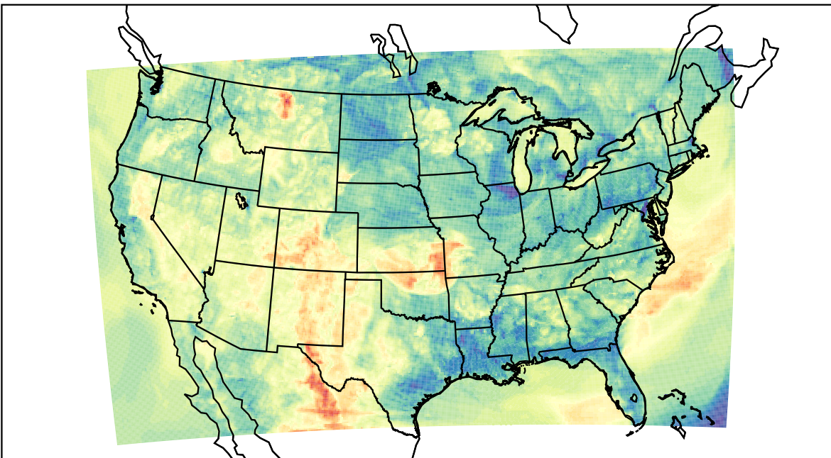
WRF (2023-05-10_04:00:00)
