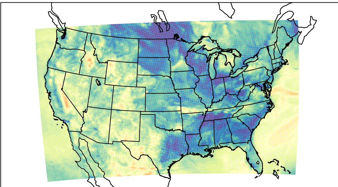
WRF (2023-05-09_08:00:00)
