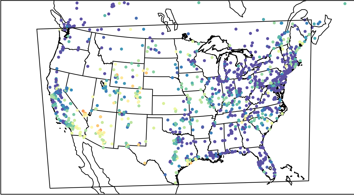
AirNOW (2023-05-10_10:00:00)
