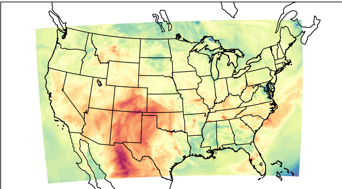
WRF (2023-05-09_22:00:00)
