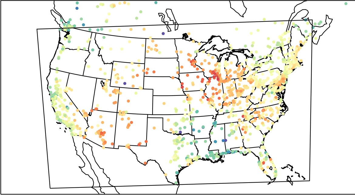
AirNOW (2023-05-10_22:00:00)
