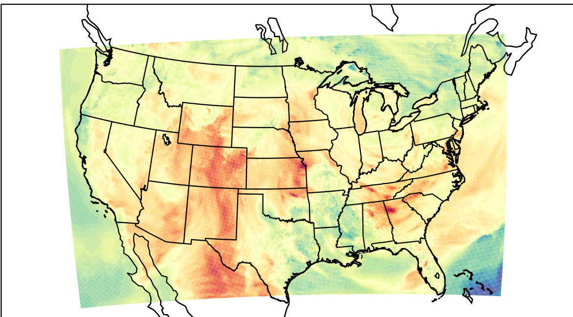
WRF (2023-05-10_22:00:00)
