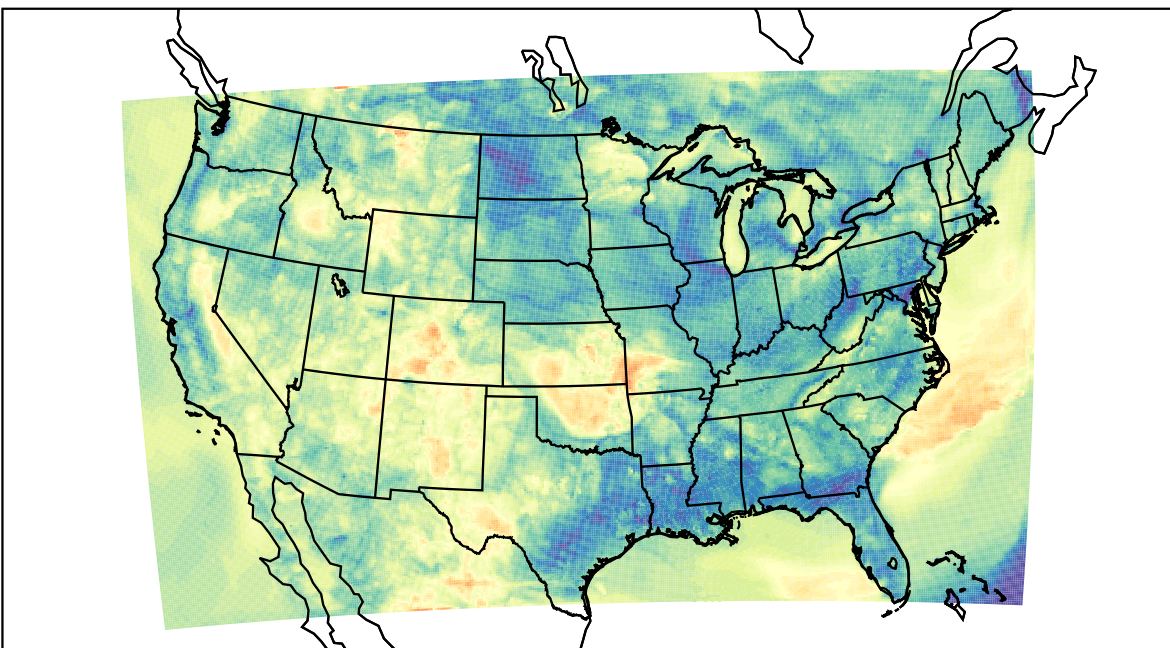
WRF (2023-05-10_07:00:00)
