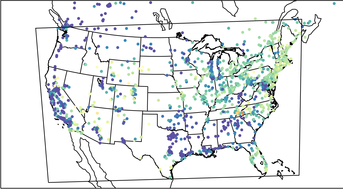
AirNOW (2023-05-09_13:00:00)
