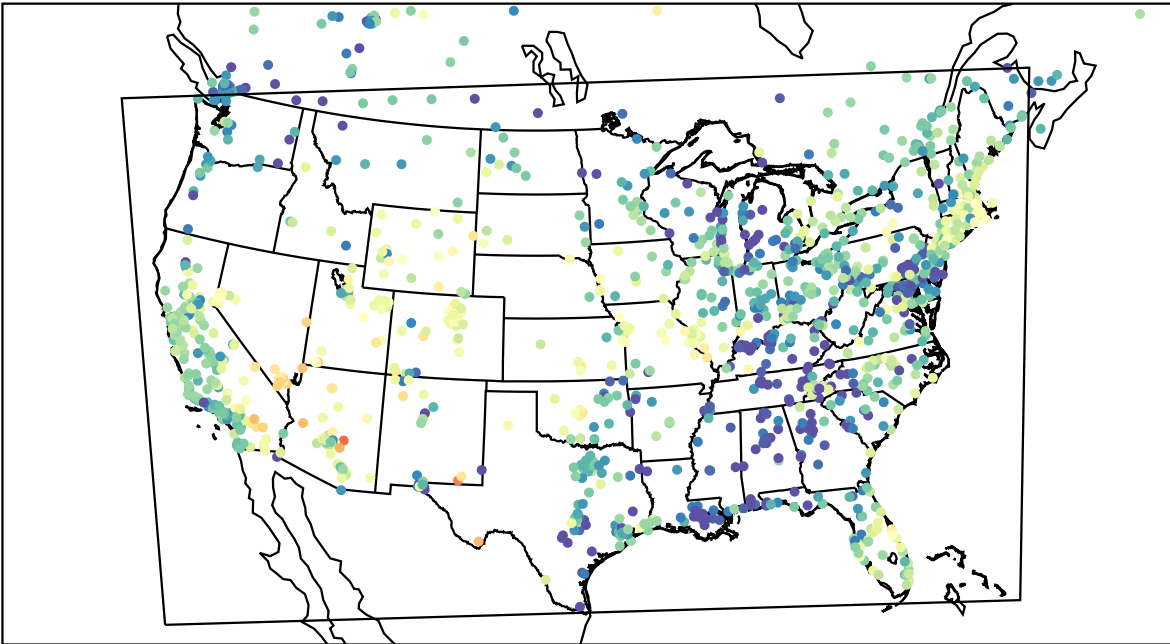
AirNOW (2023-05-09_03:00:00)
