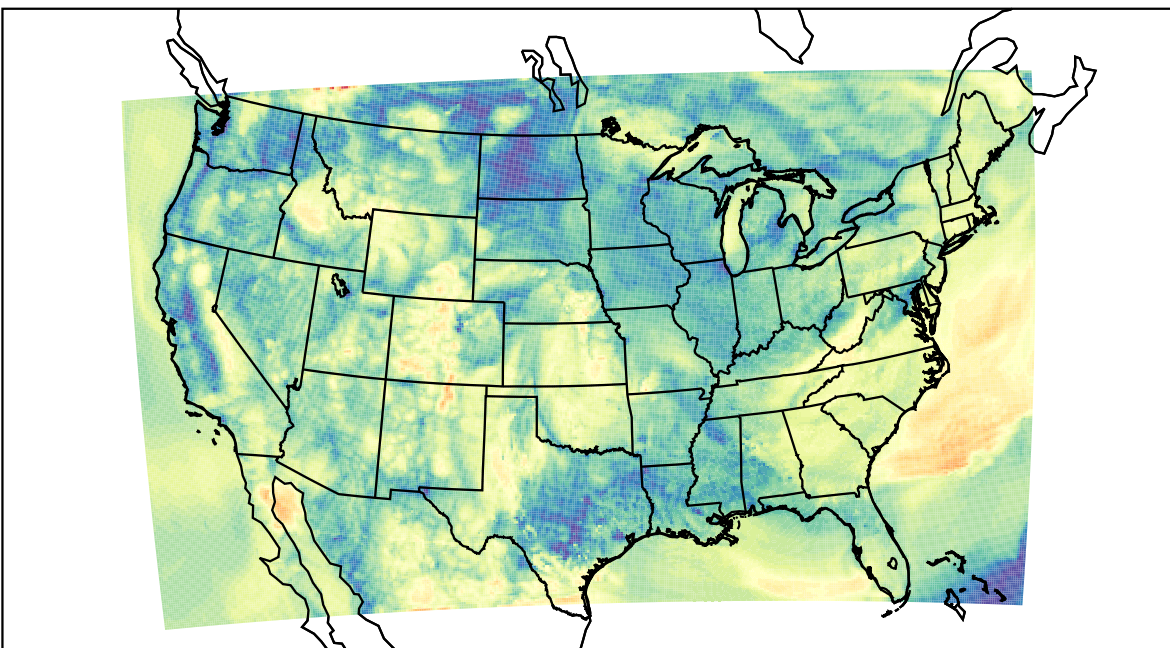
WRF (2023-05-10_14:00:00)
