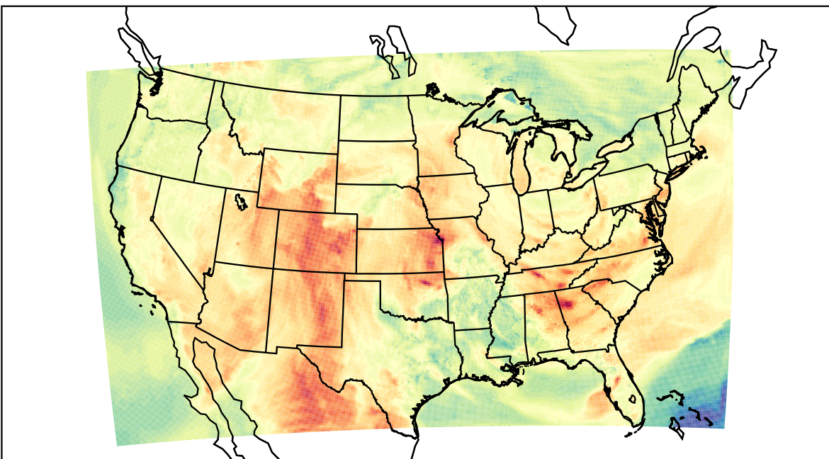
WRF (2023-05-10_21:00:00)
