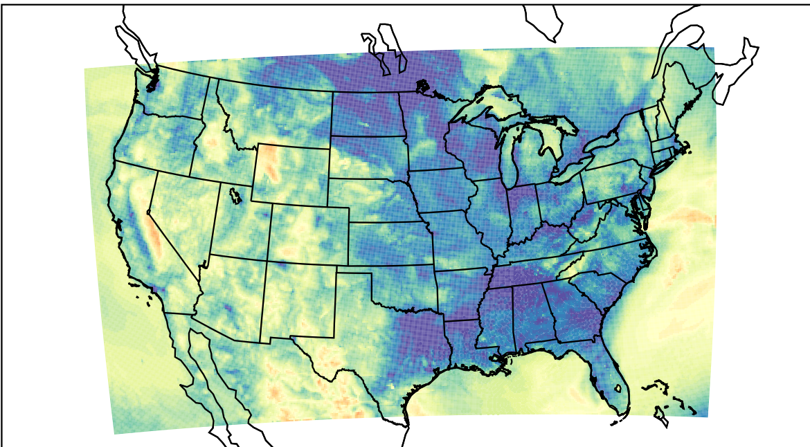
WRF (2023-05-09_12:00:00)
