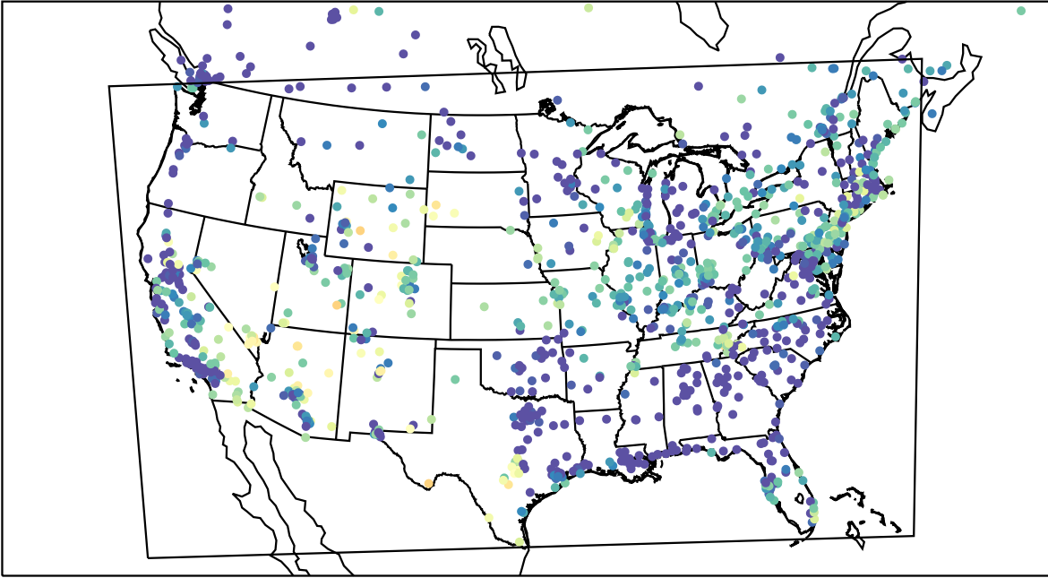
AirNOW (2023-05-09_10:00:00)
