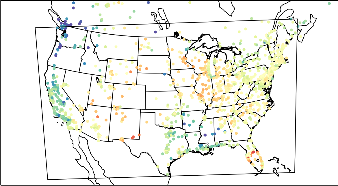
AirNOW (2023-05-10_17:00:00)
