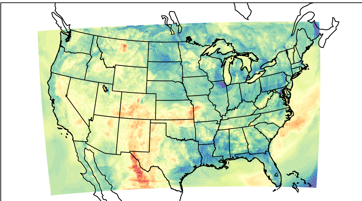
WRF (2023-05-10_03:00:00)
