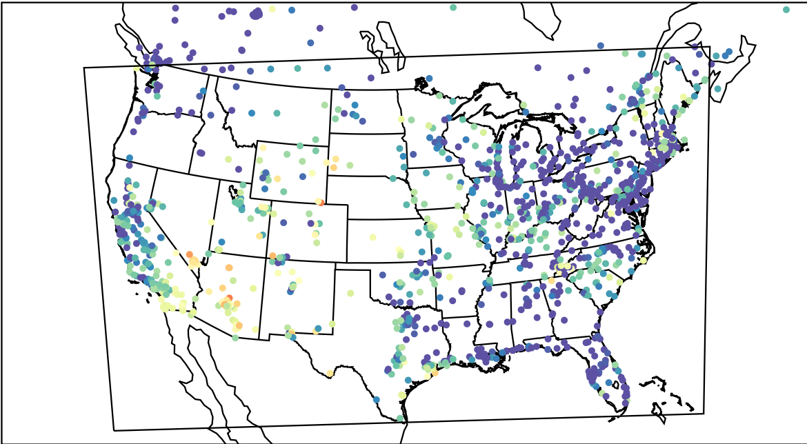
AirNOW (2023-05-10_09:00:00)
