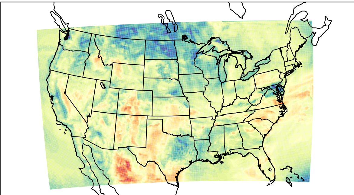
WRF (2023-05-09_16:00:00)
