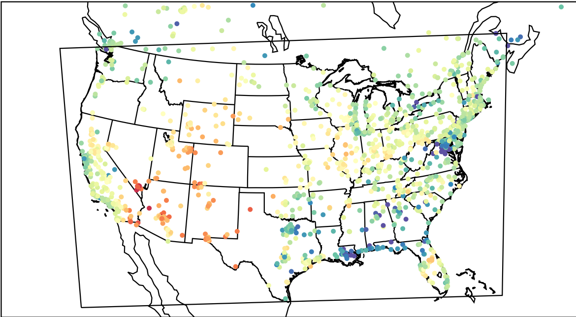
AirNOW (2023-05-10_00:00:00)
