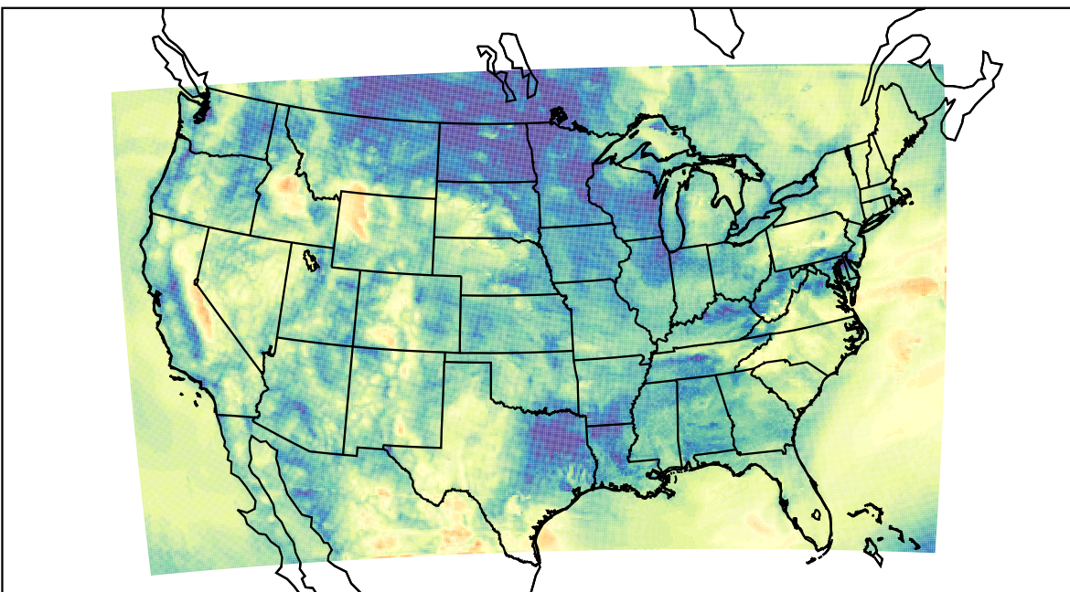
WRF (2023-05-09_14:00:00)
