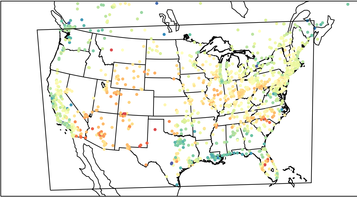
AirNOW (2023-05-09_21:00:00)
