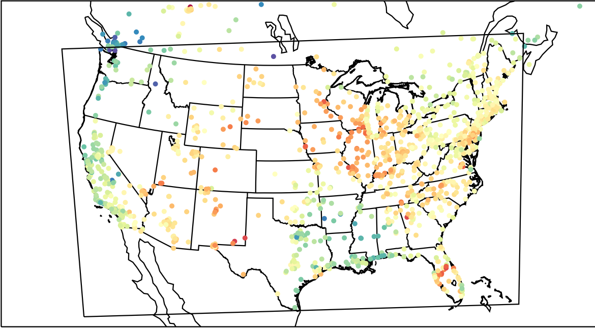
AirNOW (2023-05-10_19:00:00)
