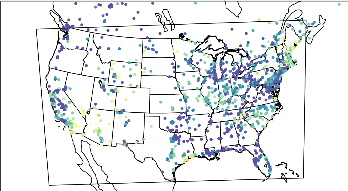
AirNOW (2023-05-10_12:00:00)
