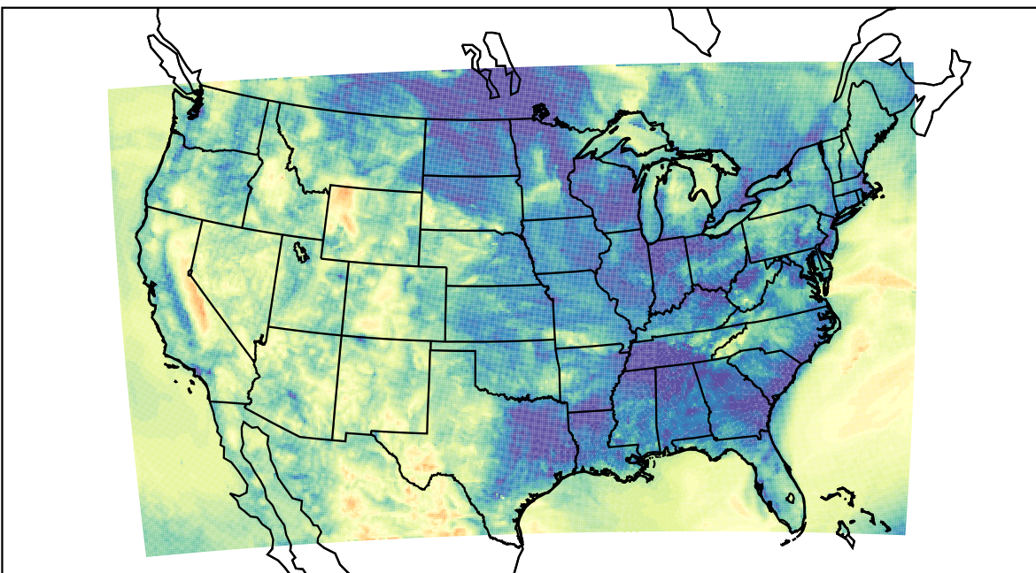
WRF (2023-05-09_11:00:00)
