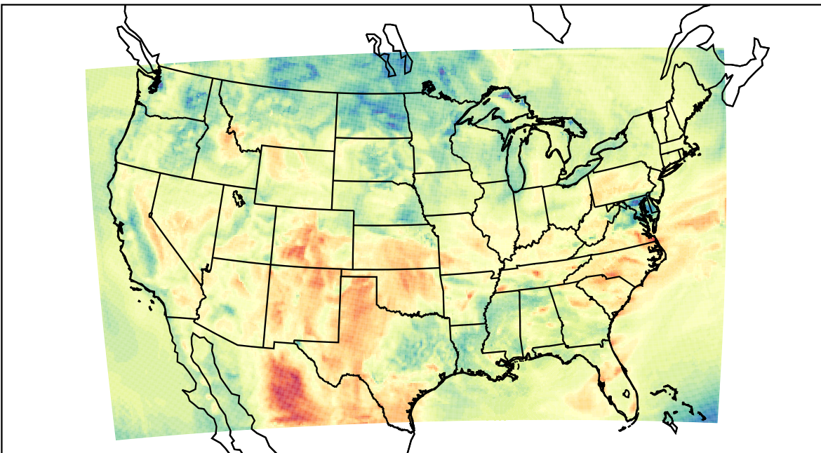
WRF (2023-05-09_17:00:00)
