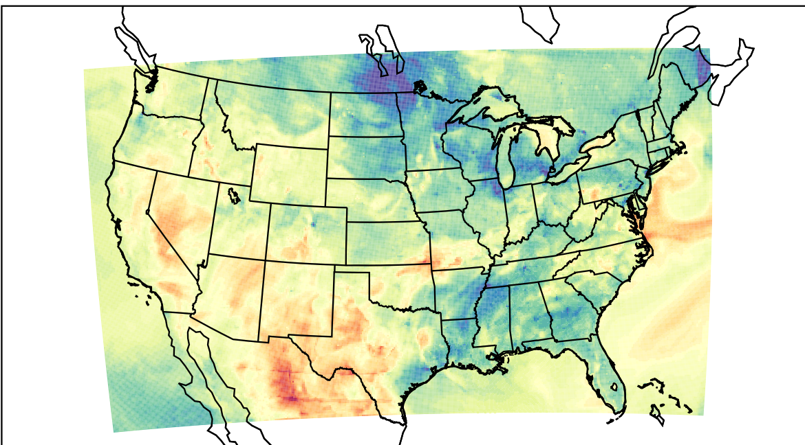
WRF (2023-05-09_01:00:00)
