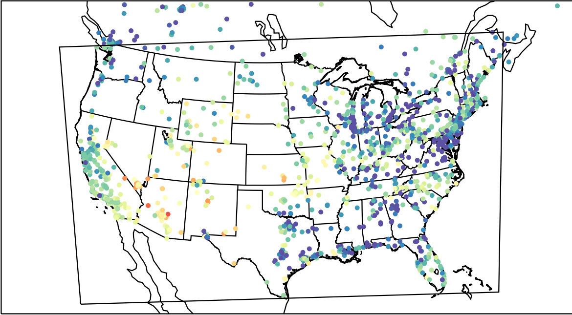
AirNOW (2023-05-10_04:00:00)
