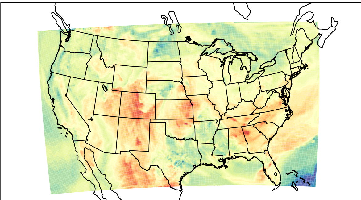
WRF (2023-05-10_18:00:00)
