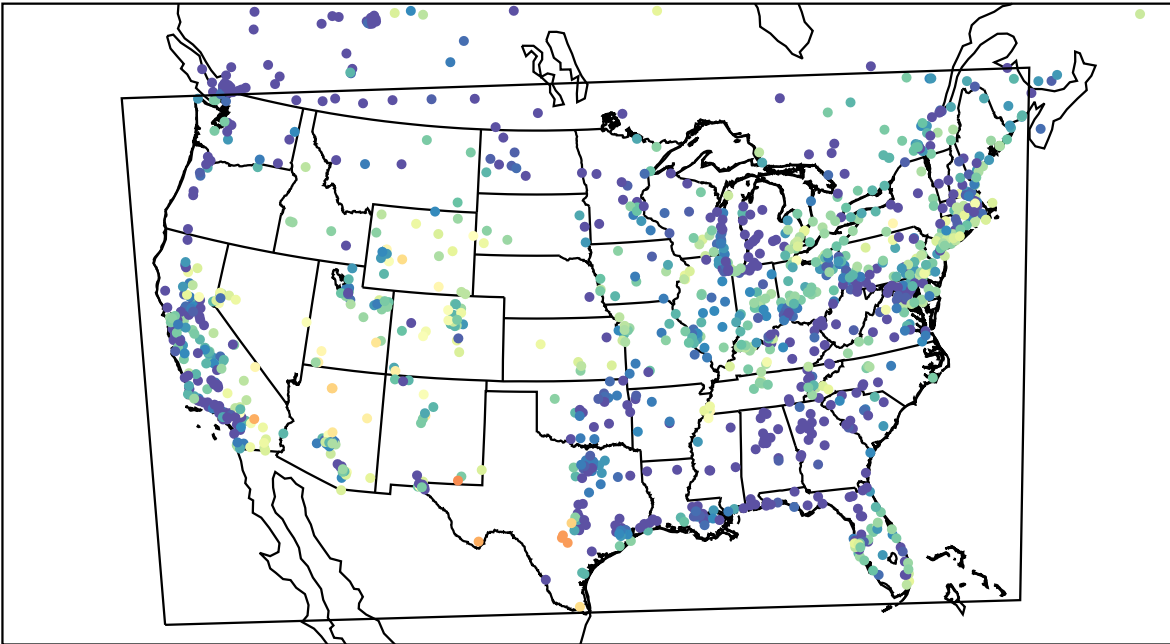
AirNOW (2023-05-09_08:00:00)
