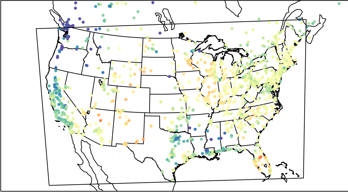
AirNOW (2023-05-10_16:00:00)
