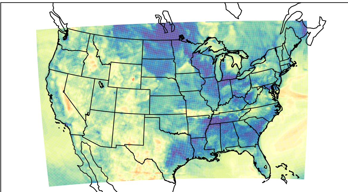
WRF (2023-05-09_07:00:00)
