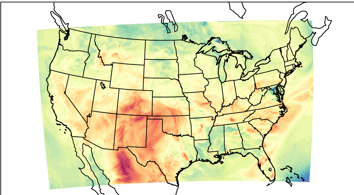
WRF (2023-05-09_20:00:00)
