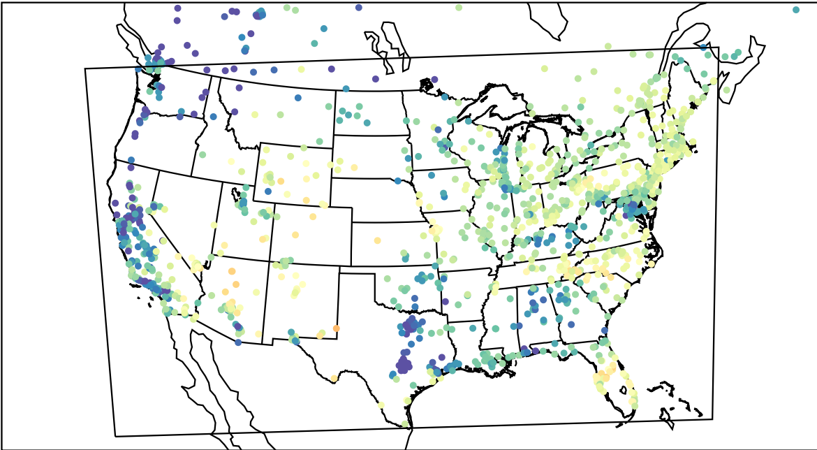
AirNOW (2023-05-09_15:00:00)
