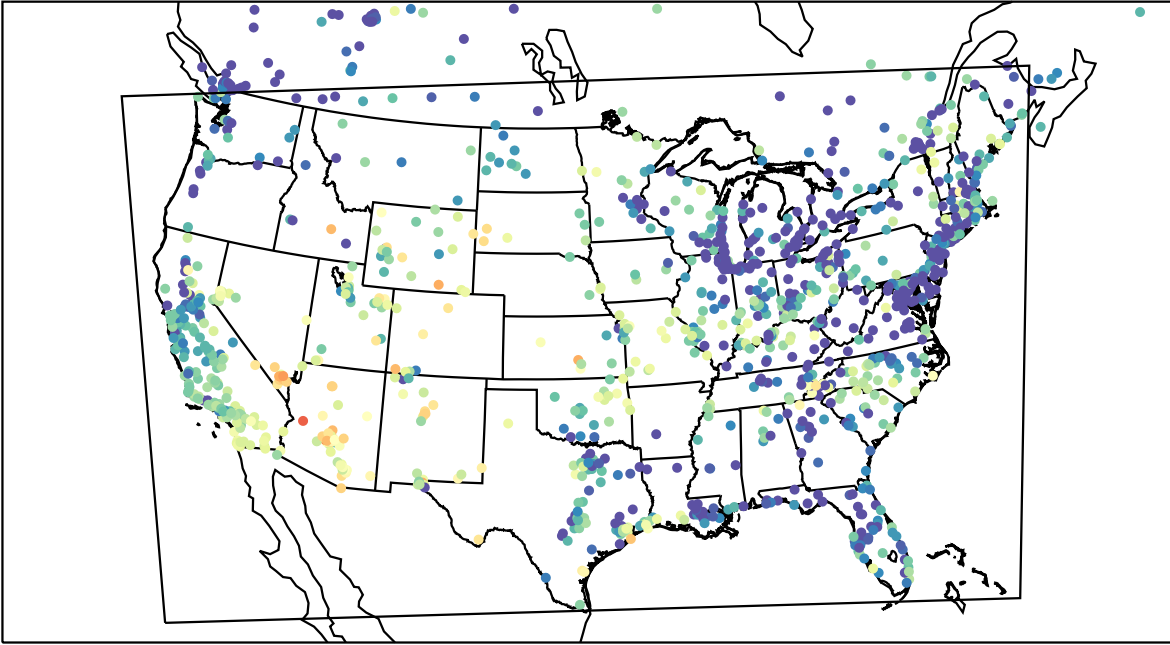
AirNOW (2023-05-10_06:00:00)
