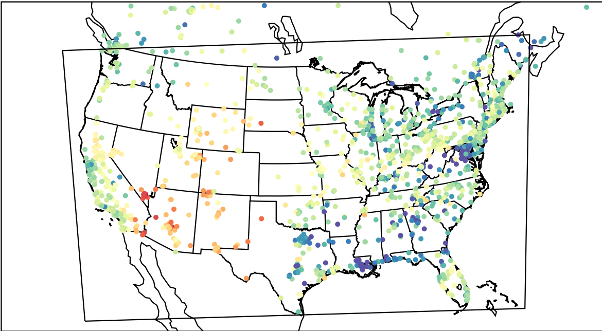
AirNOW (2023-05-10_01:00:00)
