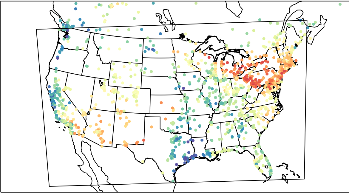
AirNOW (2023-05-12_17:00:00)
