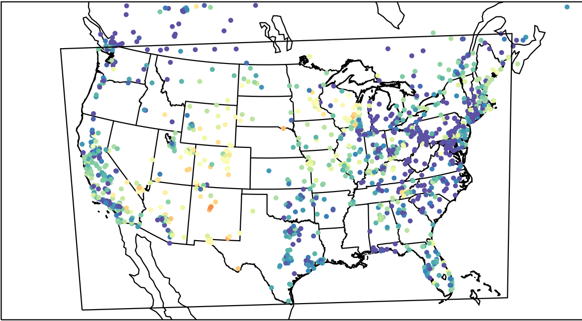
AirNOW (2023-05-11_07:00:00)
