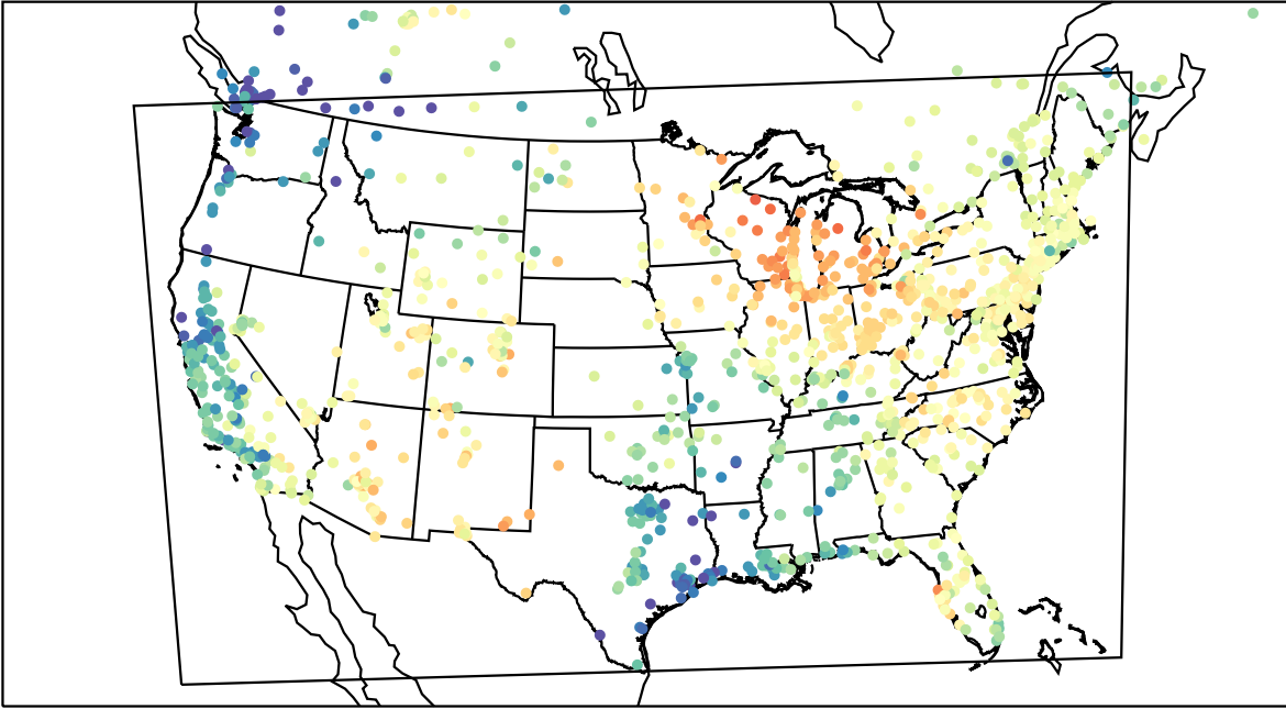
AirNOW (2023-05-11_16:00:00)
