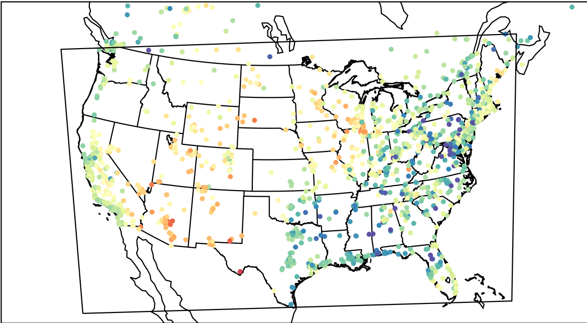
AirNOW (2023-05-11_01:00:00)
