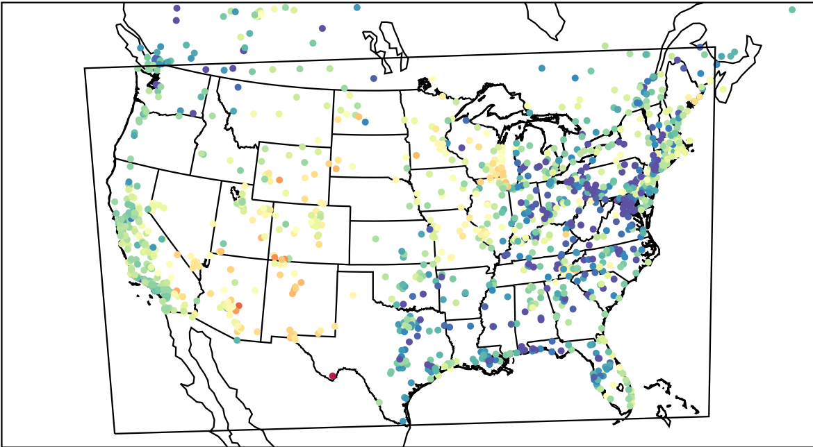
AirNOW (2023-05-11_03:00:00)
