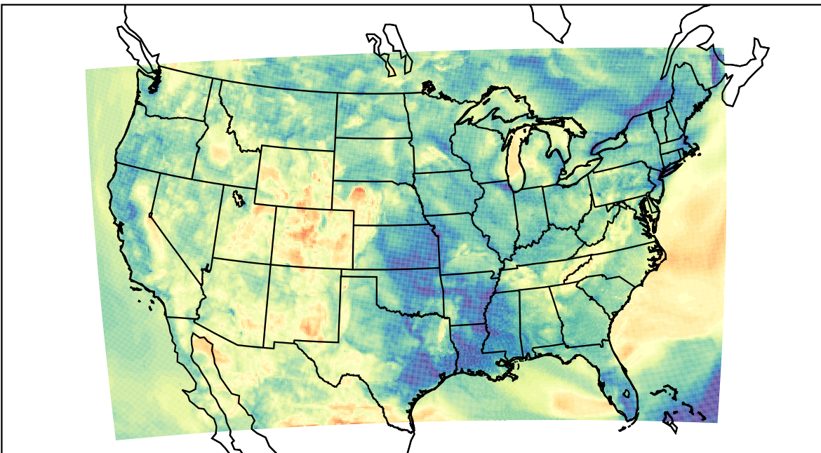
WRF (2023-05-11_06:00:00)
