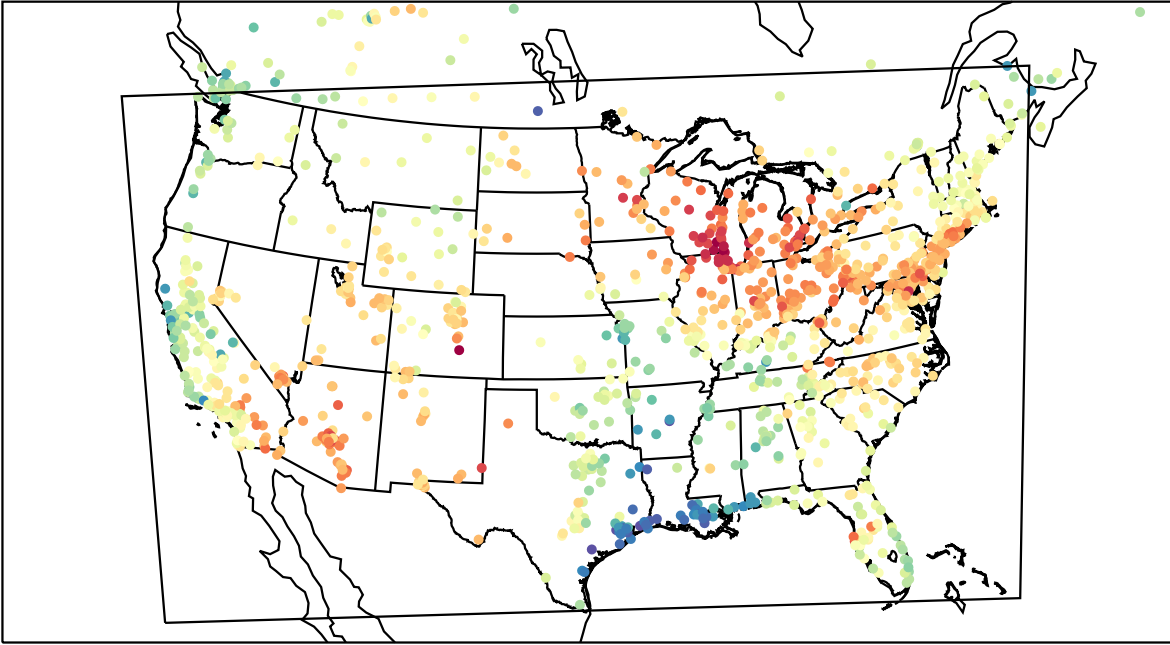
AirNOW (2023-05-11_20:00:00)
