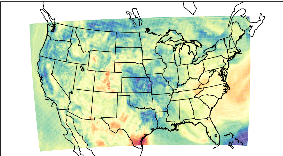
WRF (2023-05-11_15:00:00)
