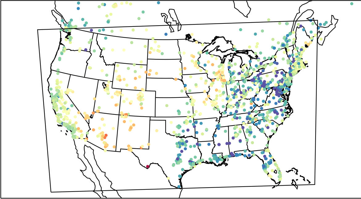
AirNOW (2023-05-11_02:00:00)
