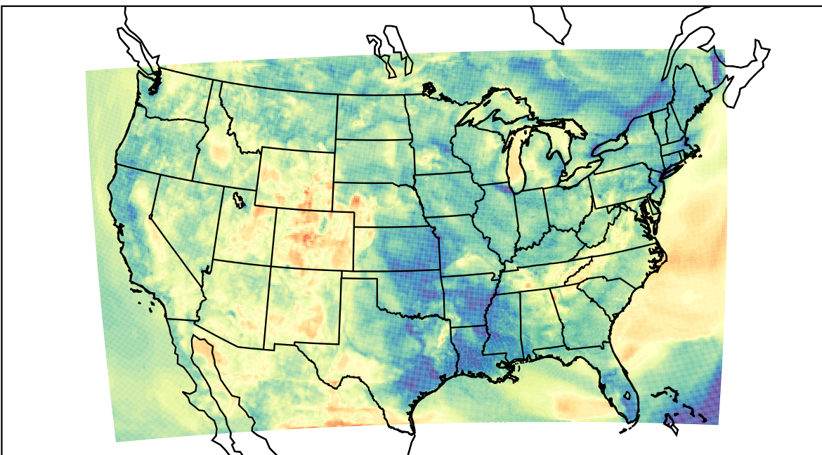
WRF (2023-05-11_05:00:00)
