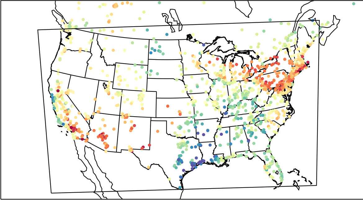
AirNOW (2023-05-12_22:00:00)
