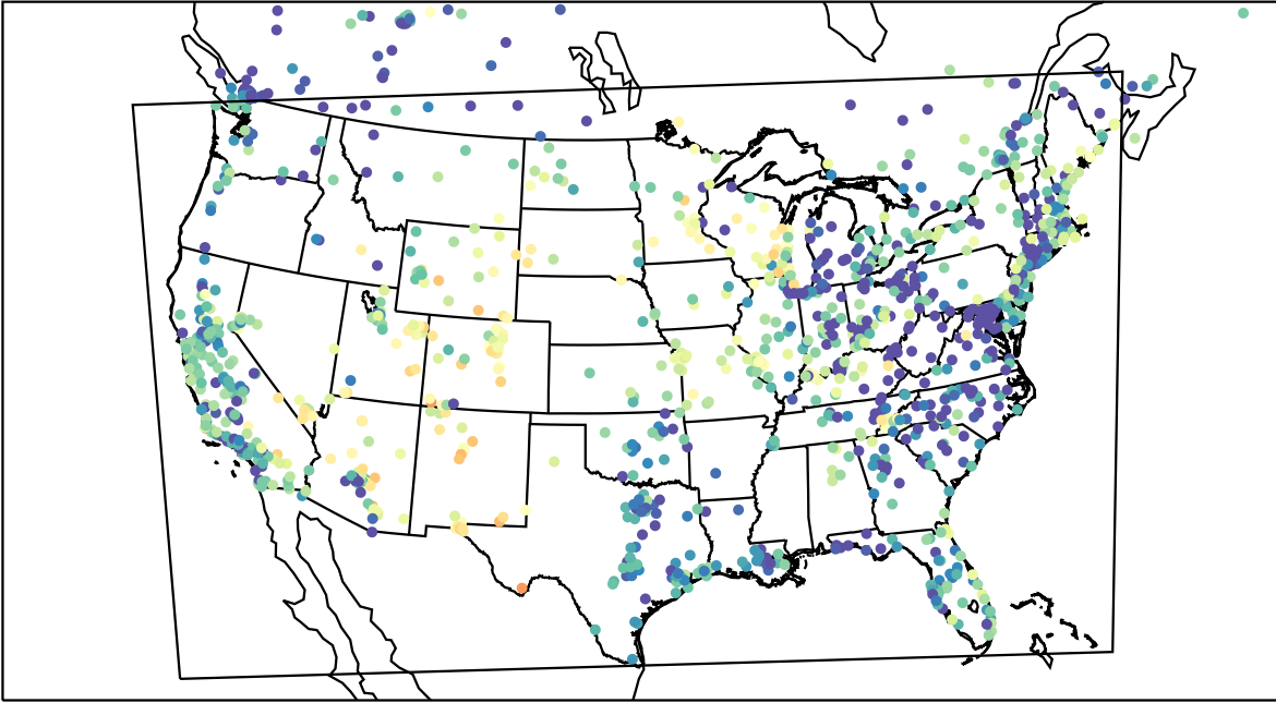
AirNOW (2023-05-11_06:00:00)
