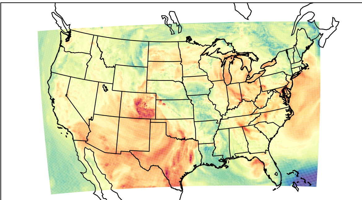
WRF (2023-05-11_22:00:00)
