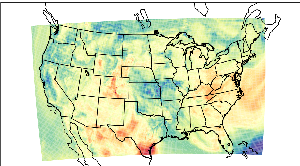
WRF (2023-05-11_16:00:00)
