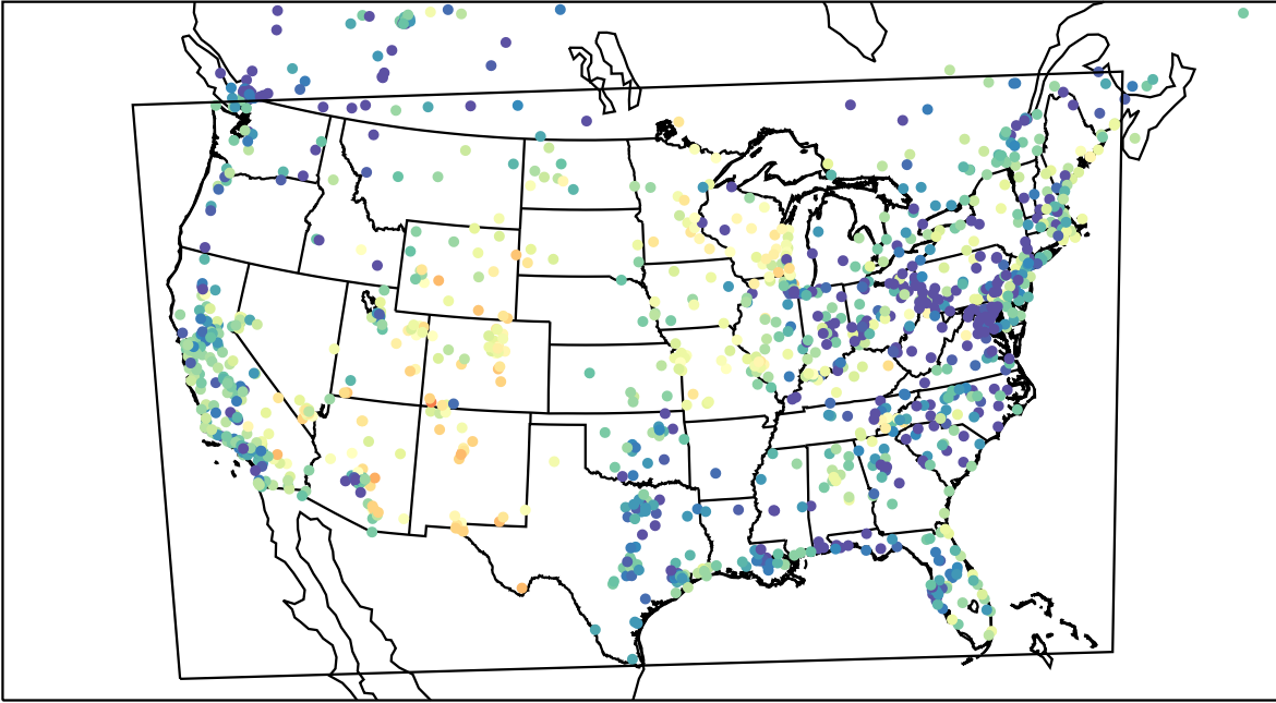
AirNOW (2023-05-11_05:00:00)
