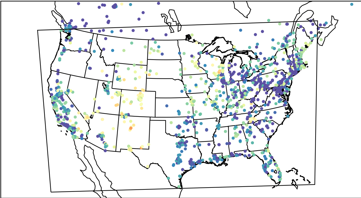
AirNOW (2023-05-11_08:00:00)
