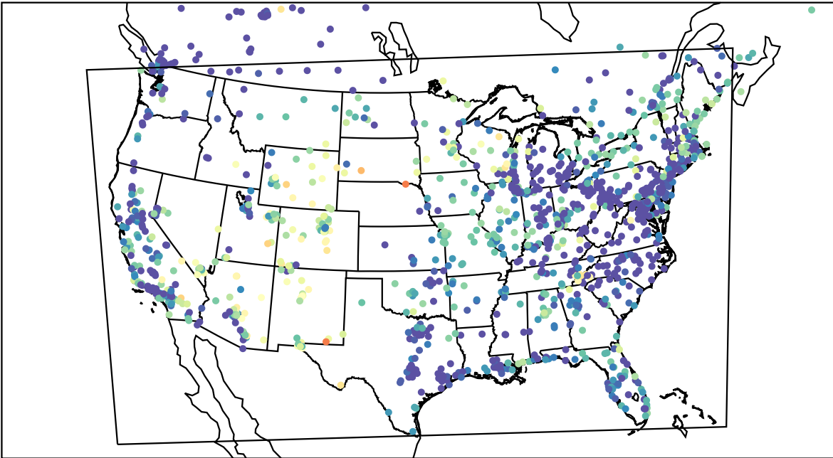
AirNOW (2023-05-11_11:00:00)
