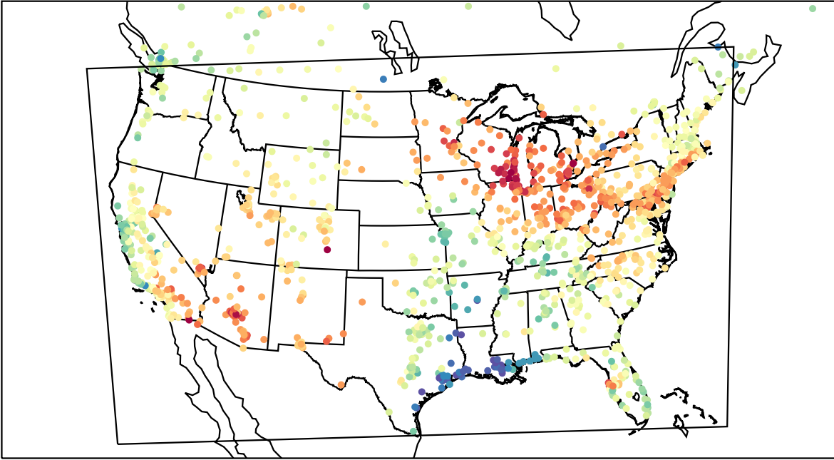
AirNOW (2023-05-11_22:00:00)
