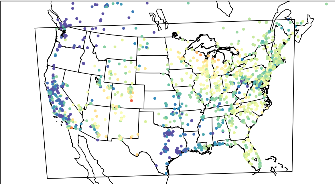
AirNOW (2023-05-11_14:00:00)
