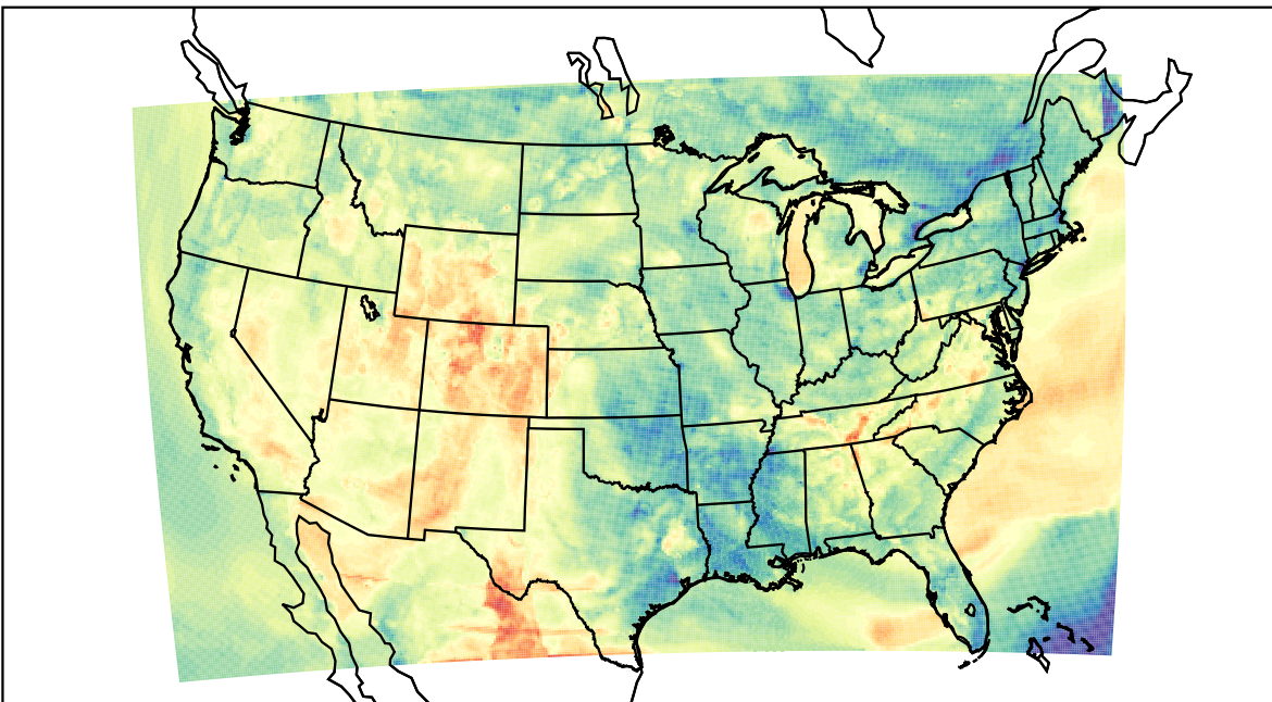
WRF (2023-05-11_02:00:00)
