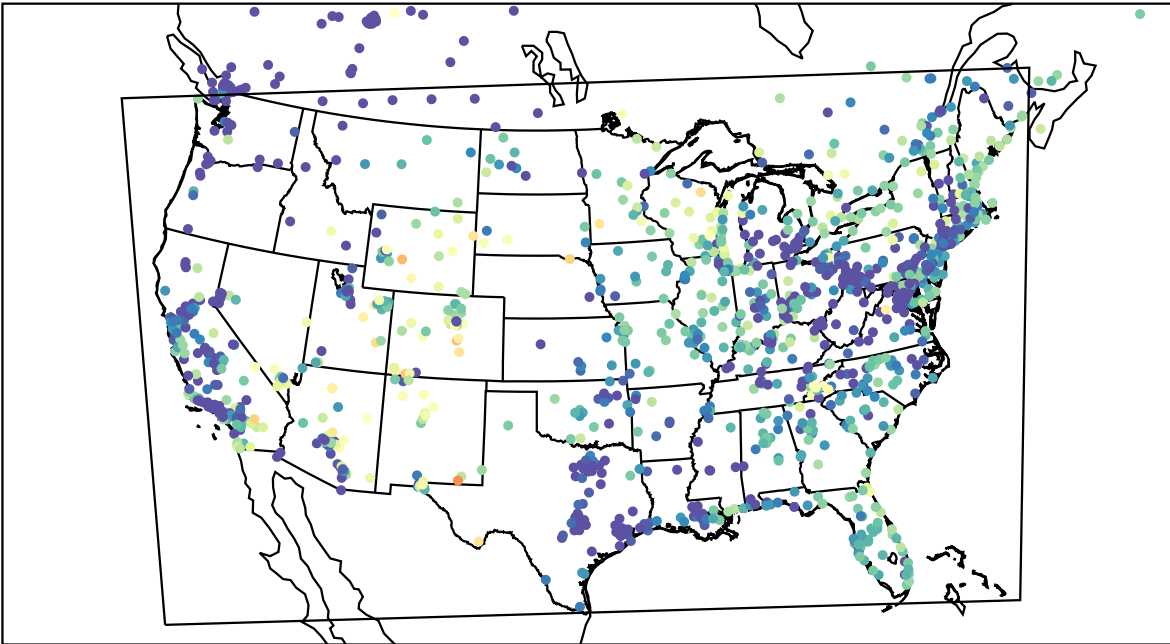
AirNOW (2023-05-11_12:00:00)
