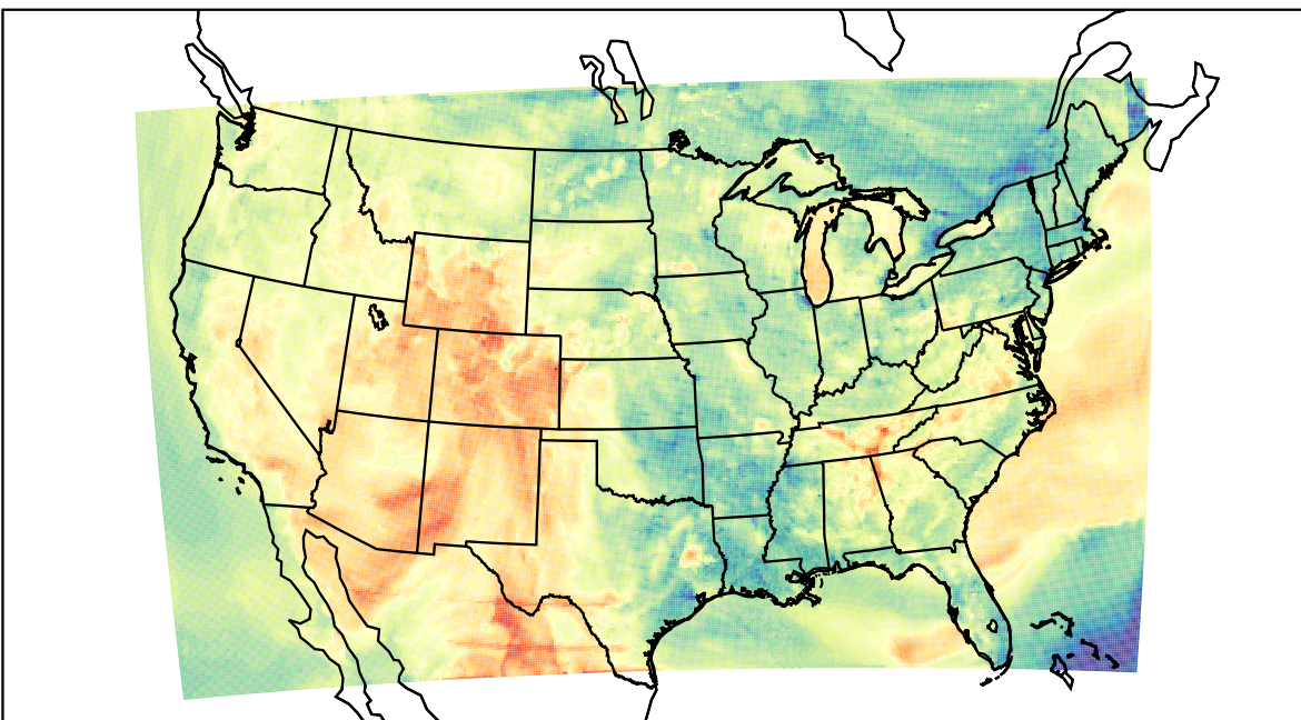
WRF (2023-05-11_01:00:00)
