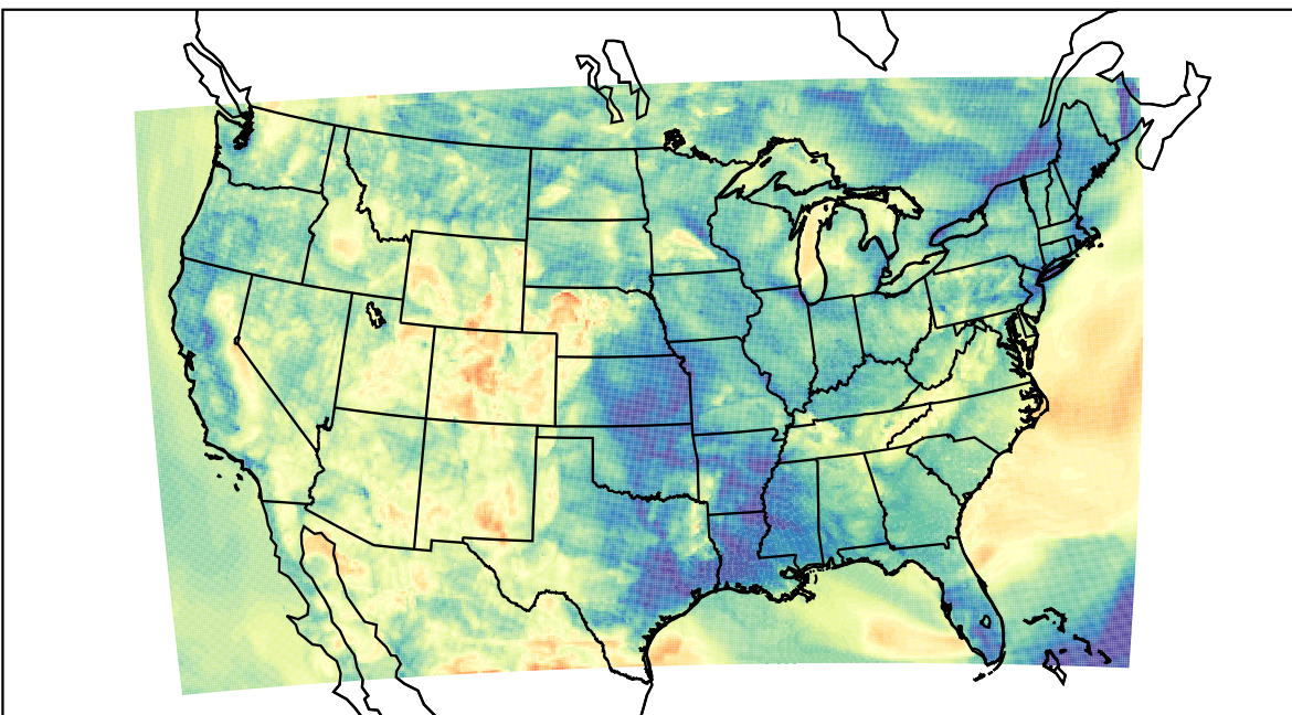
WRF (2023-05-11_07:00:00)
