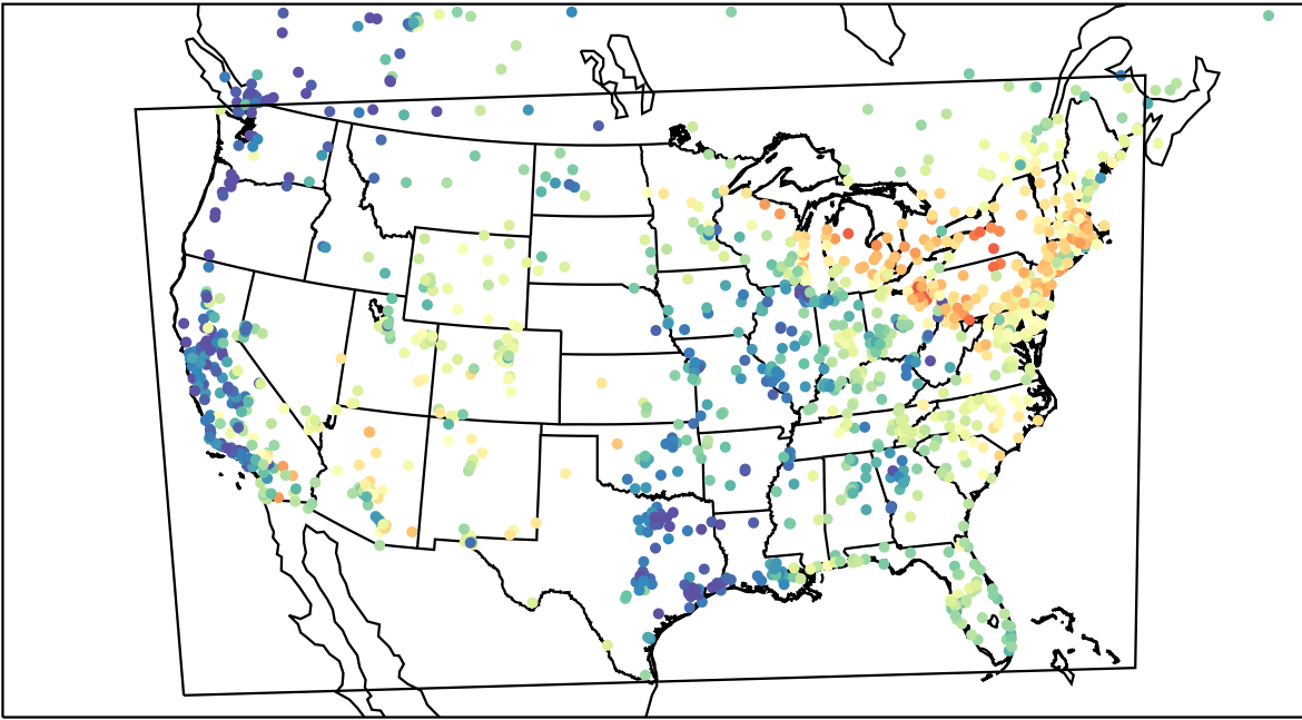
AirNOW (2023-05-12_15:00:00)
