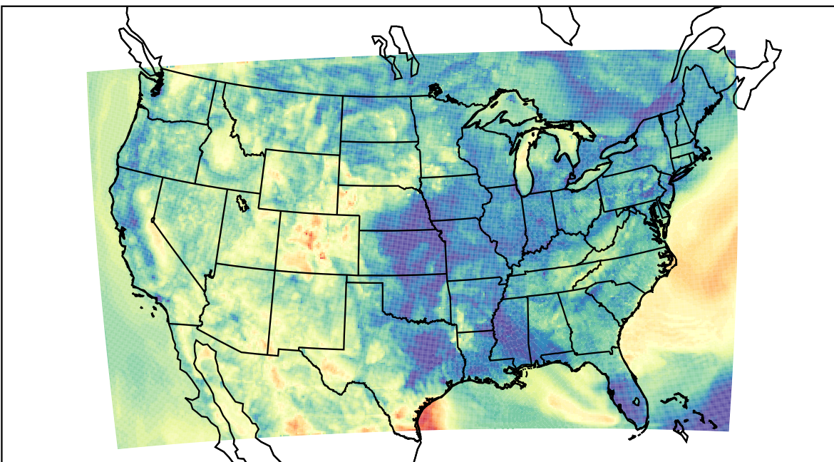
WRF (2023-05-11_12:00:00)
