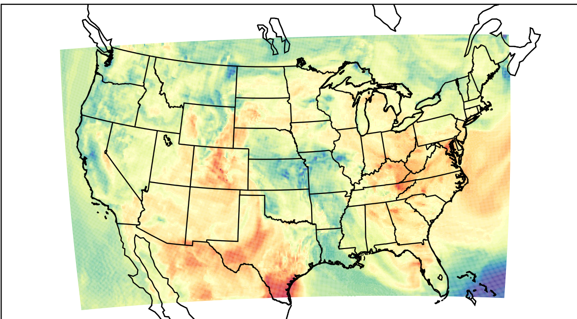
WRF (2023-05-11_17:00:00)
