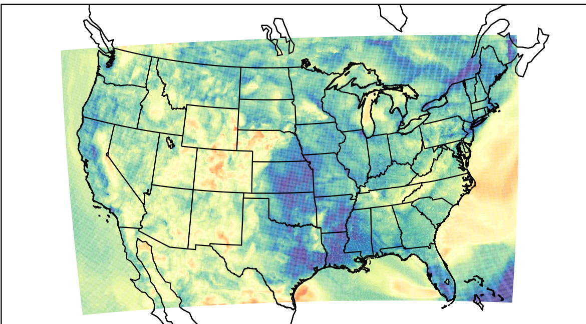
WRF (2023-05-11_08:00:00)
