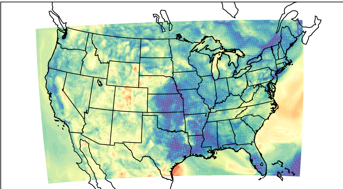
WRF (2023-05-11_10:00:00)
