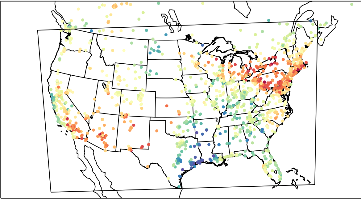
AirNOW (2023-05-12_21:00:00)
