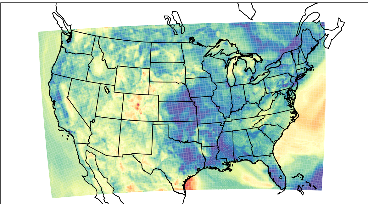
WRF (2023-05-11_11:00:00)
