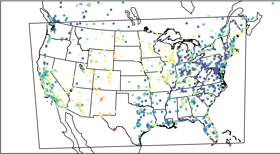
AirNOW (2023-05-11_04:00:00)
