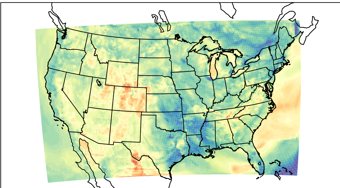
WRF (2023-05-11_03:00:00)
