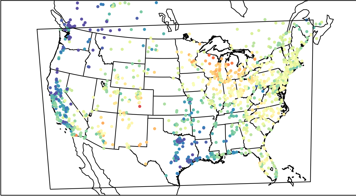
AirNOW (2023-05-11_15:00:00)
