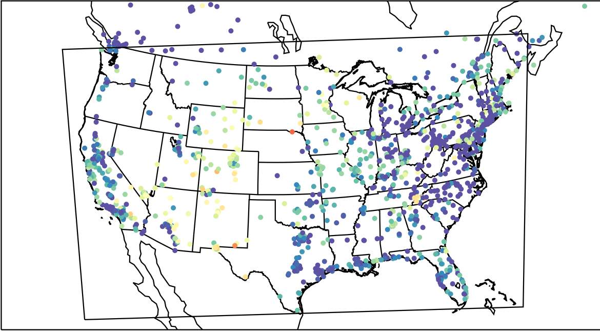
AirNOW (2023-05-11_10:00:00)
