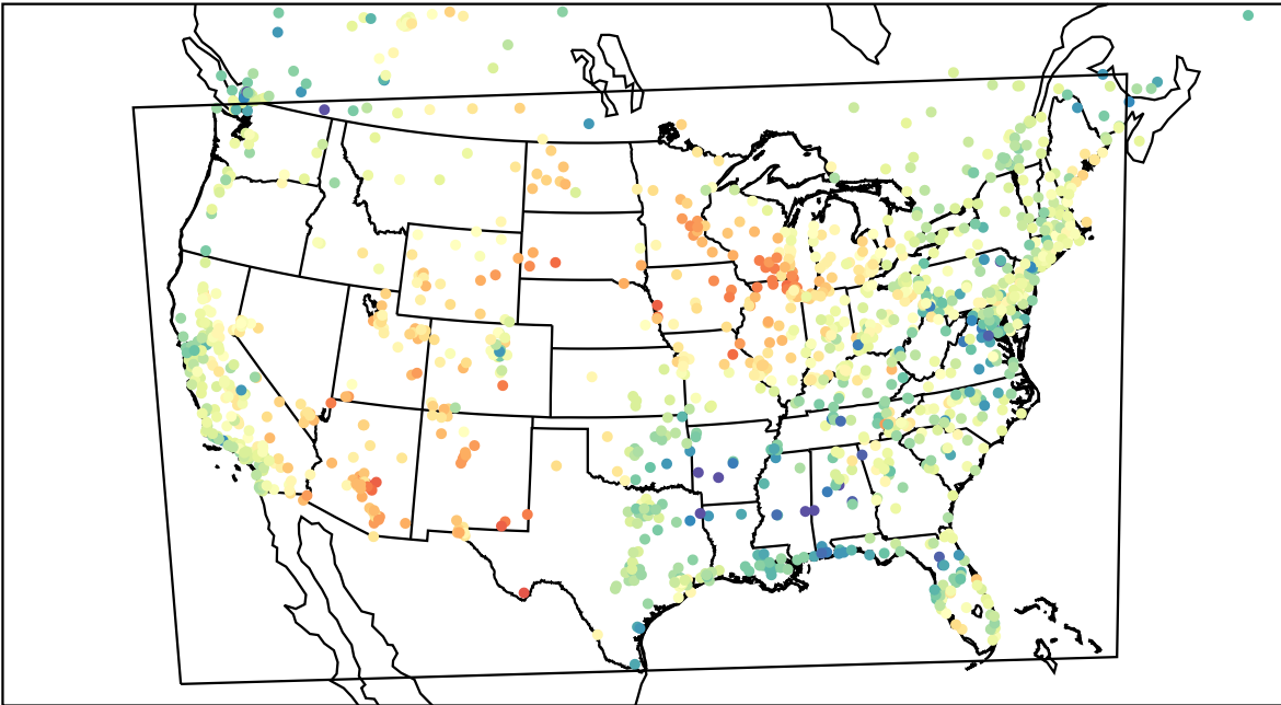
AirNOW (2023-05-11_00:00:00)
