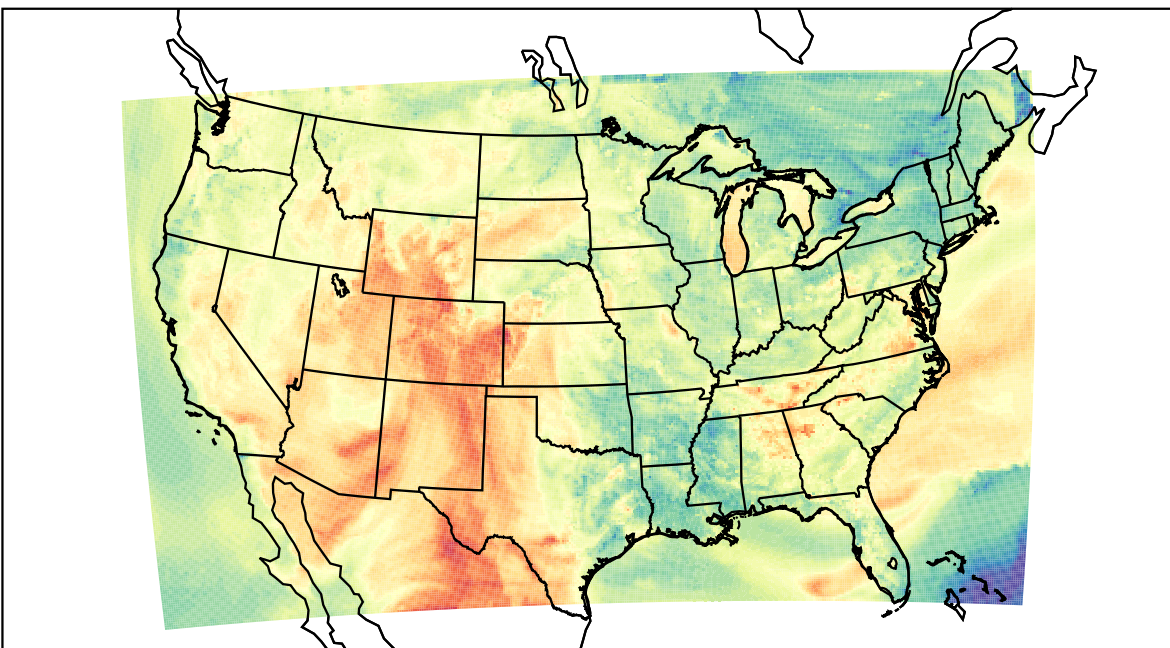
WRF (2023-05-11_00:00:00)
