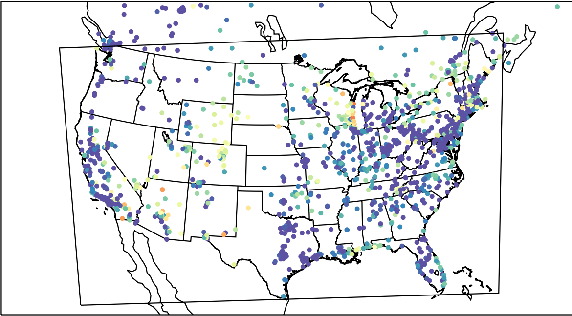
AirNOW (2023-05-12_11:00:00)
