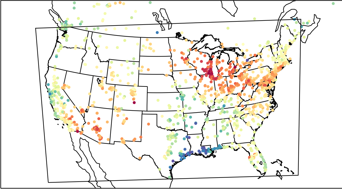
AirNOW (2023-05-11_21:00:00)
