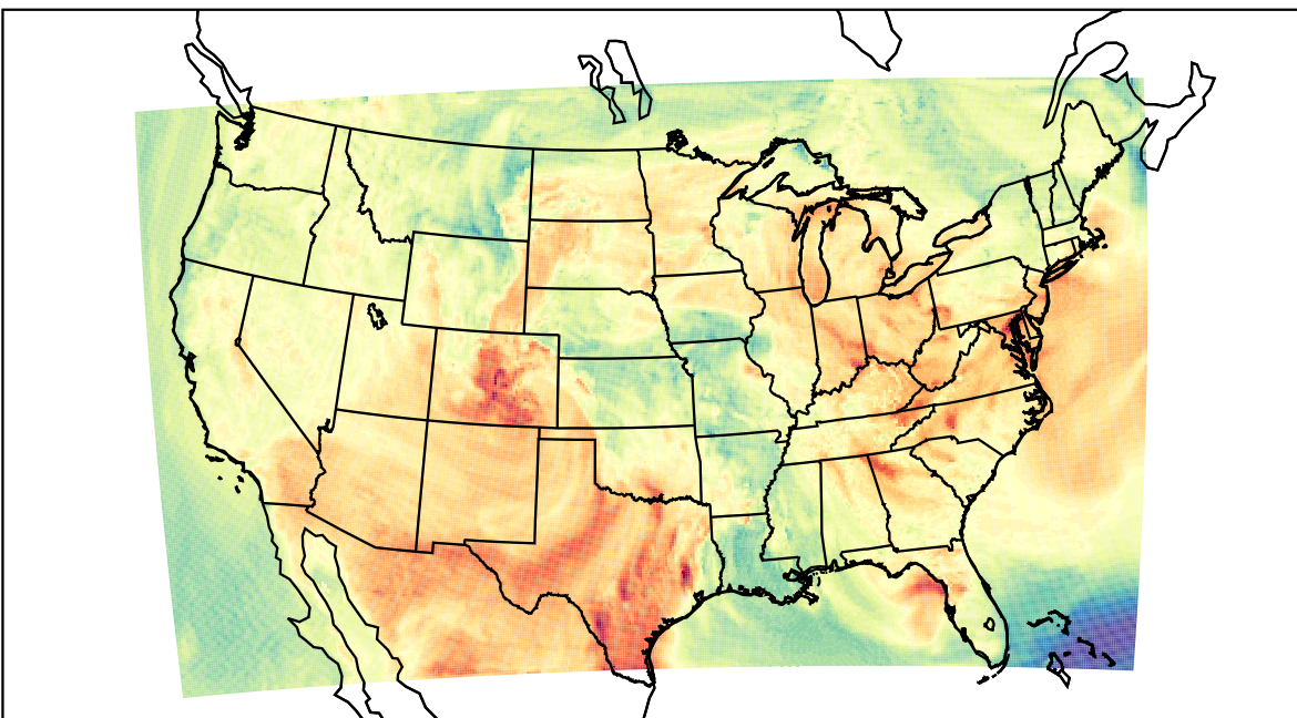
WRF (2023-05-11_20:00:00)
