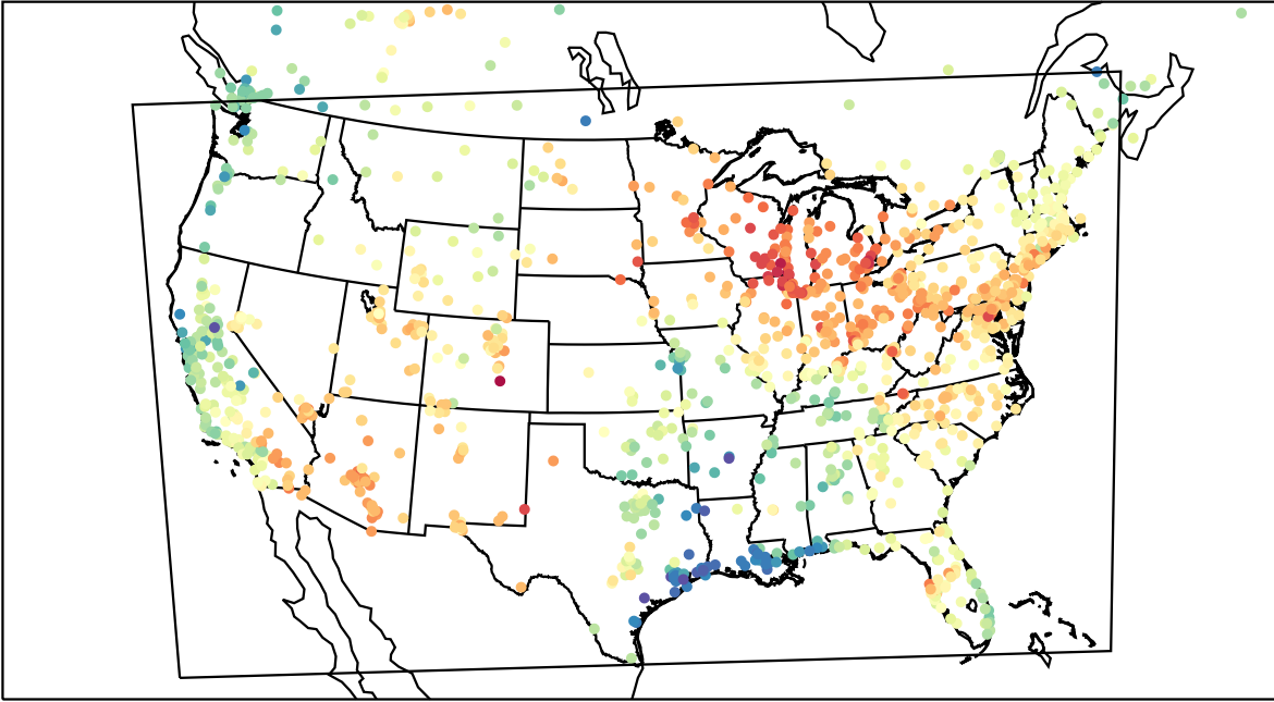
AirNOW (2023-05-11_19:00:00)
