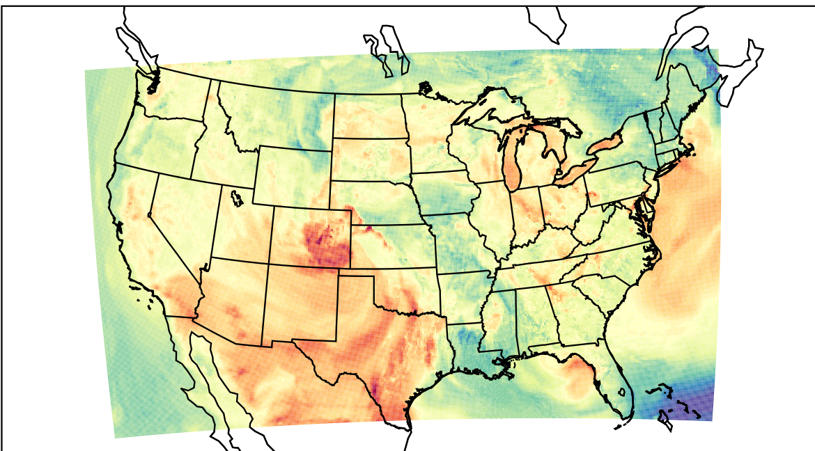
WRF (2023-05-11_23:00:00)
