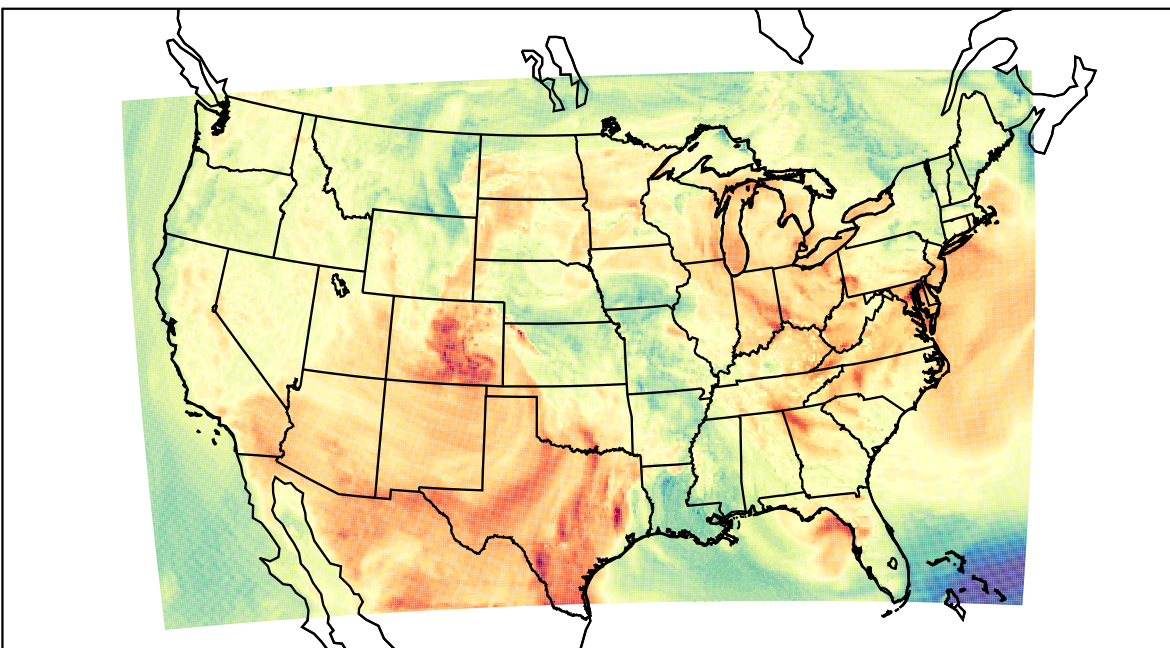
WRF (2023-05-11_21:00:00)
