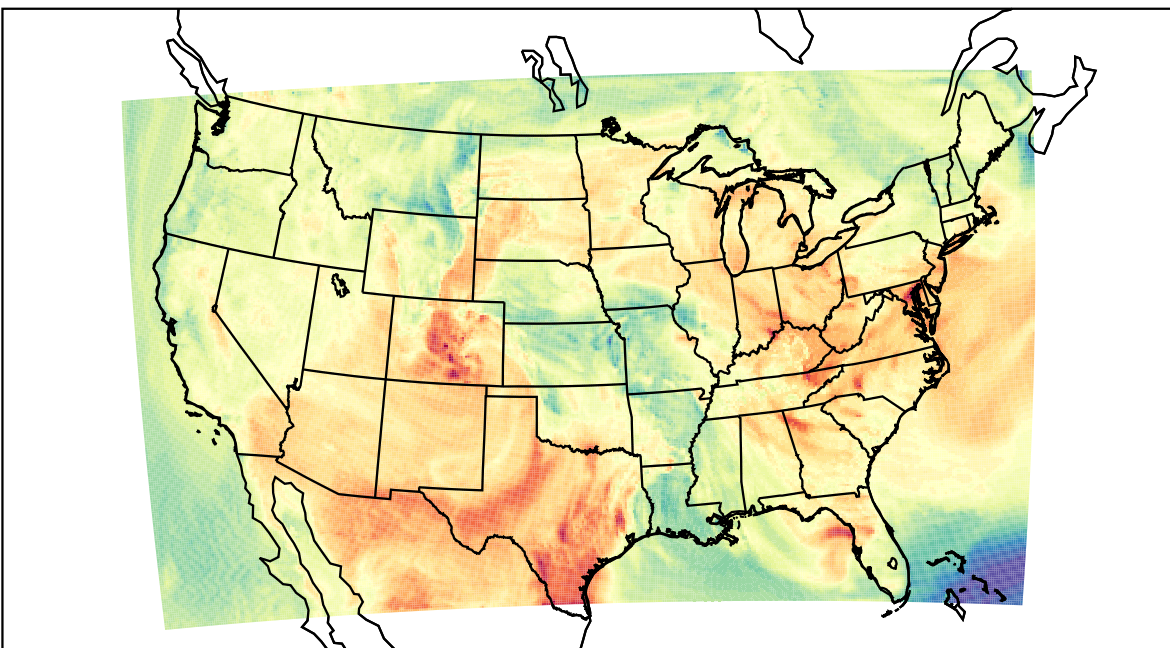
WRF (2023-05-11_19:00:00)
