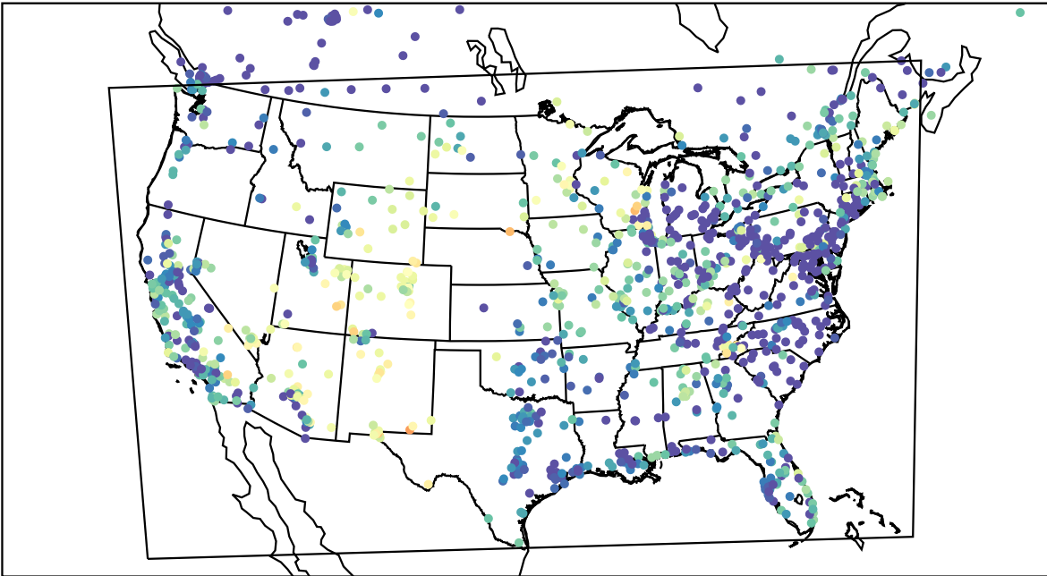
AirNOW (2023-05-11_09:00:00)
