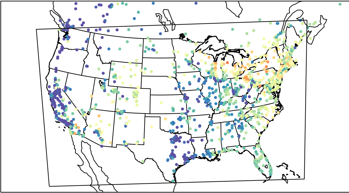
AirNOW (2023-05-12_14:00:00)
