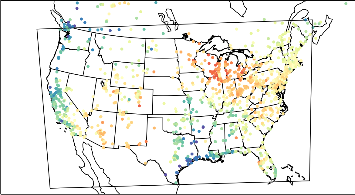
AirNOW (2023-05-11_17:00:00)
