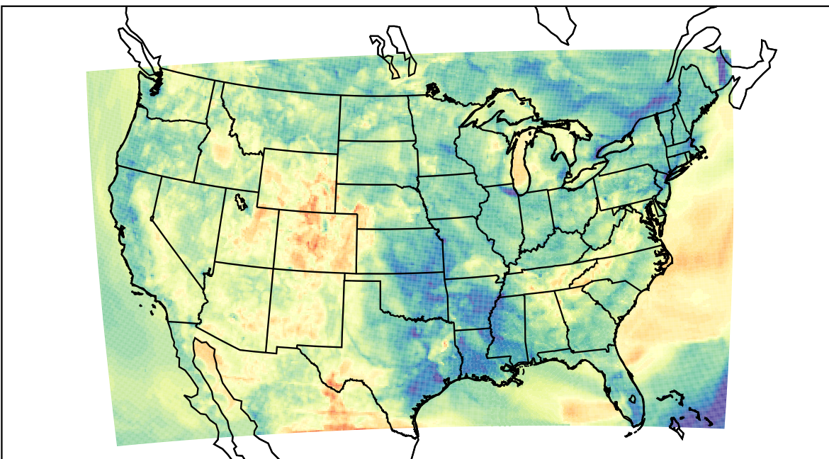
WRF (2023-05-11_04:00:00)
