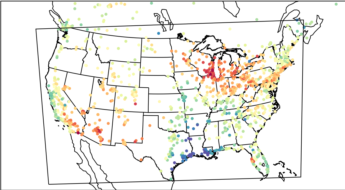
AirNOW (2023-05-11_23:00:00)
