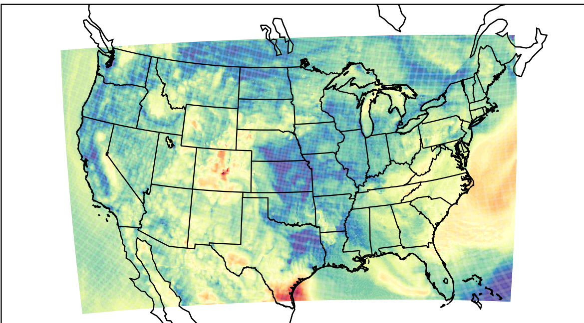
WRF (2023-05-11_14:00:00)
