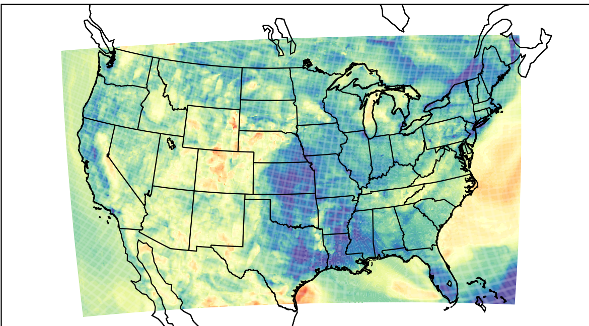
WRF (2023-05-11_09:00:00)
