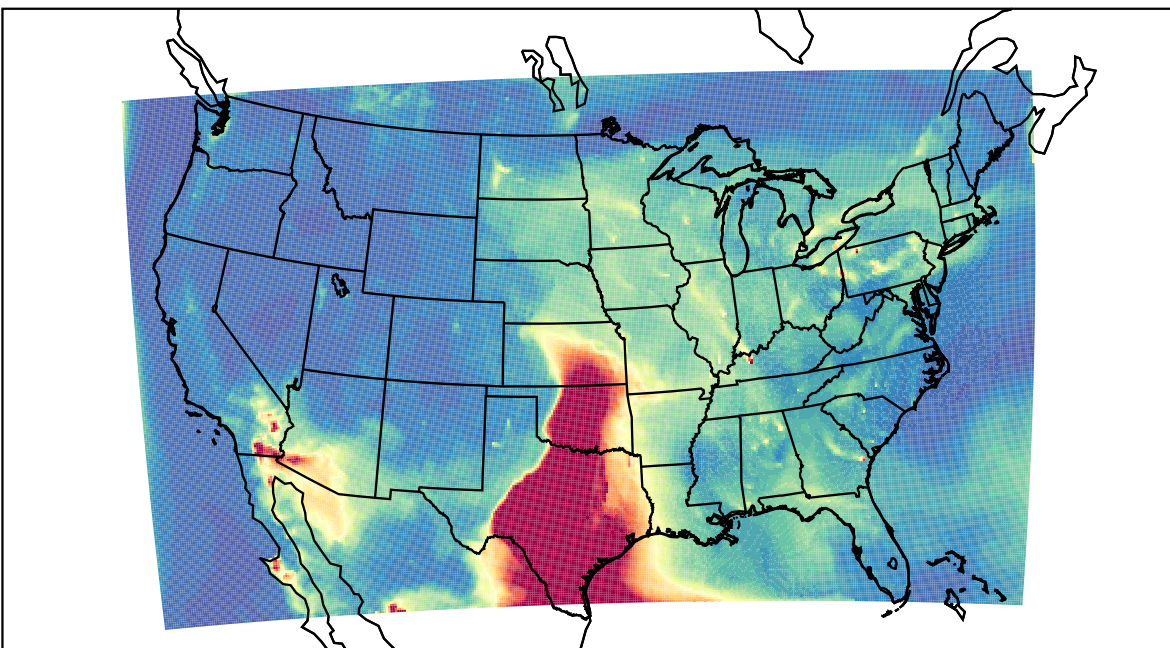
WRF 2023-05-12_09:00:00
