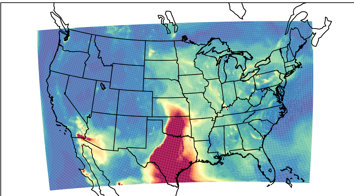
WRF 2023-05-12_08:00:00
