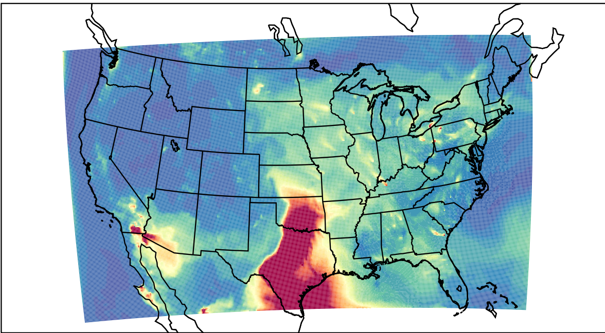
WRF 2023-05-12_06:00:00
