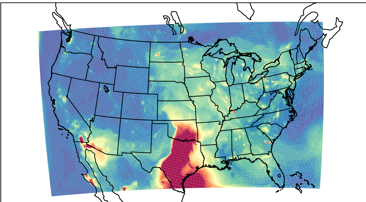
WRF 2023-05-12_04:00:00
