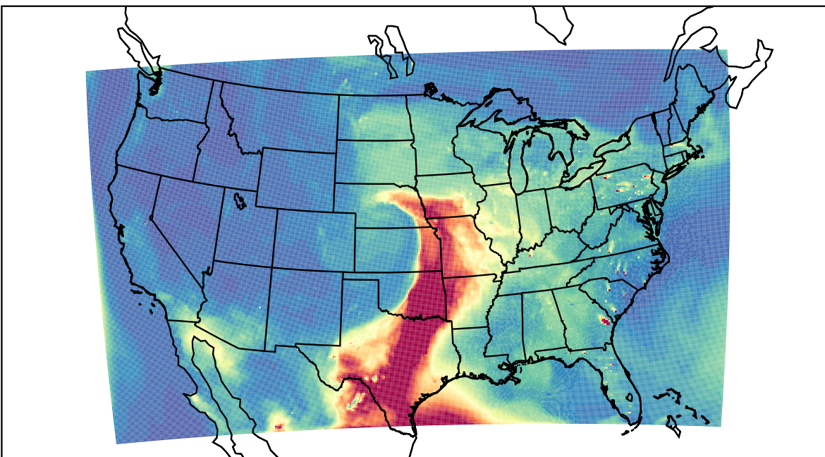
WRF 2023-05-12_22:00:00
