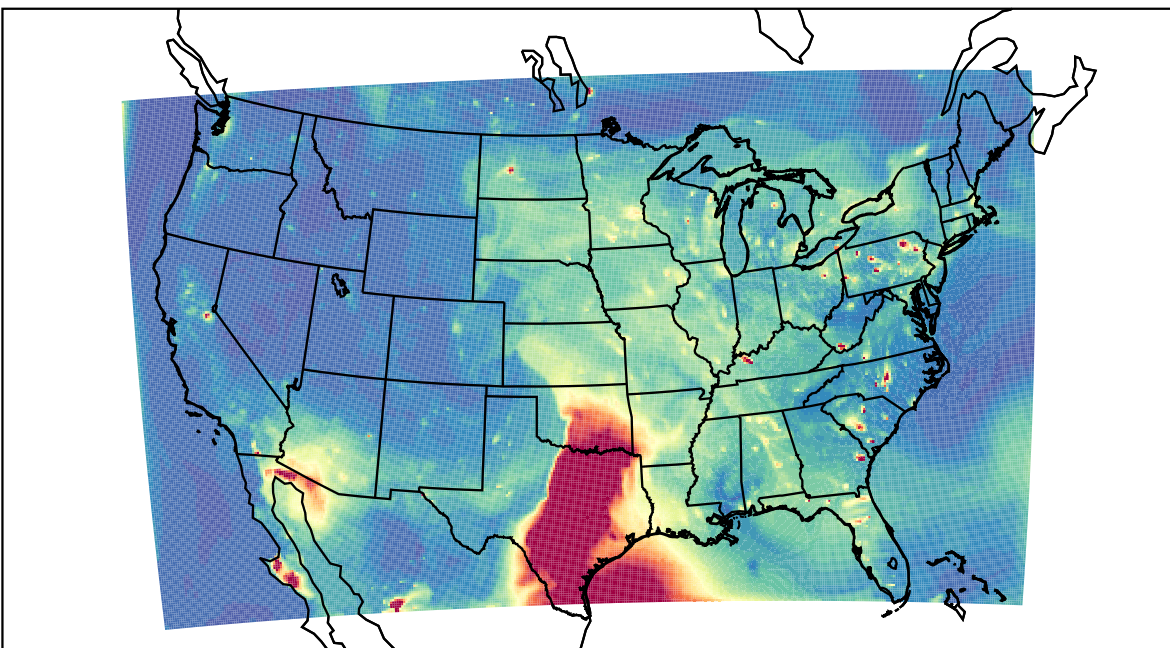
WRF 2023-05-12_02:00:00
