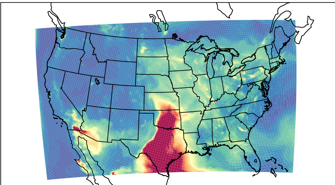
WRF 2023-05-12_07:00:00
