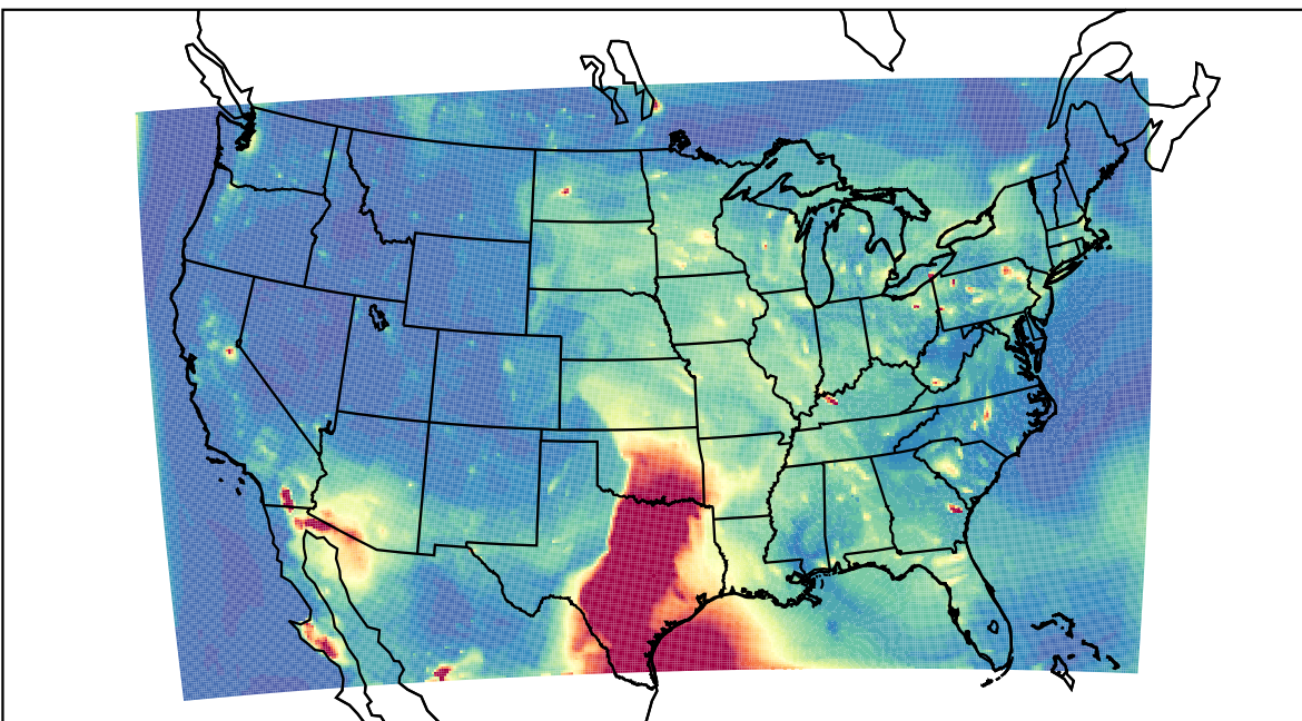
WRF 2023-05-12_03:00:00
