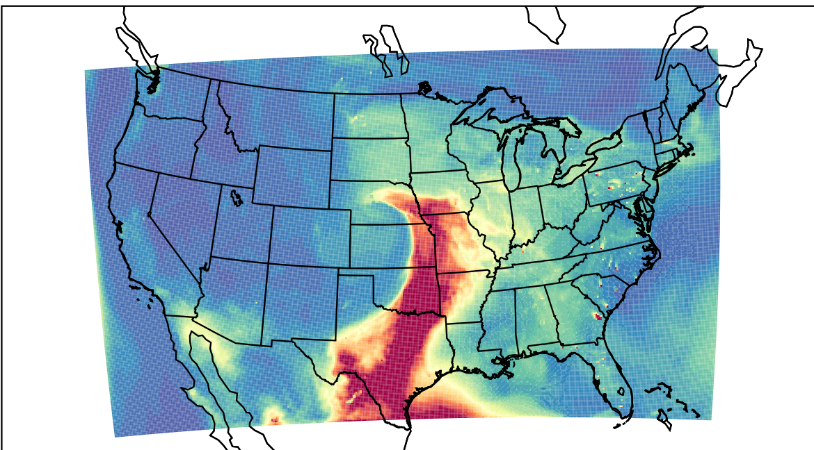
WRF 2023-05-12_21:00:00
