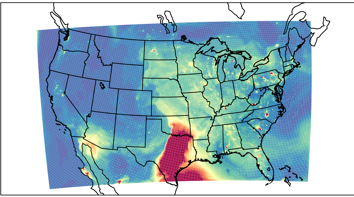
WRF 2023-05-12_01:00:00
