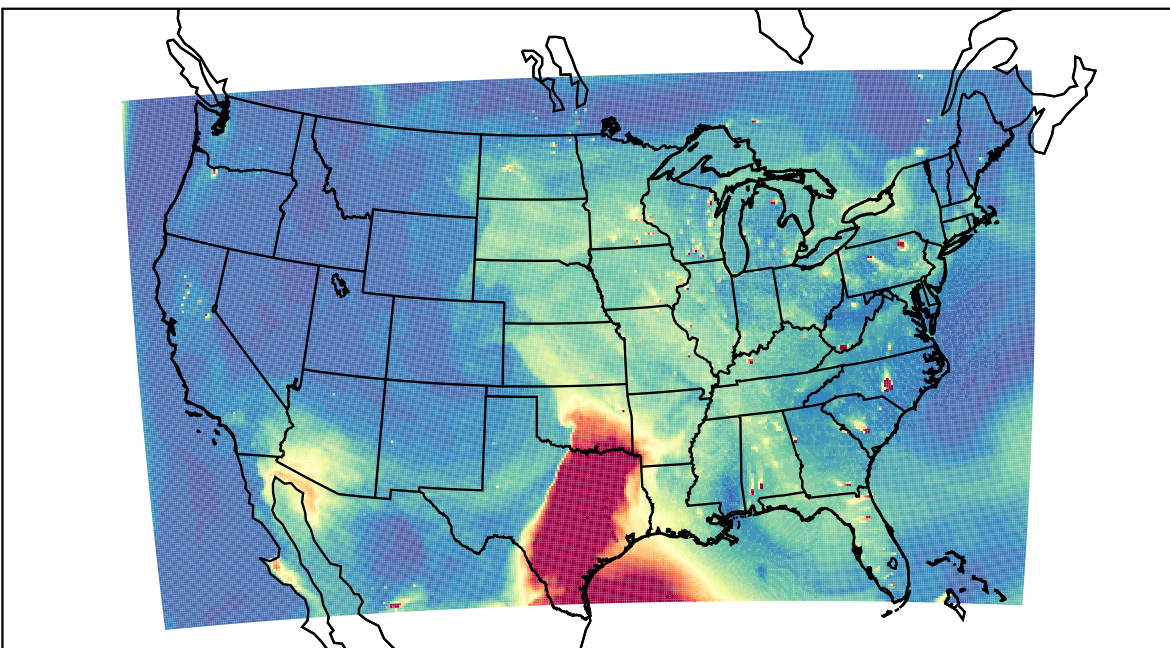
WRF 2023-05-12_00:00:00
