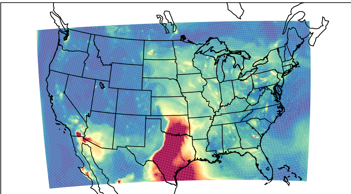
WRF 2023-05-12_05:00:00
