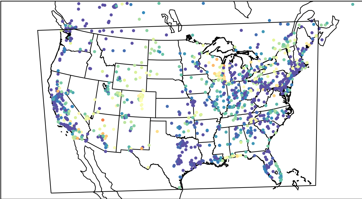
AirNOW (2023-05-12_09:00:00)
