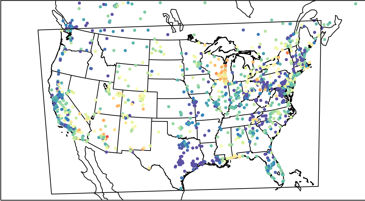
AirNOW (2023-05-12_05:00:00)
