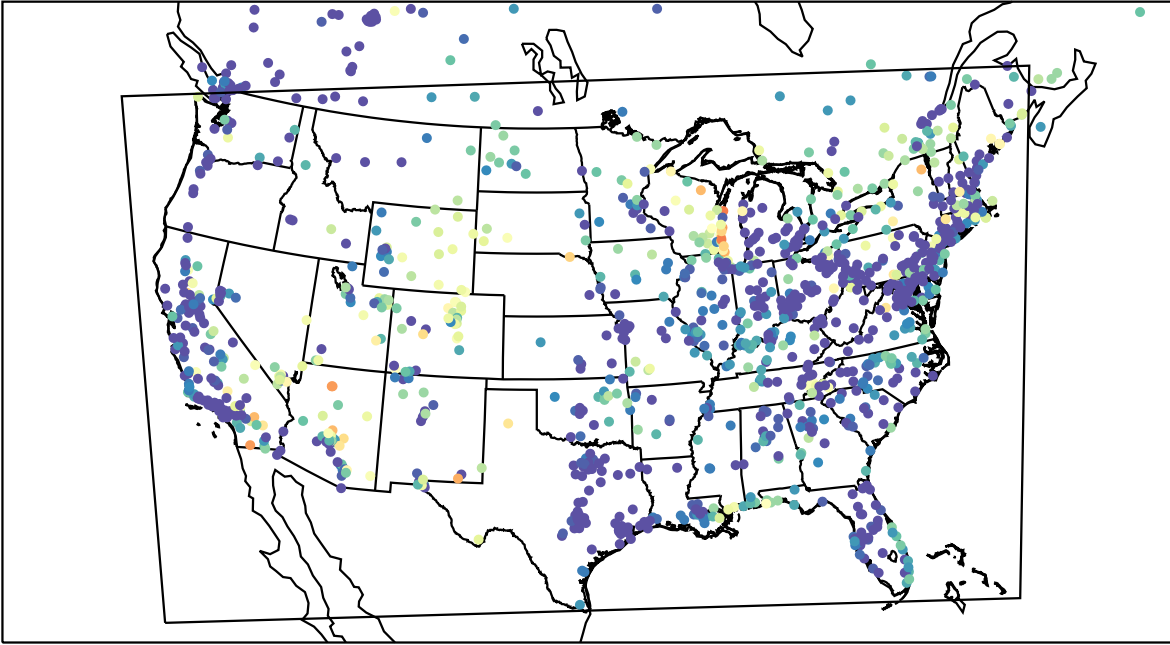
AirNOW (2023-05-12_11:00:00)
