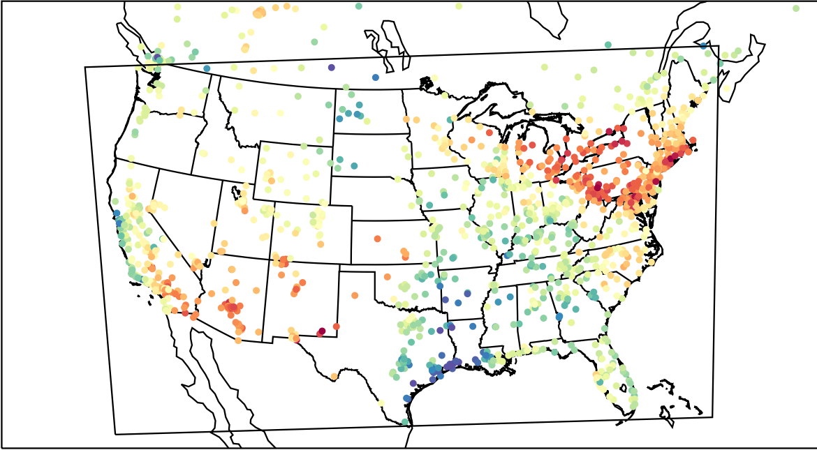
AirNOW (2023-05-12_20:00:00)
