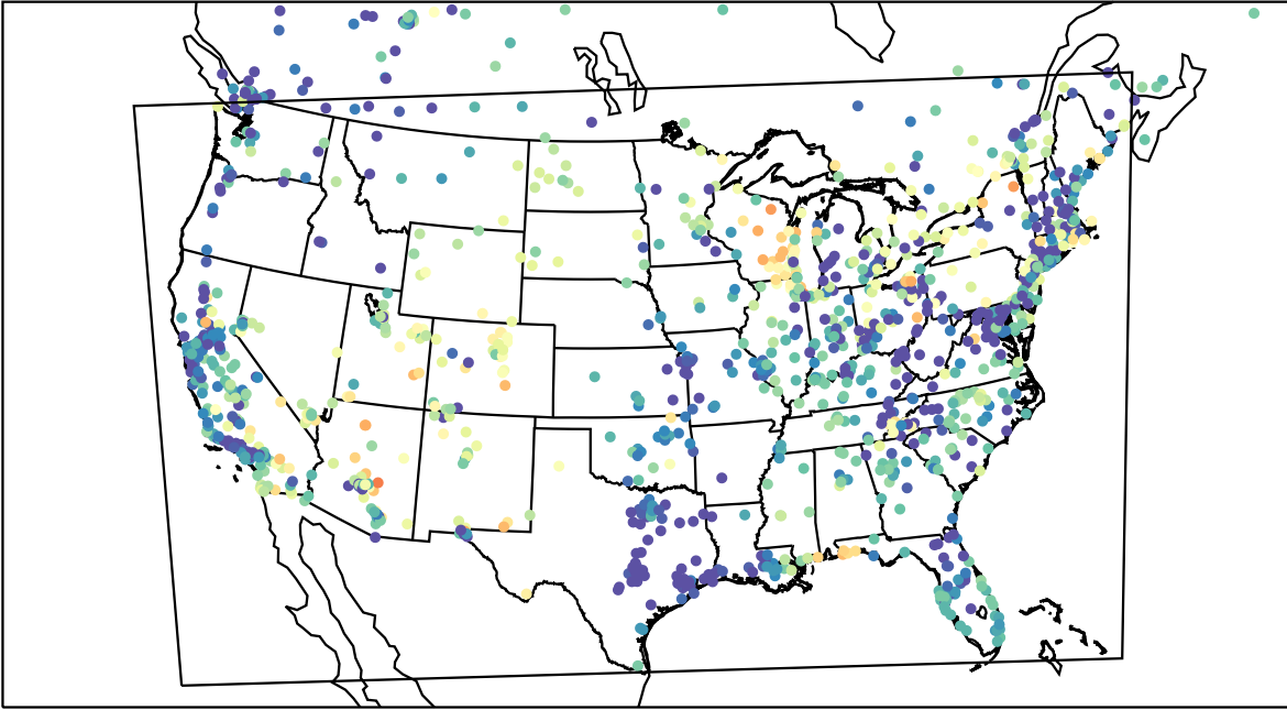
AirNOW (2023-05-12_06:00:00)
