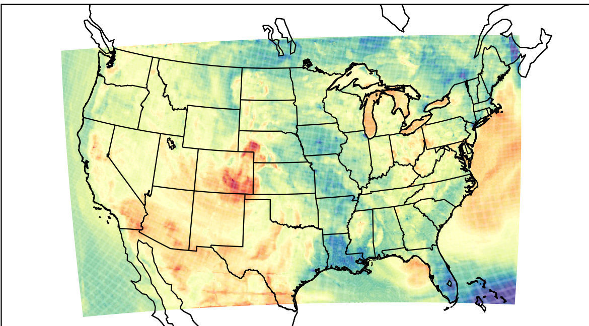
WRF (2023-05-12_01:00:00)
