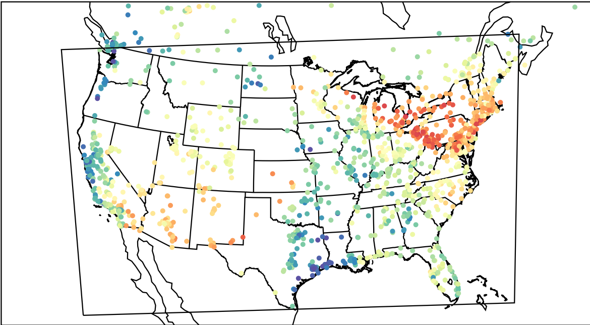
AirNOW (2023-05-12_17:00:00)
