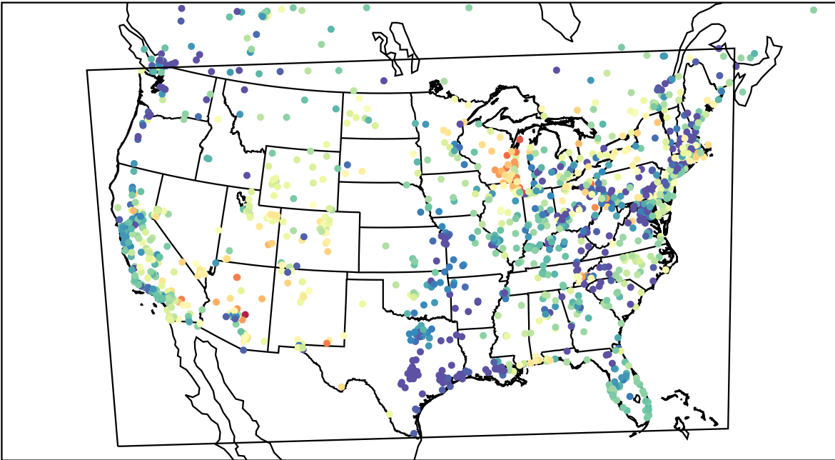
AirNOW (2023-05-12_04:00:00)
