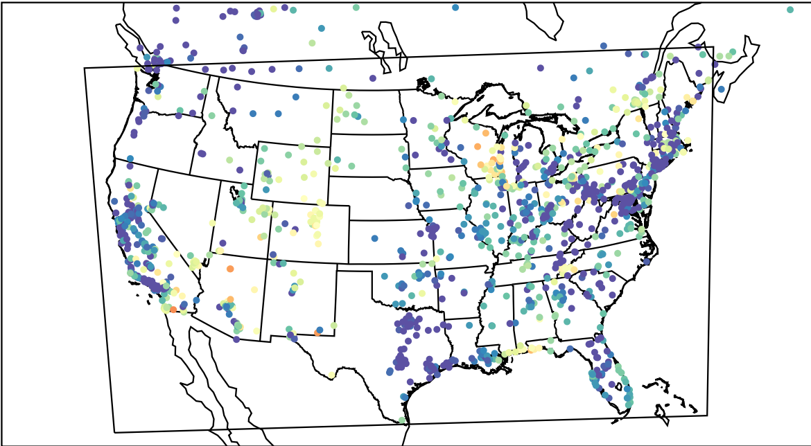
AirNOW (2023-05-12_08:00:00)
