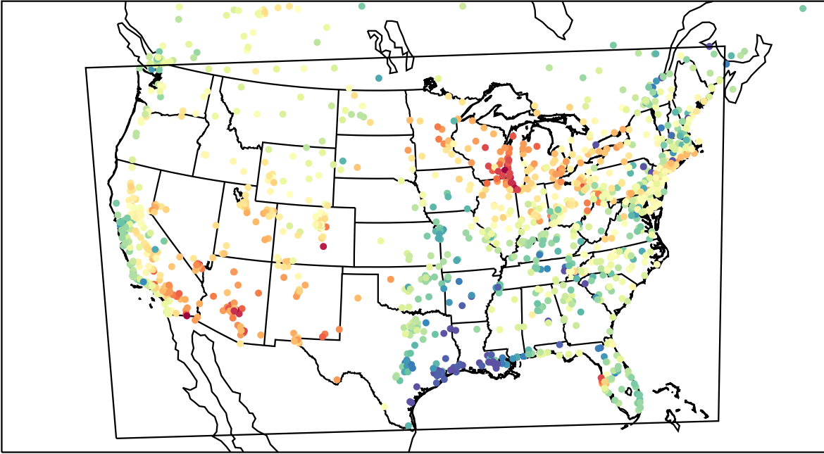
AirNOW (2023-05-12_00:00:00)
