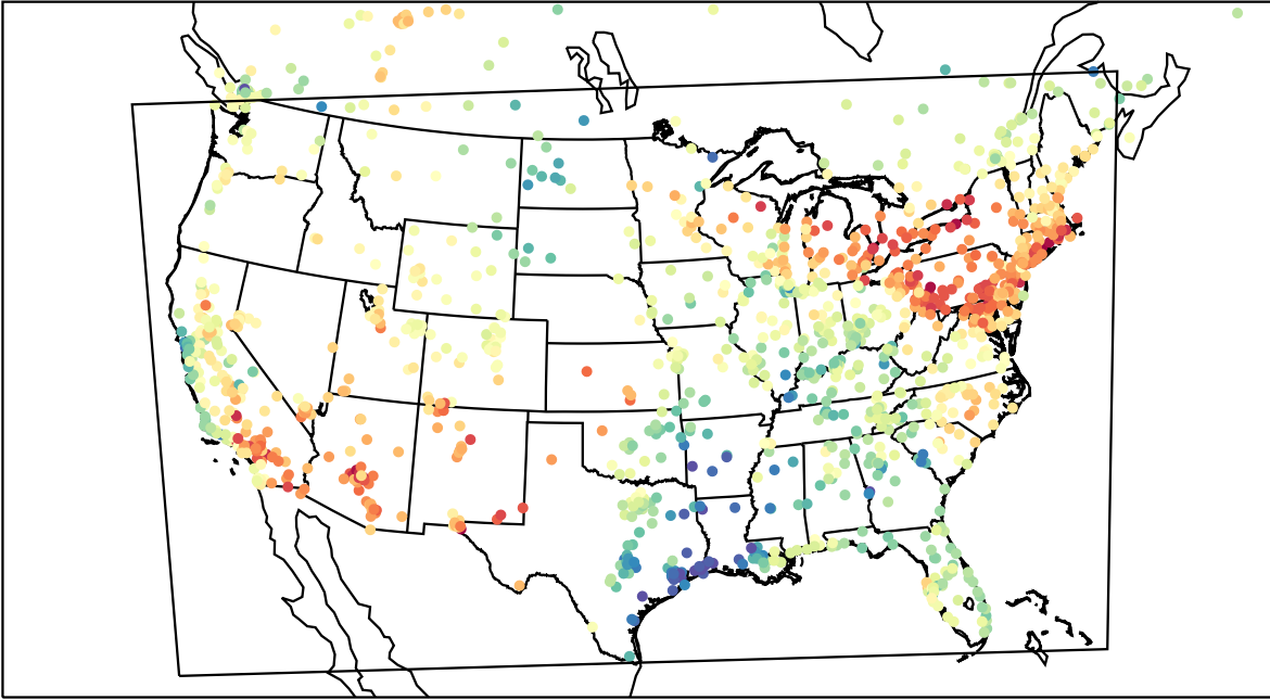
AirNOW (2023-05-12_21:00:00)
