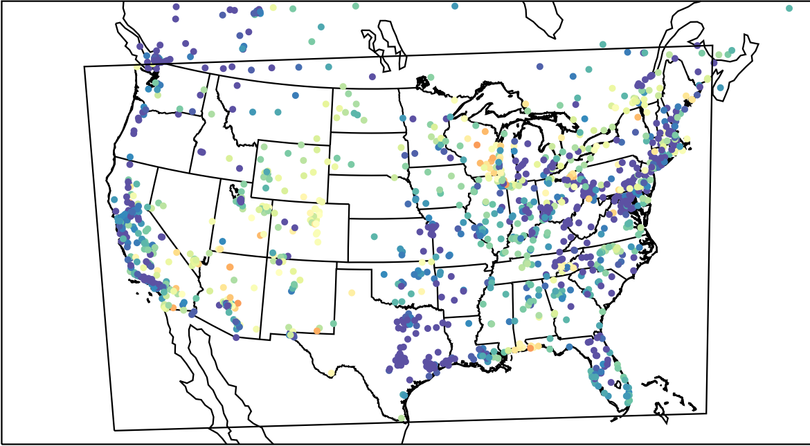
AirNOW (2023-05-12_07:00:00)
