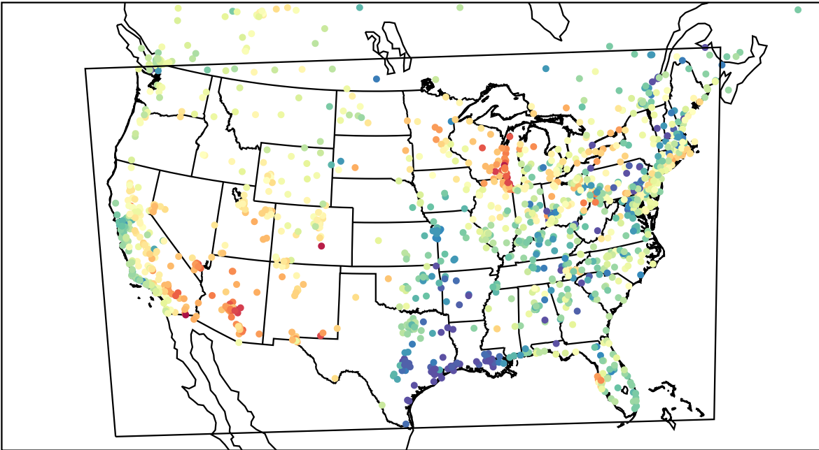
AirNOW (2023-05-12_01:00:00)
