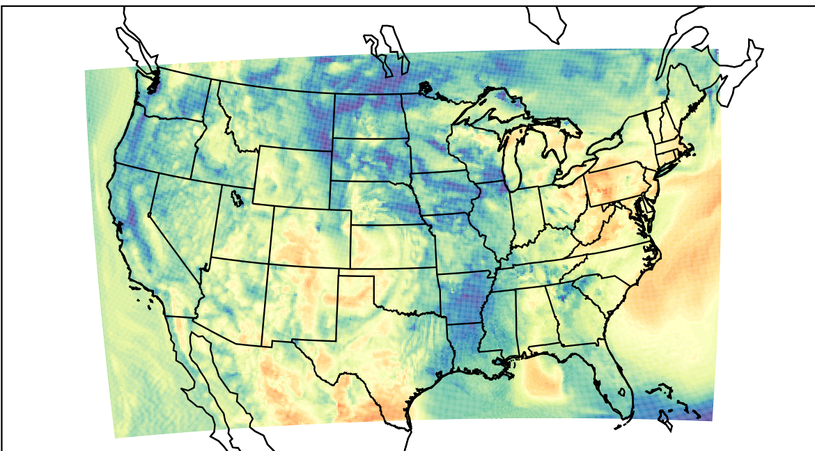
WRF (2023-05-12_15:00:00)
