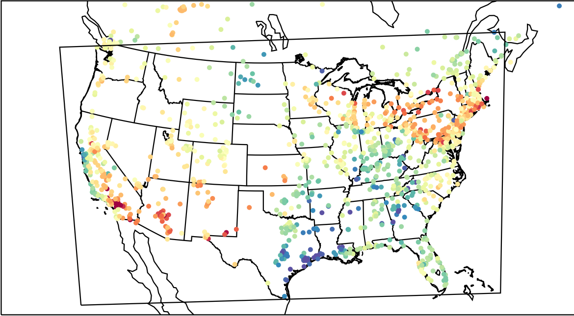
AirNOW (2023-05-12_23:00:00)
