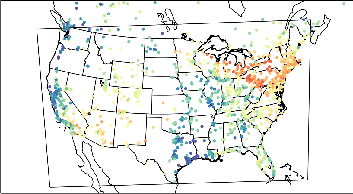
AirNOW (2023-05-12_16:00:00)
