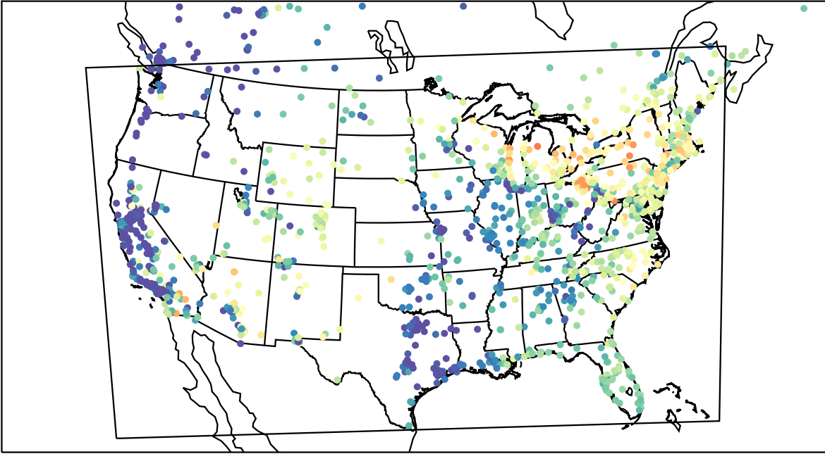
AirNOW (2023-05-12_14:00:00)
