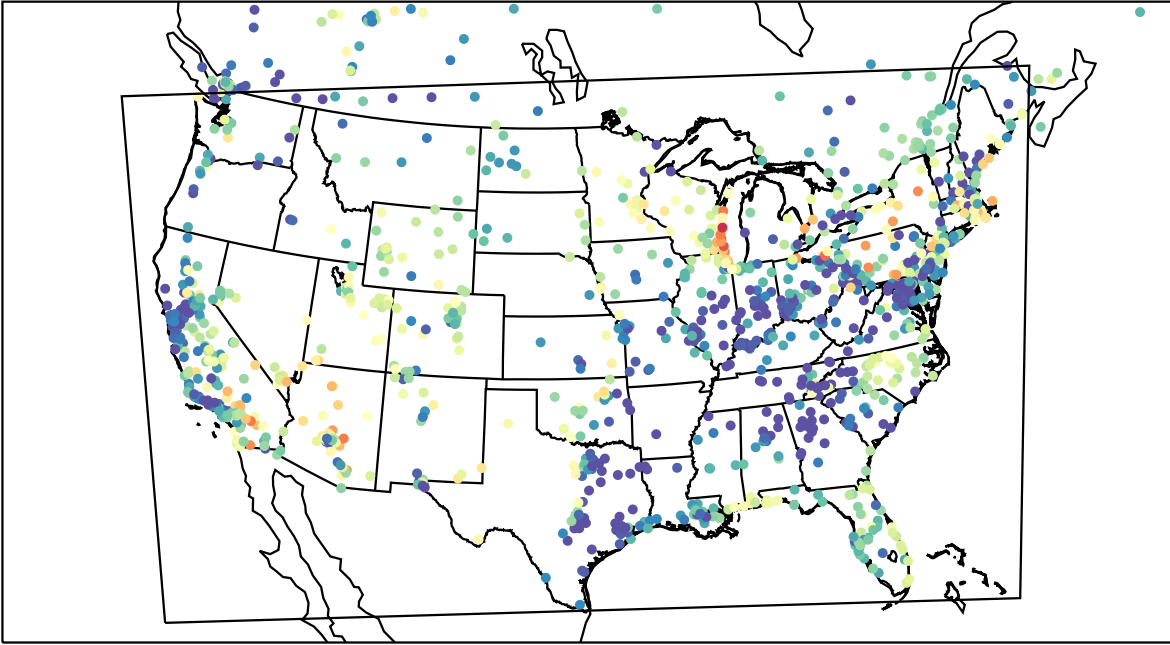
AirNOW (2023-05-13_05:00:00)
