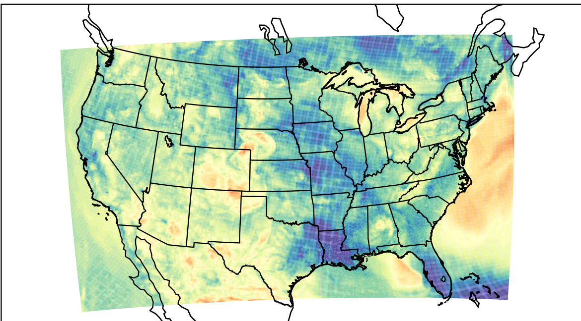
WRF (2023-05-12_06:00:00)
