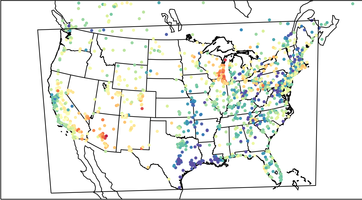
AirNOW (2023-05-12_02:00:00)
