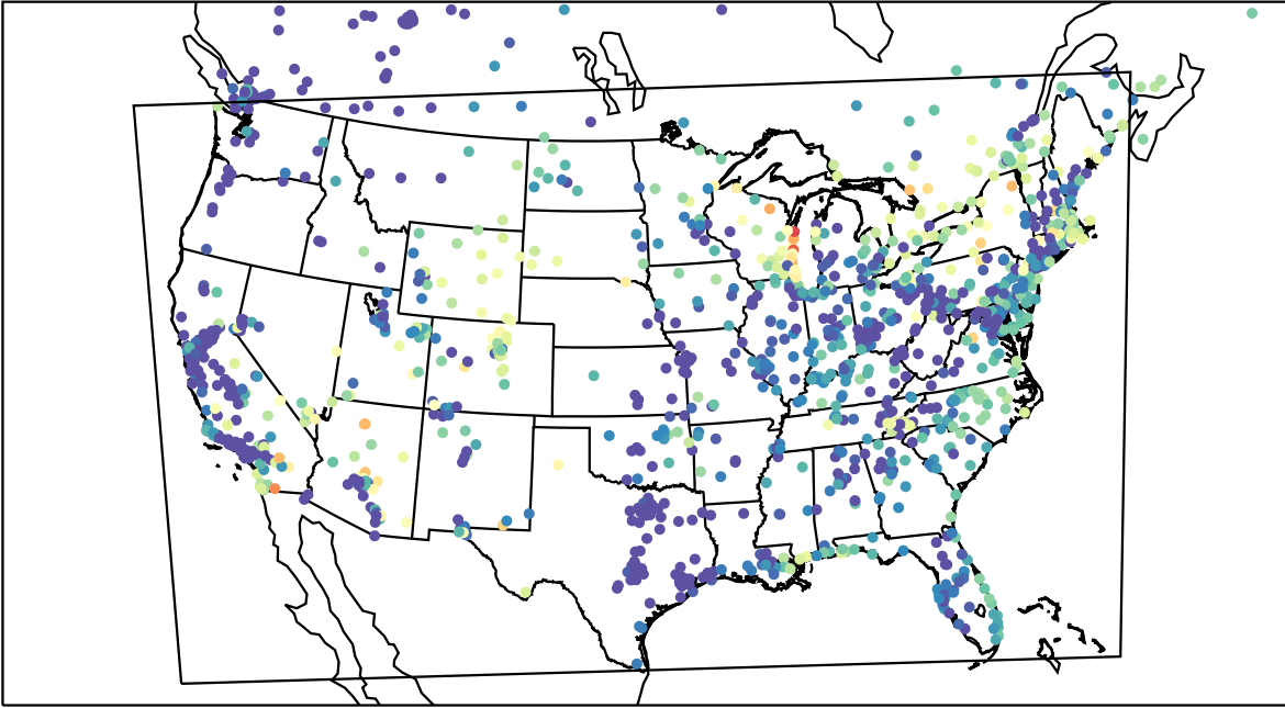
AirNOW (2023-05-12_12:00:00)
