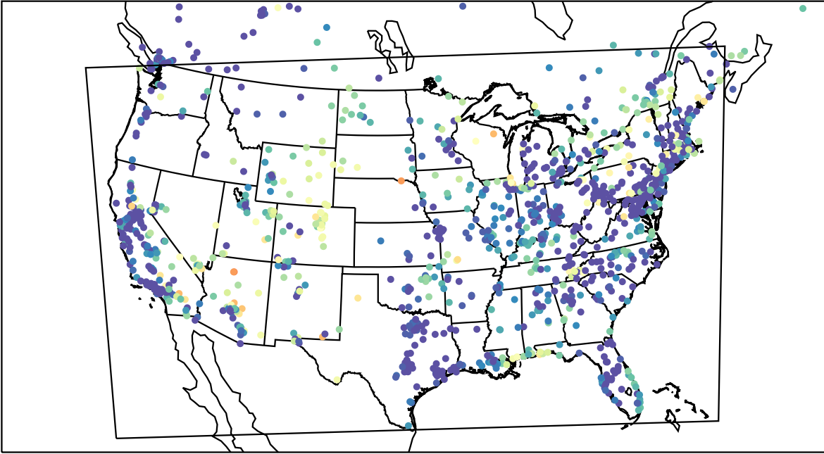
AirNOW (2023-05-12_10:00:00)
