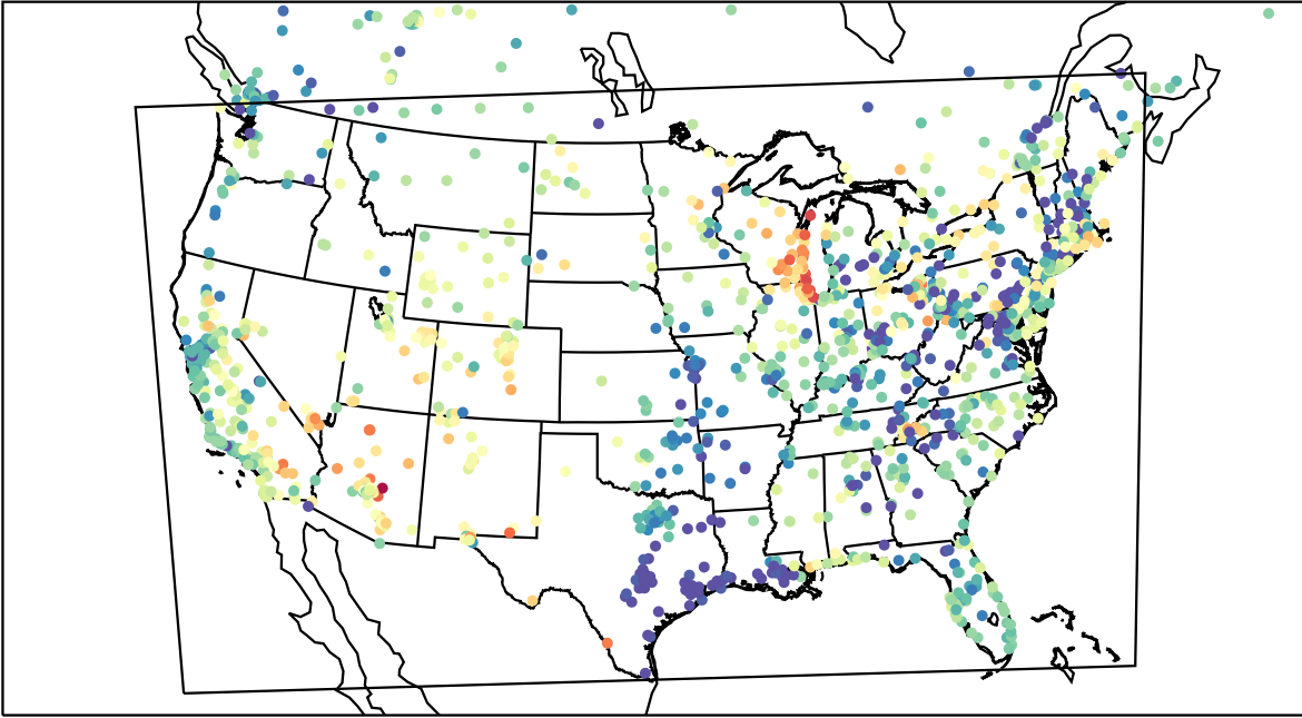
AirNOW (2023-05-12_03:00:00)
