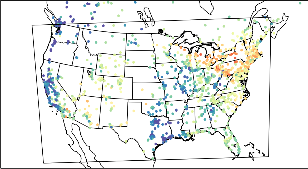
AirNOW (2023-05-12_15:00:00)
