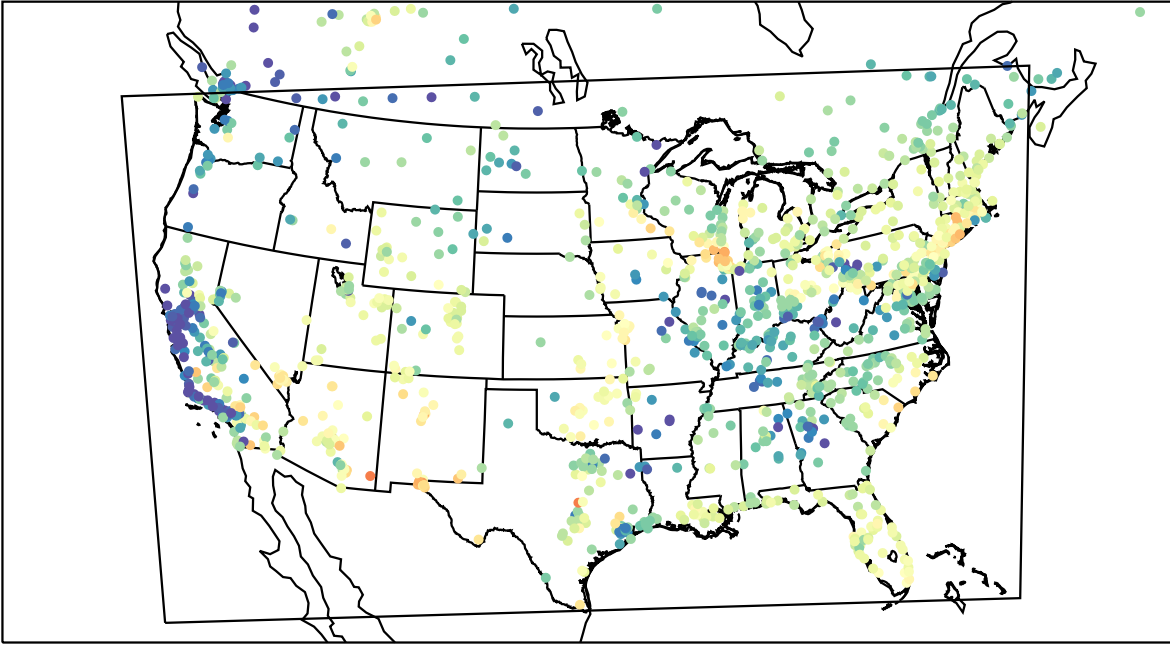
AirNOW (2023-05-13_15:00:00)
