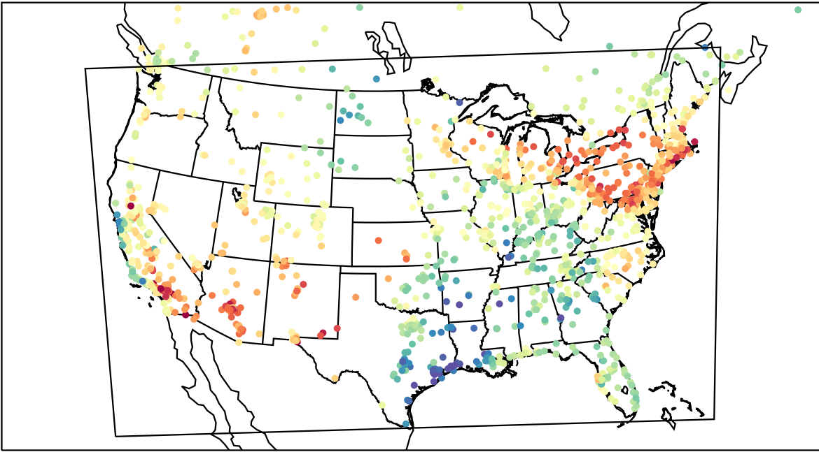
AirNOW (2023-05-12_22:00:00)
