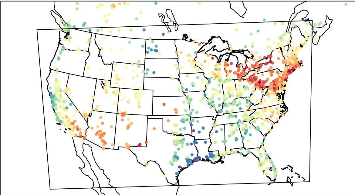
AirNOW (2023-05-12_19:00:00)
