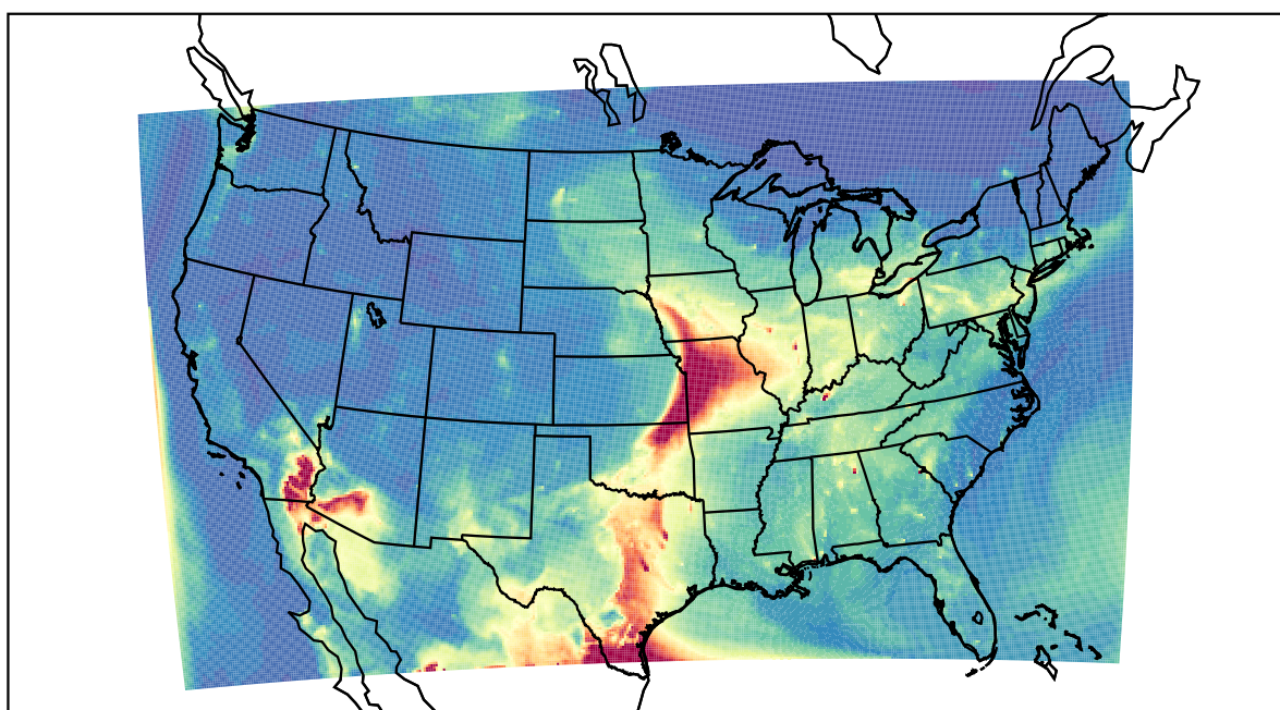
WRF 2023-05-13_11:00:00
