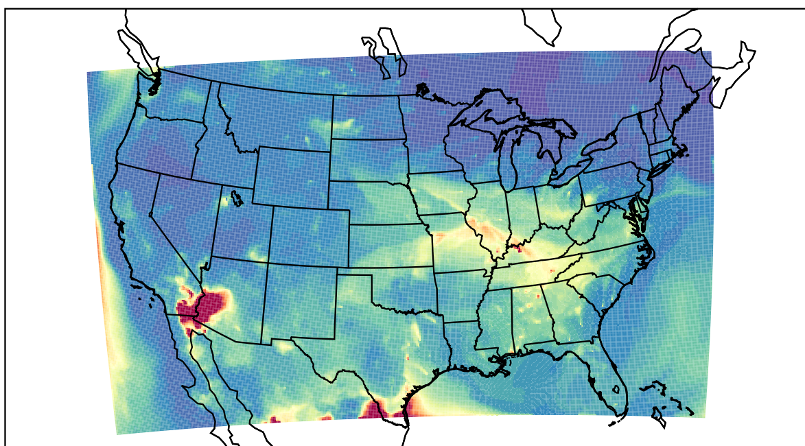
WRF 2023-05-14_08:00:00
