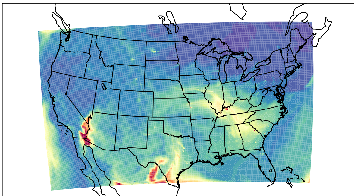
WRF 2023-05-14_17:00:00
