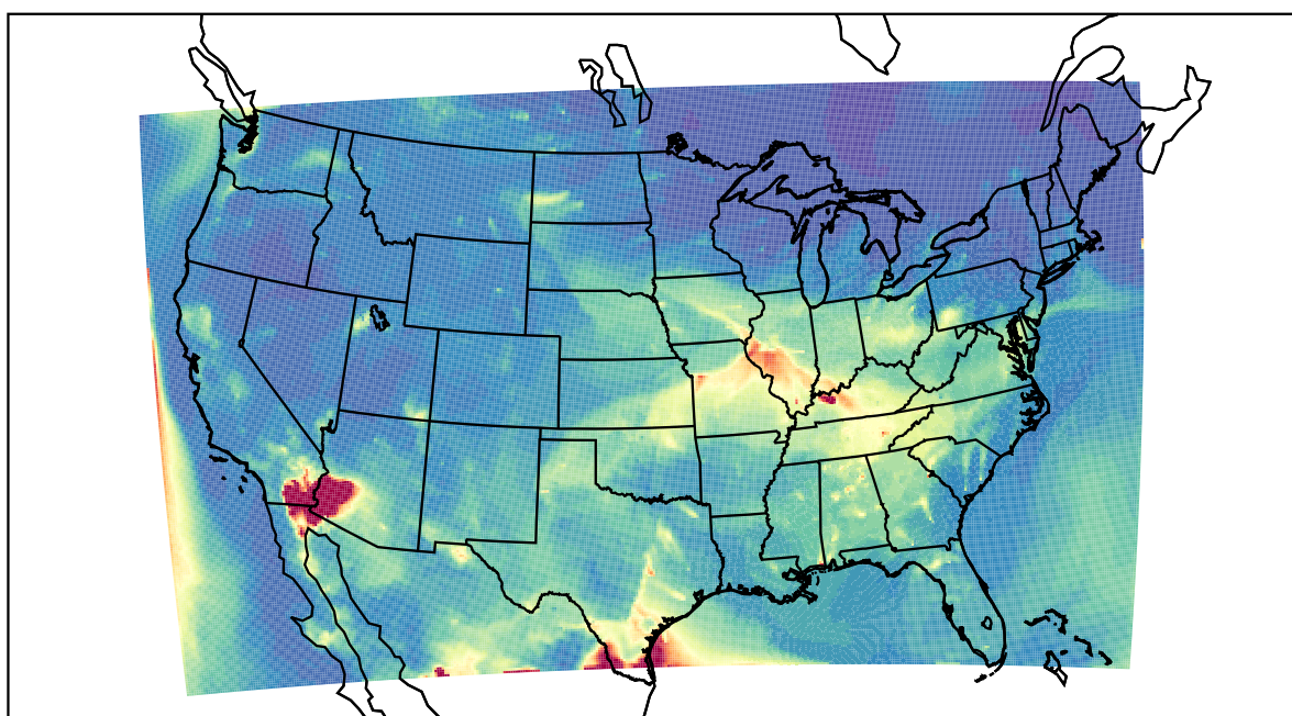
WRF 2023-05-14_06:00:00
