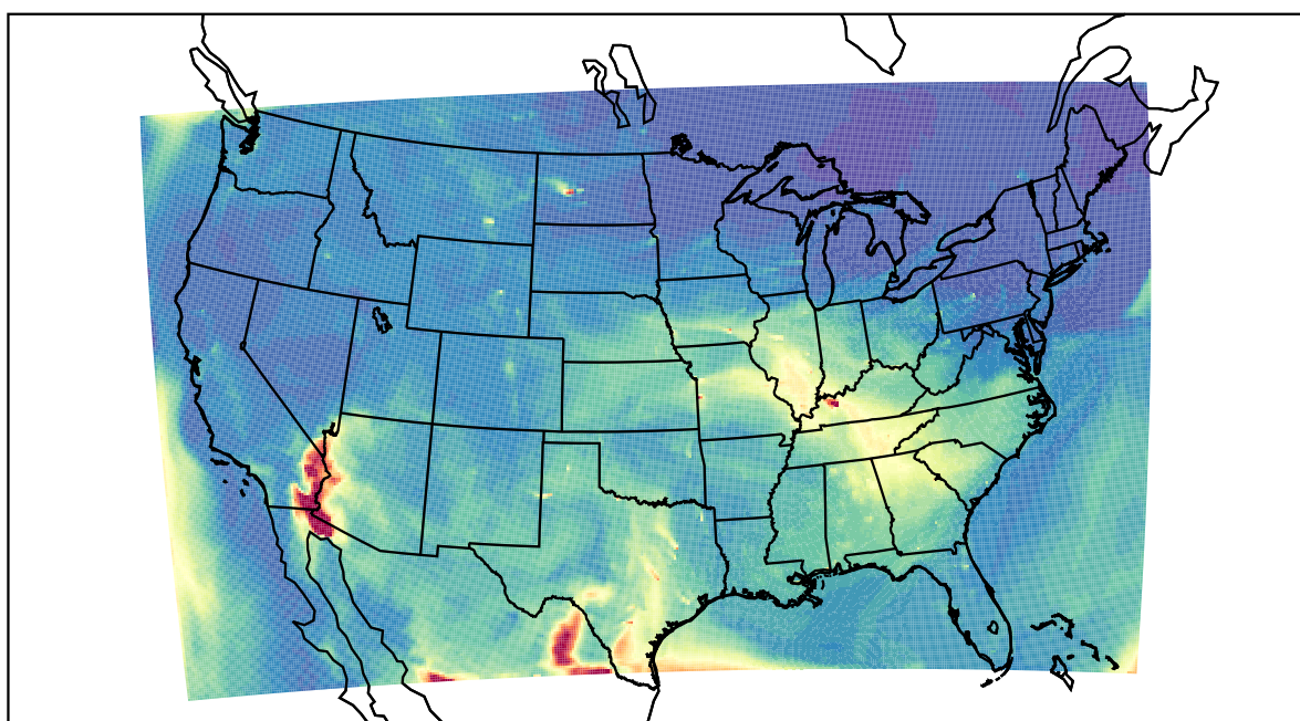
WRF 2023-05-14_16:00:00
