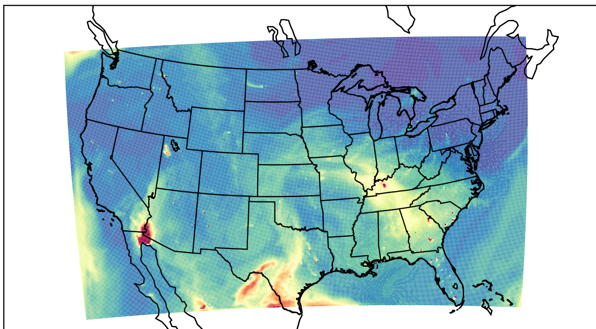
WRF 2023-05-14_22:00:00
