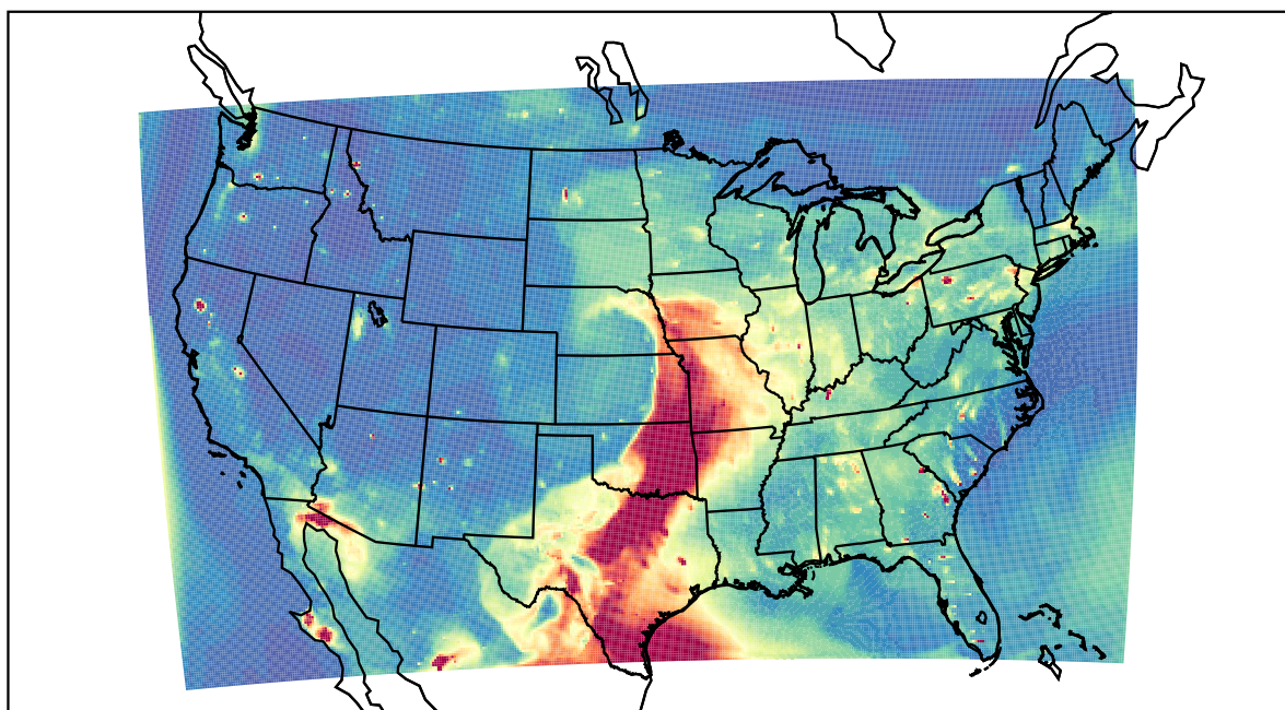
WRF 2023-05-13_02:00:00
