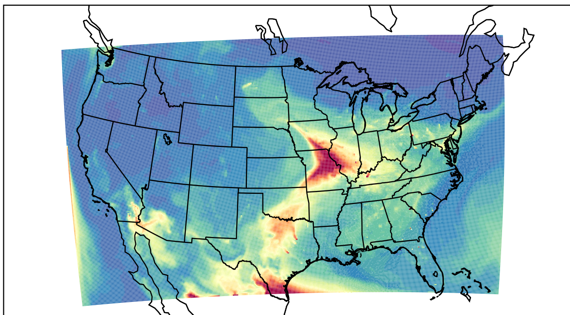
WRF 2023-05-13_17:00:00
