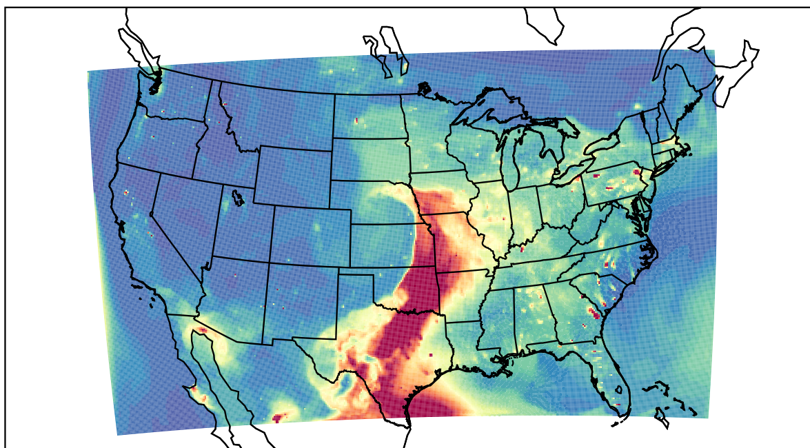
WRF 2023-05-13_01:00:00
