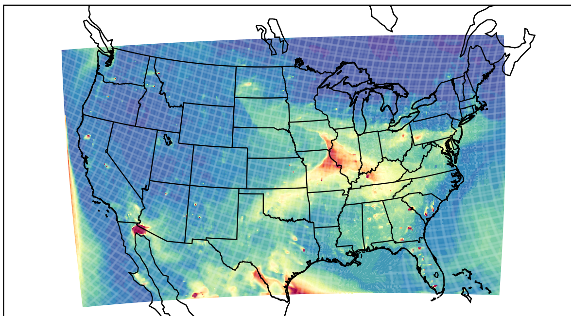
WRF 2023-05-14_01:00:00
