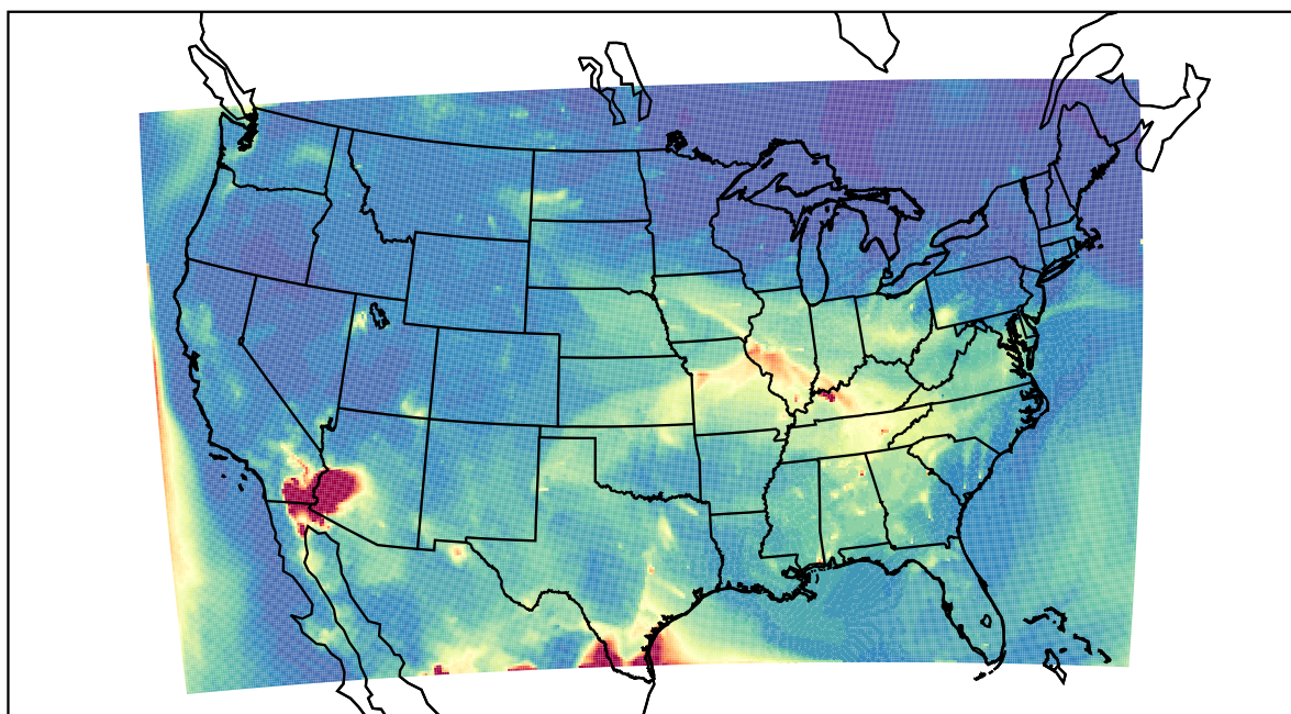
WRF 2023-05-14_07:00:00
