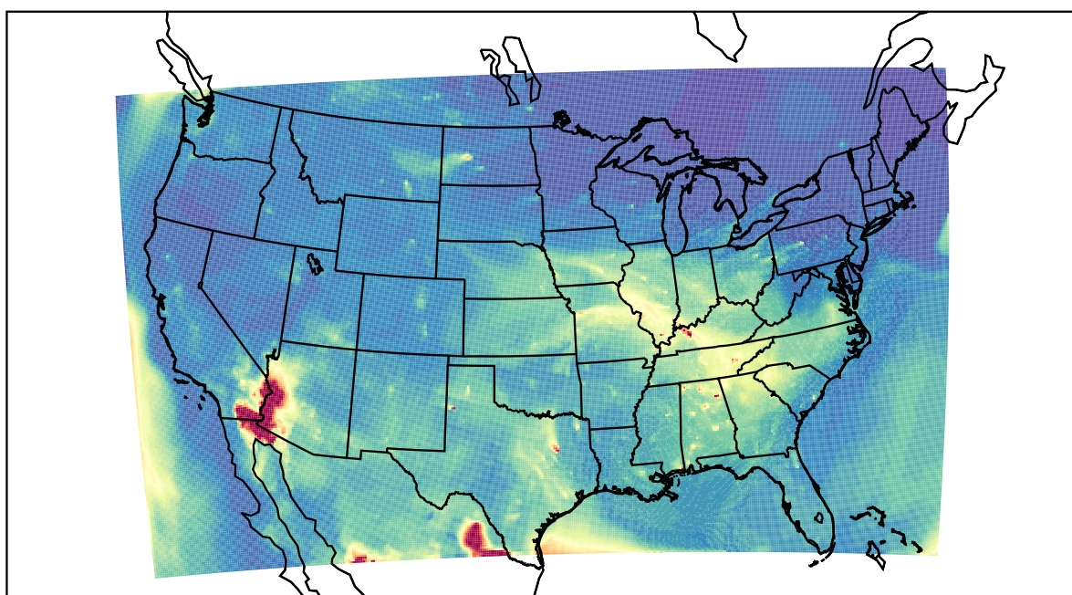
WRF 2023-05-14_13:00:00
