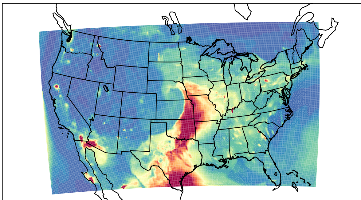
WRF 2023-05-13_04:00:00
