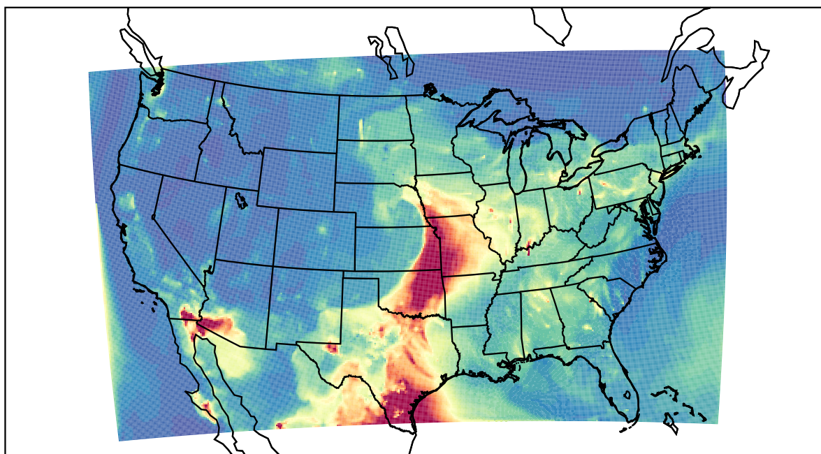
WRF 2023-05-13_06:00:00
