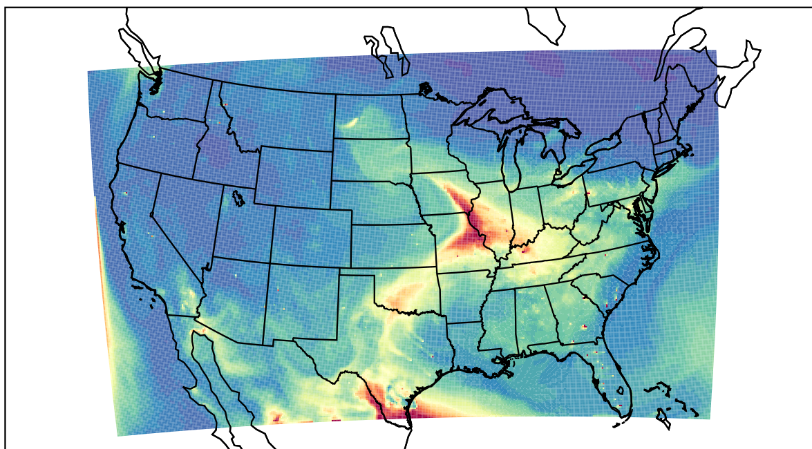
WRF 2023-05-13_21:00:00
