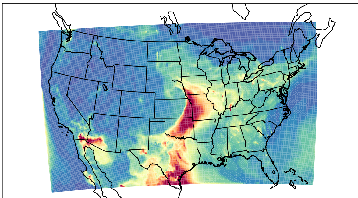
WRF 2023-05-13_07:00:00
