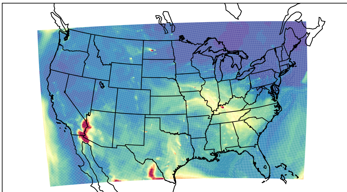
WRF 2023-05-14_15:00:00
