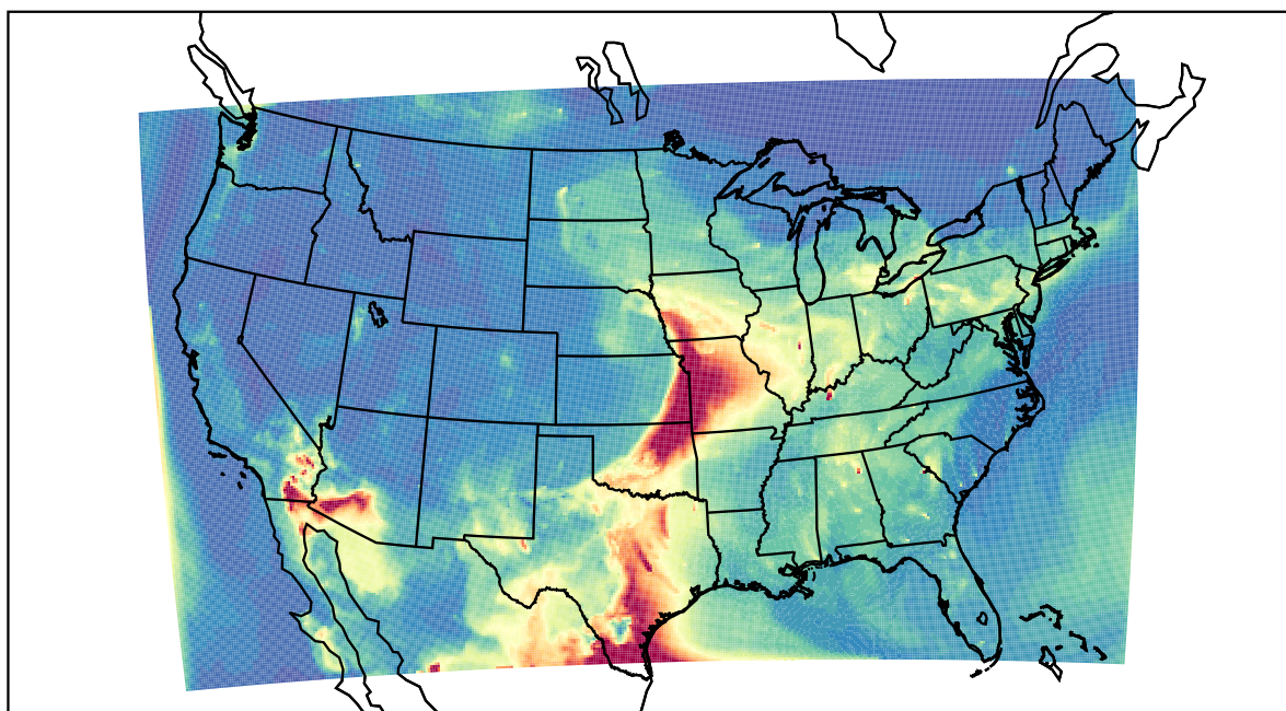
WRF 2023-05-13_09:00:00
