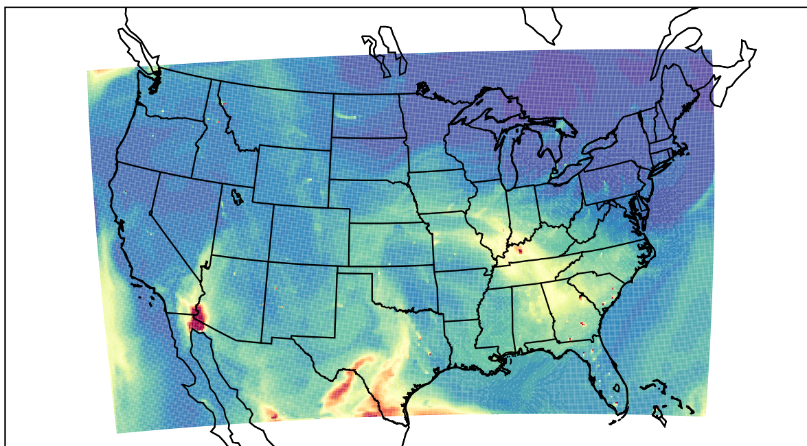
WRF 2023-05-14_21:00:00
