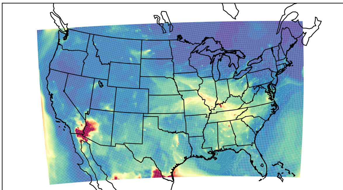
WRF 2023-05-14_10:00:00
