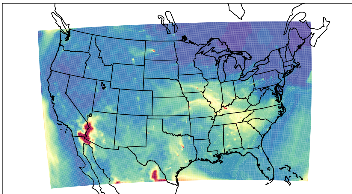
WRF 2023-05-14_14:00:00
