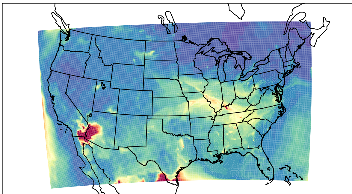
WRF 2023-05-14_09:00:00
