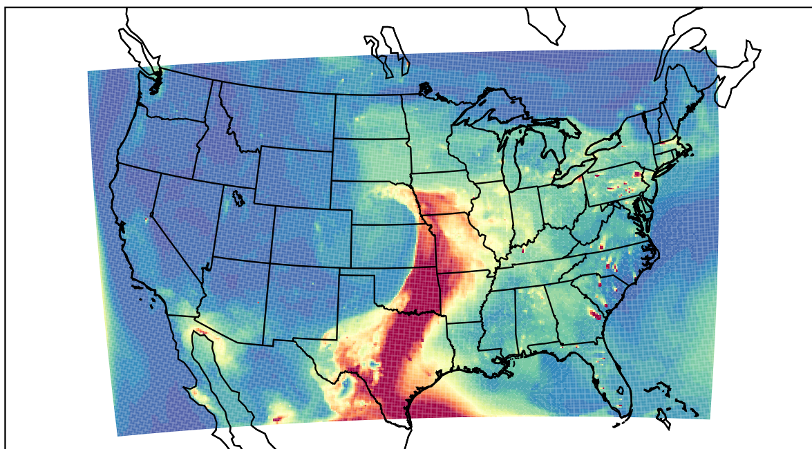
WRF 2023-05-13_00:00:00
