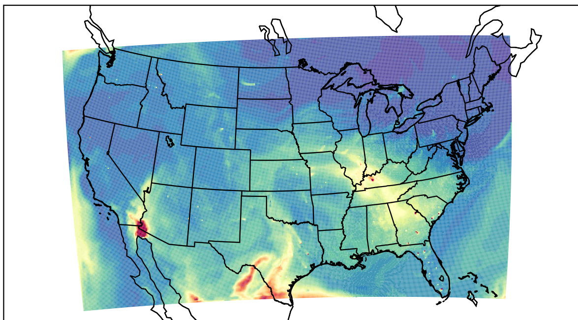
WRF 2023-05-14_20:00:00
