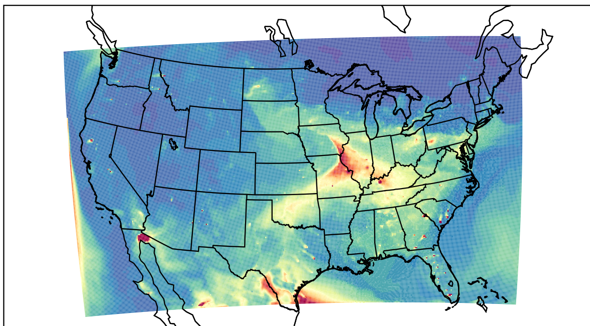
WRF 2023-05-14_00:00:00
