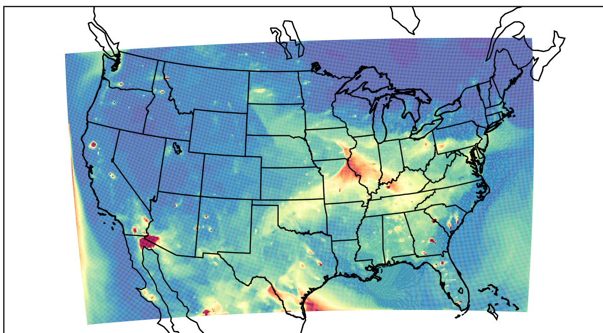
WRF 2023-05-14_02:00:00
