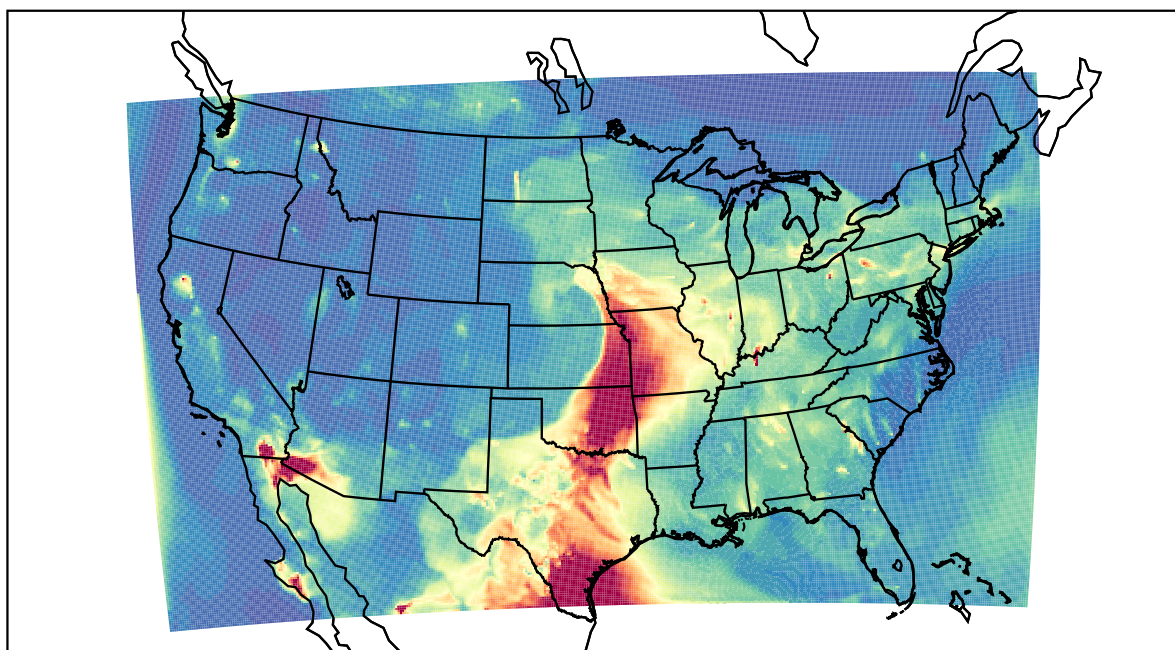
WRF 2023-05-13_05:00:00
