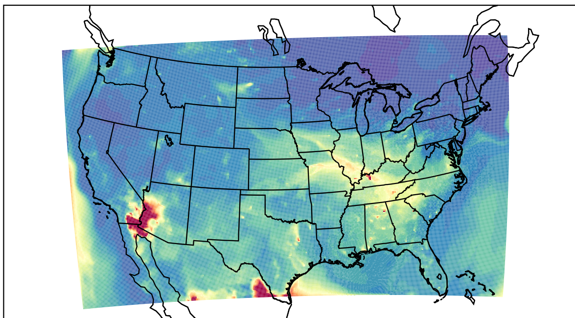
WRF 2023-05-14_11:00:00
