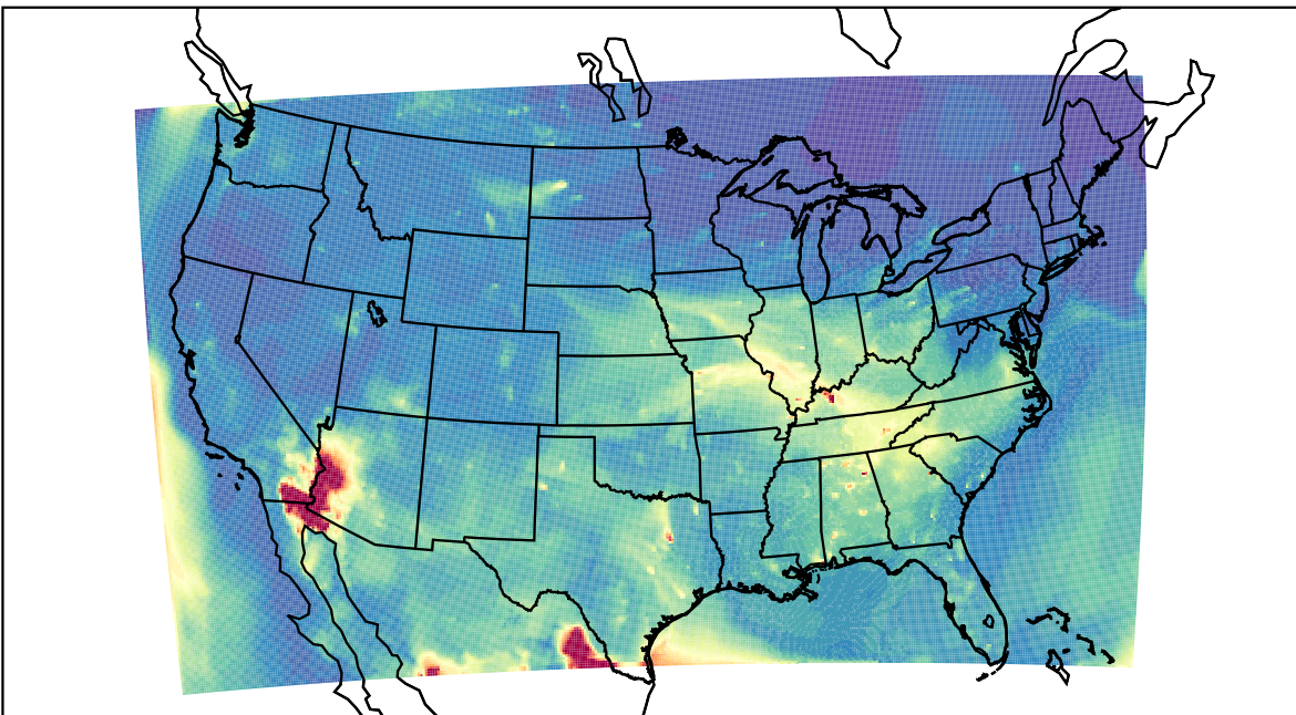
WRF 2023-05-14_12:00:00
