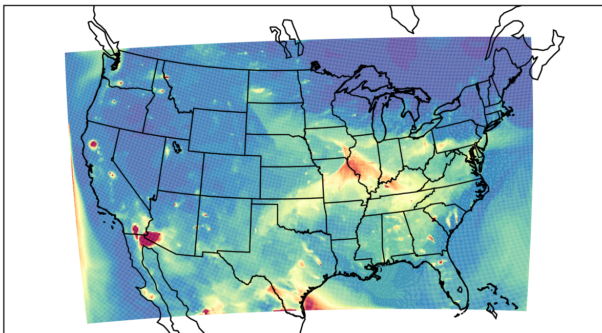
WRF 2023-05-14_03:00:00
