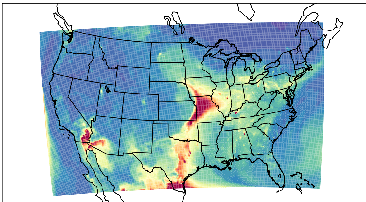
WRF 2023-05-13_12:00:00
