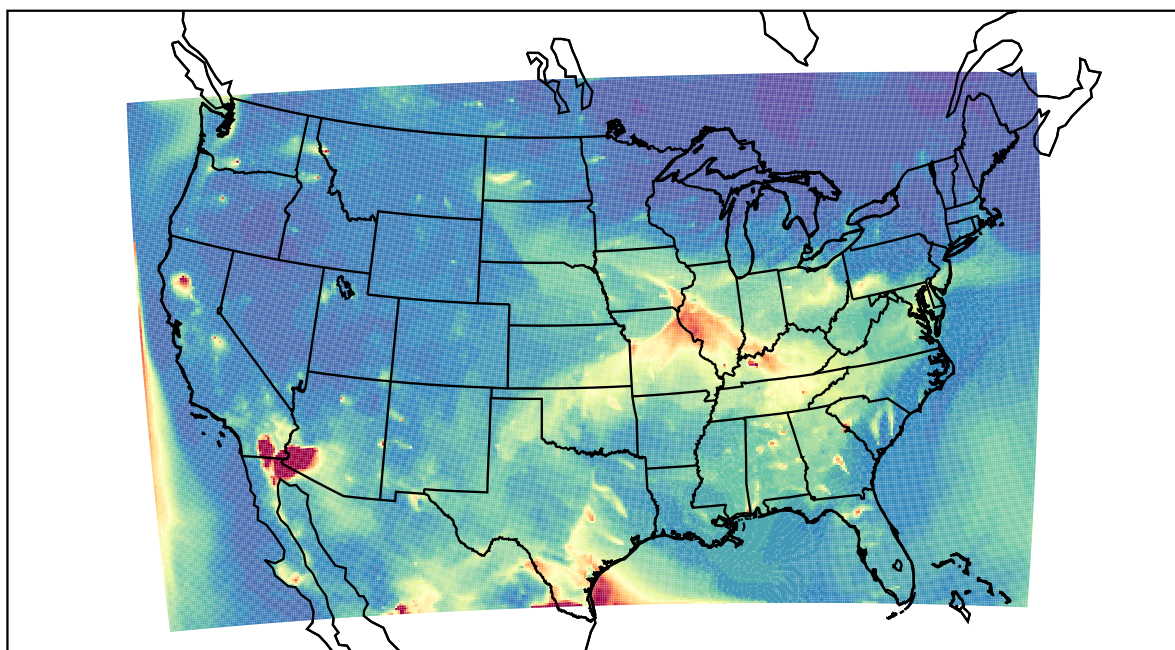
WRF 2023-05-14_04:00:00
