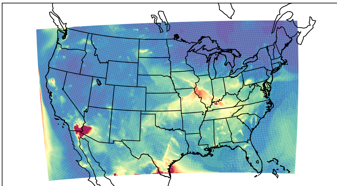
WRF 2023-05-14_05:00:00
