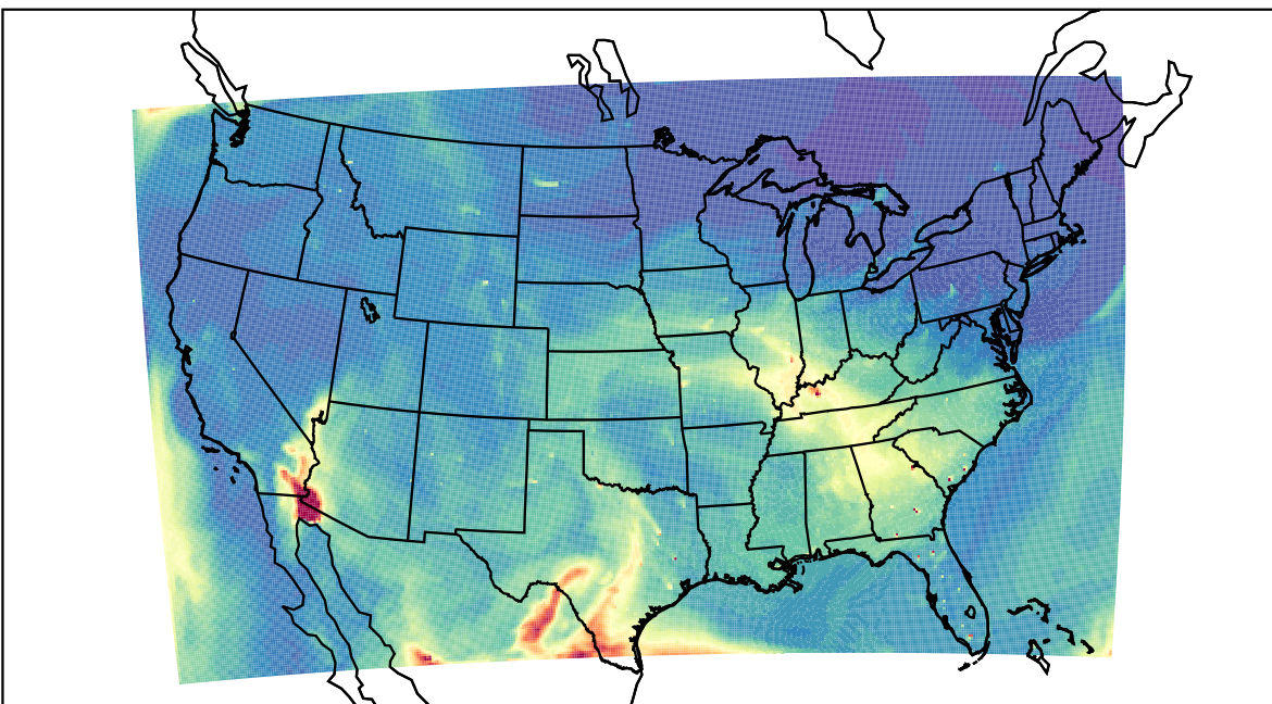
WRF 2023-05-14_19:00:00
