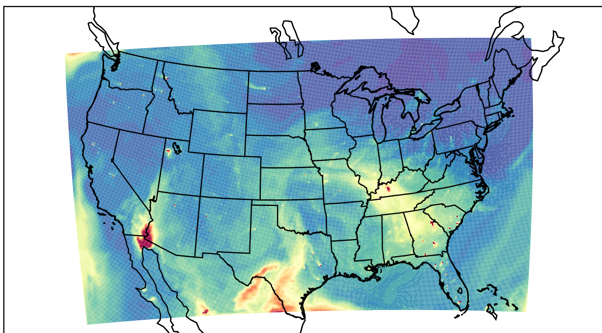
WRF 2023-05-14_23:00:00
