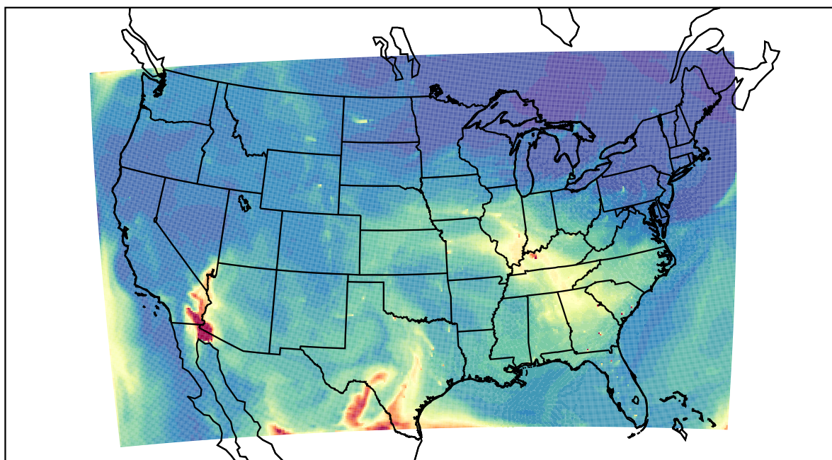
WRF 2023-05-14_18:00:00
