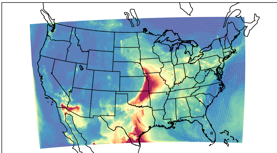
WRF 2023-05-13_08:00:00
