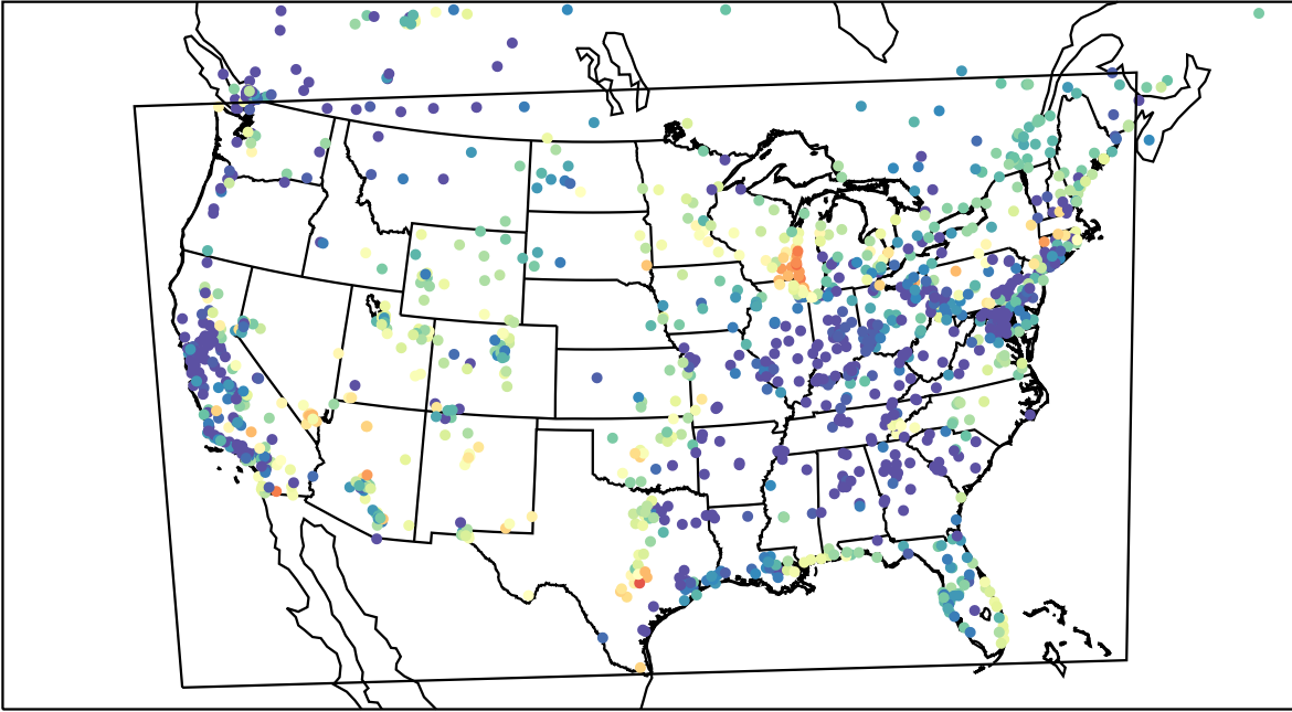
AirNOW (2023-05-13_08:00:00)
