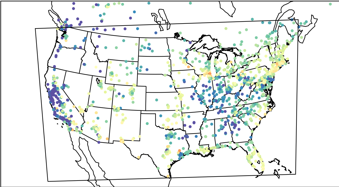
AirNOW (2023-05-13_14:00:00)
