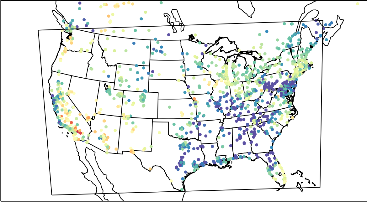
AirNOW (2023-05-14_03:00:00)
