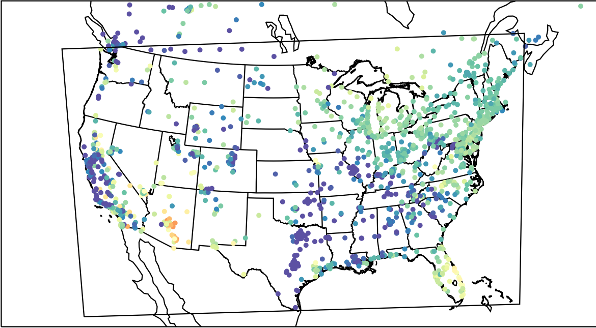
AirNOW (2023-05-14_13:00:00)
