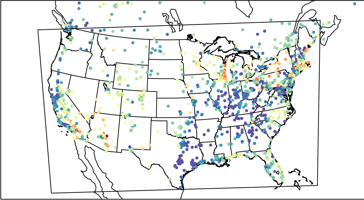
AirNOW (2023-05-13_04:00:00)
