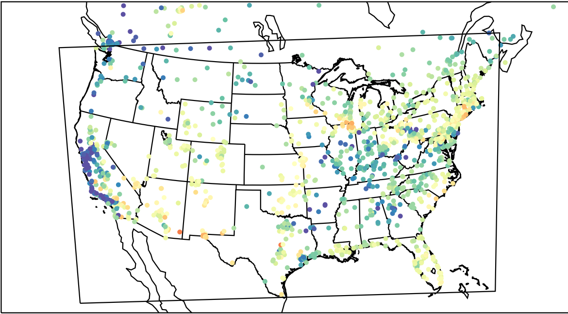
AirNOW (2023-05-13_15:00:00)
