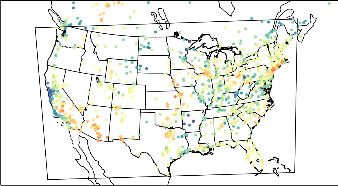
AirNOW (2023-05-13_17:00:00)
