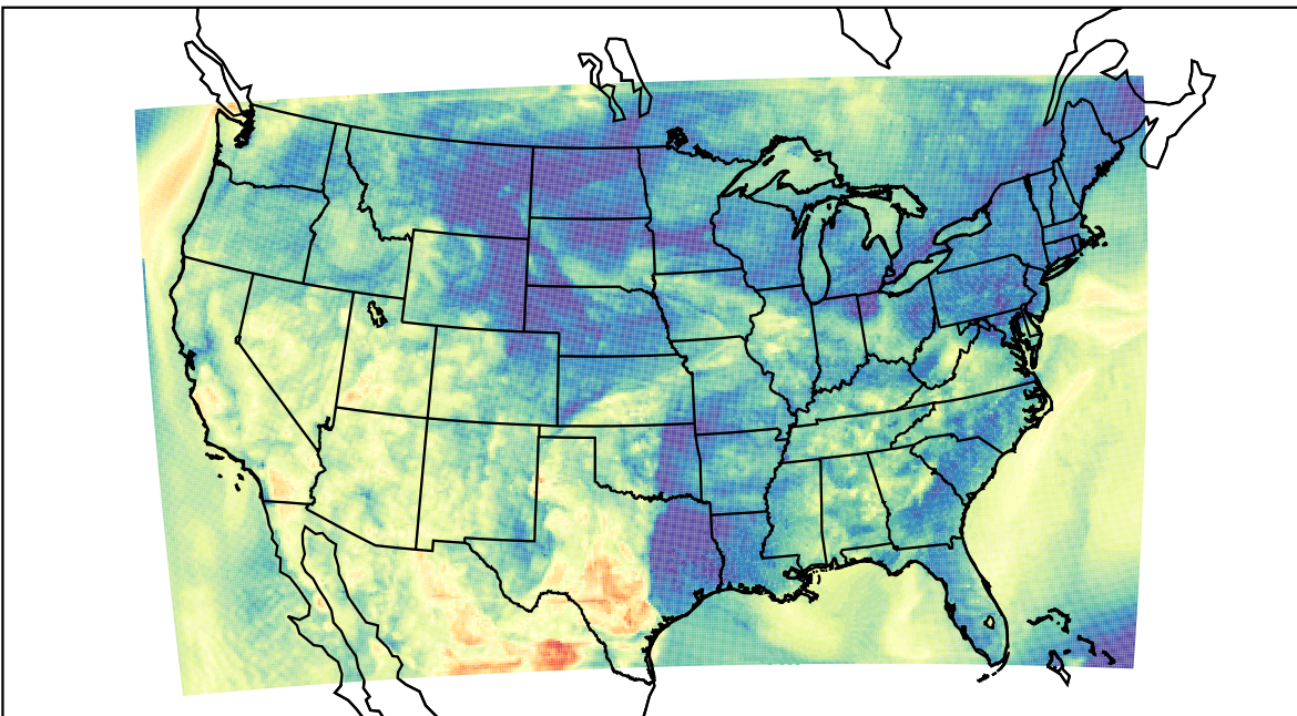
WRF (2023-05-14_08:00:00)
