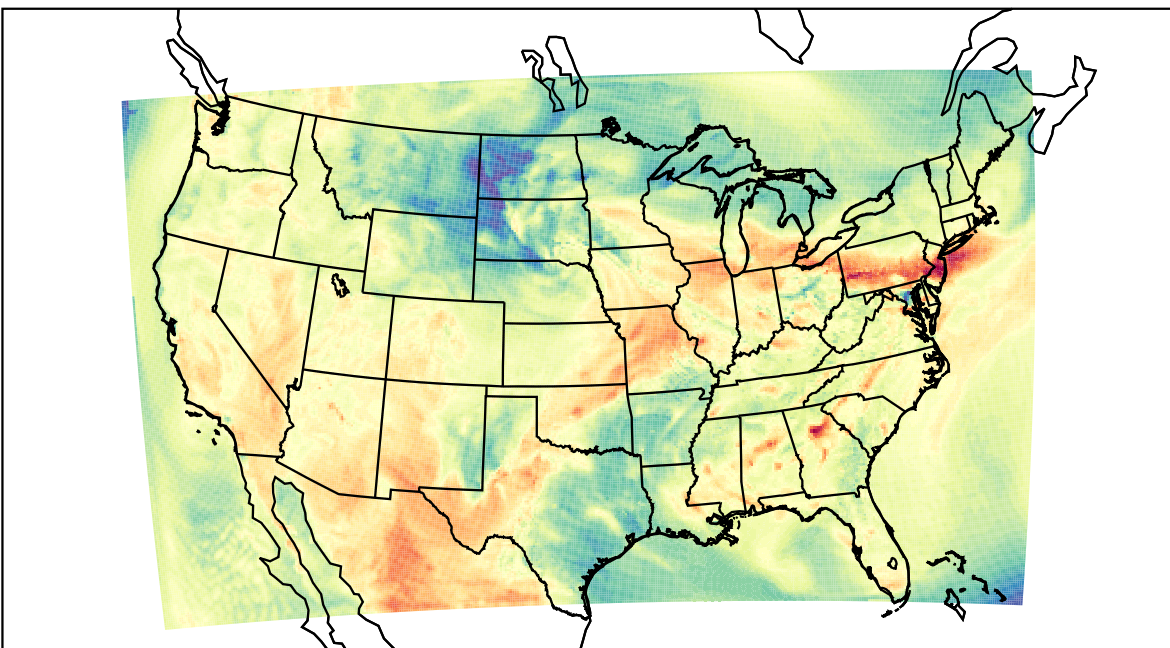
WRF (2023-05-13_19:00:00)
