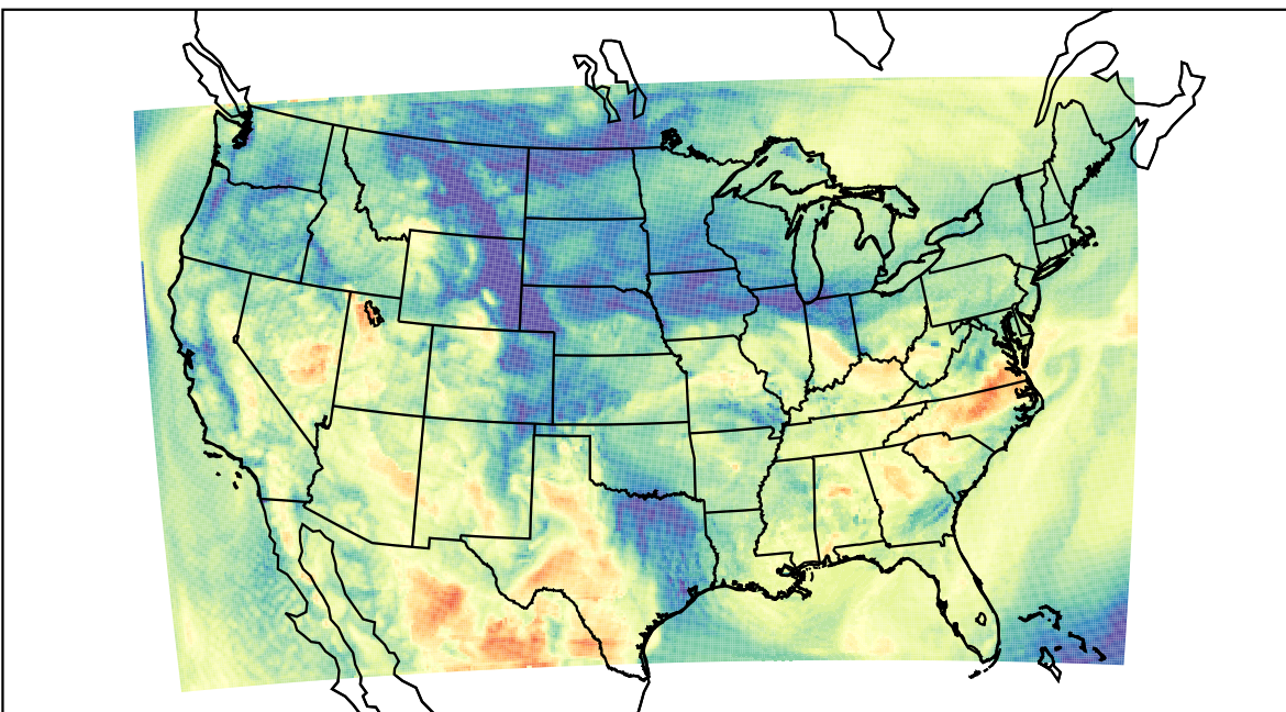
WRF (2023-05-14_15:00:00)
