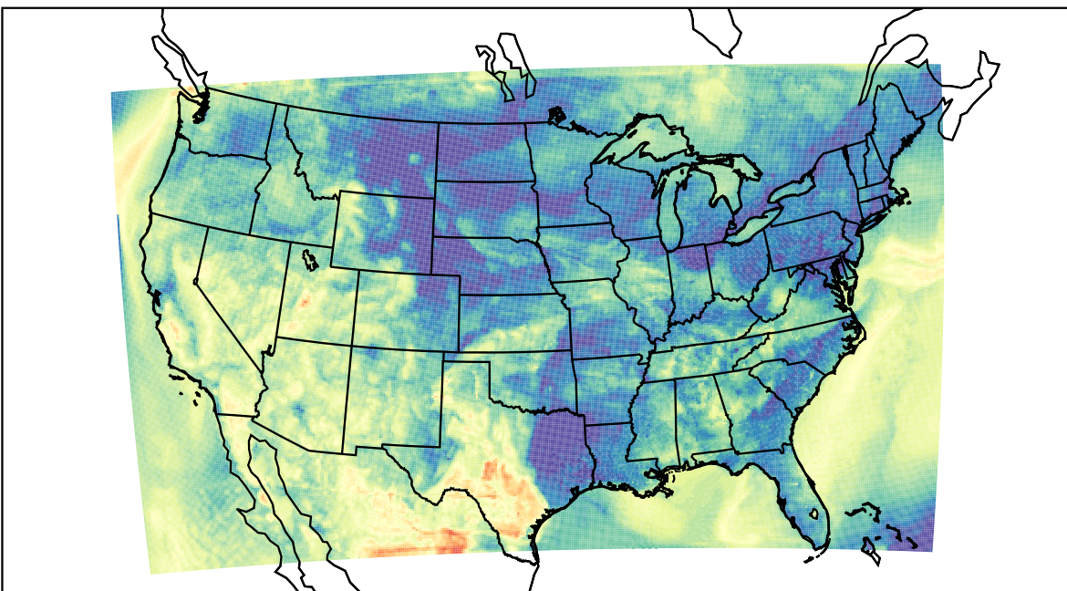
WRF (2023-05-14_10:00:00)
