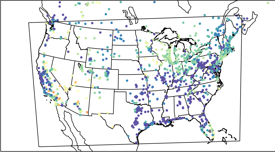
AirNOW (2023-05-14_08:00:00)
