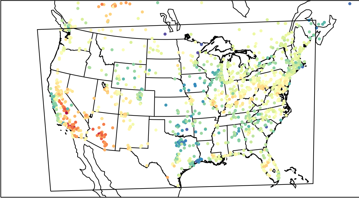
AirNOW (2023-05-14_20:00:00)
