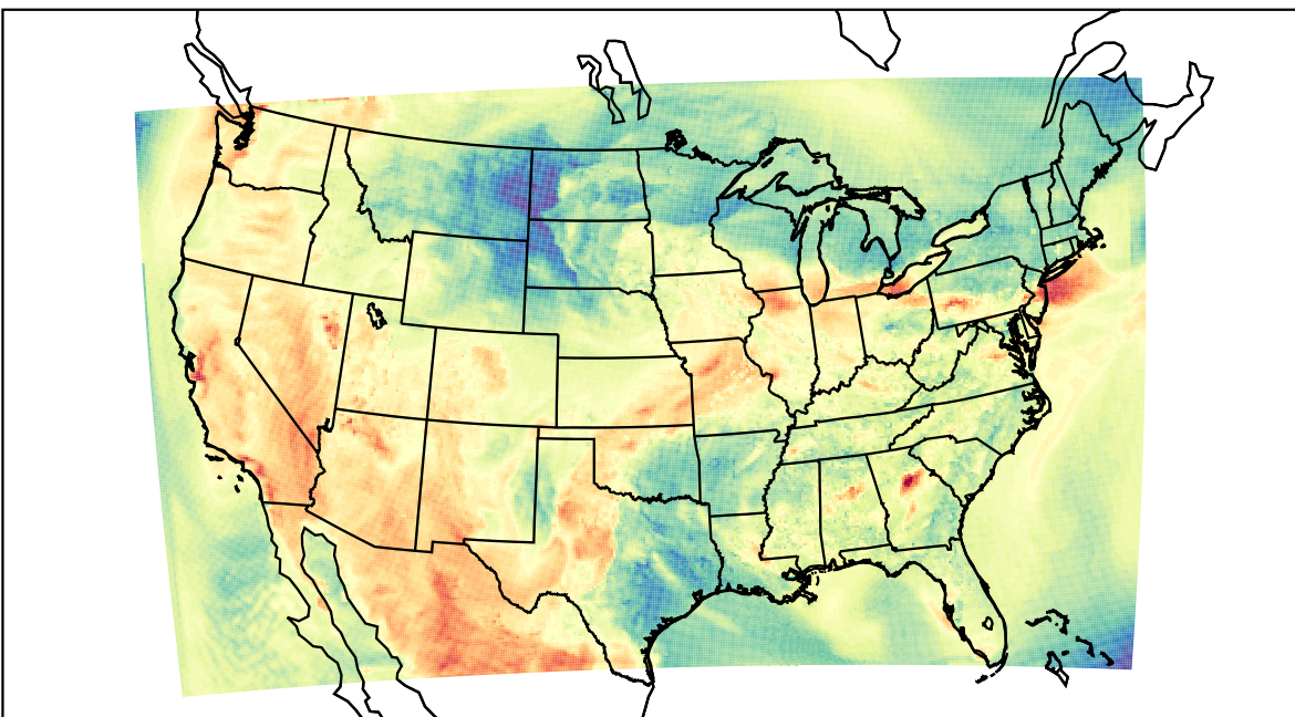
WRF (2023-05-13_23:00:00)
