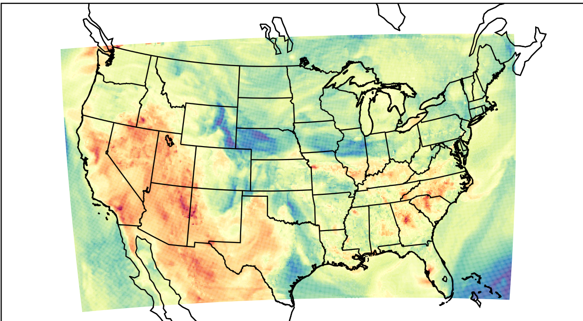
WRF (2023-05-14_23:00:00)
