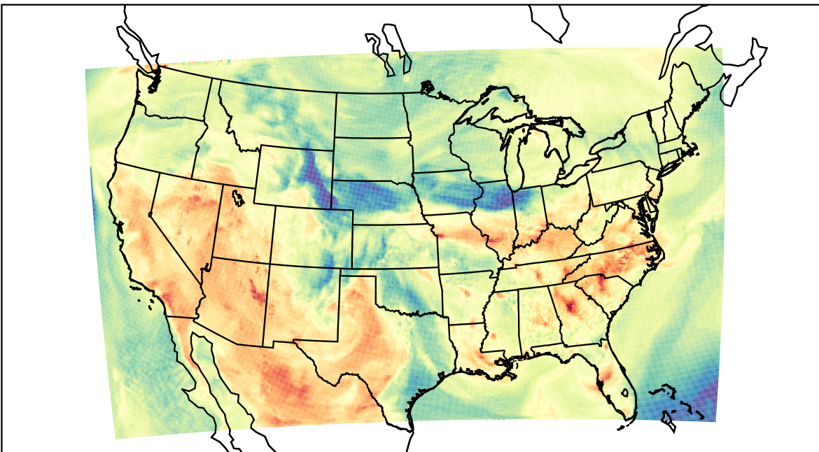
WRF (2023-05-14_20:00:00)
