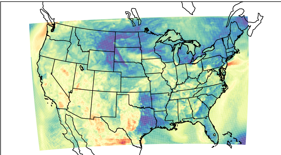
WRF (2023-05-14_04:00:00)
