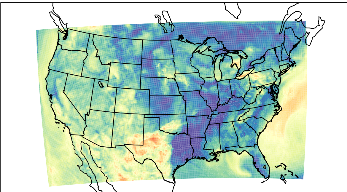
WRF (2023-05-13_10:00:00)
