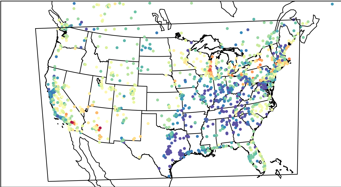
AirNOW (2023-05-13_03:00:00)
