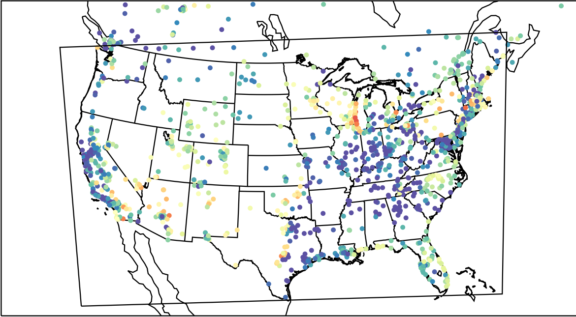
AirNOW (2023-05-13_06:00:00)
