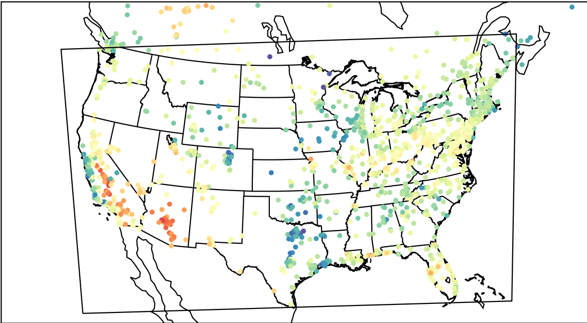
AirNOW (2023-05-14_18:00:00)
