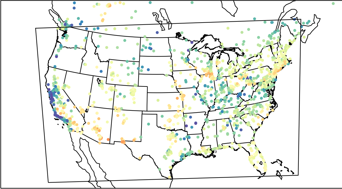
AirNOW (2023-05-13_16:00:00)
