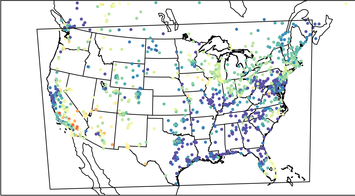
AirNOW (2023-05-14_05:00:00)
