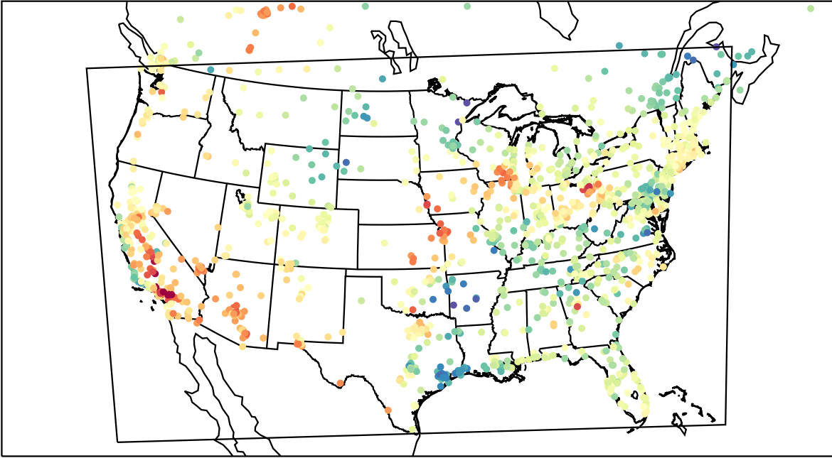
AirNOW (2023-05-13_22:00:00)
