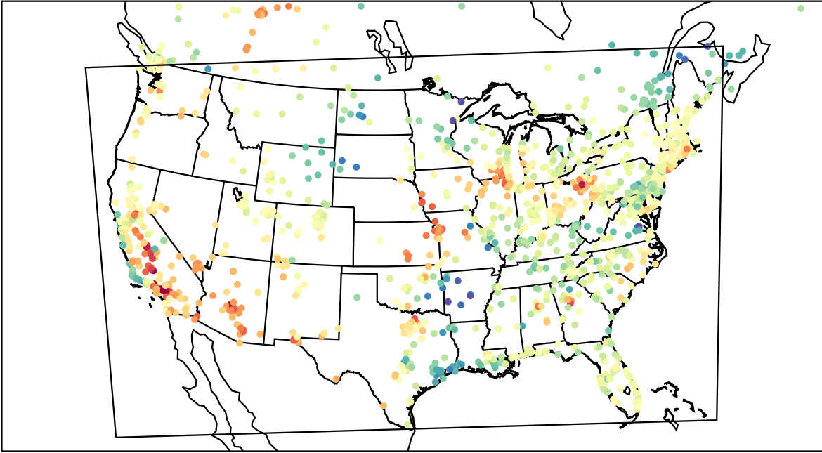
AirNOW (2023-05-13_21:00:00)
