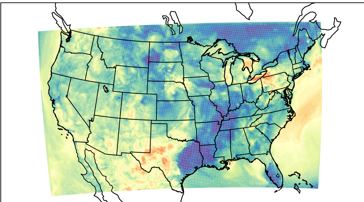
WRF (2023-05-13_06:00:00)
