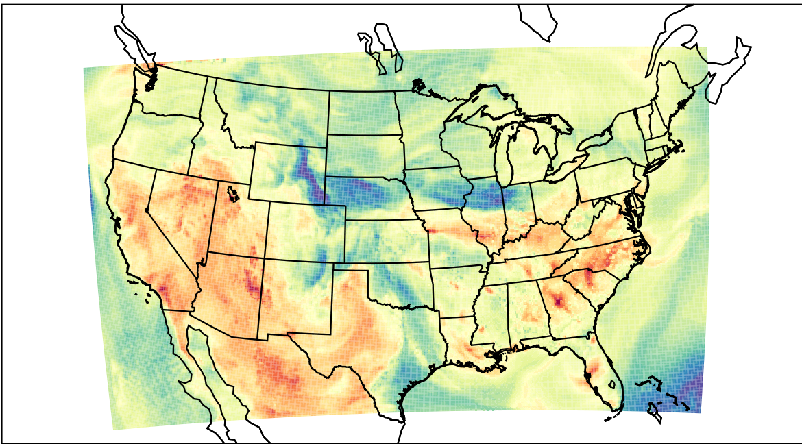
WRF (2023-05-14_21:00:00)
