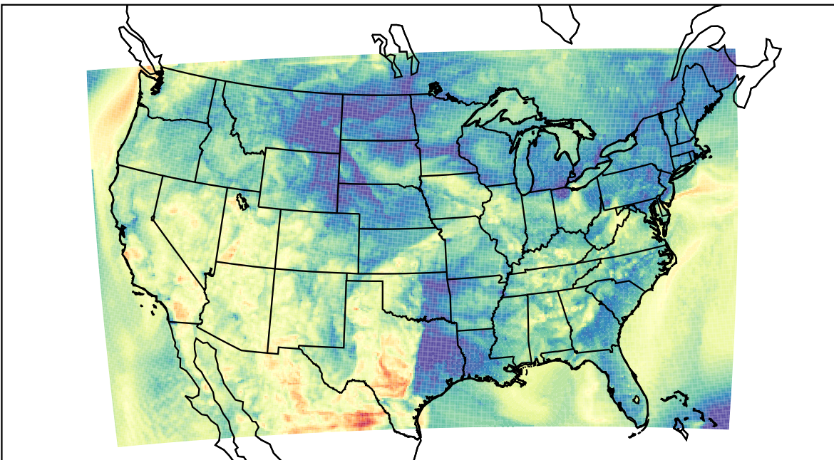
WRF (2023-05-14_06:00:00)
