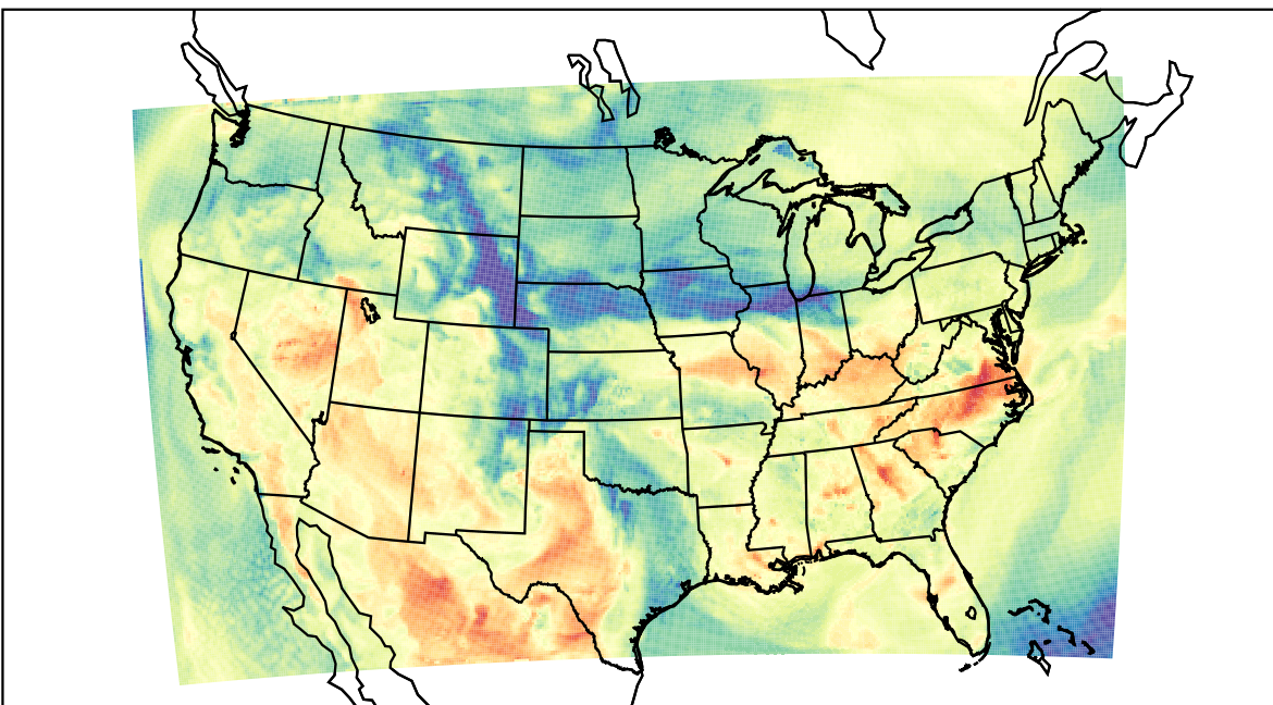
WRF (2023-05-14_17:00:00)
