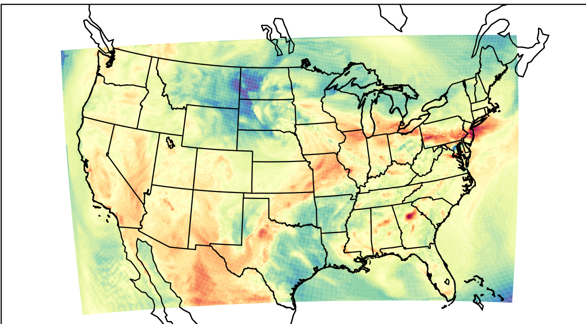
WRF (2023-05-13_20:00:00)
