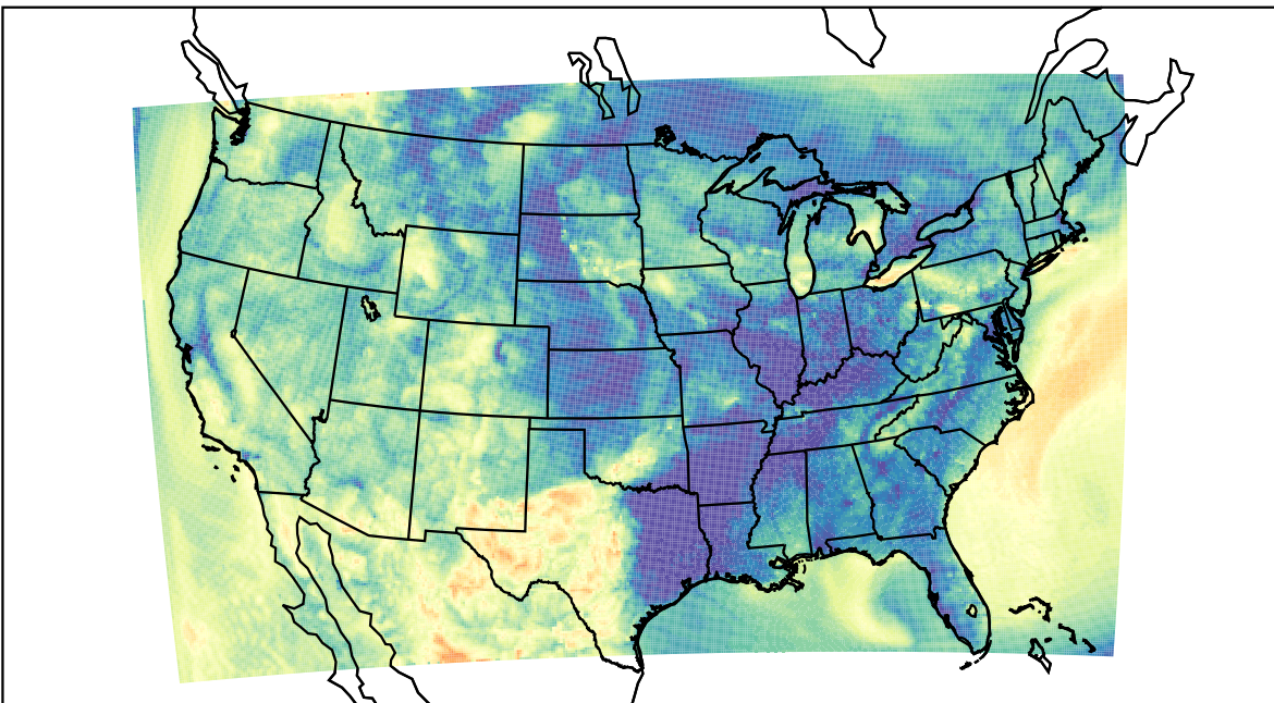
WRF (2023-05-13_12:00:00)
