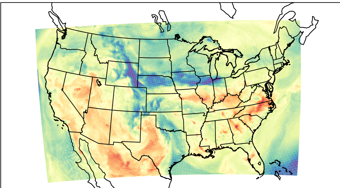
WRF (2023-05-14_18:00:00)
