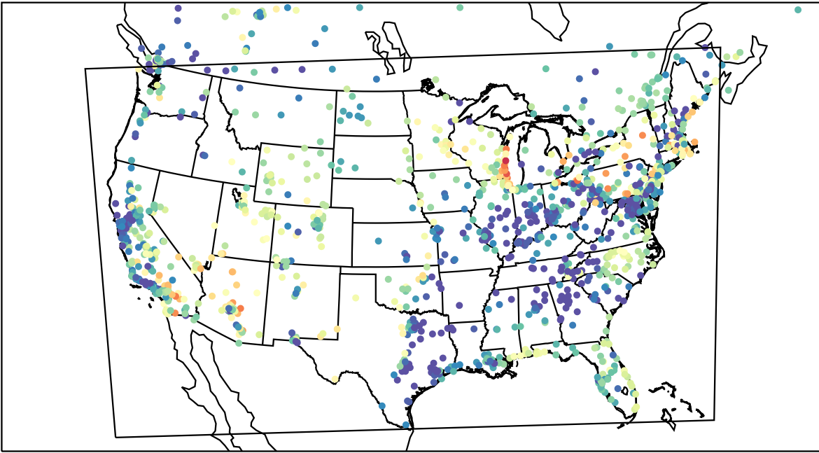
AirNOW (2023-05-13_05:00:00)
