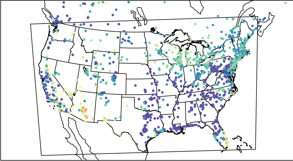
AirNOW (2023-05-14_11:00:00)
