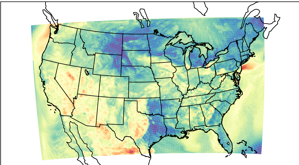
WRF (2023-05-14_03:00:00)
