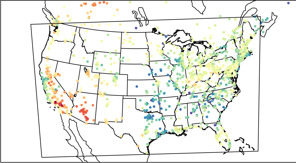
AirNOW (2023-05-14_23:00:00)
