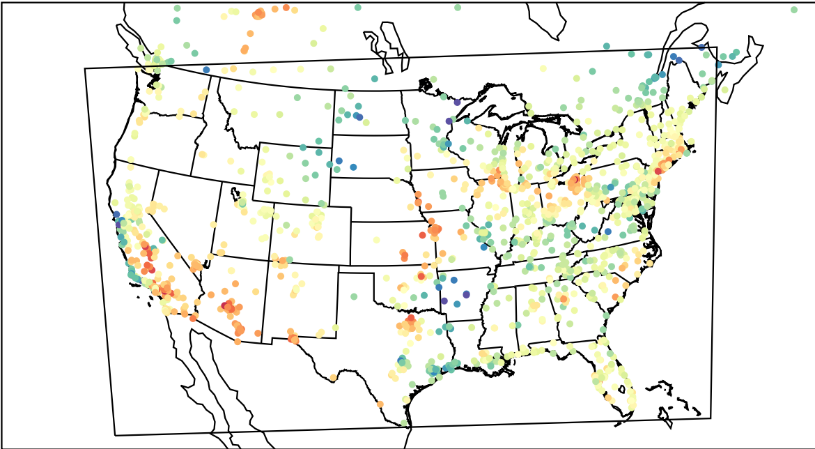
AirNOW (2023-05-13_19:00:00)
