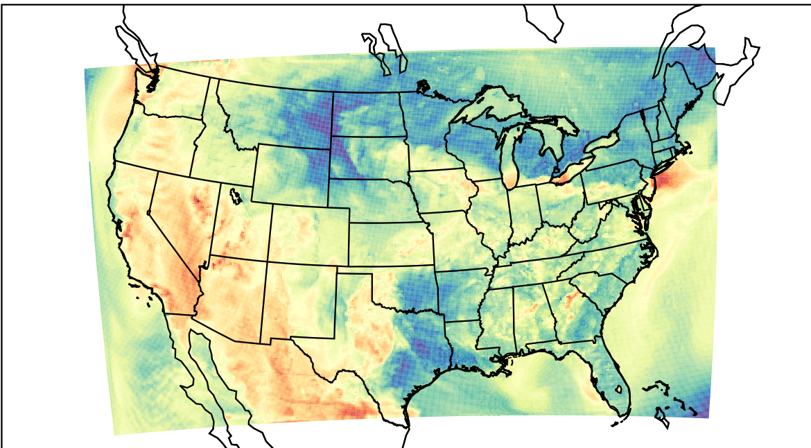
WRF (2023-05-14_01:00:00)
