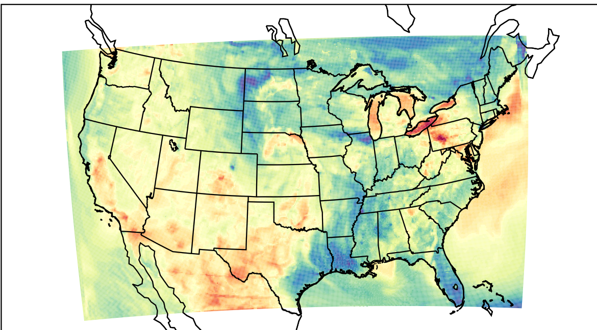
WRF (2023-05-13_01:00:00)
