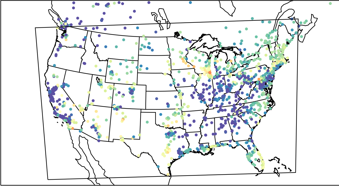
AirNOW (2023-05-13_12:00:00)
