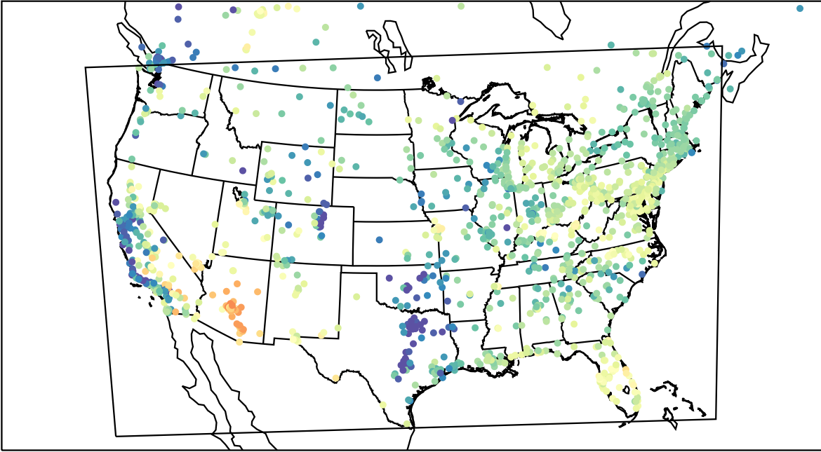
AirNOW (2023-05-14_15:00:00)
