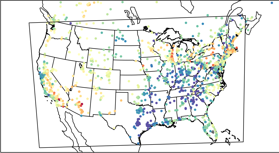
AirNOW (2023-05-13_02:00:00)
