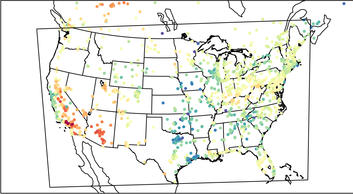
AirNOW (2023-05-14_22:00:00)
