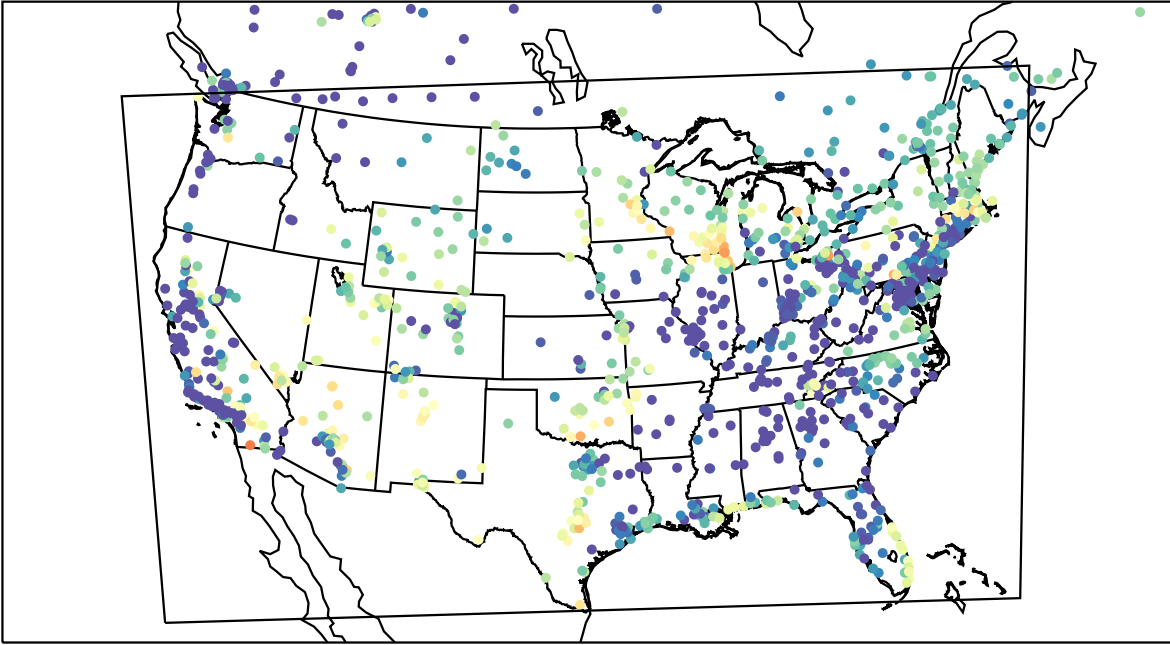
AirNOW (2023-05-13_11:00:00)
