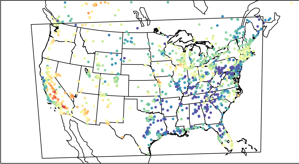
AirNOW (2023-05-14_02:00:00)
