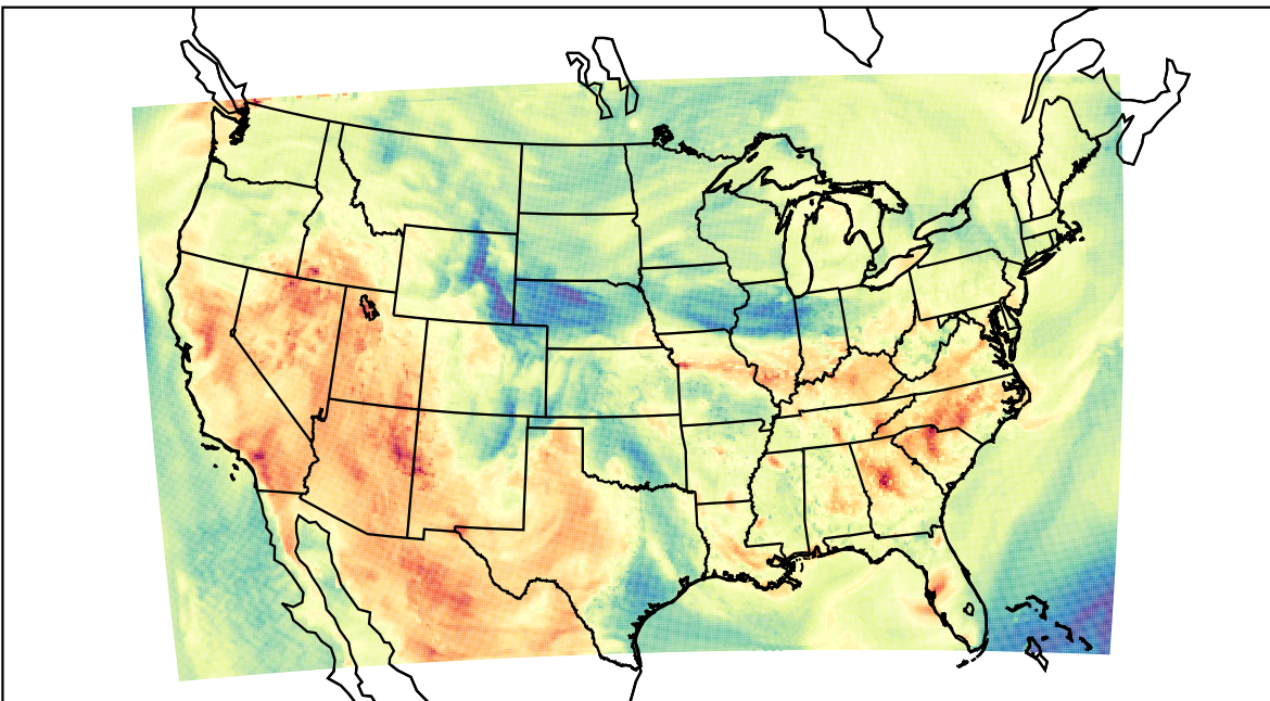
WRF (2023-05-14_22:00:00)
