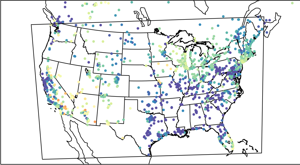
AirNOW (2023-05-14_07:00:00)
