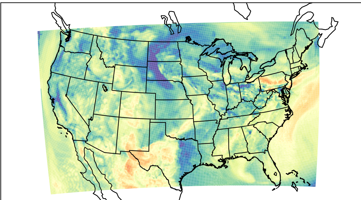
WRF (2023-05-13_15:00:00)
