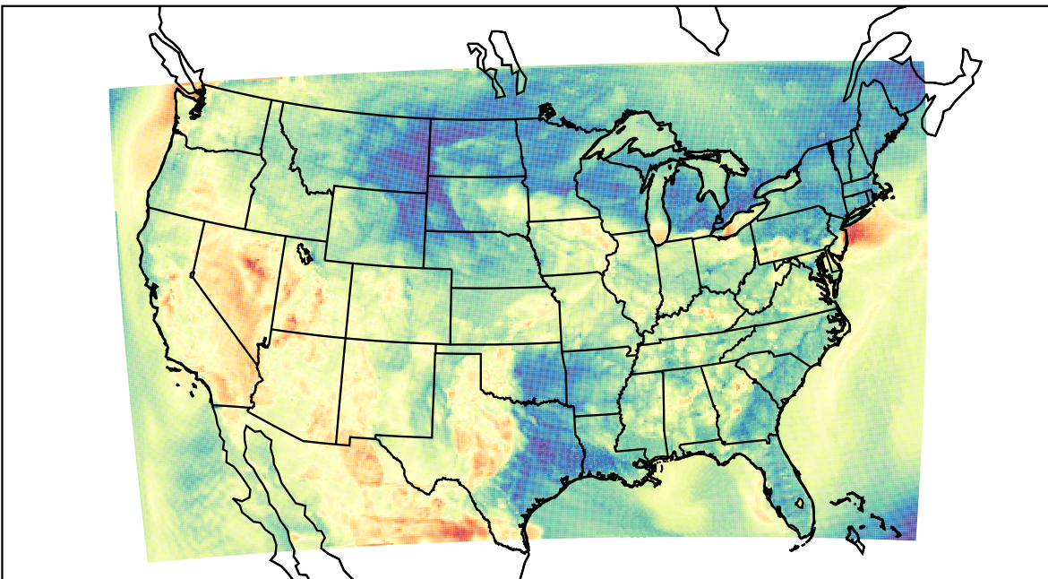
WRF (2023-05-14_02:00:00)
