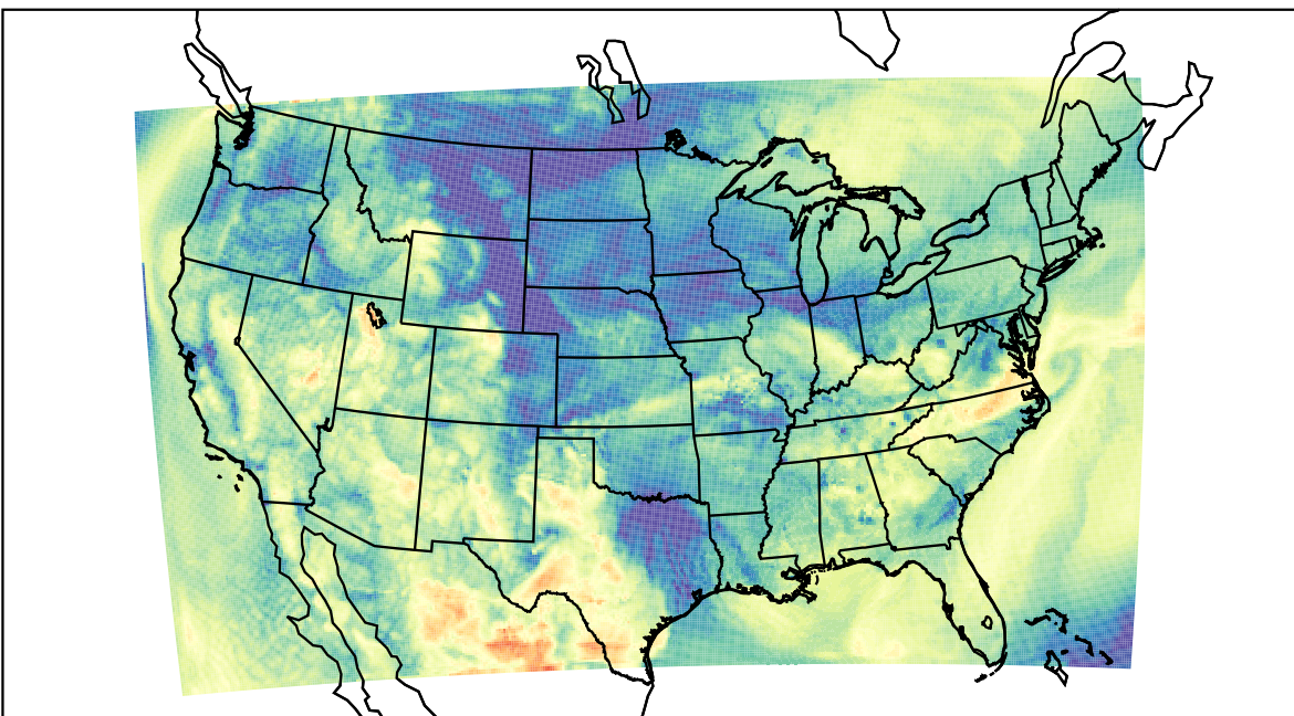
WRF (2023-05-14_14:00:00)
