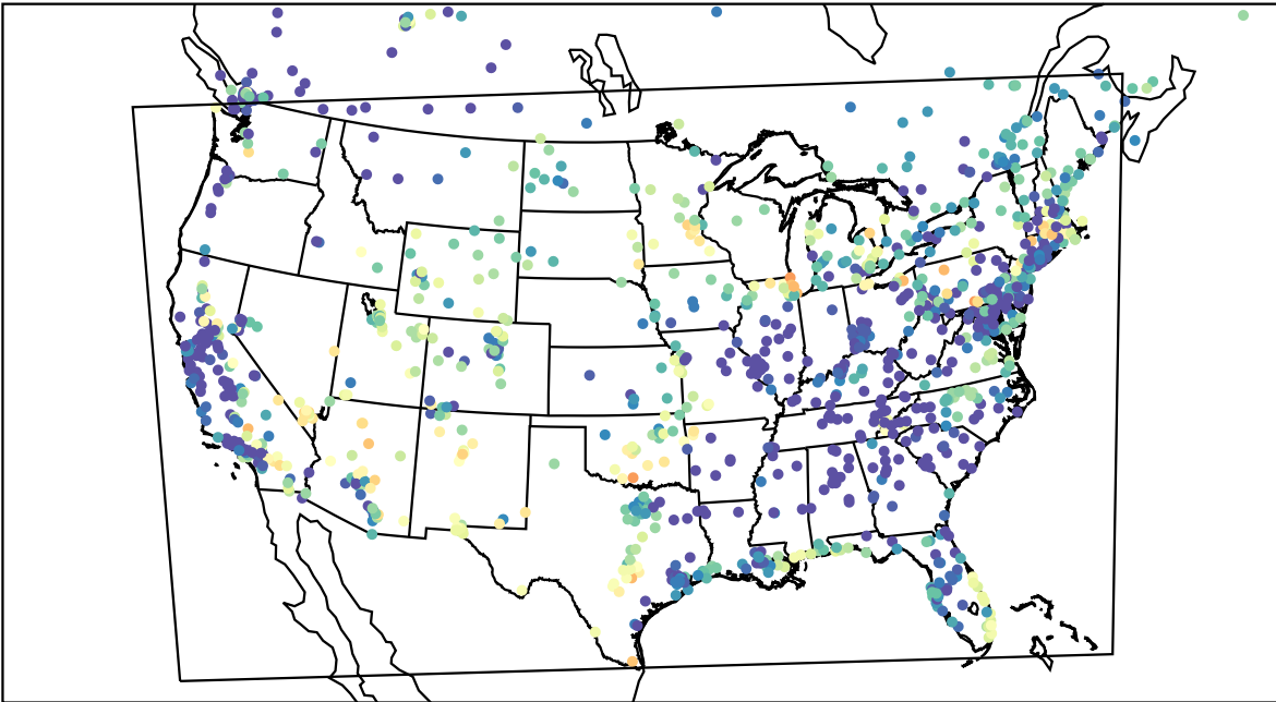
AirNOW (2023-05-13_10:00:00)
