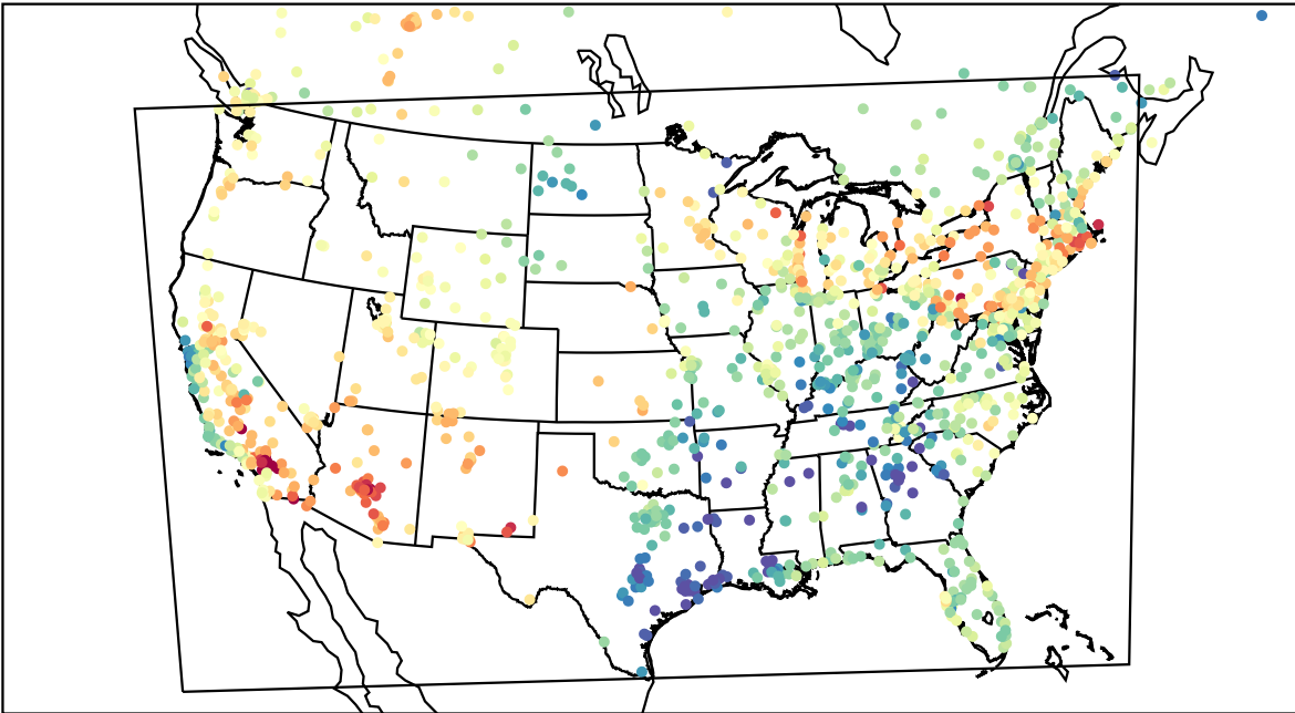
AirNOW (2023-05-13_00:00:00)
