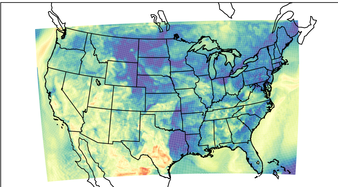
WRF (2023-05-14_09:00:00)
