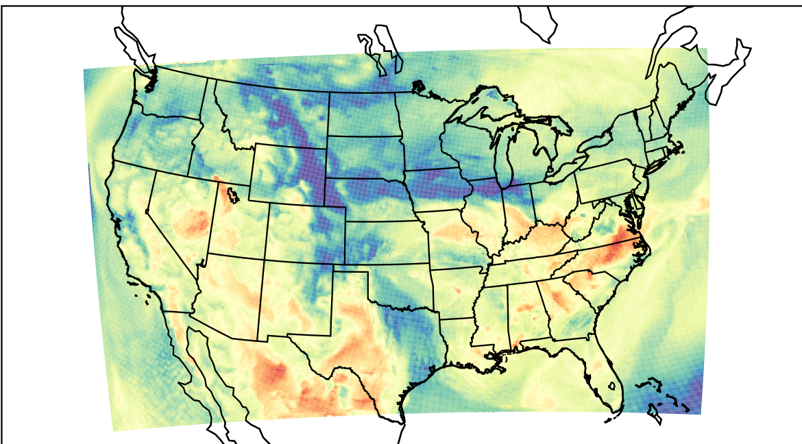
WRF (2023-05-14_16:00:00)
