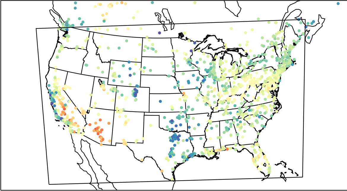
AirNOW (2023-05-14_17:00:00)
