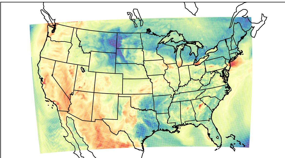
WRF (2023-05-14_00:00:00)
