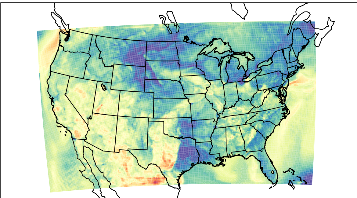
WRF (2023-05-14_05:00:00)
