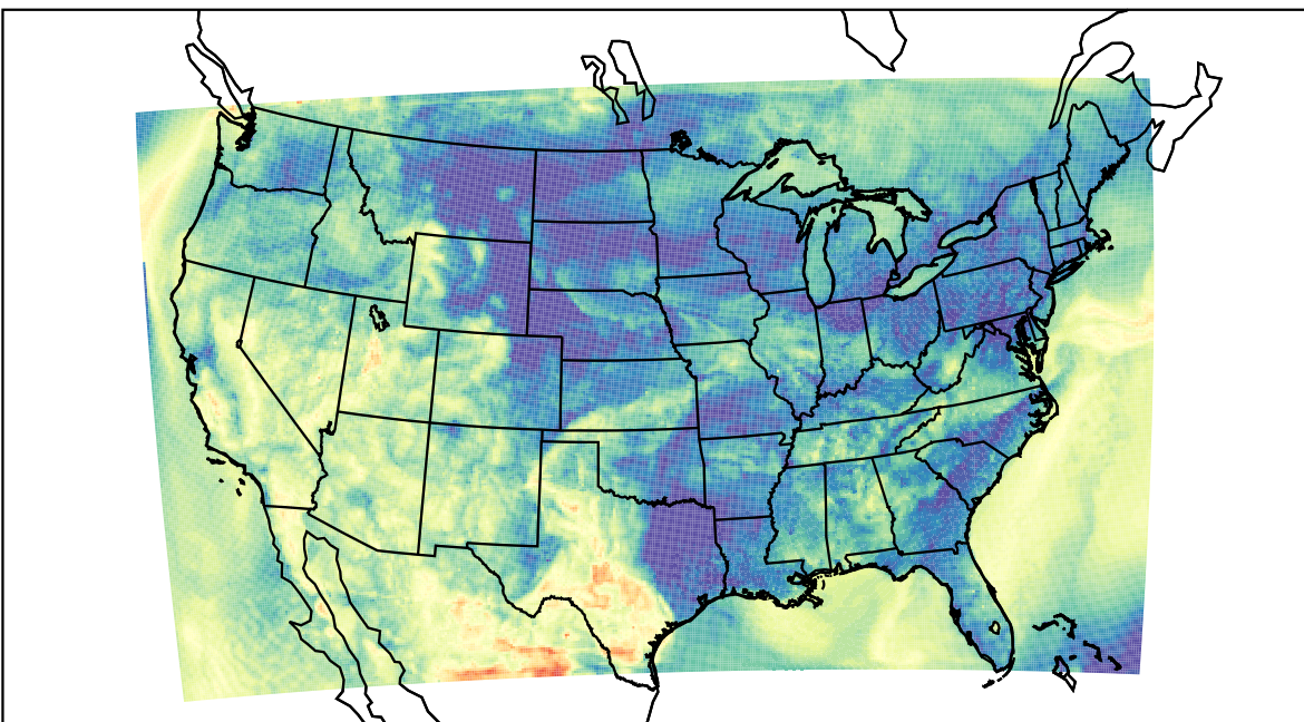
WRF (2023-05-14_11:00:00)
