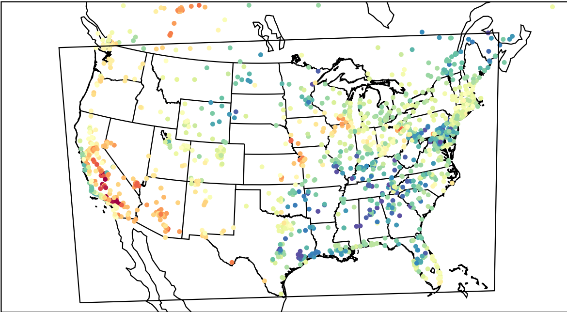
AirNOW (2023-05-14_00:00:00)
