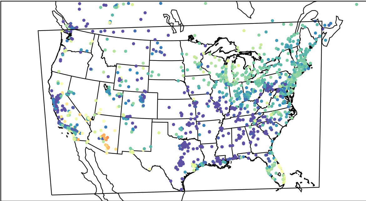
AirNOW (2023-05-14_12:00:00)
