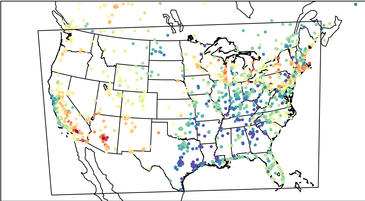
AirNOW (2023-05-13_01:00:00)
