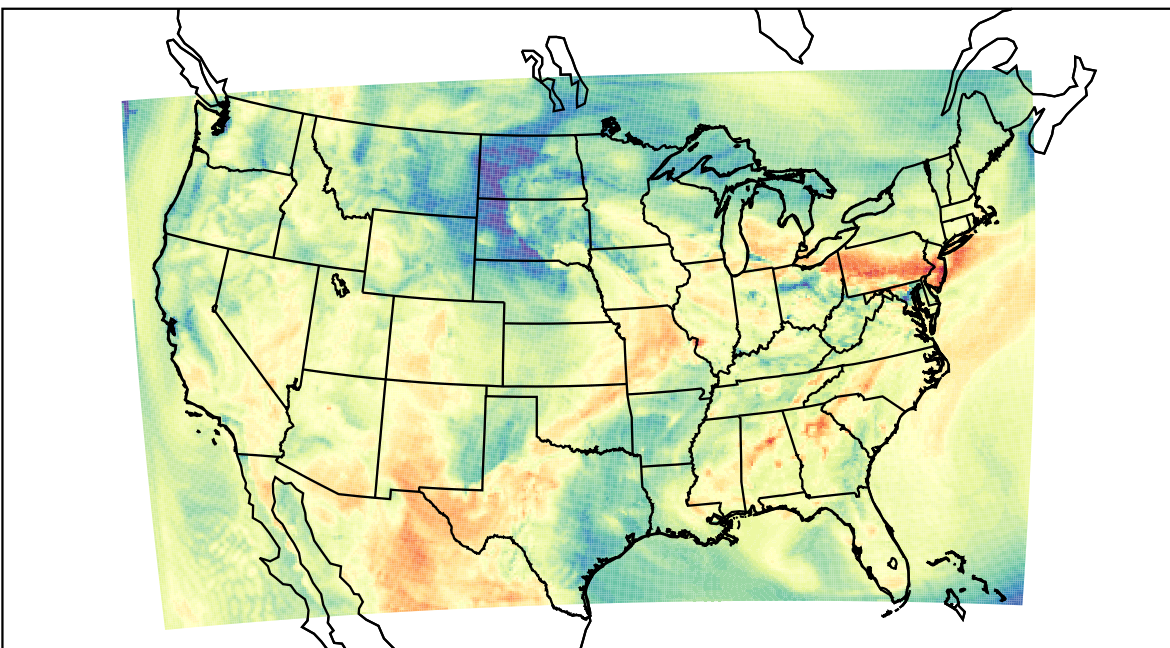
WRF (2023-05-13_17:00:00)
