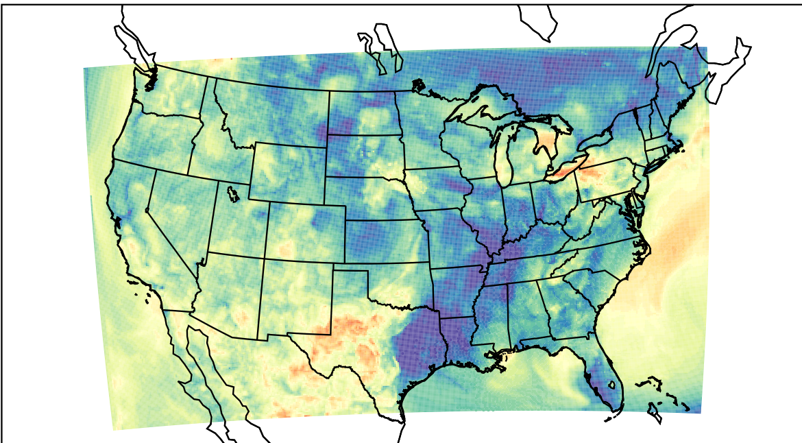
WRF (2023-05-13_07:00:00)
