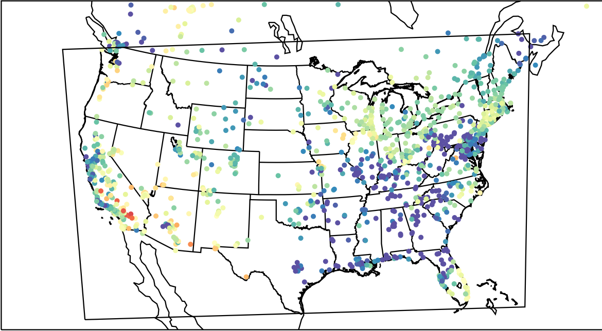
AirNOW (2023-05-14_04:00:00)
