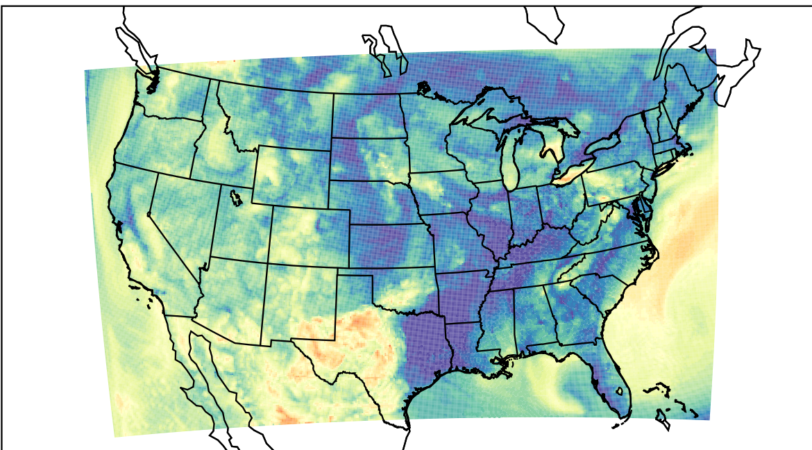
WRF (2023-05-13_11:00:00)
