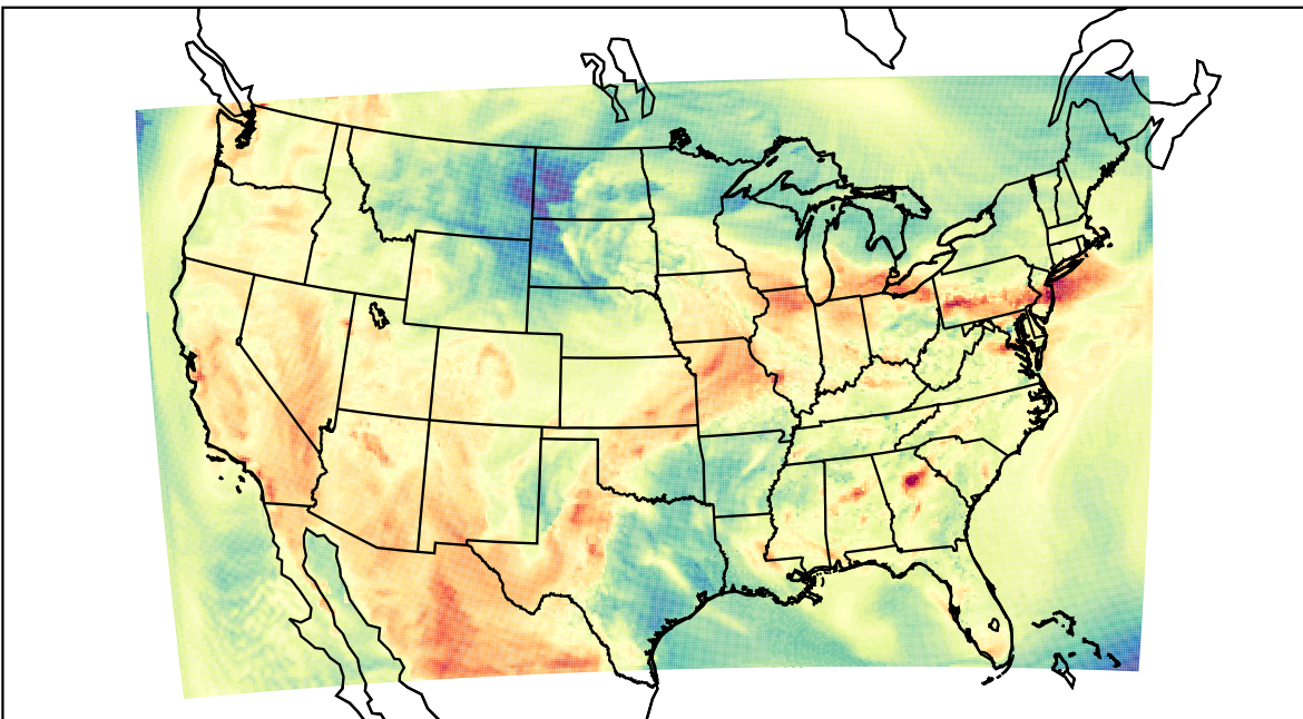
WRF (2023-05-13_21:00:00)
