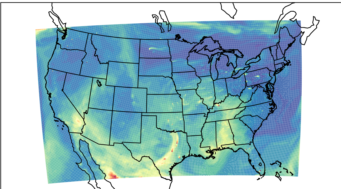
WRF 2023-05-15_21:00:00
