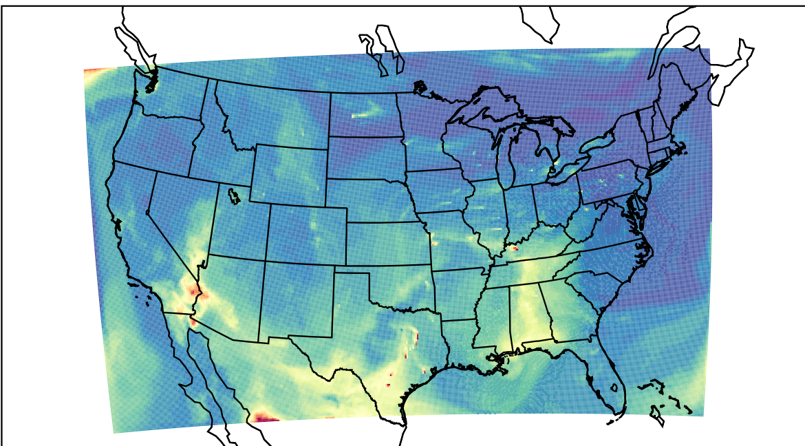
WRF 2023-05-15_16:00:00
