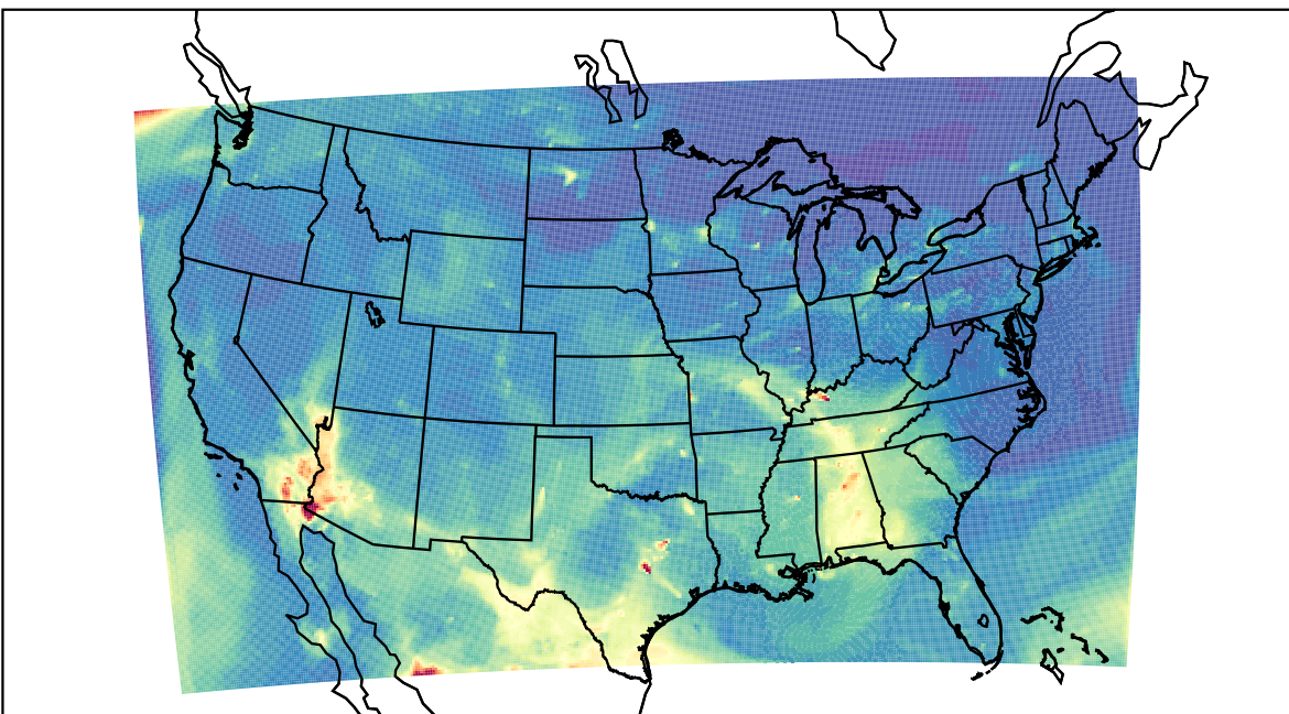
WRF 2023-05-15_10:00:00
