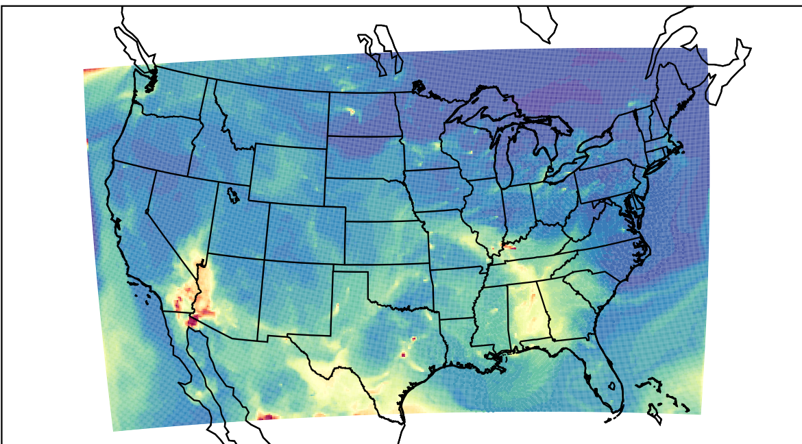
WRF 2023-05-15_08:00:00
