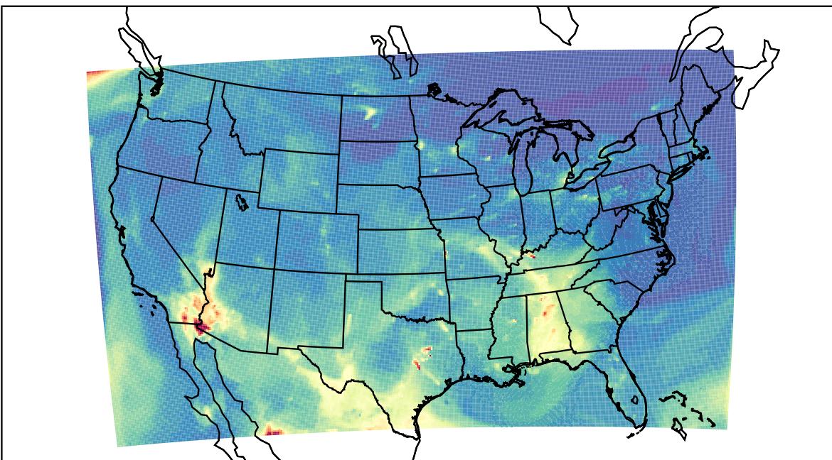
WRF 2023-05-15_11:00:00
