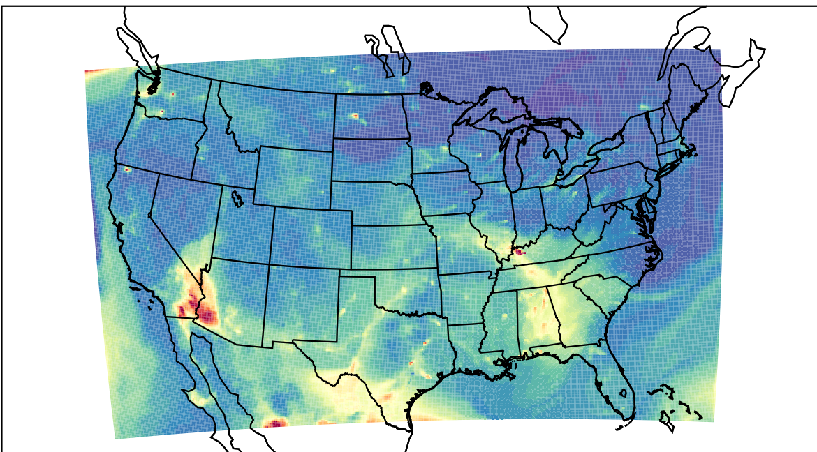
WRF 2023-05-15_05:00:00
