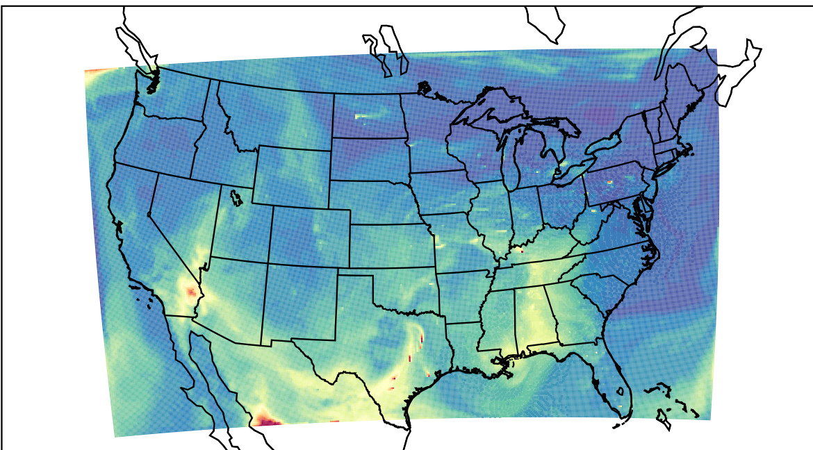
WRF 2023-05-15_18:00:00
