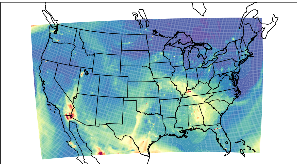
WRF 2023-05-15_01:00:00
