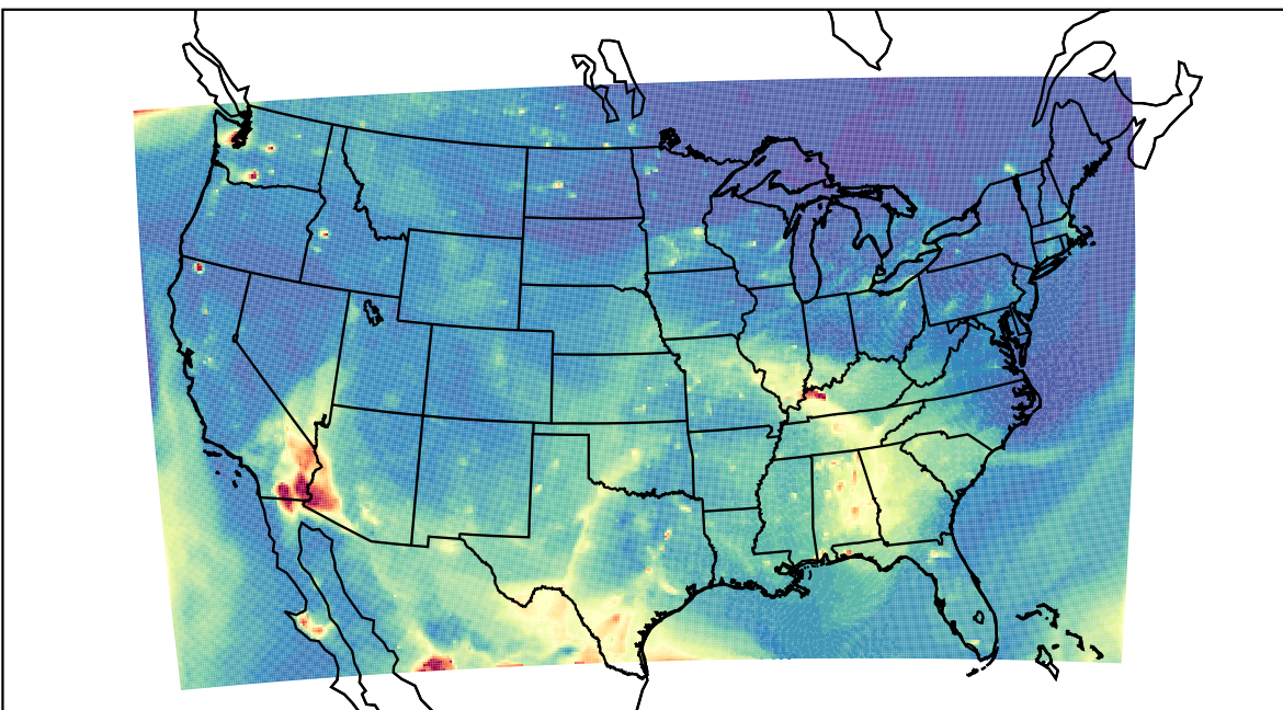
WRF 2023-05-15_03:00:00
