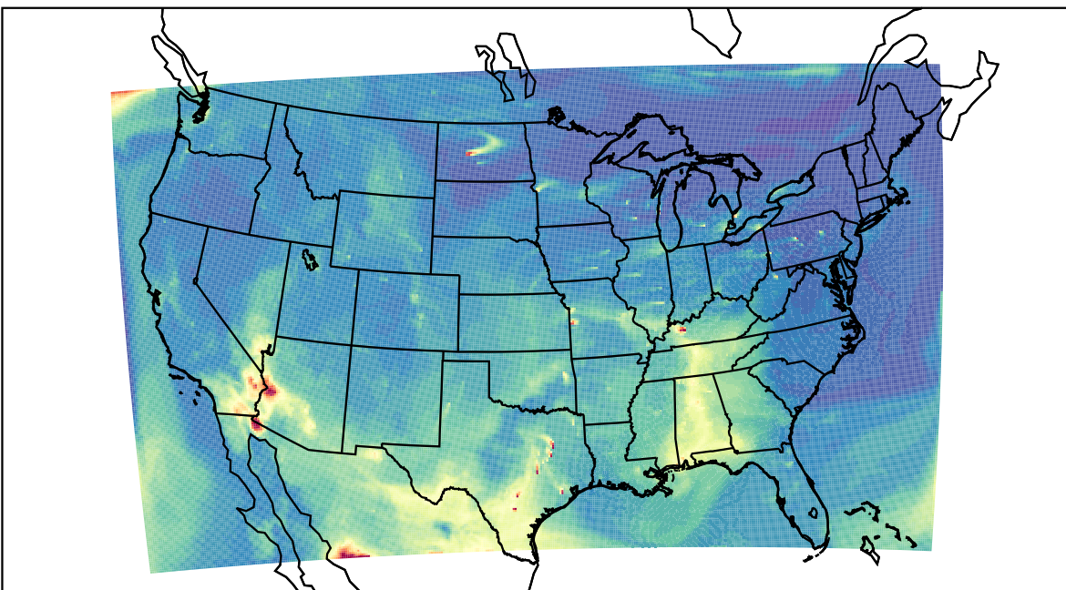
WRF 2023-05-15_15:00:00
