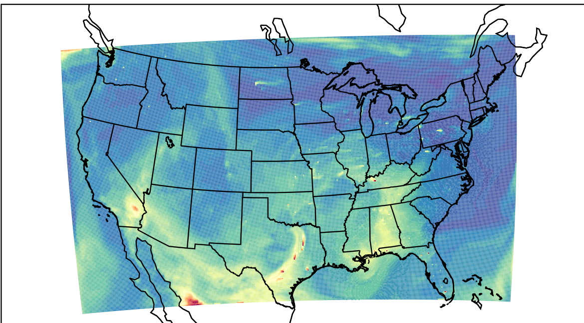
WRF 2023-05-15_20:00:00
