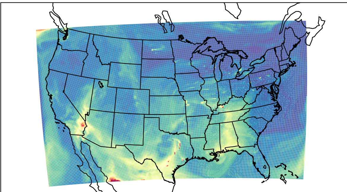
WRF 2023-05-15_17:00:00
