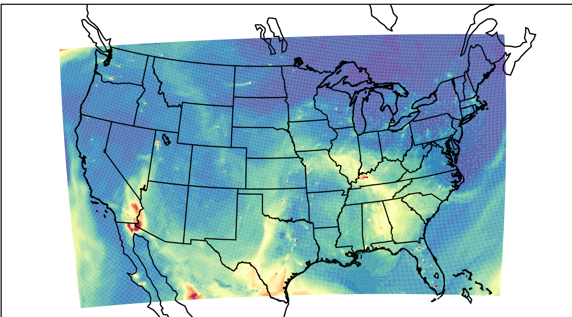
WRF 2023-05-15_00:00:00
