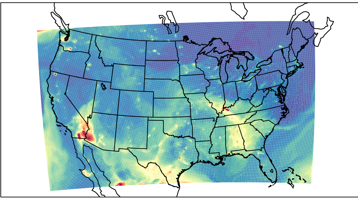
WRF 2023-05-15_04:00:00
