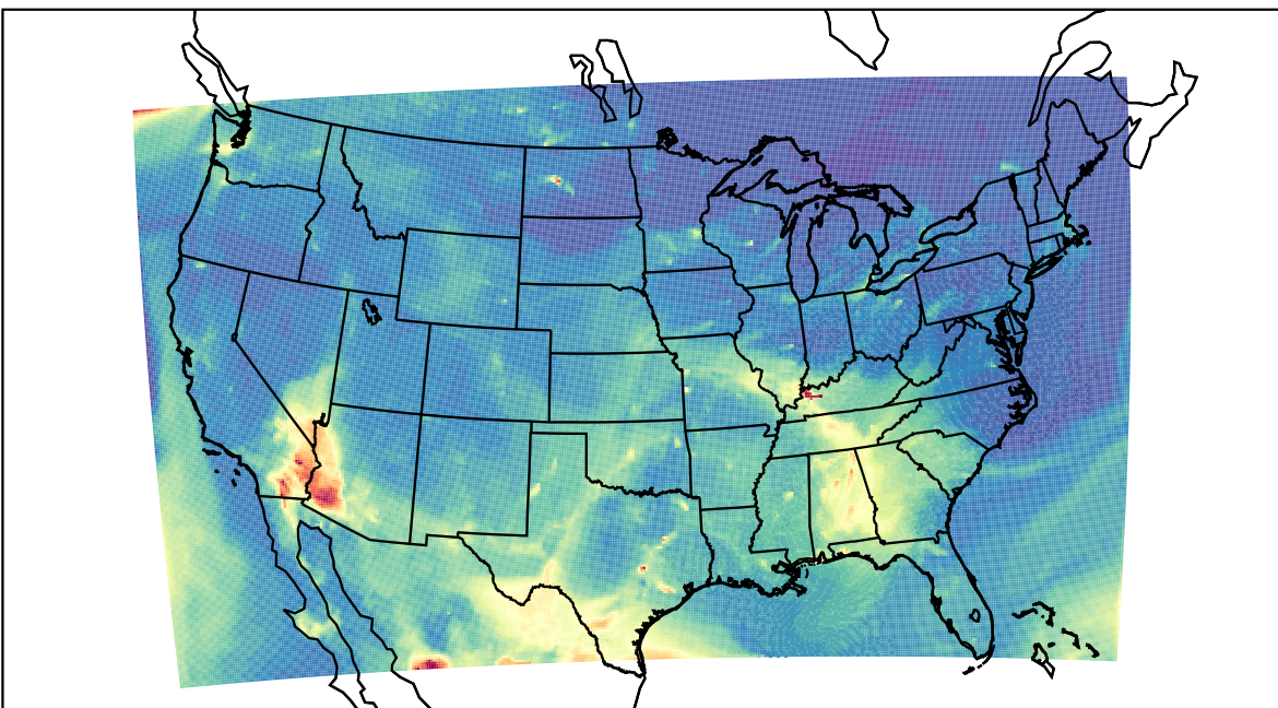
WRF 2023-05-15_06:00:00
