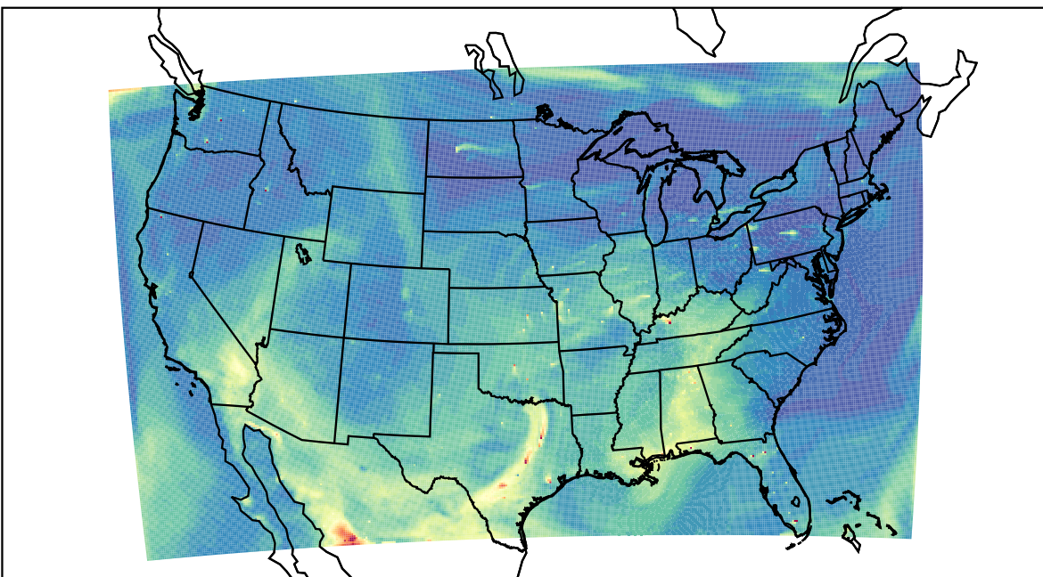
WRF 2023-05-15_22:00:00
