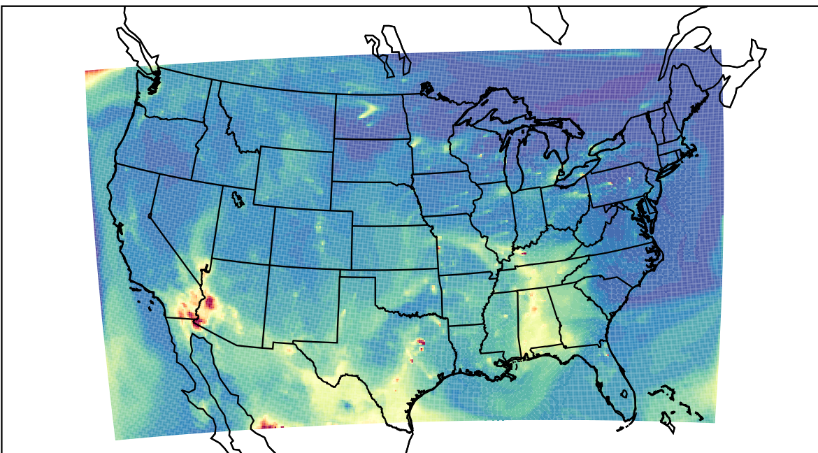
WRF 2023-05-15_13:00:00
