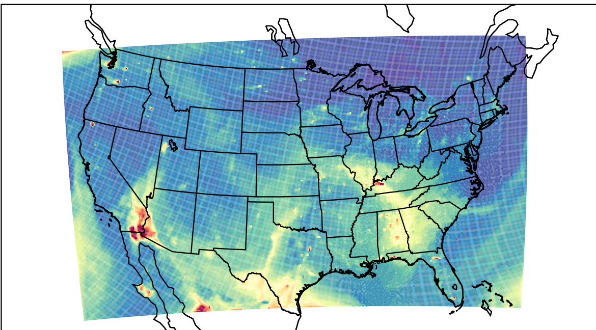
WRF 2023-05-15_02:00:00
