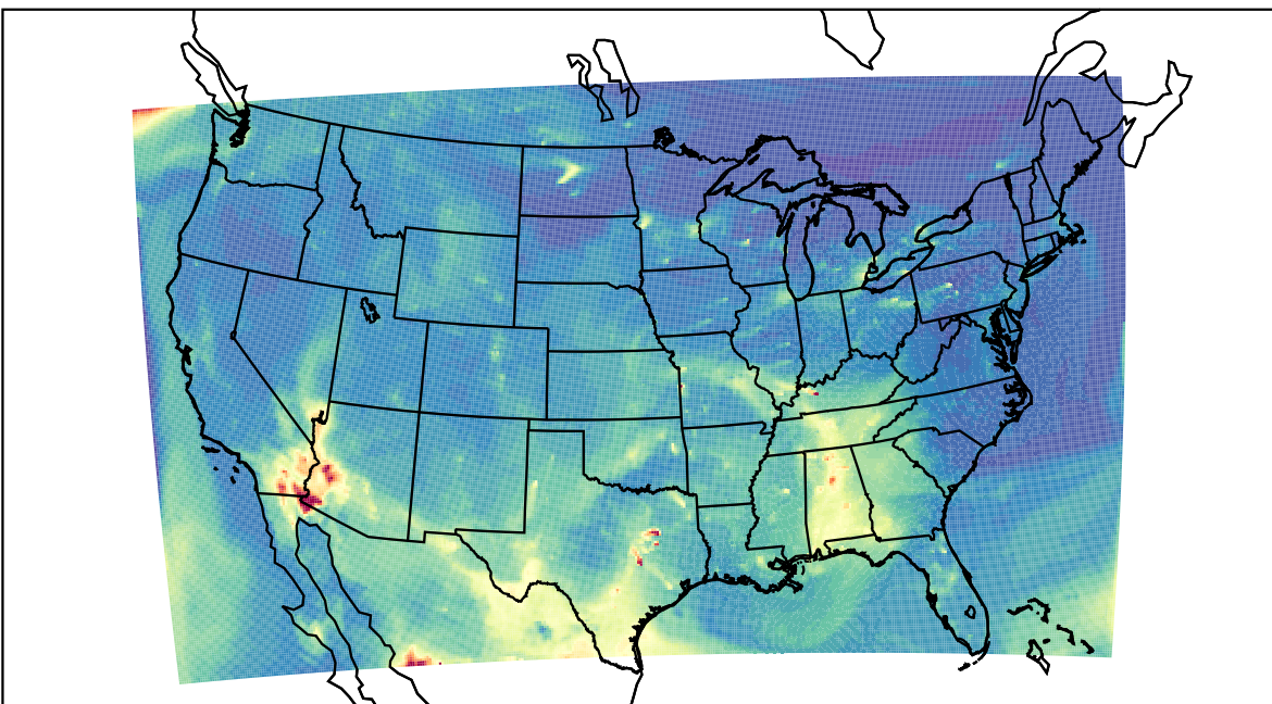
WRF 2023-05-15_12:00:00
