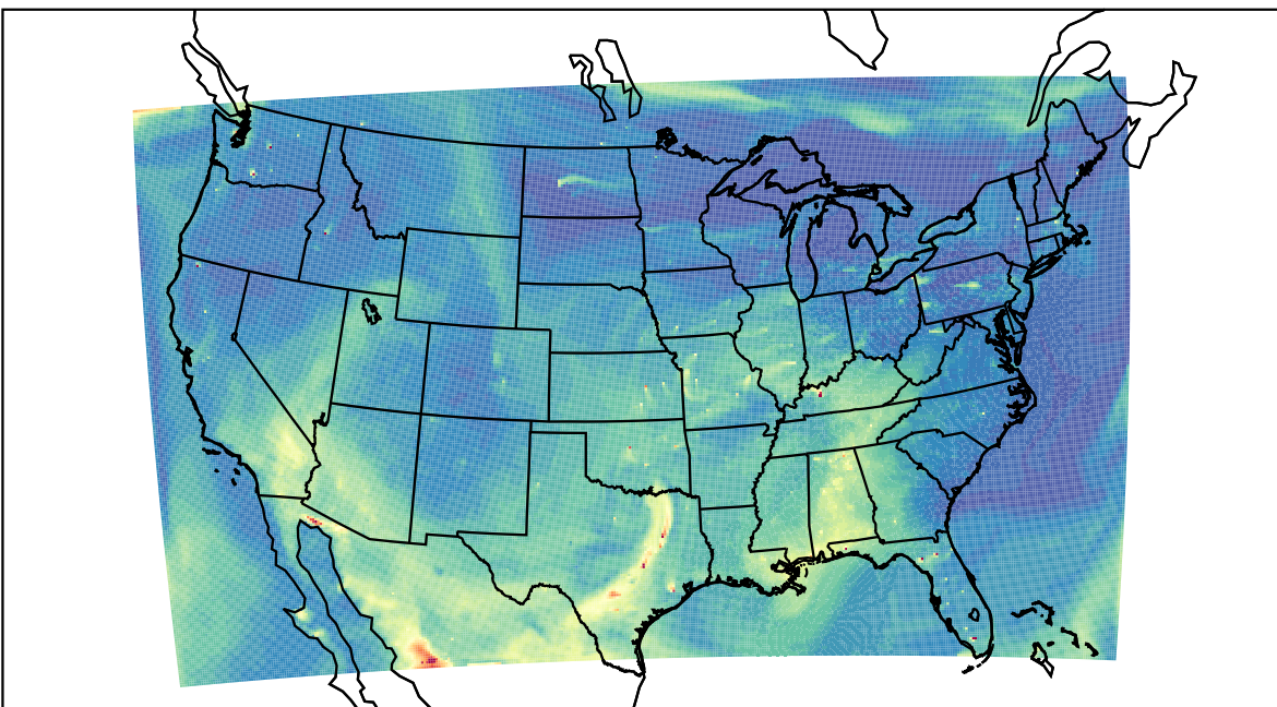
WRF 2023-05-15_23:00:00
