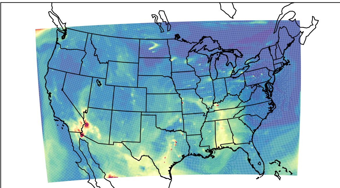
WRF 2023-05-15_14:00:00
