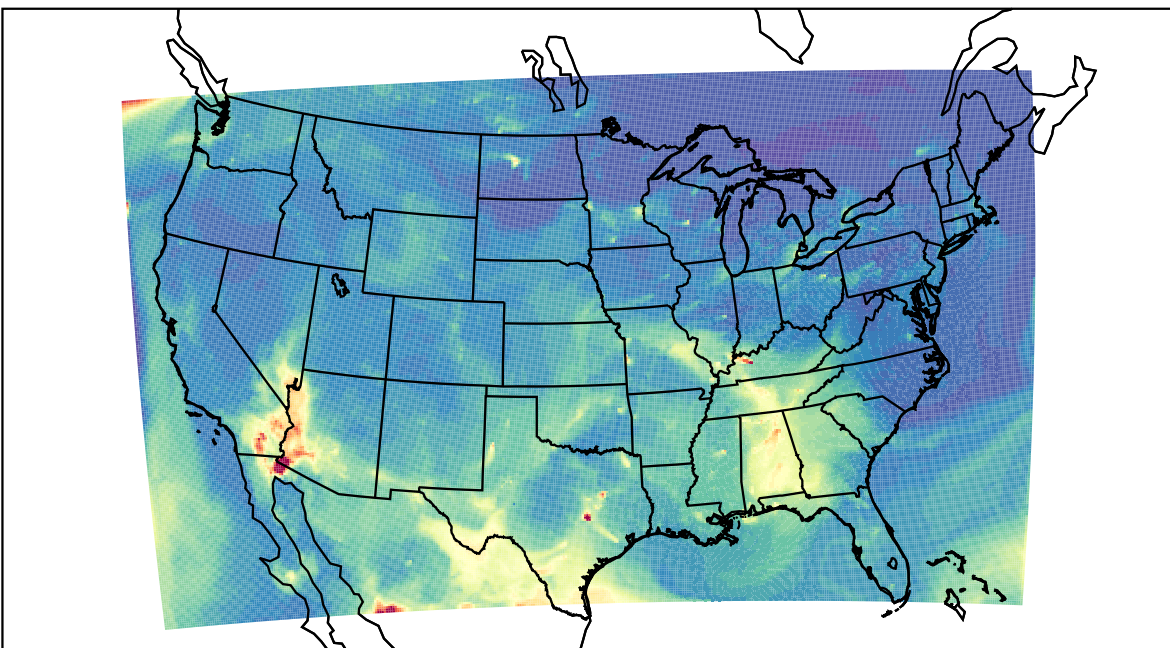
WRF 2023-05-15_09:00:00
