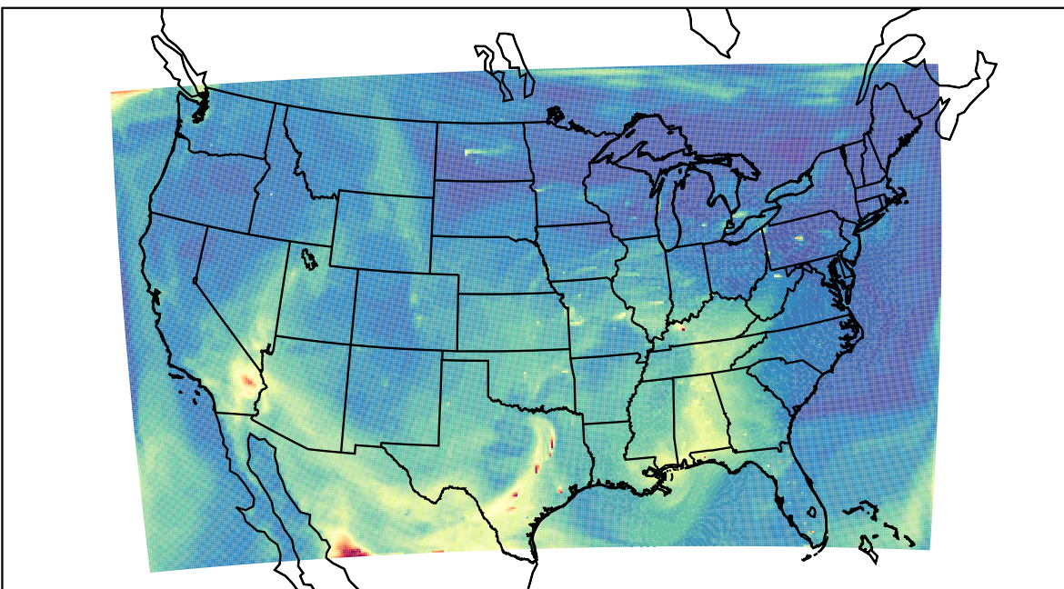
WRF 2023-05-15_19:00:00
