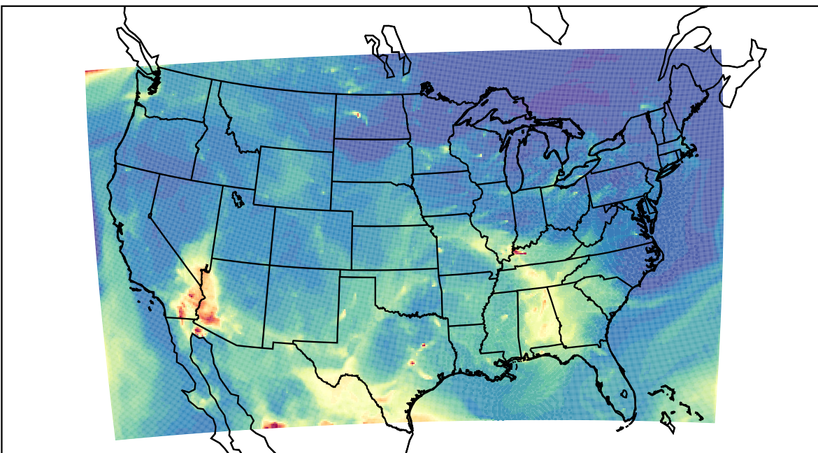
WRF 2023-05-15_07:00:00
