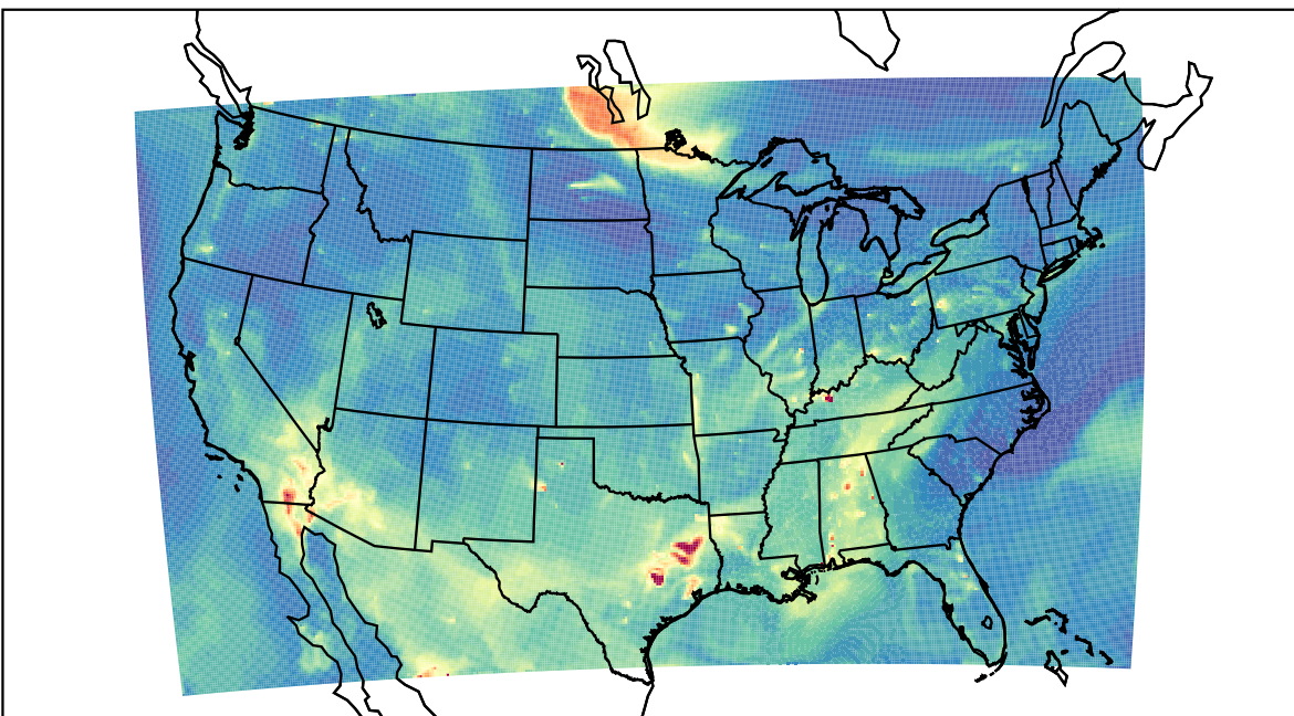
WRF 2023-05-16_12:00:00
