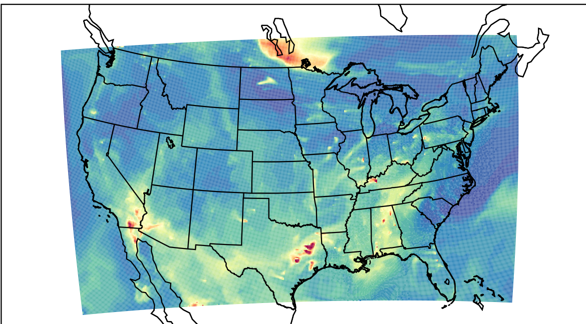
WRF 2023-05-16_10:00:00
