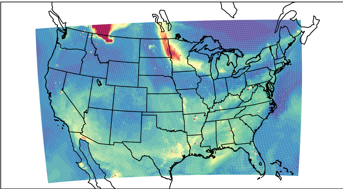
WRF 2023-05-16_23:00:00
