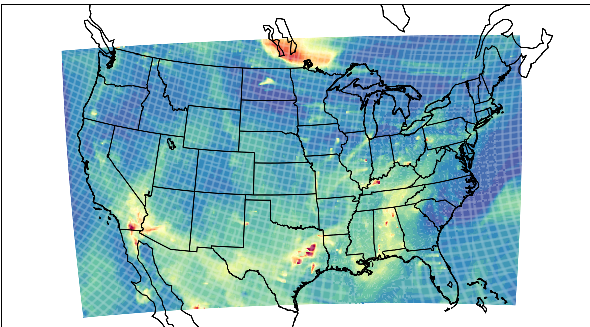
WRF 2023-05-16_09:00:00
