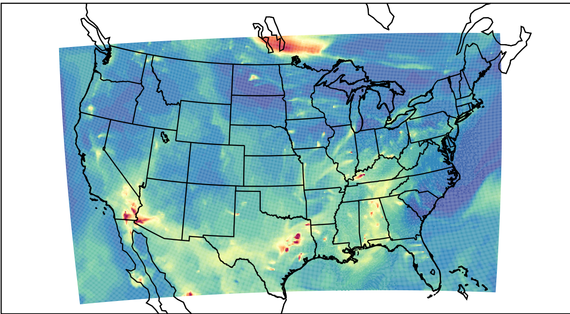
WRF 2023-05-16_07:00:00
