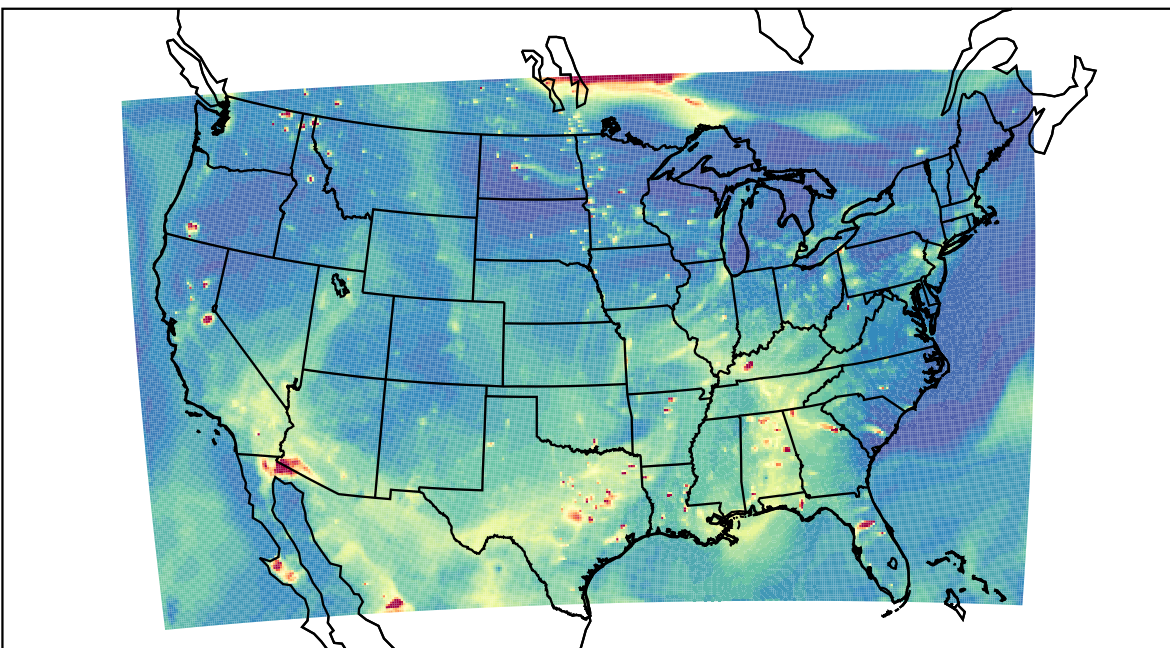
WRF 2023-05-16_02:00:00
