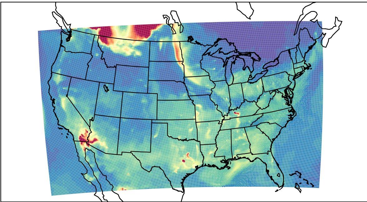
WRF 2023-05-17_08:00:00
