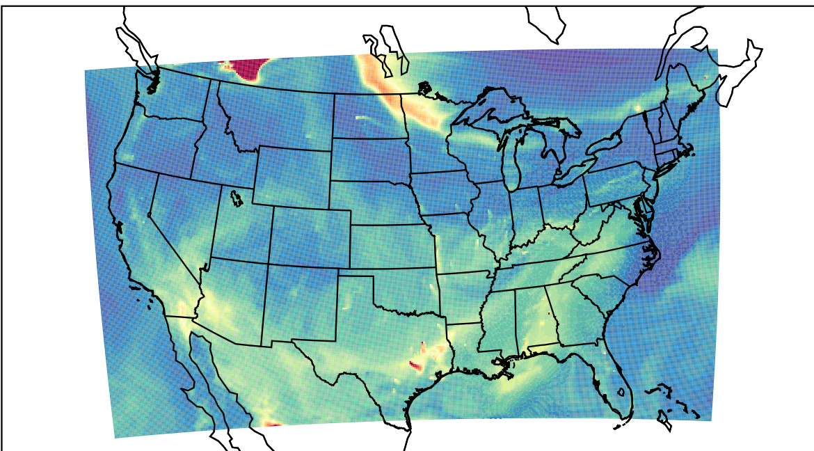
WRF 2023-05-16_17:00:00
