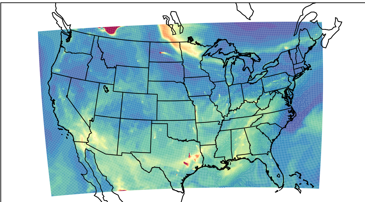
WRF 2023-05-16_16:00:00
