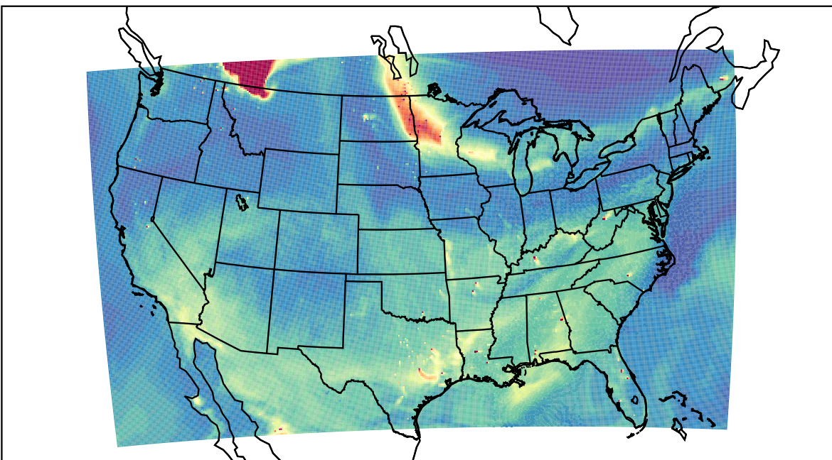
WRF 2023-05-16_21:00:00
