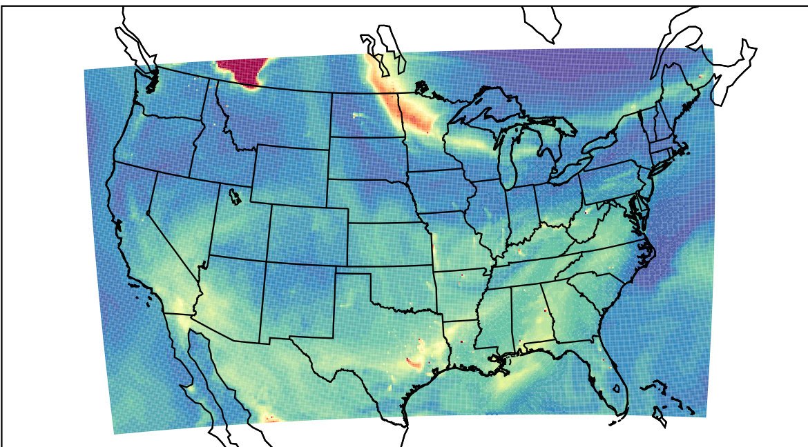
WRF 2023-05-16_19:00:00
