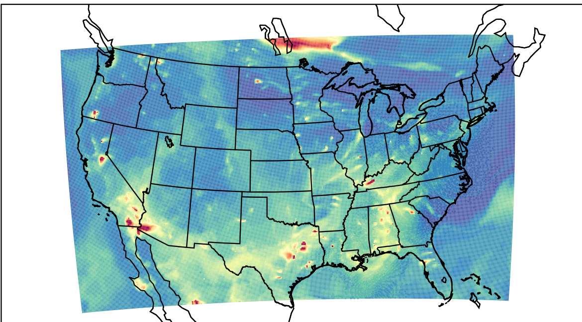
WRF 2023-05-16_05:00:00
