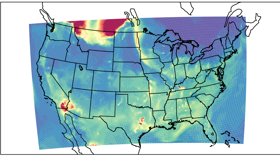
WRF 2023-05-17_11:00:00
