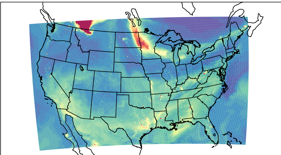
WRF 2023-05-16_22:00:00
