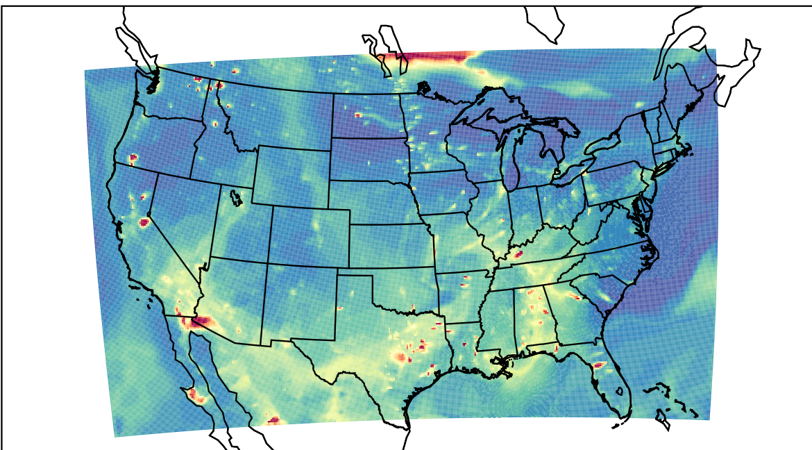
WRF 2023-05-16_03:00:00
