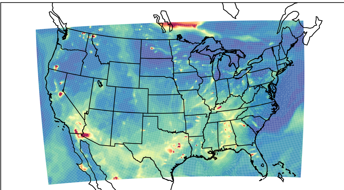
WRF 2023-05-16_04:00:00
