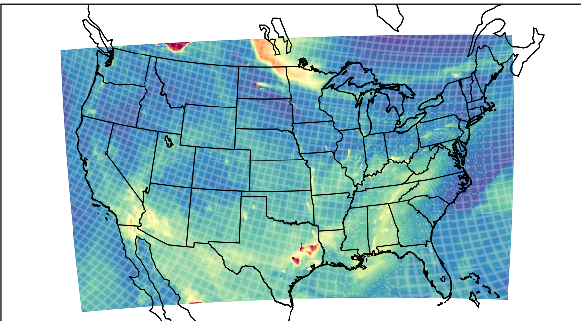
WRF 2023-05-16_15:00:00
