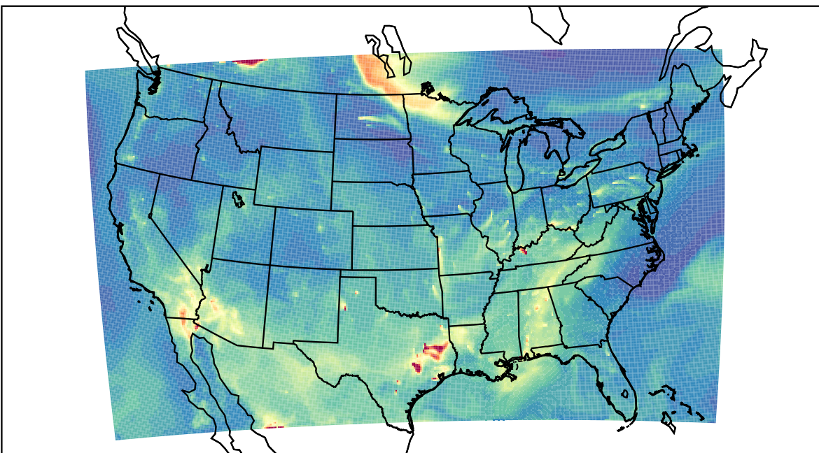
WRF 2023-05-16_14:00:00
