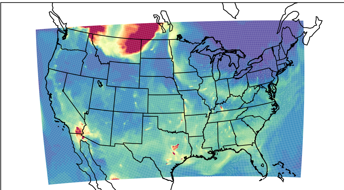
WRF 2023-05-17_14:00:00
