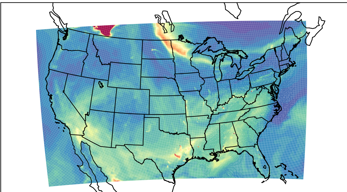
WRF 2023-05-16_18:00:00
