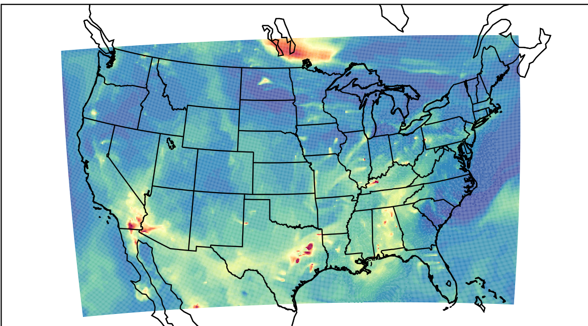
WRF 2023-05-16_08:00:00
