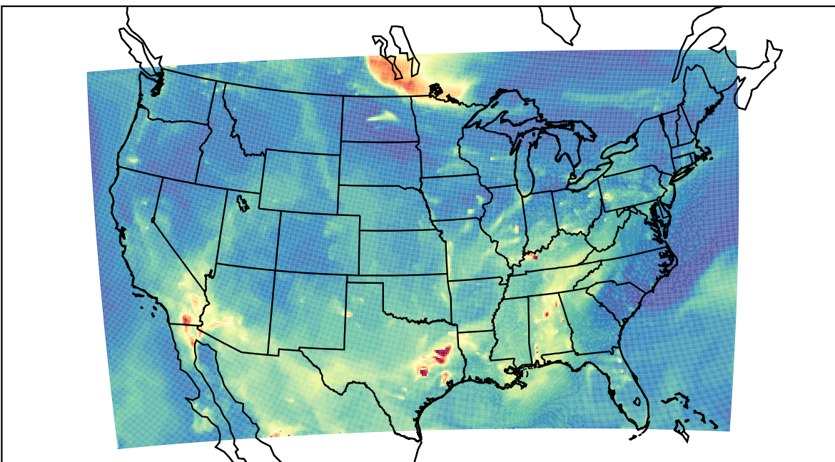
WRF 2023-05-16_11:00:00
