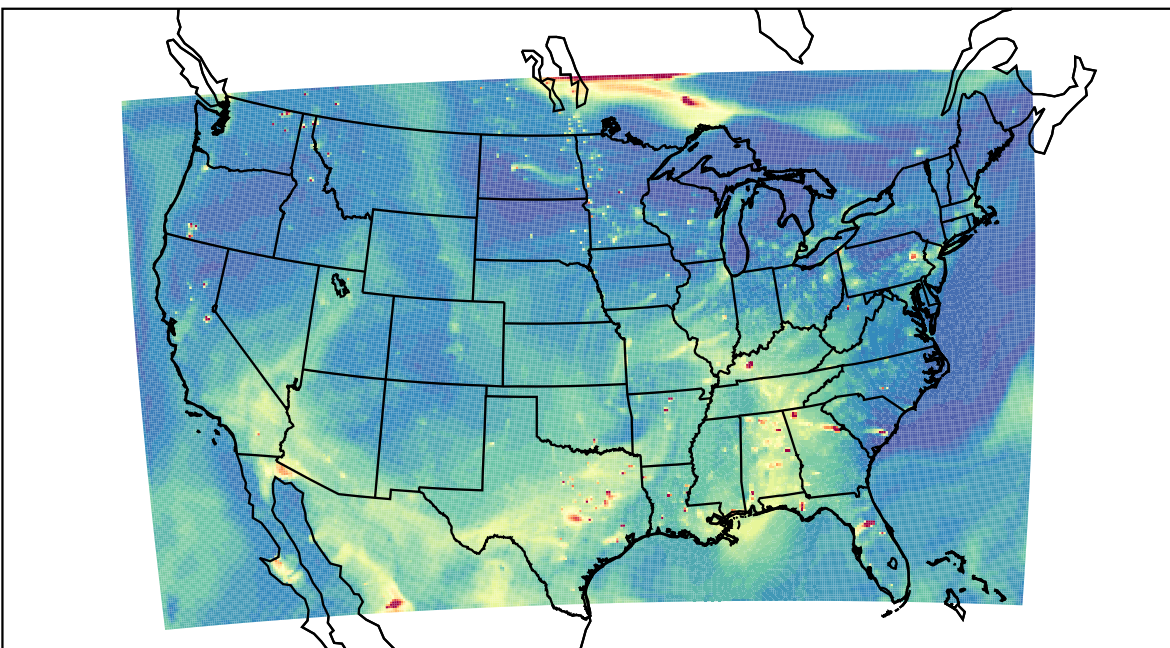
WRF 2023-05-16_01:00:00
