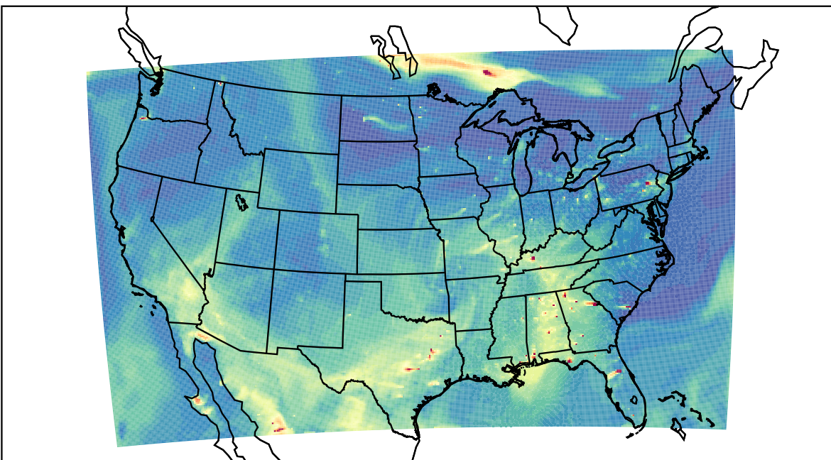
WRF 2023-05-16_00:00:00
