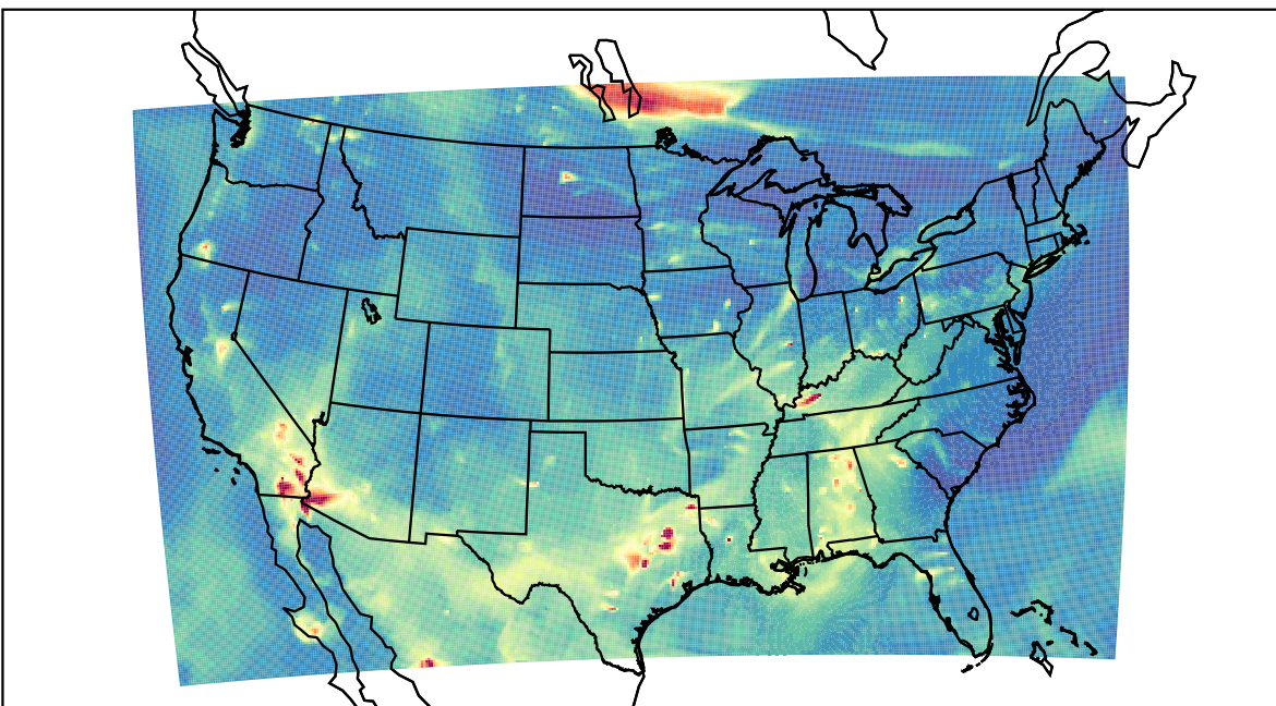
WRF 2023-05-16_06:00:00
