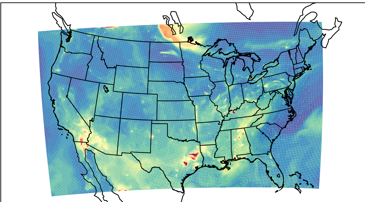
WRF 2023-05-16_13:00:00
