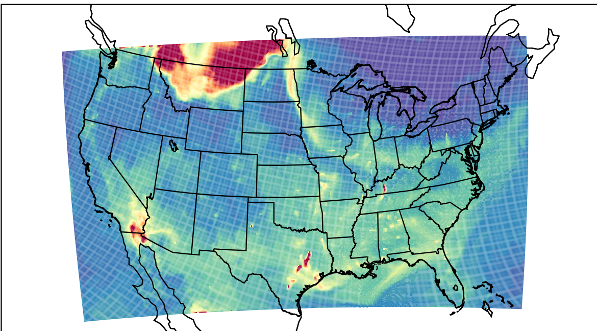
WRF 2023-05-17_13:00:00
