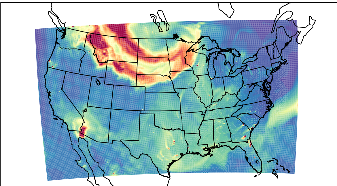
WRF 2023-05-18_22:00:00
