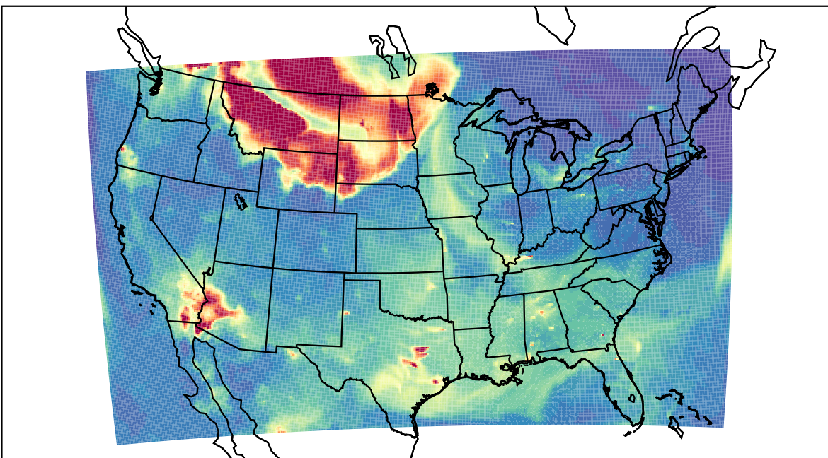
WRF 2023-05-18_09:00:00
