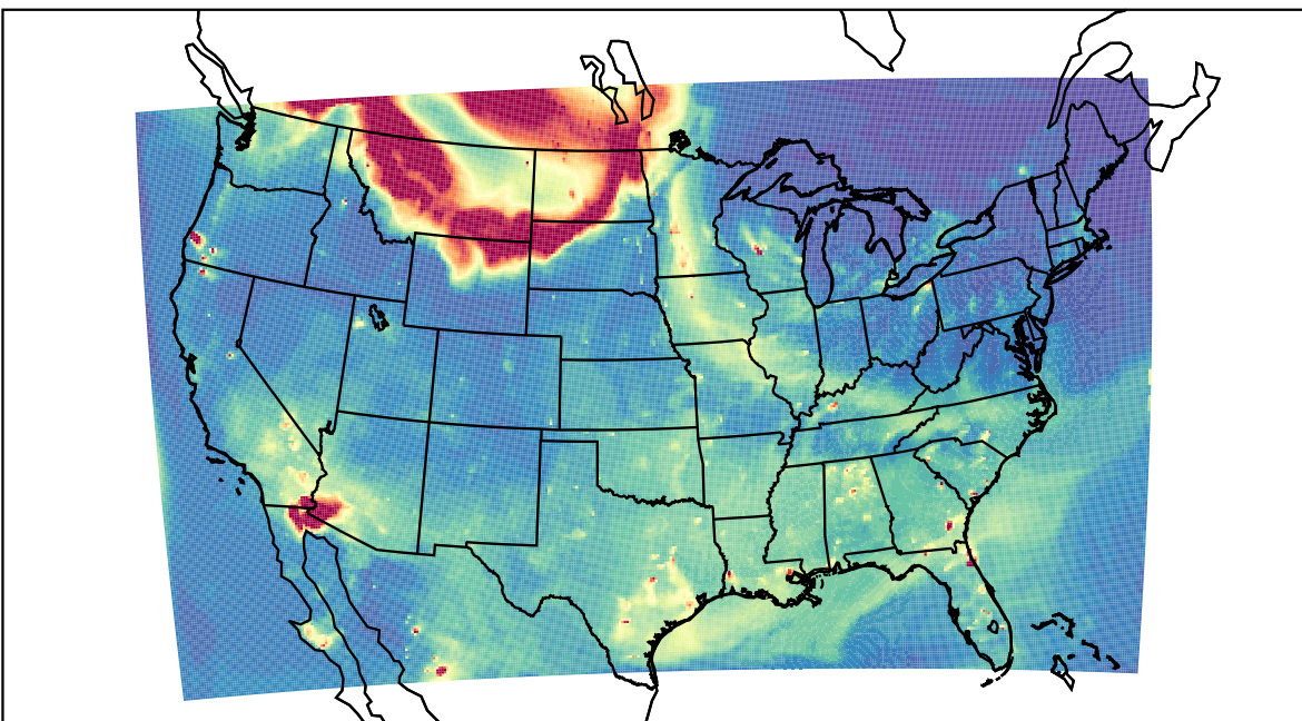
WRF 2023-05-18_02:00:00
