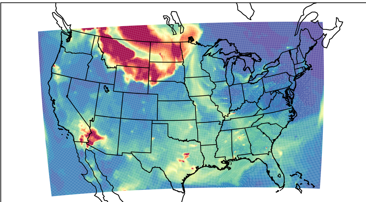
WRF 2023-05-18_08:00:00
