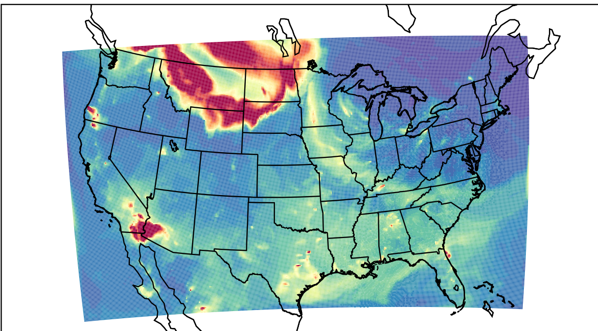
WRF 2023-05-18_04:00:00
