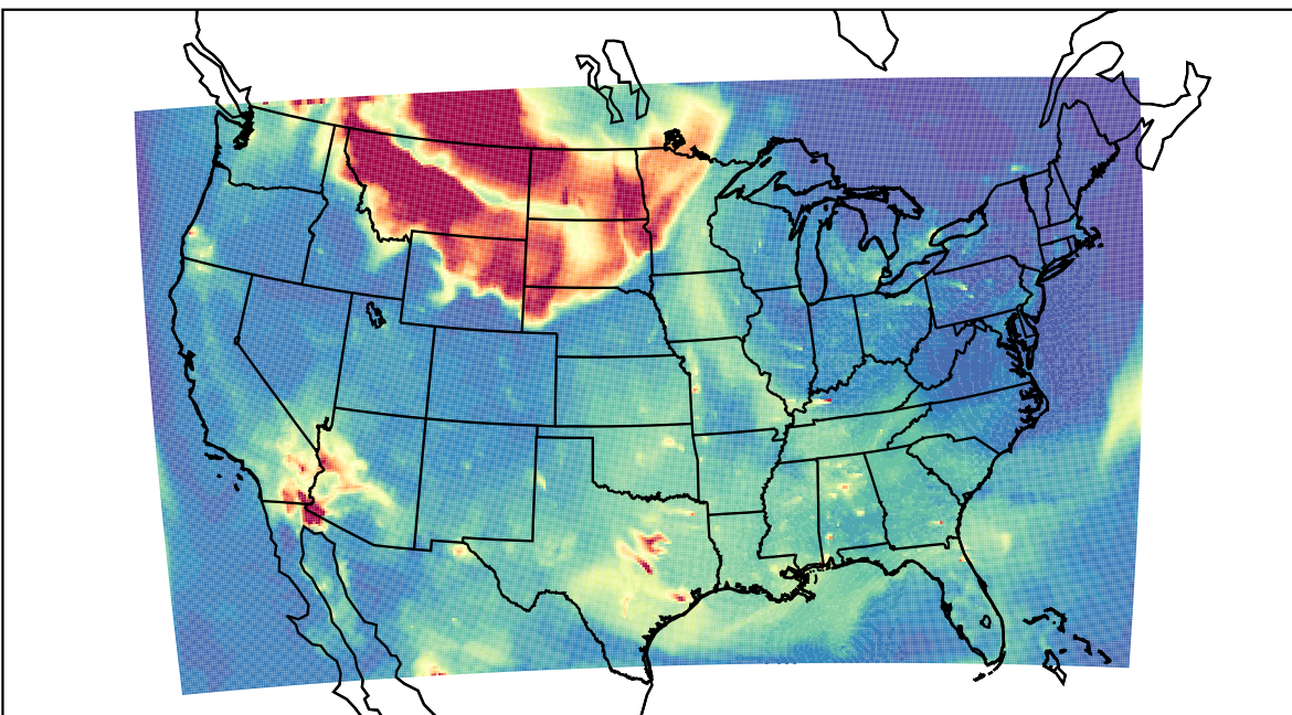
WRF 2023-05-18_12:00:00
