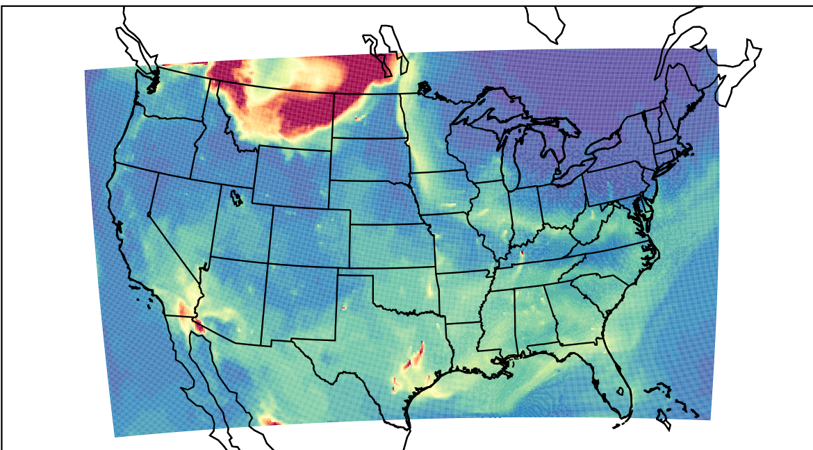
WRF 2023-05-17_16:00:00
