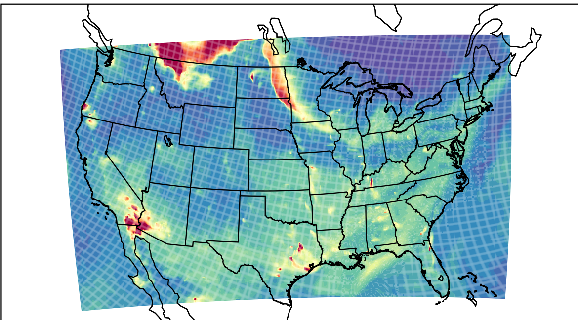
WRF 2023-05-17_05:00:00
