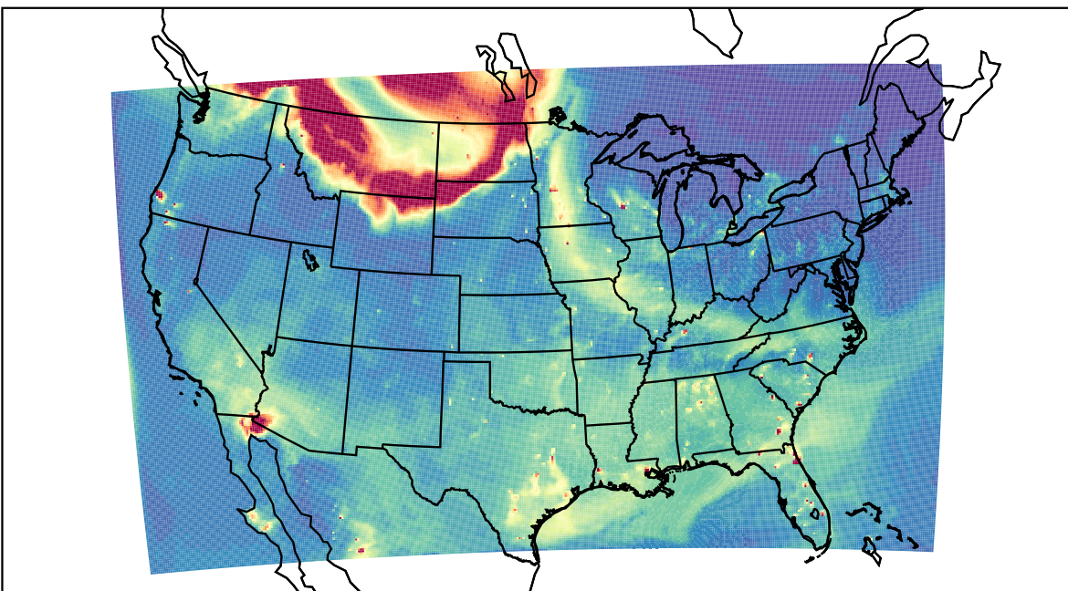
WRF 2023-05-18_01:00:00
