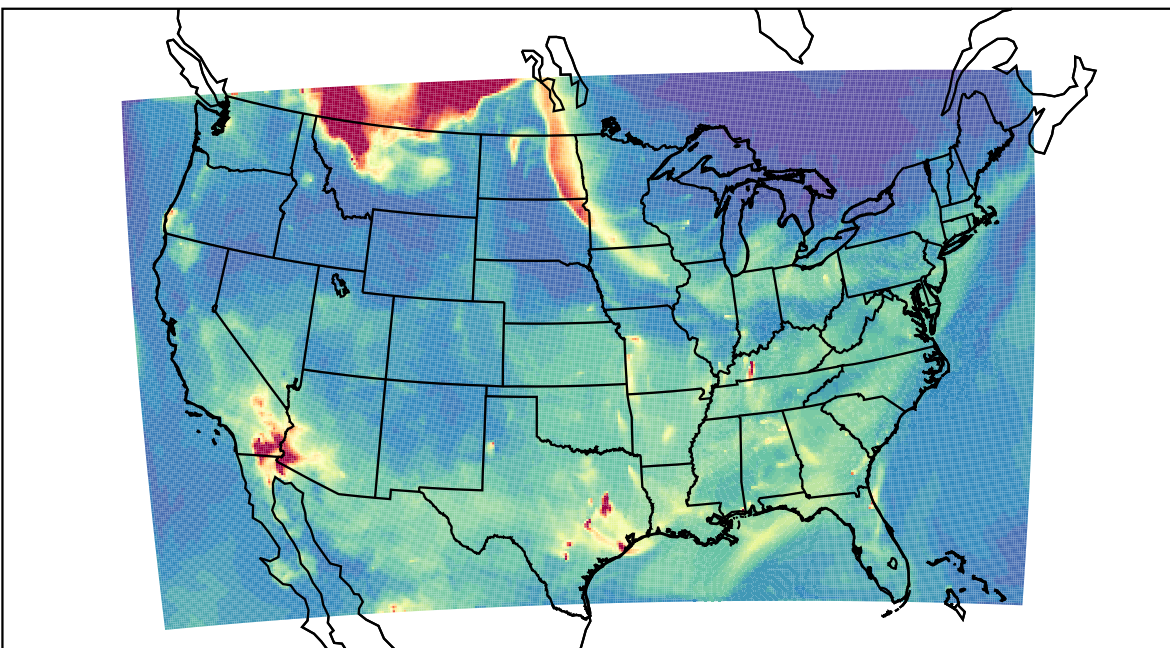
WRF 2023-05-17_07:00:00
