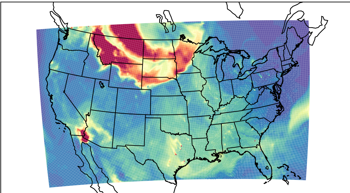
WRF 2023-05-18_17:00:00
