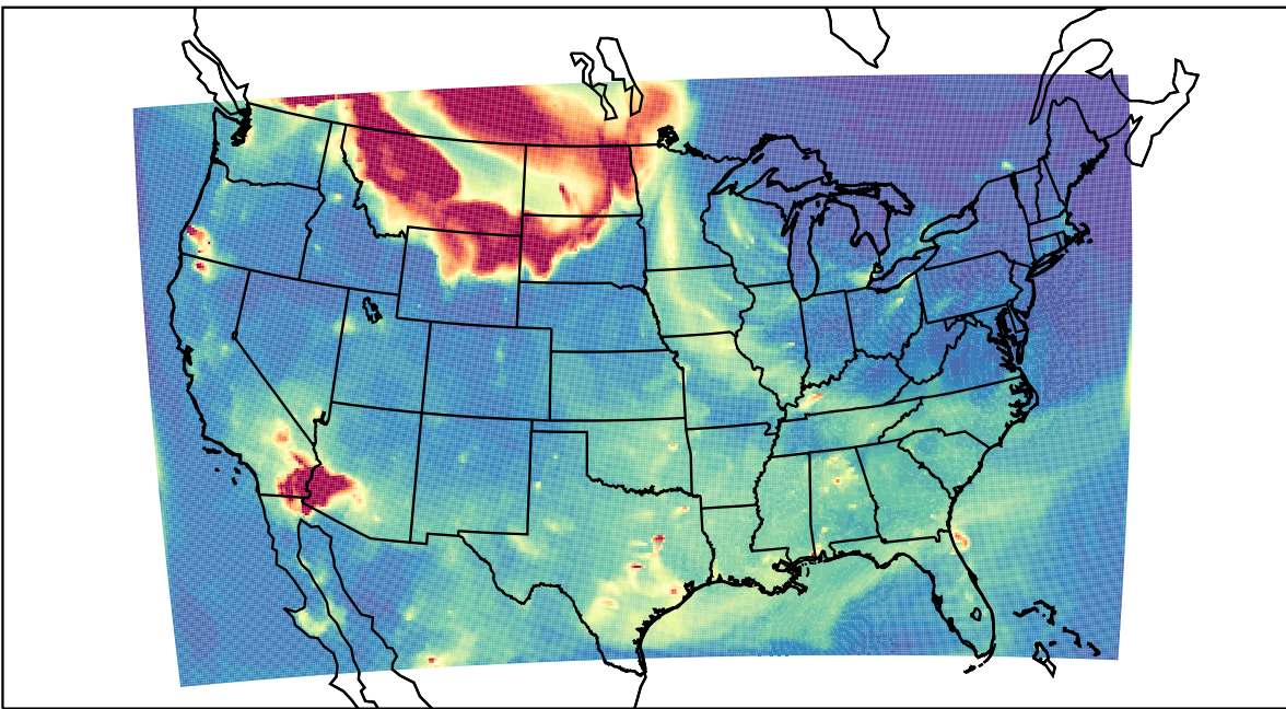
WRF 2023-05-18_05:00:00
