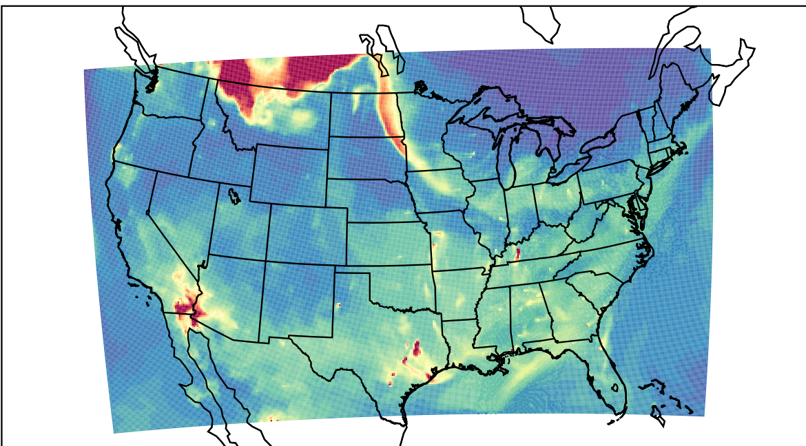
WRF 2023-05-17_08:00:00
