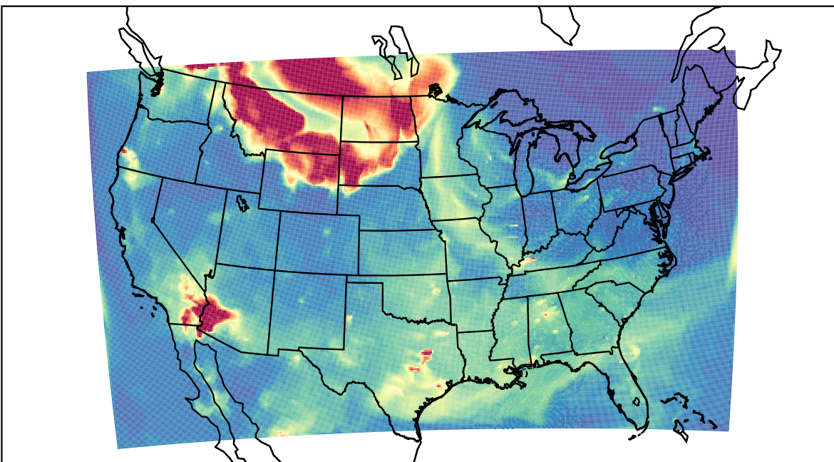
WRF 2023-05-18_07:00:00
