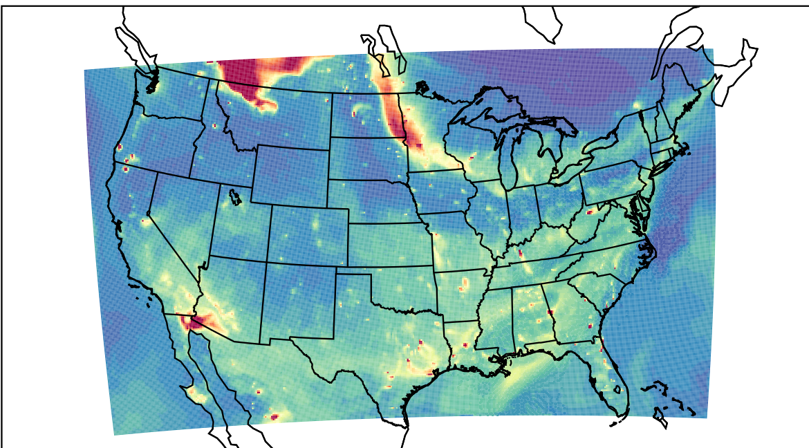
WRF 2023-05-17_02:00:00
