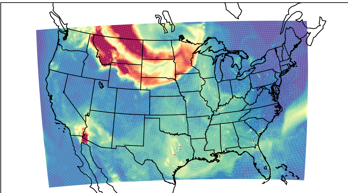
WRF 2023-05-18_19:00:00
