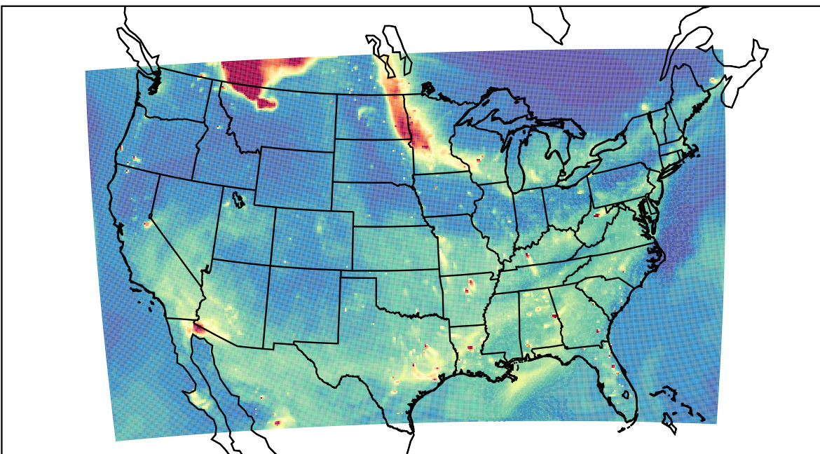
WRF 2023-05-17_01:00:00
