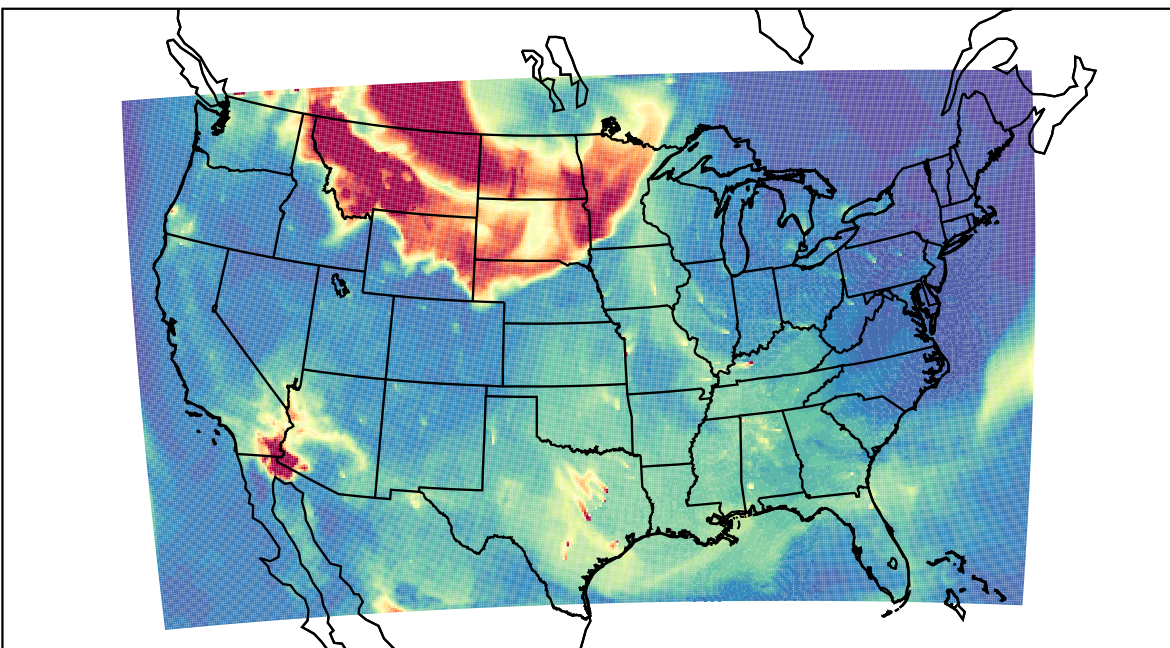
WRF 2023-05-18_15:00:00
