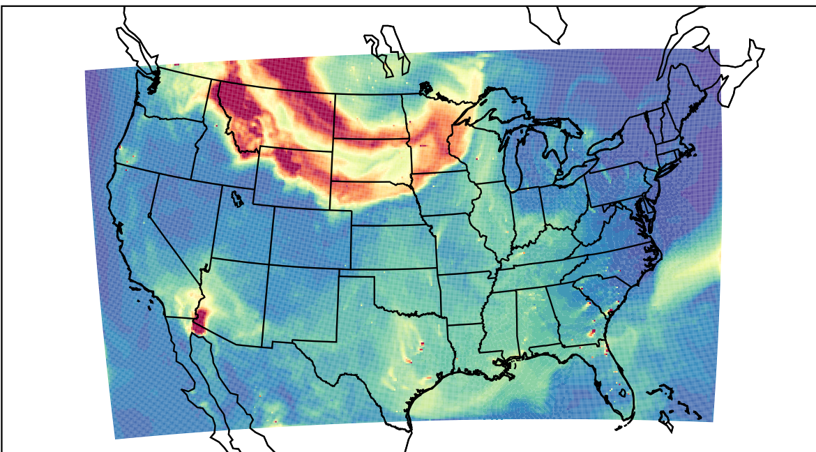
WRF 2023-05-18_21:00:00
