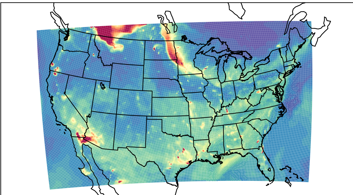
WRF 2023-05-17_03:00:00
