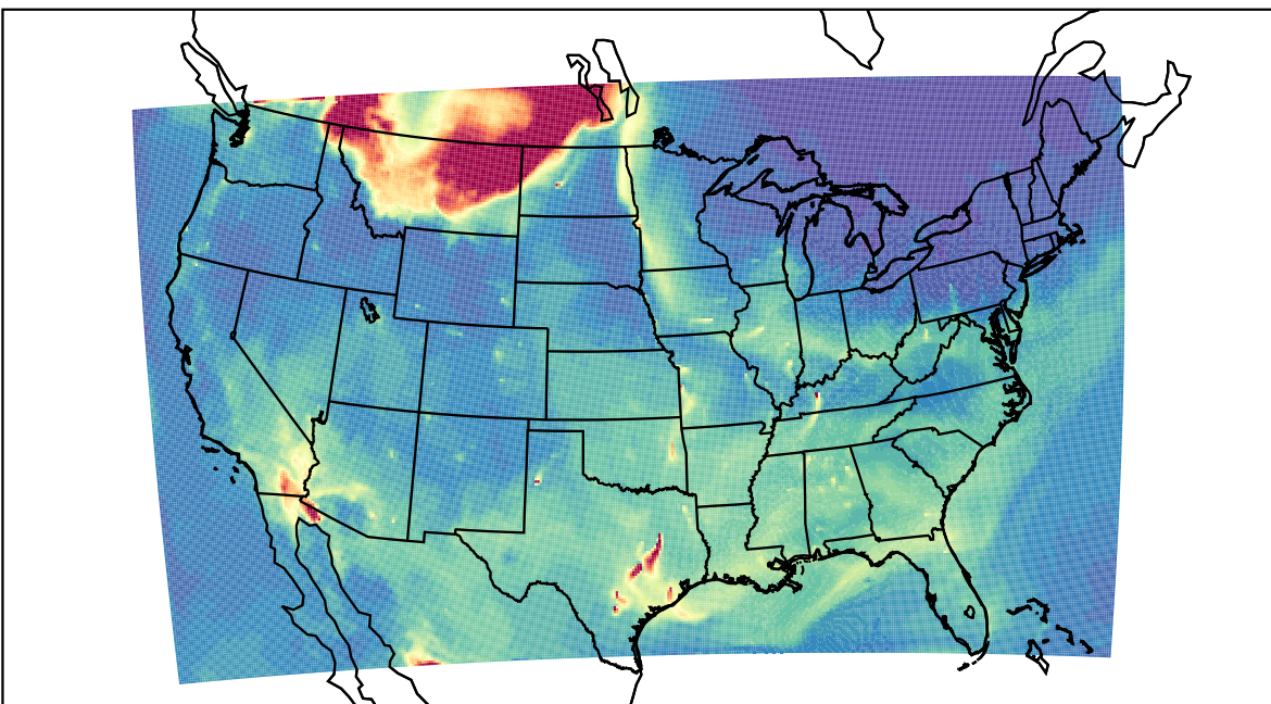
WRF 2023-05-17_15:00:00
