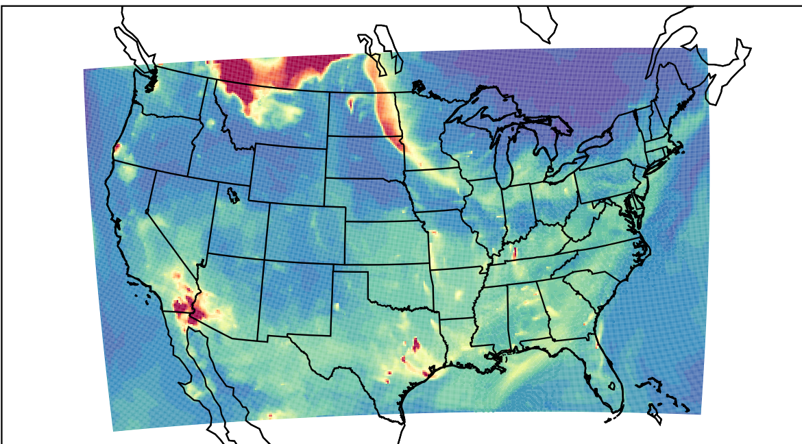
WRF 2023-05-17_06:00:00
