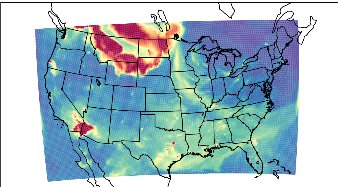
WRF 2023-05-18_06:00:00
