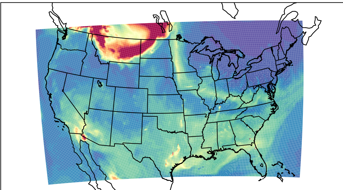
WRF 2023-05-17_18:00:00
