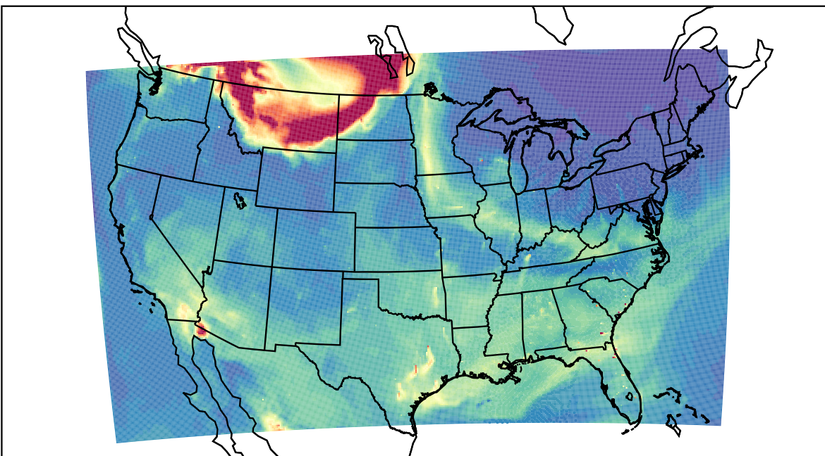
WRF 2023-05-17_19:00:00
