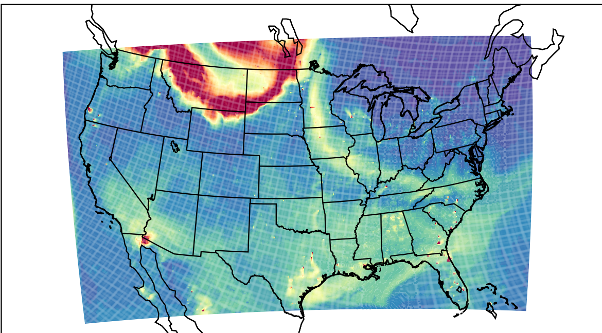
WRF 2023-05-18_00:00:00
