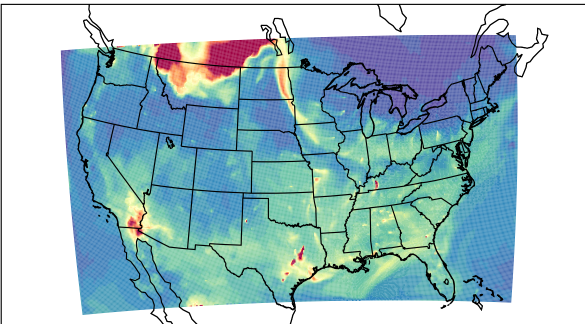
WRF 2023-05-17_11:00:00
