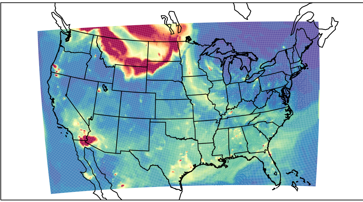
WRF 2023-05-18_03:00:00
