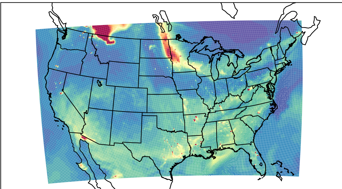
WRF 2023-05-17_00:00:00
