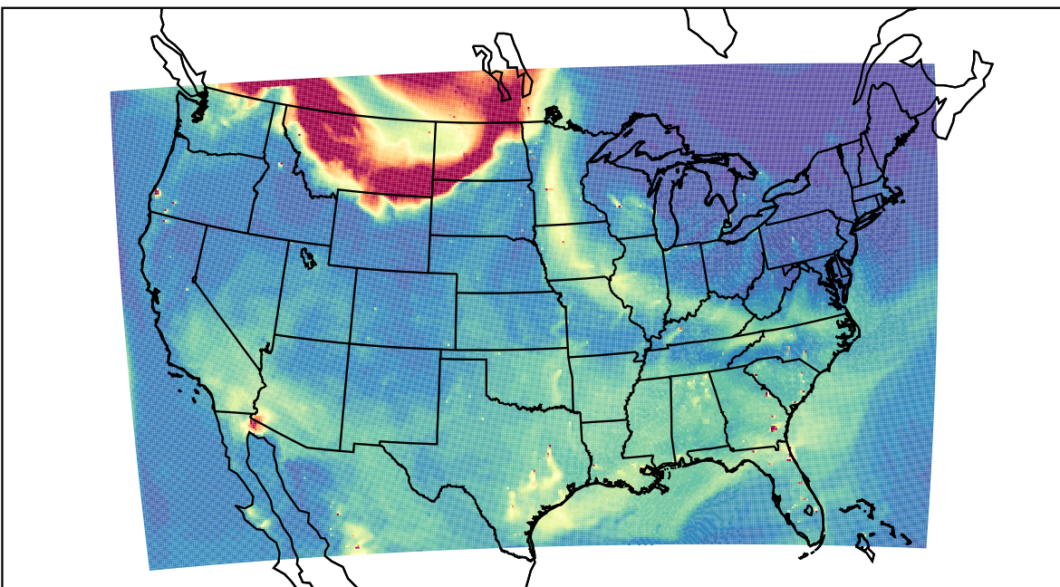
WRF 2023-05-17_23:00:00
