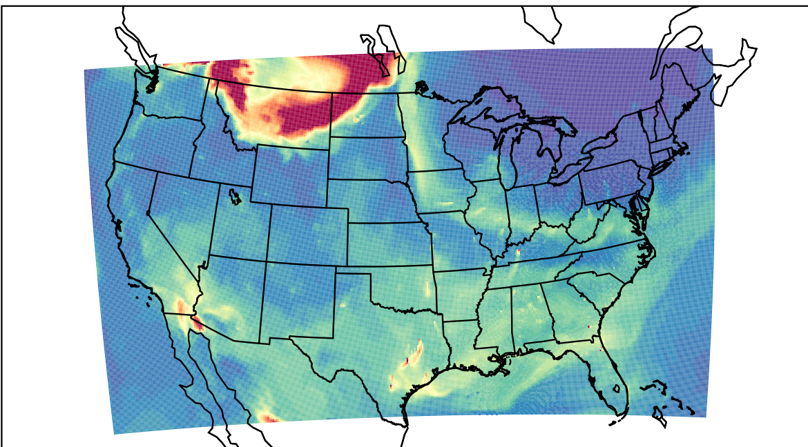
WRF 2023-05-17_17:00:00
