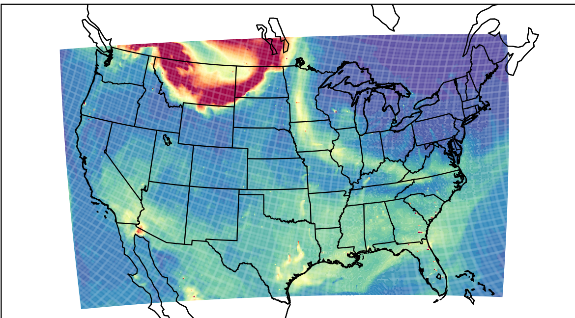
WRF 2023-05-17_21:00:00
