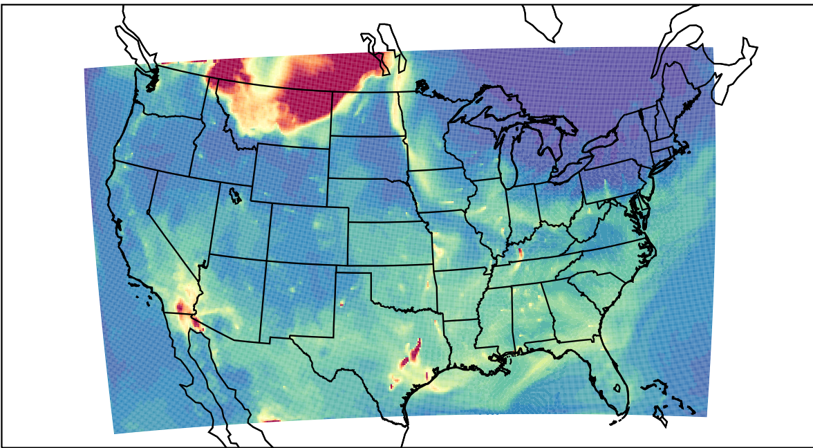
WRF 2023-05-17_14:00:00
