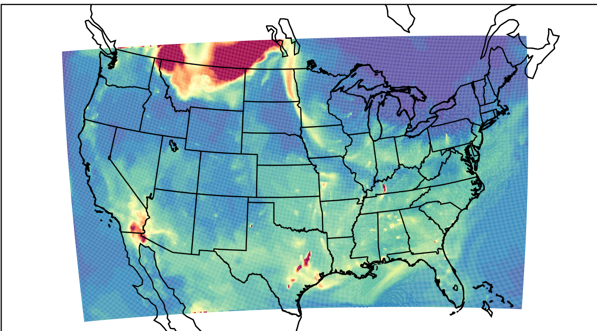
WRF 2023-05-17_12:00:00
