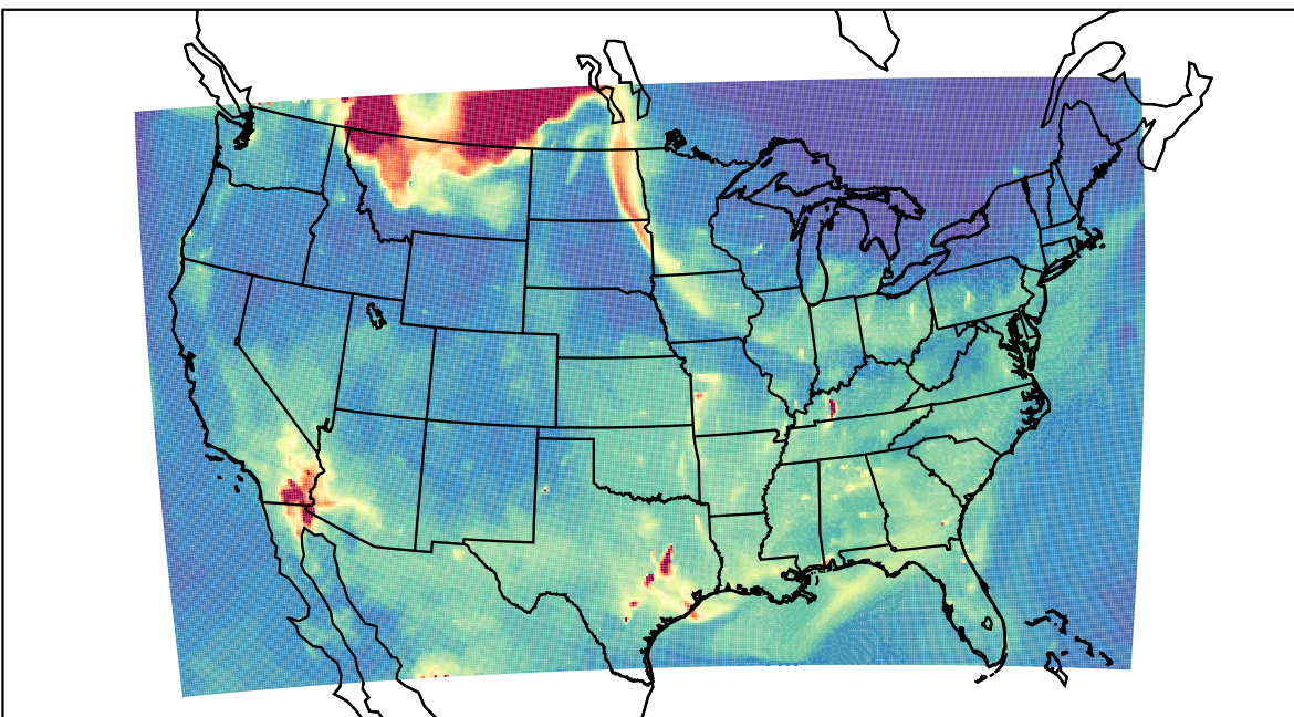
WRF 2023-05-17_10:00:00
