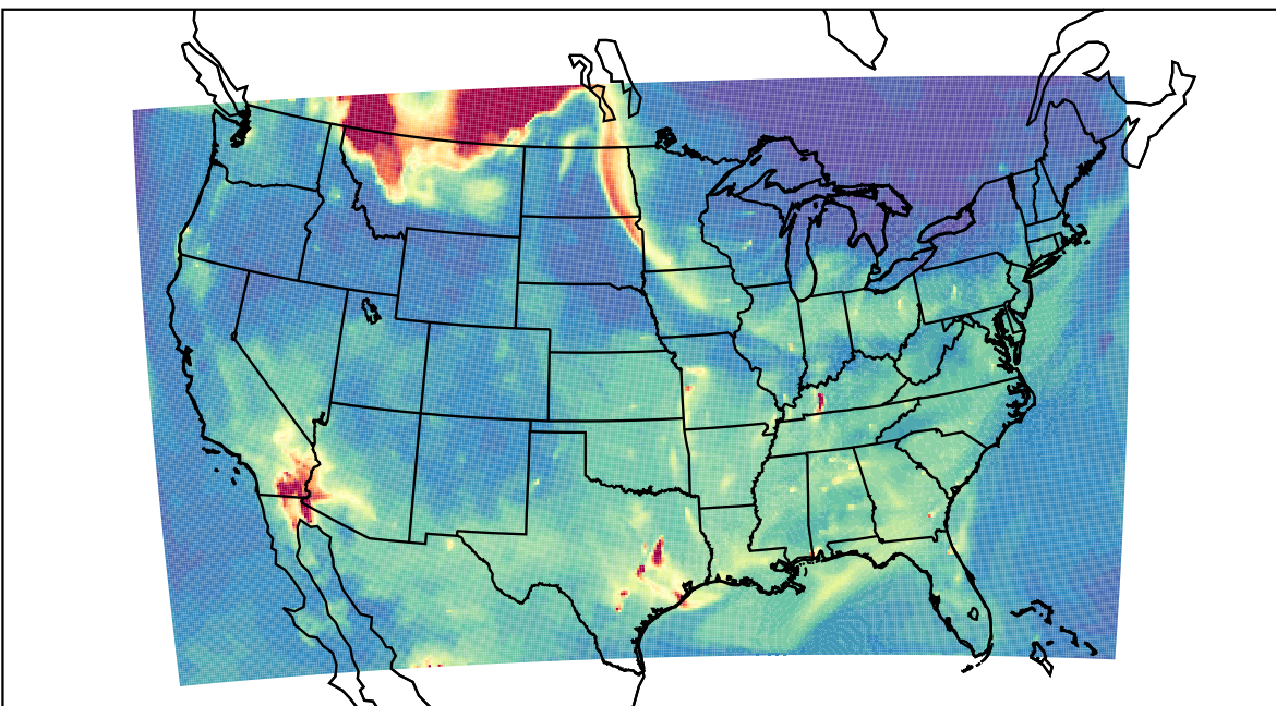
WRF 2023-05-17_09:00:00
