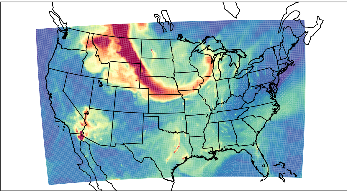
WRF 2023-05-19_14:00:00
