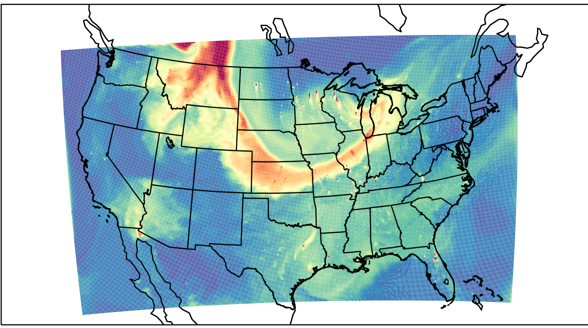
WRF 2023-05-19_22:00:00
