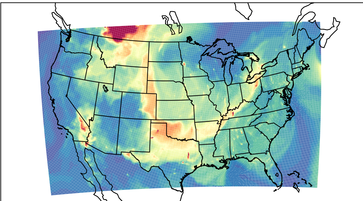
WRF 2023-05-20_12:00:00
