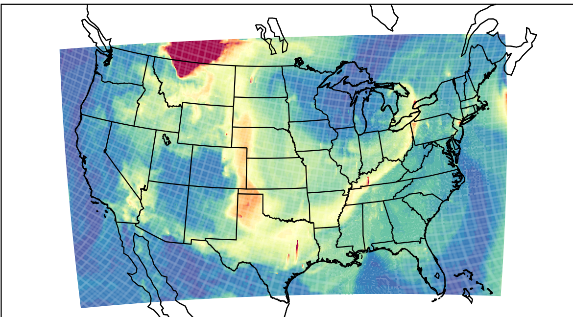
WRF 2023-05-20_16:00:00
