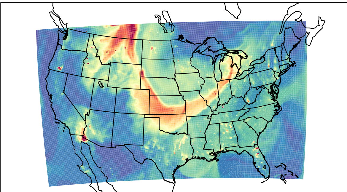
WRF 2023-05-20_01:00:00
