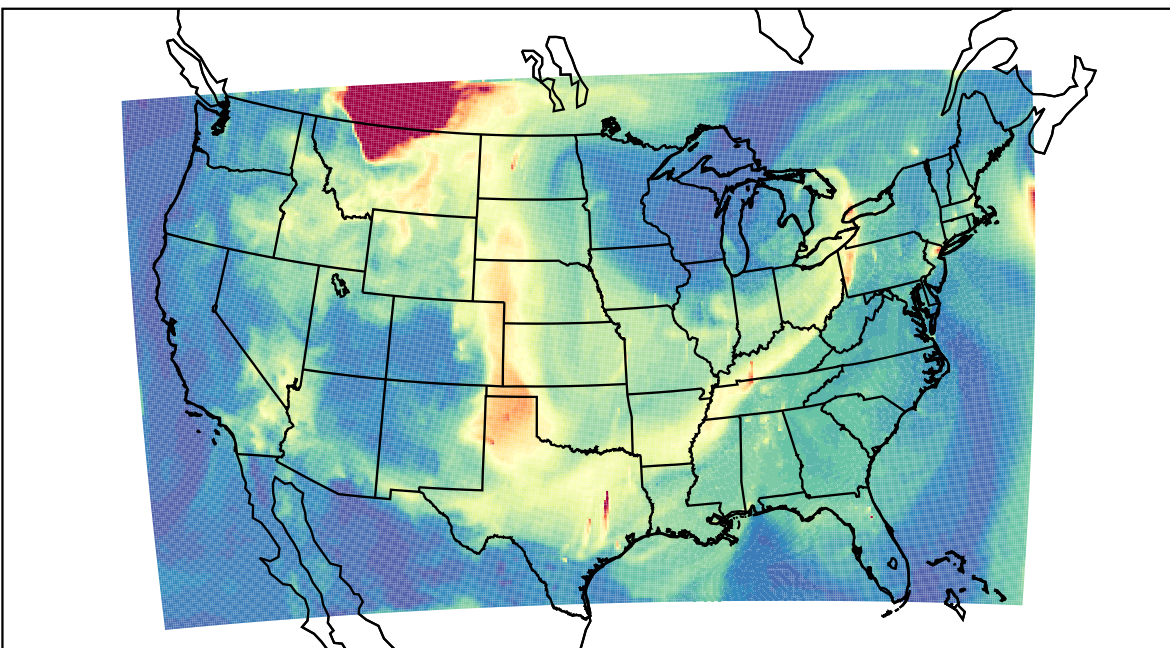
WRF 2023-05-20_17:00:00
