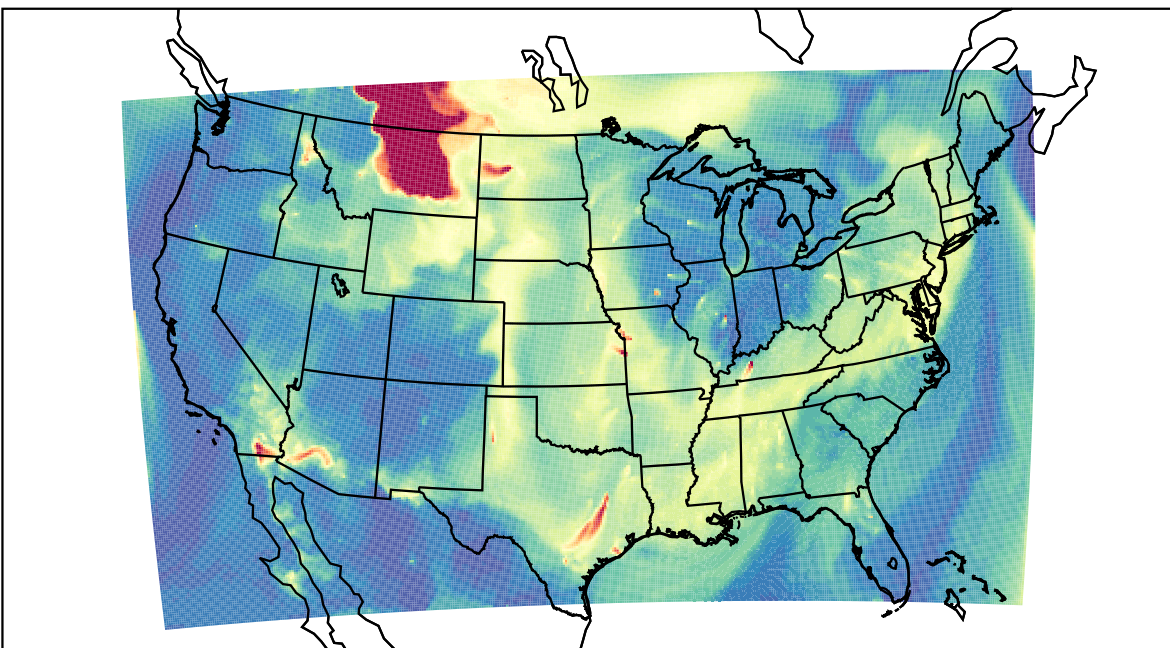
WRF 2023-05-21_09:00:00
