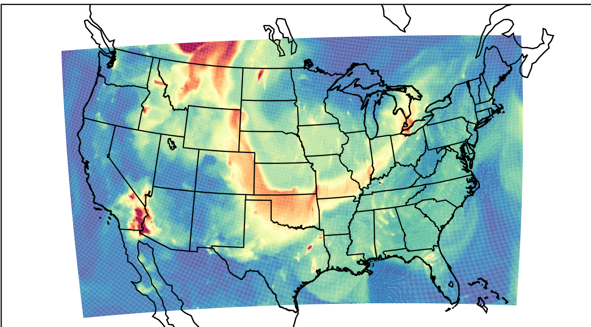
WRF 2023-05-20_06:00:00
