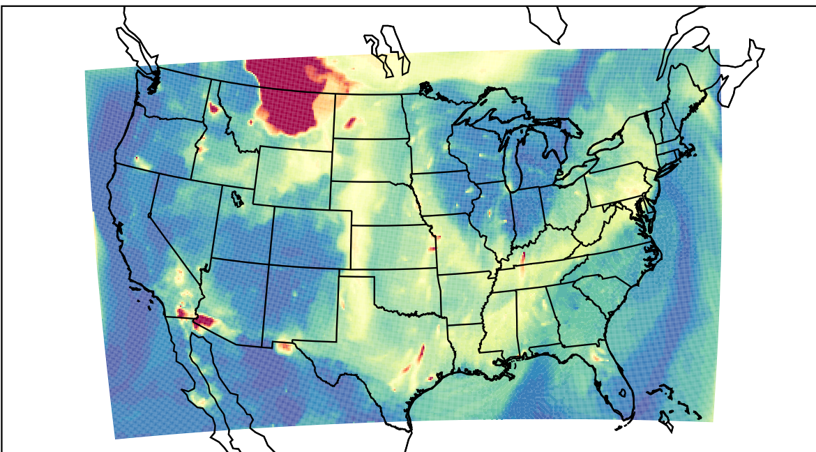
WRF 2023-05-21_05:00:00
