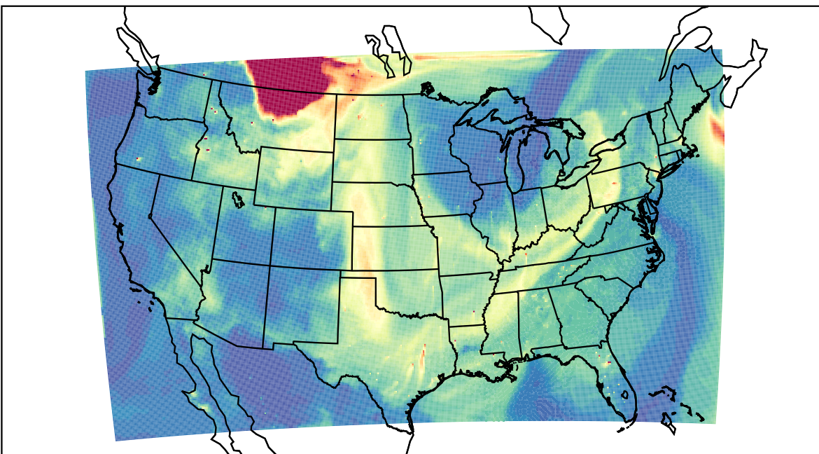
WRF 2023-05-20_22:00:00
