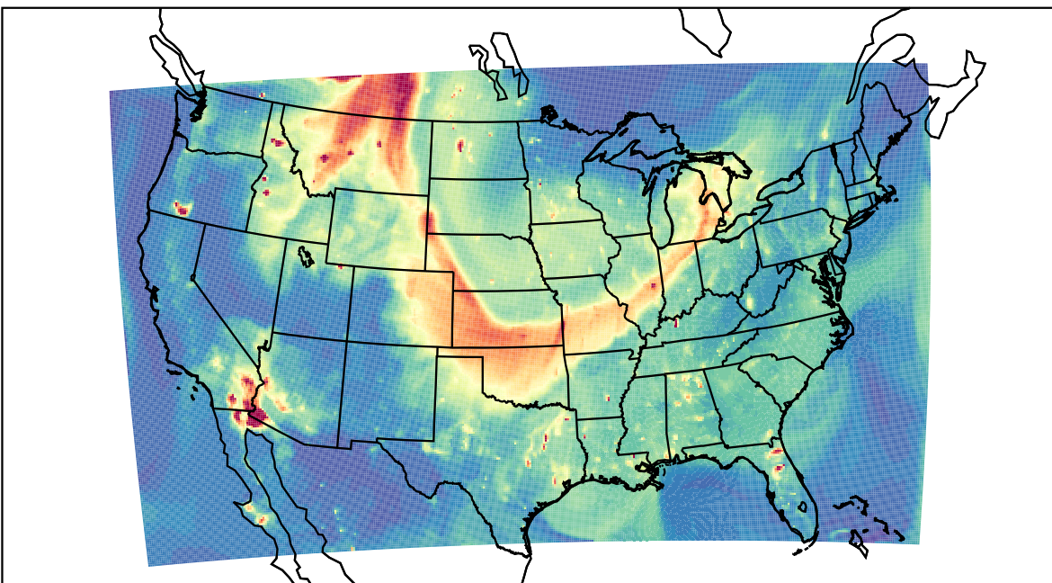
WRF 2023-05-20_02:00:00
