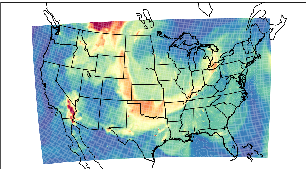
WRF 2023-05-20_09:00:00
