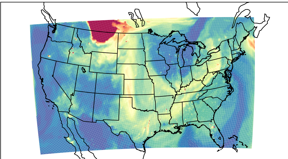
WRF 2023-05-21_00:00:00
