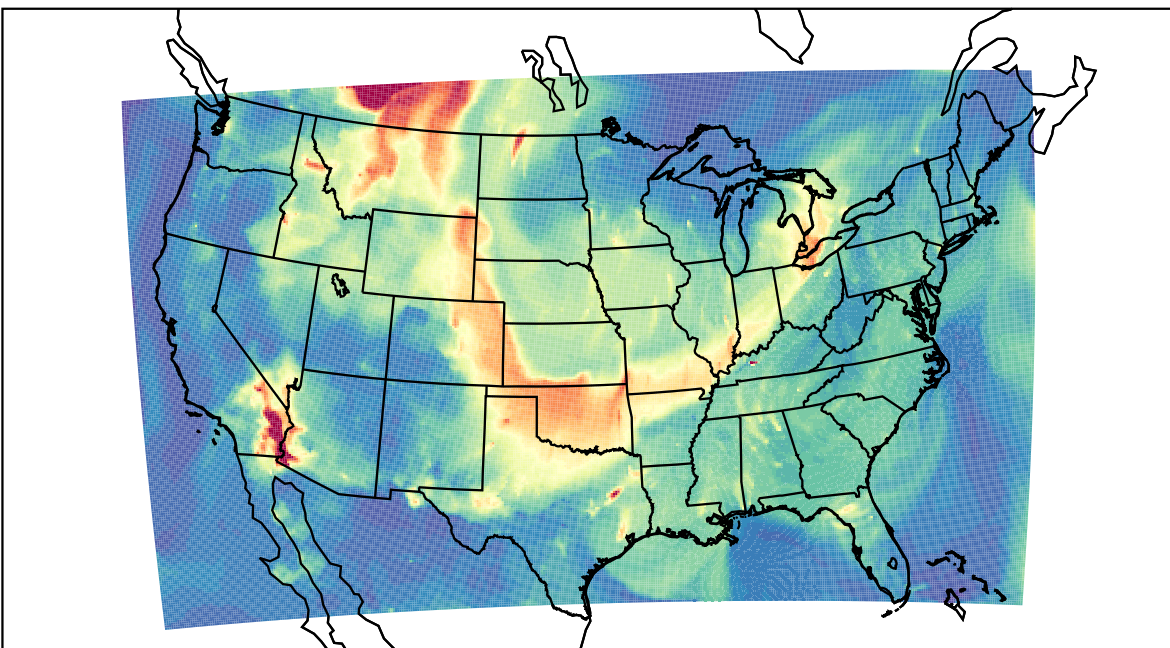
WRF 2023-05-20_07:00:00
