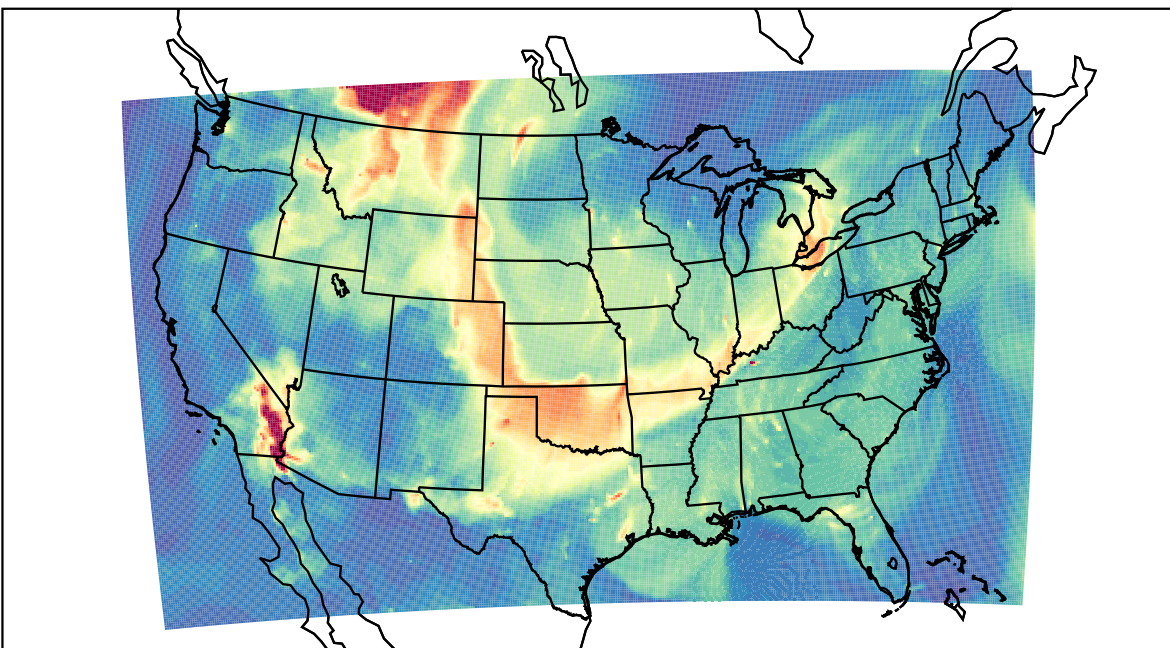
WRF 2023-05-20_08:00:00
