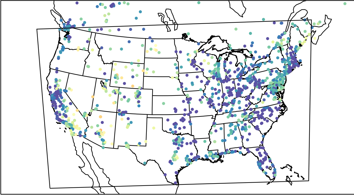
AirNOW (2023-05-21_07:00:00)
