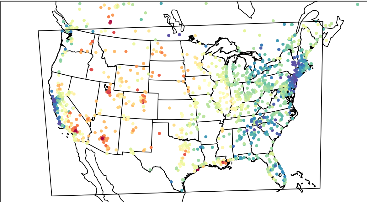
AirNOW (2023-05-20_23:00:00)
