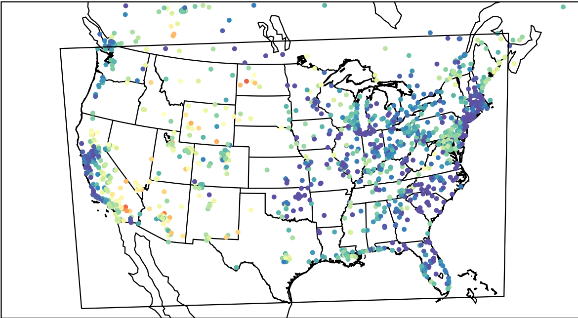
AirNOW (2023-05-21_04:00:00)
