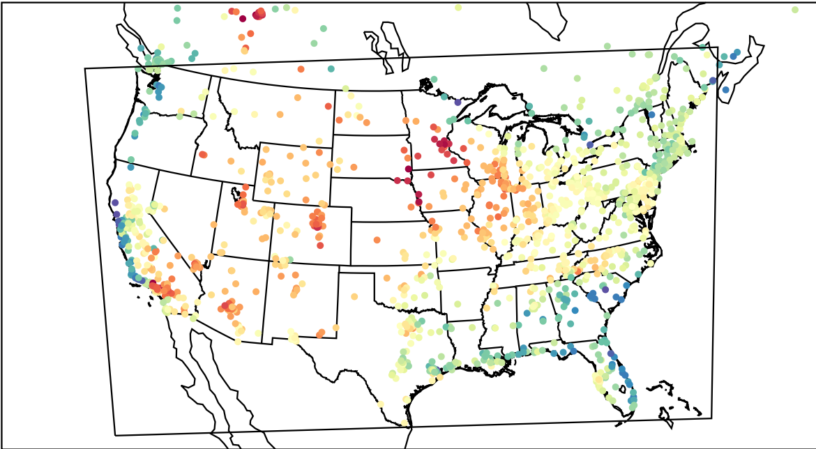
AirNOW (2023-05-21_22:00:00)
