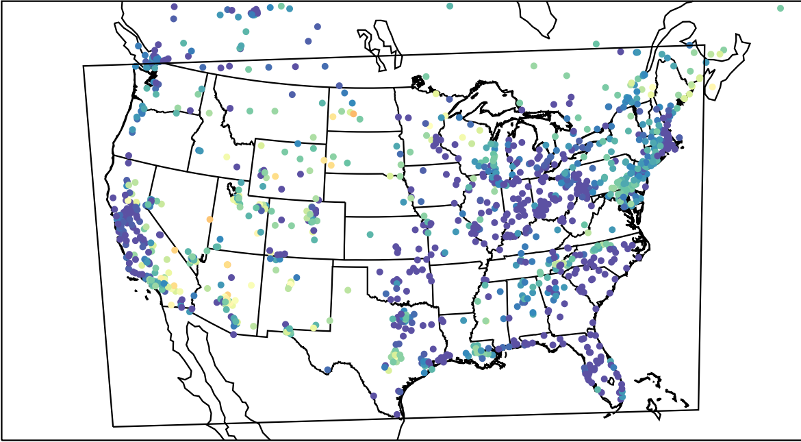
AirNOW (2023-05-21_09:00:00)
