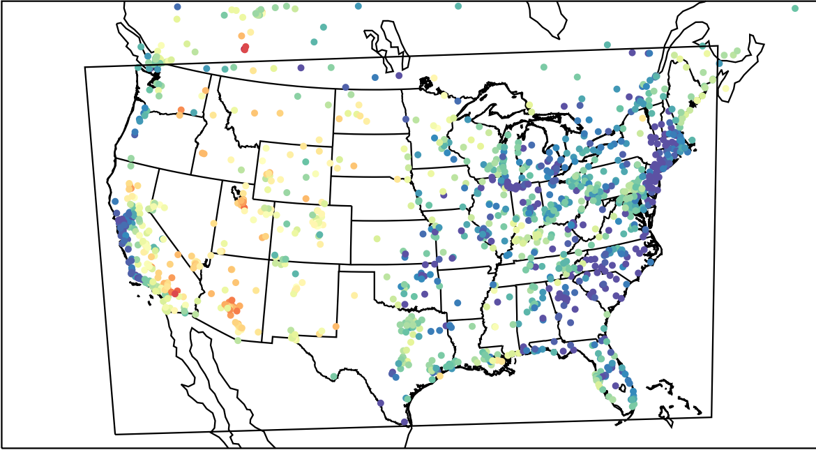
AirNOW (2023-05-21_02:00:00)
