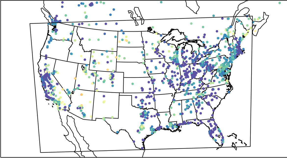
AirNOW (2023-05-21_08:00:00)
