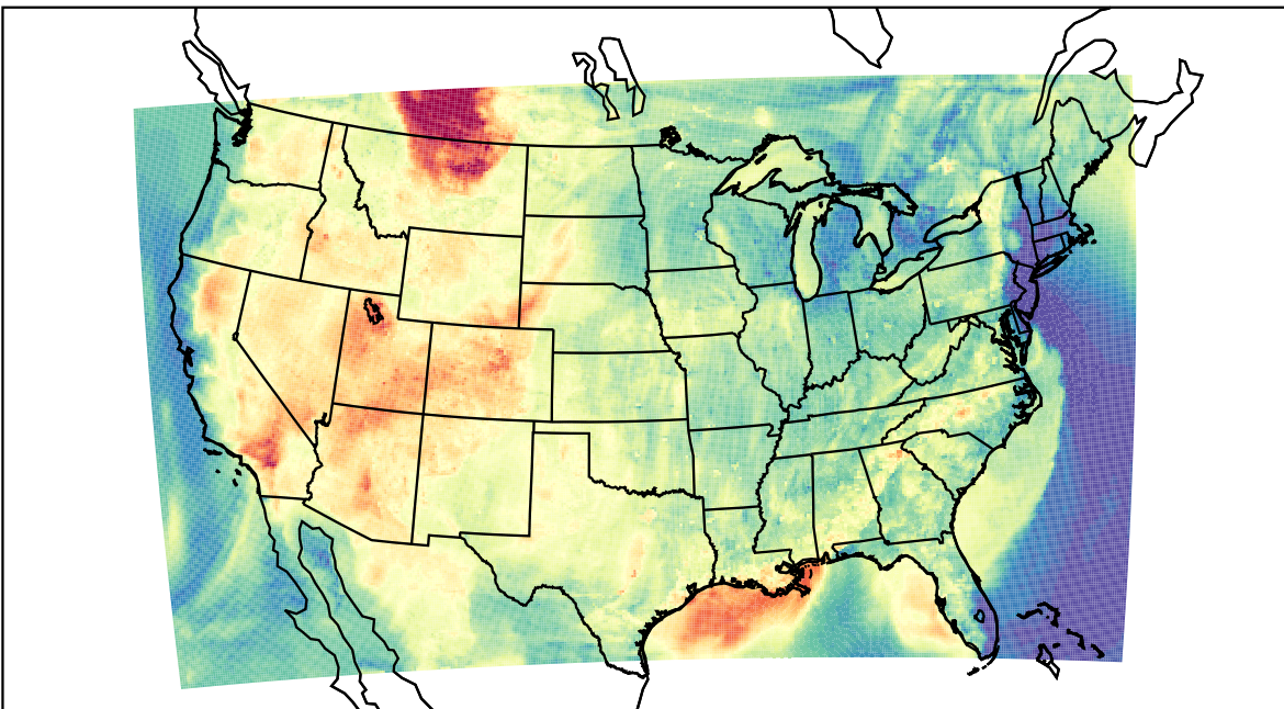
WRF (2023-05-21_01:00:00)
