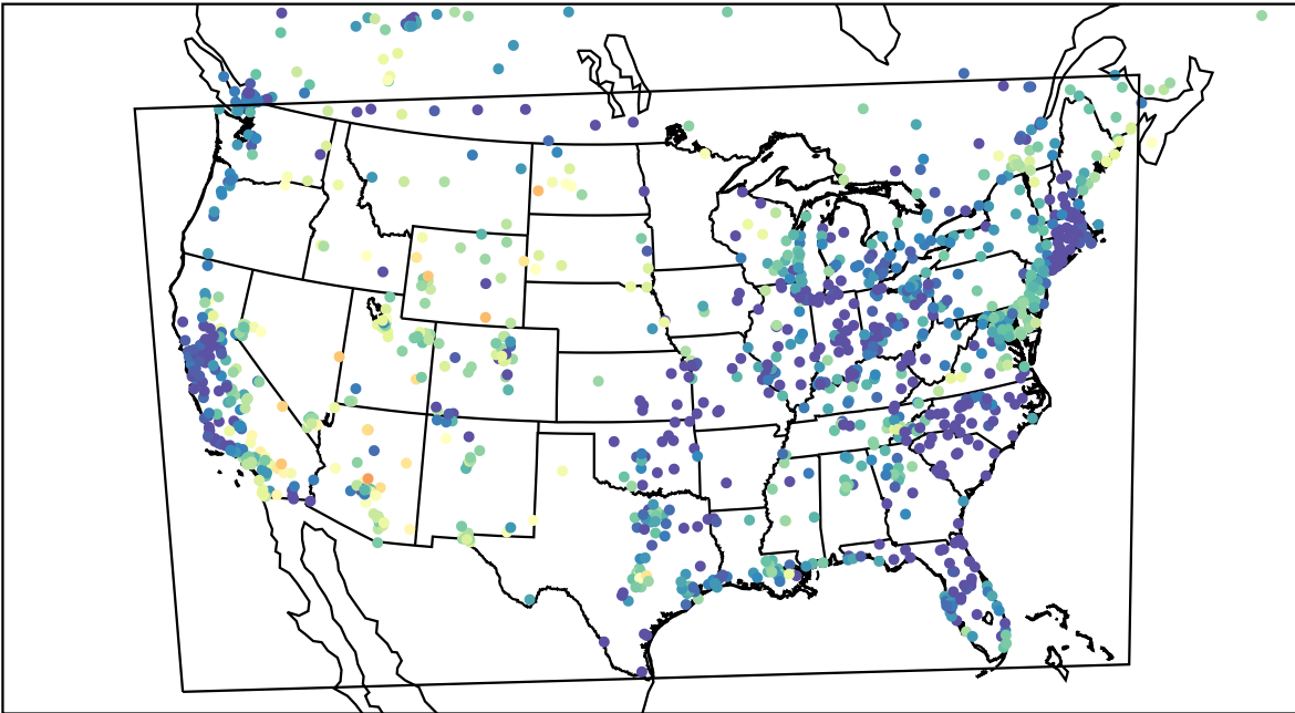
AirNOW (2023-05-21_06:00:00)
