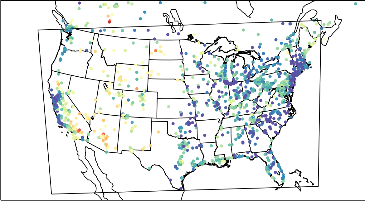
AirNOW (2023-05-21_03:00:00)
