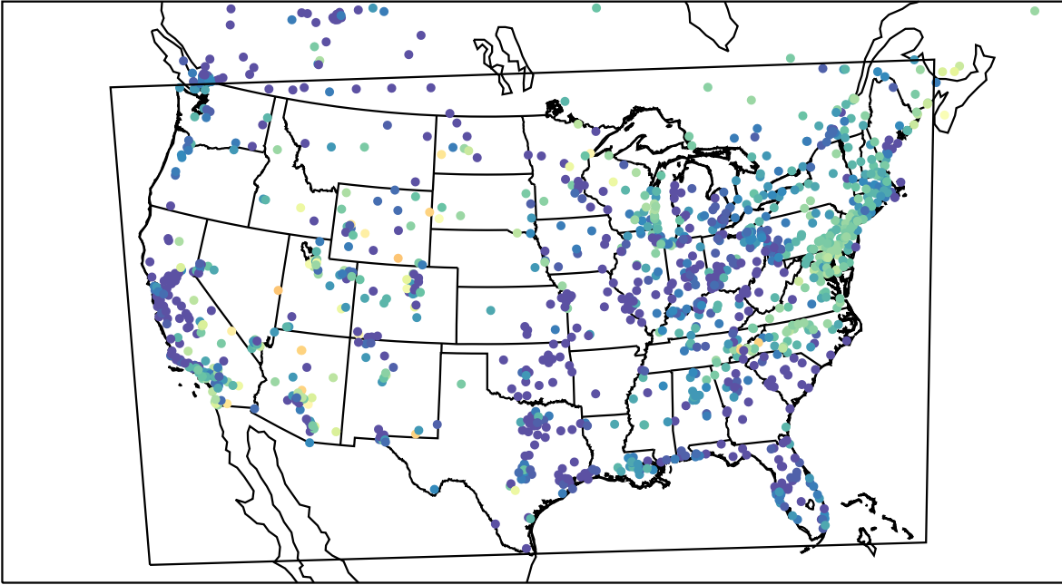
AirNOW (2023-05-21_12:00:00)
