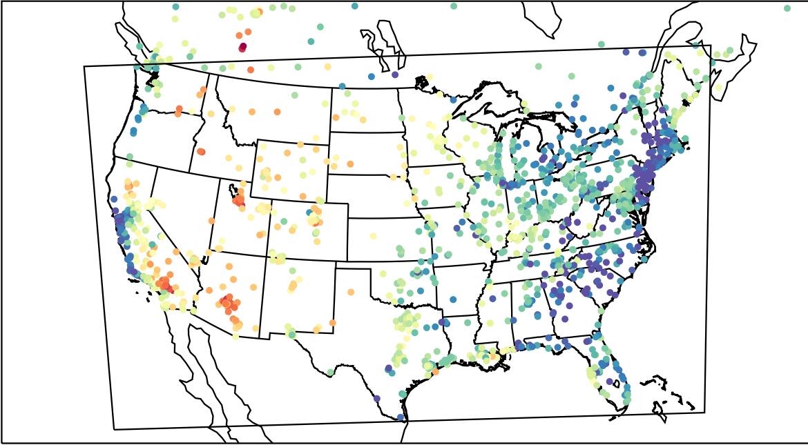
AirNOW (2023-05-21_01:00:00)
