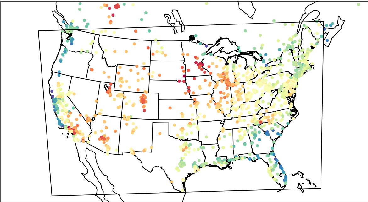
AirNOW (2023-05-21_21:00:00)
