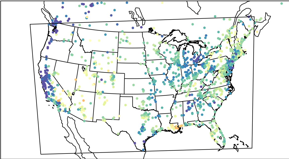
AirNOW (2023-05-20_15:00:00)
