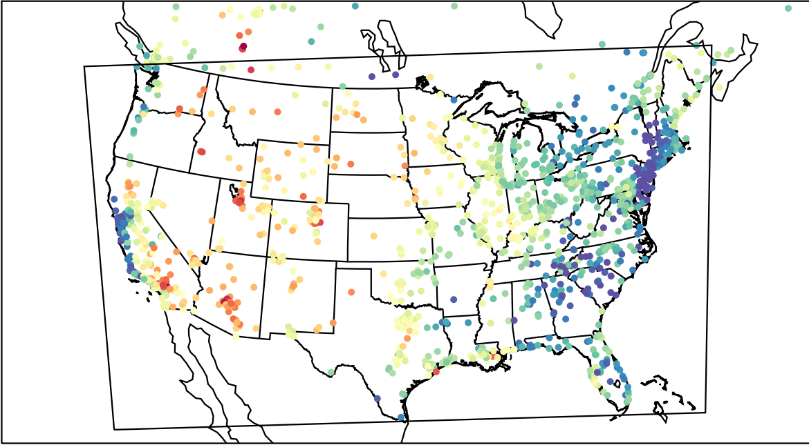
AirNOW (2023-05-21_00:00:00)
