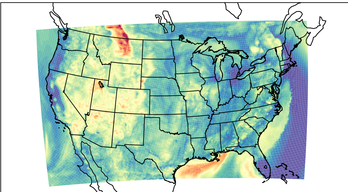
WRF (2023-05-21_07:00:00)
