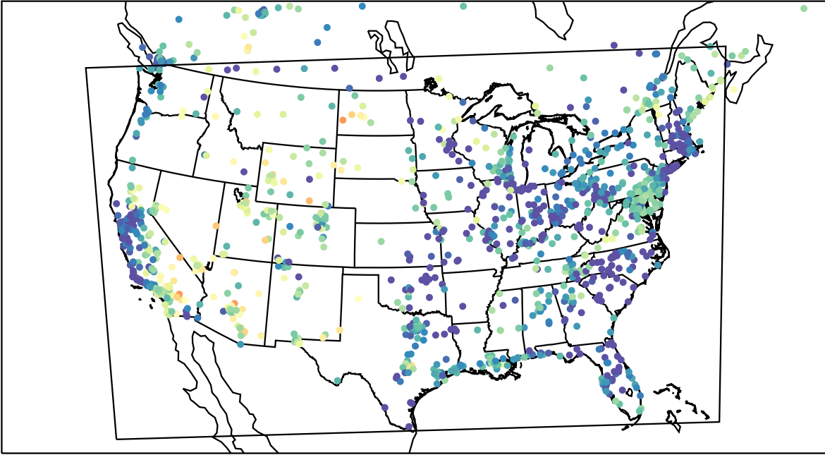
AirNOW (2023-05-21_05:00:00)
