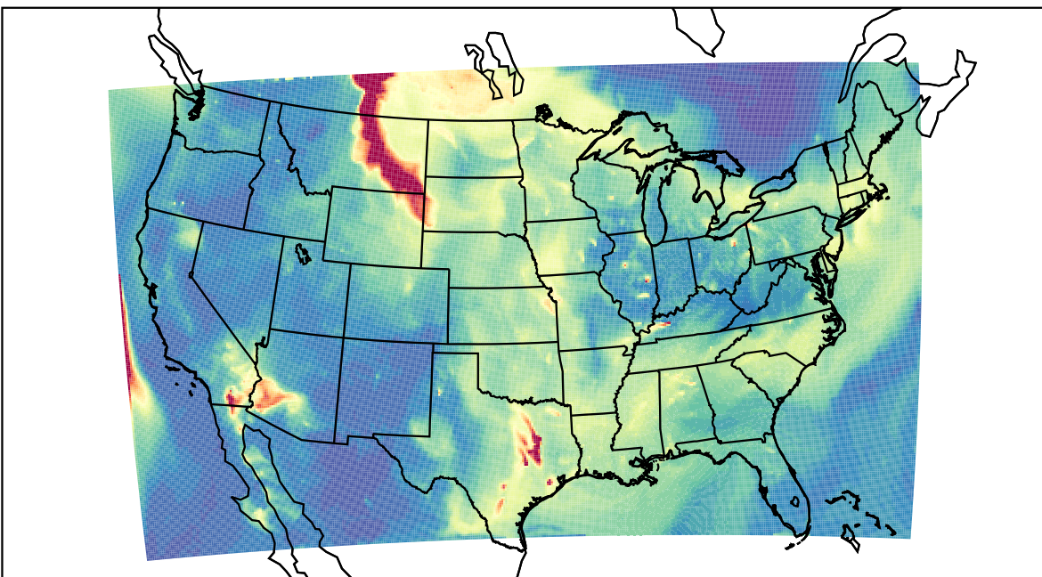
WRF 2023-05-22_08:00:00
