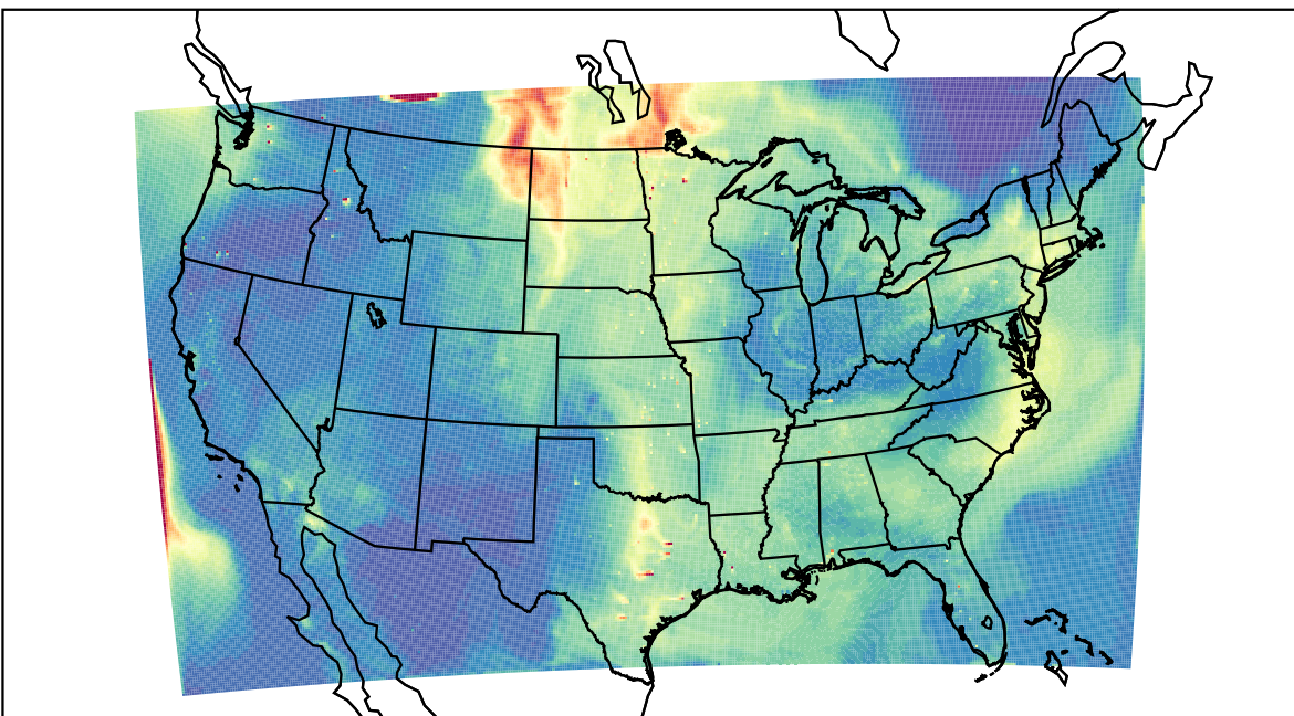
WRF 2023-05-22_21:00:00
