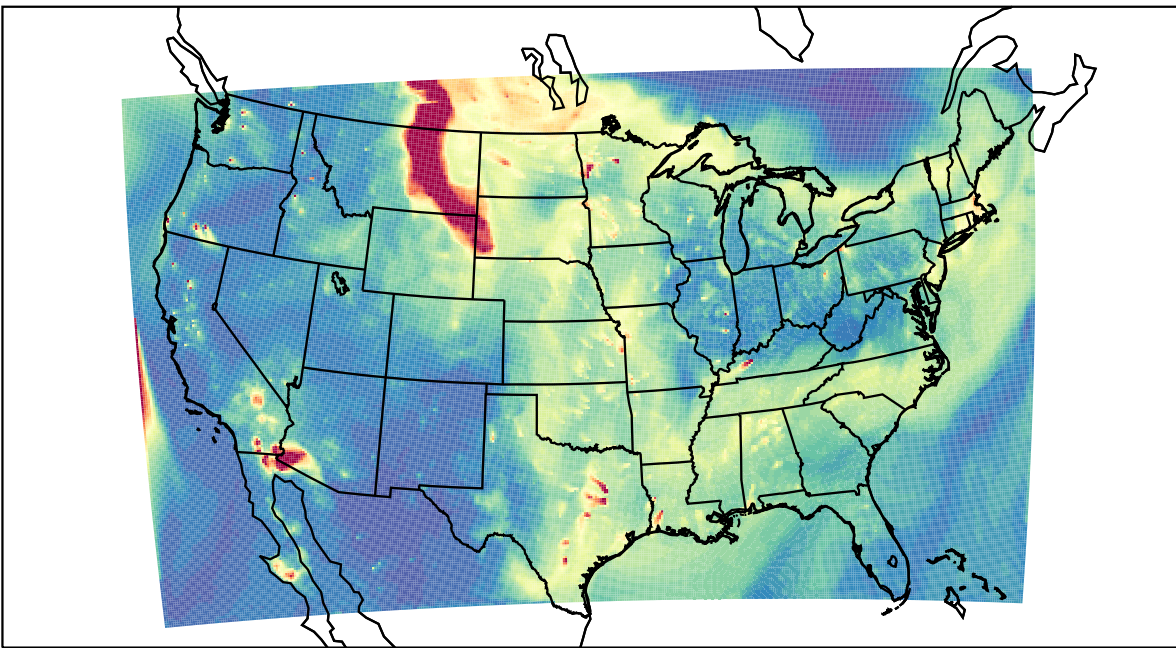
WRF 2023-05-22_03:00:00
