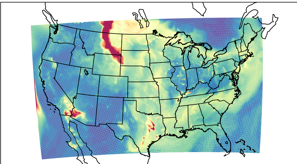
WRF 2023-05-22_06:00:00
