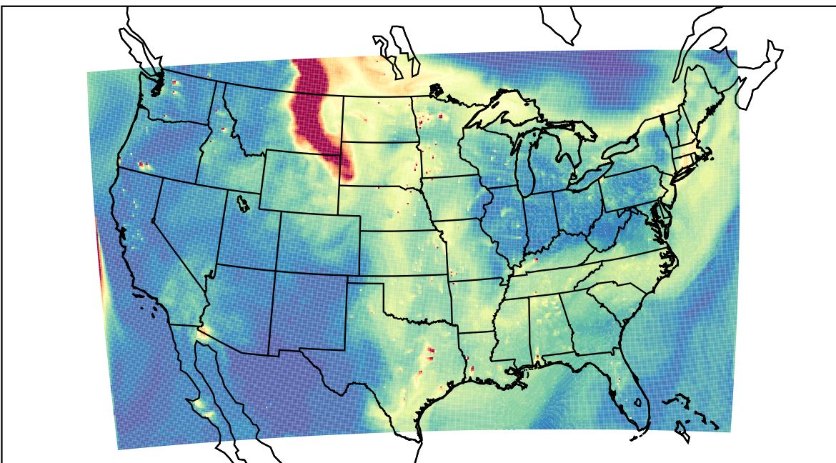
WRF 2023-05-22_00:00:00
