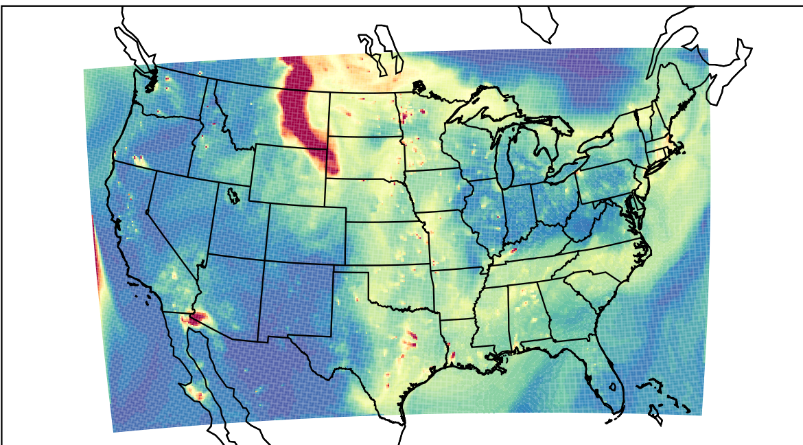
WRF 2023-05-22_02:00:00
