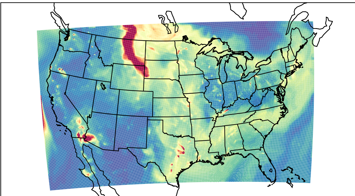
WRF 2023-05-22_04:00:00
