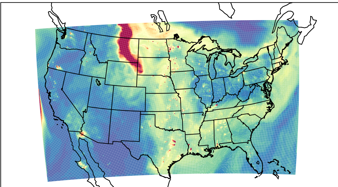
WRF 2023-05-22_01:00:00
