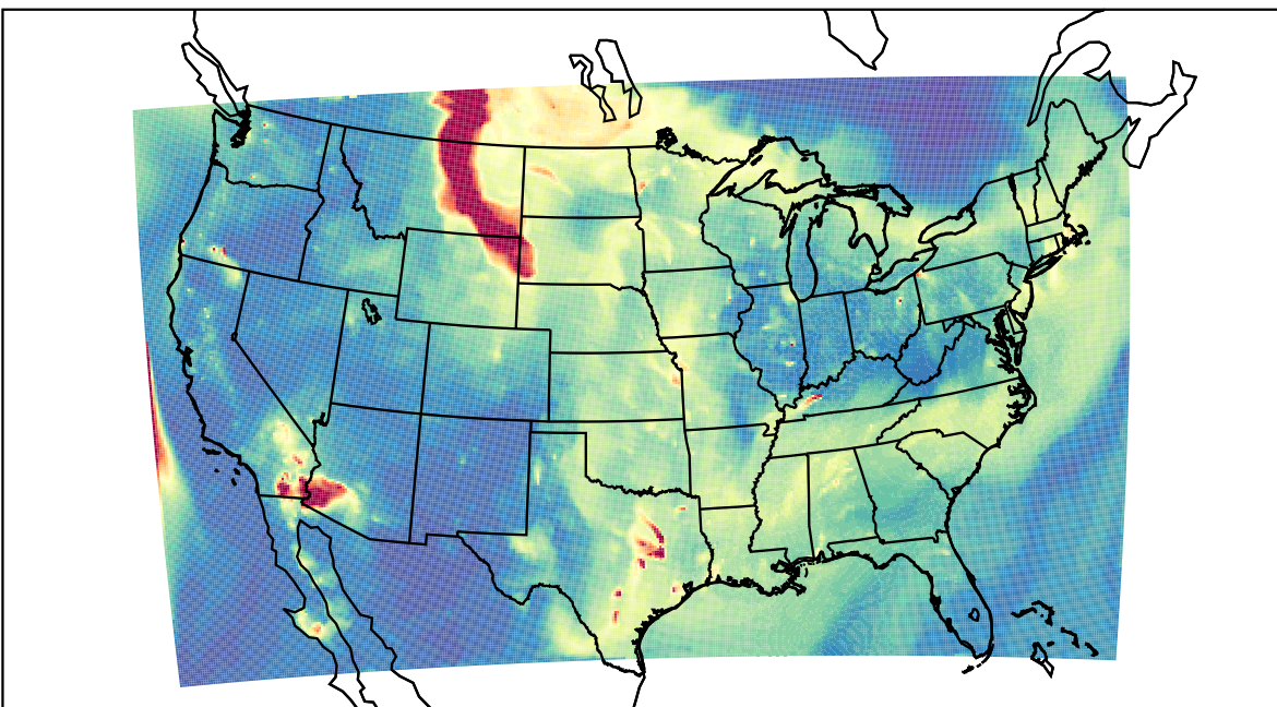
WRF 2023-05-22_05:00:00
