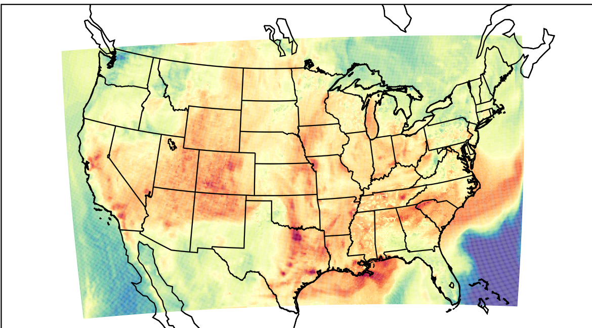
WRF (2023-05-22_22:00:00)
