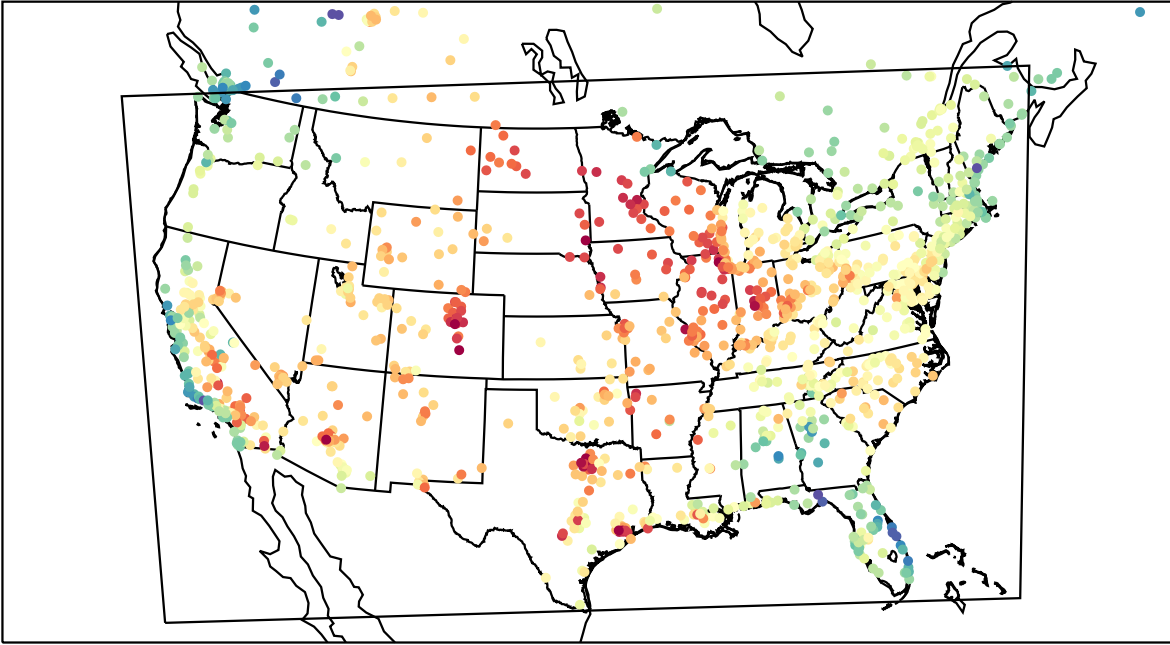
AirNOW (2023-05-22_20:00:00)
