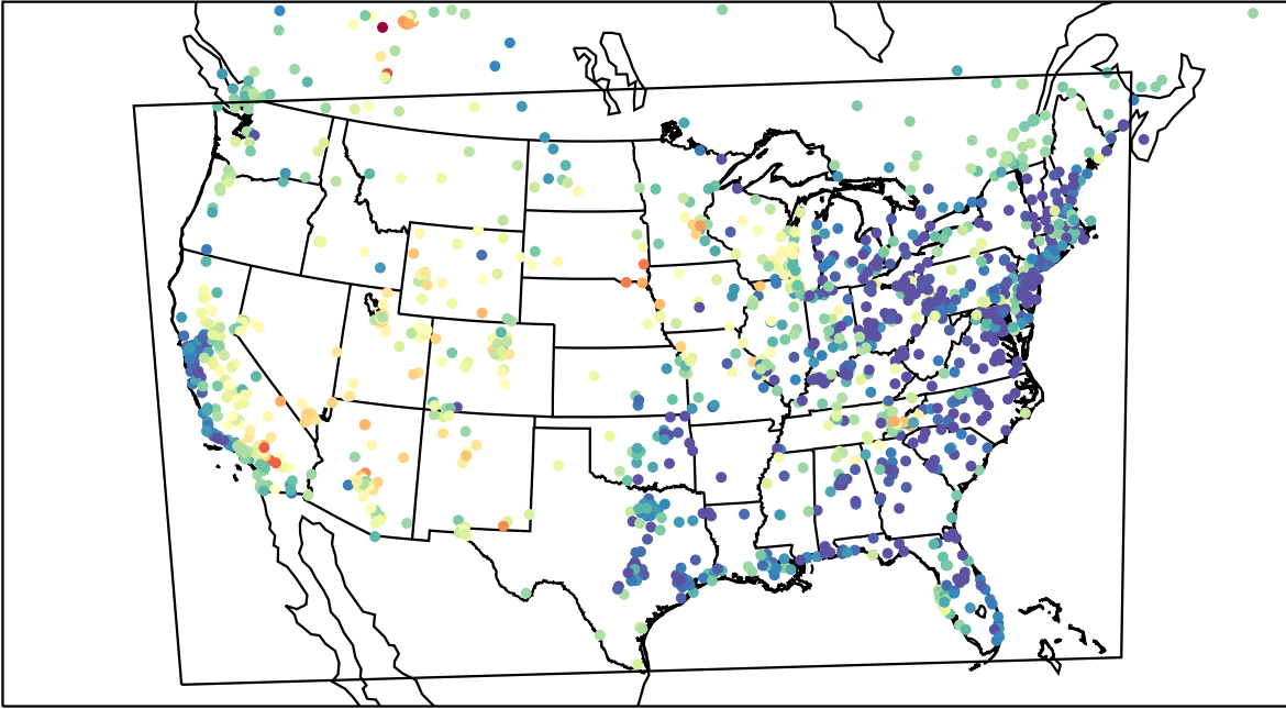
AirNOW (2023-05-22_03:00:00)
