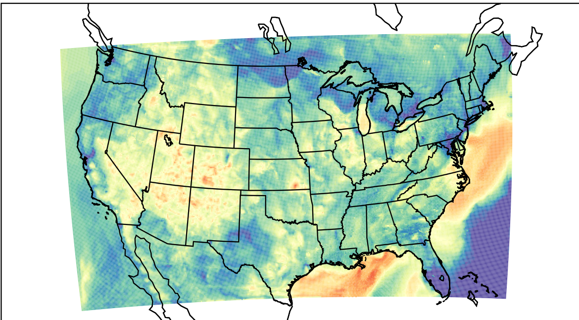
WRF (2023-05-22_07:00:00)
