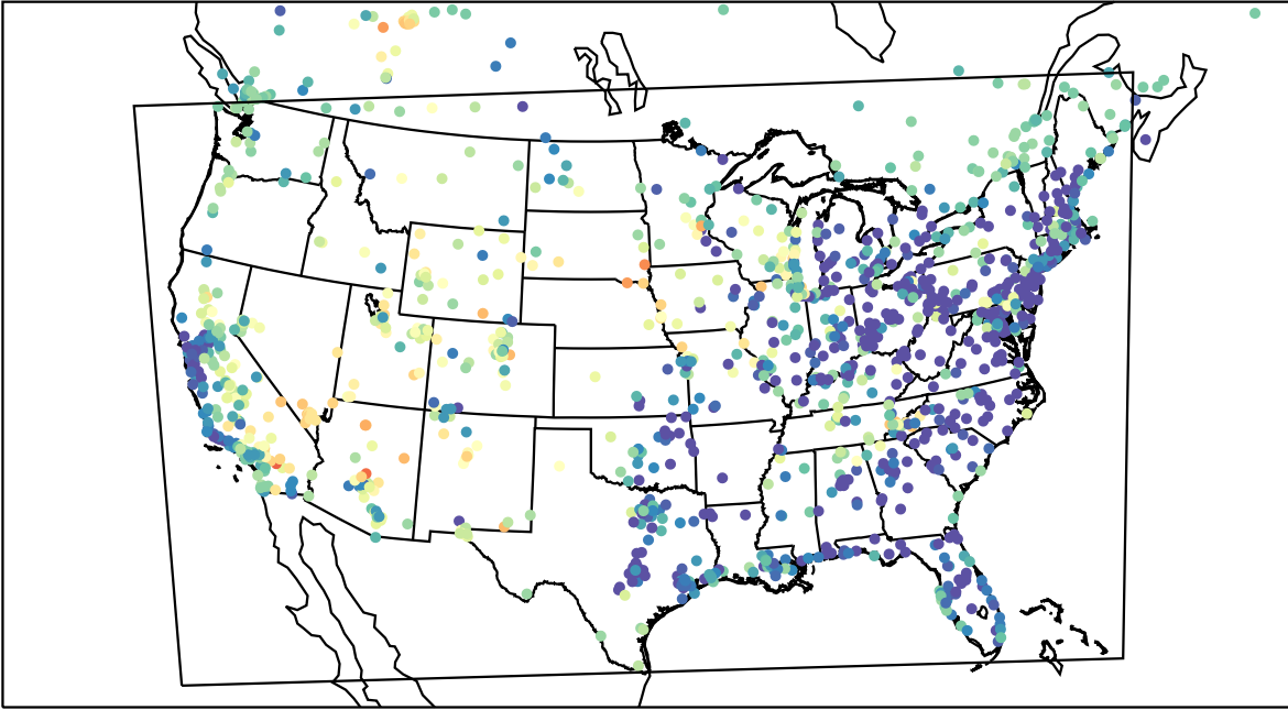
AirNOW (2023-05-22_04:00:00)
