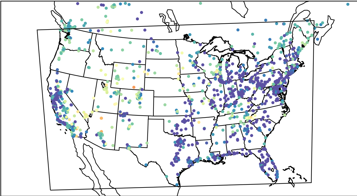
AirNOW (2023-05-22_08:00:00)
