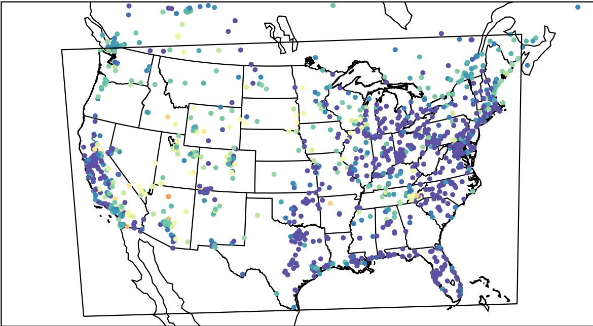
AirNOW (2023-05-22_09:00:00)
