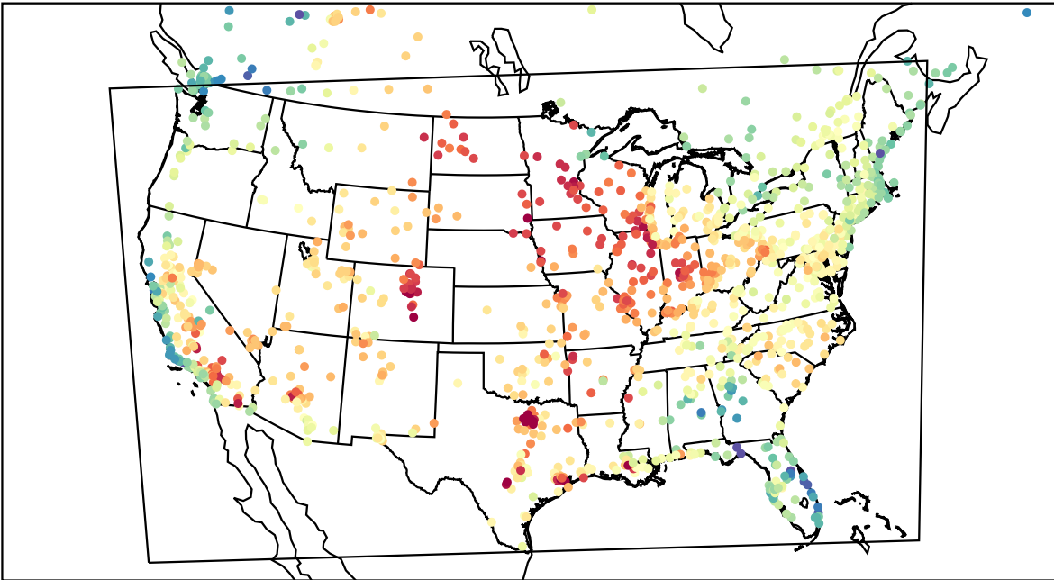
AirNOW (2023-05-22_21:00:00)
