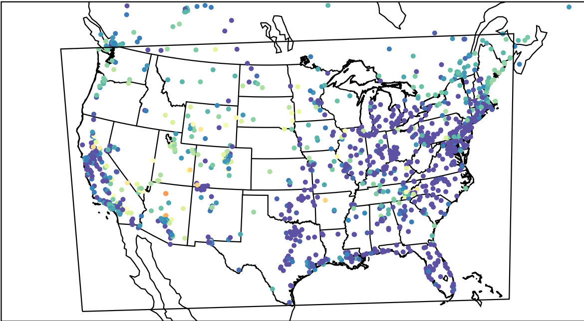
AirNOW (2023-05-22_10:00:00)
