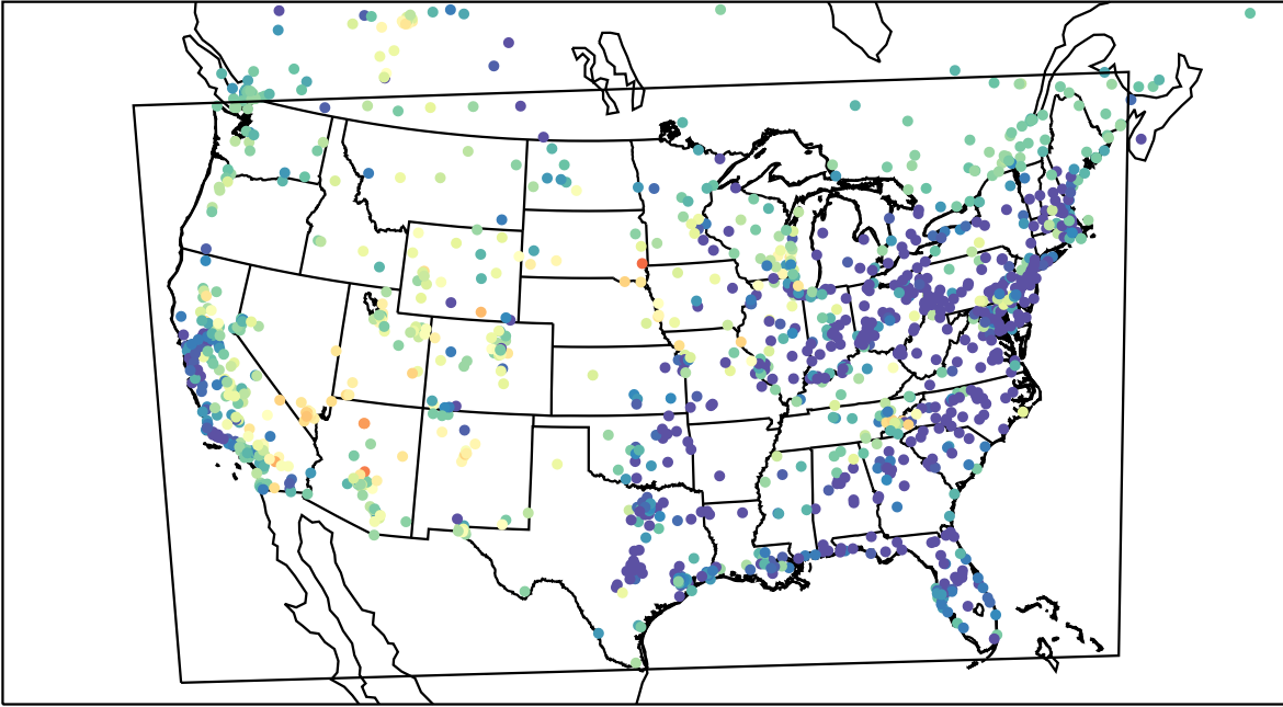
AirNOW (2023-05-22_05:00:00)
