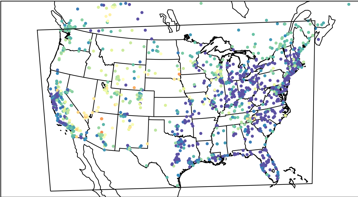
AirNOW (2023-05-22_06:00:00)
