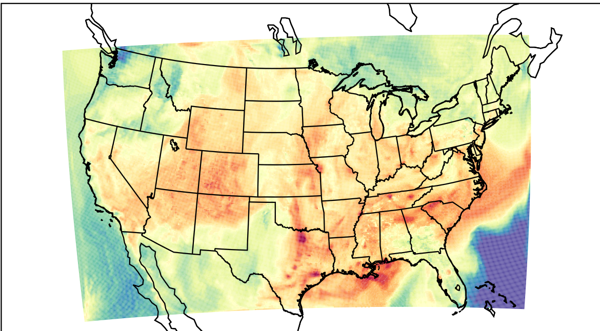
WRF (2023-05-22_19:00:00)
