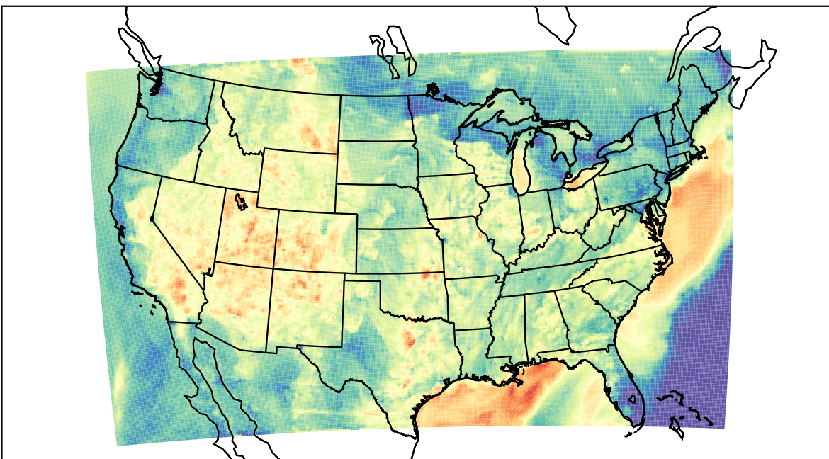
WRF (2023-05-22_03:00:00)
