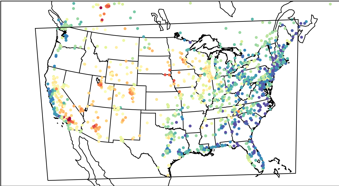
AirNOW (2023-05-22_01:00:00)
