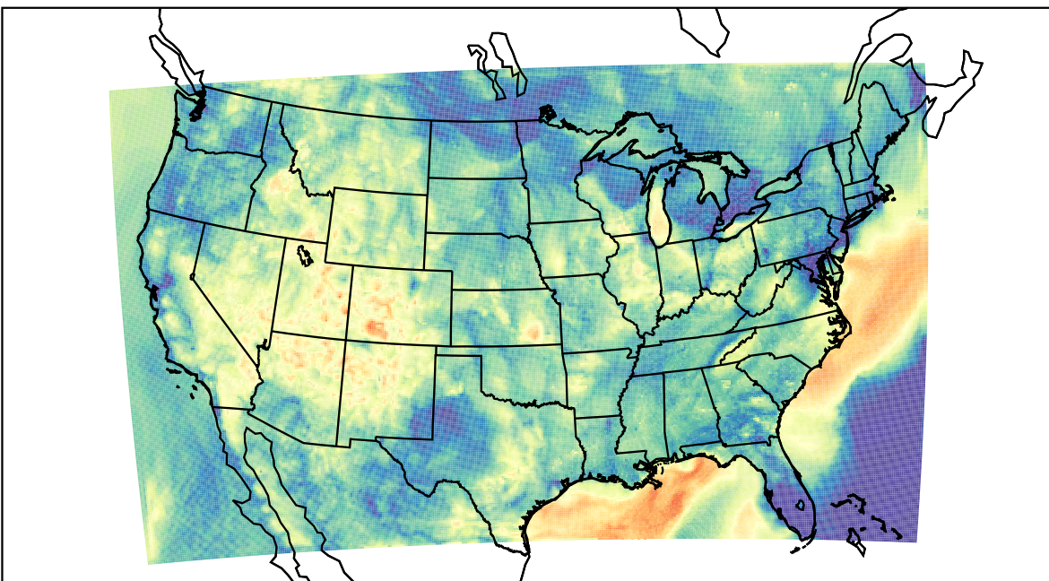
WRF (2023-05-22_09:00:00)
