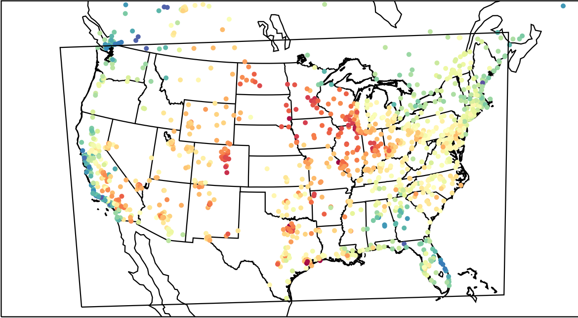
AirNOW (2023-05-22_19:00:00)
