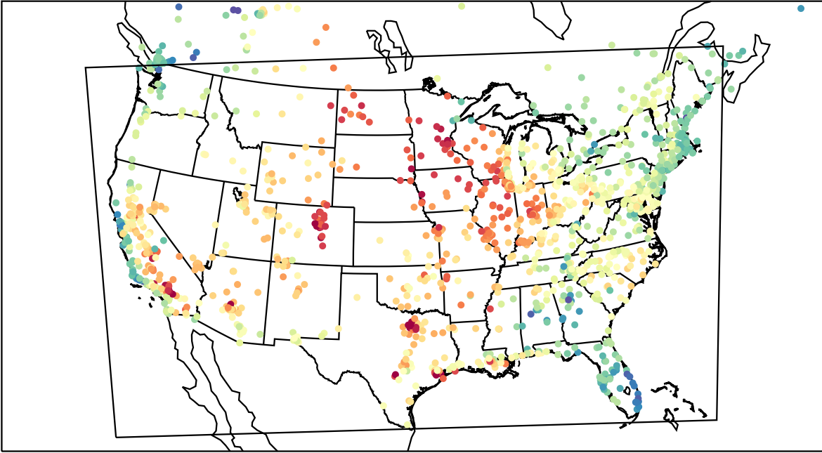
AirNOW (2023-05-22_23:00:00)
