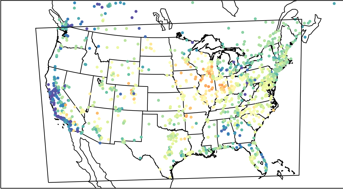
AirNOW (2023-05-22_15:00:00)
