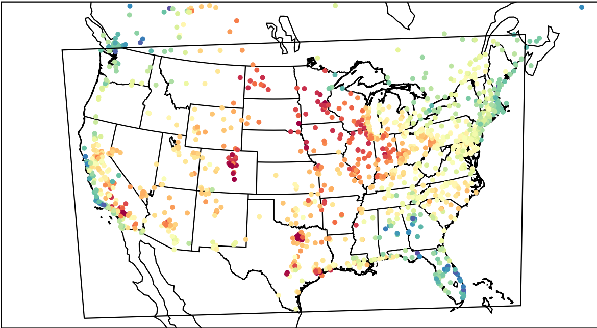
AirNOW (2023-05-22_22:00:00)
