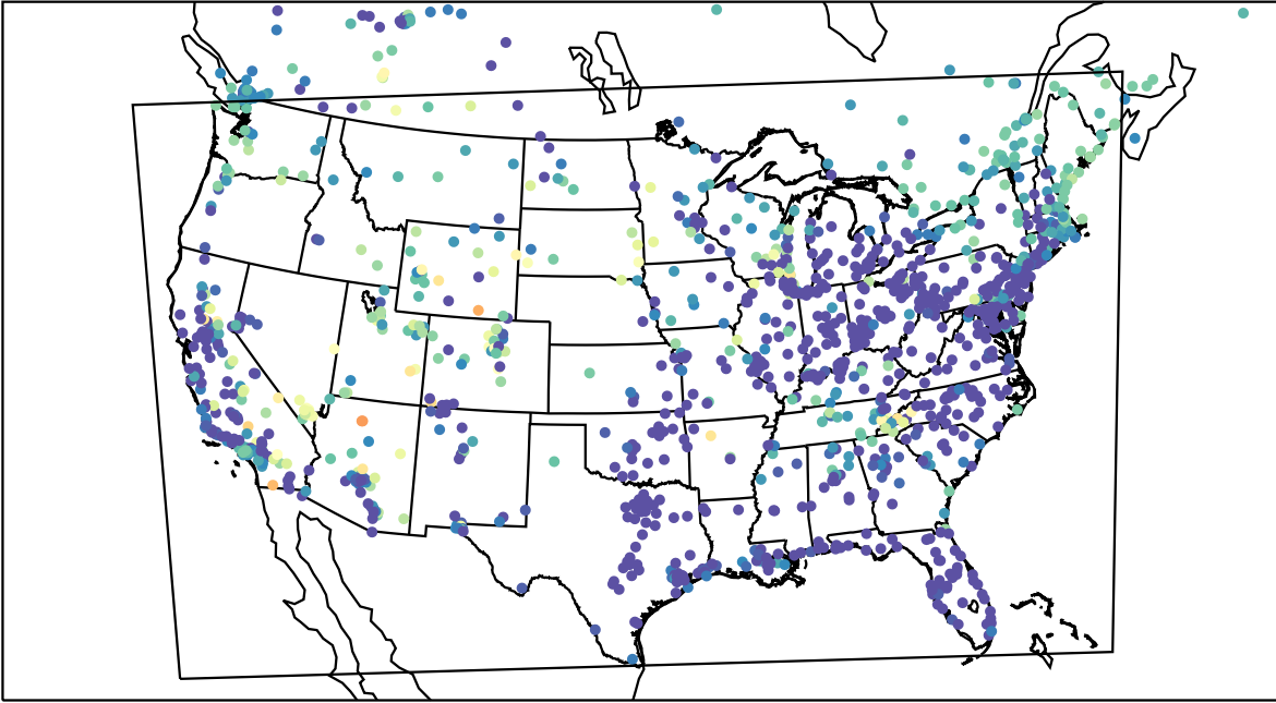
AirNOW (2023-05-22_11:00:00)
