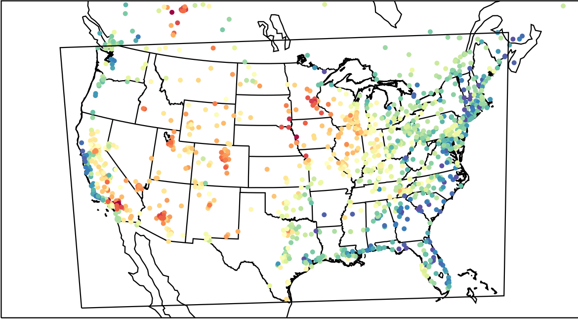
AirNOW (2023-05-22_00:00:00)
