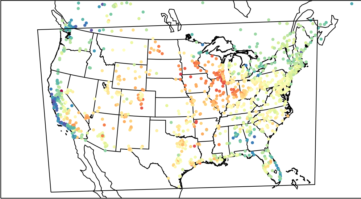
AirNOW (2023-05-22_17:00:00)
