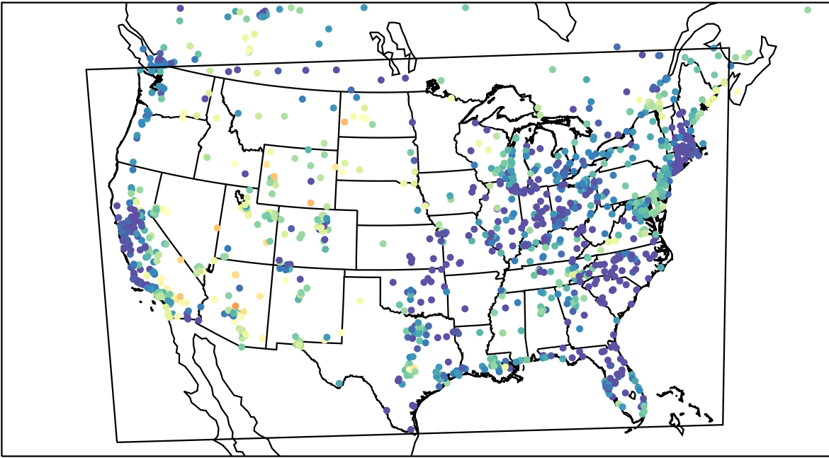
AirNOW (2023-05-21_06:00:00)
