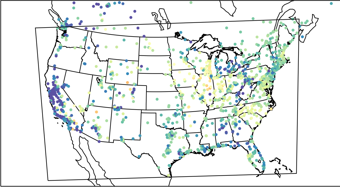
AirNOW (2023-05-22_14:00:00)
