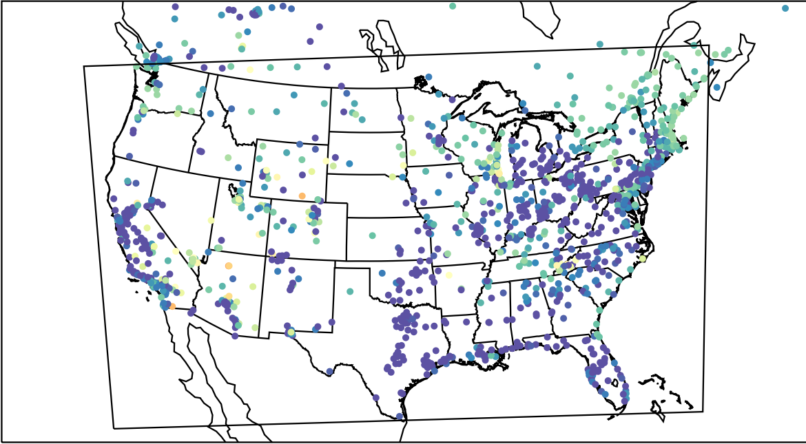
AirNOW (2023-05-22_12:00:00)
