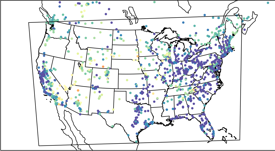
AirNOW (2023-05-22_07:00:00)
