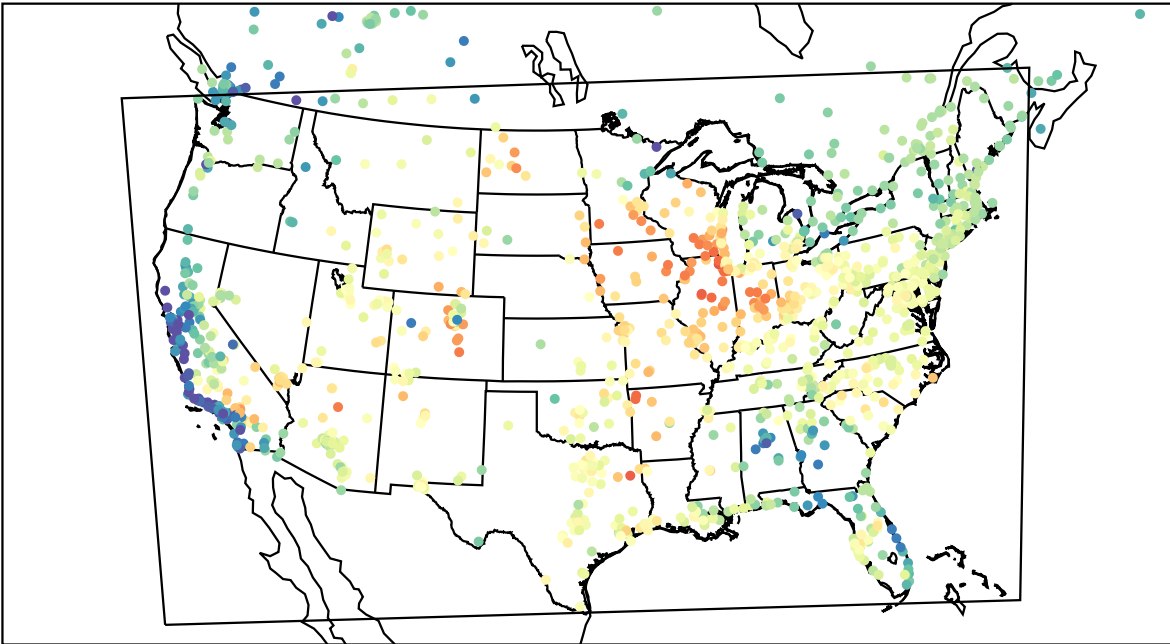
AirNOW (2023-05-22_16:00:00)
