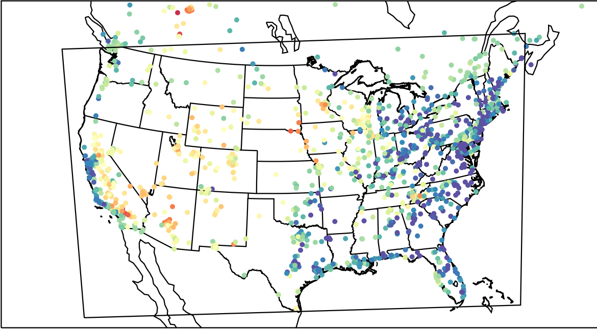
AirNOW (2023-05-22_02:00:00)
