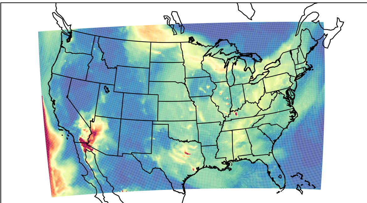
WRF 2023-05-24_10:00:00
