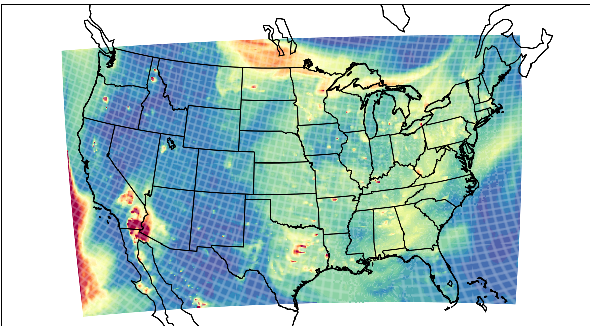
WRF 2023-05-24_03:00:00
