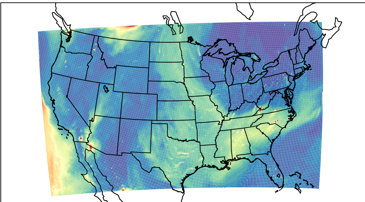
WRF 2023-05-25_23:00:00
