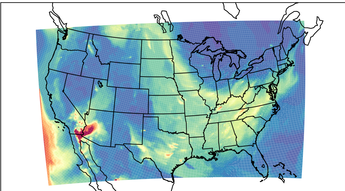
WRF 2023-05-25_08:00:00
