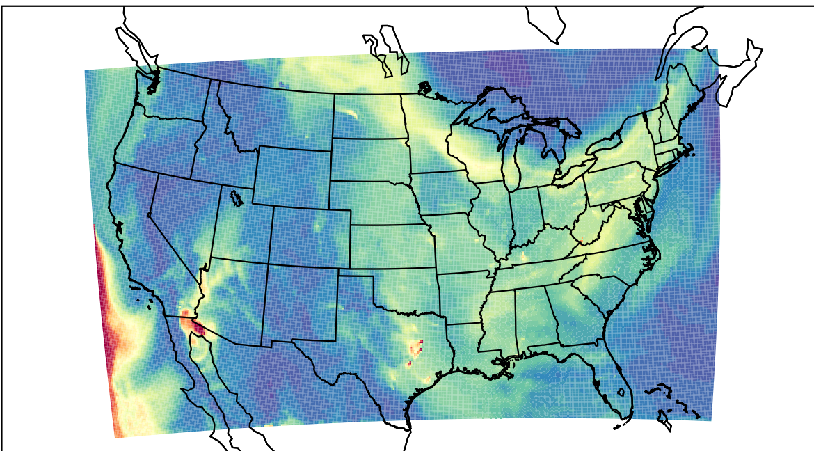
WRF 2023-05-24_17:00:00
