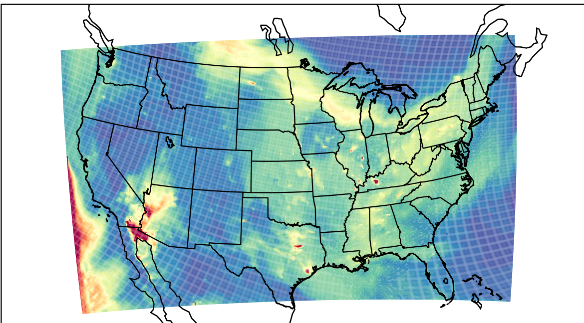
WRF 2023-05-24_13:00:00
