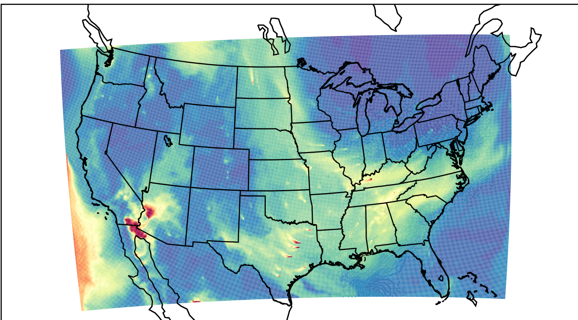
WRF 2023-05-25_14:00:00
