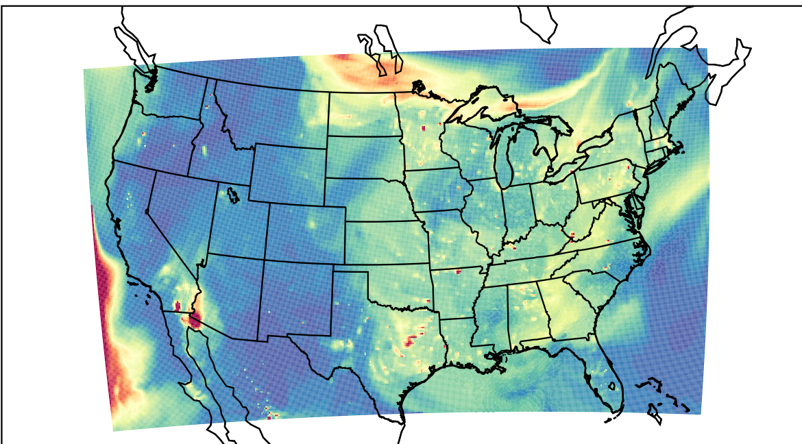
WRF 2023-05-24_01:00:00
