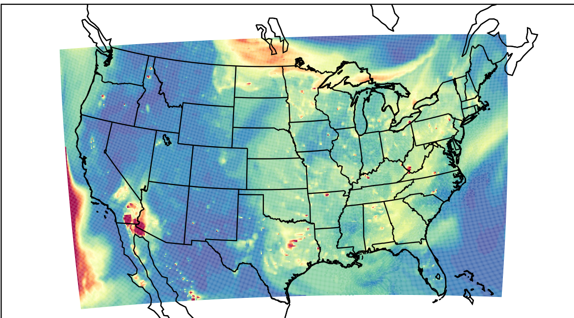
WRF 2023-05-24_02:00:00
