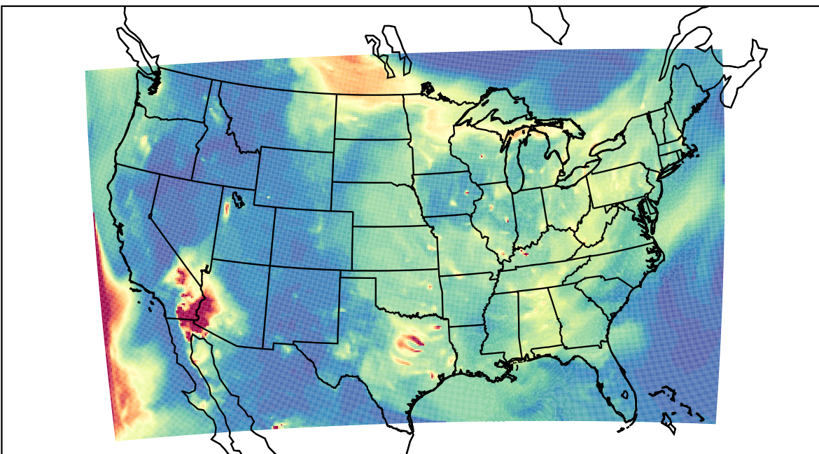
WRF 2023-05-24_06:00:00
