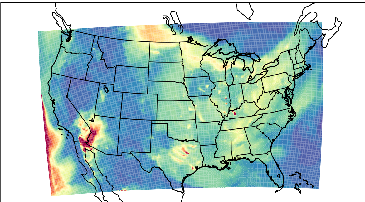
WRF 2023-05-24_09:00:00
