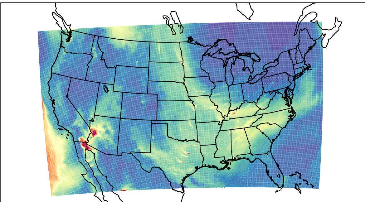
WRF 2023-05-25_15:00:00
