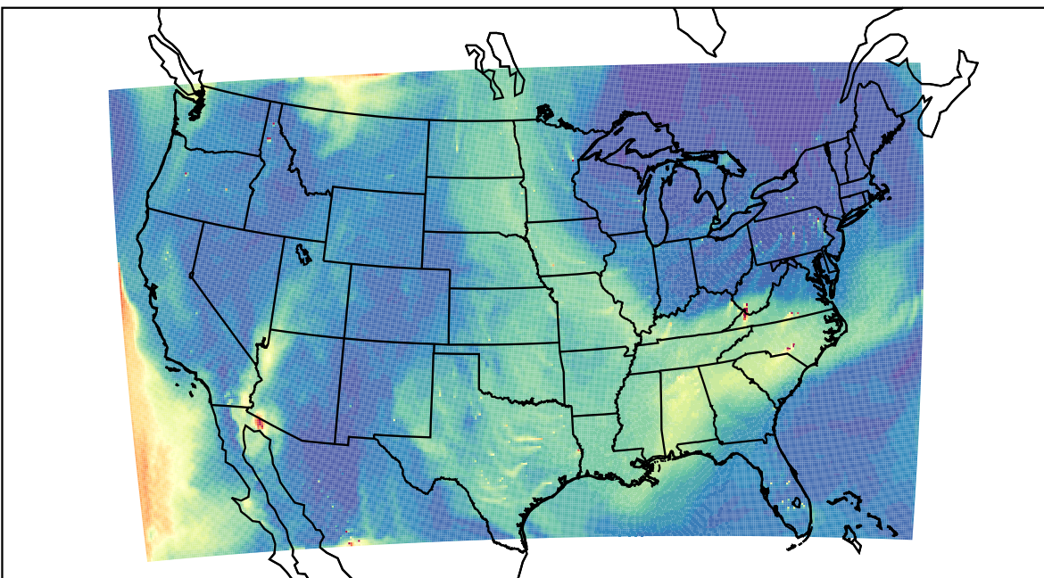
WRF 2023-05-25_21:00:00
