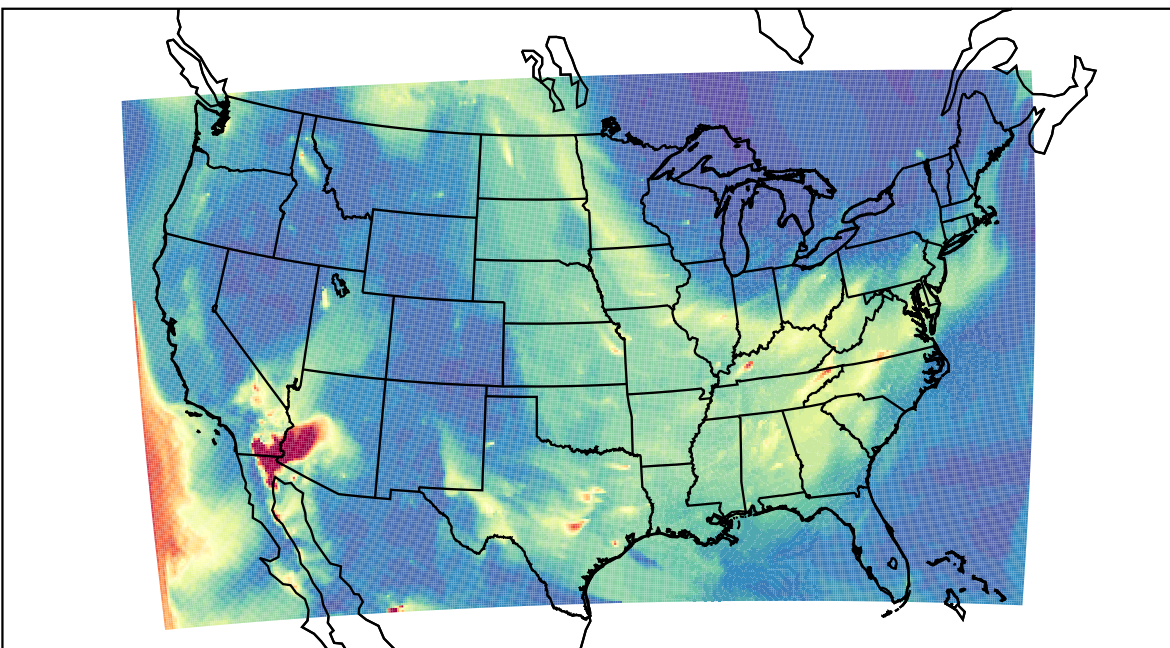
WRF 2023-05-25_07:00:00
