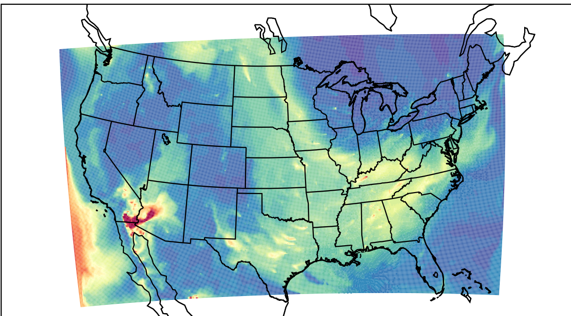
WRF 2023-05-25_10:00:00
