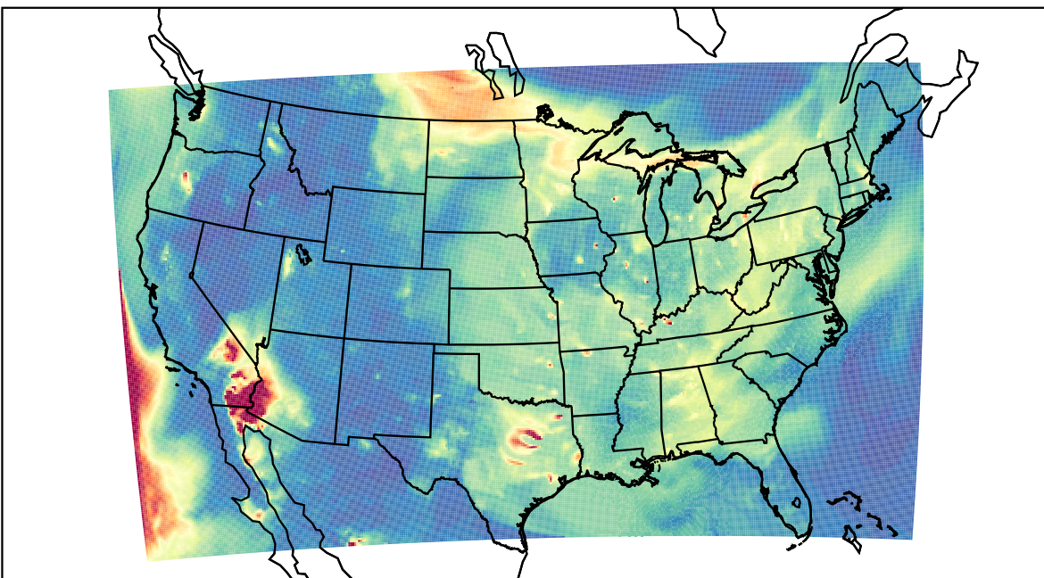
WRF 2023-05-24_05:00:00
