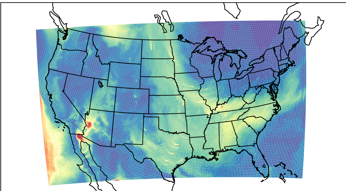
WRF 2023-05-25_16:00:00
