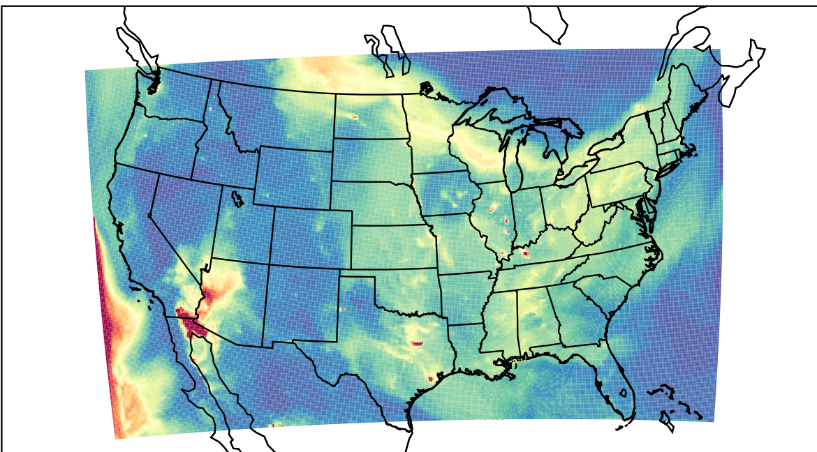
WRF 2023-05-24_12:00:00
