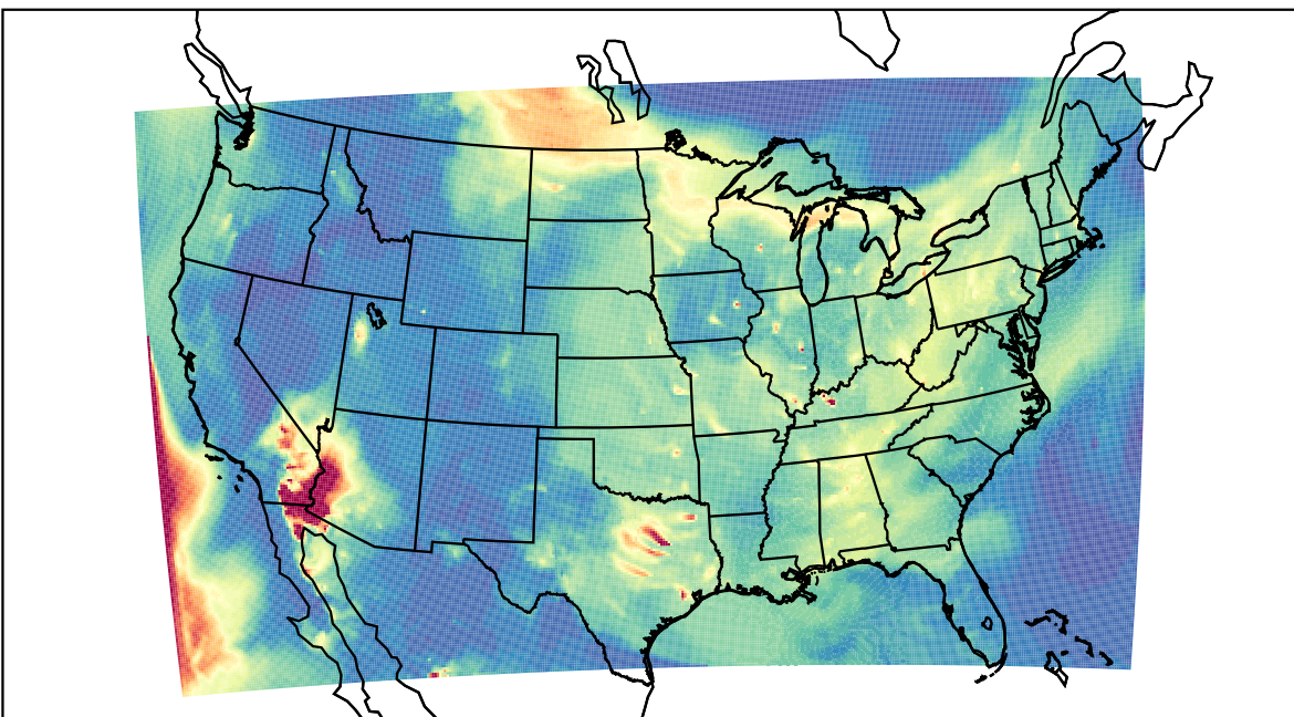
WRF 2023-05-24_07:00:00
