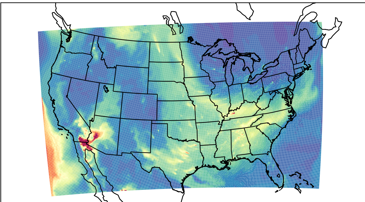
WRF 2023-05-25_12:00:00
