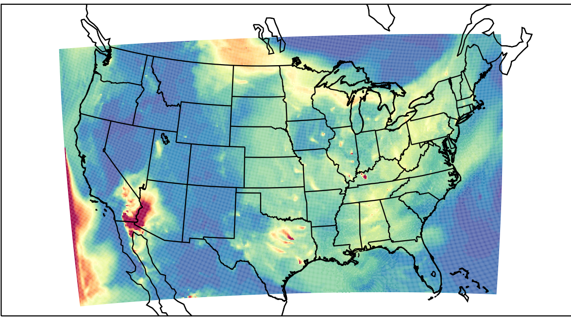
WRF 2023-05-24_08:00:00
