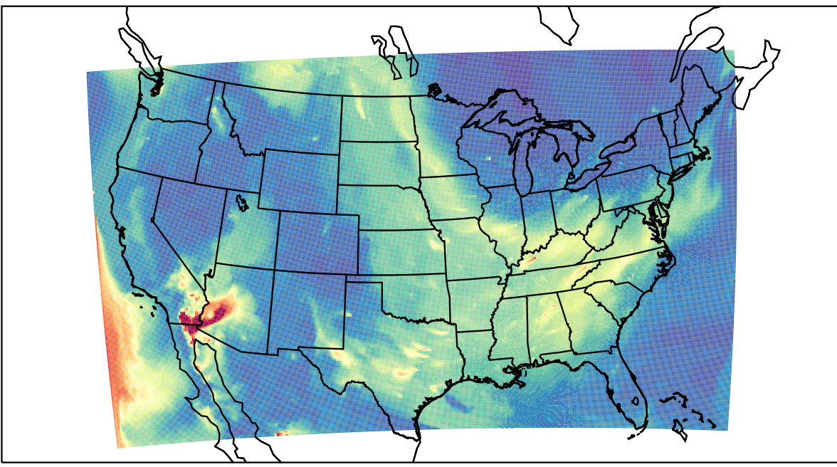
WRF 2023-05-25_09:00:00
