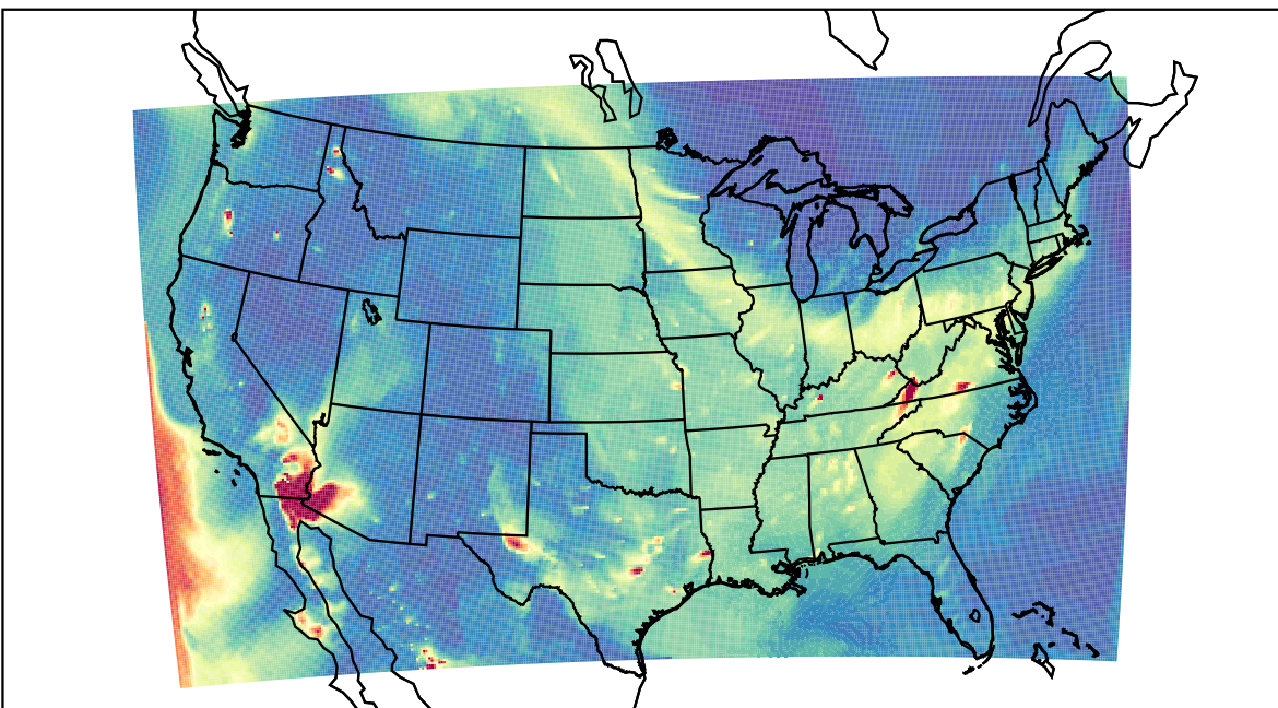
WRF 2023-05-25_03:00:00
