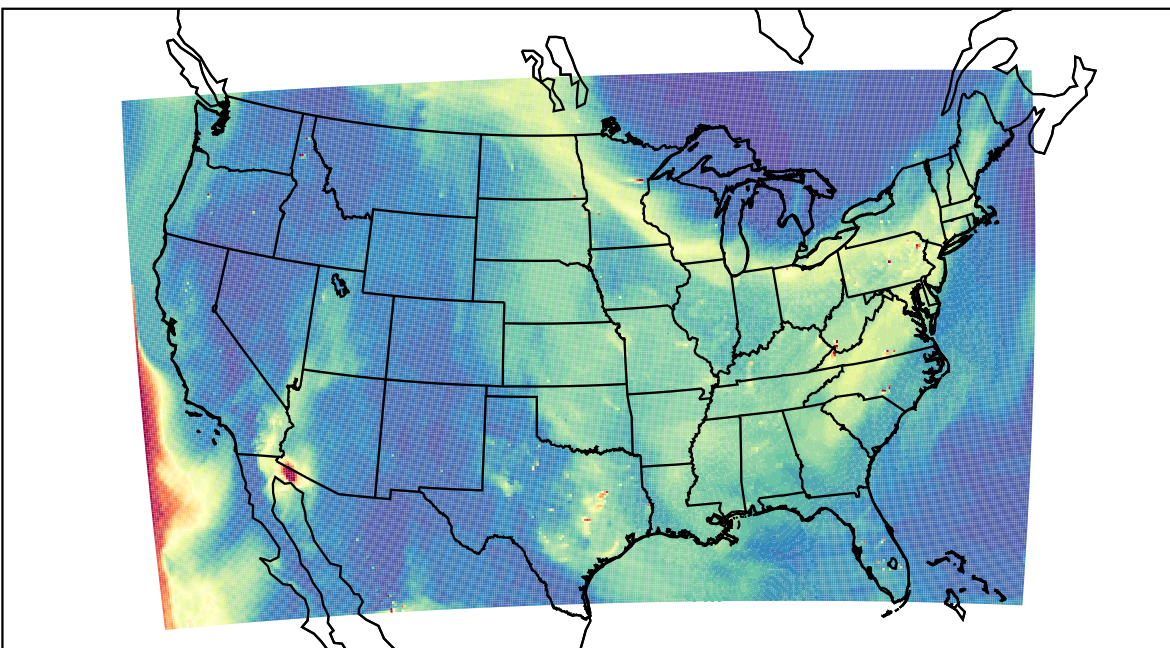
WRF 2023-05-24_21:00:00
