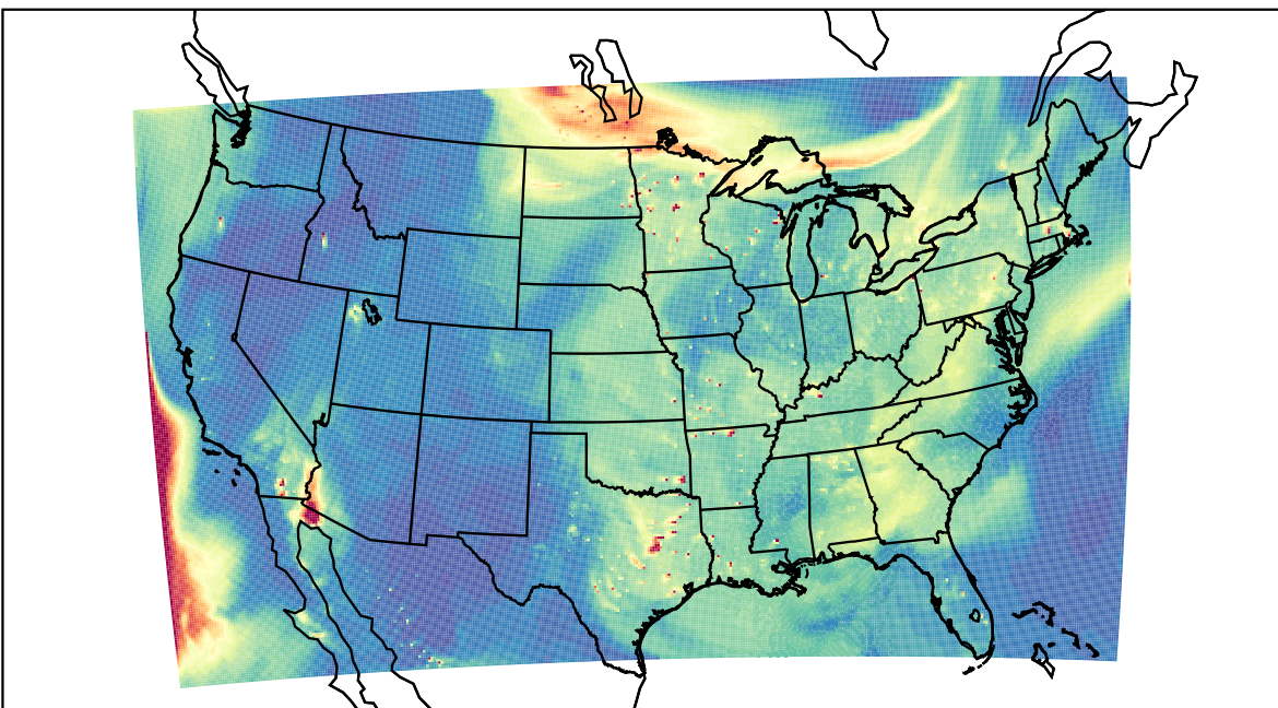
WRF 2023-05-24_00:00:00
