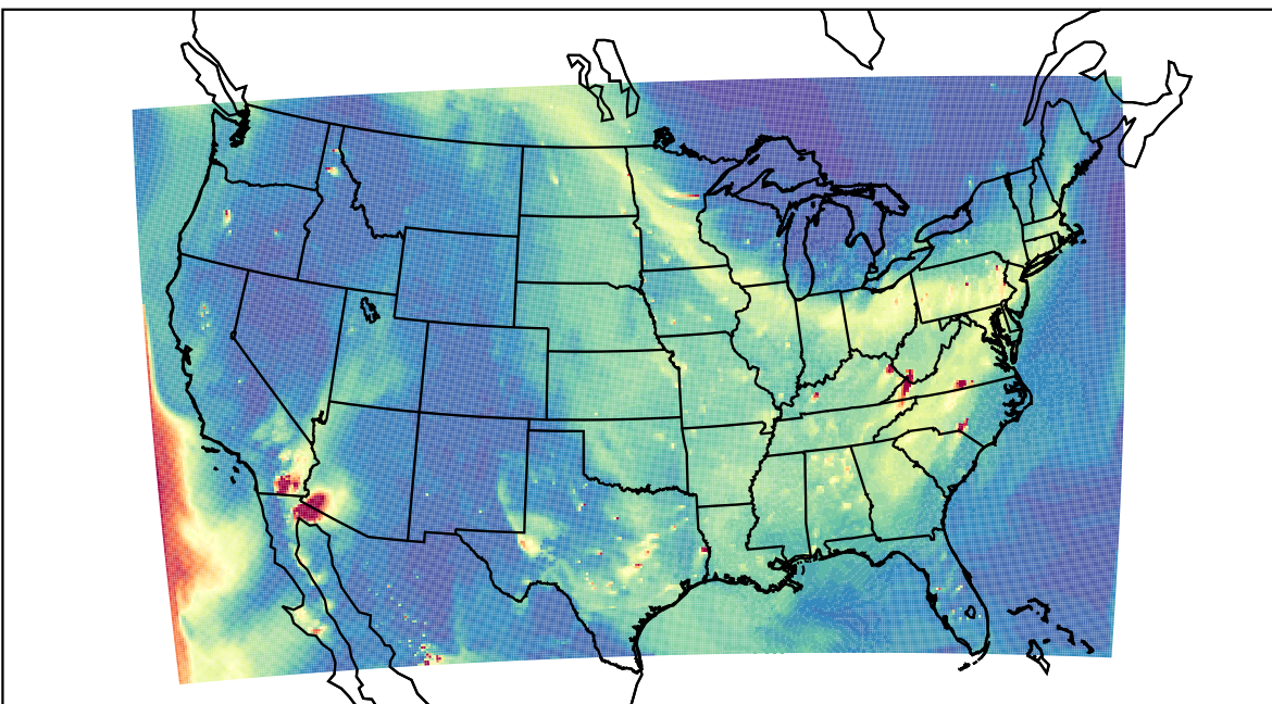
WRF 2023-05-25_01:00:00
