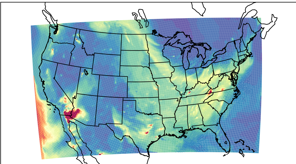
WRF 2023-05-25_05:00:00
