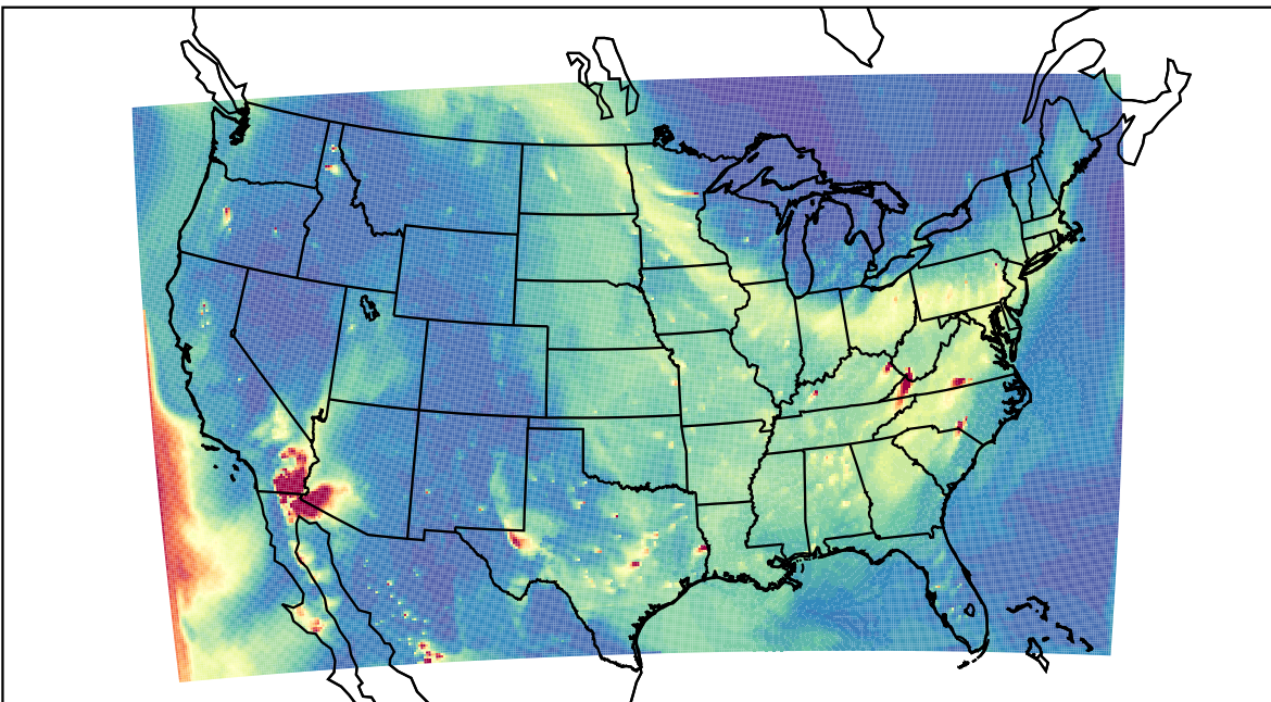
WRF 2023-05-25_02:00:00
