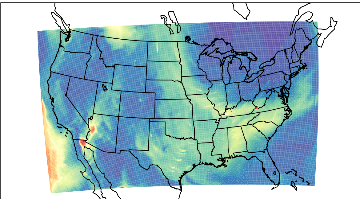
WRF 2023-05-25_17:00:00
