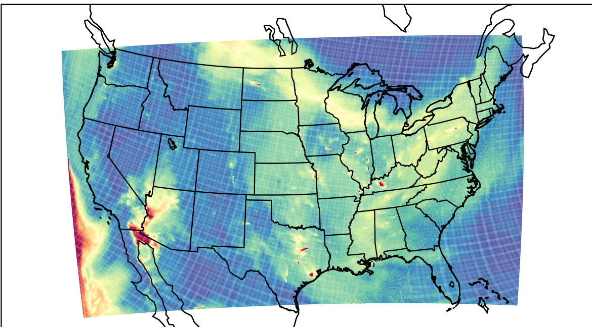
WRF 2023-05-24_14:00:00
