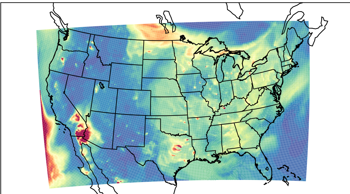
WRF 2023-05-24_04:00:00
