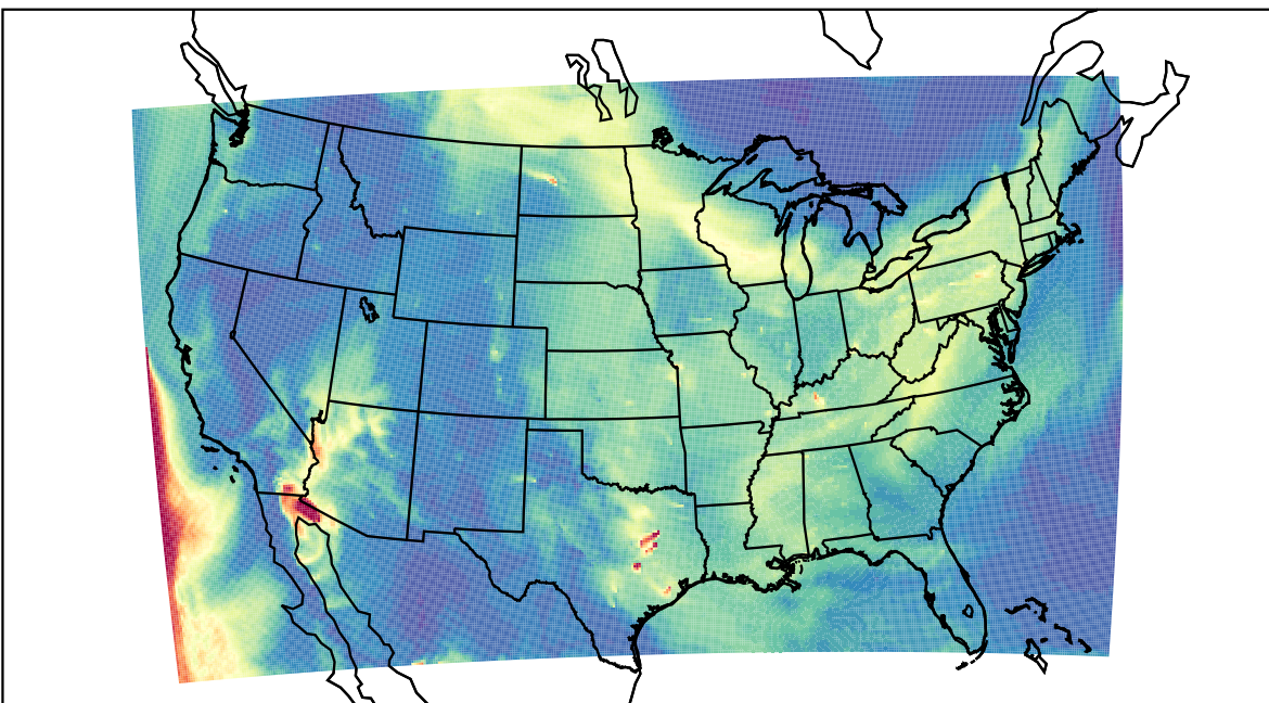
WRF 2023-05-24_16:00:00
