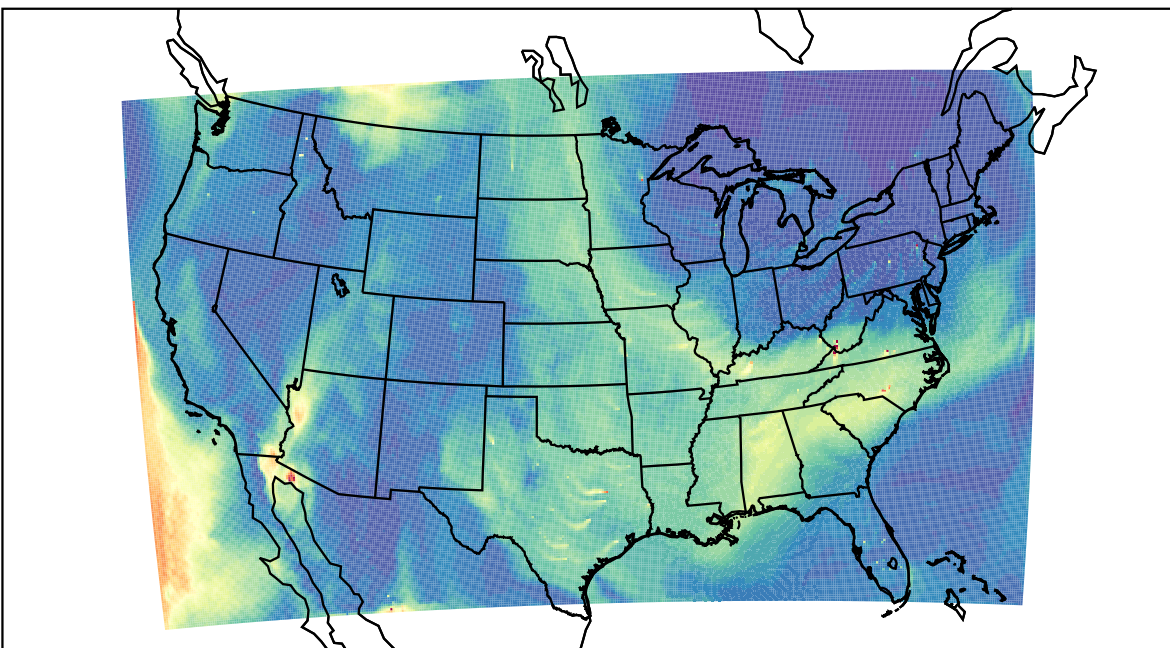
WRF 2023-05-25_19:00:00
