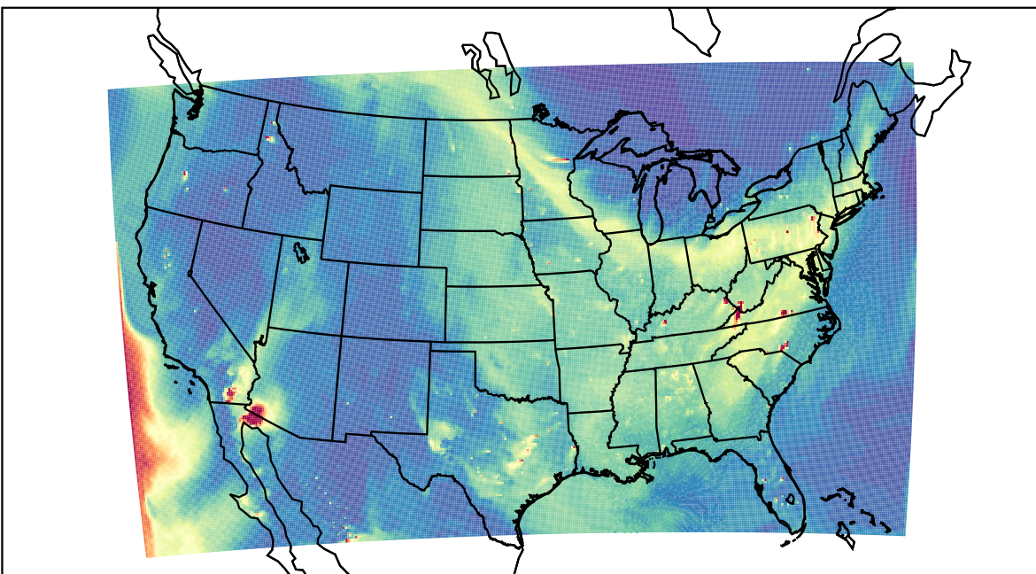
WRF 2023-05-25_00:00:00
