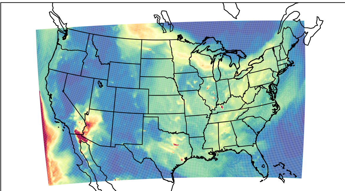
WRF 2023-05-24_11:00:00
