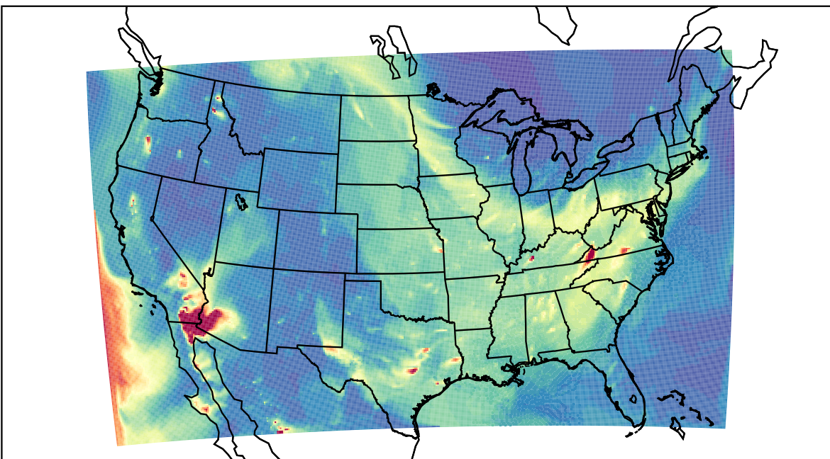
WRF 2023-05-25_04:00:00
