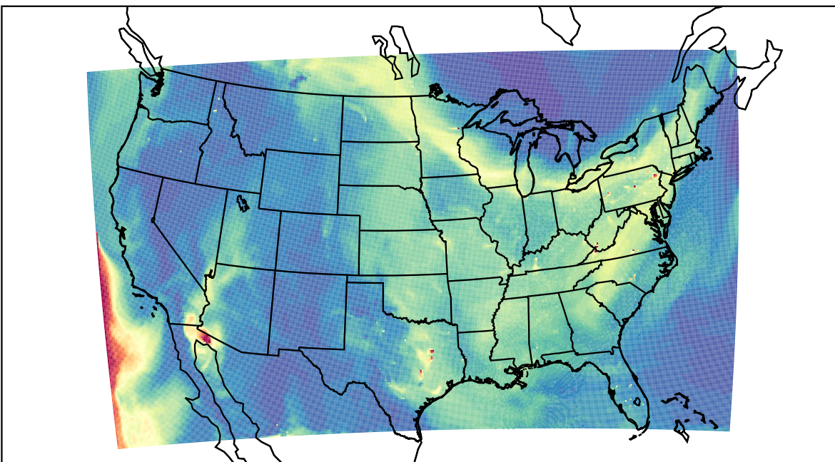
WRF 2023-05-24_19:00:00
