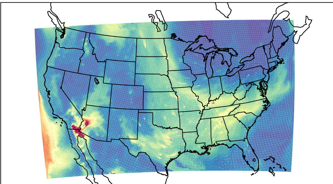
WRF 2023-05-25_13:00:00
