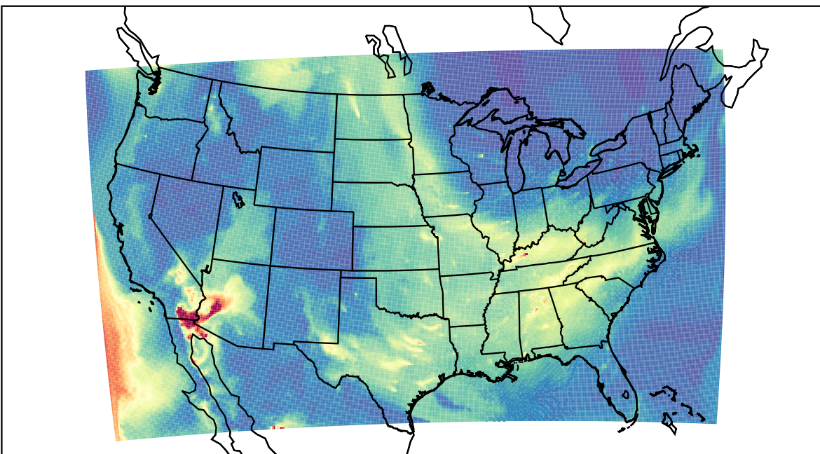
WRF 2023-05-25_11:00:00
