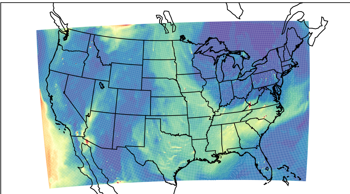
WRF 2023-05-25_22:00:00
