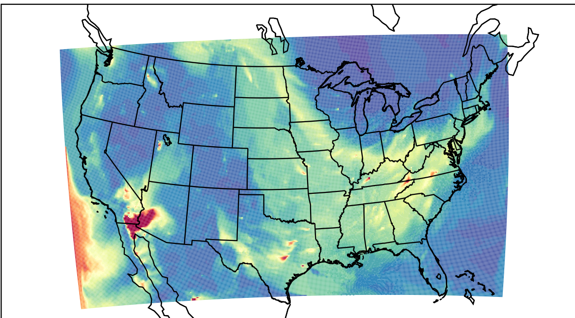
WRF 2023-05-25_06:00:00
