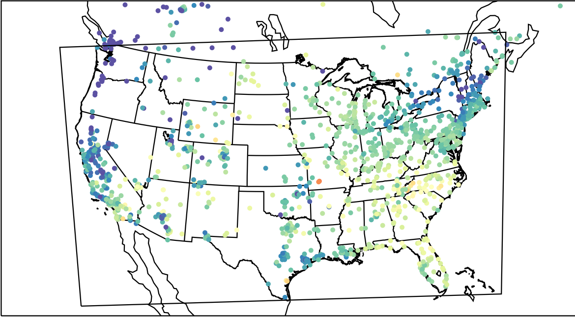
AirNOW (2023-05-25_14:00:00)
