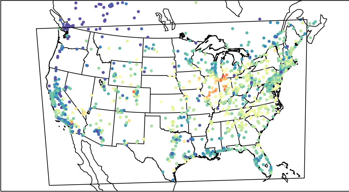
AirNOW (2023-05-24_14:00:00)
