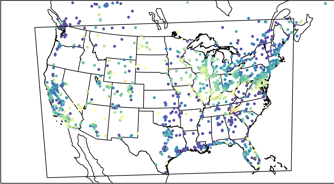
AirNOW (2023-05-25_08:00:00)
