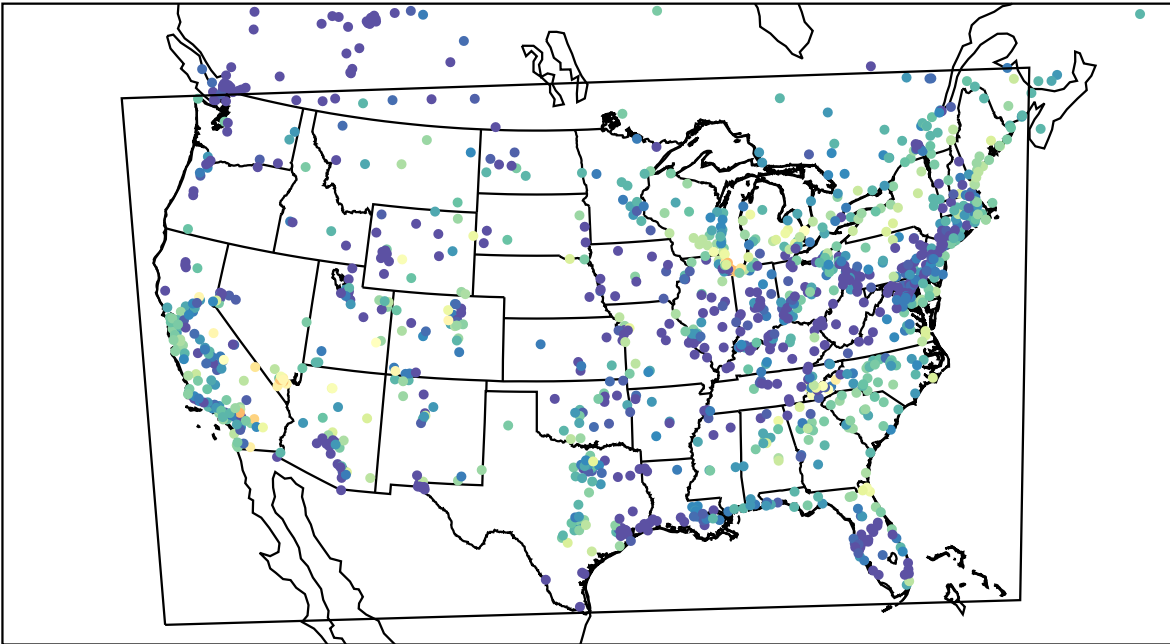
AirNOW (2023-05-24_12:00:00)
