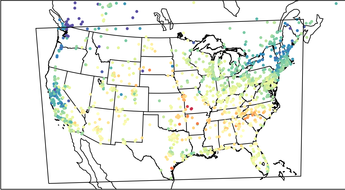
AirNOW (2023-05-25_16:00:00)
