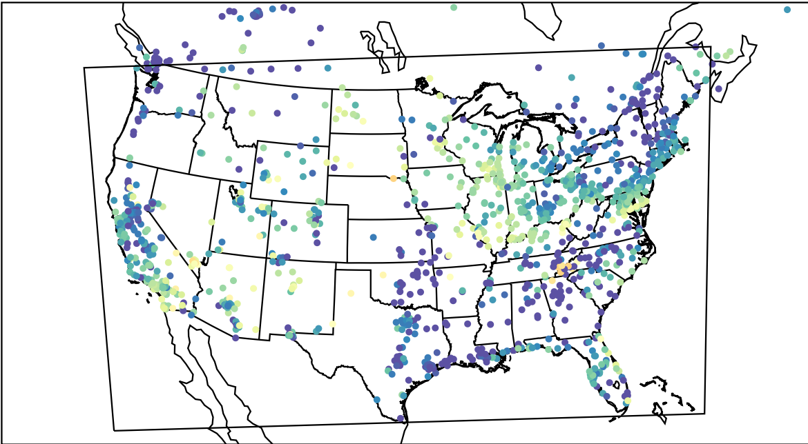
AirNOW (2023-05-25_09:00:00)
