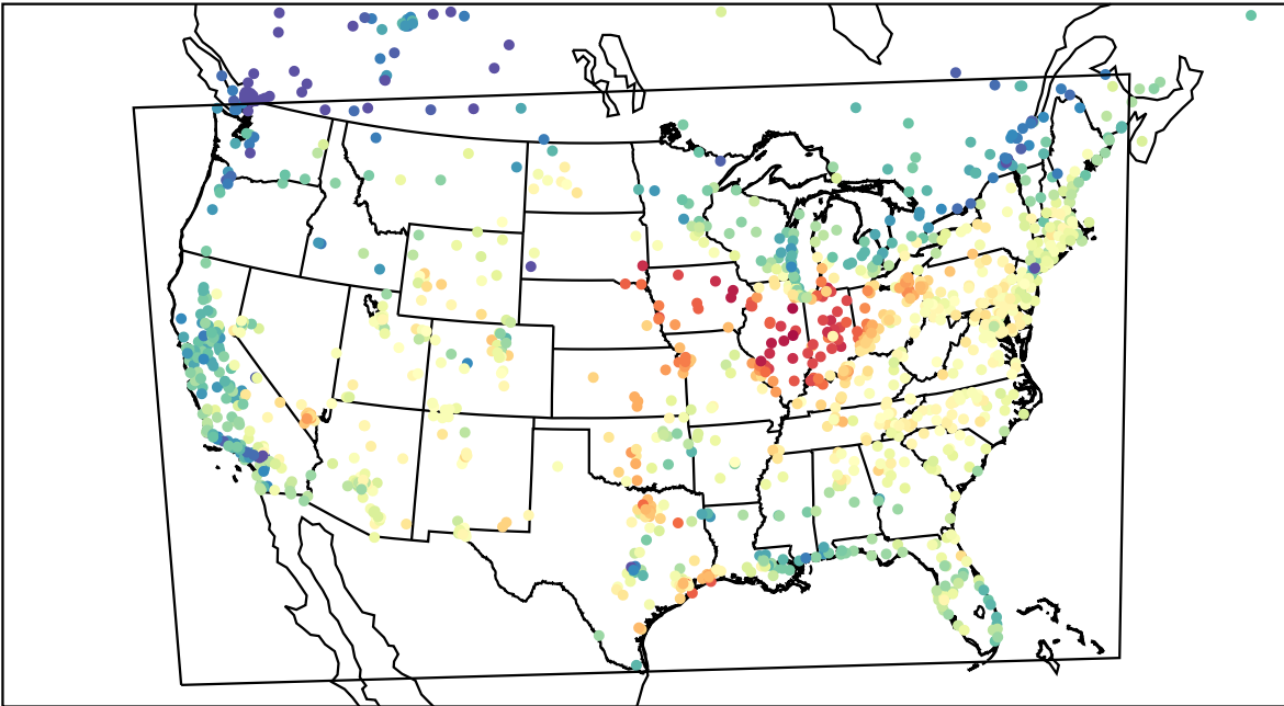
AirNOW (2023-05-24_16:00:00)
