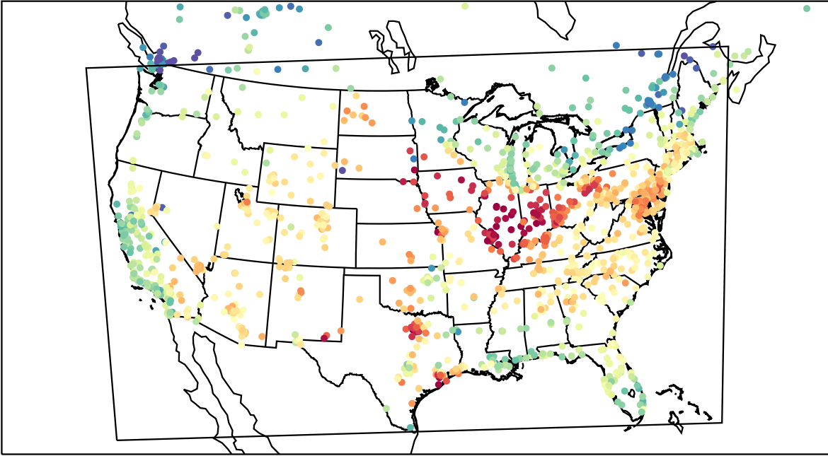
AirNOW (2023-05-24_19:00:00)
