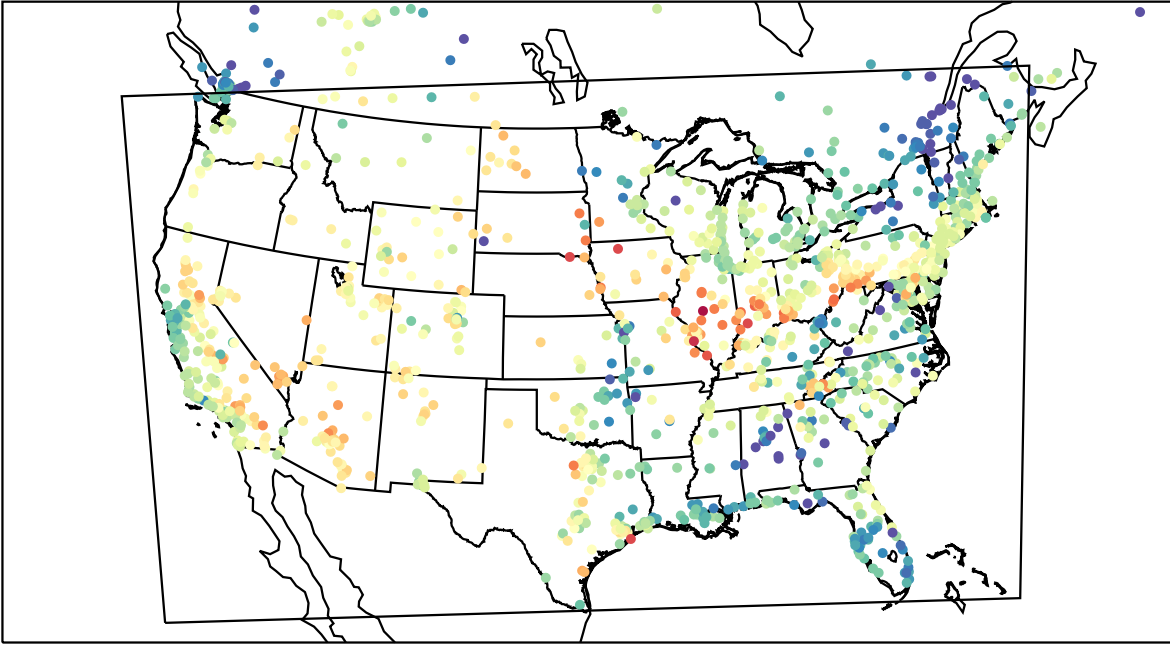
AirNOW (2023-05-25_01:00:00)
