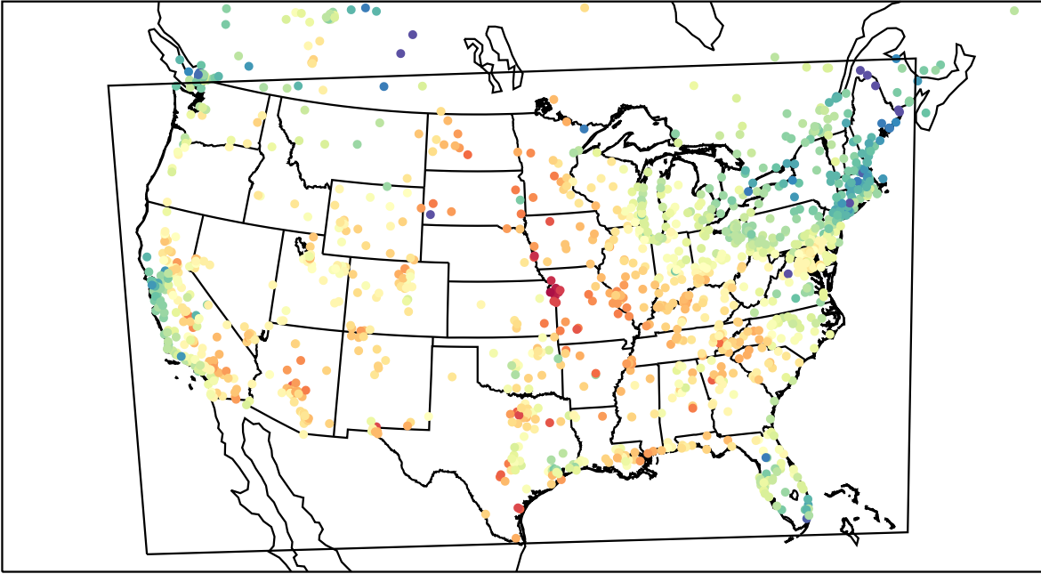
AirNOW (2023-05-25_23:00:00)
