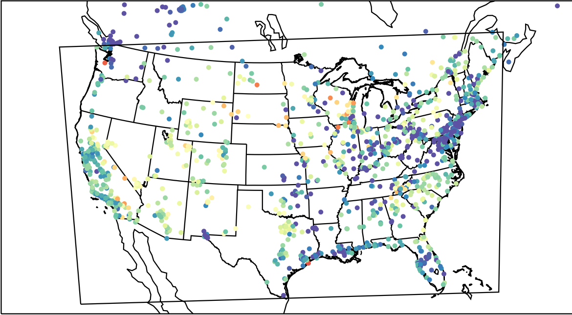
AirNOW (2023-05-24_05:00:00)
