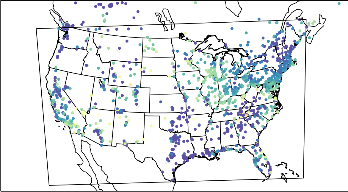
AirNOW (2023-05-25_11:00:00)
