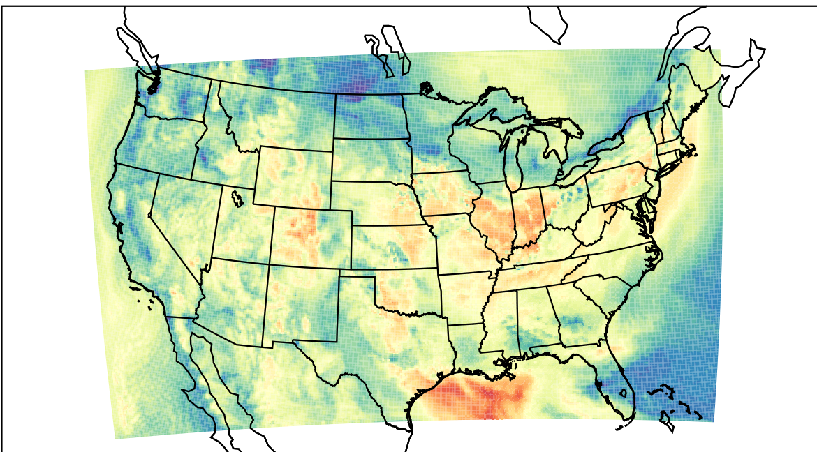
WRF (2023-05-24_15:00:00)
