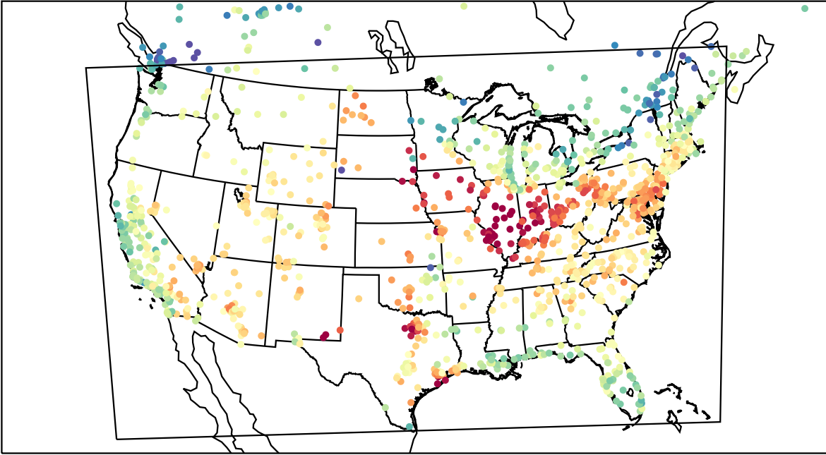
AirNOW (2023-05-24_20:00:00)
