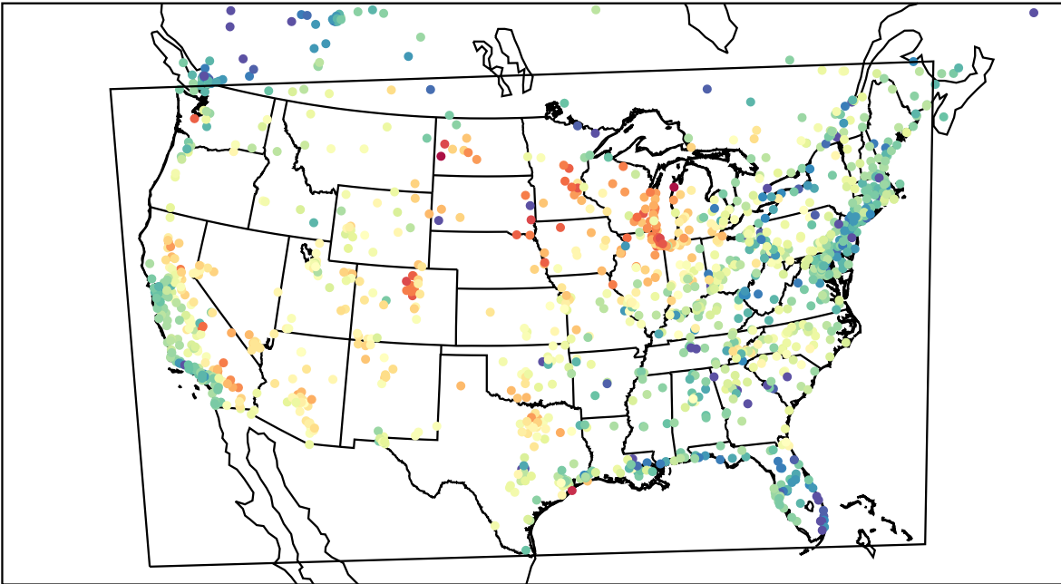
AirNOW (2023-05-24_01:00:00)
