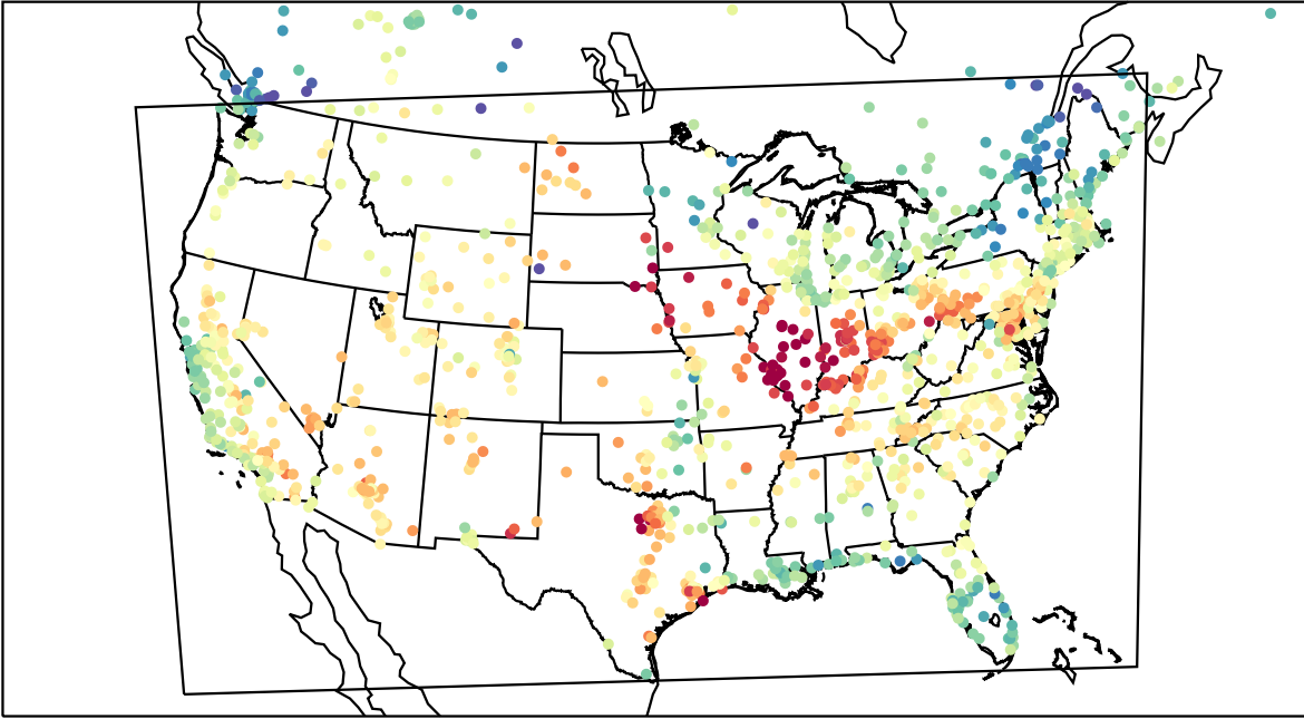
AirNOW (2023-05-24_23:00:00)
