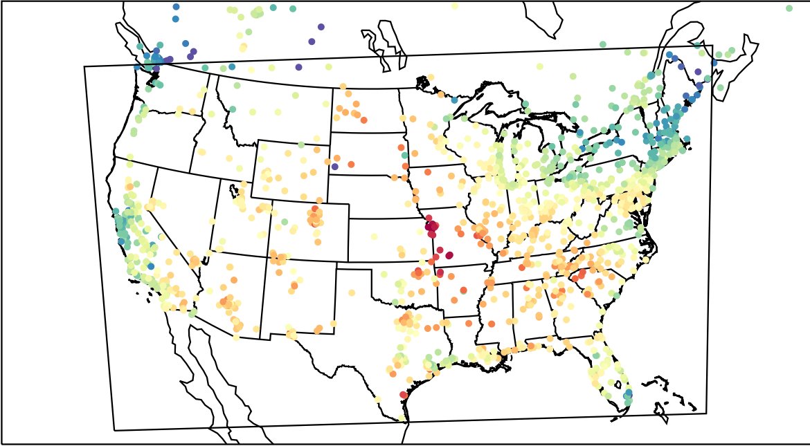
AirNOW (2023-05-25_19:00:00)
