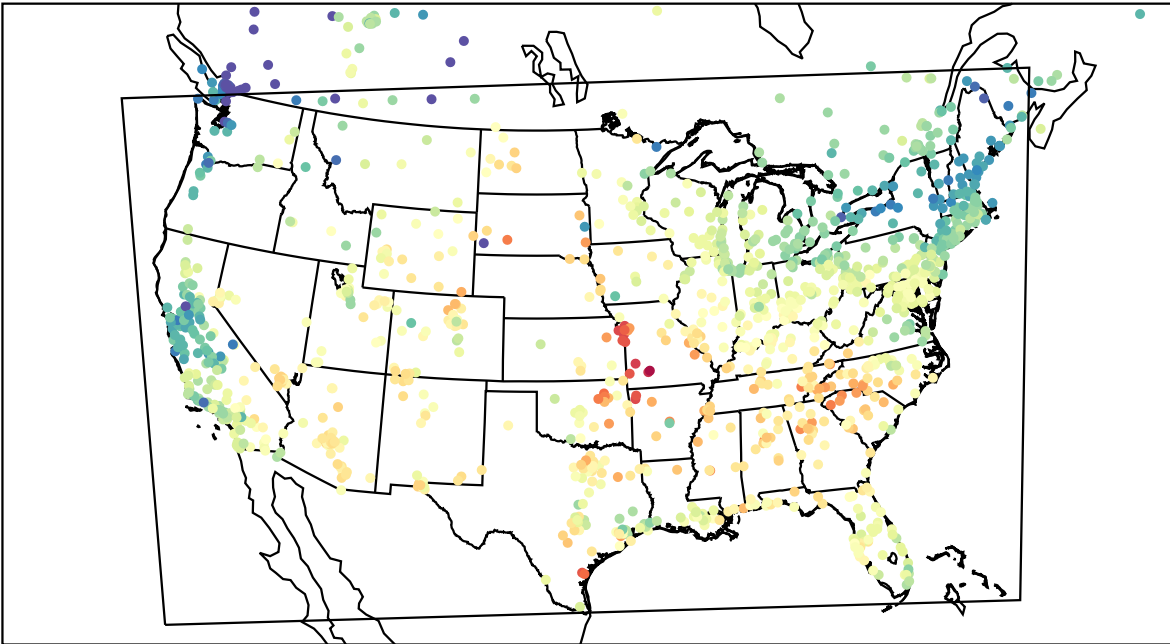
AirNOW (2023-05-25_17:00:00)
