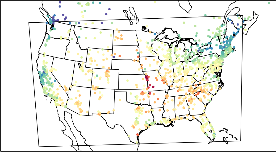
AirNOW (2023-05-25_18:00:00)
