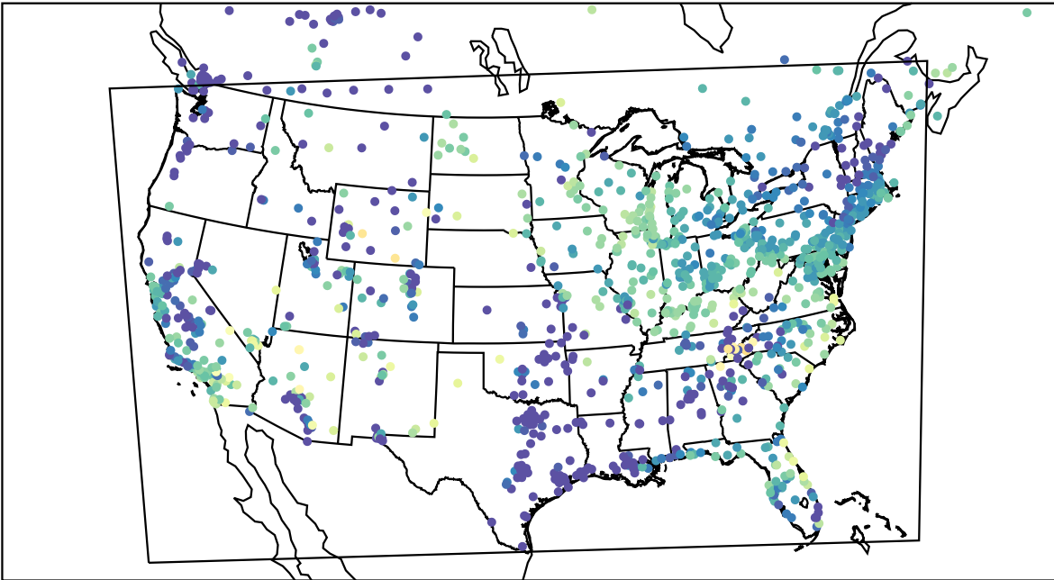
AirNOW (2023-05-25_12:00:00)
