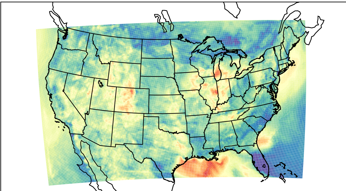
WRF (2023-05-24_08:00:00)
