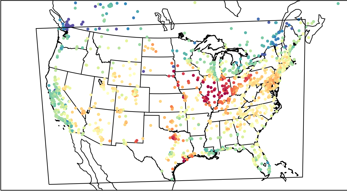
AirNOW (2023-05-24_18:00:00)
