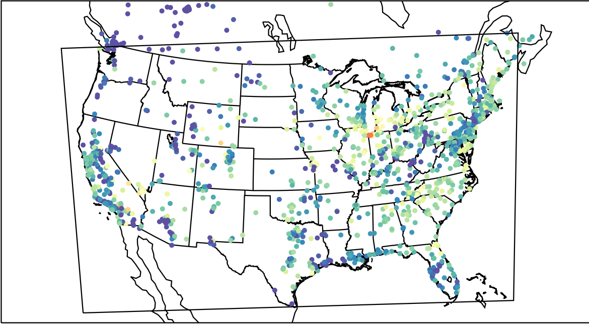
AirNOW (2023-05-24_13:00:00)
