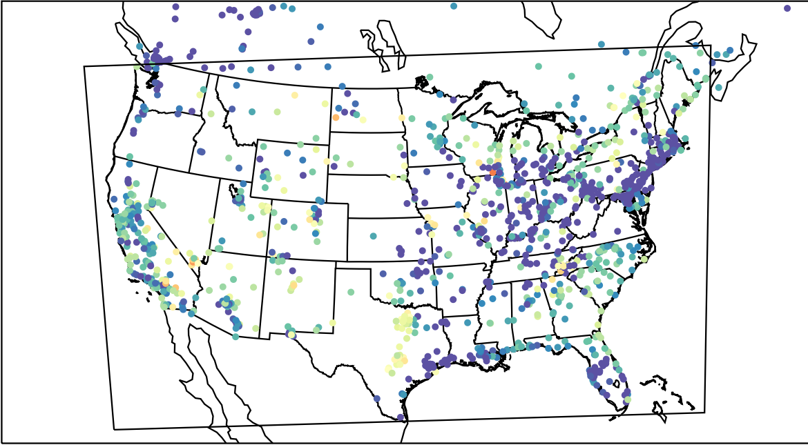
AirNOW (2023-05-24_09:00:00)
