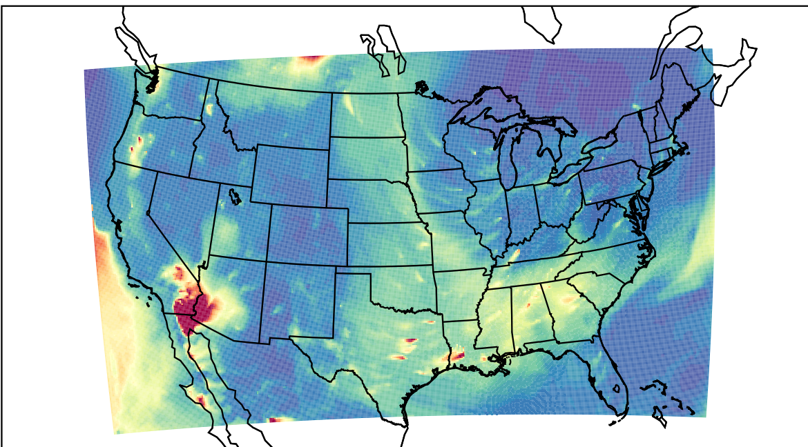
WRF 2023-05-26_05:00:00
