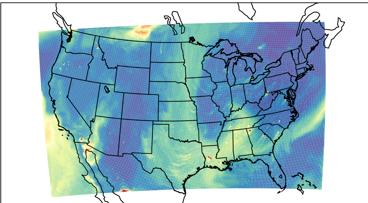
WRF 2023-05-26_22:00:00
