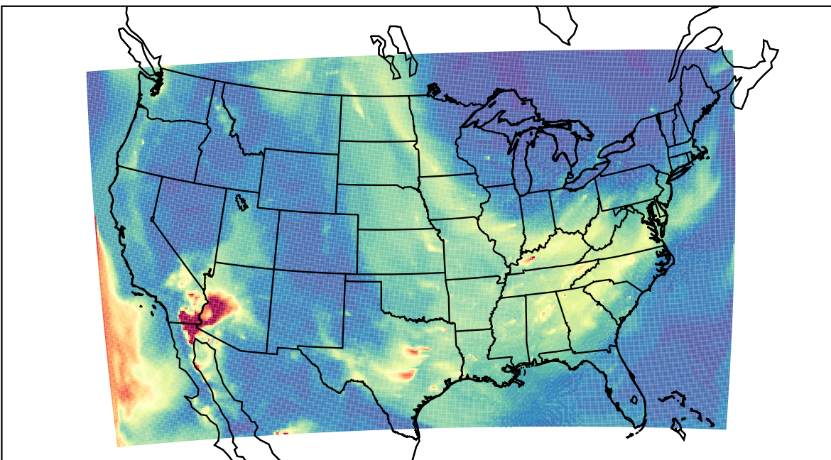
WRF 2023-05-25_09:00:00
