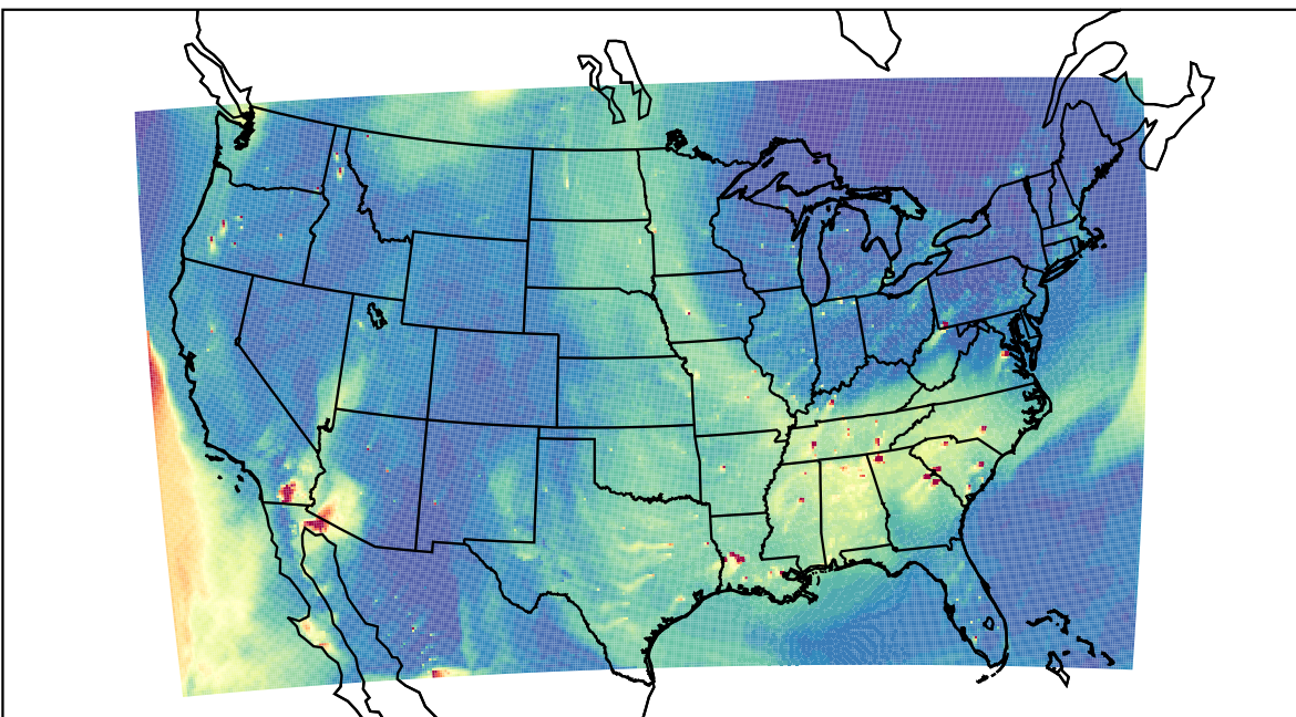
WRF 2023-05-26_00:00:00
