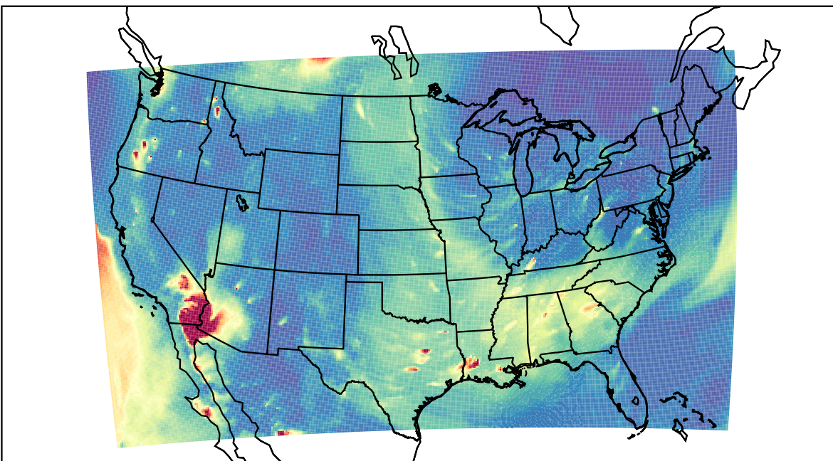
WRF 2023-05-26_04:00:00
