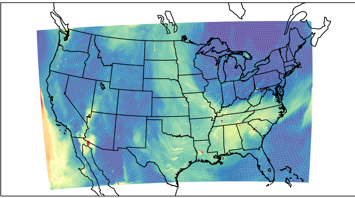
WRF 2023-05-25_21:00:00
