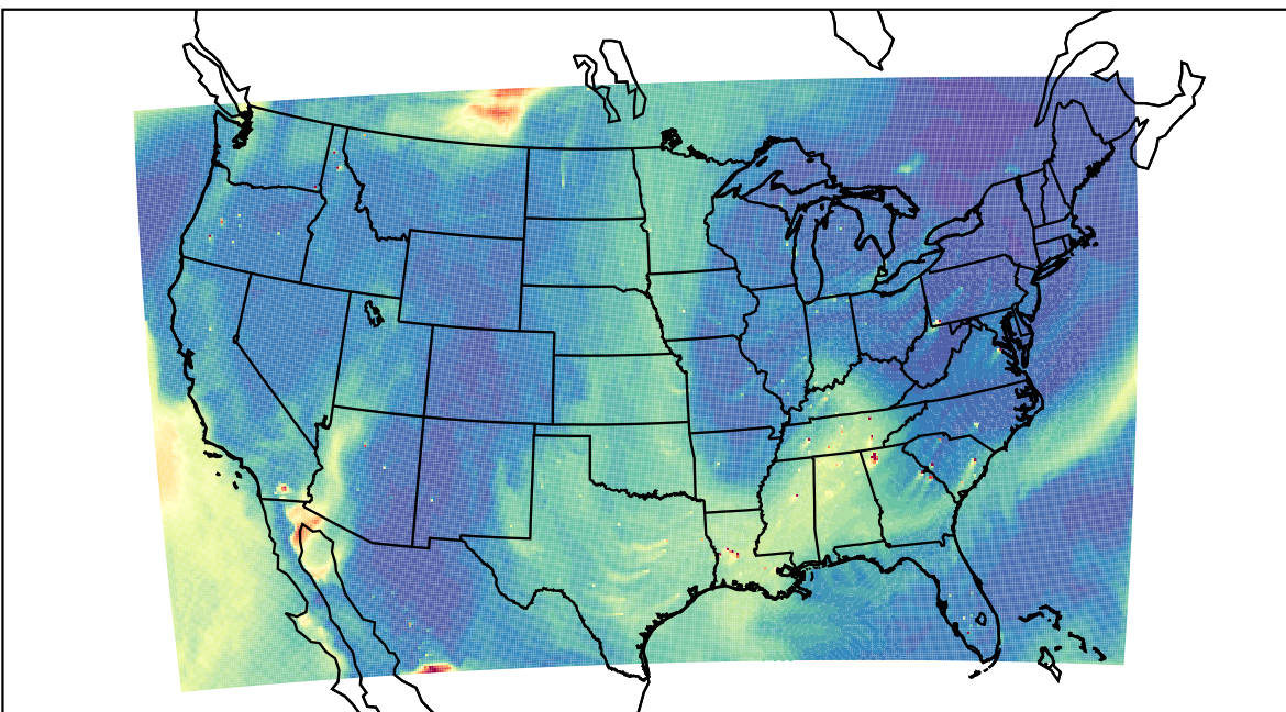
WRF 2023-05-26_21:00:00
