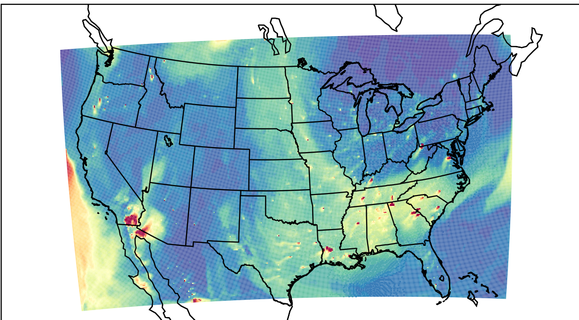
WRF 2023-05-26_01:00:00
