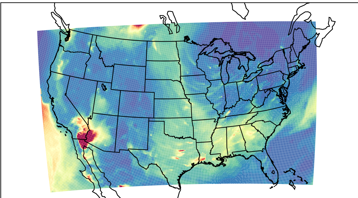
WRF 2023-05-26_06:00:00
