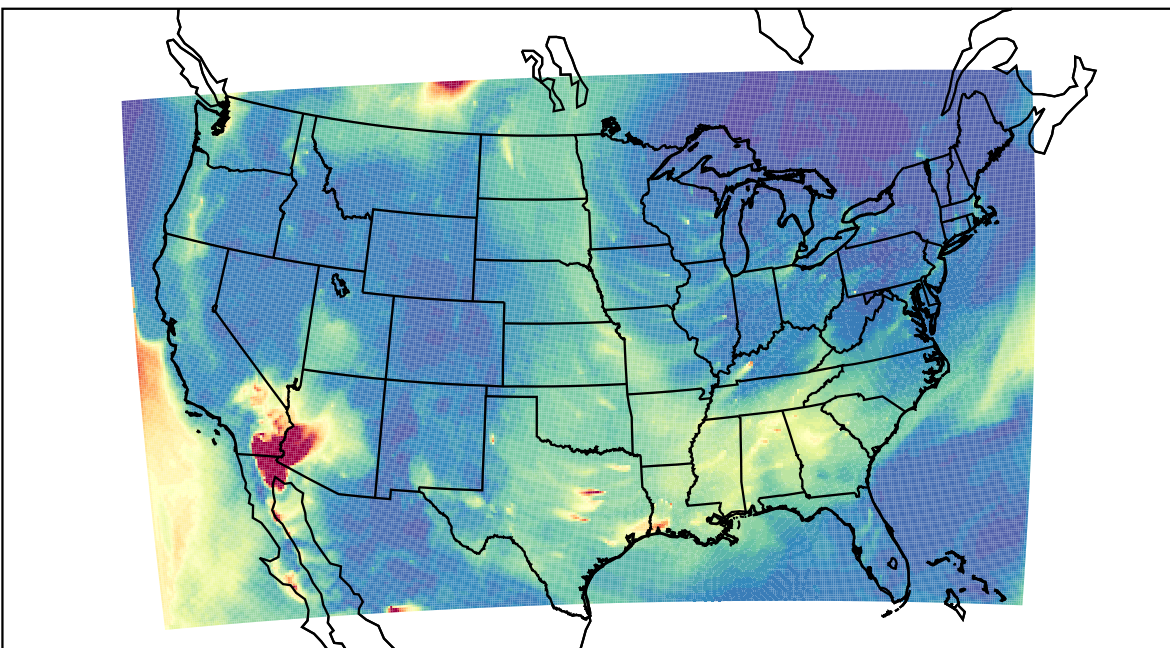
WRF 2023-05-26_07:00:00
