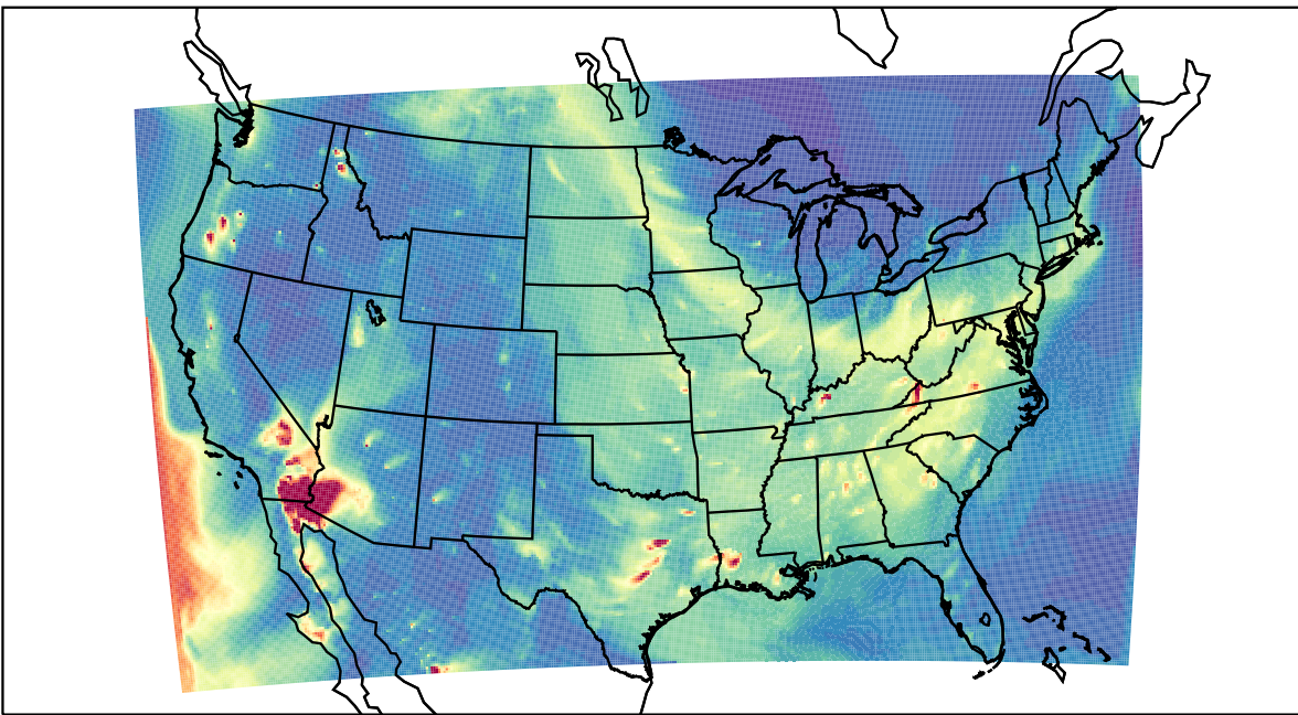
WRF 2023-05-25_04:00:00
