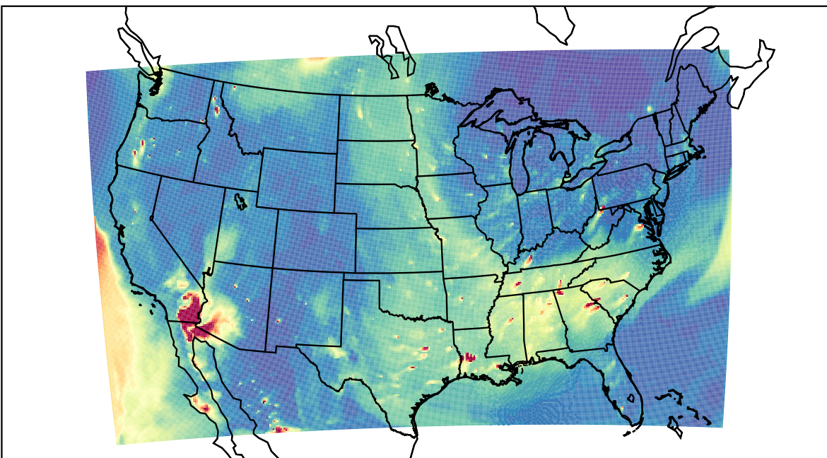
WRF 2023-05-26_02:00:00
