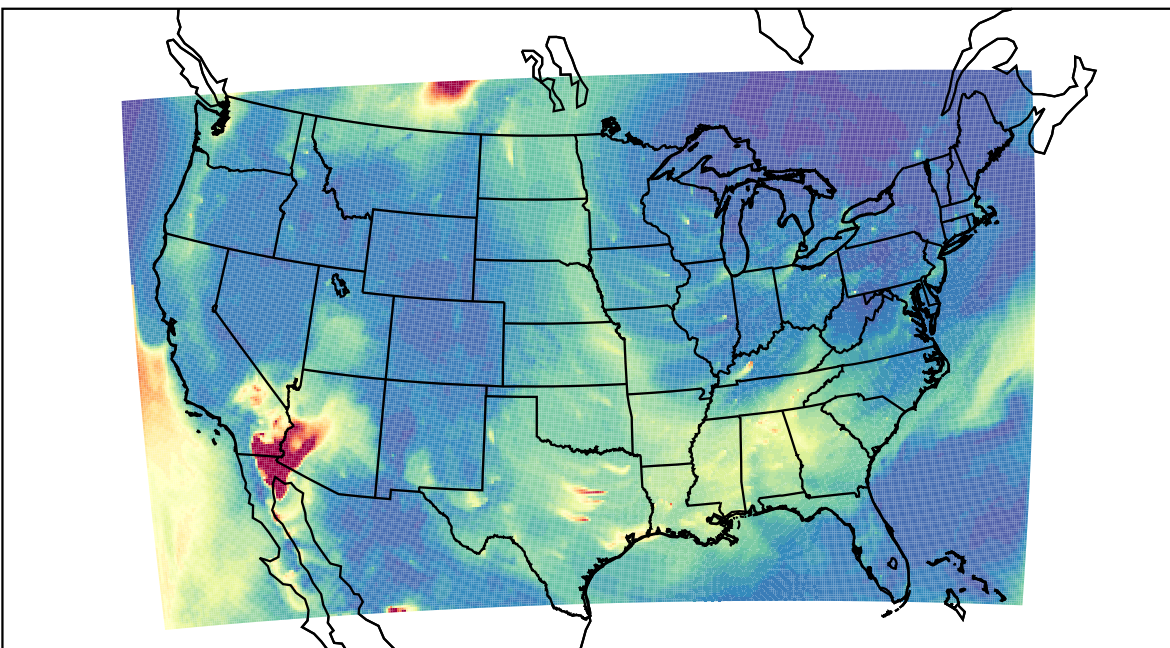
WRF 2023-05-26_09:00:00
