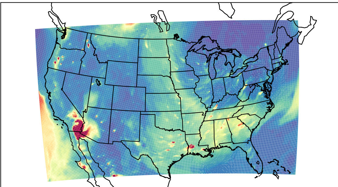
WRF 2023-05-26_03:00:00
