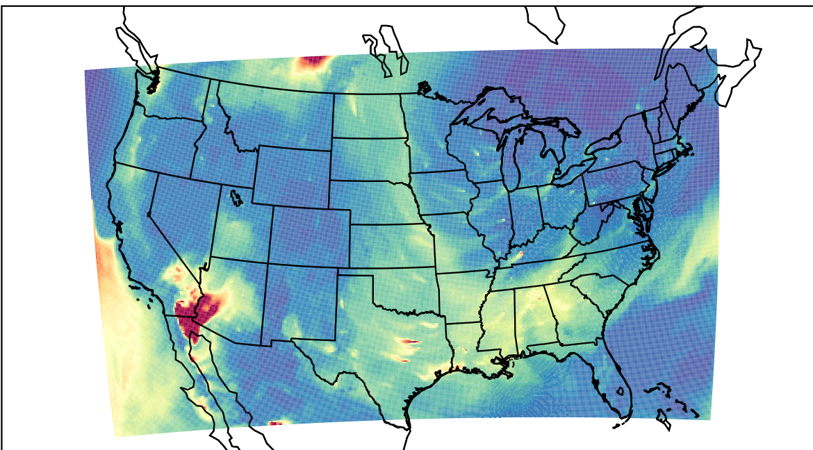
WRF 2023-05-26_08:00:00
