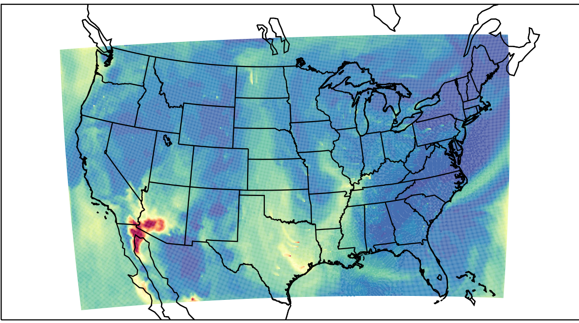
WRF 2023-05-27_16:00:00
