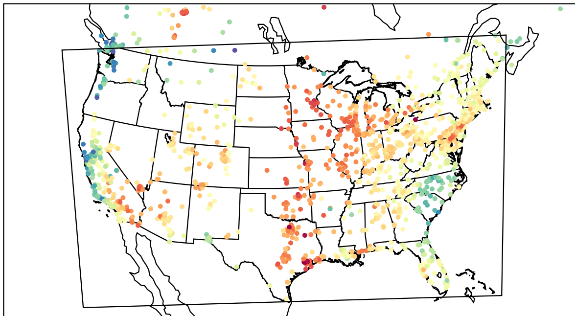
AirNOW (2023-05-27_20:00:00)
