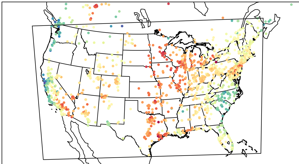
AirNOW (2023-05-27_21:00:00)
