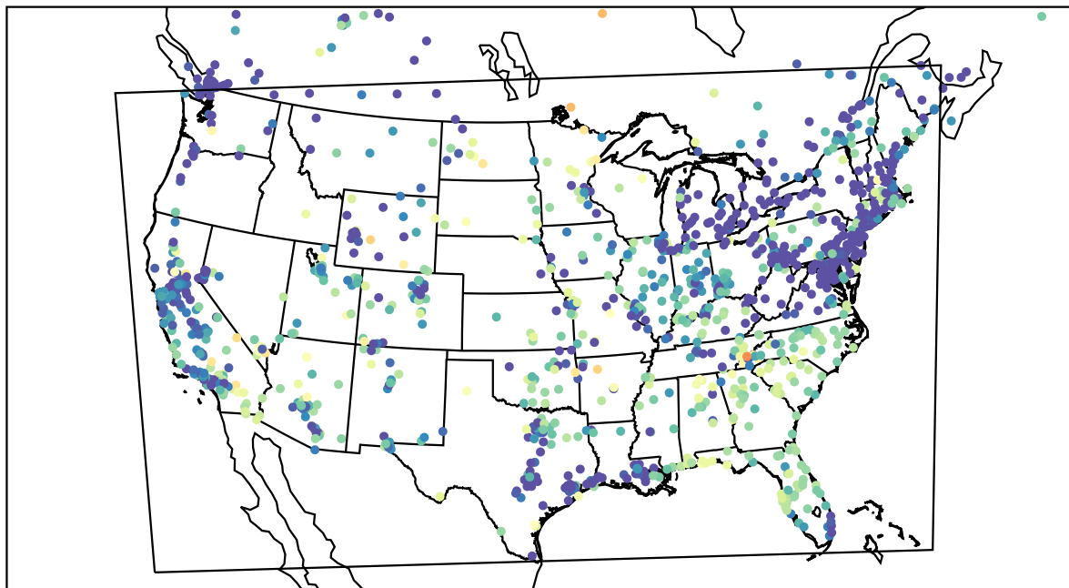
AirNOW (2023-05-27_10:00:00)
