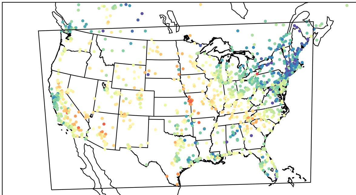
AirNOW (2023-05-26_01:00:00)
