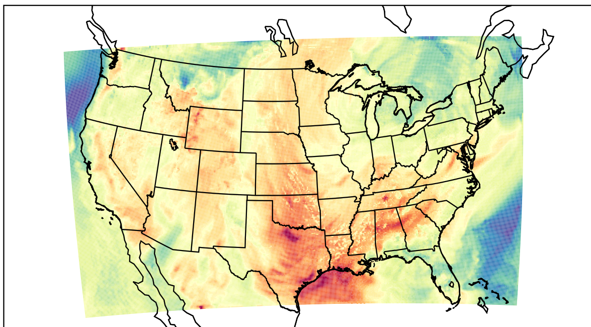
WRF (2023-05-26_22:00:00)
