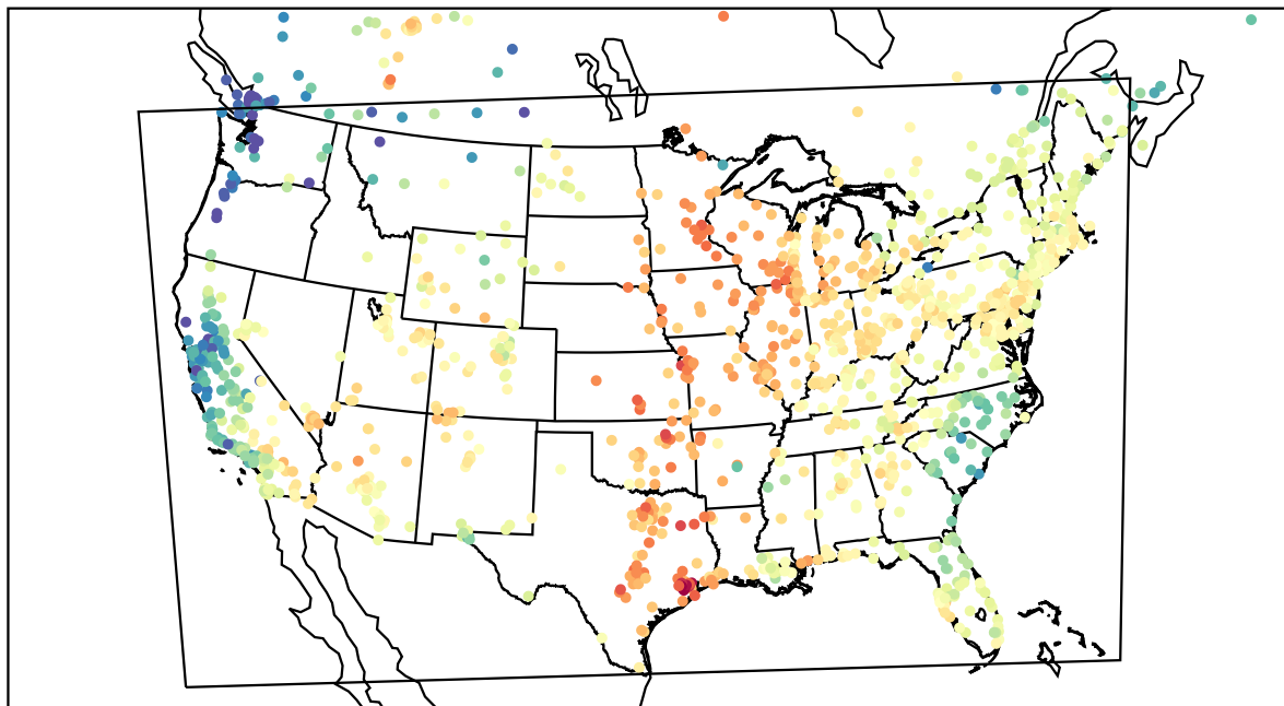
AirNOW (2023-05-27_17:00:00)
