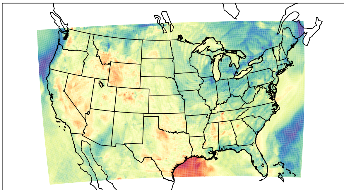
WRF (2023-05-27_02:00:00)
