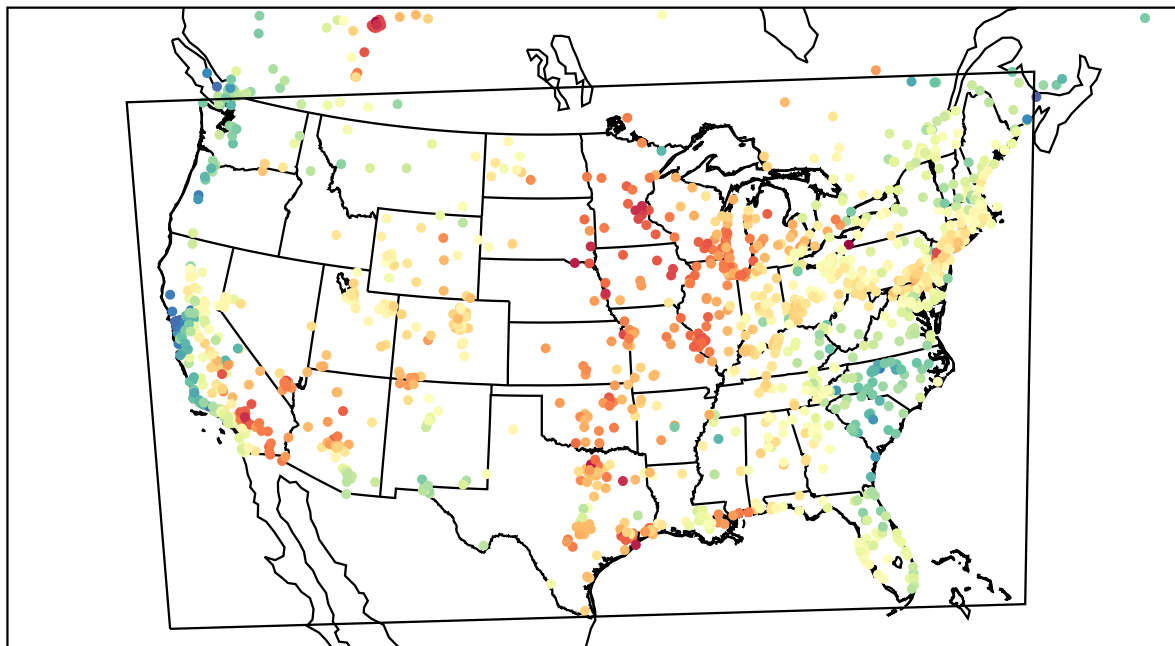
AirNOW (2023-05-27_23:00:00)
