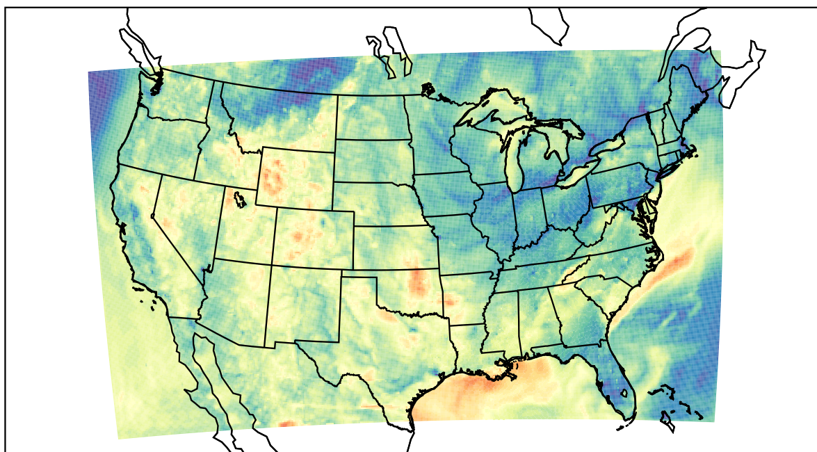
WRF (2023-05-26_05:00:00)
