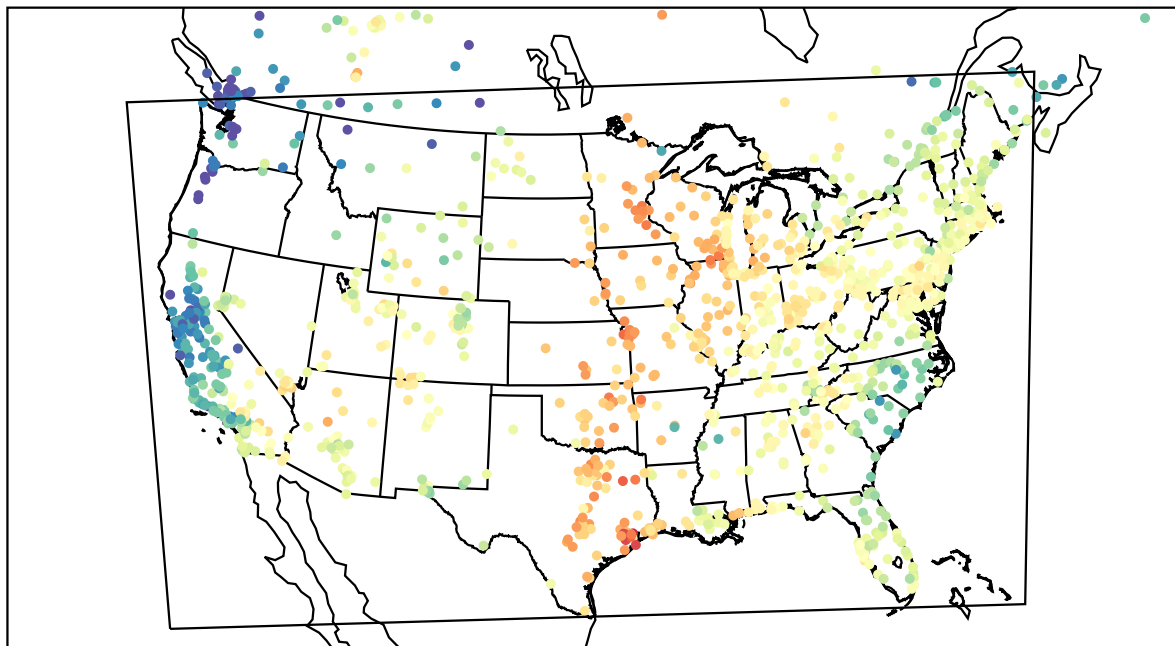
AirNOW (2023-05-27_16:00:00)
