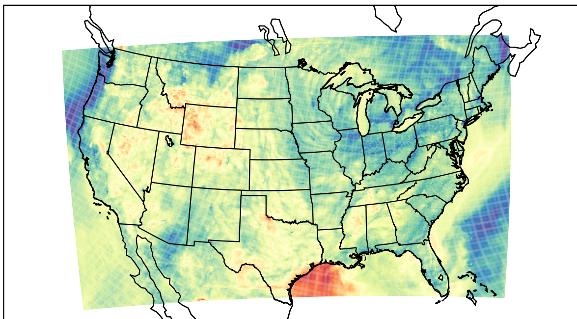
WRF (2023-05-27_04:00:00)
