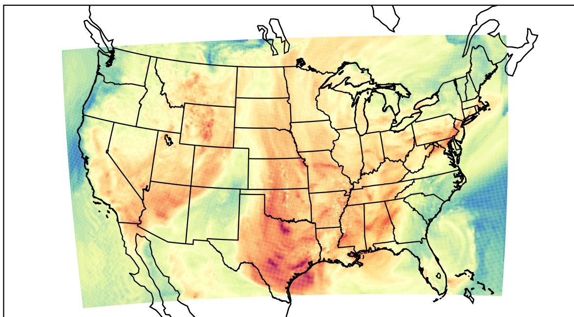
WRF (2023-05-27_21:00:00)
