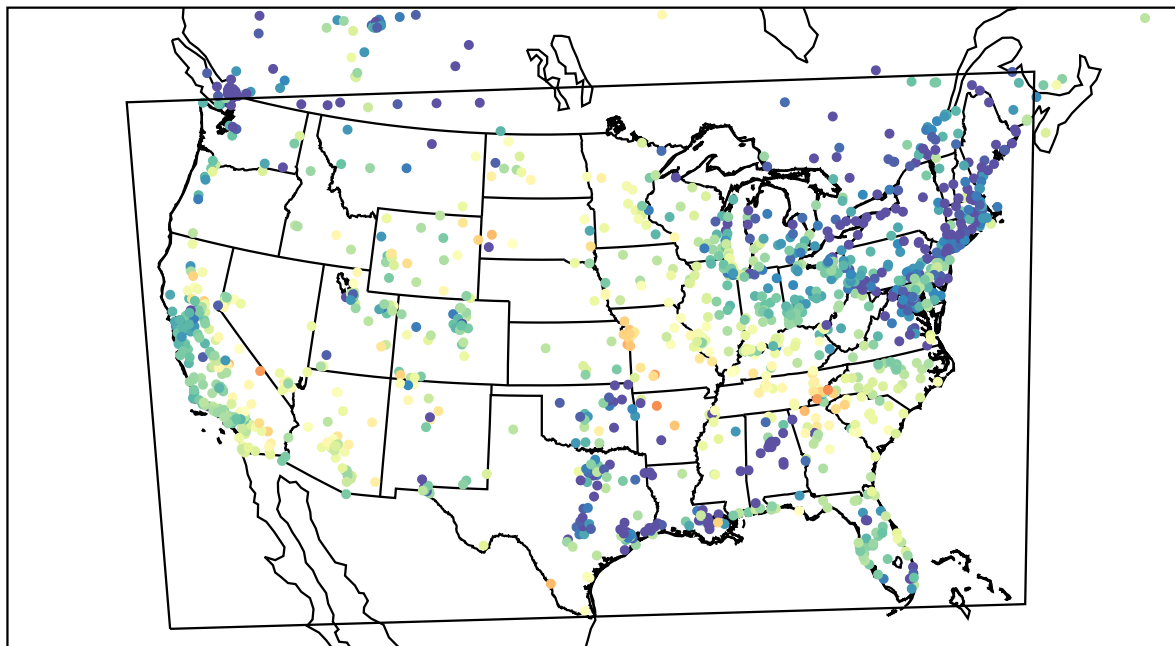
AirNOW (2023-05-26_04:00:00)
