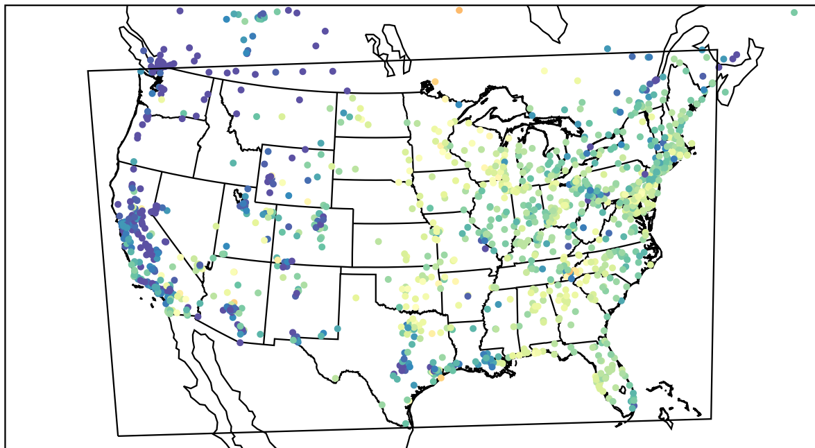
AirNOW (2023-05-27_13:00:00)
