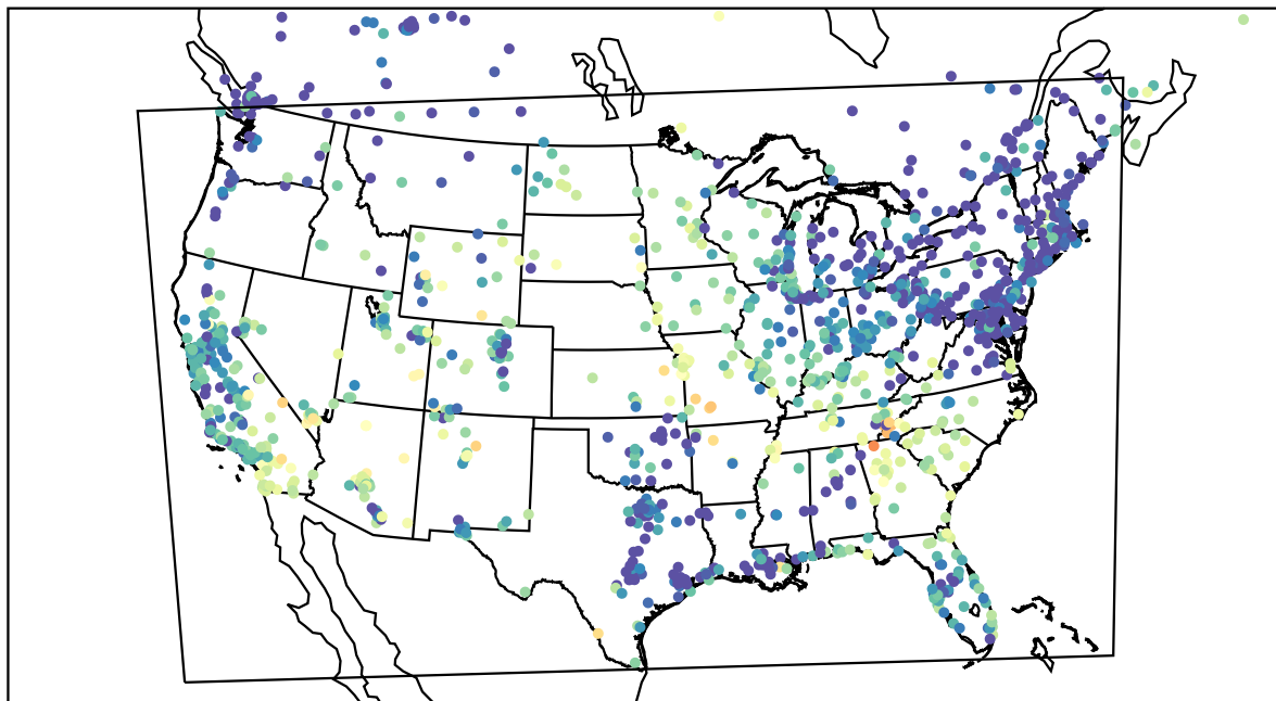
AirNOW (2023-05-26_08:00:00)
