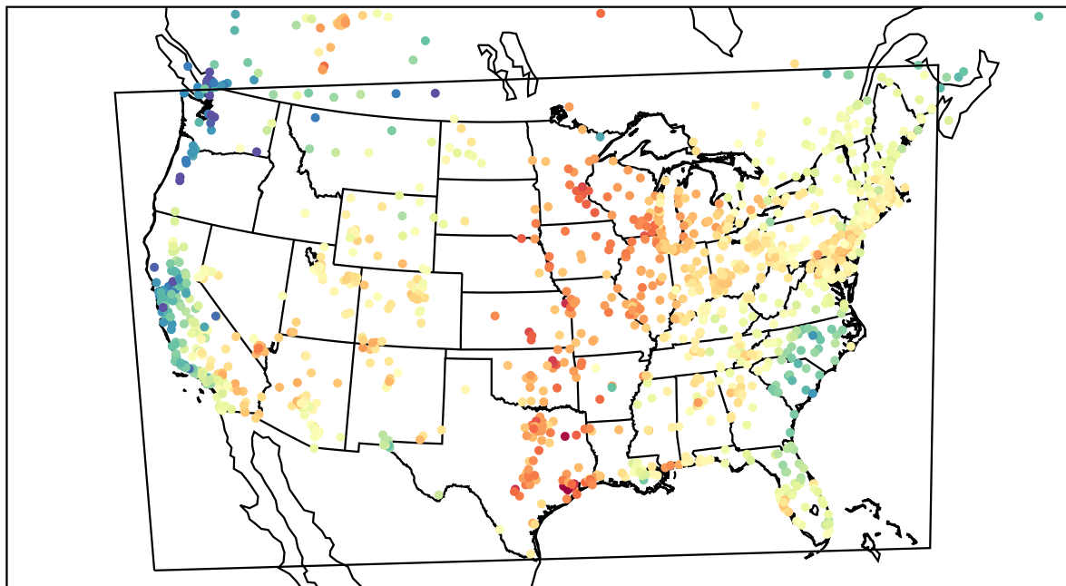
AirNOW (2023-05-27_18:00:00)
