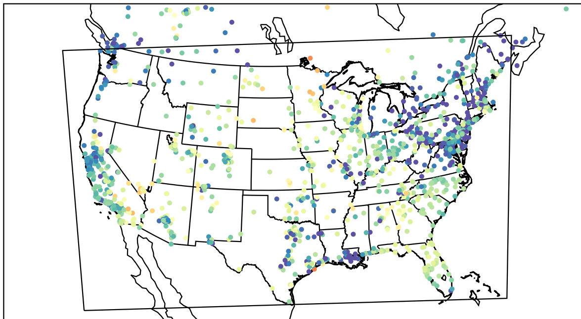
AirNOW (2023-05-27_05:00:00)
