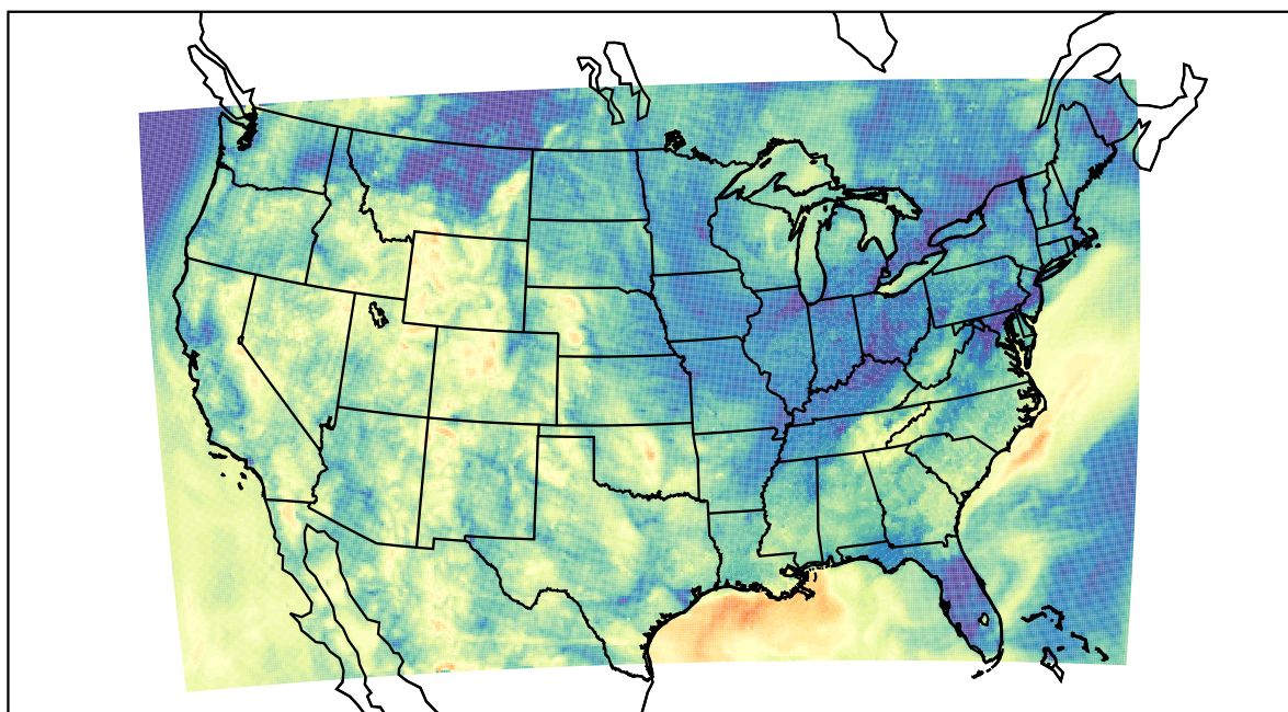
WRF (2023-05-26_11:00:00)
