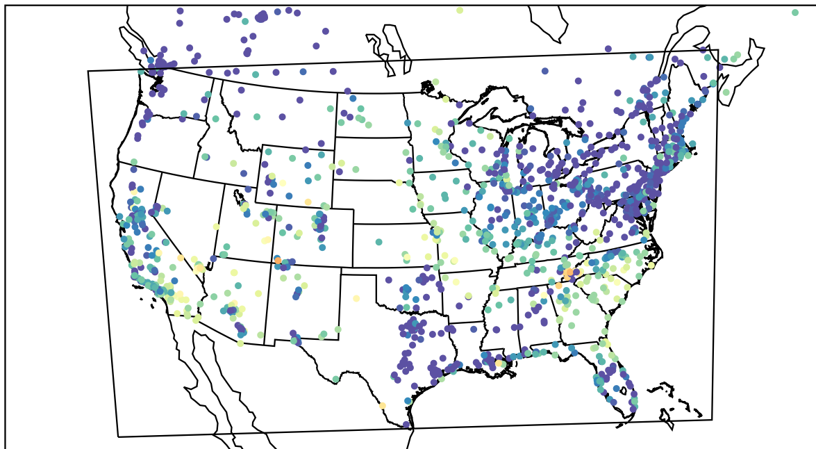
AirNOW (2023-05-26_11:00:00)
