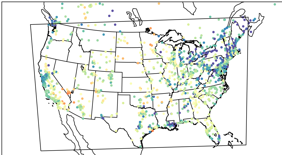
AirNOW (2023-05-27_03:00:00)
