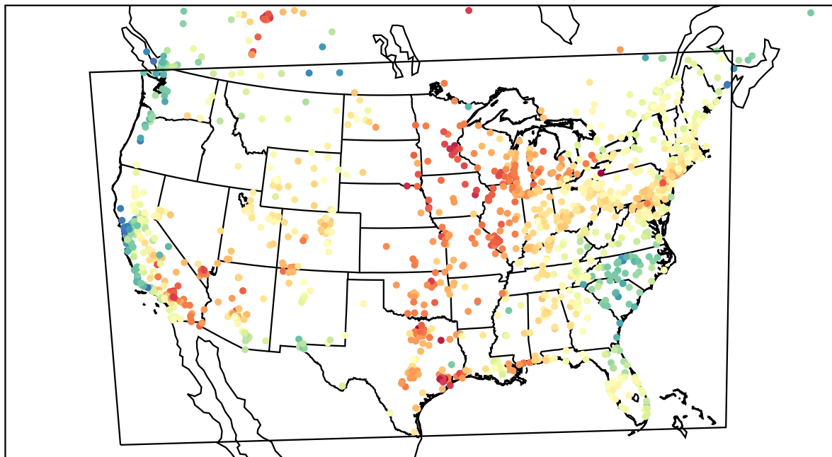
AirNOW (2023-05-27_22:00:00)
