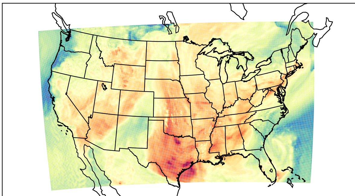
WRF (2023-05-27_19:00:00)
