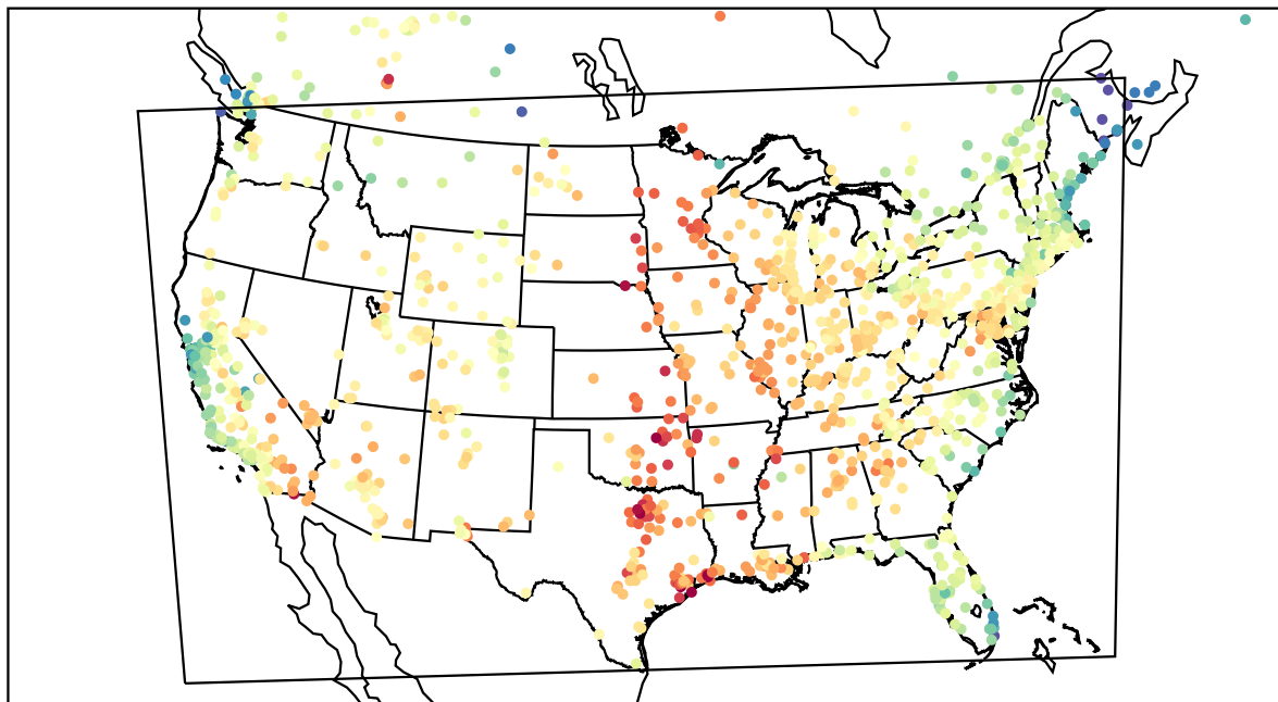
AirNOW (2023-05-26_22:00:00)
