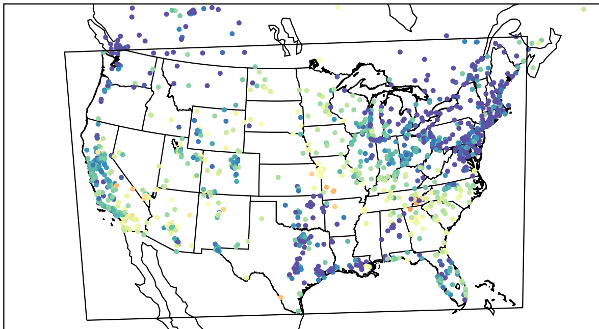
AirNOW (2023-05-26_07:00:00)
