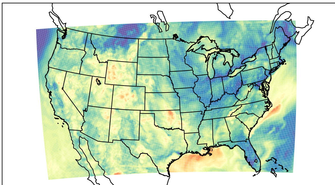
WRF (2023-05-26_07:00:00)
