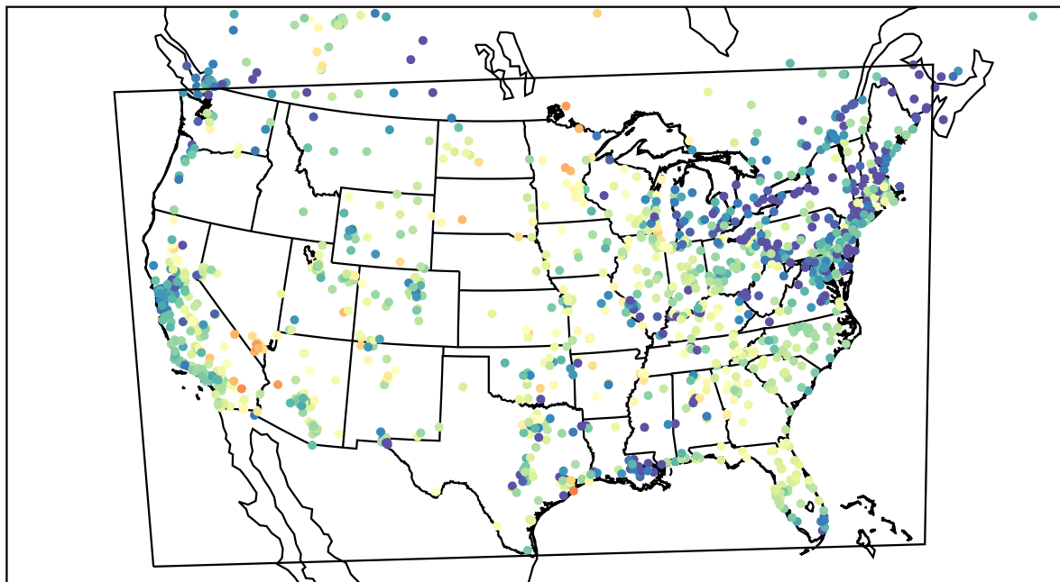
AirNOW (2023-05-27_04:00:00)
