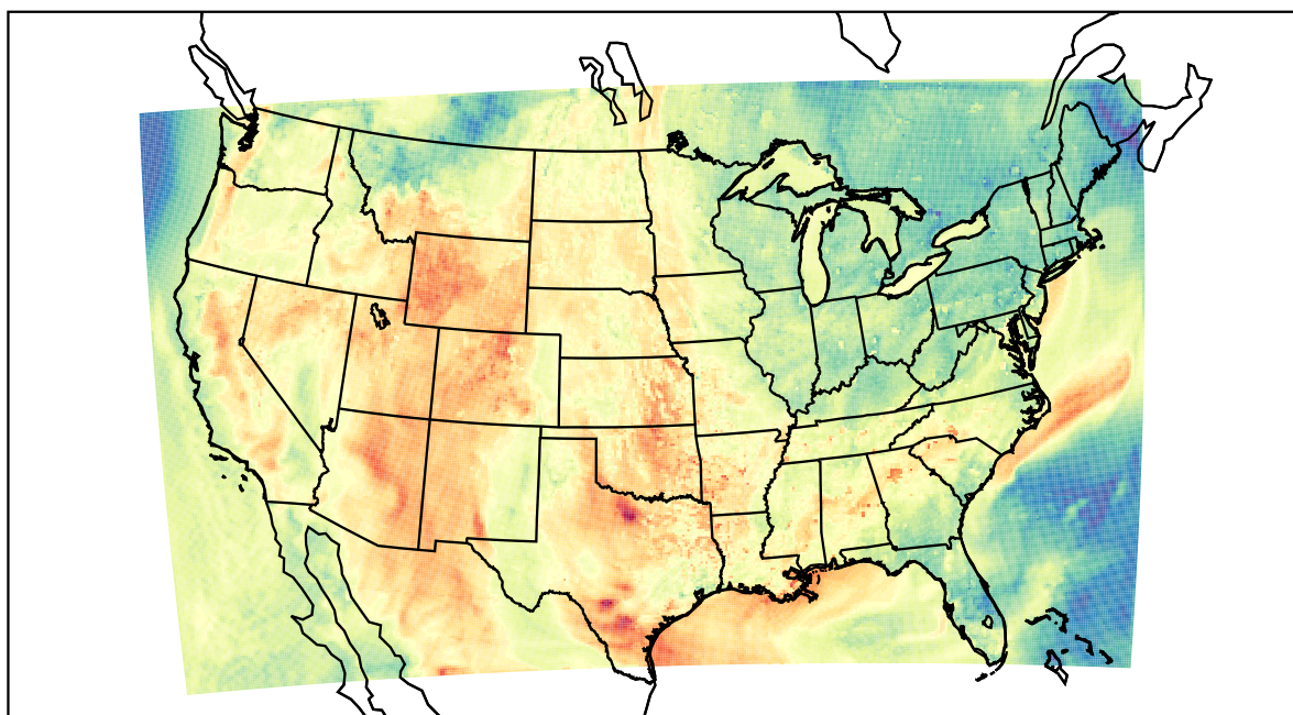
WRF (2023-05-26_00:00:00)
