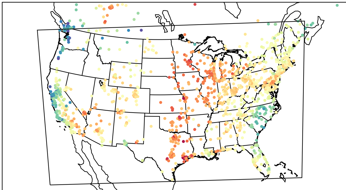
AirNOW (2023-05-27_19:00:00)
