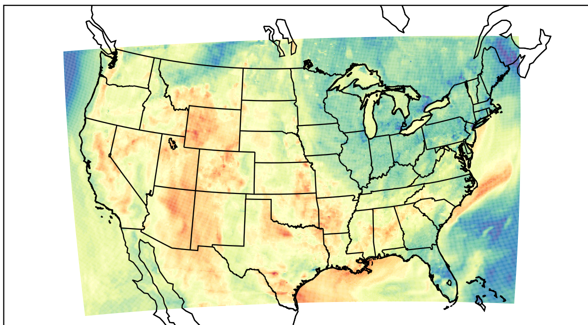
WRF (2023-05-26_01:00:00)
