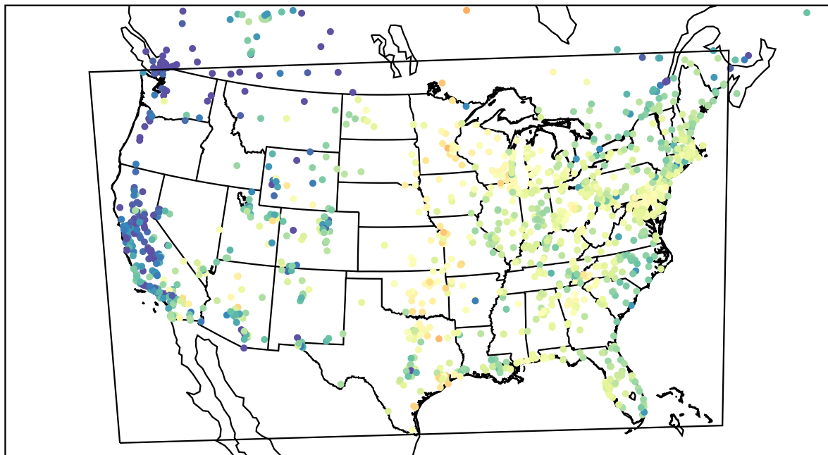
AirNOW (2023-05-27_14:00:00)
