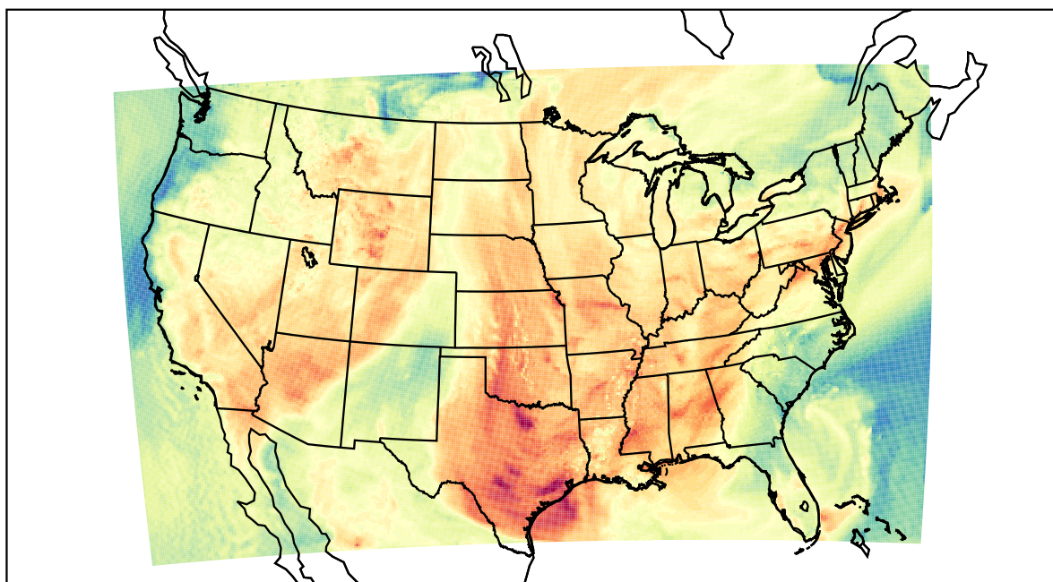
WRF (2023-05-27_20:00:00)
