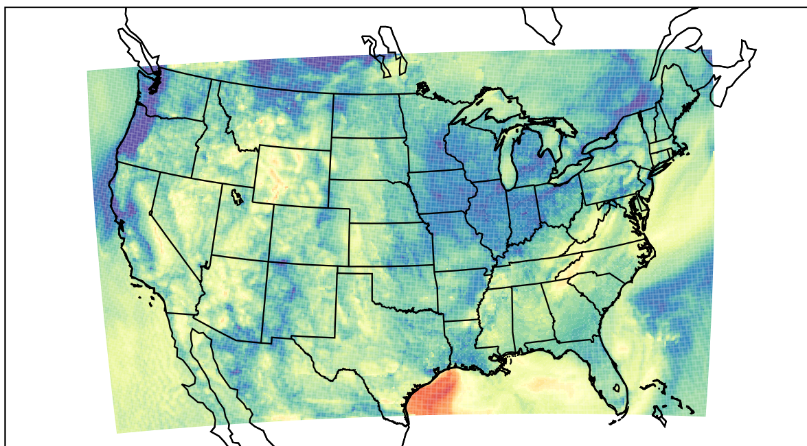
WRF (2023-05-27_13:00:00)
