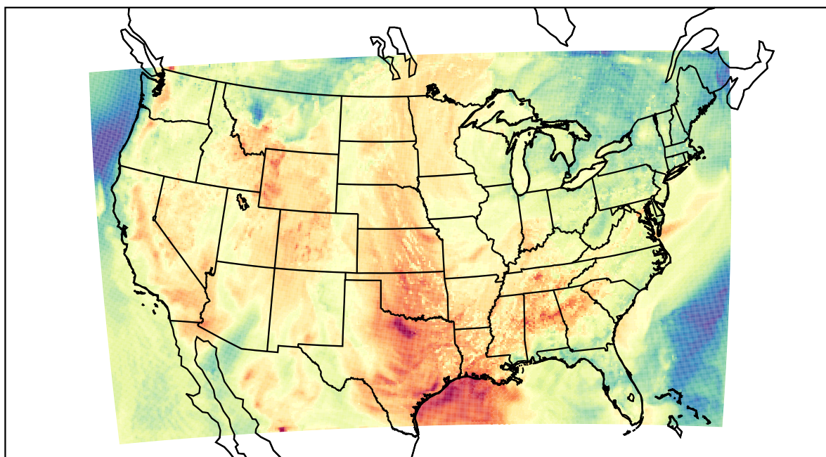
WRF (2023-05-26_23:00:00)
