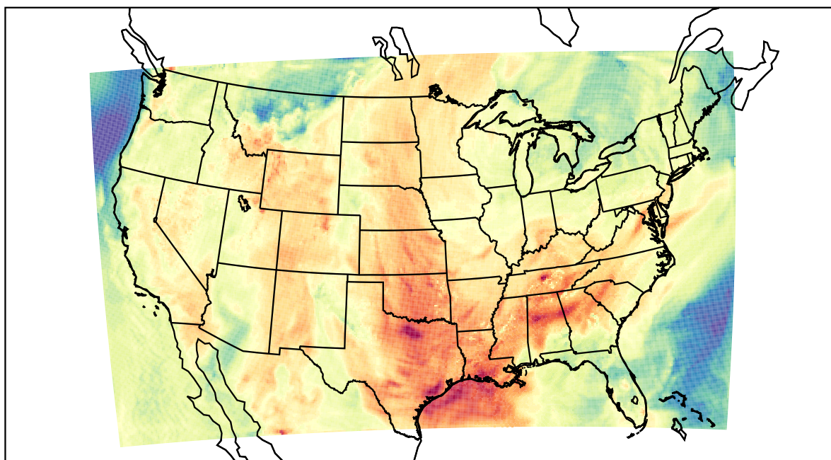
WRF (2023-05-26_20:00:00)
