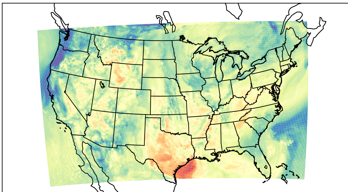
WRF (2023-05-27_15:00:00)
