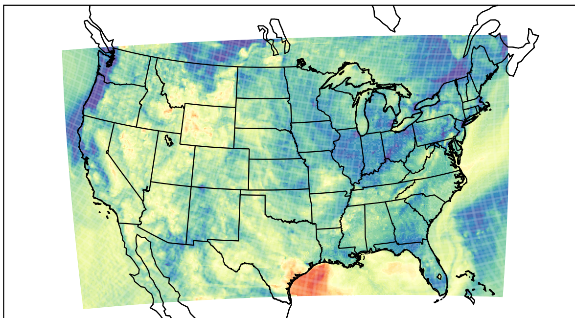
WRF (2023-05-27_10:00:00)
