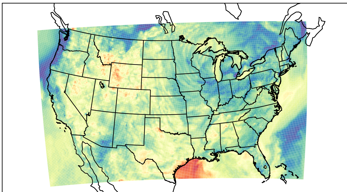
WRF (2023-05-27_05:00:00)
