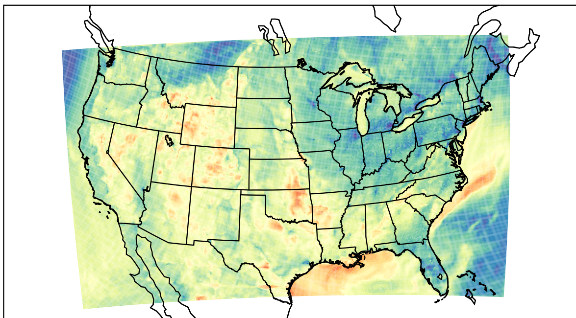
WRF (2023-05-26_03:00:00)
