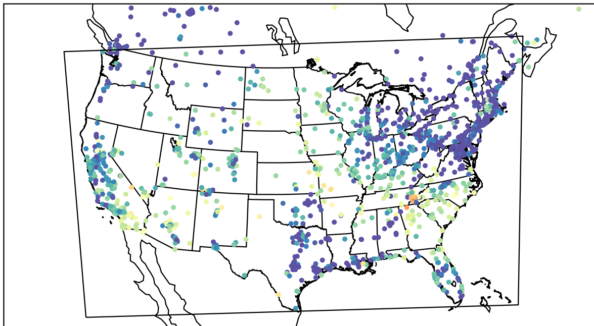
AirNOW (2023-05-26_09:00:00)
