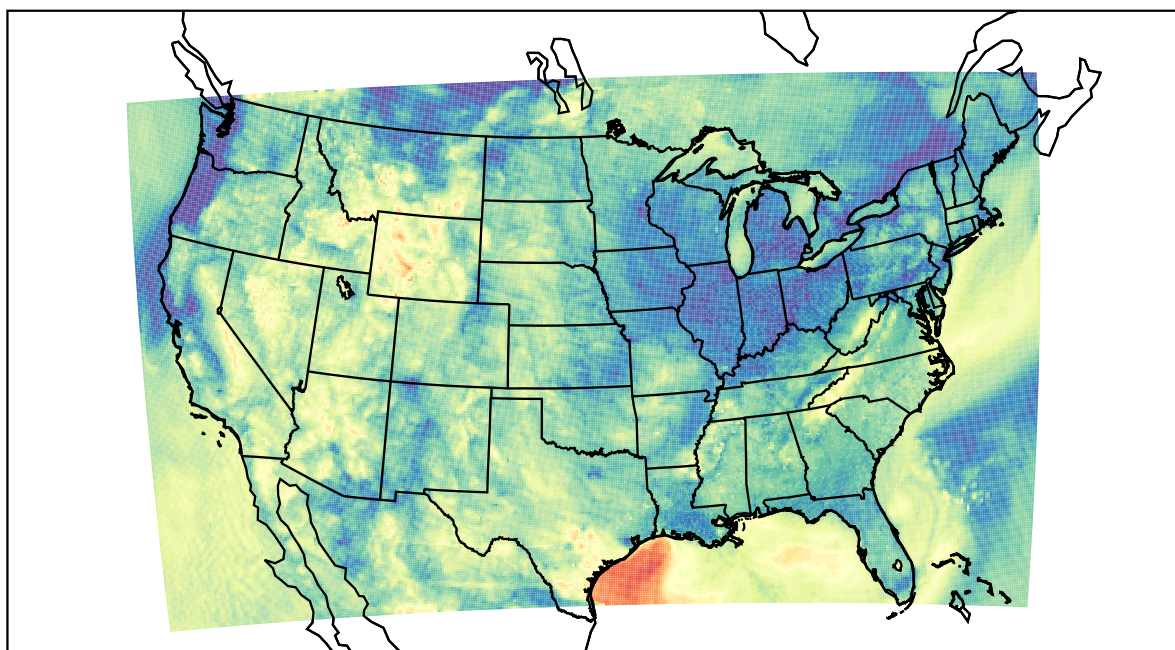
WRF (2023-05-27_12:00:00)
