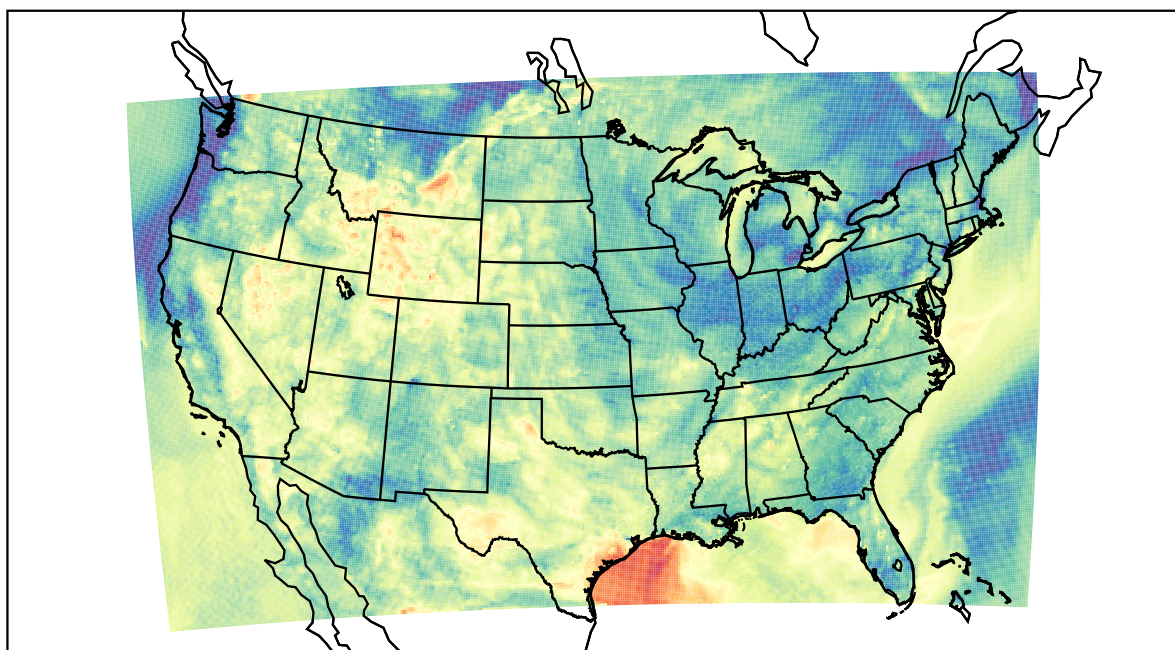
WRF (2023-05-27_07:00:00)
