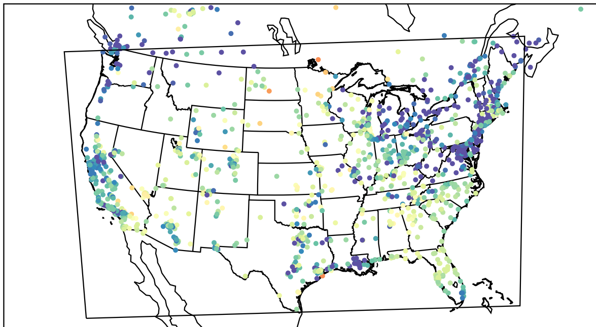
AirNOW (2023-05-27_06:00:00)
