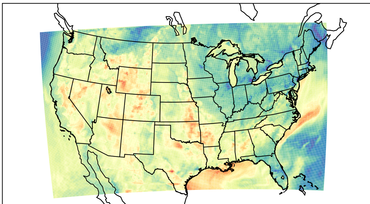
WRF (2023-05-26_02:00:00)
