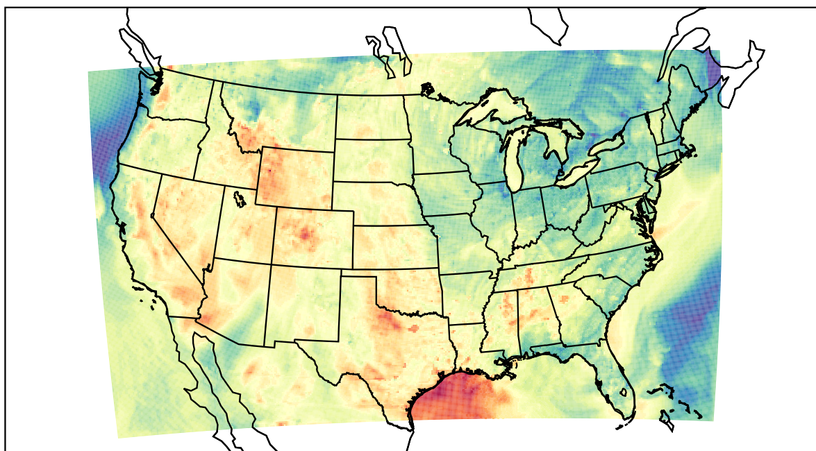
WRF (2023-05-27_01:00:00)
