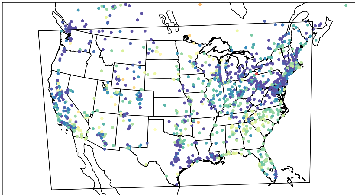
AirNOW (2023-05-27_11:00:00)
