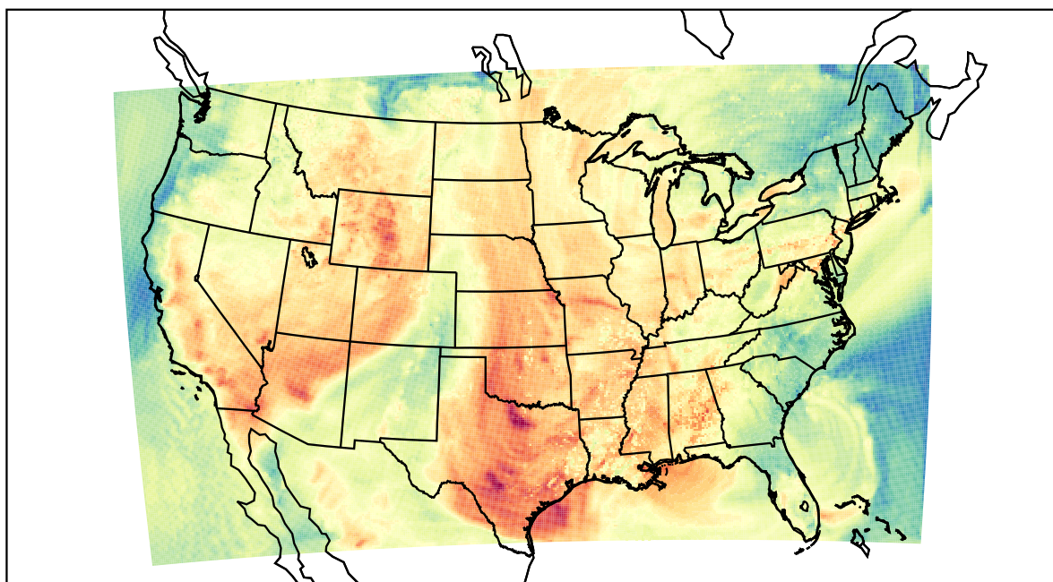
WRF (2023-05-27_23:00:00)
