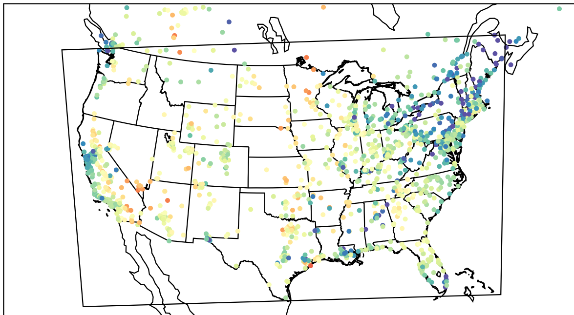
AirNOW (2023-05-27_02:00:00)
