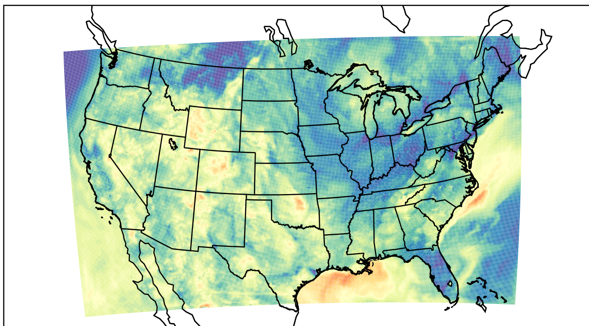
WRF (2023-05-26_09:00:00)
