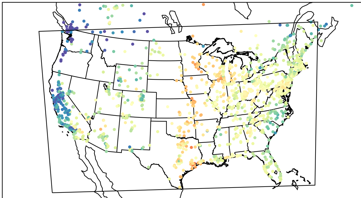
AirNOW (2023-05-27_15:00:00)
