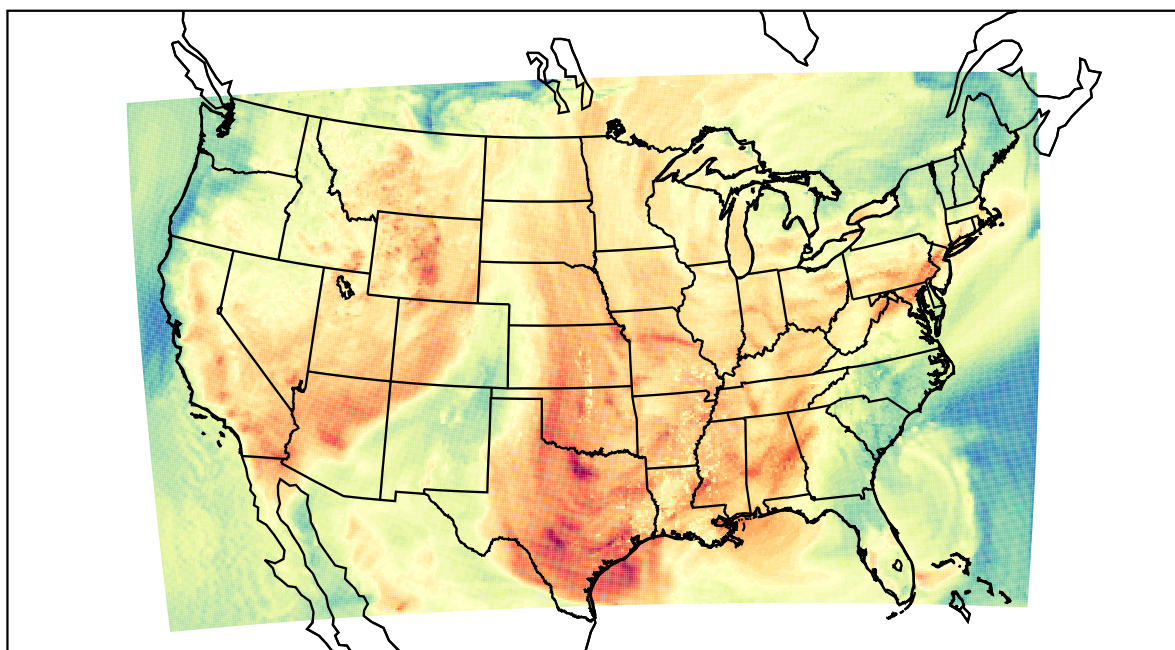
WRF (2023-05-27_22:00:00)
