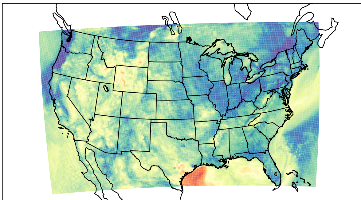
WRF (2023-05-27_11:00:00)
