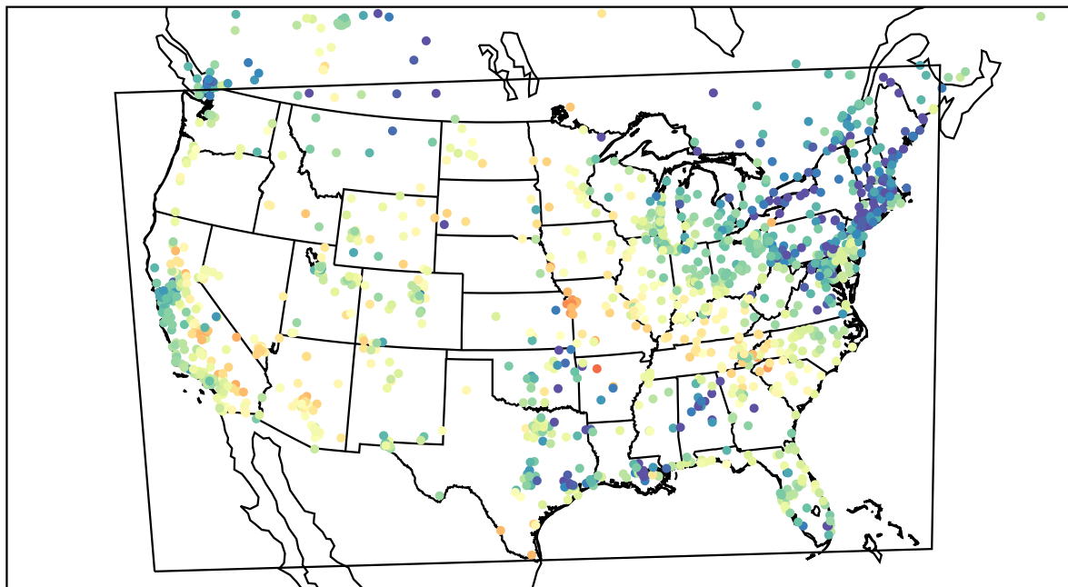
AirNOW (2023-05-26_02:00:00)
