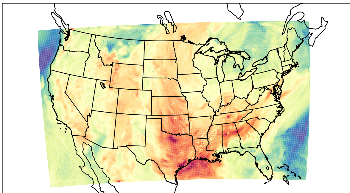
WRF (2023-05-26_21:00:00)
