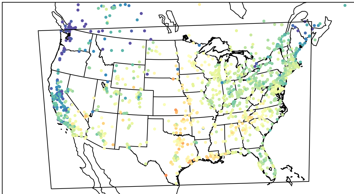
AirNOW (2023-05-26_15:00:00)
