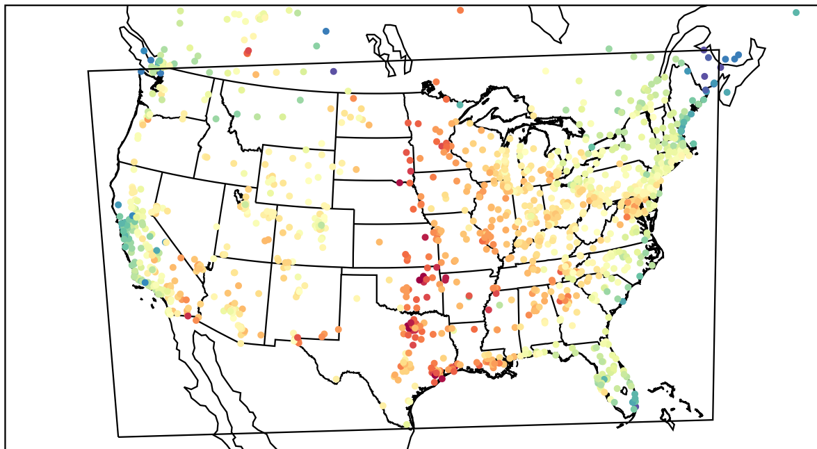
AirNOW (2023-05-26_21:00:00)
