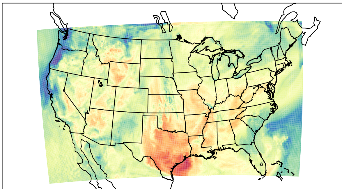
WRF (2023-05-27_16:00:00)
