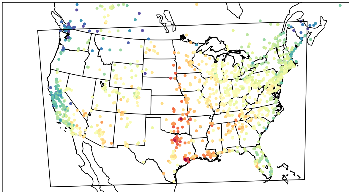
AirNOW (2023-05-26_17:00:00)
