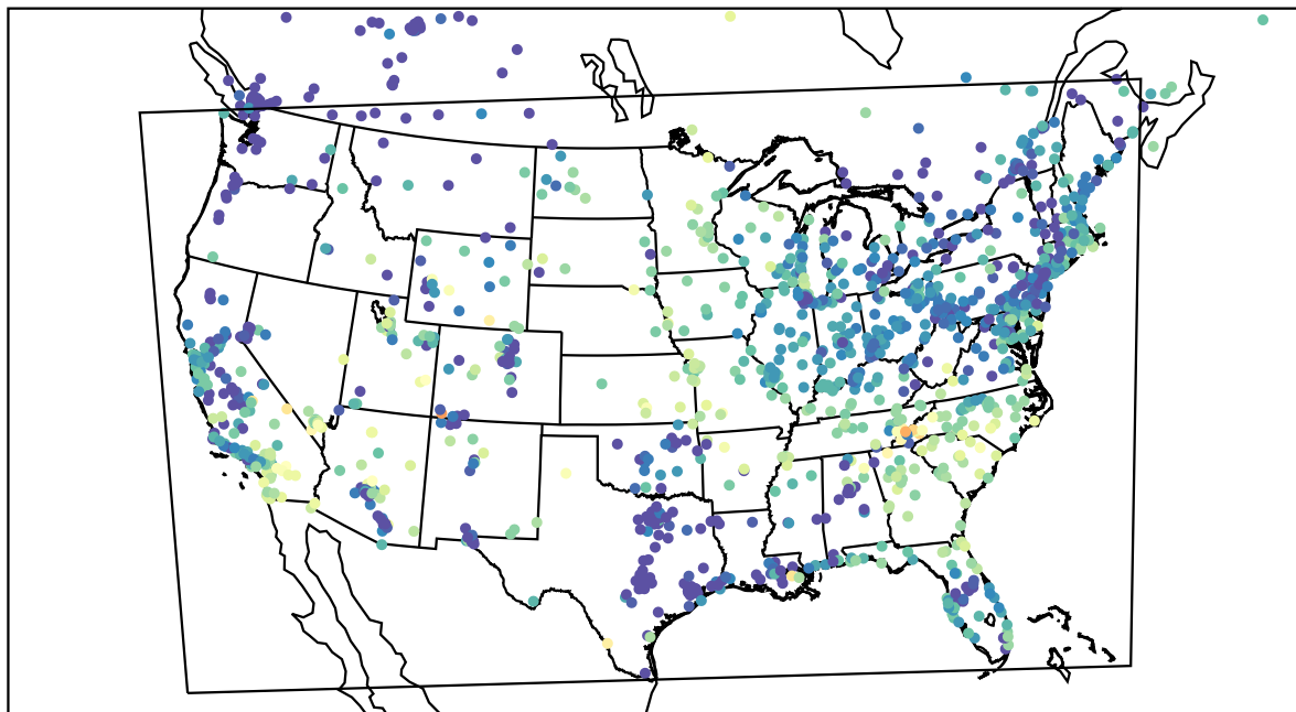
AirNOW (2023-05-26_12:00:00)
