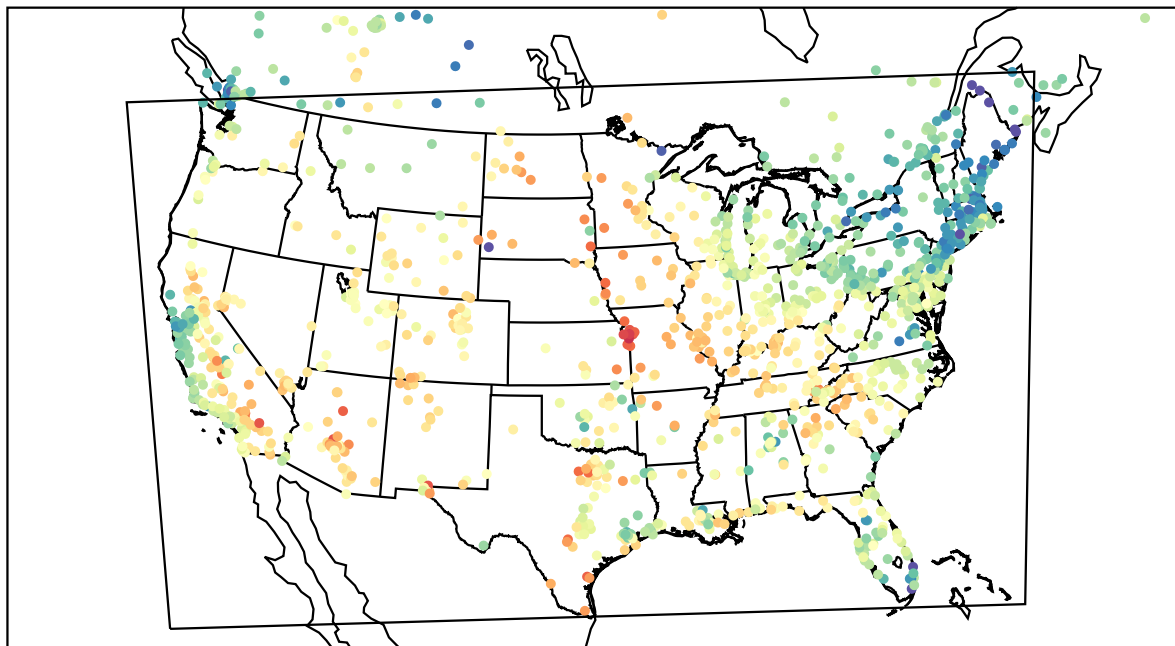
AirNOW (2023-05-26_00:00:00)
