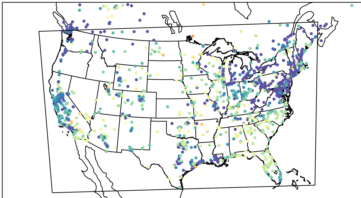
AirNOW (2023-05-27_07:00:00)
