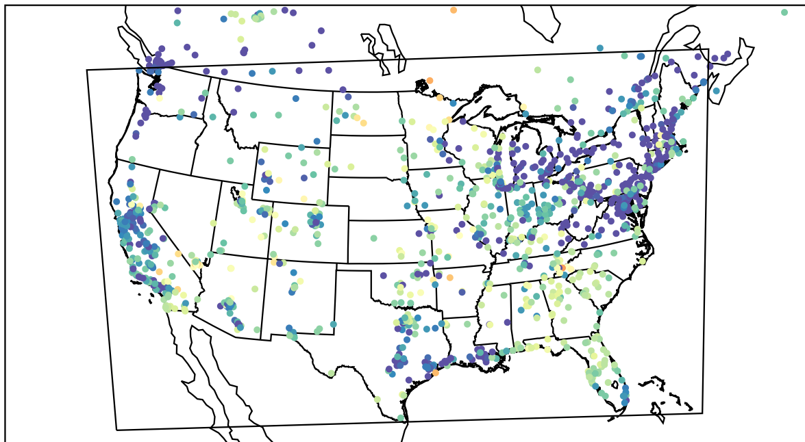
AirNOW (2023-05-27_08:00:00)
