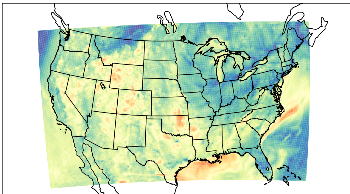
WRF (2023-05-26_04:00:00)
