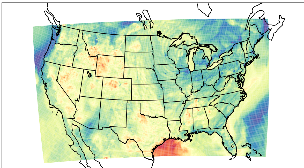
WRF (2023-05-27_03:00:00)
