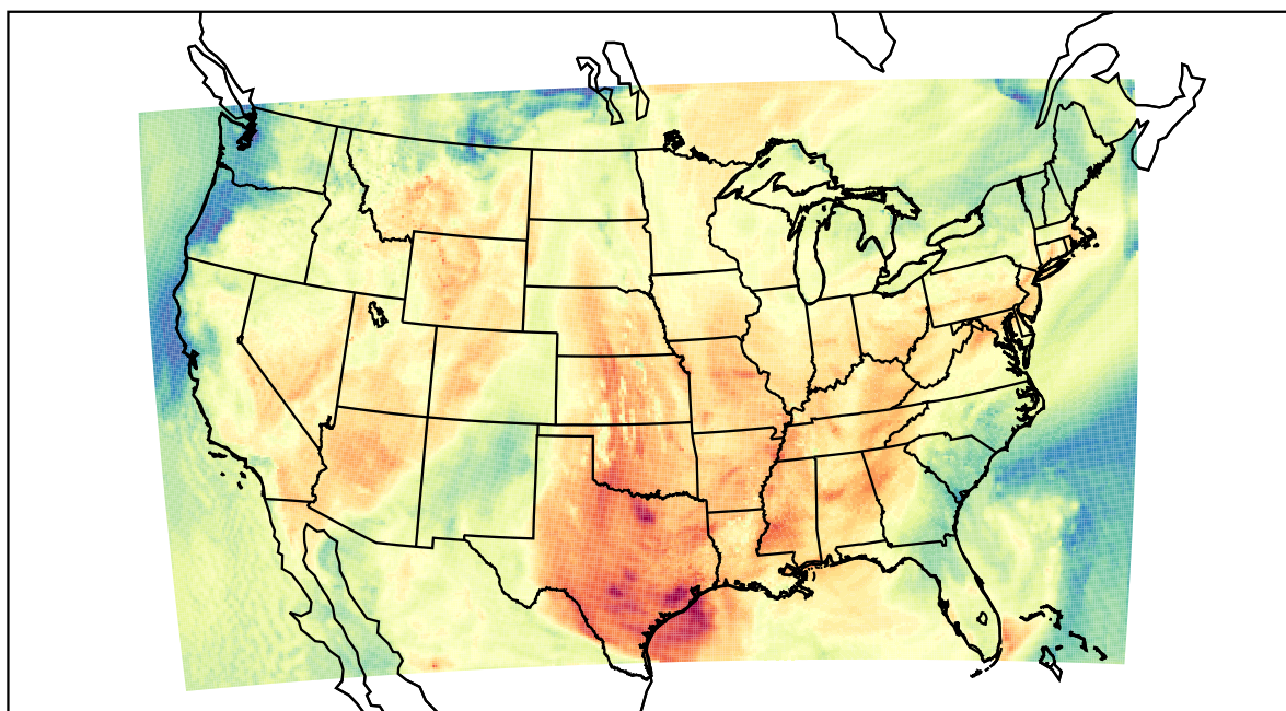
WRF (2023-05-27_18:00:00)
