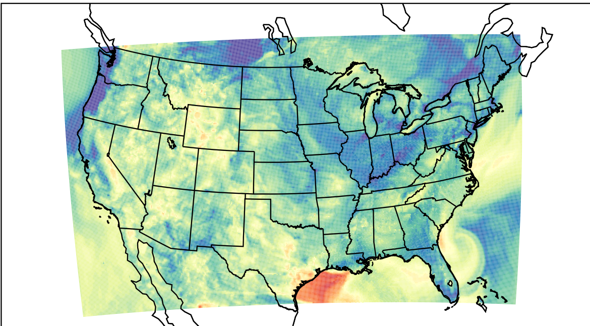
WRF (2023-05-27_10:00:00)
