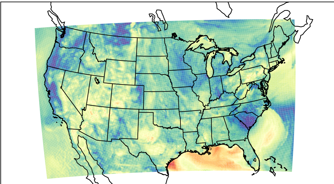
WRF (2023-05-28_13:00:00)
