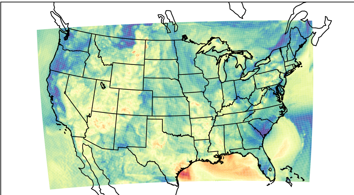
WRF (2023-05-28_09:00:00)
