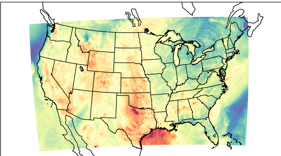
WRF (2023-05-27_00:00:00)
