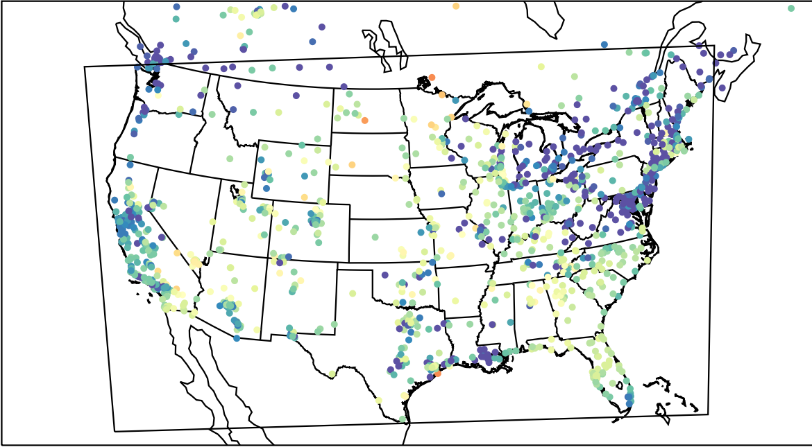
AirNOW (2023-05-27_06:00:00)
