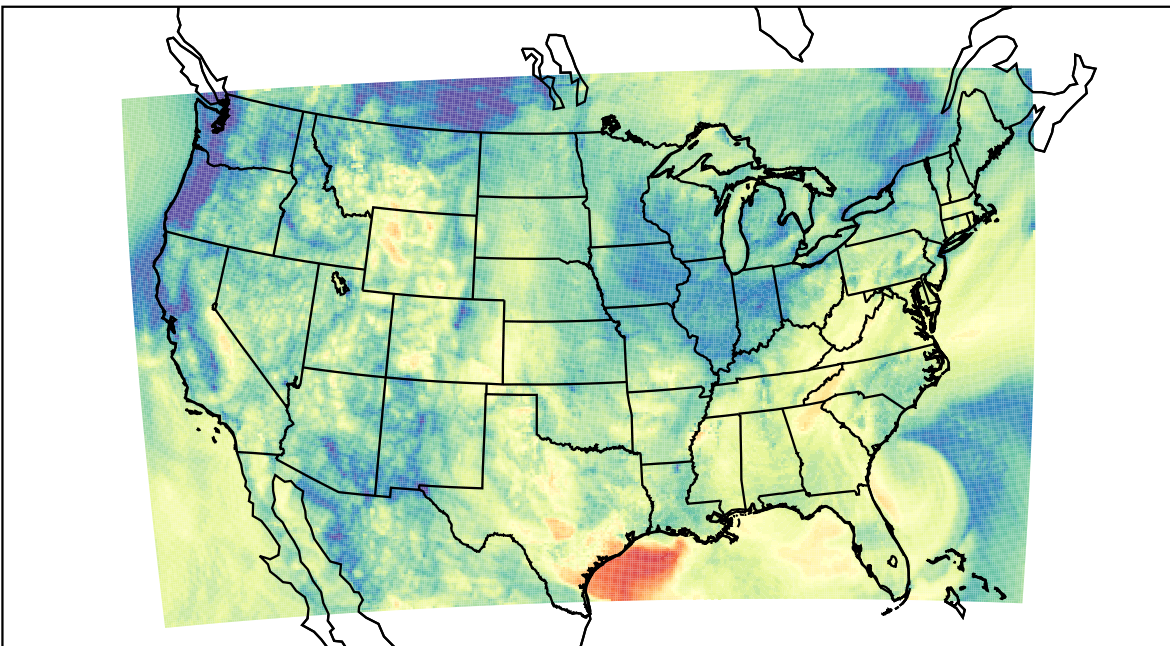
WRF (2023-05-27_14:00:00)
