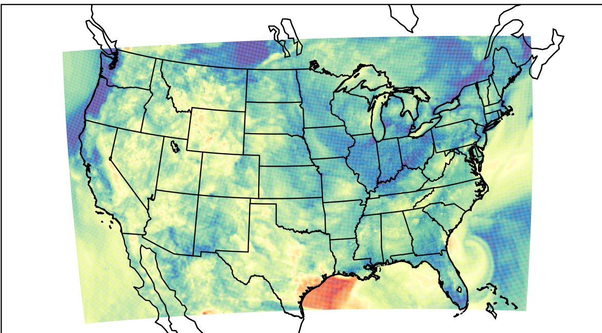
WRF (2023-05-27_09:00:00)
