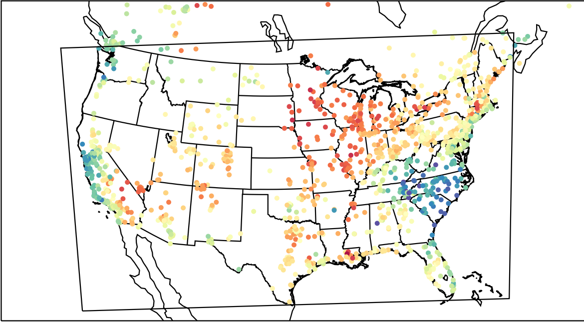
AirNOW (2023-05-28_23:00:00)
