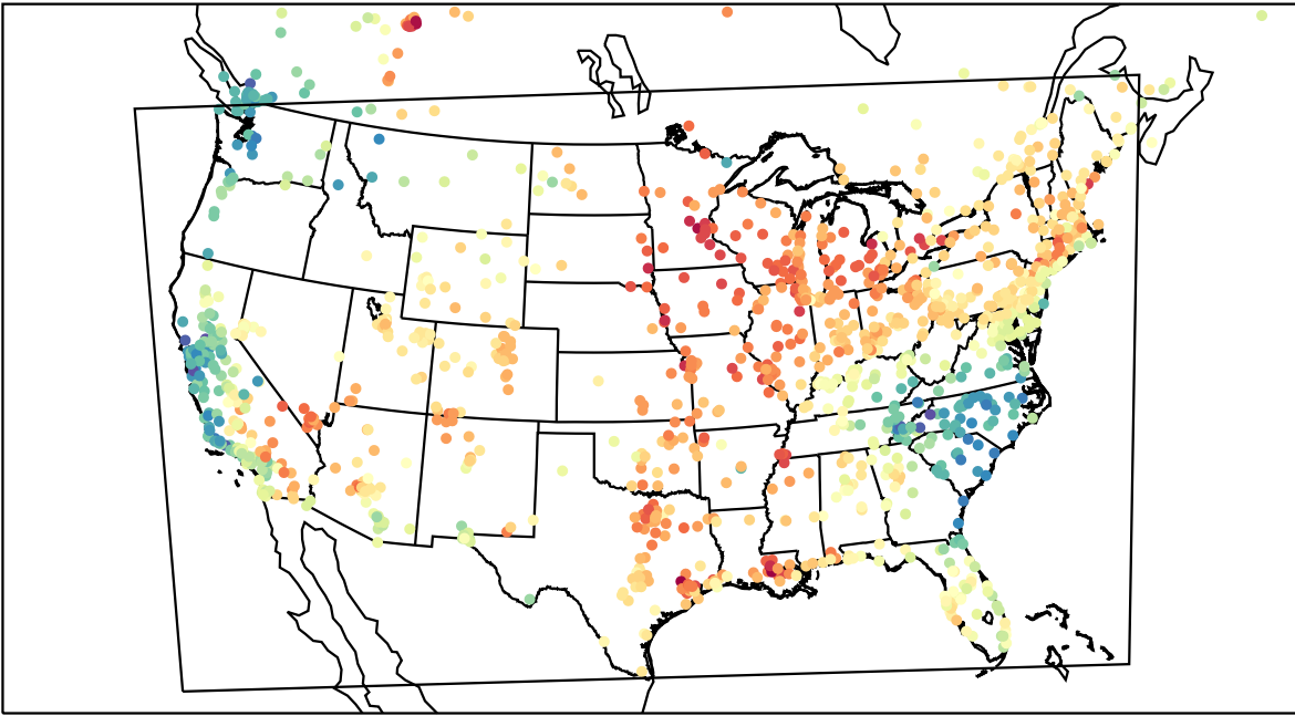
AirNOW (2023-05-28_19:00:00)
