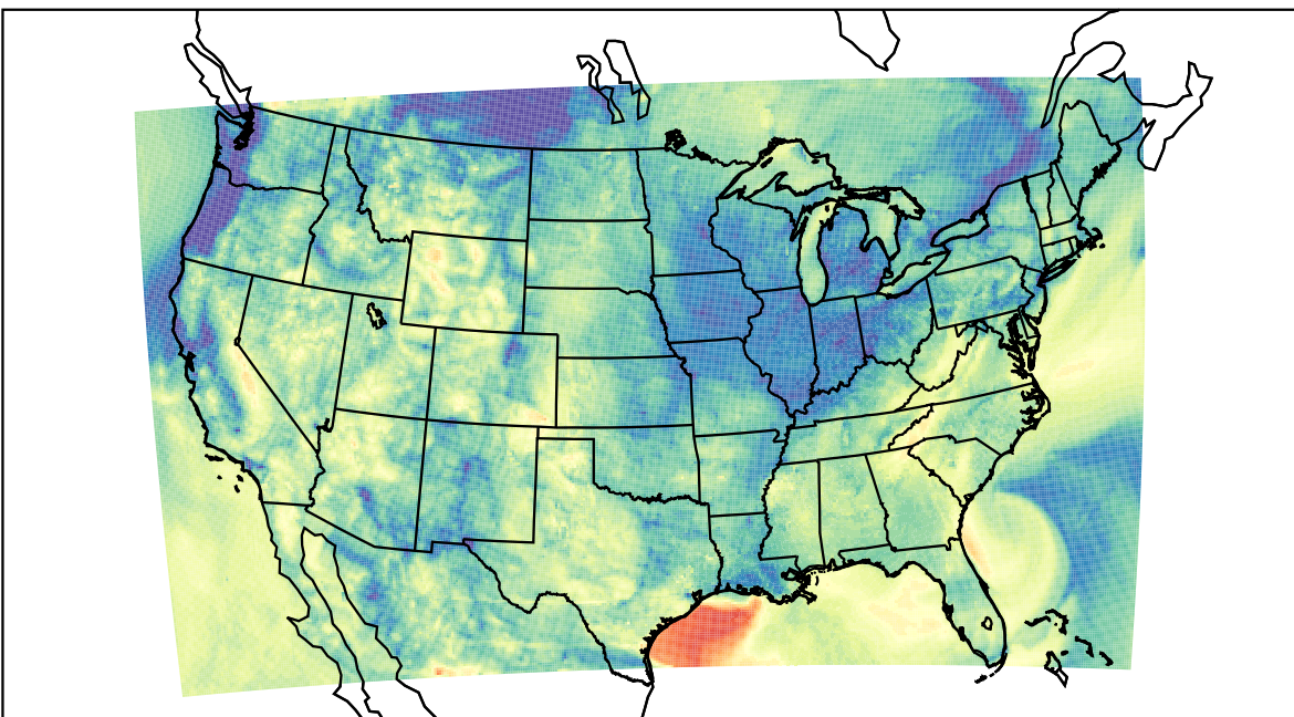
WRF (2023-05-27_13:00:00)
