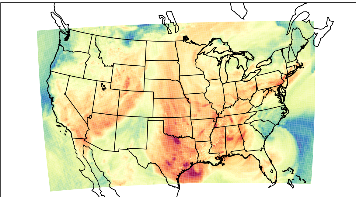
WRF (2023-05-27_21:00:00)
