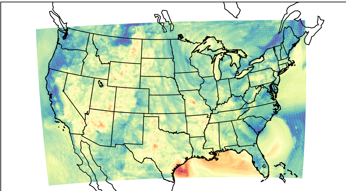
WRF (2023-05-28_06:00:00)
