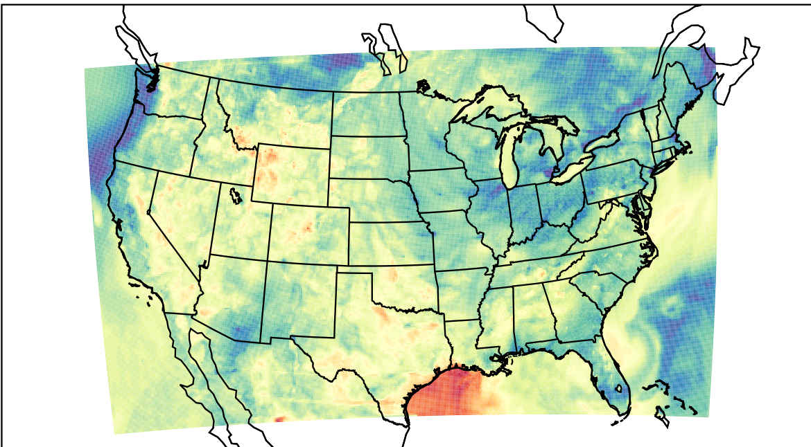
WRF (2023-05-27_04:00:00)
