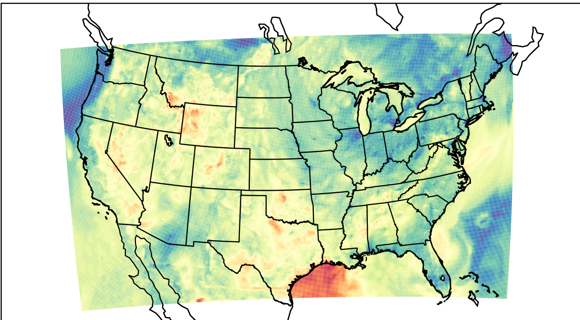
WRF (2023-05-27_03:00:00)
