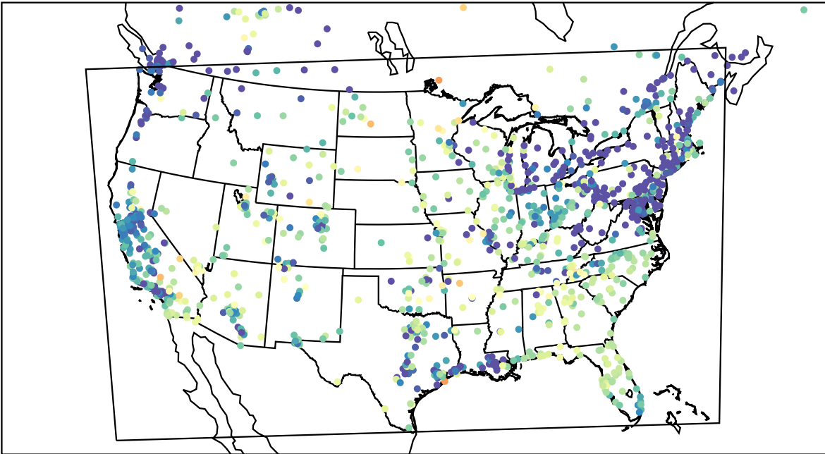
AirNOW (2023-05-27_07:00:00)
