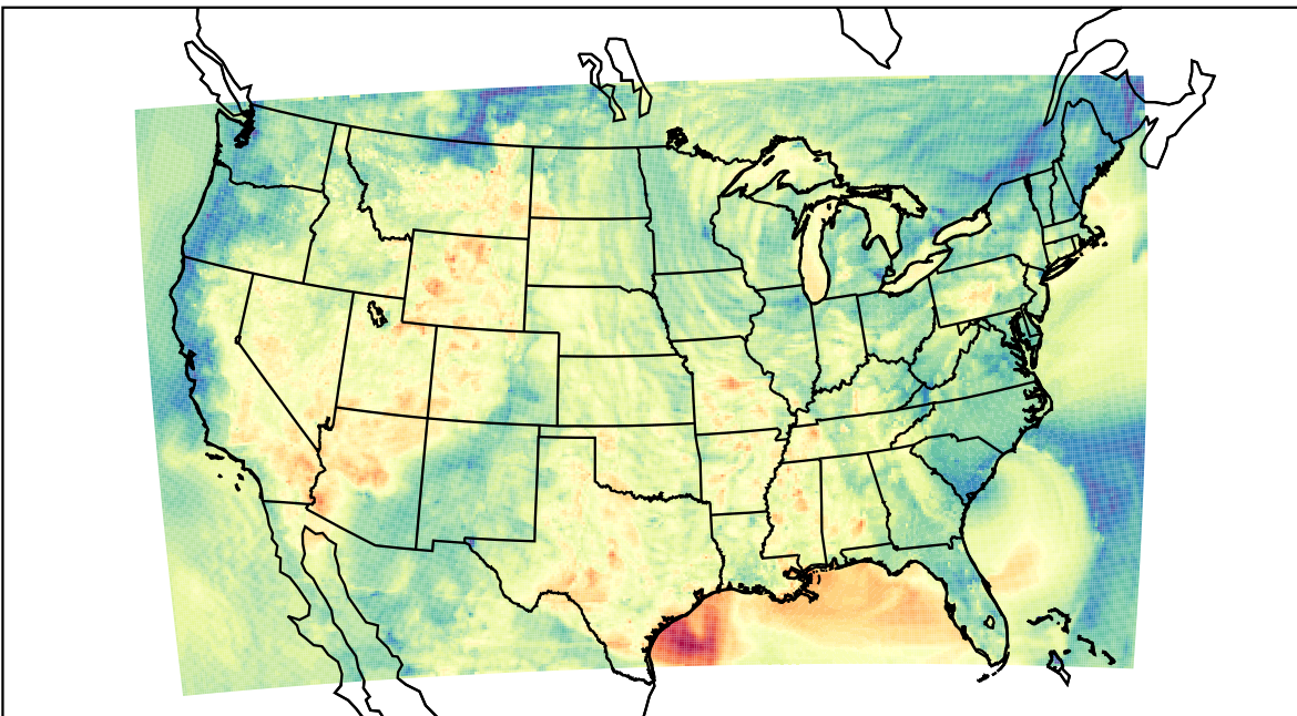
WRF (2023-05-28_03:00:00)
