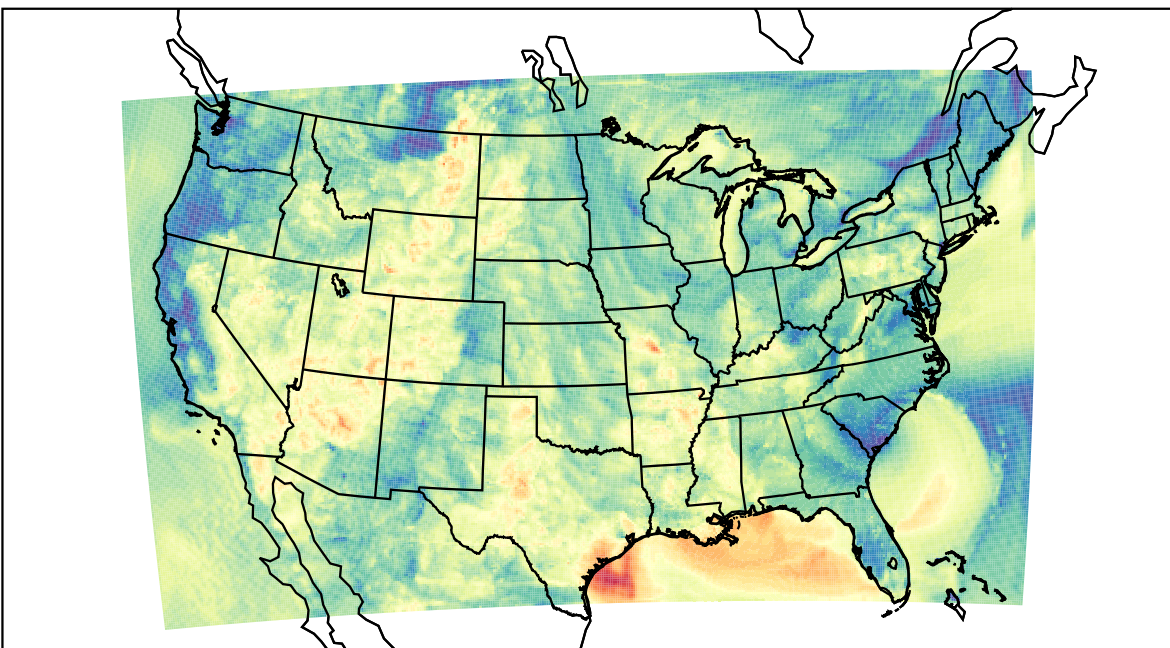
WRF (2023-05-28_07:00:00)
