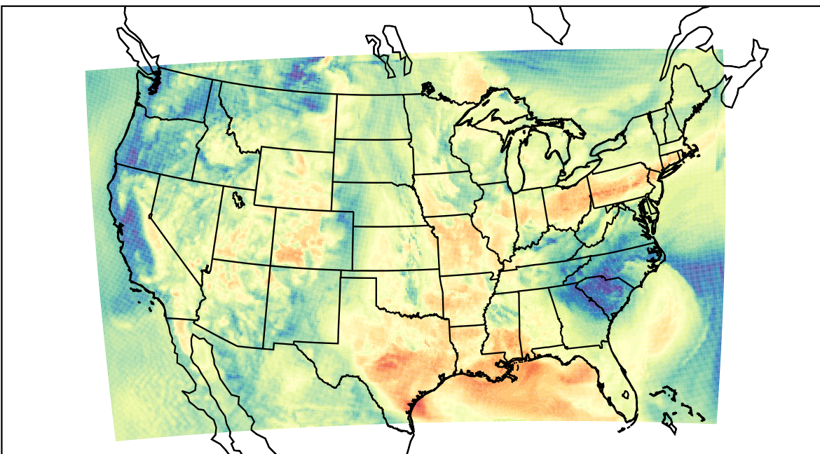
WRF (2023-05-28_15:00:00)
