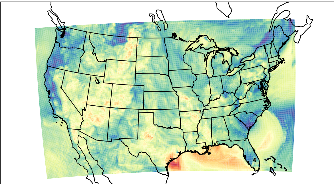
WRF (2023-05-28_08:00:00)
