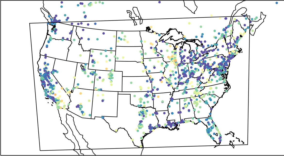
AirNOW (2023-05-28_08:00:00)
