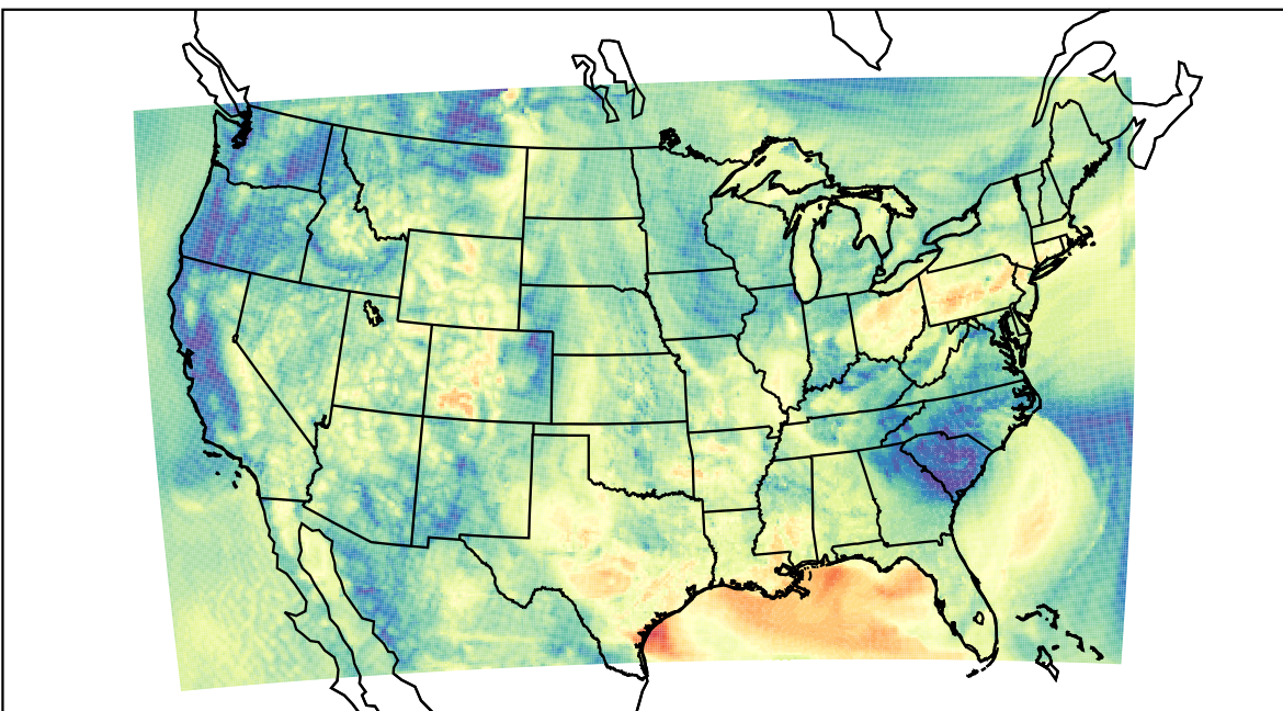
WRF (2023-05-28_14:00:00)
