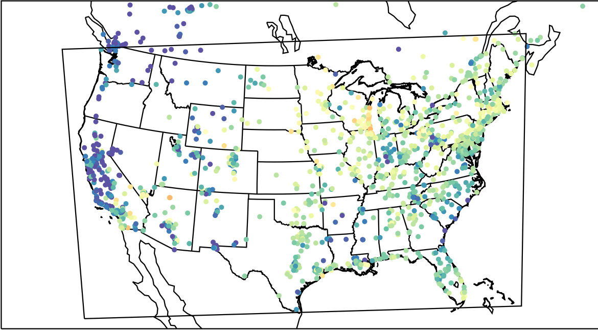
AirNOW (2023-05-28_13:00:00)
