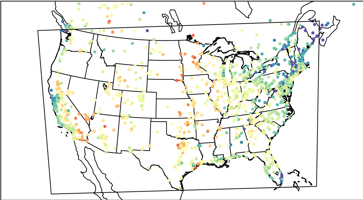
AirNOW (2023-05-27_01:00:00)
