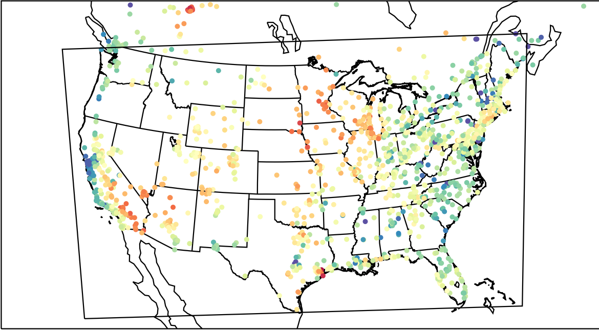
AirNOW (2023-05-28_01:00:00)
