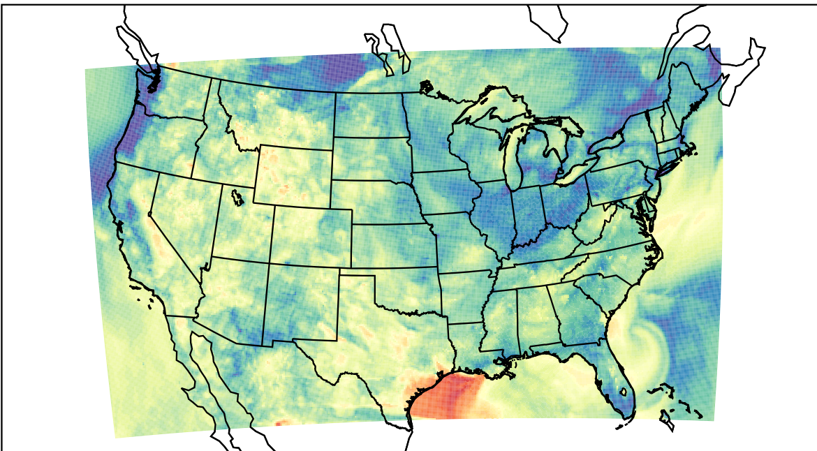
WRF (2023-05-27_08:00:00)
