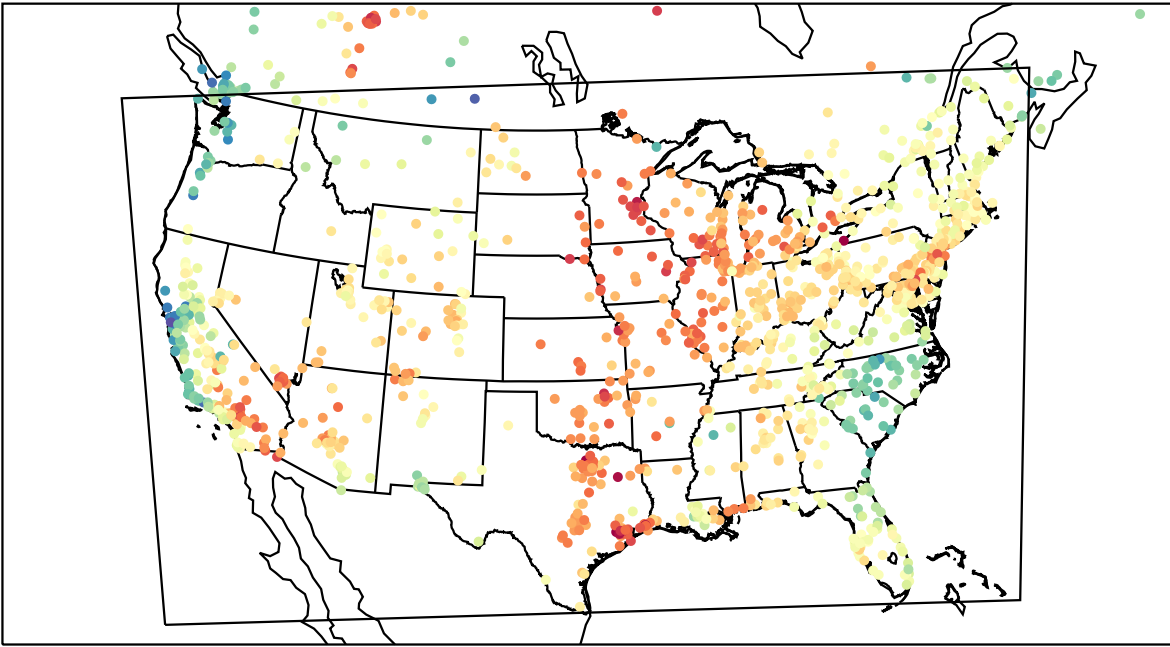
AirNOW (2023-05-27_21:00:00)
