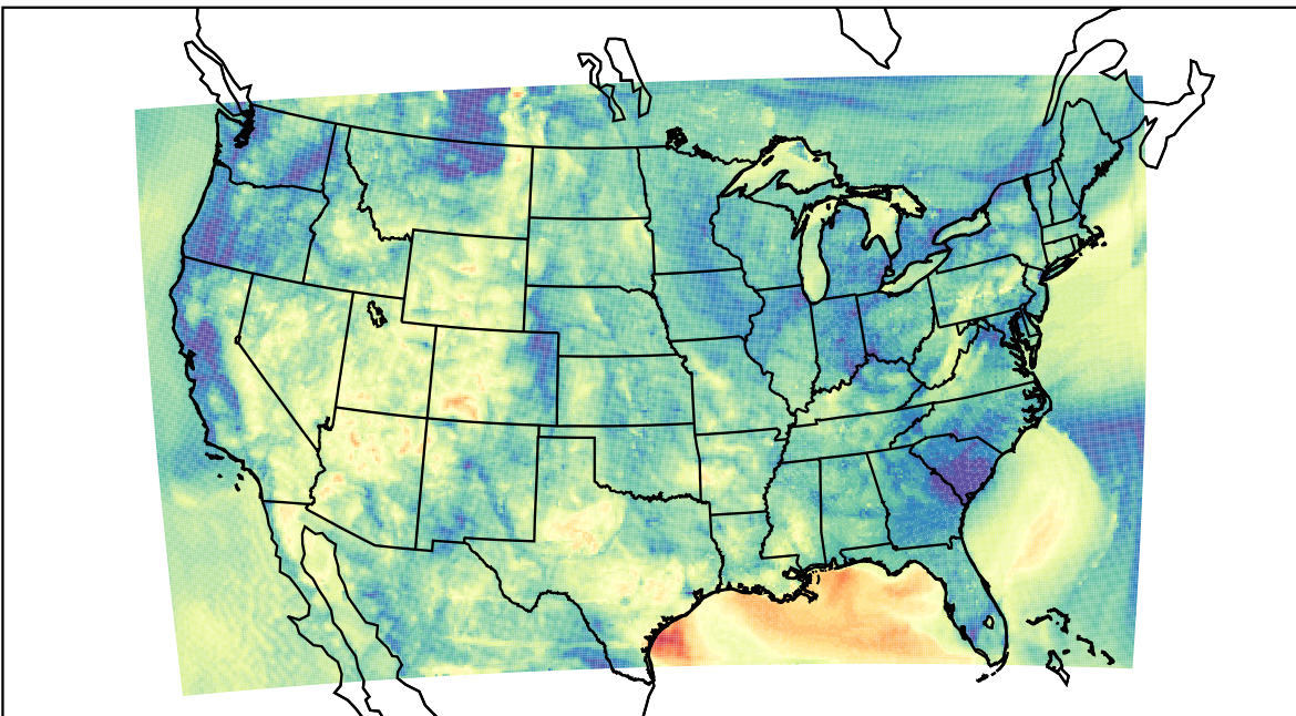
WRF (2023-05-28_12:00:00)
