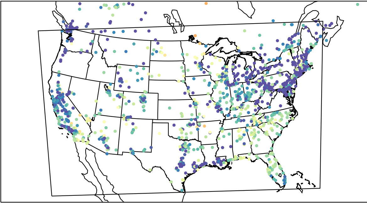
AirNOW (2023-05-27_09:00:00)
