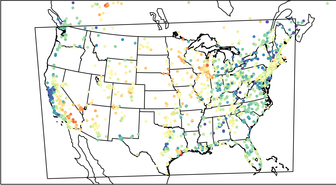
AirNOW (2023-05-28_02:00:00)
