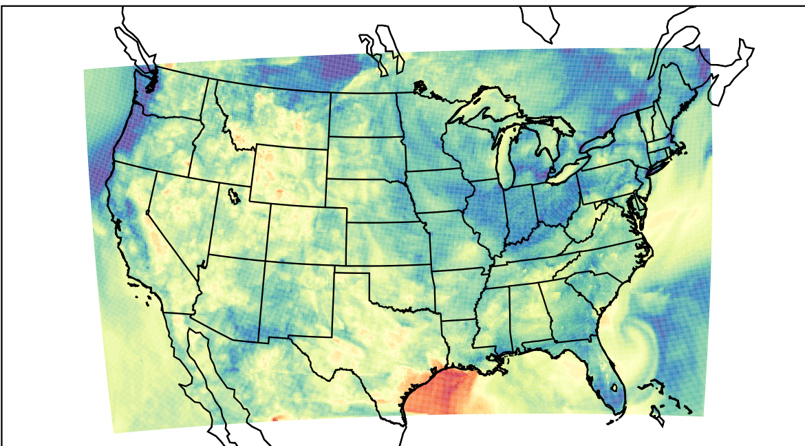
WRF (2023-05-27_07:00:00)
