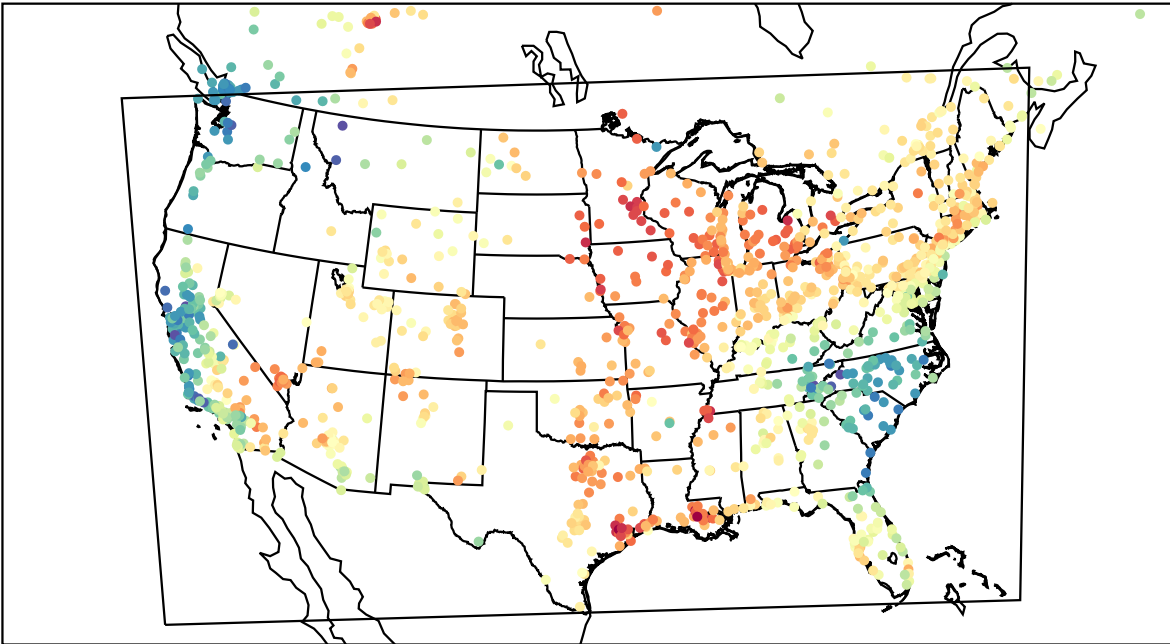
AirNOW (2023-05-28_18:00:00)
