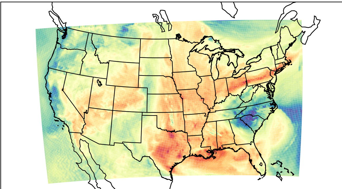
WRF (2023-05-28_17:00:00)
