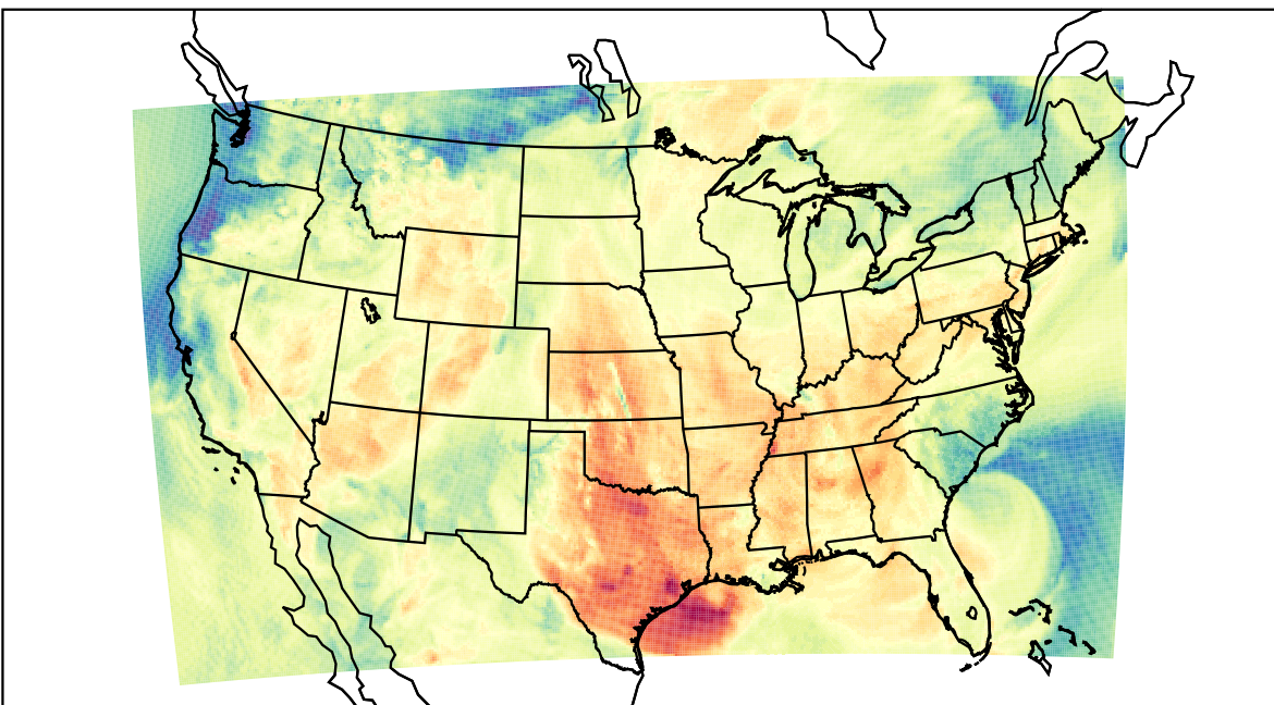
WRF (2023-05-27_17:00:00)
