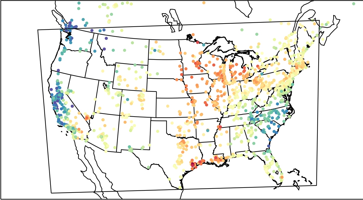
AirNOW (2023-05-28_16:00:00)
