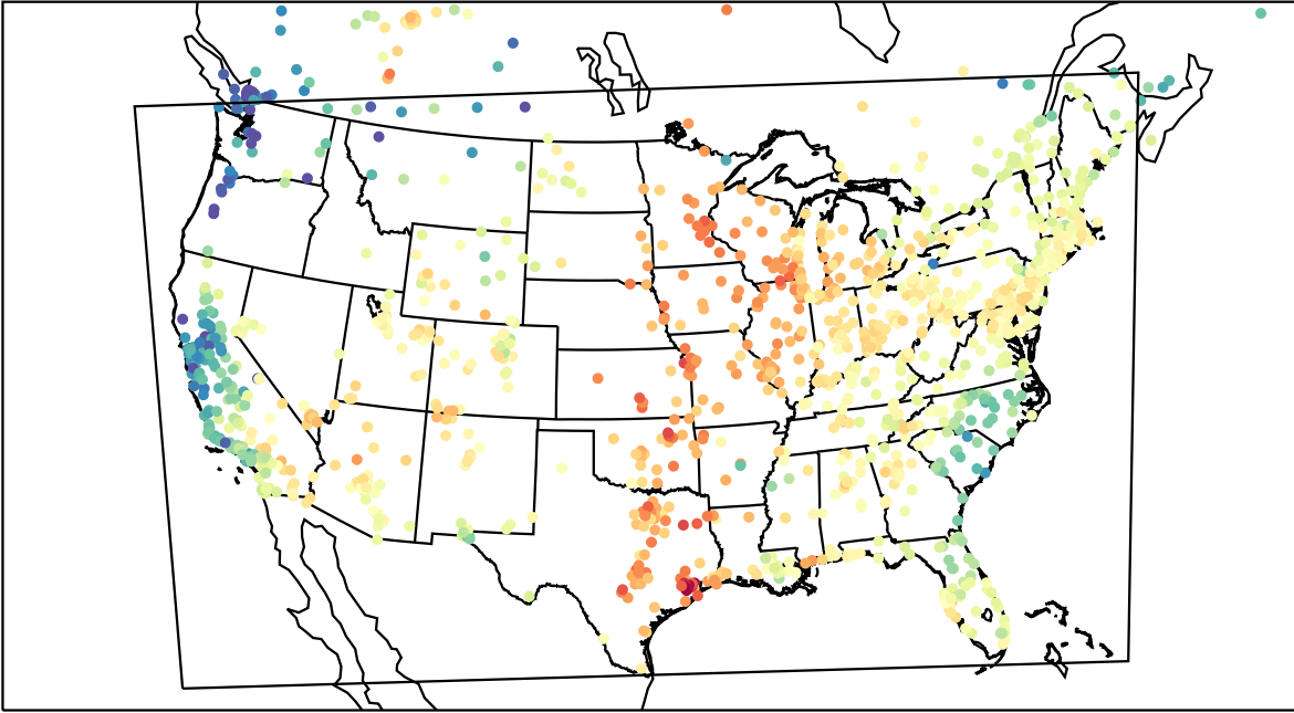
AirNOW (2023-05-27_17:00:00)
