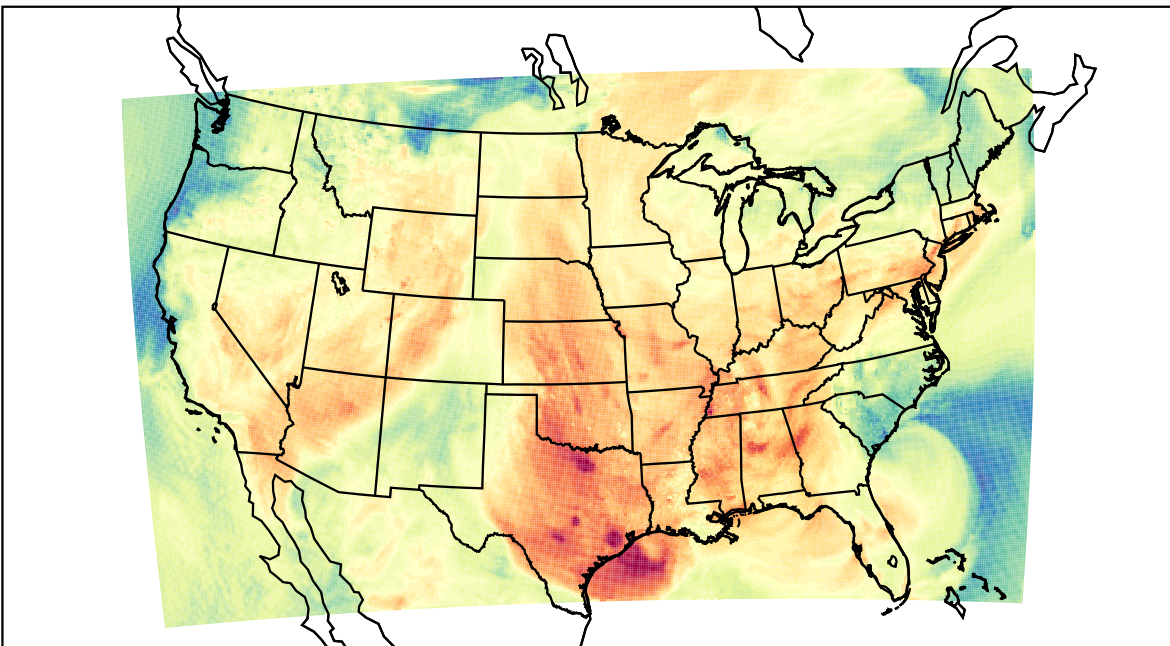
WRF (2023-05-27_19:00:00)
