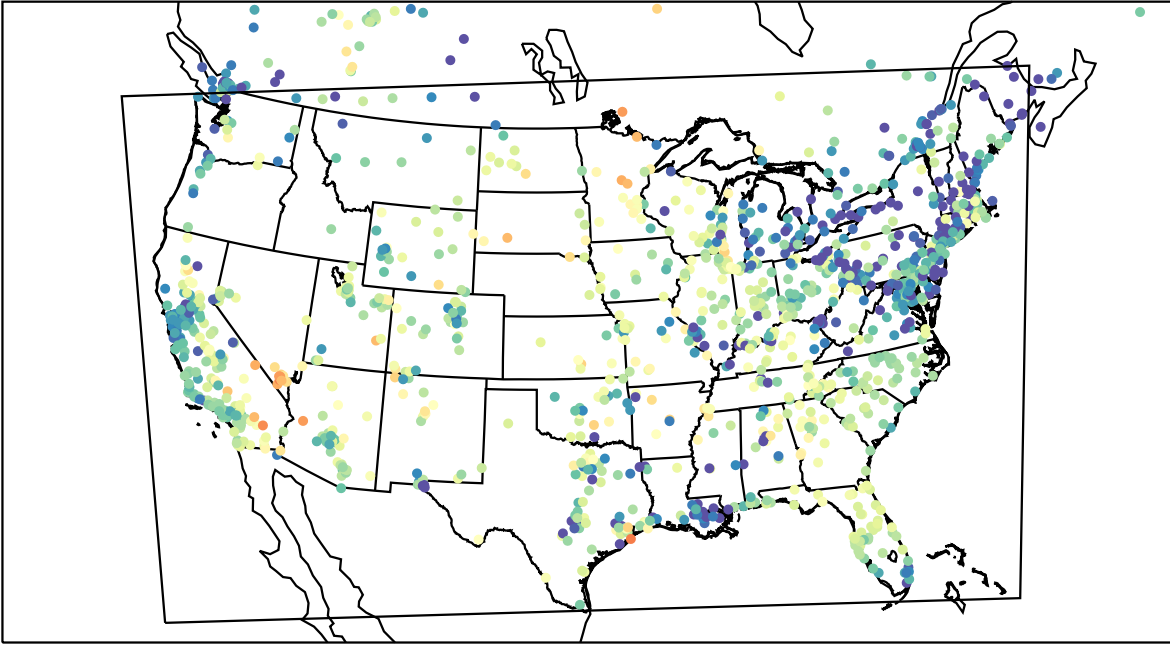
AirNOW (2023-05-27_04:00:00)
