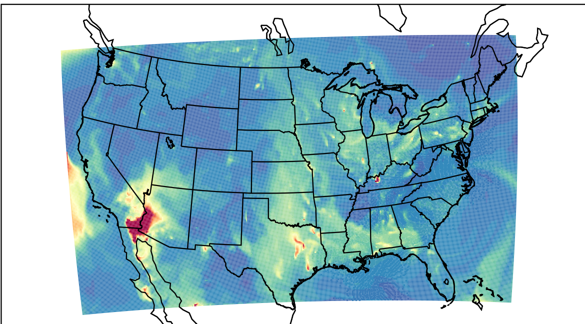
WRF 2023-05-29_08:00:00
