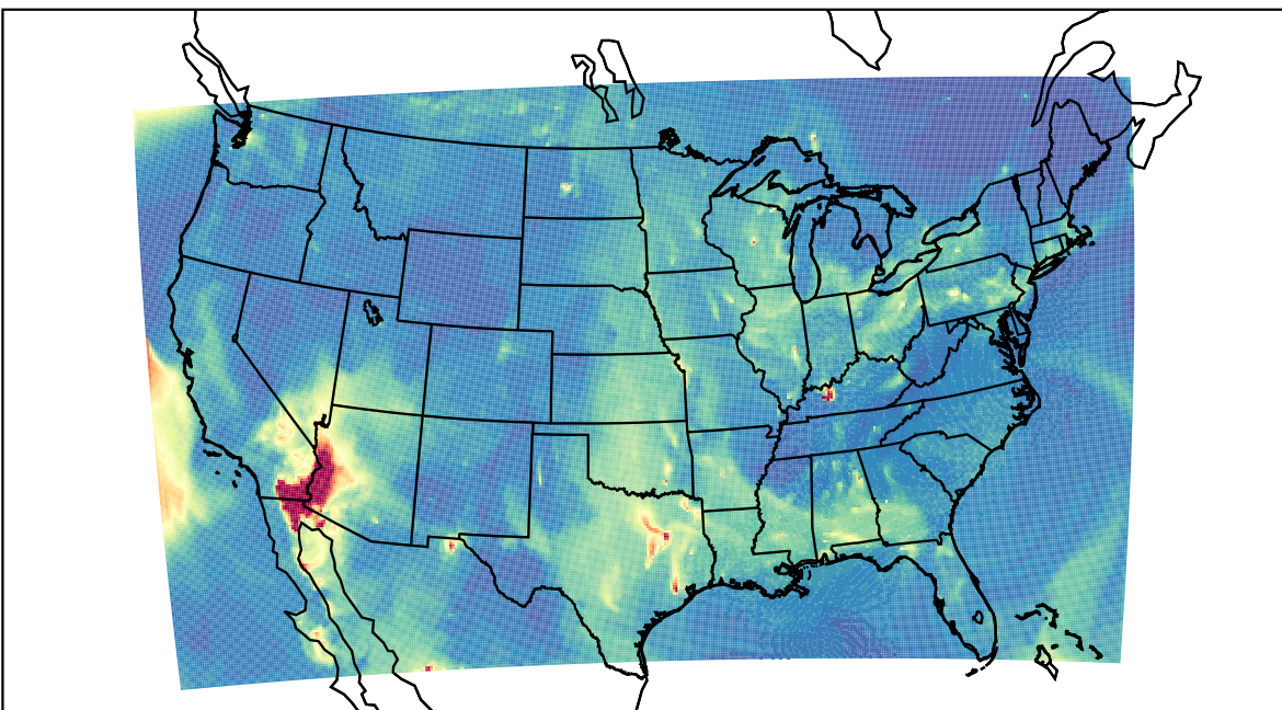
WRF 2023-05-29_09:00:00
