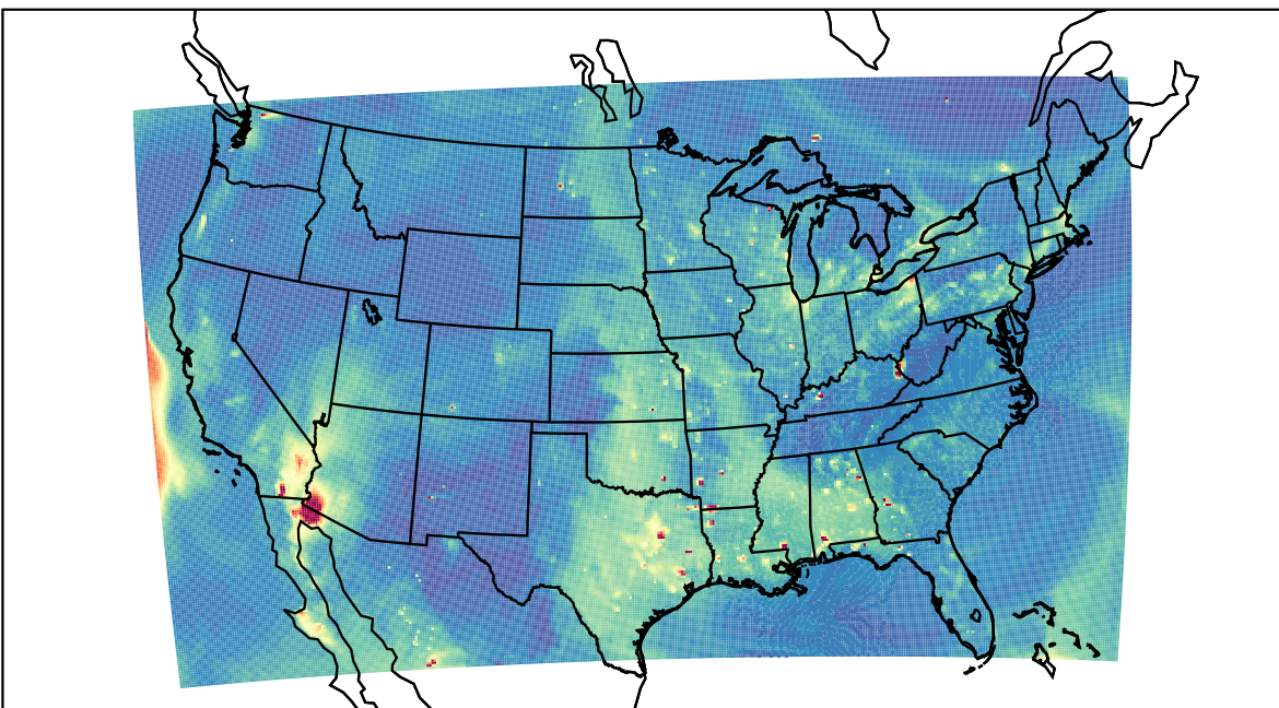
WRF 2023-05-29_01:00:00
