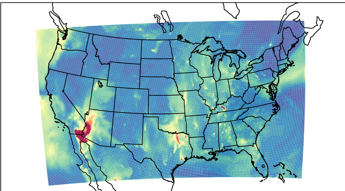
WRF 2023-05-30_12:00:00
