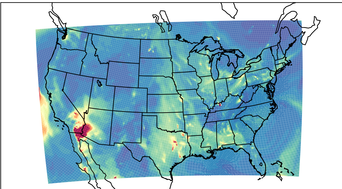
WRF 2023-05-29_06:00:00
