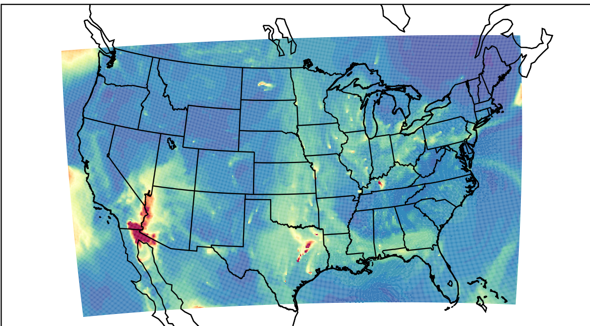
WRF 2023-05-29_14:00:00
