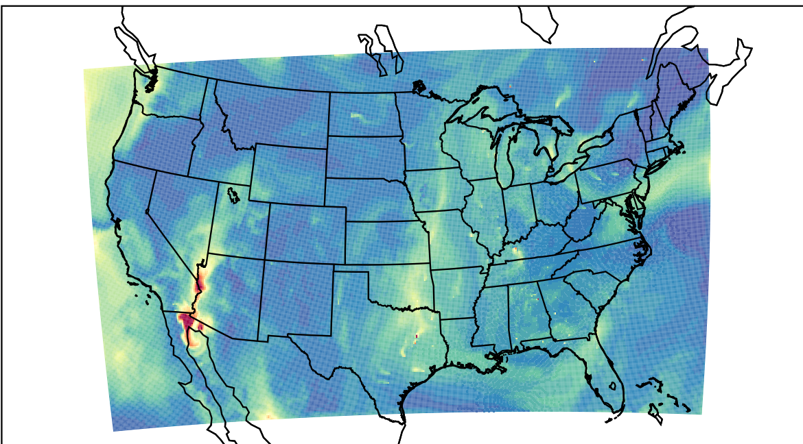
WRF 2023-05-30_17:00:00
