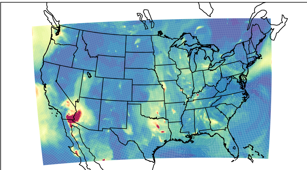
WRF 2023-05-30_06:00:00
