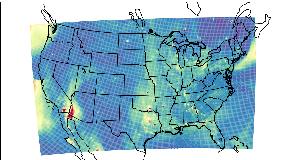
WRF 2023-05-30_01:00:00
