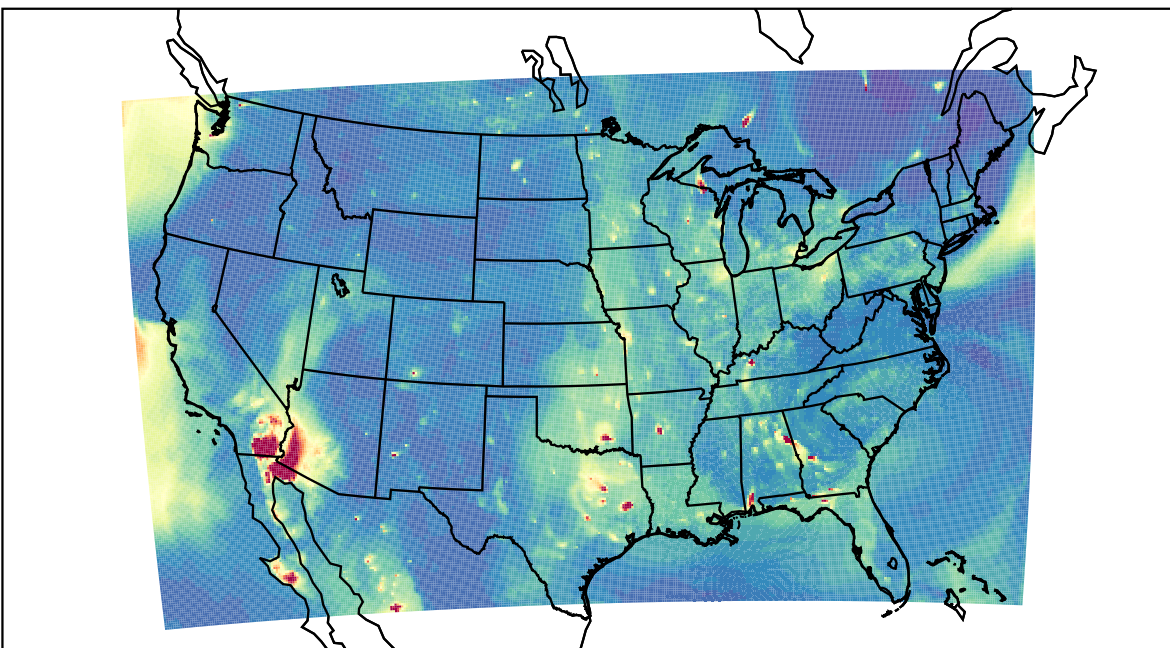
WRF 2023-05-30_02:00:00
