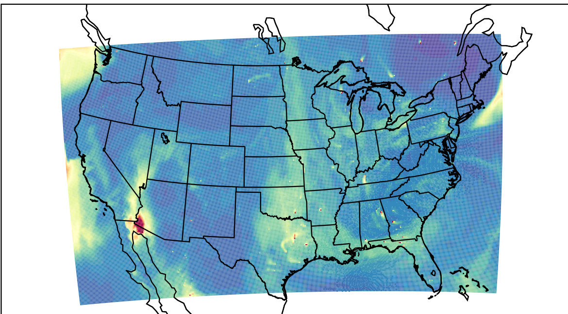
WRF 2023-05-29_21:00:00
