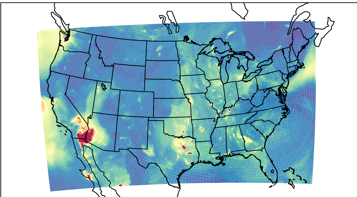
WRF 2023-05-30_05:00:00
