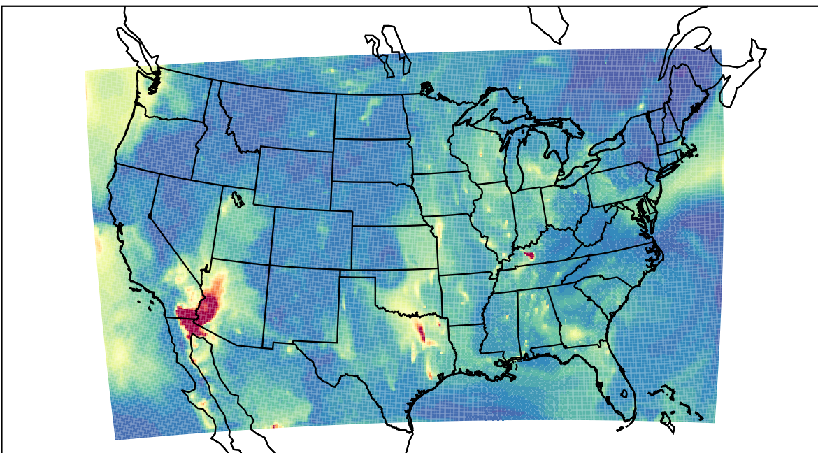
WRF 2023-05-30_10:00:00
