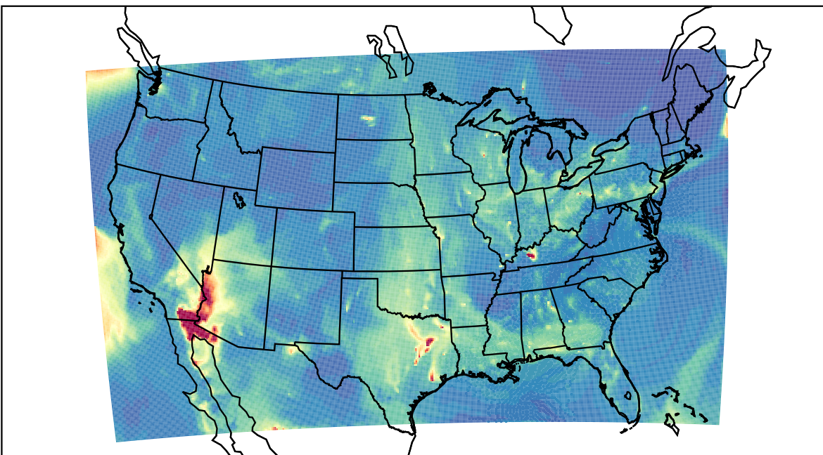
WRF 2023-05-29_12:00:00
