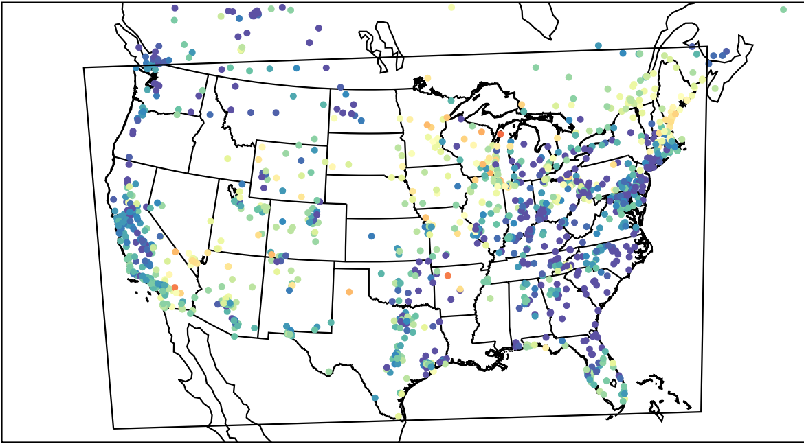
AirNOW (2023-05-29_07:00:00)
