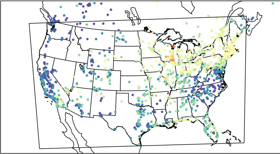
AirNOW (2023-05-29_13:00:00)
