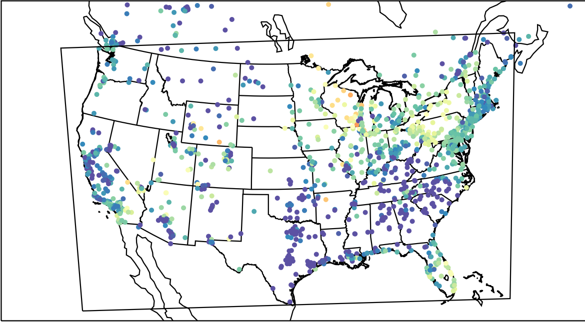
AirNOW (2023-05-30_12:00:00)
