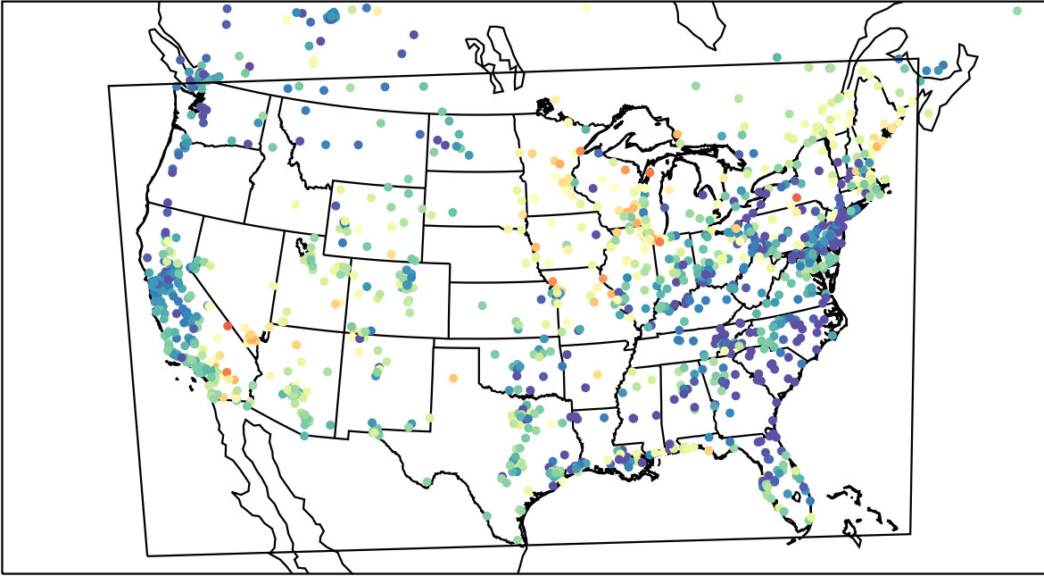
AirNOW (2023-05-29_05:00:00)
