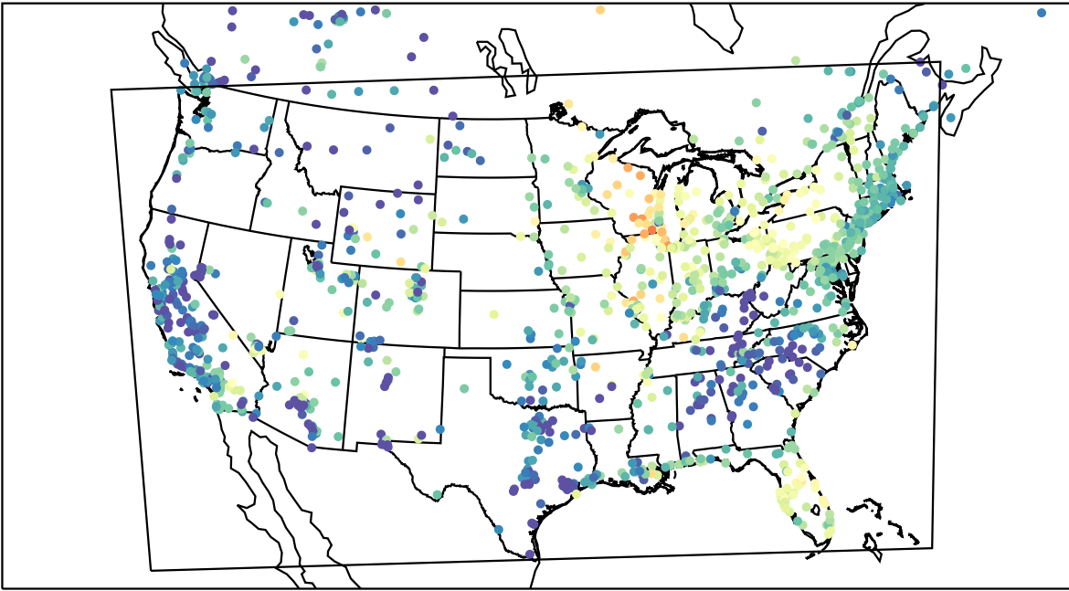
AirNOW (2023-05-30_13:00:00)
