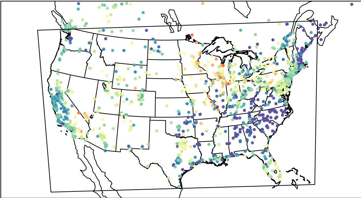
AirNOW (2023-05-30_04:00:00)
