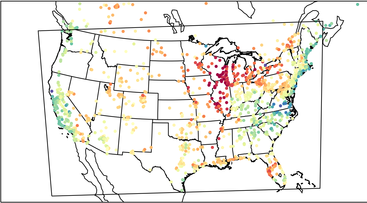
AirNOW (2023-05-30_21:00:00)
