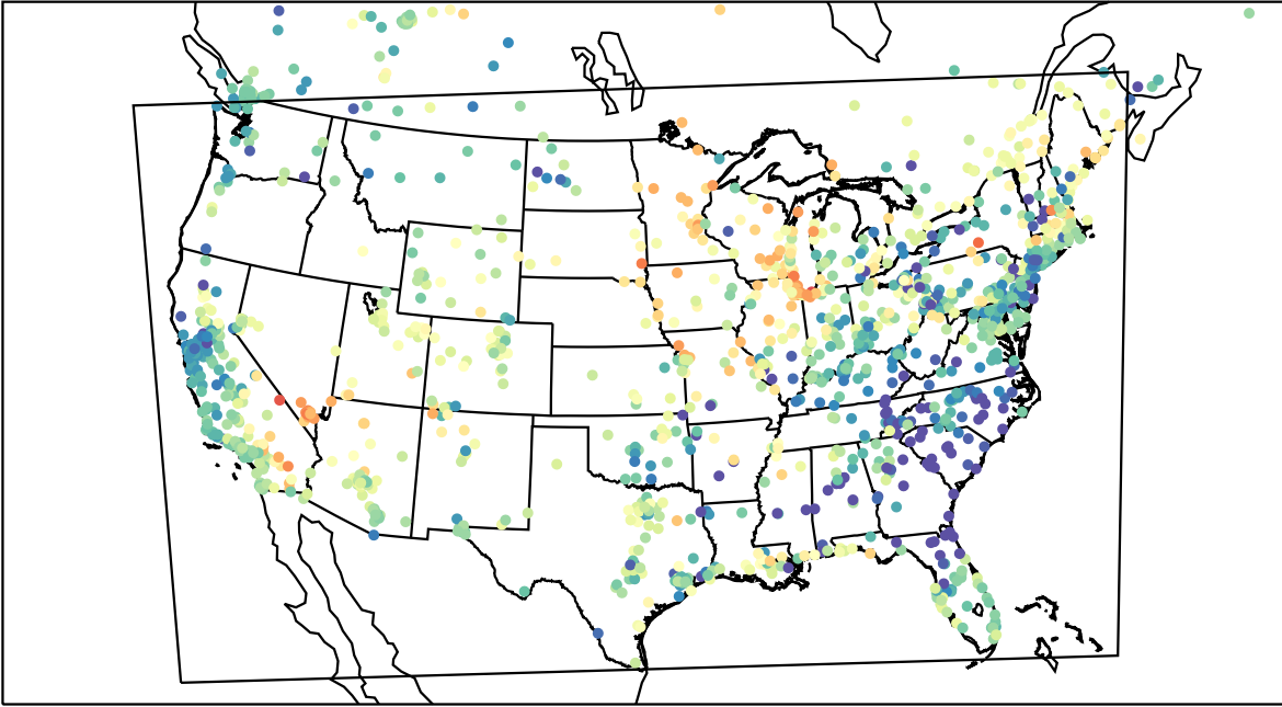
AirNOW (2023-05-29_03:00:00)
