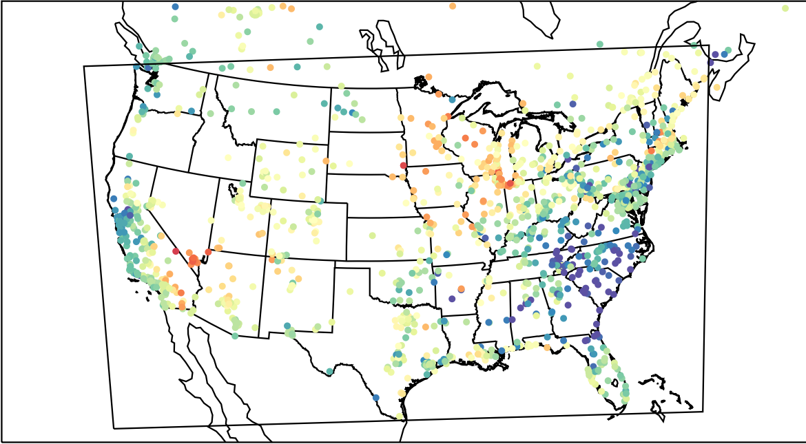
AirNOW (2023-05-29_02:00:00)
