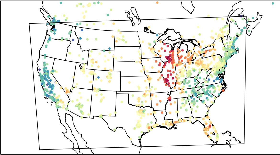
AirNOW (2023-05-30_16:00:00)
