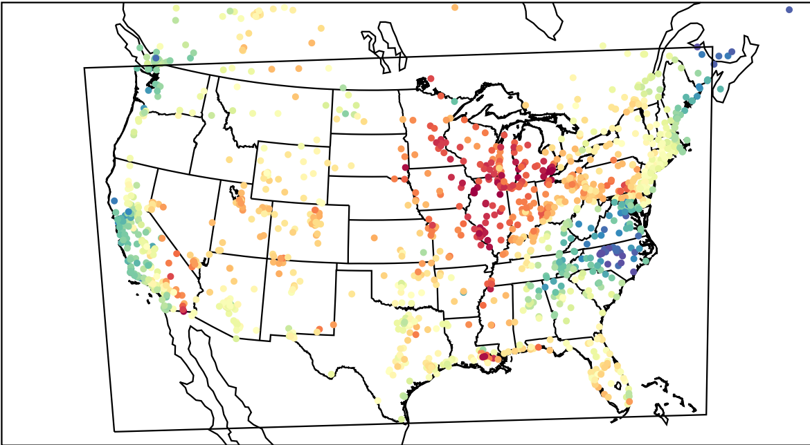
AirNOW (2023-05-29_22:00:00)
