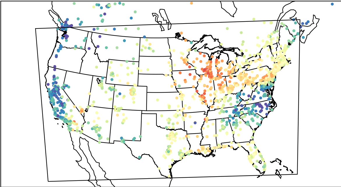
AirNOW (2023-05-29_15:00:00)
