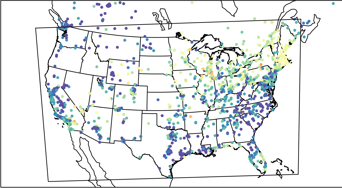
AirNOW (2023-05-29_12:00:00)
