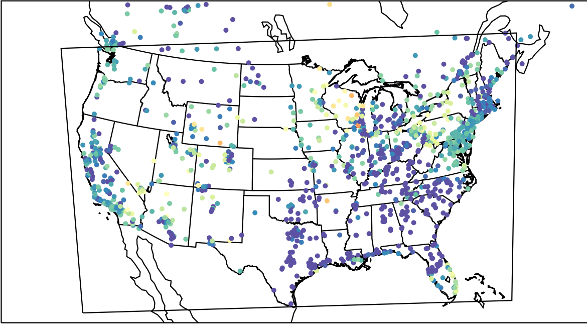
AirNOW (2023-05-30_11:00:00)
