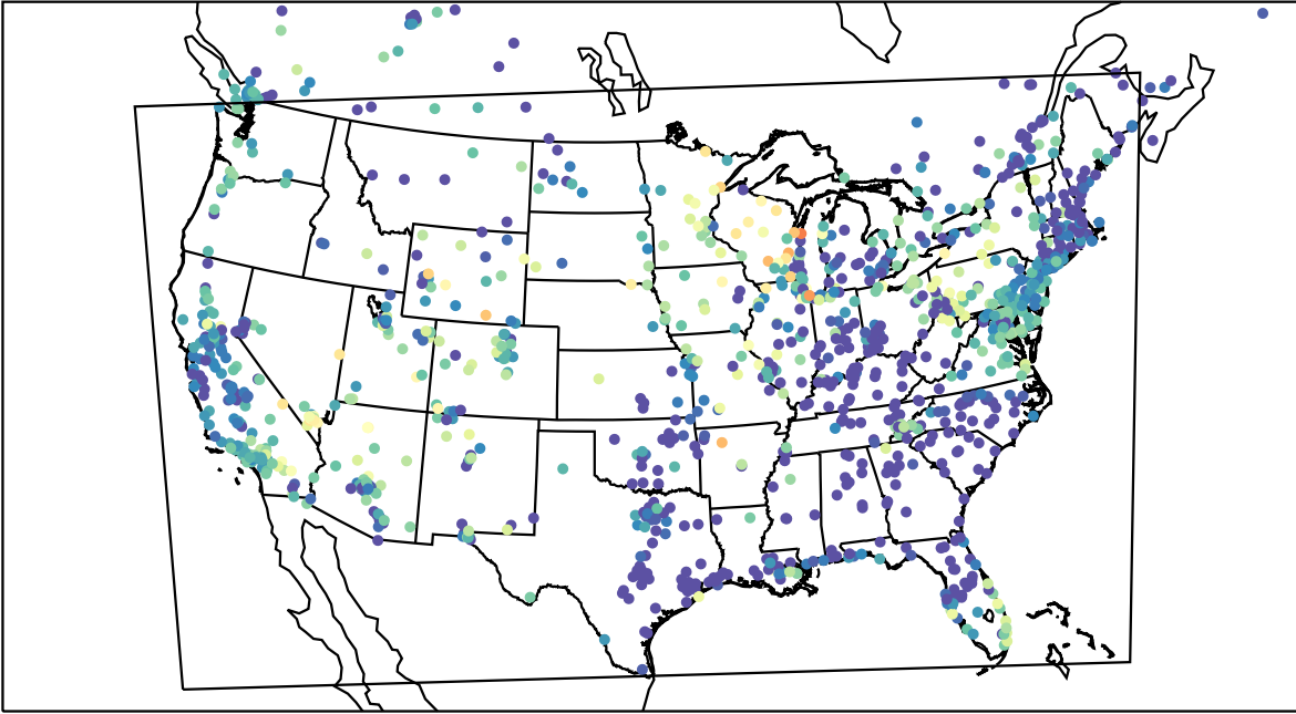
AirNOW (2023-05-30_10:00:00)
