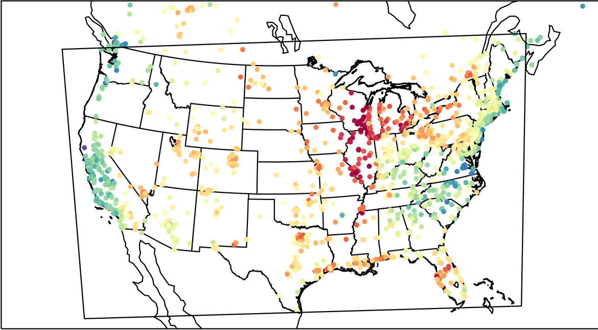
AirNOW (2023-05-30_18:00:00)
