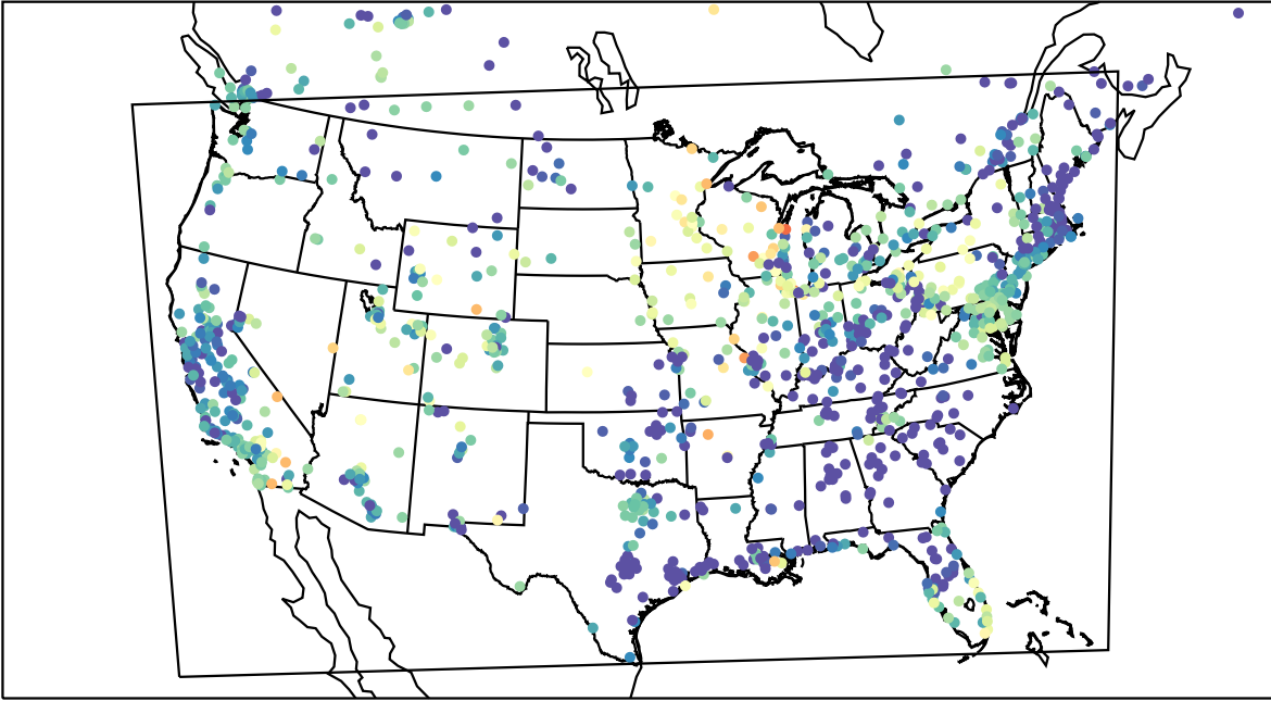
AirNOW (2023-05-30_08:00:00)
