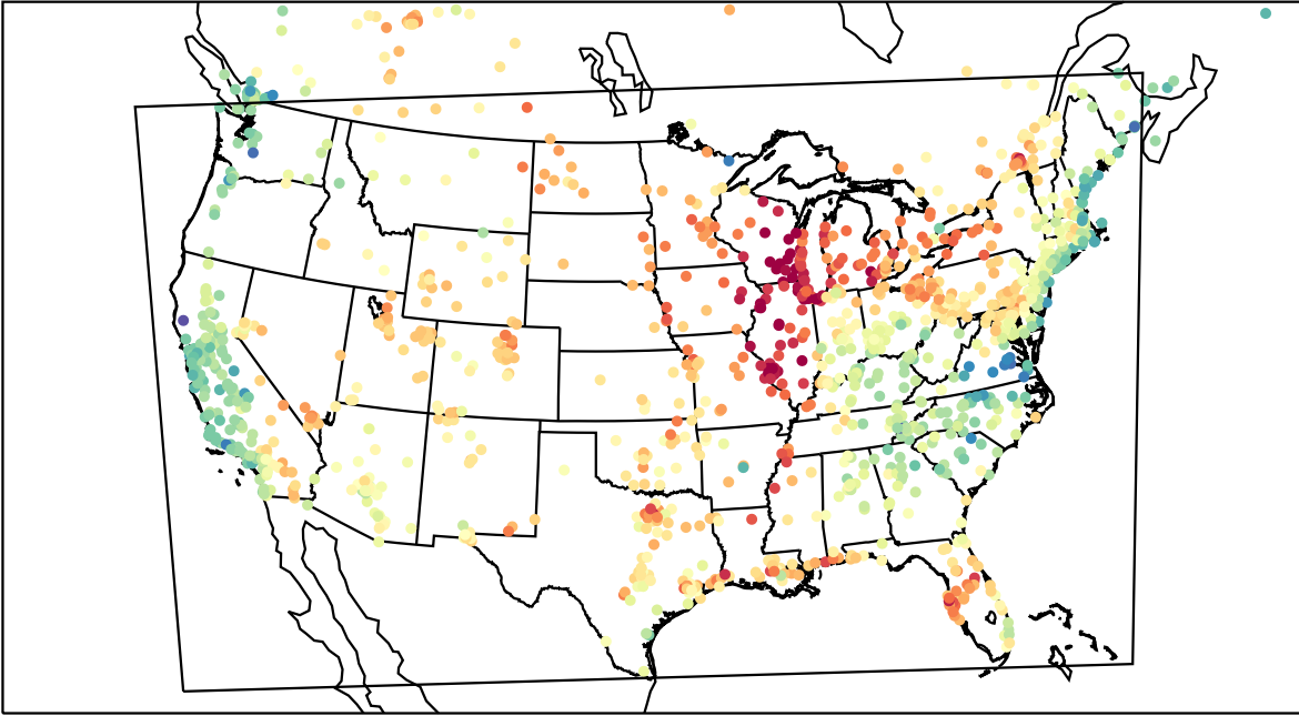
AirNOW (2023-05-30_19:00:00)
