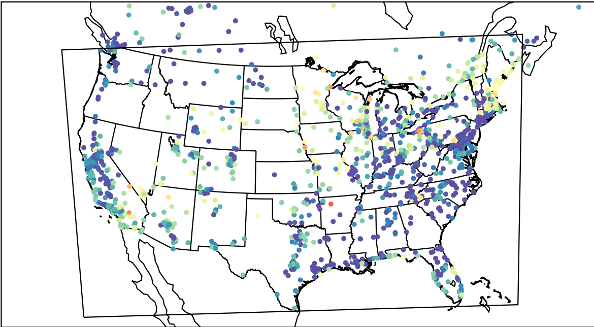
AirNOW (2023-05-29_09:00:00)
