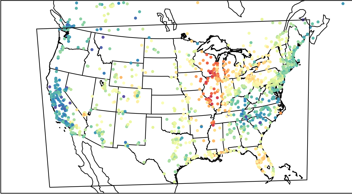
AirNOW (2023-05-30_15:00:00)
