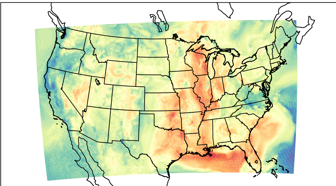
WRF (2023-05-30_16:00:00)
