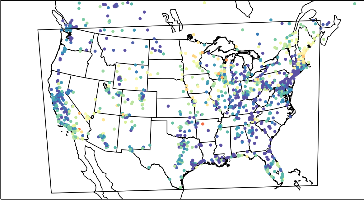
AirNOW (2023-05-29_08:00:00)
