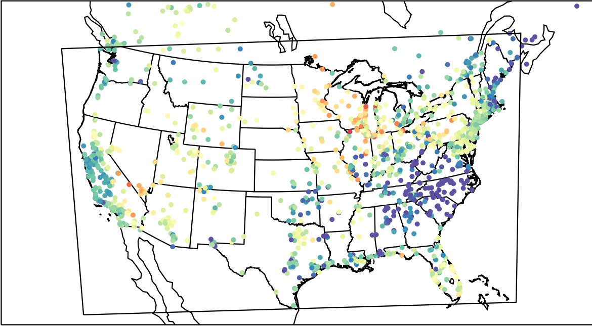
AirNOW (2023-05-30_03:00:00)
