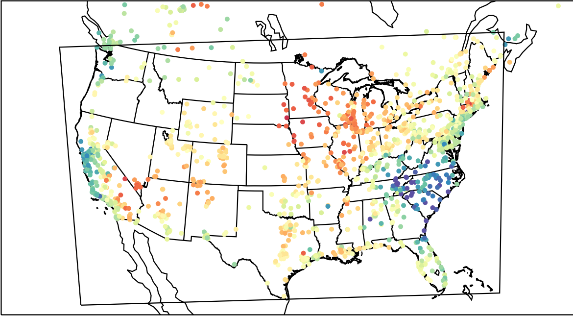
AirNOW (2023-05-29_00:00:00)
