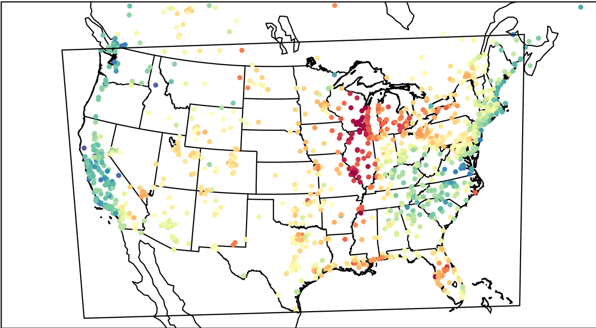
AirNOW (2023-05-30_17:00:00)
