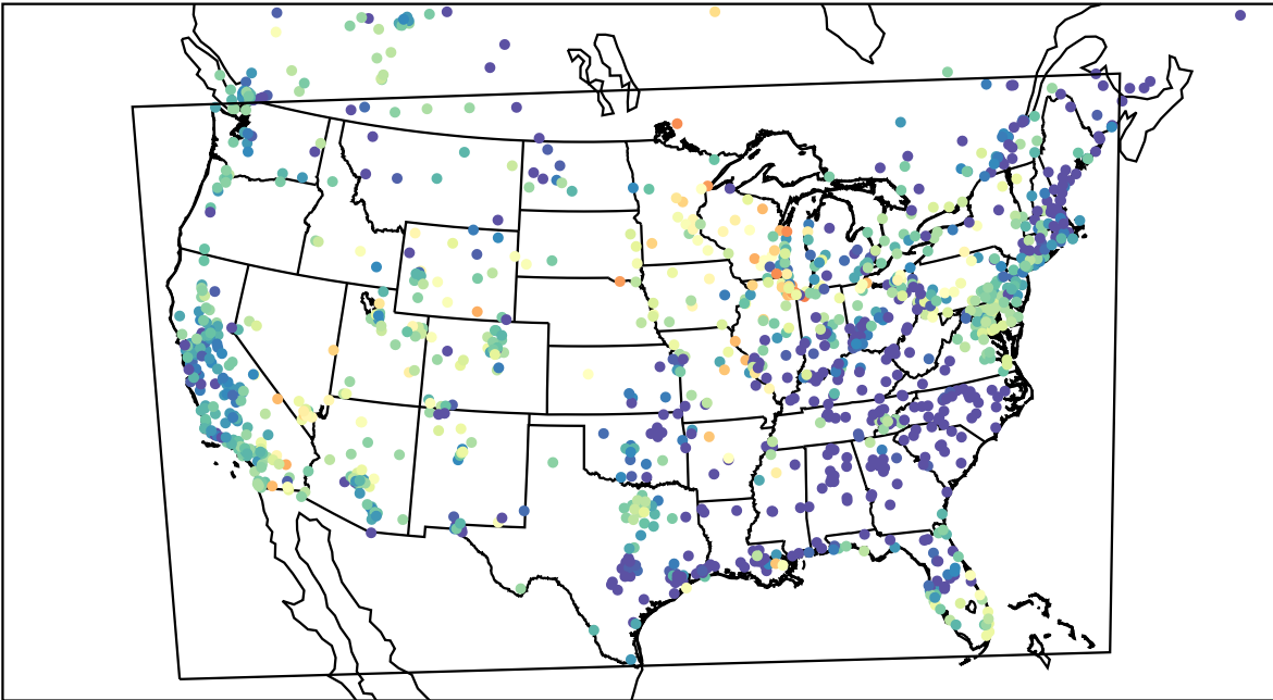
AirNOW (2023-05-30_07:00:00)
