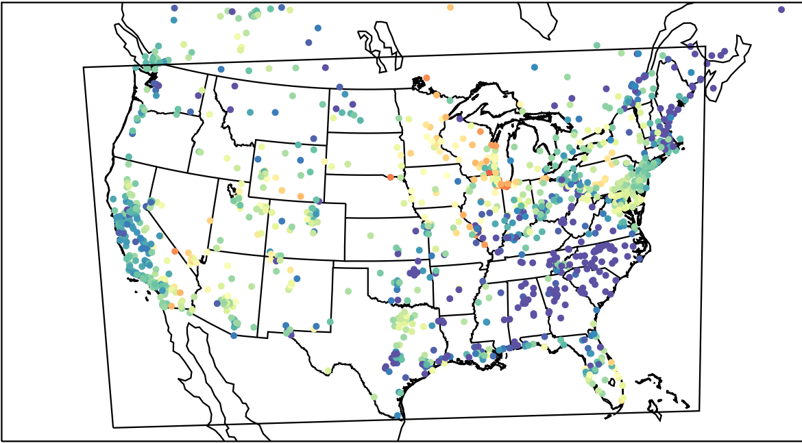
AirNOW (2023-05-30_05:00:00)
