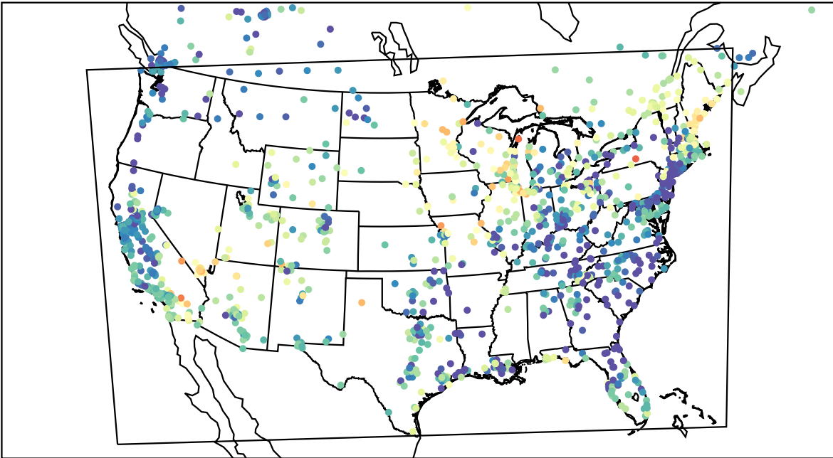
AirNOW (2023-05-29_06:00:00)
