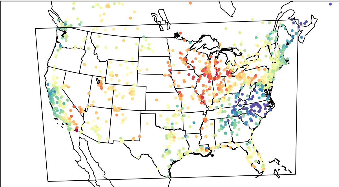
AirNOW (2023-05-30_00:00:00)
