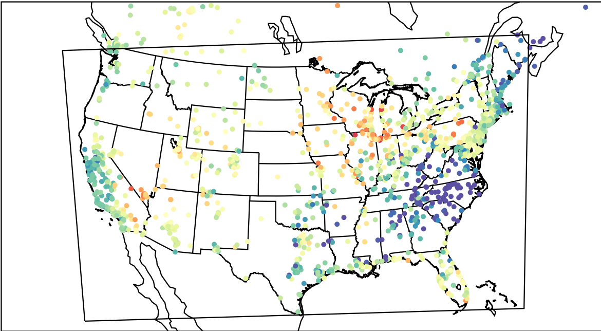
AirNOW (2023-05-30_02:00:00)
