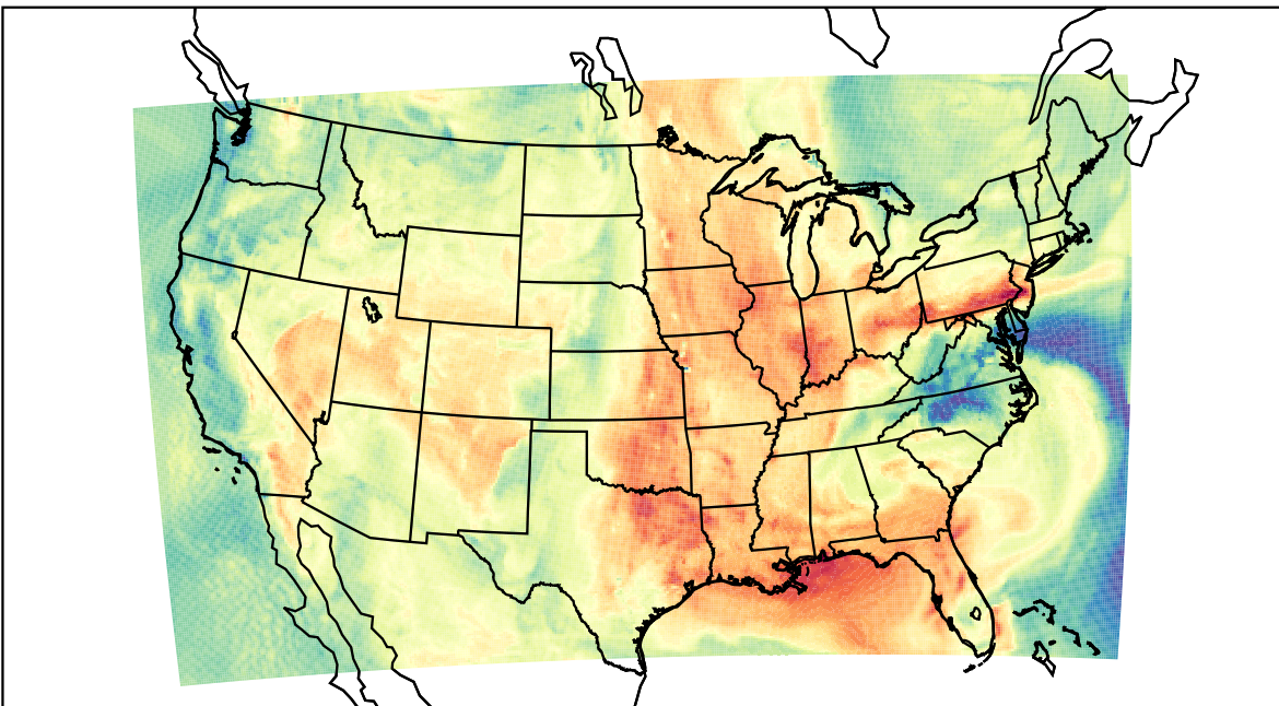
WRF (2023-05-29_17:00:00)
