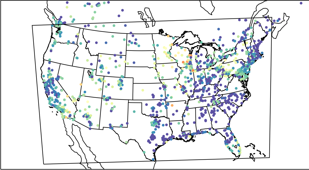
AirNOW (2023-05-30_09:00:00)
