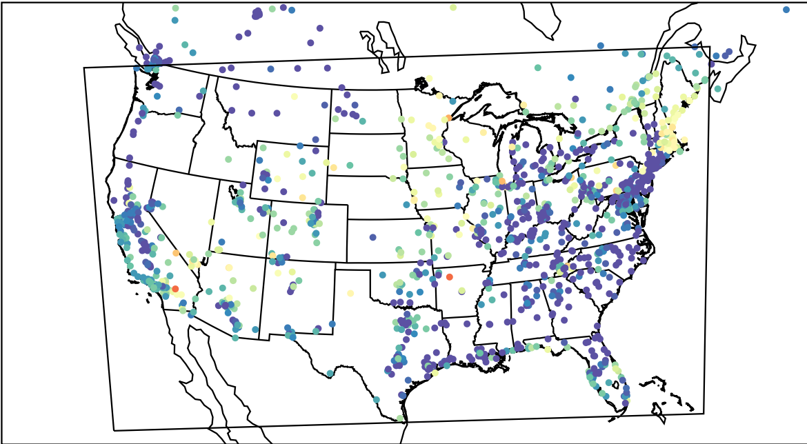
AirNOW (2023-05-29_10:00:00)
