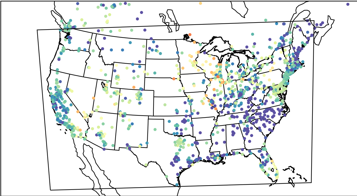
AirNOW (2023-05-30_06:00:00)
