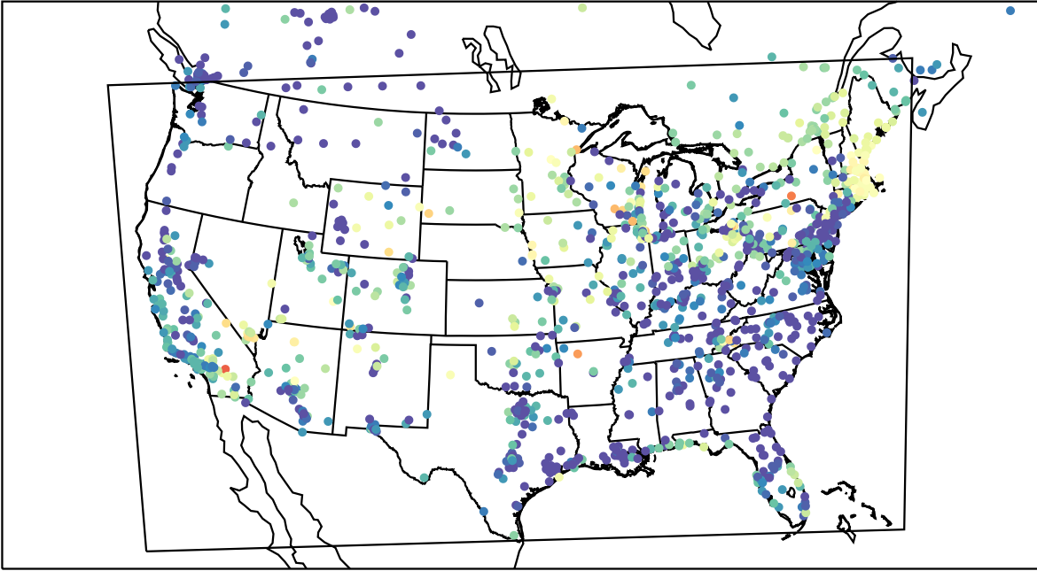
AirNOW (2023-05-29_11:00:00)
