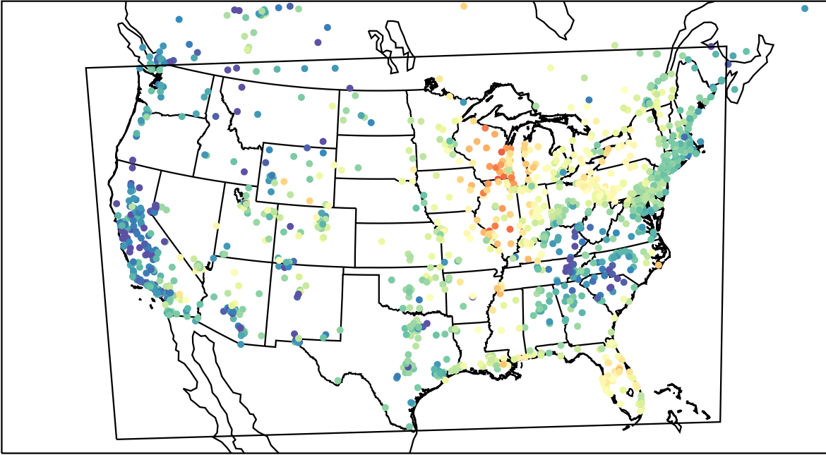
AirNOW (2023-05-30_14:00:00)
