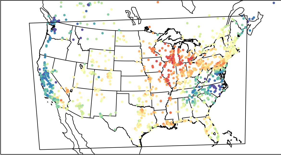
AirNOW (2023-05-29_16:00:00)
