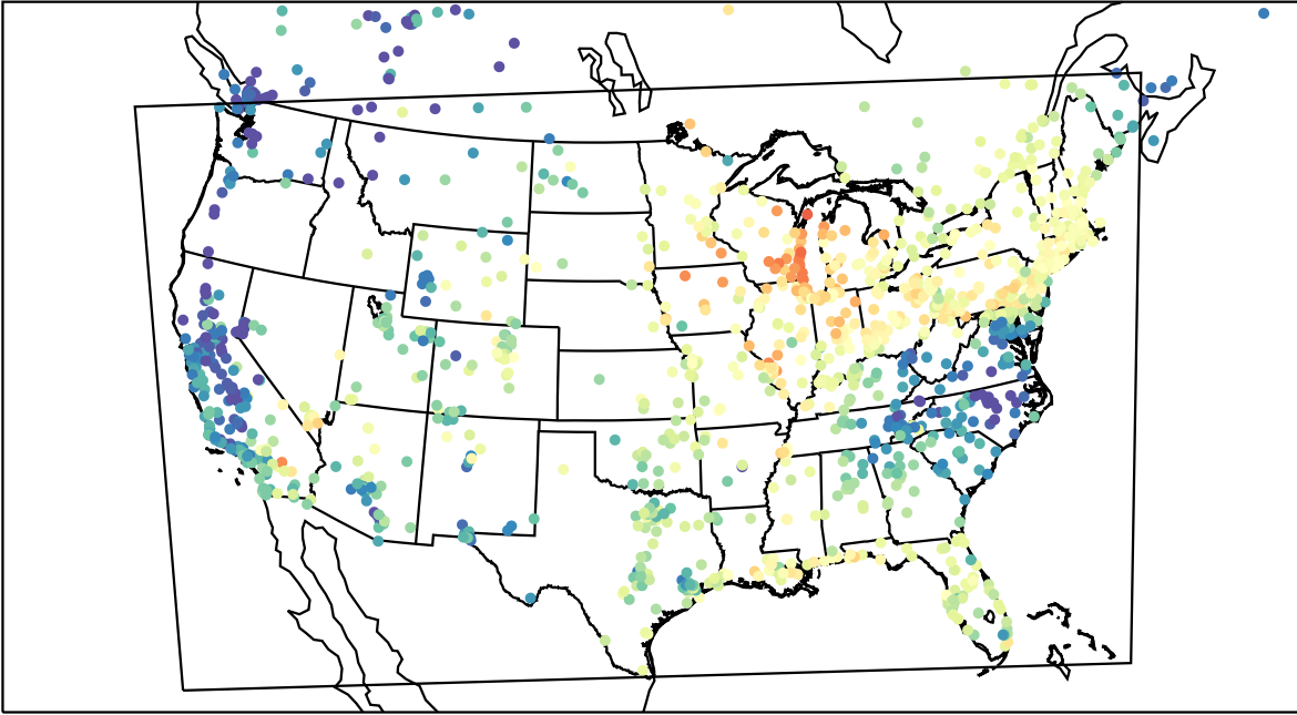
AirNOW (2023-05-29_14:00:00)
