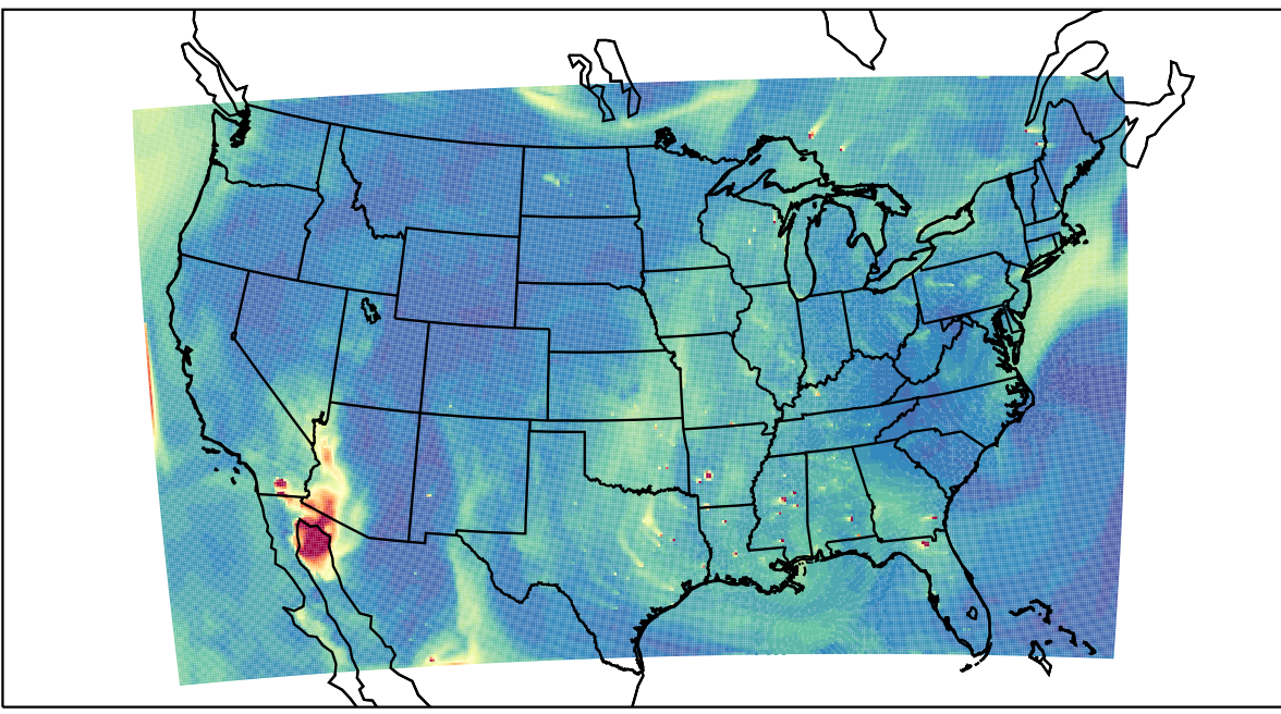
WRF 2023-05-31_21:00:00
