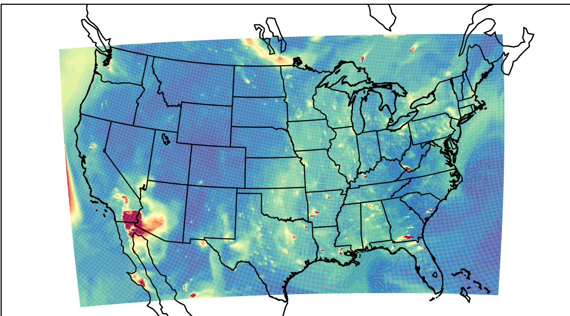
WRF 2023-06-01_02:00:00
