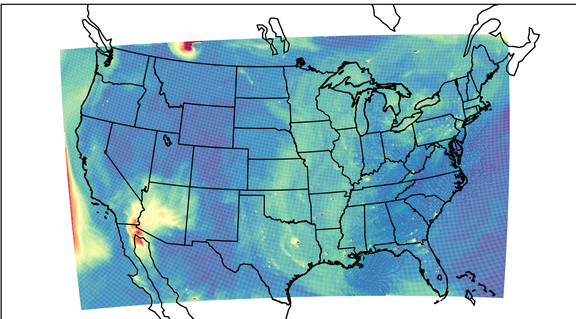
WRF 2023-06-01_21:00:00
