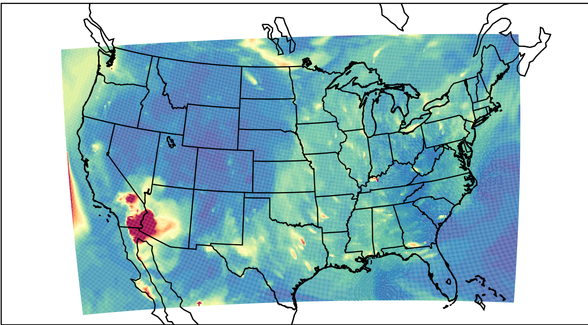
WRF 2023-06-01_05:00:00
