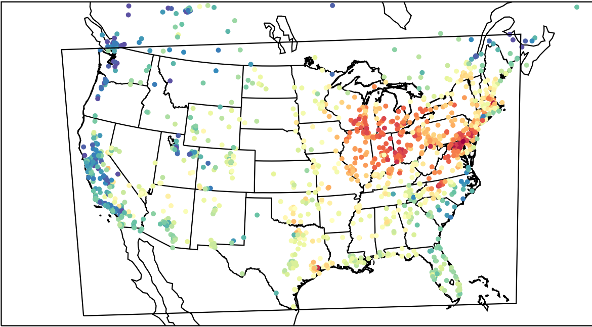
AirNOW (2023-06-02_15:00:00)
