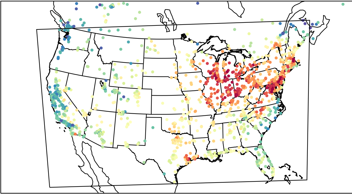
AirNOW (2023-06-02_16:00:00)
