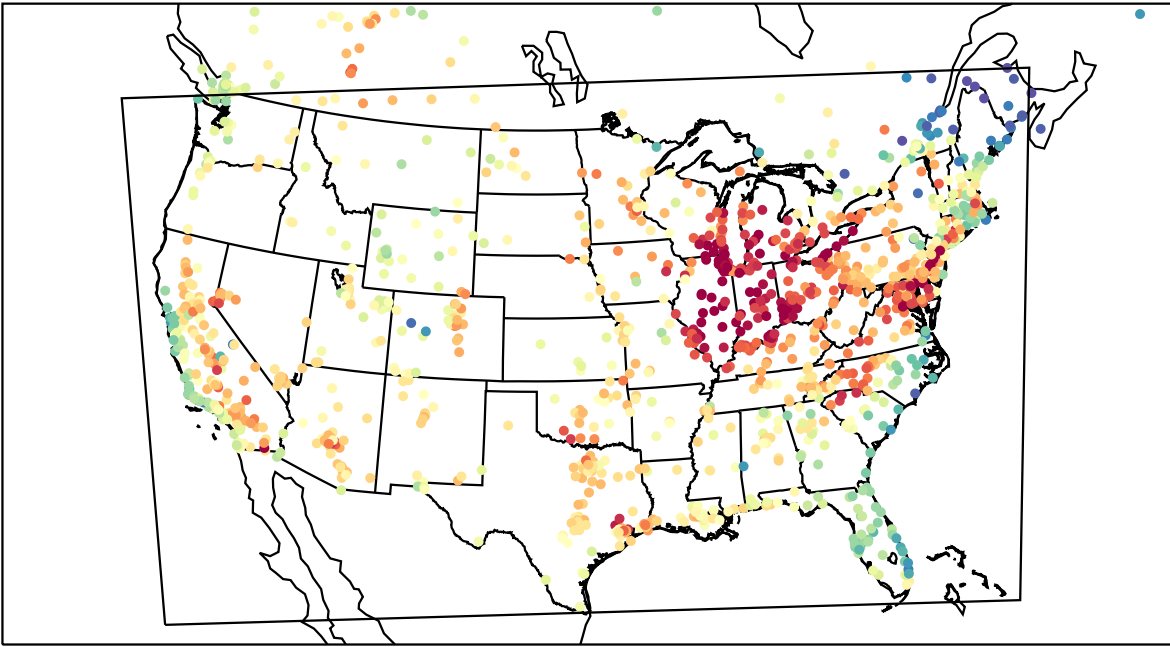
AirNOW (2023-06-02_22:00:00)
