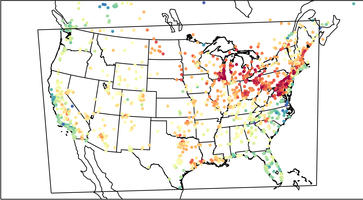
AirNOW (2023-06-01_21:00:00)
