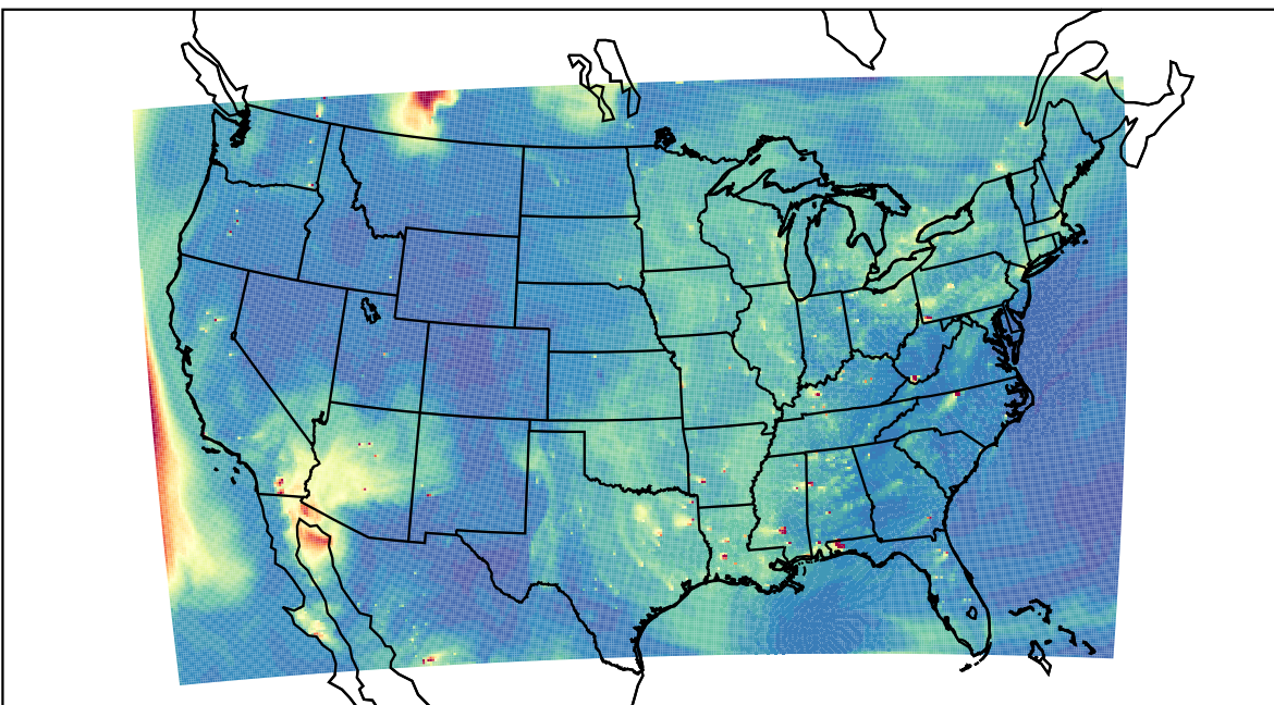
WRF 2023-06-02_00:00:00
