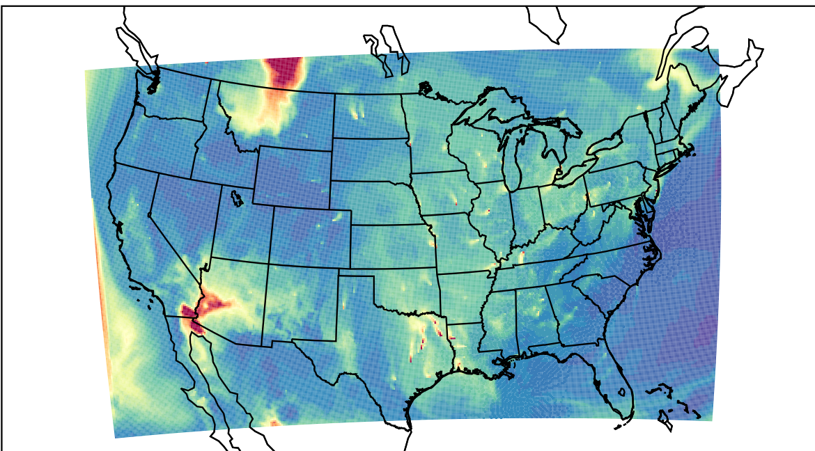
WRF 2023-06-02_15:00:00
