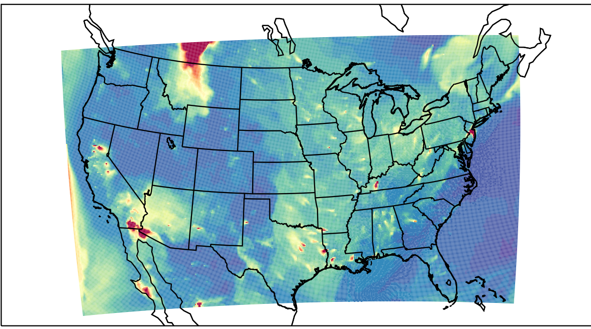
WRF 2023-06-03_04:00:00
