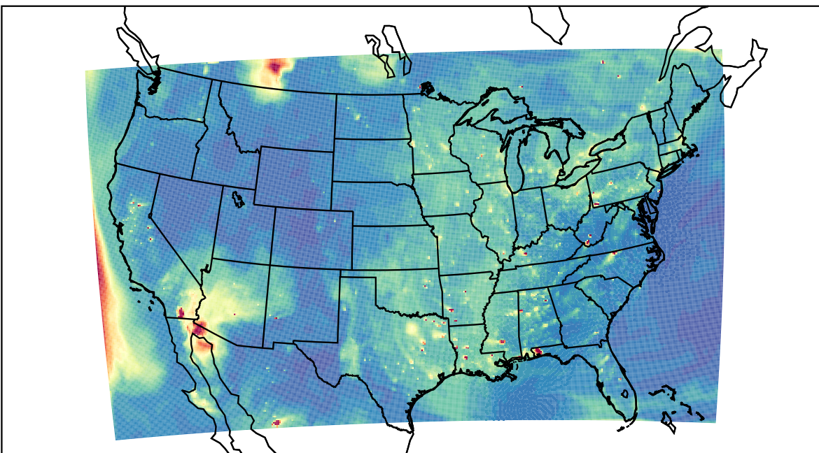
WRF 2023-06-02_01:00:00
