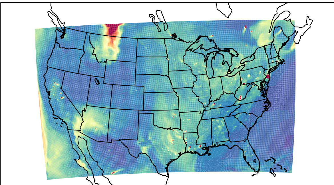
WRF 2023-06-03_00:00:00
