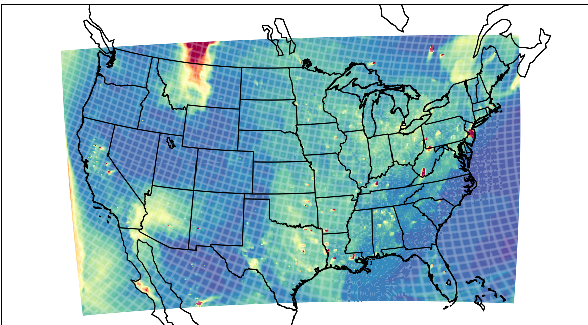
WRF 2023-06-03_01:00:00
