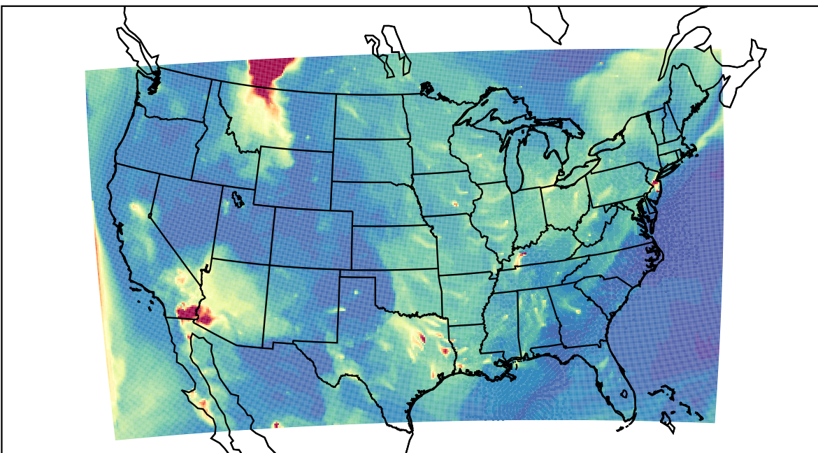
WRF 2023-06-03_07:00:00
