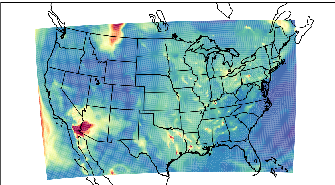
WRF 2023-06-02_09:00:00
