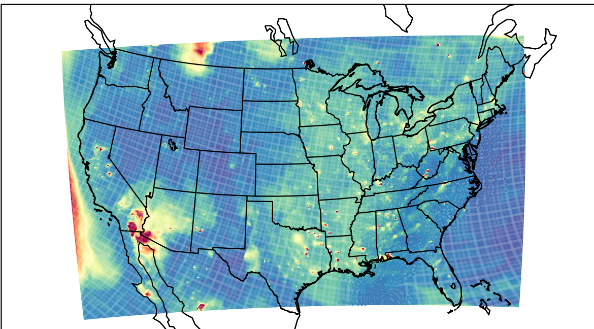
WRF 2023-06-02_02:00:00
