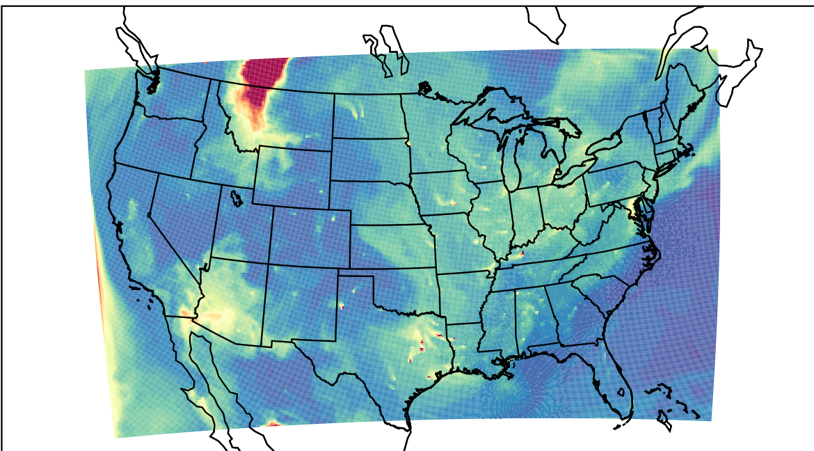
WRF 2023-06-03_15:00:00
