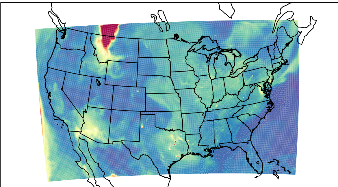
WRF 2023-06-03_17:00:00
