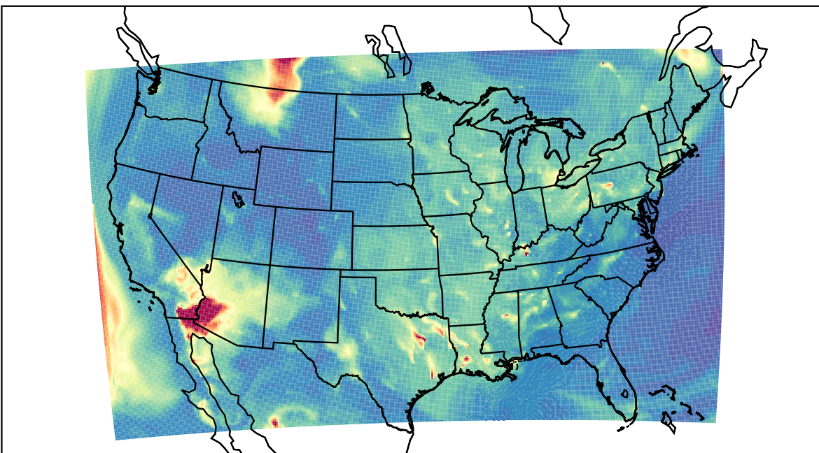
WRF 2023-06-02_08:00:00
