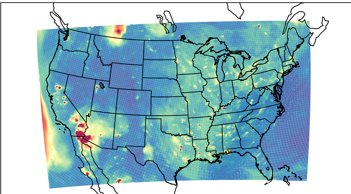
WRF 2023-06-02_03:00:00
