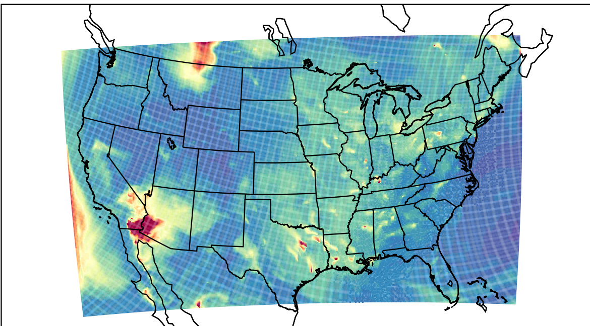
WRF 2023-06-02_07:00:00
