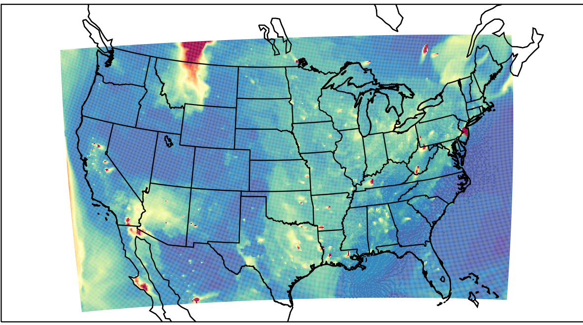
WRF 2023-06-03_02:00:00
