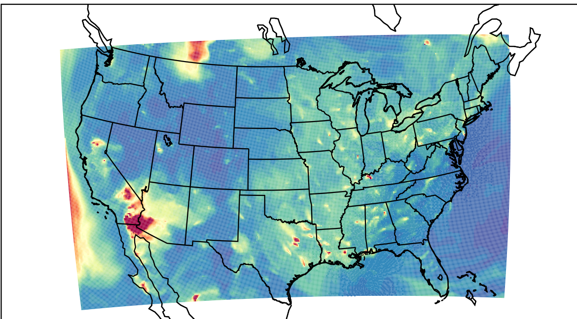
WRF 2023-06-02_05:00:00
