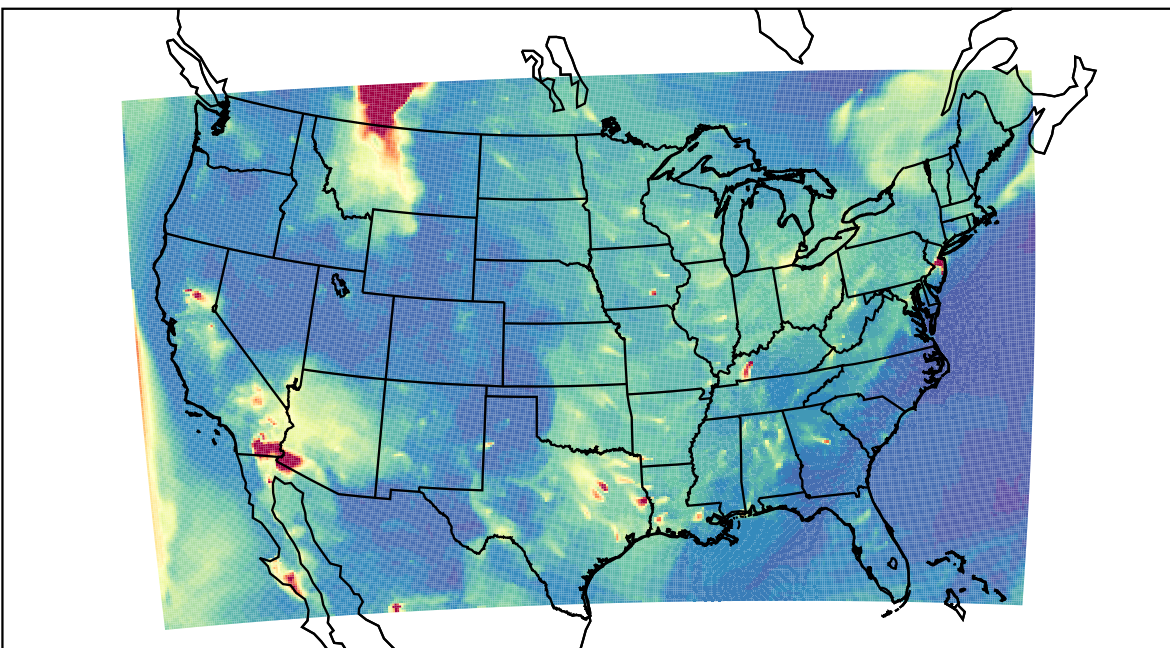
WRF 2023-06-03_05:00:00
