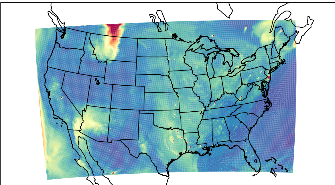
WRF 2023-06-02_22:00:00
