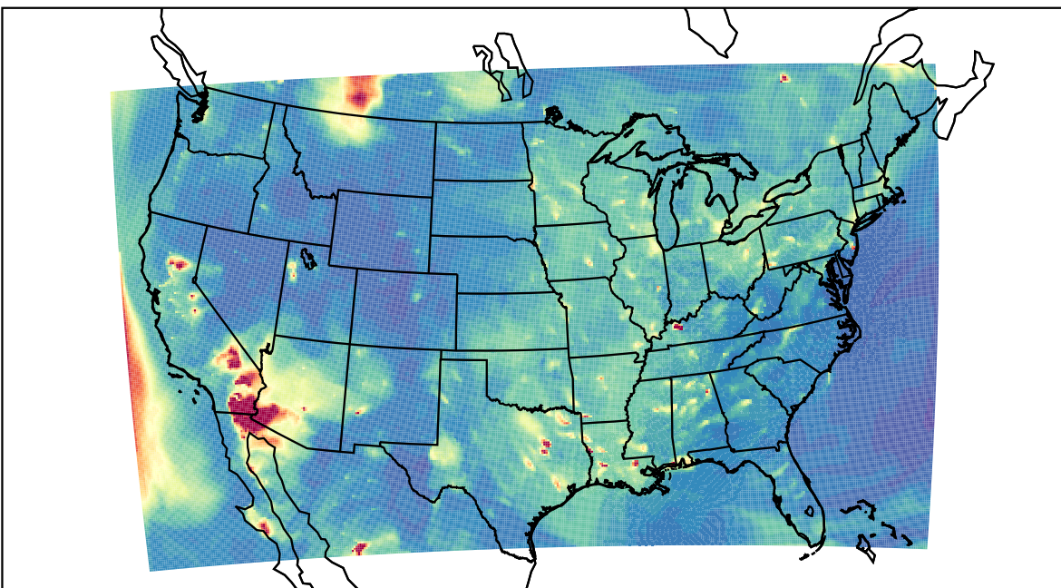
WRF 2023-06-02_04:00:00
