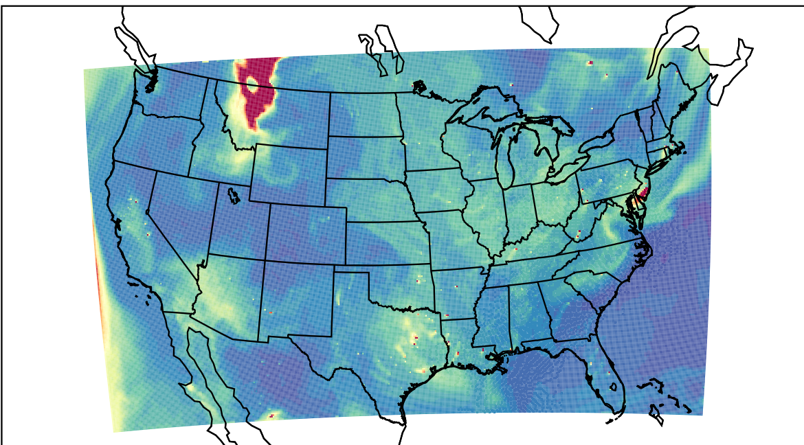
WRF 2023-06-03_21:00:00
