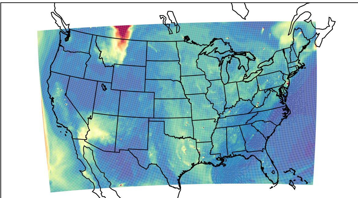
WRF 2023-06-02_21:00:00
