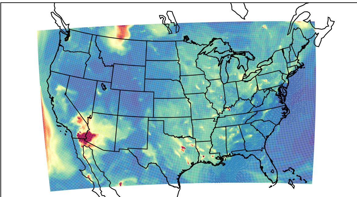
WRF 2023-06-02_06:00:00
