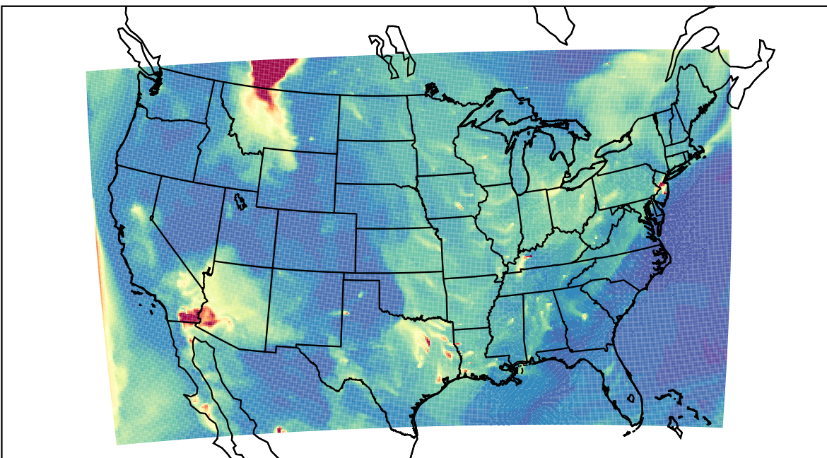
WRF 2023-06-03_08:00:00
