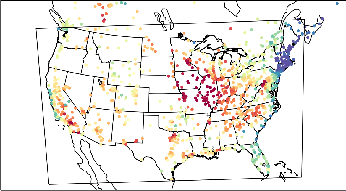
AirNOW (2023-06-03_21:00:00)
