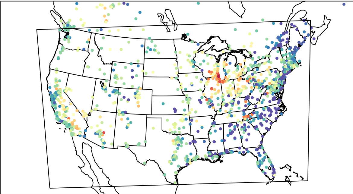
AirNOW (2023-06-03_04:00:00)
