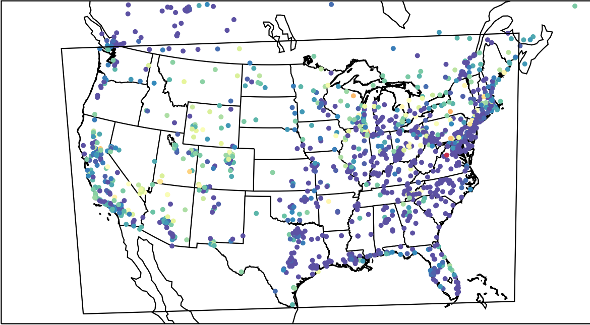
AirNOW (2023-06-02_11:00:00)
