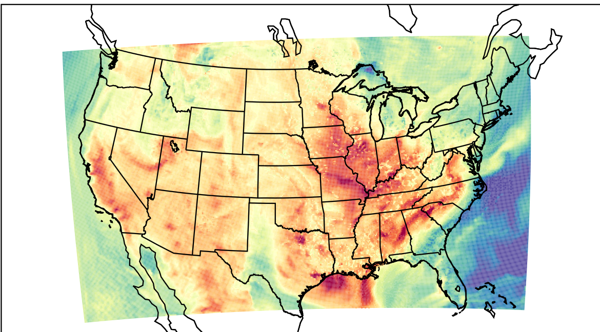
WRF (2023-06-03_22:00:00)
