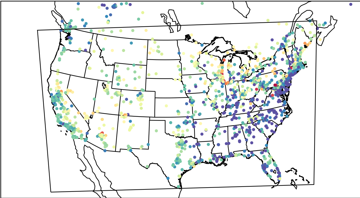
AirNOW (2023-06-02_04:00:00)
