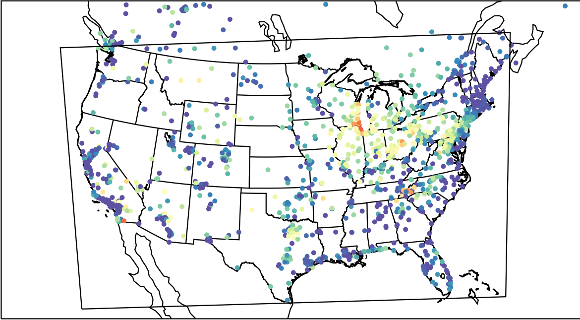
AirNOW (2023-06-03_12:00:00)
