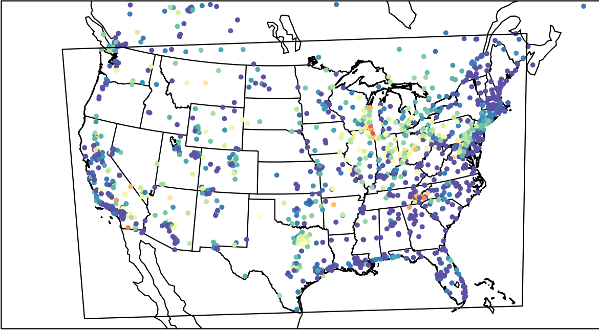
AirNOW (2023-06-03_11:00:00)
