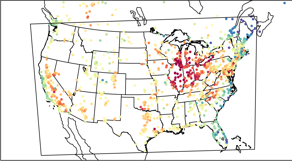
AirNOW (2023-06-02_23:00:00)
