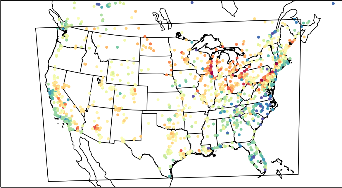
AirNOW (2023-06-02_00:00:00)
