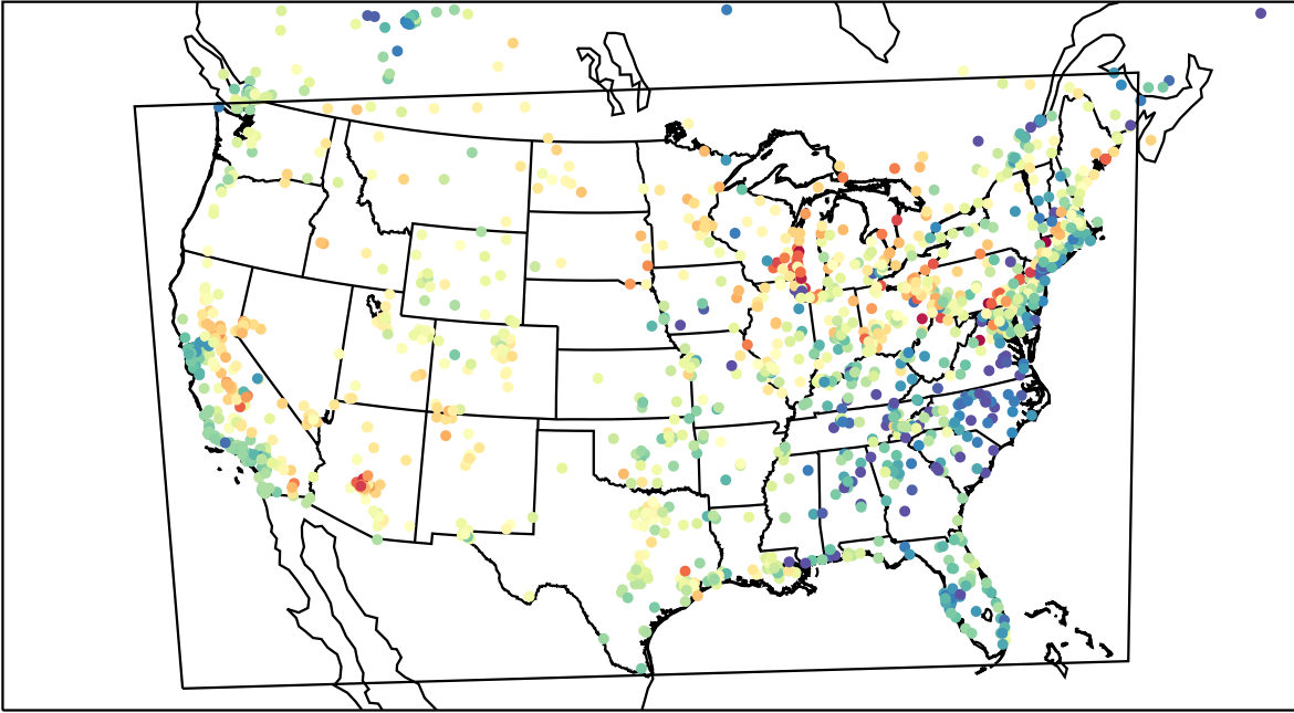
AirNOW (2023-06-02_01:00:00)
