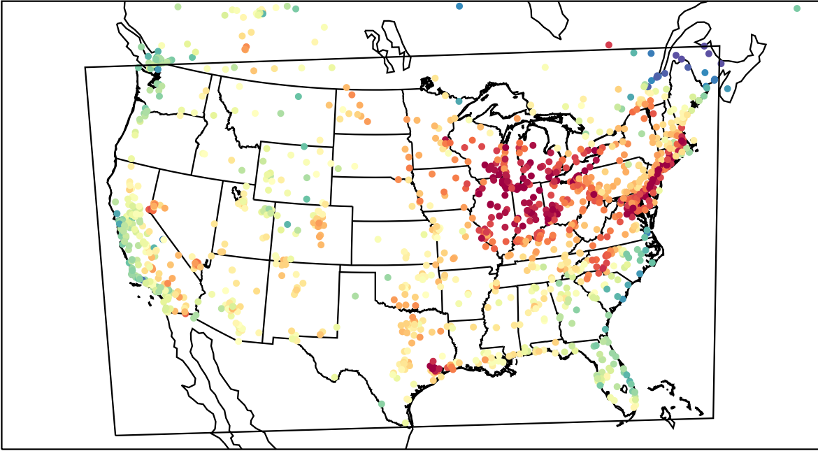
AirNOW (2023-06-02_19:00:00)
