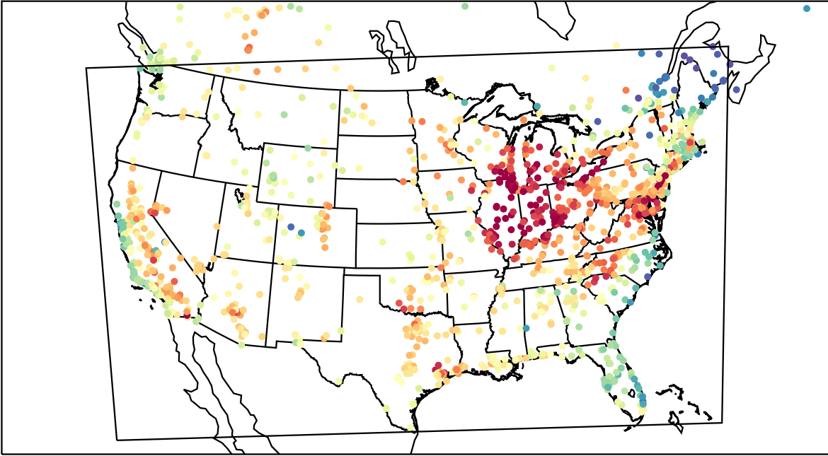
AirNOW (2023-06-02_22:00:00)
