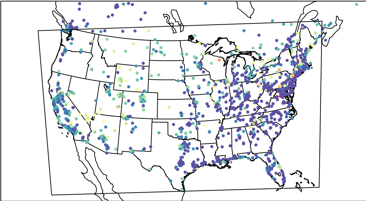
AirNOW (2023-06-02_10:00:00)
