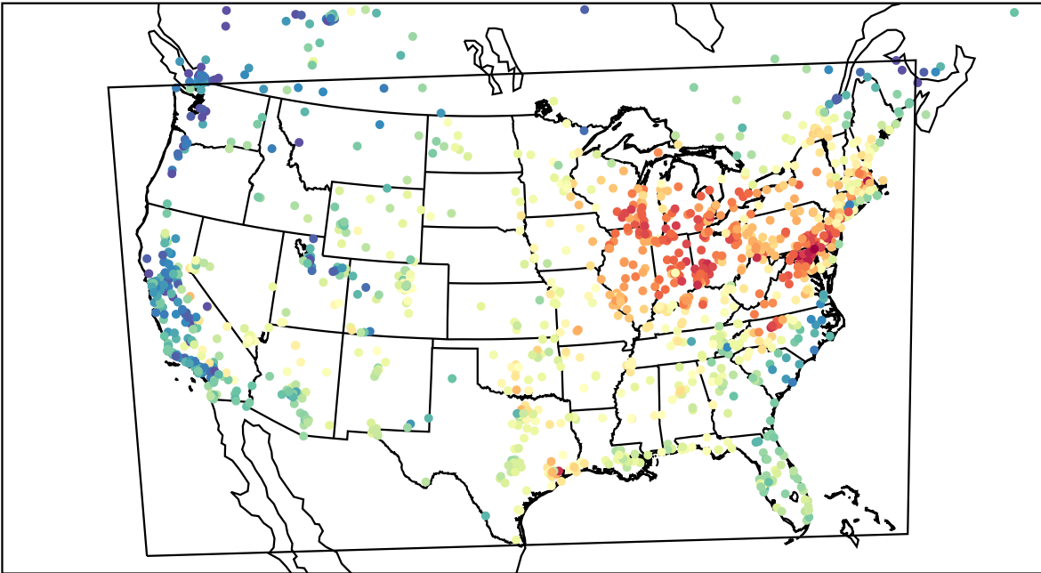
AirNOW (2023-06-02_15:00:00)
