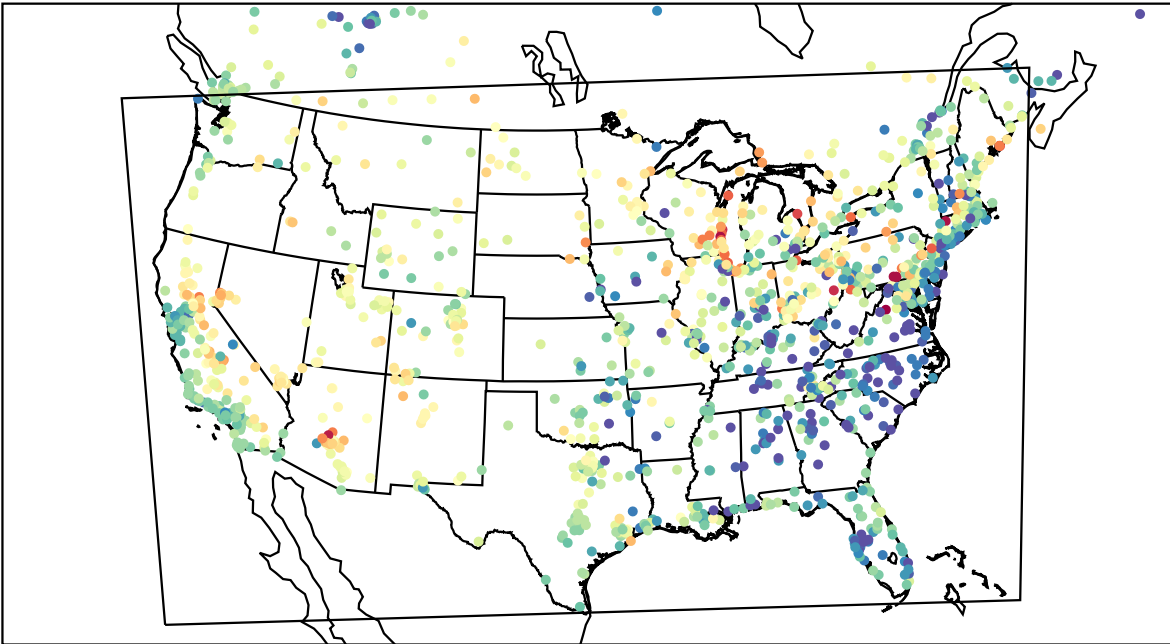
AirNOW (2023-06-02_02:00:00)
