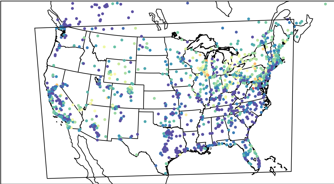
AirNOW (2023-06-02_12:00:00)
