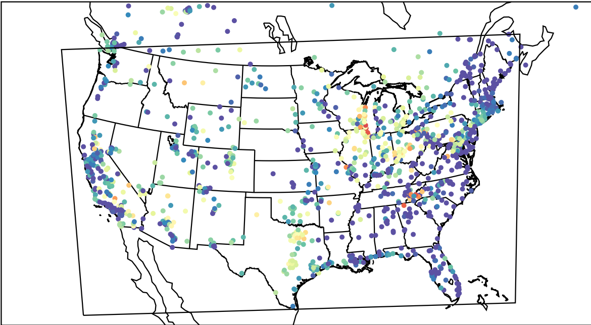
AirNOW (2023-06-03_09:00:00)
