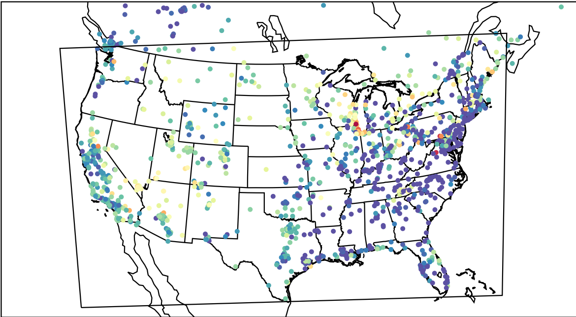
AirNOW (2023-06-02_07:00:00)
