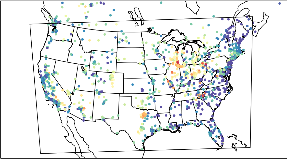
AirNOW (2023-06-03_06:00:00)
