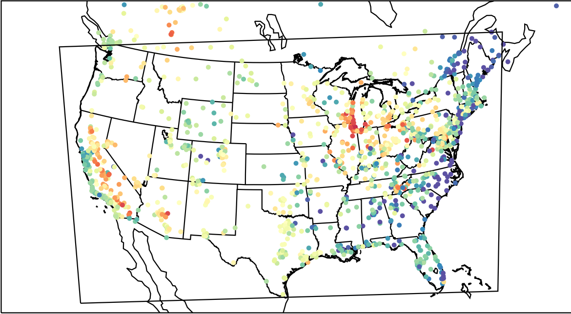
AirNOW (2023-06-03_02:00:00)
