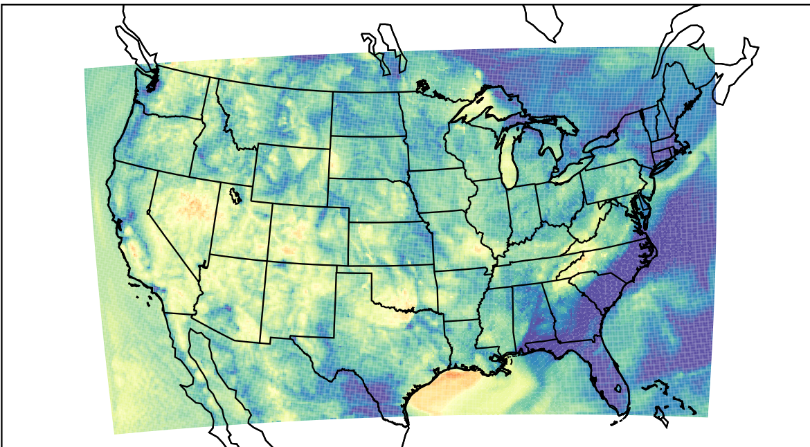
WRF (2023-06-03_12:00:00)
