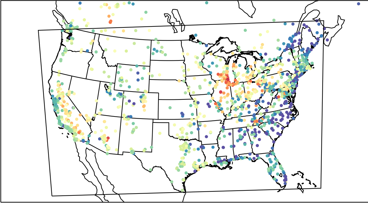
AirNOW (2023-06-03_03:00:00)
