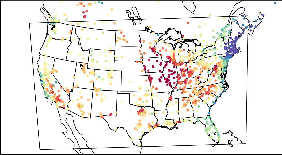
AirNOW (2023-06-03_20:00:00)
