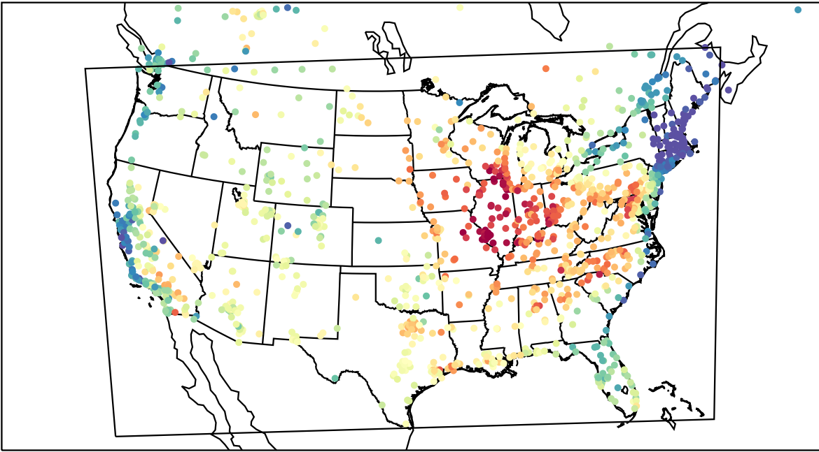
AirNOW (2023-06-03_16:00:00)
