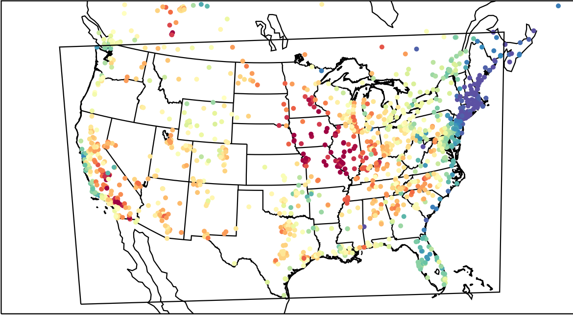
AirNOW (2023-06-03_23:00:00)
