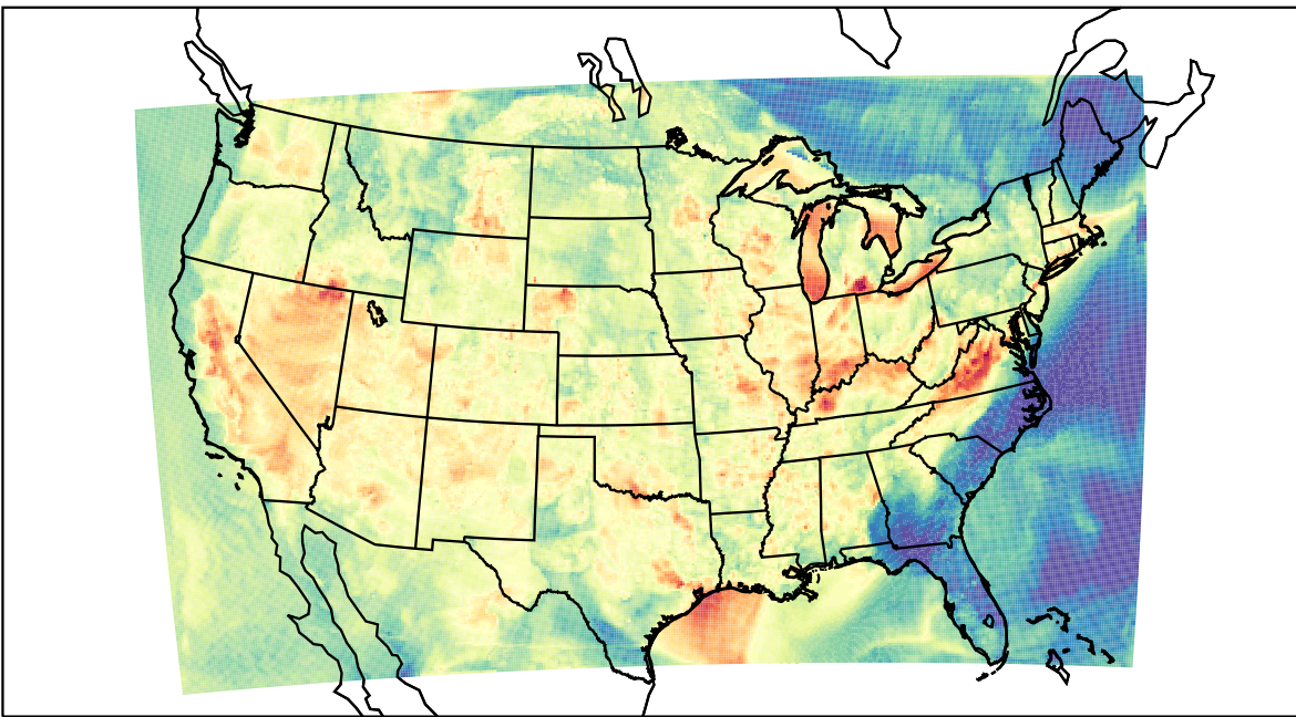
WRF (2023-06-03_02:00:00)
