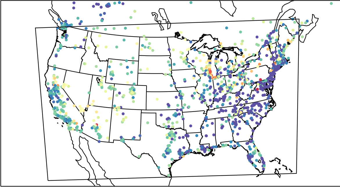
AirNOW (2023-06-02_06:00:00)
