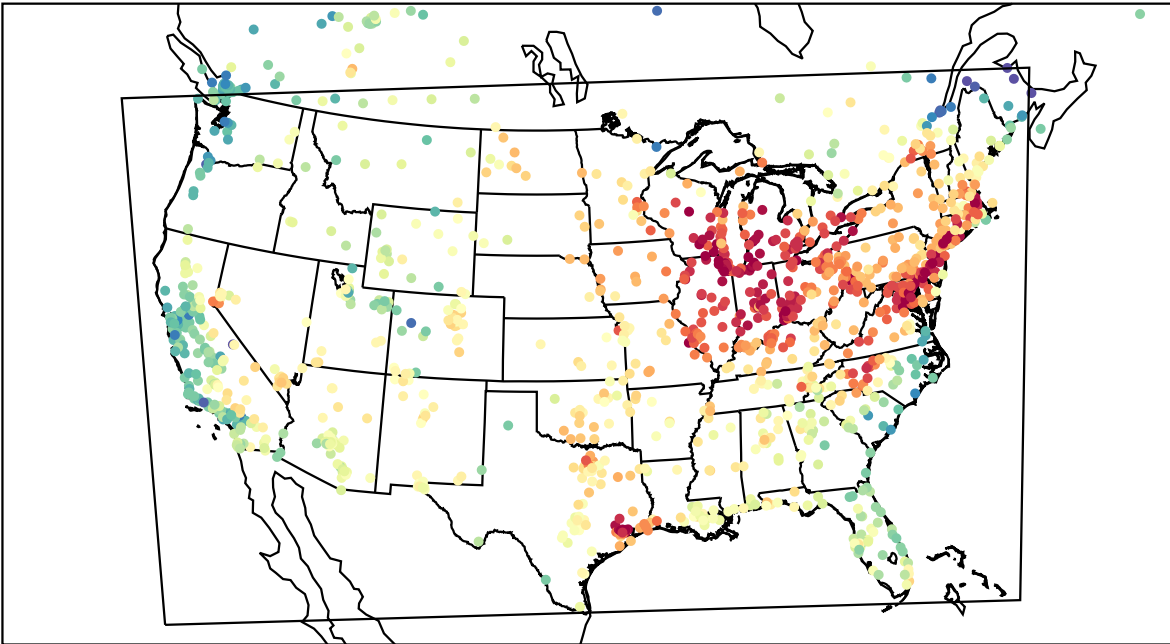
AirNOW (2023-06-02_17:00:00)
