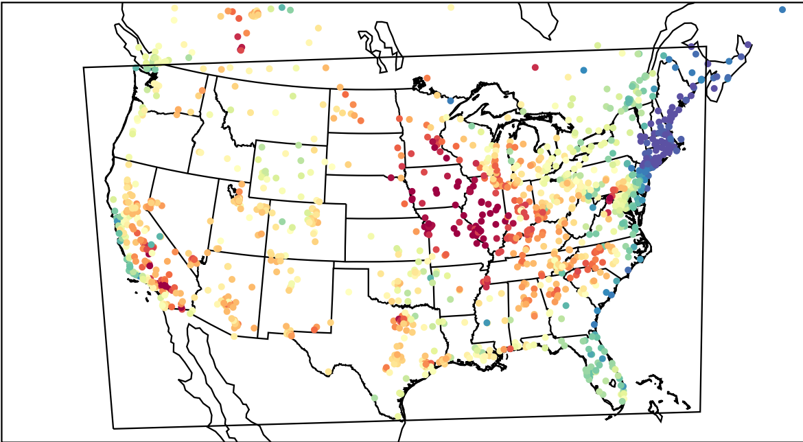
AirNOW (2023-06-03_22:00:00)
