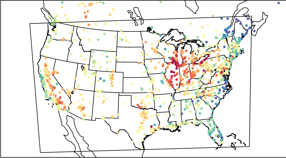
AirNOW (2023-06-03_00:00:00)
