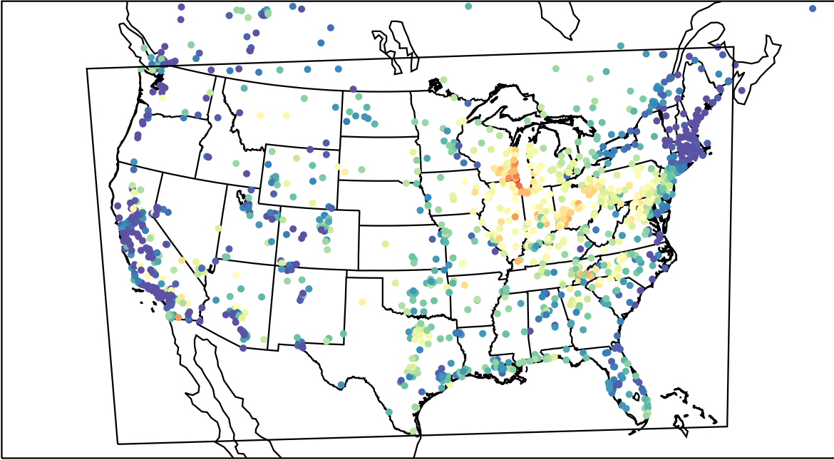
AirNOW (2023-06-03_13:00:00)
