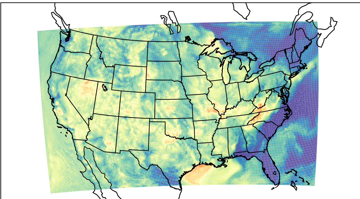
WRF (2023-06-03_09:00:00)
