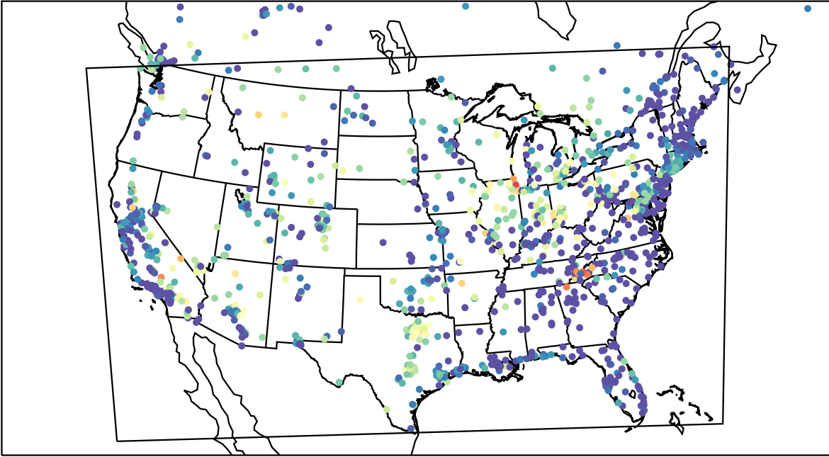
AirNOW (2023-06-03_10:00:00)
