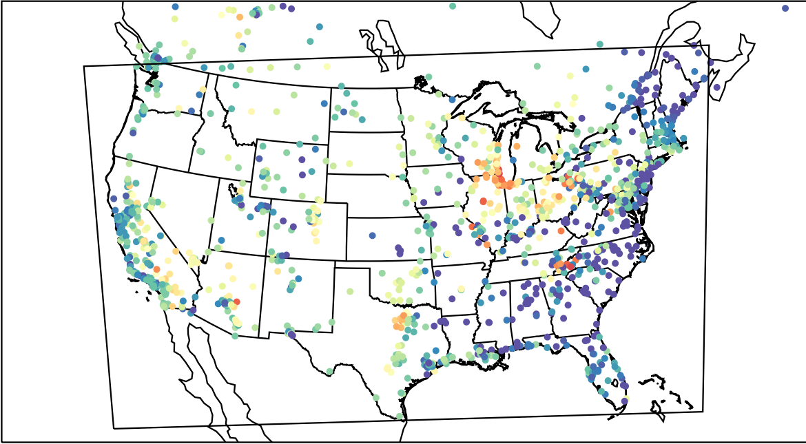
AirNOW (2023-06-03_05:00:00)
