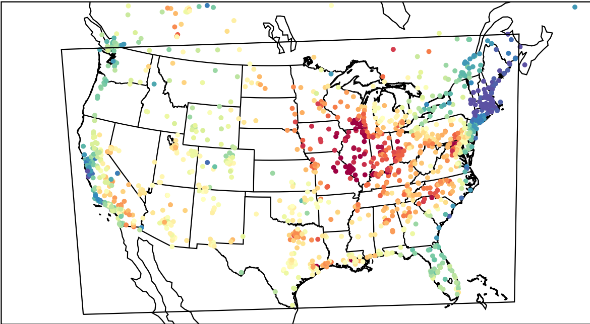
AirNOW (2023-06-03_17:00:00)
