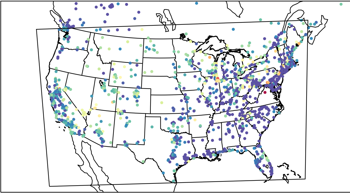
AirNOW (2023-06-02_09:00:00)
