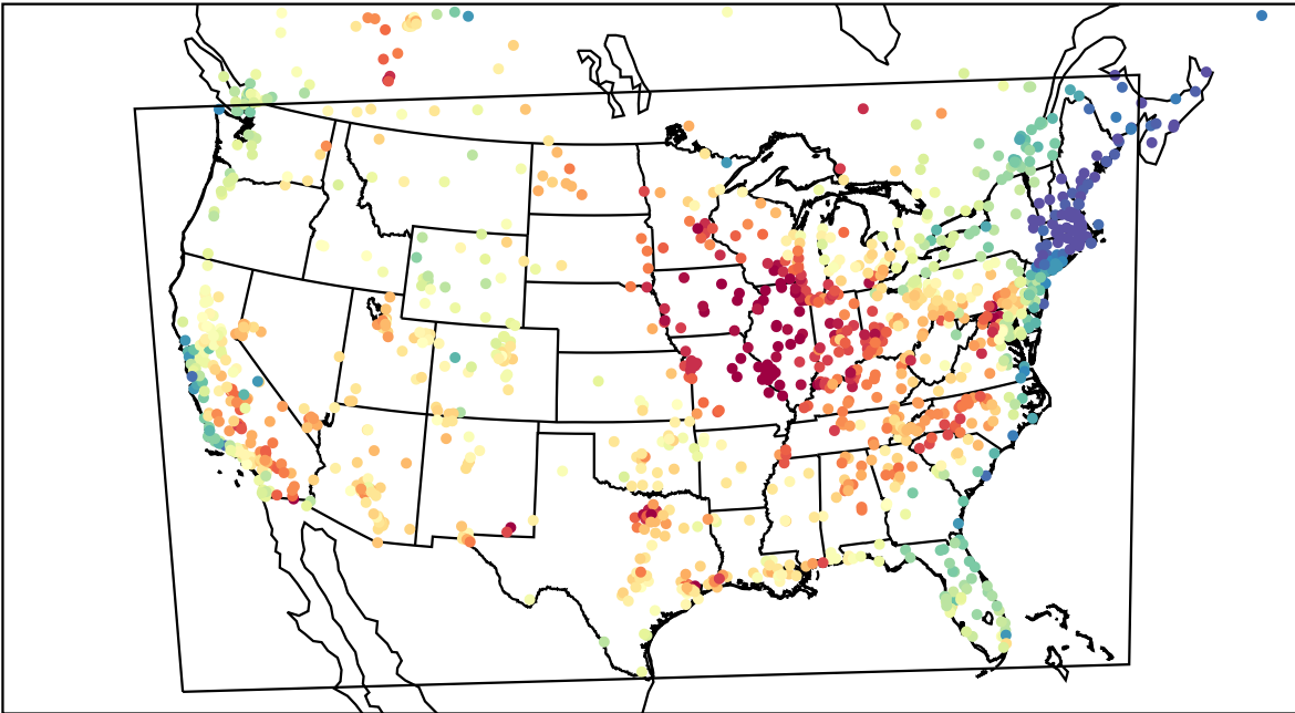
AirNOW (2023-06-03_19:00:00)
