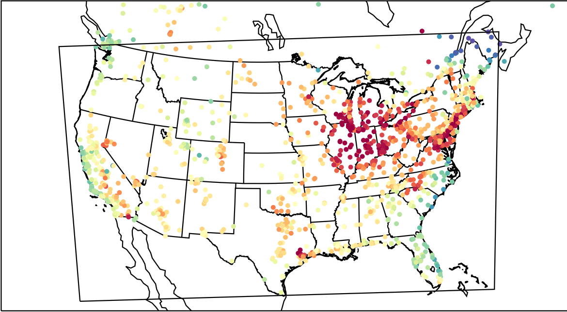
AirNOW (2023-06-02_20:00:00)
