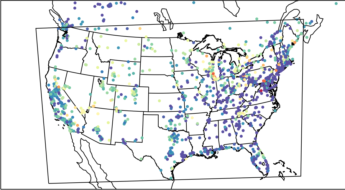
AirNOW (2023-06-02_08:00:00)
