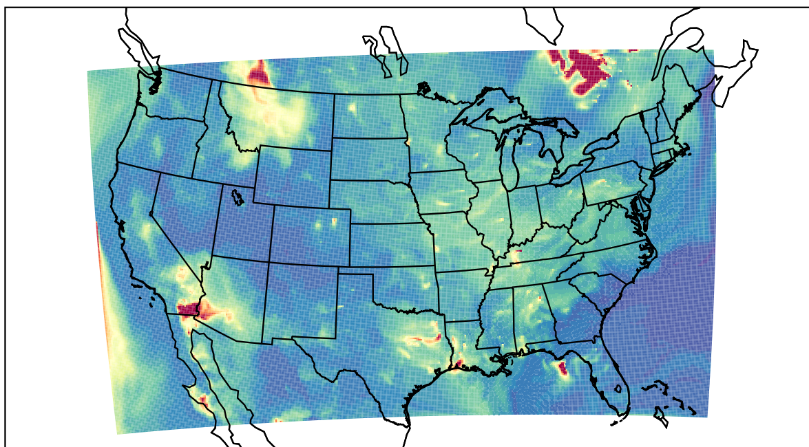
WRF 2023-06-04_07:00:00
