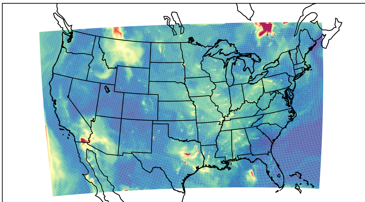
WRF 2023-06-04_13:00:00
