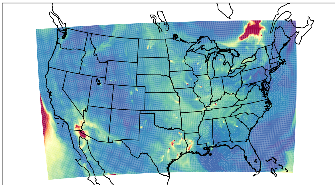
WRF 2023-06-05_15:00:00
