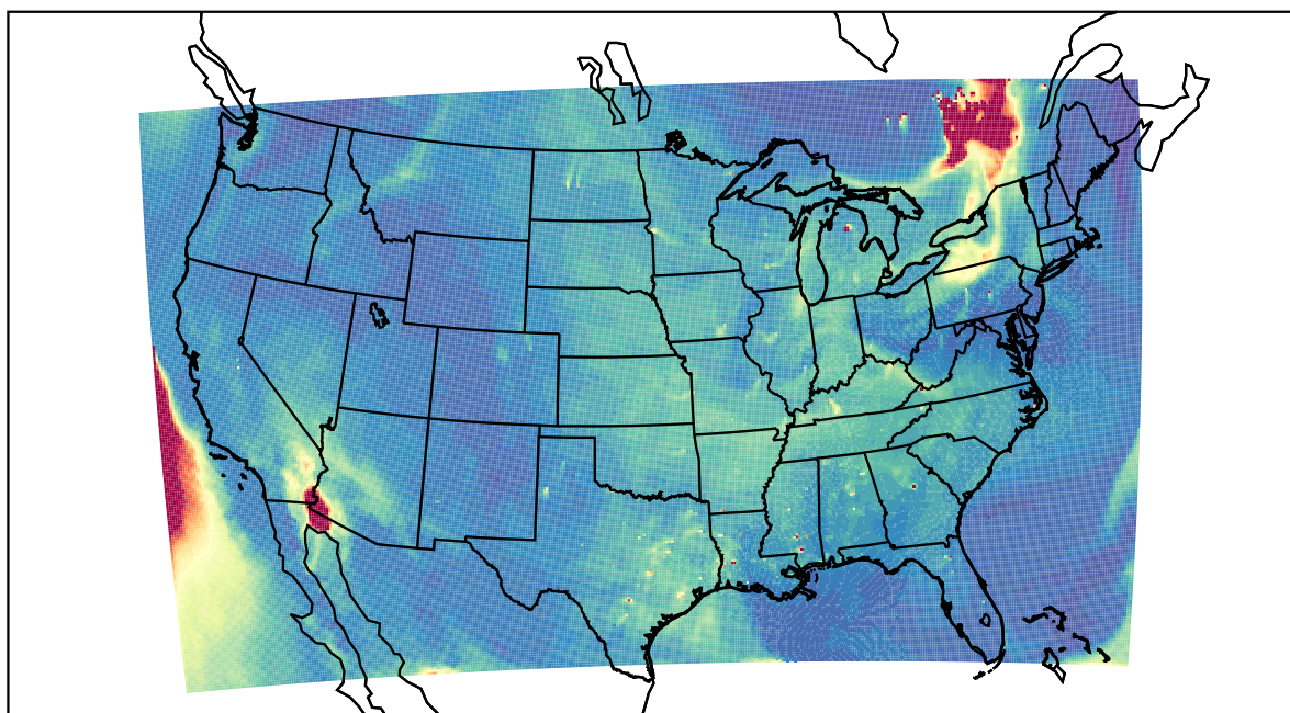
WRF 2023-06-05_19:00:00
