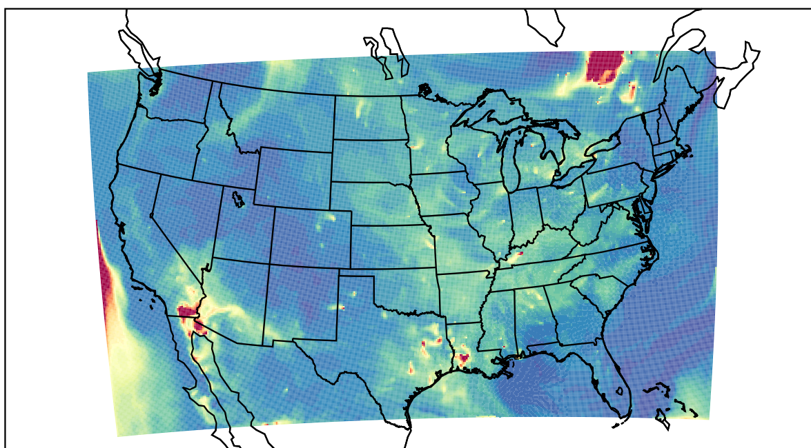
WRF 2023-06-05_10:00:00
