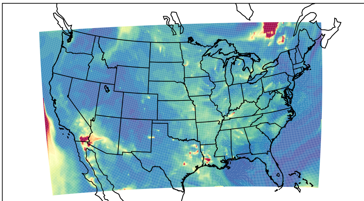
WRF 2023-06-05_08:00:00
