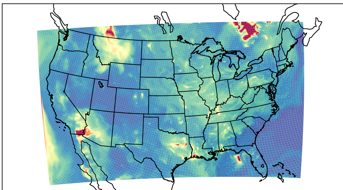
WRF 2023-06-04_08:00:00
