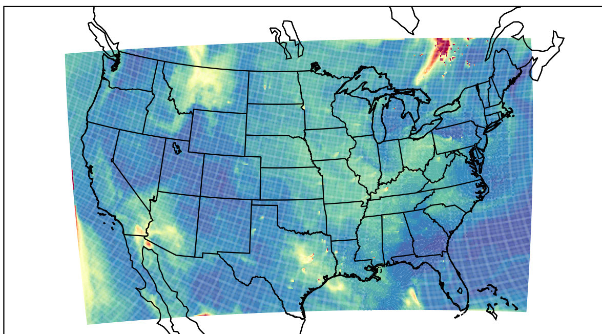
WRF 2023-06-04_17:00:00
