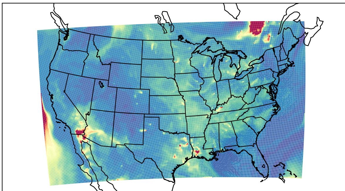
WRF 2023-06-05_09:00:00
