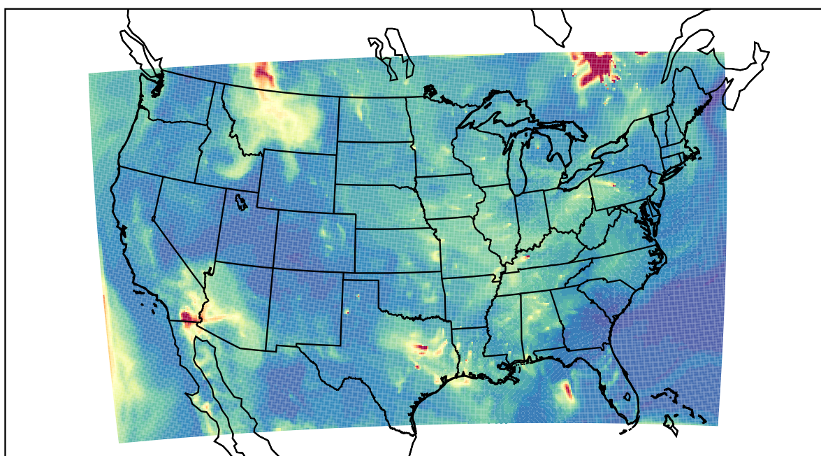
WRF 2023-06-04_12:00:00
