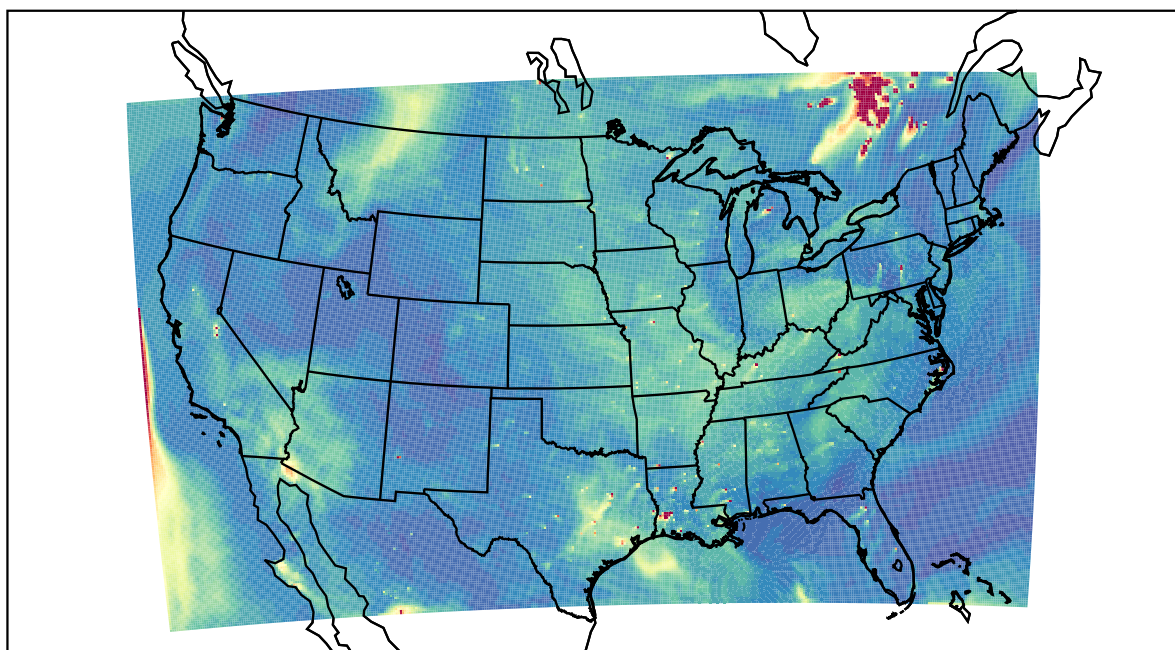
WRF 2023-06-04_23:00:00
