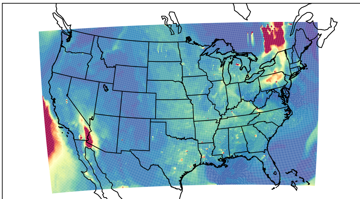
WRF 2023-06-05_23:00:00
