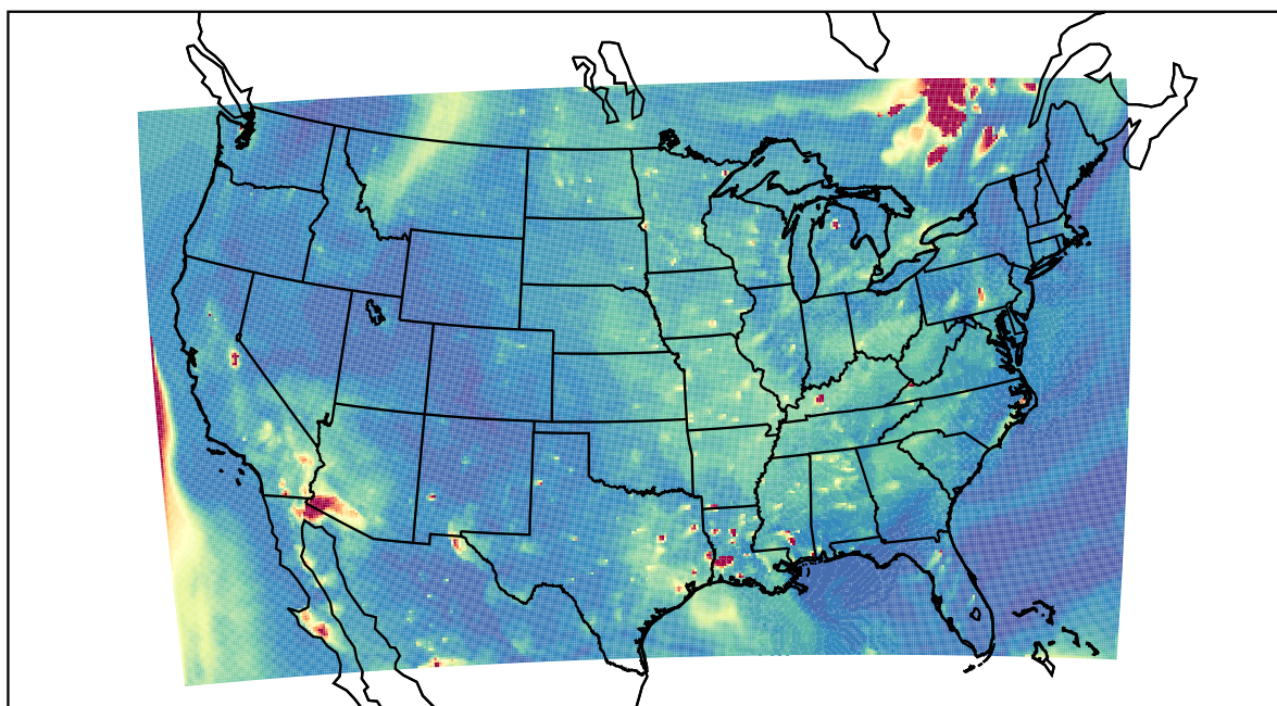
WRF 2023-06-05_02:00:00
