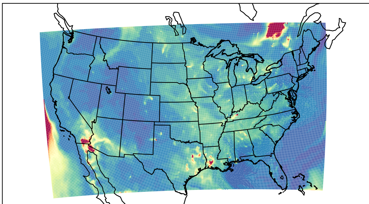
WRF 2023-06-05_11:00:00
