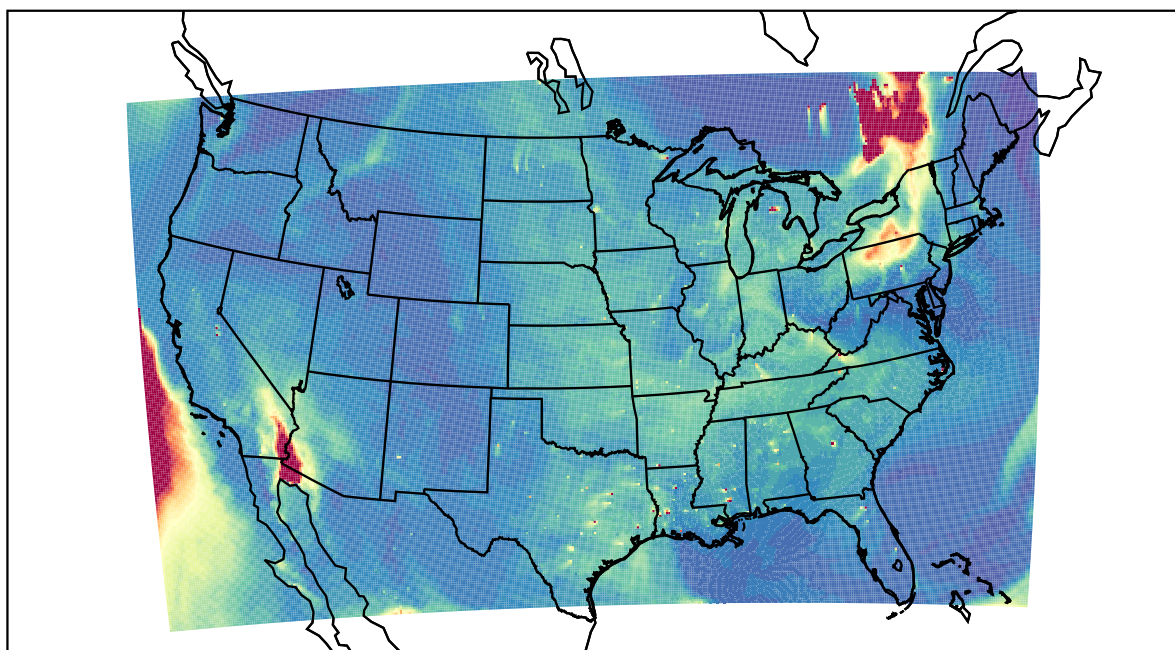
WRF 2023-06-05_21:00:00
