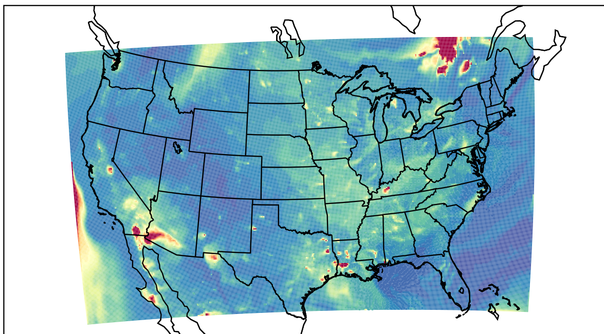
WRF 2023-06-05_04:00:00
