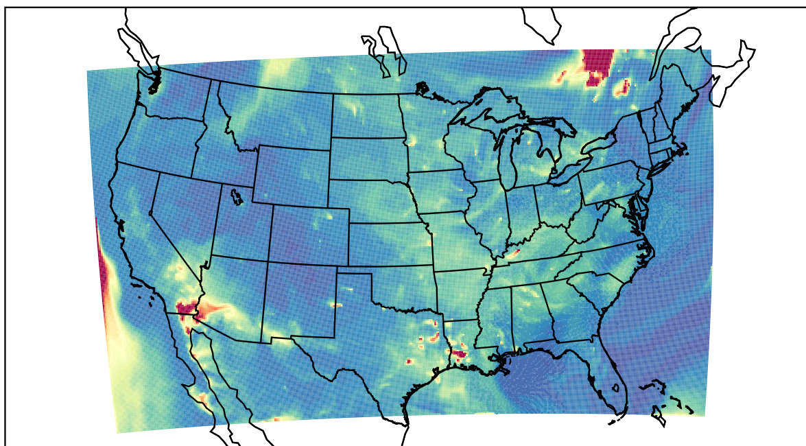
WRF 2023-06-05_07:00:00
