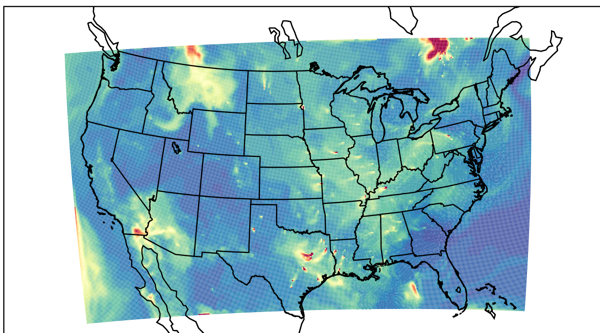
WRF 2023-06-04_14:00:00
