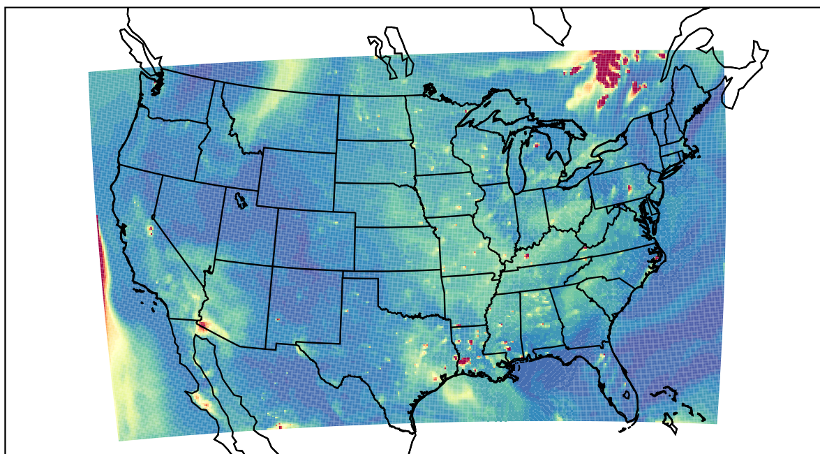
WRF 2023-06-05_01:00:00
