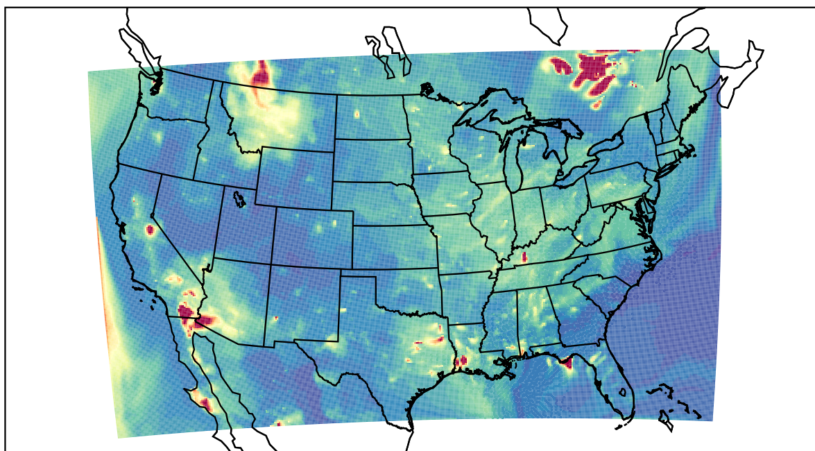
WRF 2023-06-04_04:00:00
