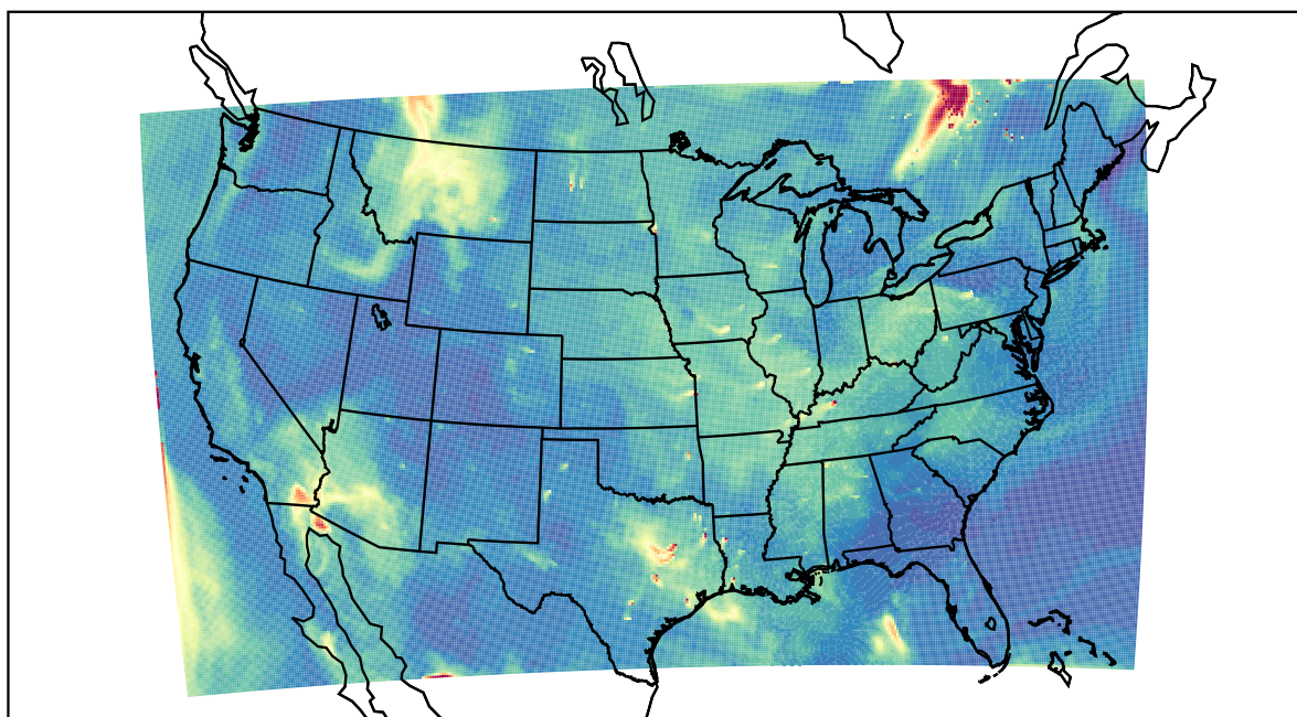
WRF 2023-06-04_16:00:00
