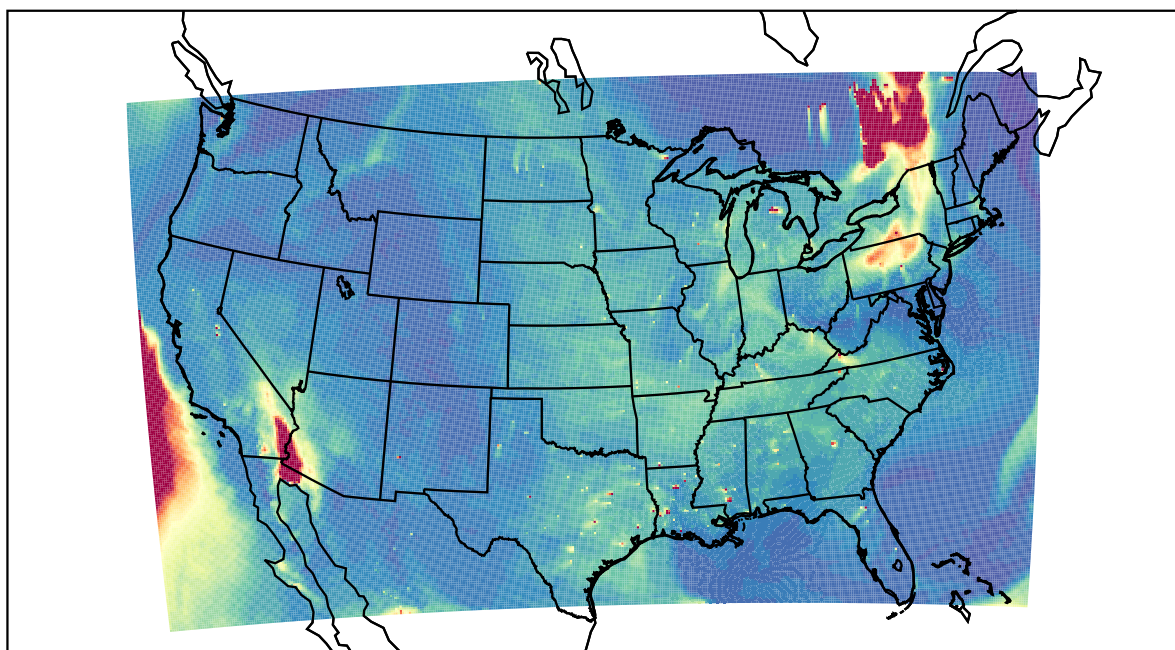
WRF 2023-06-05_22:00:00
