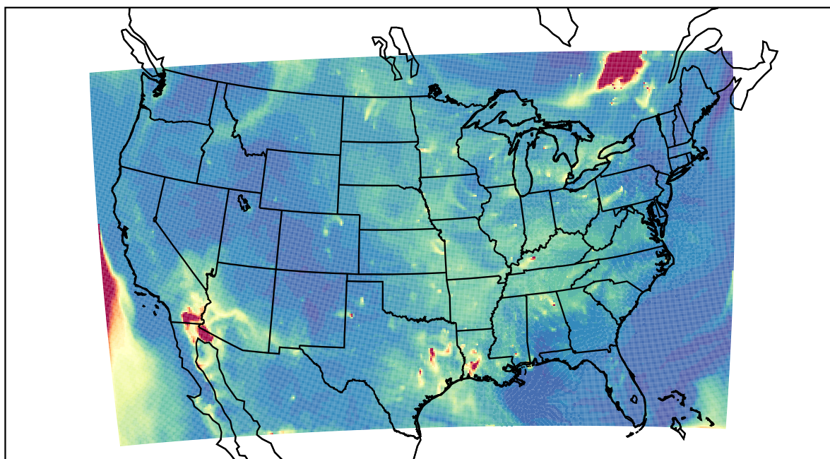
WRF 2023-06-05_12:00:00
