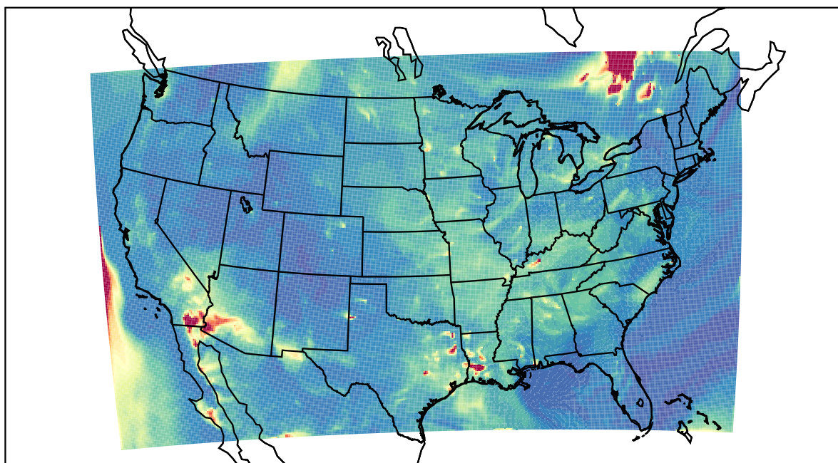
WRF 2023-06-05_06:00:00
