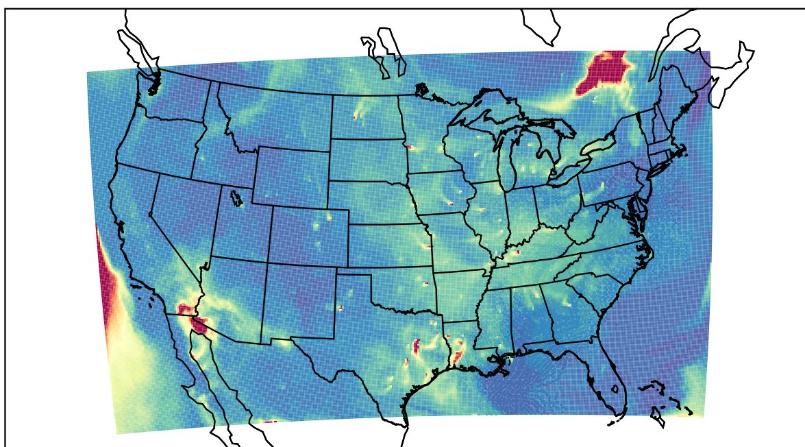
WRF 2023-06-05_14:00:00
