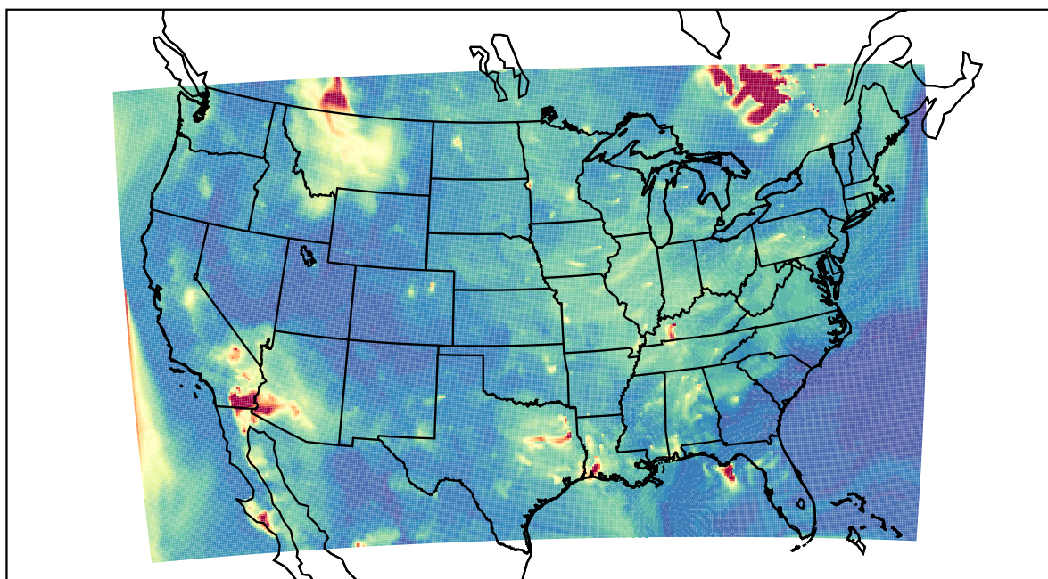
WRF 2023-06-04_06:00:00
