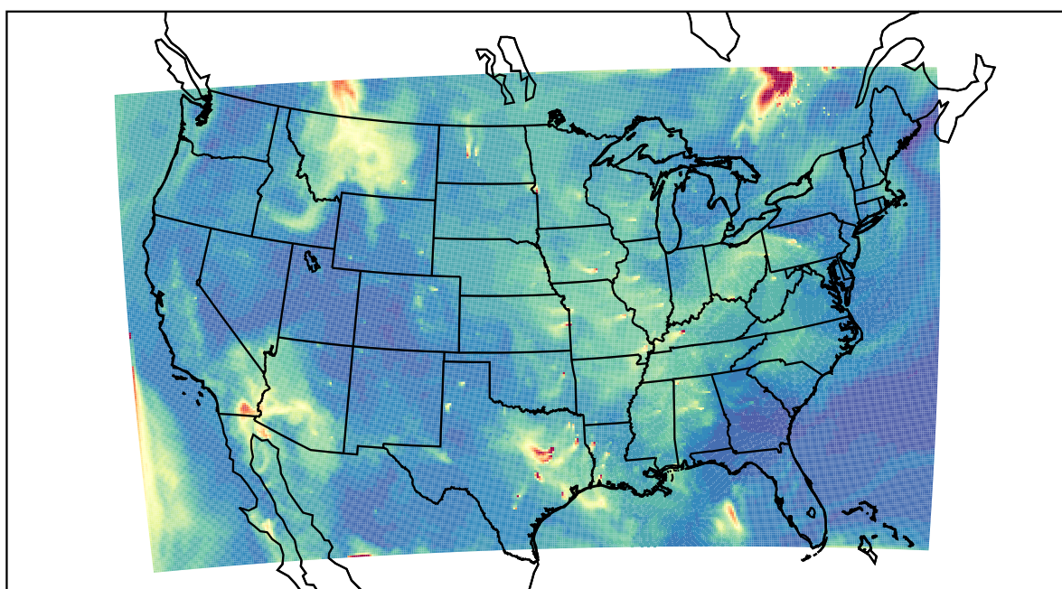
WRF 2023-06-04_15:00:00
