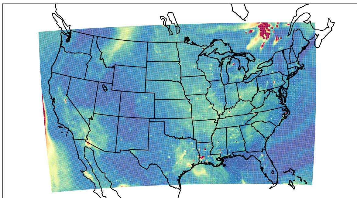
WRF 2023-06-05_00:00:00
