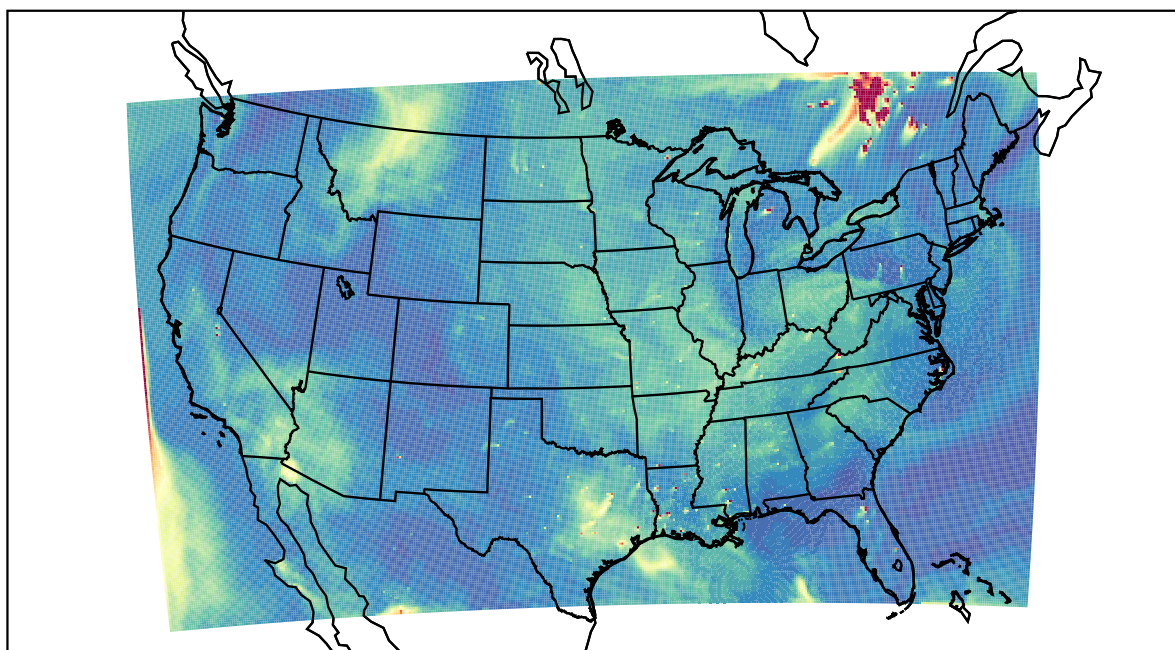
WRF 2023-06-04_21:00:00
