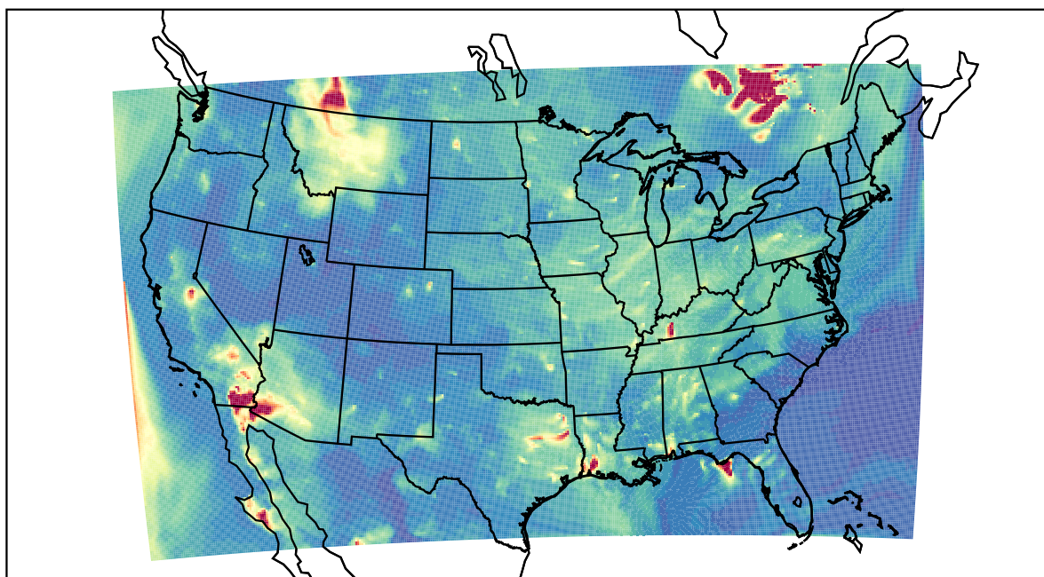
WRF 2023-06-04_05:00:00
