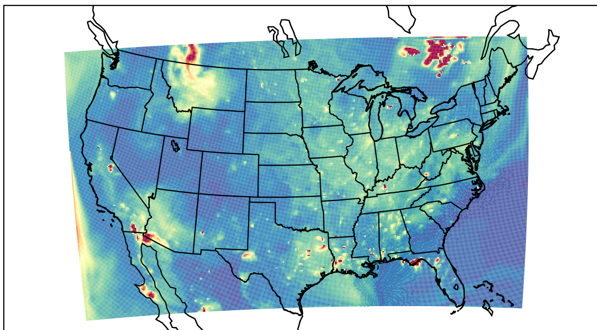
WRF 2023-06-04_02:00:00
