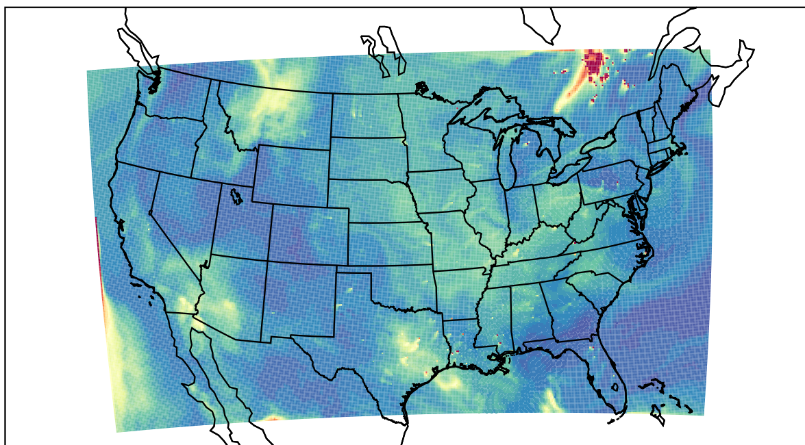
WRF 2023-06-04_19:00:00
