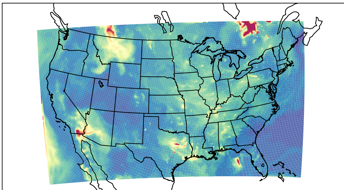
WRF 2023-06-04_11:00:00
