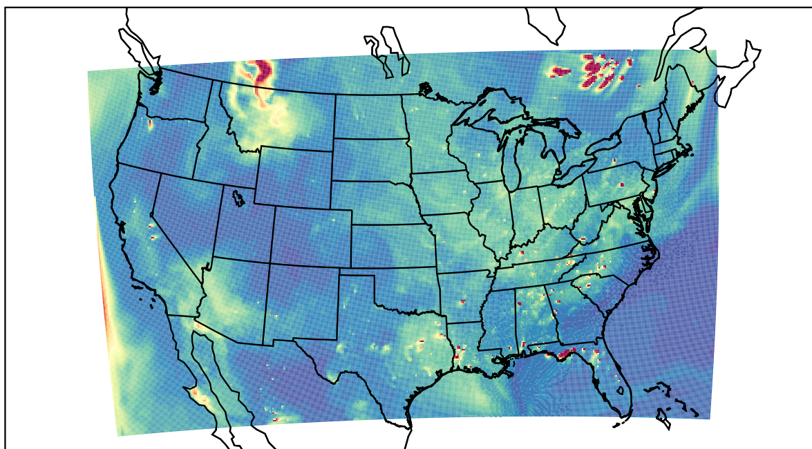
WRF 2023-06-04_00:00:00
