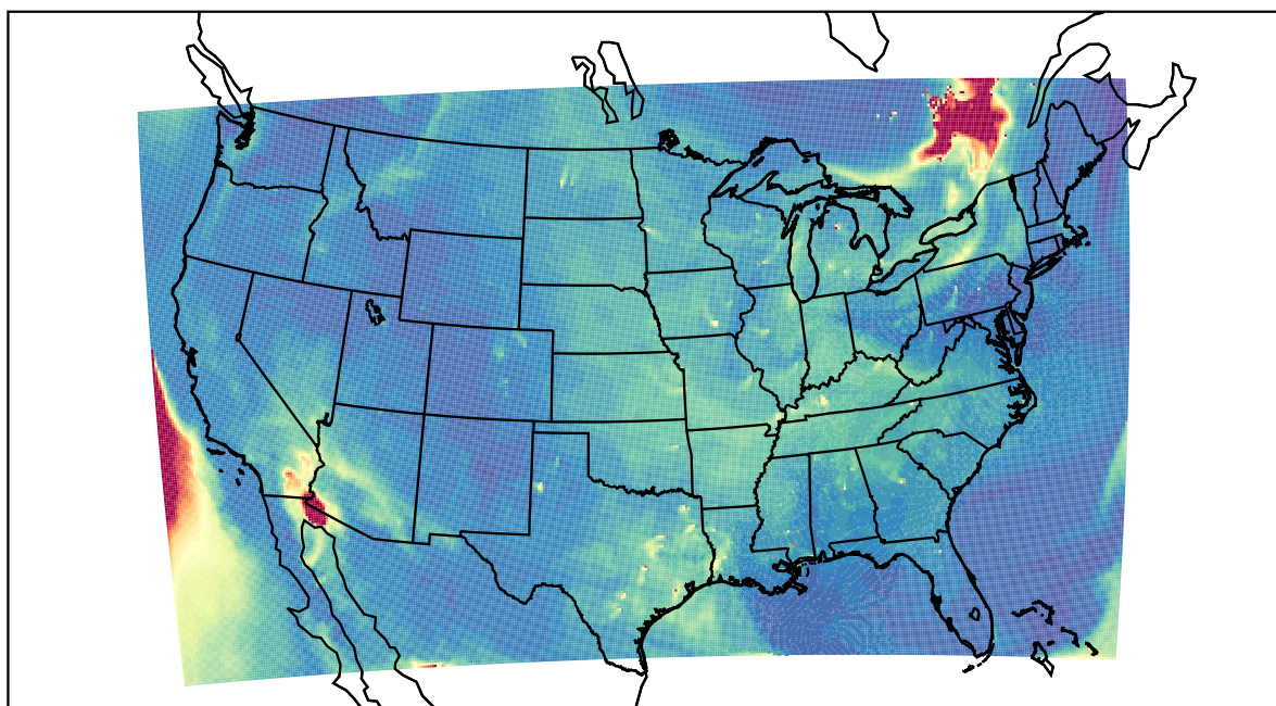
WRF 2023-06-05_17:00:00
