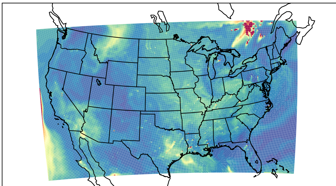
WRF 2023-06-04_22:00:00
