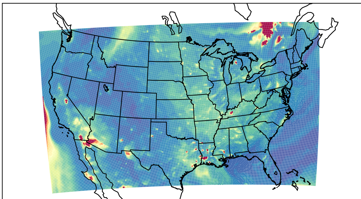
WRF 2023-06-05_03:00:00
