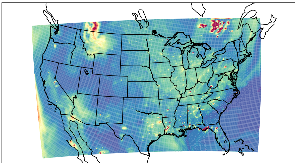
WRF 2023-06-04_01:00:00
