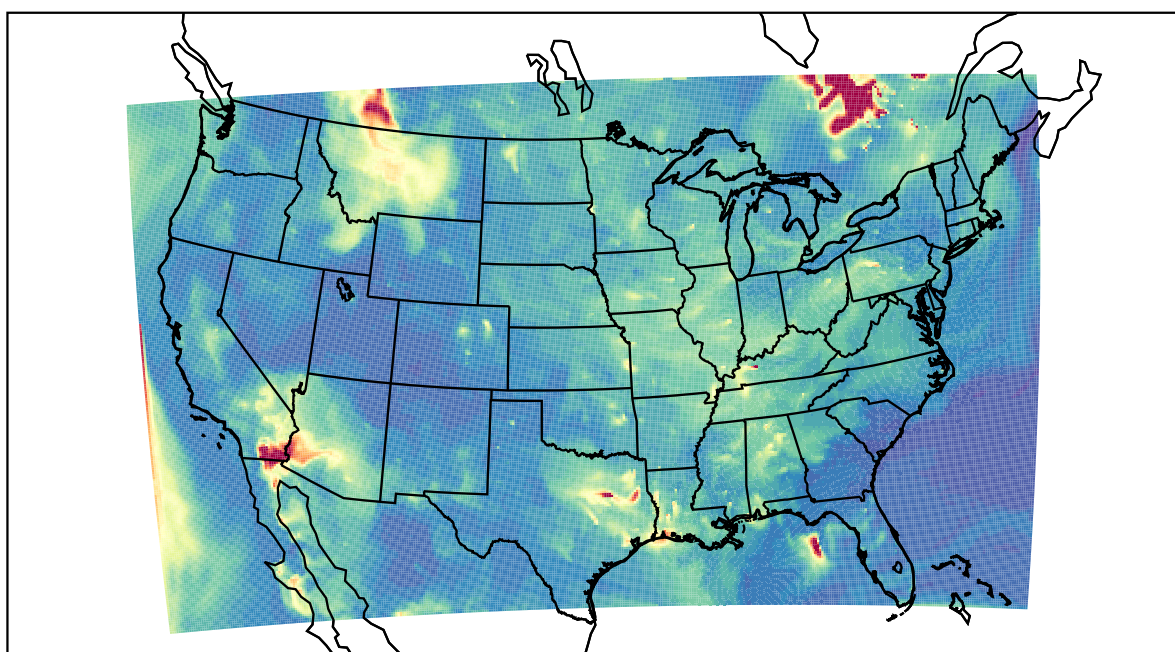
WRF 2023-06-04_09:00:00
