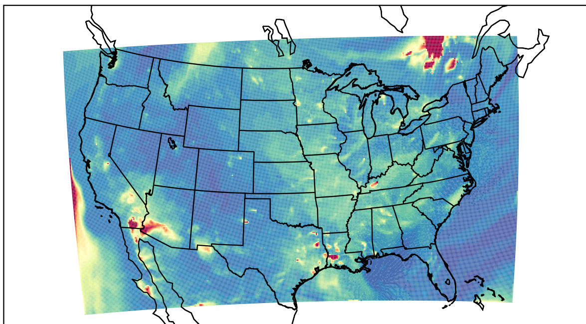
WRF 2023-06-05_05:00:00
