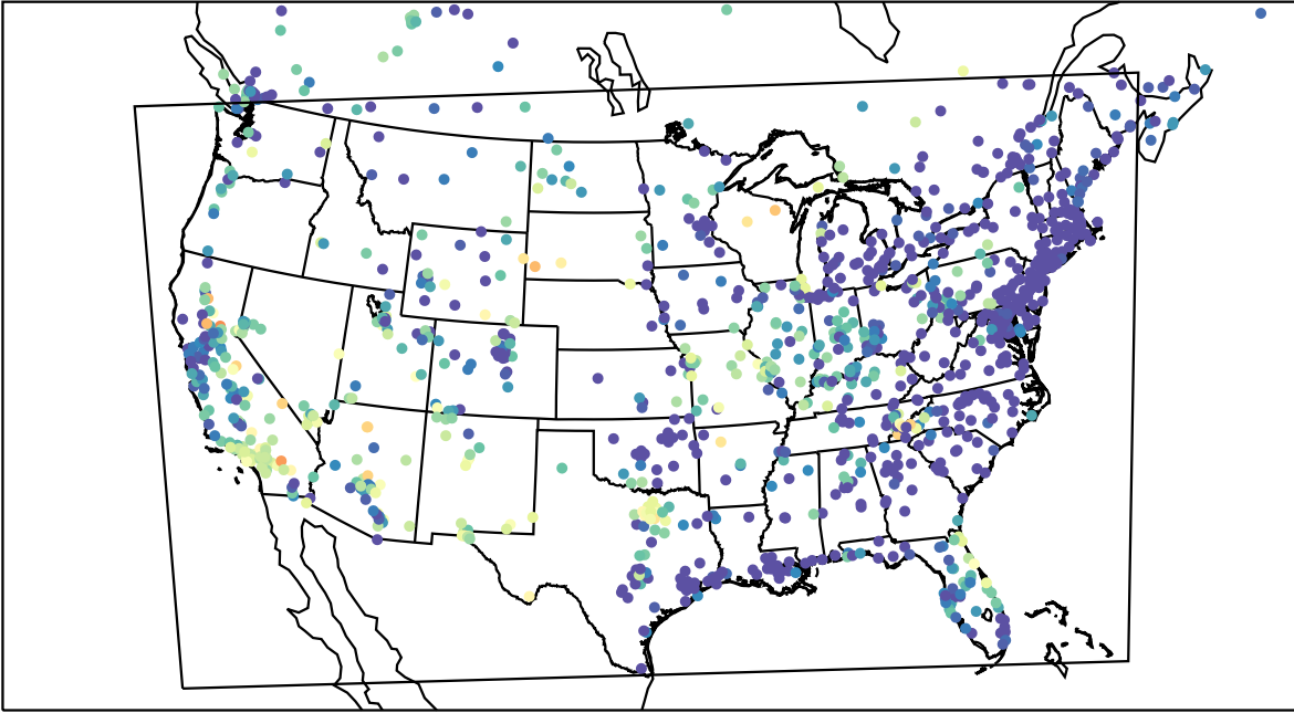
AirNOW (2023-06-05_10:00:00)
