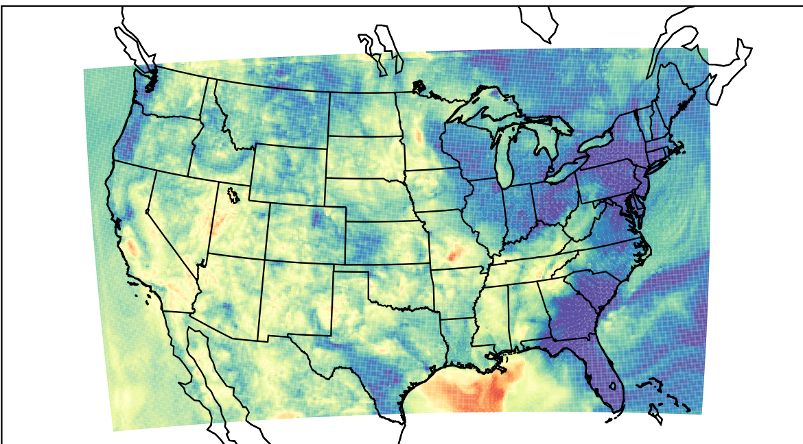
WRF (2023-06-04_11:00:00)
