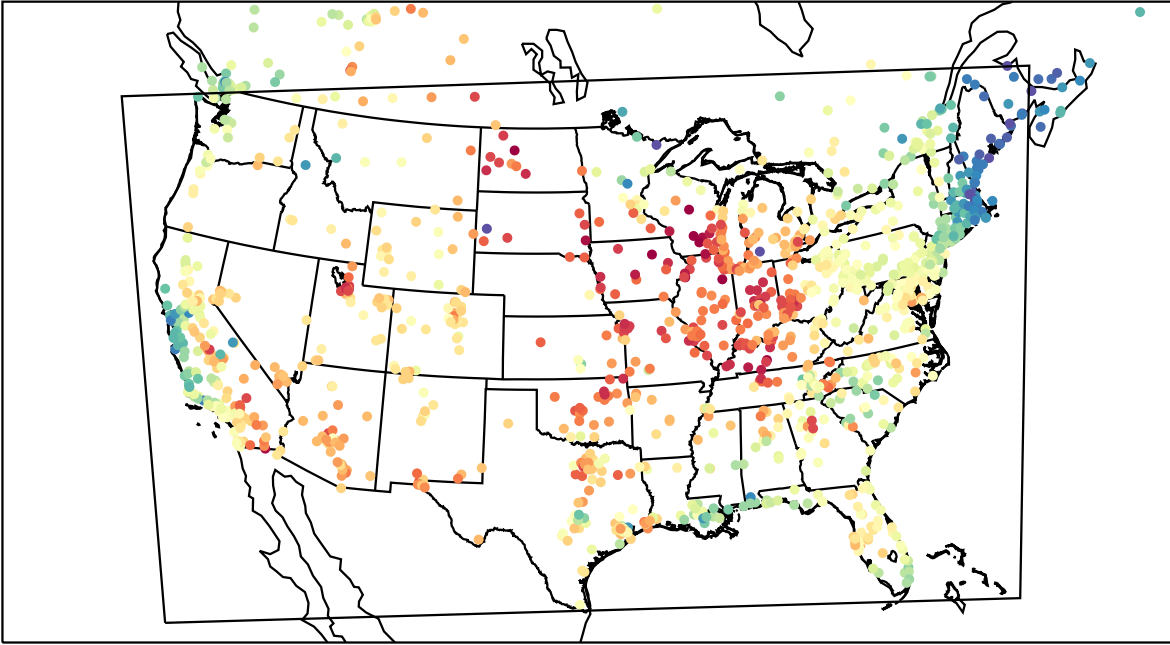
AirNOW (2023-06-05_21:00:00)
