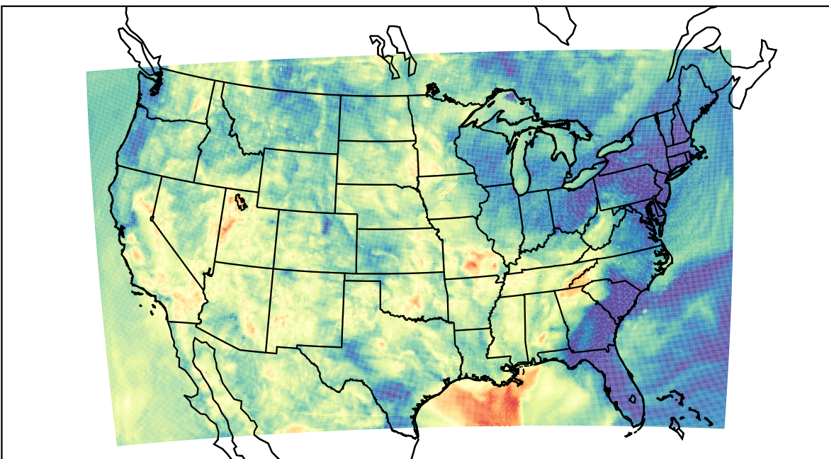
WRF (2023-06-04_08:00:00)
