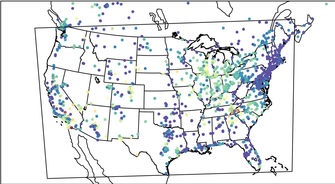
AirNOW (2023-06-04_11:00:00)
