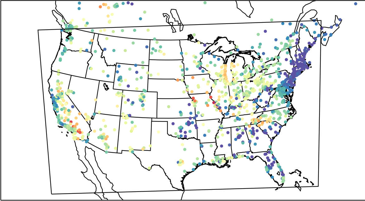
AirNOW (2023-06-04_04:00:00)
