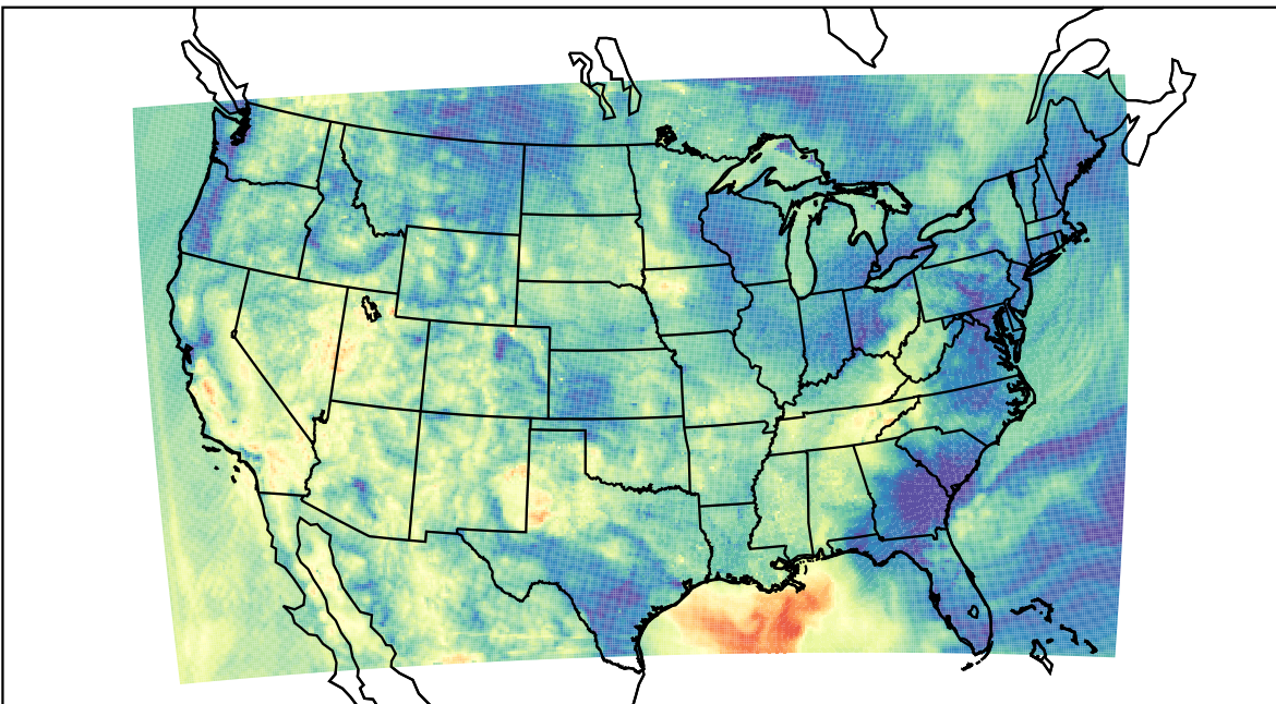
WRF (2023-06-04_13:00:00)
