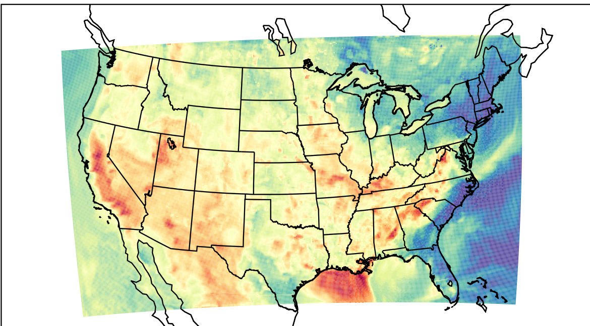
WRF (2023-06-04_01:00:00)
