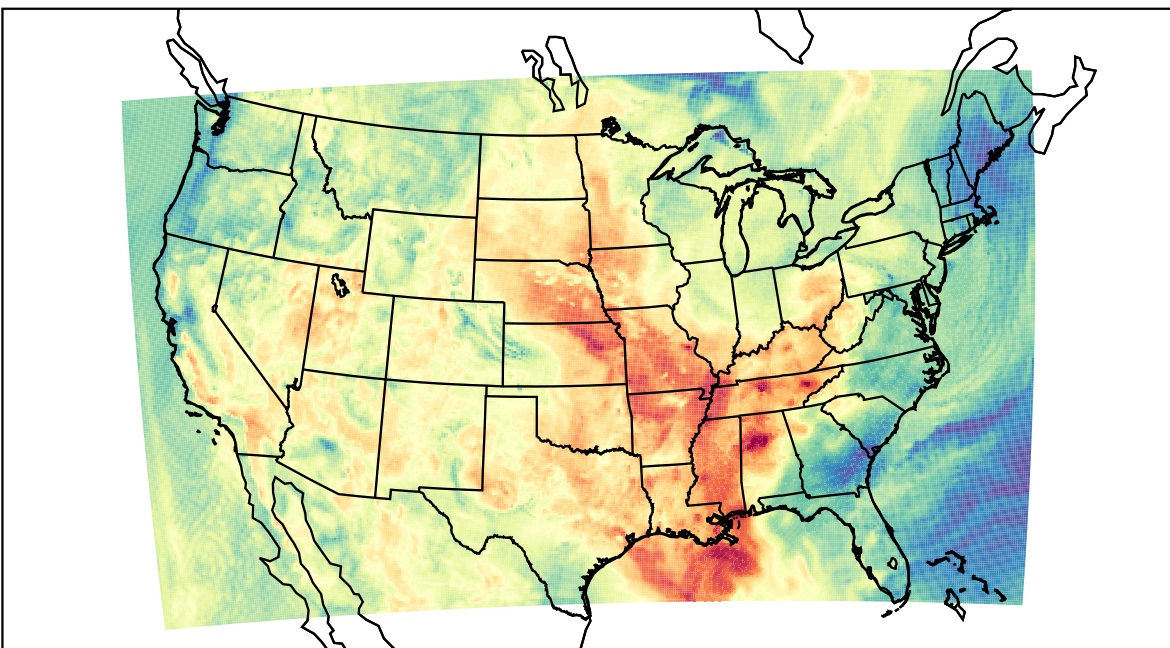
WRF (2023-06-04_16:00:00)
