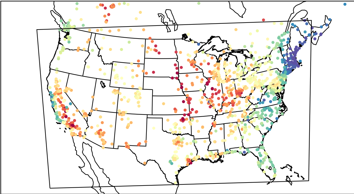
AirNOW (2023-06-04_22:00:00)
