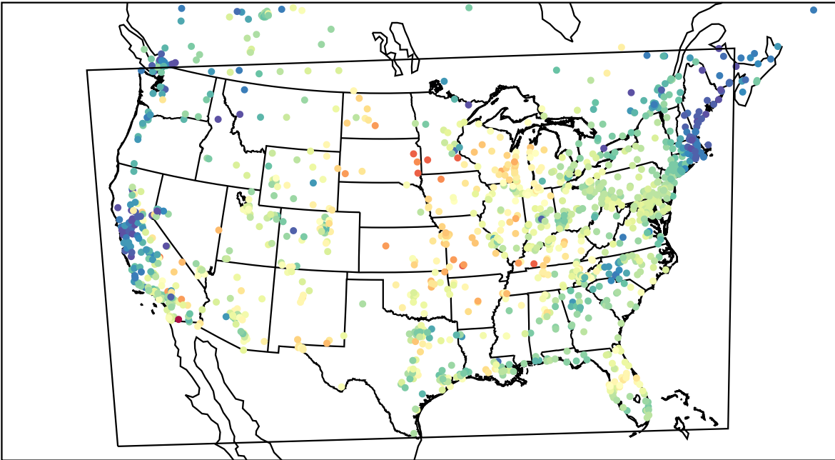
AirNOW (2023-06-05_15:00:00)
