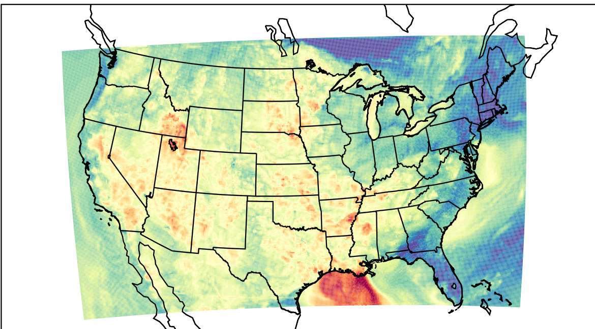
WRF (2023-06-05_04:00:00)
