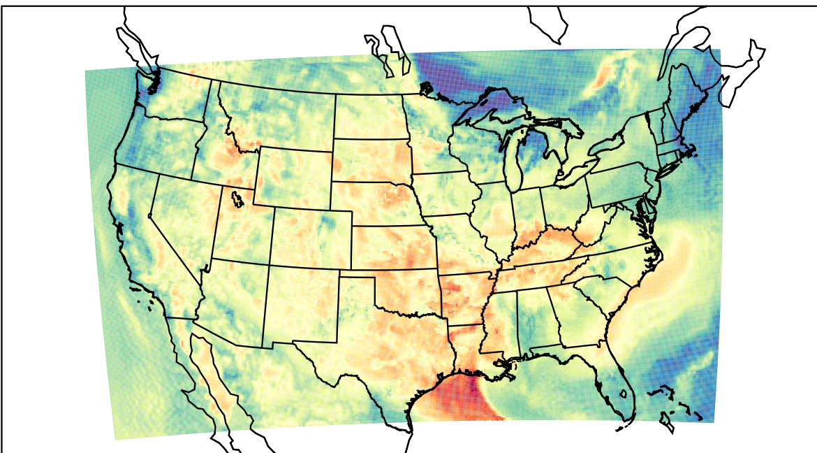
WRF (2023-06-05_15:00:00)
