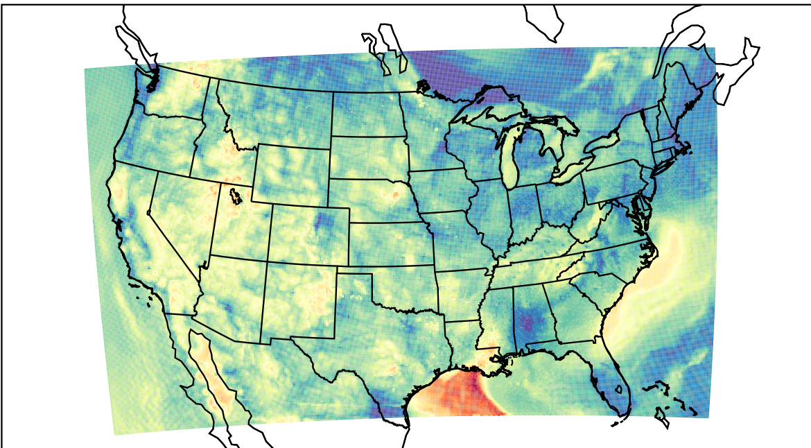
WRF (2023-06-05_13:00:00)
