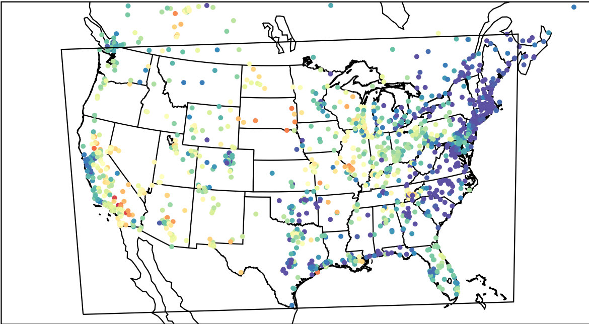
AirNOW (2023-06-05_04:00:00)
