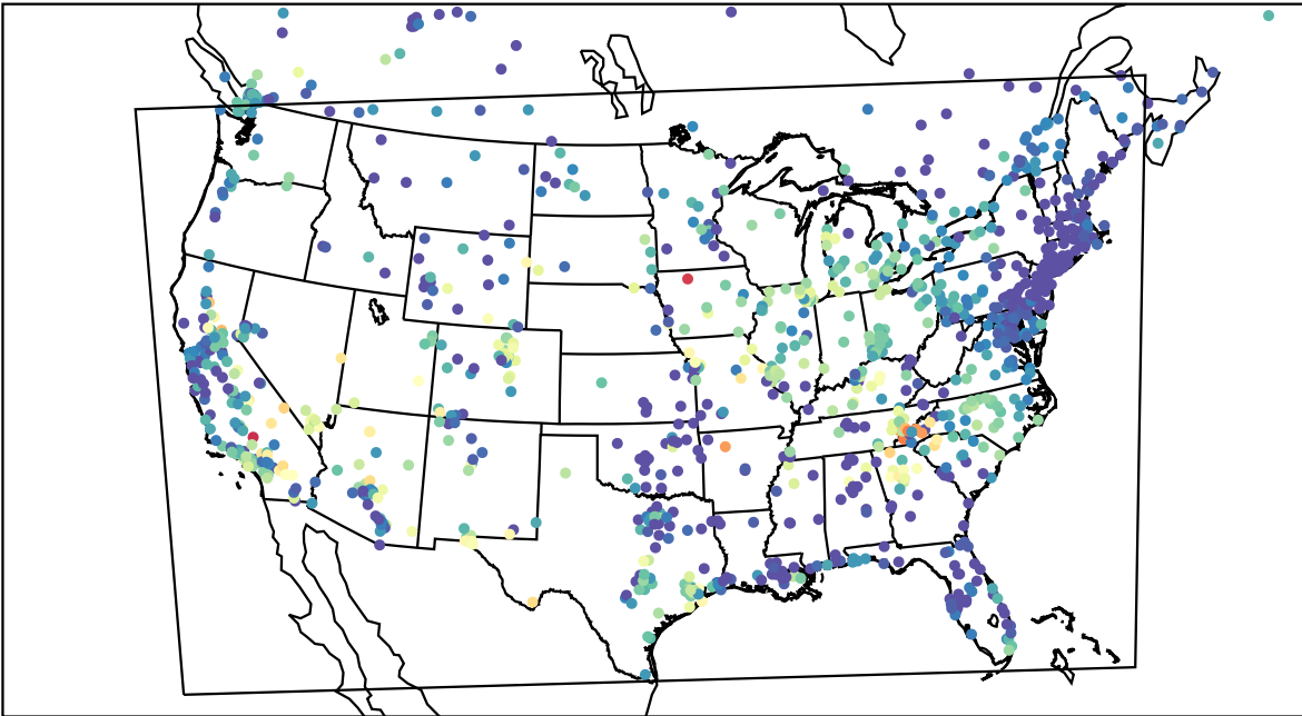
AirNOW (2023-06-04_10:00:00)
