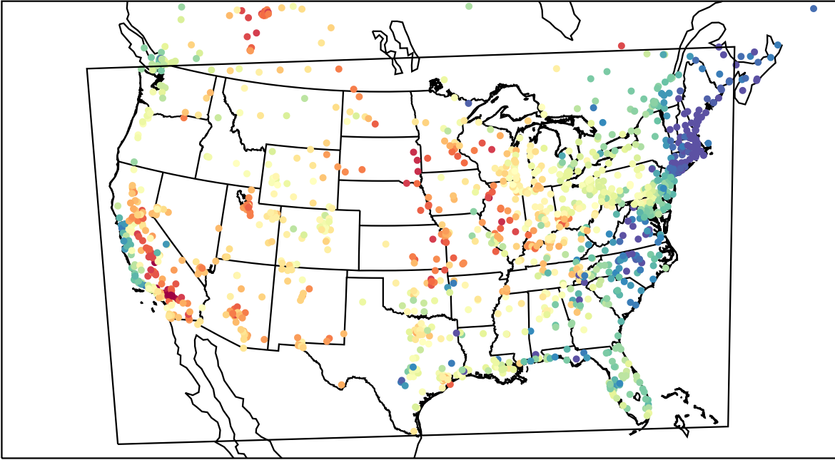
AirNOW (2023-06-05_00:00:00)
