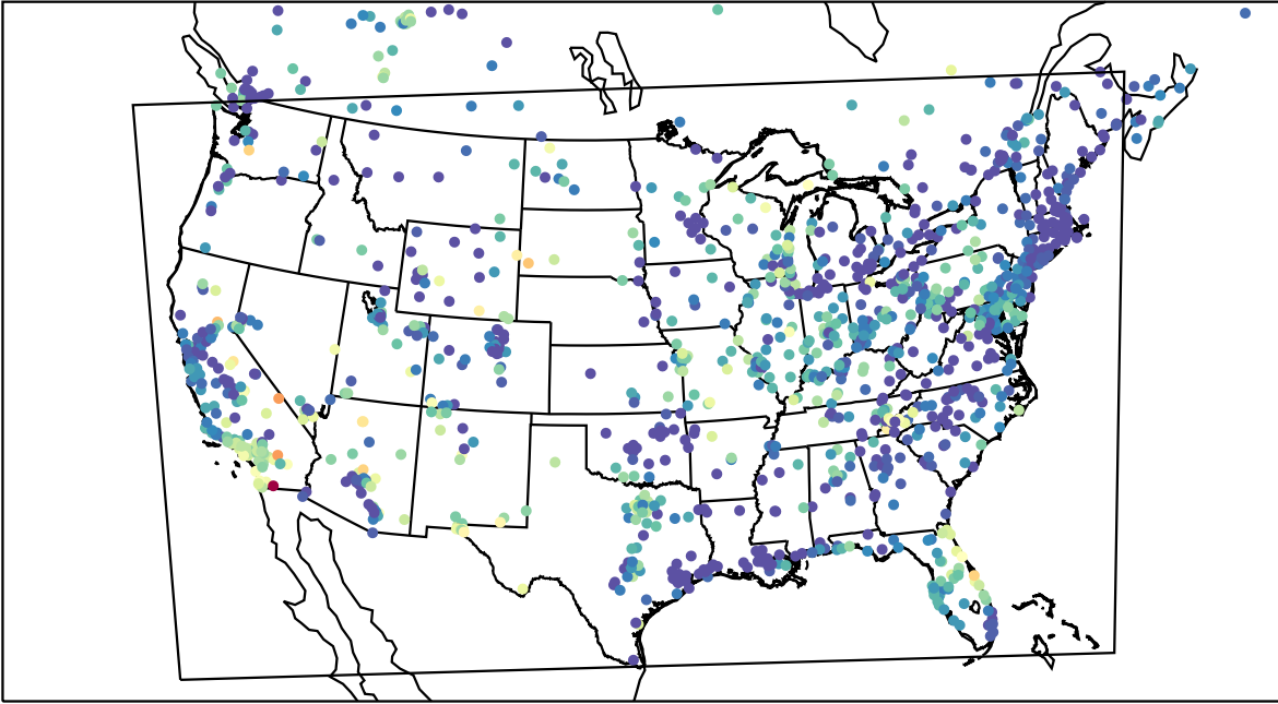
AirNOW (2023-06-05_12:00:00)
