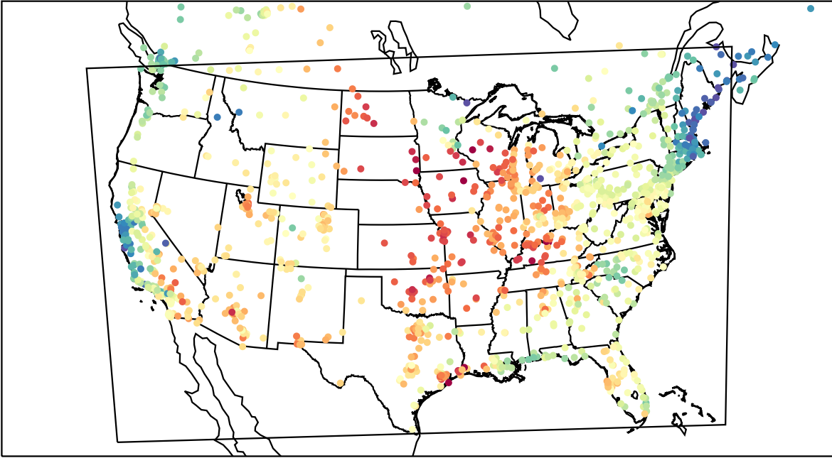
AirNOW (2023-06-05_18:00:00)
