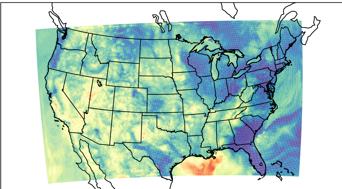
WRF (2023-06-04_12:00:00)
