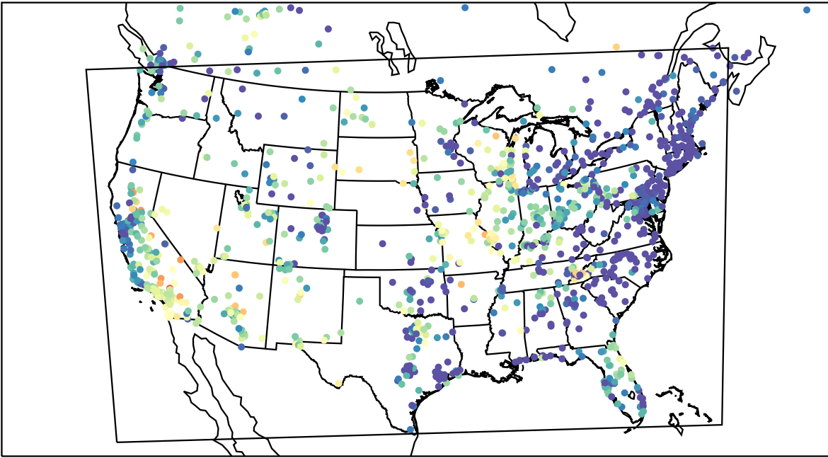
AirNOW (2023-06-05_07:00:00)
