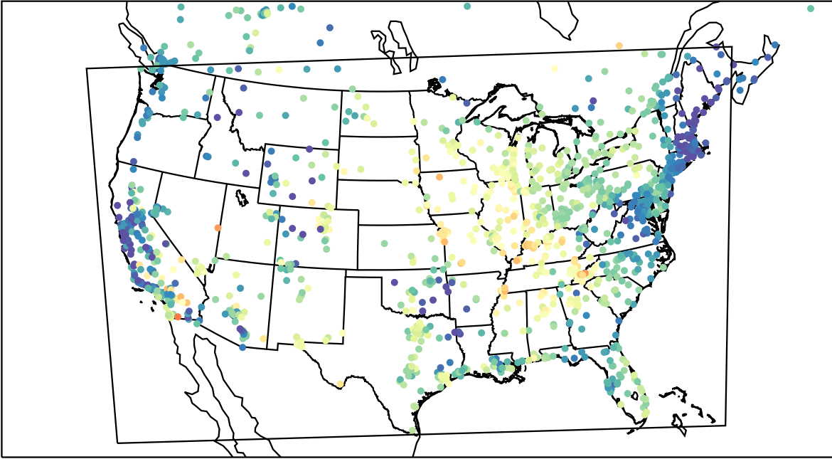
AirNOW (2023-06-04_14:00:00)
