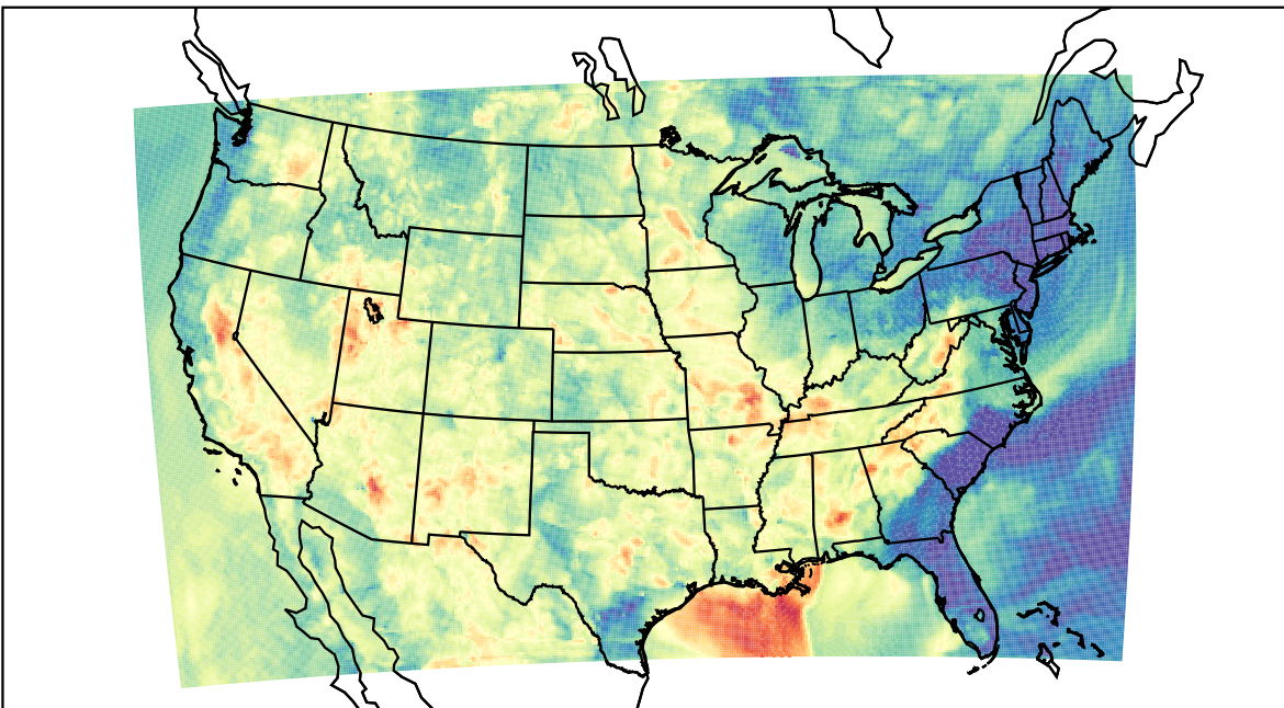
WRF (2023-06-04_04:00:00)
