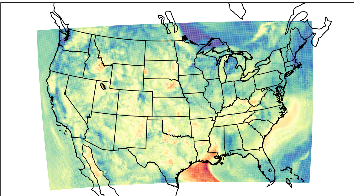
WRF (2023-06-05_14:00:00)
