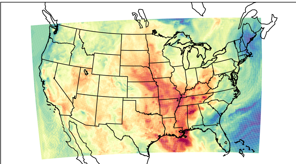
WRF (2023-06-04_17:00:00)
