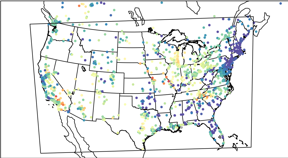
AirNOW (2023-06-04_05:00:00)
