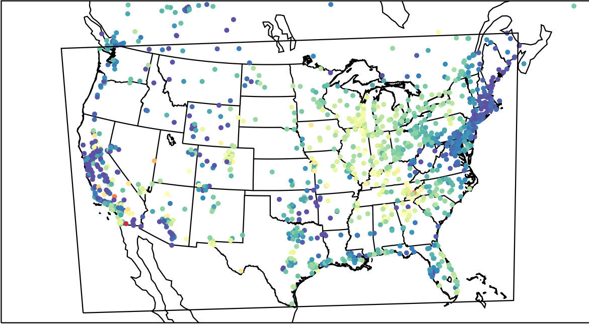
AirNOW (2023-06-04_13:00:00)
