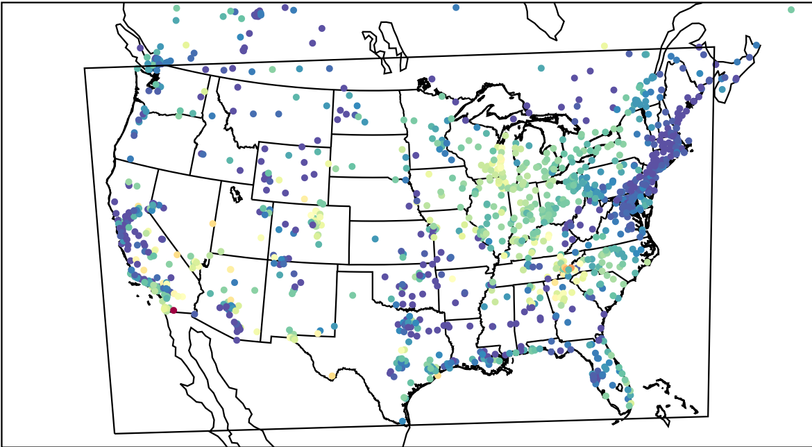
AirNOW (2023-06-04_12:00:00)
