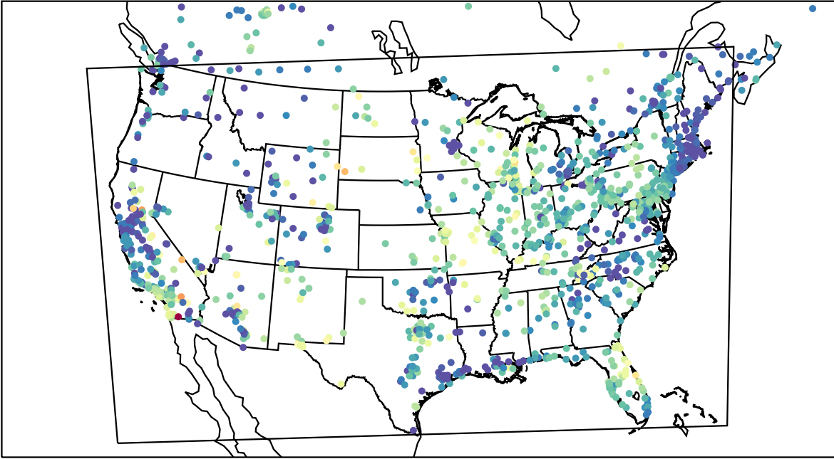
AirNOW (2023-06-05_13:00:00)
