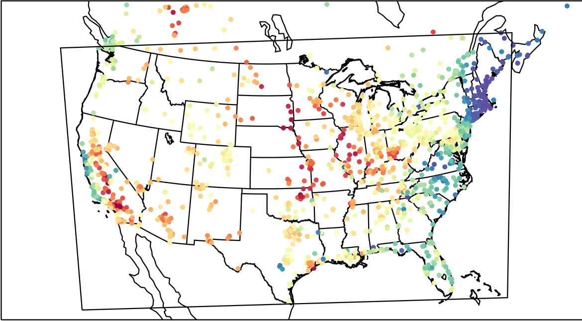
AirNOW (2023-06-04_23:00:00)
