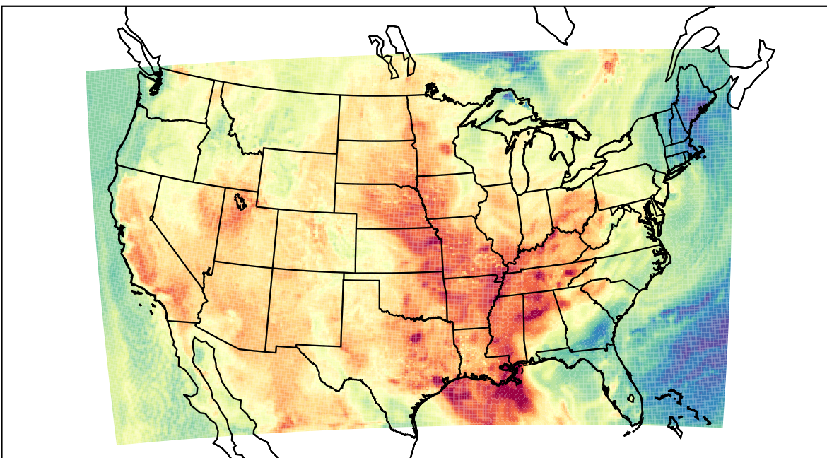
WRF (2023-06-04_19:00:00)
