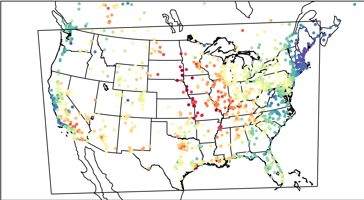
AirNOW (2023-06-04_17:00:00)
