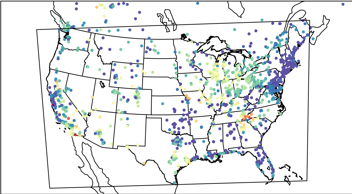
AirNOW (2023-06-04_08:00:00)
