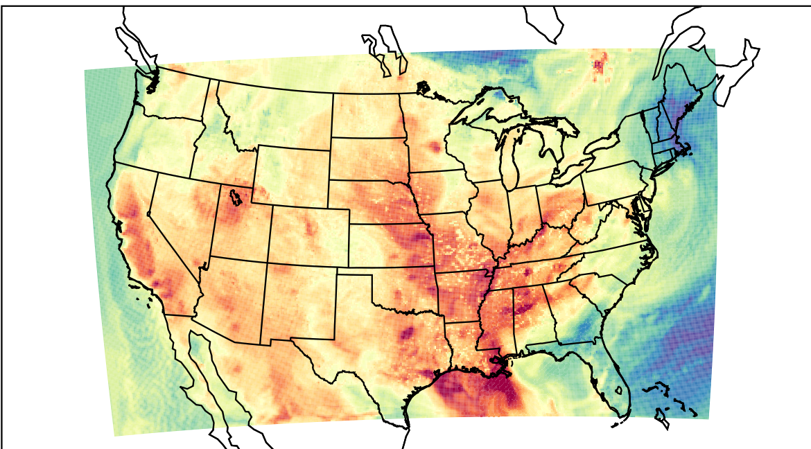
WRF (2023-06-04_21:00:00)
