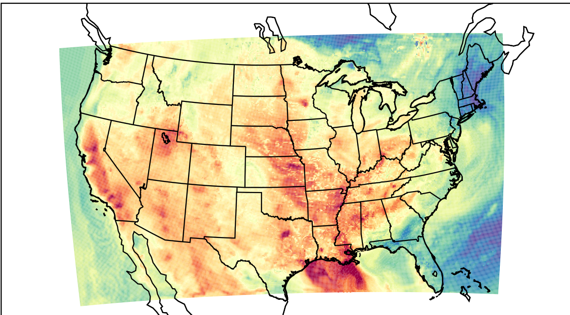
WRF (2023-06-04_23:00:00)
