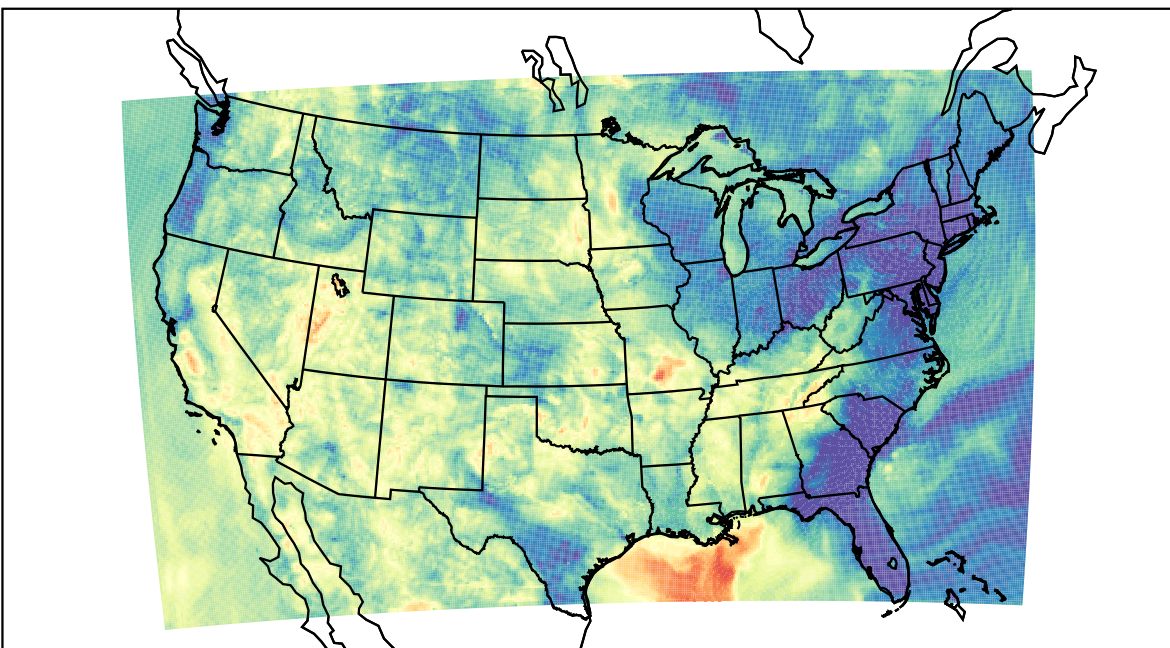
WRF (2023-06-04_10:00:00)
