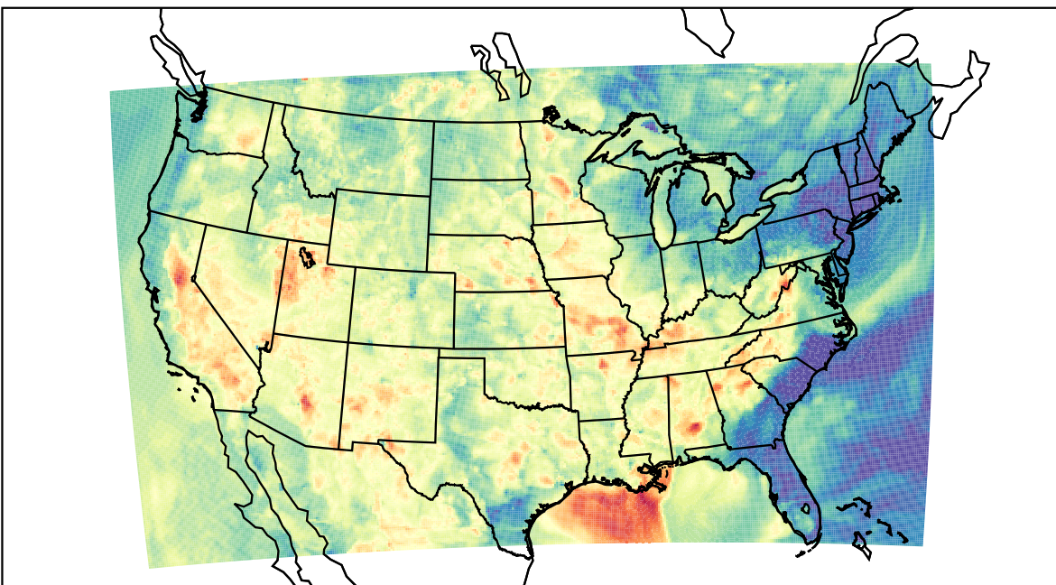
WRF (2023-06-04_03:00:00)
