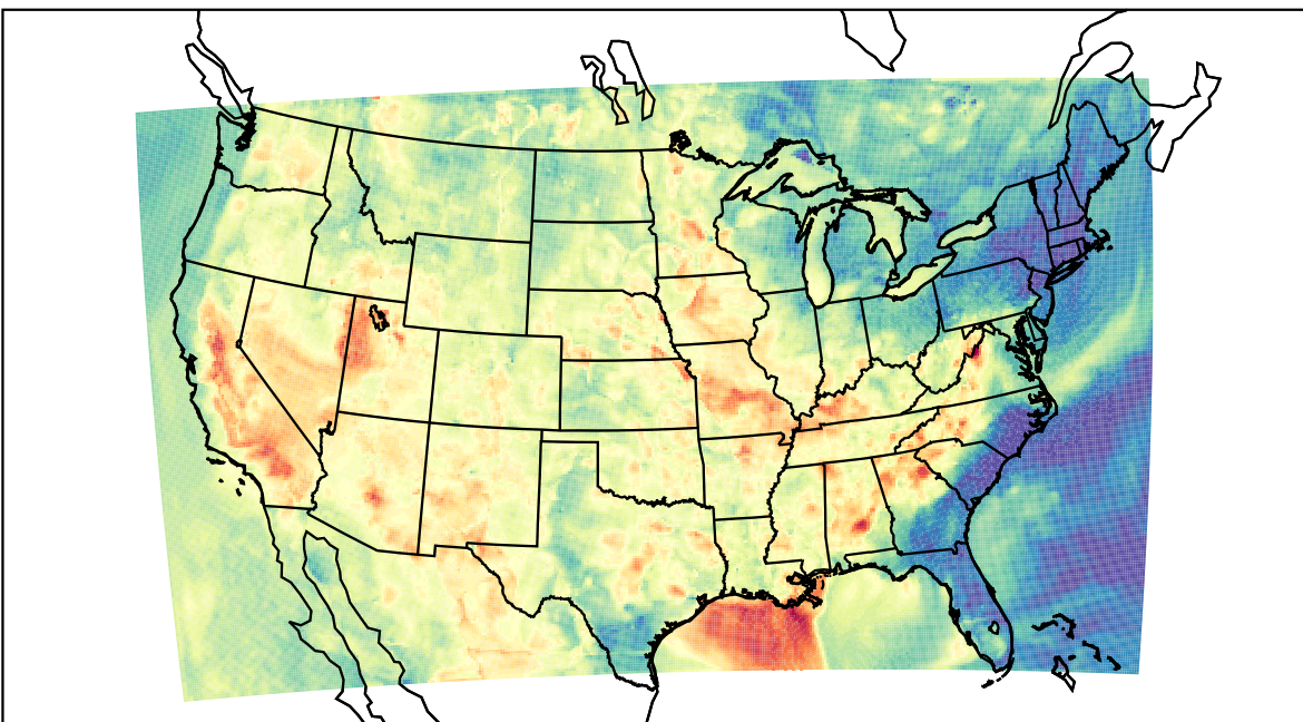
WRF (2023-06-04_02:00:00)
