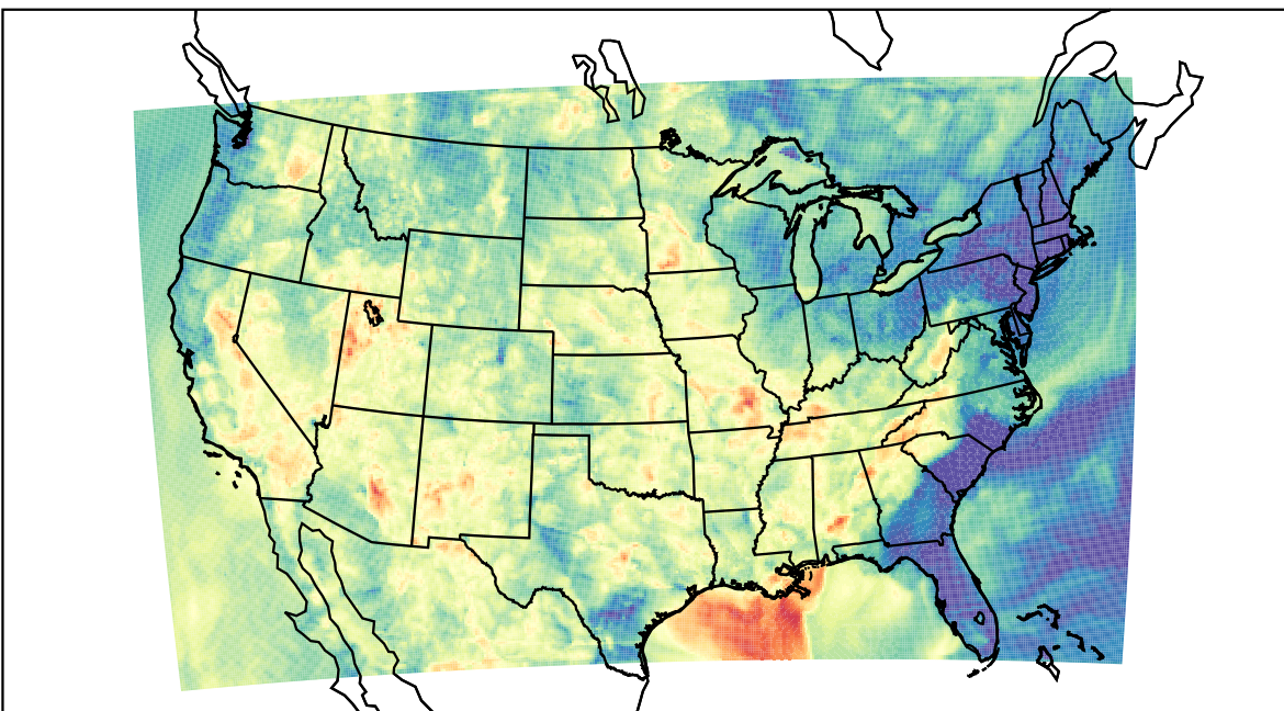
WRF (2023-06-04_05:00:00)
