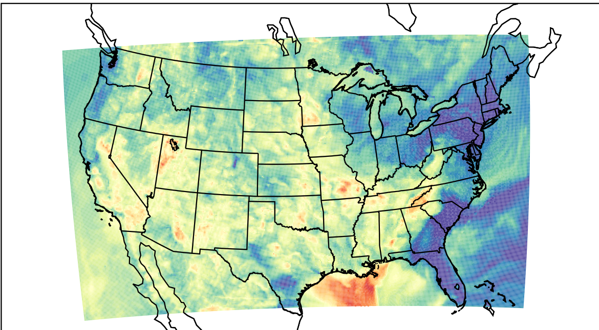
WRF (2023-06-04_07:00:00)
