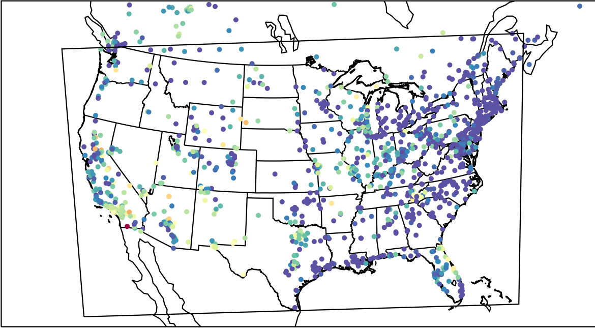
AirNOW (2023-06-05_11:00:00)
