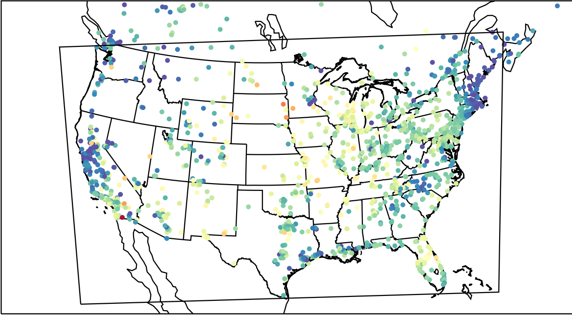
AirNOW (2023-06-05_14:00:00)
