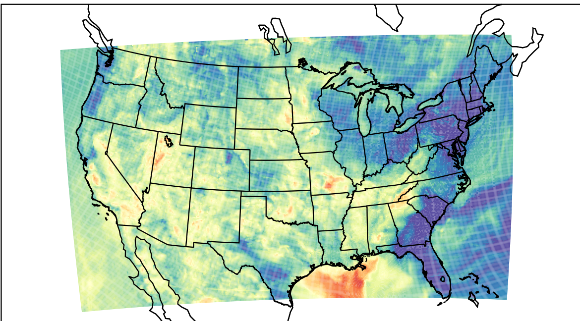
WRF (2023-06-04_09:00:00)
