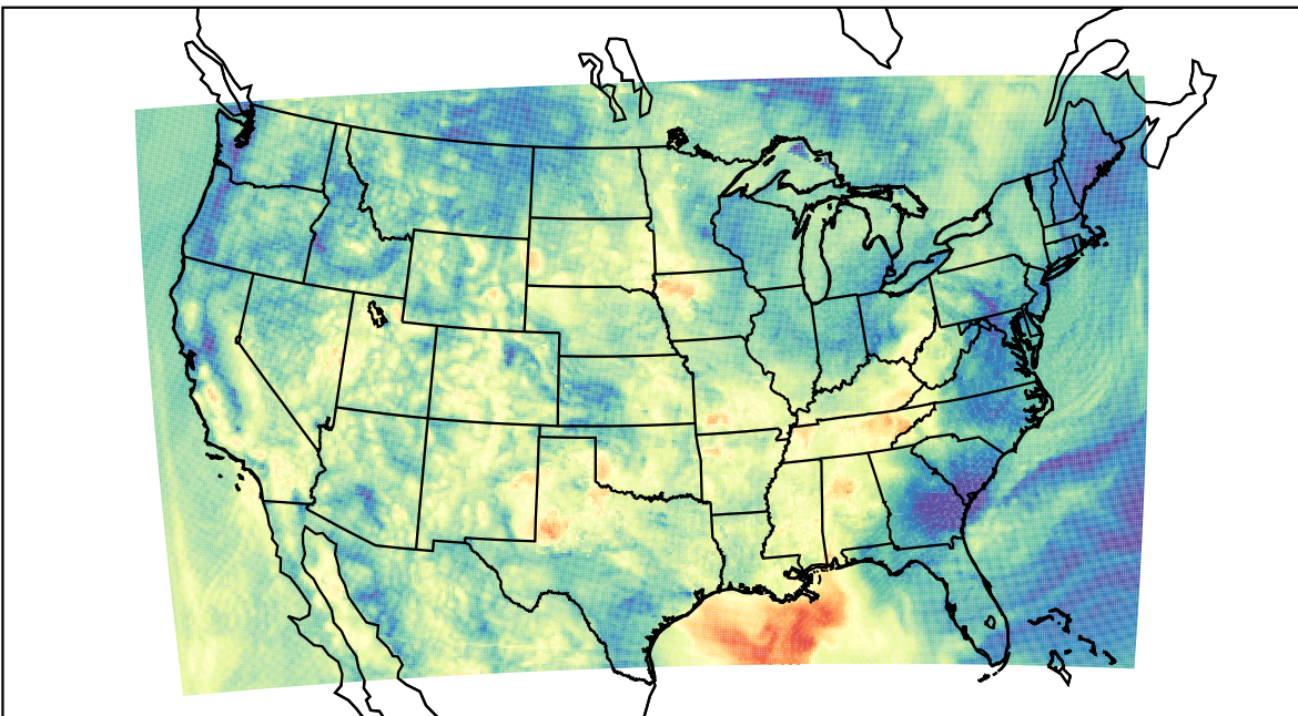
WRF (2023-06-04_14:00:00)
