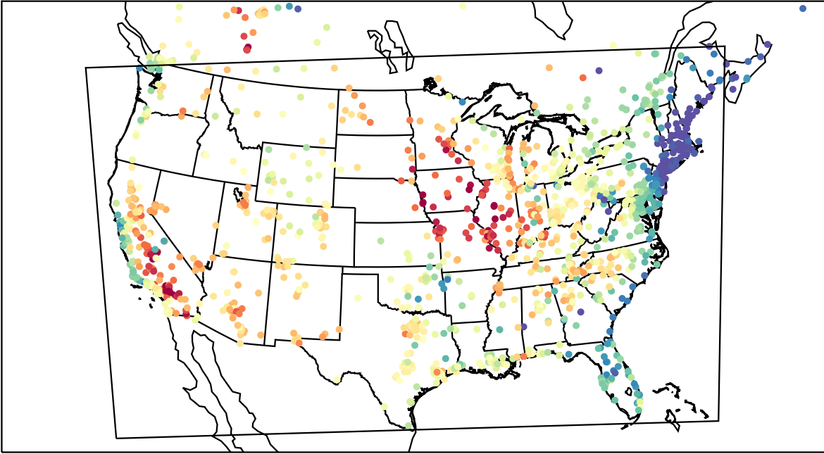
AirNOW (2023-06-04_00:00:00)
