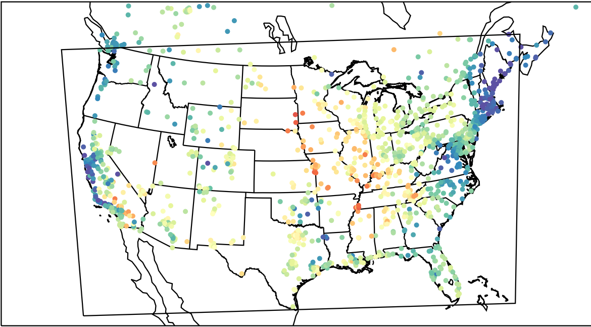
AirNOW (2023-06-04_15:00:00)
