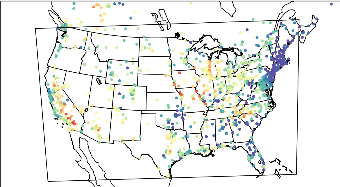
AirNOW (2023-06-04_03:00:00)
