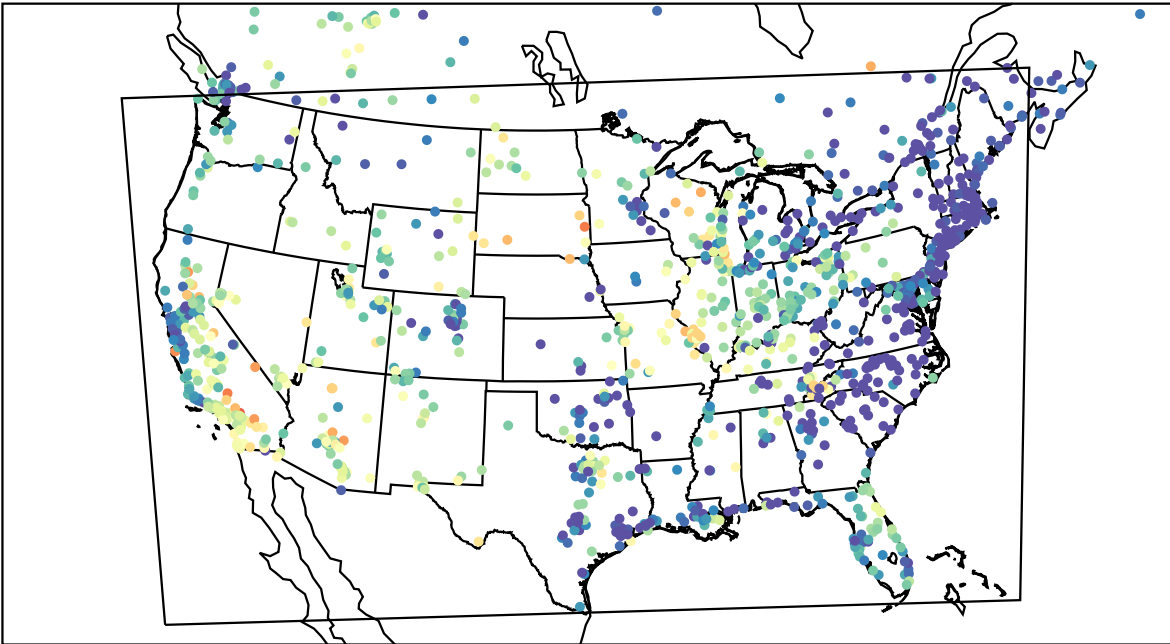
AirNOW (2023-06-05_06:00:00)
