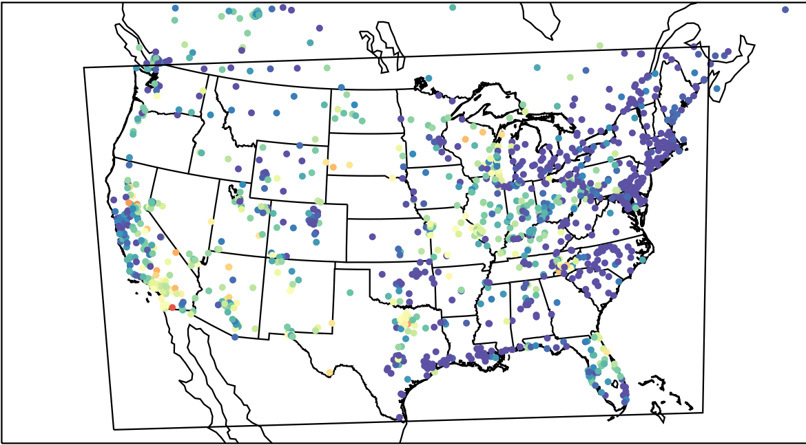
AirNOW (2023-06-05_09:00:00)
