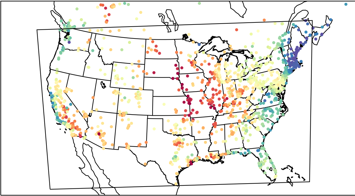
AirNOW (2023-06-04_19:00:00)
