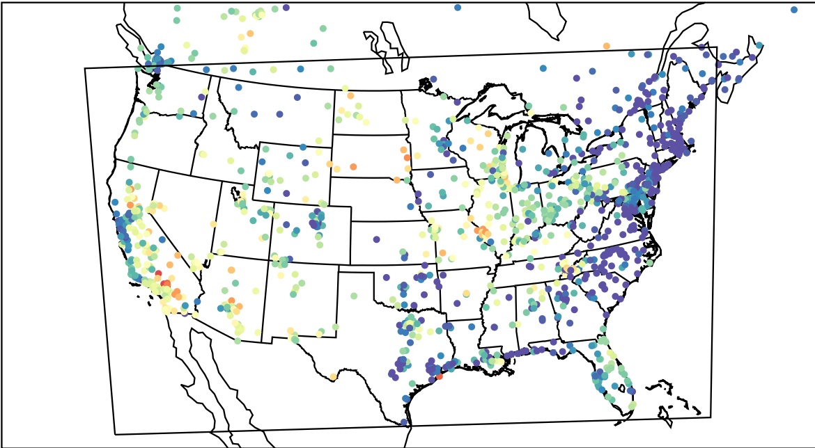
AirNOW (2023-06-05_05:00:00)
