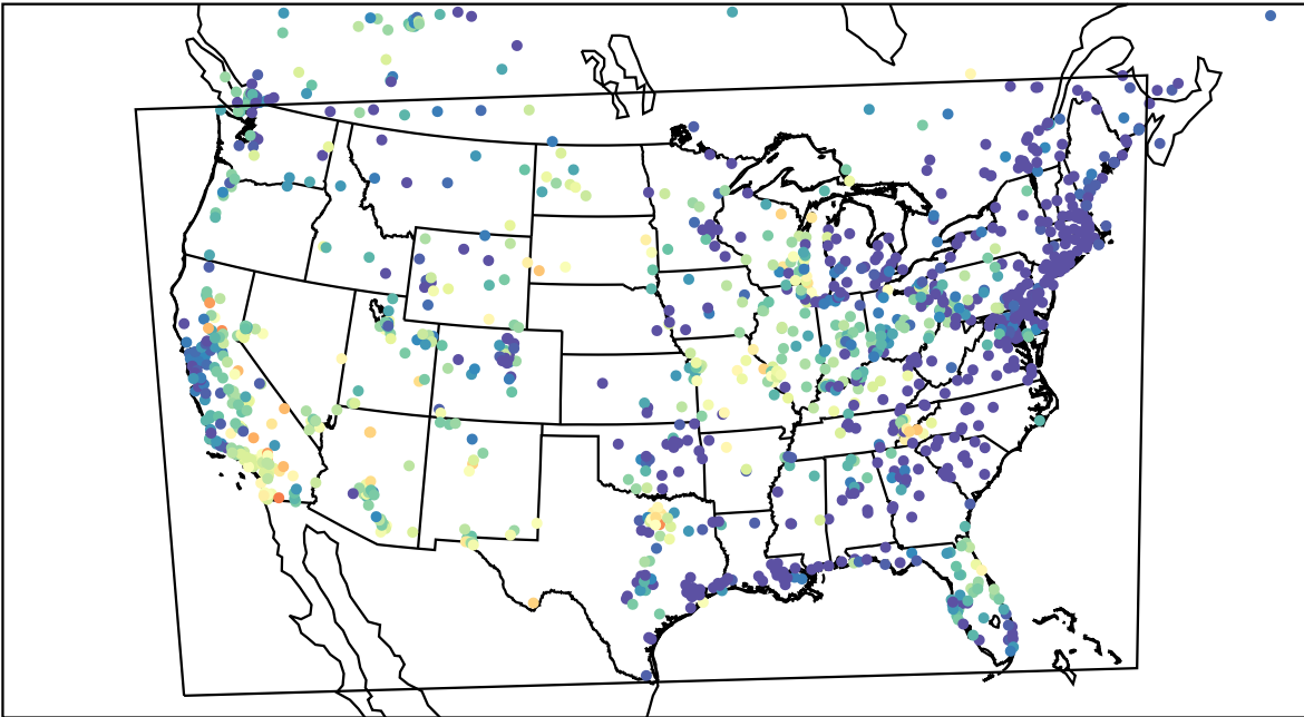
AirNOW (2023-06-05_08:00:00)
