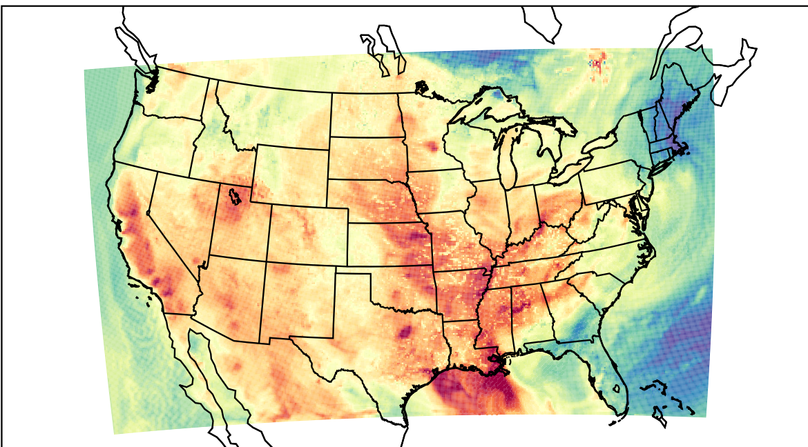
WRF (2023-06-04_22:00:00)
