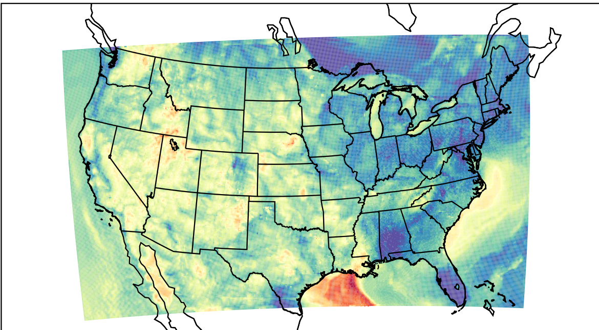
WRF (2023-06-05_12:00:00)
