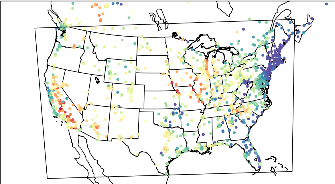
AirNOW (2023-06-04_02:00:00)
