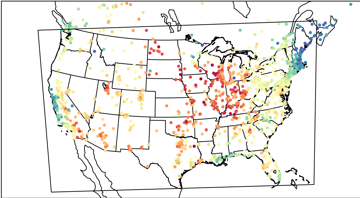
AirNOW (2023-06-05_20:00:00)
