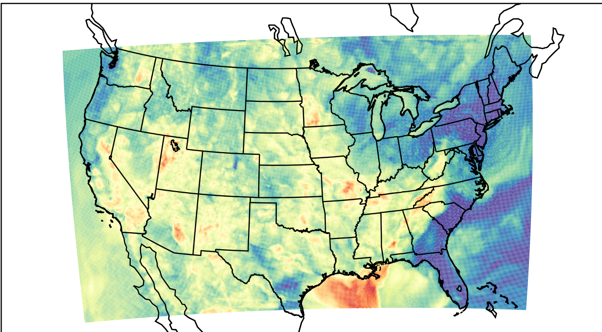
WRF (2023-06-04_06:00:00)
