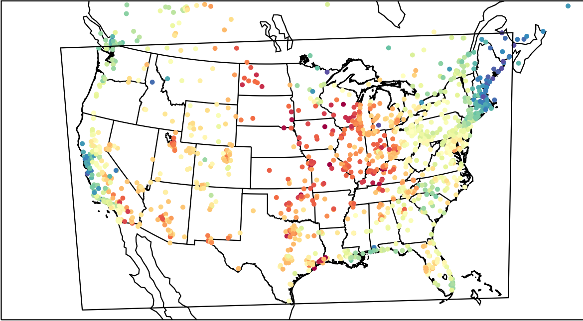
AirNOW (2023-06-05_19:00:00)
