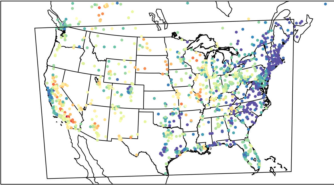
AirNOW (2023-06-05_03:00:00)
