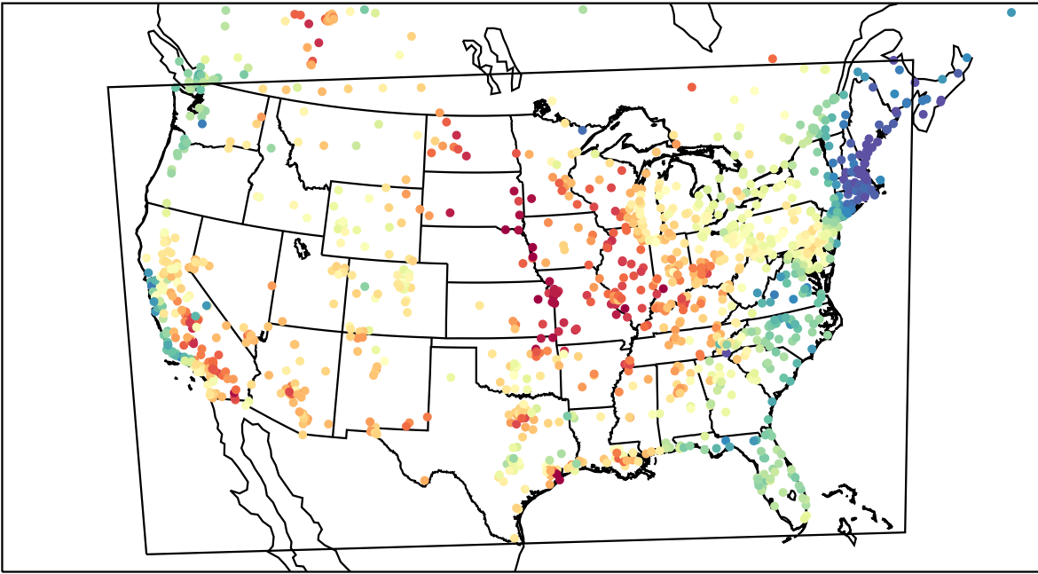
AirNOW (2023-06-04_20:00:00)
