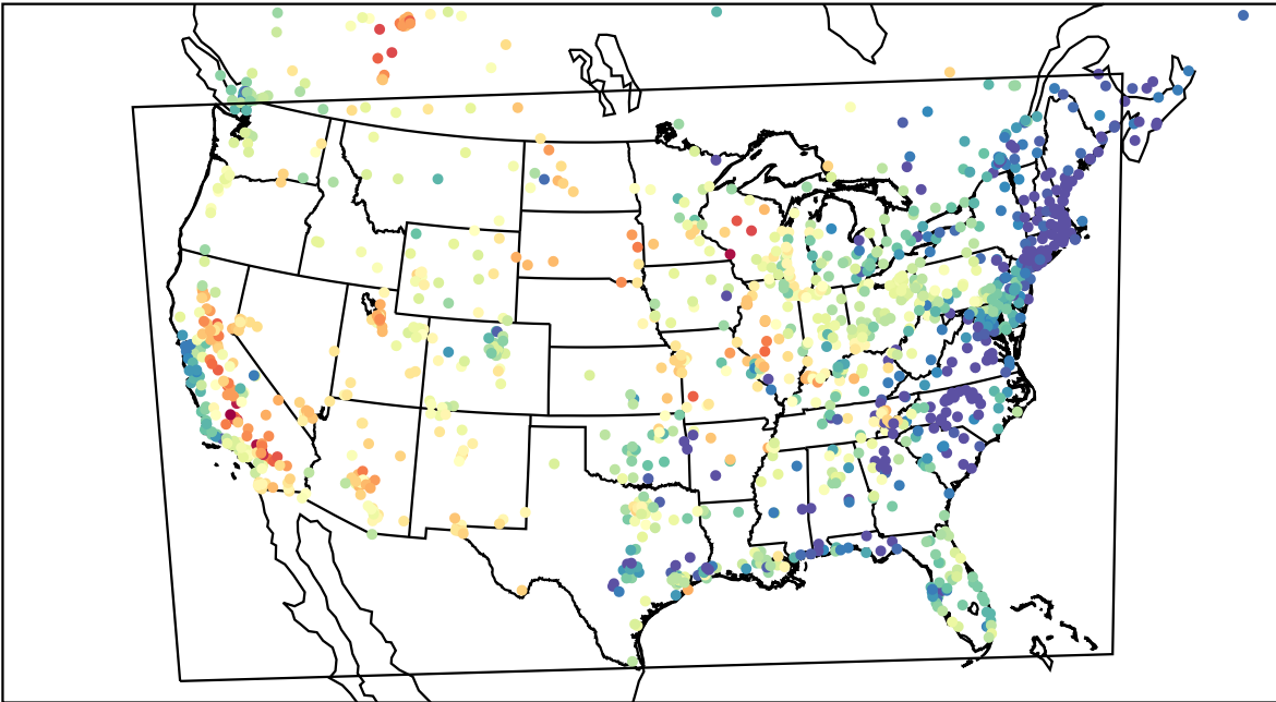
AirNOW (2023-06-05_02:00:00)
