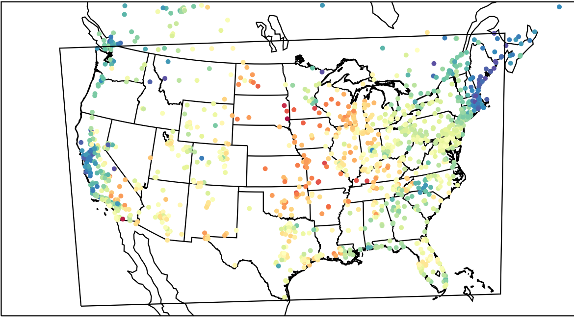
AirNOW (2023-06-05_16:00:00)
