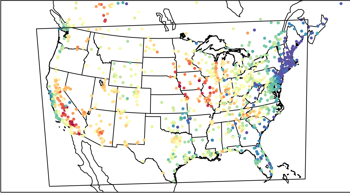
AirNOW (2023-06-04_01:00:00)
