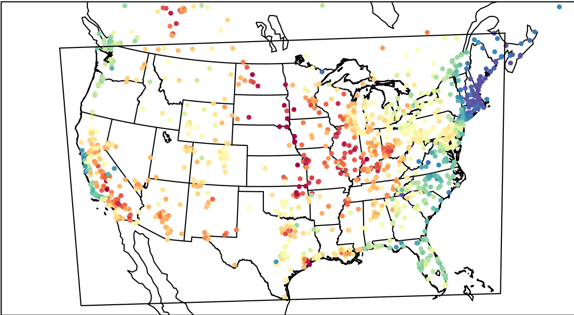
AirNOW (2023-06-04_21:00:00)
