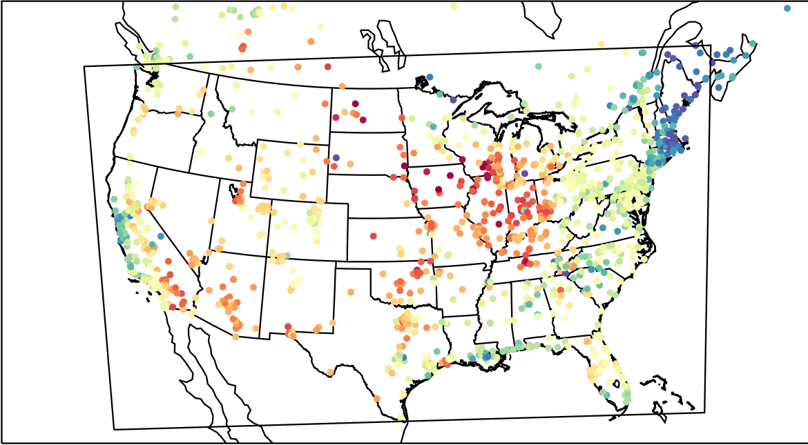
AirNOW (2023-06-05_23:00:00)
