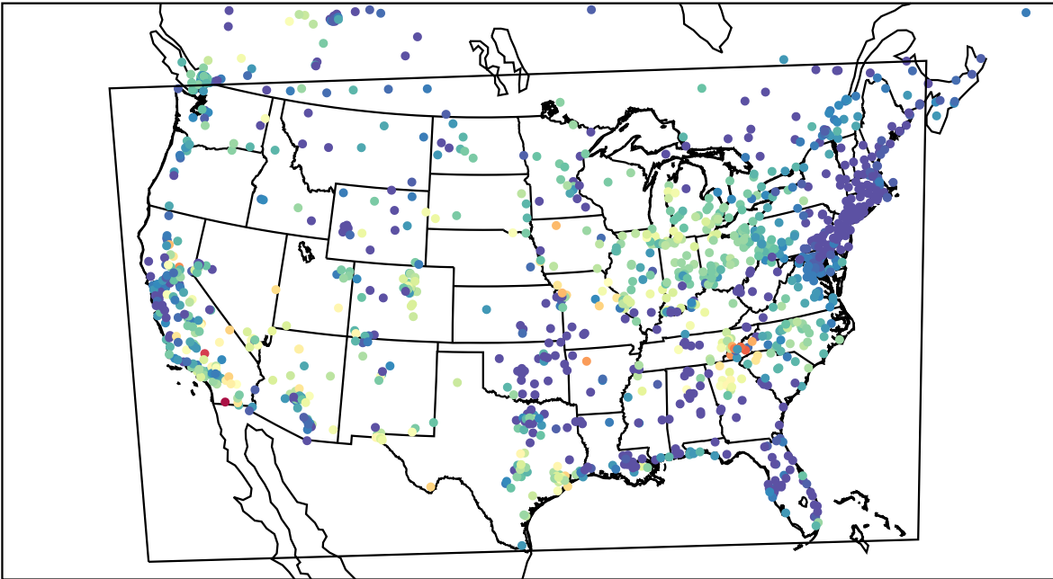
AirNOW (2023-06-04_09:00:00)
