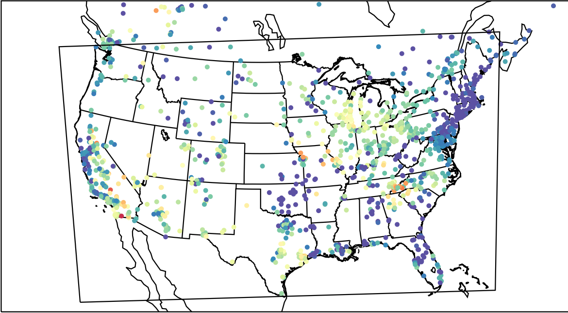
AirNOW (2023-06-04_07:00:00)
