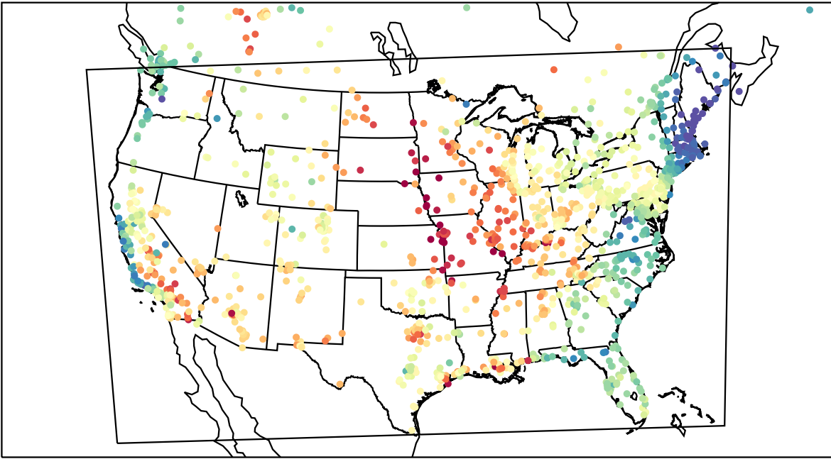
AirNOW (2023-06-04_18:00:00)
