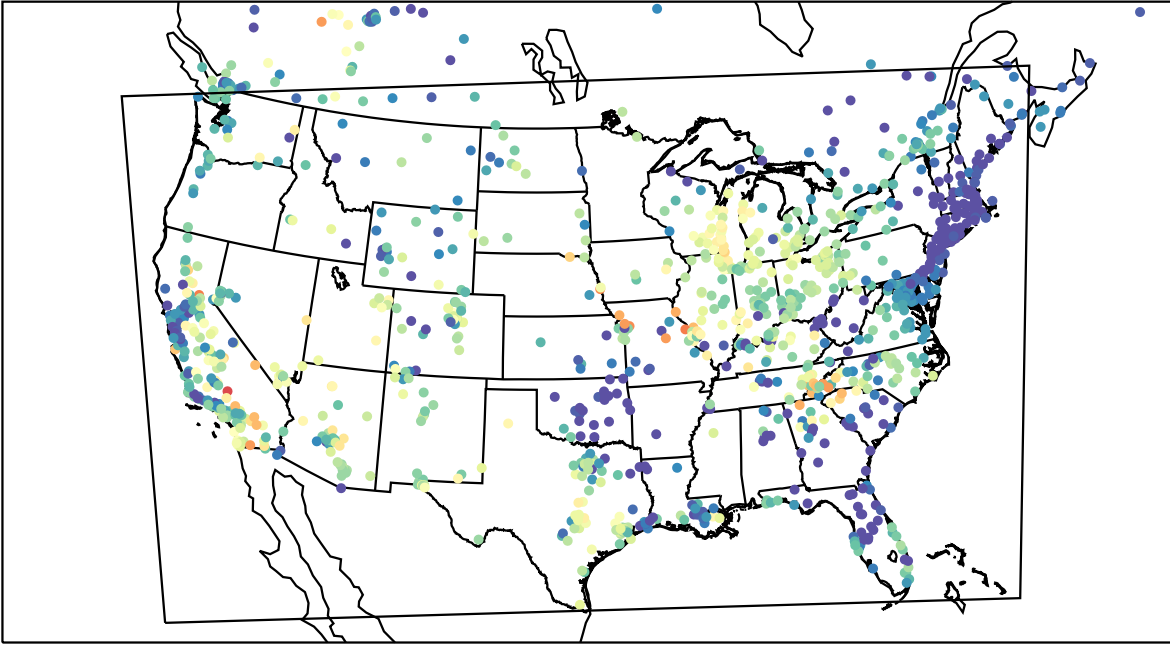
AirNOW (2023-06-04_06:00:00)
