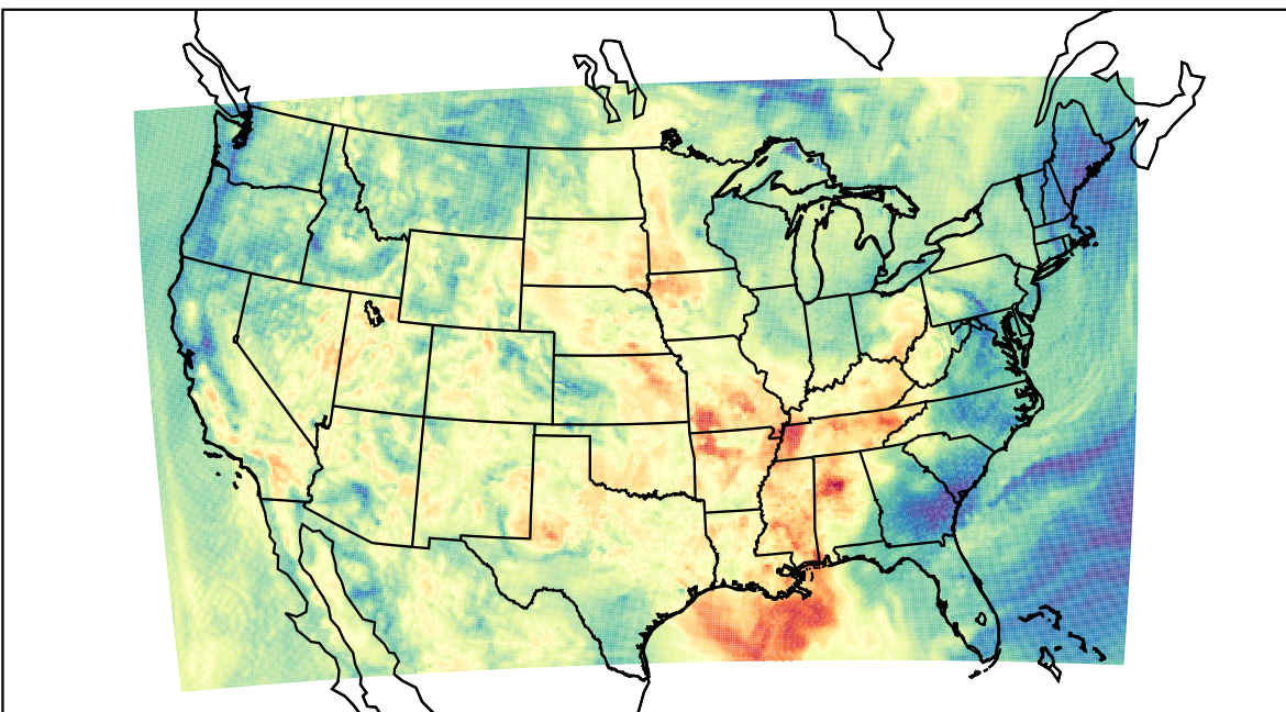
WRF (2023-06-04_15:00:00)
