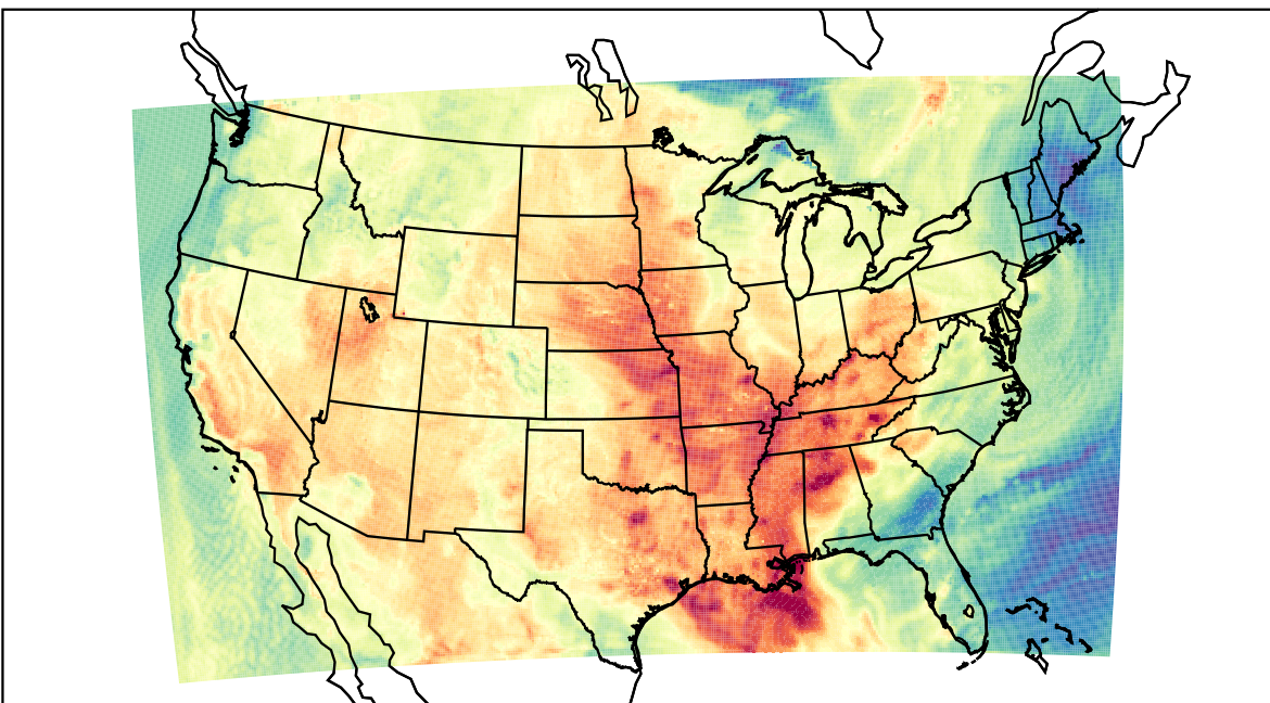
WRF (2023-06-04_18:00:00)
