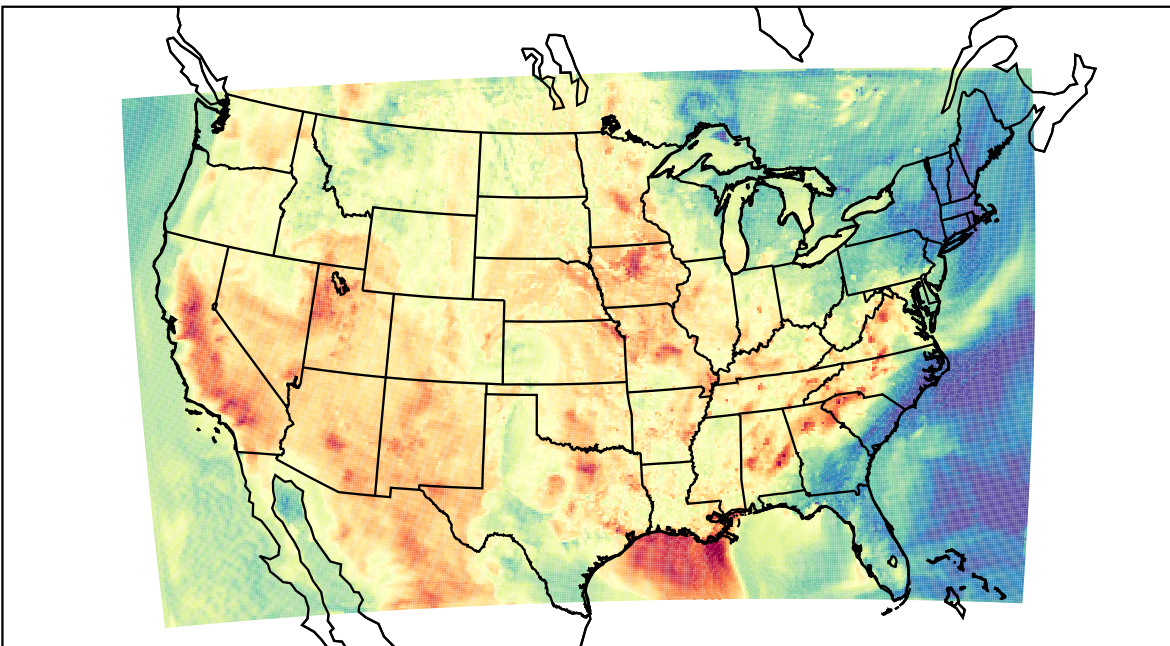
WRF (2023-06-04_00:00:00)
