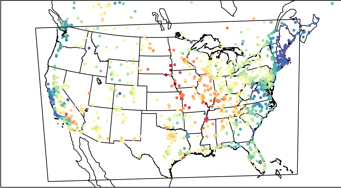
AirNOW (2023-06-04_16:00:00)
