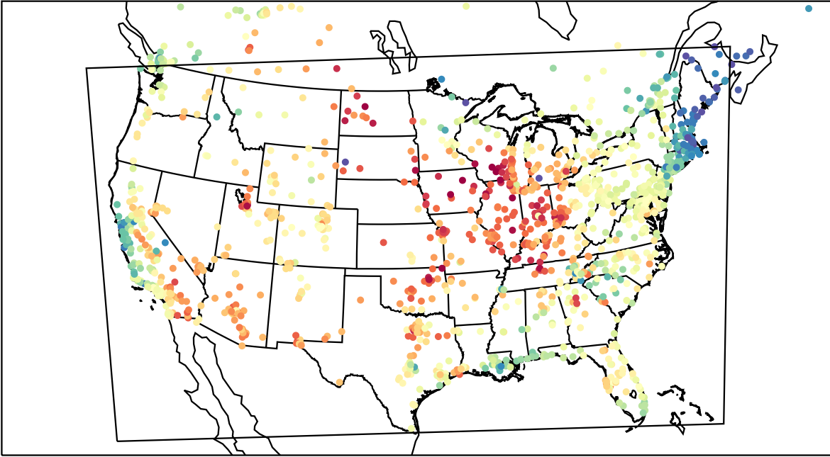
AirNOW (2023-06-05_22:00:00)
