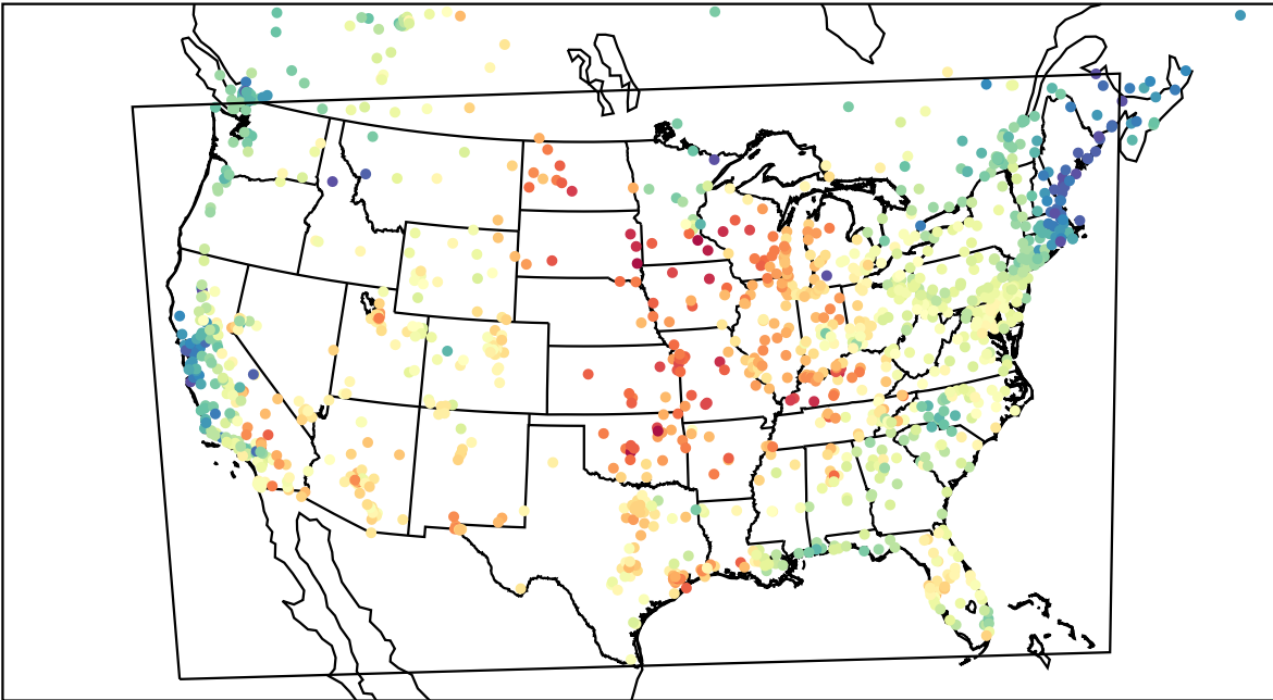
AirNOW (2023-06-05_17:00:00)
