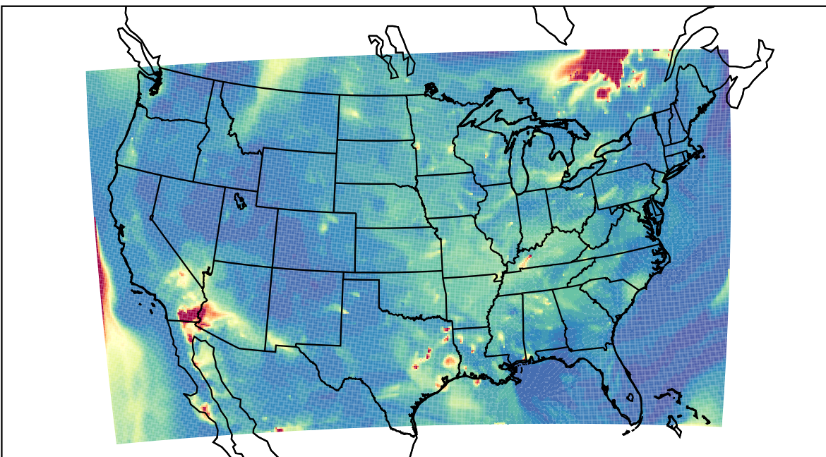
WRF 2023-06-05_07:00:00
