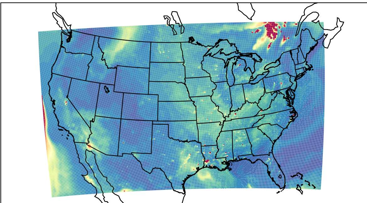
WRF 2023-06-05_00:00:00
