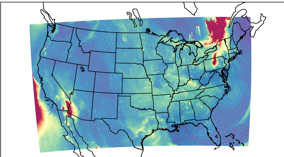
WRF 2023-06-05_23:00:00
