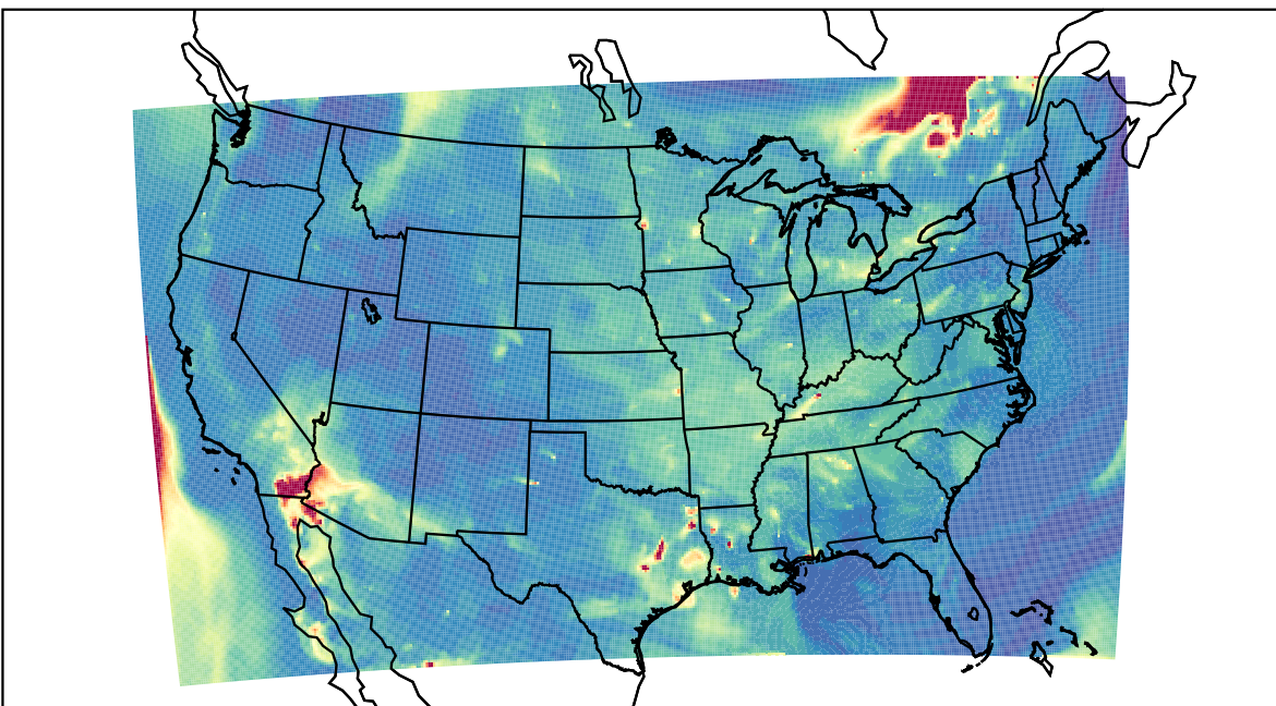
WRF 2023-06-05_09:00:00
