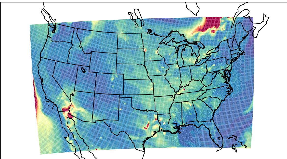
WRF 2023-06-05_11:00:00
