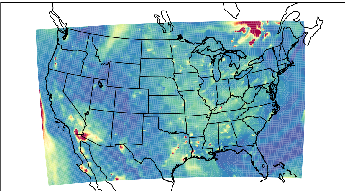
WRF 2023-06-05_03:00:00
