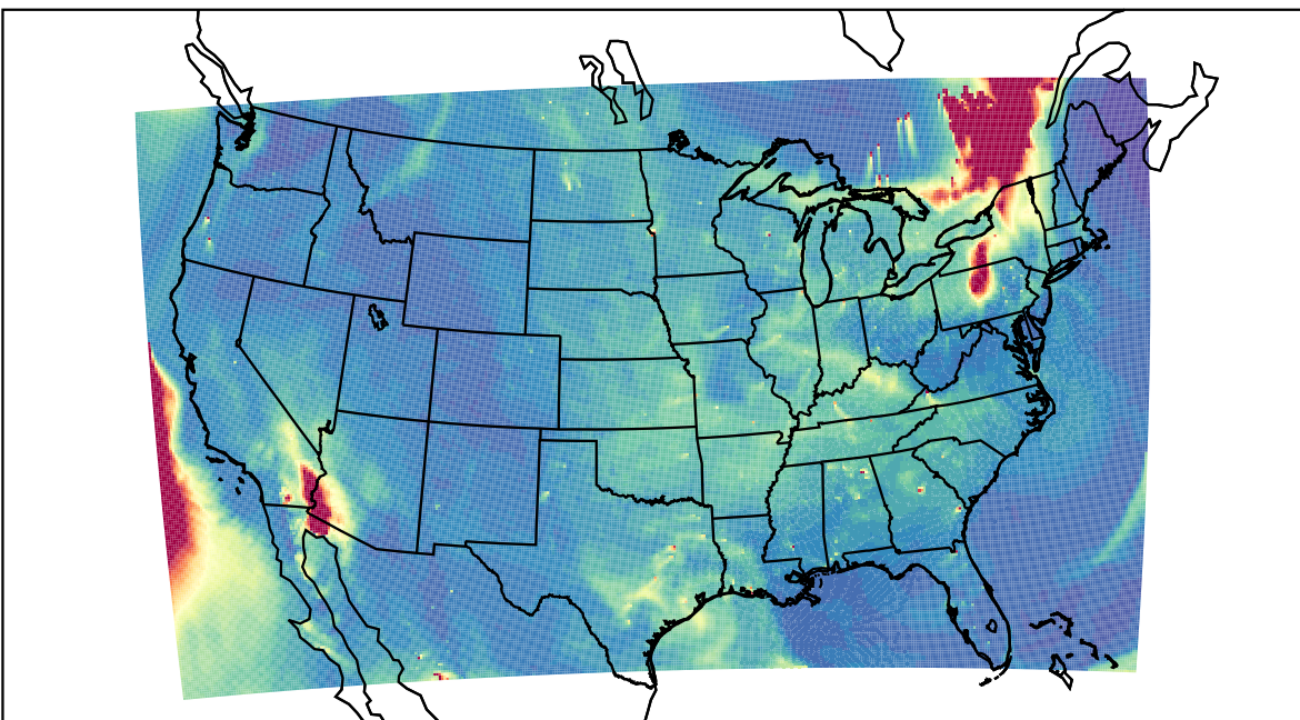
WRF 2023-06-05_22:00:00
