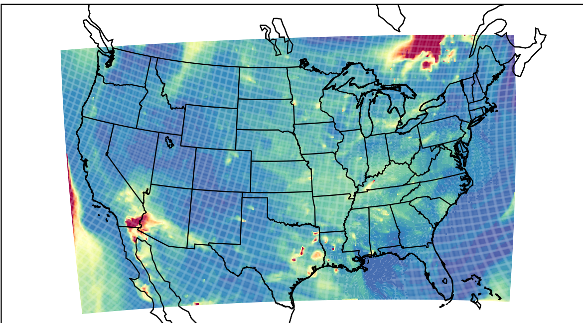
WRF 2023-06-05_08:00:00
