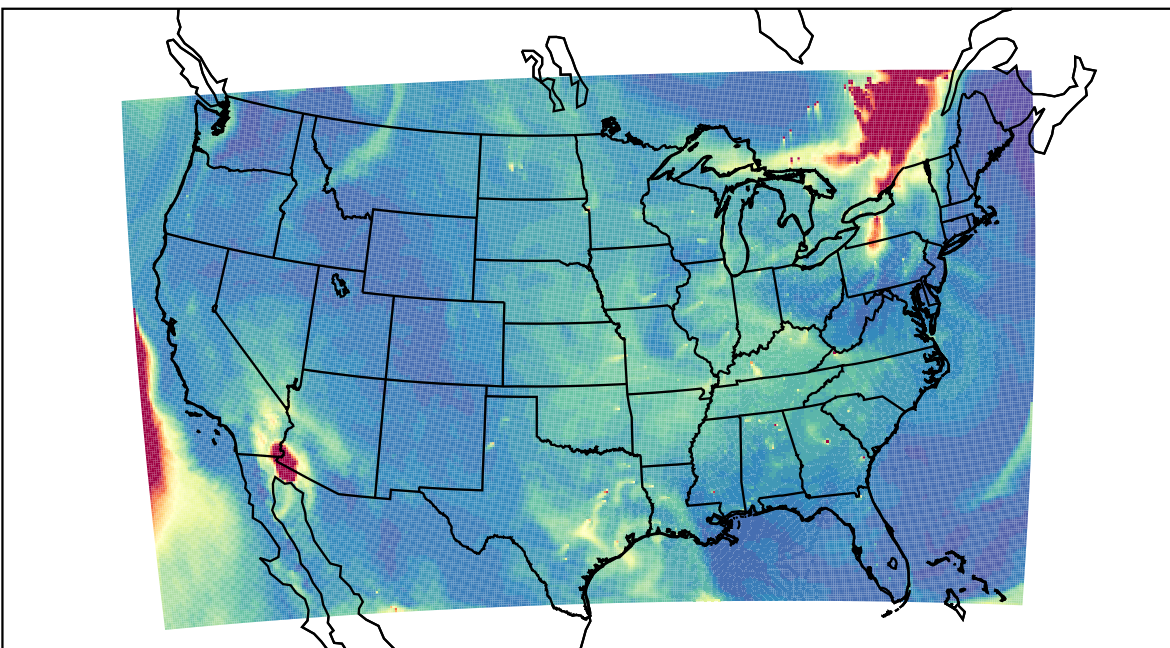
WRF 2023-06-05_19:00:00
