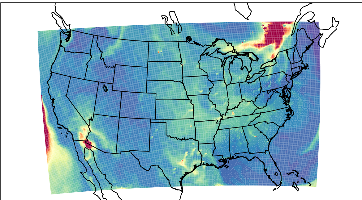
WRF 2023-06-05_17:00:00
