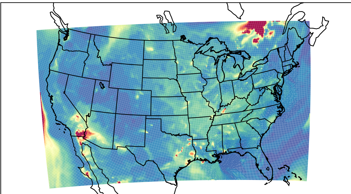
WRF 2023-06-05_06:00:00
