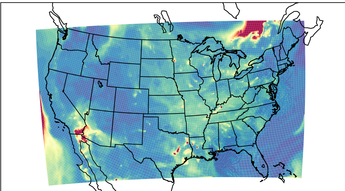
WRF 2023-06-05_10:00:00
