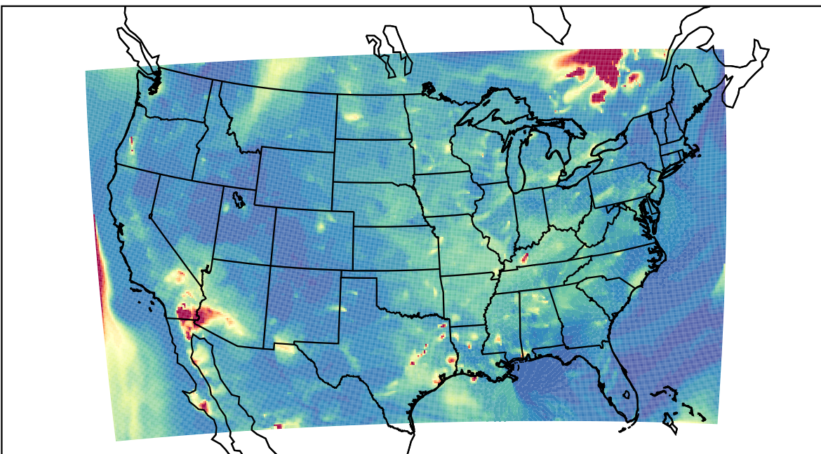
WRF 2023-06-05_05:00:00
