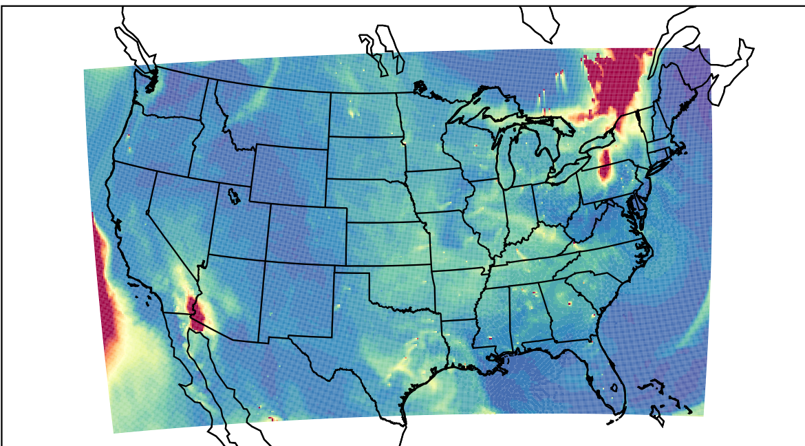
WRF 2023-06-05_21:00:00
