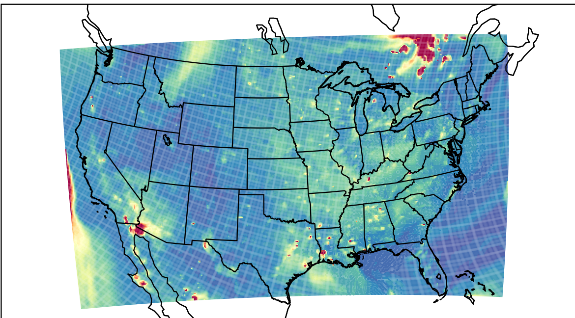
WRF 2023-06-05_02:00:00
