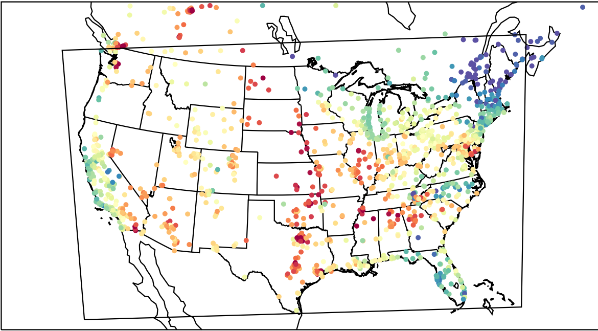
AirNOW (2023-06-07_23:00:00)
