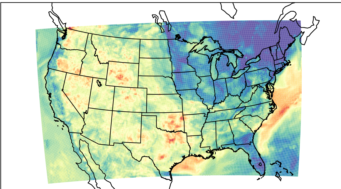
WRF (2023-06-08_07:00:00)
