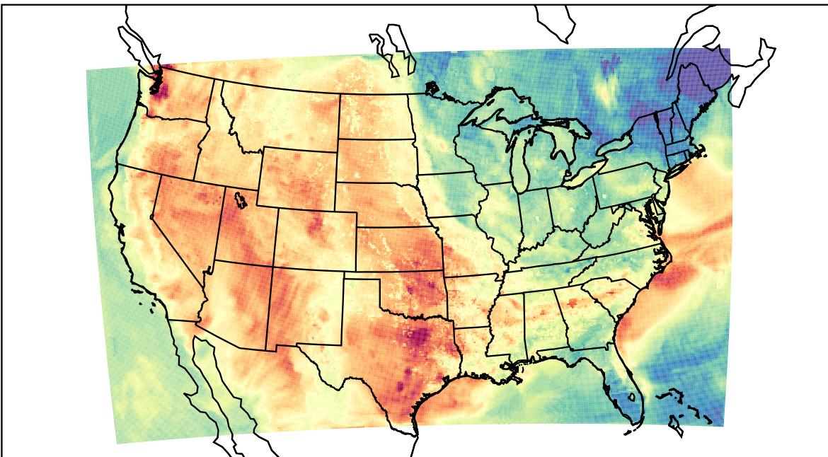
WRF (2023-06-08_00:00:00)
