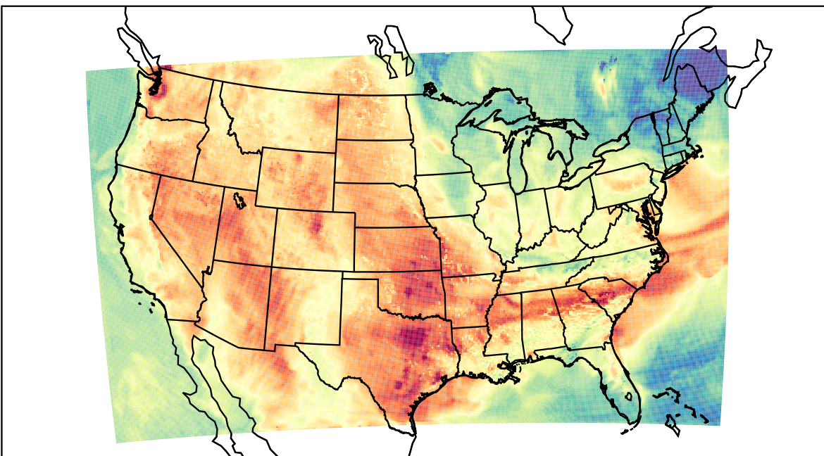
WRF (2023-06-07_22:00:00)
