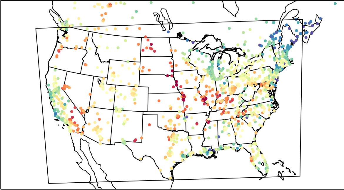
AirNOW (2023-06-07_00:00:00)
