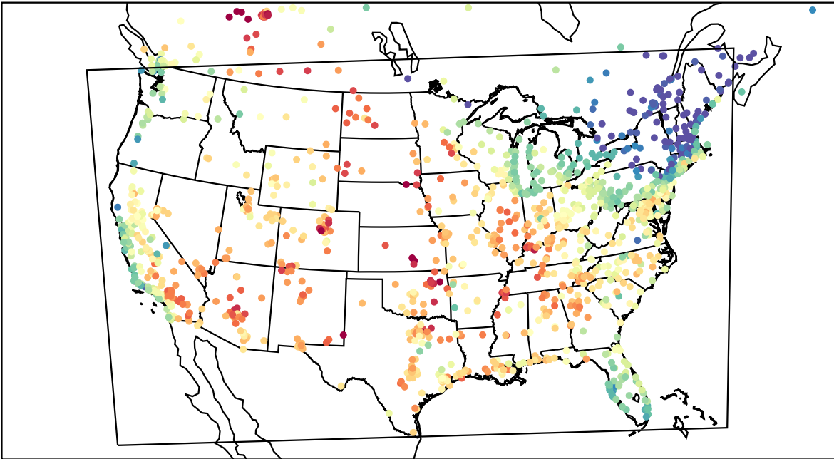
AirNOW (2023-06-08_23:00:00)
