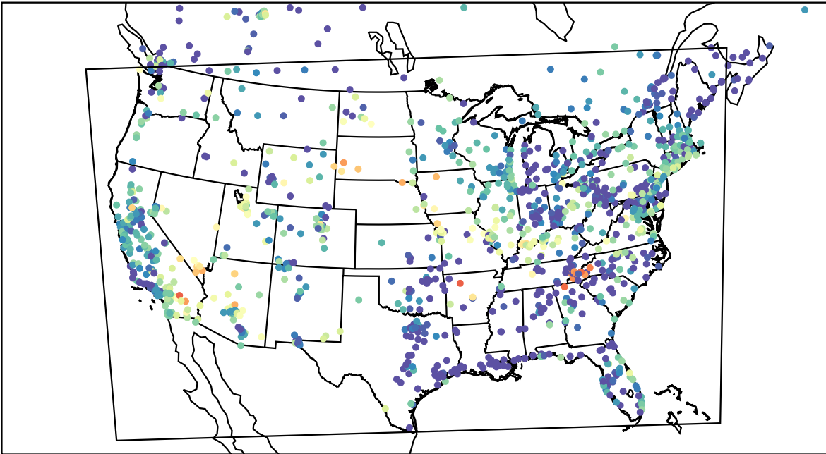
AirNOW (2023-06-07_09:00:00)
