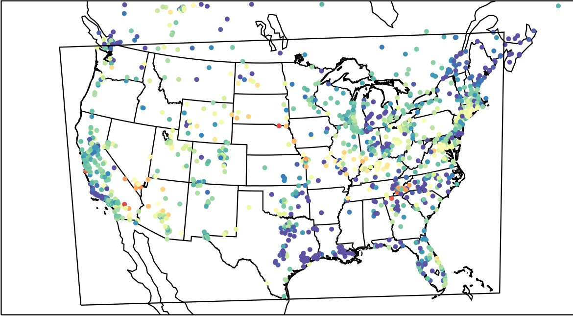
AirNOW (2023-06-07_06:00:00)
