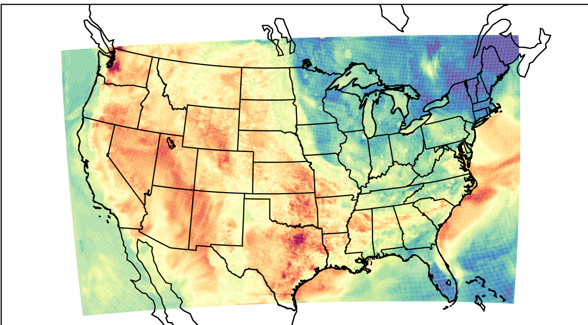
WRF (2023-06-08_01:00:00)
