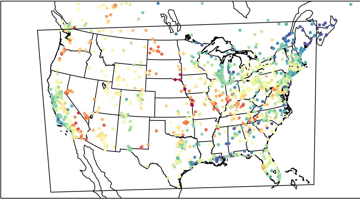
AirNOW (2023-06-07_01:00:00)
