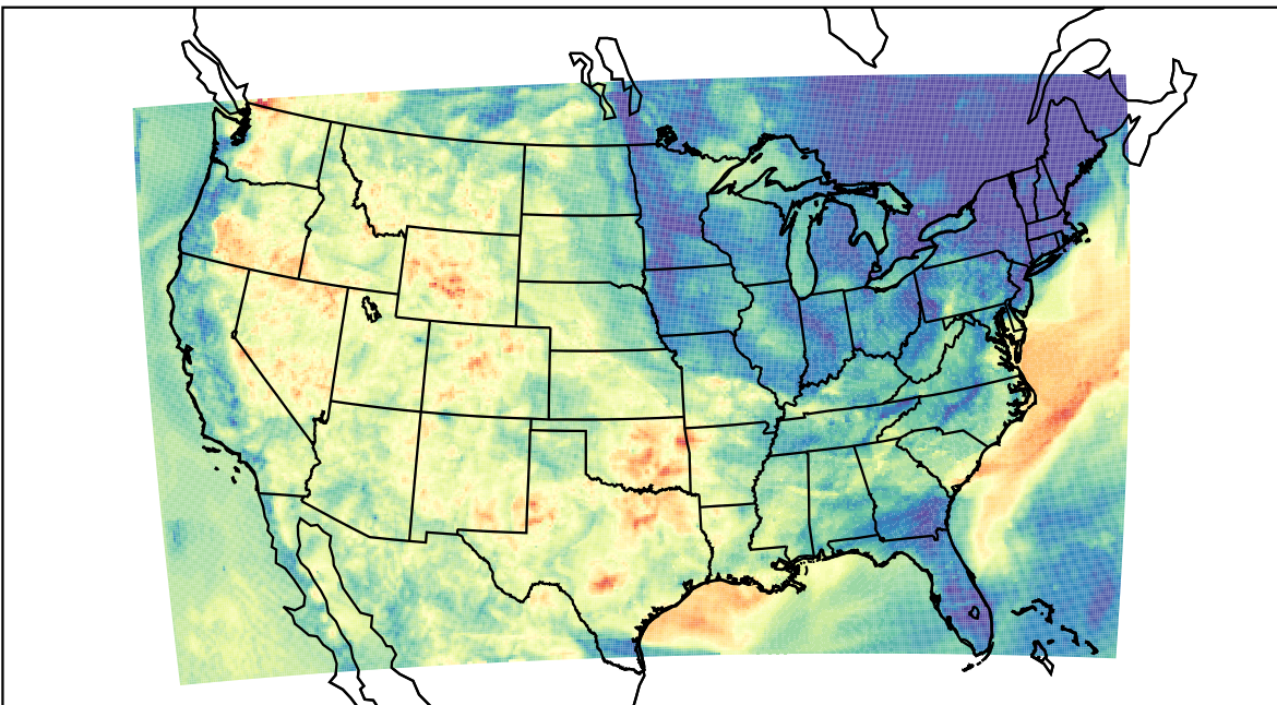
WRF (2023-06-08_08:00:00)
