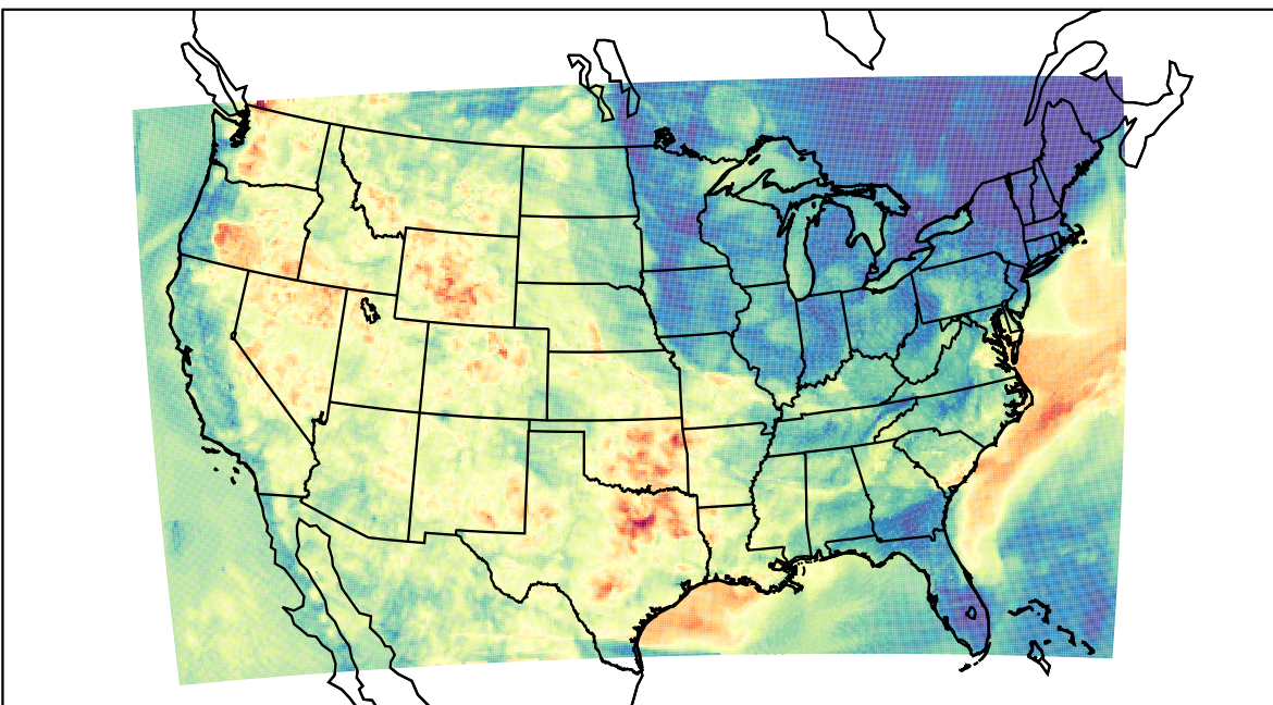
WRF (2023-06-08_06:00:00)
