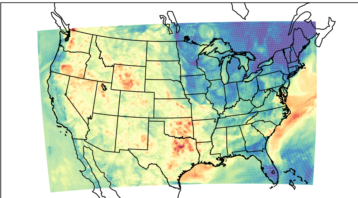
WRF (2023-06-08_05:00:00)
