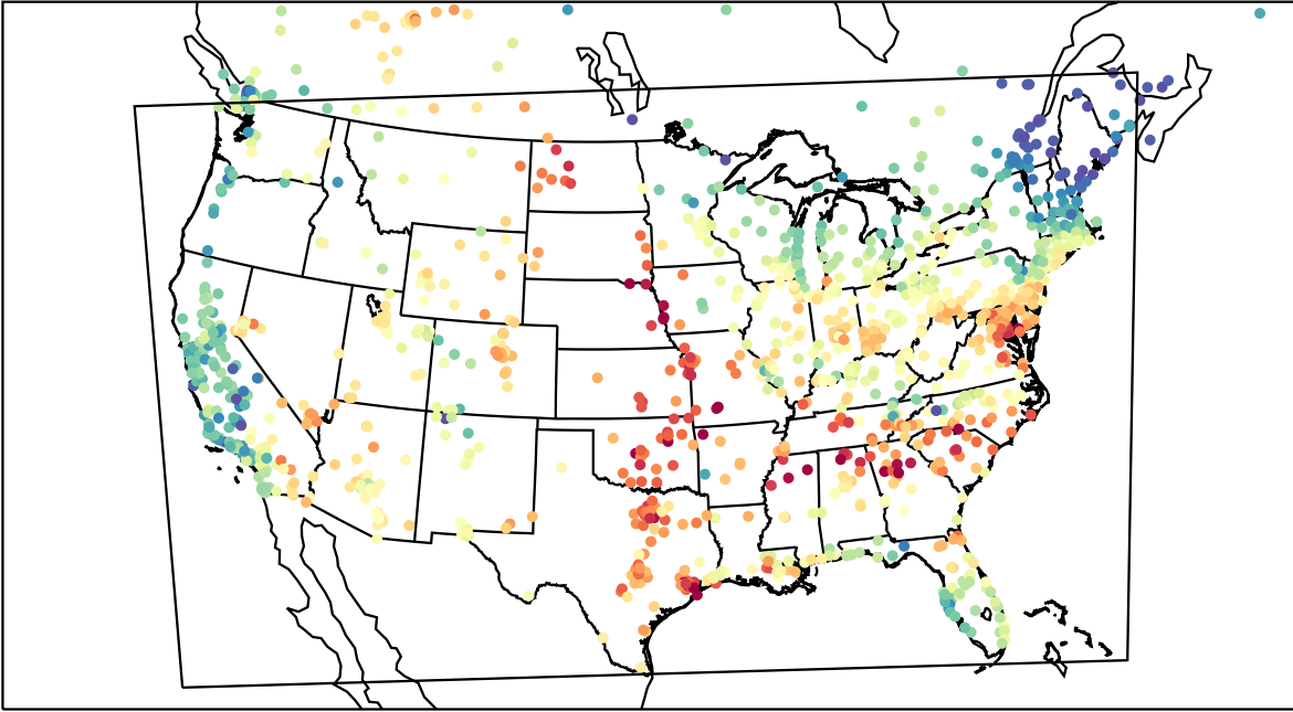
AirNOW (2023-06-07_17:00:00)
