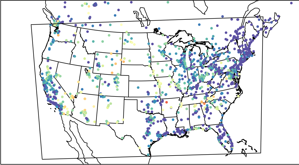
AirNOW (2023-06-08_08:00:00)
