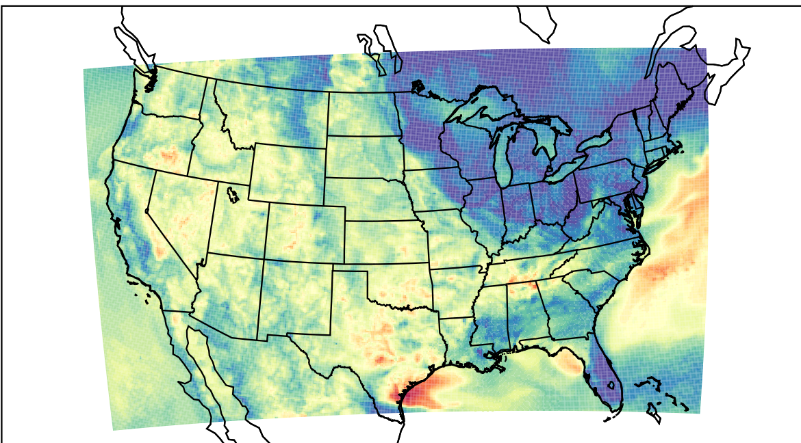
WRF (2023-06-07_11:00:00)
