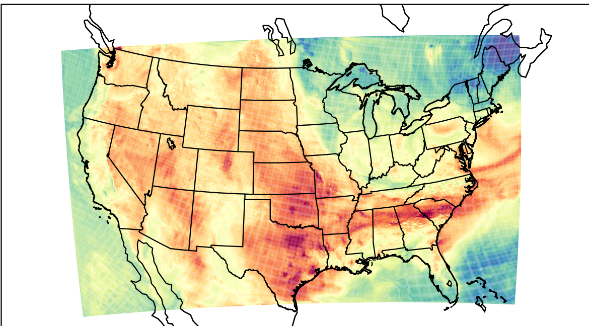
WRF (2023-06-07_20:00:00)
