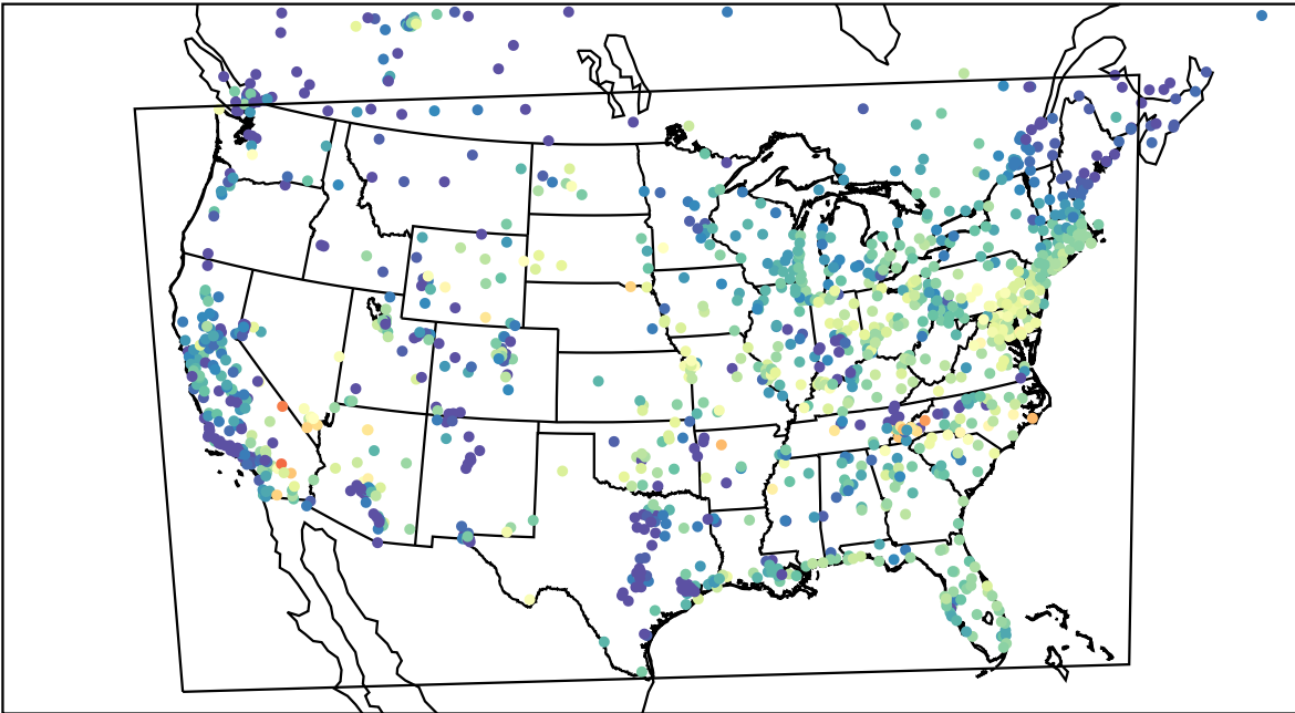
AirNOW (2023-06-07_13:00:00)
