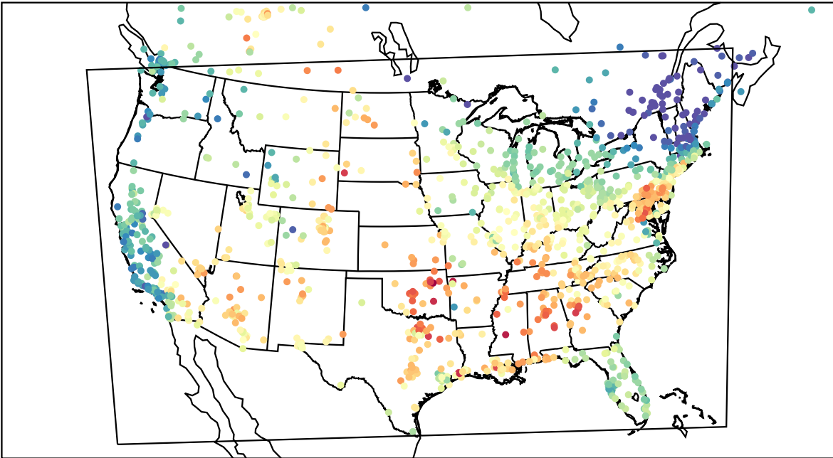
AirNOW (2023-06-08_16:00:00)
