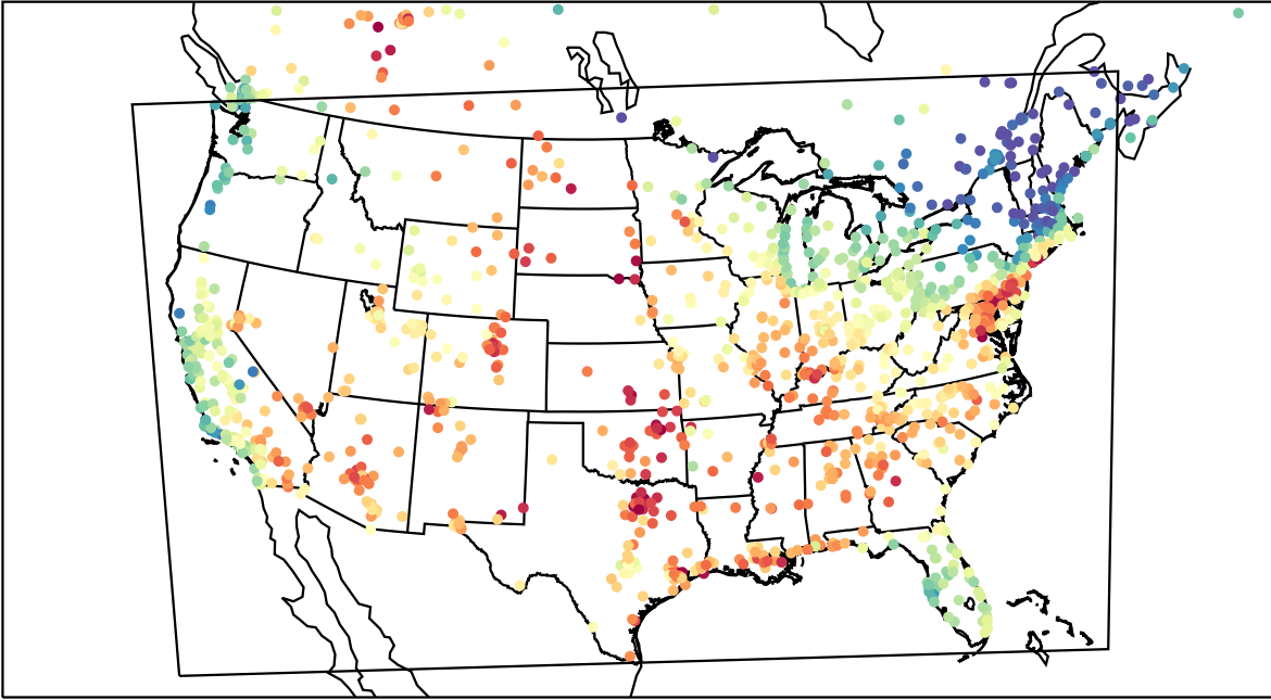
AirNOW (2023-06-08_19:00:00)
