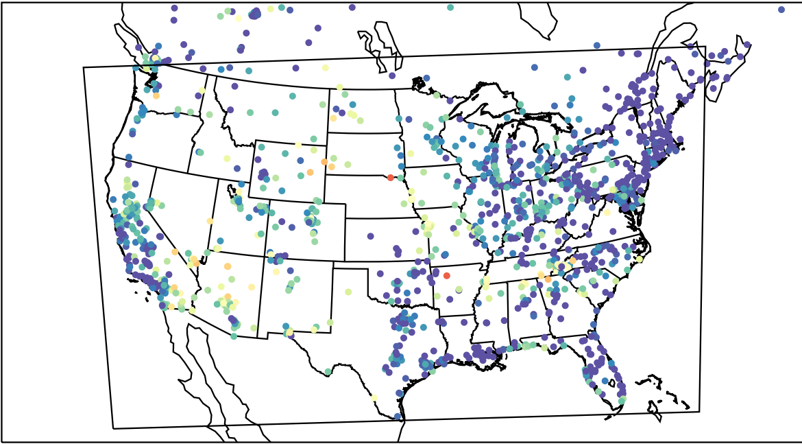
AirNOW (2023-06-08_09:00:00)
