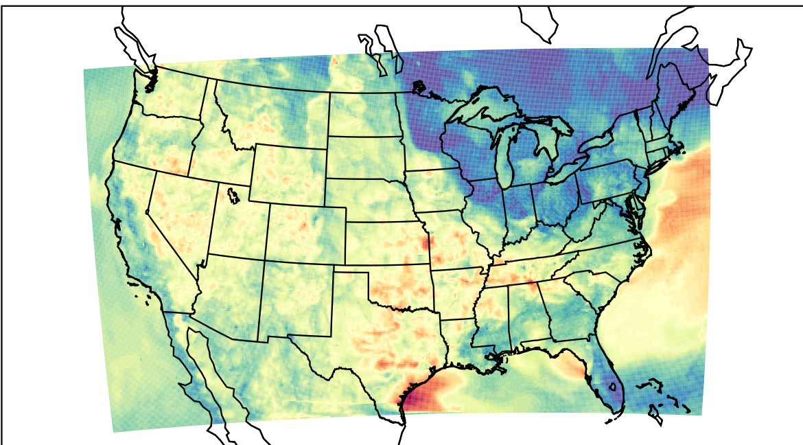
WRF (2023-06-07_06:00:00)
