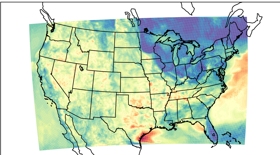
WRF (2023-06-07_08:00:00)
