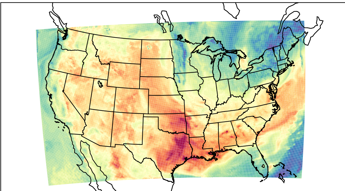
WRF (2023-06-08_17:00:00)
