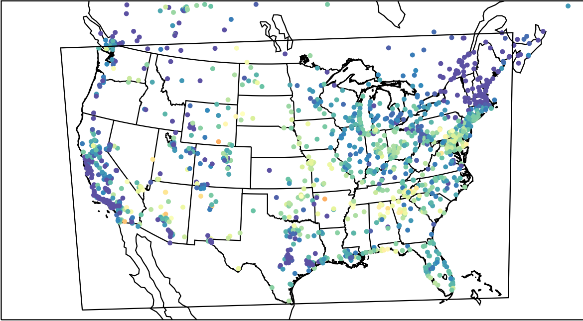
AirNOW (2023-06-08_13:00:00)
