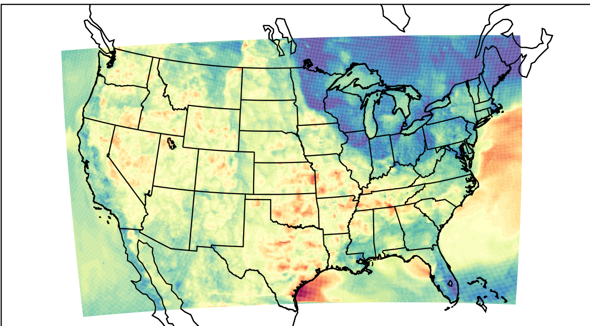
WRF (2023-06-07_05:00:00)
