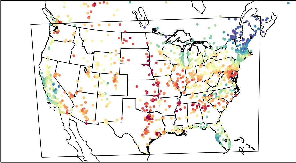
AirNOW (2023-06-07_21:00:00)
