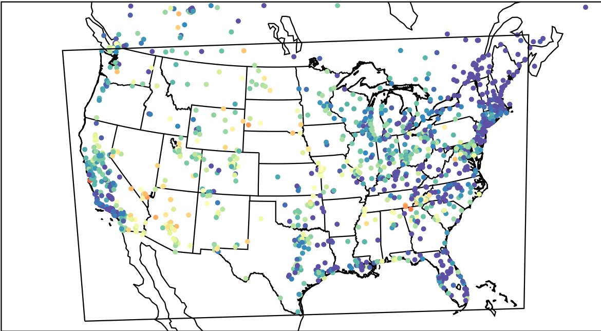
AirNOW (2023-06-08_06:00:00)
