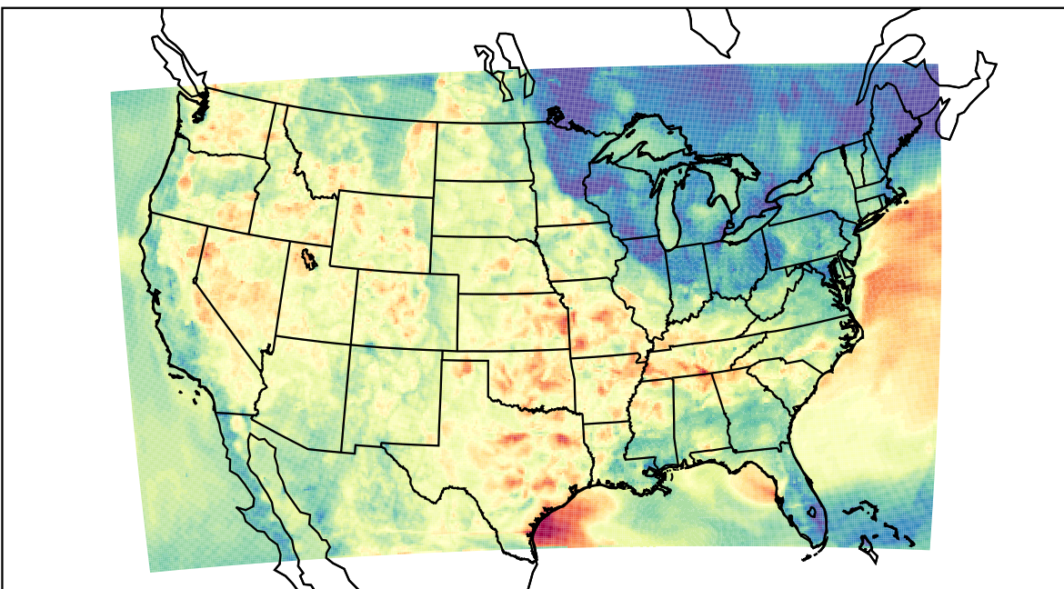
WRF (2023-06-07_04:00:00)
