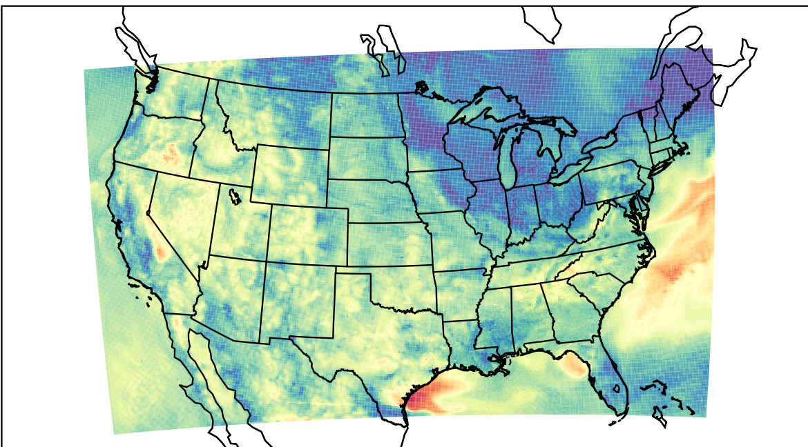
WRF (2023-06-07_13:00:00)
