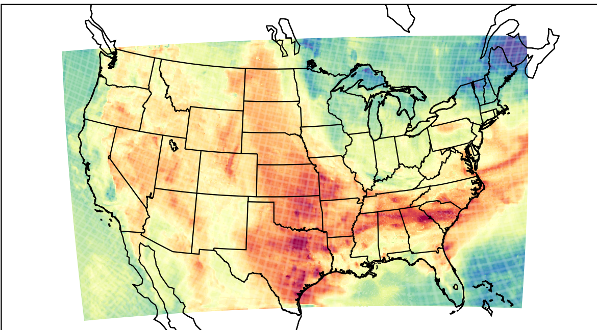
WRF (2023-06-07_18:00:00)
