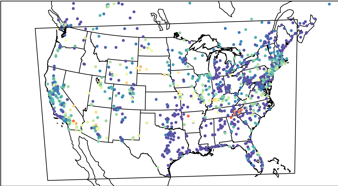
AirNOW (2023-06-07_10:00:00)
