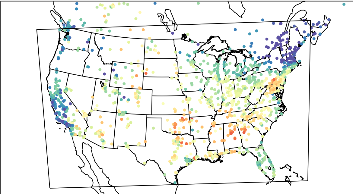
AirNOW (2023-06-08_15:00:00)
