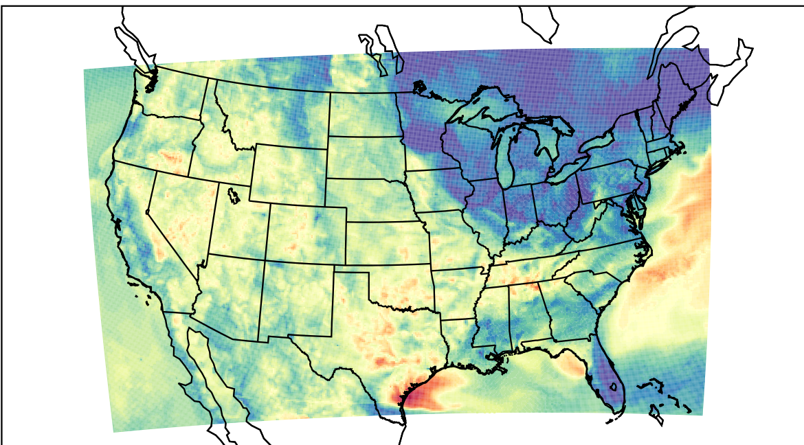
WRF (2023-06-07_10:00:00)
