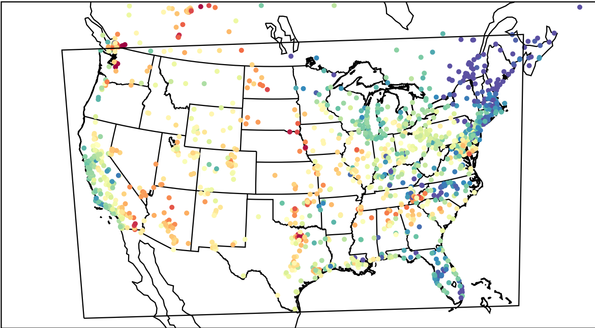
AirNOW (2023-06-08_01:00:00)
