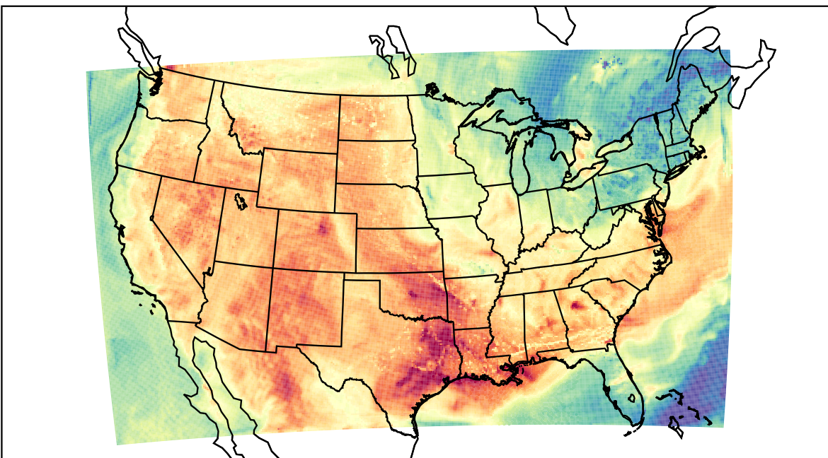
WRF (2023-06-08_21:00:00)
