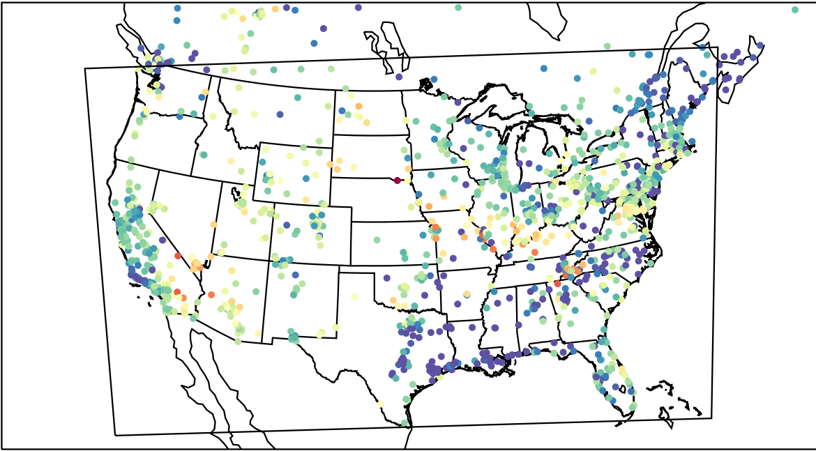
AirNOW (2023-06-07_05:00:00)
