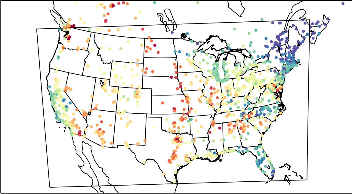
AirNOW (2023-06-08_00:00:00)
