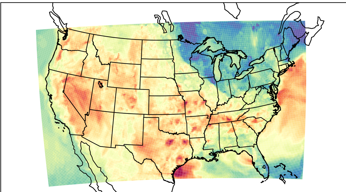
WRF (2023-06-07_01:00:00)
