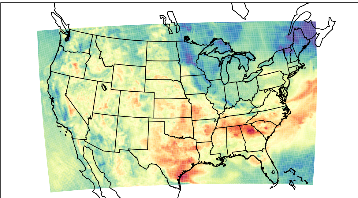
WRF (2023-06-07_15:00:00)
