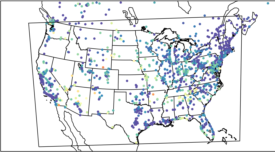
AirNOW (2023-06-08_12:00:00)
