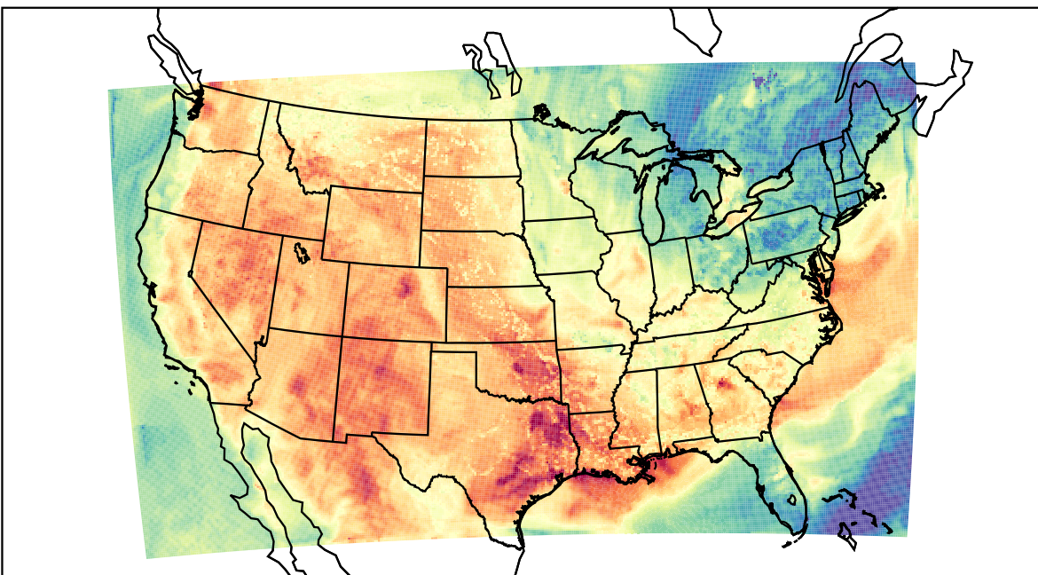
WRF (2023-06-08_23:00:00)
