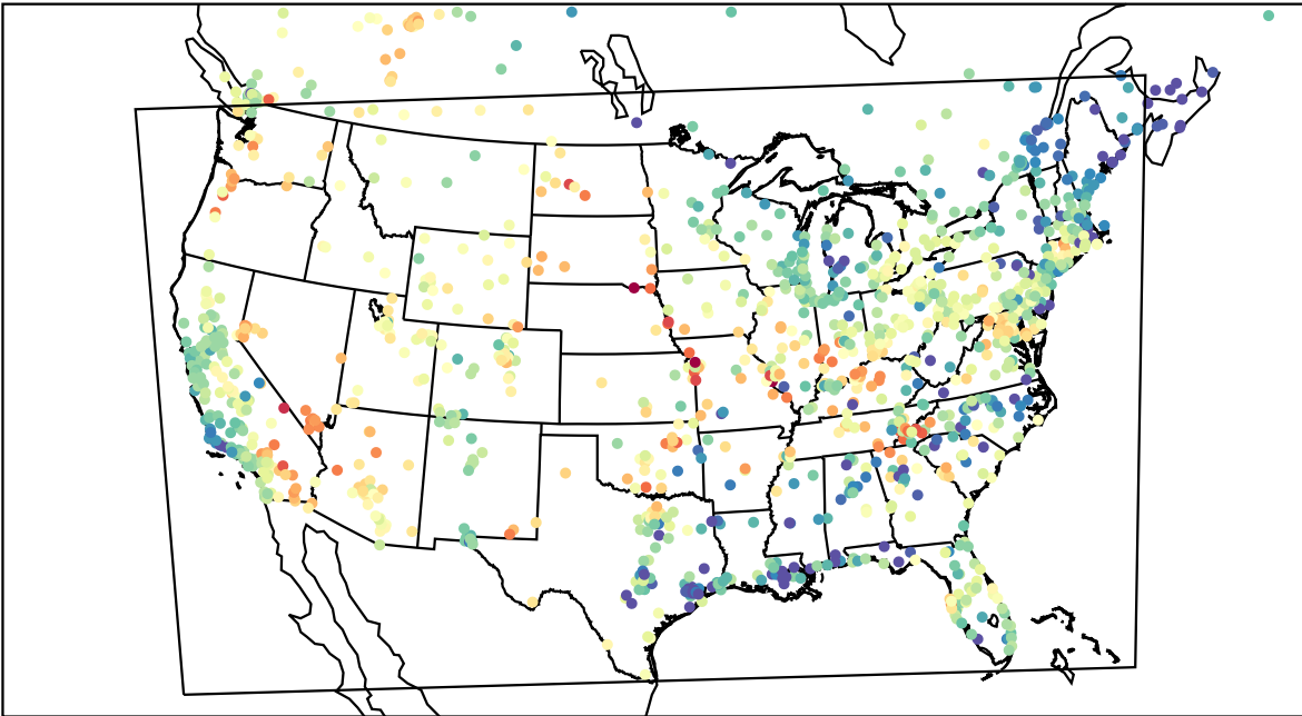
AirNOW (2023-06-07_02:00:00)
