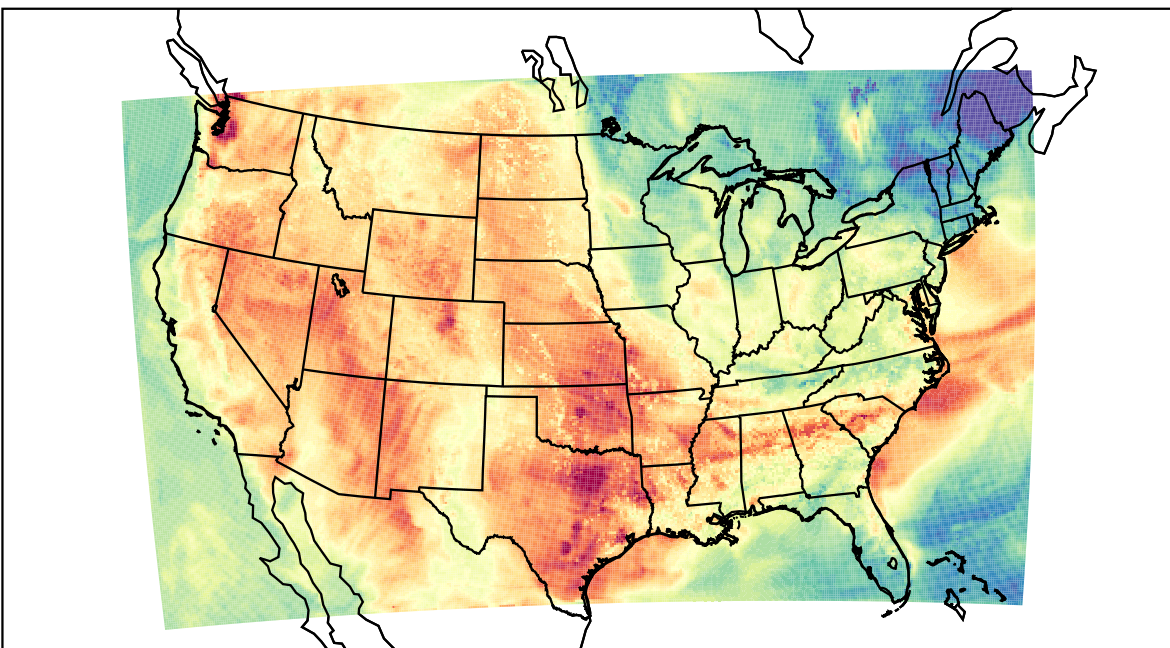
WRF (2023-06-07_23:00:00)
