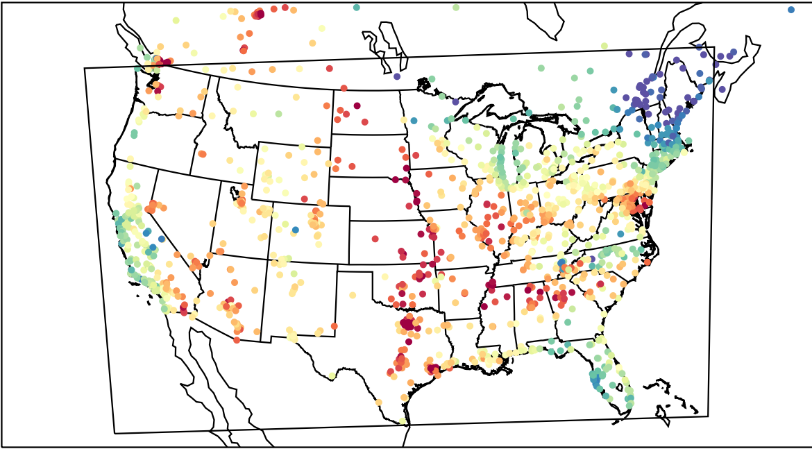
AirNOW (2023-06-07_22:00:00)
