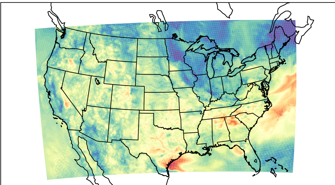
WRF (2023-06-07_14:00:00)
