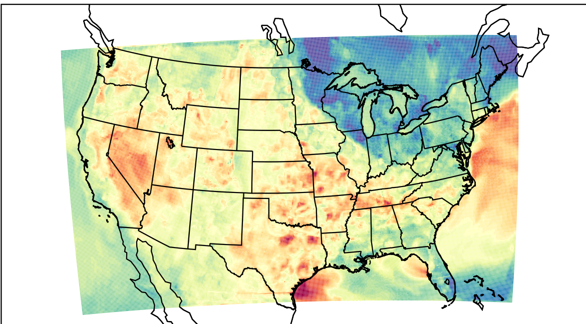
WRF (2023-06-07_02:00:00)
