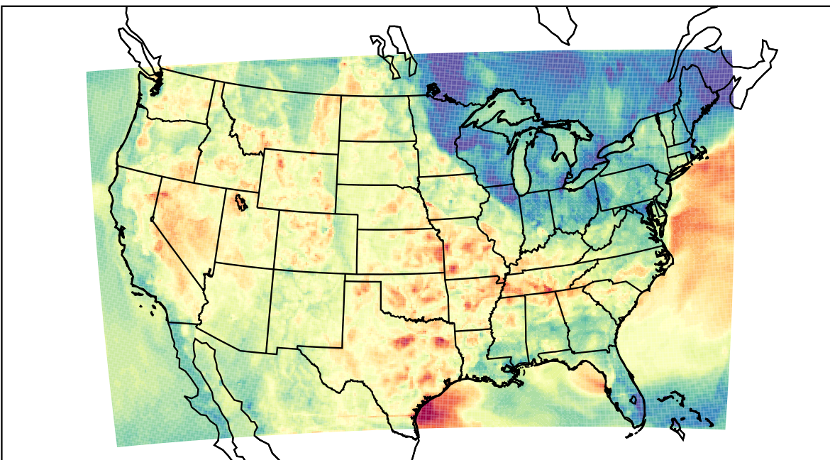
WRF (2023-06-07_03:00:00)
