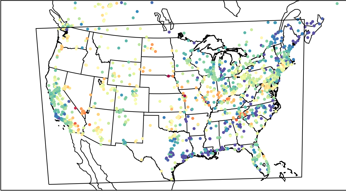
AirNOW (2023-06-07_03:00:00)
