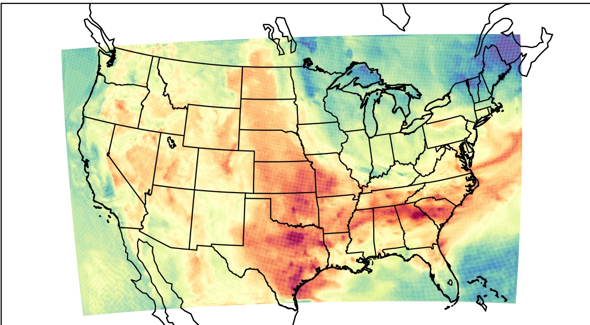
WRF (2023-06-07_17:00:00)
