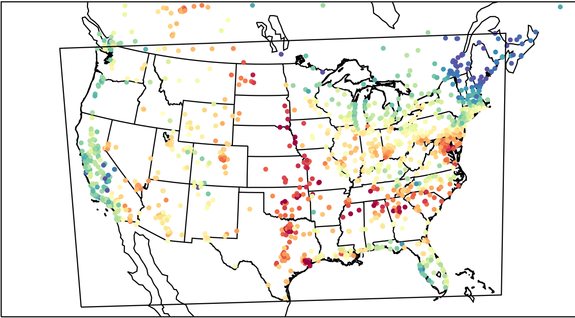
AirNOW (2023-06-07_18:00:00)
