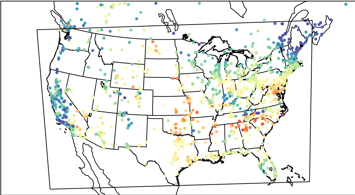
AirNOW (2023-06-07_15:00:00)
