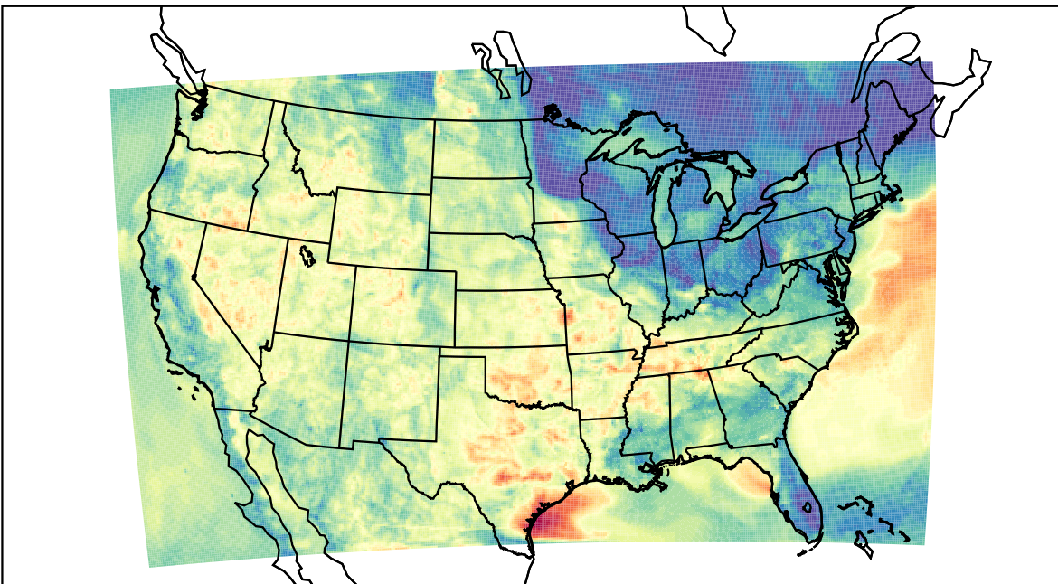
WRF (2023-06-07_07:00:00)
