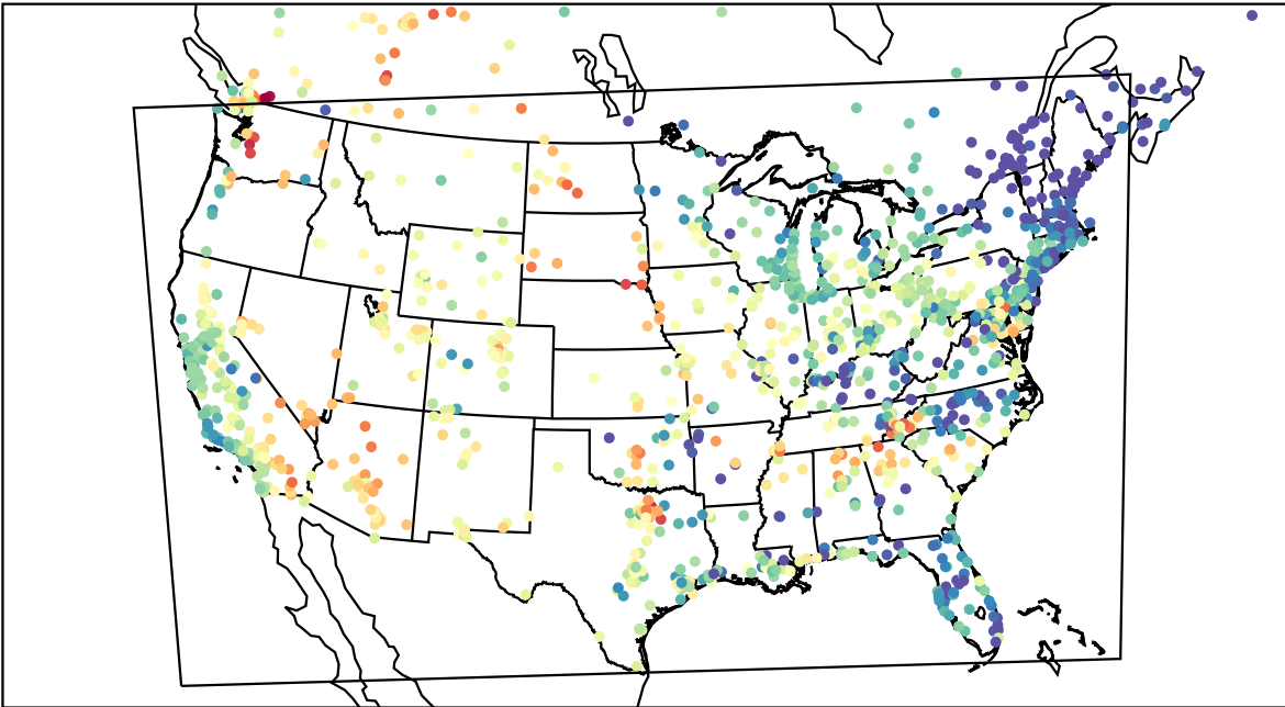
AirNOW (2023-06-08_02:00:00)
