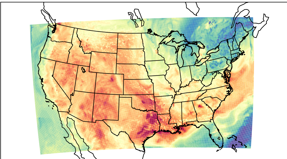
WRF (2023-06-08_22:00:00)
