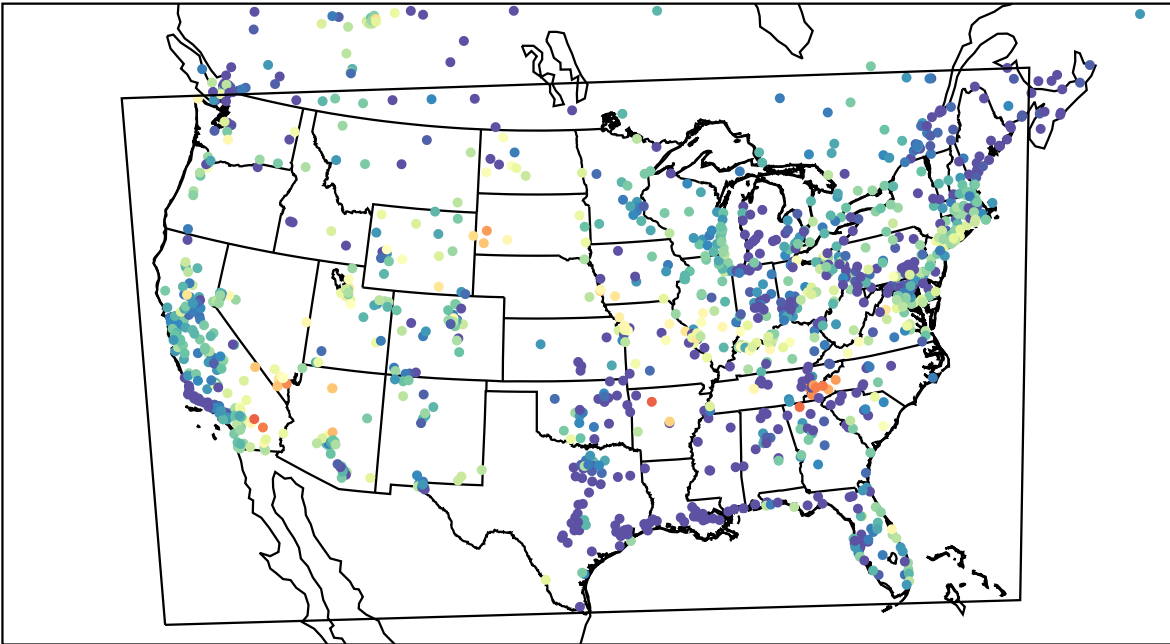
AirNOW (2023-06-07_08:00:00)
