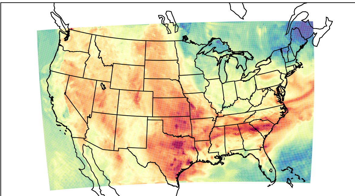
WRF (2023-06-07_19:00:00)
