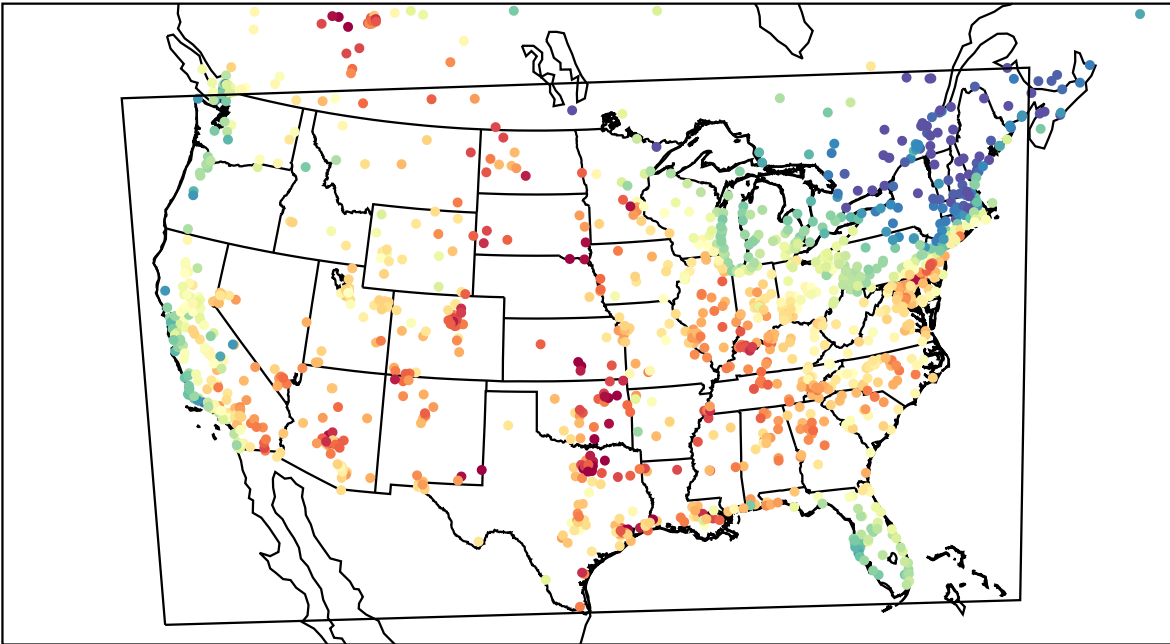
AirNOW (2023-06-08_21:00:00)
