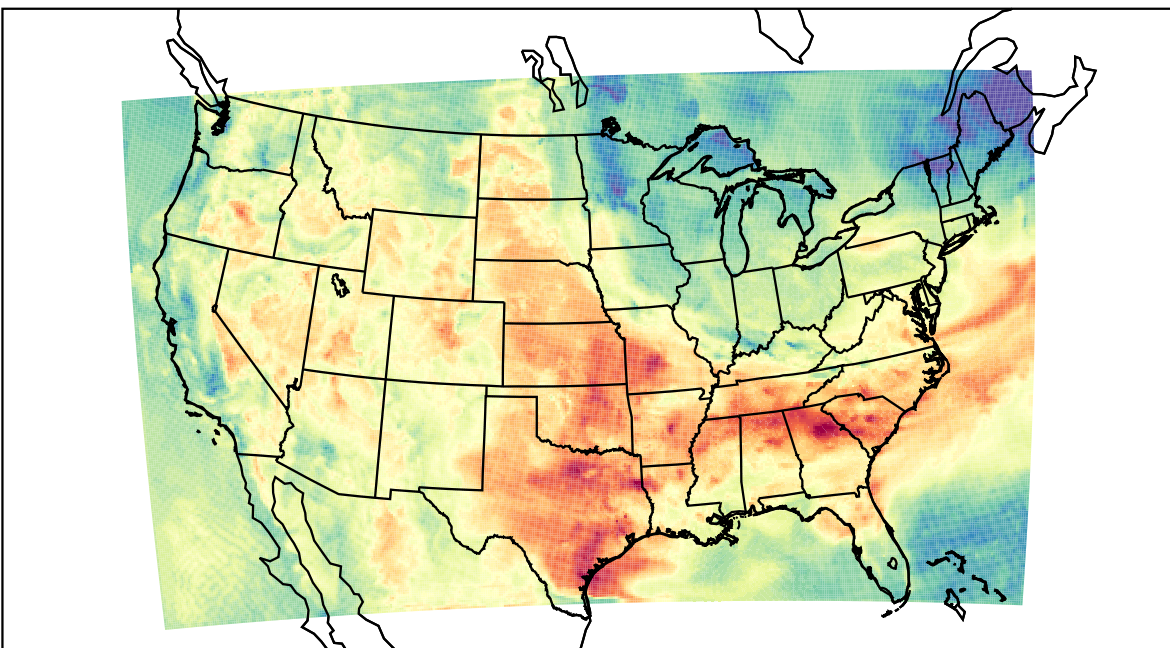
WRF (2023-06-07_16:00:00)
