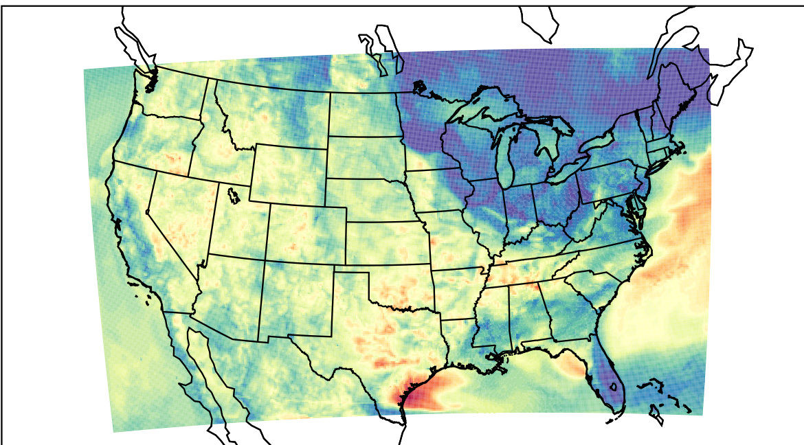
WRF (2023-06-07_09:00:00)
