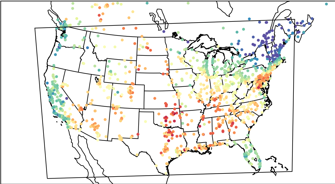
AirNOW (2023-06-08_17:00:00)
