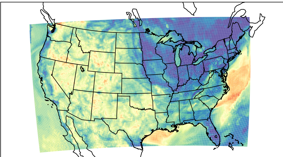
WRF (2023-06-08_12:00:00)
