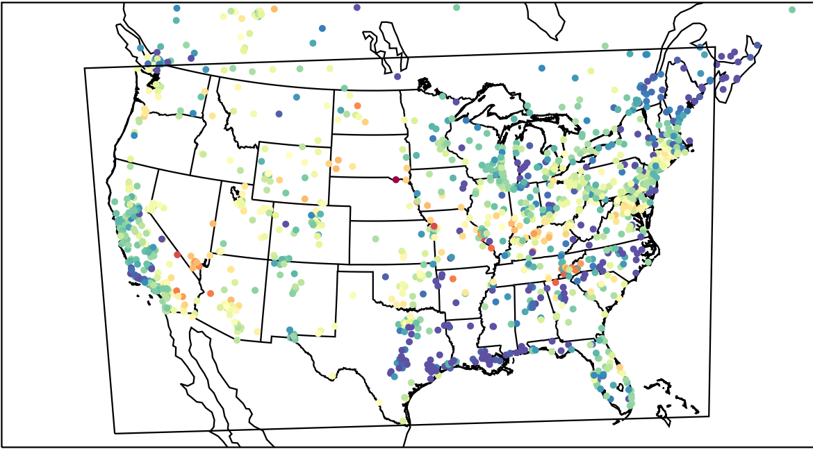
AirNOW (2023-06-07_04:00:00)
