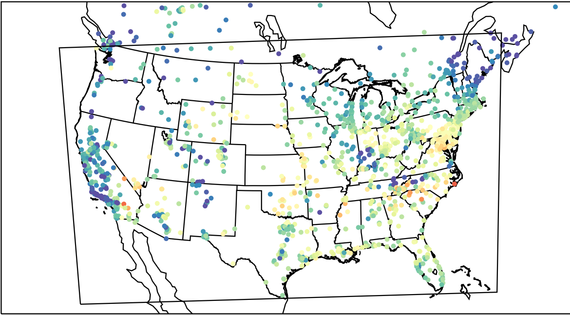
AirNOW (2023-06-07_14:00:00)
