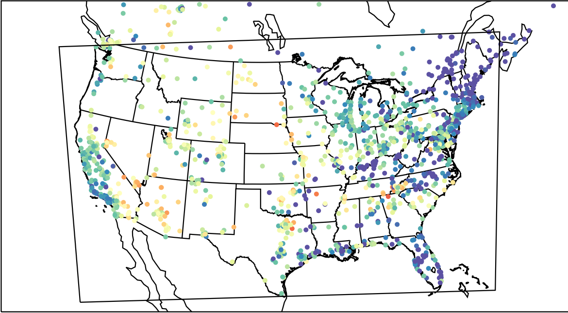
AirNOW (2023-06-08_04:00:00)
