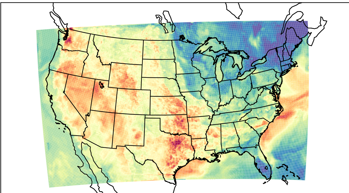
WRF (2023-06-08_02:00:00)
