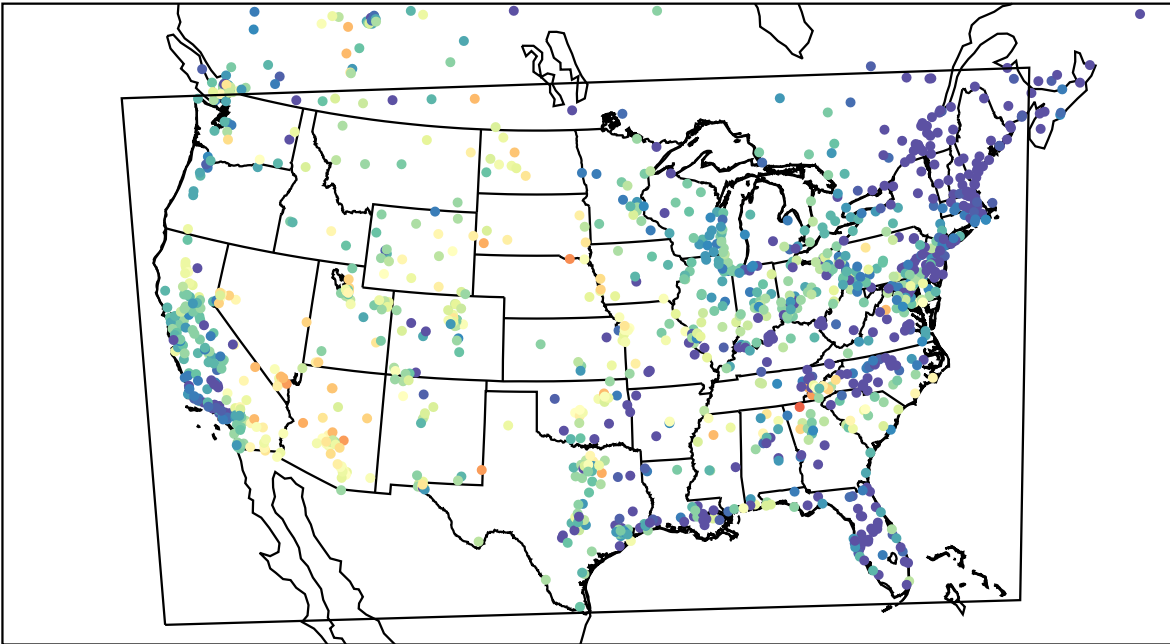
AirNOW (2023-06-08_05:00:00)
