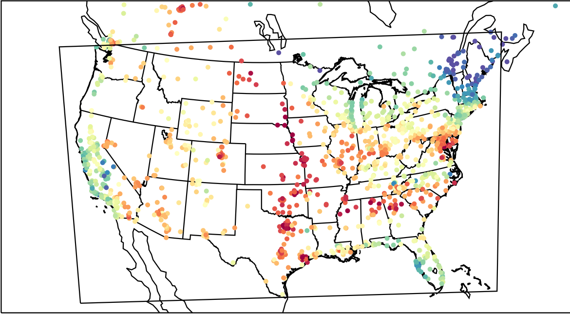
AirNOW (2023-06-07_20:00:00)
