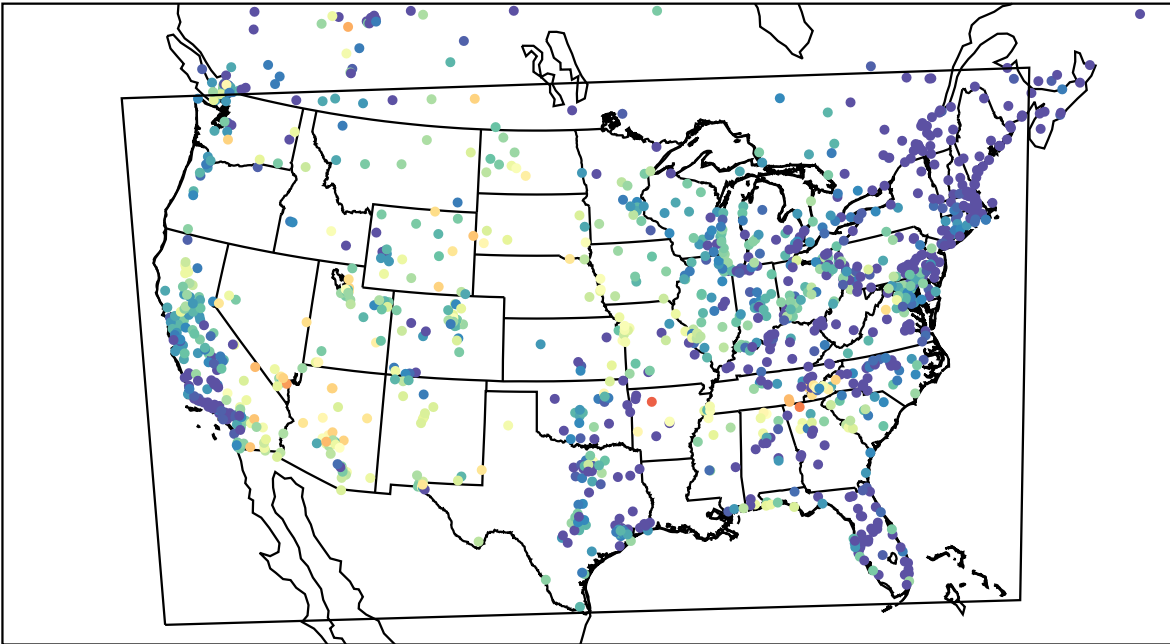
AirNOW (2023-06-08_07:00:00)
