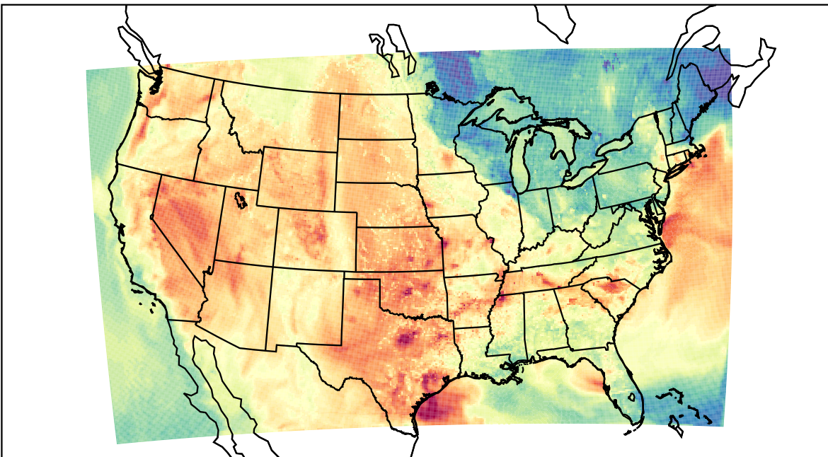
WRF (2023-06-07_00:00:00)
