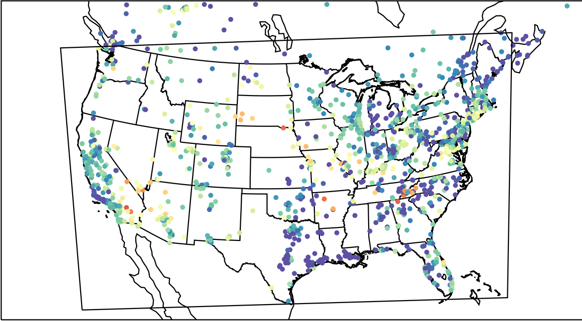
AirNOW (2023-06-07_07:00:00)
