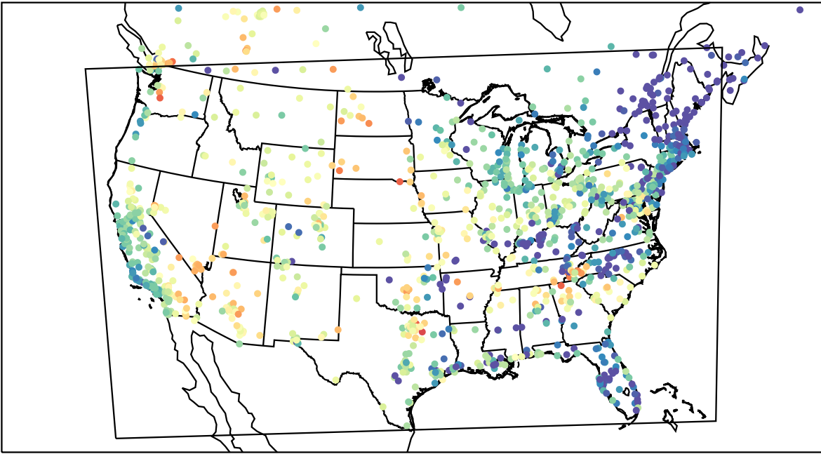
AirNOW (2023-06-08_03:00:00)
