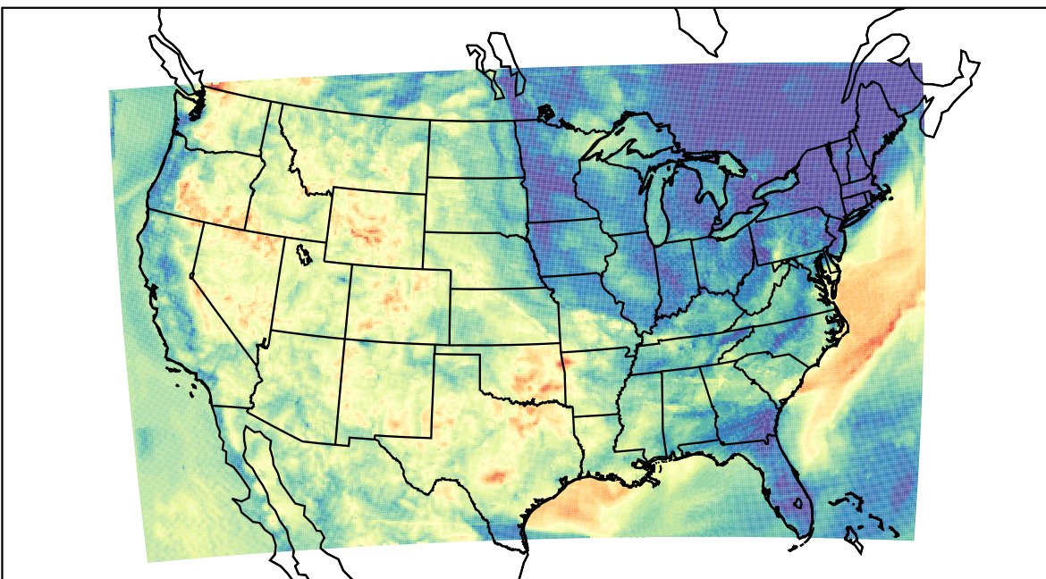
WRF (2023-06-08_09:00:00)
