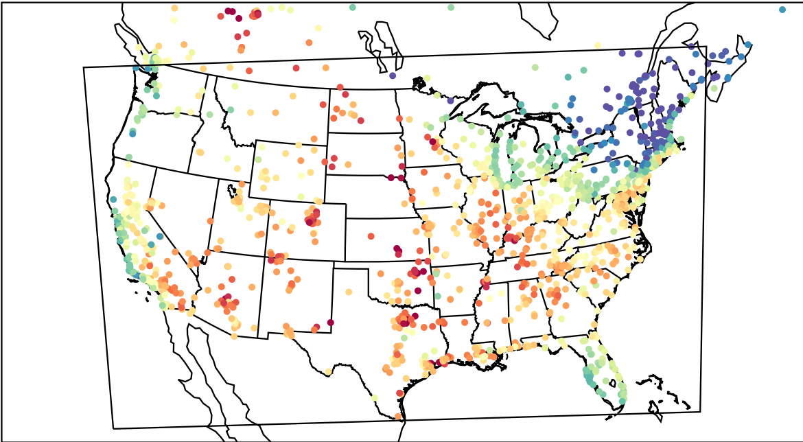
AirNOW (2023-06-08_22:00:00)
