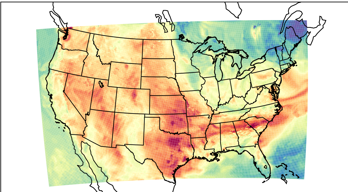
WRF (2023-06-07_21:00:00)
