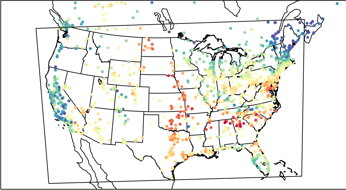
AirNOW (2023-06-07_16:00:00)
