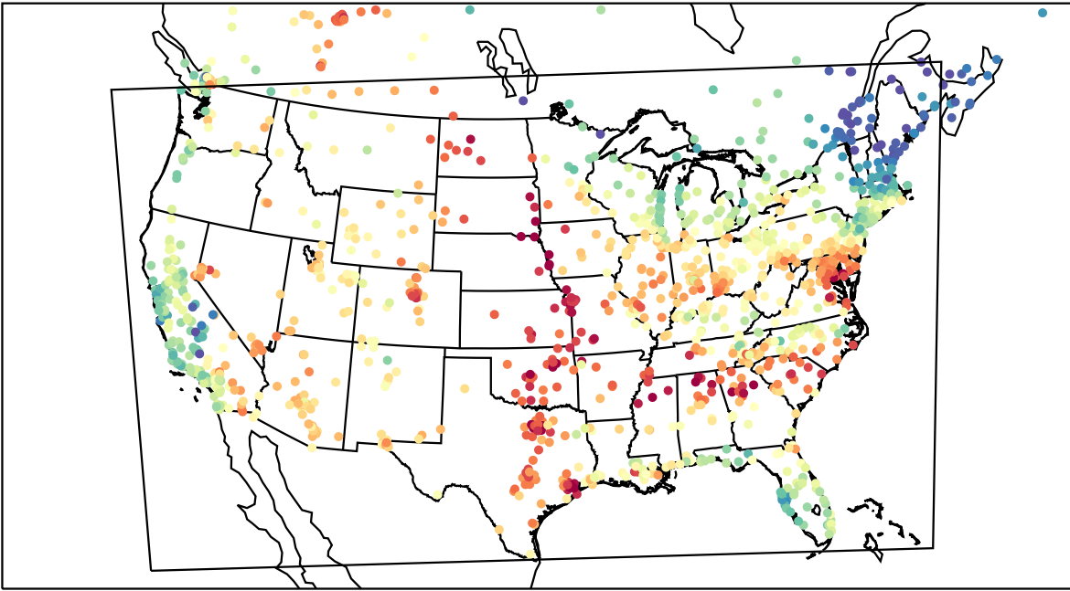
AirNOW (2023-06-07_19:00:00)
