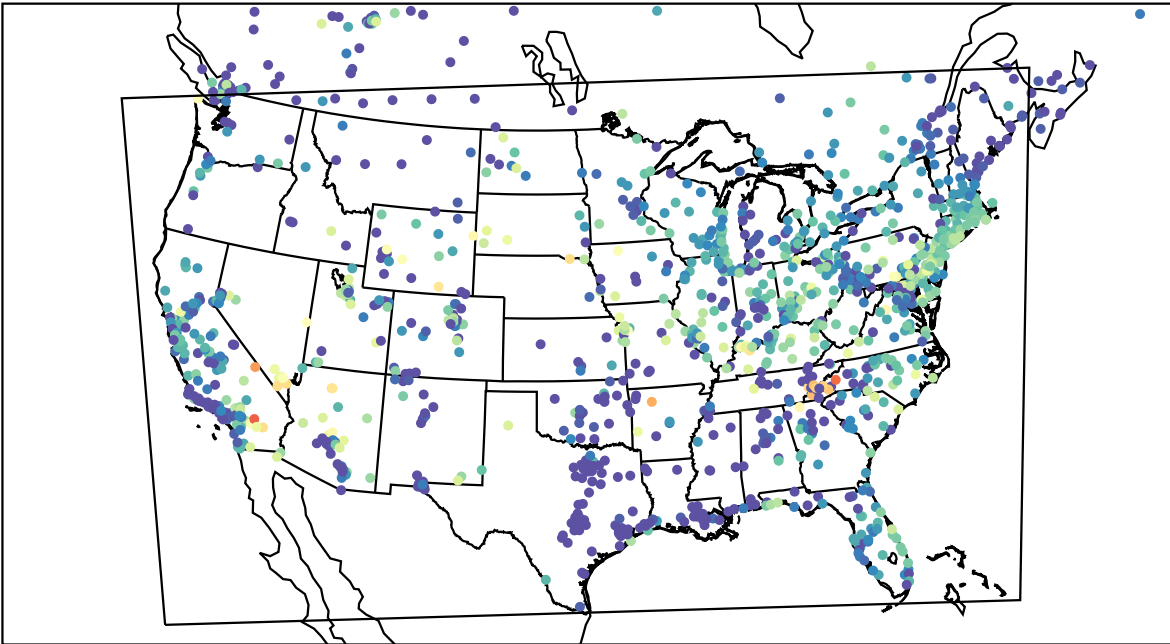
AirNOW (2023-06-07_12:00:00)
