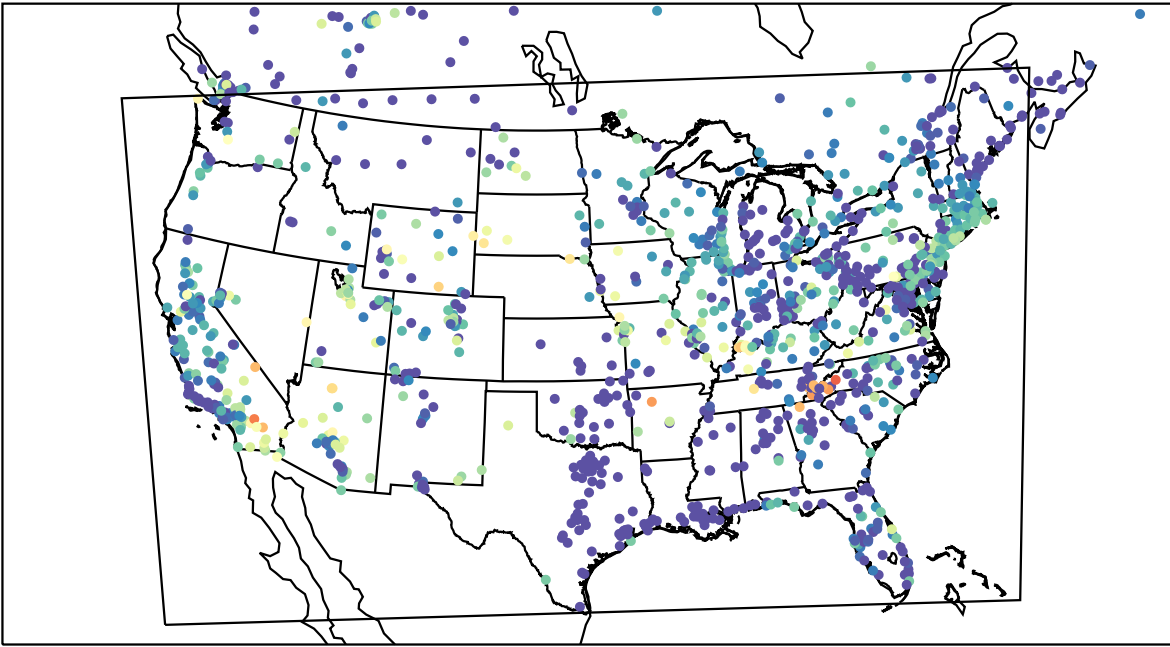
AirNOW (2023-06-07_11:00:00)
