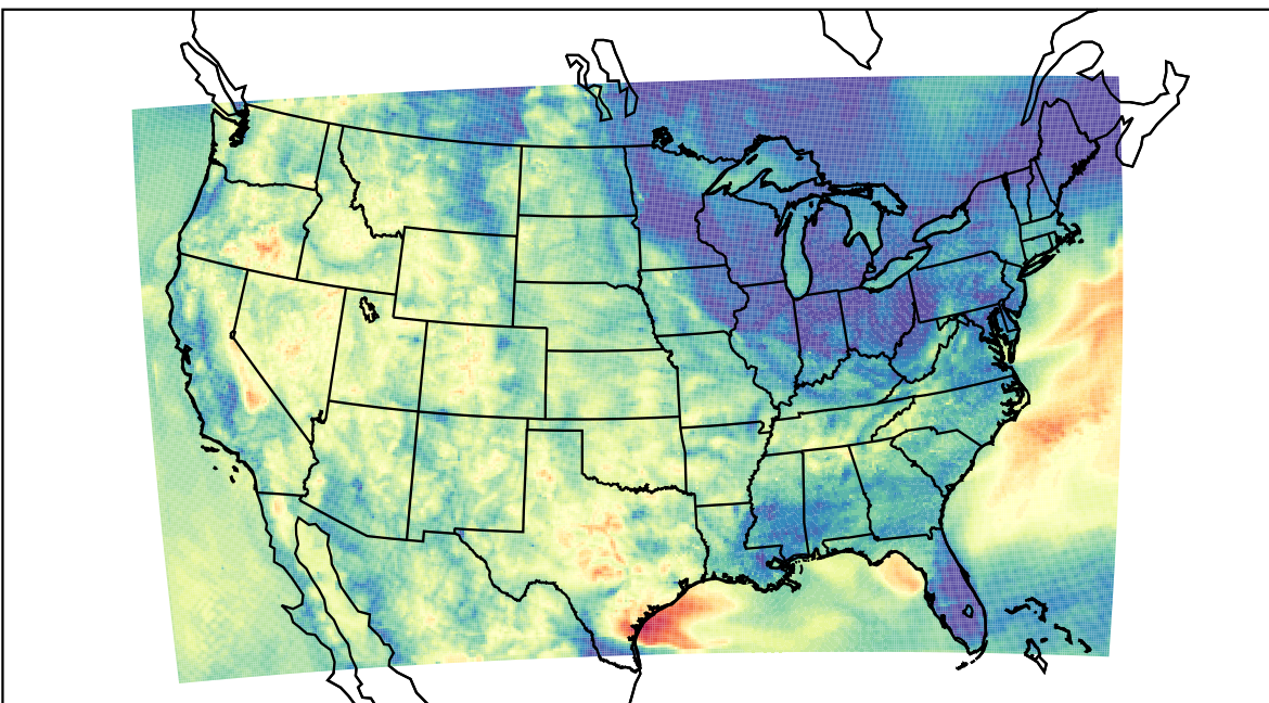
WRF (2023-06-07_12:00:00)
