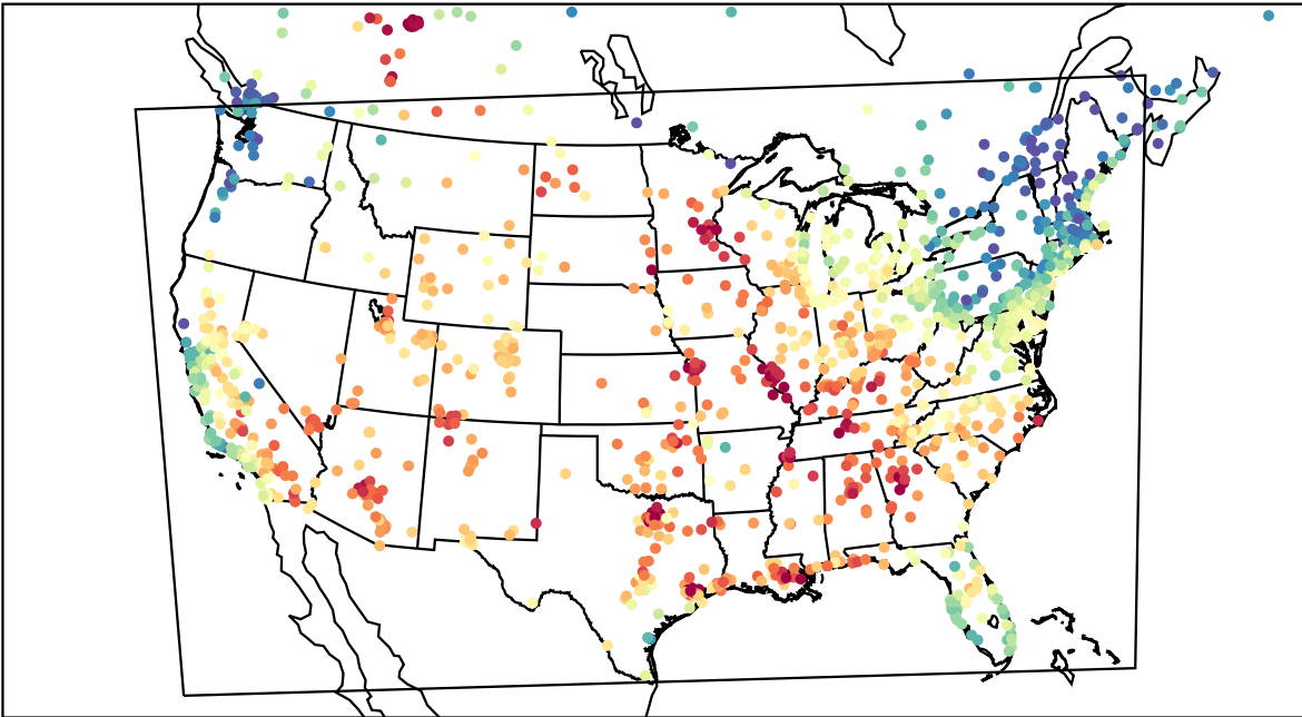
AirNOW (2023-06-09_22:00:00)
