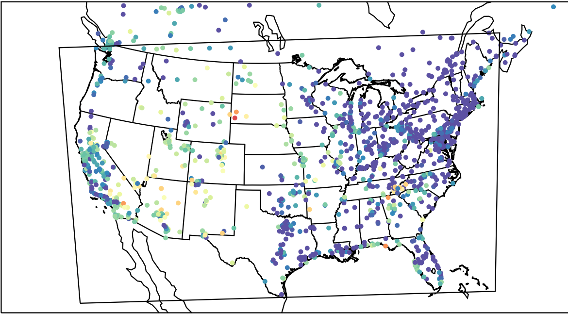
AirNOW (2023-06-09_09:00:00)
