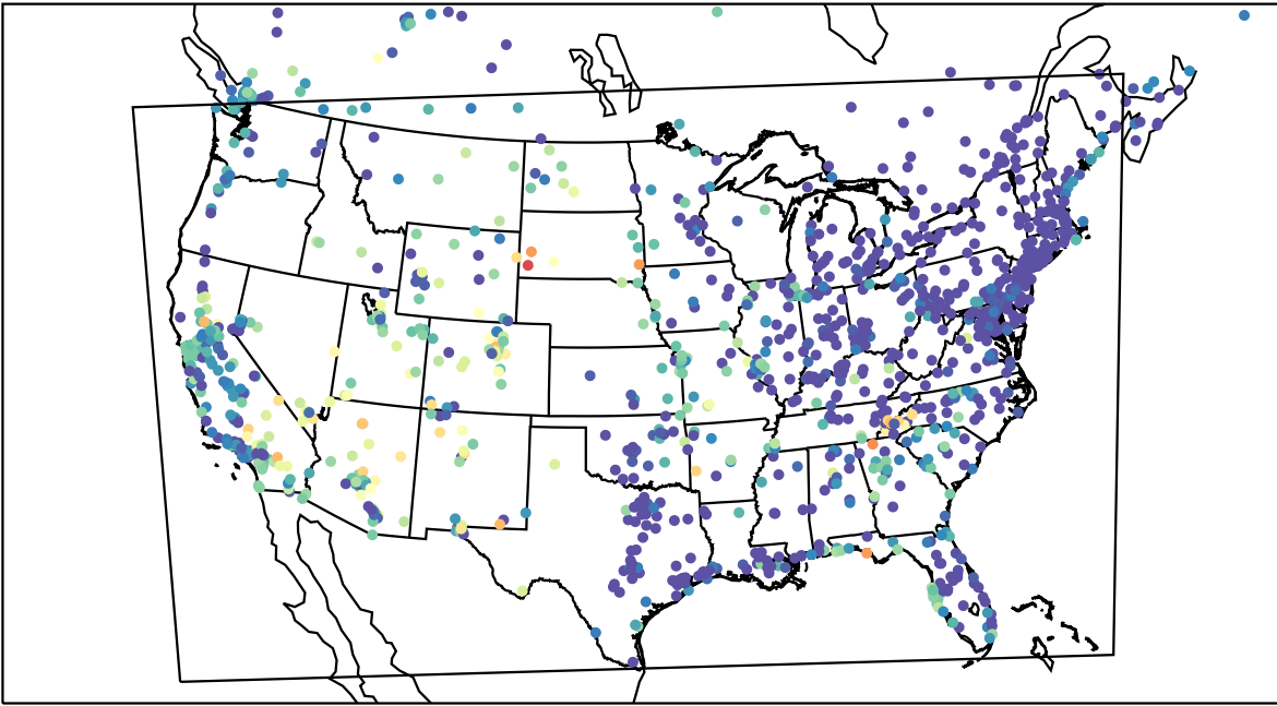
AirNOW (2023-06-09_10:00:00)
