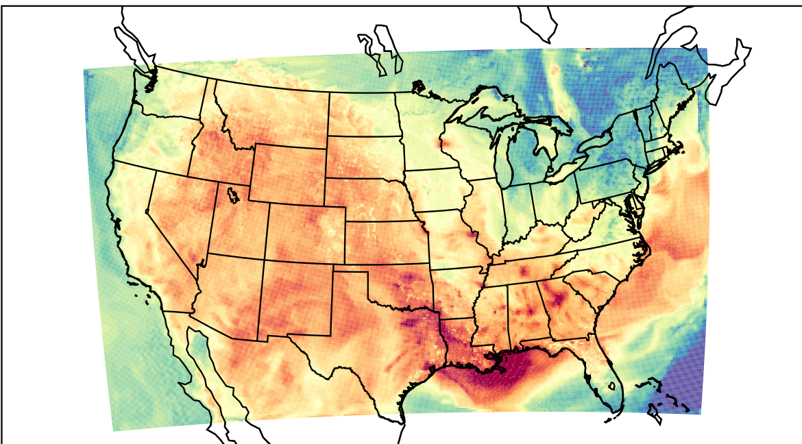
WRF (2023-06-09_21:00:00)
