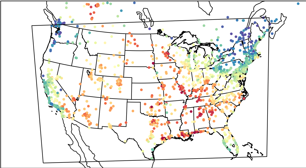
AirNOW (2023-06-09_18:00:00)
