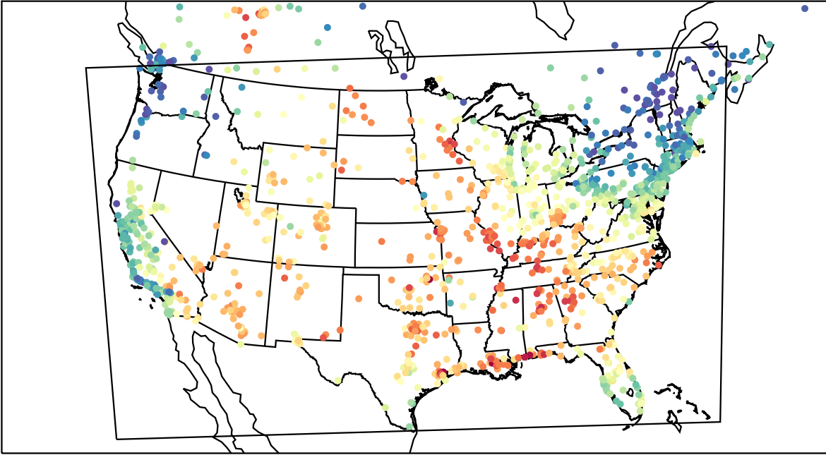
AirNOW (2023-06-09_17:00:00)
