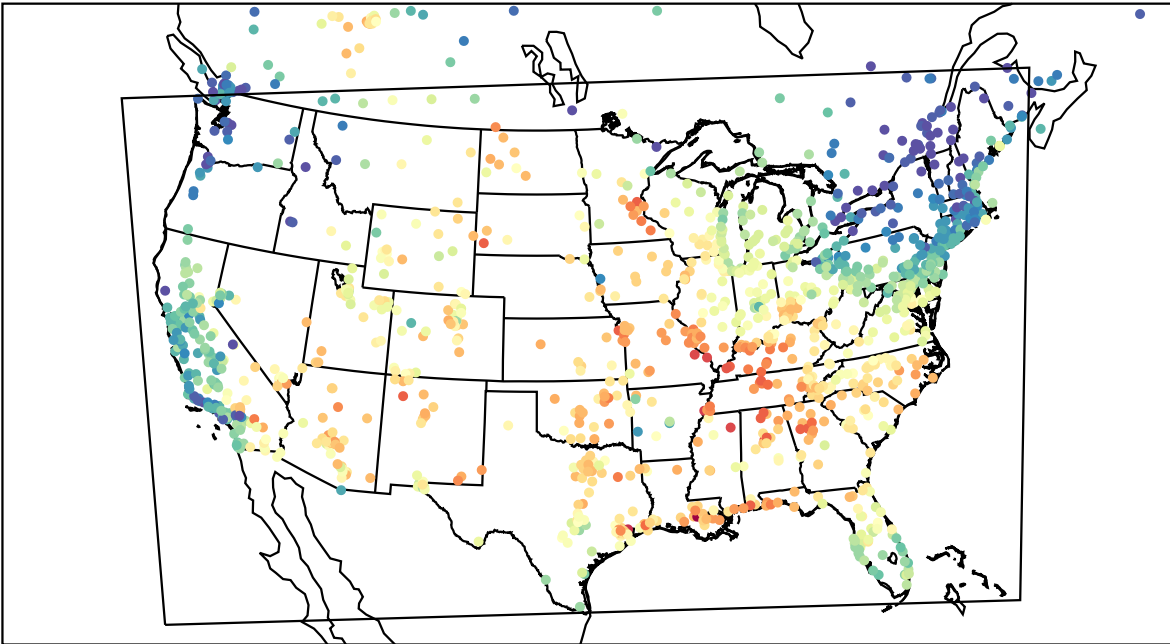
AirNOW (2023-06-09_16:00:00)
