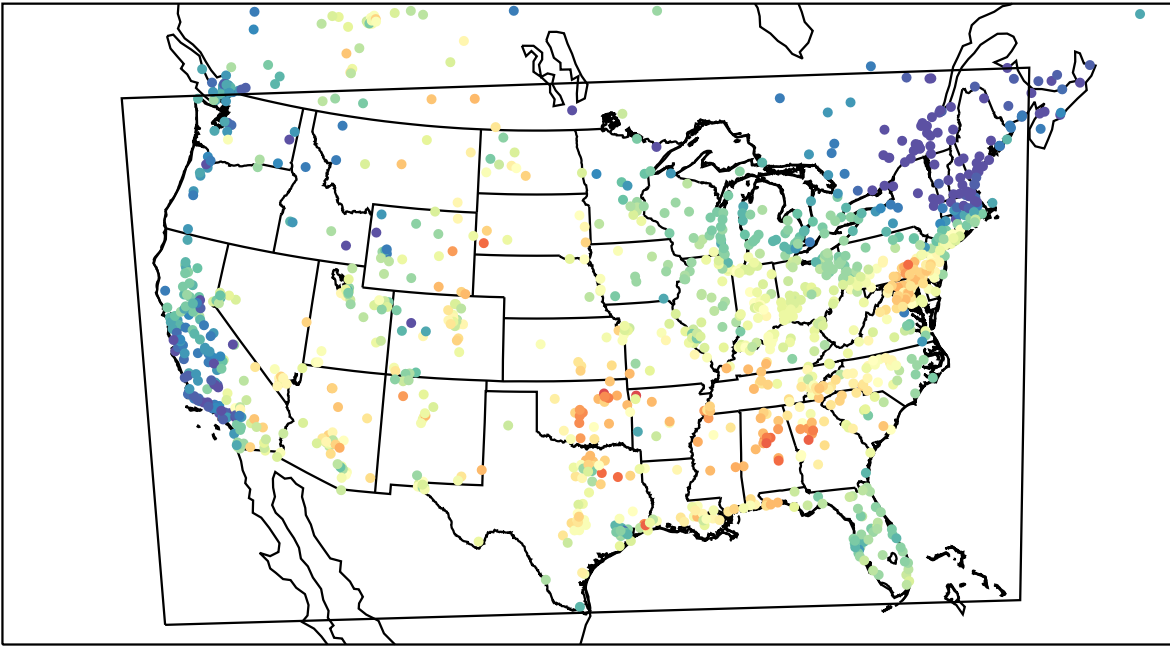
AirNOW (2023-06-08_15:00:00)
