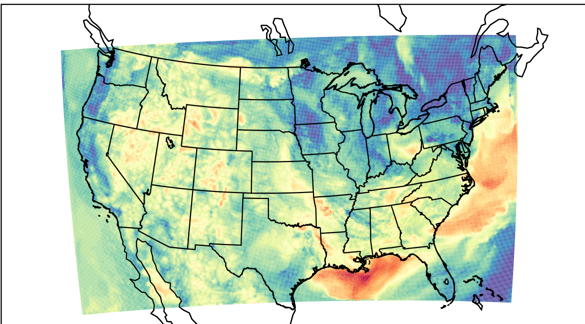
WRF (2023-06-09_14:00:00)
