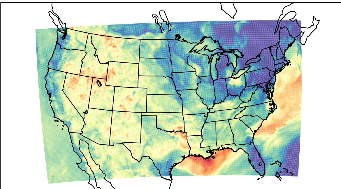
WRF (2023-06-09_08:00:00)
