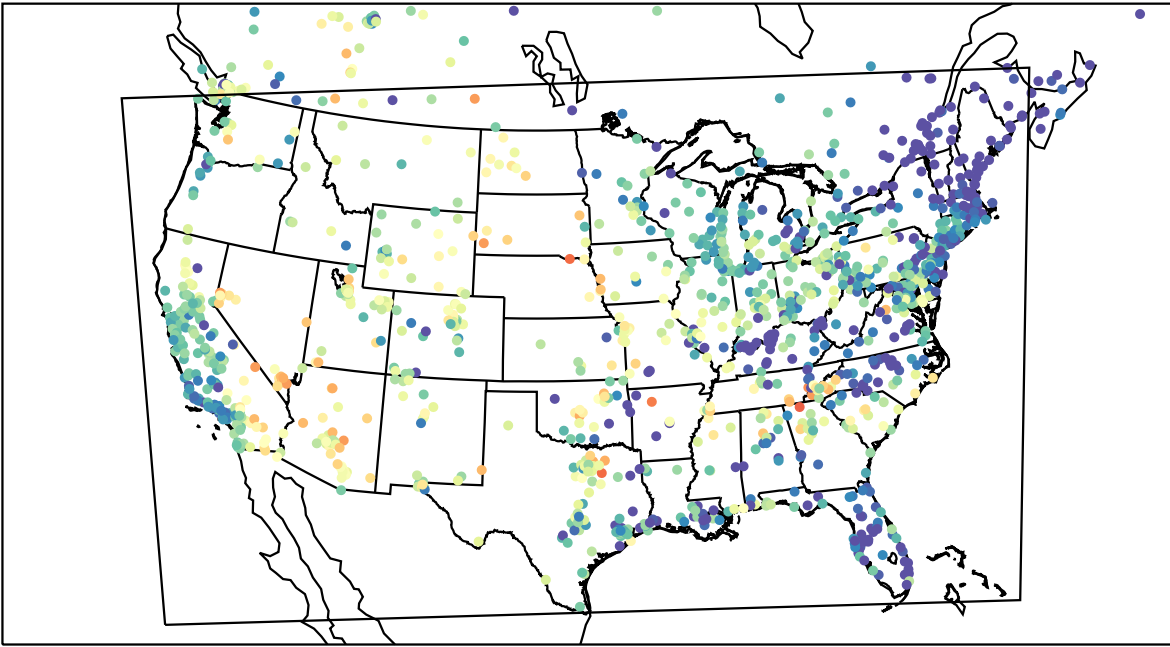
AirNOW (2023-06-08_04:00:00)
