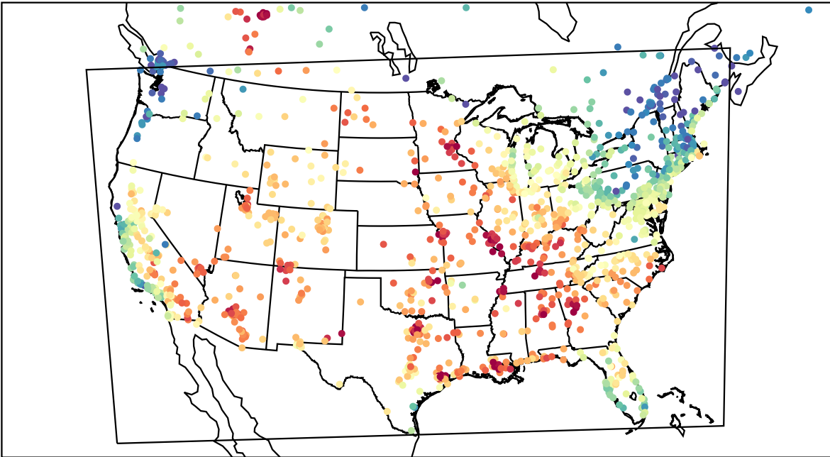
AirNOW (2023-06-09_21:00:00)
