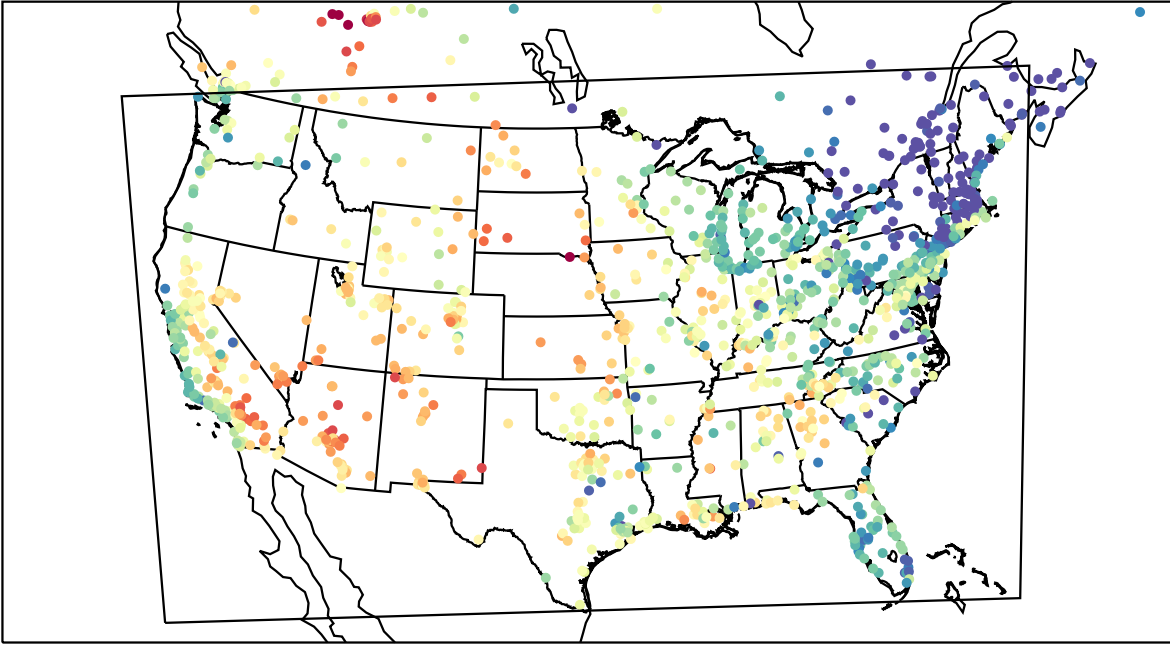
AirNOW (2023-06-09_01:00:00)
