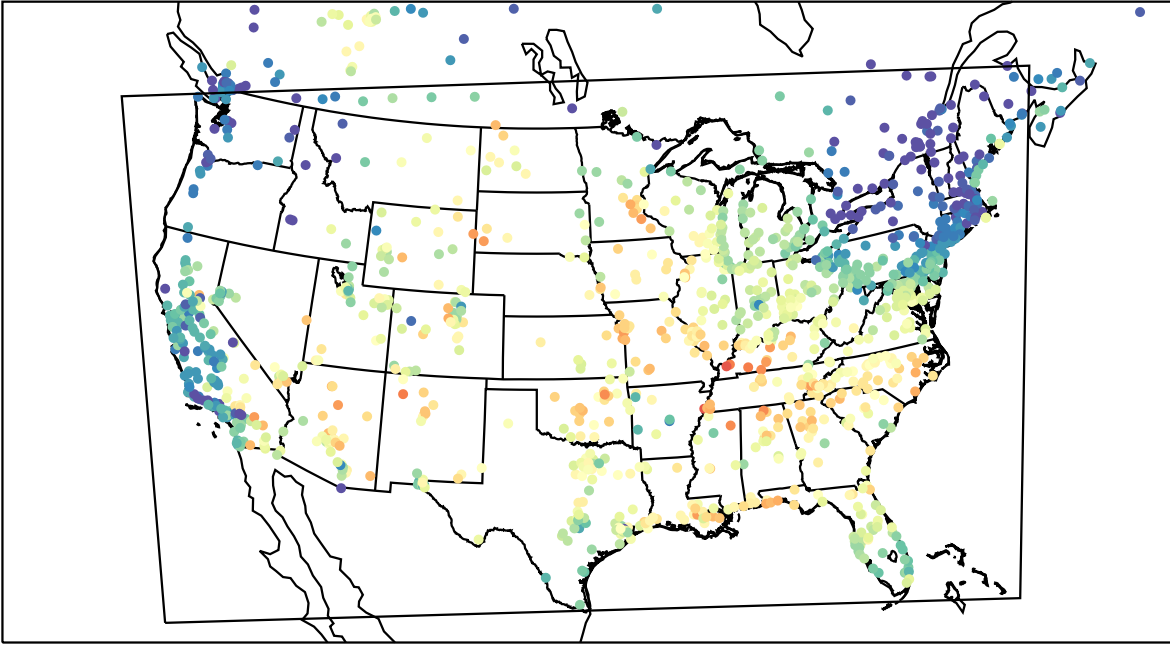
AirNOW (2023-06-09_15:00:00)
