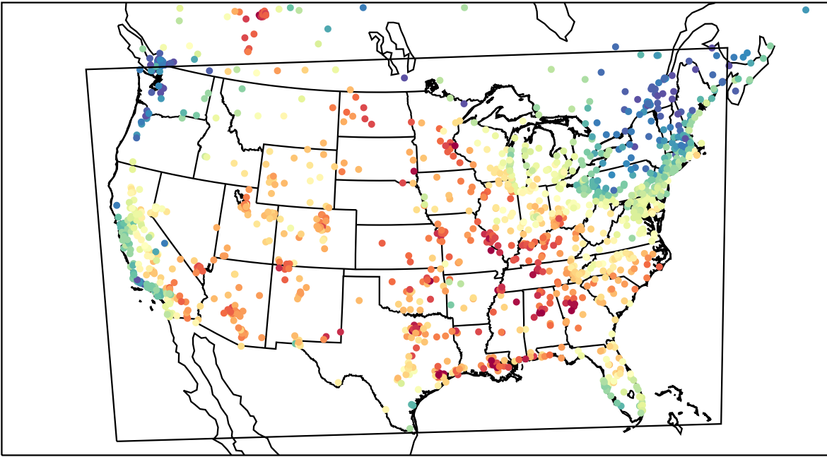
AirNOW (2023-06-09_19:00:00)
