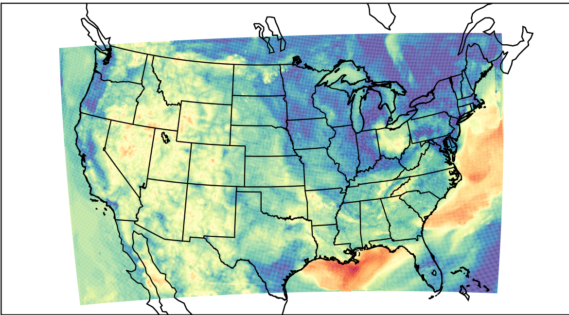
WRF (2023-06-09_13:00:00)
