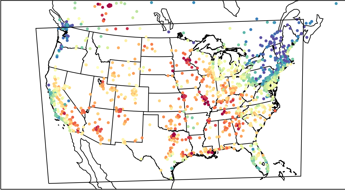
AirNOW (2023-06-09_23:00:00)
