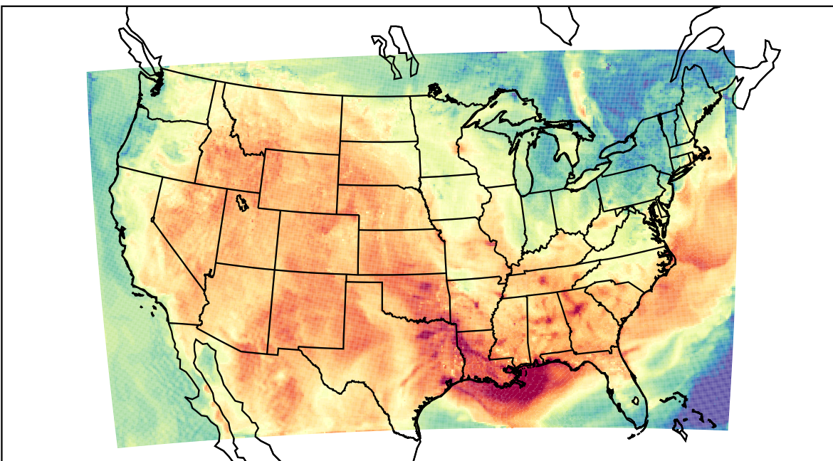
WRF (2023-06-09_19:00:00)
