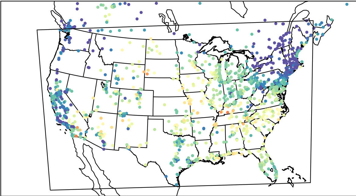
AirNOW (2023-06-09_14:00:00)
