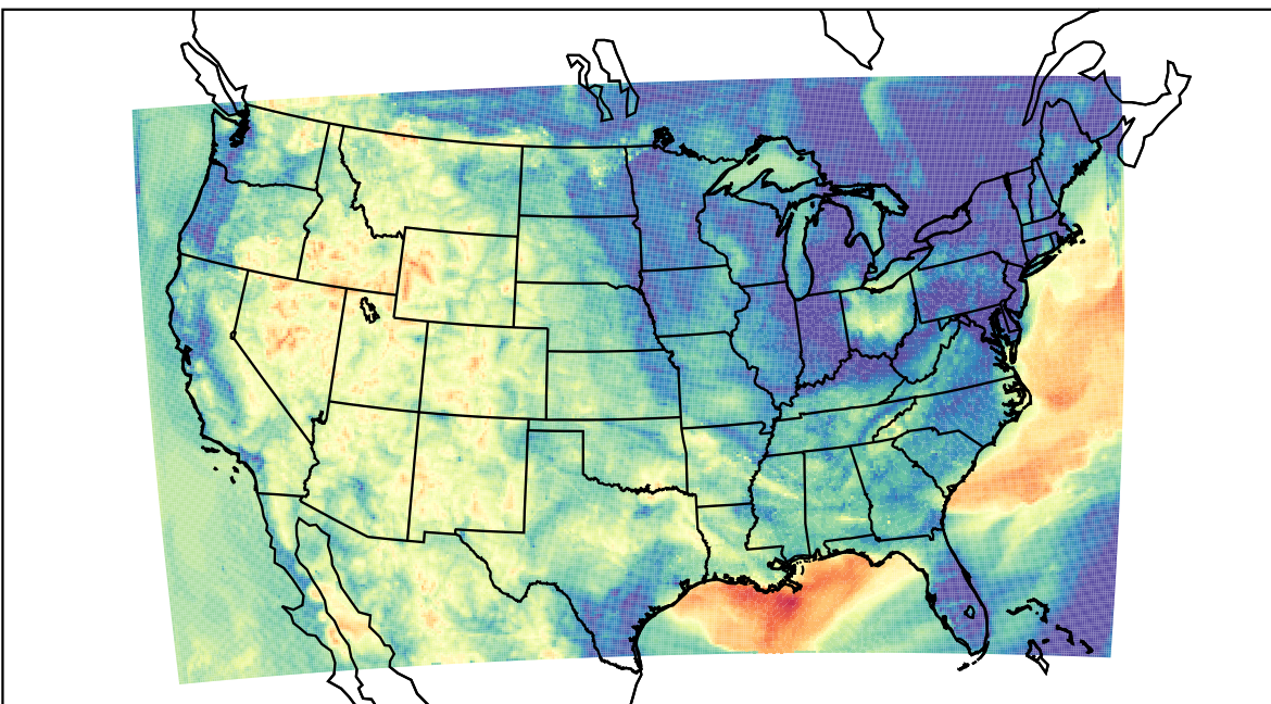
WRF (2023-06-09_12:00:00)
