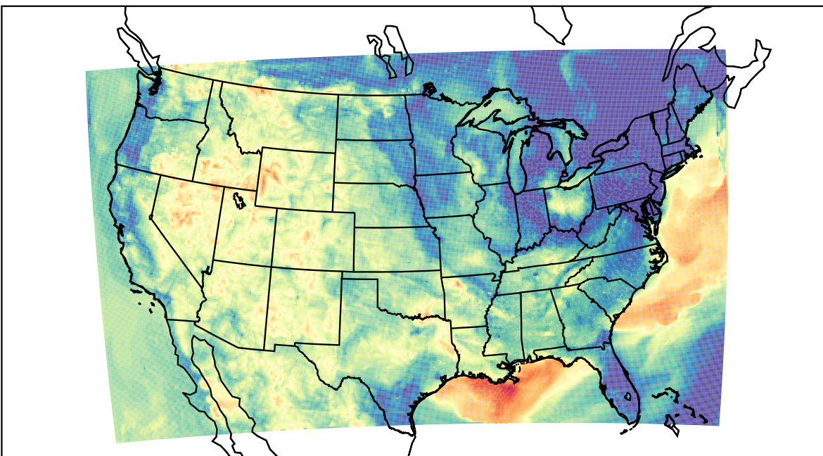
WRF (2023-06-09_11:00:00)
