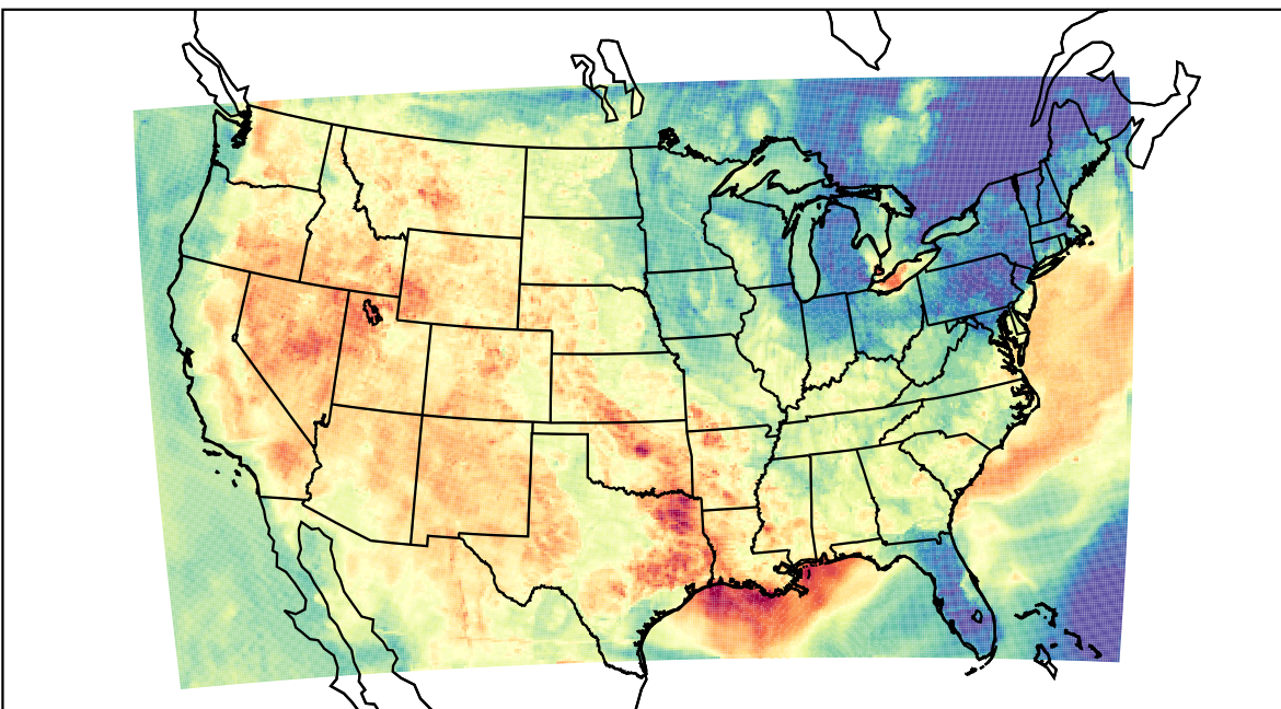
WRF (2023-06-09_02:00:00)
