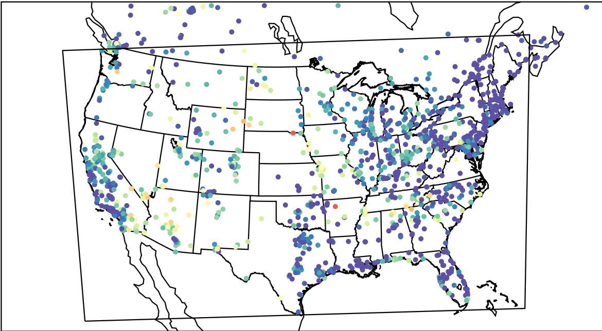
AirNOW (2023-06-08_09:00:00)
