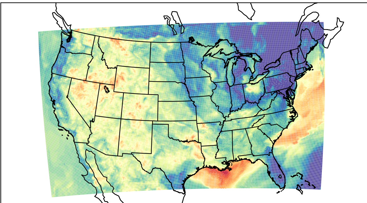
WRF (2023-06-09_09:00:00)
