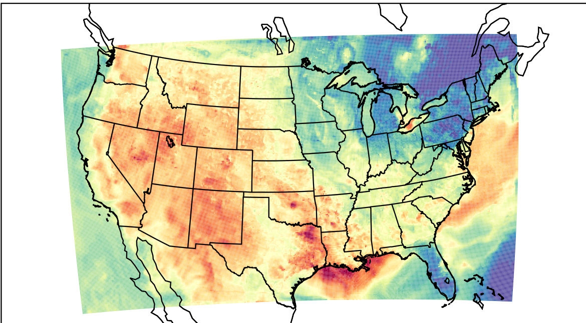
WRF (2023-06-09_01:00:00)
