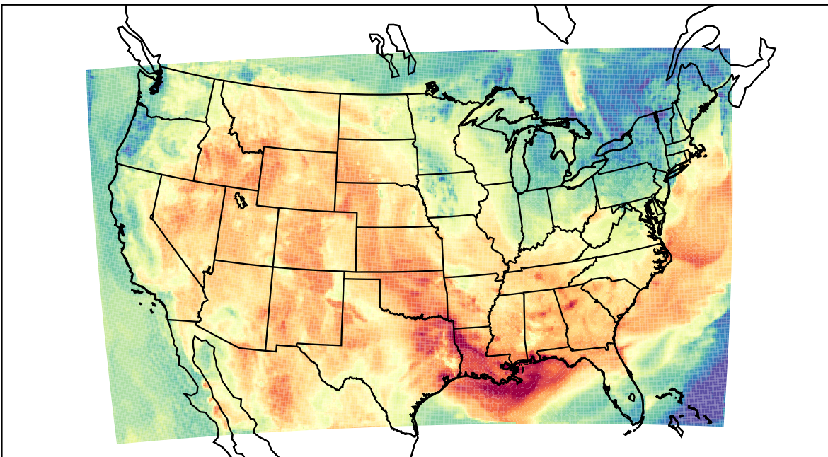
WRF (2023-06-09_17:00:00)
