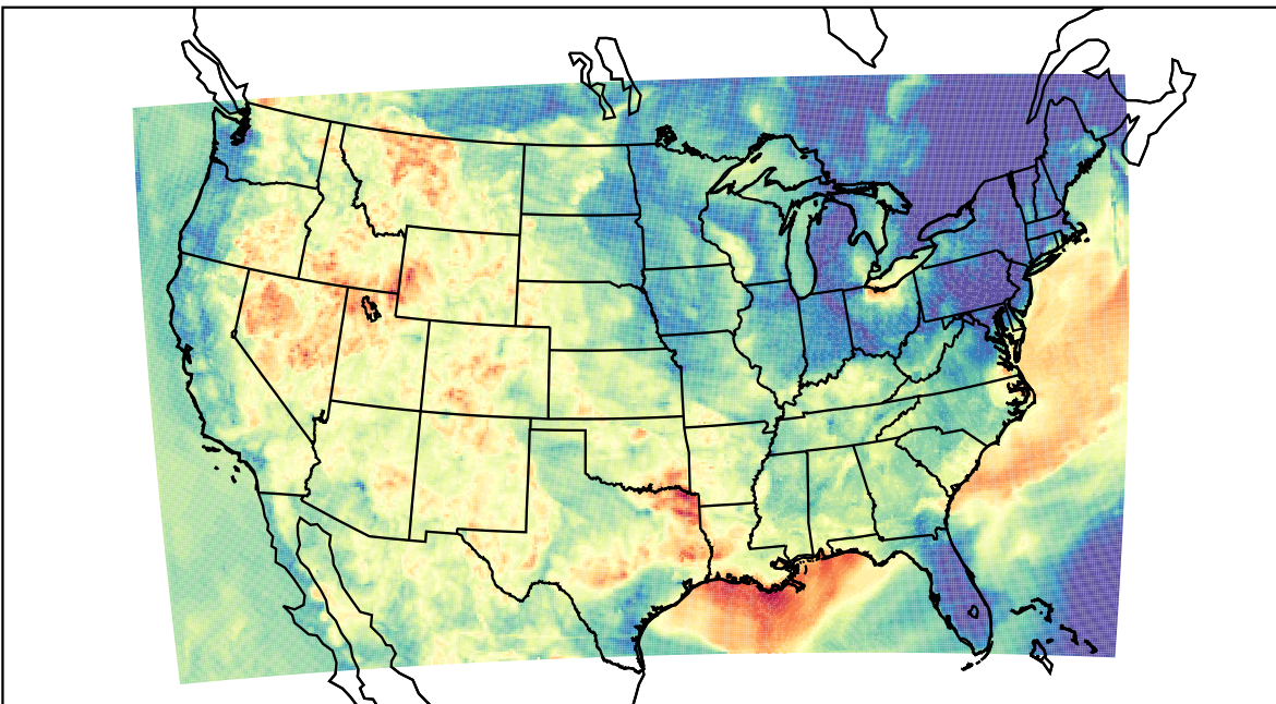
WRF (2023-06-09_06:00:00)
