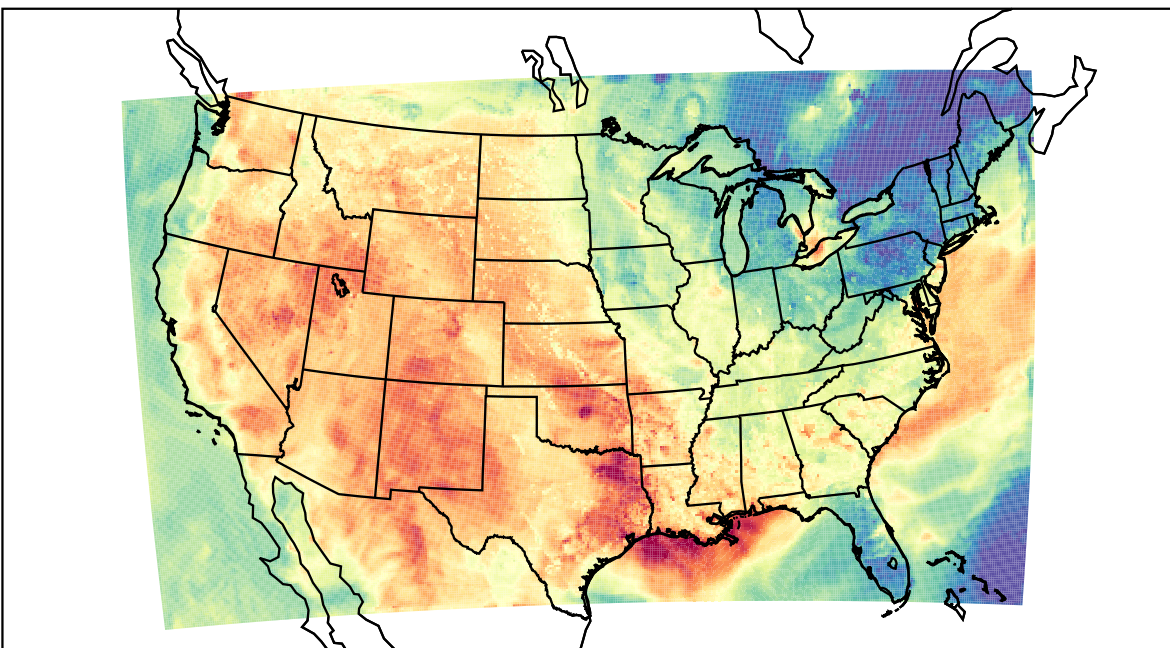
WRF (2023-06-09_00:00:00)
