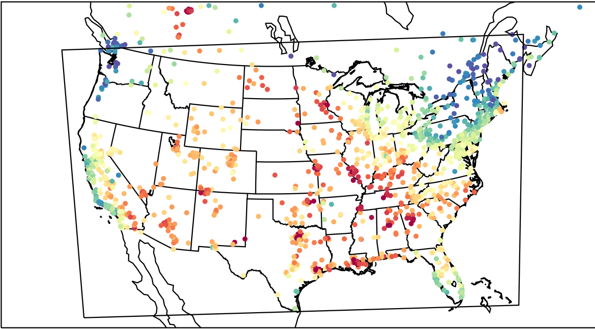
AirNOW (2023-06-09_20:00:00)
