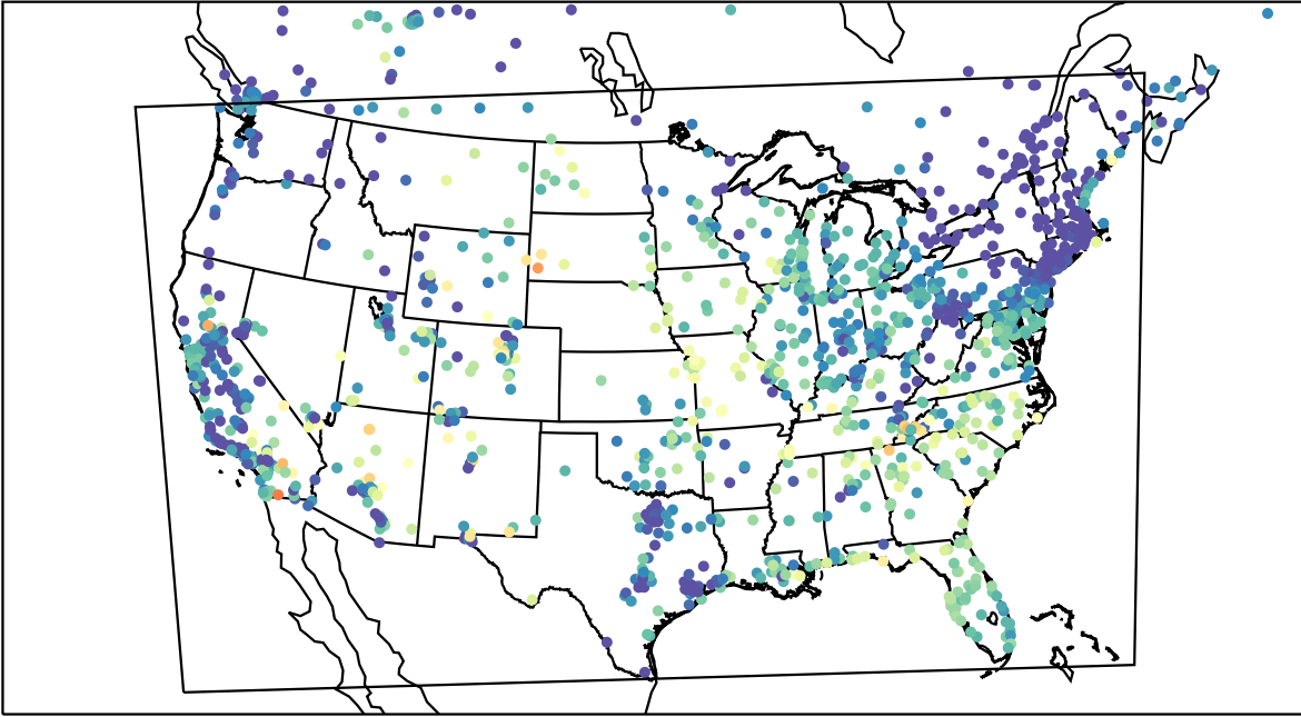
AirNOW (2023-06-09_13:00:00)
