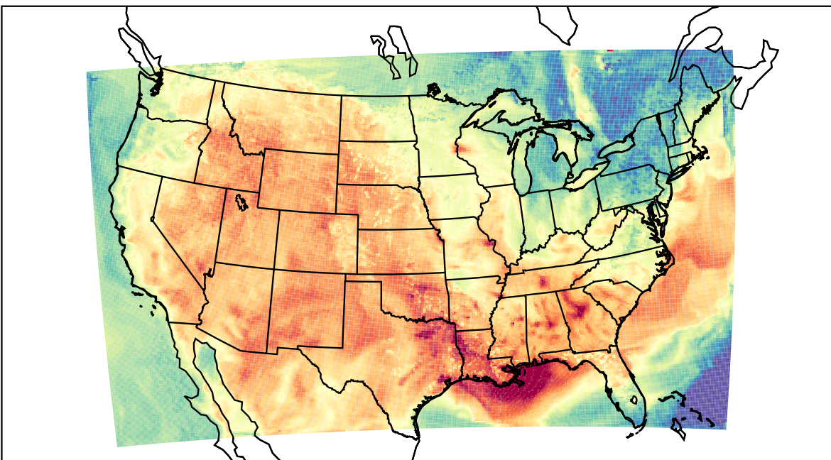
WRF (2023-06-09_22:00:00)
