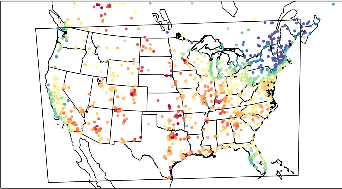
AirNOW (2023-06-08_22:00:00)
