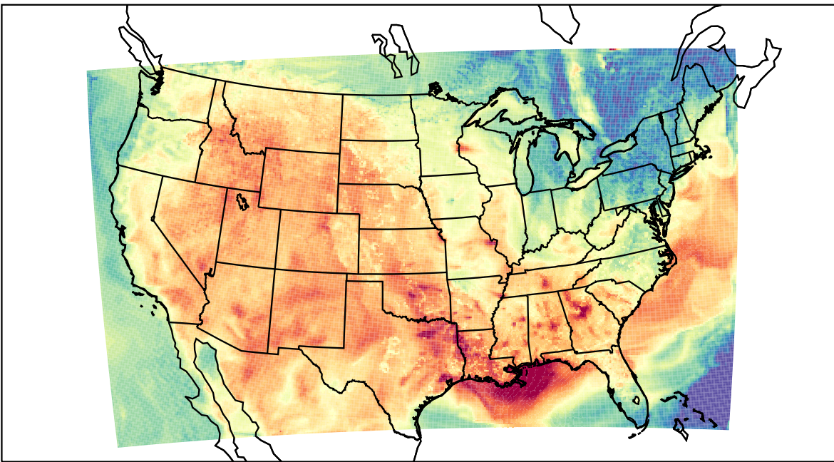
WRF (2023-06-09_23:00:00)
