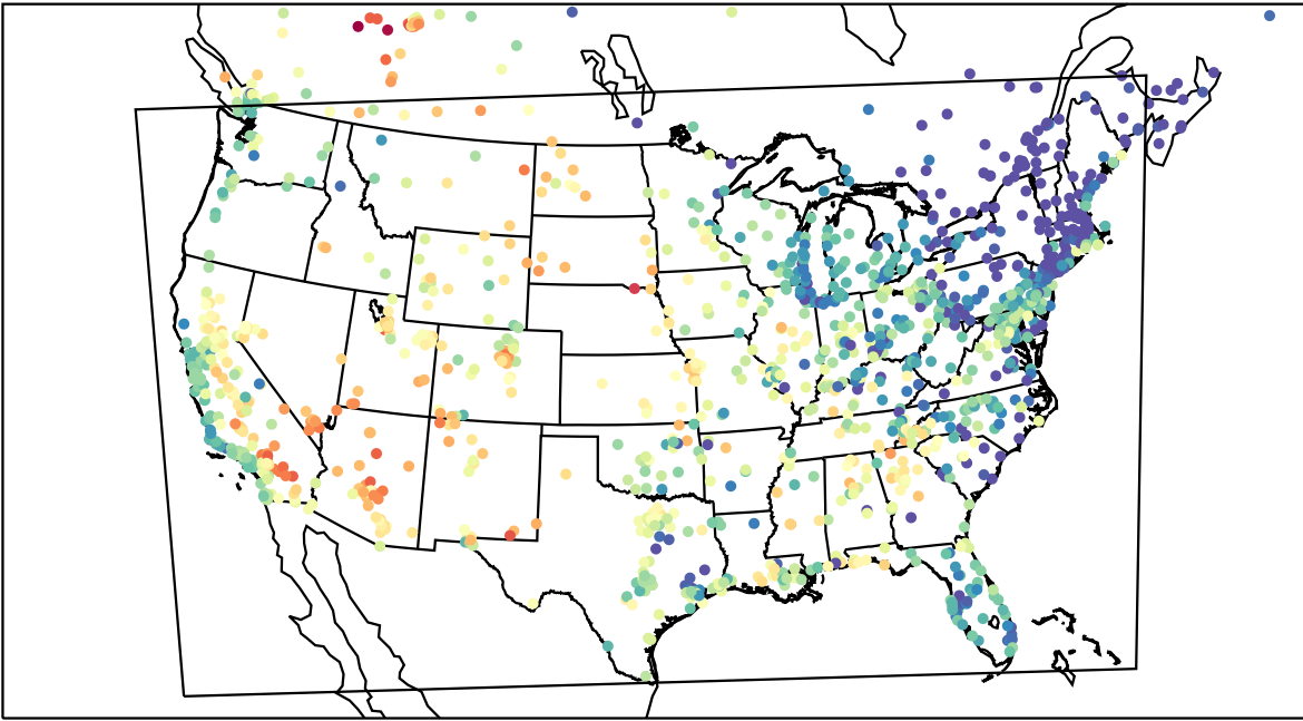
AirNOW (2023-06-09_02:00:00)
