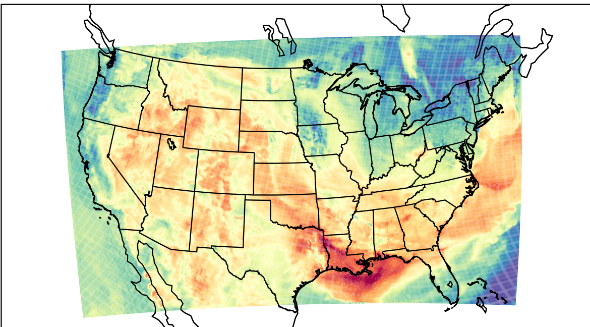
WRF (2023-06-09_16:00:00)
