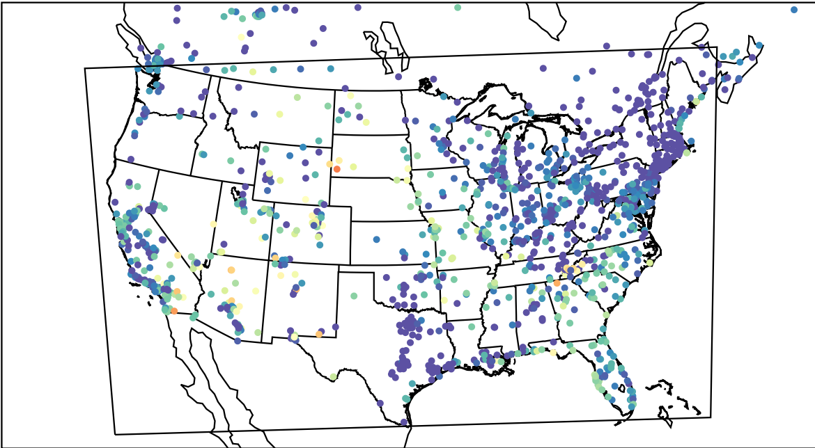
AirNOW (2023-06-09_12:00:00)
