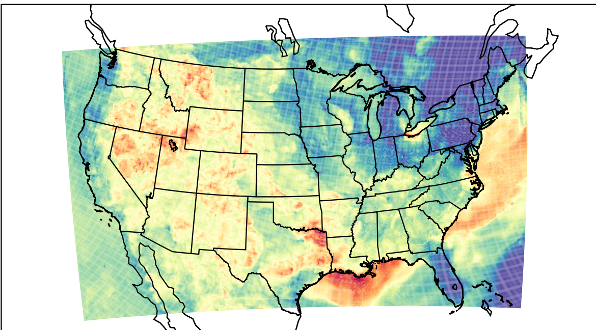
WRF (2023-06-09_05:00:00)
