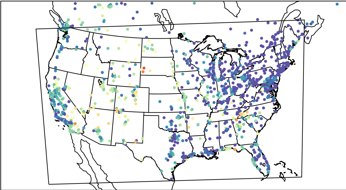
AirNOW (2023-06-09_08:00:00)
