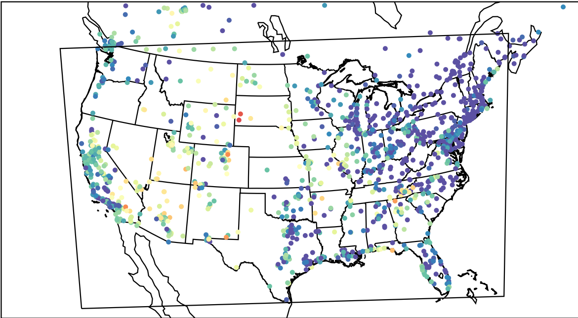
AirNOW (2023-06-09_07:00:00)
