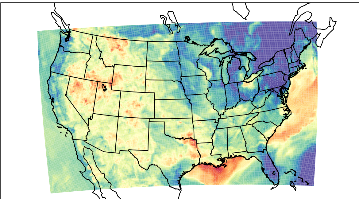
WRF (2023-06-09_07:00:00)
