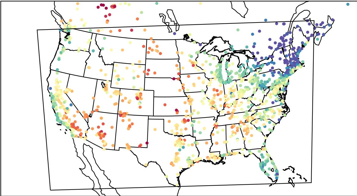
AirNOW (2023-06-09_00:00:00)
