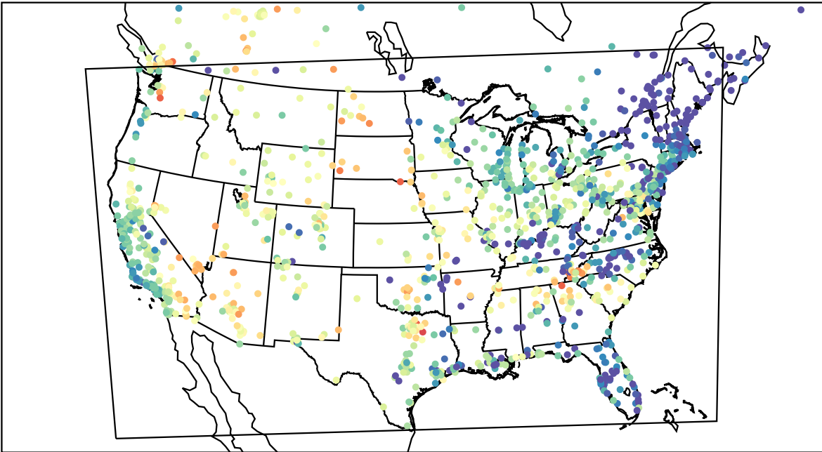
AirNOW (2023-06-08_03:00:00)
