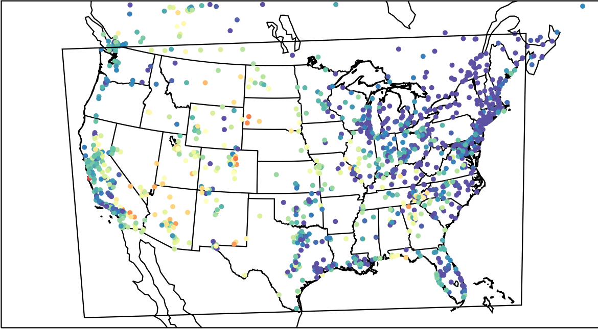
AirNOW (2023-06-09_06:00:00)
