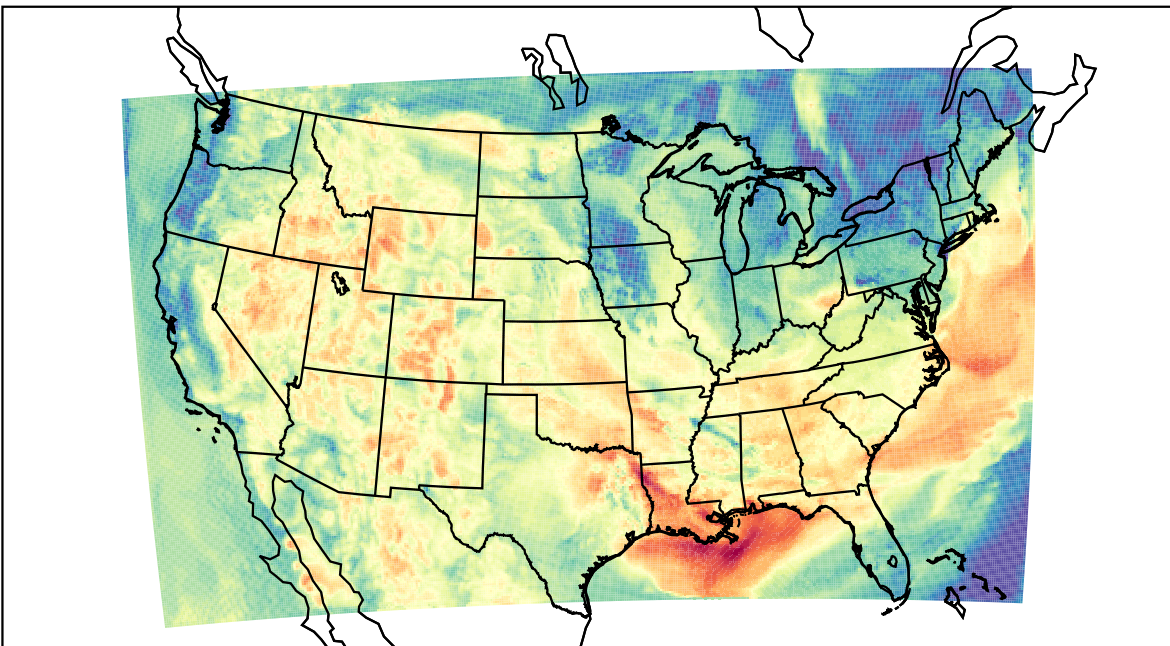
WRF (2023-06-09_15:00:00)
