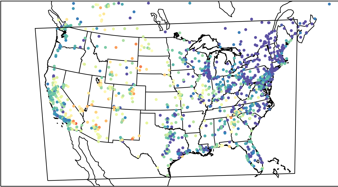
AirNOW (2023-06-09_05:00:00)
