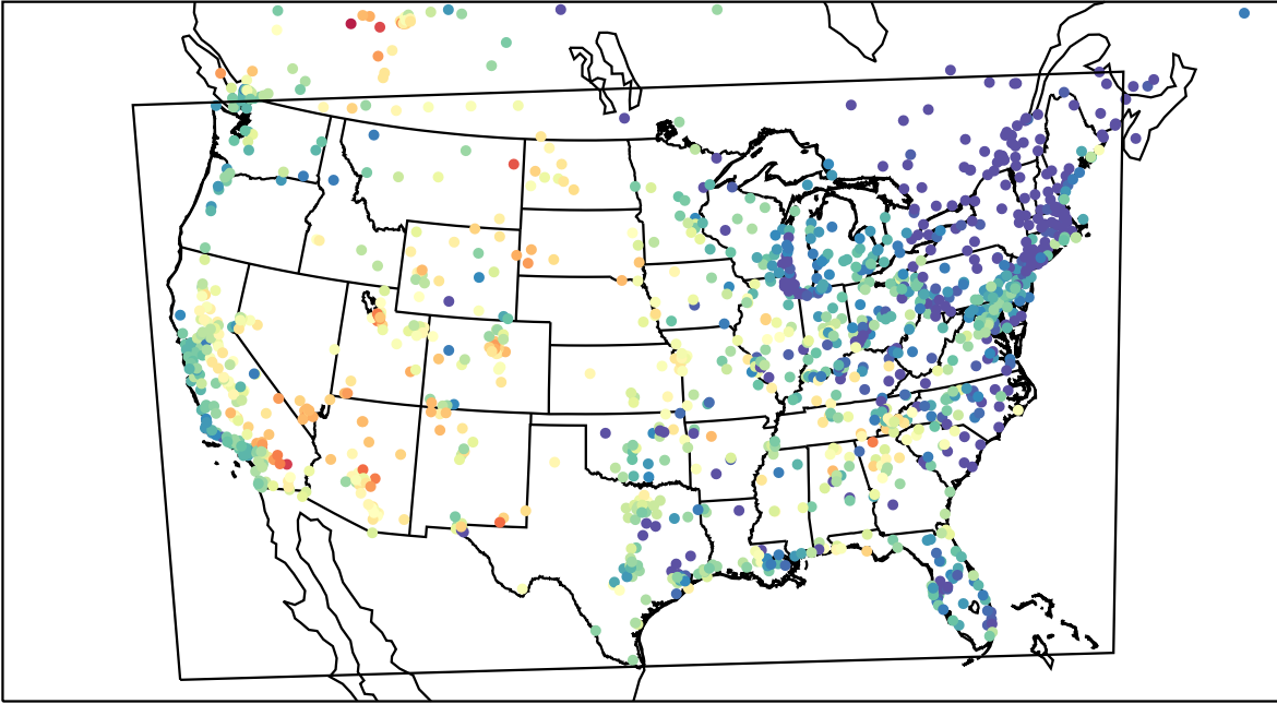
AirNOW (2023-06-09_03:00:00)
