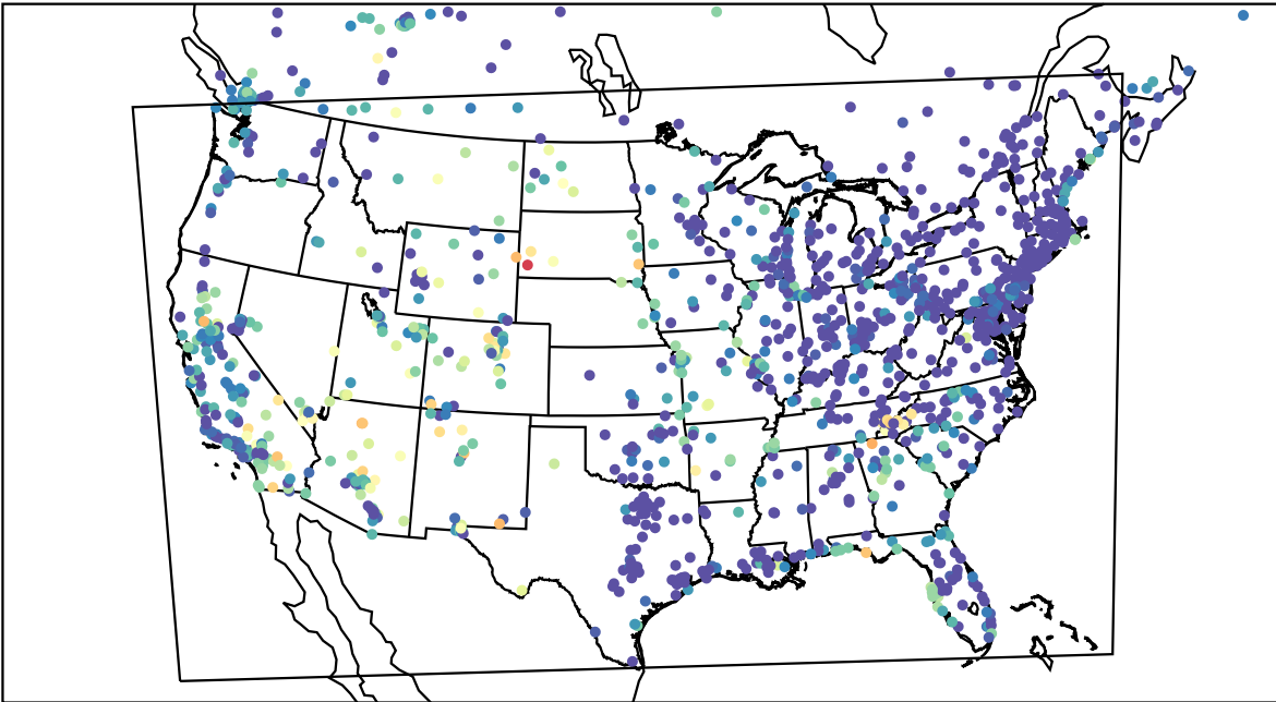
AirNOW (2023-06-09_11:00:00)
