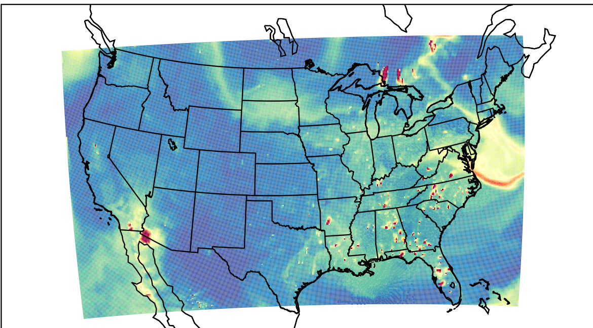
WRF 2023-06-11_00:00:00
