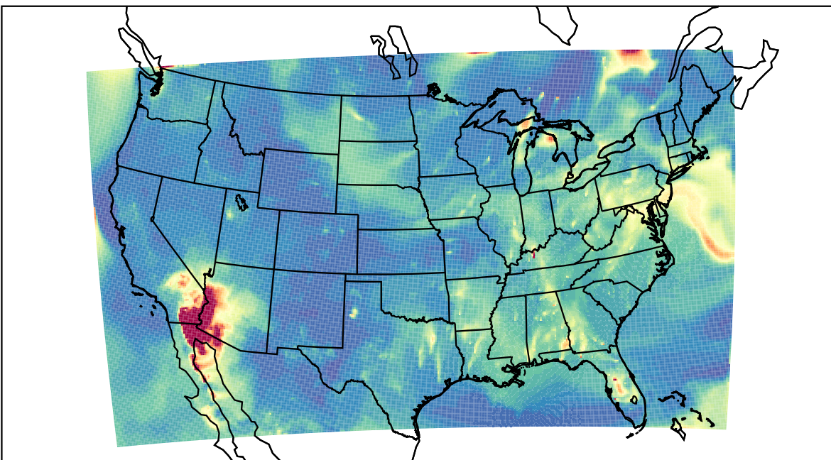
WRF 2023-06-11_09:00:00
