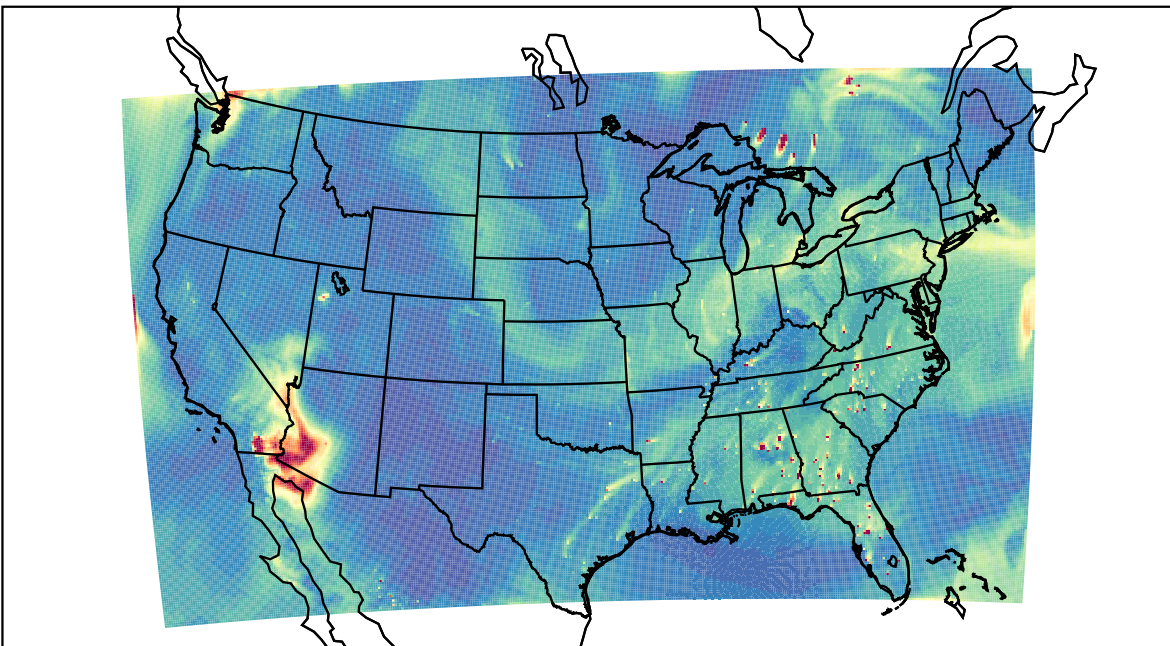
WRF 2023-06-11_21:00:00
