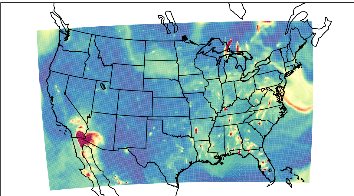
WRF 2023-06-11_03:00:00
