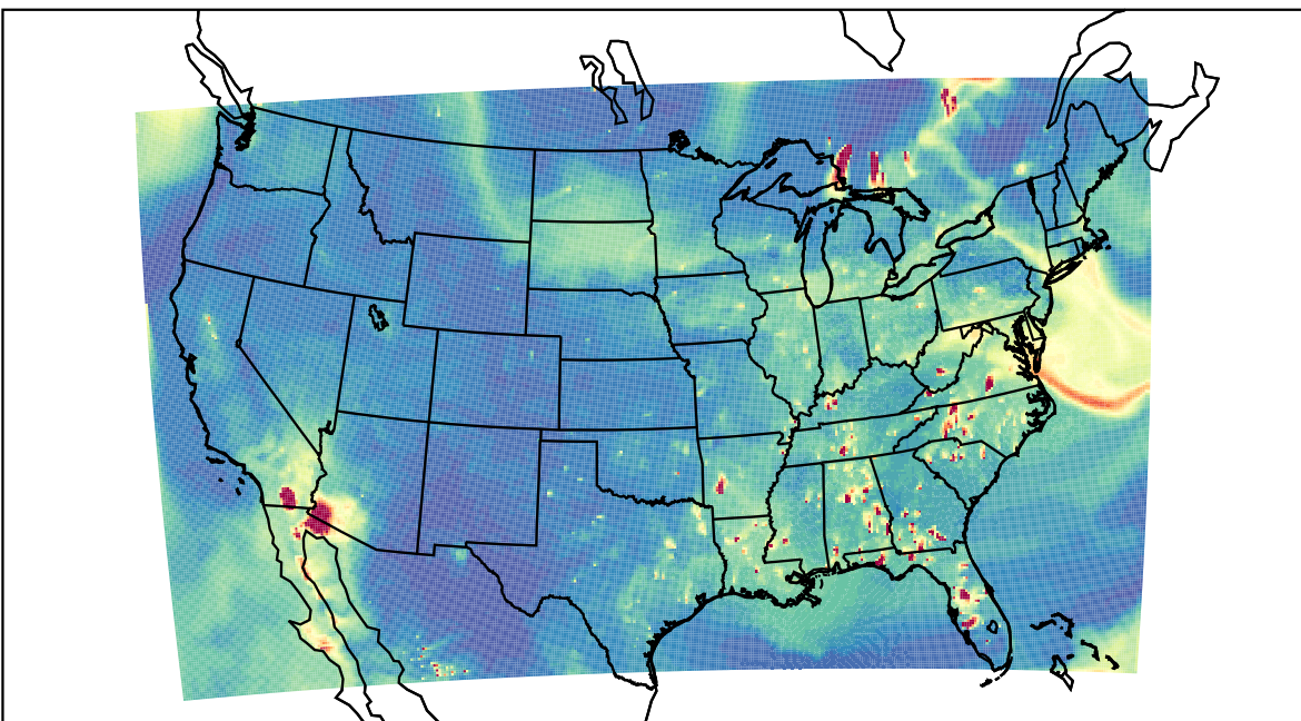
WRF 2023-06-11_01:00:00
