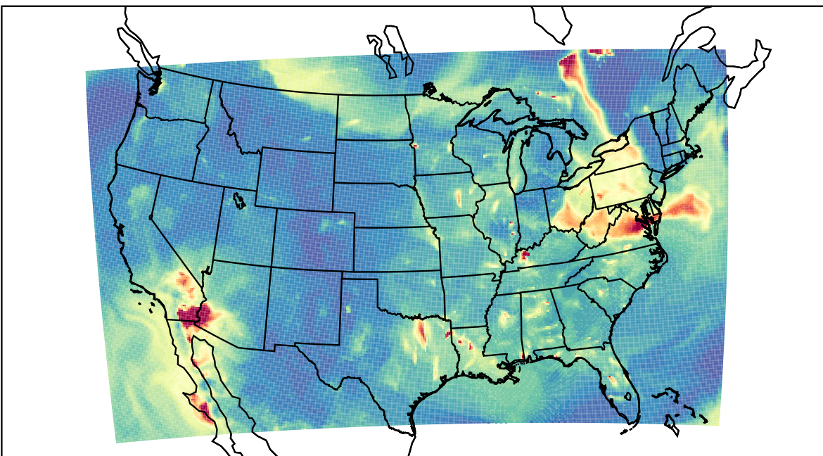
WRF 2023-06-10_07:00:00
