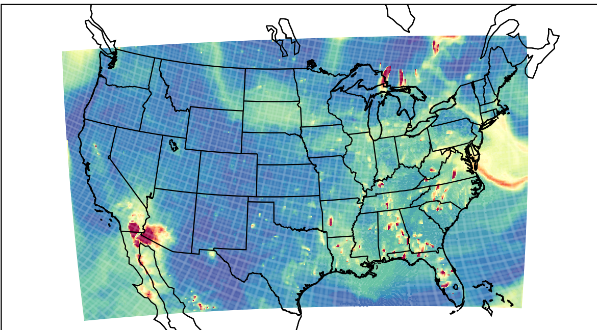
WRF 2023-06-11_02:00:00
