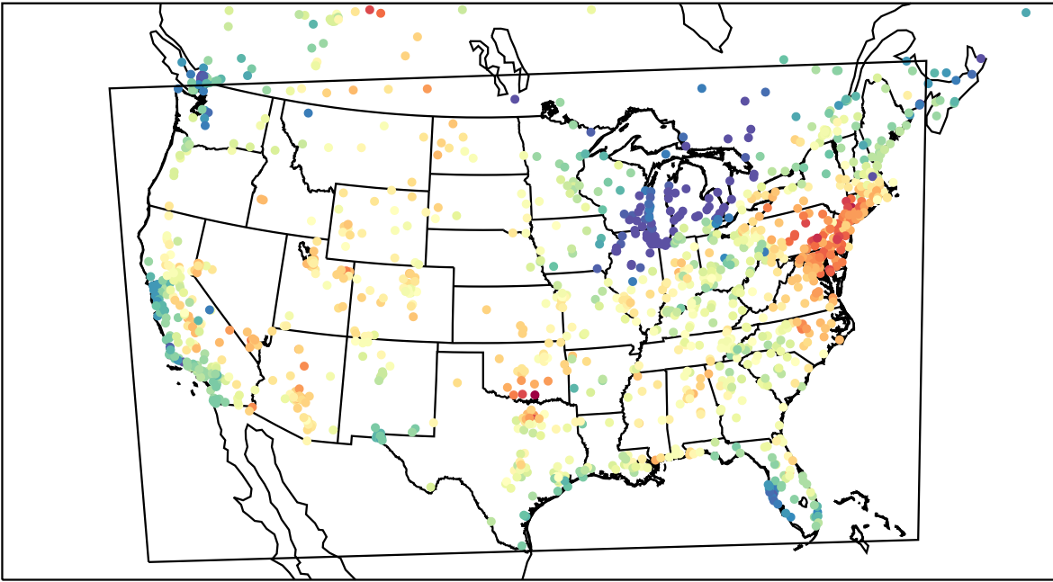
AirNOW (2023-06-11_22:00:00)
