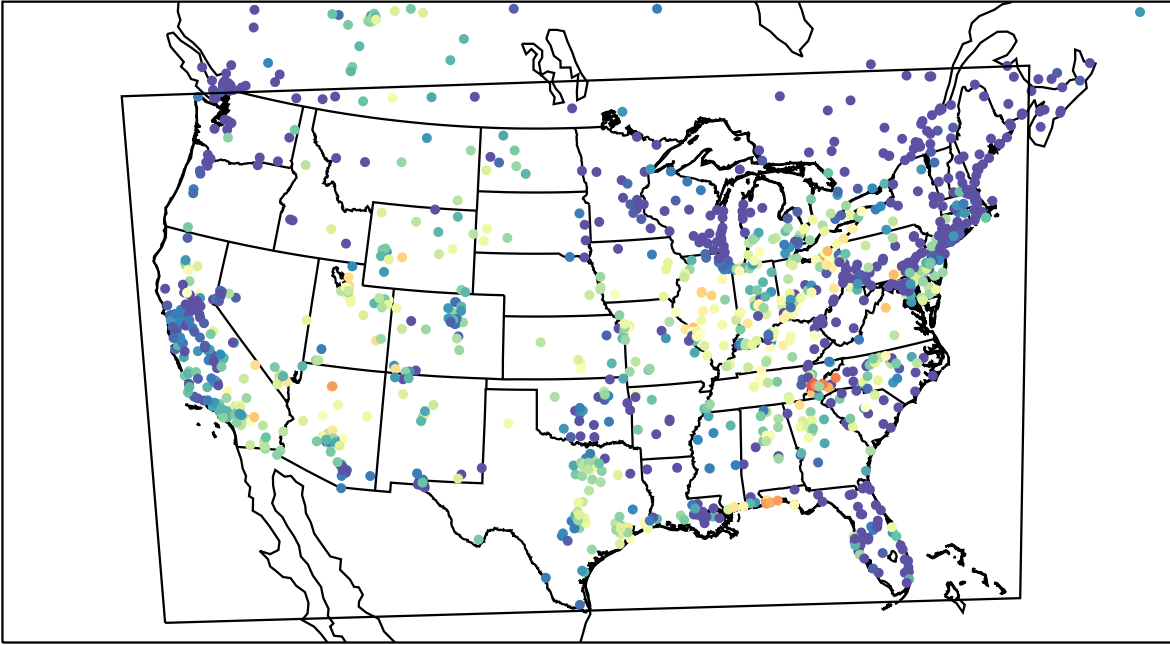
AirNOW (2023-06-11_09:00:00)
