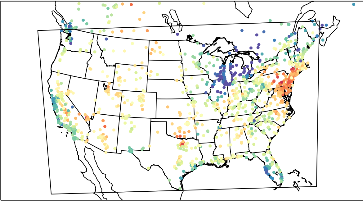
AirNOW (2023-06-11_23:00:00)
