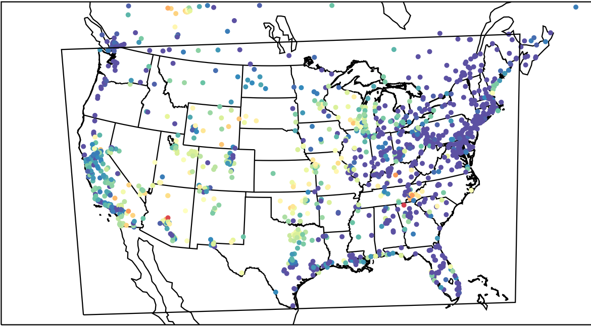
AirNOW (2023-06-10_08:00:00)
