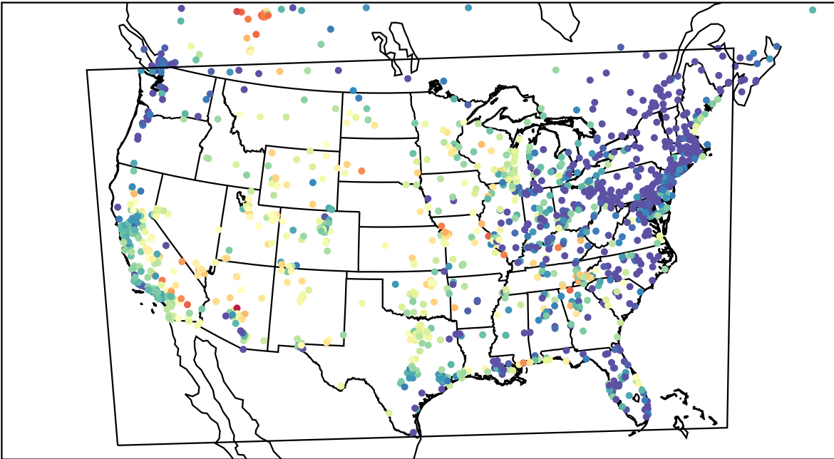
AirNOW (2023-06-10_04:00:00)
