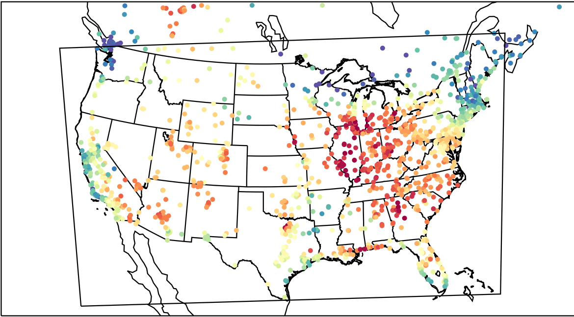
AirNOW (2023-06-10_21:00:00)
