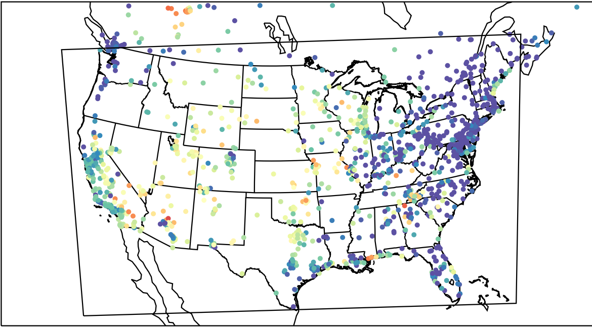
AirNOW (2023-06-10_05:00:00)
