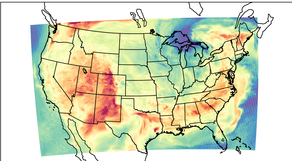
WRF (2023-06-12_22:00:00)
