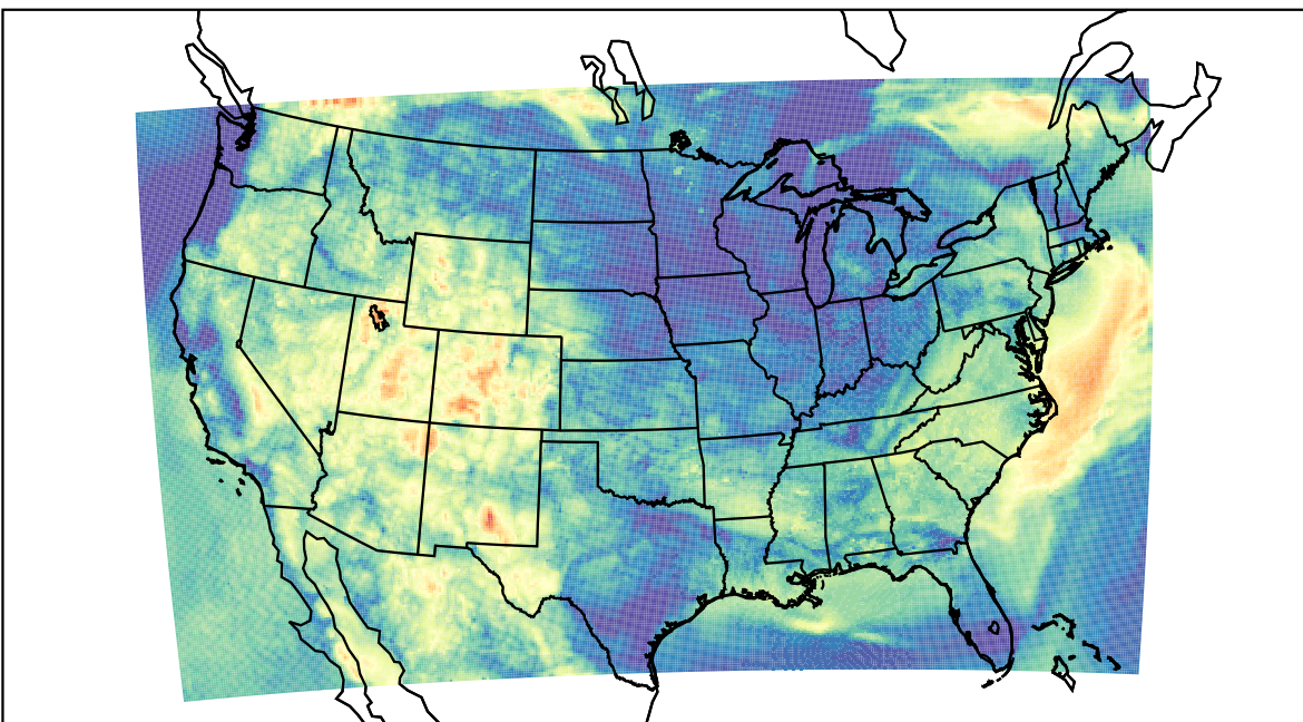
WRF (2023-06-13_13:00:00)
