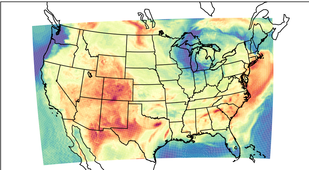
WRF (2023-06-13_19:00:00)
