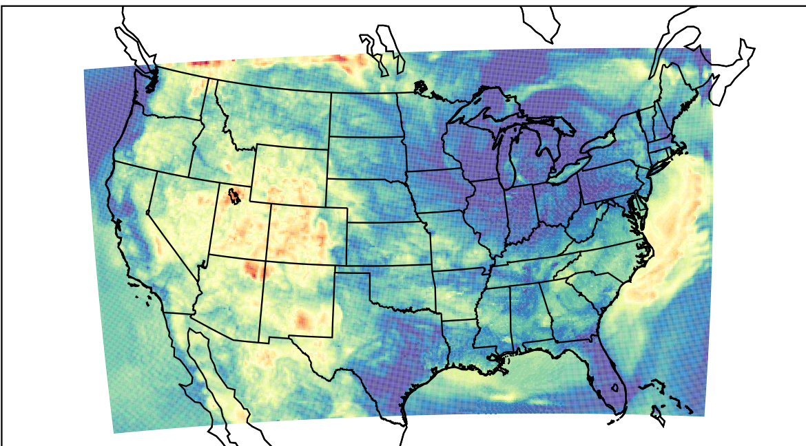
WRF (2023-06-13_10:00:00)
