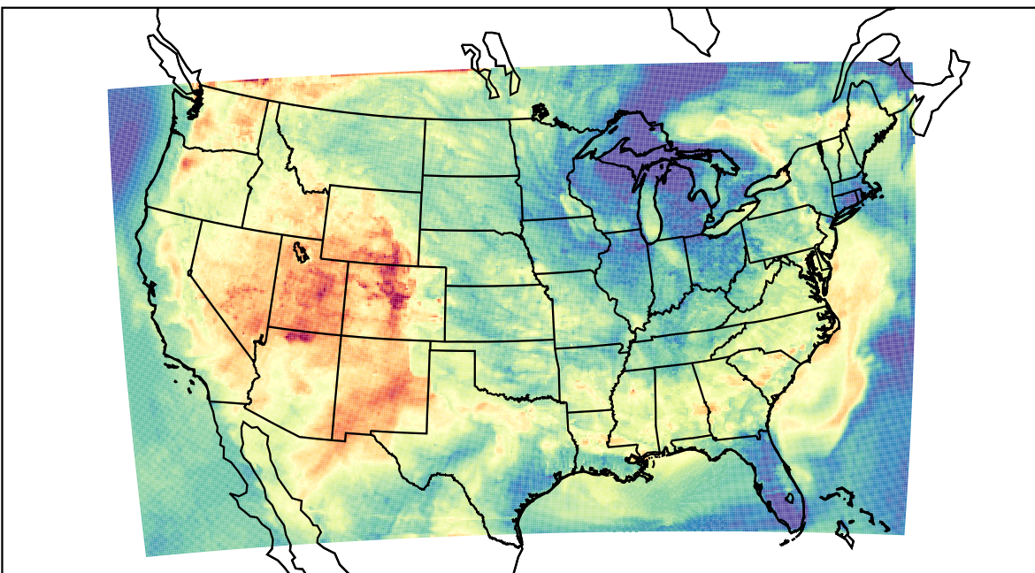
WRF (2023-06-13_02:00:00)
