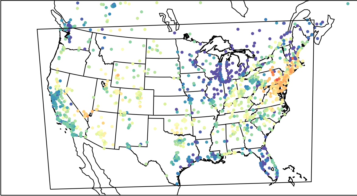
AirNOW (2023-06-12_03:00:00)
