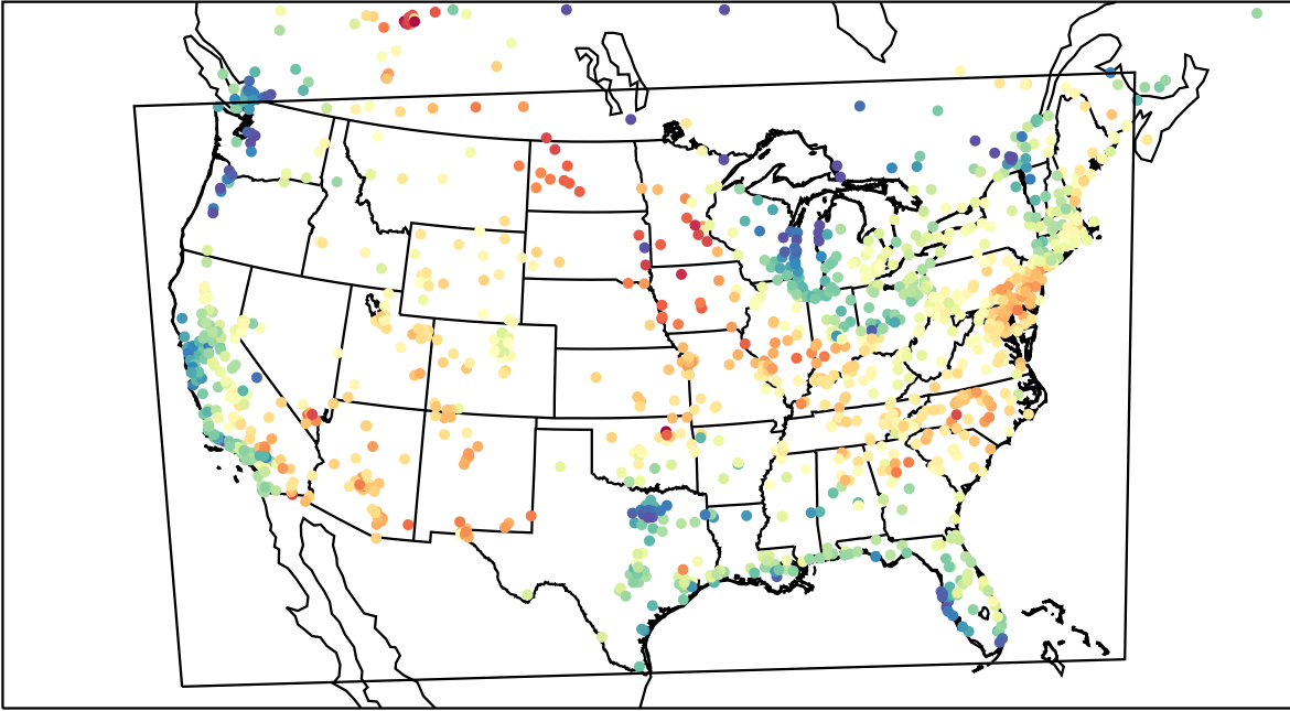
AirNOW (2023-06-13_19:00:00)
