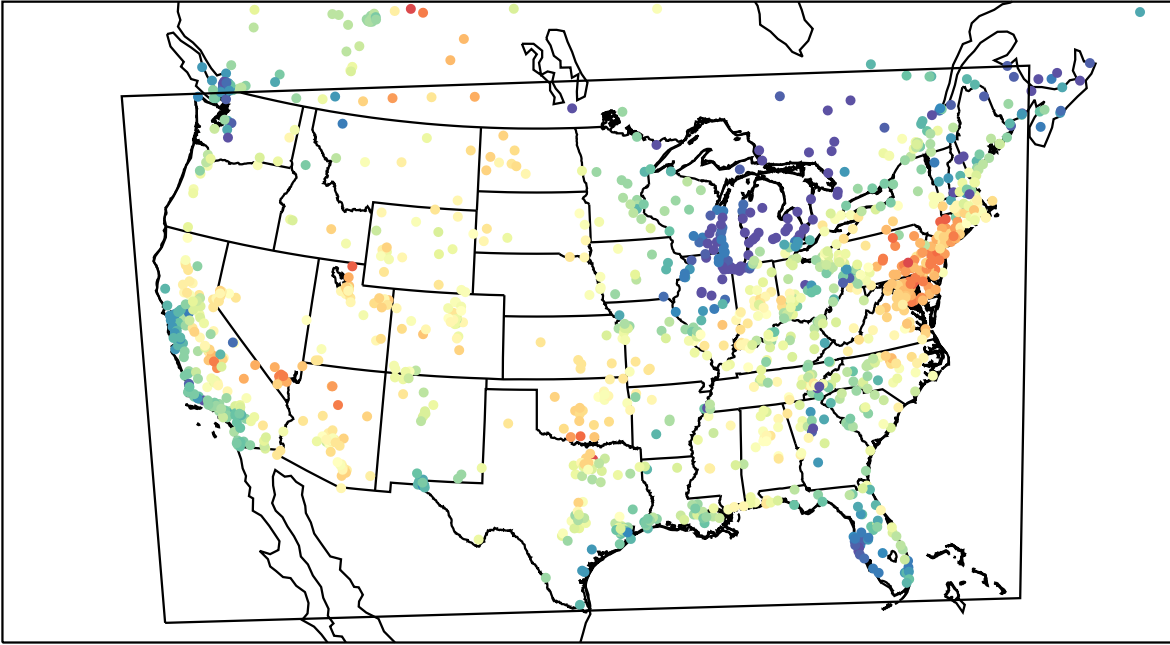
AirNOW (2023-06-12_00:00:00)
