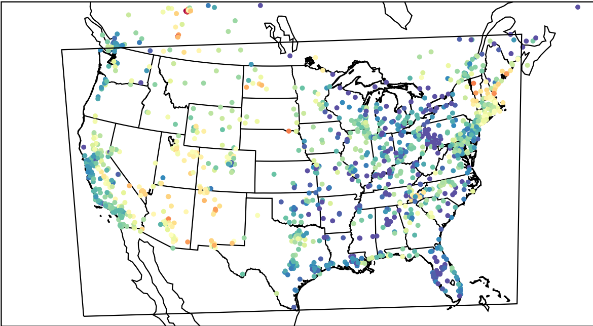
AirNOW (2023-06-13_03:00:00)
