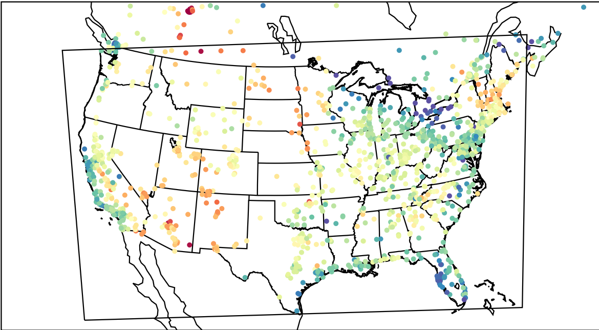
AirNOW (2023-06-13_00:00:00)
