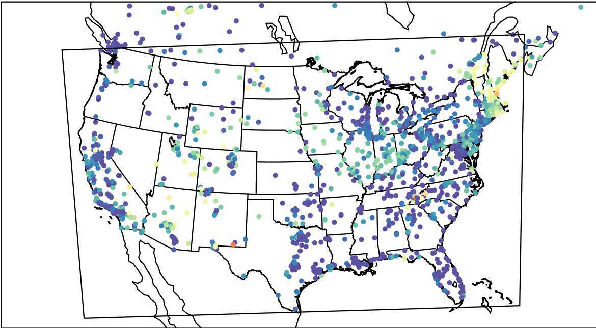
AirNOW (2023-06-13_11:00:00)
