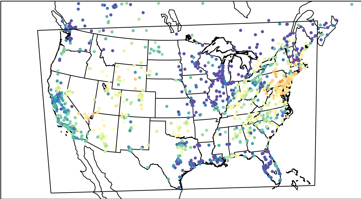
AirNOW (2023-06-12_05:00:00)
