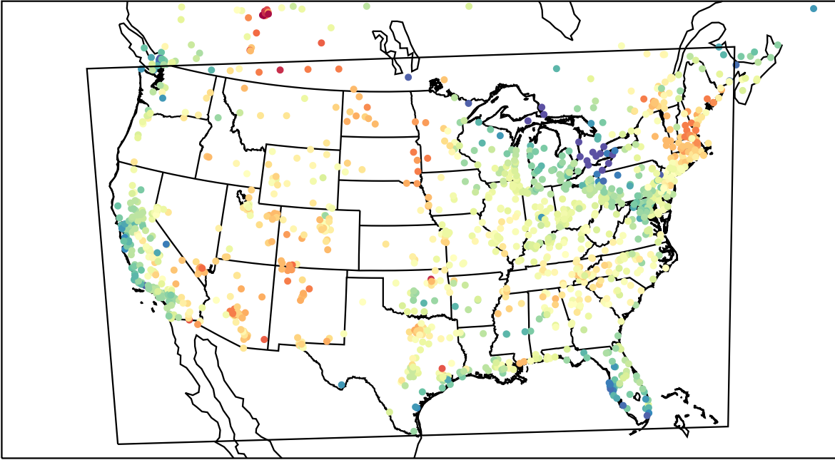
AirNOW (2023-06-12_21:00:00)
