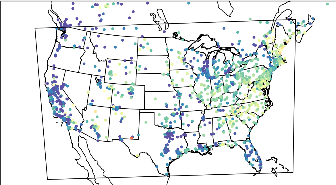
AirNOW (2023-06-13_13:00:00)
