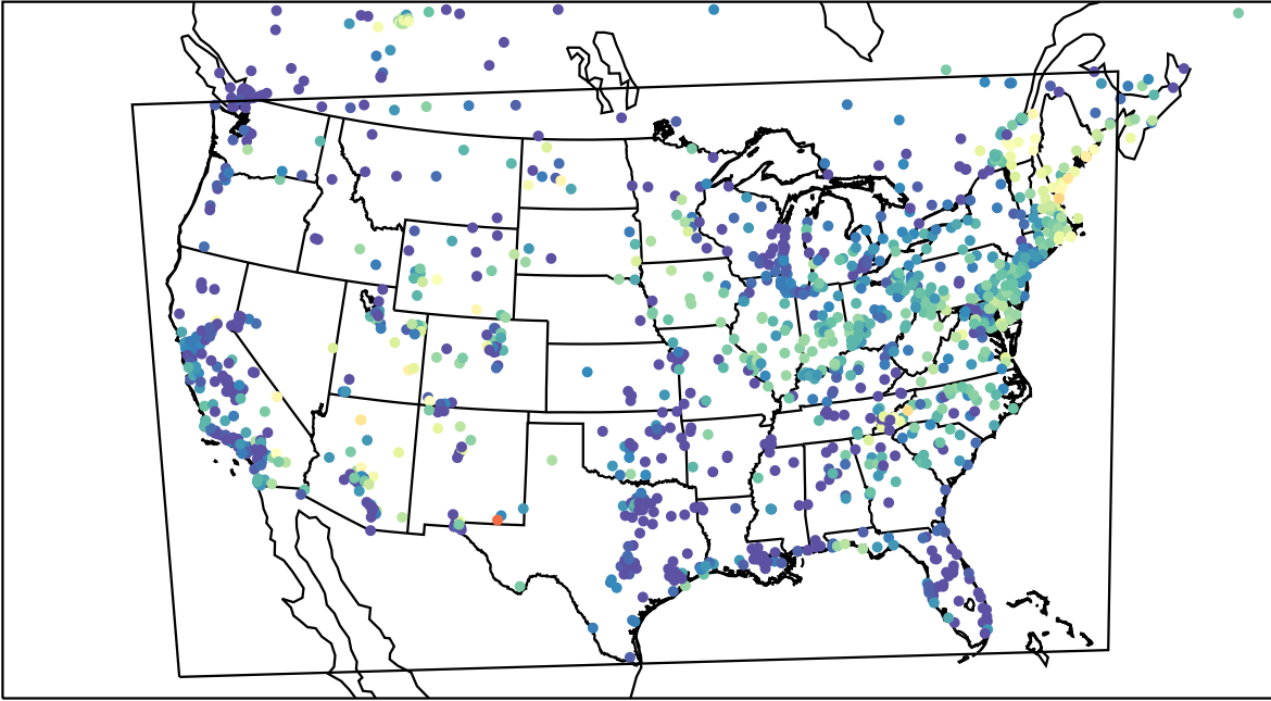
AirNOW (2023-06-13_12:00:00)
