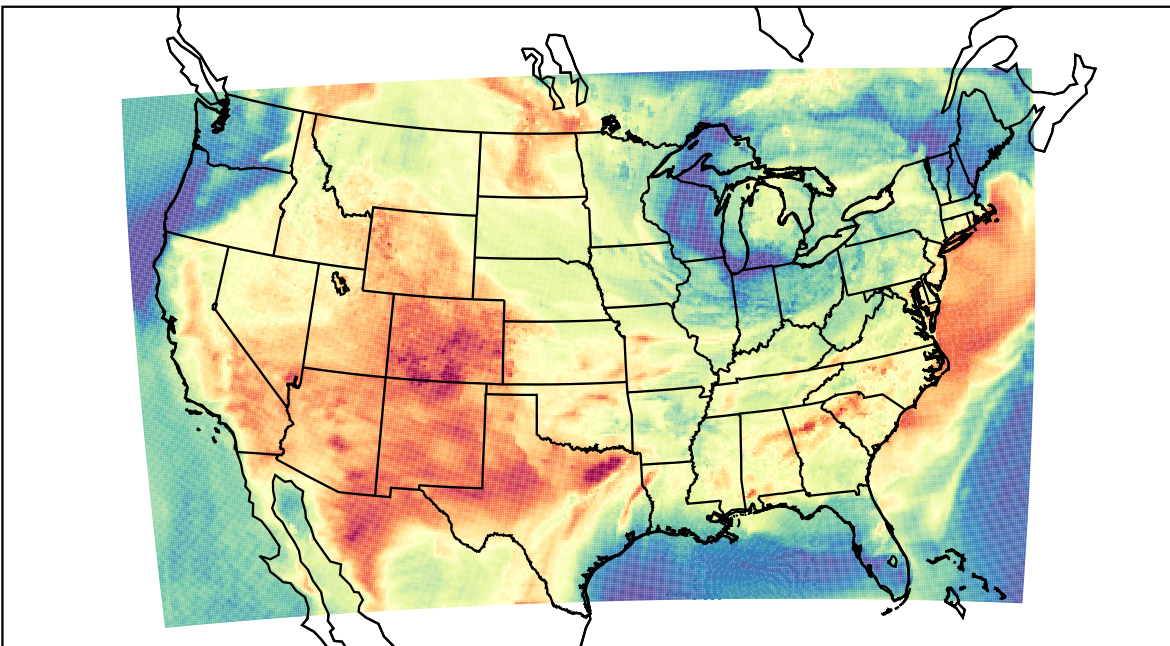
WRF (2023-06-13_23:00:00)
