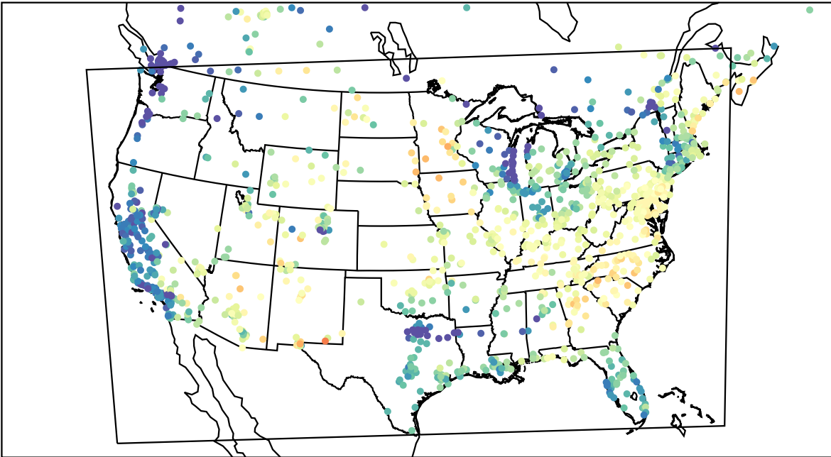
AirNOW (2023-06-13_15:00:00)
