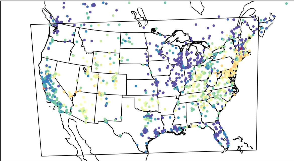
AirNOW (2023-06-12_06:00:00)
