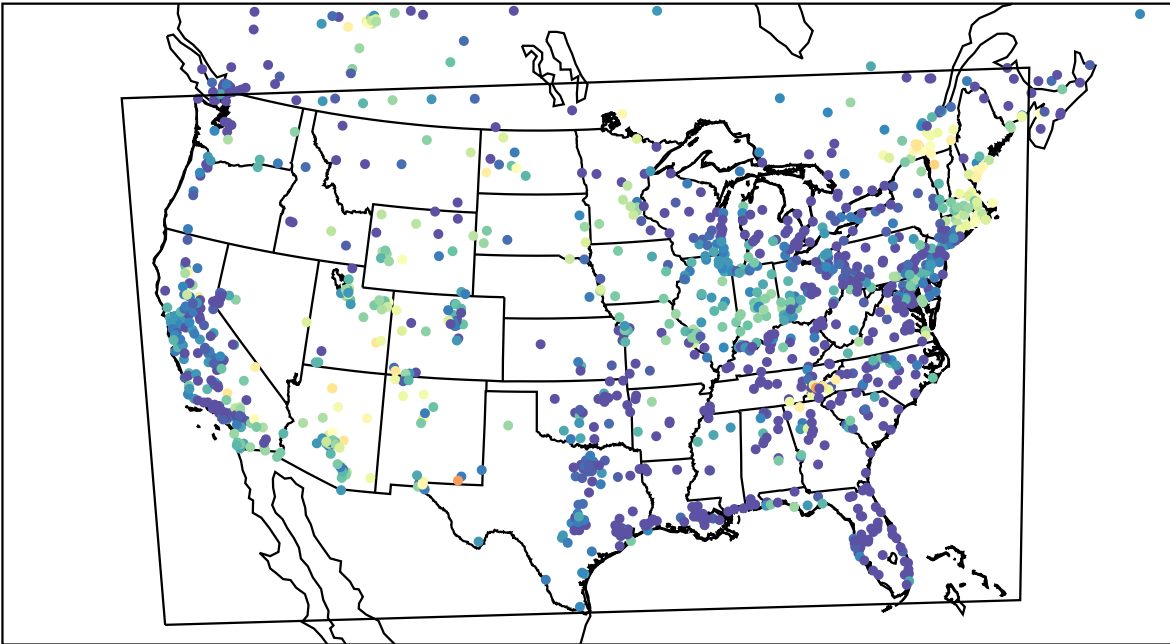
AirNOW (2023-06-13_09:00:00)
