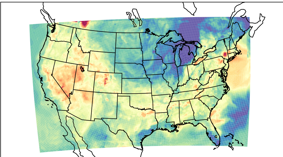
WRF (2023-06-12_02:00:00)
