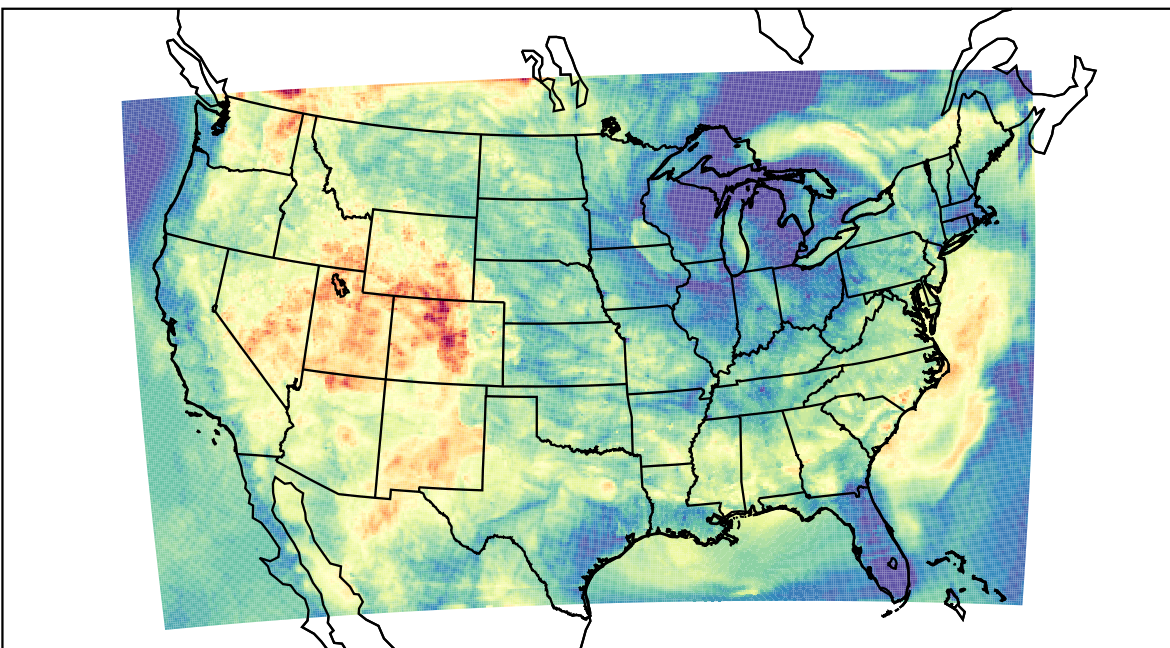
WRF (2023-06-13_04:00:00)
