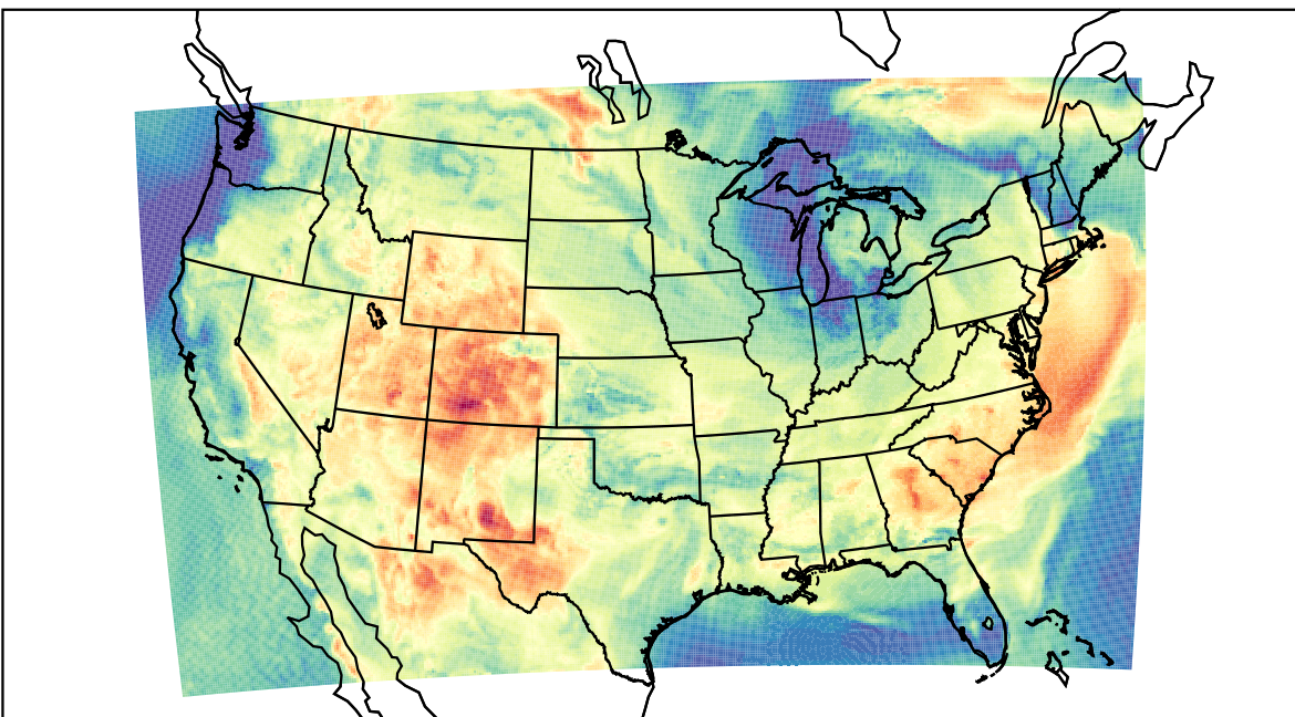
WRF (2023-06-13_16:00:00)
