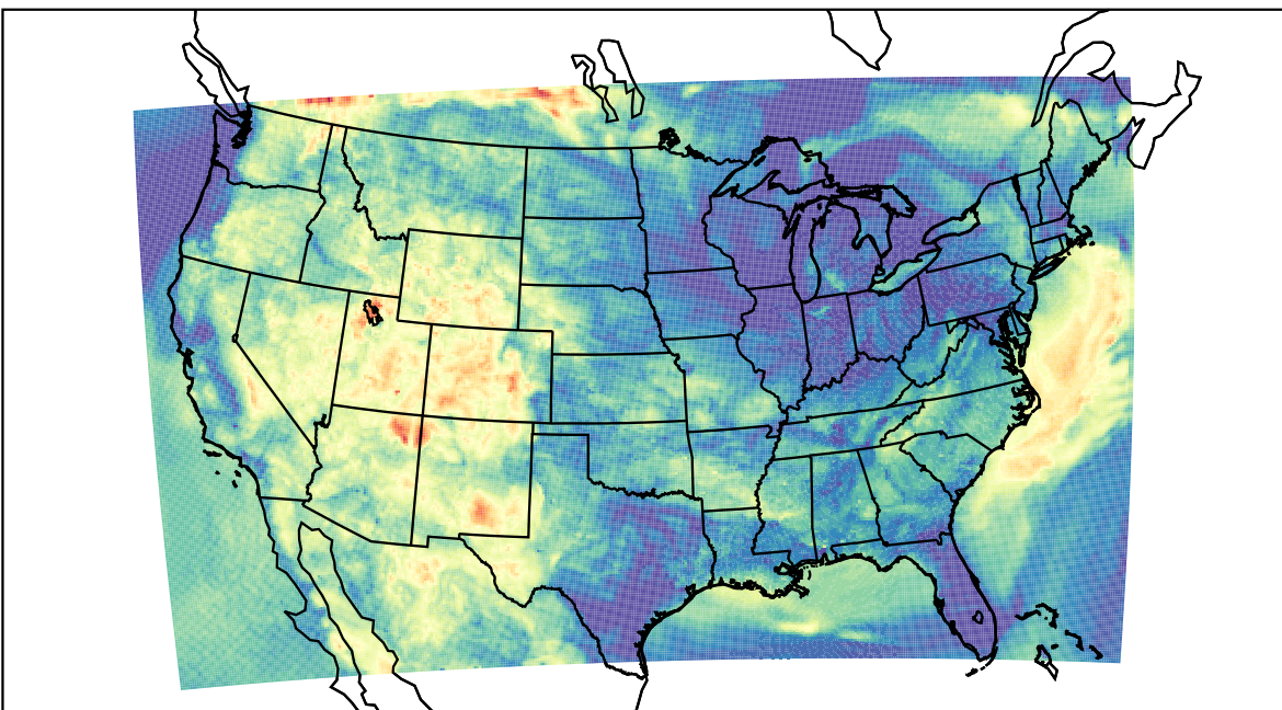
WRF (2023-06-13_11:00:00)
