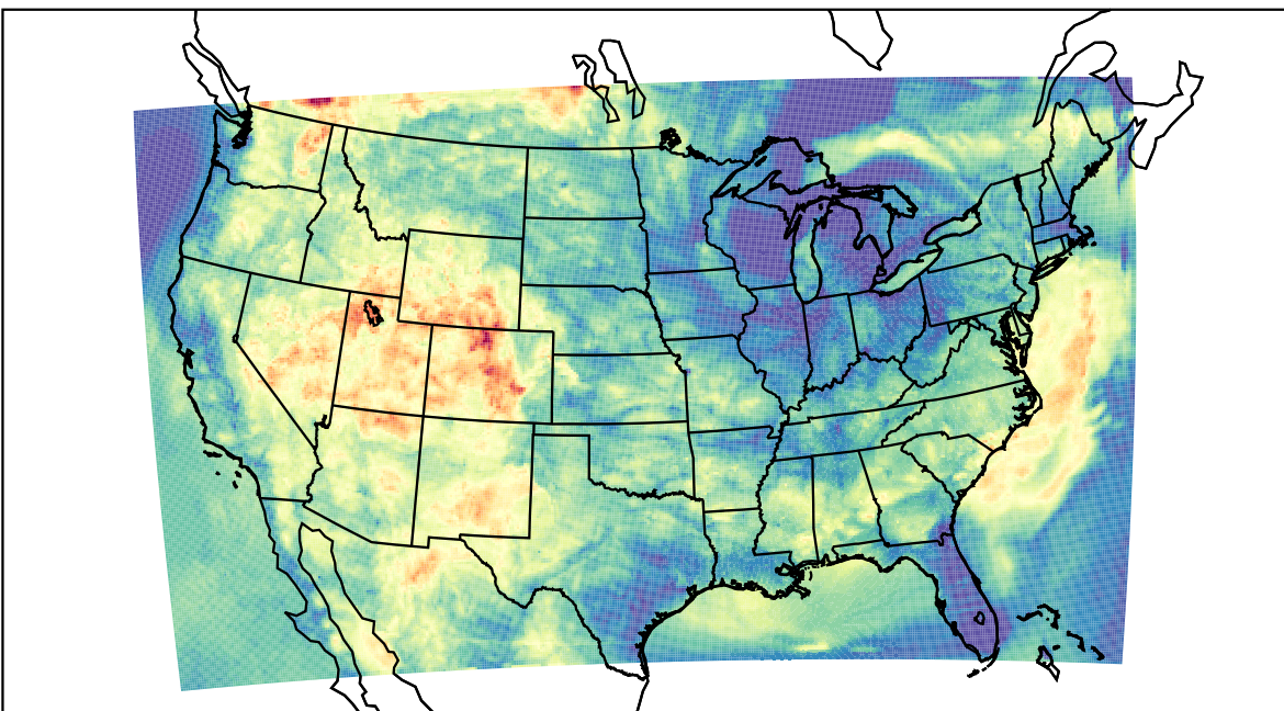
WRF (2023-06-13_06:00:00)
