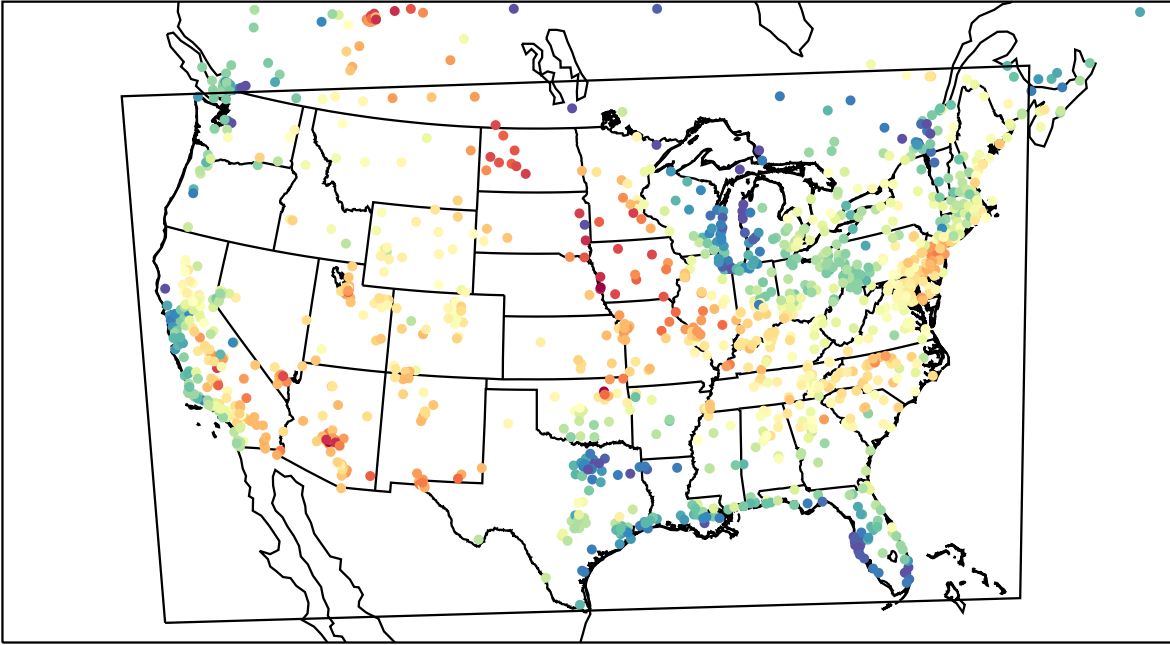
AirNOW (2023-06-13_23:00:00)
