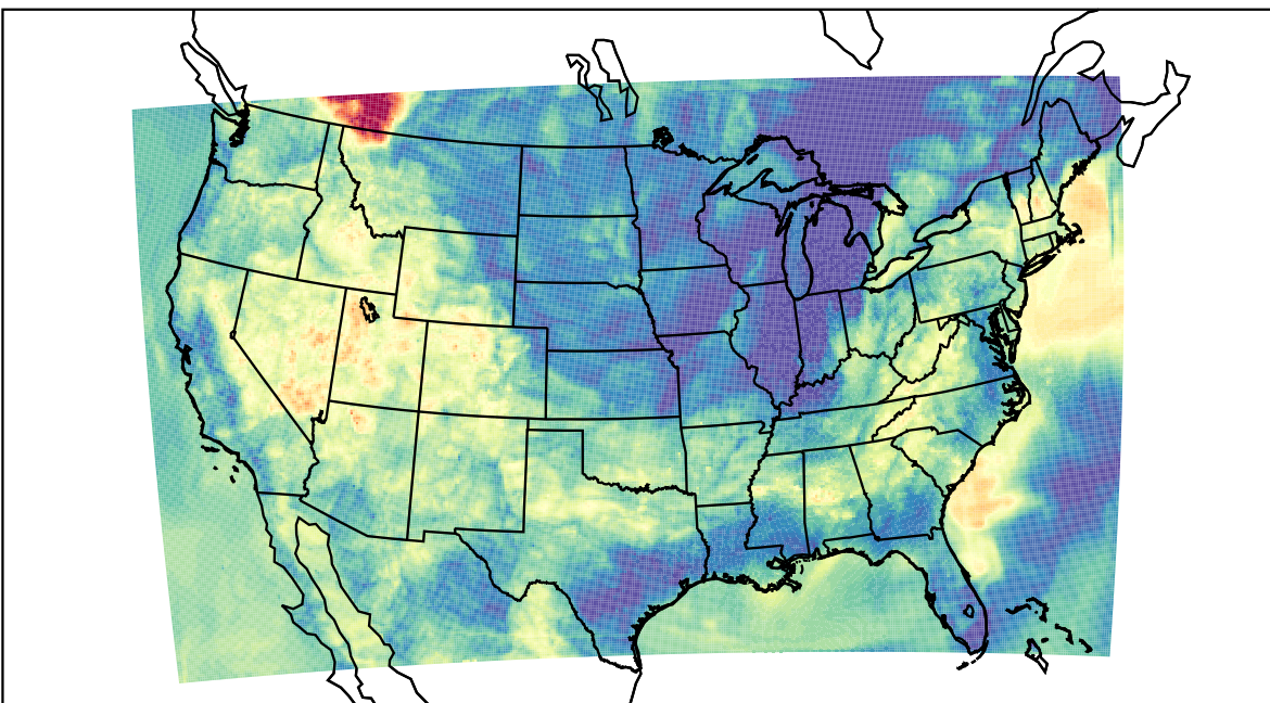
WRF (2023-06-12_08:00:00)
