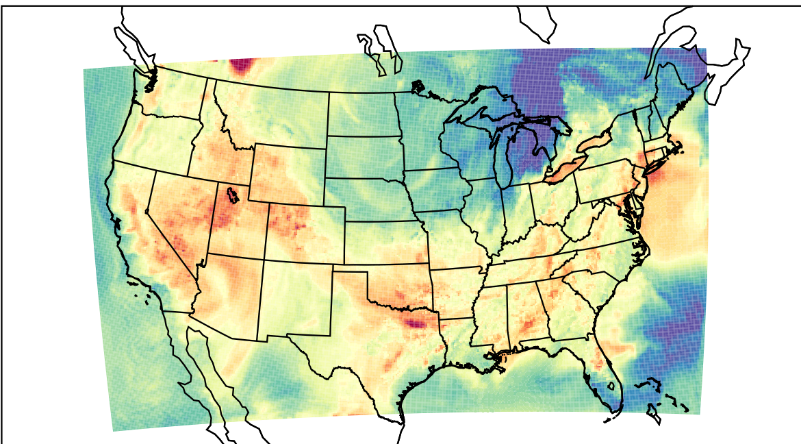
WRF (2023-06-12_00:00:00)
