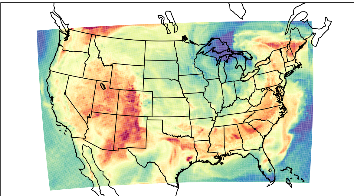
WRF (2023-06-12_21:00:00)
