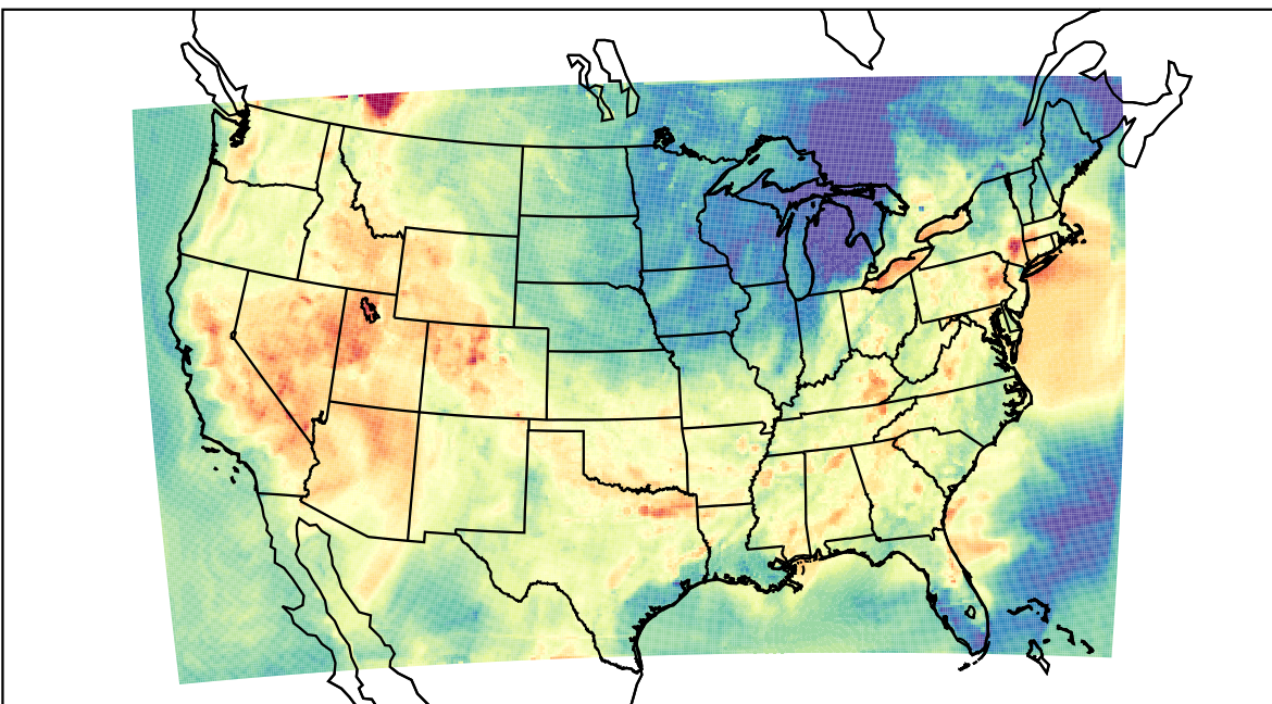
WRF (2023-06-12_01:00:00)
