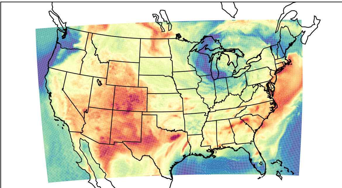
WRF (2023-06-13_21:00:00)
