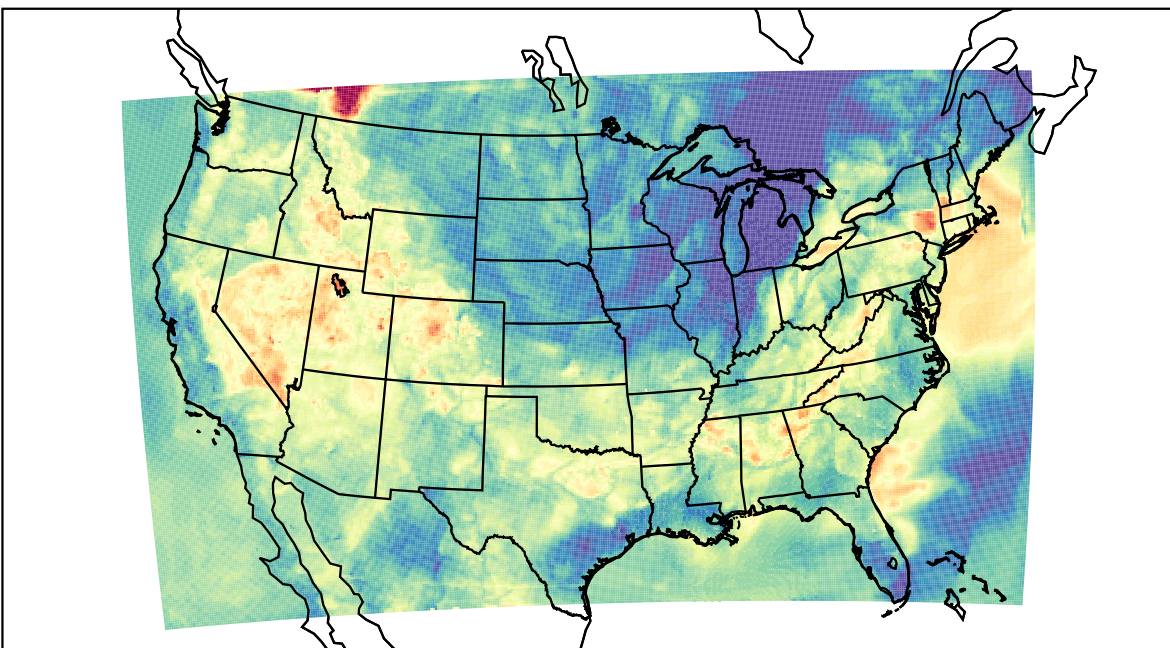
WRF (2023-06-12_04:00:00)
