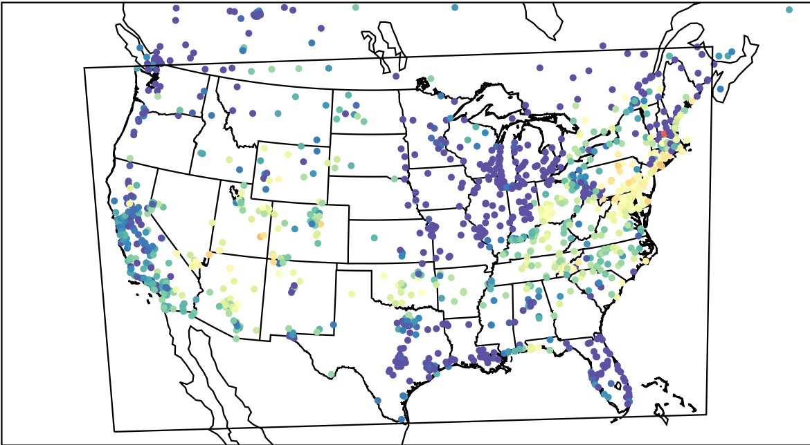
AirNOW (2023-06-12_09:00:00)
