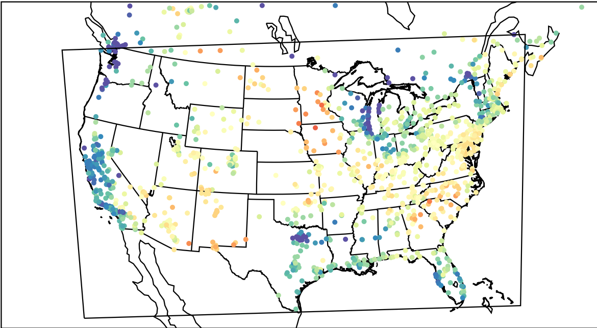
AirNOW (2023-06-13_16:00:00)
