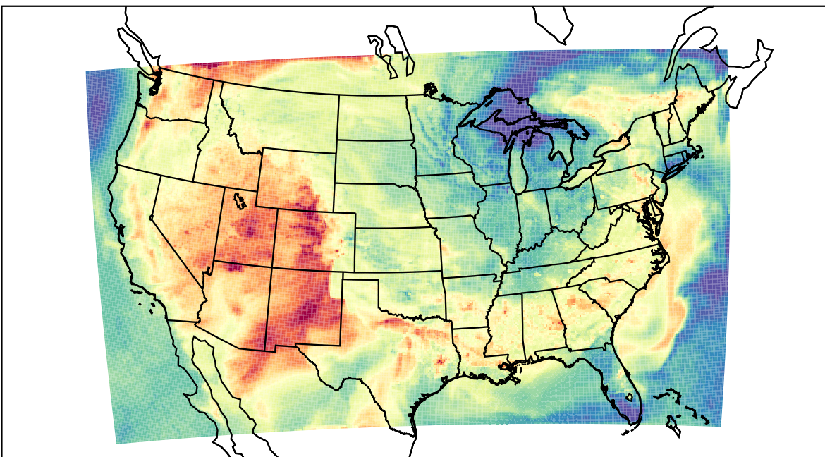
WRF (2023-06-13_00:00:00)
