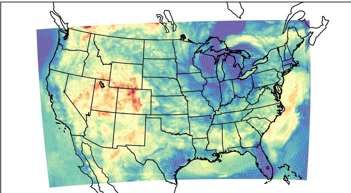
WRF (2023-06-13_05:00:00)
