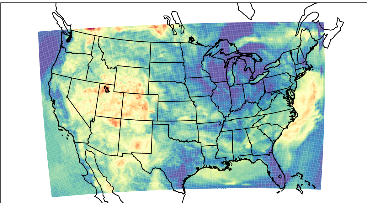
WRF (2023-06-13_08:00:00)
