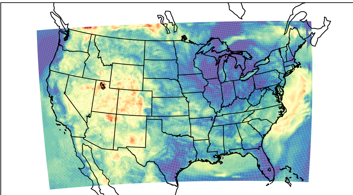
WRF (2023-06-13_09:00:00)
