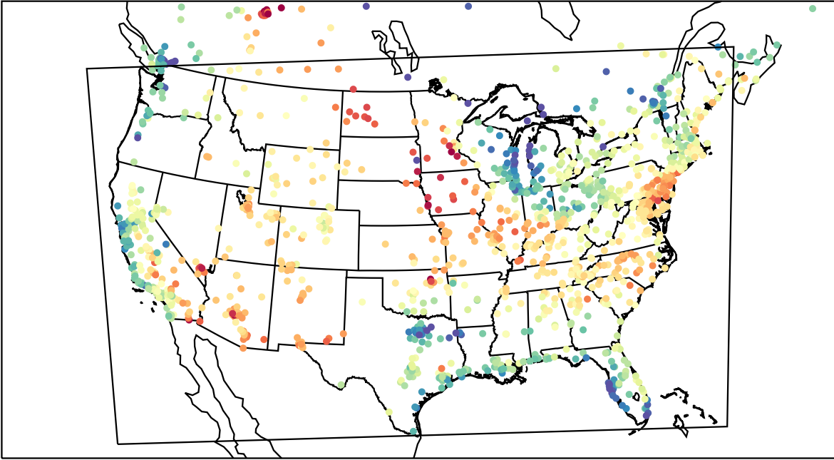
AirNOW (2023-06-13_21:00:00)
