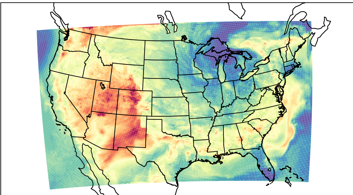
WRF (2023-06-13_01:00:00)
