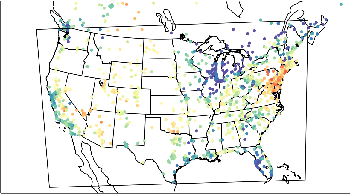
AirNOW (2023-06-12_01:00:00)
