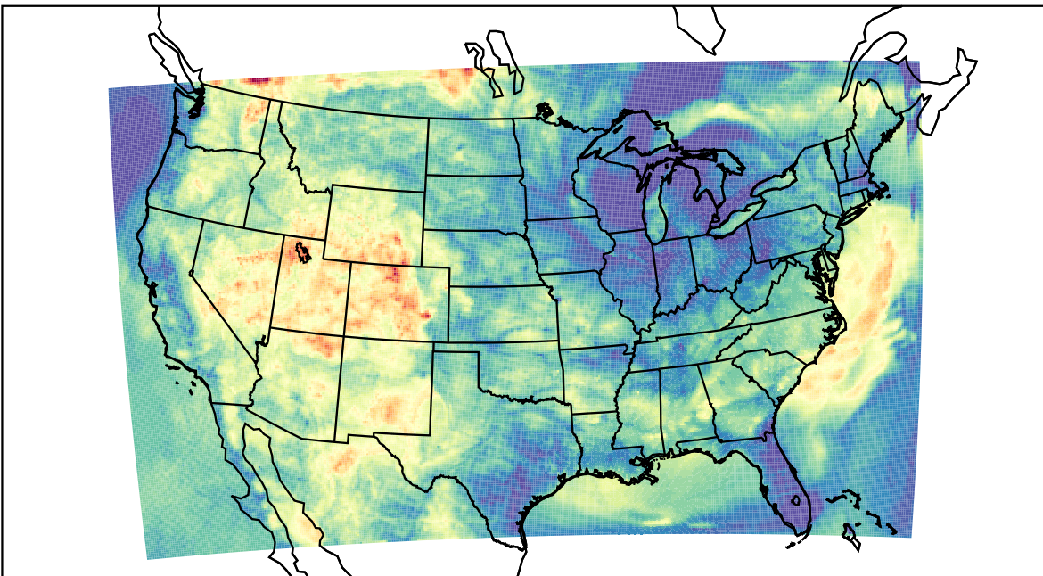
WRF (2023-06-13_07:00:00)
