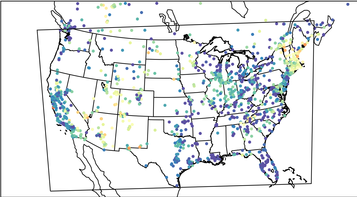
AirNOW (2023-06-13_06:00:00)
