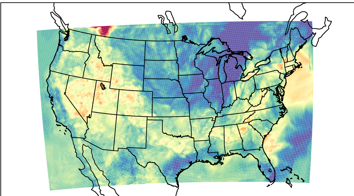
WRF (2023-06-12_05:00:00)
