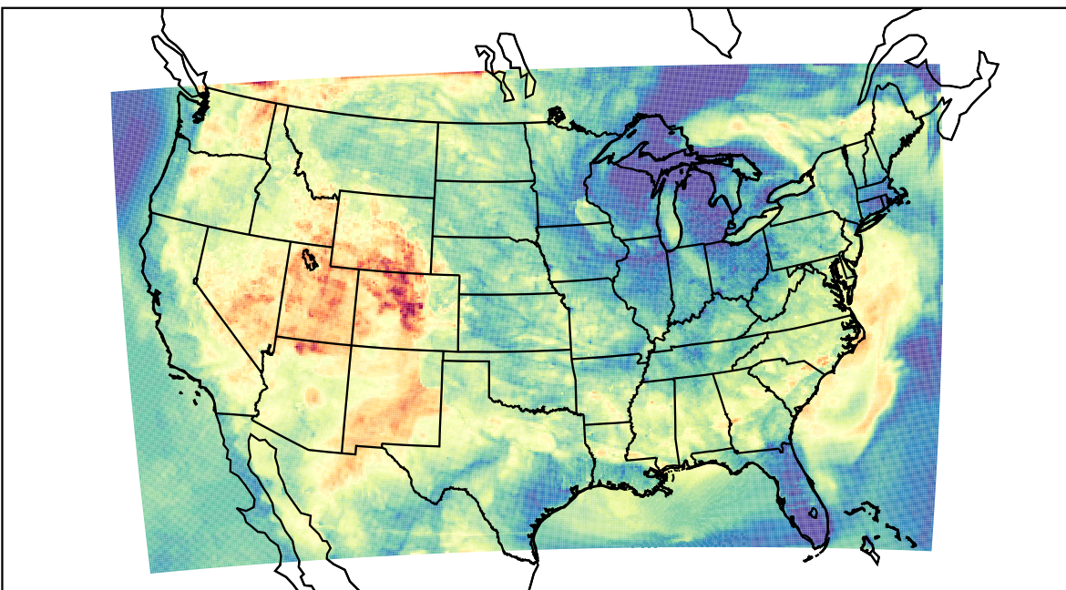
WRF (2023-06-13_03:00:00)
