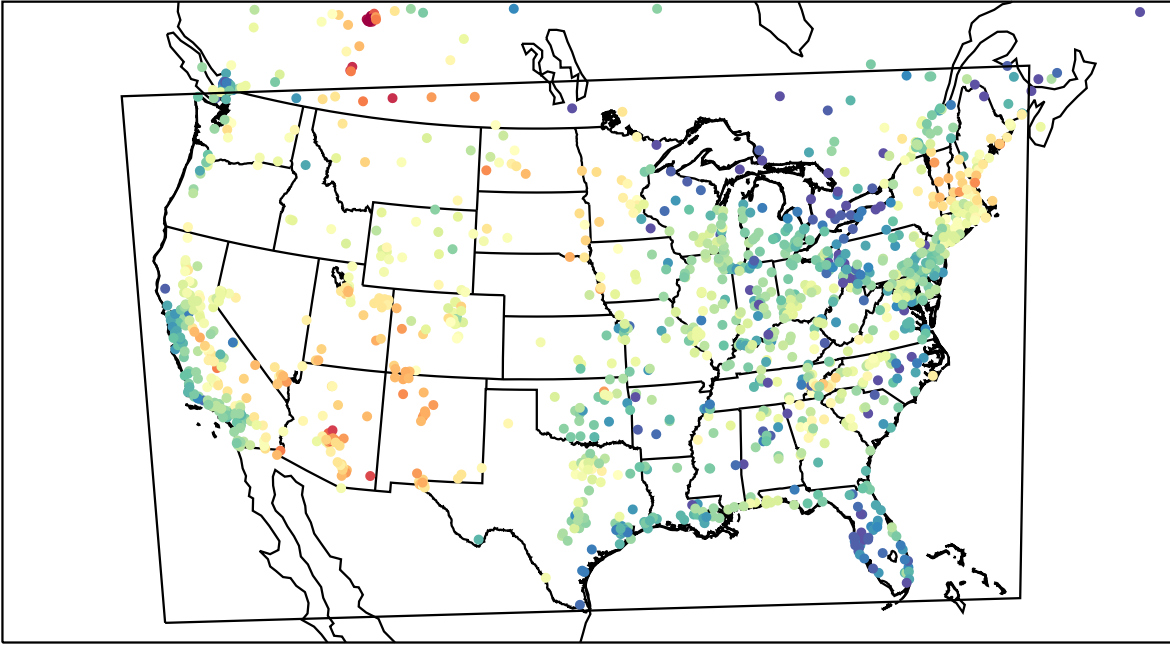
AirNOW (2023-06-13_01:00:00)
