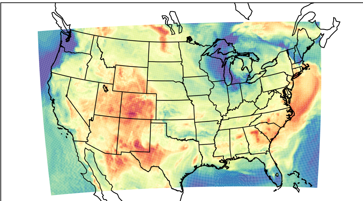
WRF (2023-06-13_17:00:00)
