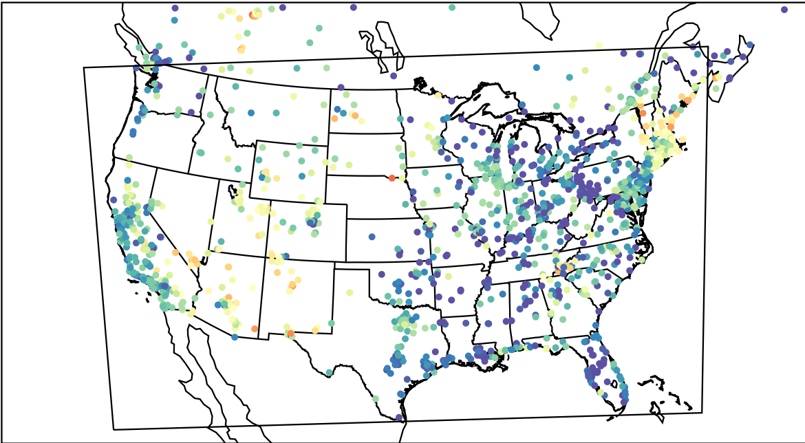
AirNOW (2023-06-13_04:00:00)
