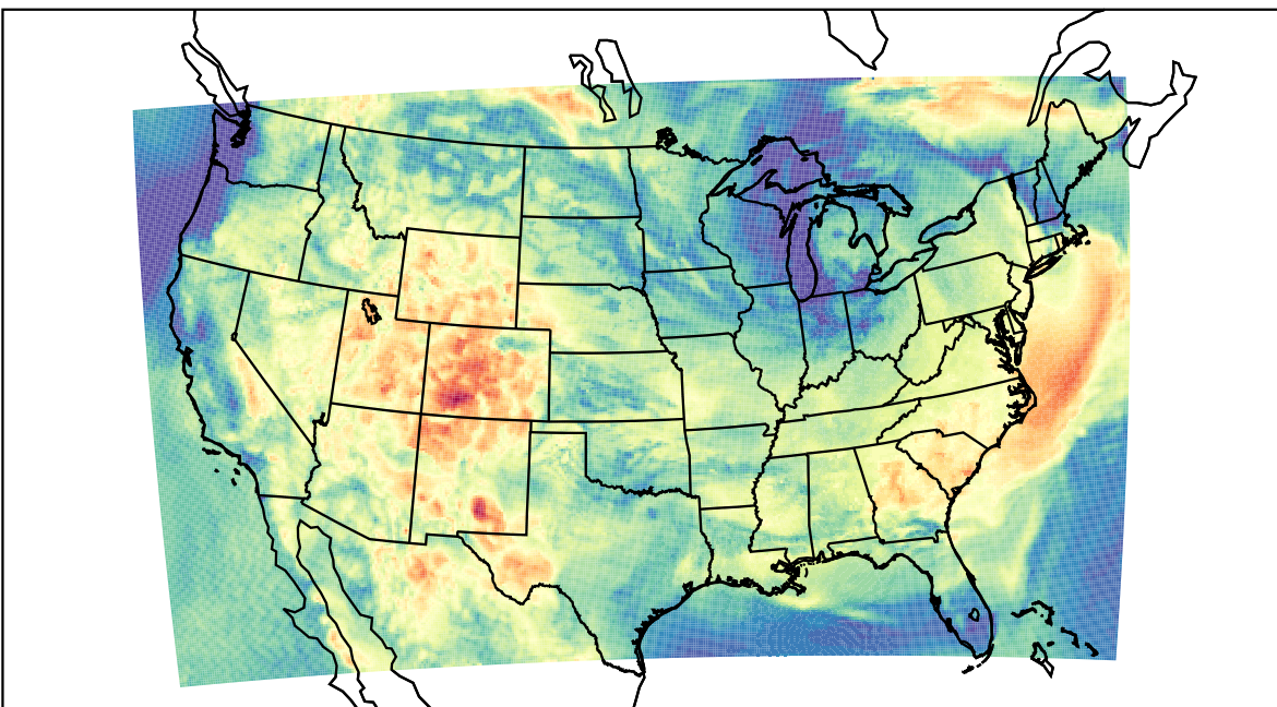
WRF (2023-06-13_15:00:00)
