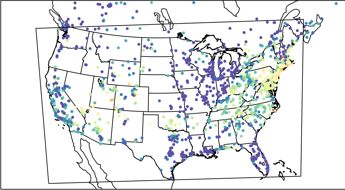
AirNOW (2023-06-12_11:00:00)
