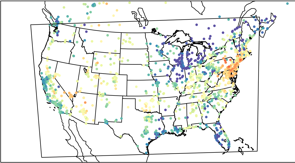
AirNOW (2023-06-12_02:00:00)
