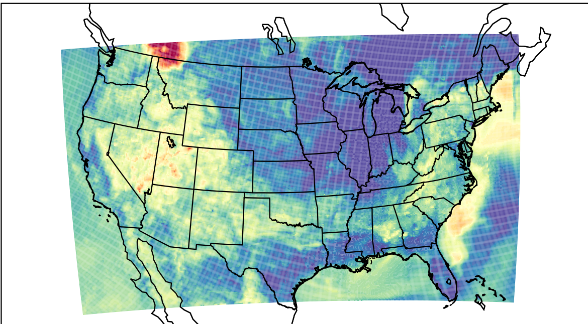
WRF (2023-06-12_11:00:00)
