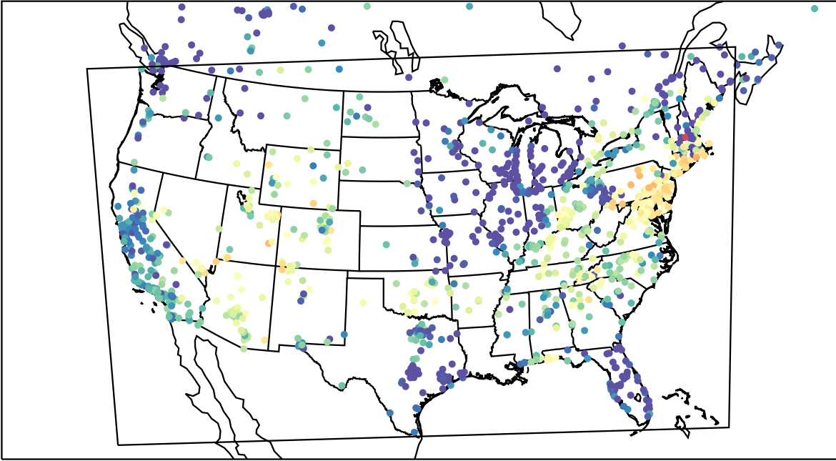
AirNOW (2023-06-12_07:00:00)
