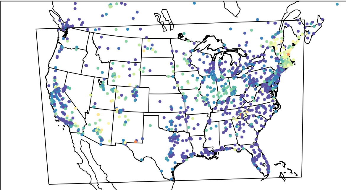
AirNOW (2023-06-13_10:00:00)
