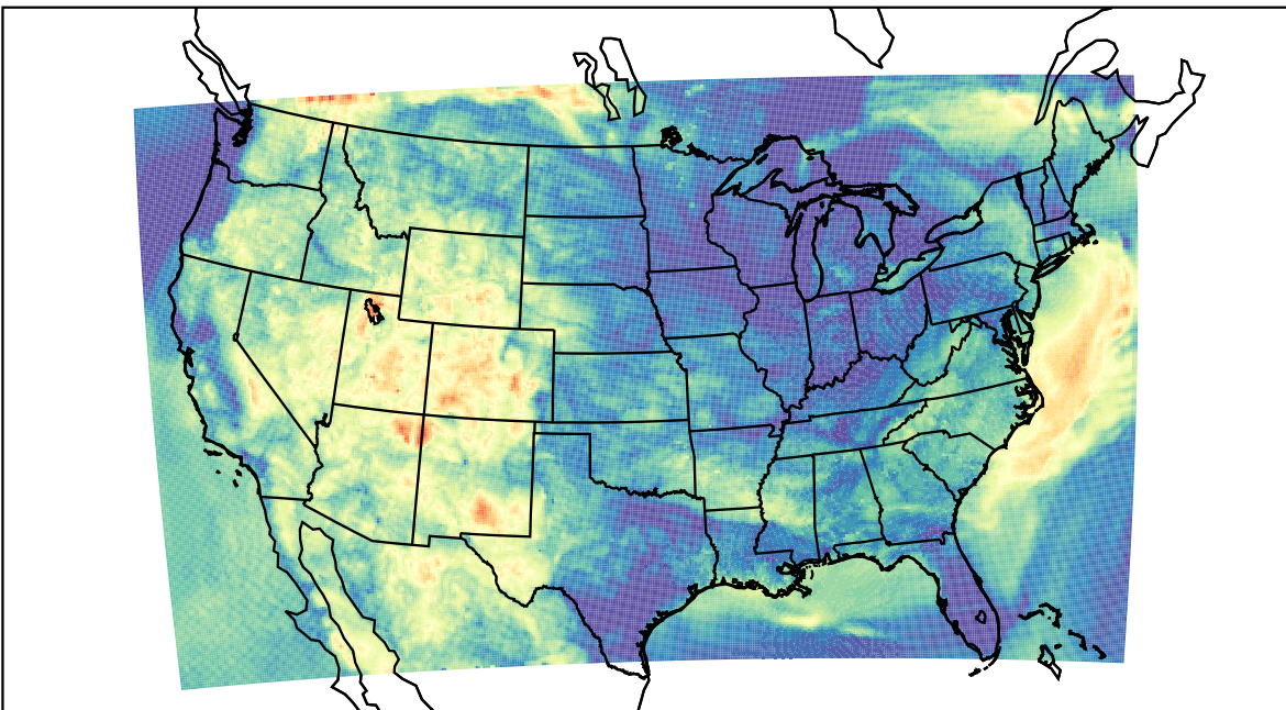
WRF (2023-06-13_12:00:00)
