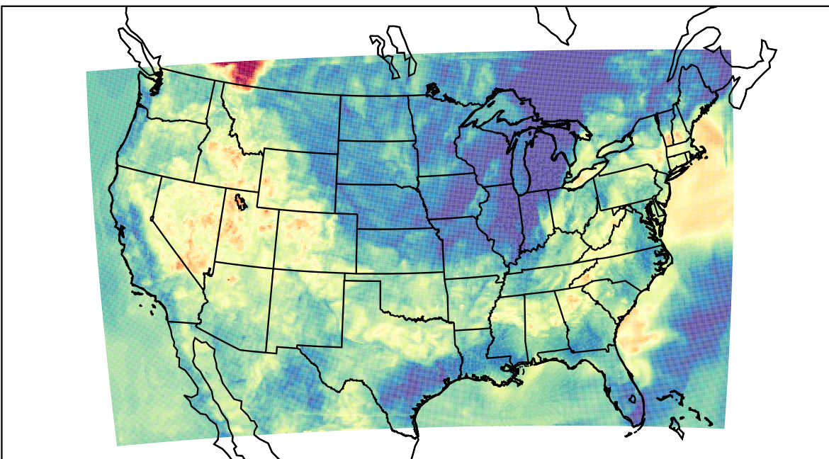
WRF (2023-06-12_06:00:00)
