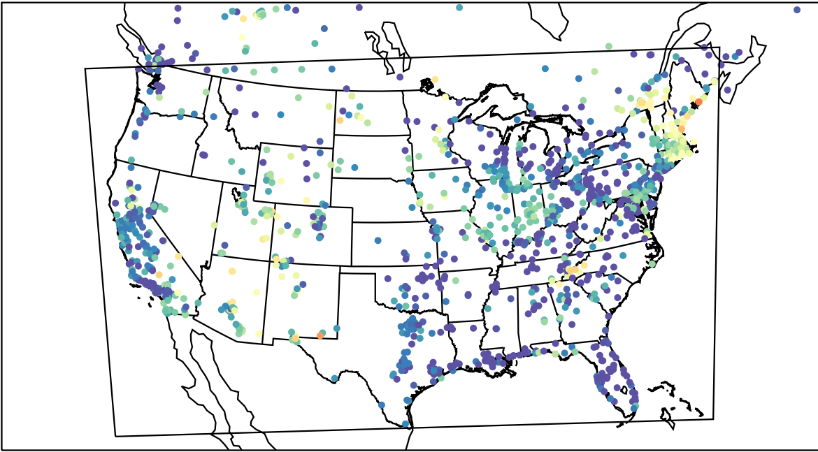
AirNOW (2023-06-13_08:00:00)
