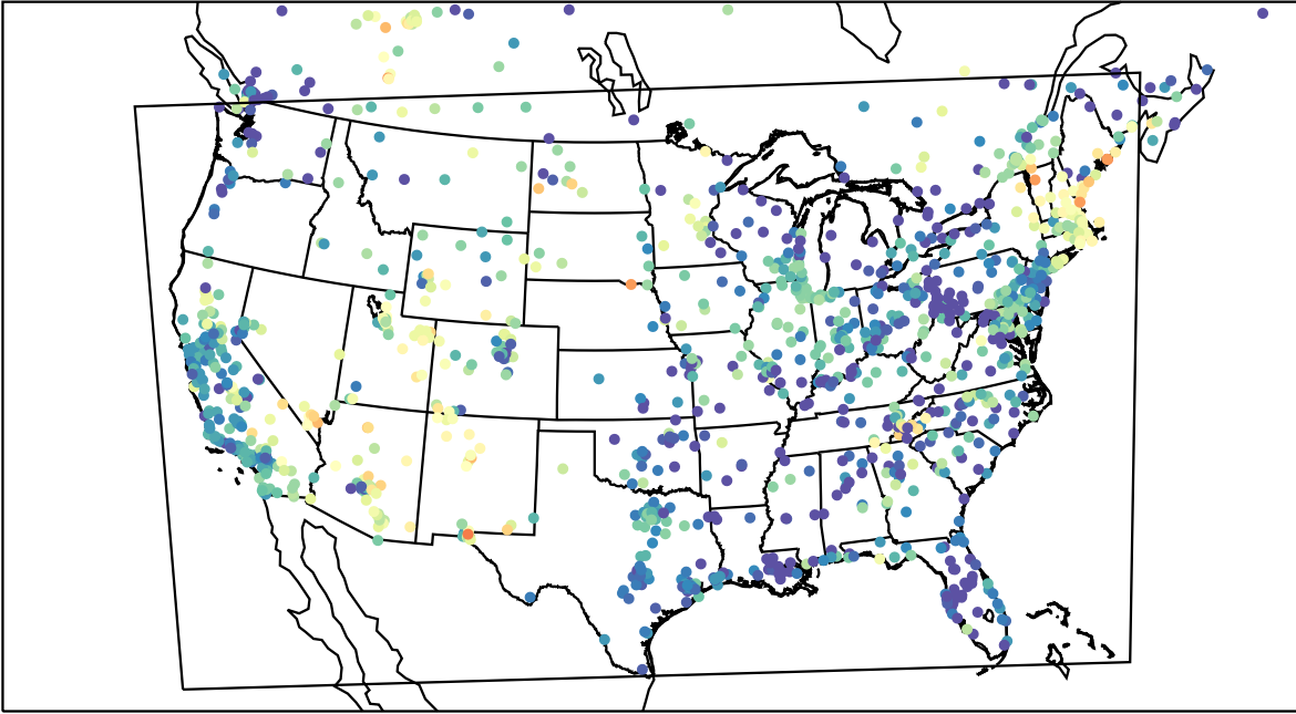
AirNOW (2023-06-13_05:00:00)
