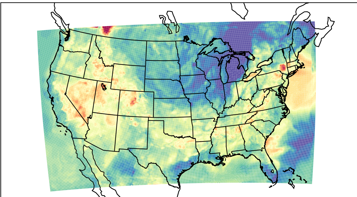
WRF (2023-06-12_03:00:00)
