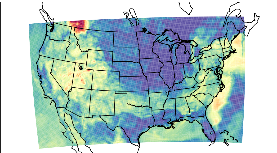
WRF (2023-06-12_12:00:00)
