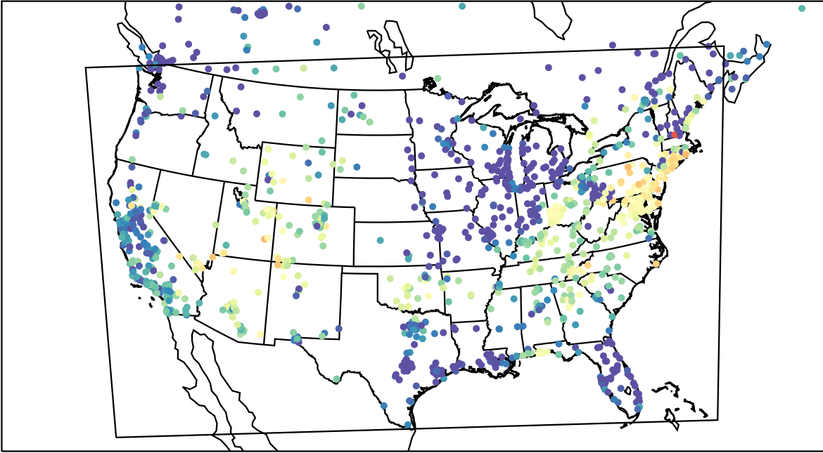
AirNOW (2023-06-12_08:00:00)
