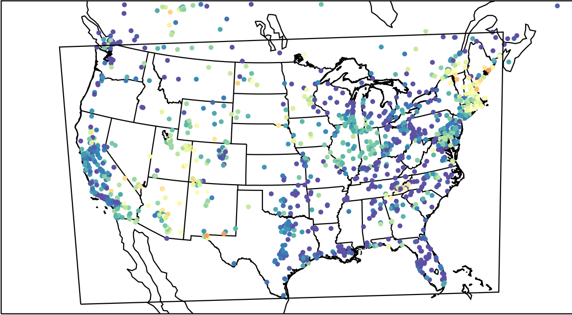
AirNOW (2023-06-13_07:00:00)
