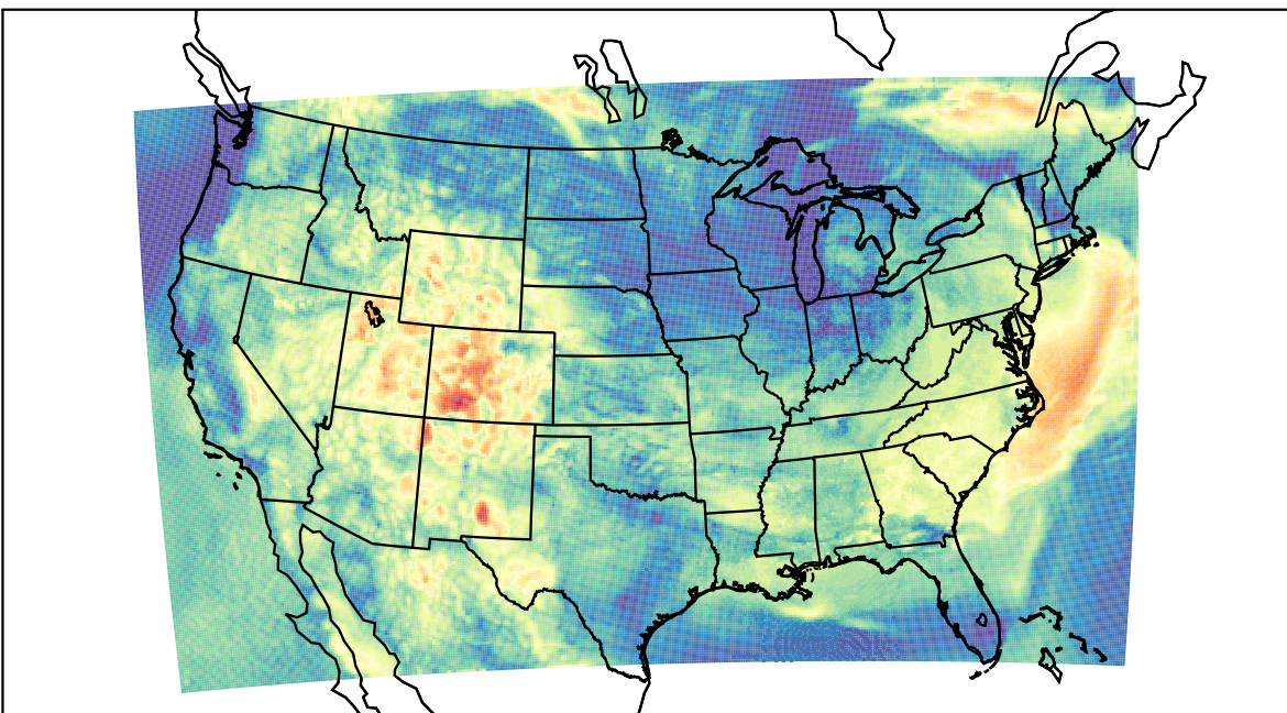
WRF (2023-06-13_14:00:00)
