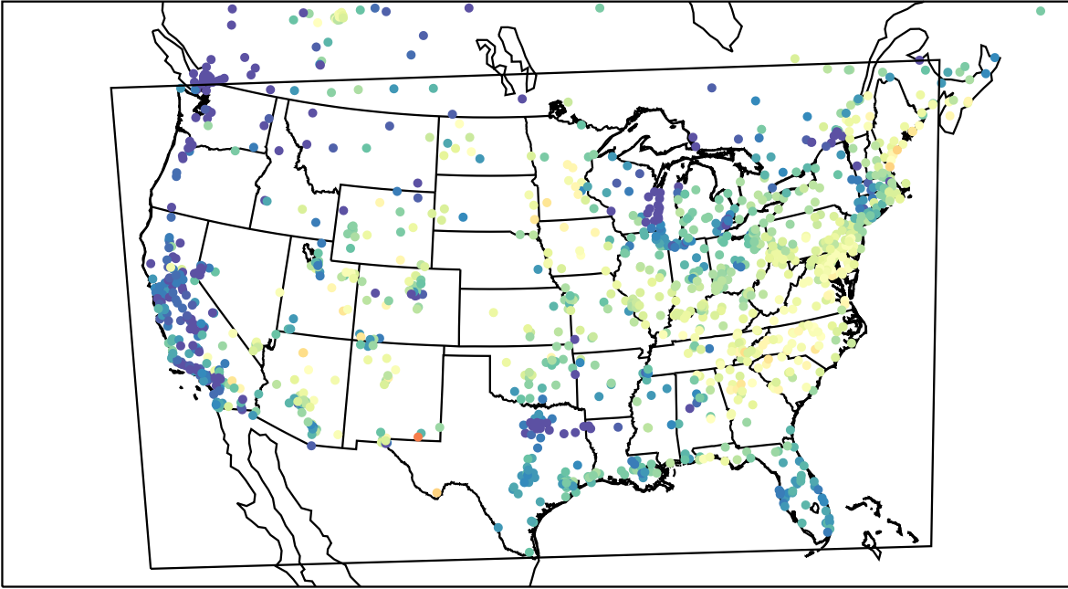
AirNOW (2023-06-13_14:00:00)
