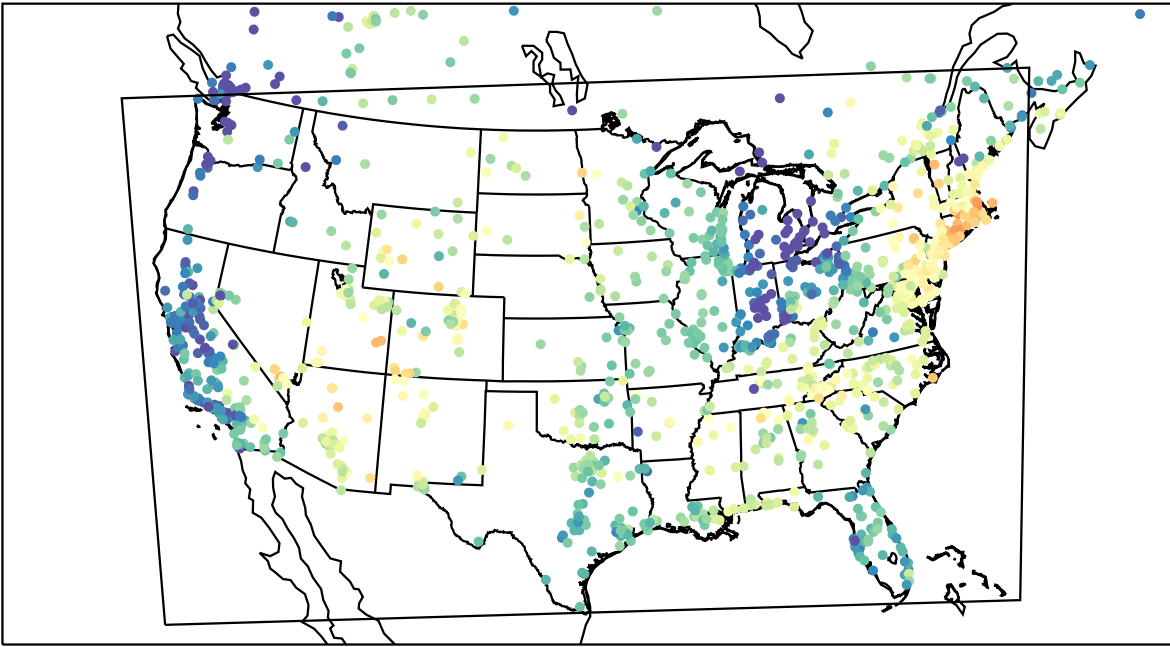
AirNOW (2023-06-12_15:00:00)
