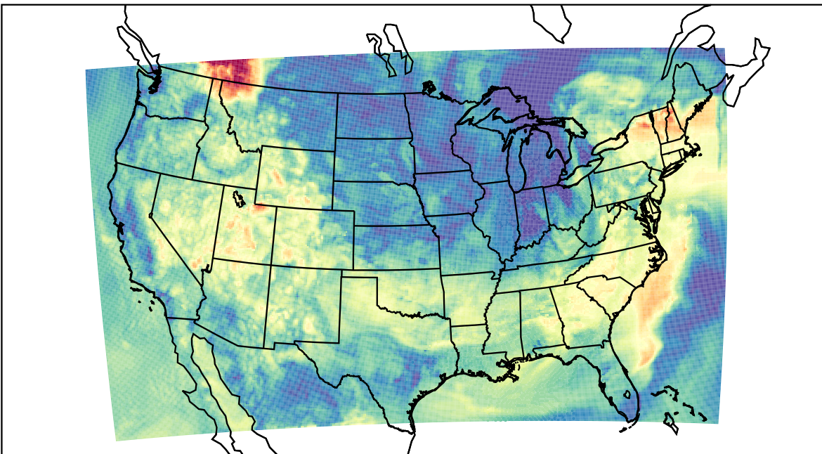
WRF (2023-06-12_14:00:00)
