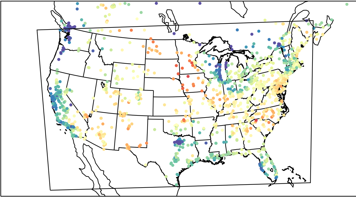
AirNOW (2023-06-13_17:00:00)
