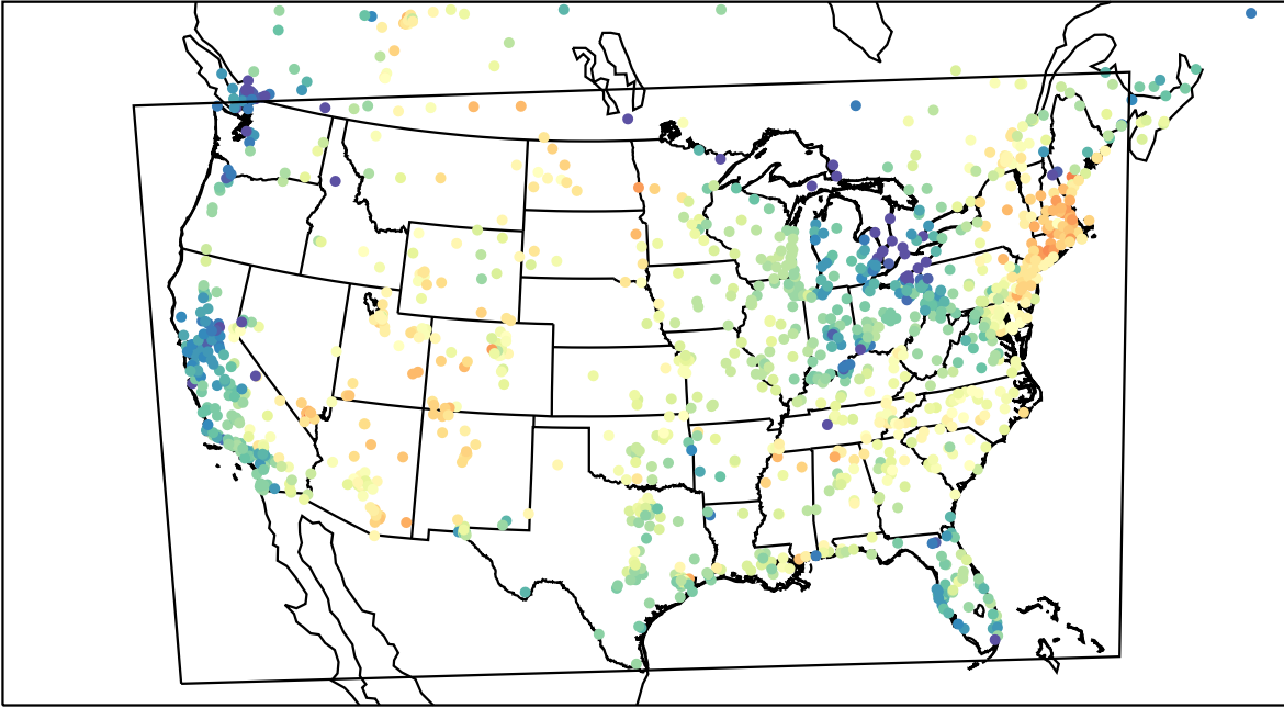
AirNOW (2023-06-12_17:00:00)
