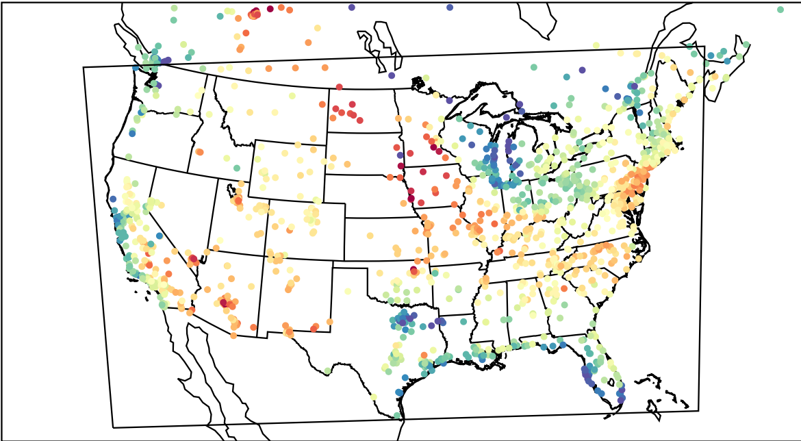
AirNOW (2023-06-13_22:00:00)
