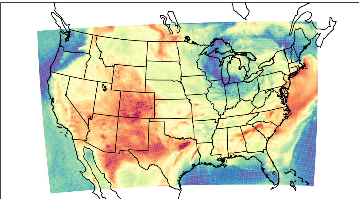
WRF (2023-06-13_22:00:00)
