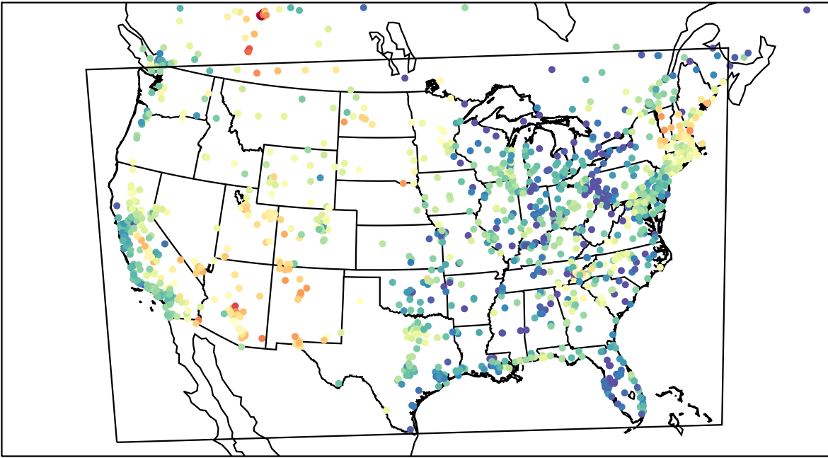
AirNOW (2023-06-13_02:00:00)
