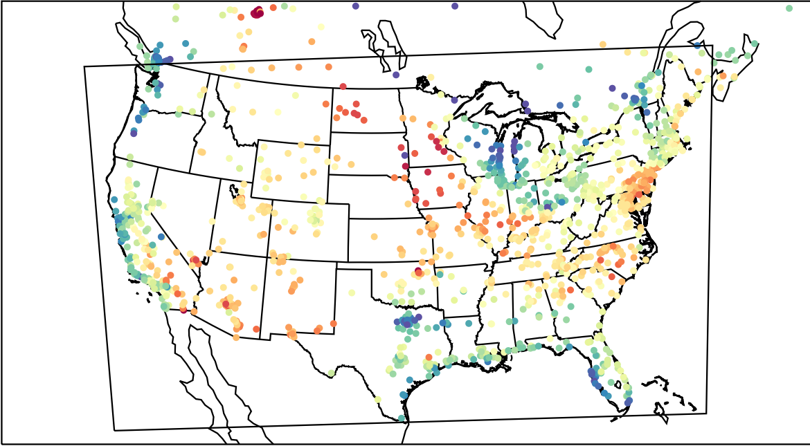
AirNOW (2023-06-13_20:00:00)
