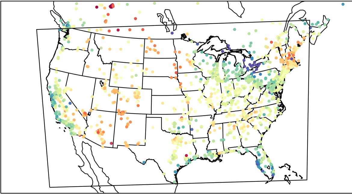
AirNOW (2023-06-12_22:00:00)
