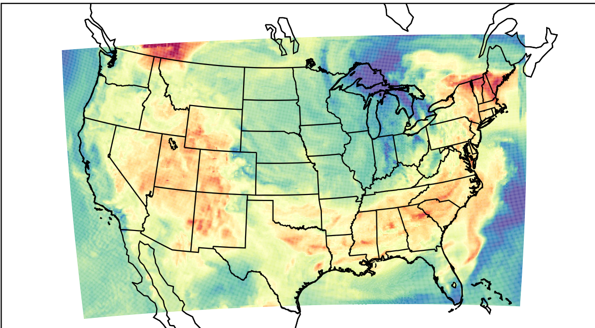
WRF (2023-06-12_17:00:00)
