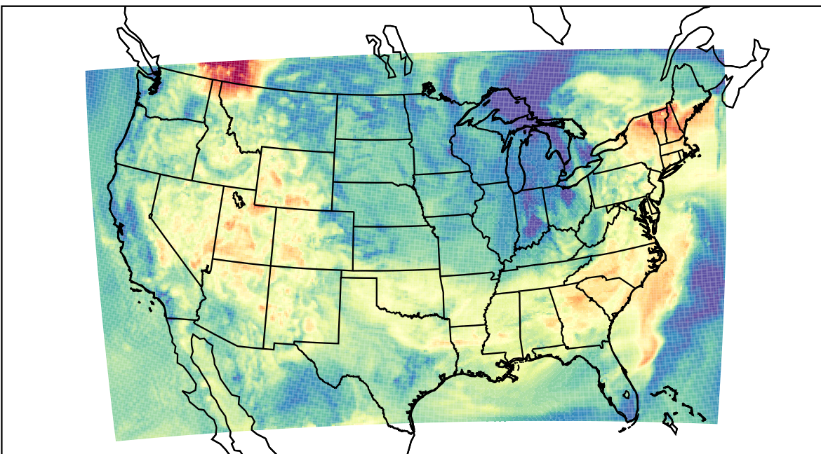
WRF (2023-06-12_15:00:00)
