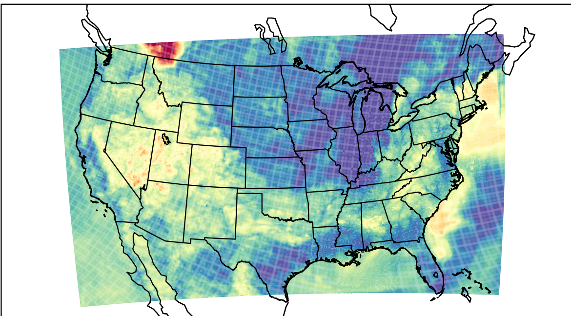
WRF (2023-06-12_09:00:00)
