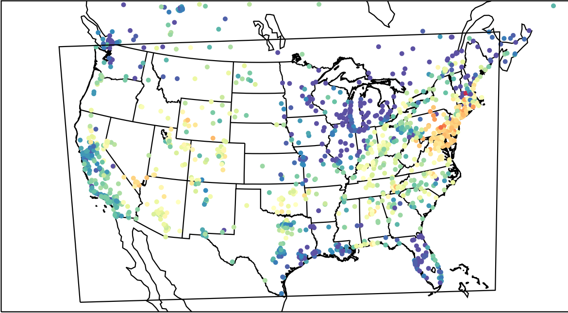
AirNOW (2023-06-12_04:00:00)
