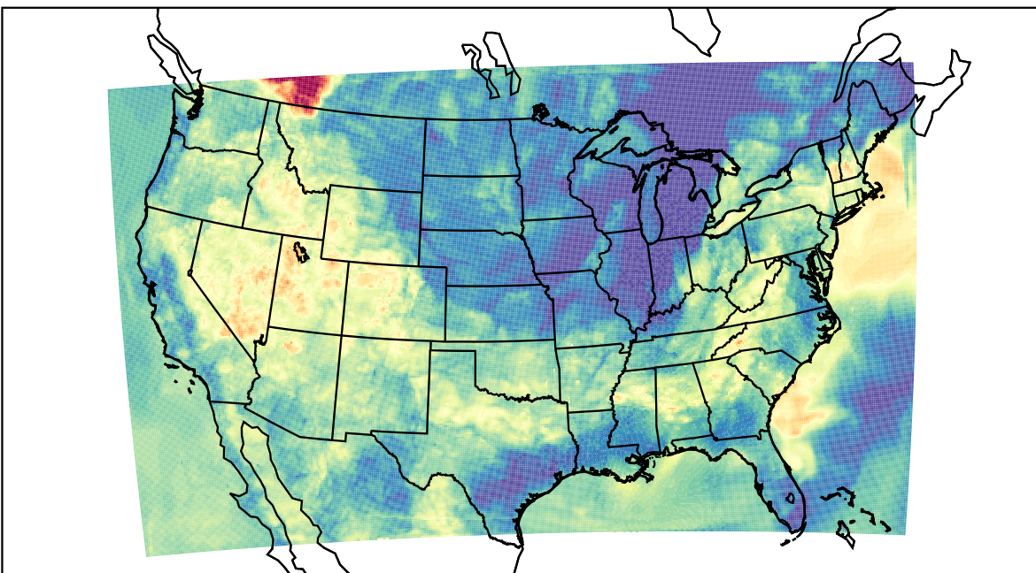
WRF (2023-06-12_07:00:00)
