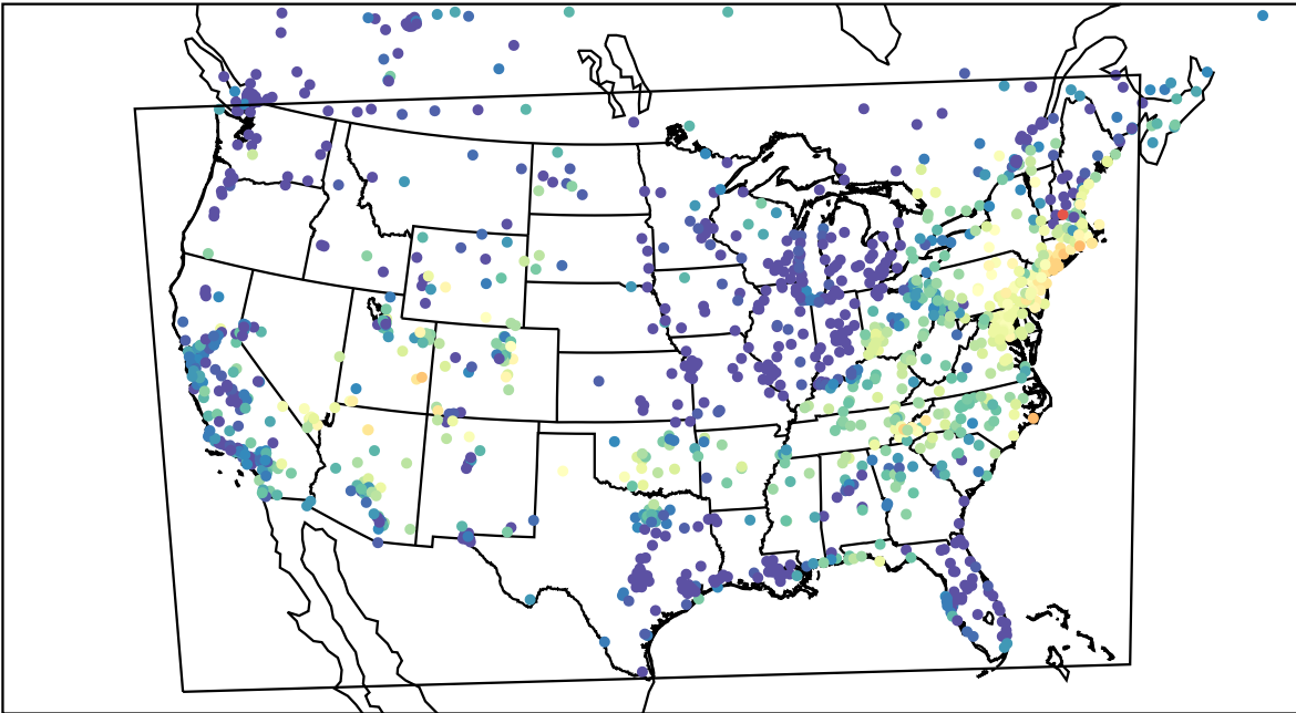
AirNOW (2023-06-12_12:00:00)
