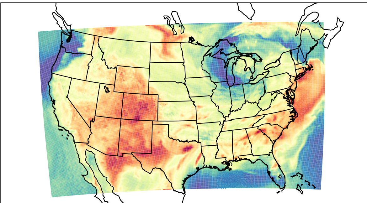
WRF (2023-06-13_20:00:00)
