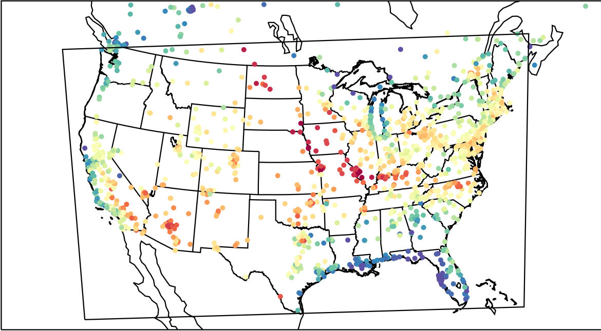
AirNOW (2023-06-14_21:00:00)
