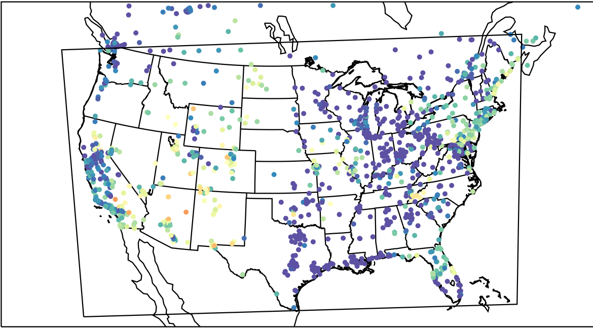
AirNOW (2023-06-15_08:00:00)
