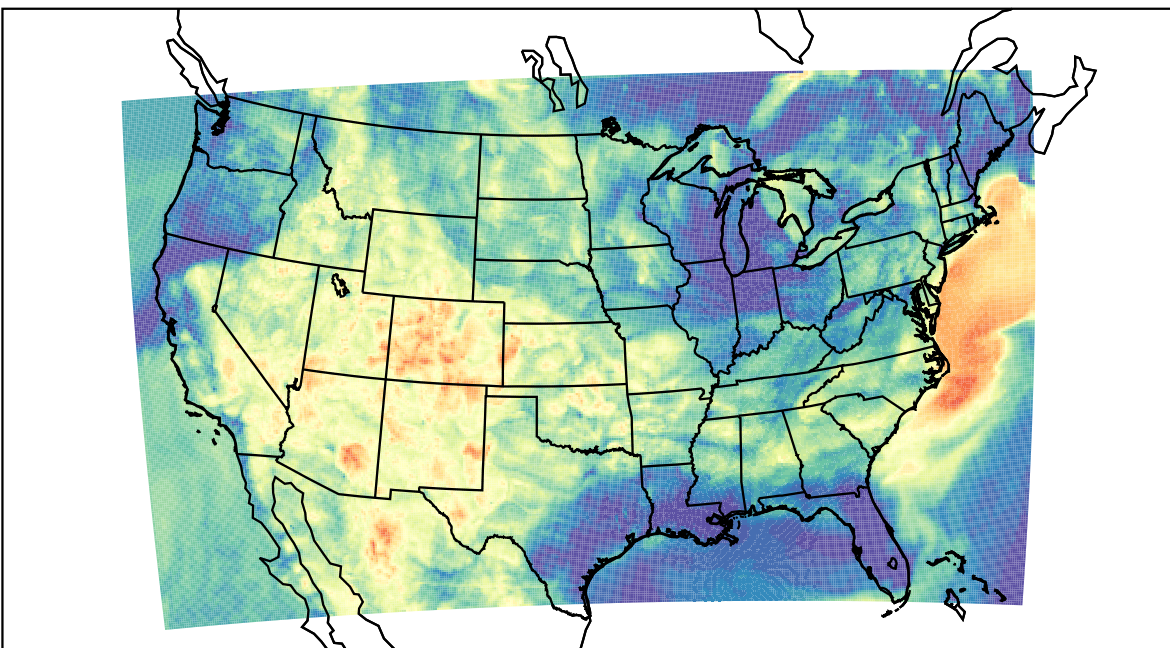
WRF (2023-06-14_06:00:00)
