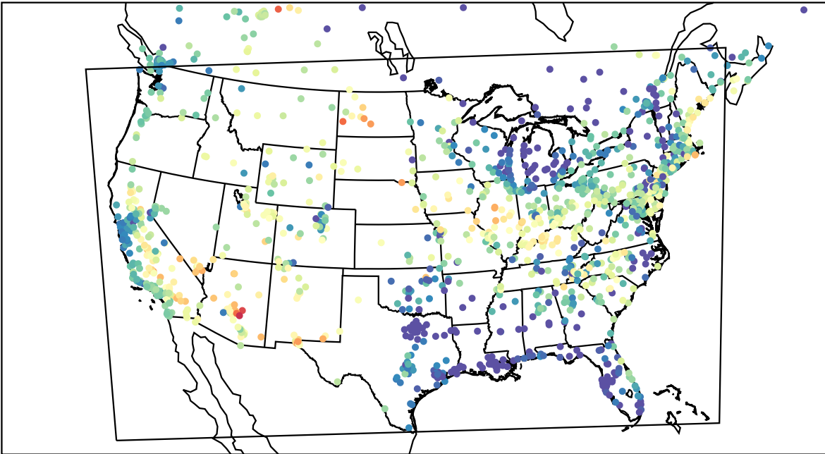
AirNOW (2023-06-14_03:00:00)
