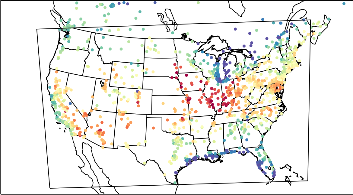
AirNOW (2023-06-15_22:00:00)
