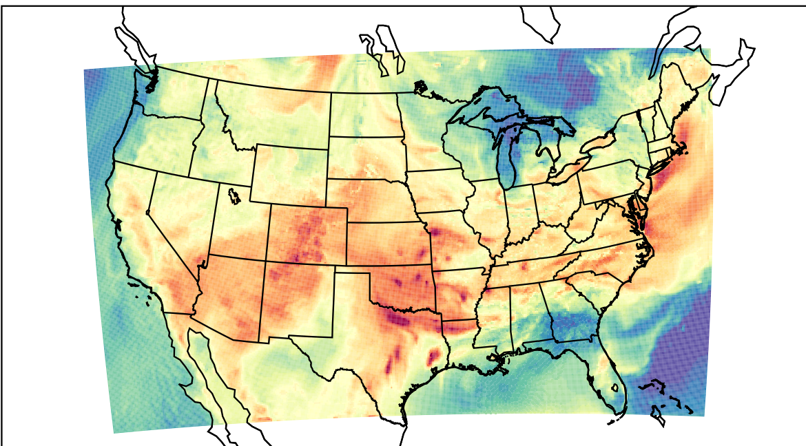
WRF (2023-06-15_20:00:00)
