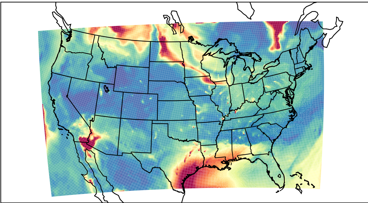
WRF 2023-06-15_14:00:00
