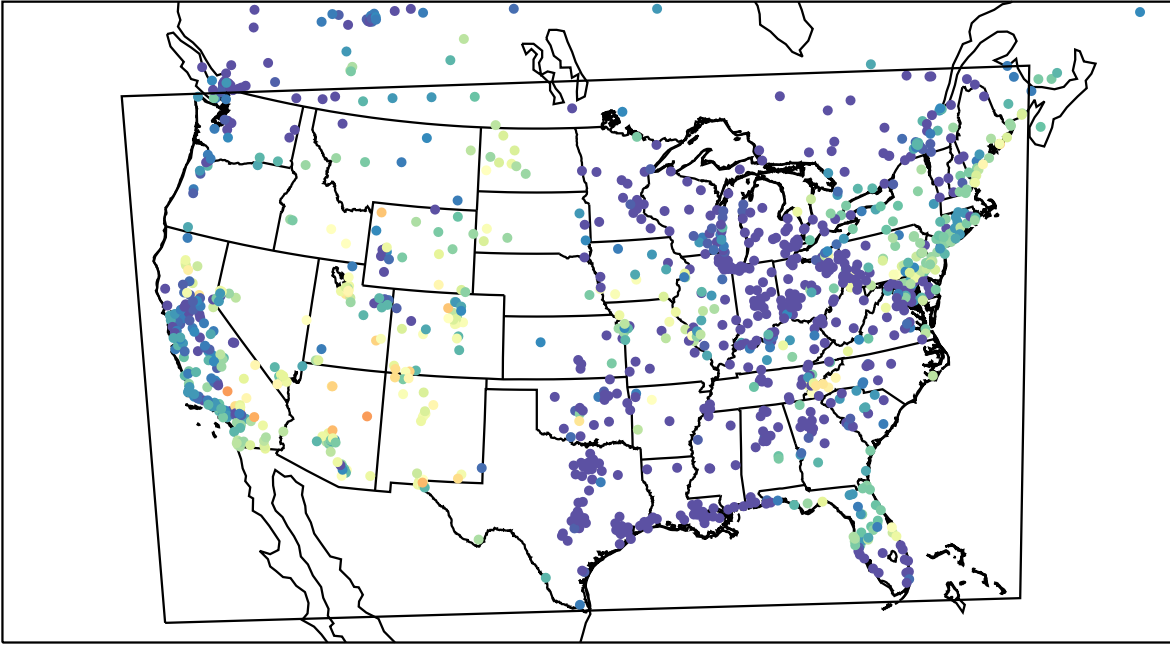
AirNOW (2023-06-15_08:00:00)
