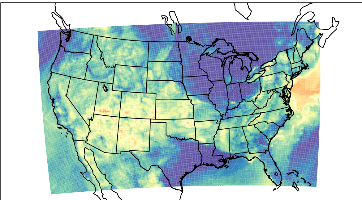
WRF (2023-06-16_12:00:00)
