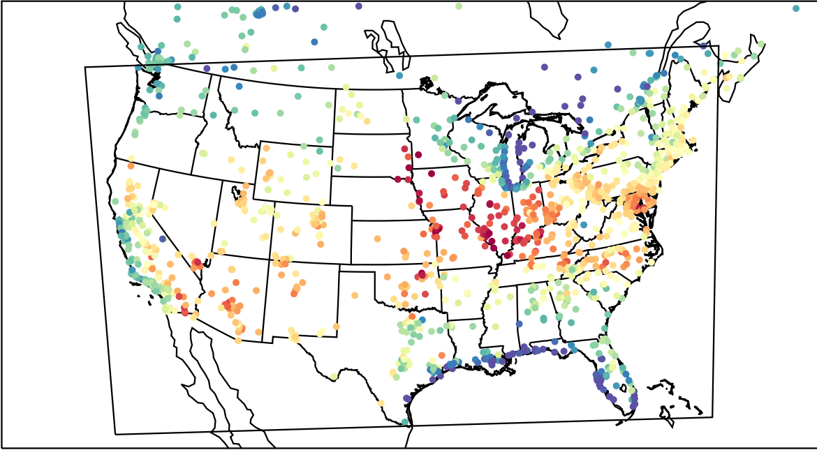
AirNOW (2023-06-15_20:00:00)
