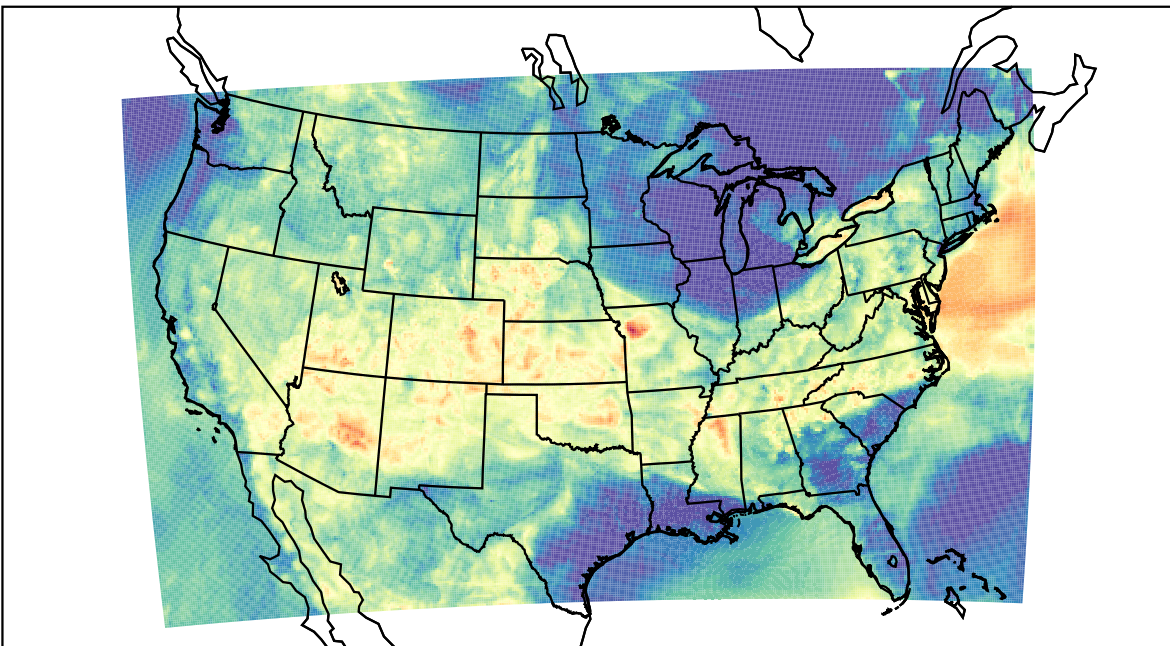
WRF (2023-06-16_06:00:00)
