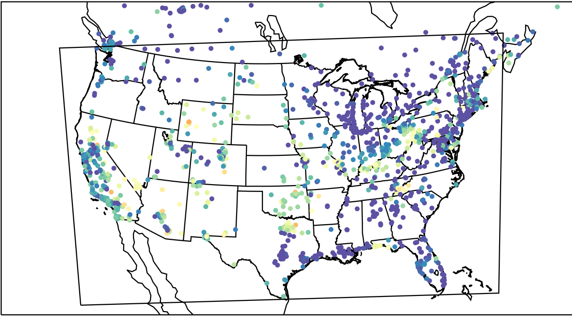
AirNOW (2023-06-16_08:00:00)
