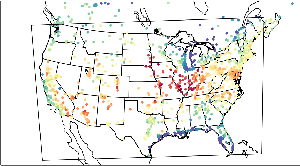
AirNOW (2023-06-15_22:00:00)
