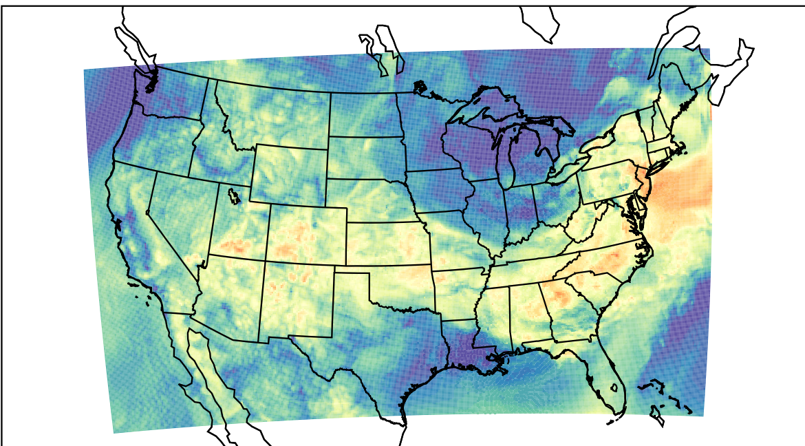
WRF (2023-06-16_14:00:00)
