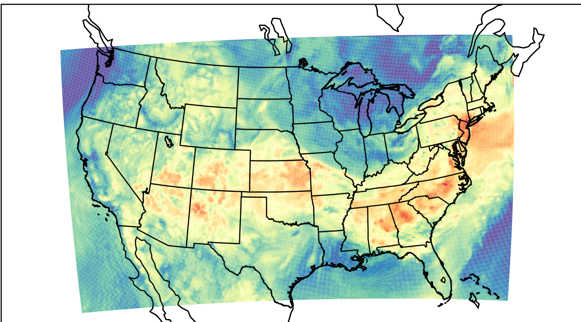
WRF (2023-06-16_15:00:00)
