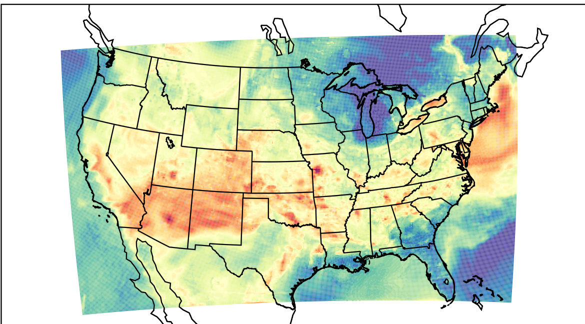
WRF (2023-06-16_01:00:00)
