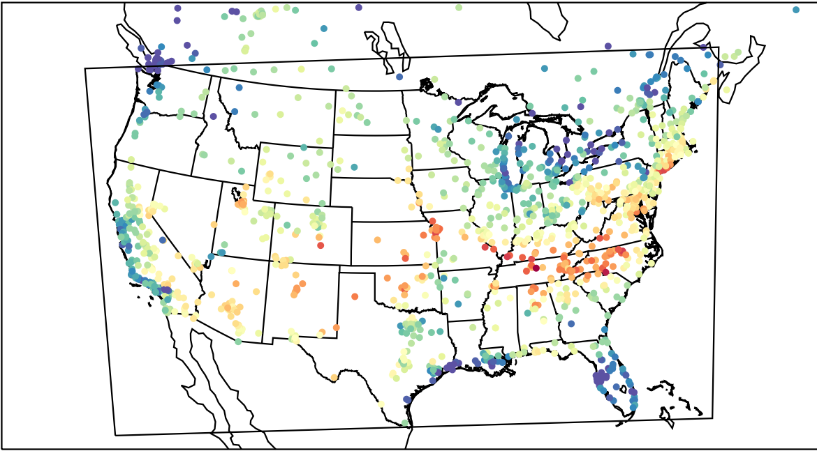
AirNOW (2023-06-16_17:00:00)
