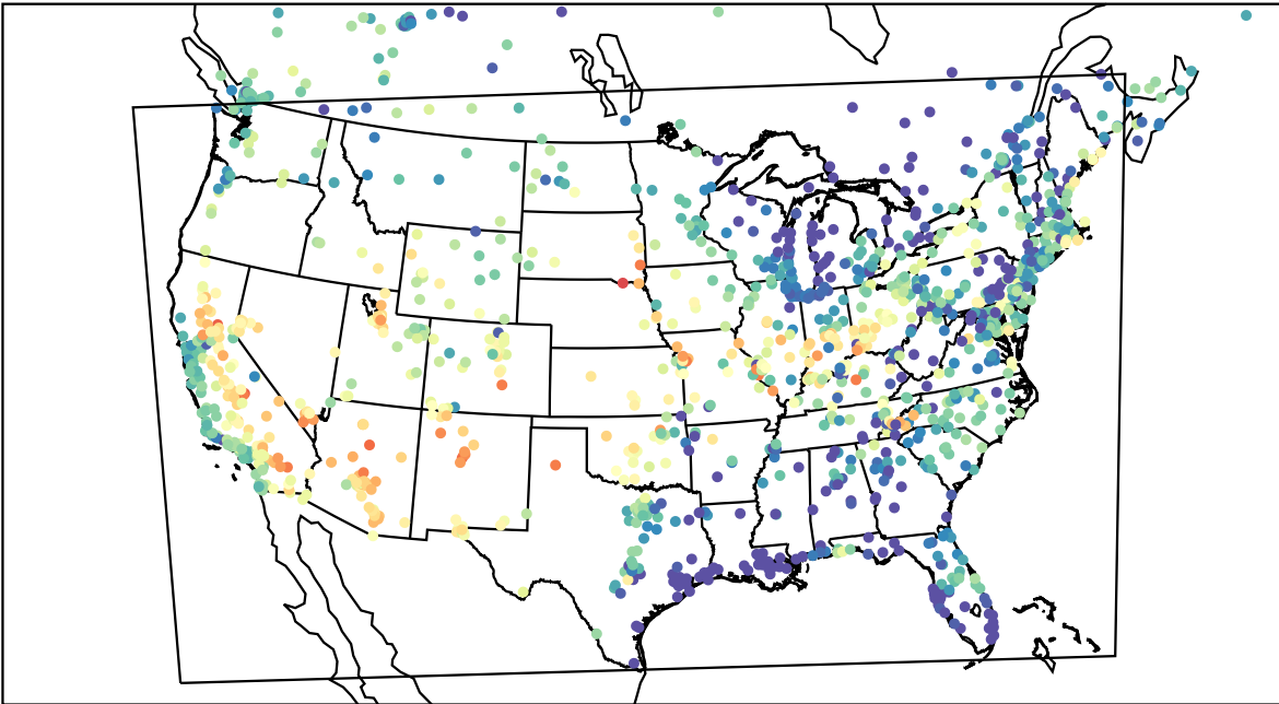
AirNOW (2023-06-16_02:00:00)
