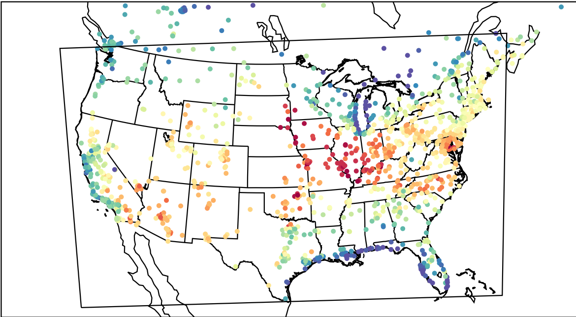
AirNOW (2023-06-15_19:00:00)
