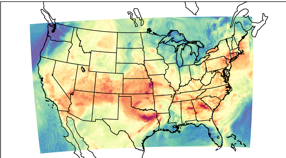
WRF (2023-06-16_22:00:00)
