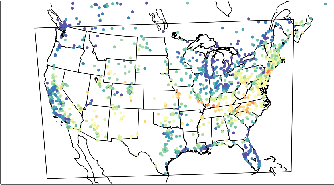
AirNOW (2023-06-16_15:00:00)
