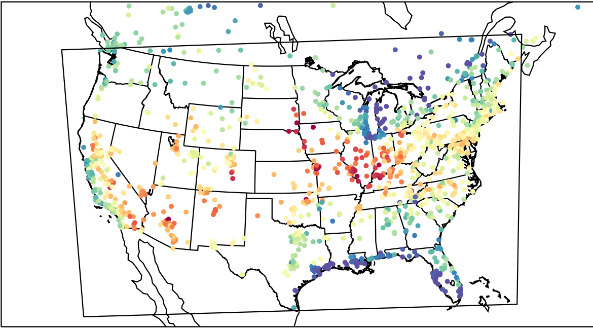
AirNOW (2023-06-15_23:00:00)
