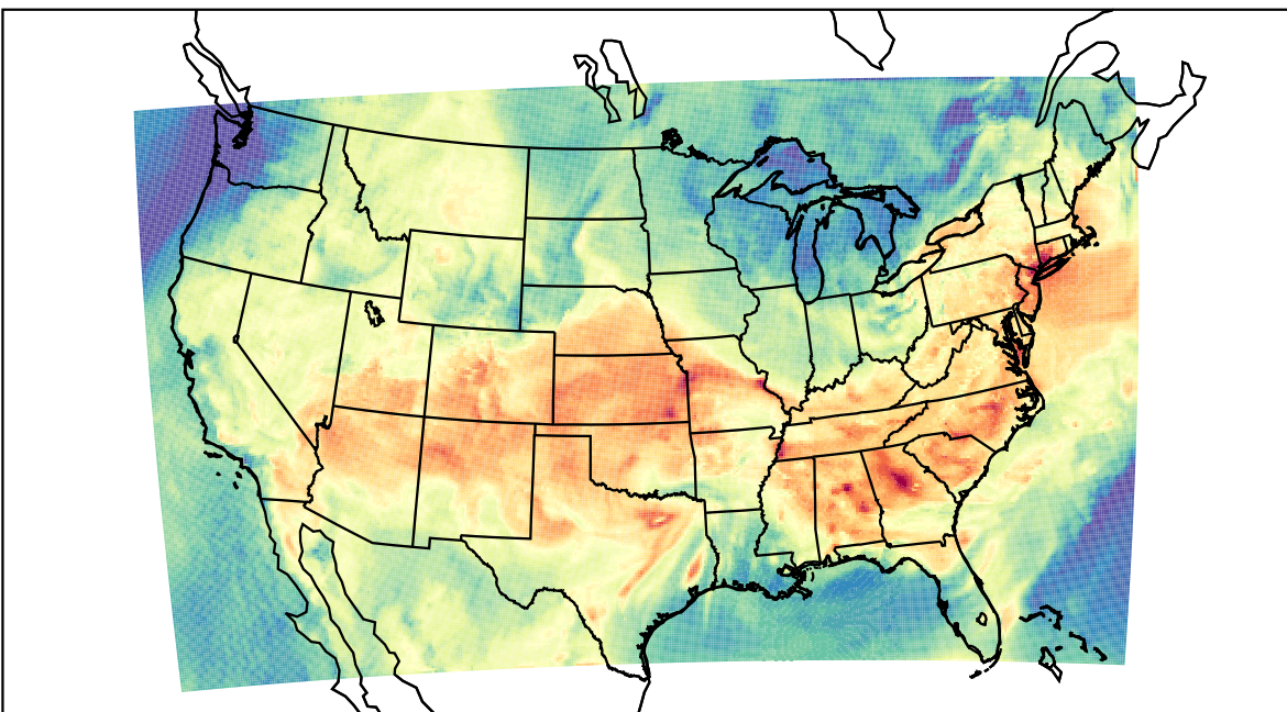
WRF (2023-06-16_17:00:00)
