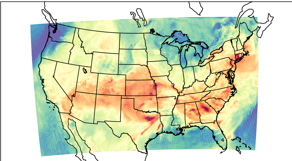
WRF (2023-06-16_19:00:00)
