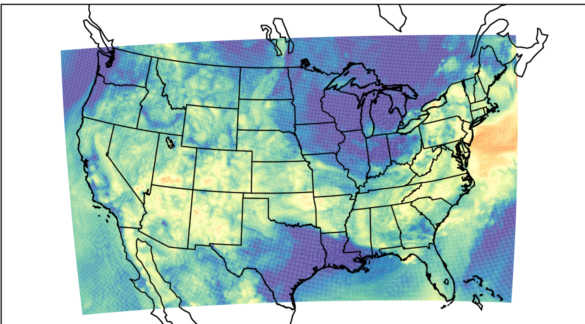
WRF (2023-06-16_13:00:00)
