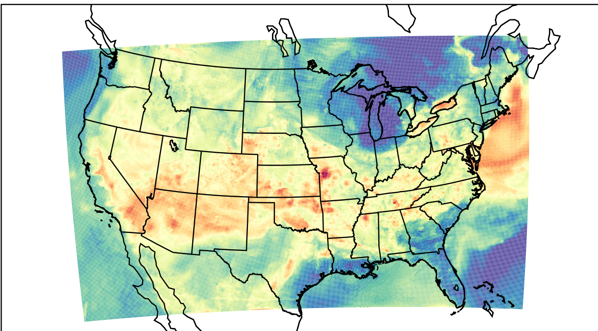
WRF (2023-06-16_02:00:00)
