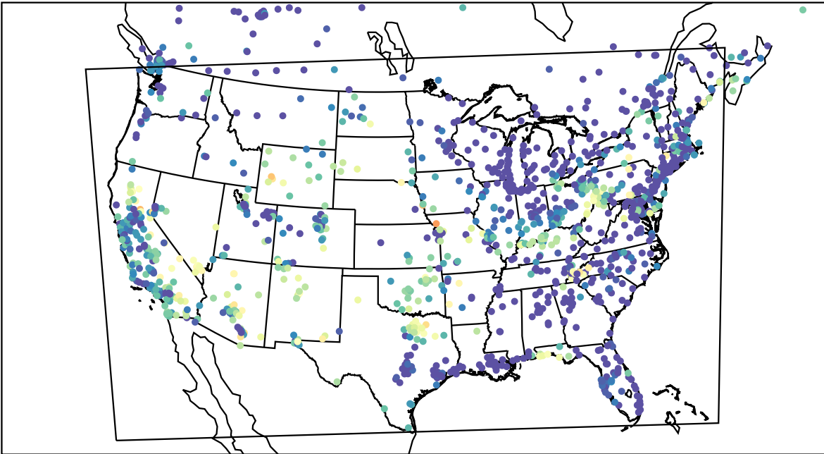
AirNOW (2023-06-16_09:00:00)
