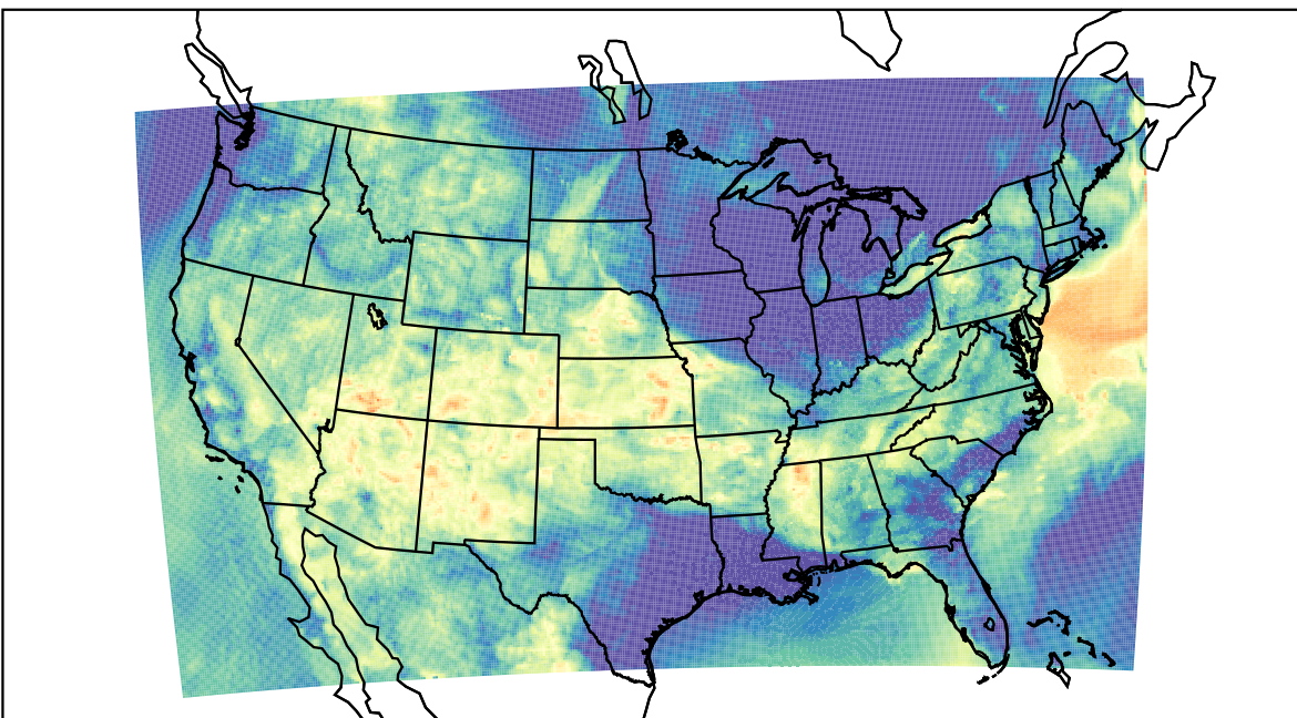
WRF (2023-06-16_11:00:00)
