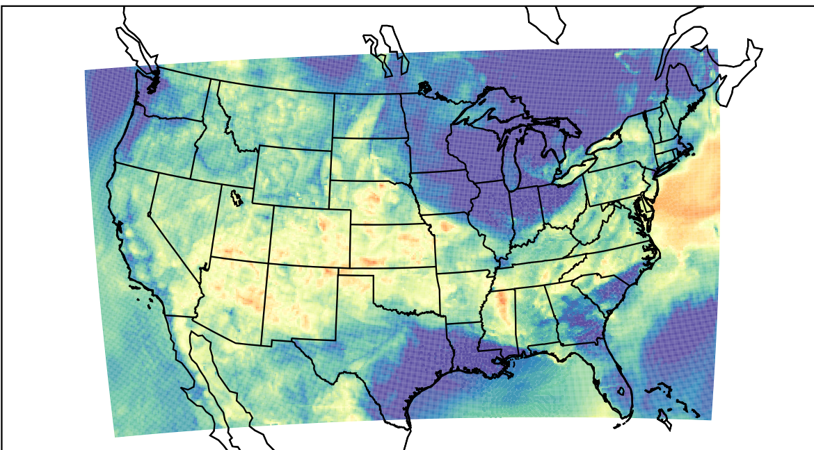
WRF (2023-06-16_09:00:00)
