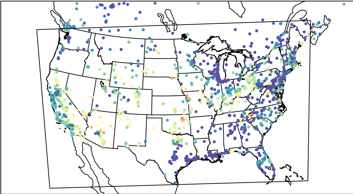
AirNOW (2023-06-16_05:00:00)
