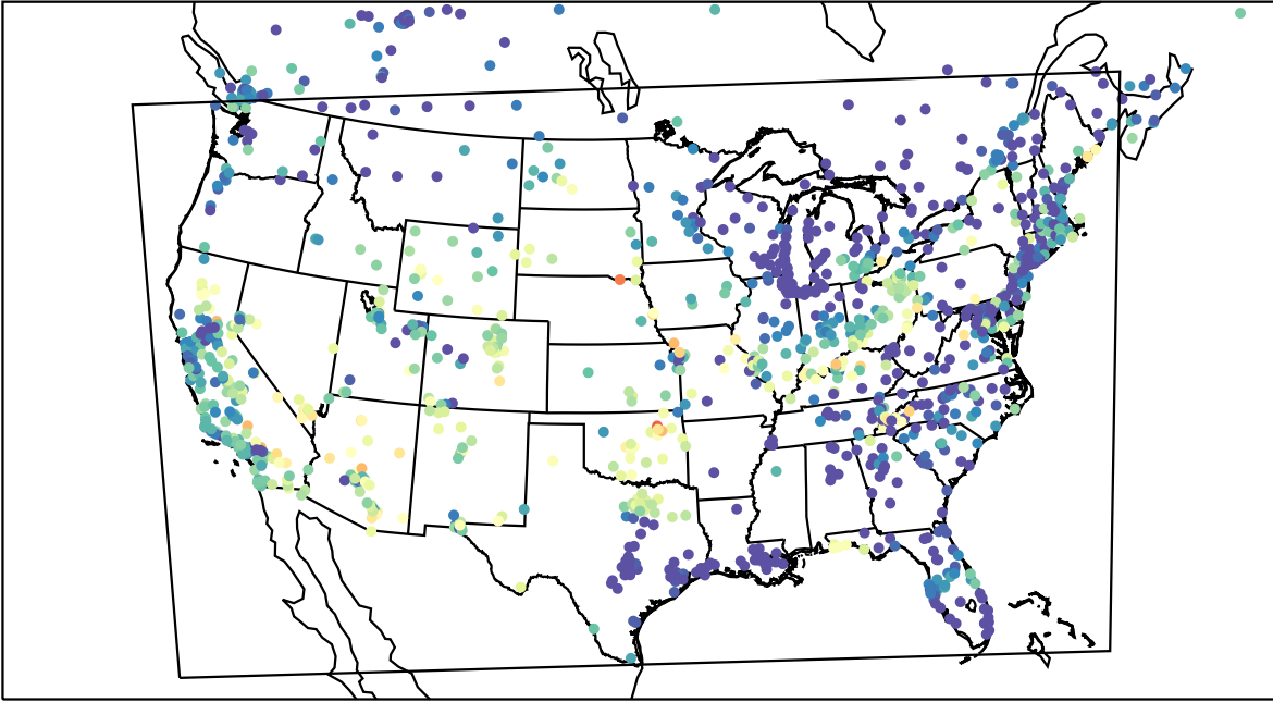
AirNOW (2023-06-16_06:00:00)
