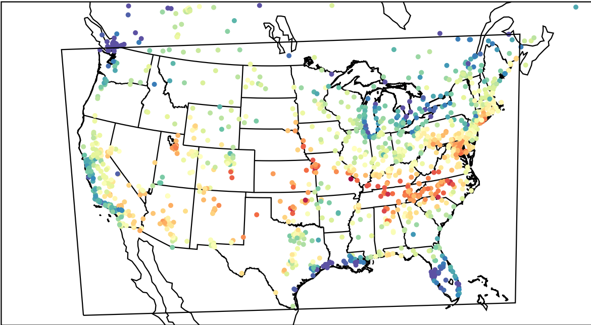
AirNOW (2023-06-16_18:00:00)
