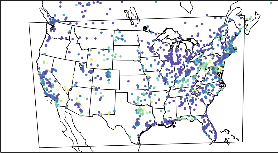
AirNOW (2023-06-16_12:00:00)
