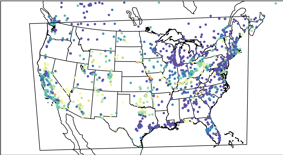
AirNOW (2023-06-16_07:00:00)
