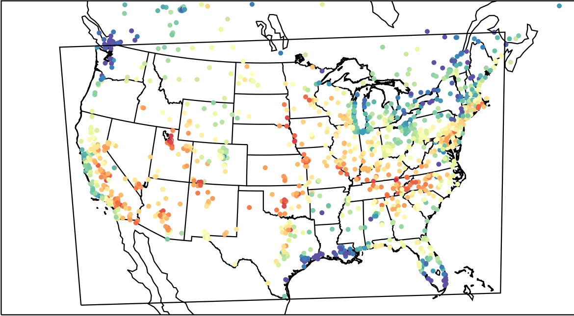
AirNOW (2023-06-16_23:00:00)
