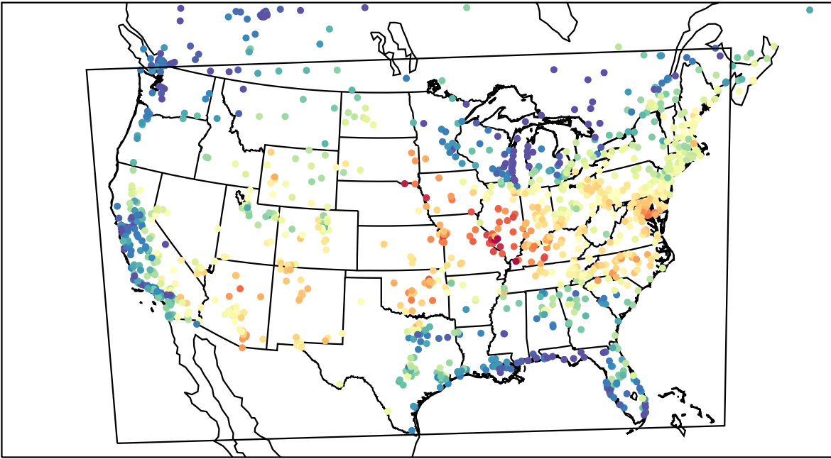
AirNOW (2023-06-15_16:00:00)
