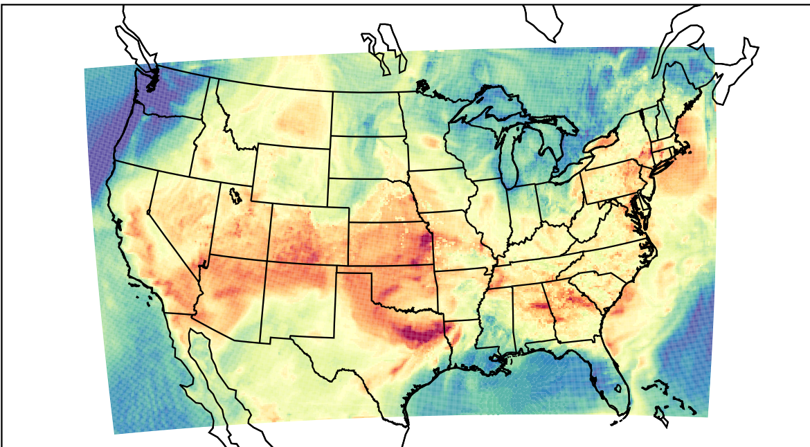
WRF (2023-06-16_23:00:00)
