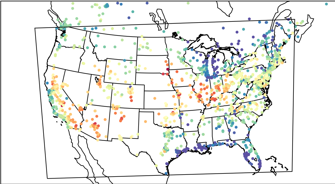
AirNOW (2023-06-16_00:00:00)
