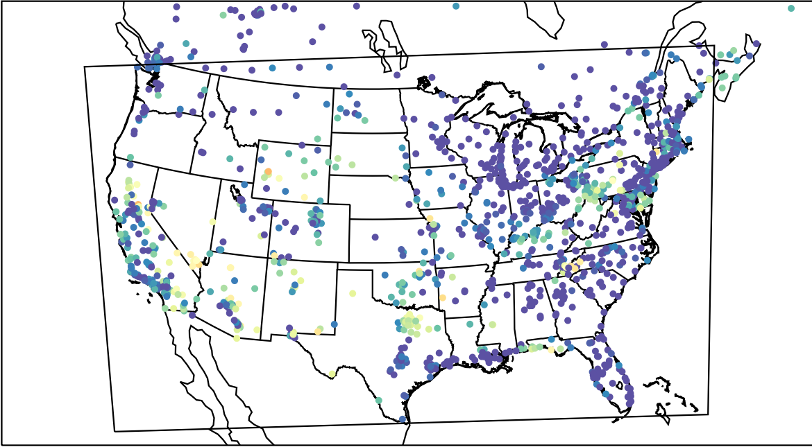
AirNOW (2023-06-16_11:00:00)
