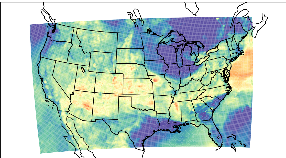
WRF (2023-06-16_07:00:00)
