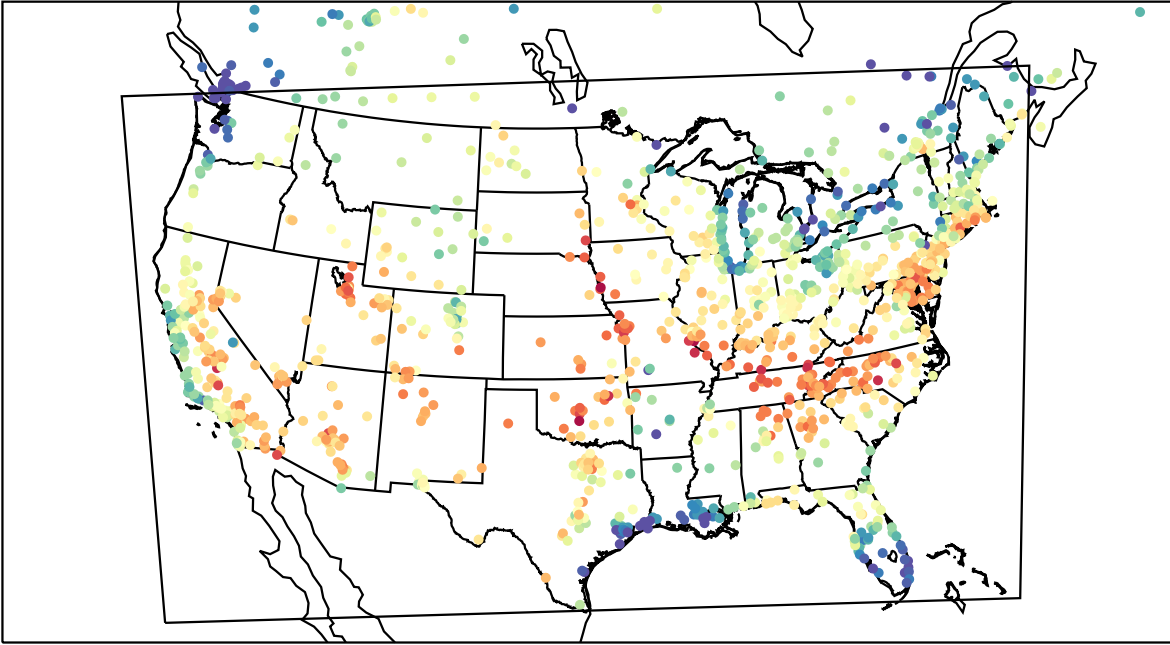
AirNOW (2023-06-16_21:00:00)
