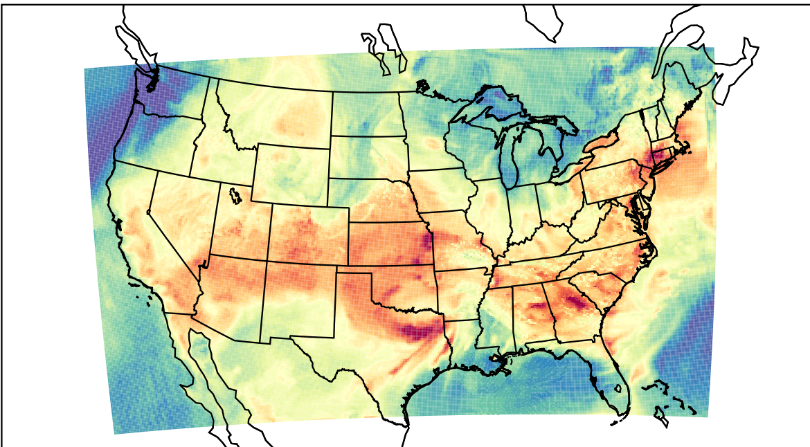
WRF (2023-06-16_21:00:00)
