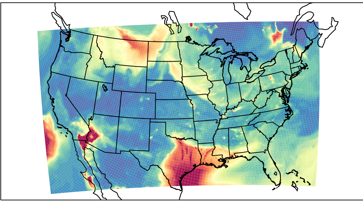
WRF 2023-06-16_09:00:00
