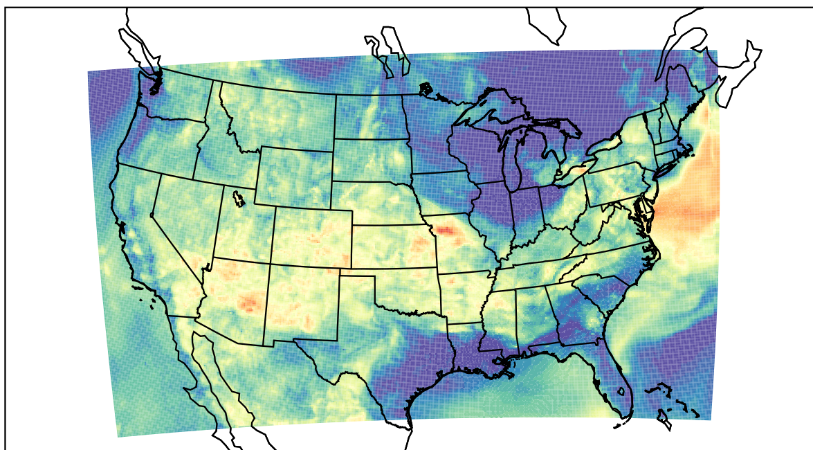
WRF (2023-06-16_07:00:00)
