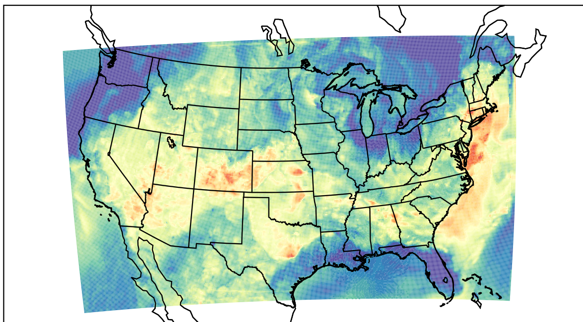
WRF (2023-06-17_04:00:00)
