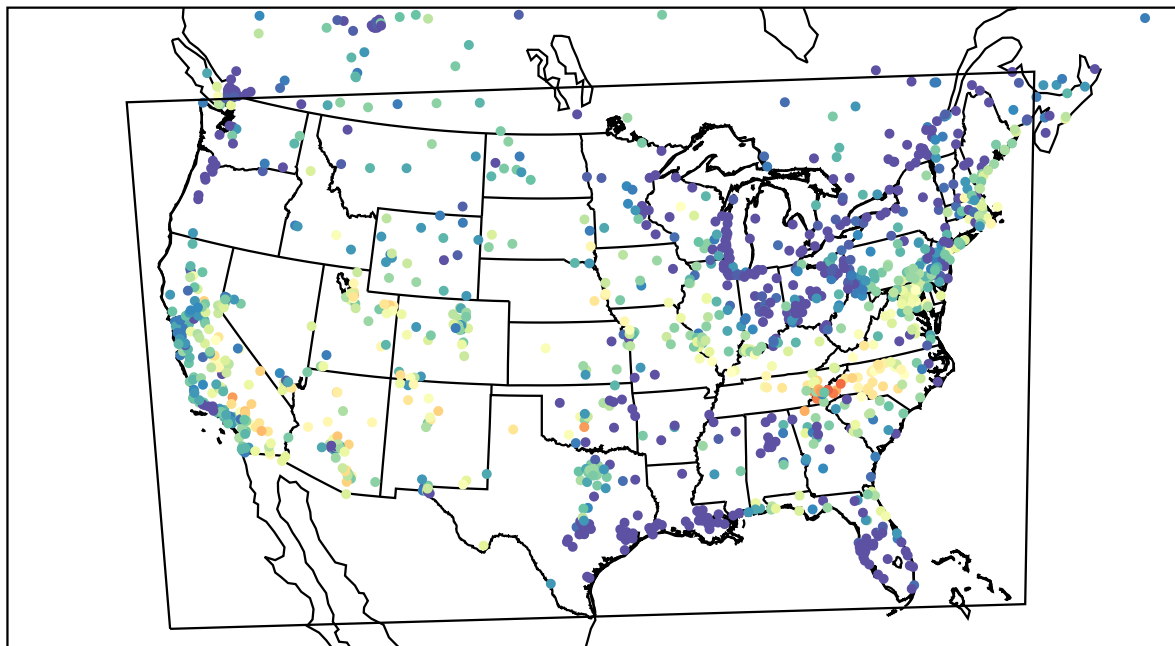
AirNOW (2023-06-17_05:00:00)
