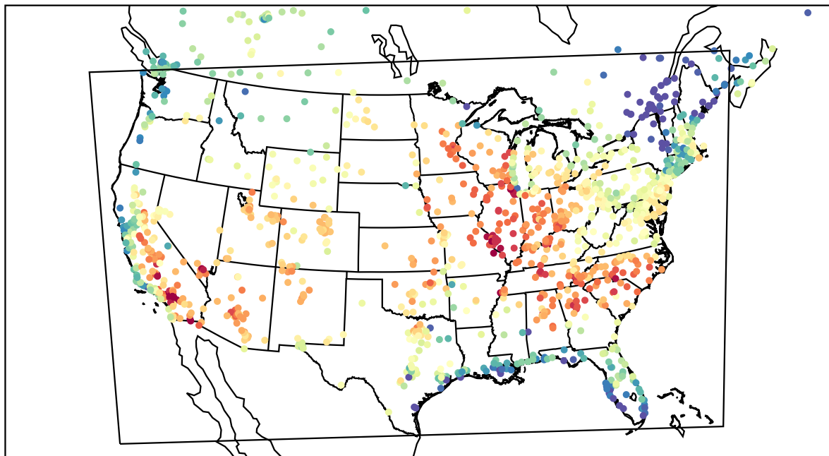
AirNOW (2023-06-17_21:00:00)
