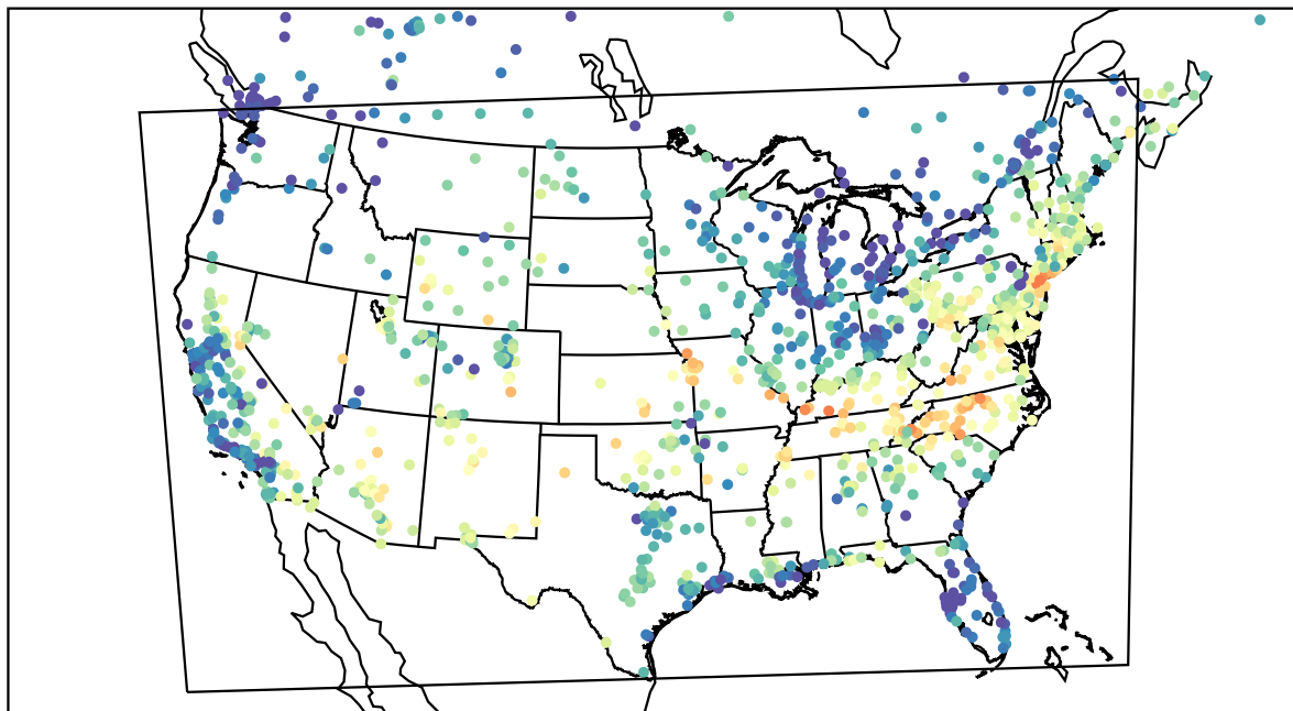
AirNOW (2023-06-16_15:00:00)
