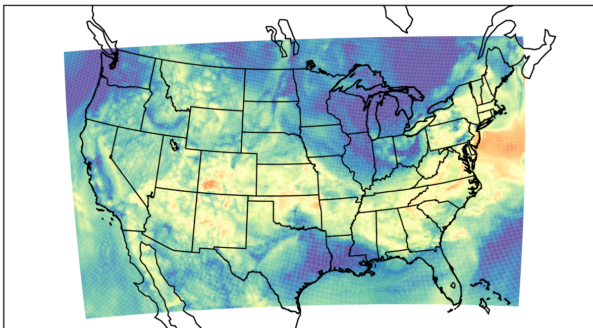
WRF (2023-06-16_14:00:00)
