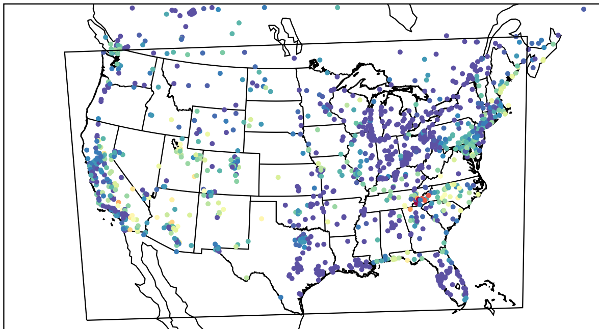
AirNOW (2023-06-17_09:00:00)
