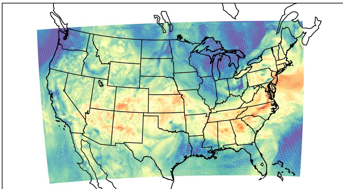
WRF (2023-06-16_15:00:00)
