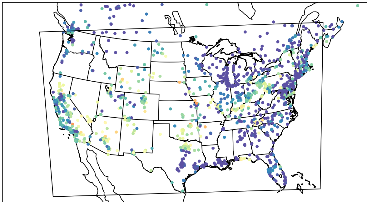
AirNOW (2023-06-16_07:00:00)
