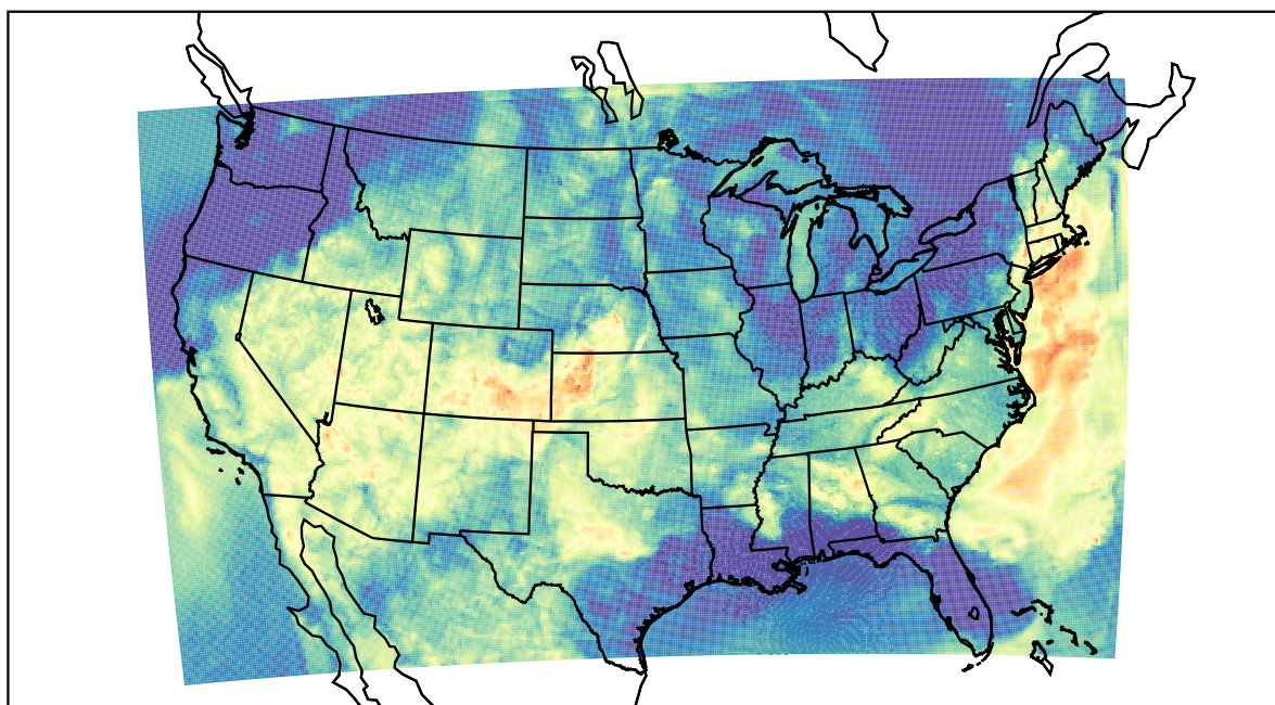
WRF (2023-06-17_09:00:00)
