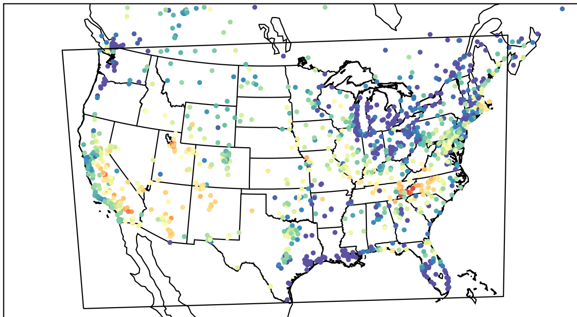
AirNOW (2023-06-17_03:00:00)
