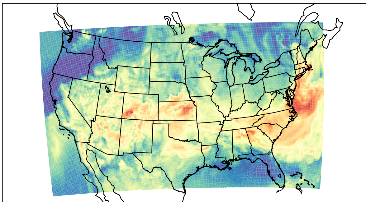
WRF (2023-06-17_15:00:00)
