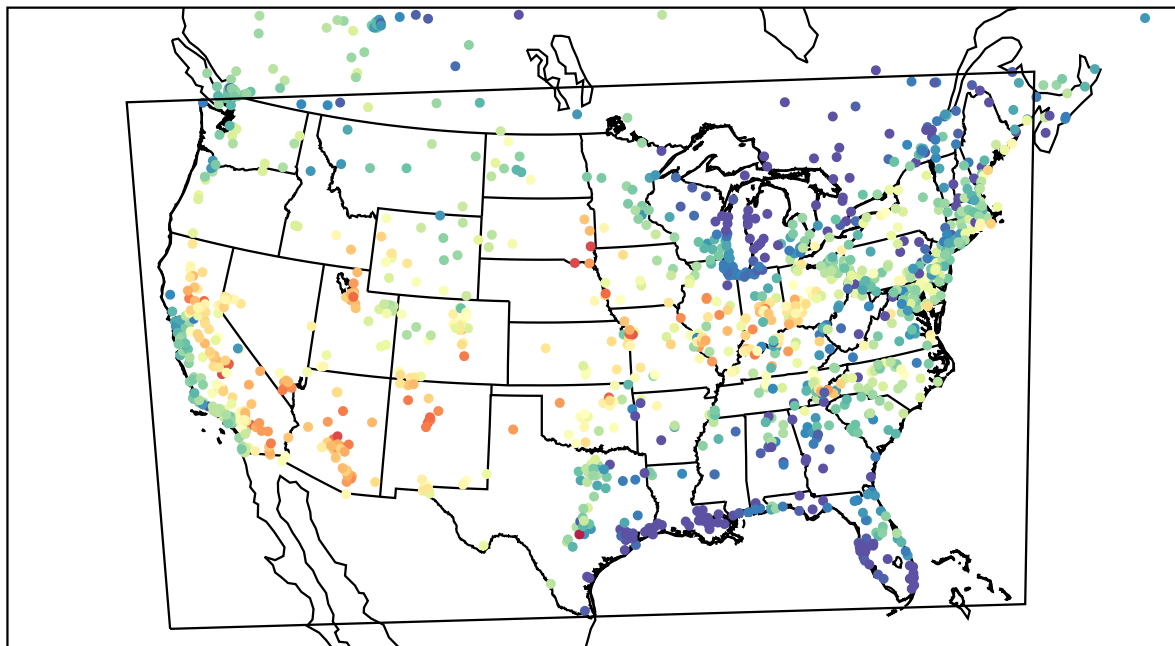
AirNOW (2023-06-16_01:00:00)
