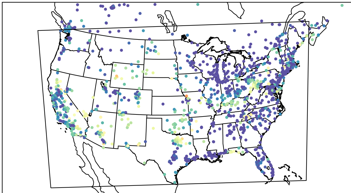
AirNOW (2023-06-16_09:00:00)
