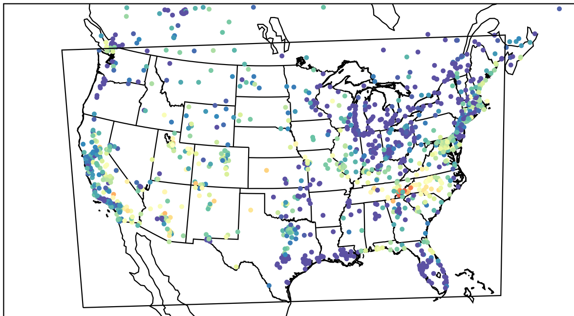
AirNOW (2023-06-17_06:00:00)
