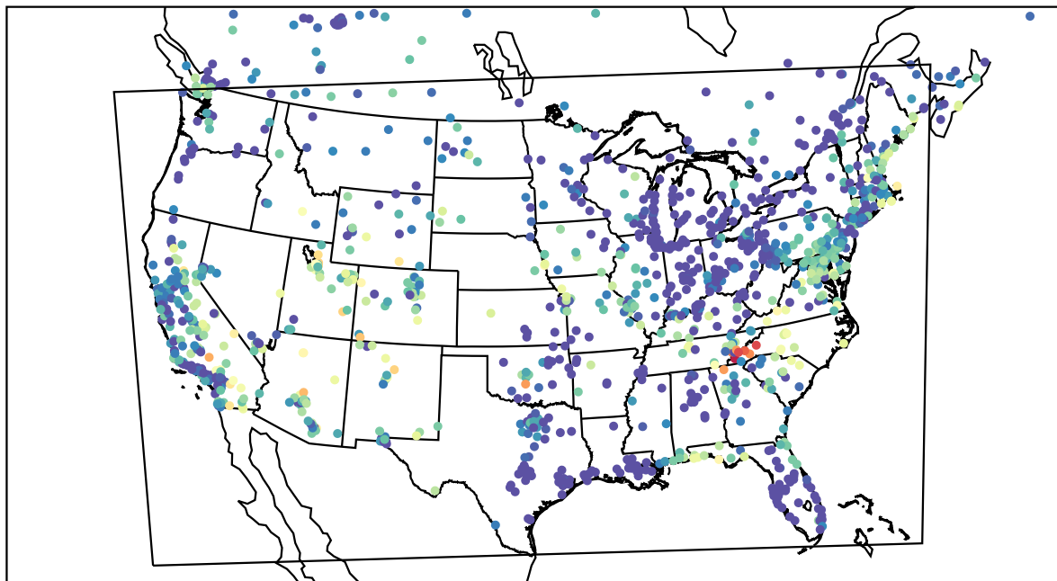
AirNOW (2023-06-17_08:00:00)
