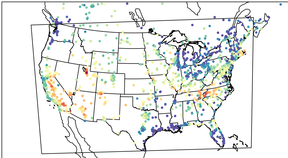
AirNOW (2023-06-17_02:00:00)
