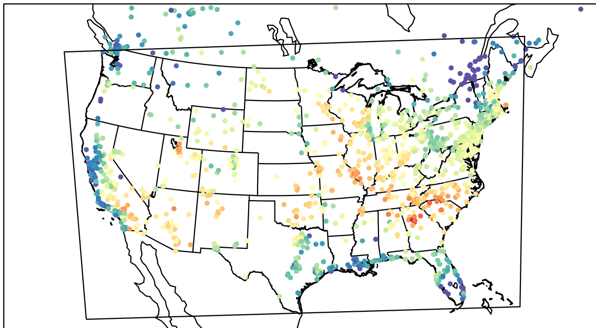
AirNOW (2023-06-17_16:00:00)
