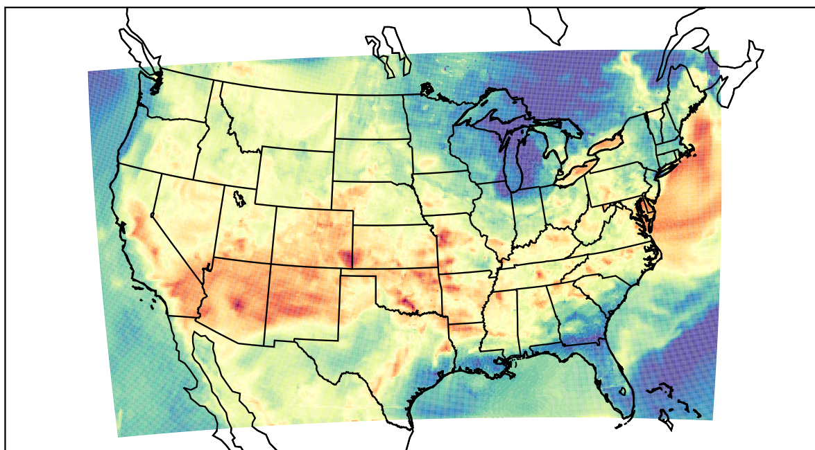
WRF (2023-06-16_01:00:00)
