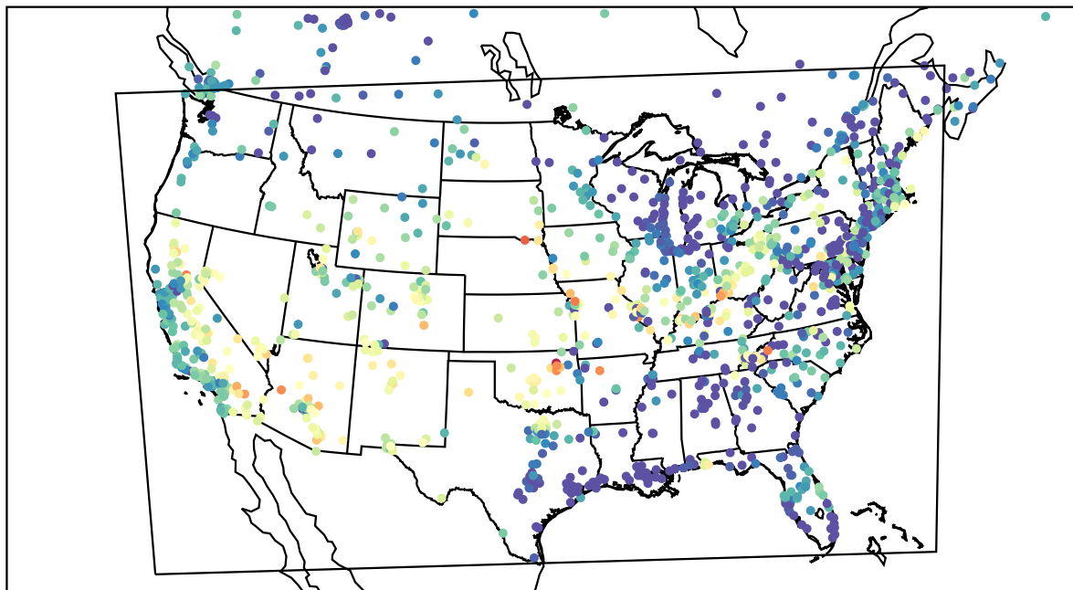
AirNOW (2023-06-16_04:00:00)
