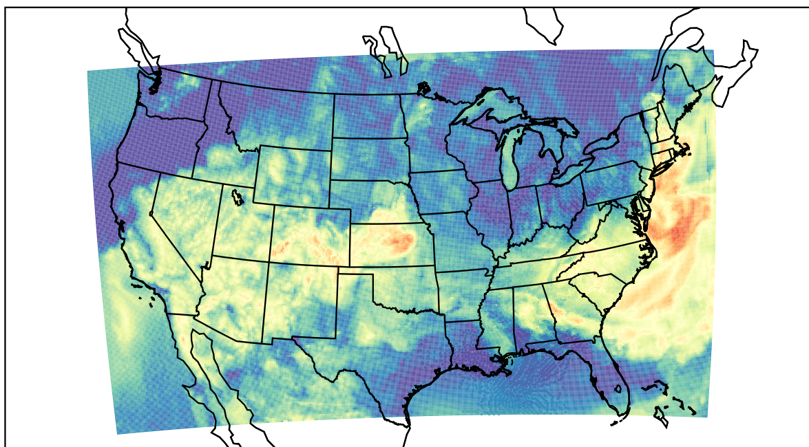
WRF (2023-06-17_13:00:00)
