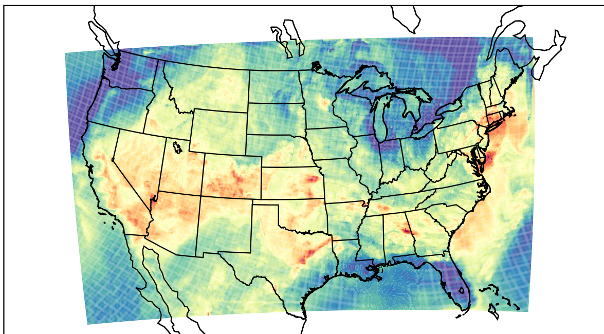
WRF (2023-06-17_02:00:00)
