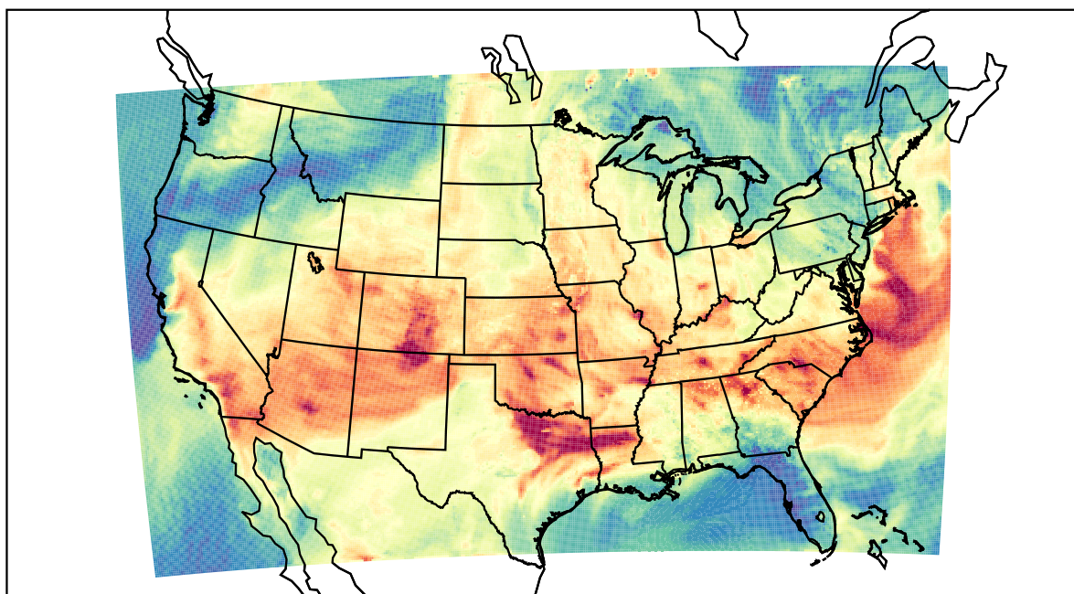
WRF (2023-06-17_22:00:00)
