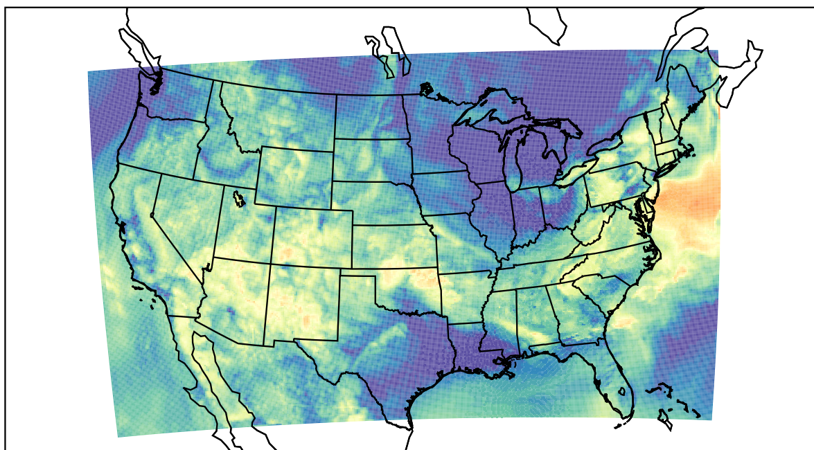
WRF (2023-06-16_13:00:00)
