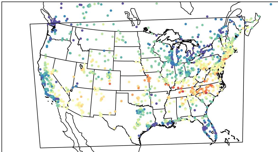
AirNOW (2023-06-16_16:00:00)
