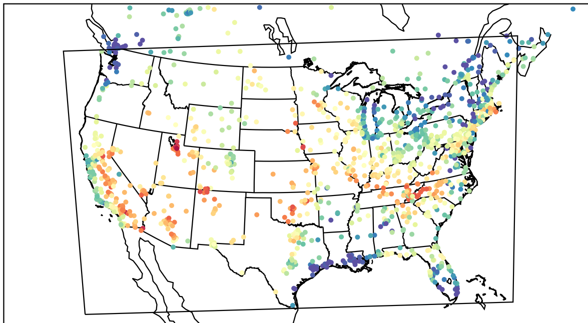
AirNOW (2023-06-17_00:00:00)
