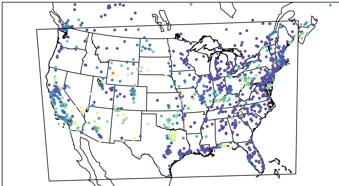
AirNOW (2023-06-16_10:00:00)
