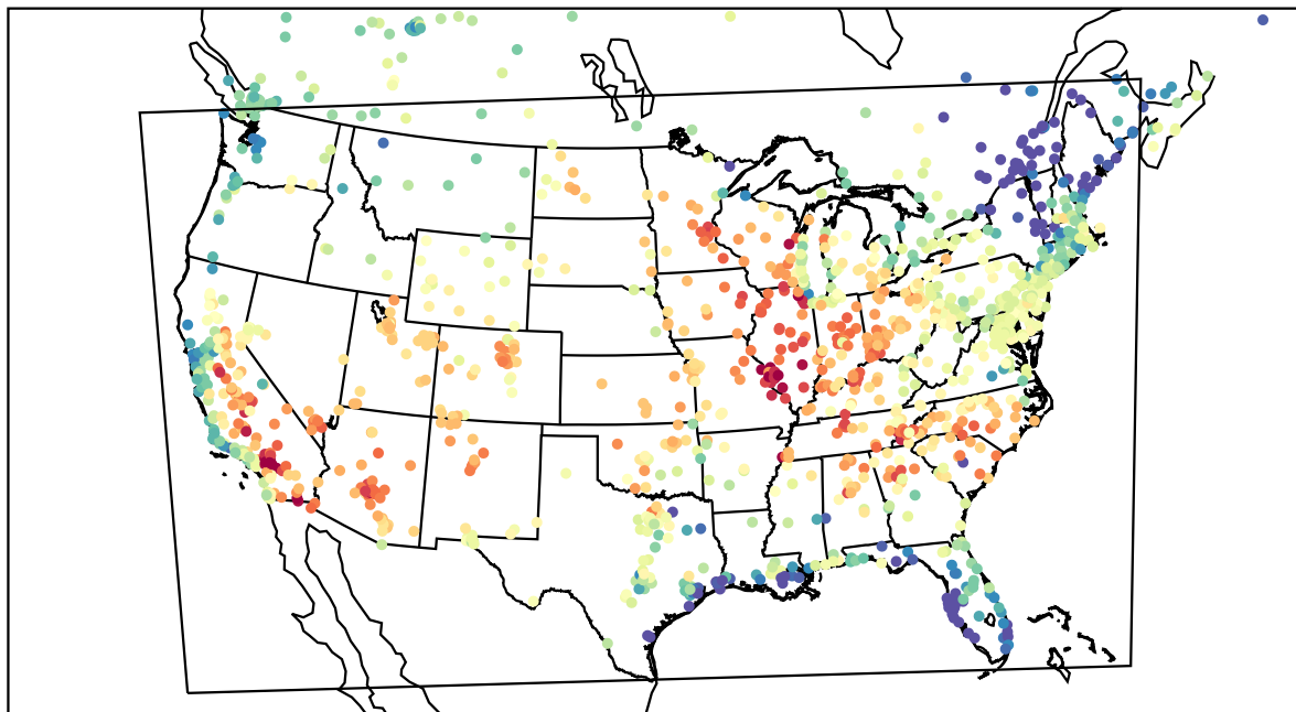
AirNOW (2023-06-17_23:00:00)
