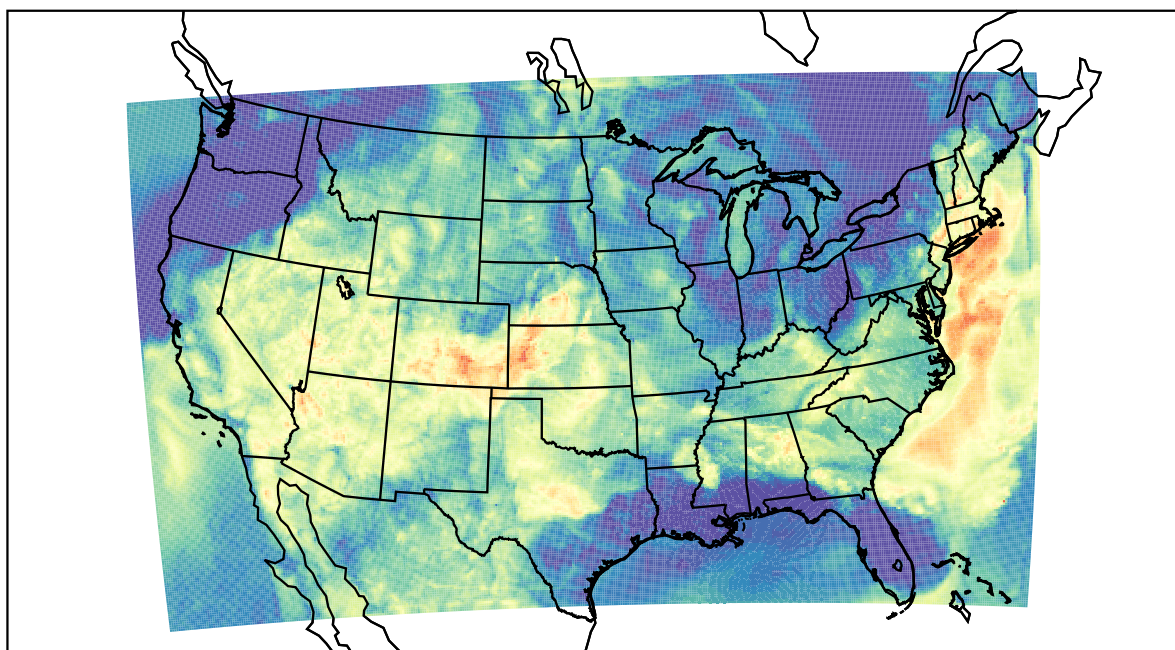
WRF (2023-06-17_08:00:00)
