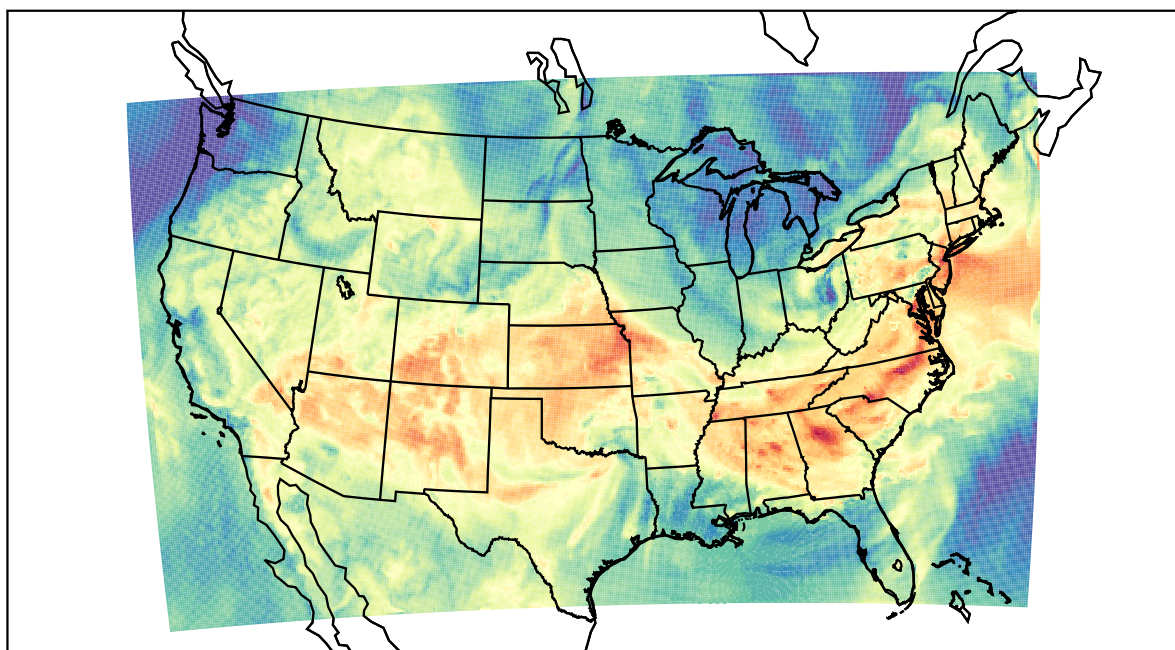
WRF (2023-06-16_16:00:00)
