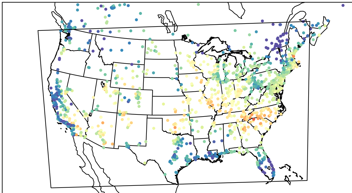
AirNOW (2023-06-17_15:00:00)
