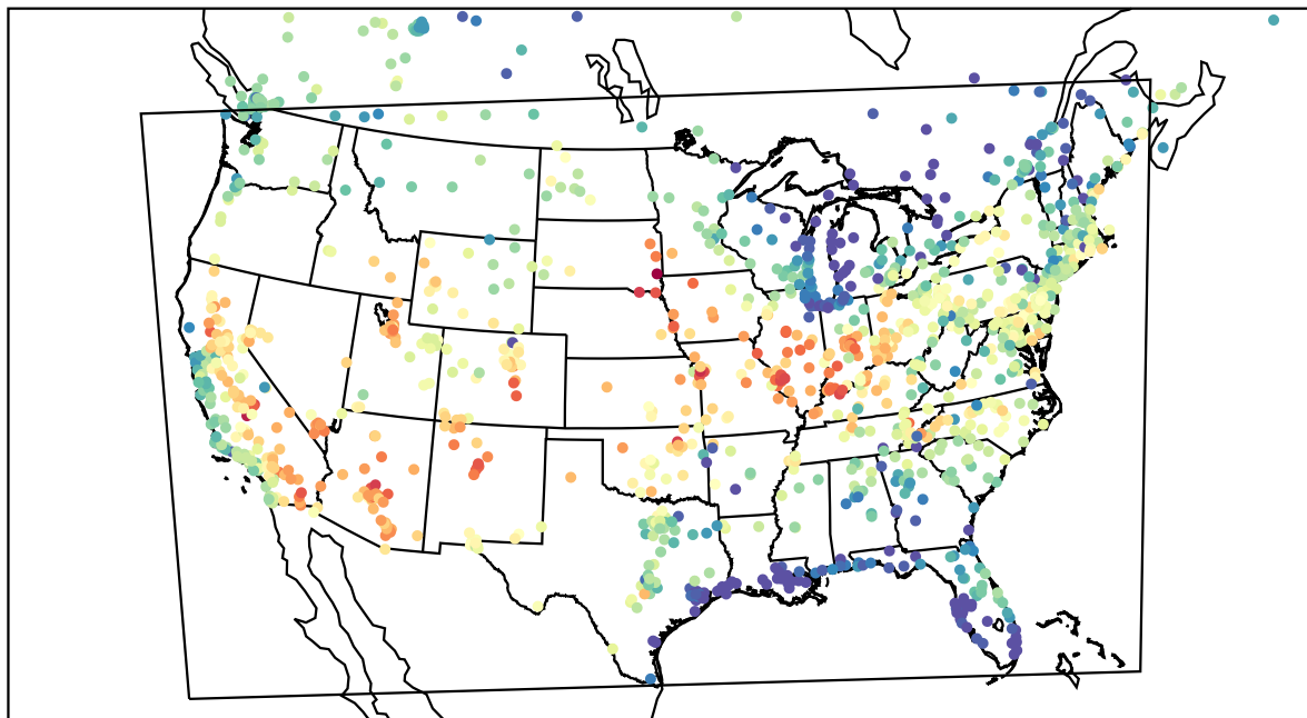
AirNOW (2023-06-16_00:00:00)
