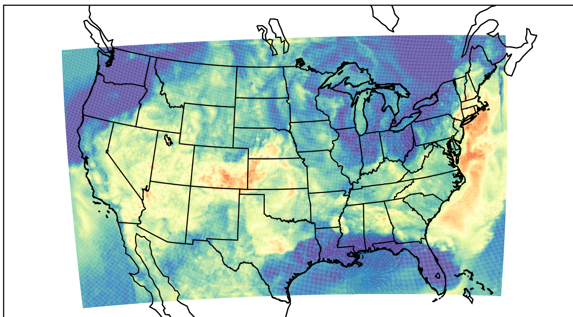
WRF (2023-06-17_07:00:00)
