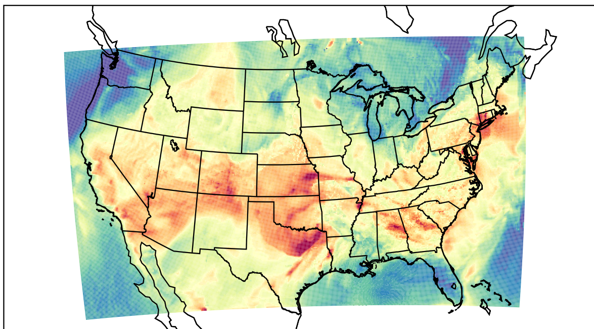
WRF (2023-06-16_23:00:00)
