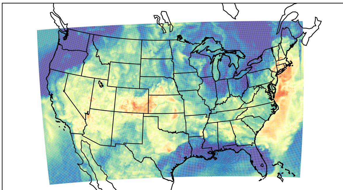
WRF (2023-06-17_06:00:00)
