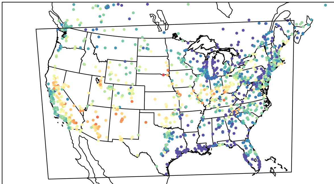
AirNOW (2023-06-16_02:00:00)
