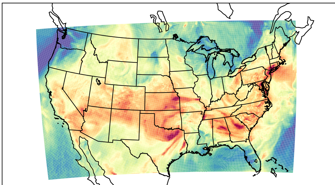
WRF (2023-06-16_21:00:00)
