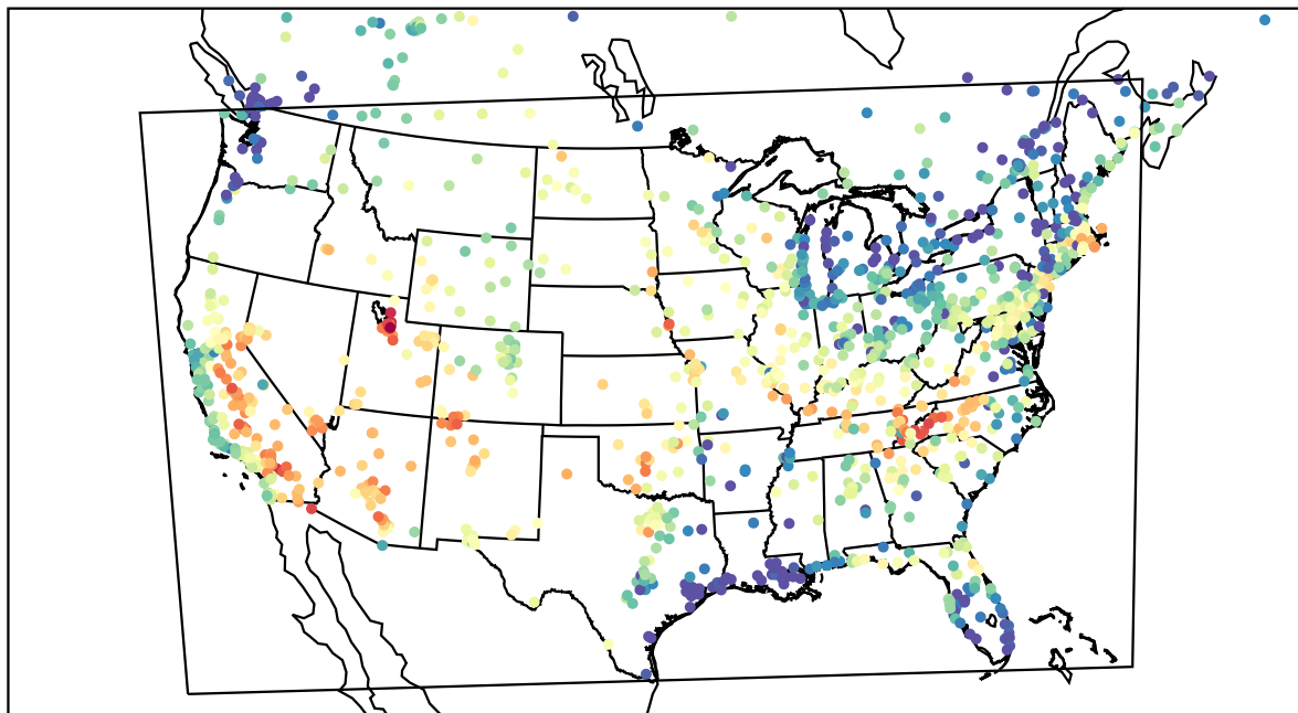
AirNOW (2023-06-17_01:00:00)
