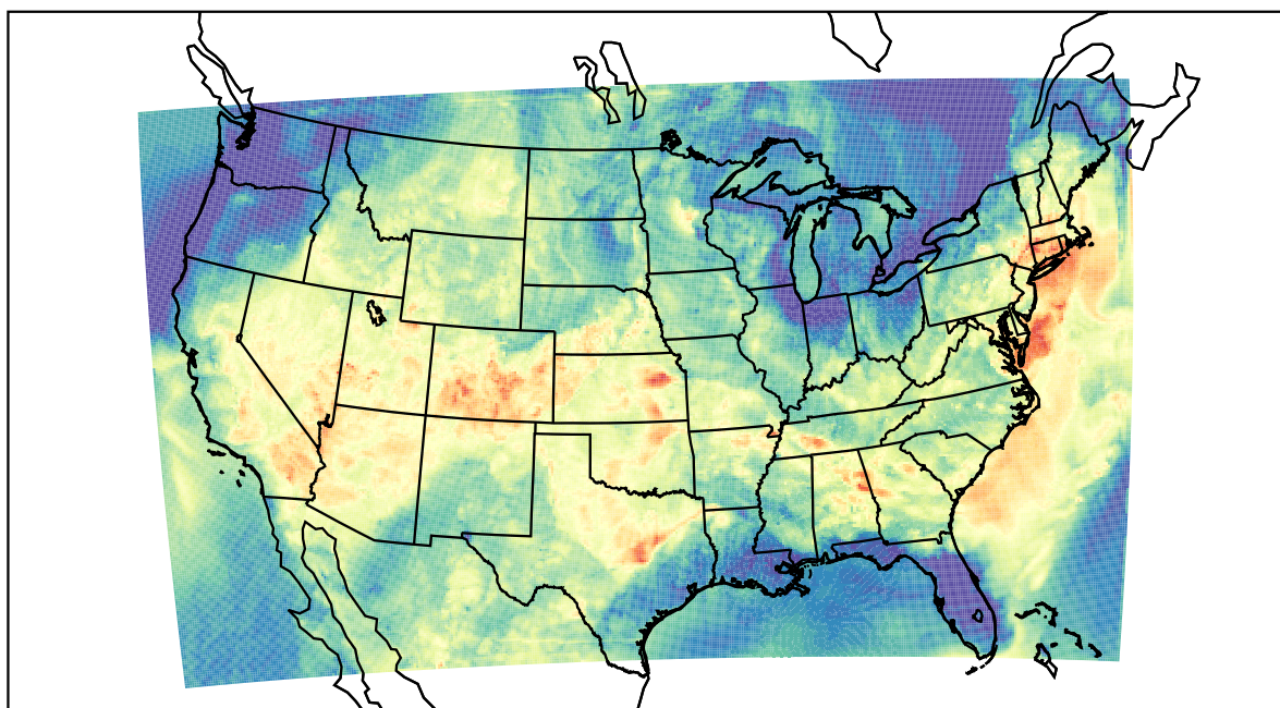
WRF (2023-06-17_03:00:00)
