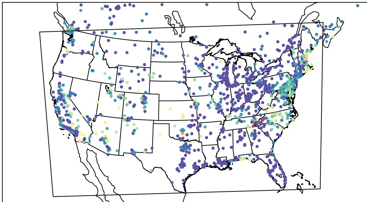
AirNOW (2023-06-17_11:00:00)
