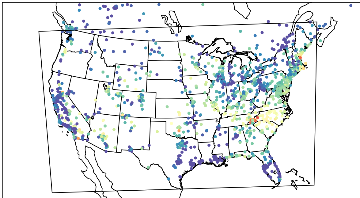
AirNOW (2023-06-17_13:00:00)
