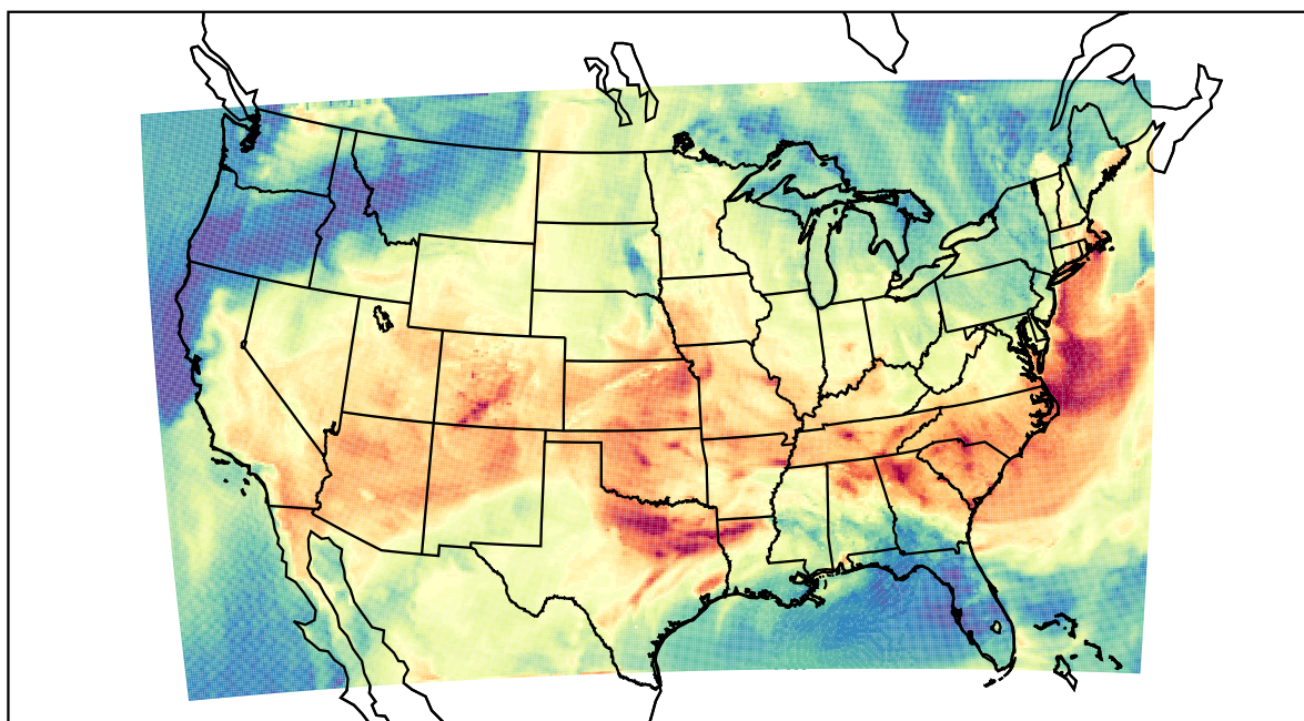
WRF (2023-06-17_18:00:00)
