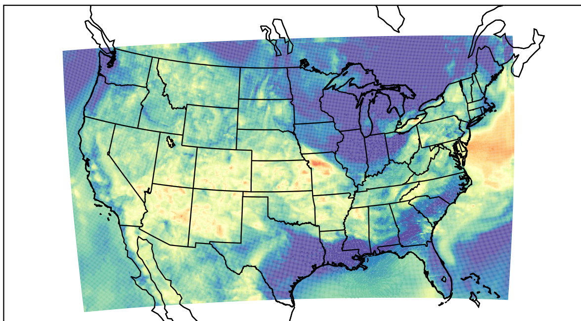
WRF (2023-06-16_09:00:00)
