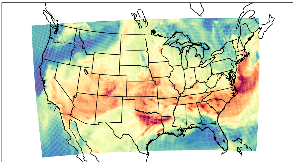
WRF (2023-06-17_19:00:00)
