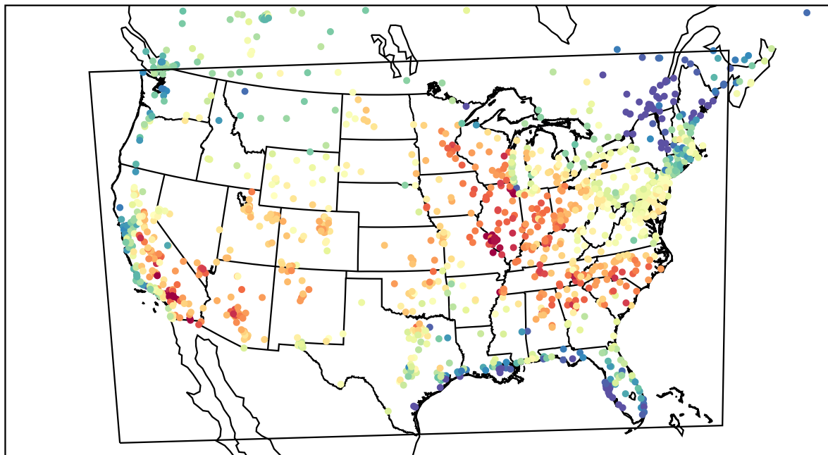
AirNOW (2023-06-17_22:00:00)
