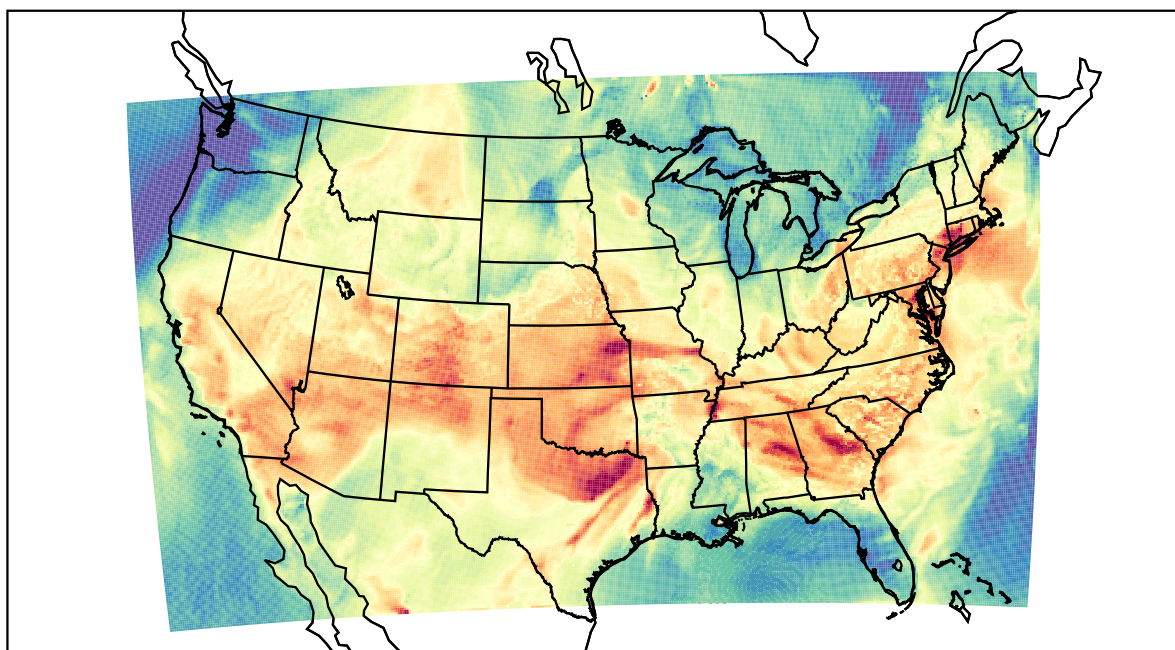
WRF (2023-06-16_22:00:00)
