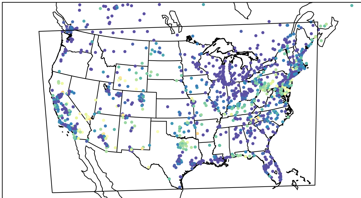
AirNOW (2023-06-16_12:00:00)
