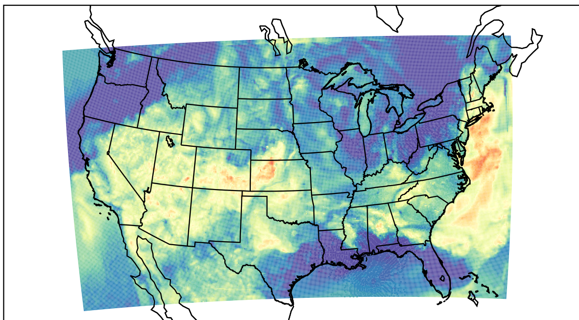
WRF (2023-06-17_10:00:00)
