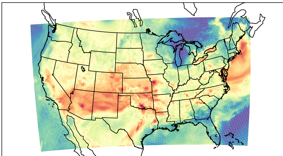
WRF (2023-06-16_00:00:00)
