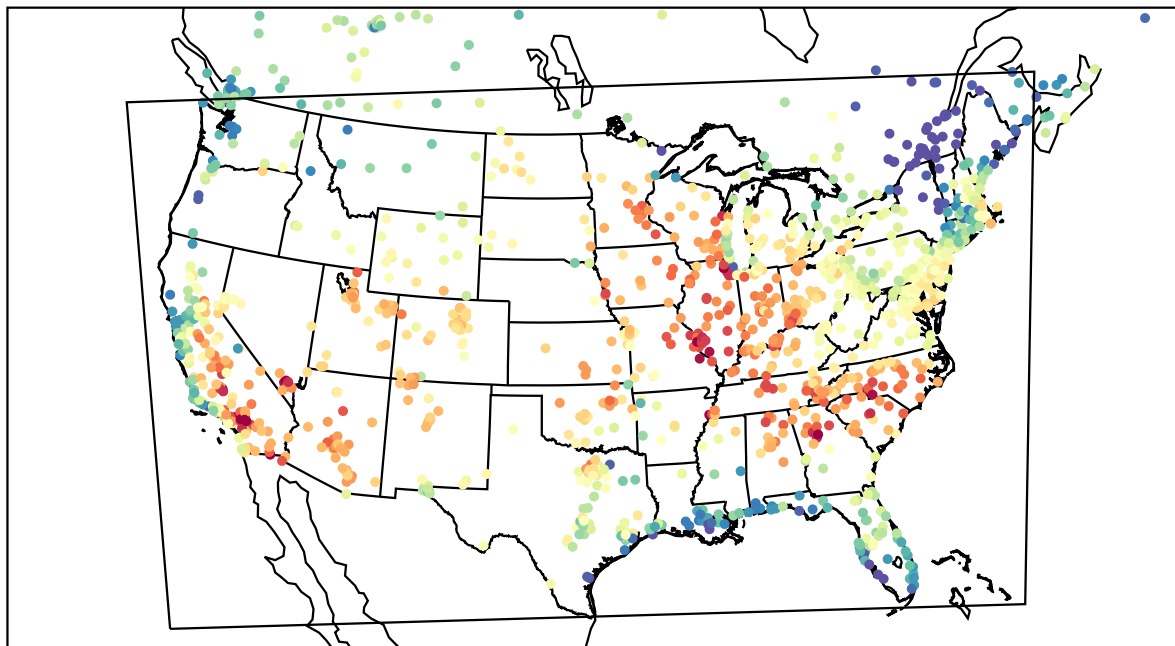
AirNOW (2023-06-17_20:00:00)
