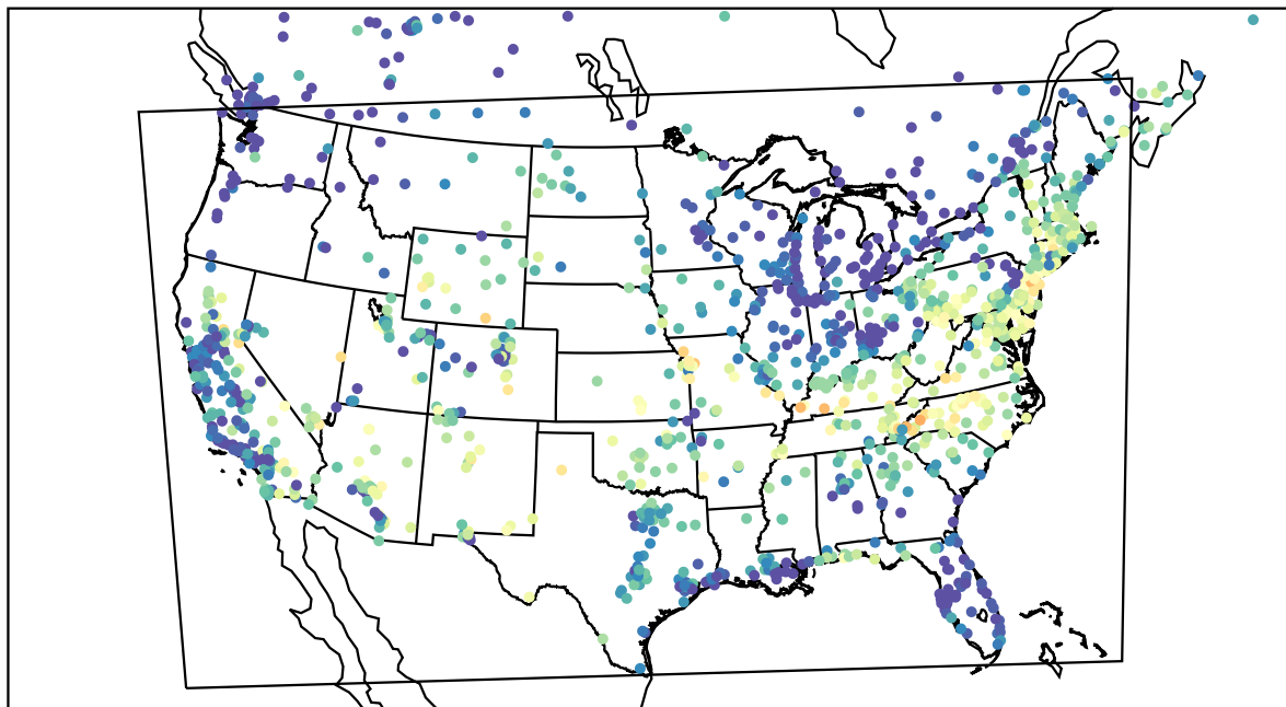
AirNOW (2023-06-16_14:00:00)
