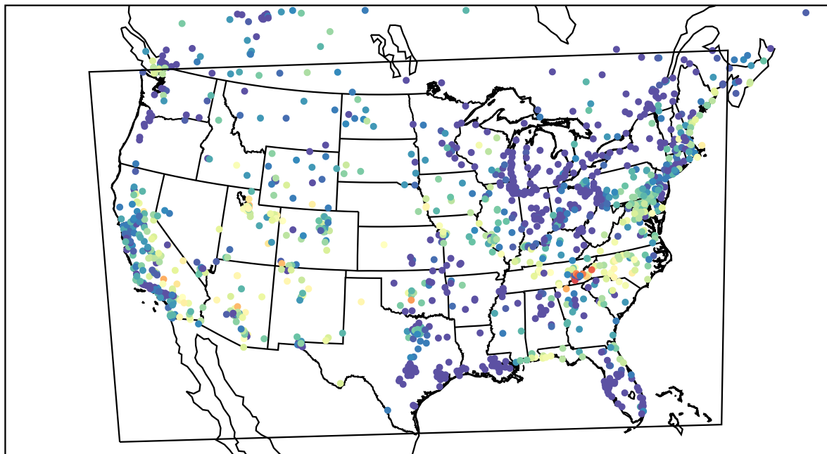
AirNOW (2023-06-17_07:00:00)
