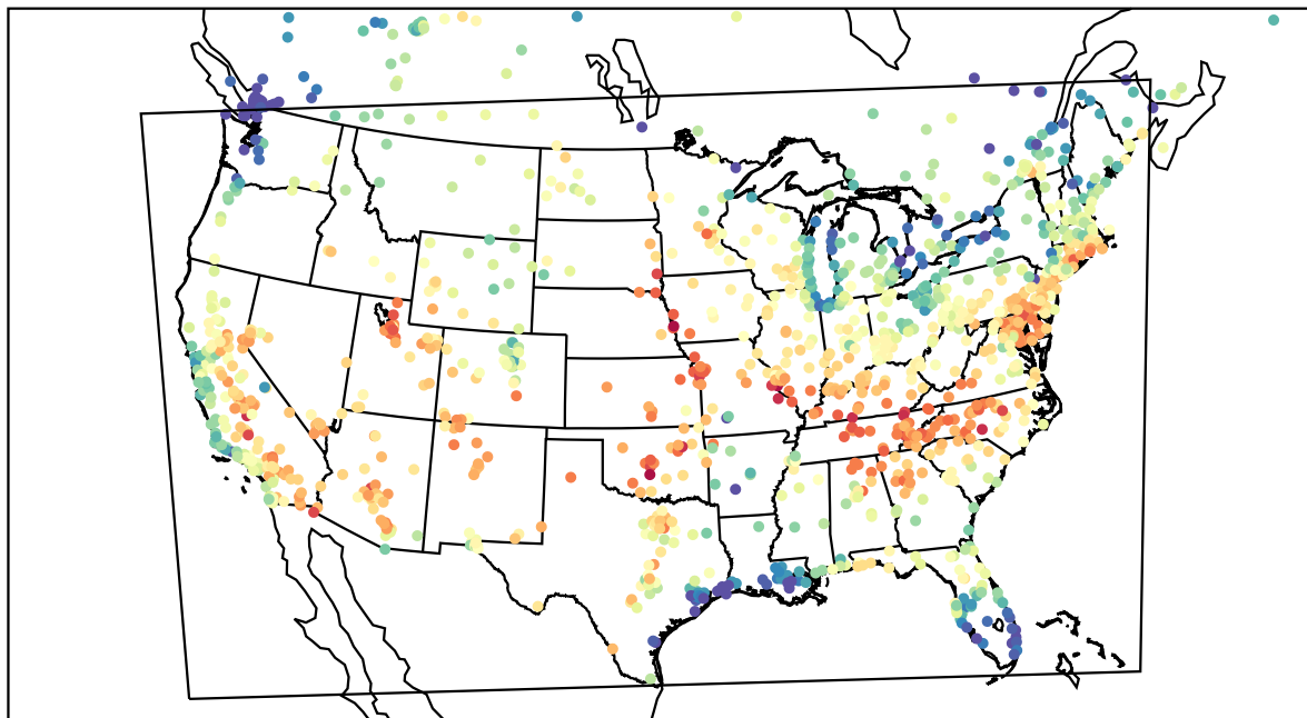
AirNOW (2023-06-16_21:00:00)
