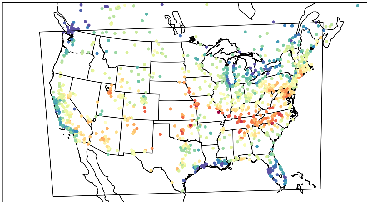
AirNOW (2023-06-16_18:00:00)
