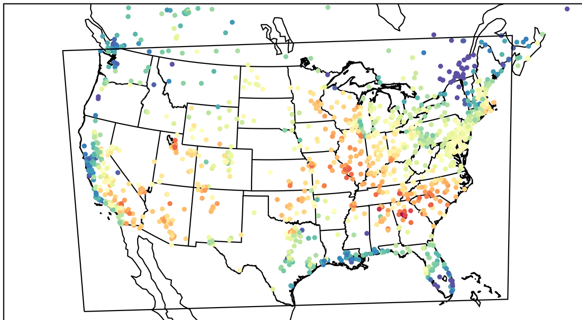
AirNOW (2023-06-17_17:00:00)
