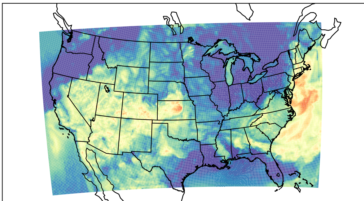
WRF (2023-06-17_12:00:00)
