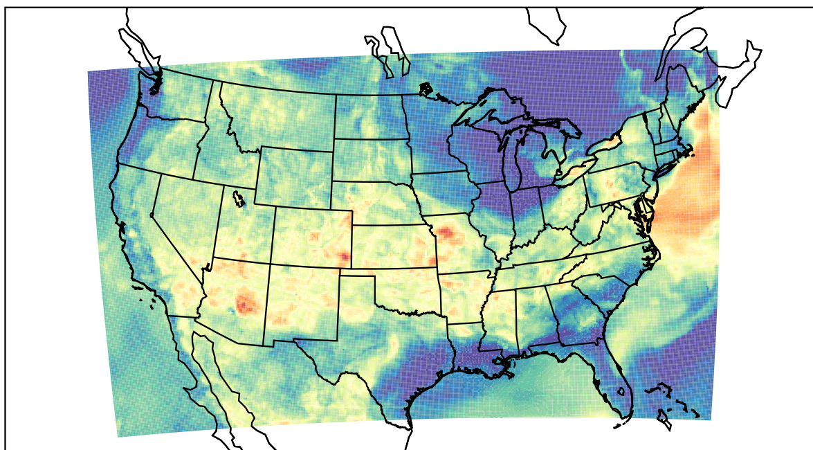
WRF (2023-06-16_05:00:00)
