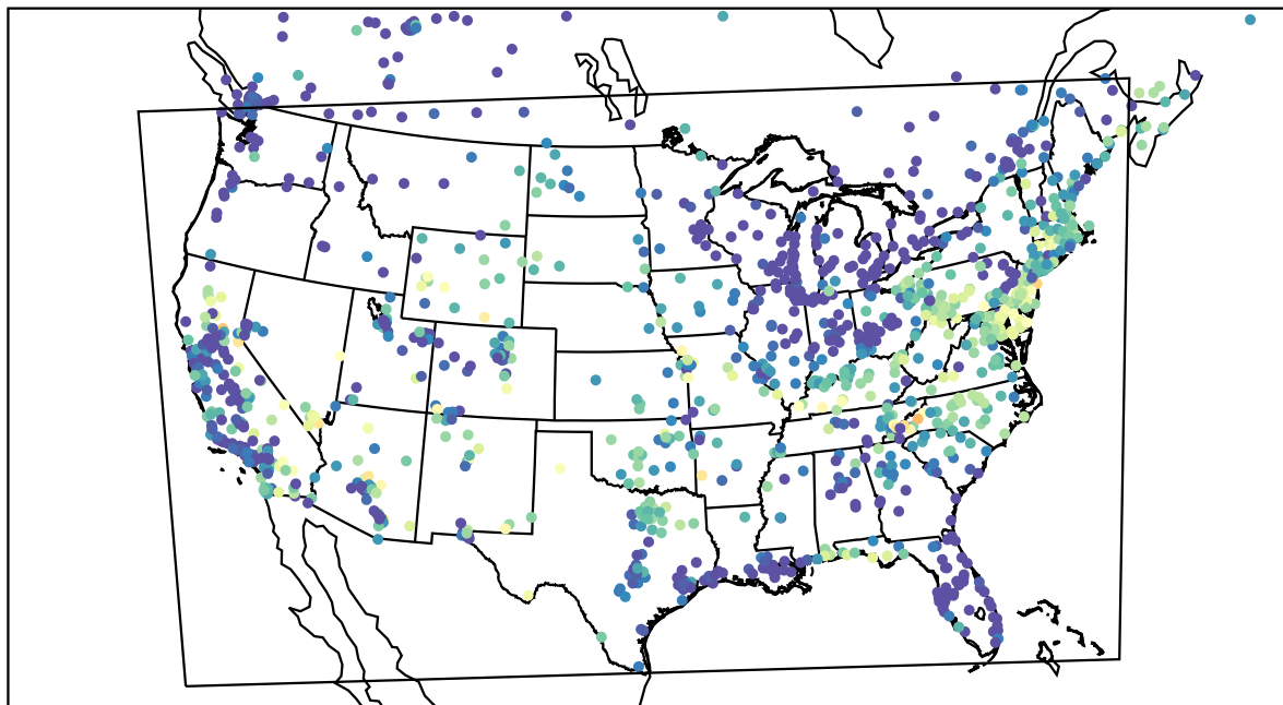
AirNOW (2023-06-16_13:00:00)
