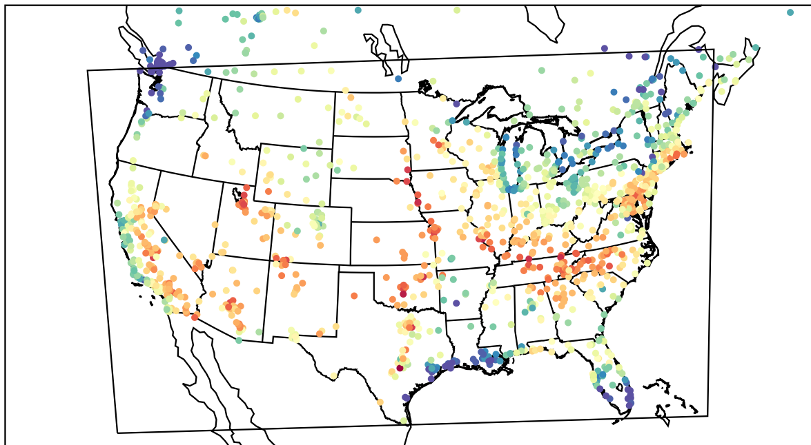
AirNOW (2023-06-16_22:00:00)
