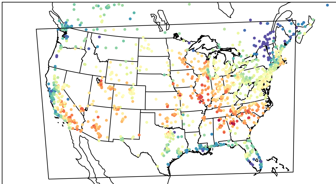
AirNOW (2023-06-17_18:00:00)
