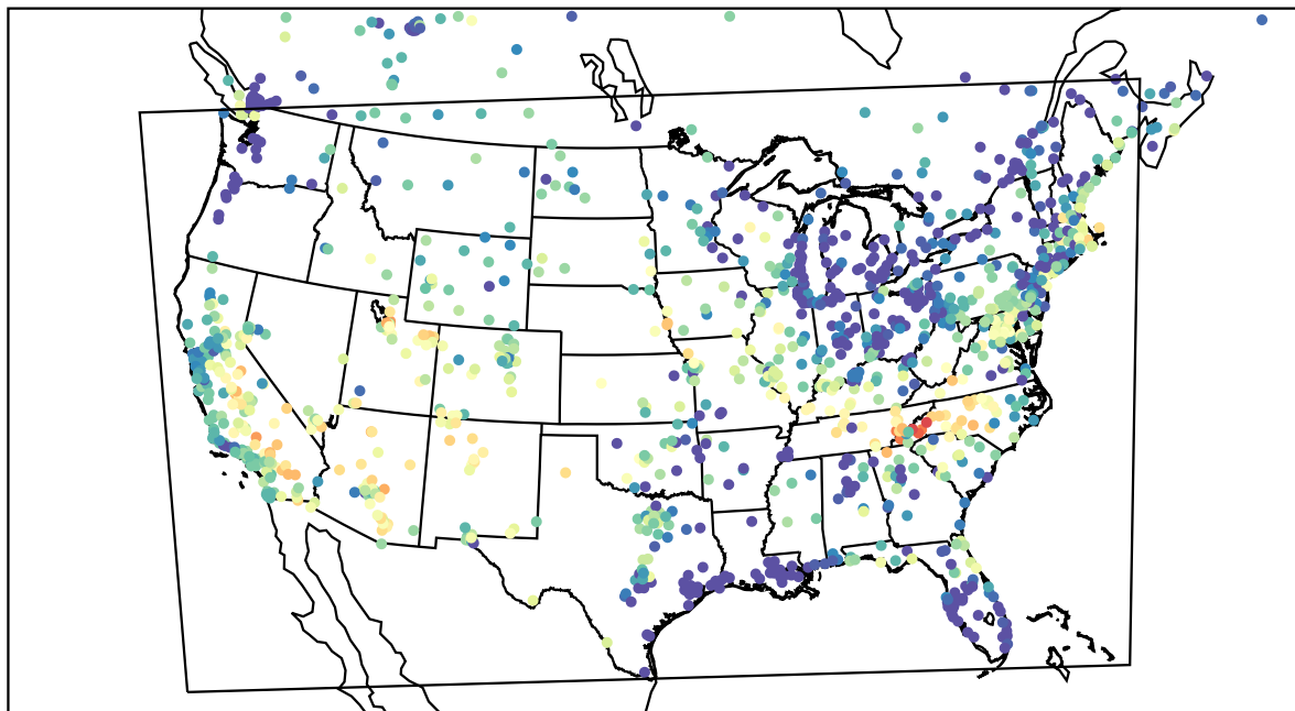
AirNOW (2023-06-17_04:00:00)
