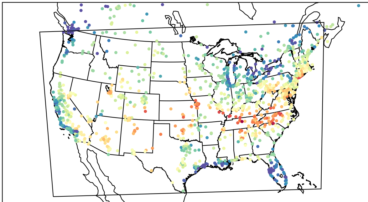
AirNOW (2023-06-16_17:00:00)
