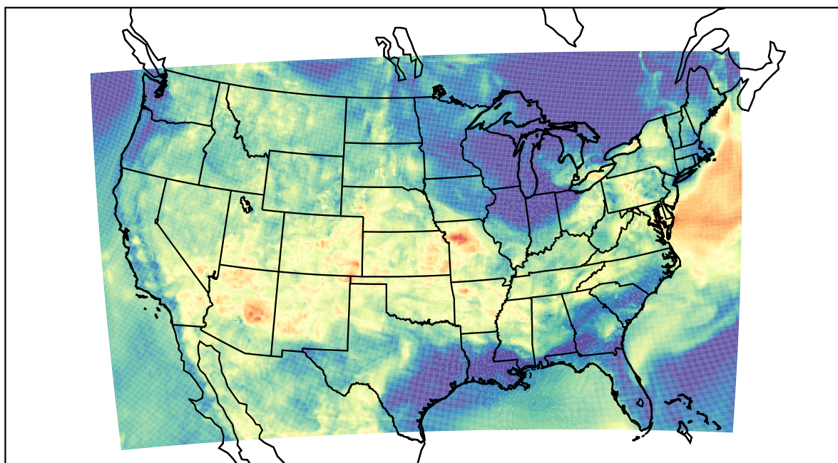
WRF (2023-06-16_06:00:00)
