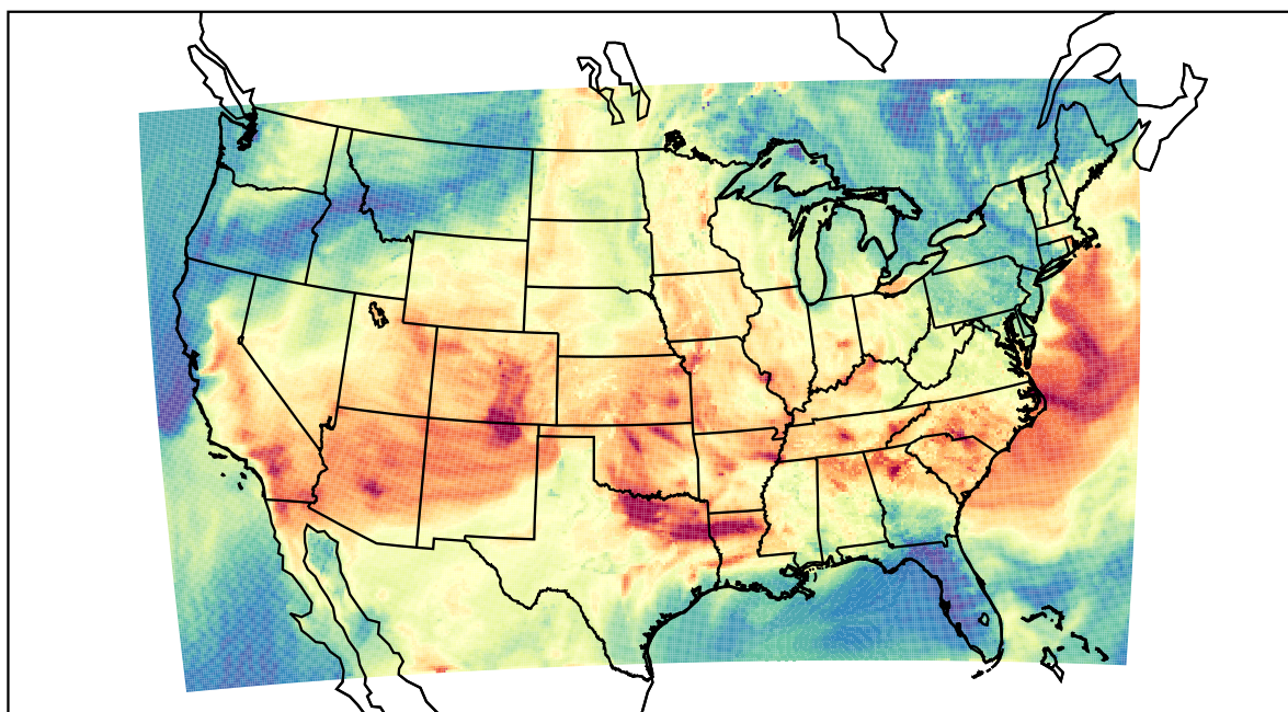
WRF (2023-06-17_23:00:00)
