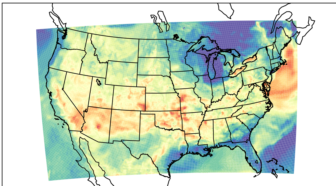
WRF (2023-06-16_02:00:00)
