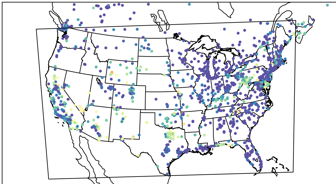
AirNOW (2023-06-16_11:00:00)
