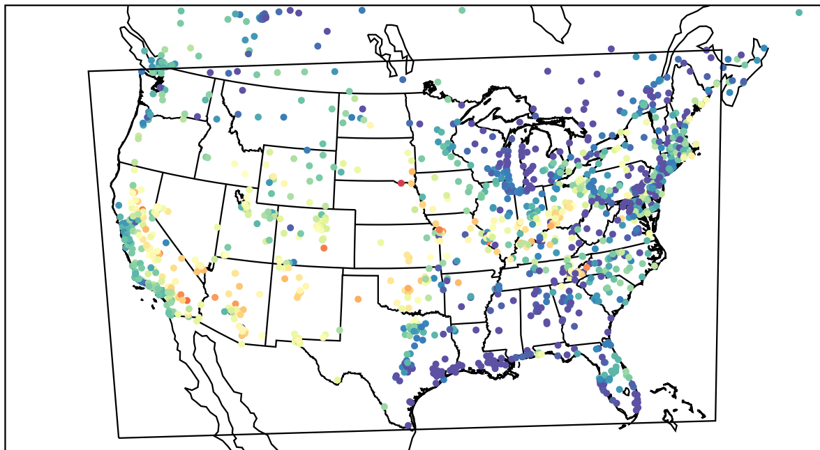
AirNOW (2023-06-16_03:00:00)
