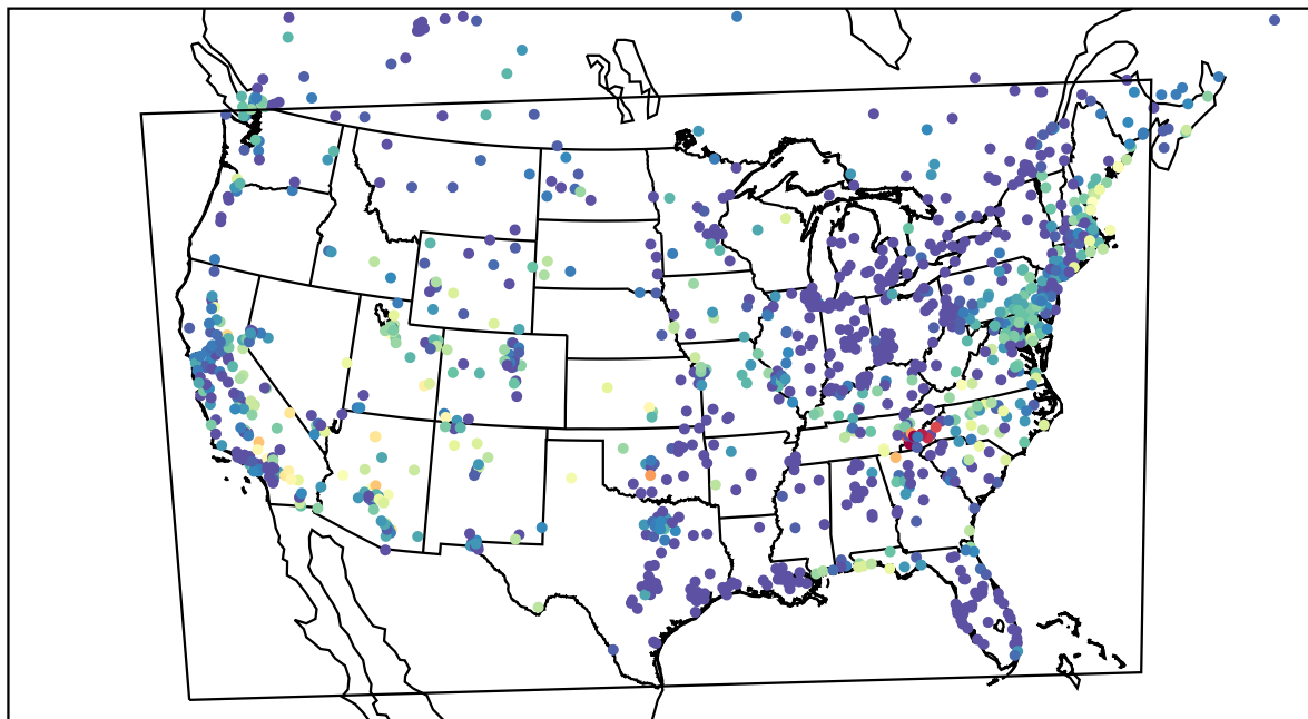
AirNOW (2023-06-17_10:00:00)
