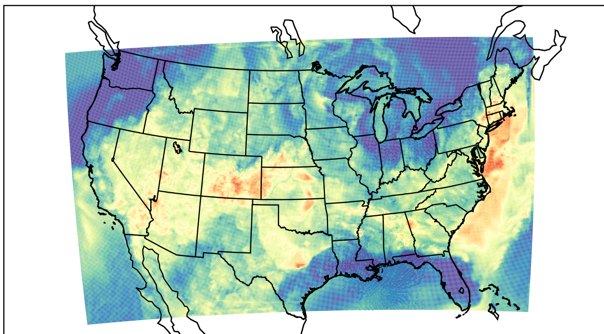
WRF (2023-06-17_05:00:00)
