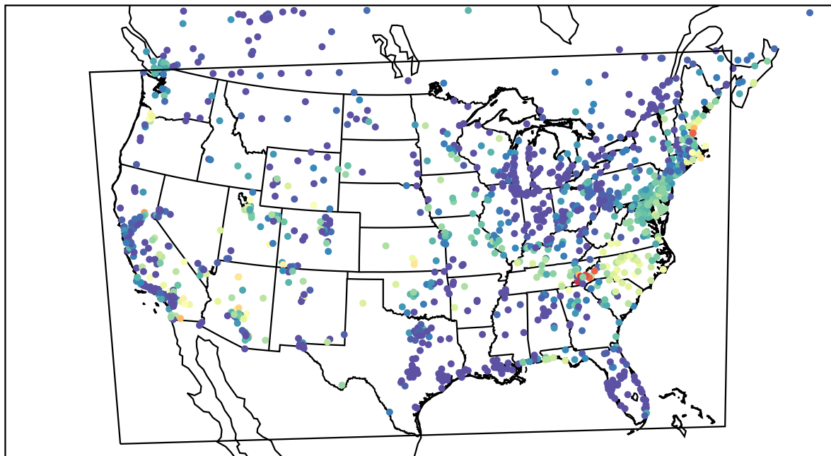
AirNOW (2023-06-17_12:00:00)
