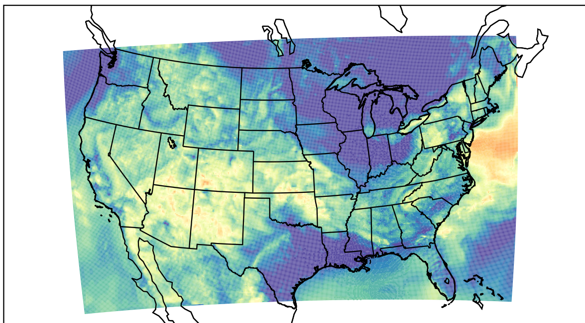
WRF (2023-06-16_12:00:00)
