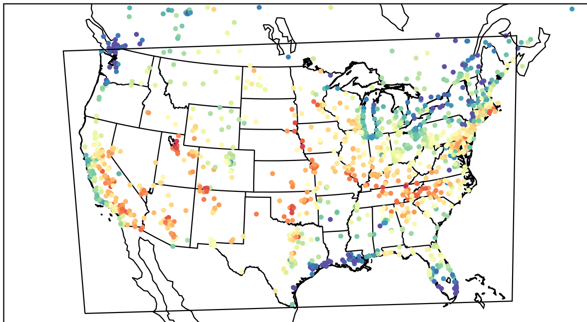
AirNOW (2023-06-16_23:00:00)
