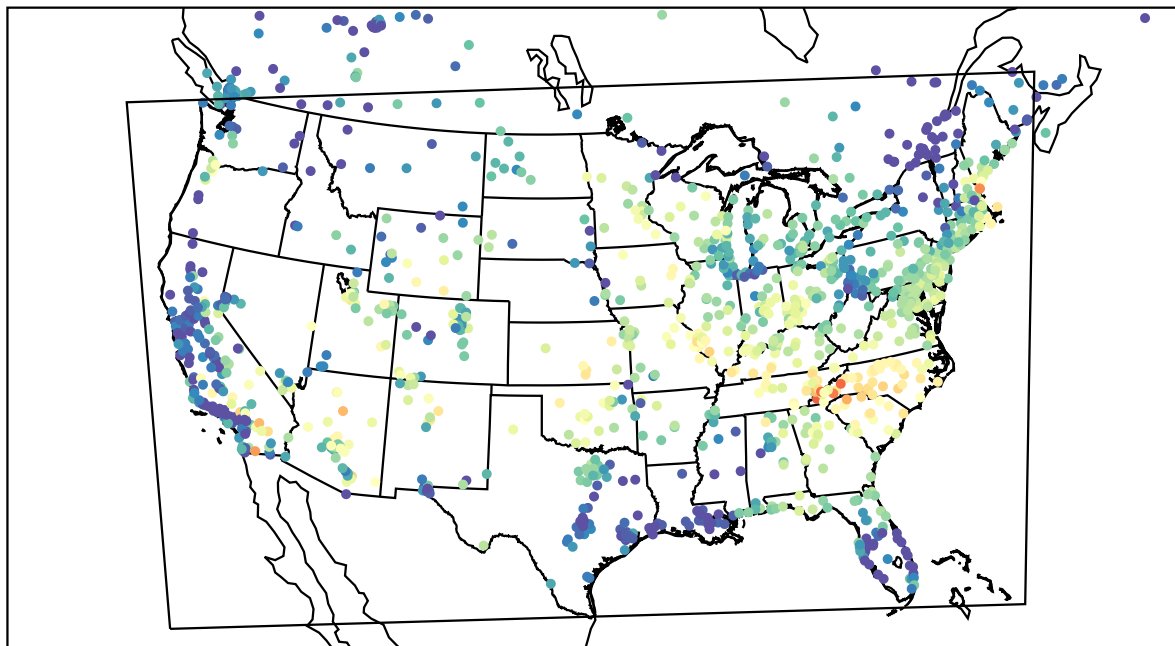
AirNOW (2023-06-17_14:00:00)
