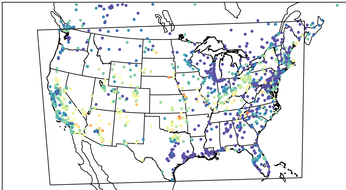
AirNOW (2023-06-16_05:00:00)
