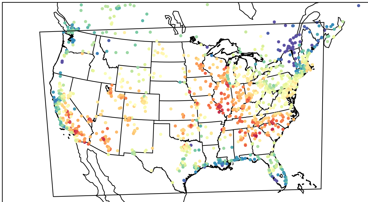
AirNOW (2023-06-17_19:00:00)
