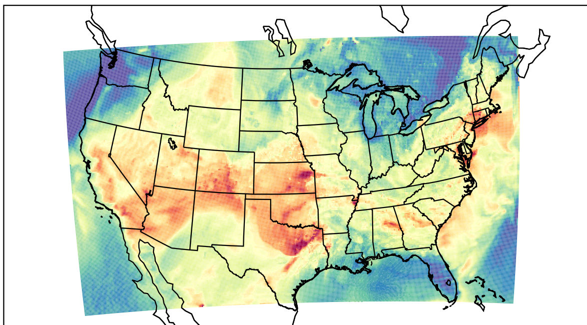
WRF (2023-06-17_00:00:00)
