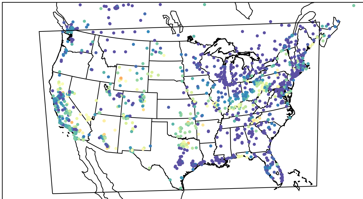
AirNOW (2023-06-16_08:00:00)
