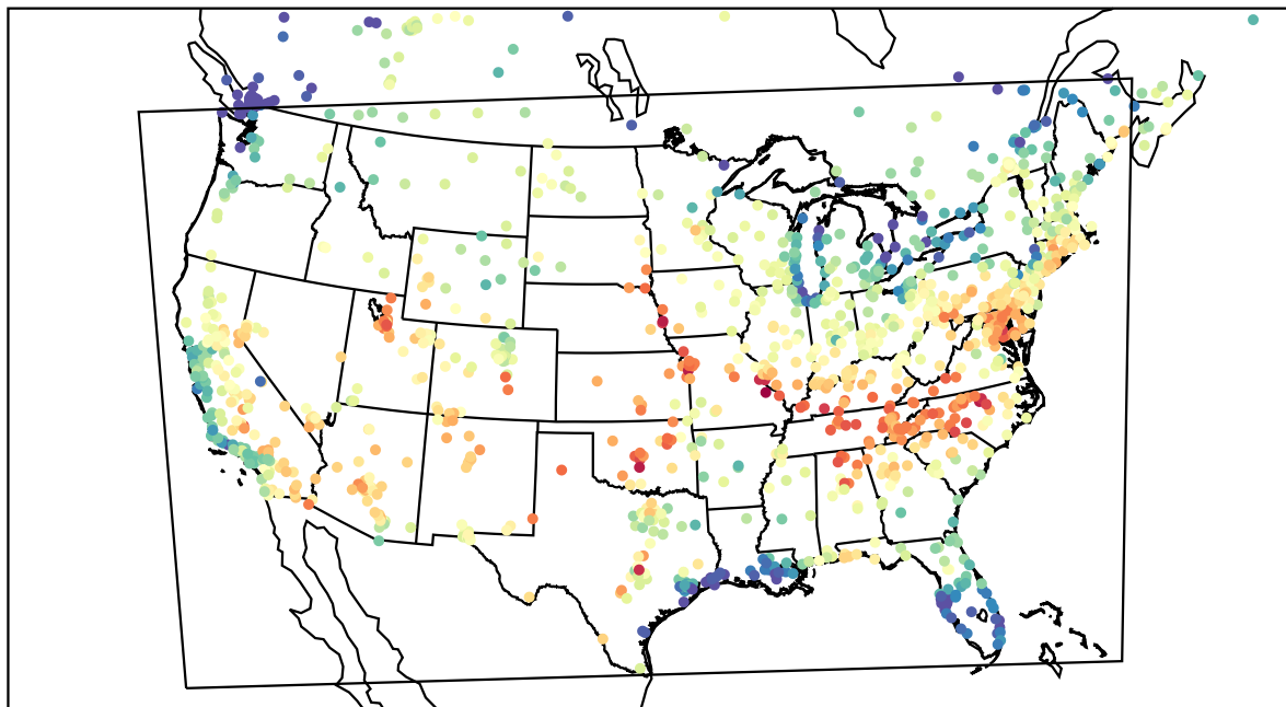
AirNOW (2023-06-16_19:00:00)
