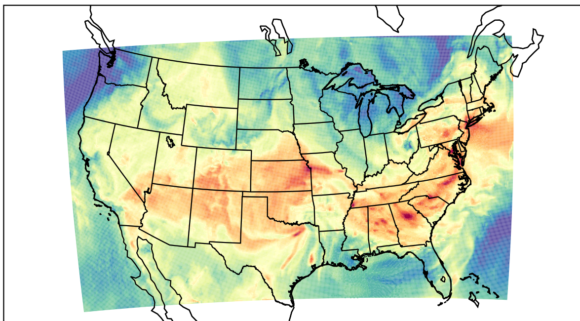
WRF (2023-06-16_17:00:00)
