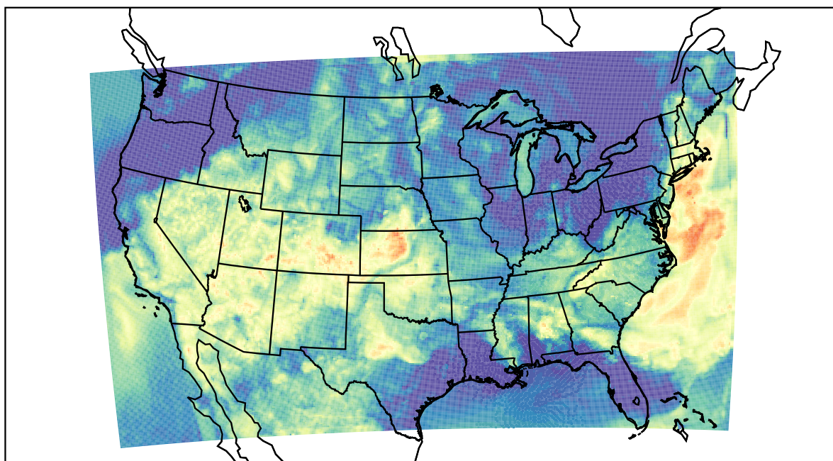
WRF (2023-06-17_11:00:00)
