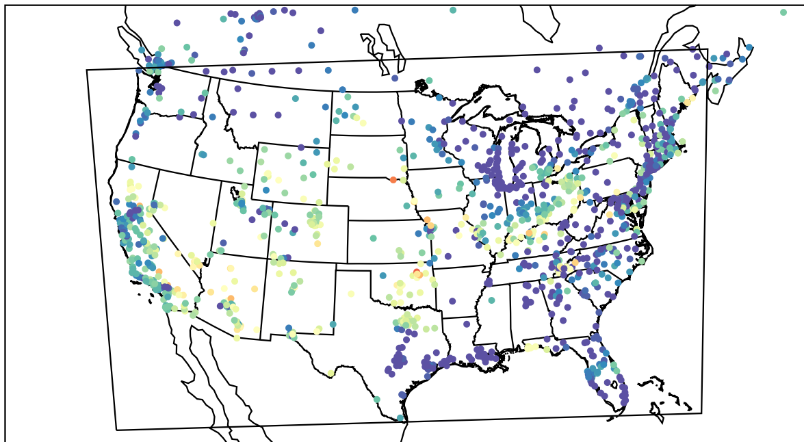
AirNOW (2023-06-16_06:00:00)
