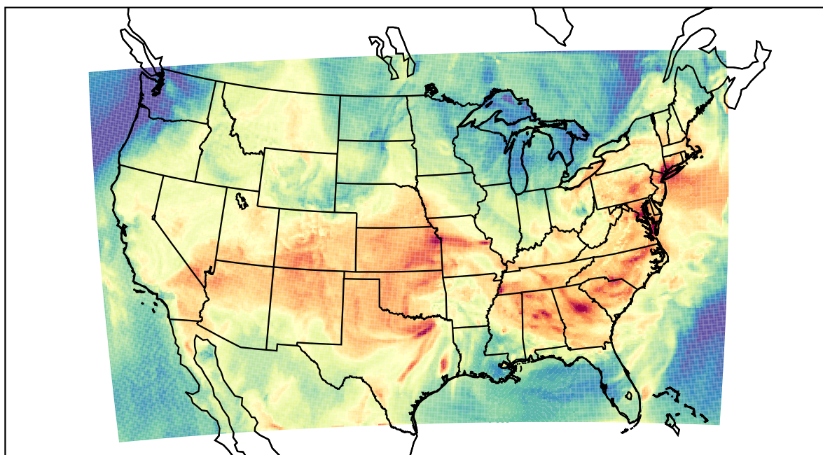
WRF (2023-06-16_18:00:00)
