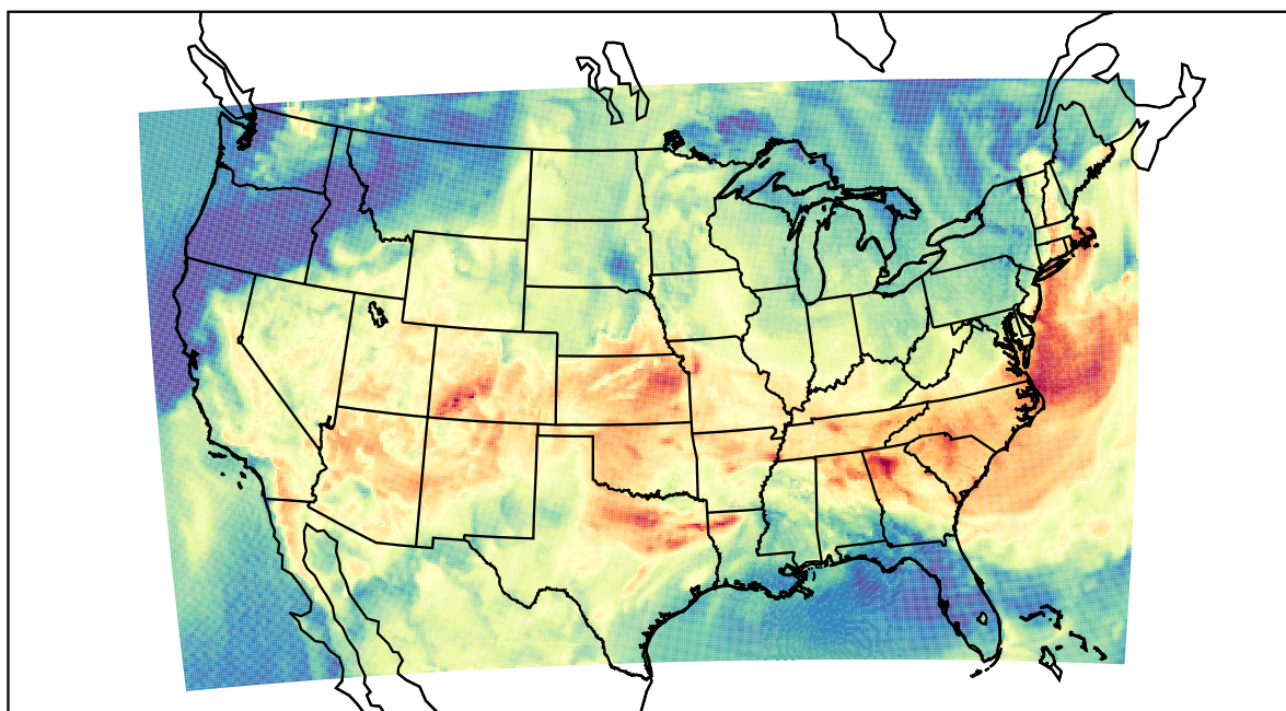
WRF (2023-06-17_16:00:00)
