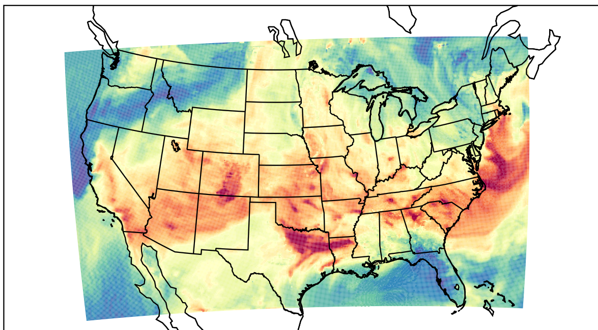
WRF (2023-06-17_21:00:00)
