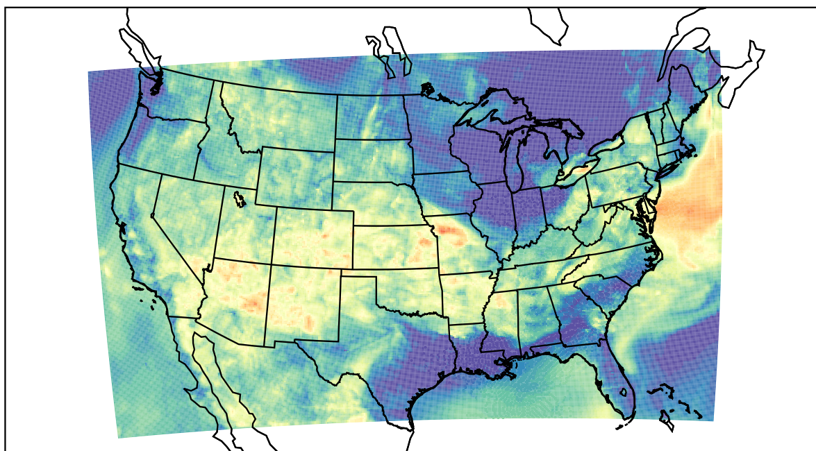
WRF (2023-06-16_08:00:00)
