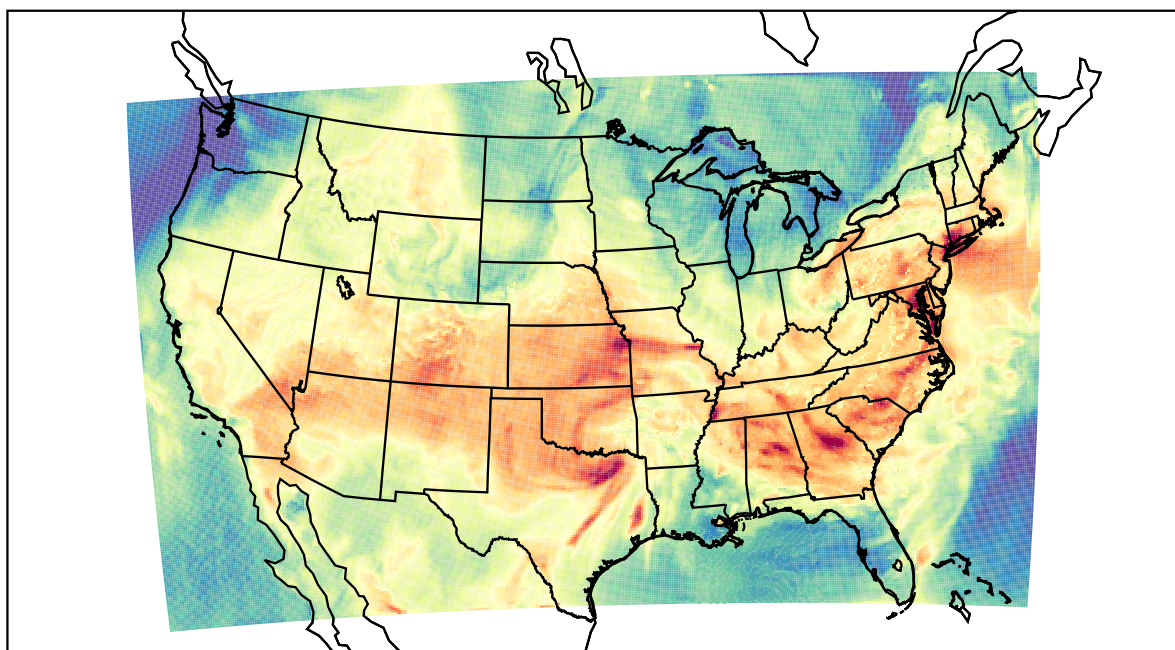
WRF (2023-06-16_19:00:00)
