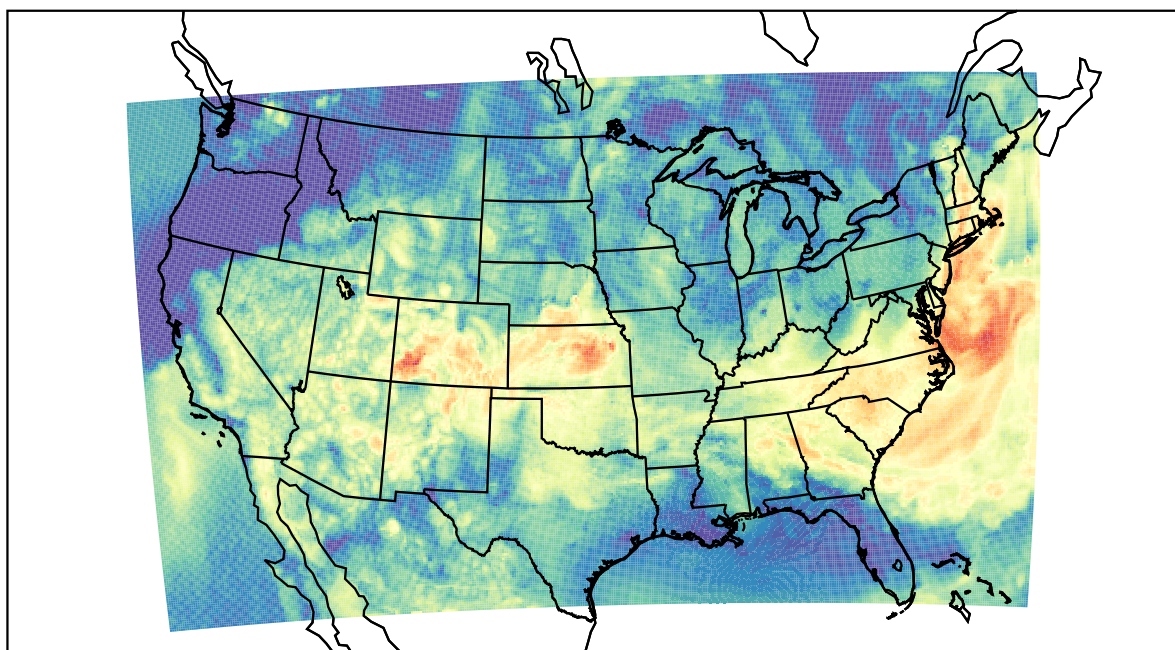
WRF (2023-06-17_14:00:00)
