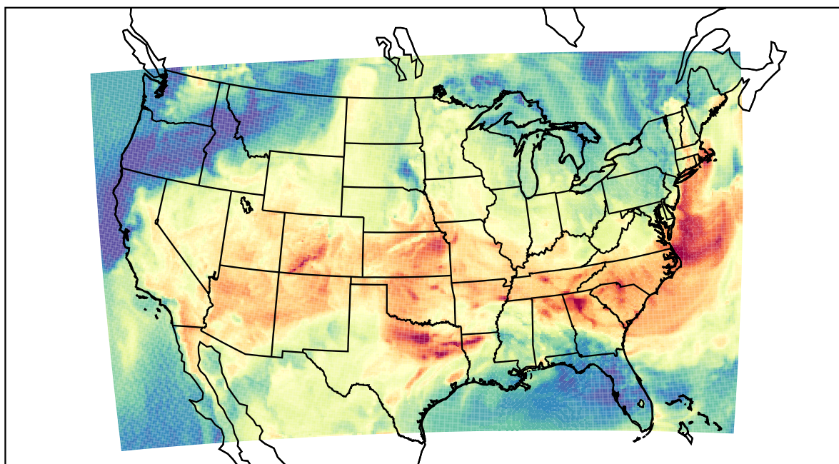
WRF (2023-06-17_17:00:00)
