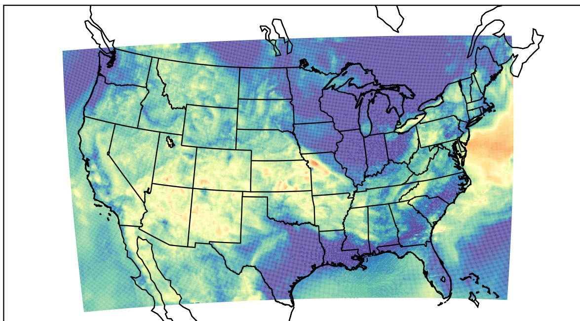
WRF (2023-06-16_11:00:00)
